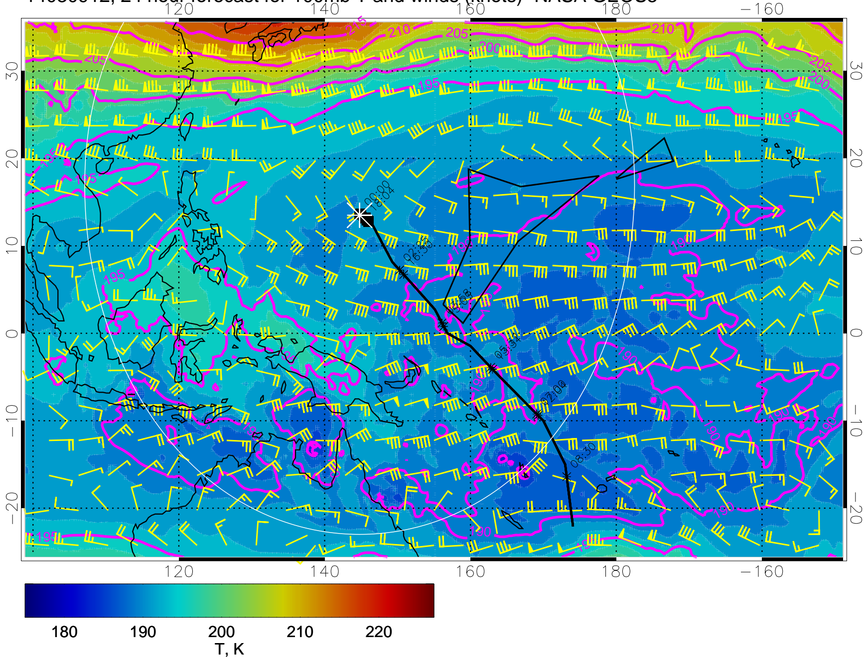
14030912, 24 hour forecast for 100mb T and winds (knots)- NASA GEOS5
