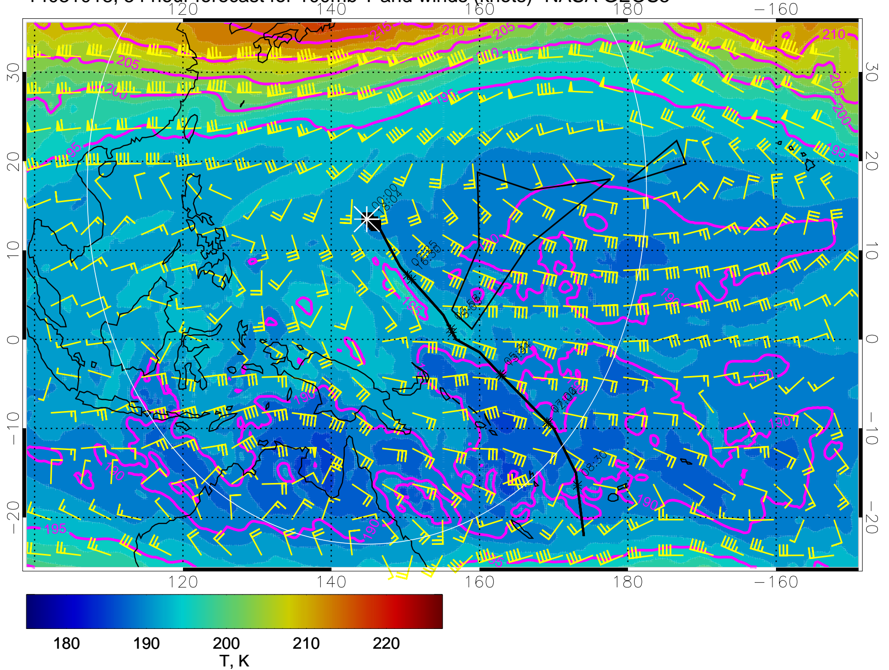
14031018, 54 hour forecast for 100mb T and winds (knots)- NASA GEOS5
