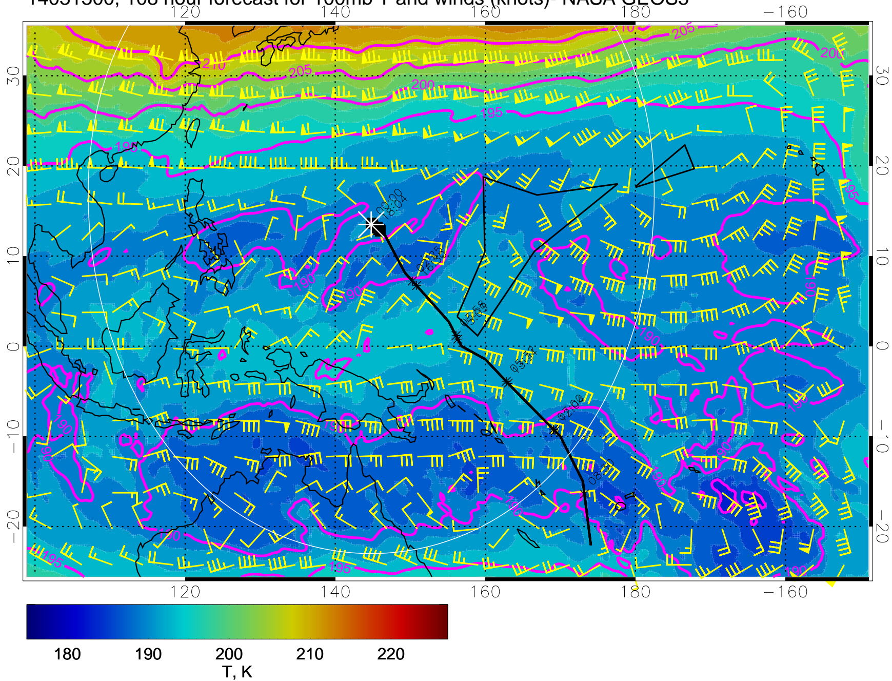
14031300, 108 hour forecast for 100mb T and winds (knots)- NASA GEOS5
