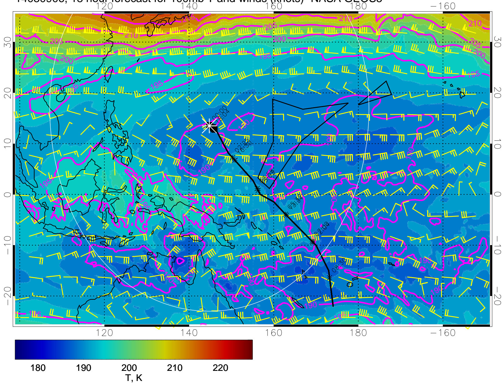
14030906, 18 hour forecast for 100mb T and winds (knots)- NASA GEOS5
