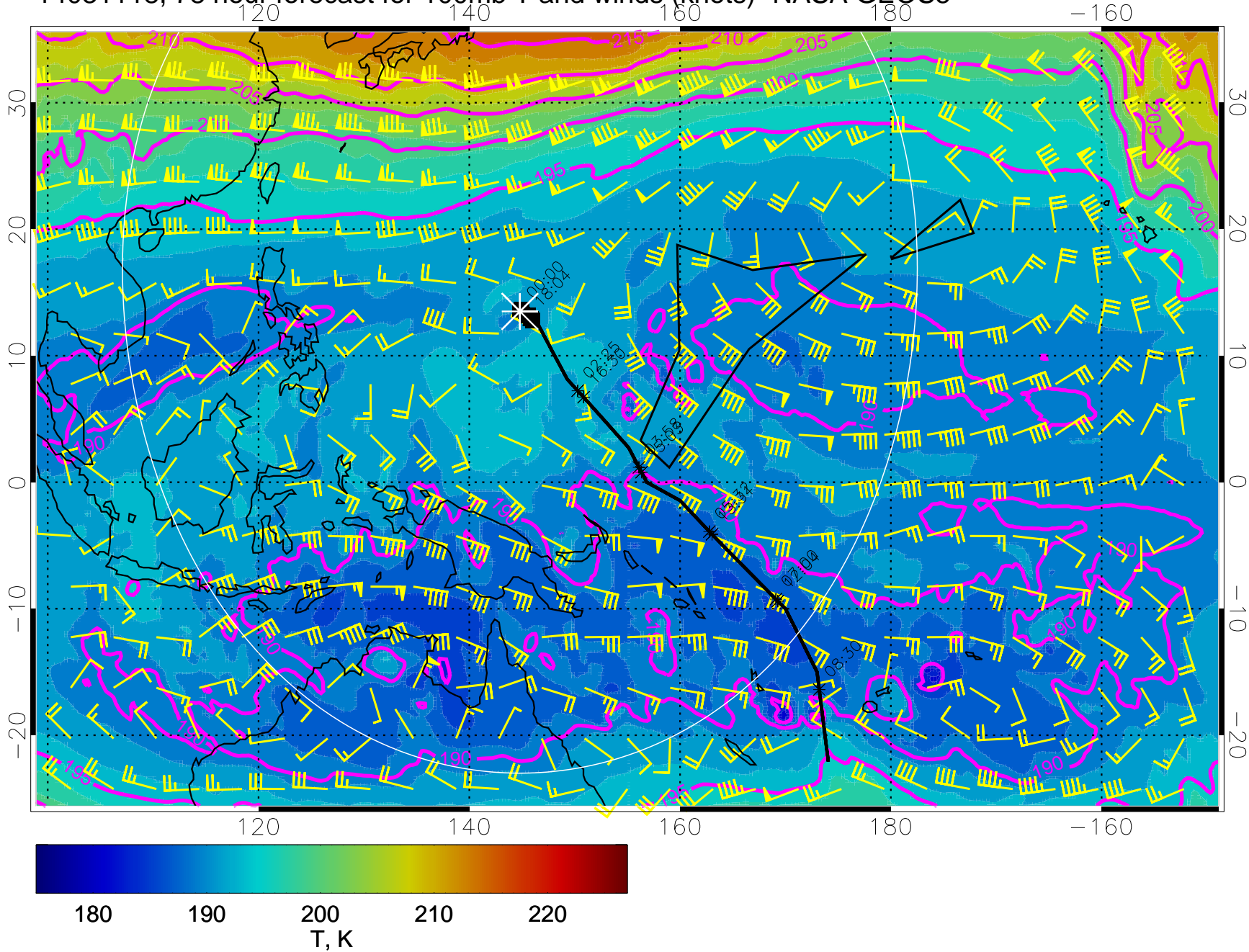
14031118, 78 hour forecast for 100mb T and winds (knots)- NASA GEOS5
