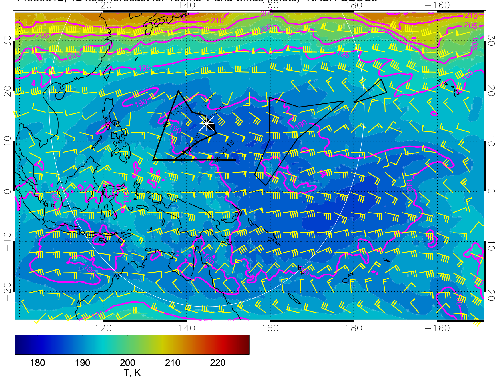
14030612, 12 hour forecast for 100mb T and winds (knots)- NASA GEOS5
