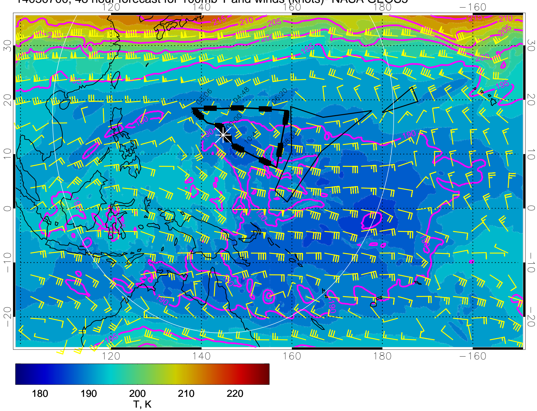
14030700, 48 hour forecast for 100mb T and winds (knots)- NASA GEOS5
