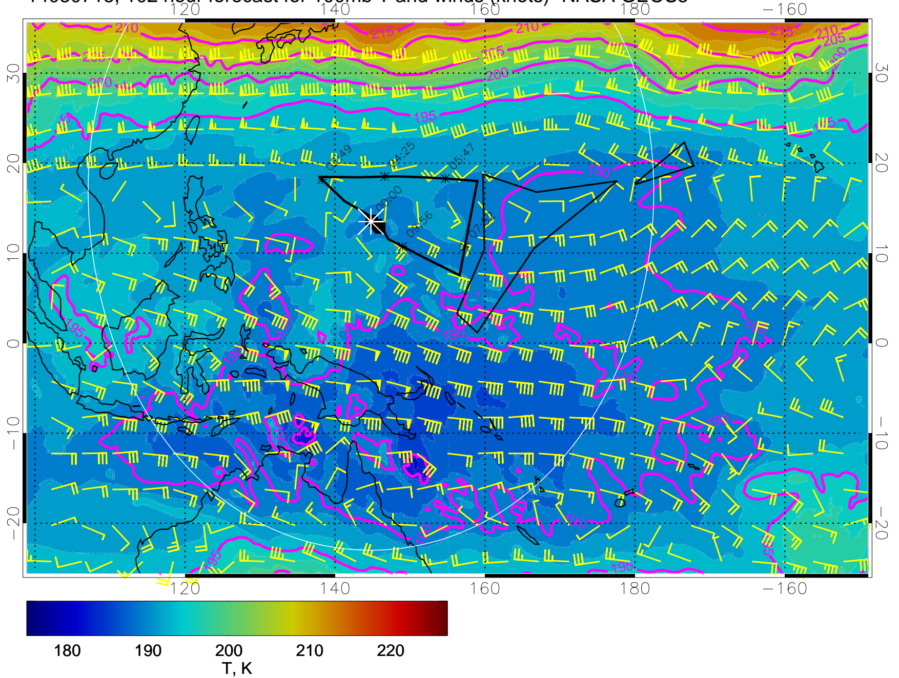
14030718, 102 hour forecast for 100mb T and winds (knots)- NASA GEOS5
