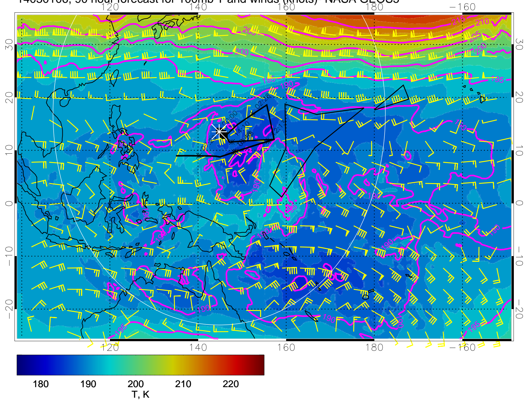
14030106, 90 hour forecast for 100mb T and winds (knots)- NASA GEOS5
