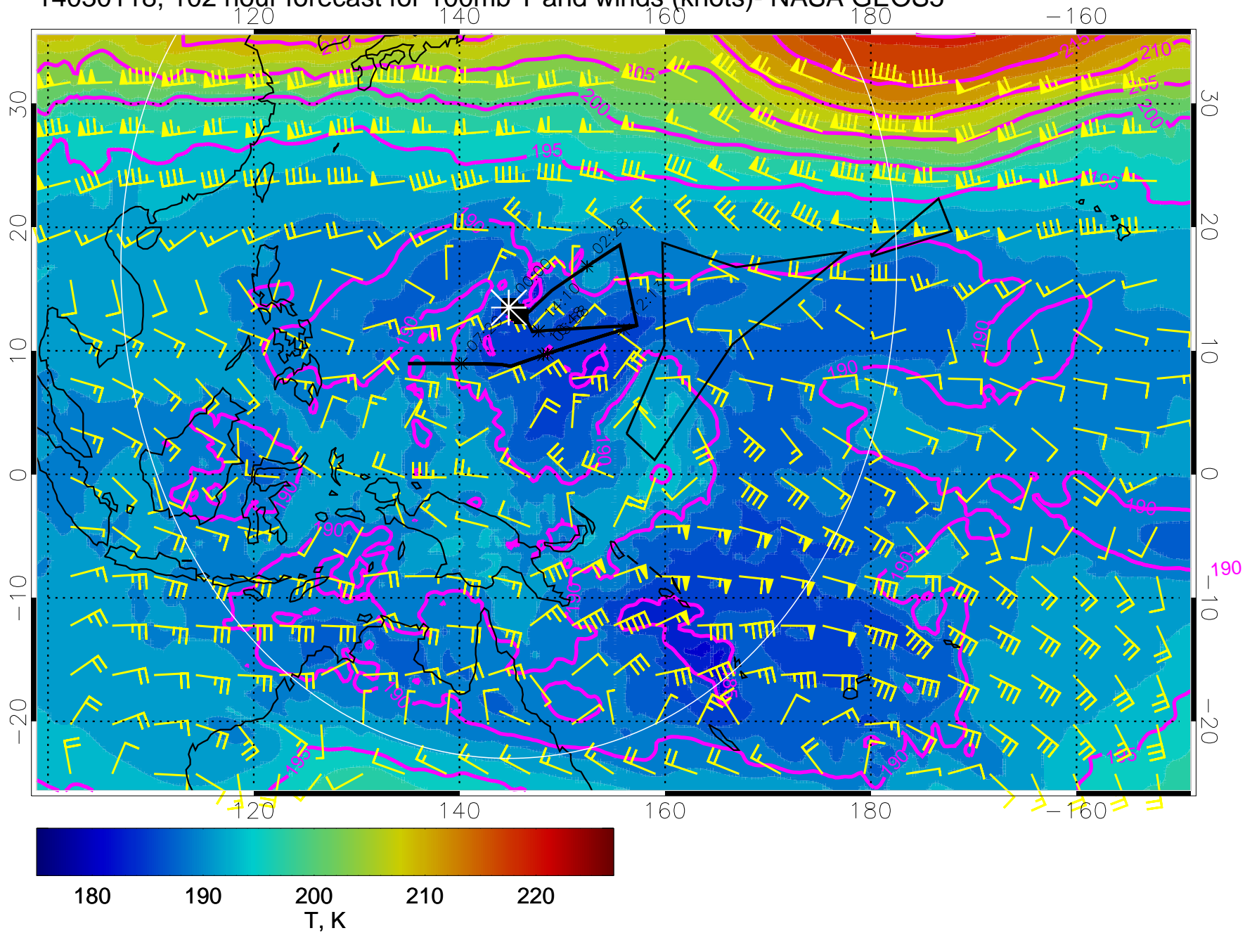
14030118, 102 hour forecast for 100mb T and winds (knots)- NASA GEOS5
