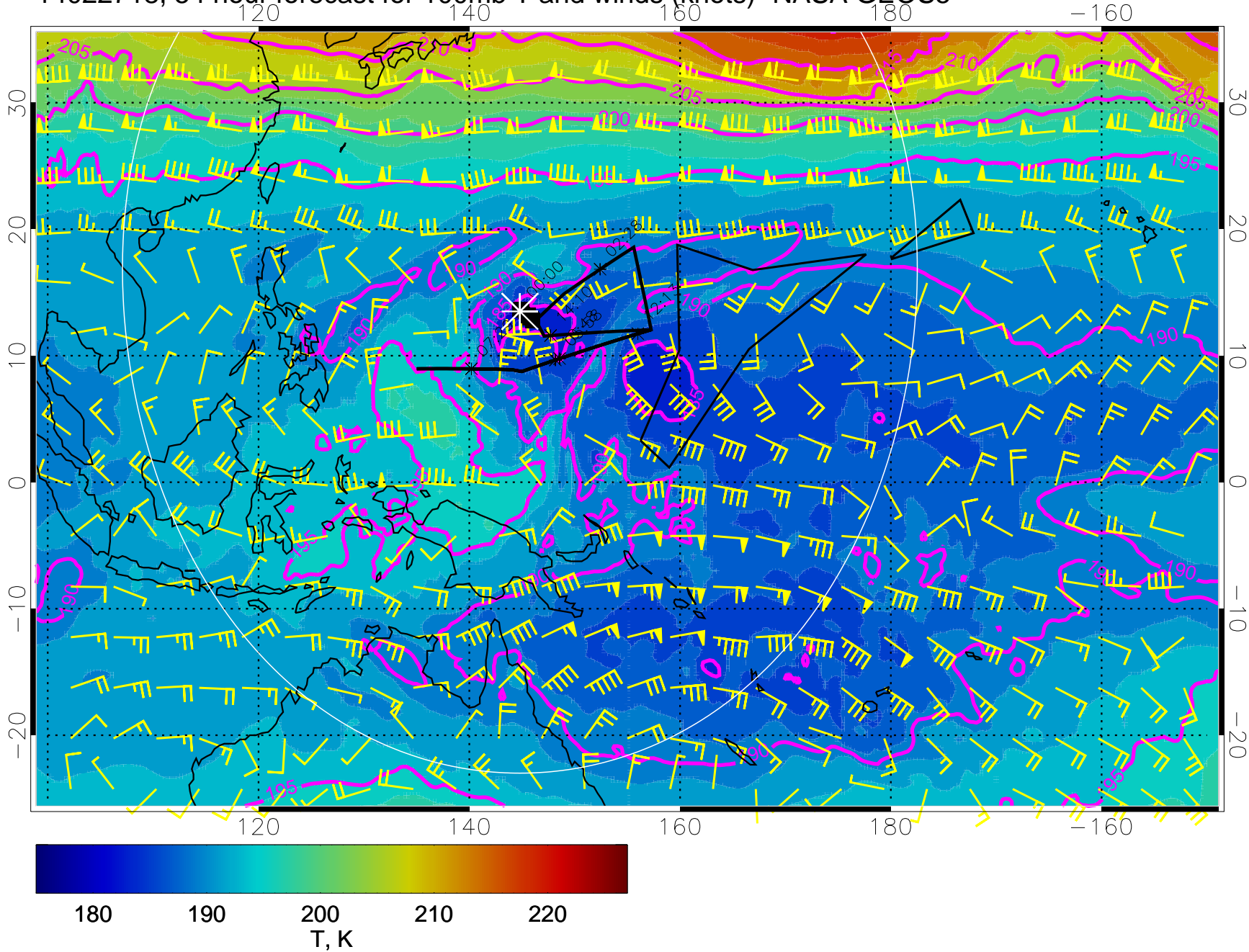
14022718, 54 hour forecast for 100mb T and winds (knots)- NASA GEOS5
