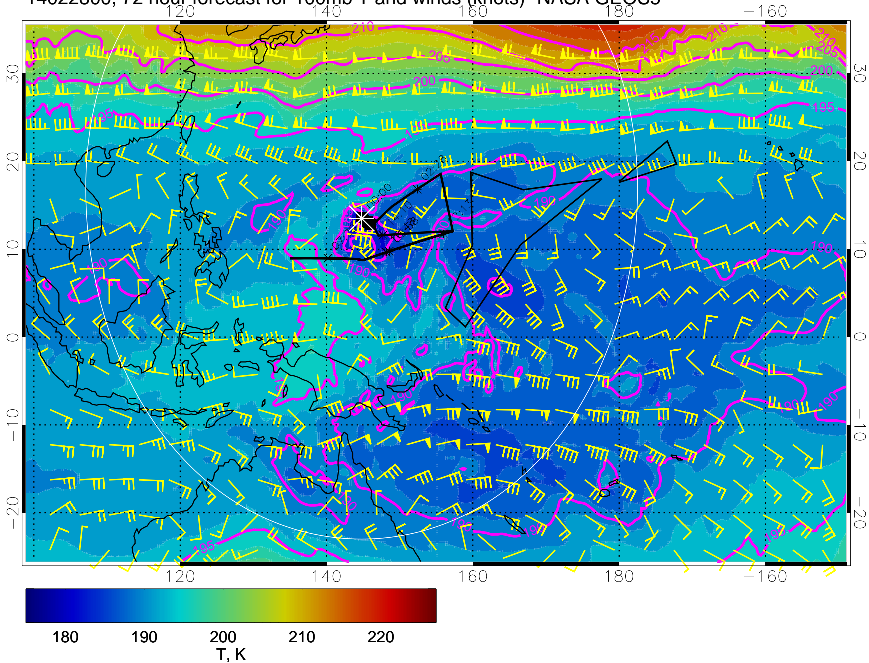
14022800, 72 hour forecast for 100mb T and winds (knots)- NASA GEOS5
