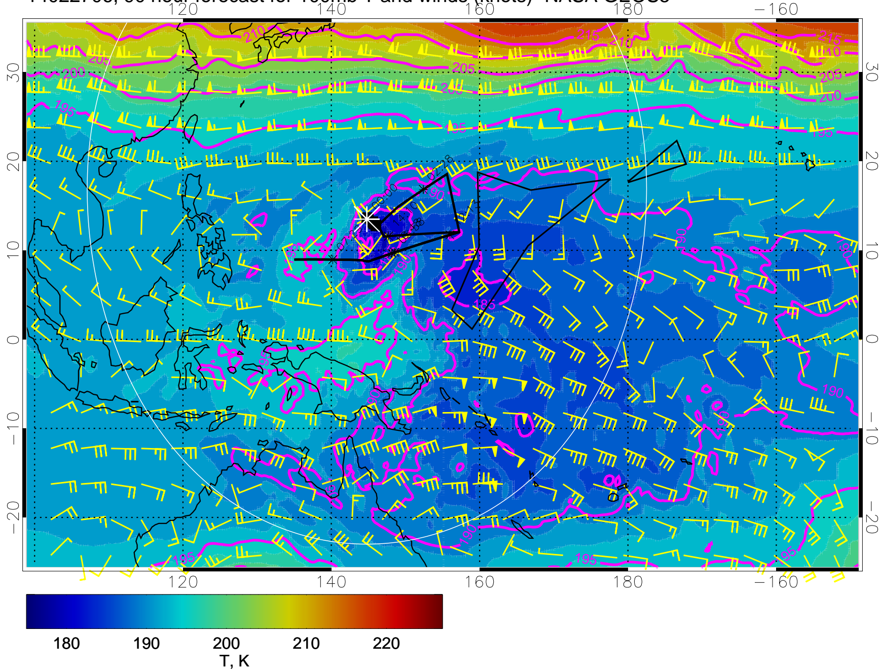
14022706, 90 hour forecast for 100mb T and winds (knots)- NASA GEOS5
