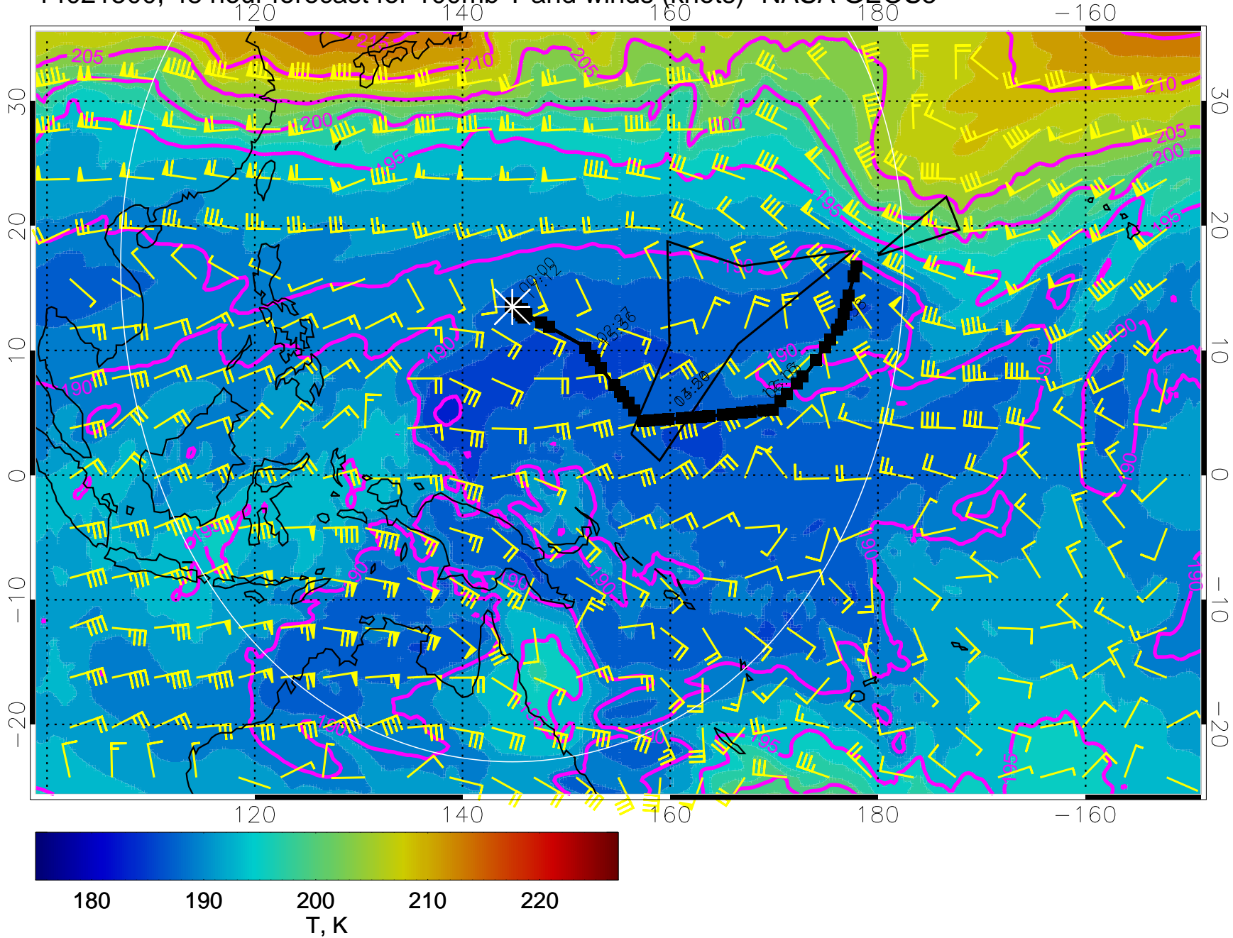
14021500, 48 hour forecast for 100mb T and winds (knots)- NASA GEOS5
