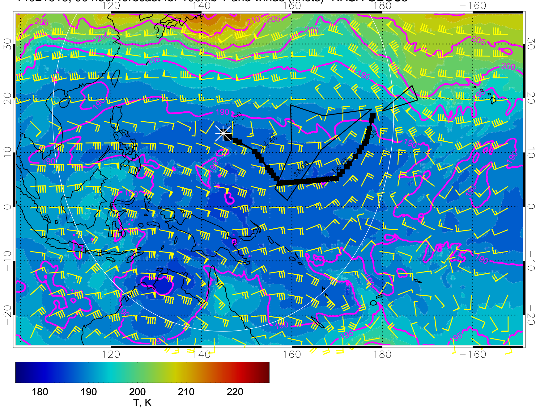
14021618, 90 hour forecast for 100mb T and winds (knots)- NASA GEOS5
