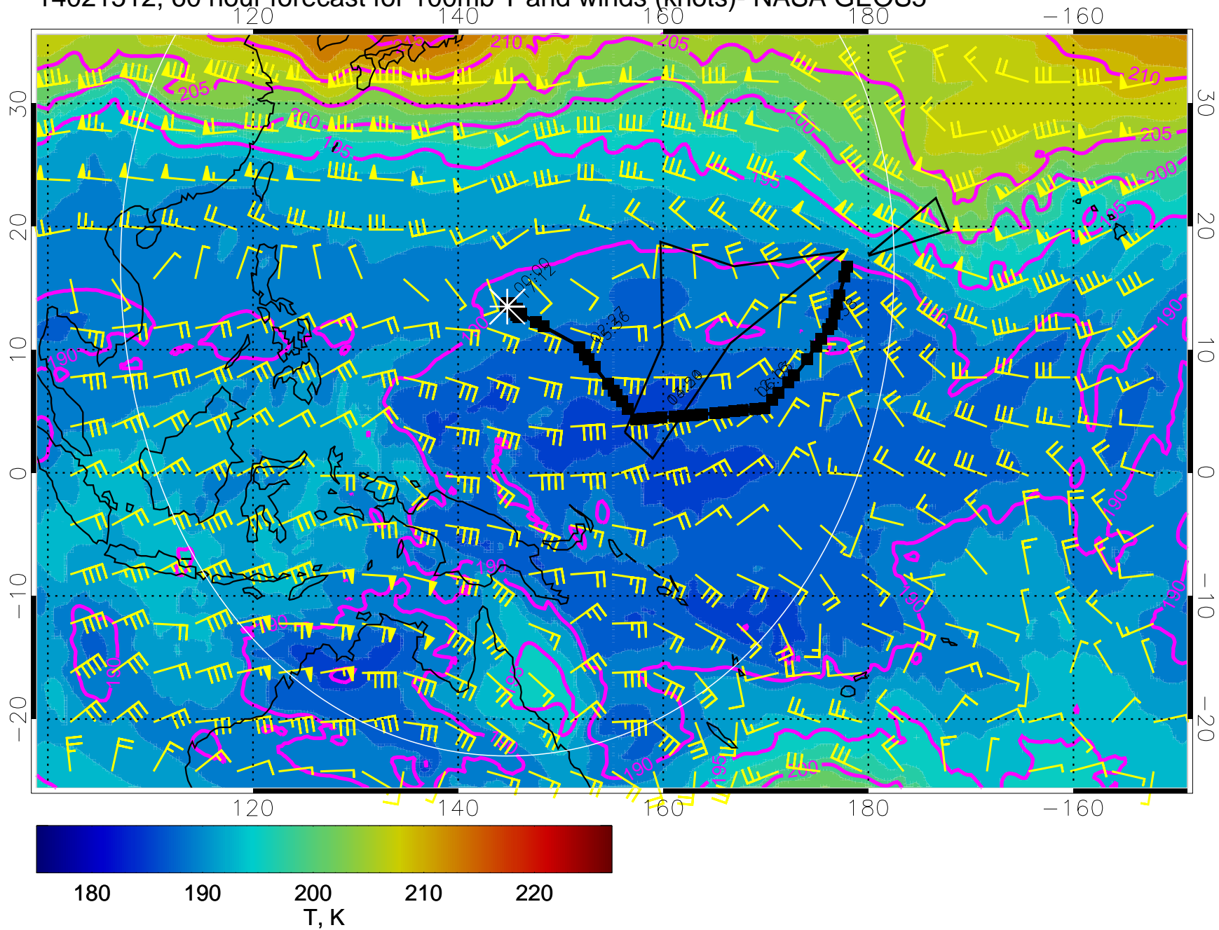
14021512, 60 hour forecast for 100mb T and winds (knots)- NASA GEOS5
