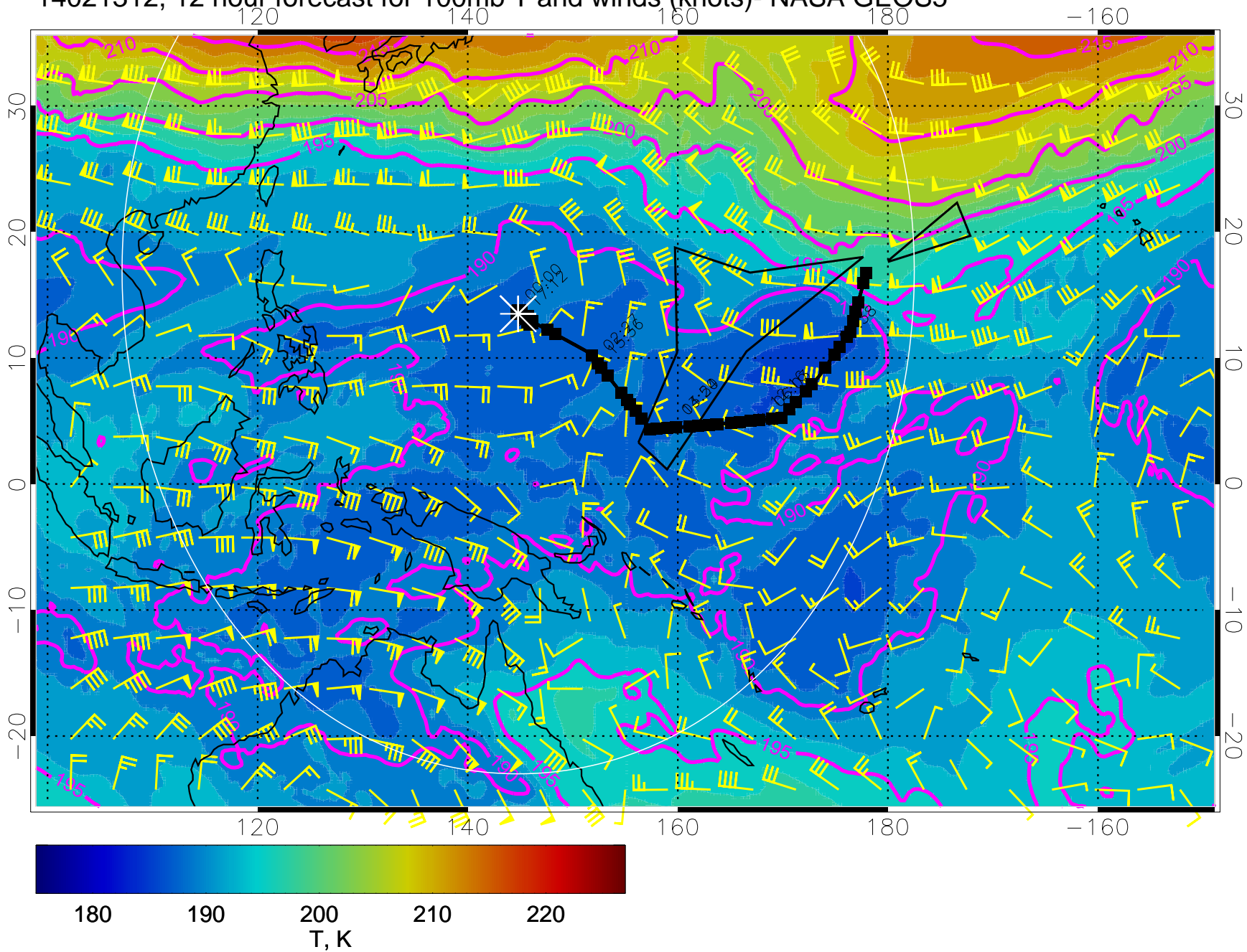
14021312, 12 hour forecast for 100mb T and winds (knots)- NASA GEOS5
