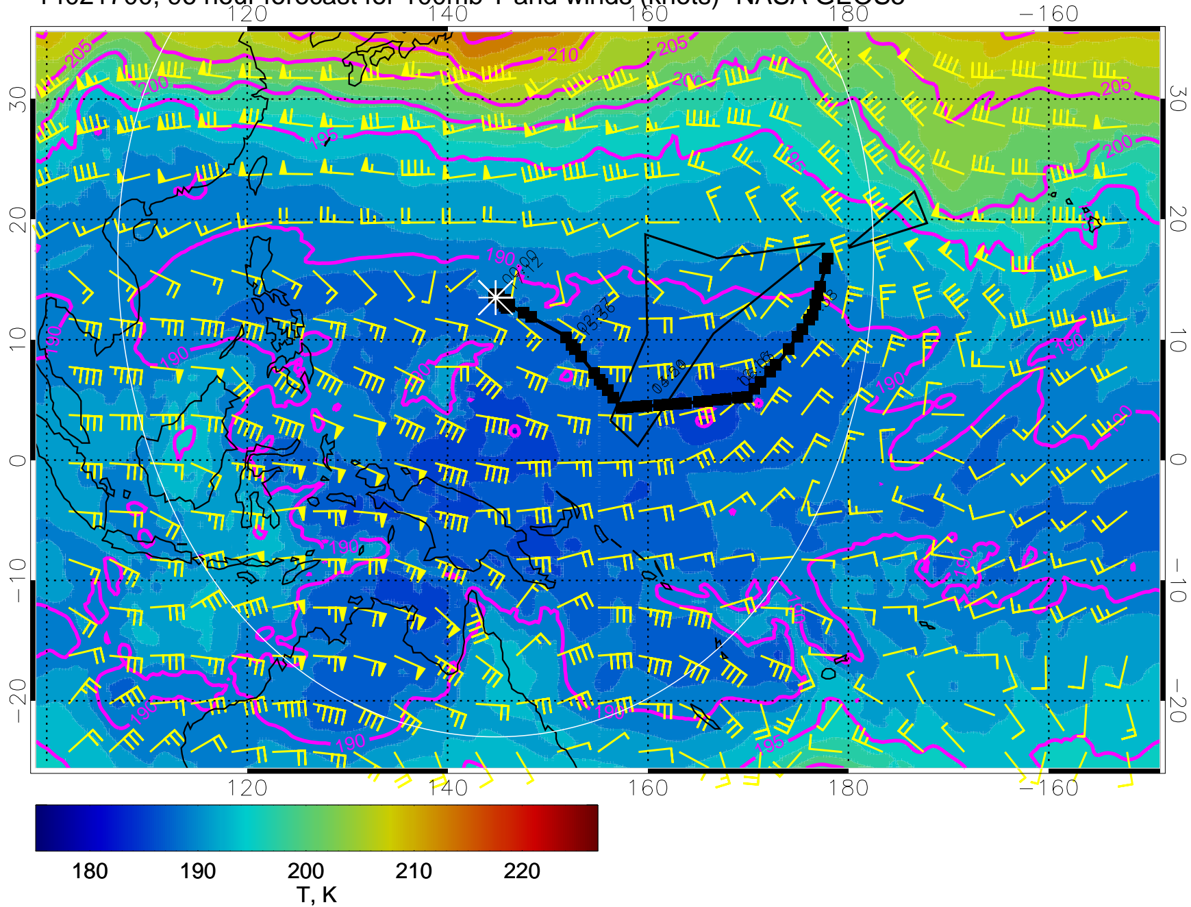
14021700, 96 hour forecast for 100mb T and winds (knots)- NASA GEOS5
