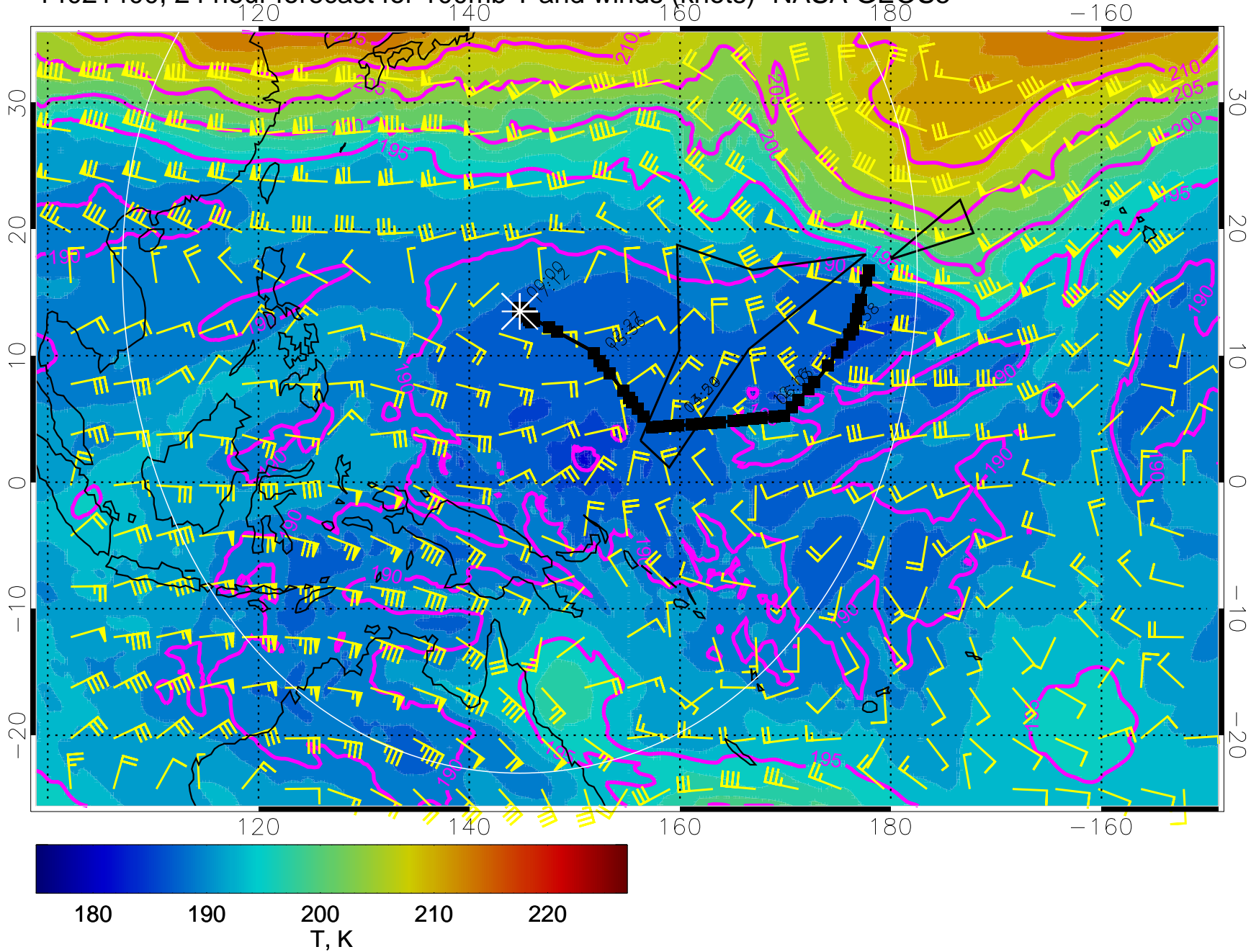
14021400, 24 hour forecast for 100mb T and winds (knots)- NASA GEOS5
