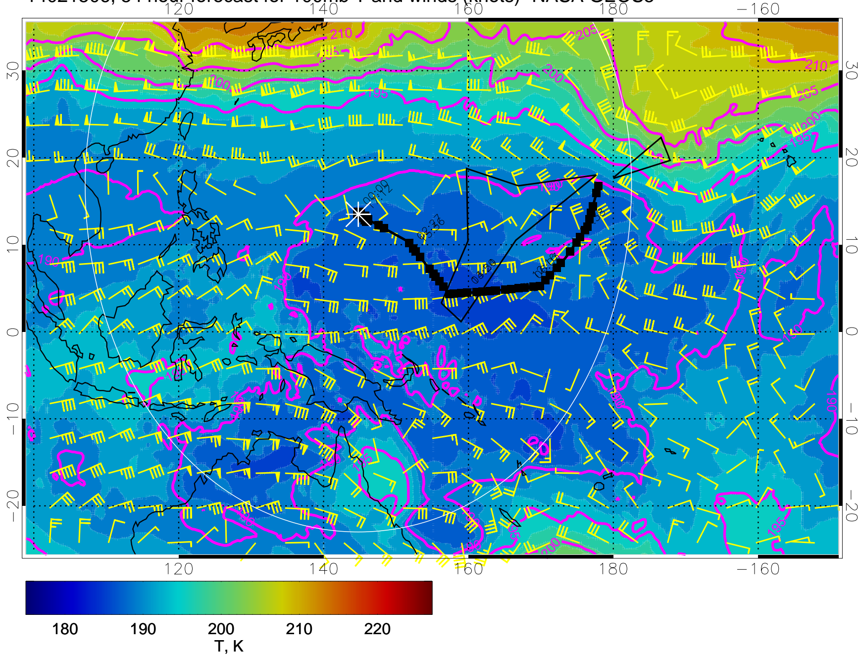
14021506, 54 hour forecast for 100mb T and winds (knots)- NASA GEOS5
