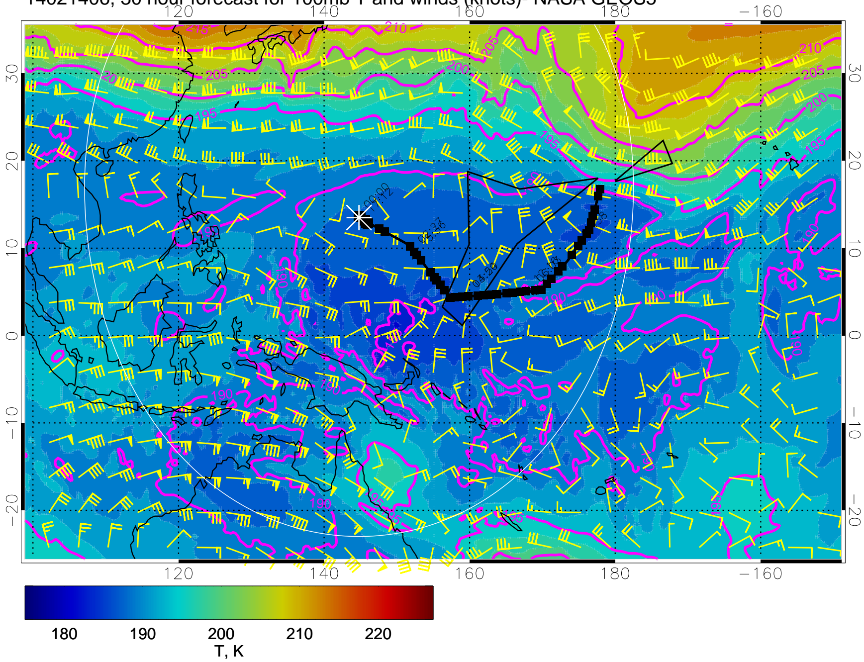
14021406, 30 hour forecast for 100mb T and winds (knots)- NASA GEOS5
