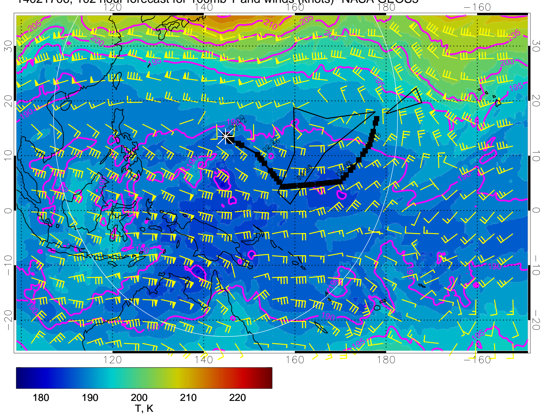
14021706, 102 hour forecast for 100mb T and winds (knots)- NASA GEOS5
