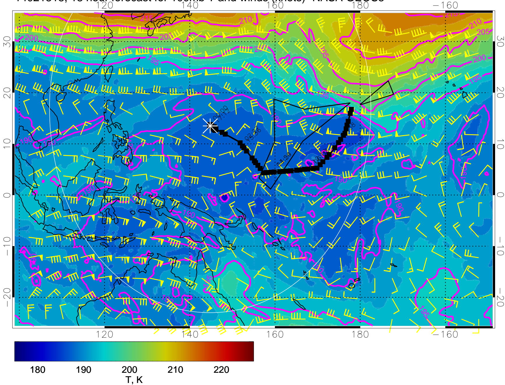
14021318, 18 hour forecast for 100mb T and winds (knots)- NASA GEOS5
