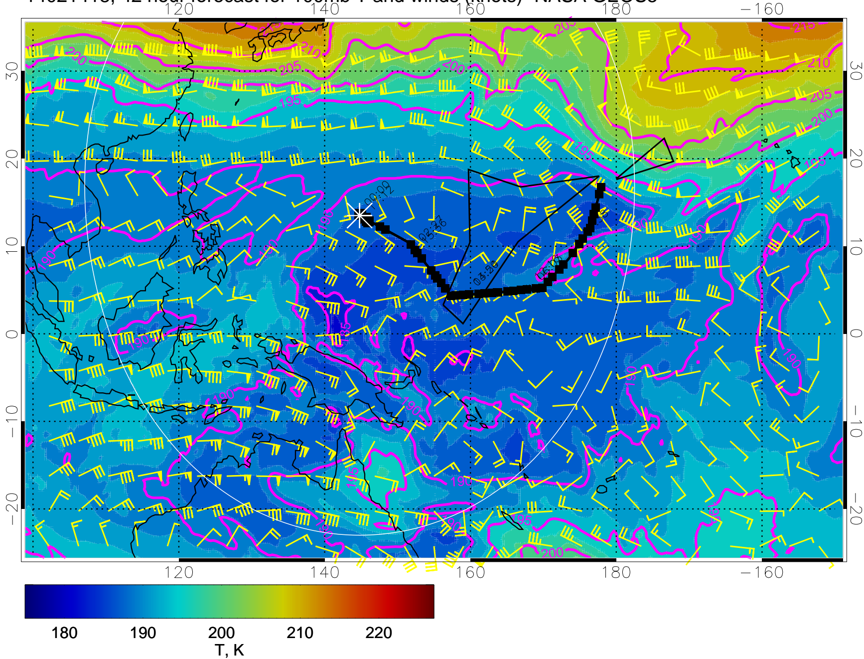
14021418, 42 hour forecast for 100mb T and winds (knots)- NASA GEOS5
