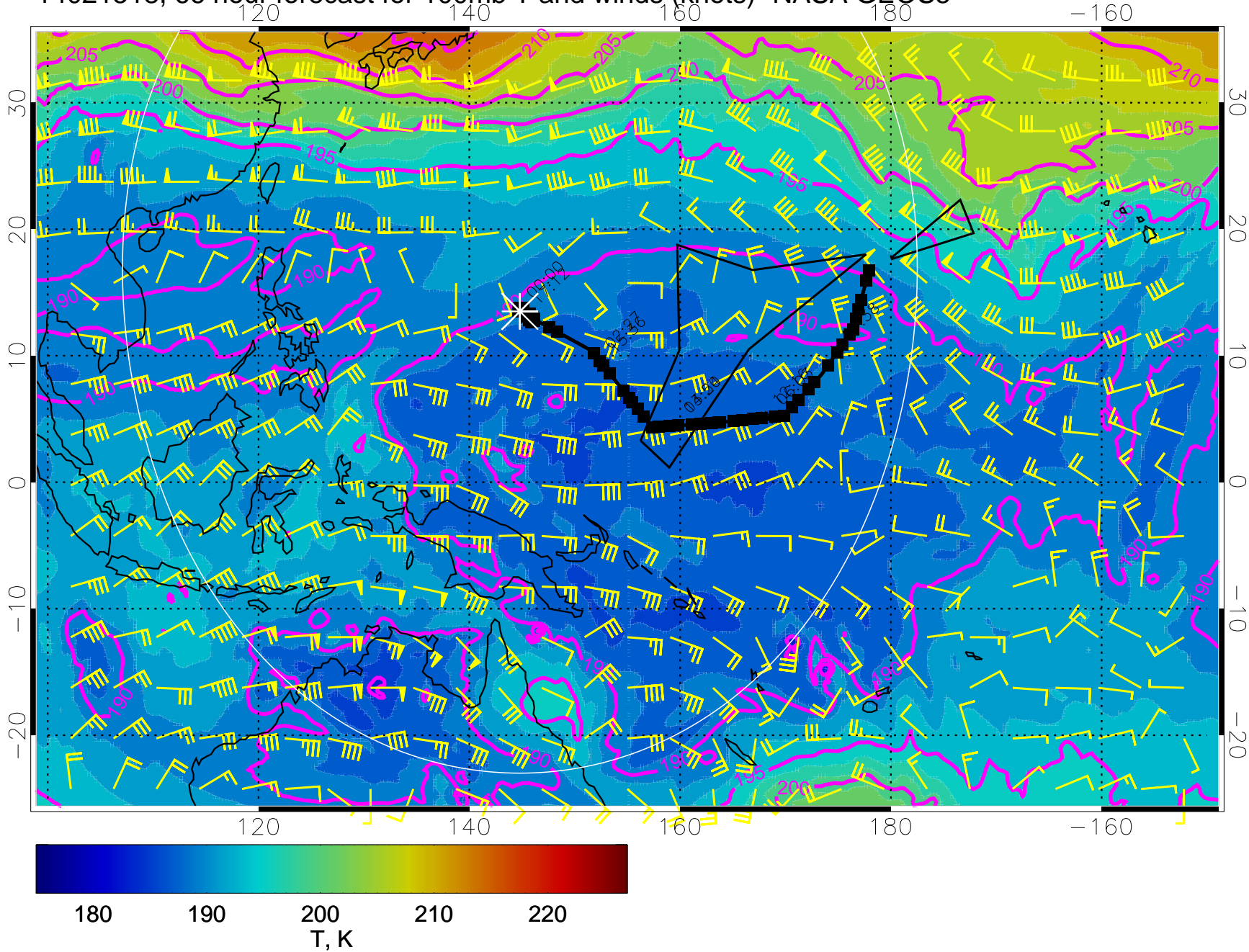
14021518, 66 hour forecast for 100mb T and winds (knots)- NASA GEOS5
