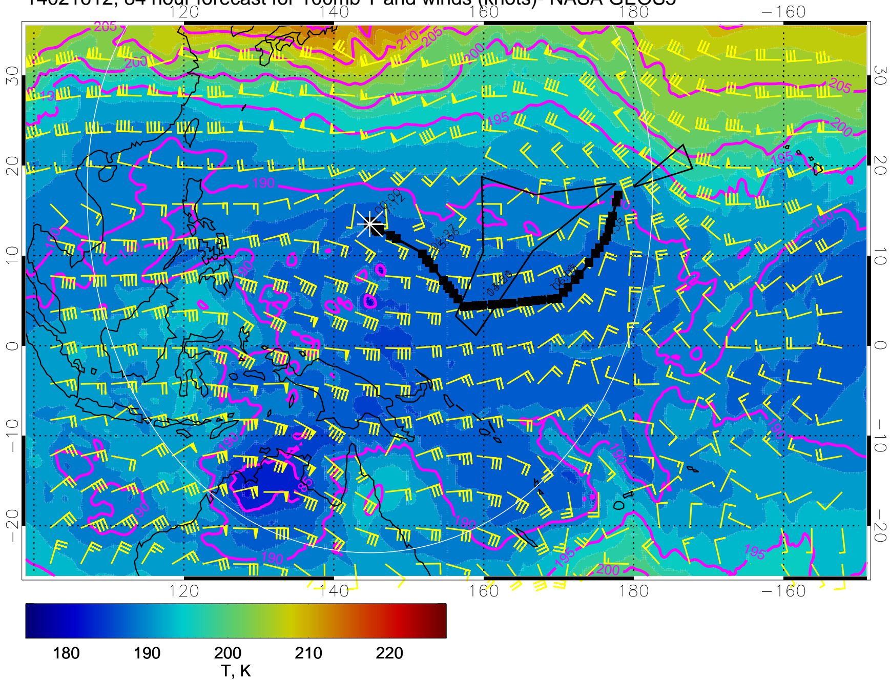
14021612, 84 hour forecast for 100mb T and winds (knots)- NASA GEOS5
