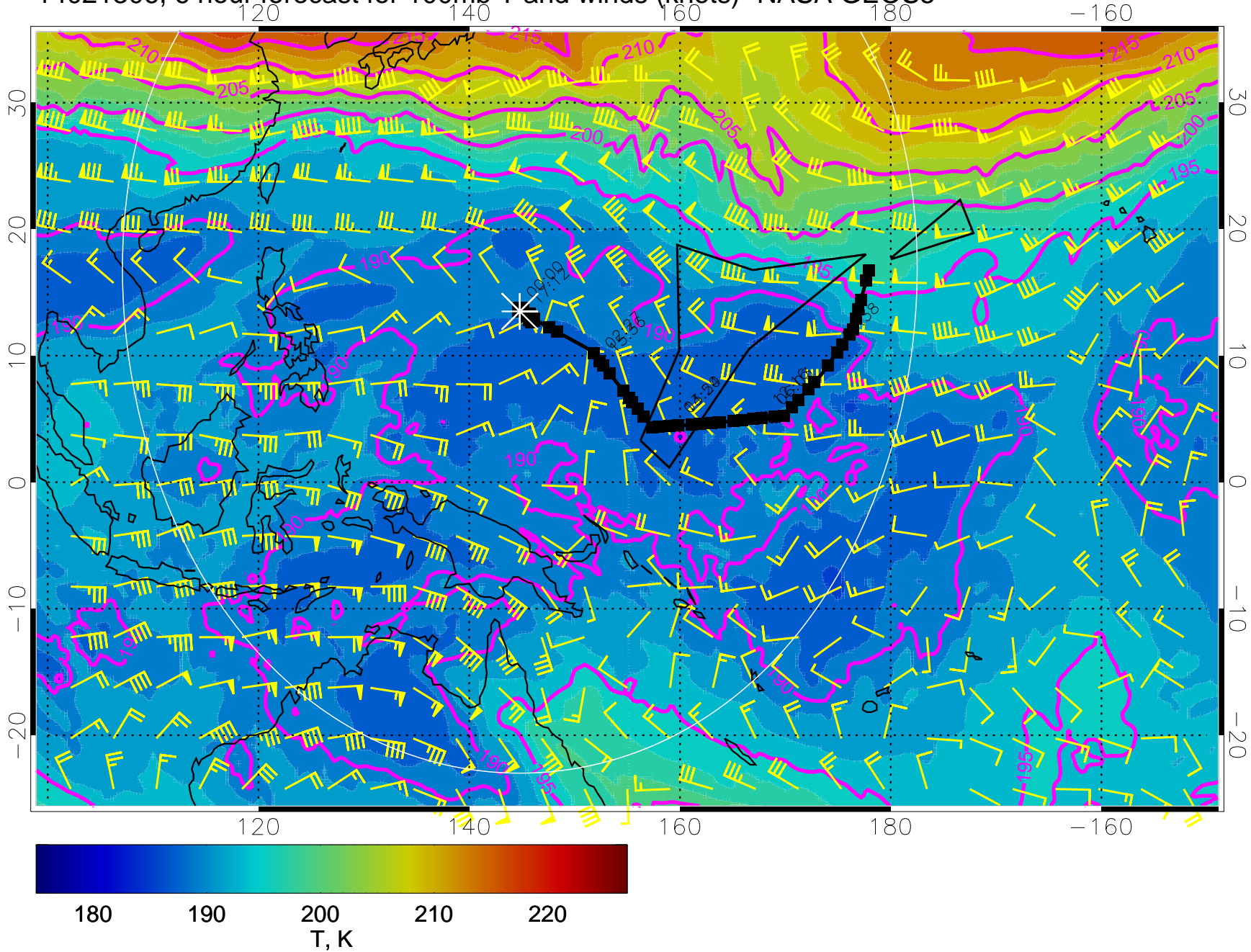
14021306, 6 hour forecast for 100mb T and winds (knots)- NASA GEOS5
