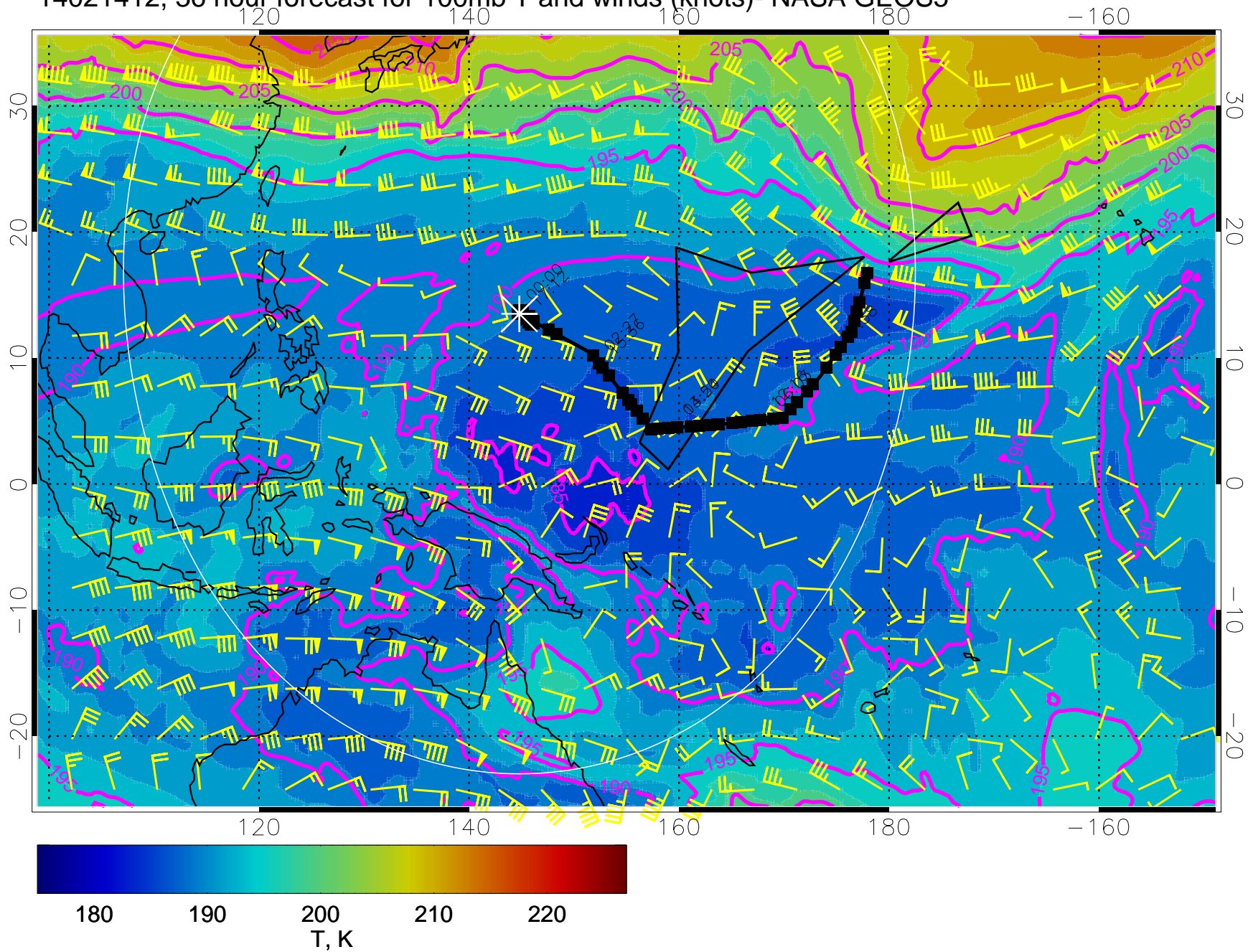
14021412, 36 hour forecast for 100mb T and winds (knots)- NASA GEOS5
