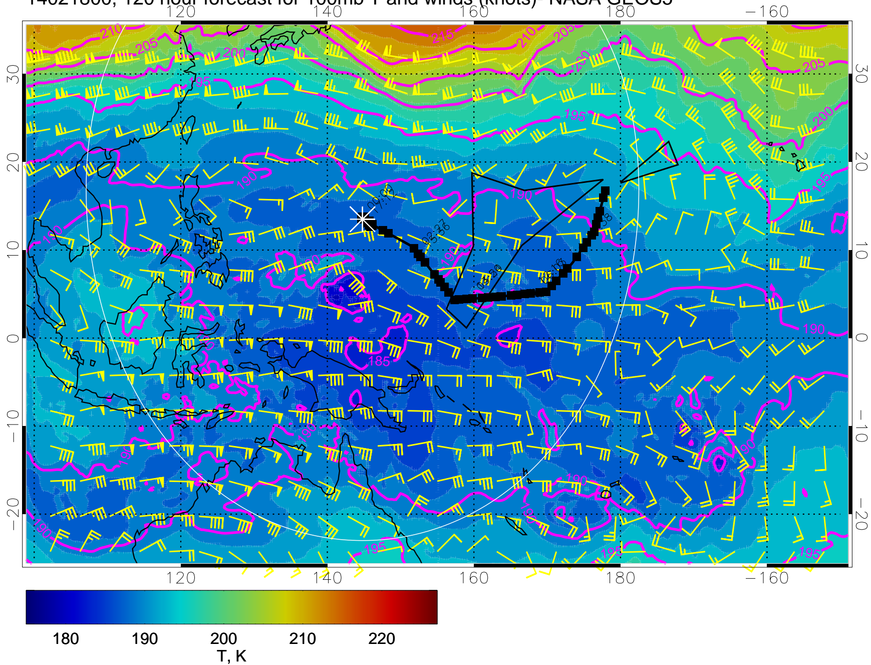
14021800, 120 hour forecast for 100mb T and winds (knots)- NASA GEOS5
