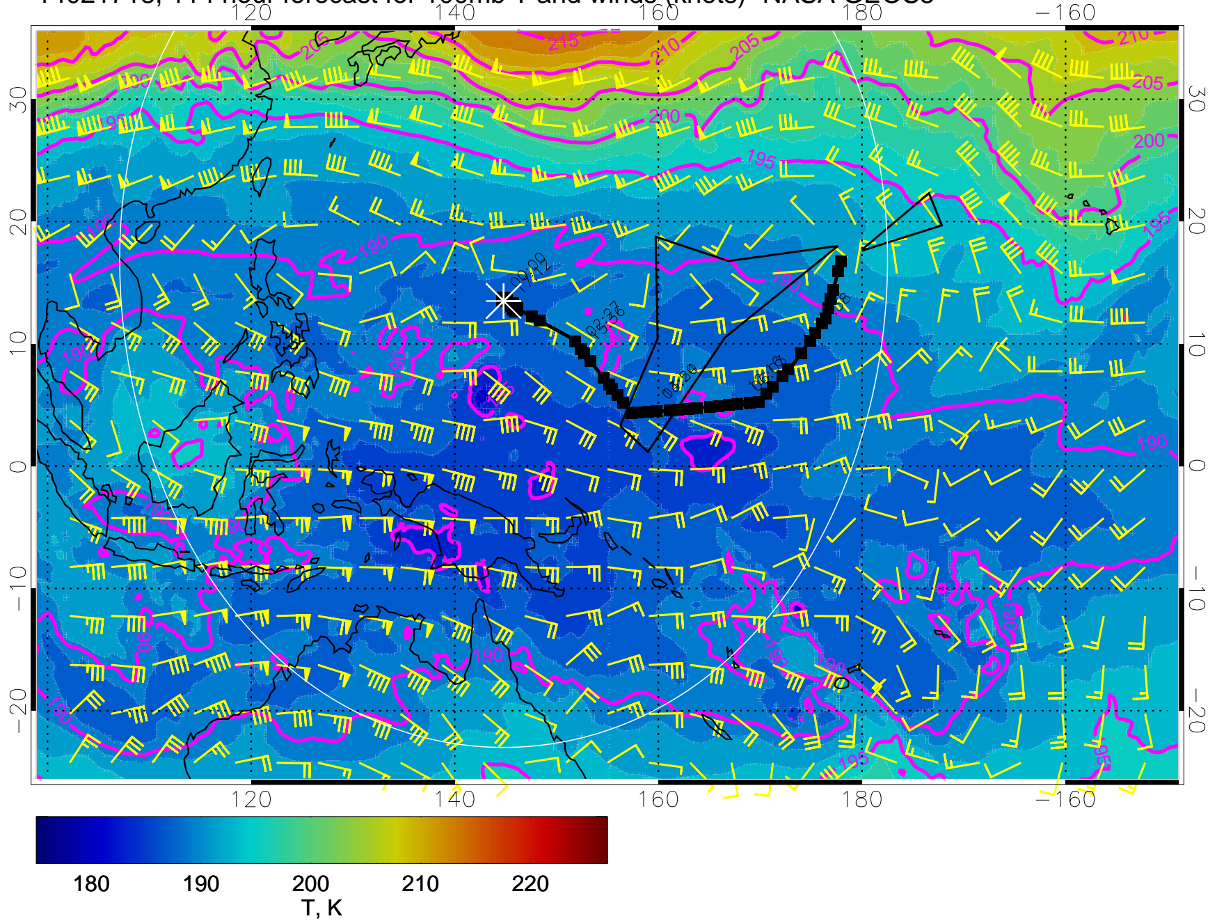
14021718, 114 hour forecast for 100mb T and winds (knots)- NASA GEOS5
