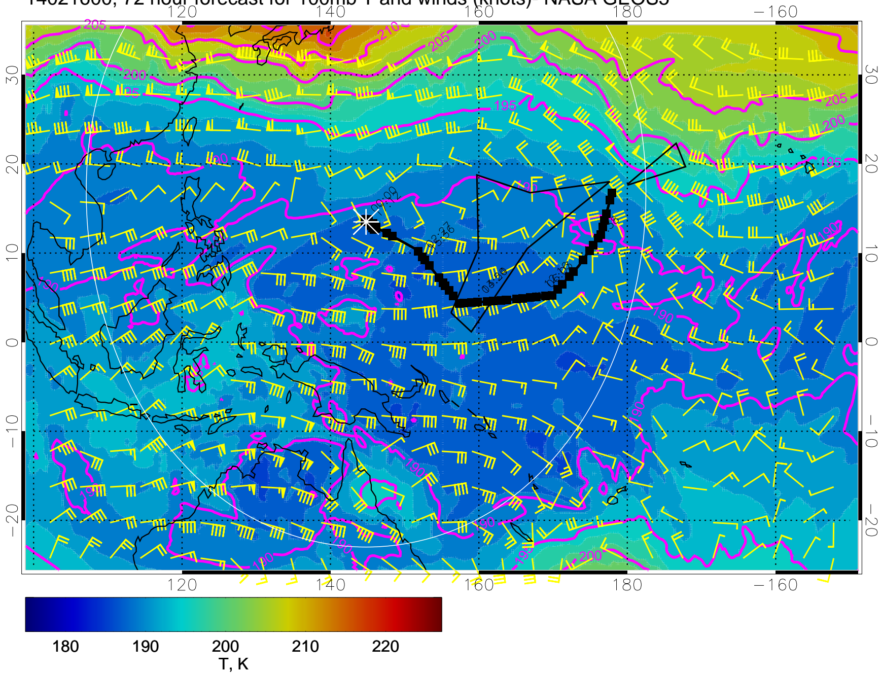
14021600, 72 hour forecast for 100mb T and winds (knots)- NASA GEOS5
