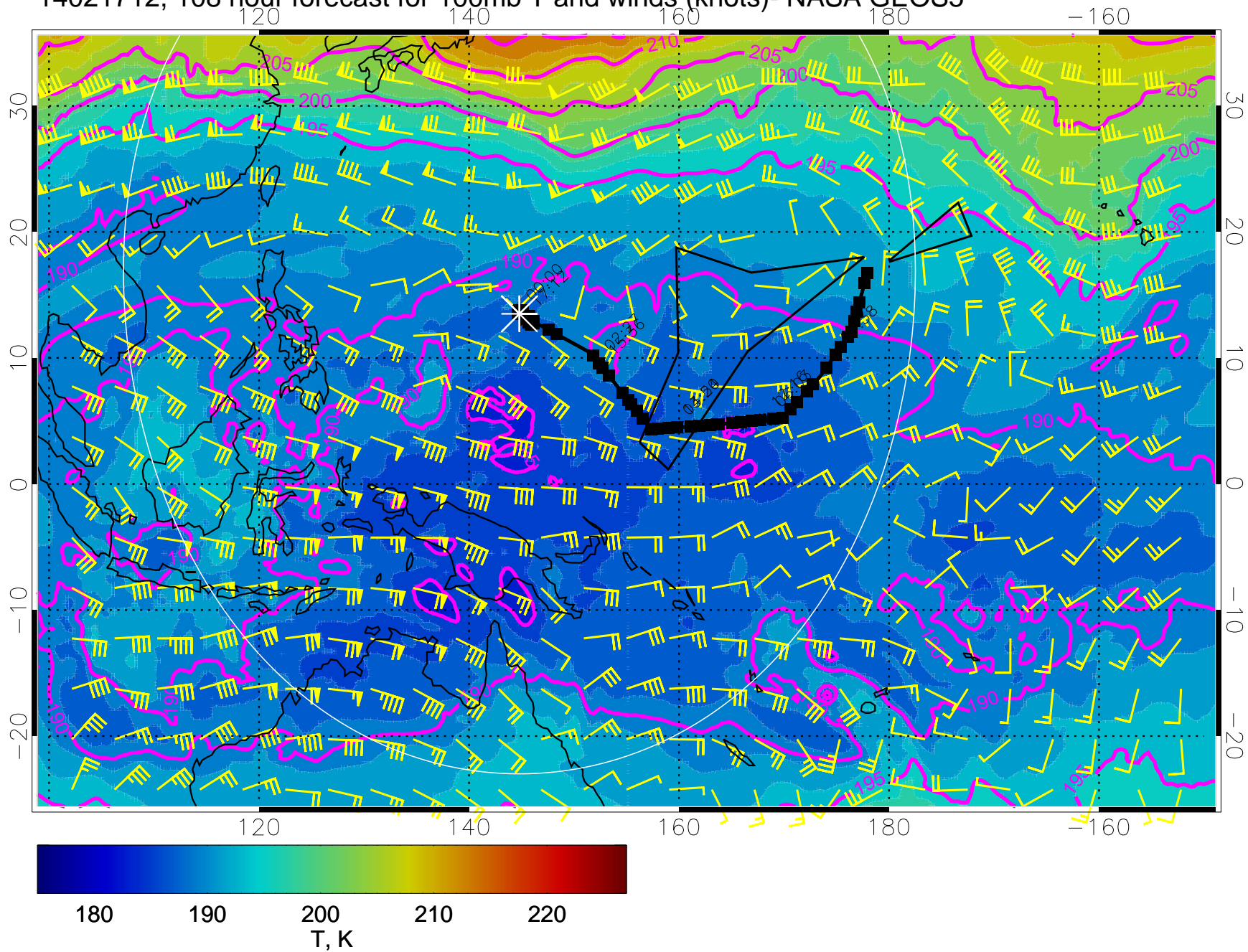
14021712, 108 hour forecast for 100mb T and winds (knots)- NASA GEOS5
