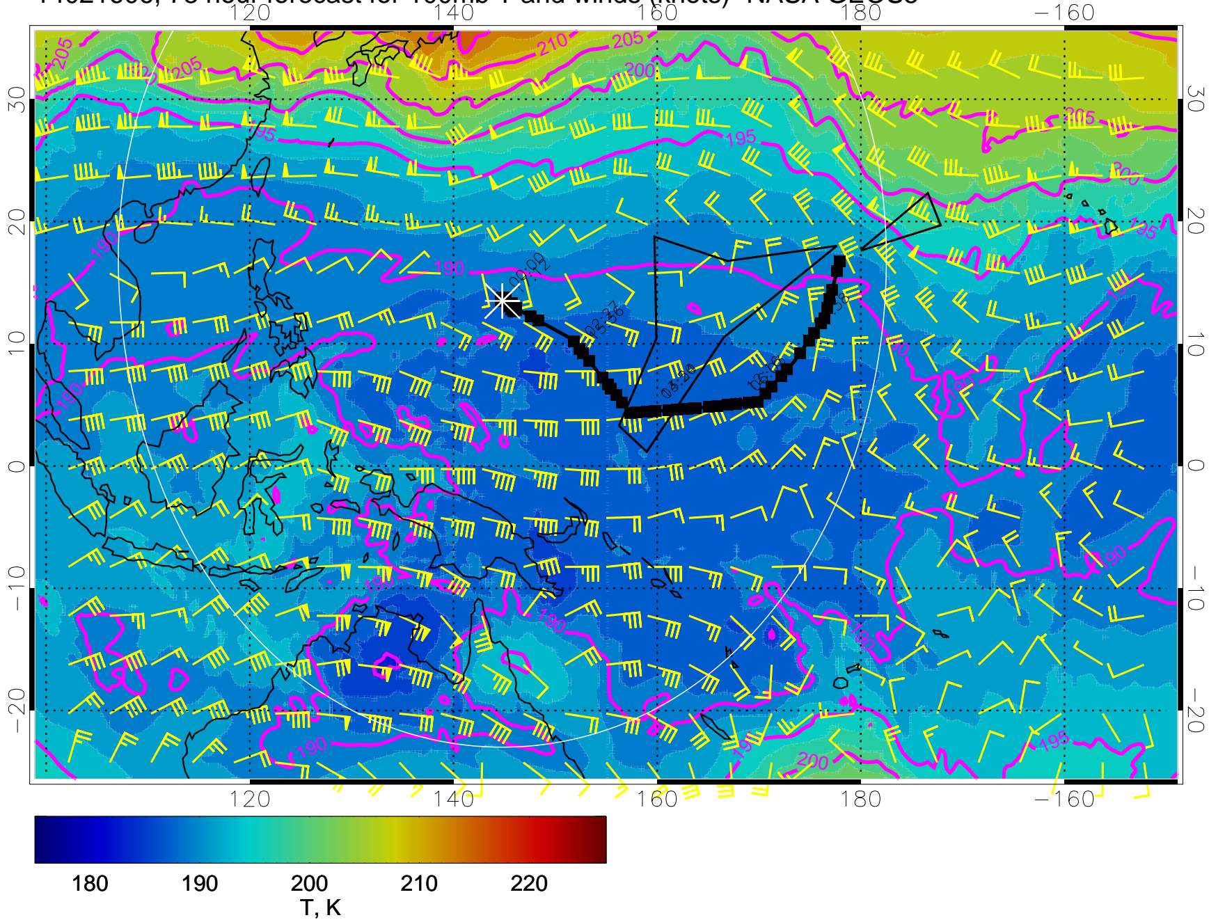
14021606, 78 hour forecast for 100mb T and winds (knots)- NASA GEOS5
