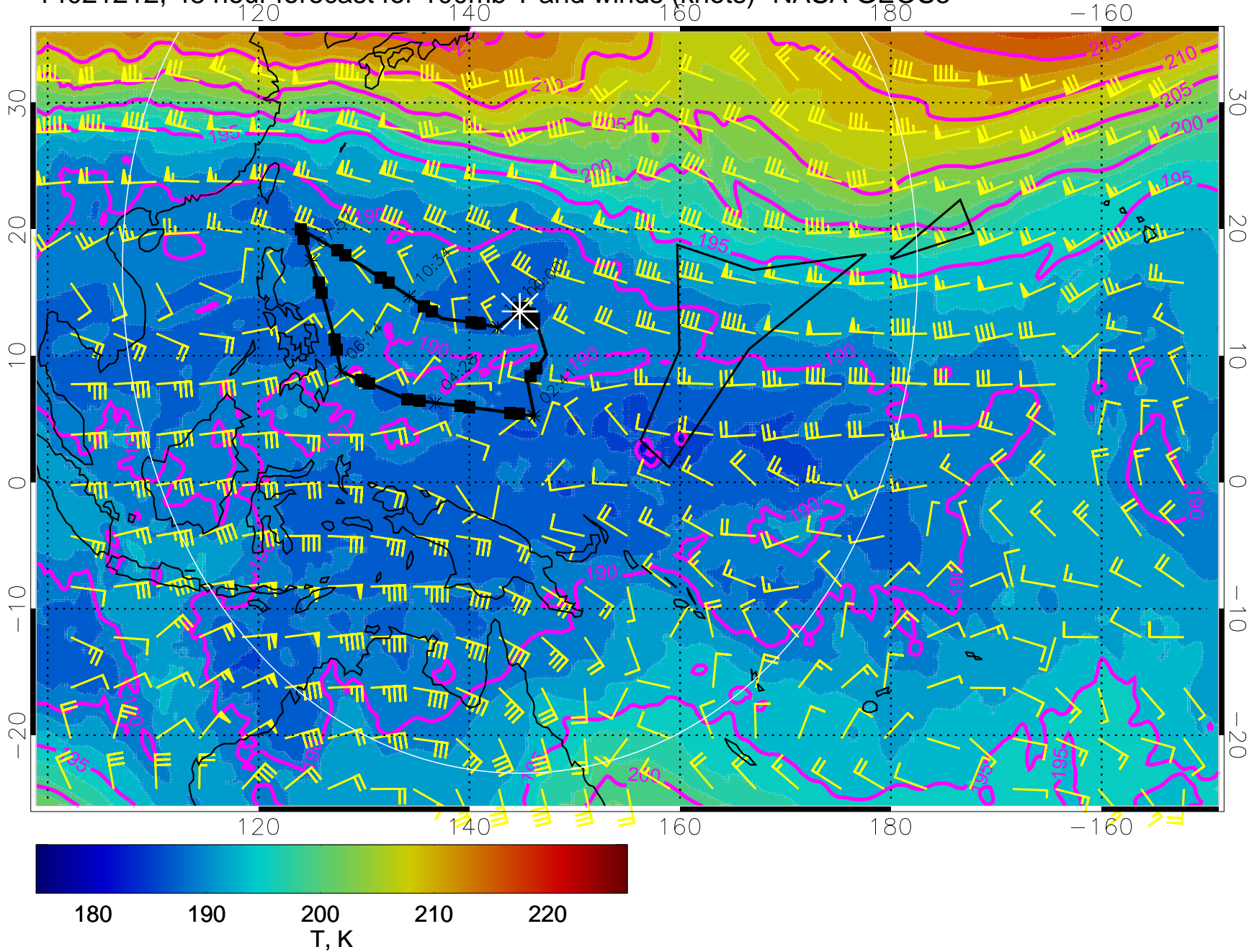
14021212, 48 hour forecast for 100mb T and winds (knots)- NASA GEOS5
