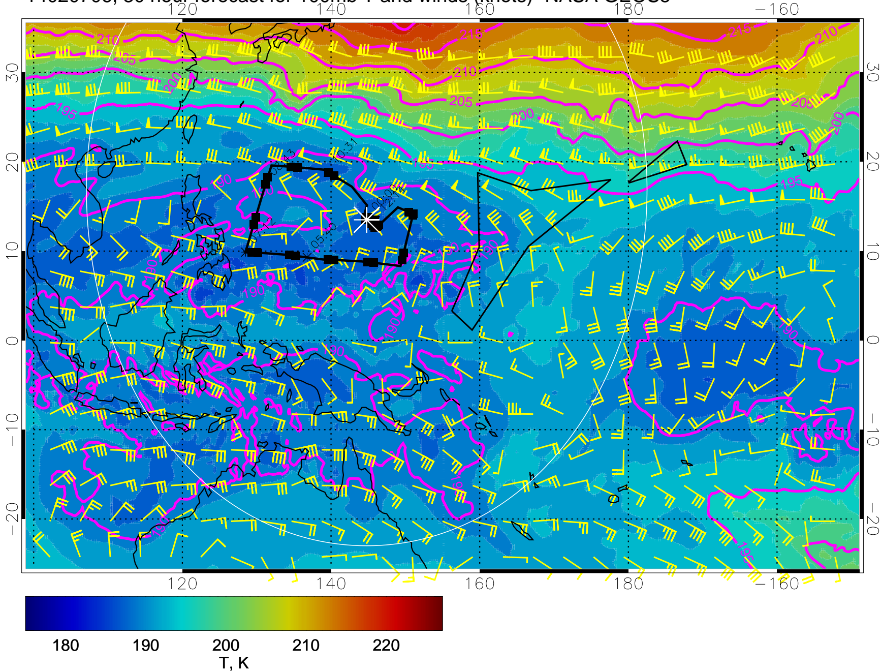
14020706, 30 hour forecast for 100mb T and winds (knots)- NASA GEOS5
