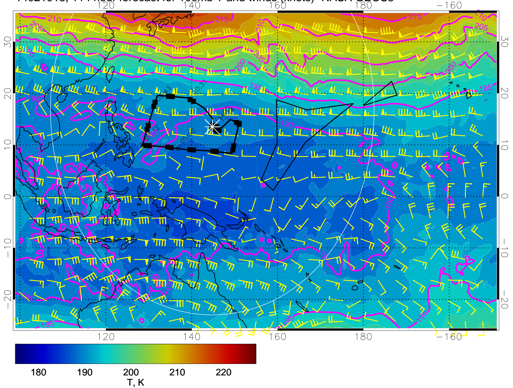
14021018, 114 hour forecast for 100mb T and winds (knots)- NASA GEOS5
