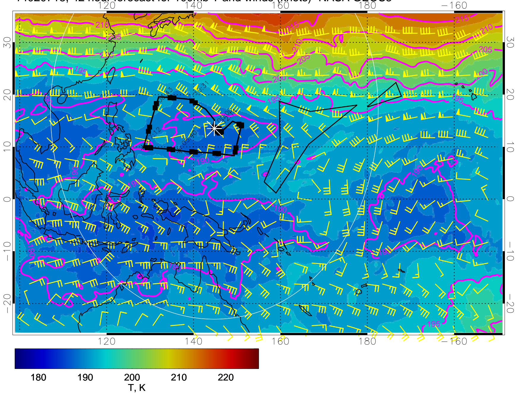
14020718, 42 hour forecast for 100mb T and winds (knots)- NASA GEOS5
