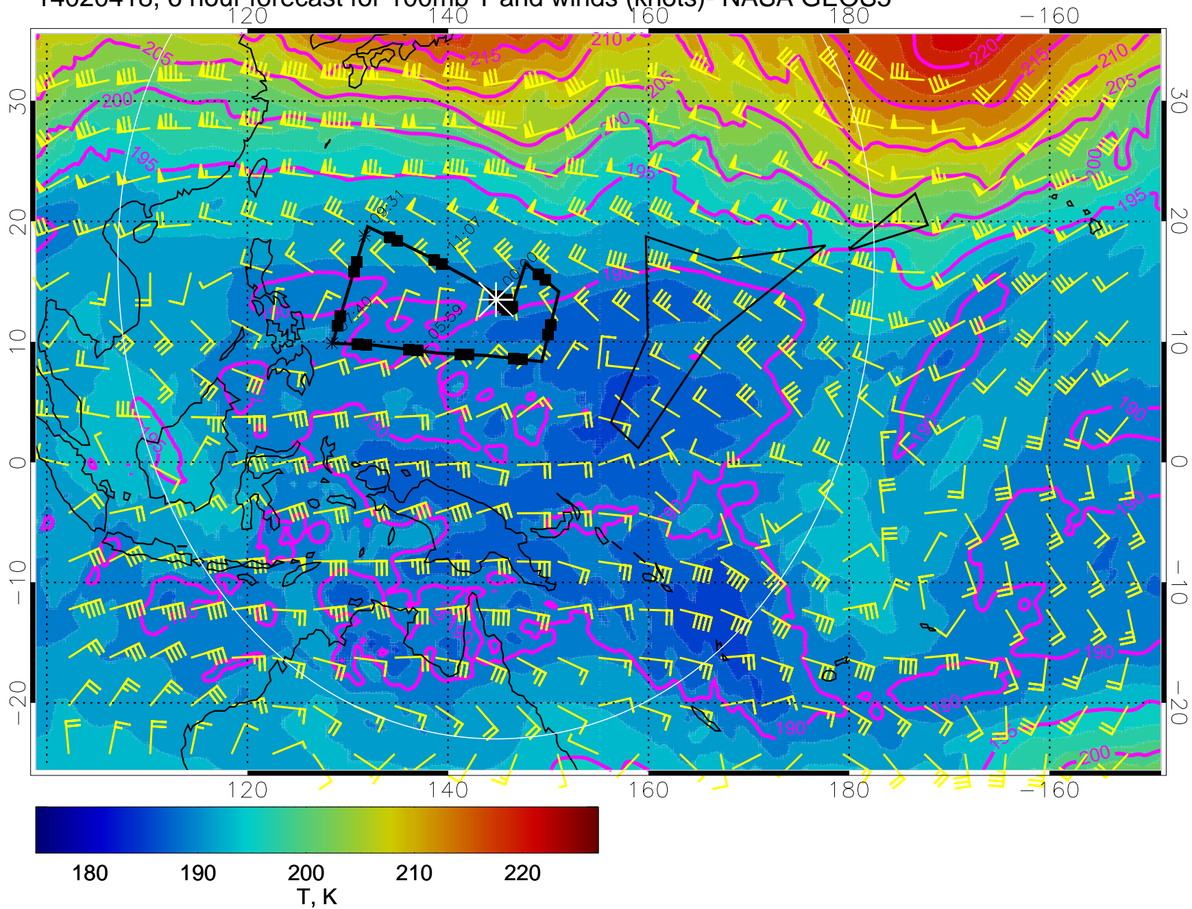
14020418, 6 hour forecast for 100mb T and winds (knots)- NASA GEOS5
