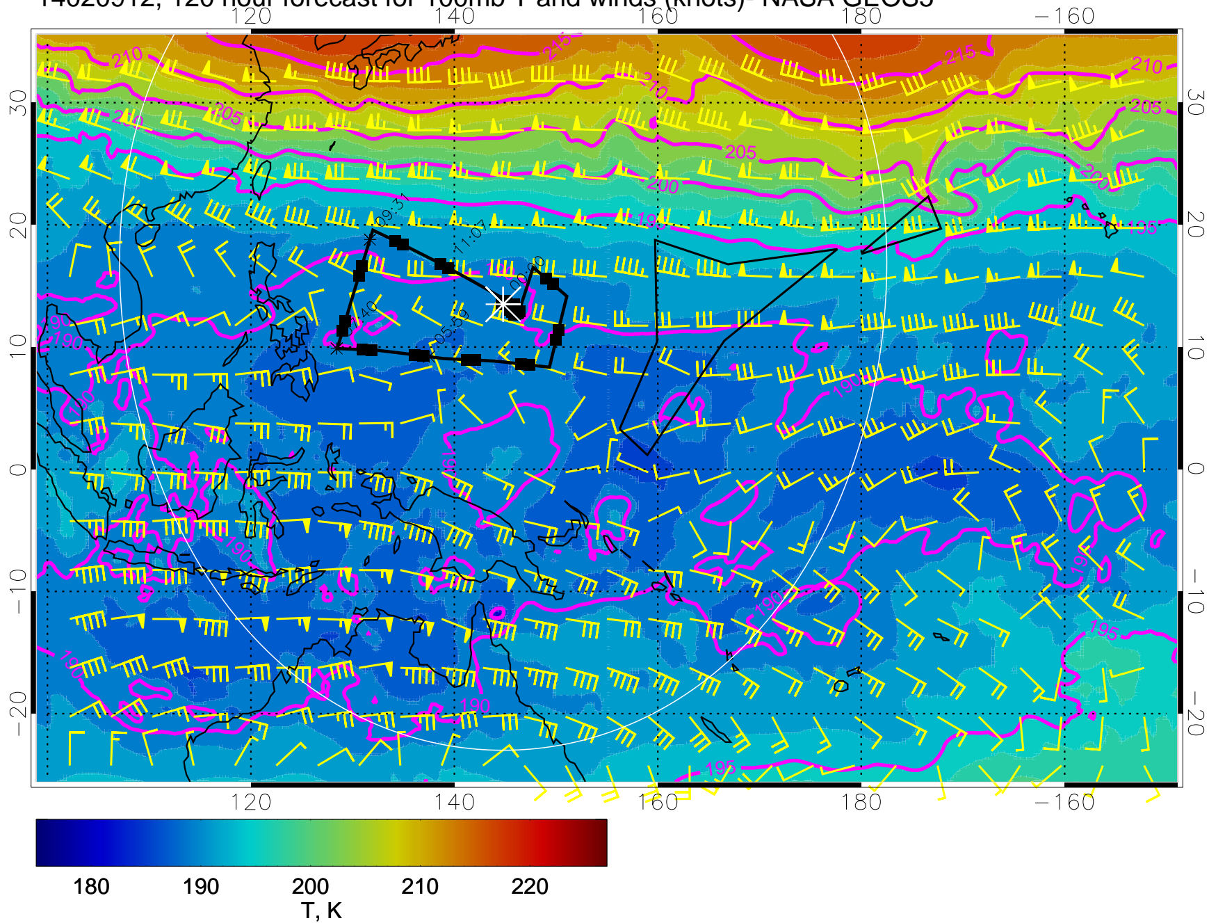
14020912, 120 hour forecast for 100mb T and winds (knots)- NASA GEOS5
