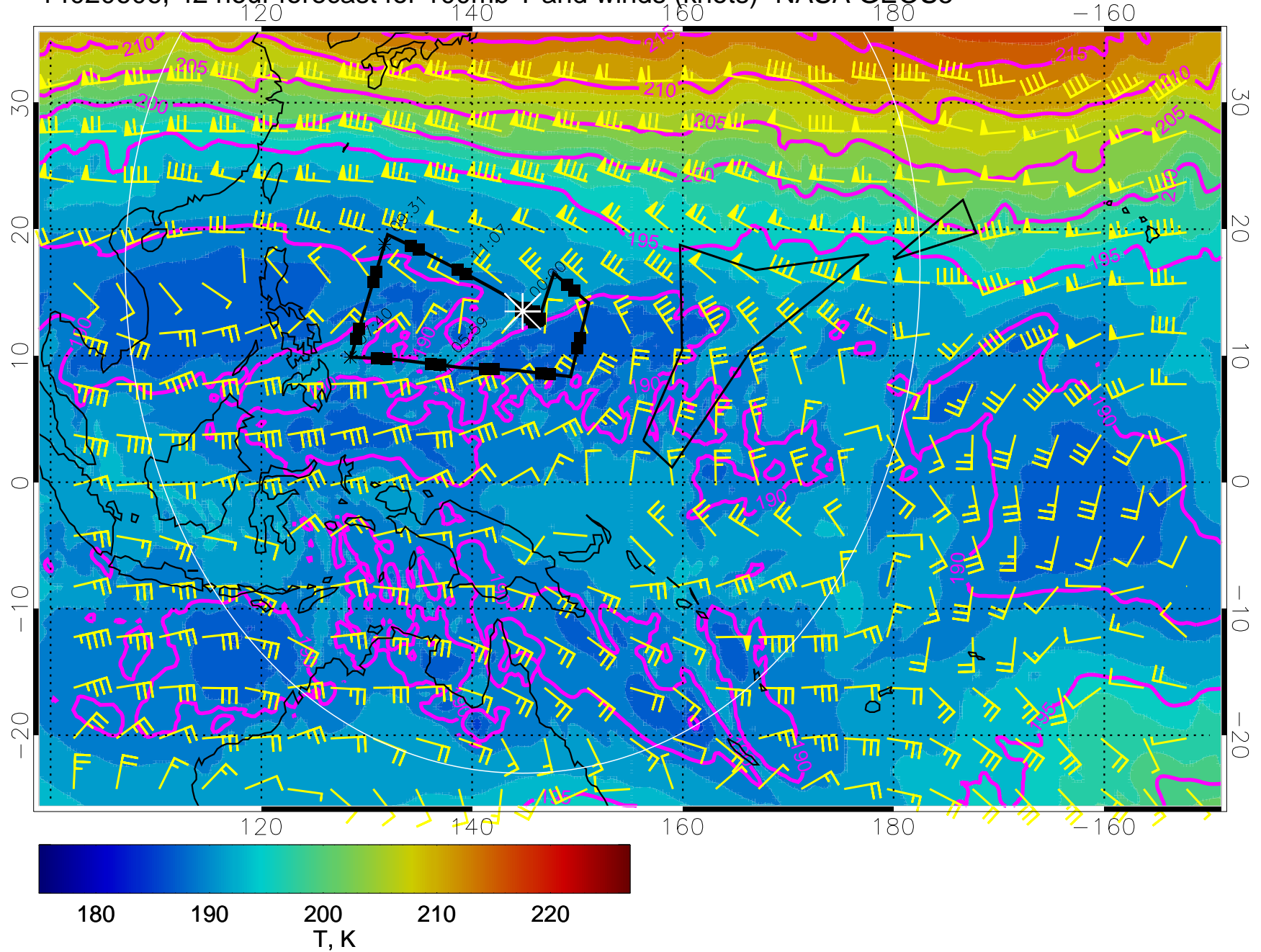
14020606, 42 hour forecast for 100mb T and winds (knots)- NASA GEOS5
