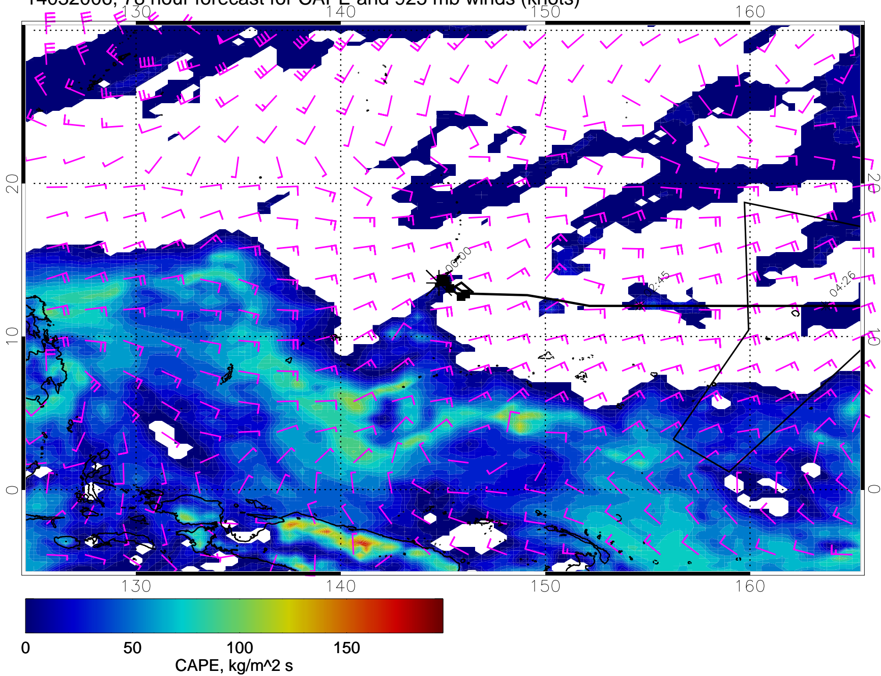
14032006, 78 hour forecast for CAPE and 925 mb winds (knots)
