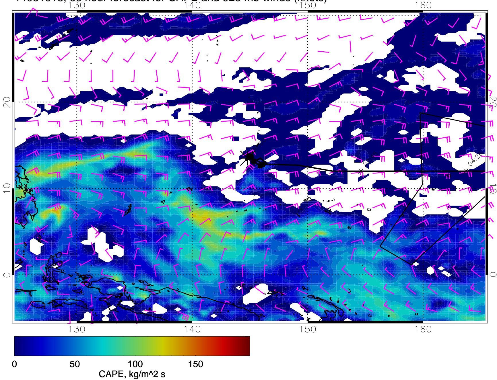
14031918, 66 hour forecast for CAPE and 925 mb winds (knots)
