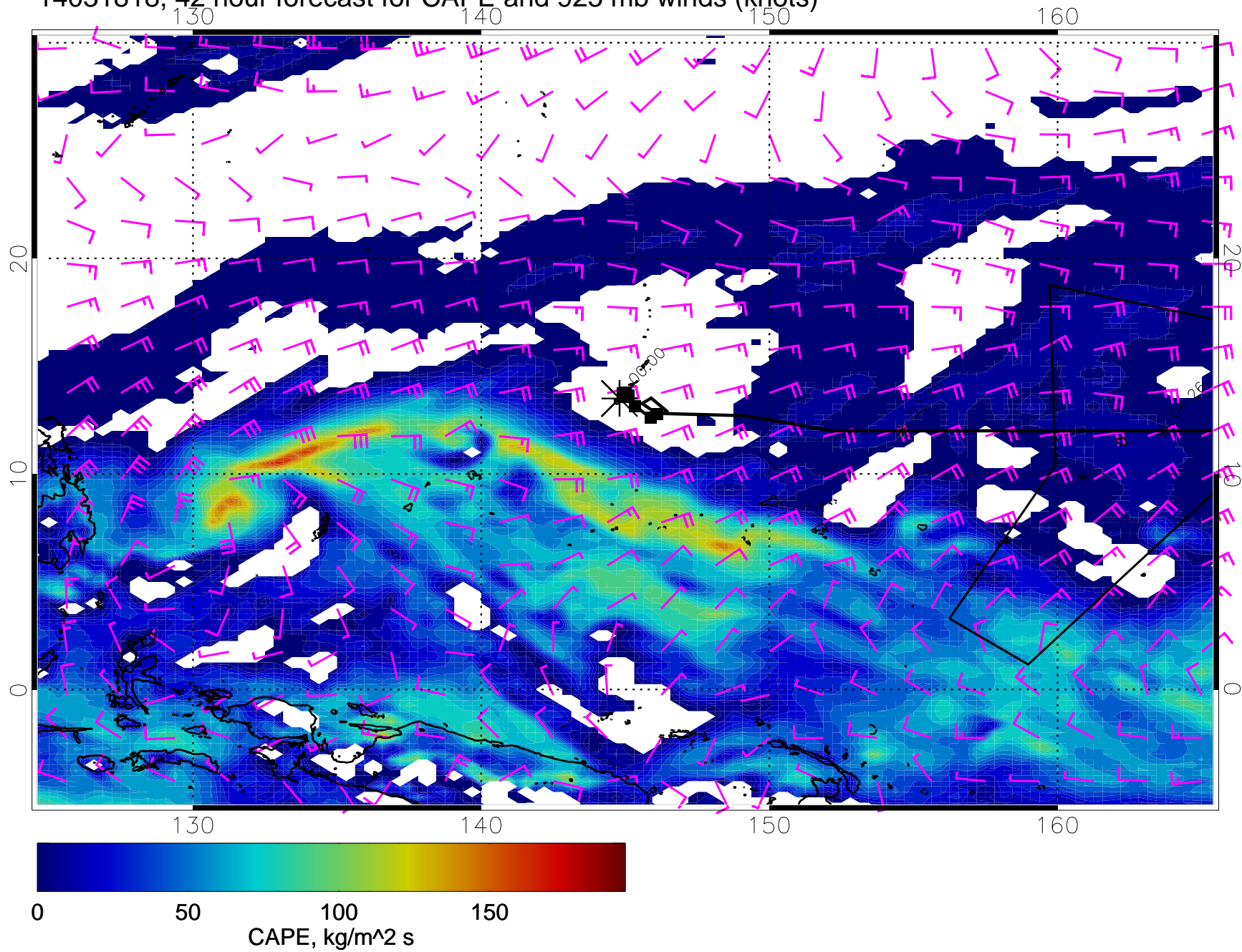
14031818, 42 hour forecast for CAPE and 925 mb winds (knots)
