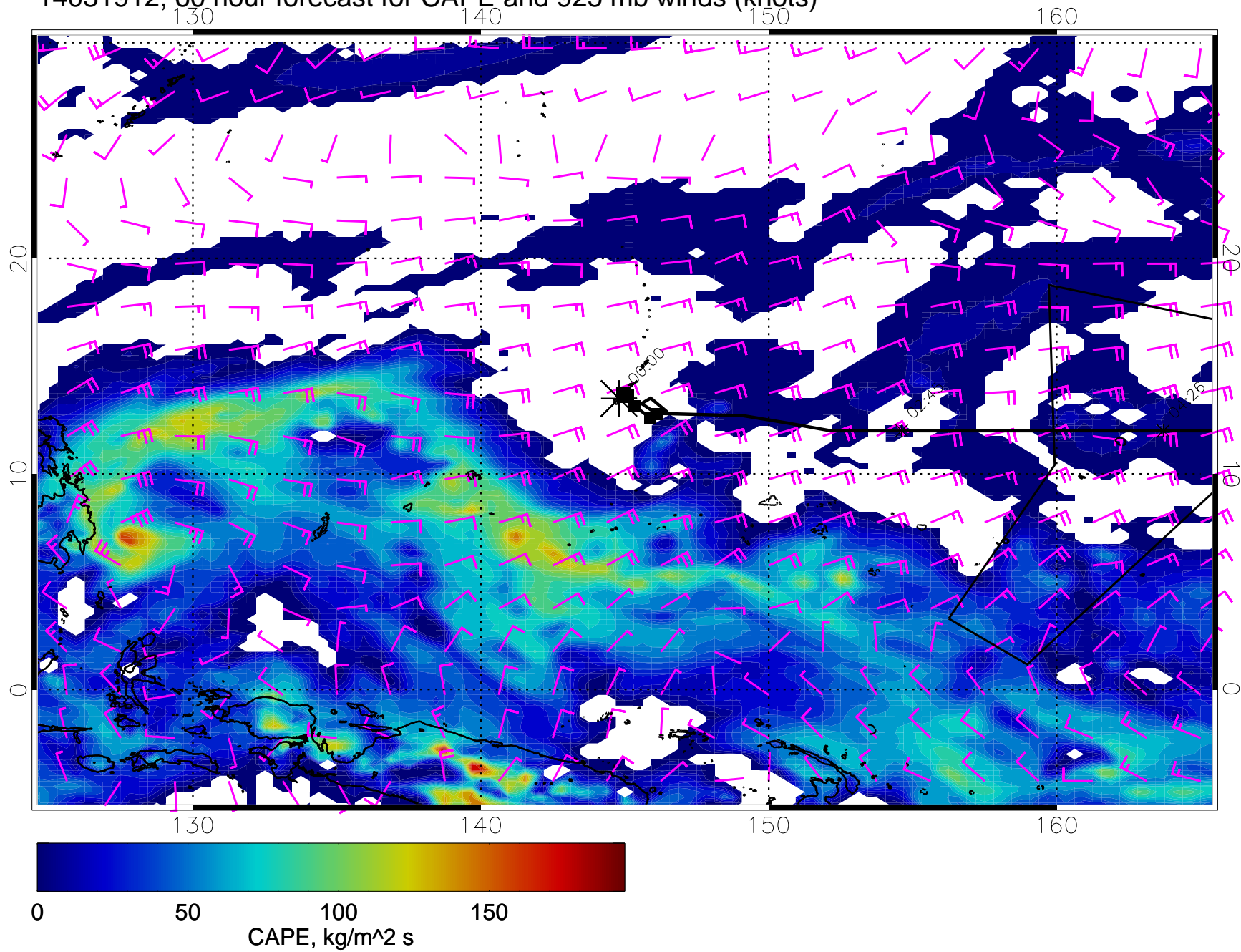
14031912, 60 hour forecast for CAPE and 925 mb winds (knots)
