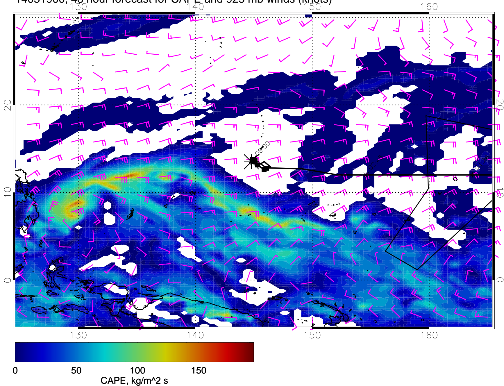
14031900, 48 hour forecast for CAPE and 925 mb winds (knots)
