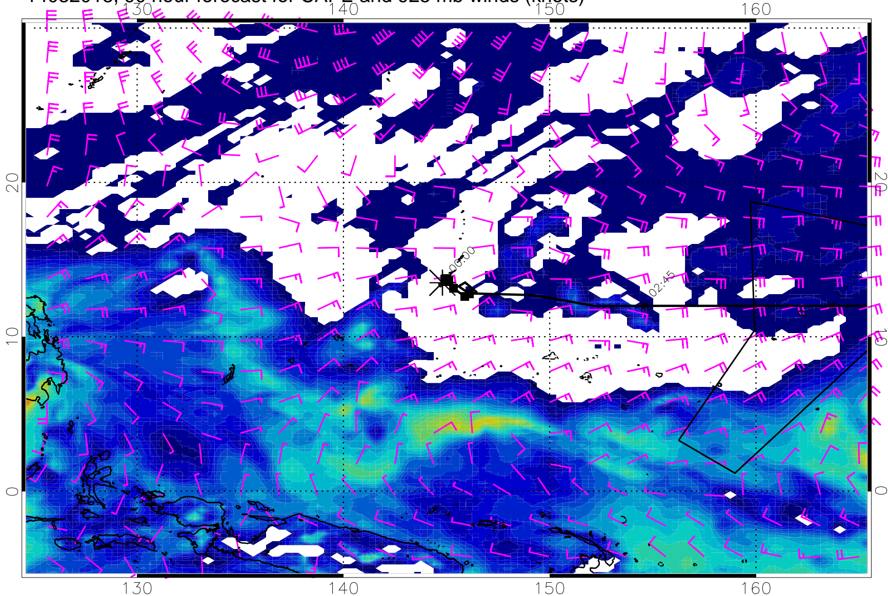
14032018, 90 hour forecast for CAPE and 925 mb winds (knots)
