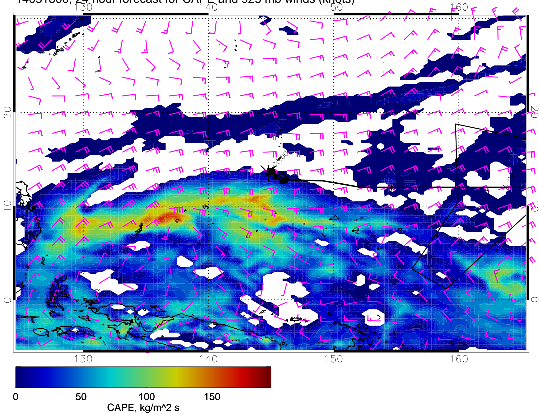
14031800, 24 hour forecast for CAPE and 925 mb winds (knots)
