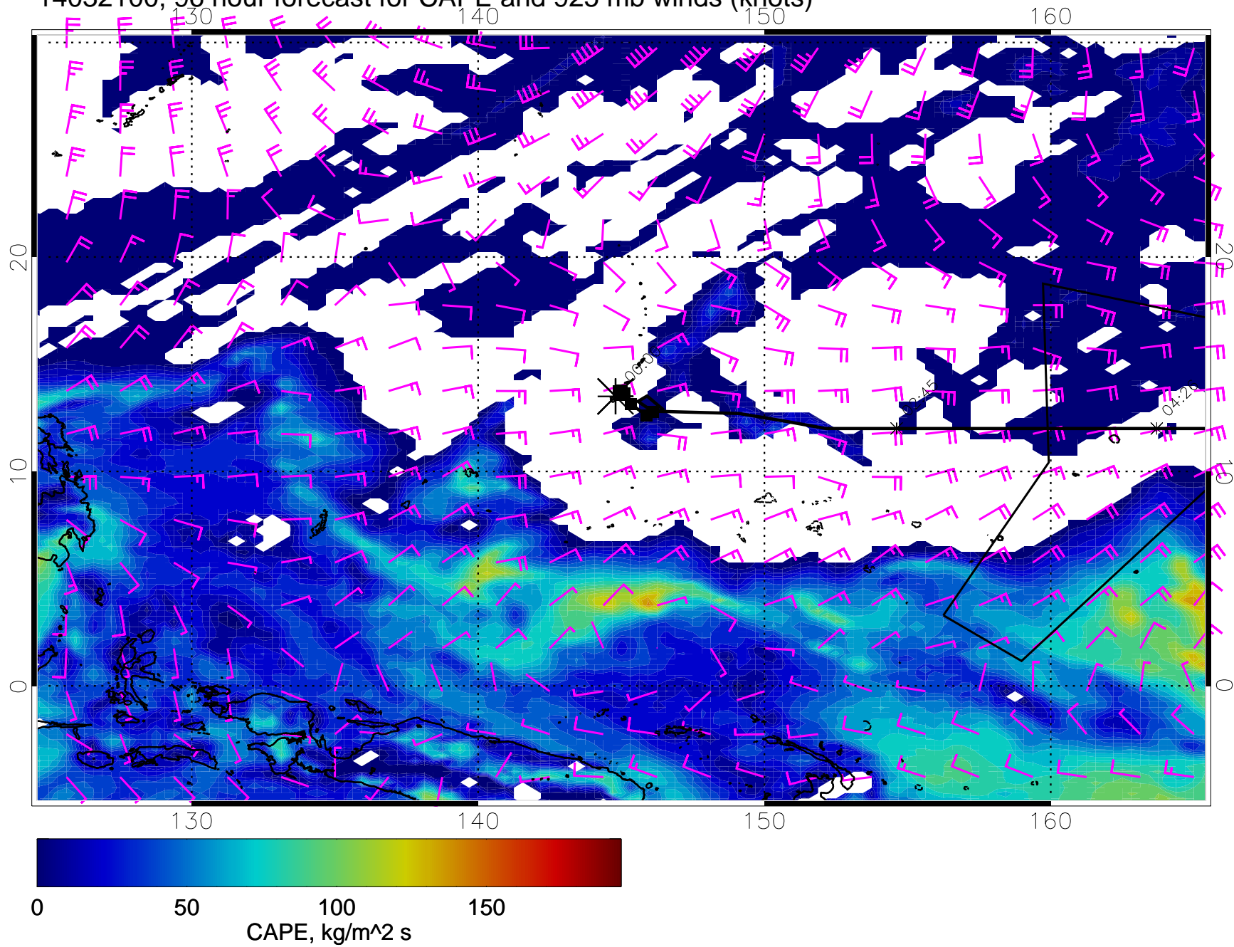
14032100, 96 hour forecast for CAPE and 925 mb winds (knots)
