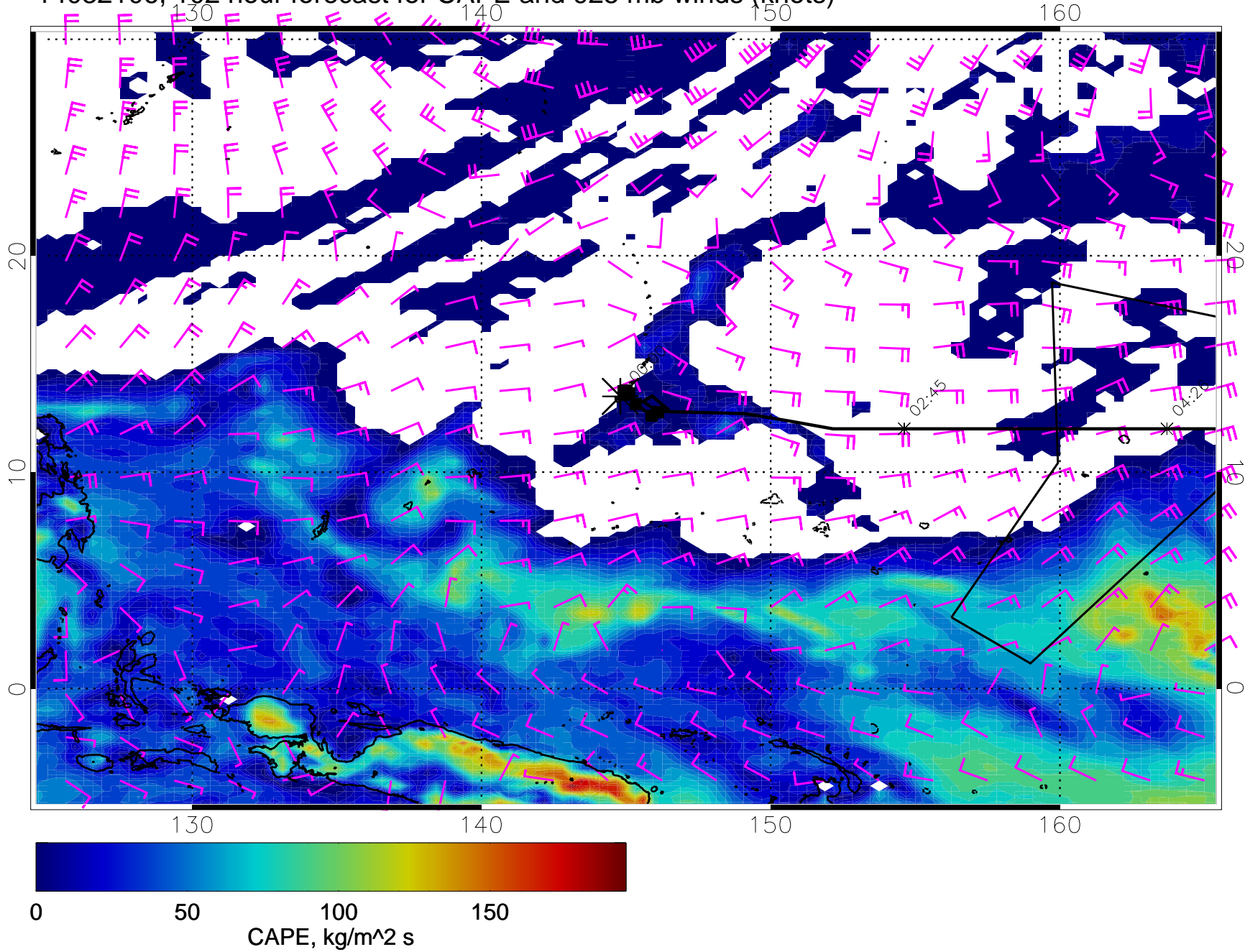
14032106, 102 hour forecast for CAPE and 925 mb winds (knots)
