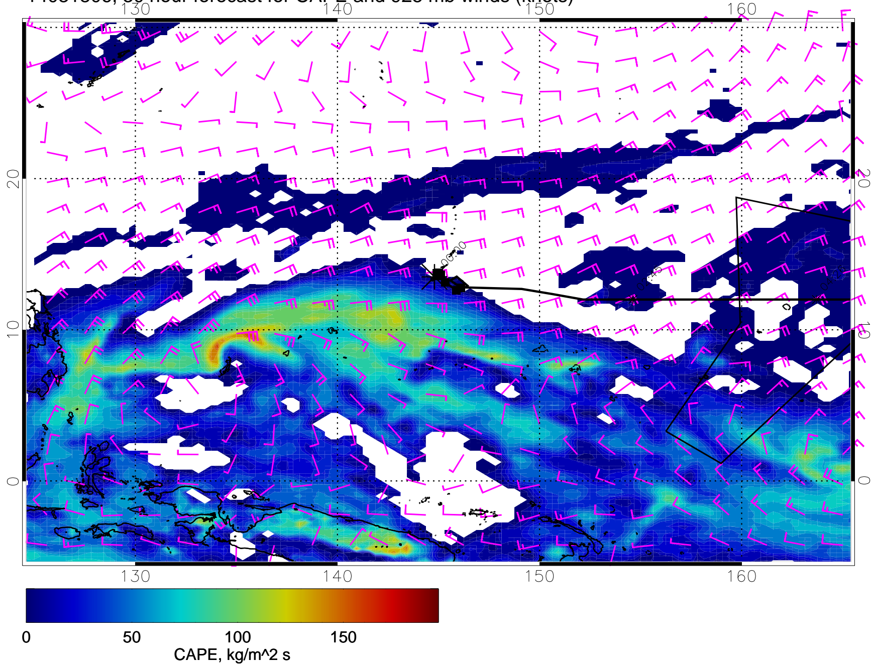
14031806, 30 hour forecast for CAPE and 925 mb winds (knots)
