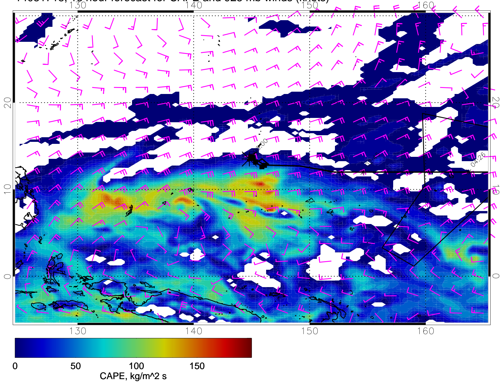
14031718, 18 hour forecast for CAPE and 925 mb winds (knots)
