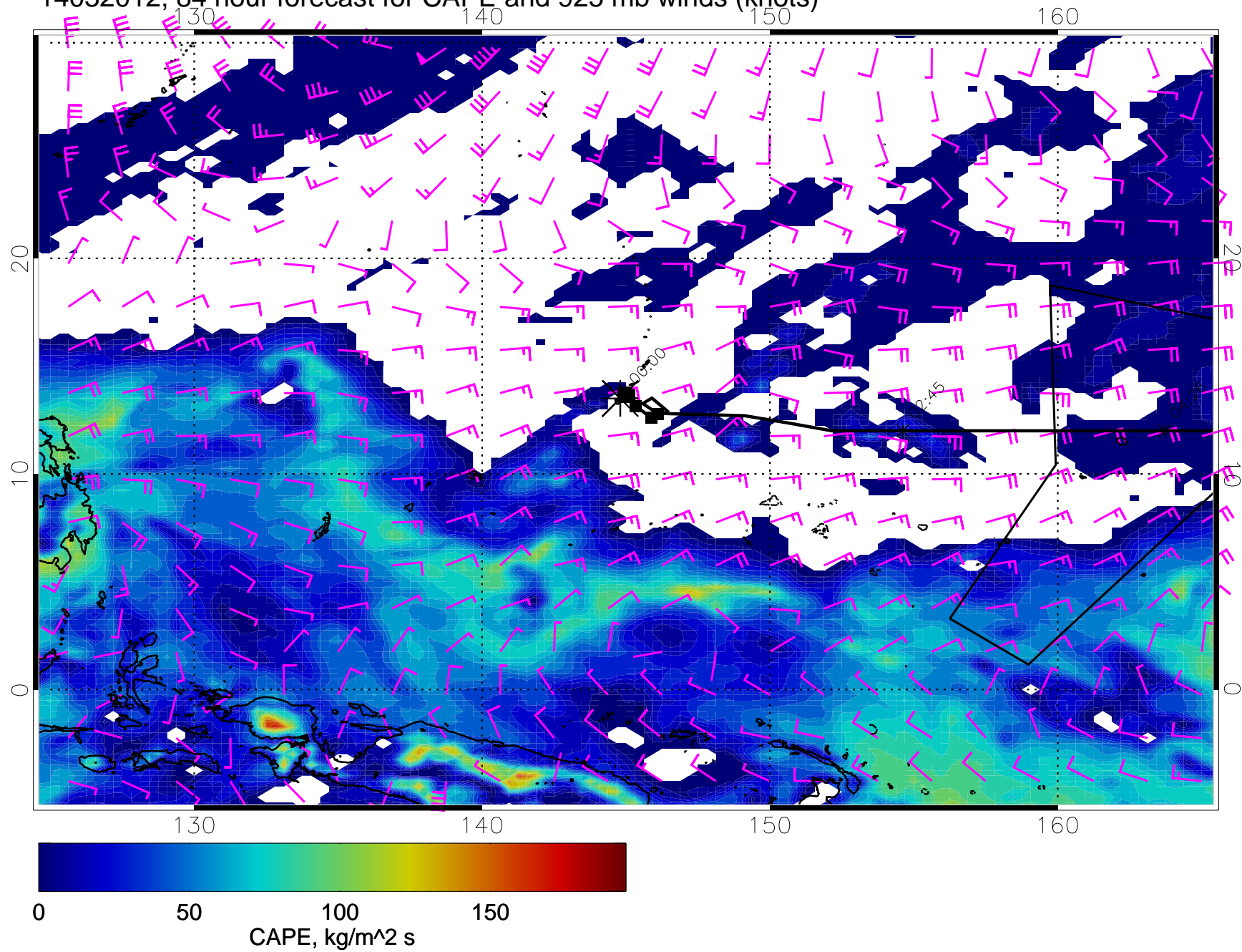
14032012, 84 hour forecast for CAPE and 925 mb winds (knots)
