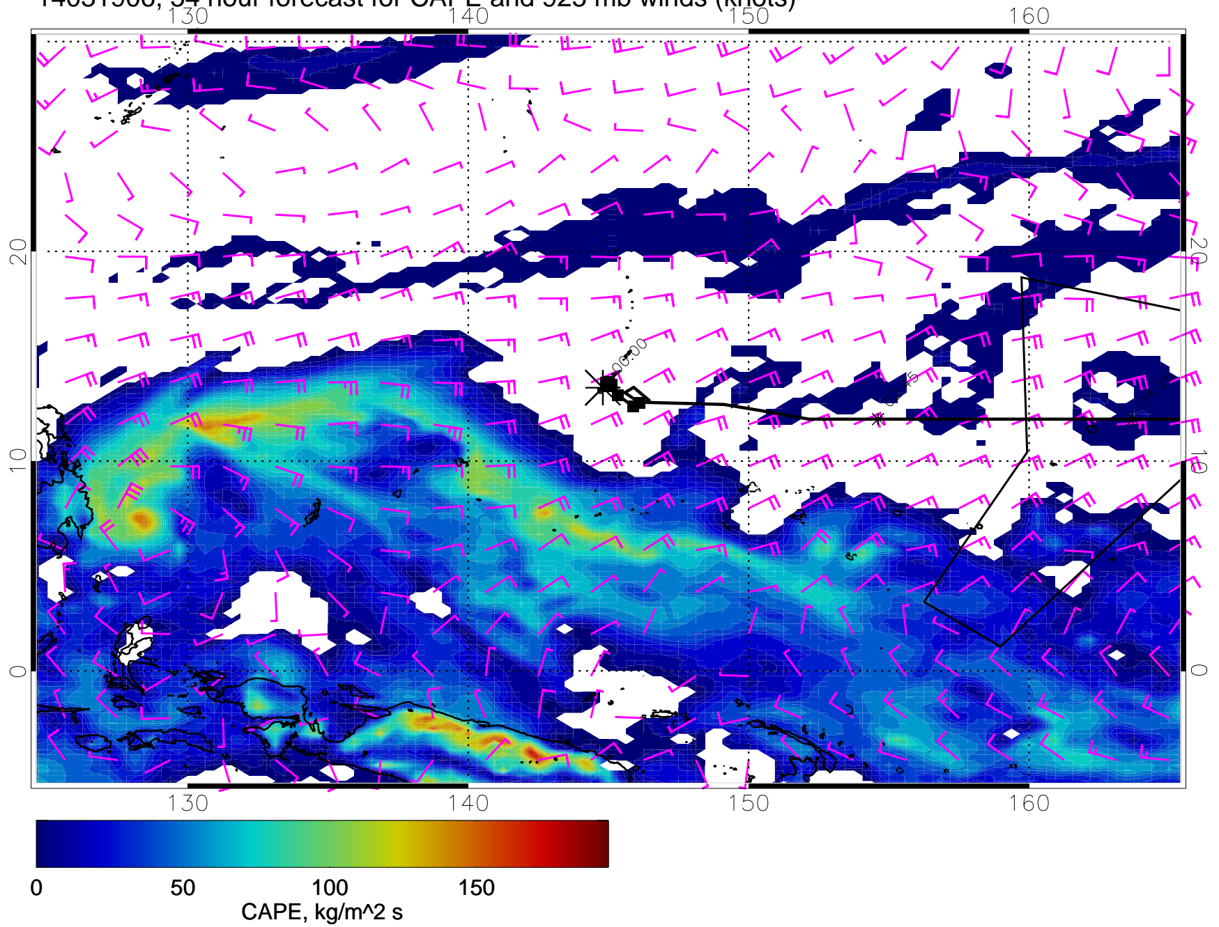
14031906, 54 hour forecast for CAPE and 925 mb winds (knots)
