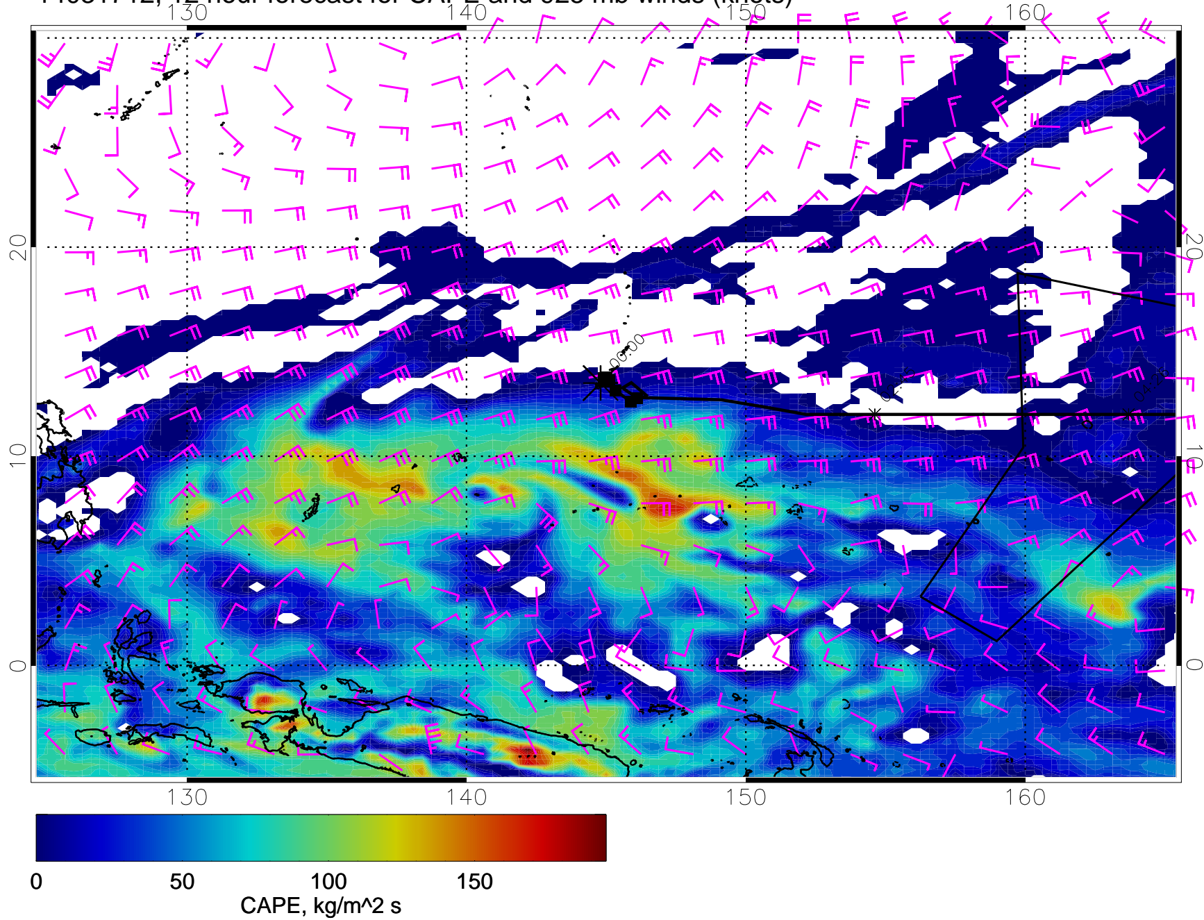
14031712, 12 hour forecast for CAPE and 925 mb winds (knots)
