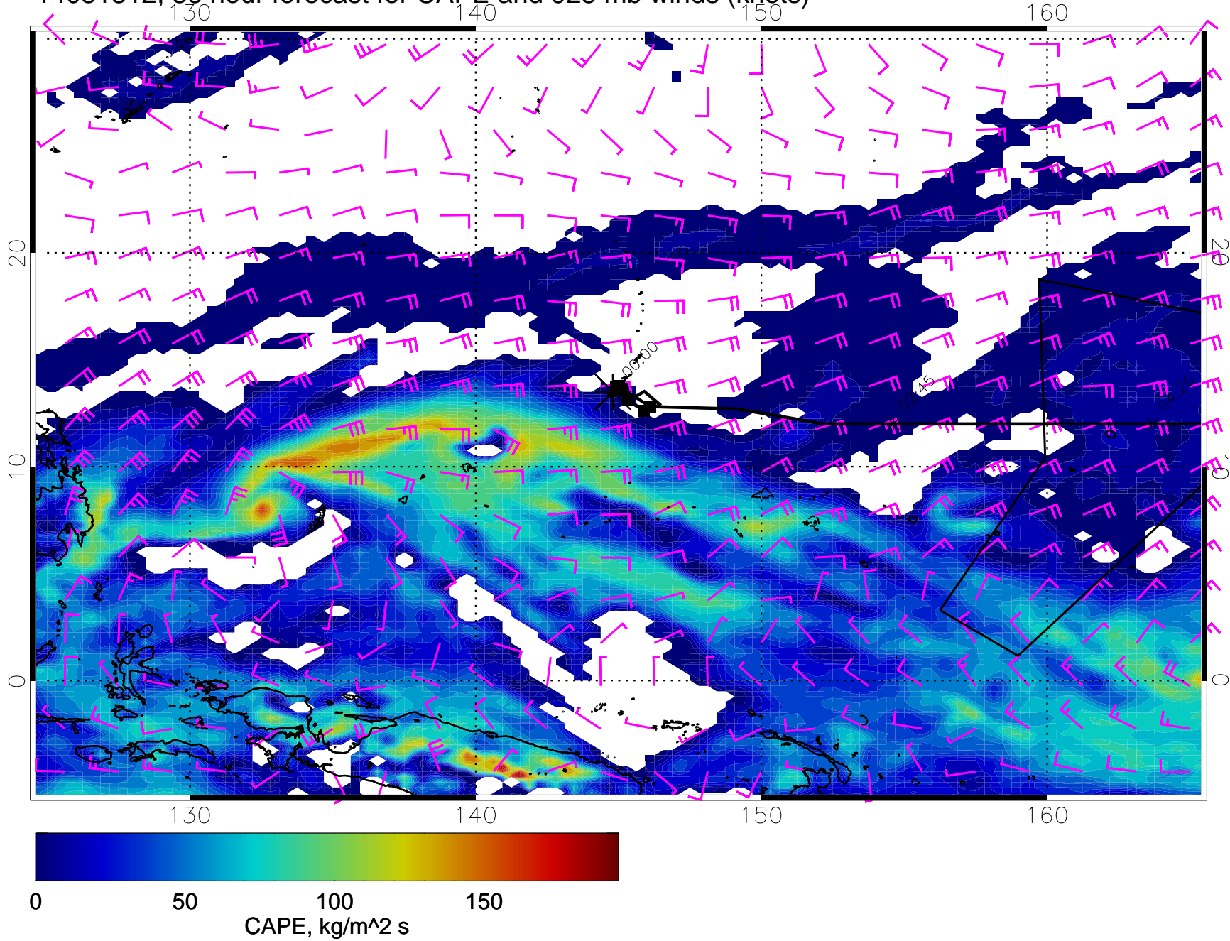
14031812, 36 hour forecast for CAPE and 925 mb winds (knots)
