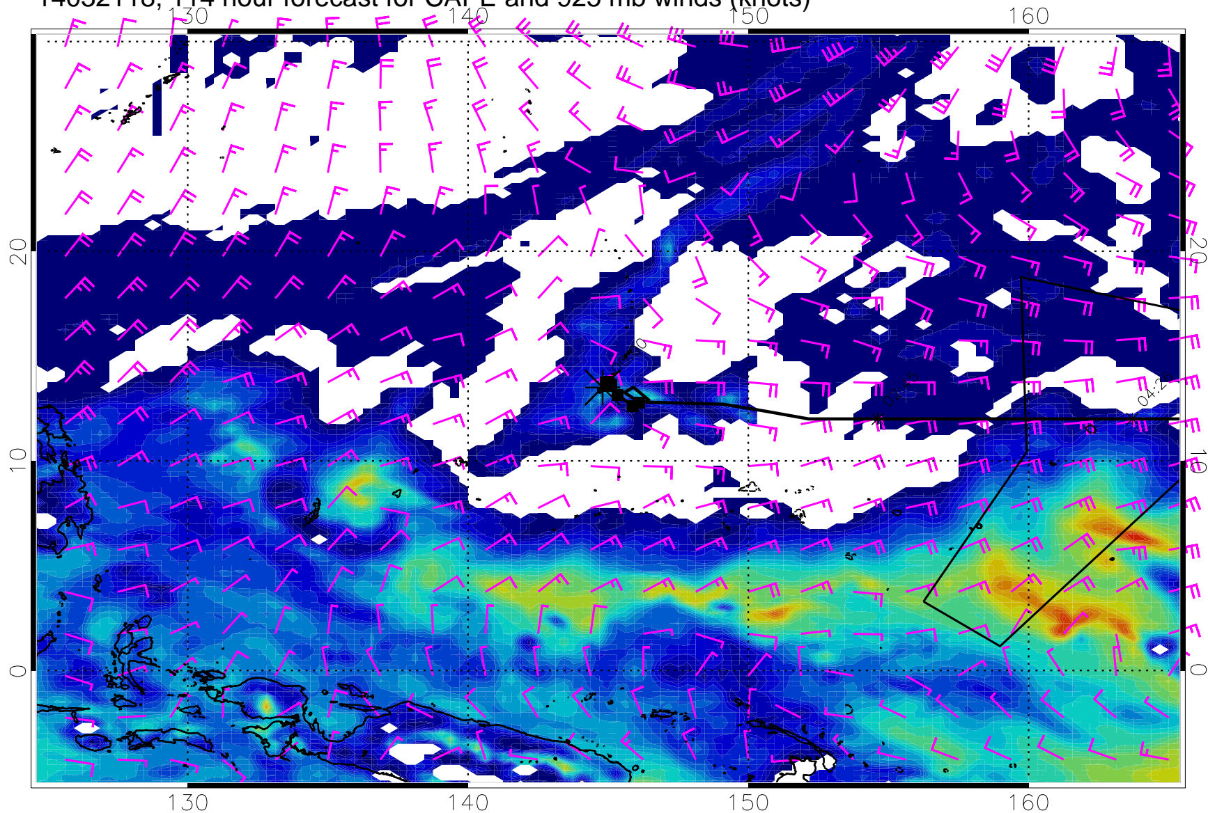
14032118, 114 hour forecast for CAPE and 925 mb winds (knots)
