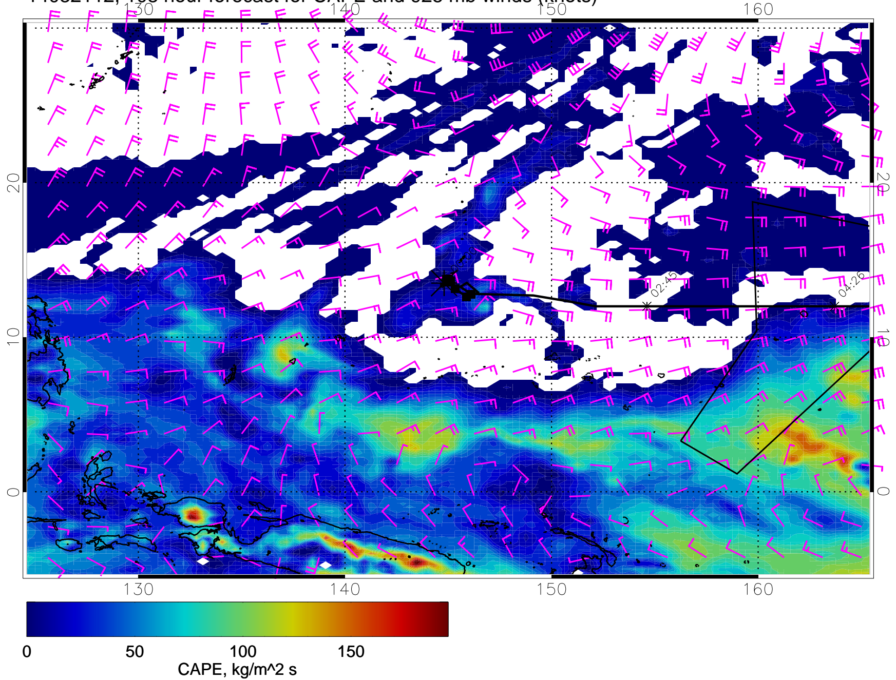
14032112, 108 hour forecast for CAPE and 925 mb winds (knots)
