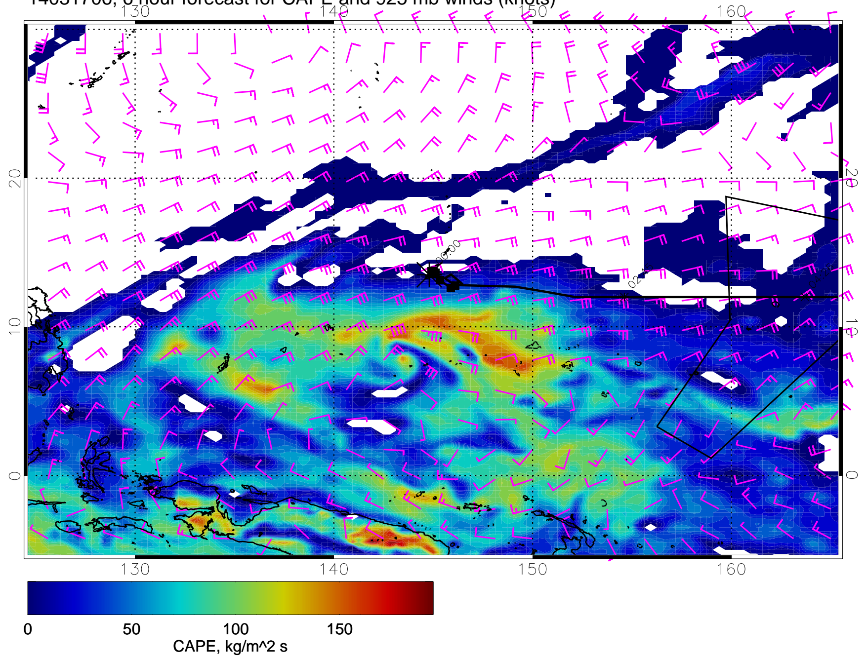
14031706, 6 hour forecast for CAPE and 925 mb winds (knots)
