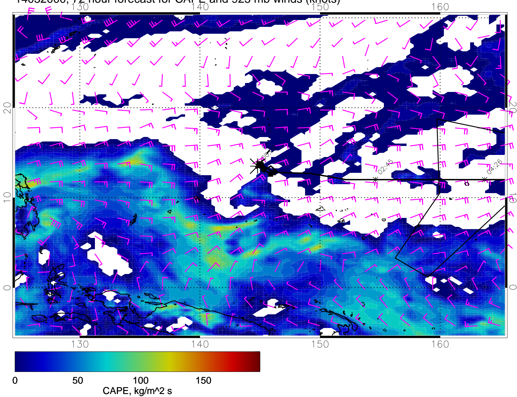
14032000, 72 hour forecast for CAPE and 925 mb winds (knots)
