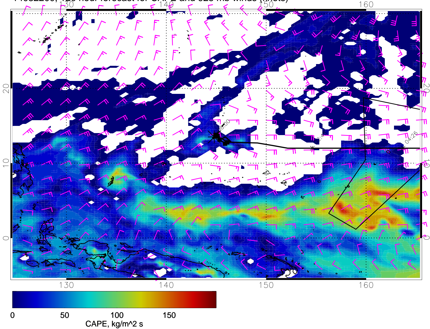
14032200, 120 hour forecast for CAPE and 925 mb winds (knots)
