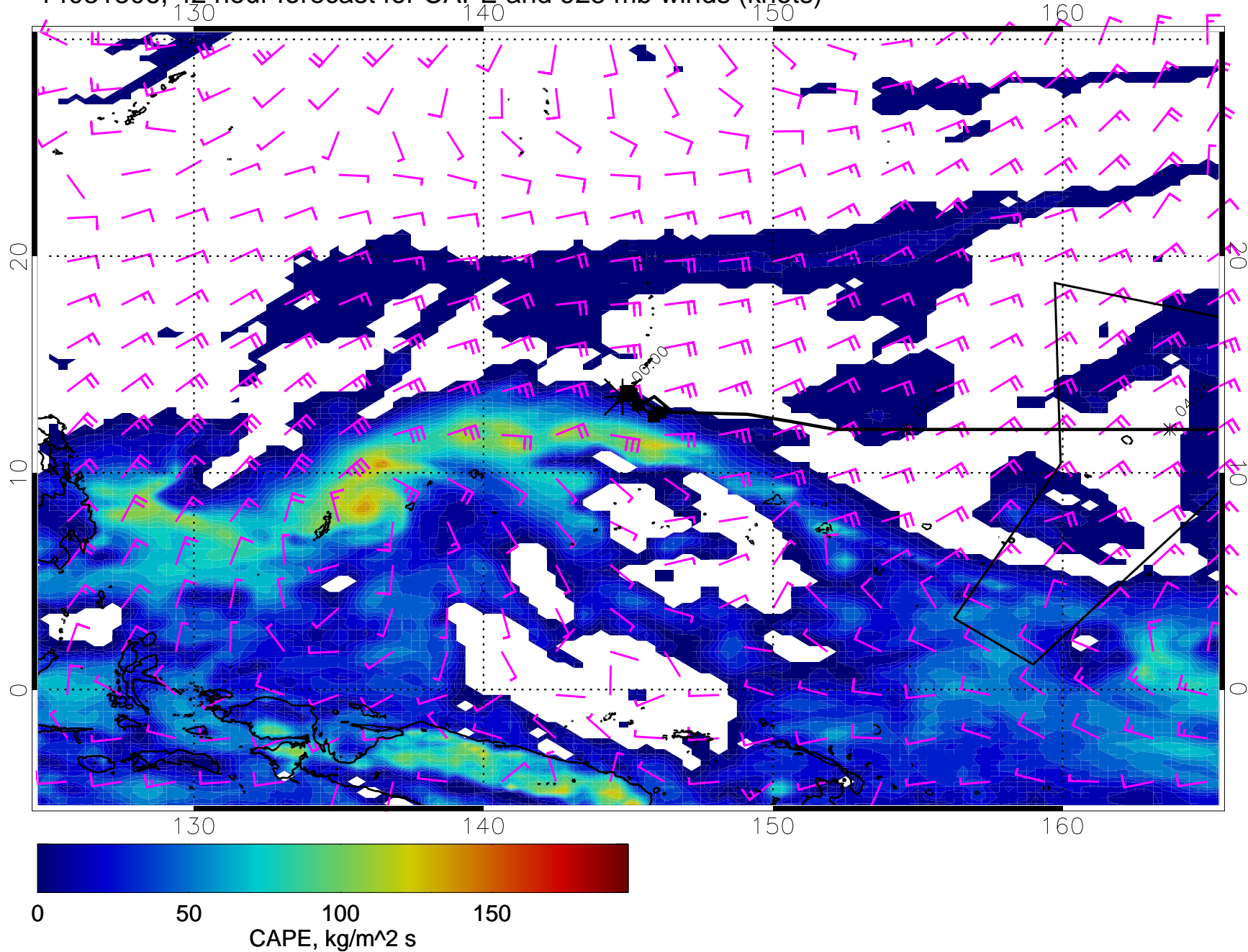
14031806, 42 hour forecast for CAPE and 925 mb winds (knots)
