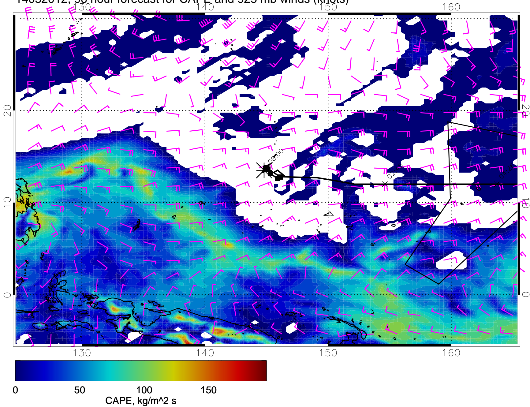
14032012, 96 hour forecast for CAPE and 925 mb winds (knots)
