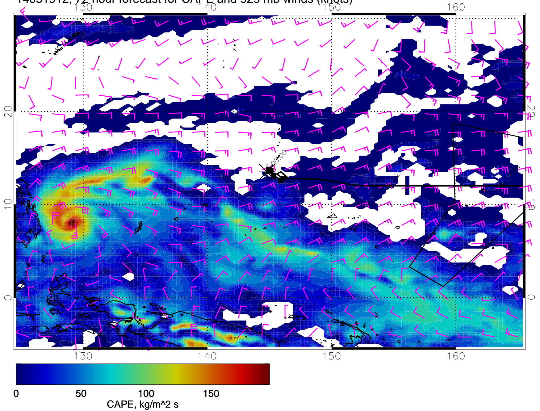
14031912, 72 hour forecast for CAPE and 925 mb winds (knots)
