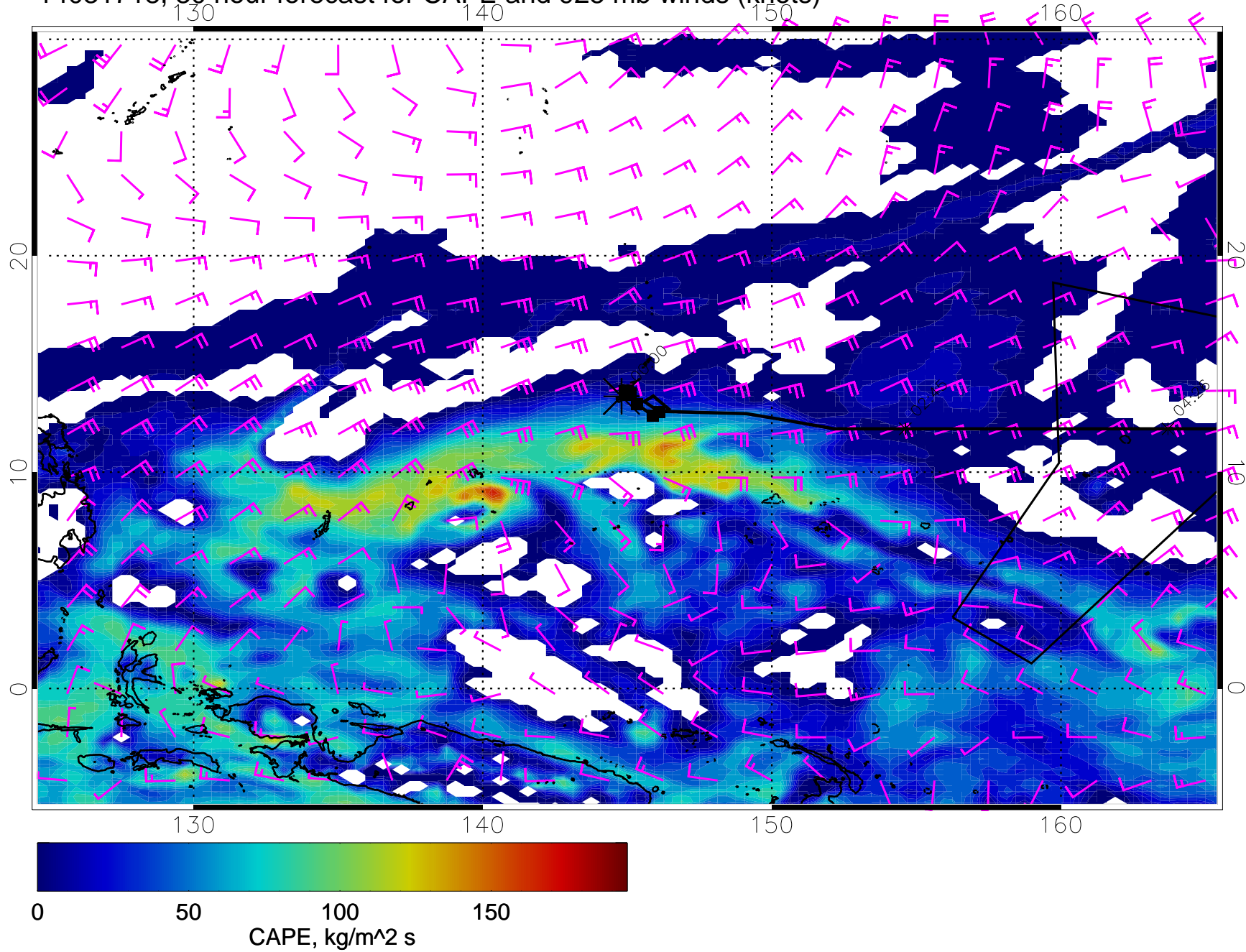
14031718, 30 hour forecast for CAPE and 925 mb winds (knots)
