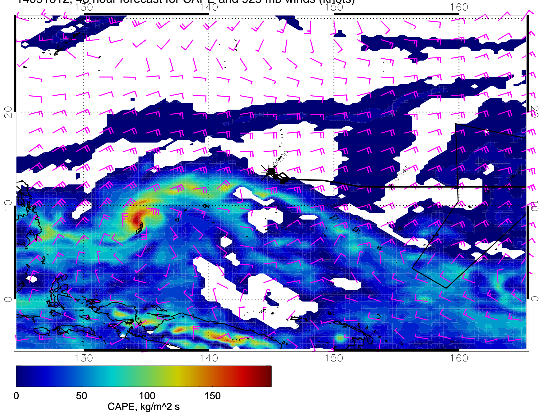
14031812, 48 hour forecast for CAPE and 925 mb winds (knots)
