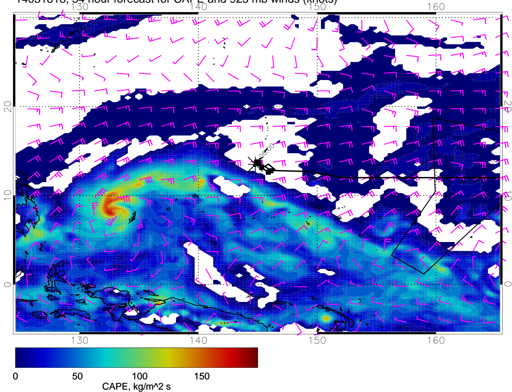
14031818, 54 hour forecast for CAPE and 925 mb winds (knots)
