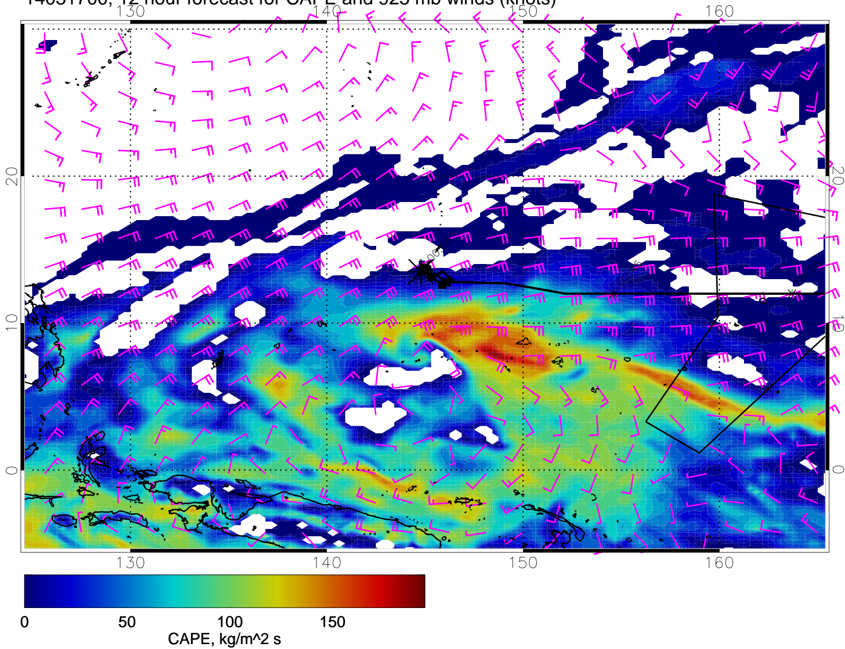
14031700, 12 hour forecast for CAPE and 925 mb winds (knots)
