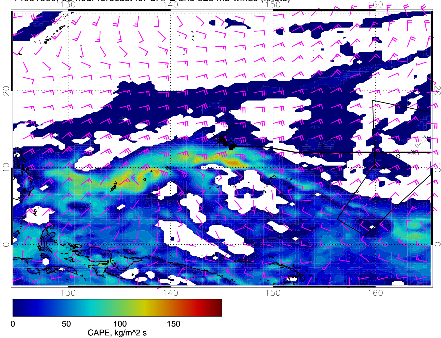
14031800, 36 hour forecast for CAPE and 925 mb winds (knots)
