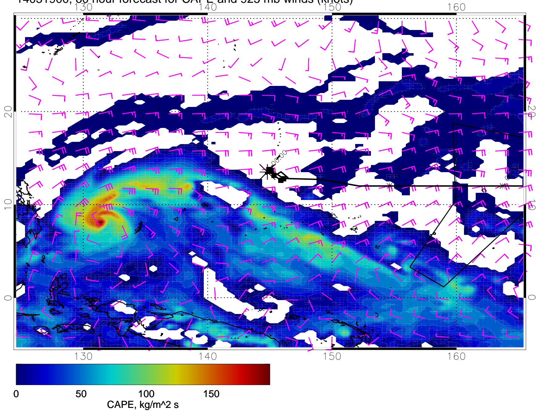
14031900, 60 hour forecast for CAPE and 925 mb winds (knots)
