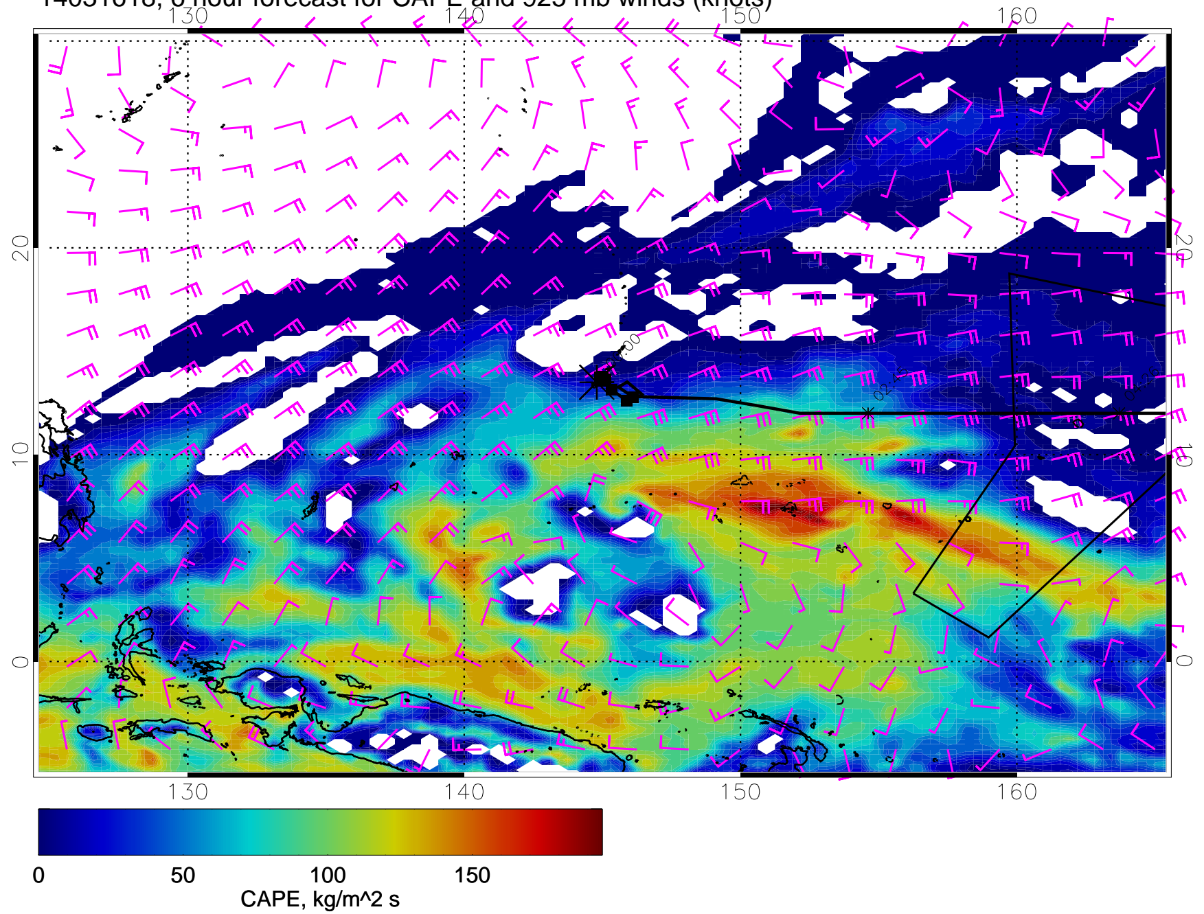
14031618, 6 hour forecast for CAPE and 925 mb winds (knots)
