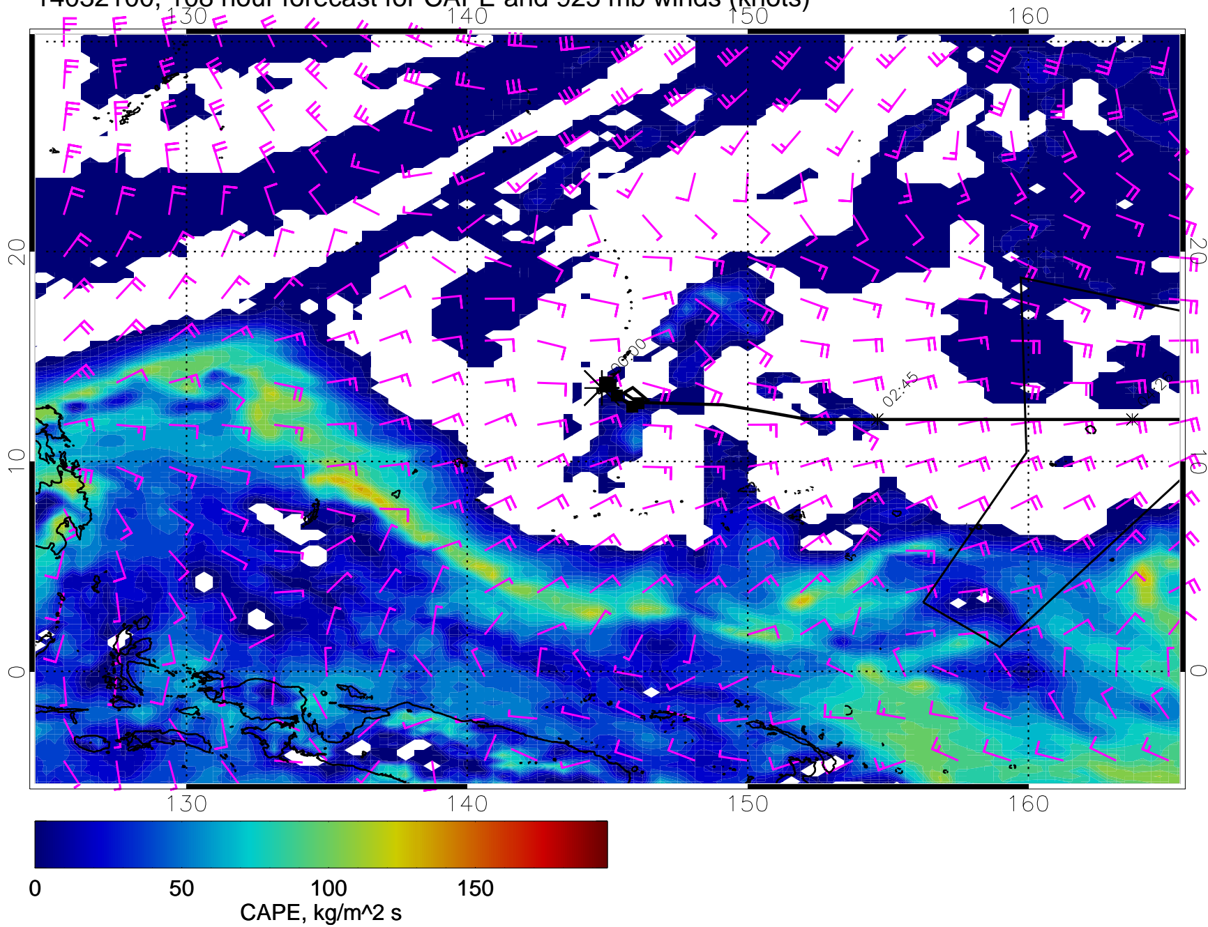
14032100, 108 hour forecast for CAPE and 925 mb winds (knots)
