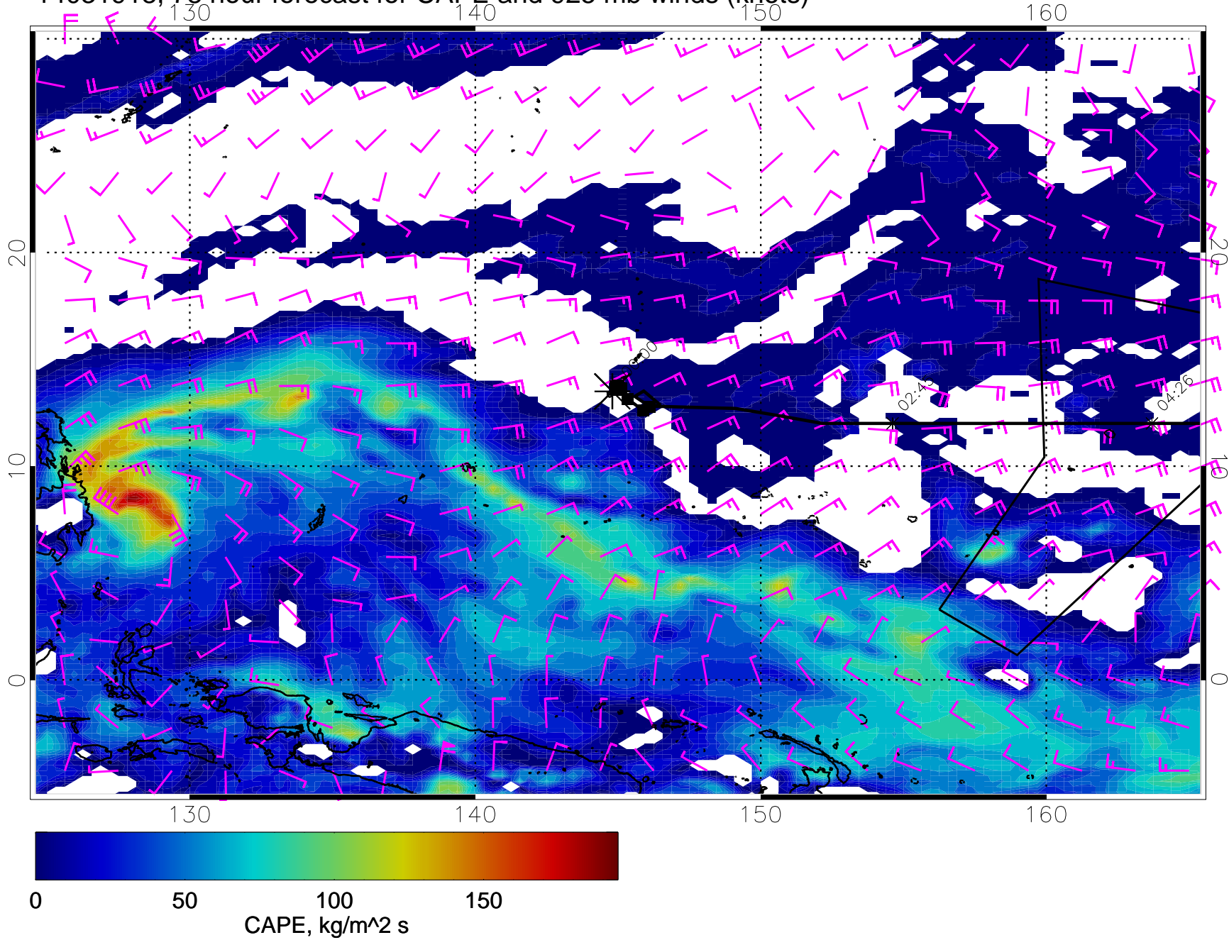
14031918, 78 hour forecast for CAPE and 925 mb winds (knots)
