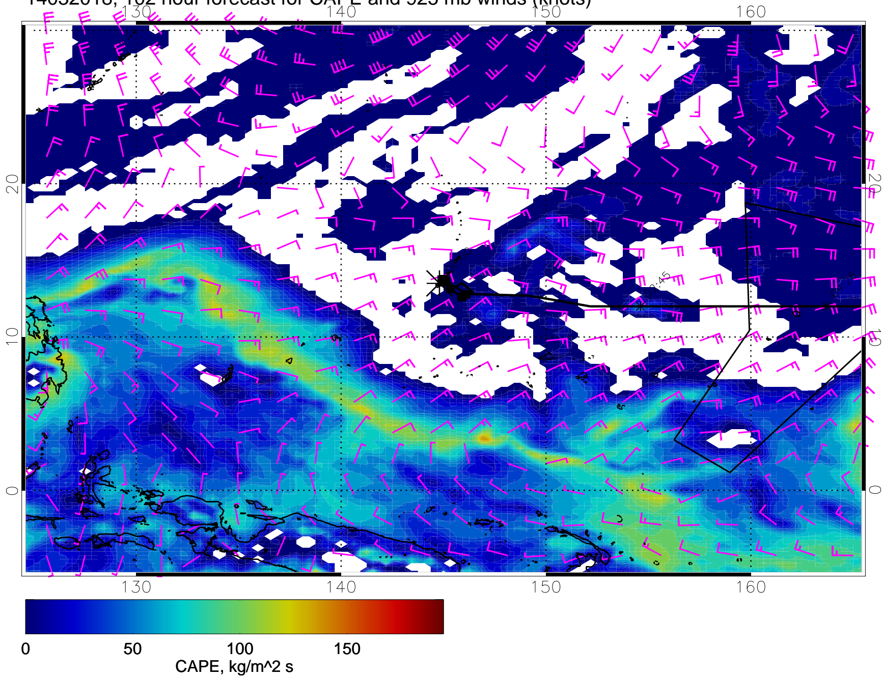
14032018, 102 hour forecast for CAPE and 925 mb winds (knots)
