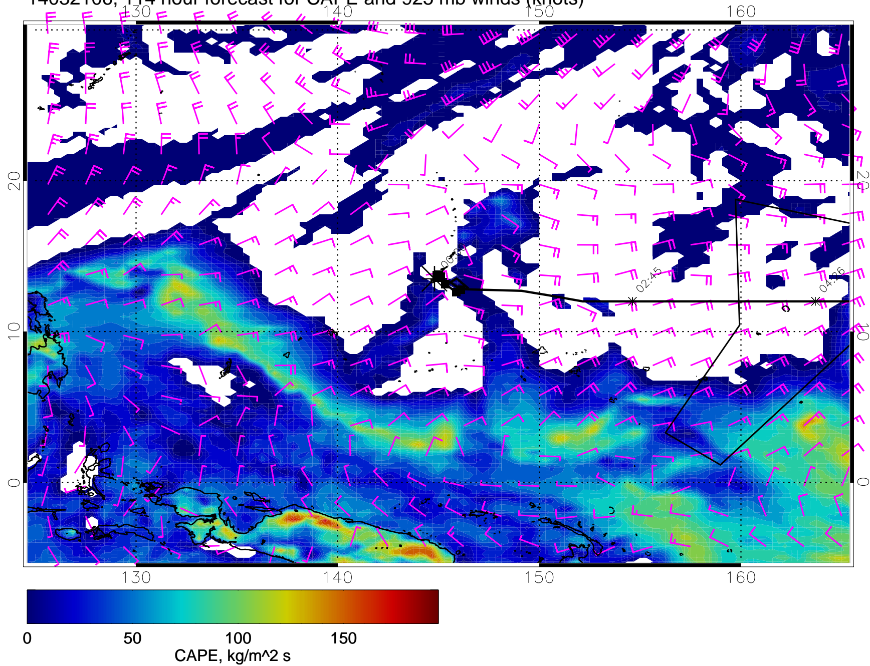
14032106, 114 hour forecast for CAPE and 925 mb winds (knots)
