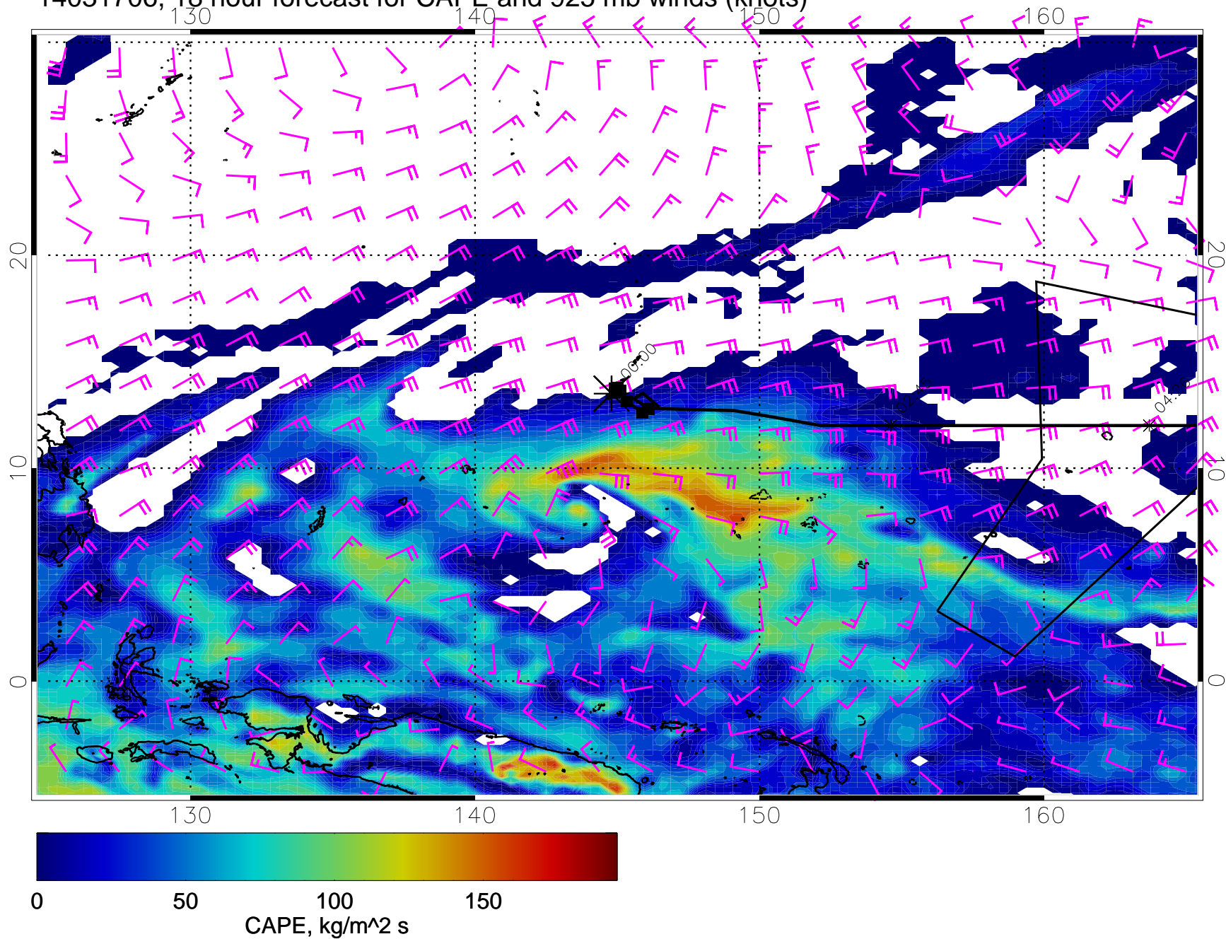
14031706, 18 hour forecast for CAPE and 925 mb winds (knots)
