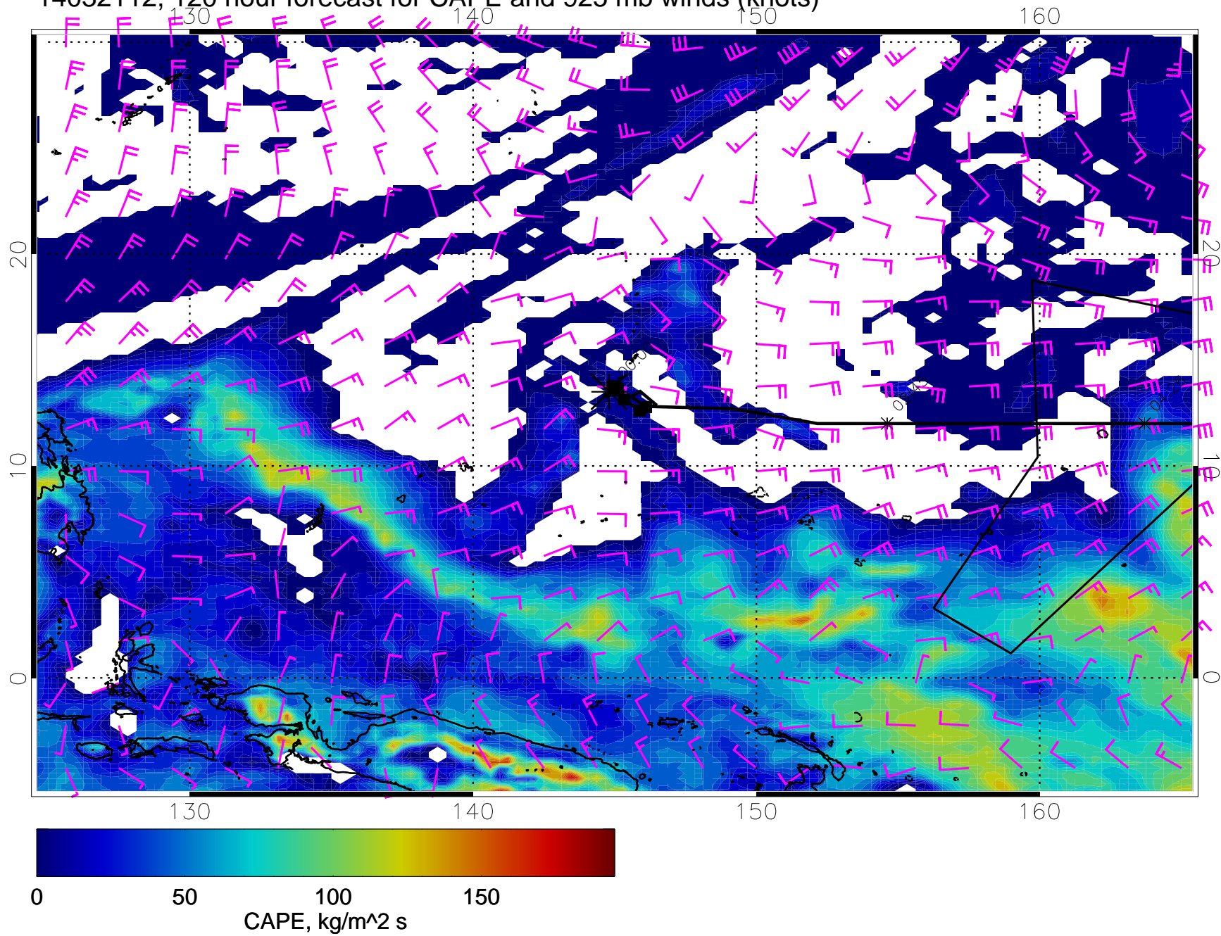
14032112, 120 hour forecast for CAPE and 925 mb winds (knots)
