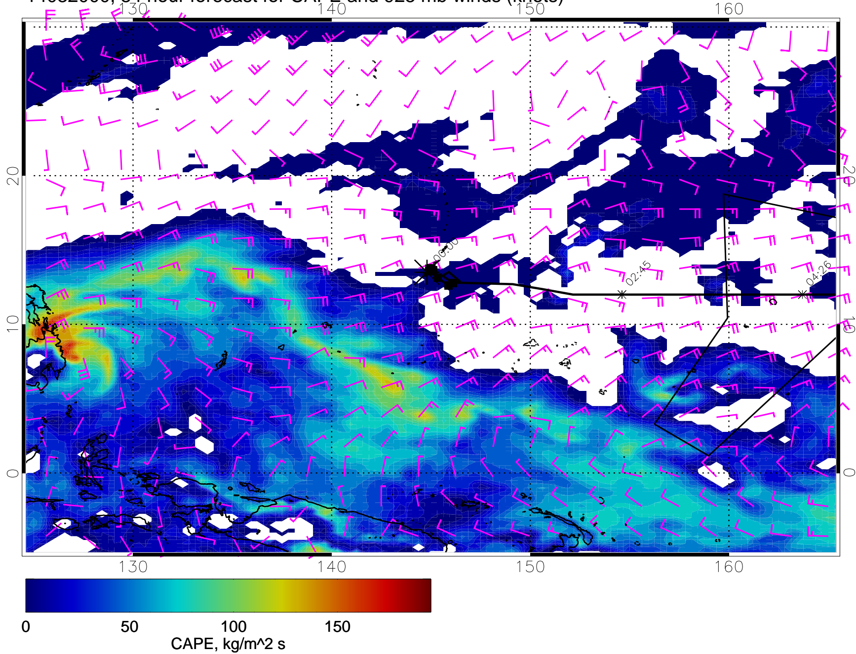
14032000, 84 hour forecast for CAPE and 925 mb winds (knots)
