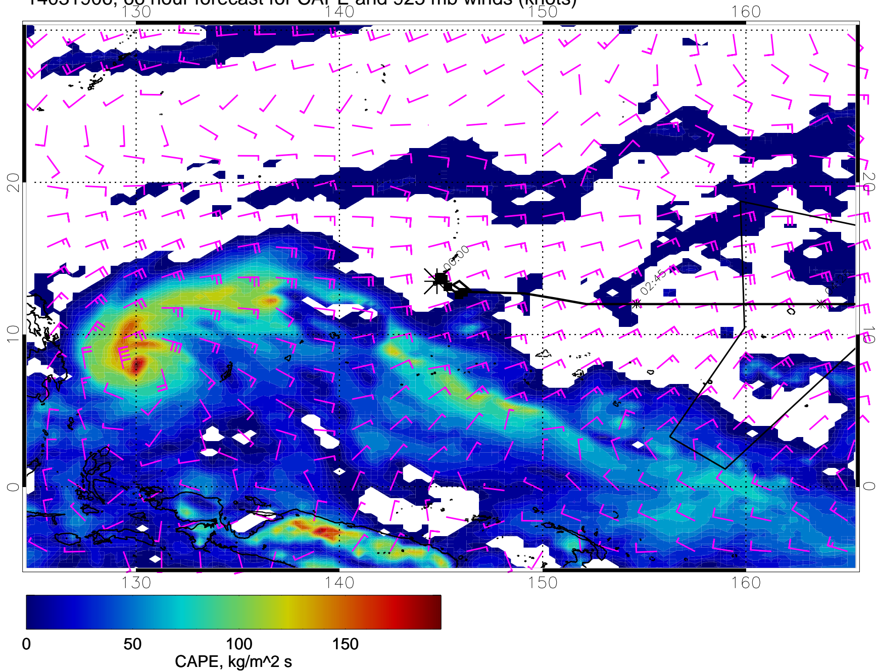
14031906, 66 hour forecast for CAPE and 925 mb winds (knots)
