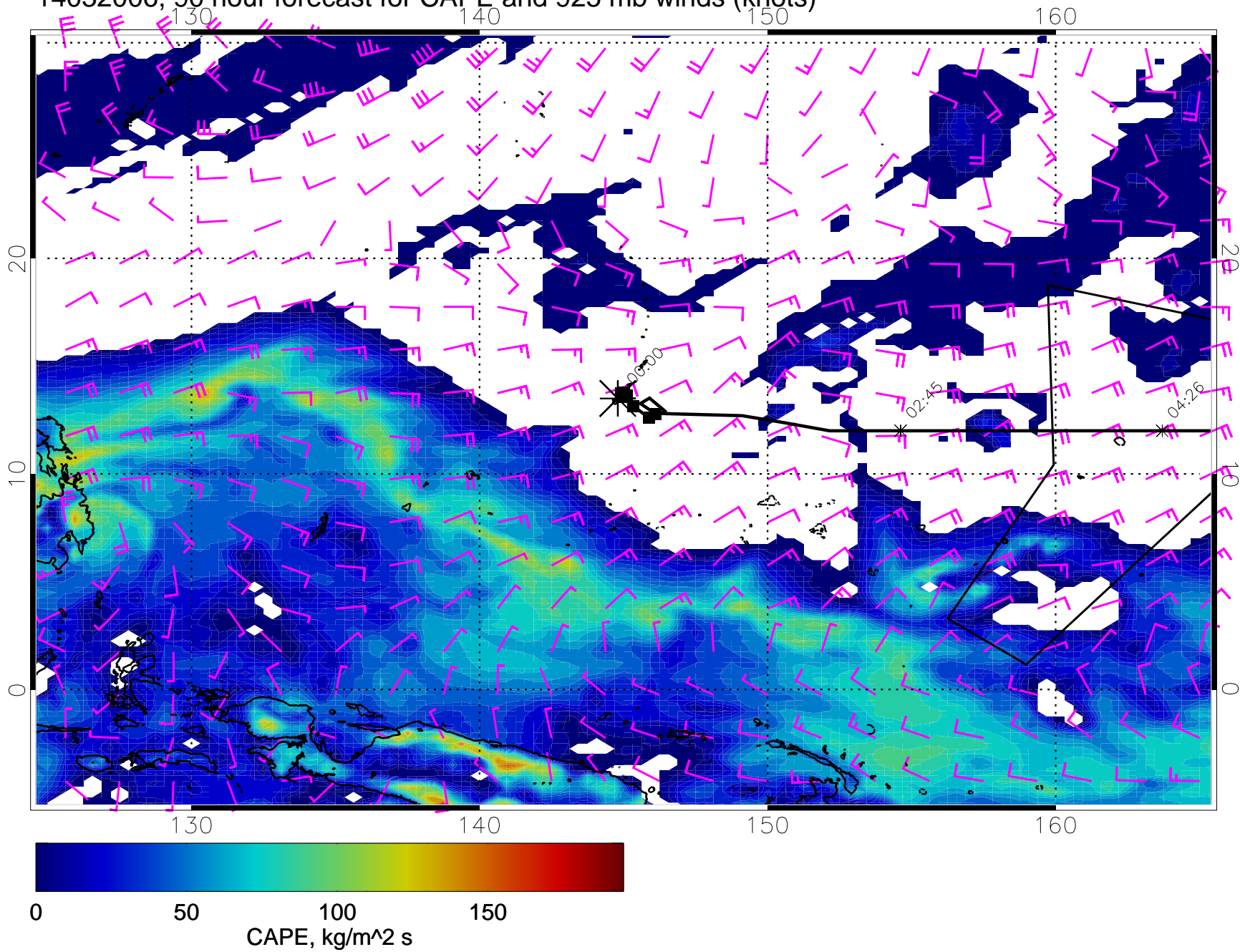
14032006, 90 hour forecast for CAPE and 925 mb winds (knots)
