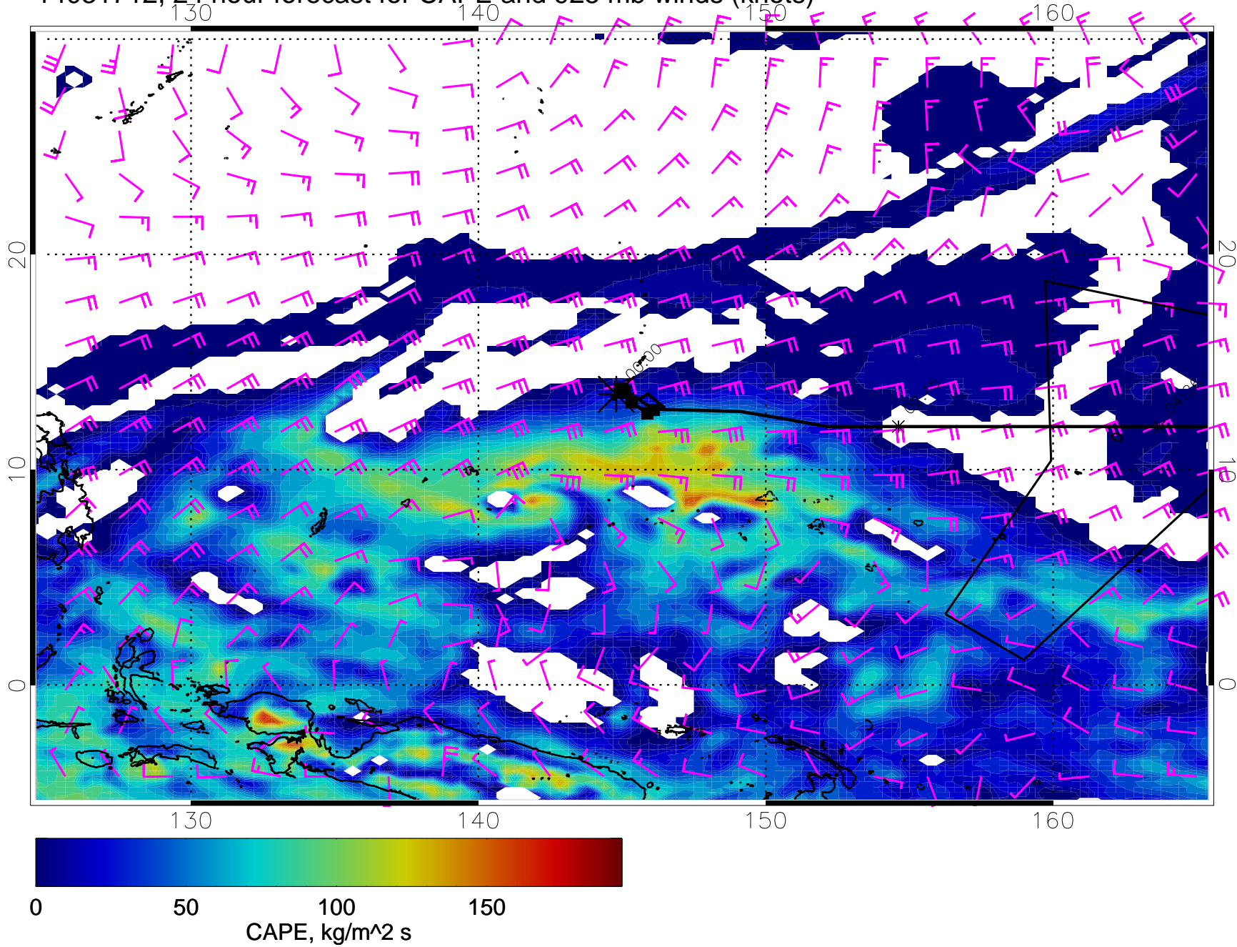
14031712, 24 hour forecast for CAPE and 925 mb winds (knots)
