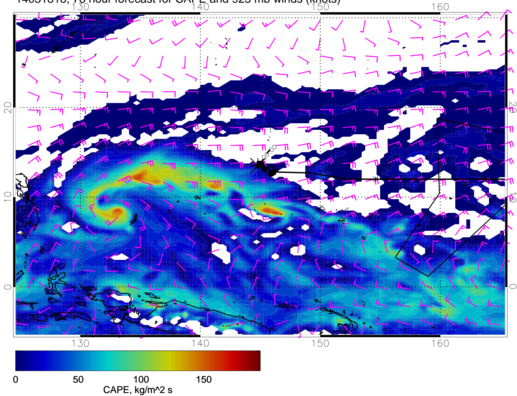
14031818, 78 hour forecast for CAPE and 925 mb winds (knots)
