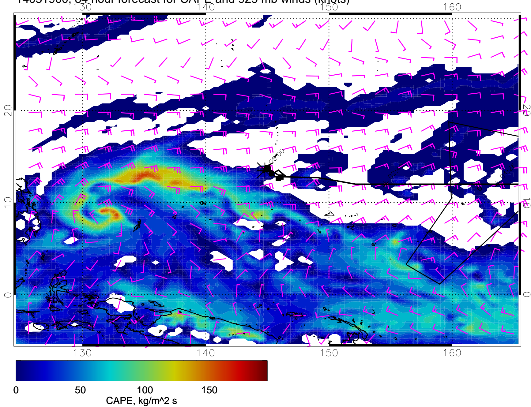
14031900, 84 hour forecast for CAPE and 925 mb winds (knots)
