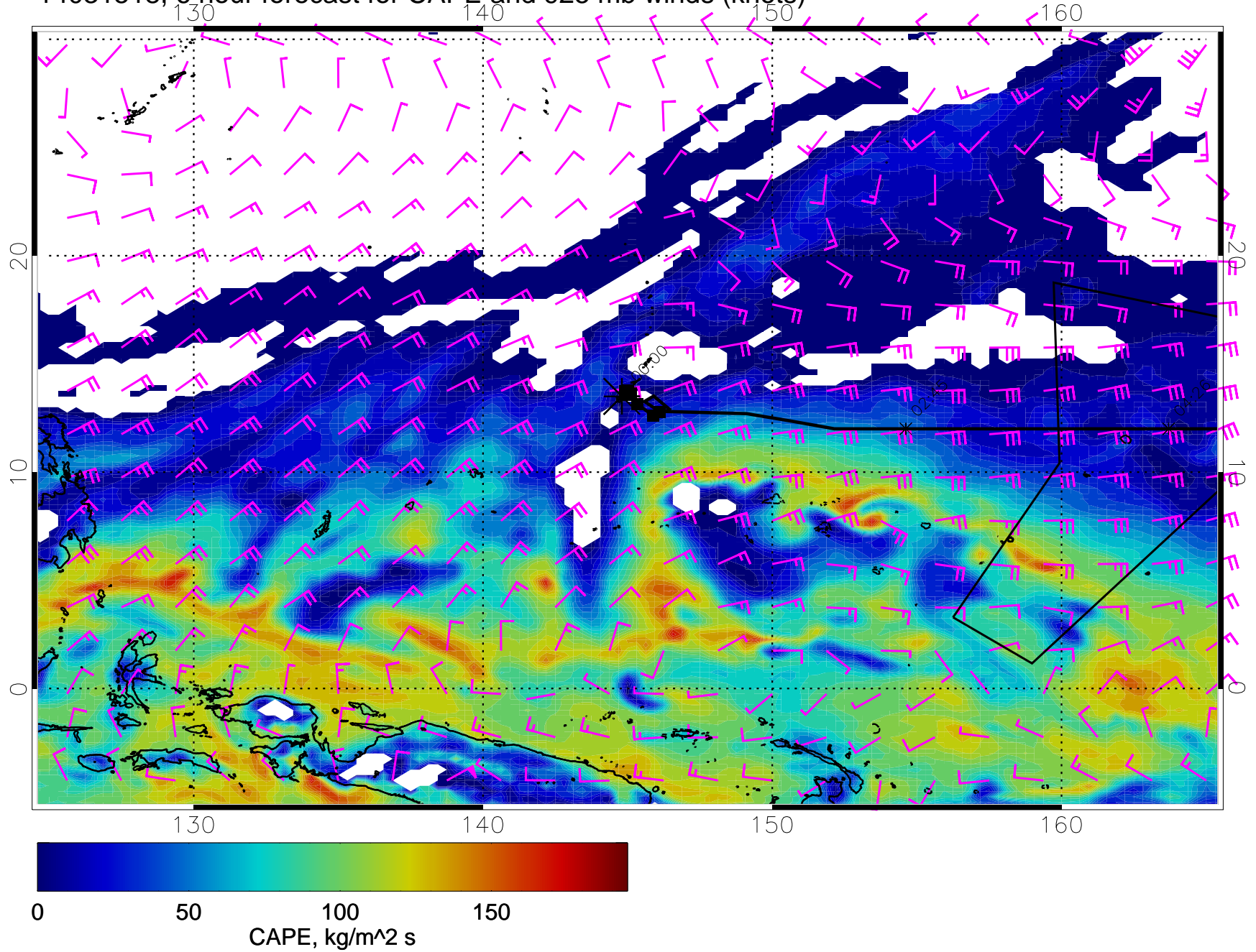
14031518, 6 hour forecast for CAPE and 925 mb winds (knots)
