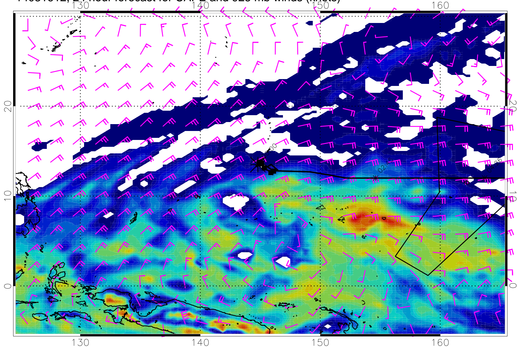
14031612, 24 hour forecast for CAPE and 925 mb winds (knots)
