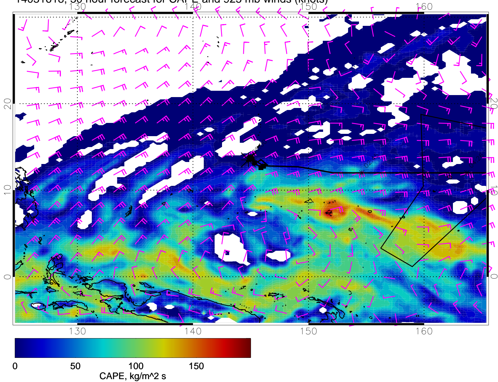
14031618, 30 hour forecast for CAPE and 925 mb winds (knots)
