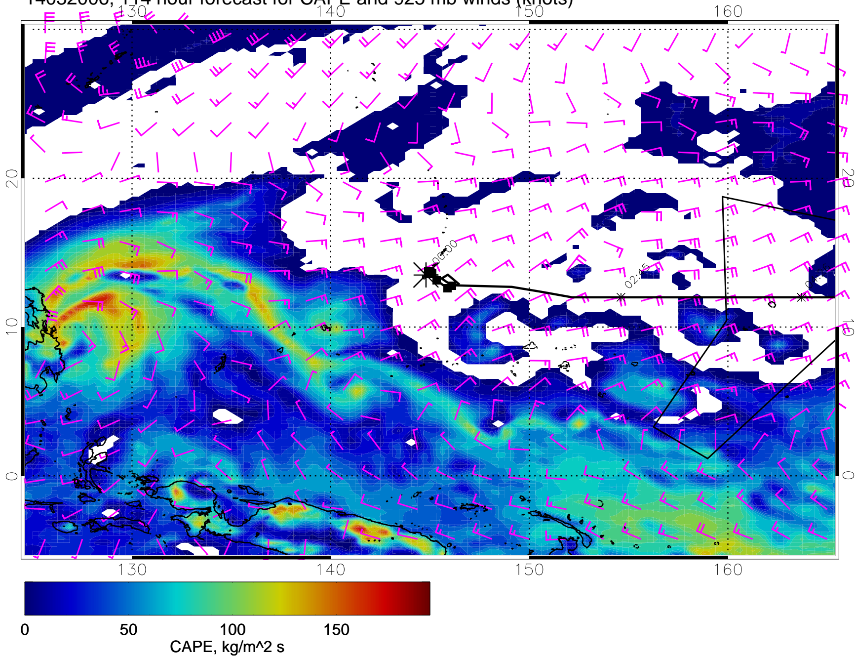
14032006, 114 hour forecast for CAPE and 925 mb winds (knots)
