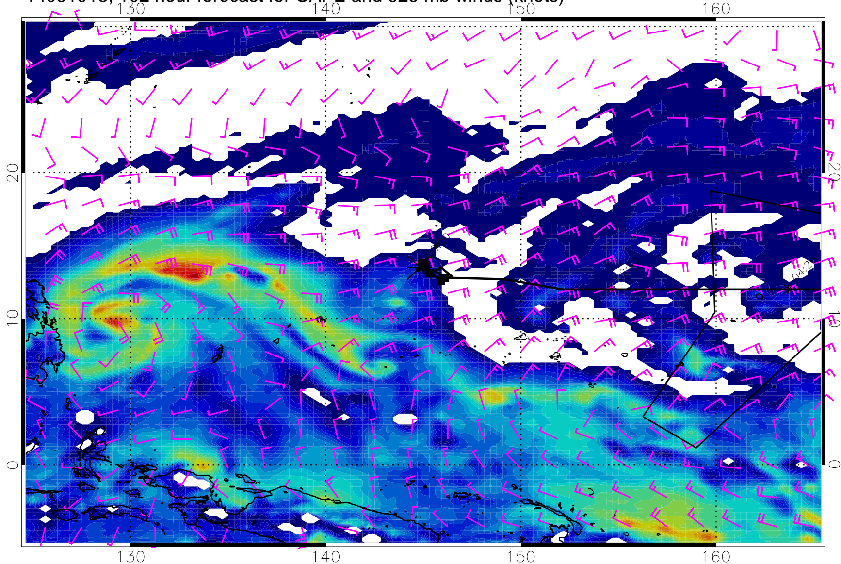
14031918, 102 hour forecast for CAPE and 925 mb winds (knots)
