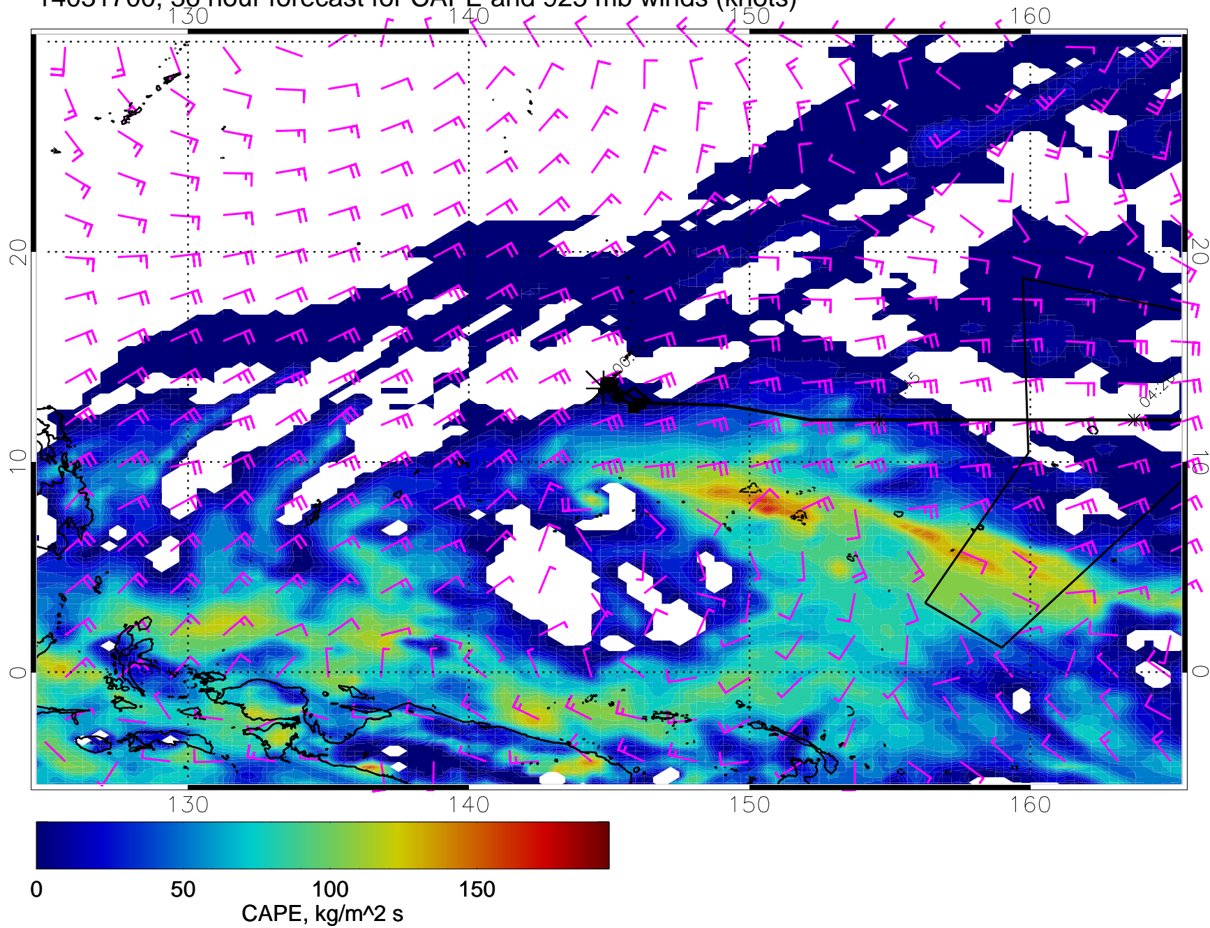
14031700, 36 hour forecast for CAPE and 925 mb winds (knots)
