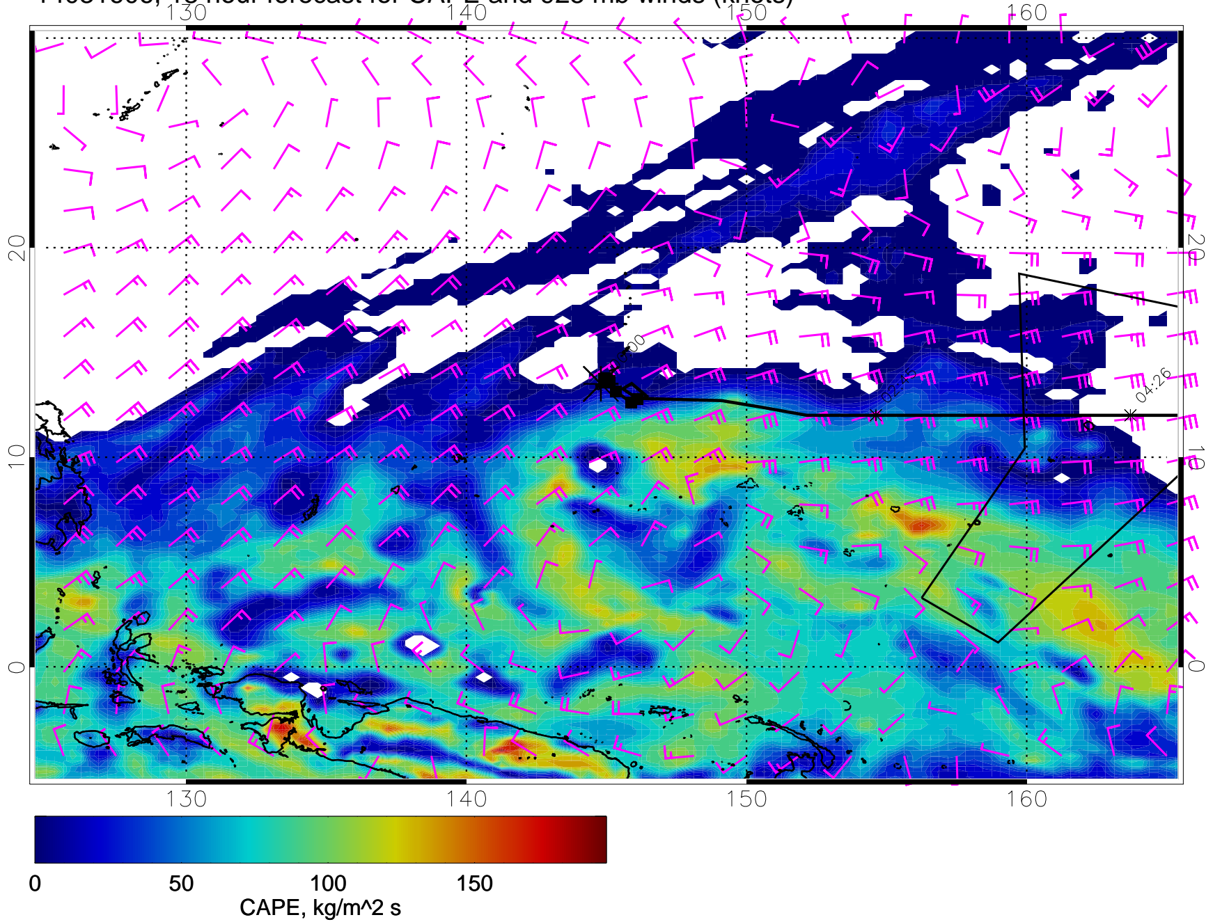
14031606, 18 hour forecast for CAPE and 925 mb winds (knots)
