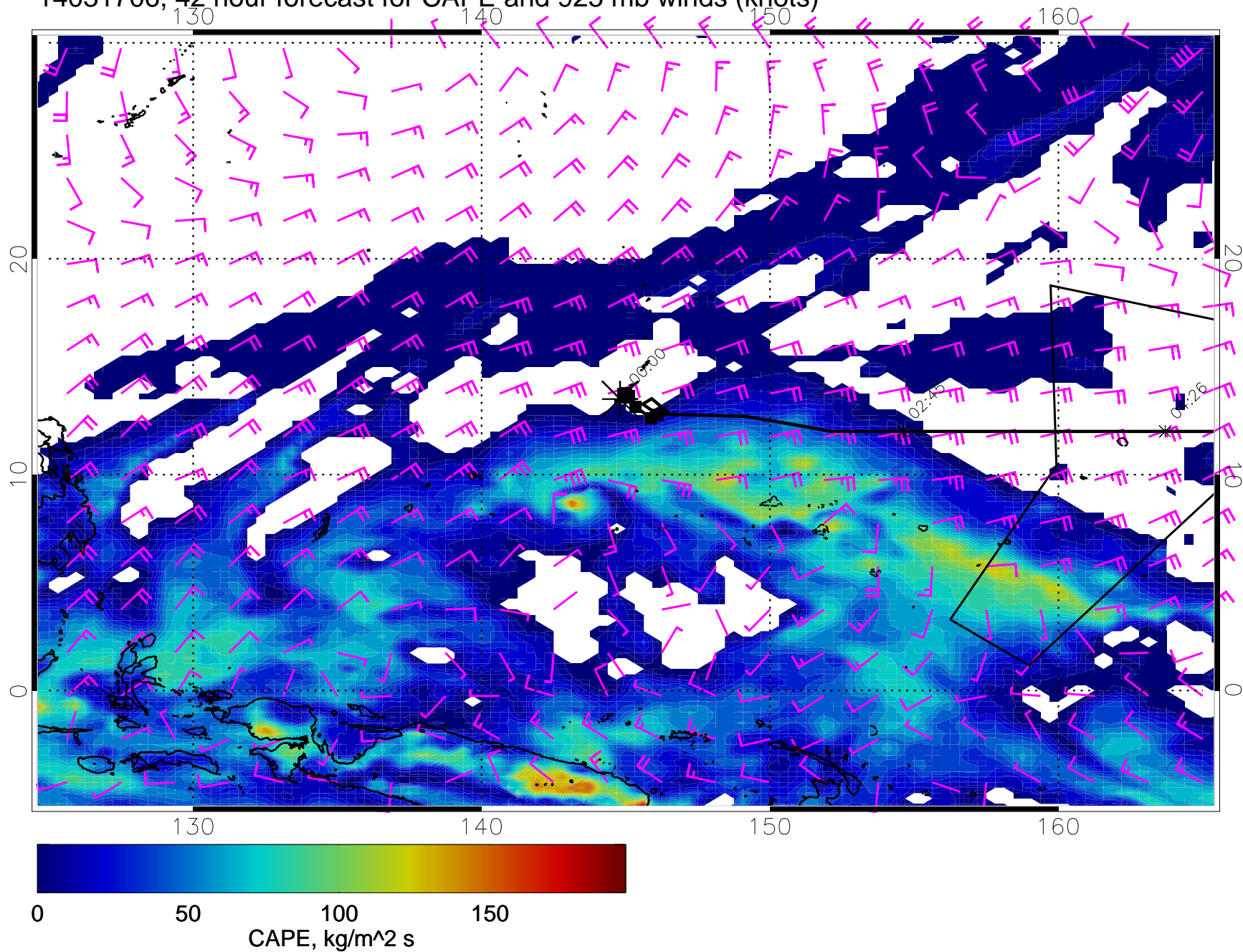
14031706, 42 hour forecast for CAPE and 925 mb winds (knots)
