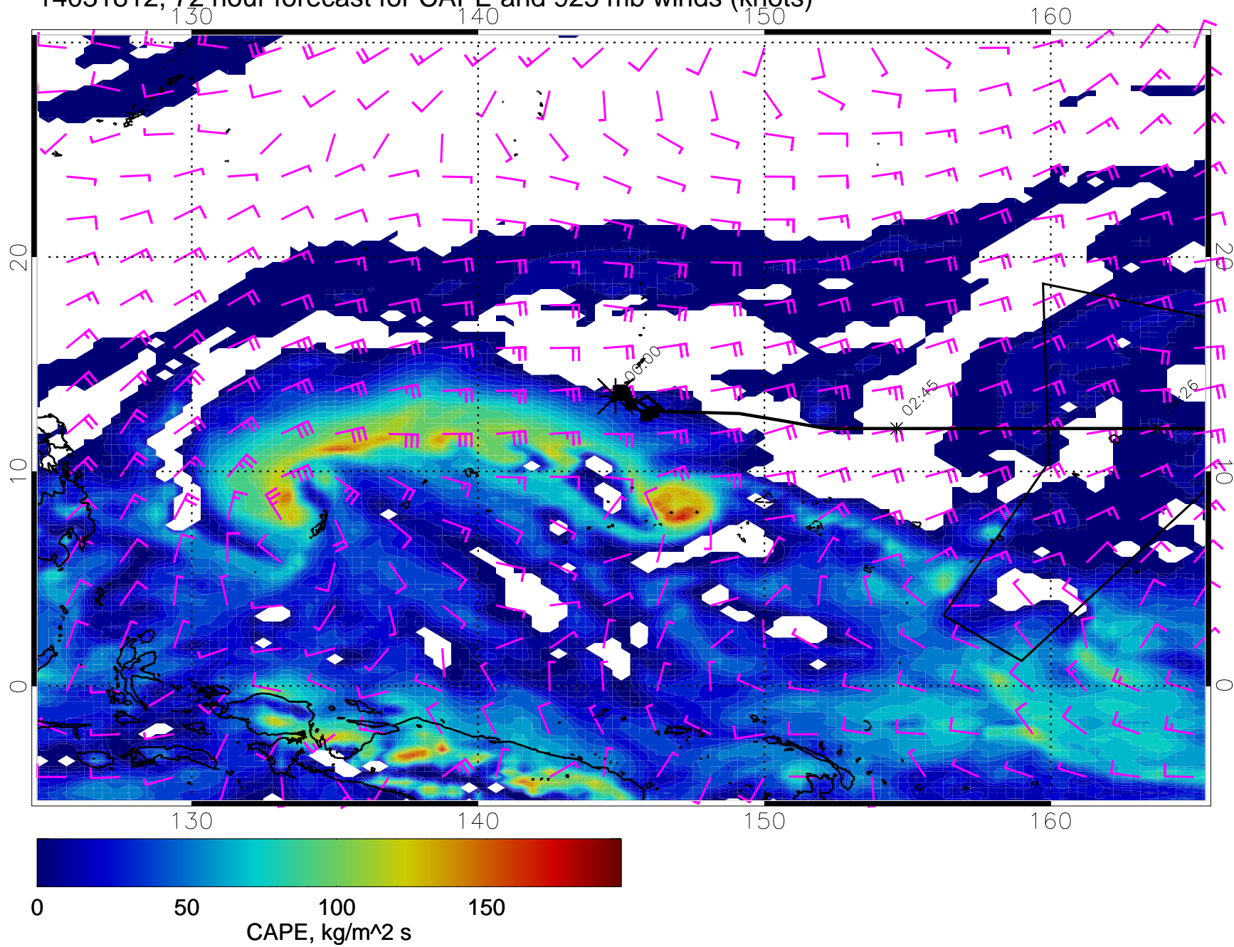
14031812, 72 hour forecast for CAPE and 925 mb winds (knots)
