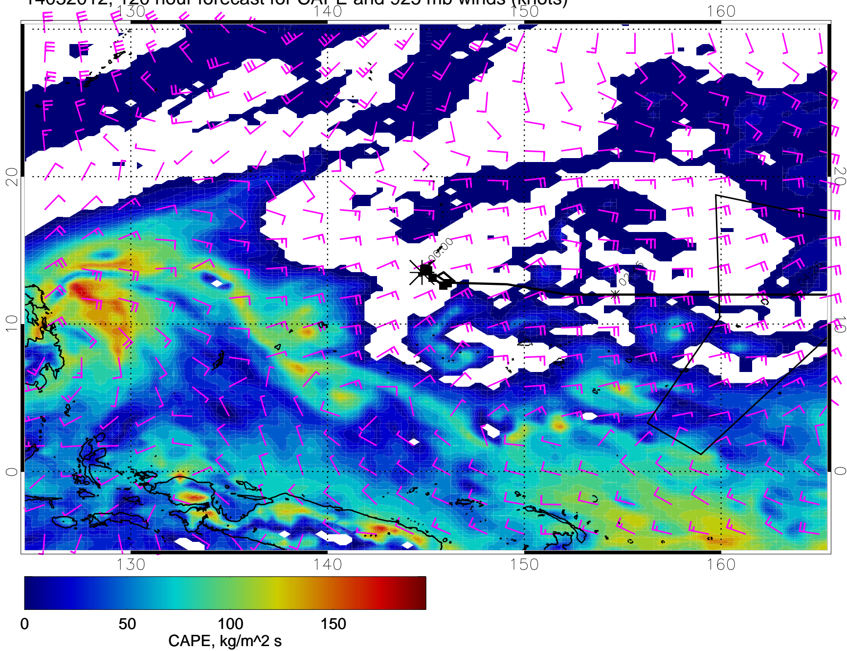
14032012, 120 hour forecast for CAPE and 925 mb winds (knots)
