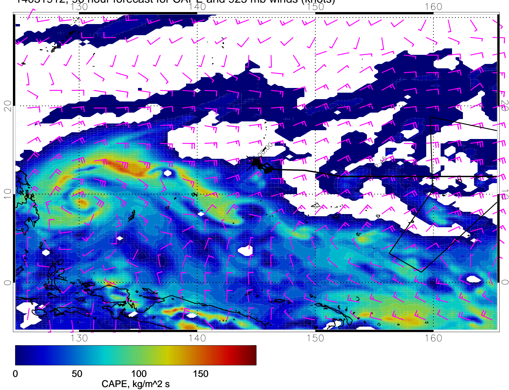
14031912, 96 hour forecast for CAPE and 925 mb winds (knots)
