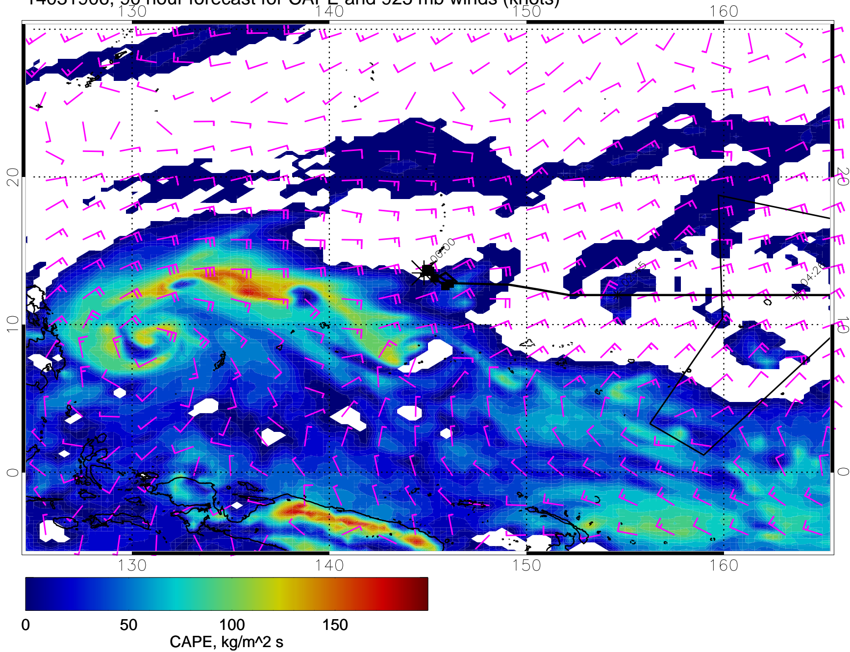
14031906, 90 hour forecast for CAPE and 925 mb winds (knots)
