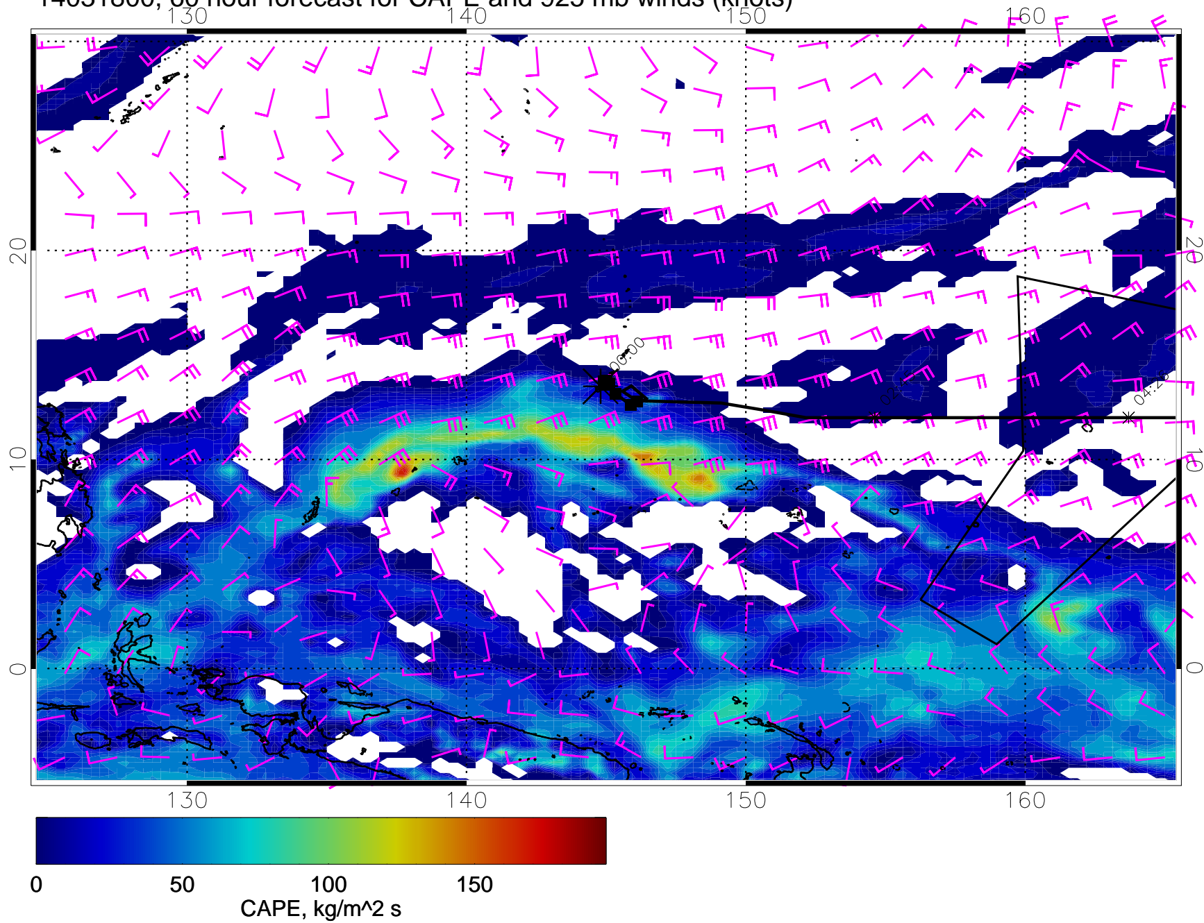
14031800, 60 hour forecast for CAPE and 925 mb winds (knots)
