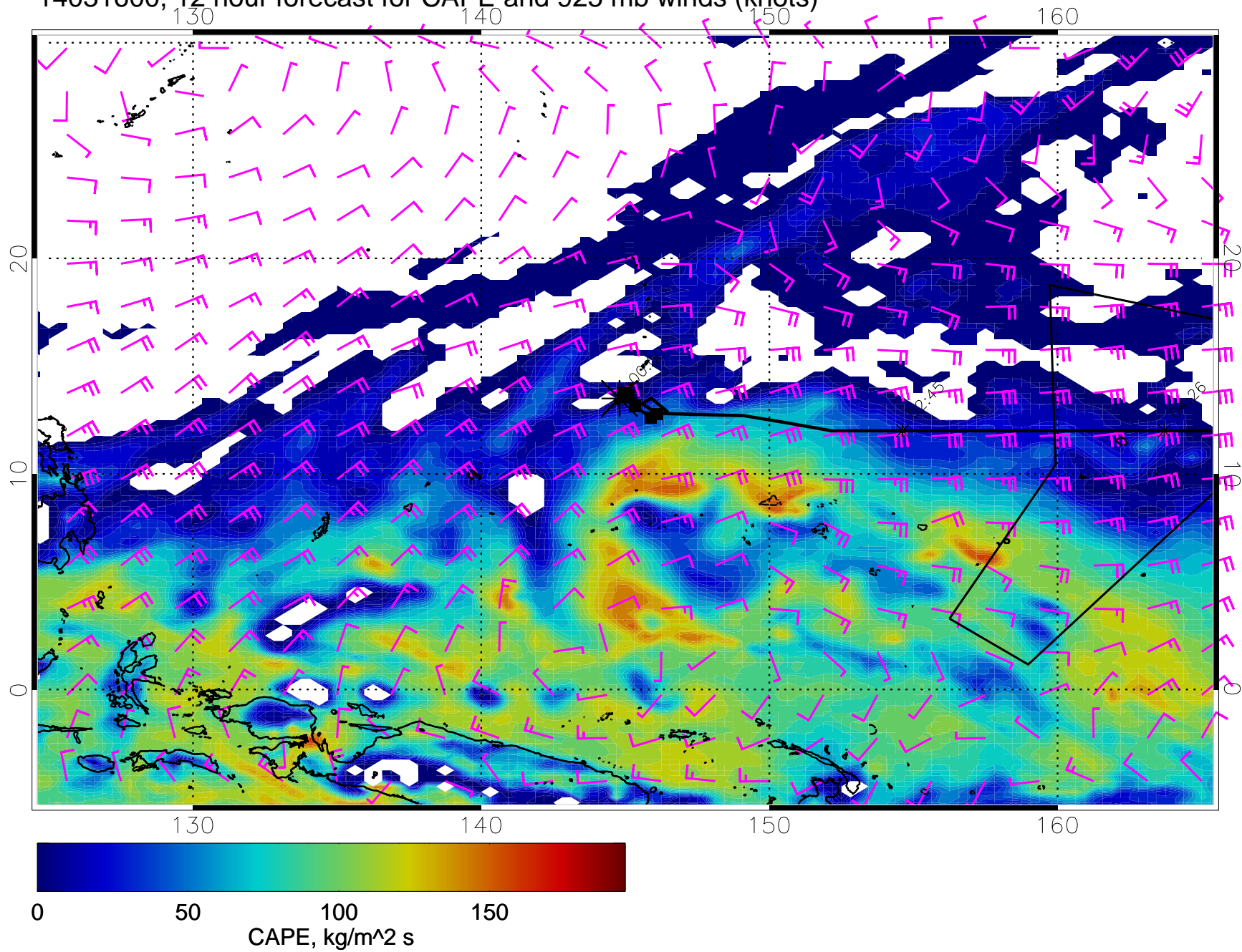
14031600, 12 hour forecast for CAPE and 925 mb winds (knots)
