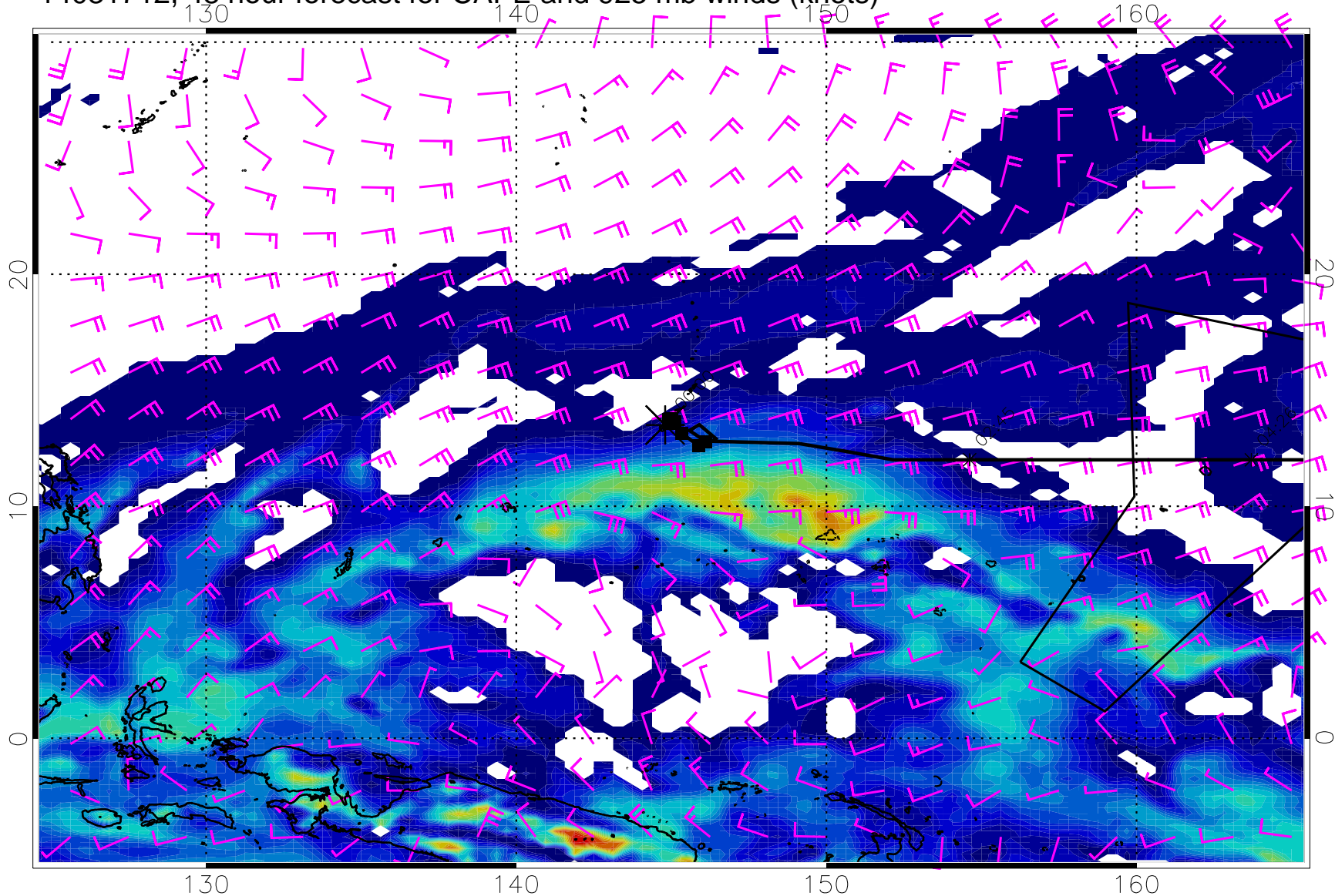
14031712, 48 hour forecast for CAPE and 925 mb winds (knots)
