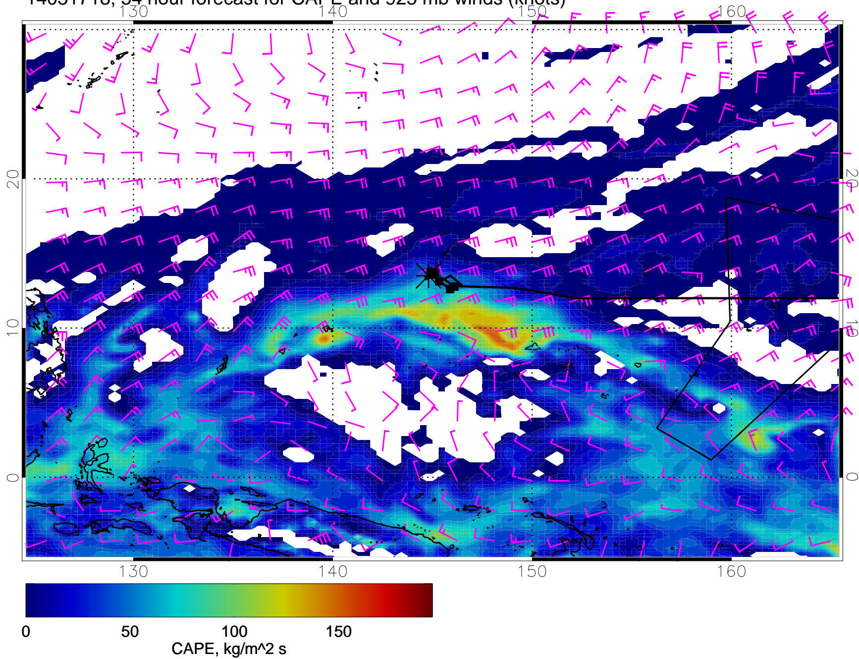
14031718, 54 hour forecast for CAPE and 925 mb winds (knots)
