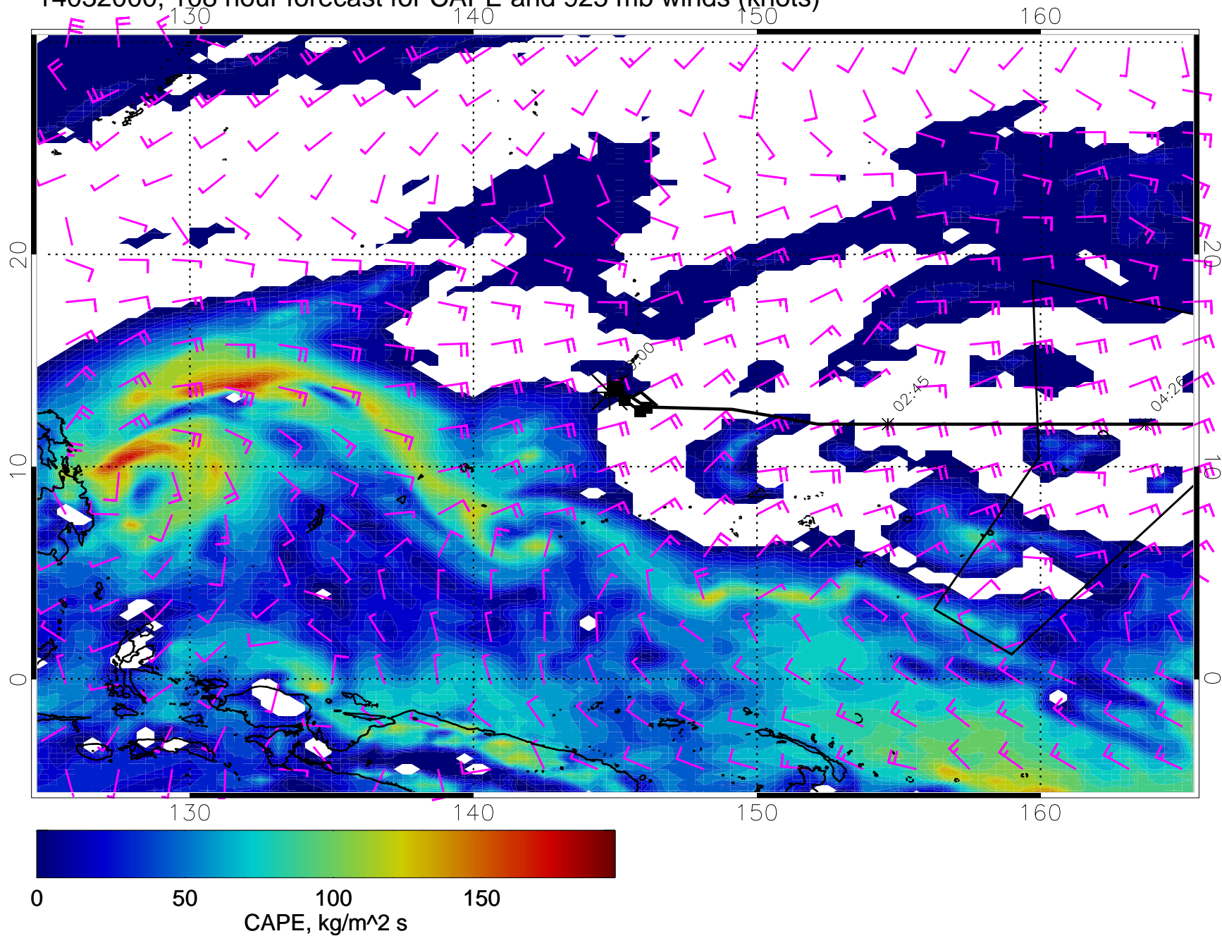
14032000, 108 hour forecast for CAPE and 925 mb winds (knots)
