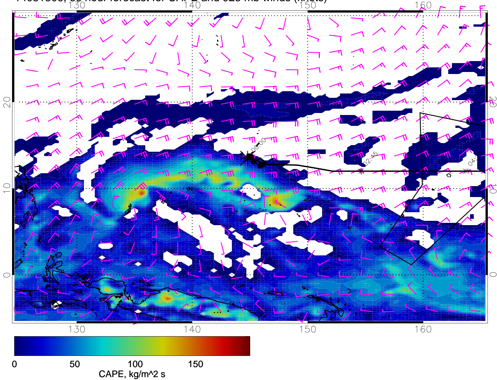
14031806, 66 hour forecast for CAPE and 925 mb winds (knots)
