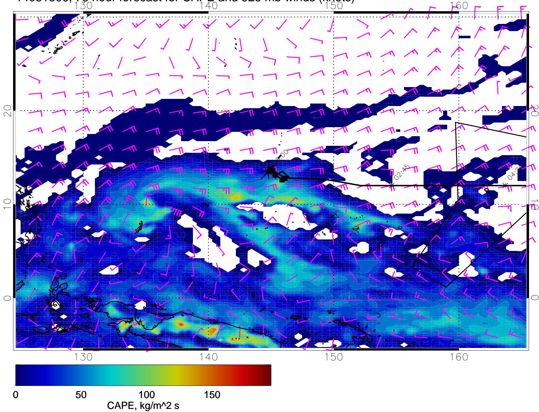
14031806, 78 hour forecast for CAPE and 925 mb winds (knots)
