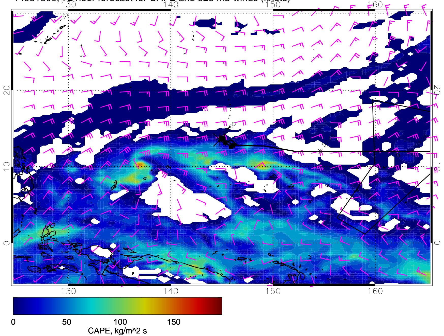
14031800, 72 hour forecast for CAPE and 925 mb winds (knots)
