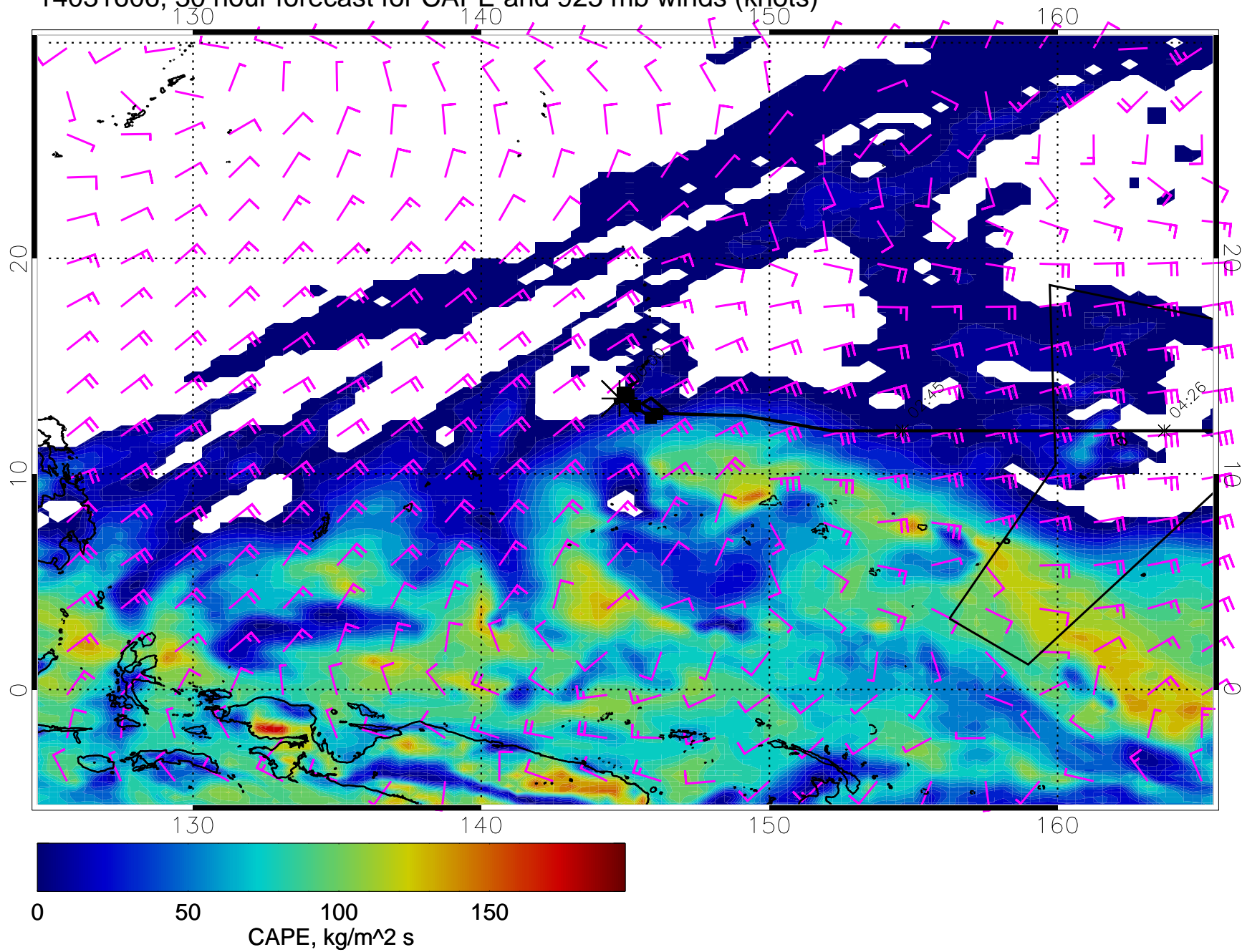
14031606, 30 hour forecast for CAPE and 925 mb winds (knots)
