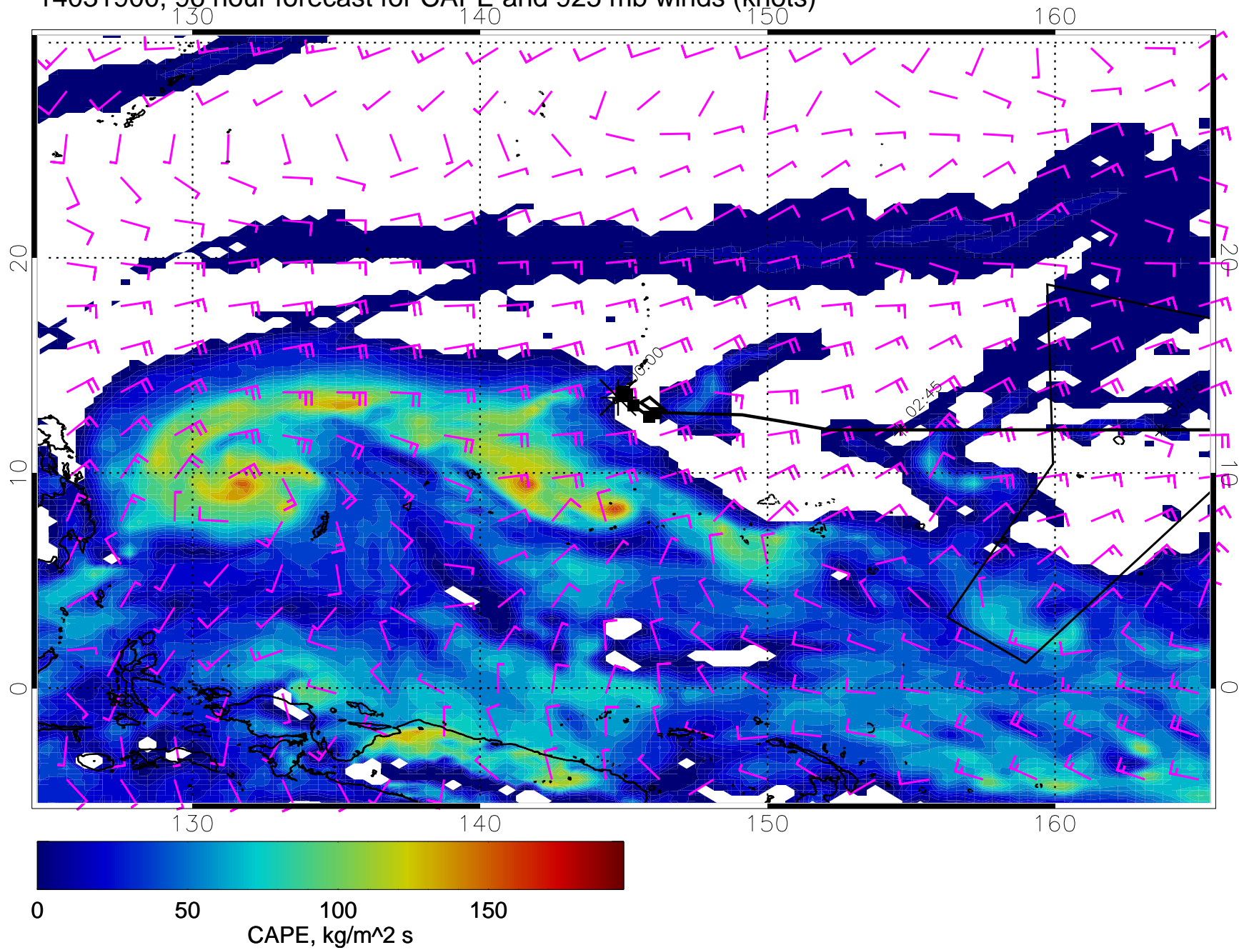
14031900, 96 hour forecast for CAPE and 925 mb winds (knots)
