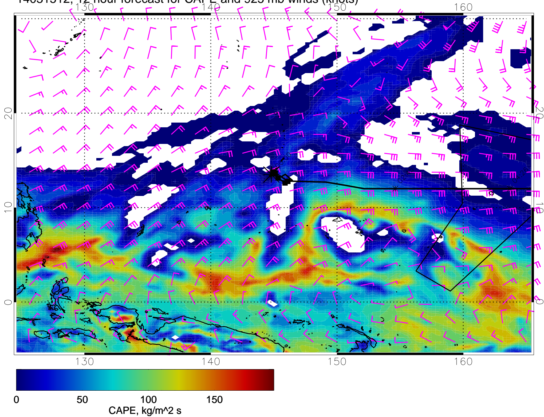
14031512, 12 hour forecast for CAPE and 925 mb winds (knots)
