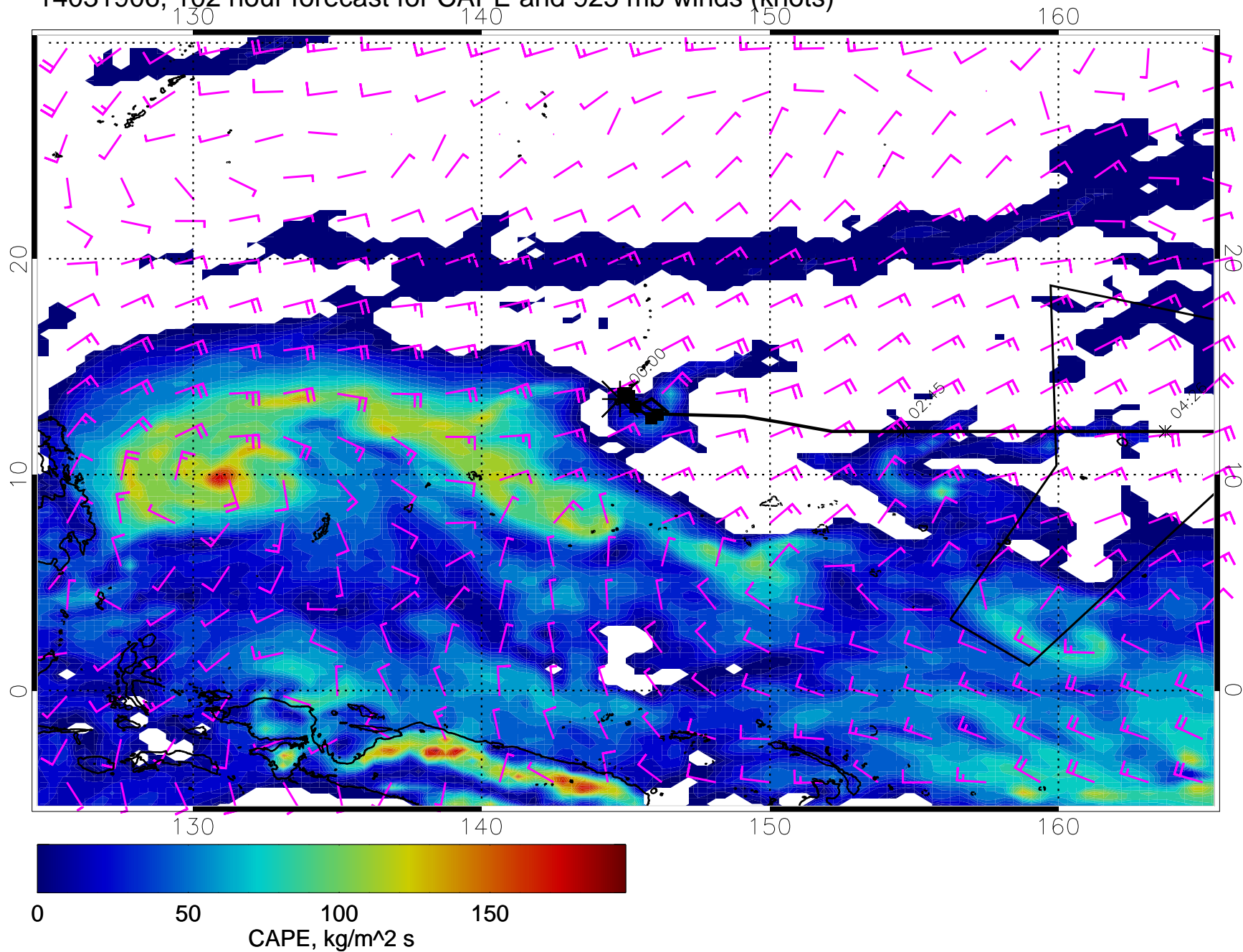
14031906, 102 hour forecast for CAPE and 925 mb winds (knots)
