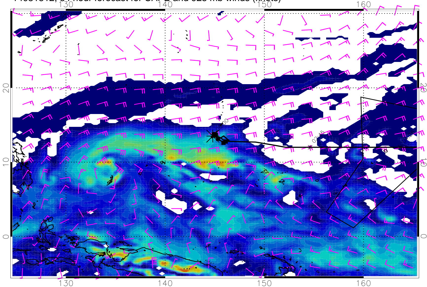
14031812, 84 hour forecast for CAPE and 925 mb winds (knots)
