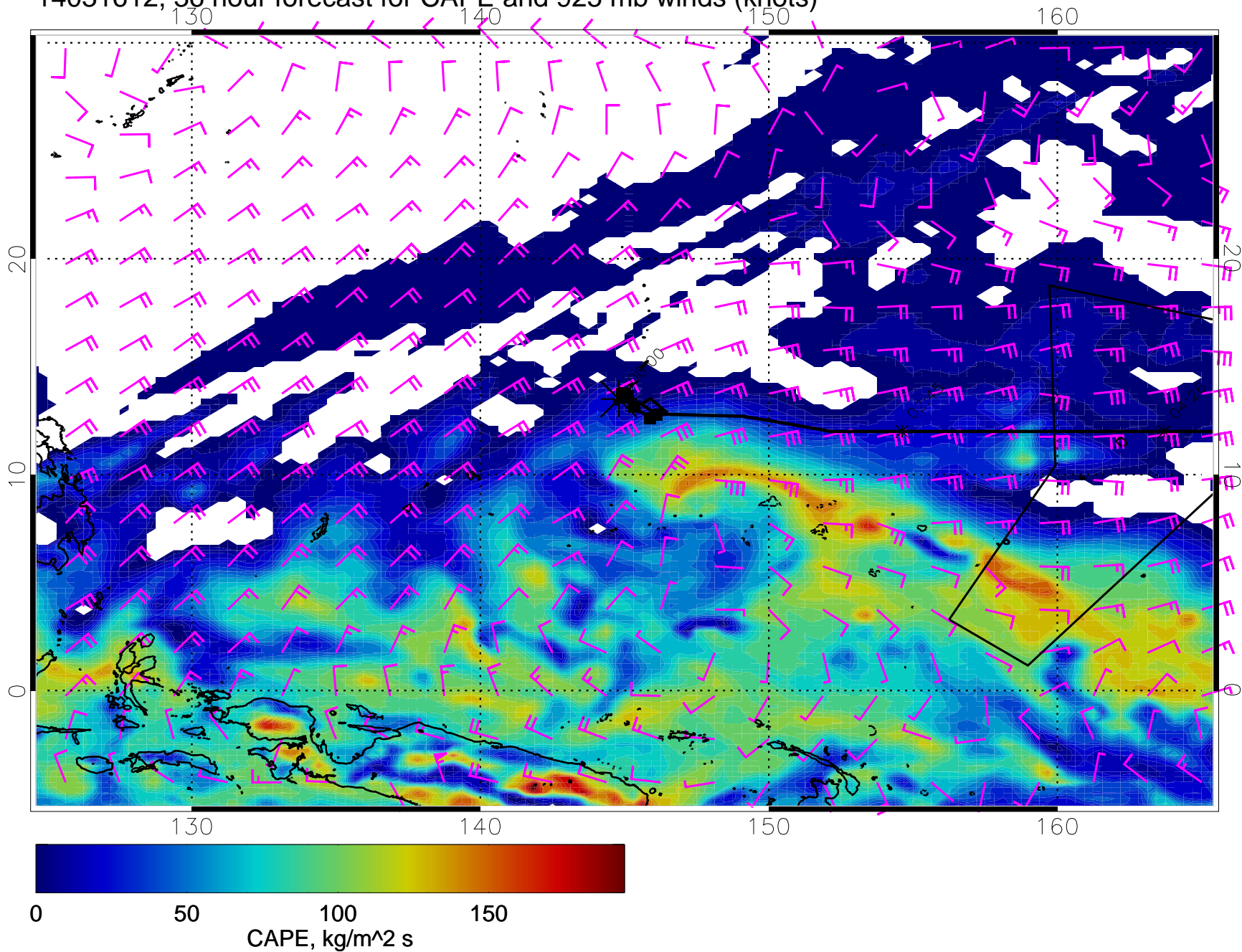
14031612, 36 hour forecast for CAPE and 925 mb winds (knots)
