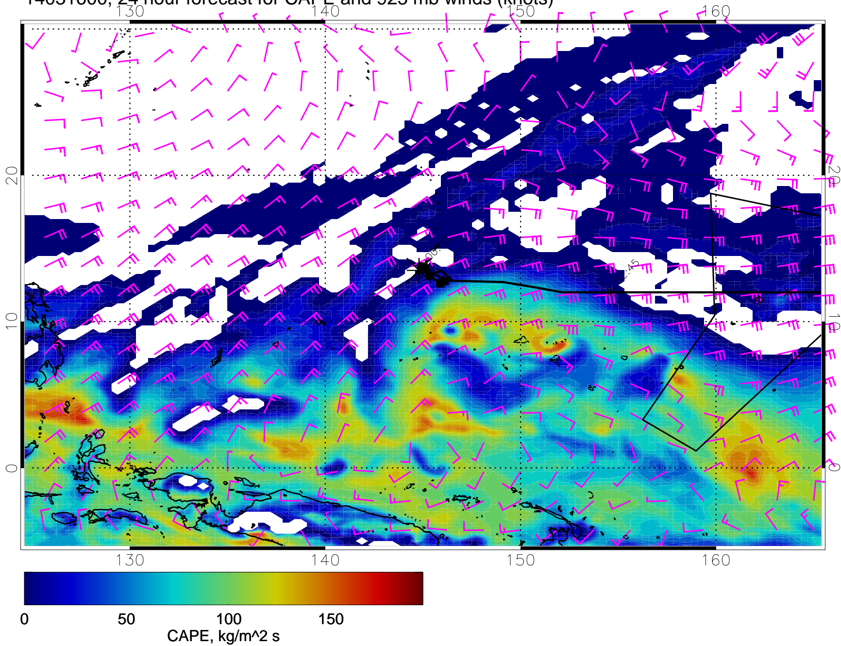
14031600, 24 hour forecast for CAPE and 925 mb winds (knots)
