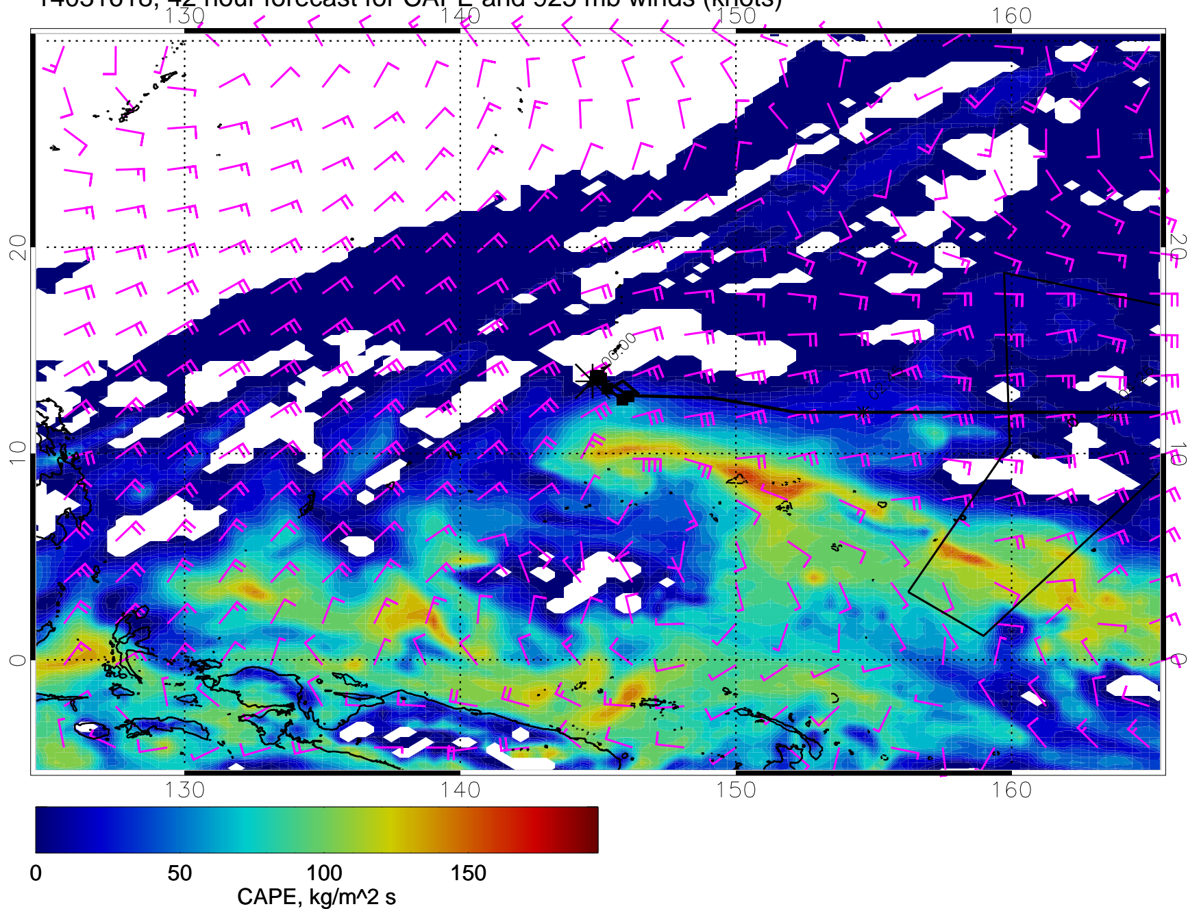
14031618, 42 hour forecast for CAPE and 925 mb winds (knots)
