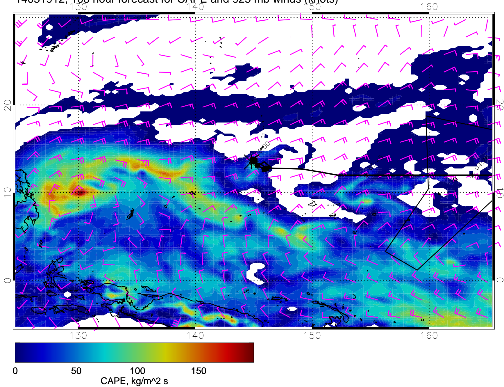
14031912, 108 hour forecast for CAPE and 925 mb winds (knots)
