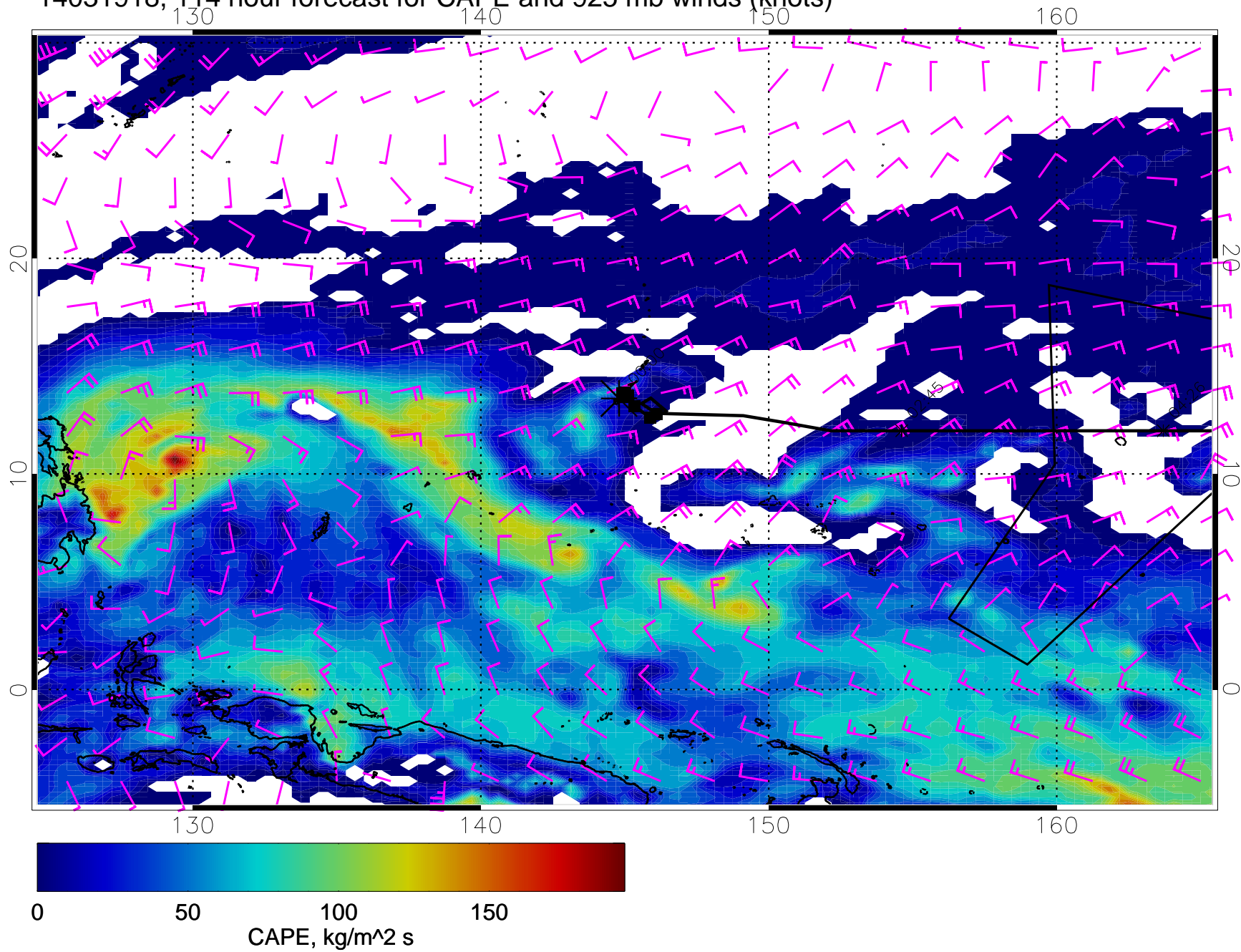
14031918, 114 hour forecast for CAPE and 925 mb winds (knots)
