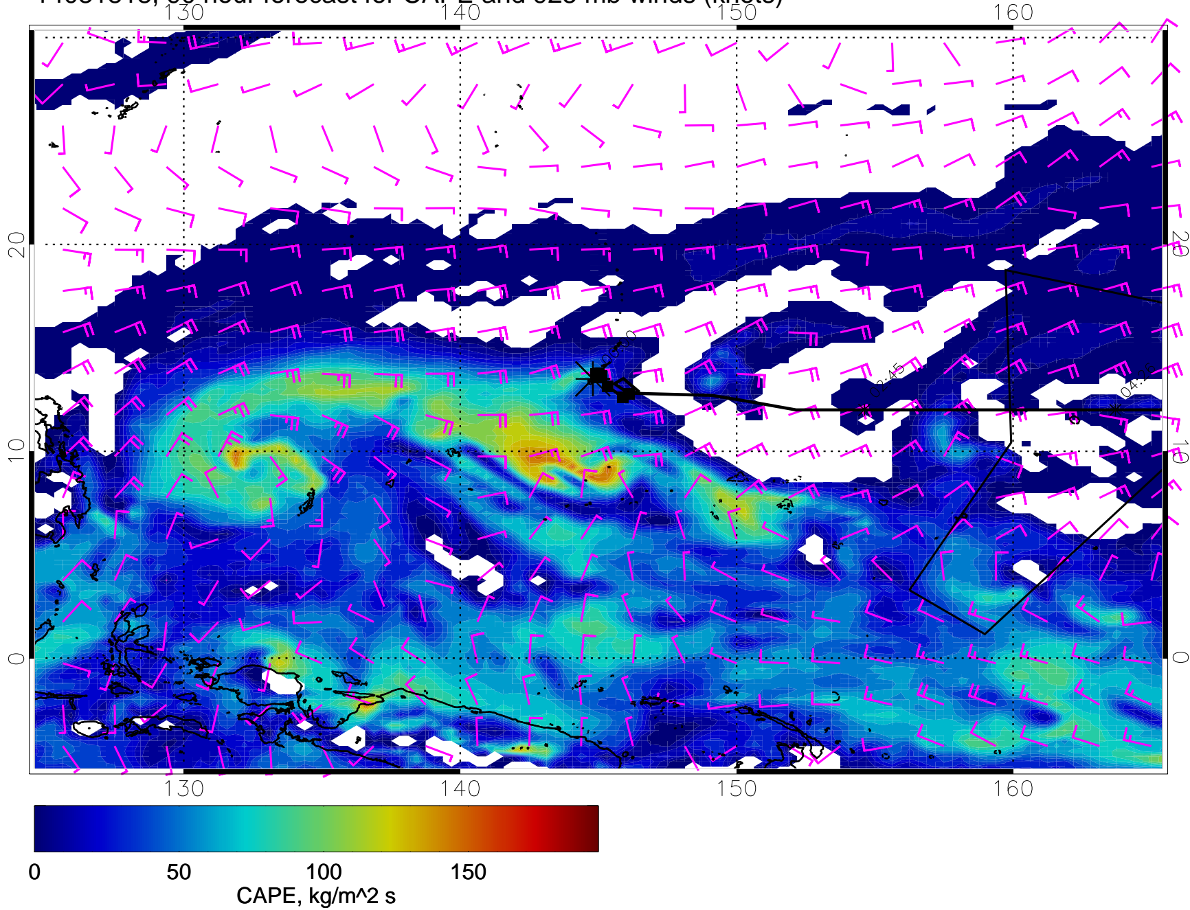
14031818, 90 hour forecast for CAPE and 925 mb winds (knots)
