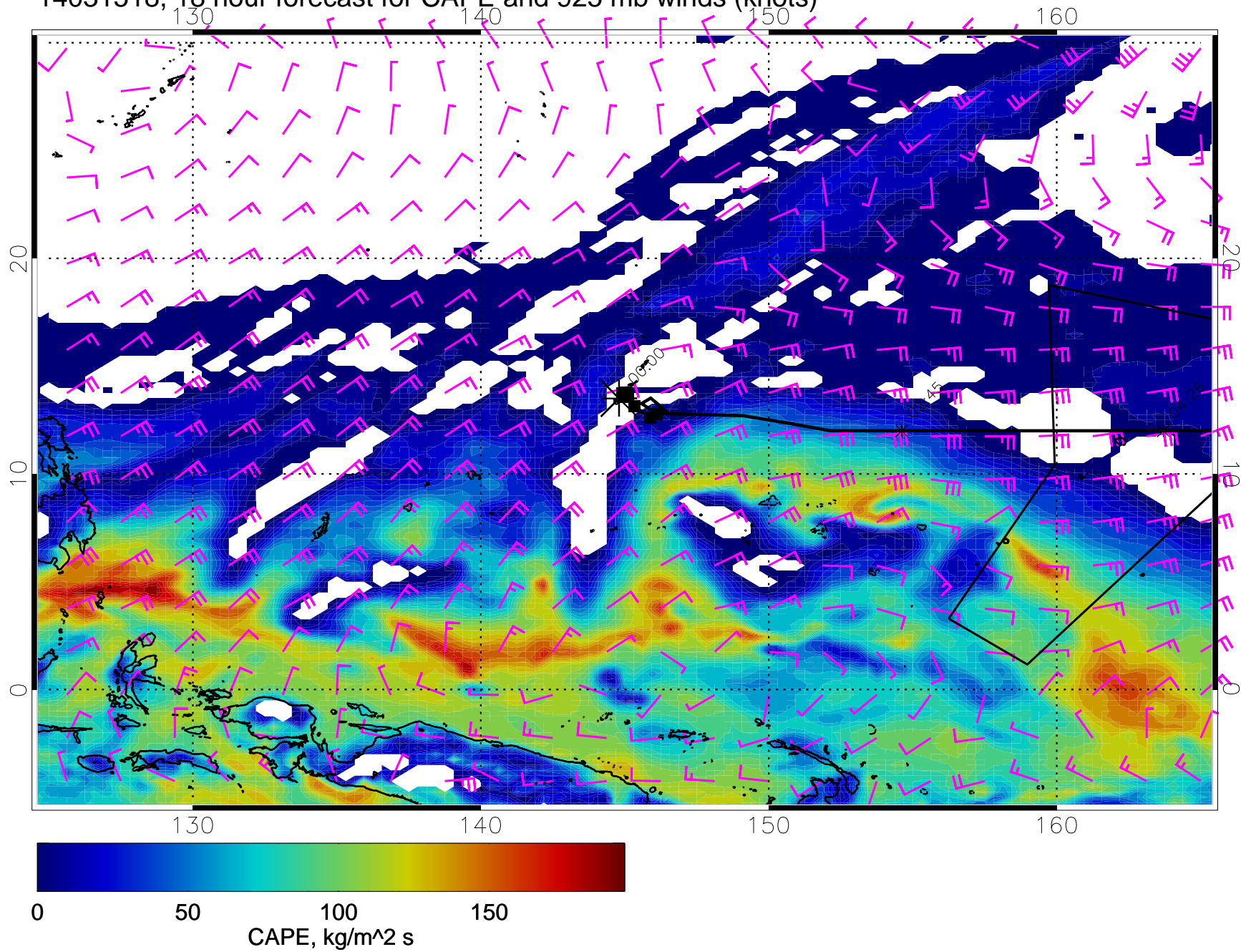
14031518, 18 hour forecast for CAPE and 925 mb winds (knots)
