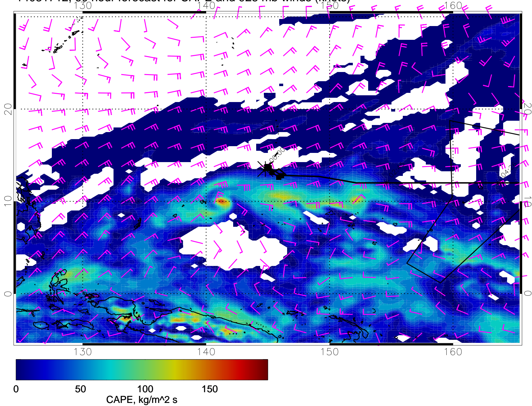
14031712, 60 hour forecast for CAPE and 925 mb winds (knots)
