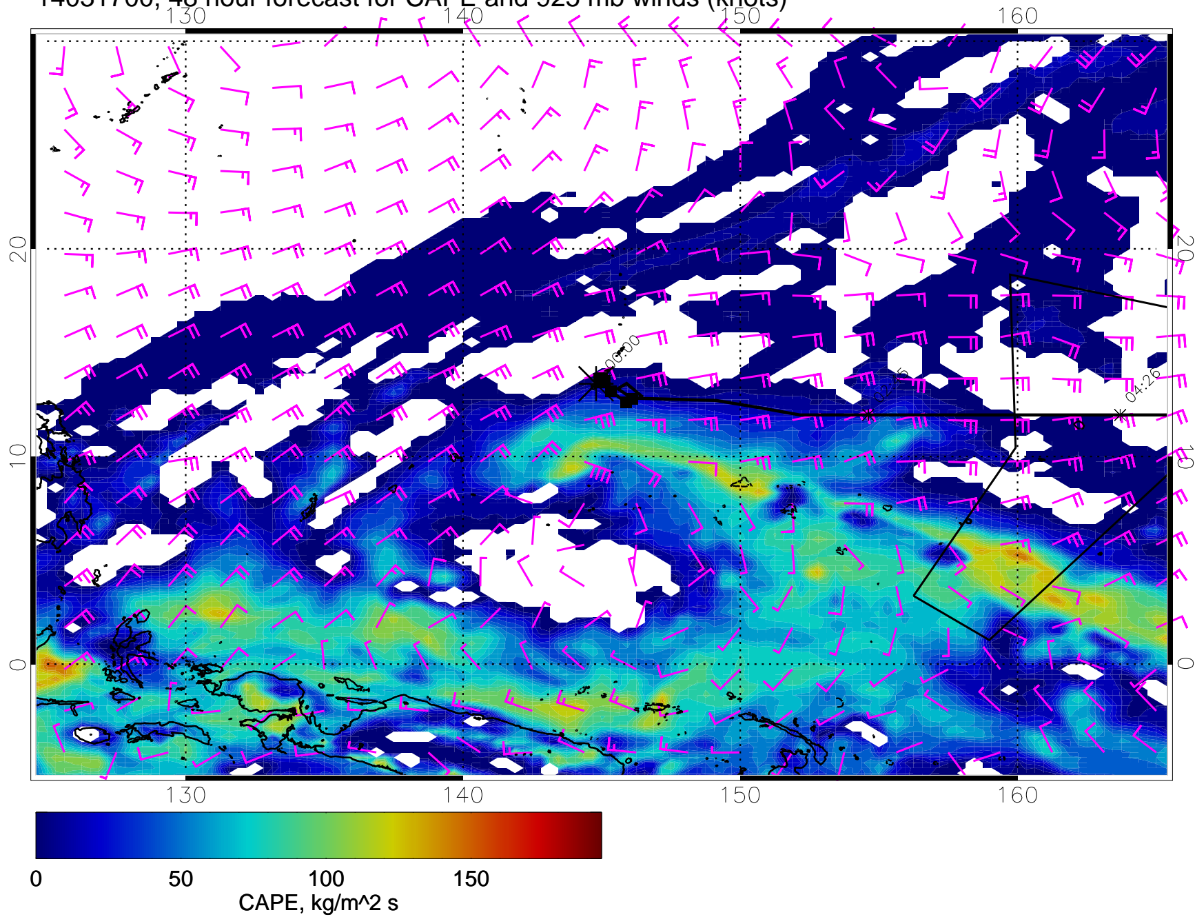
14031700, 48 hour forecast for CAPE and 925 mb winds (knots)
