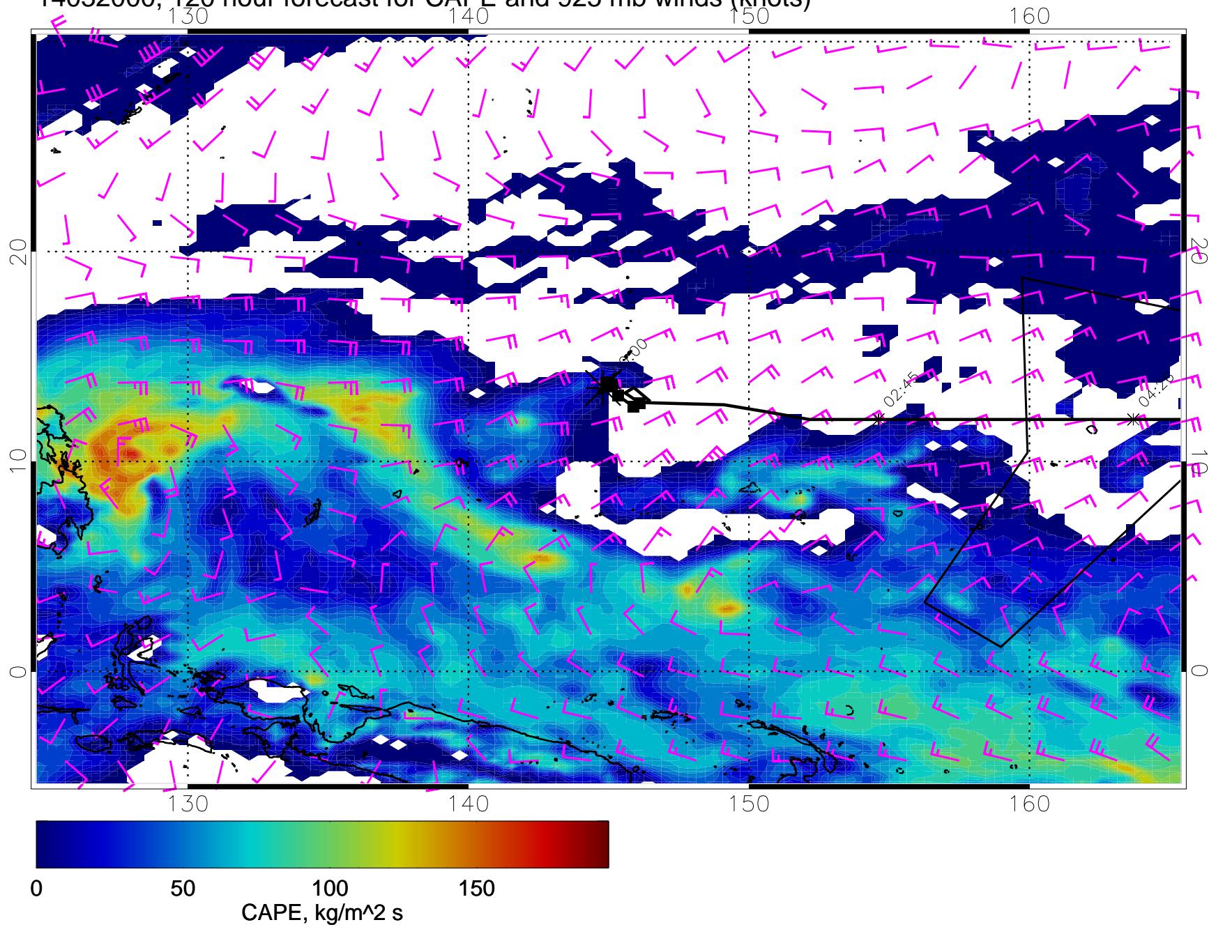
14032000, 120 hour forecast for CAPE and 925 mb winds (knots)
