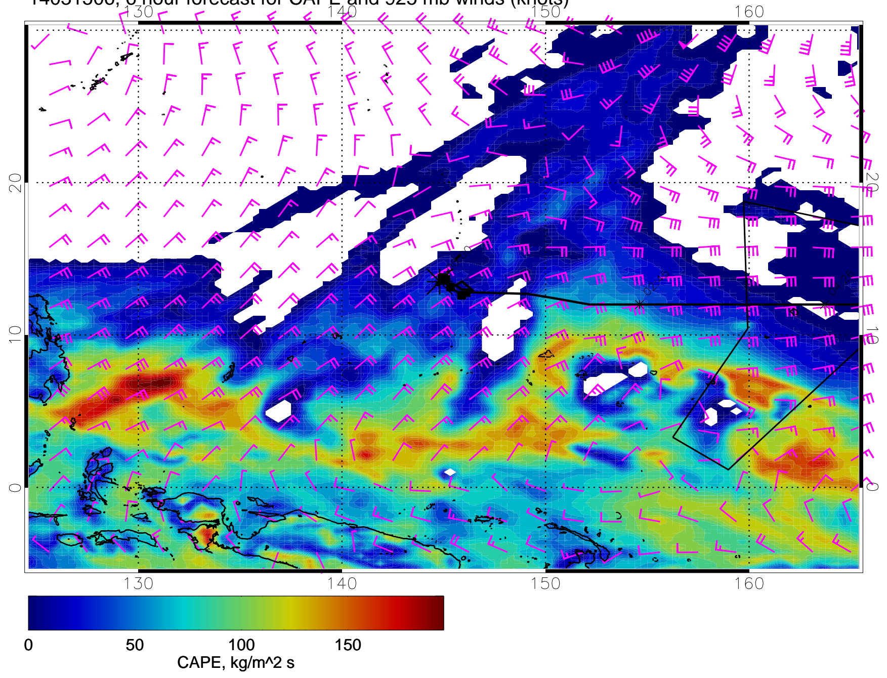
14031506, 6 hour forecast for CAPE and 925 mb winds (knots)
