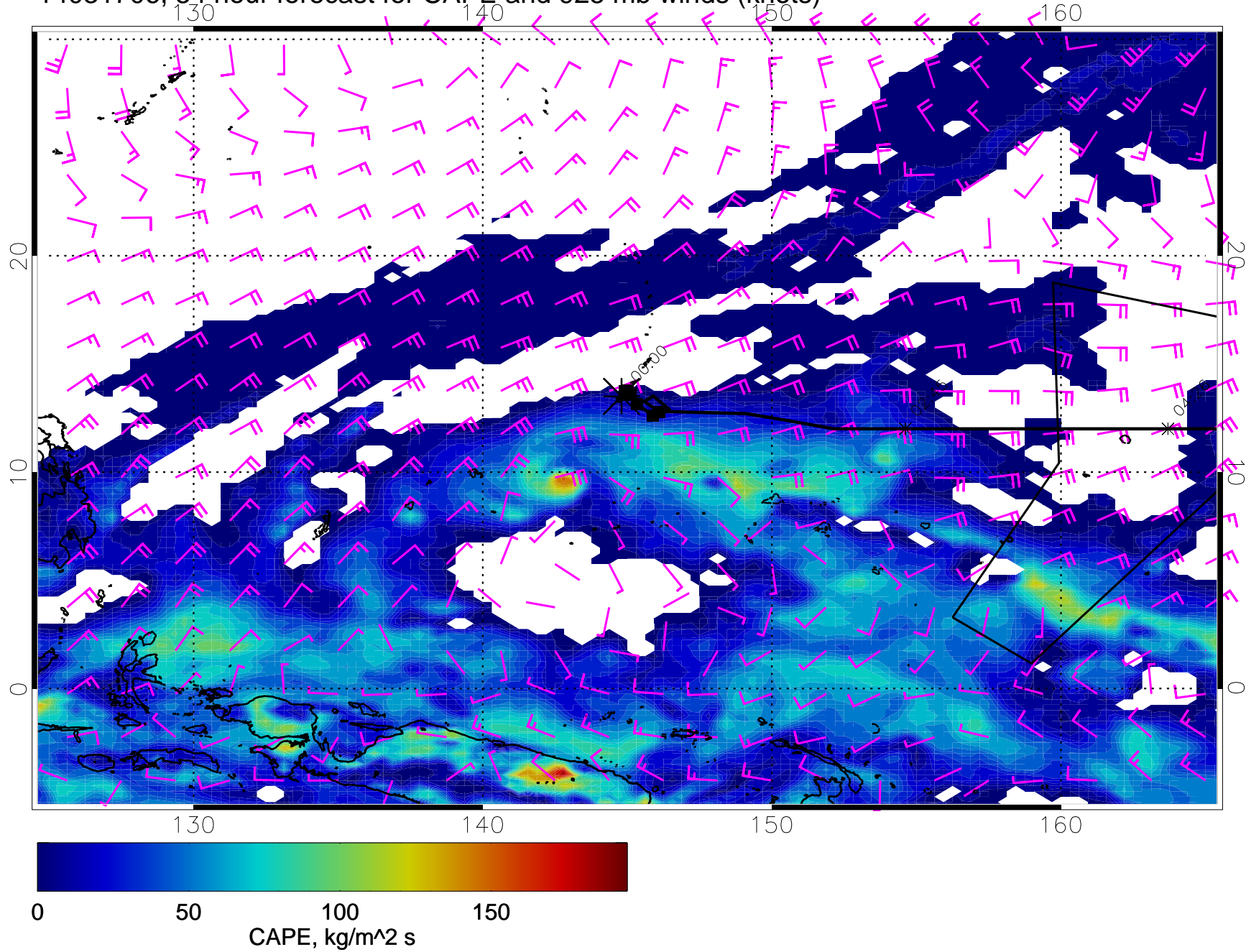
14031706, 54 hour forecast for CAPE and 925 mb winds (knots)
