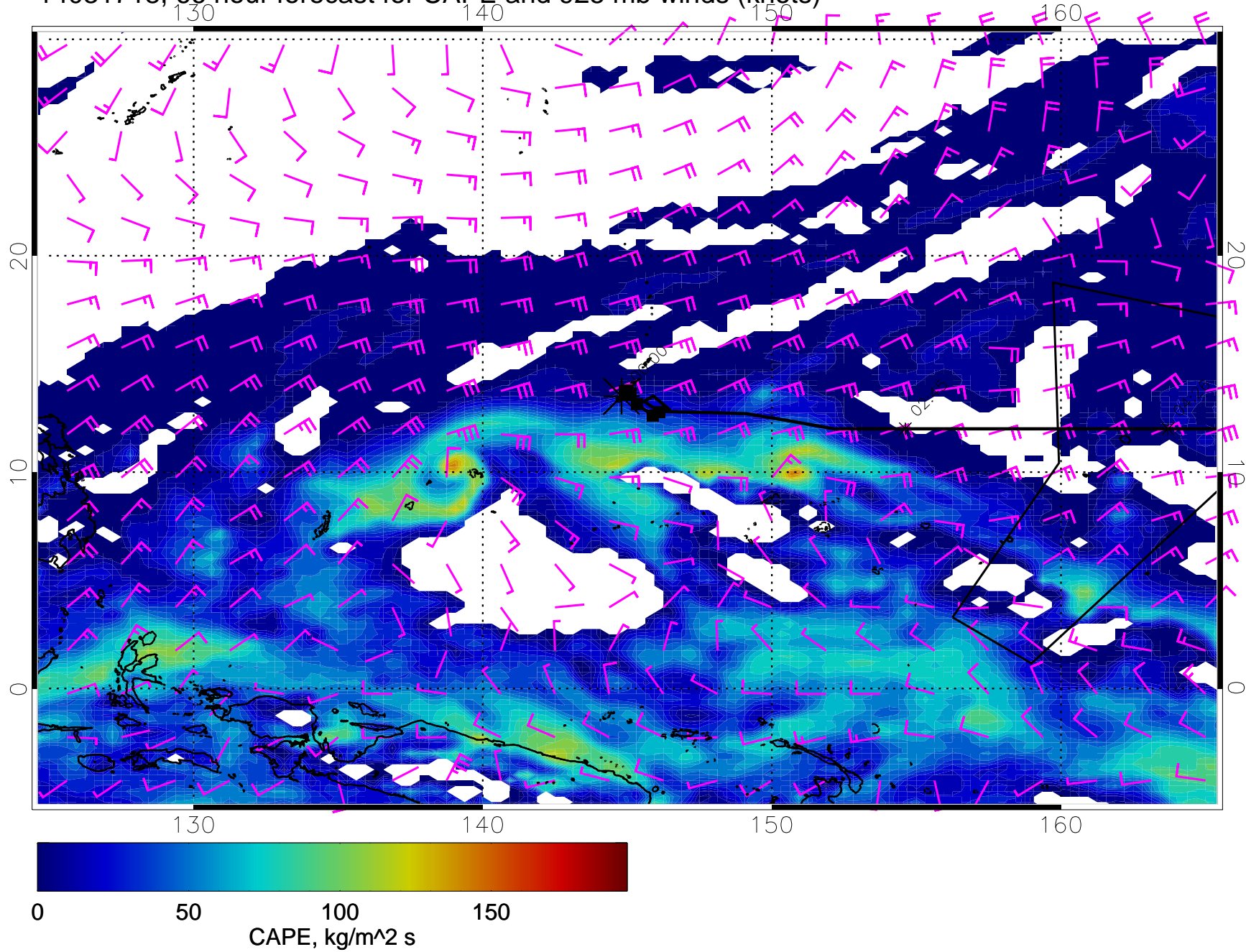
14031718, 66 hour forecast for CAPE and 925 mb winds (knots)
