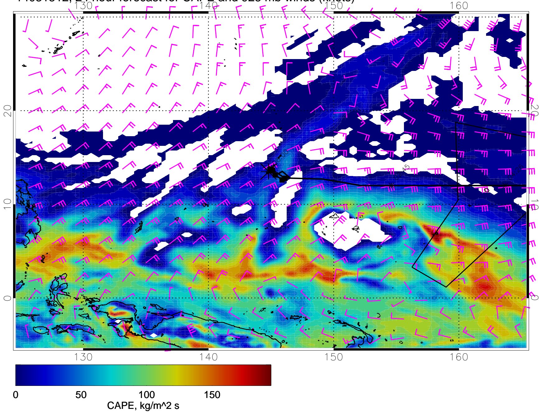
14031512, 24 hour forecast for CAPE and 925 mb winds (knots)
