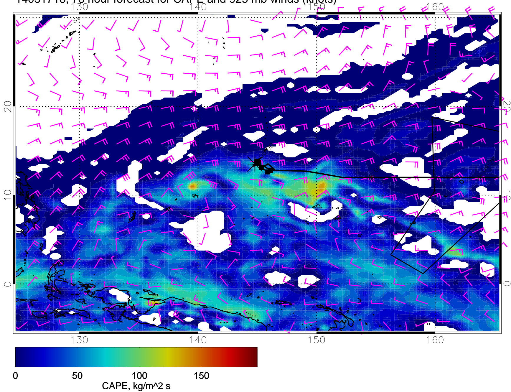
14031718, 78 hour forecast for CAPE and 925 mb winds (knots)
