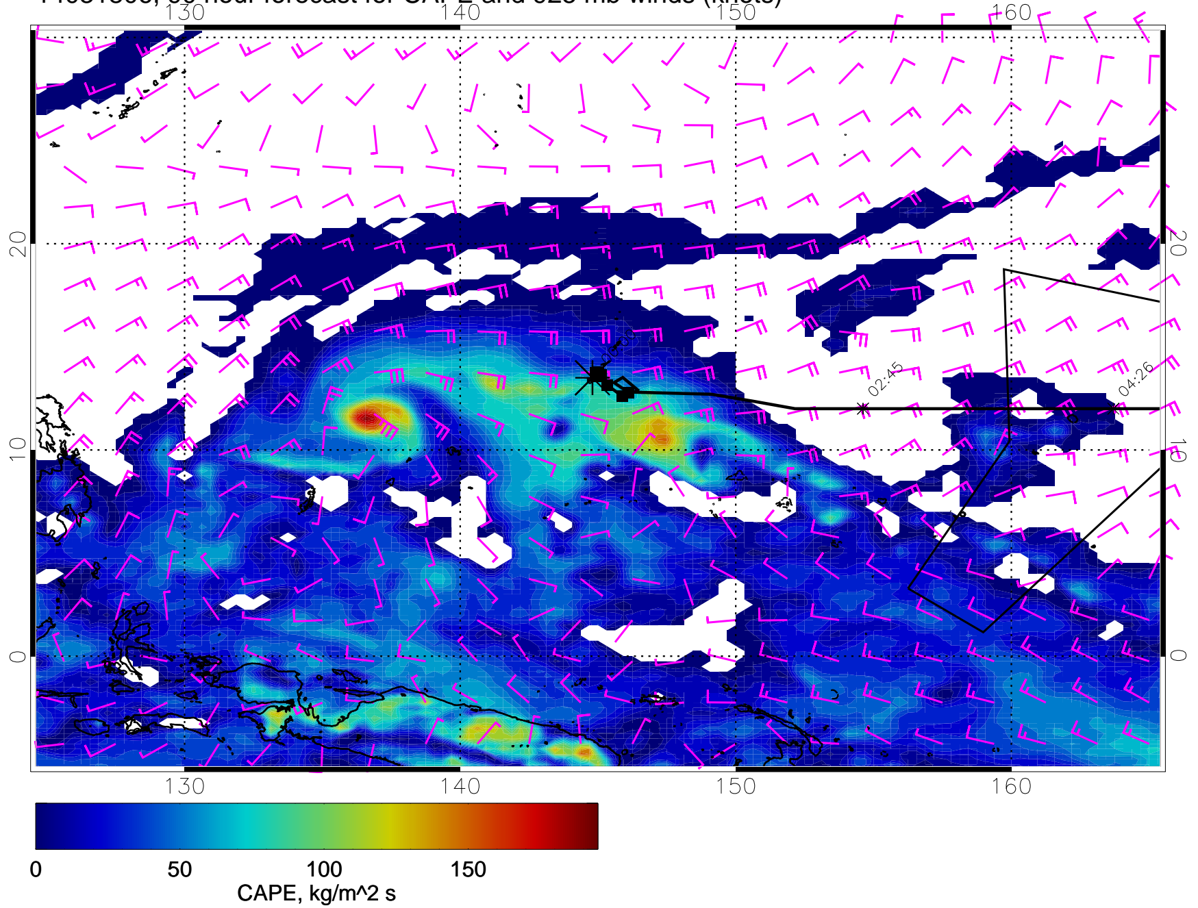
14031806, 90 hour forecast for CAPE and 925 mb winds (knots)
