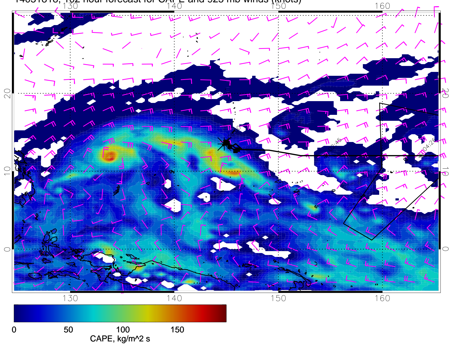
14031818, 102 hour forecast for CAPE and 925 mb winds (knots)
