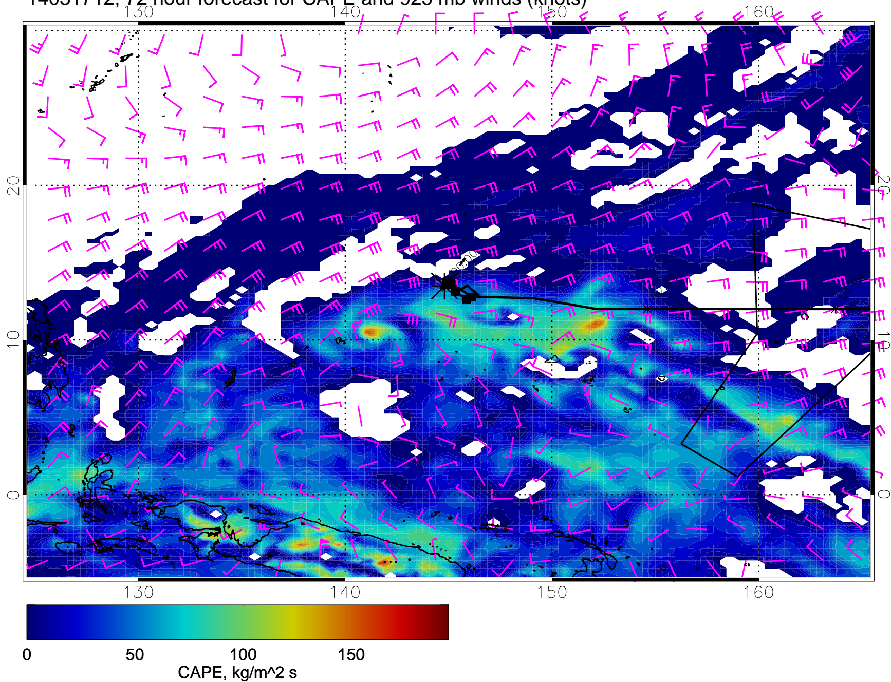
14031712, 72 hour forecast for CAPE and 925 mb winds (knots)
