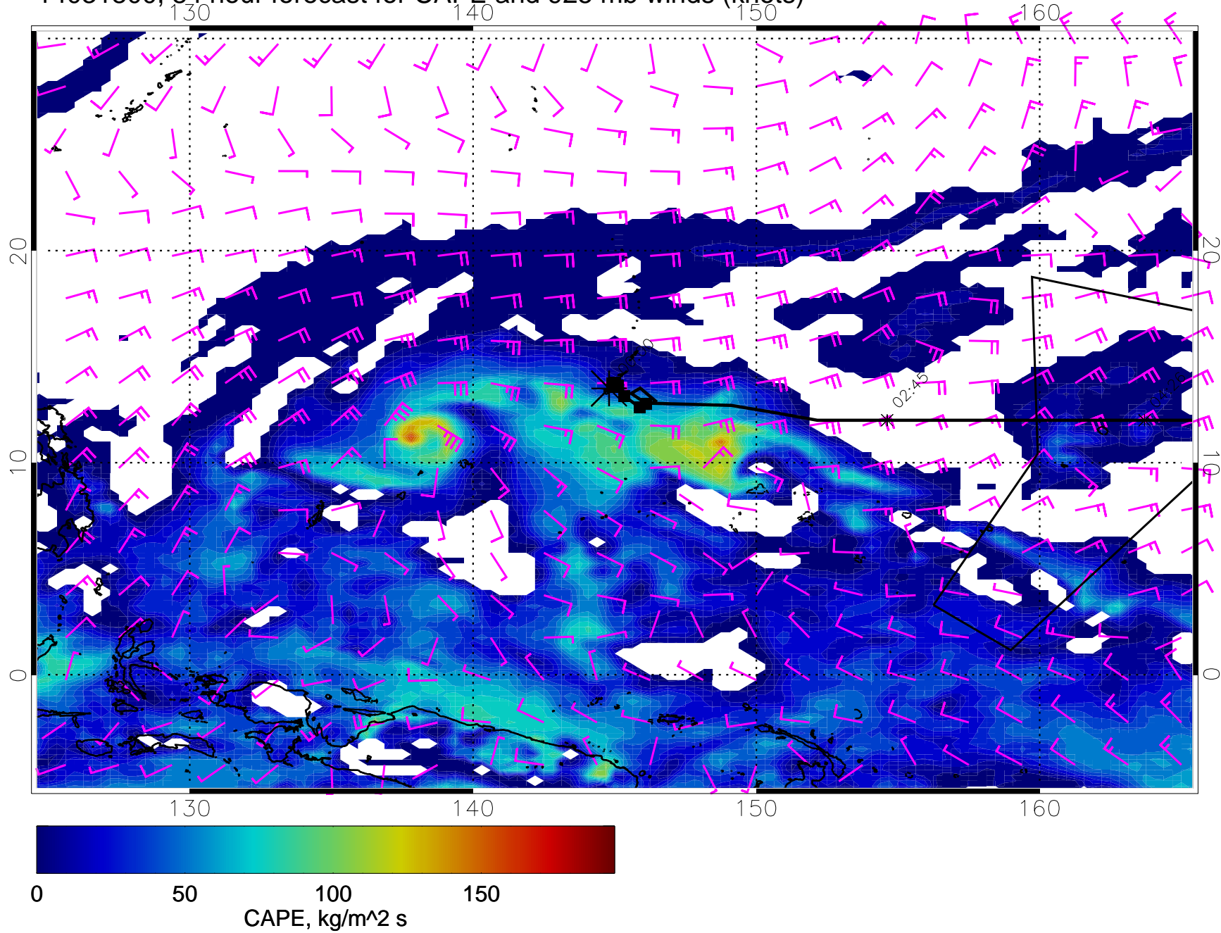
14031800, 84 hour forecast for CAPE and 925 mb winds (knots)
