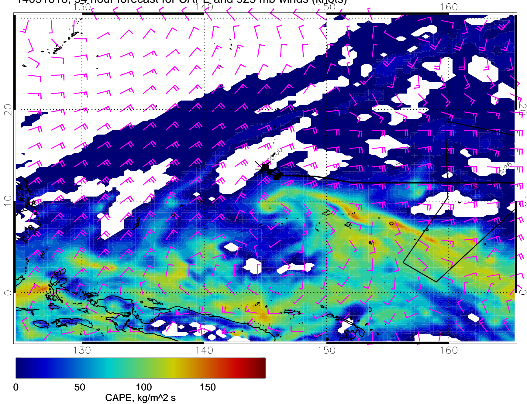
14031618, 54 hour forecast for CAPE and 925 mb winds (knots)
