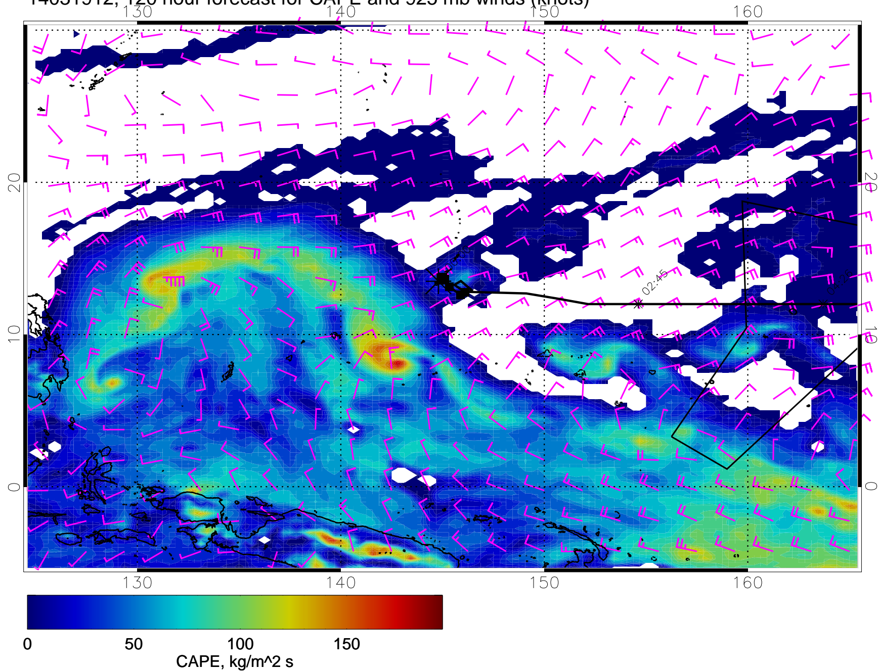
14031912, 120 hour forecast for CAPE and 925 mb winds (knots)
