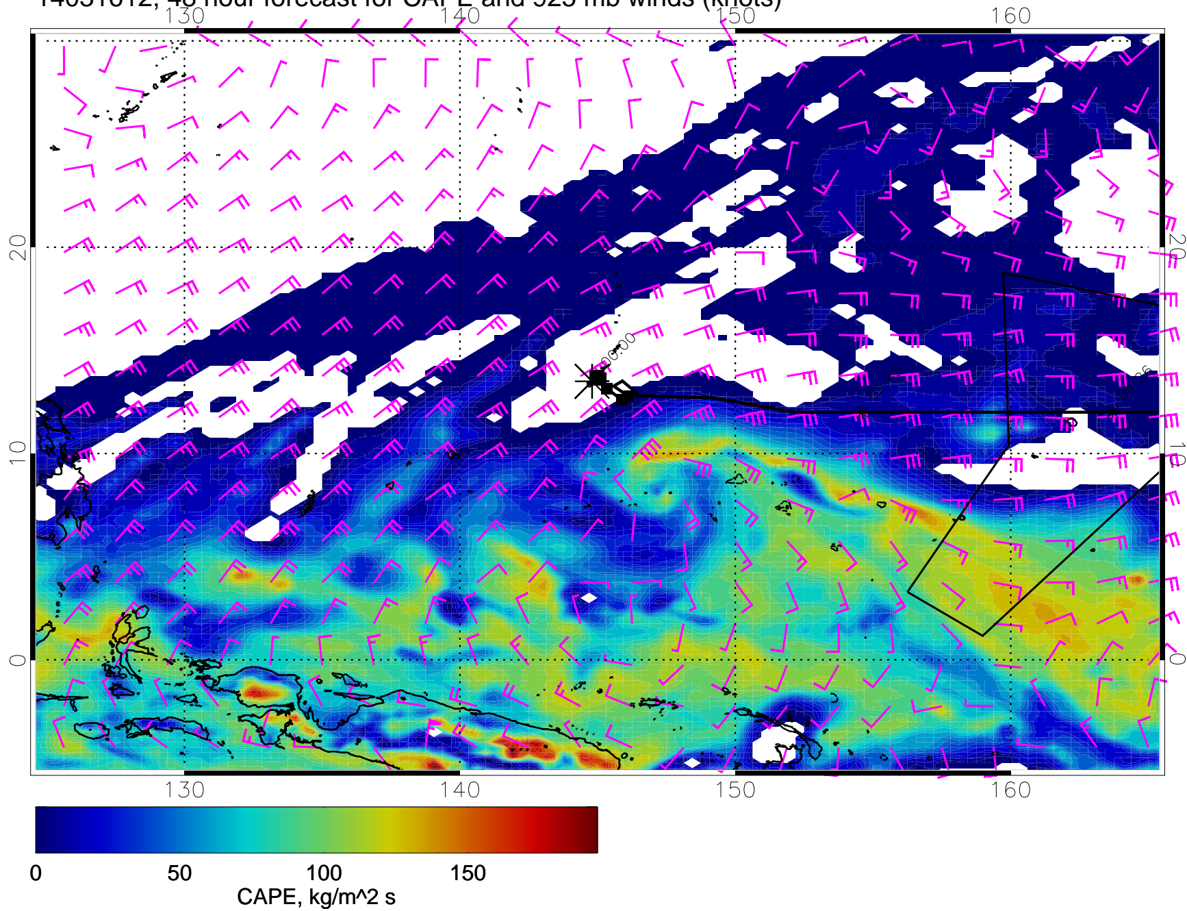
14031612, 48 hour forecast for CAPE and 925 mb winds (knots)
