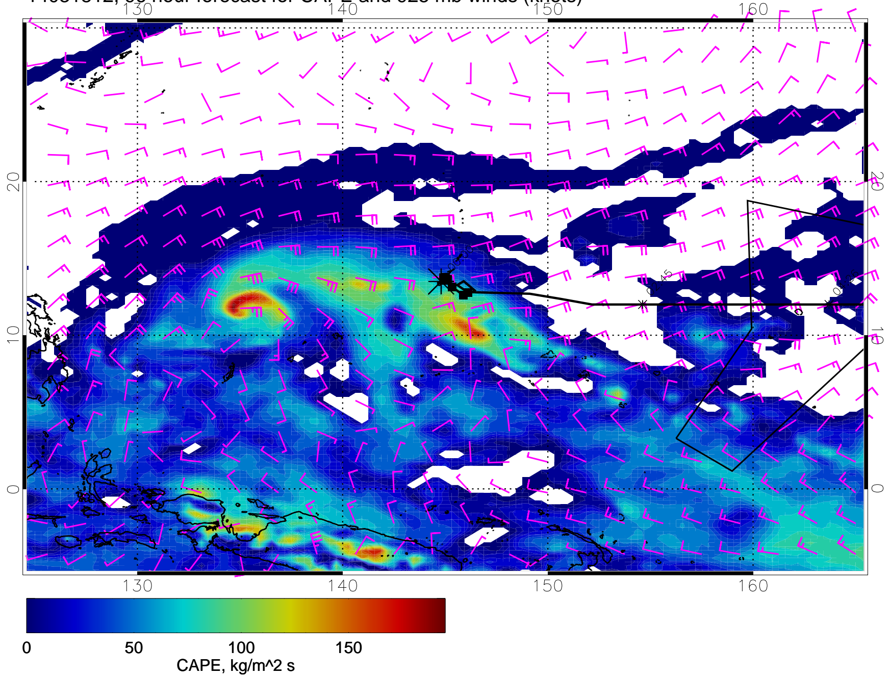
14031812, 96 hour forecast for CAPE and 925 mb winds (knots)
