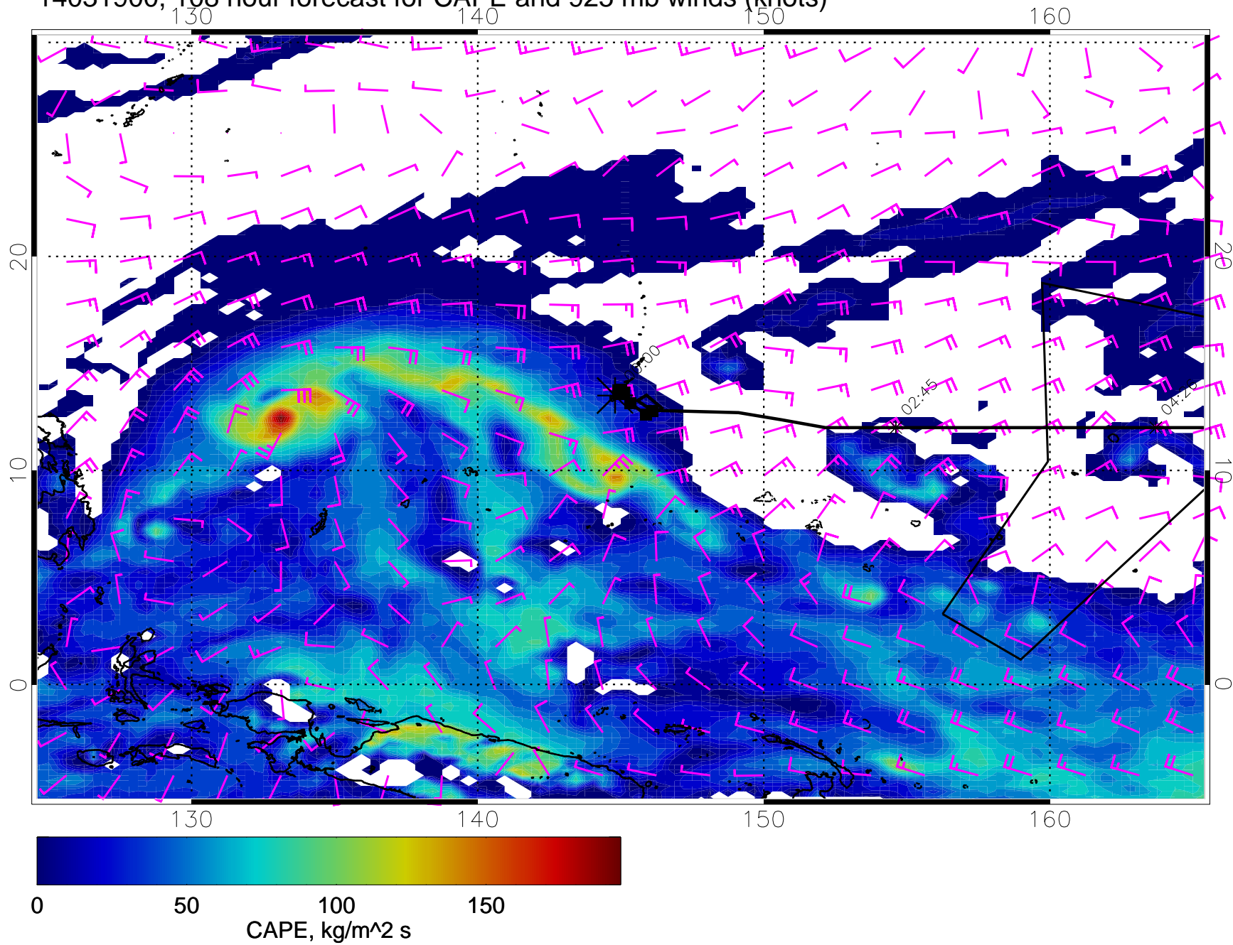
14031900, 108 hour forecast for CAPE and 925 mb winds (knots)
