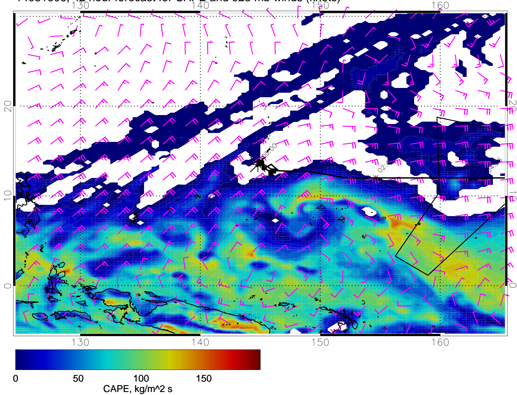
14031606, 42 hour forecast for CAPE and 925 mb winds (knots)
