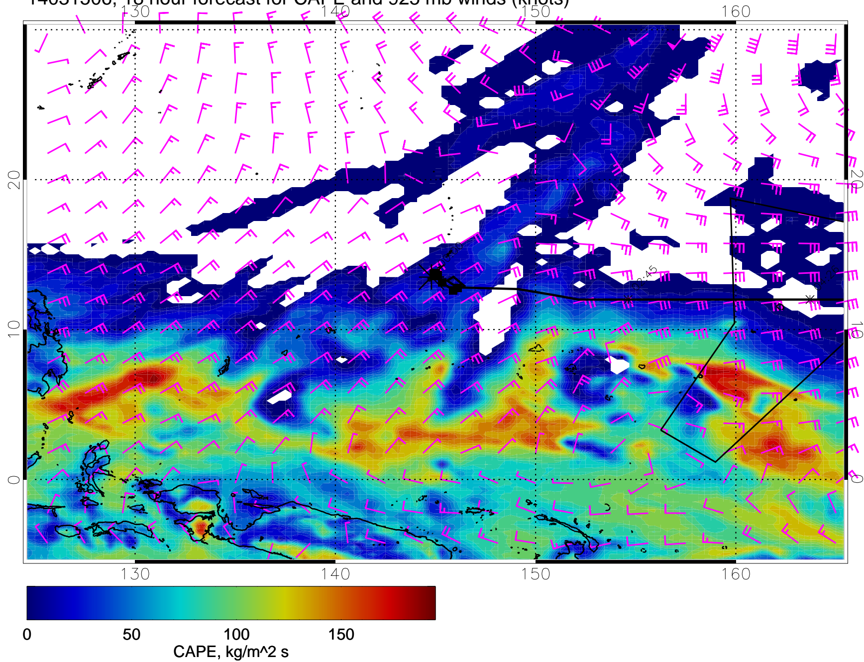
14031506, 18 hour forecast for CAPE and 925 mb winds (knots)
