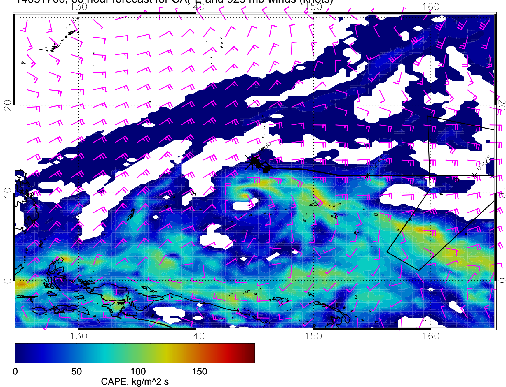
14031700, 60 hour forecast for CAPE and 925 mb winds (knots)
