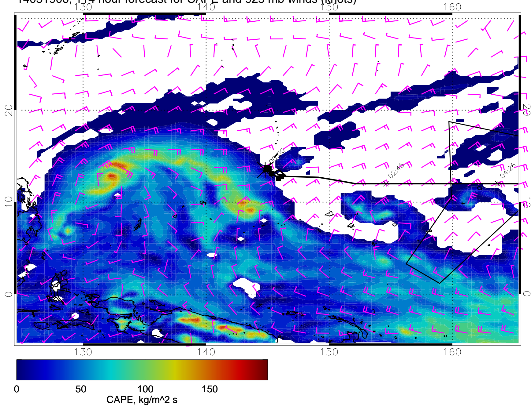
14031906, 114 hour forecast for CAPE and 925 mb winds (knots)
