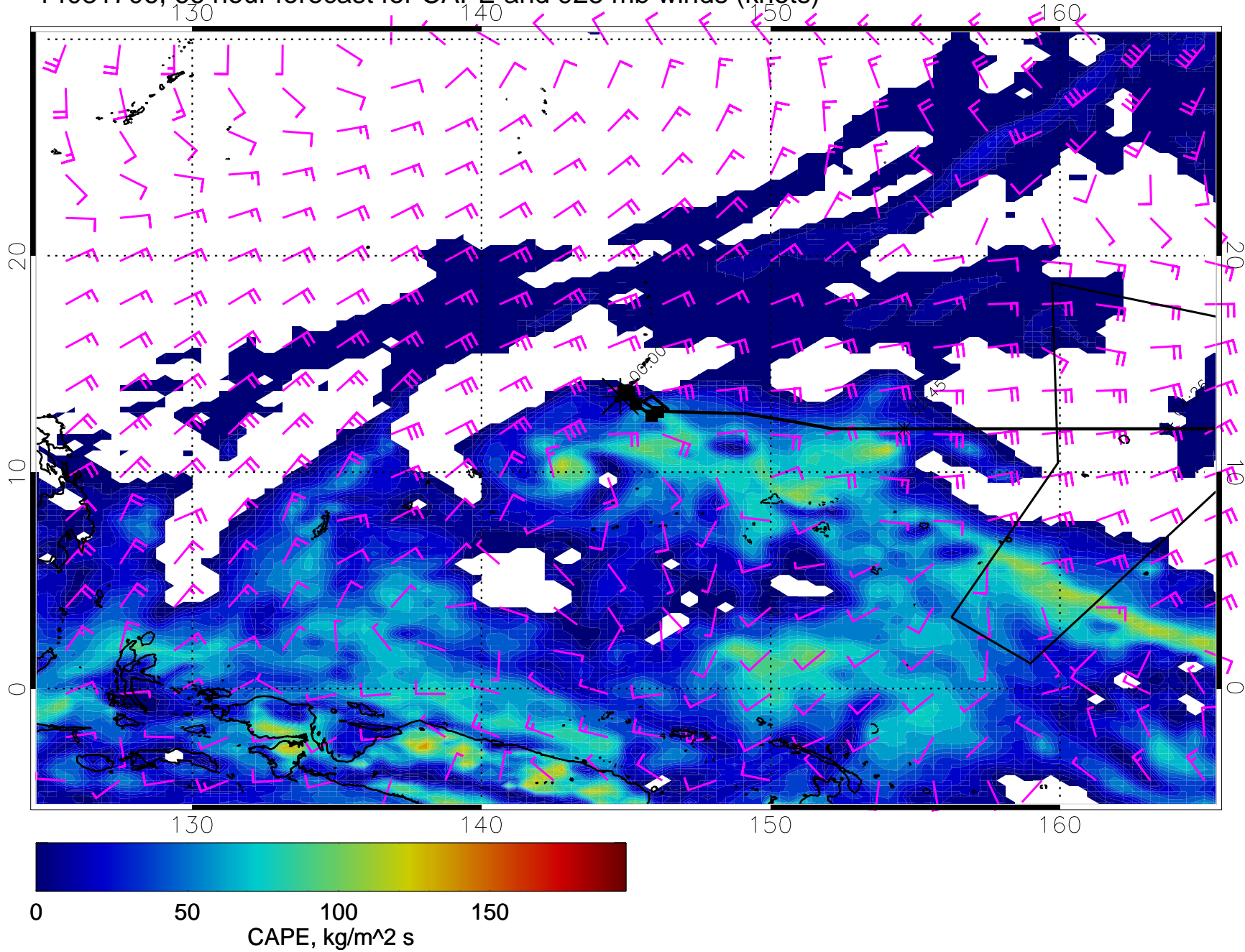
14031706, 66 hour forecast for CAPE and 925 mb winds (knots)
