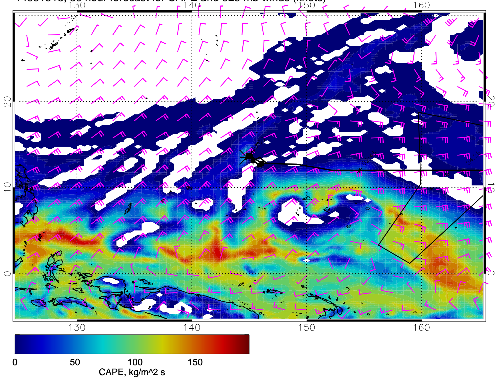
14031518, 30 hour forecast for CAPE and 925 mb winds (knots)
