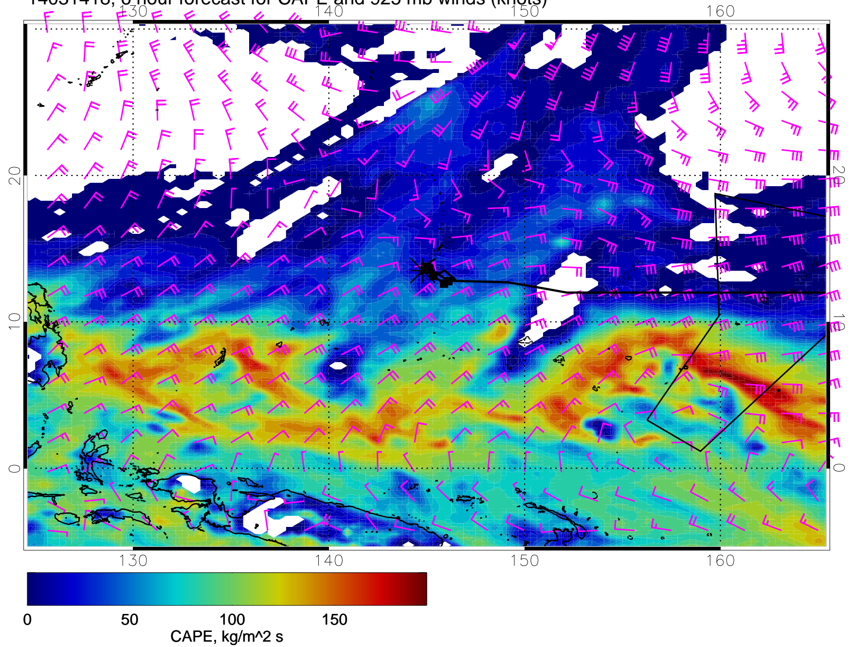
14031418, 6 hour forecast for CAPE and 925 mb winds (knots)
