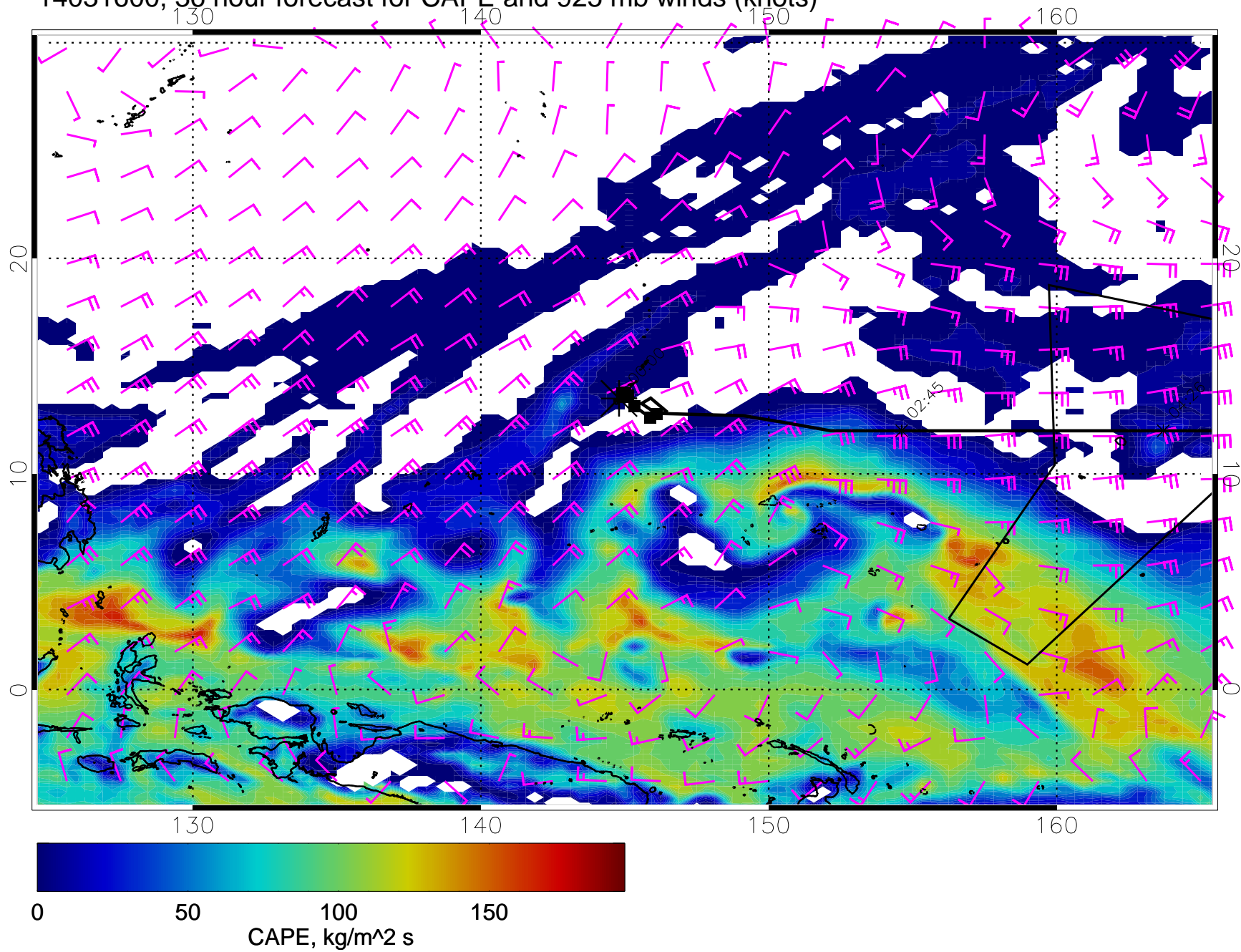
14031600, 36 hour forecast for CAPE and 925 mb winds (knots)
