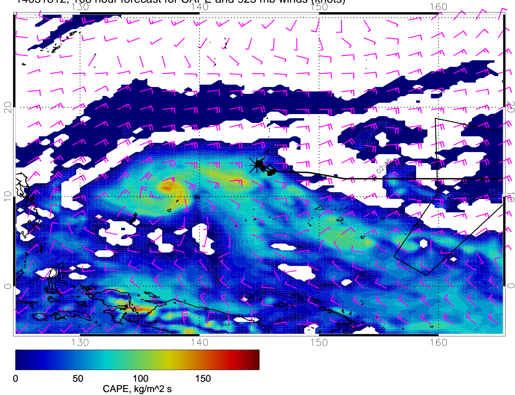
14031812, 108 hour forecast for CAPE and 925 mb winds (knots)
