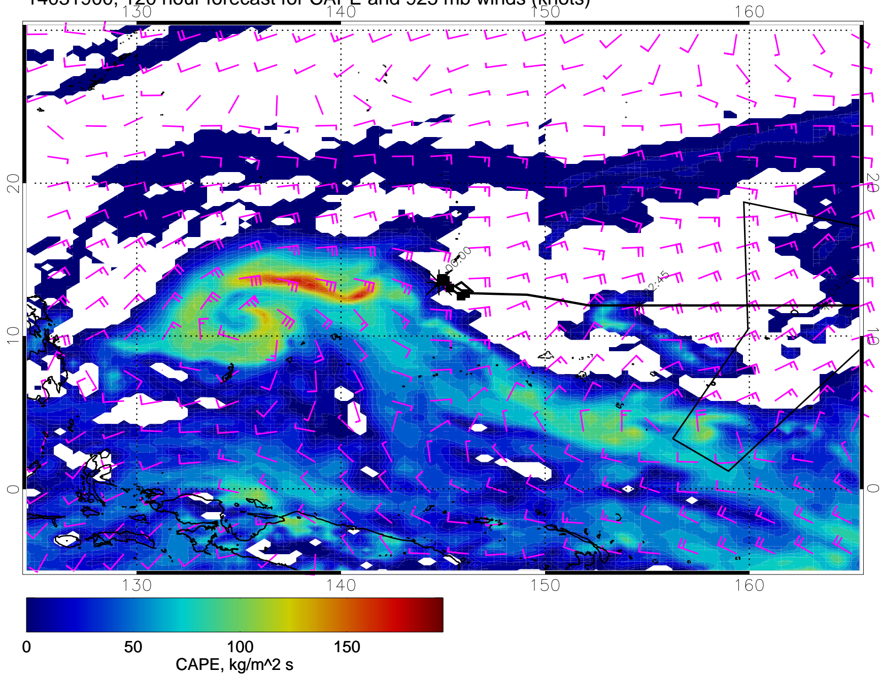
14031900, 120 hour forecast for CAPE and 925 mb winds (knots)
