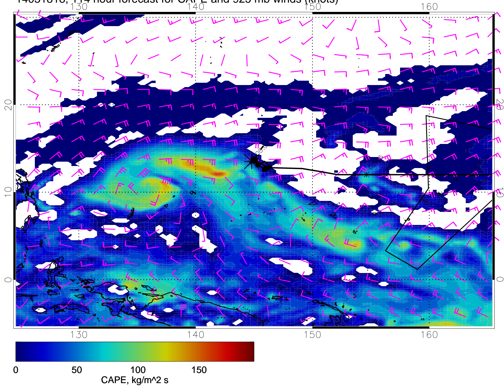
14031818, 114 hour forecast for CAPE and 925 mb winds (knots)
