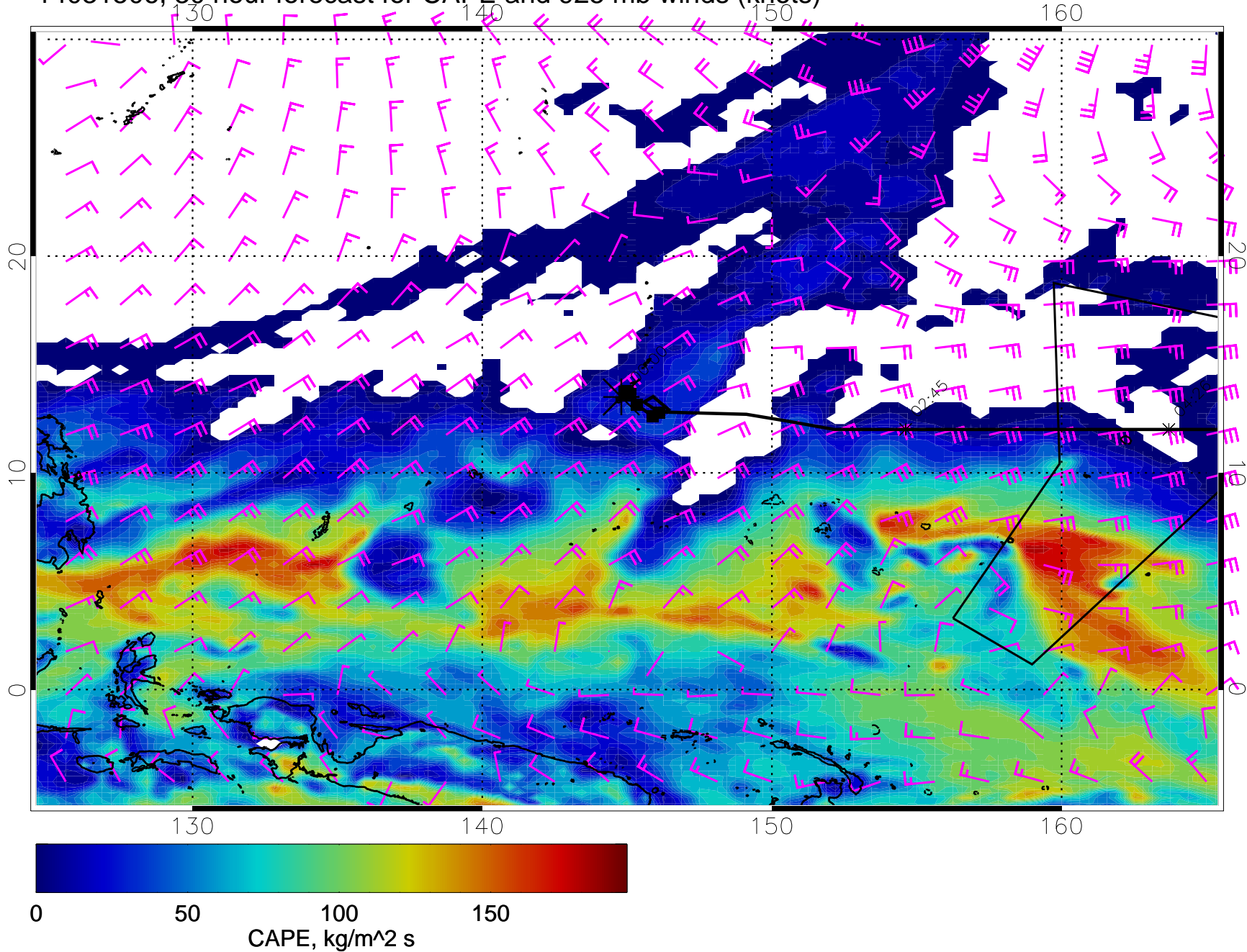
14031506, 30 hour forecast for CAPE and 925 mb winds (knots)
