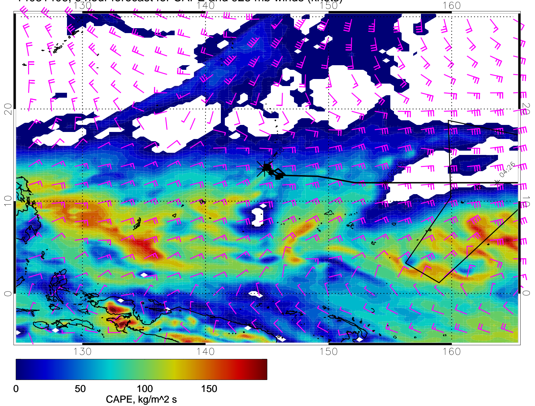
14031406, 6 hour forecast for CAPE and 925 mb winds (knots)
