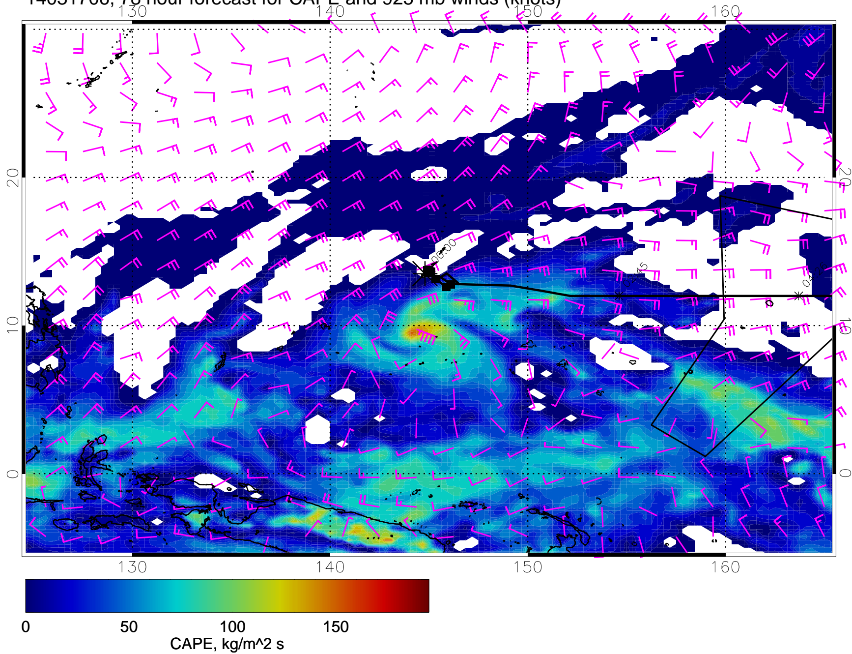
14031706, 78 hour forecast for CAPE and 925 mb winds (knots)
