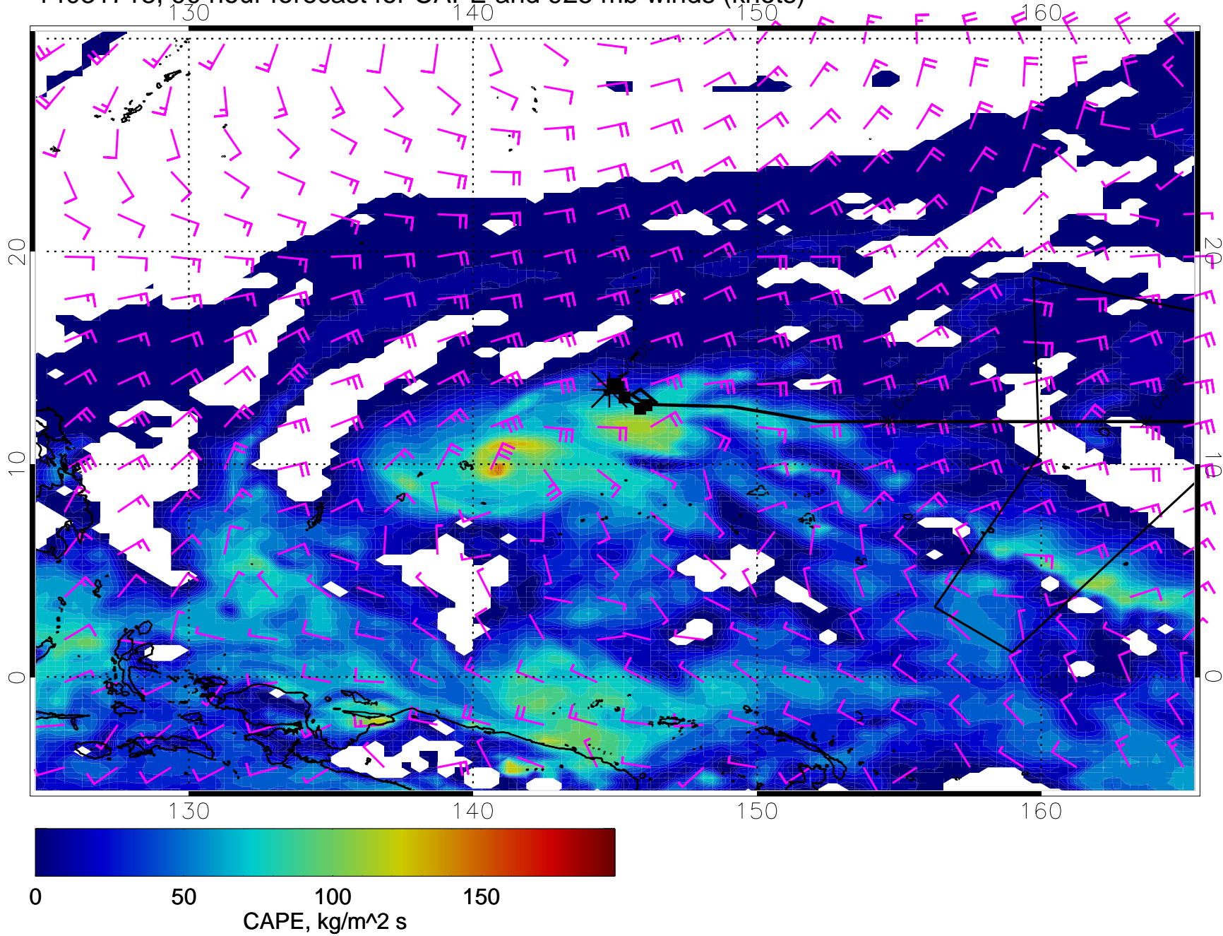
14031718, 90 hour forecast for CAPE and 925 mb winds (knots)
