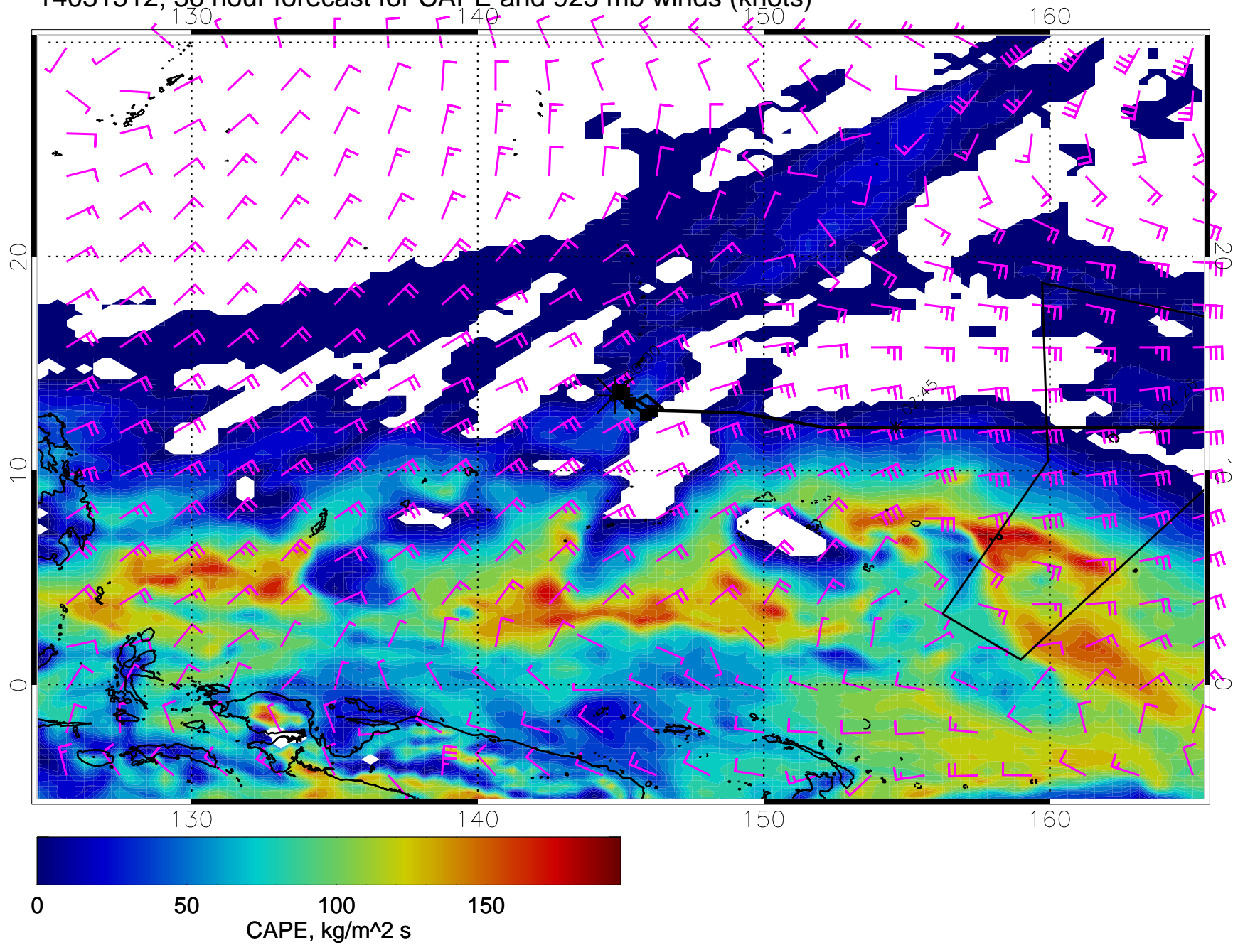
14031512, 36 hour forecast for CAPE and 925 mb winds (knots)
