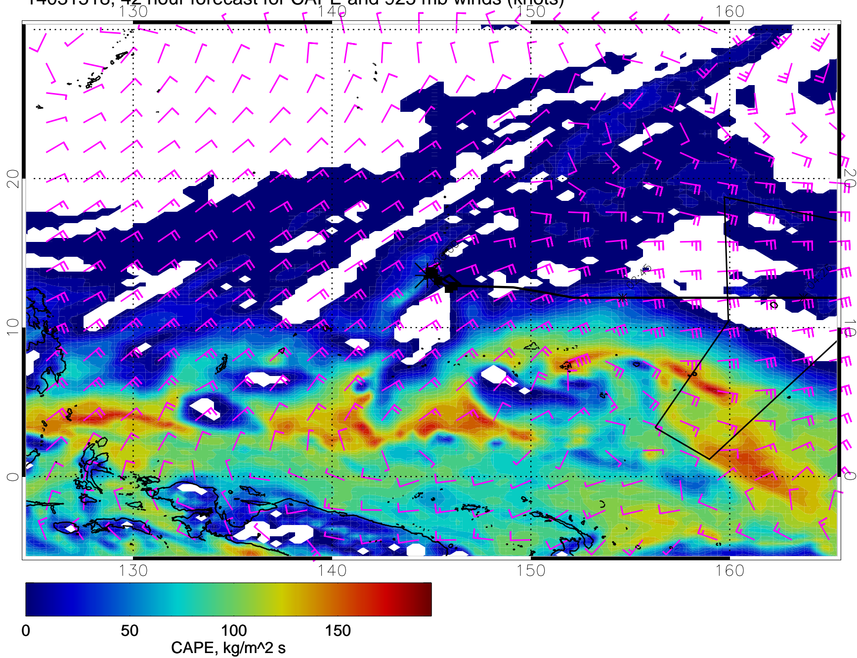
14031518, 42 hour forecast for CAPE and 925 mb winds (knots)
