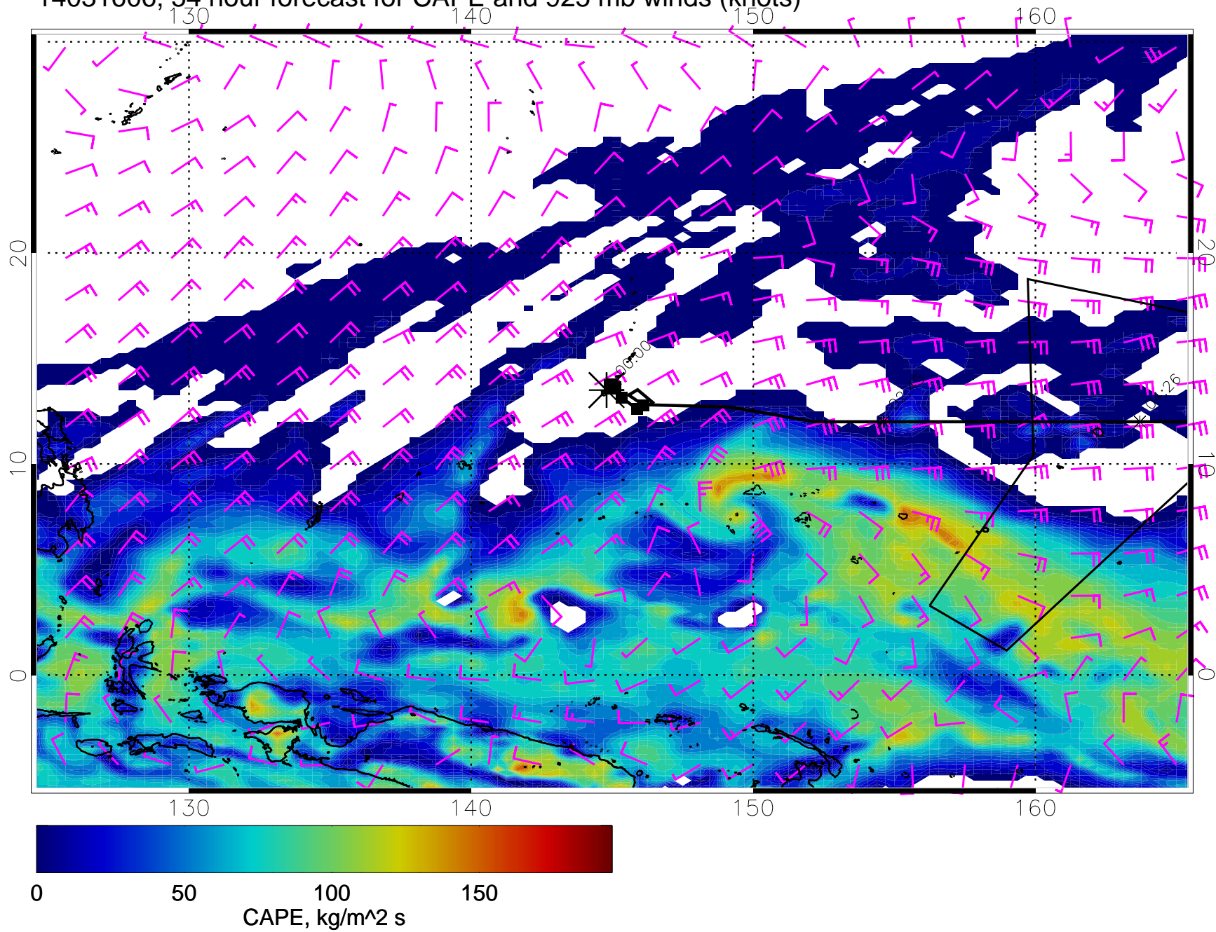
14031606, 54 hour forecast for CAPE and 925 mb winds (knots)
