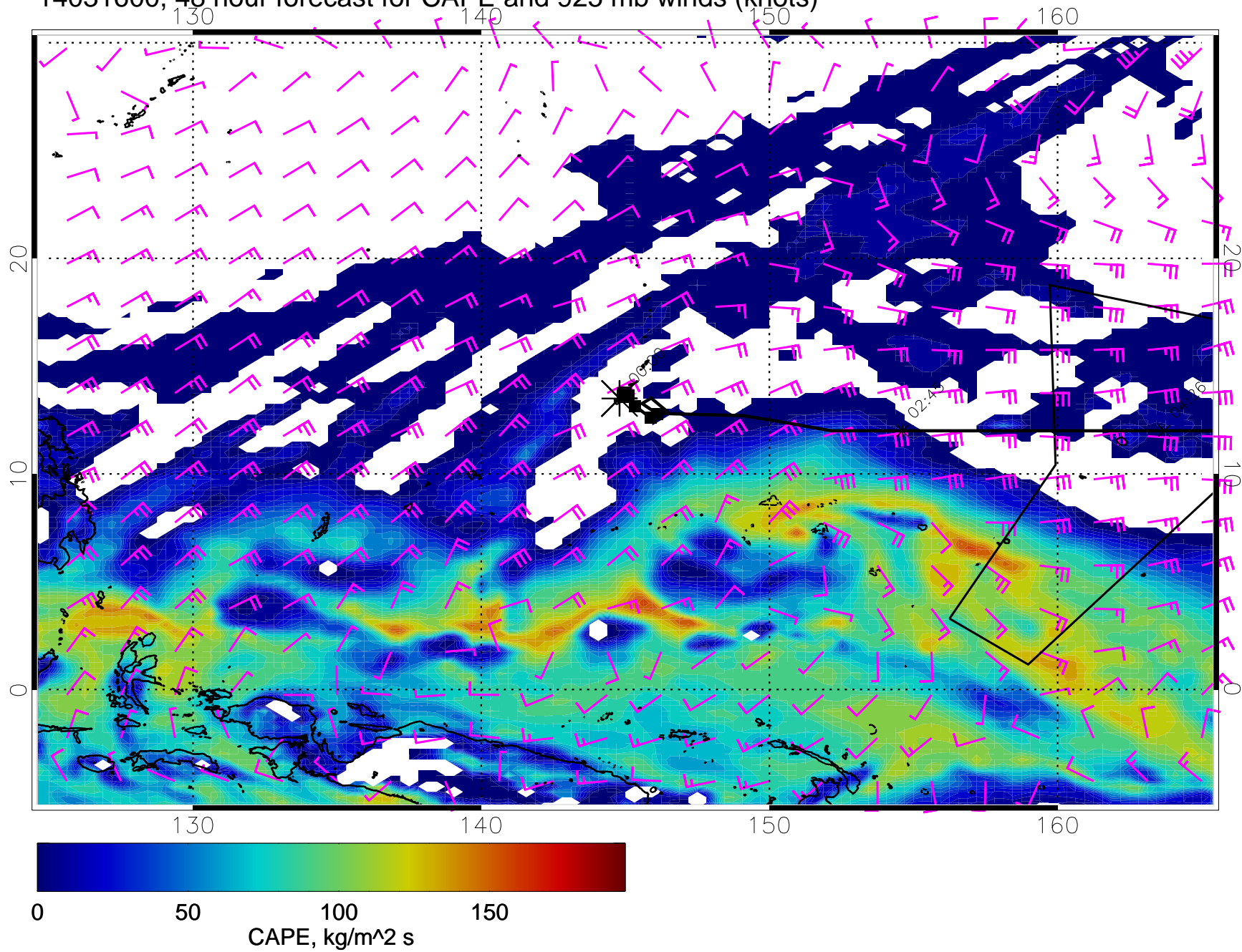
14031600, 48 hour forecast for CAPE and 925 mb winds (knots)
