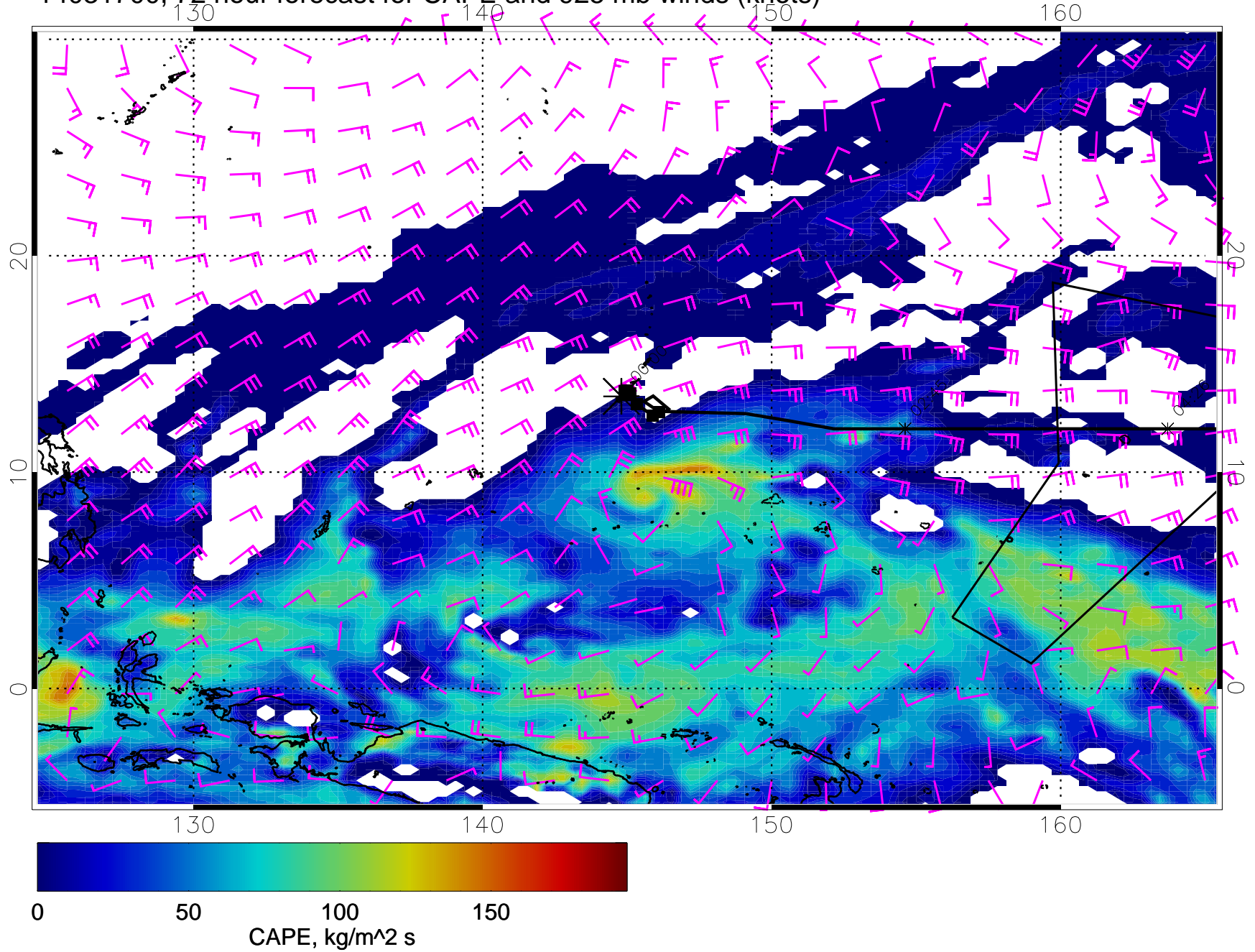
14031700, 72 hour forecast for CAPE and 925 mb winds (knots)
