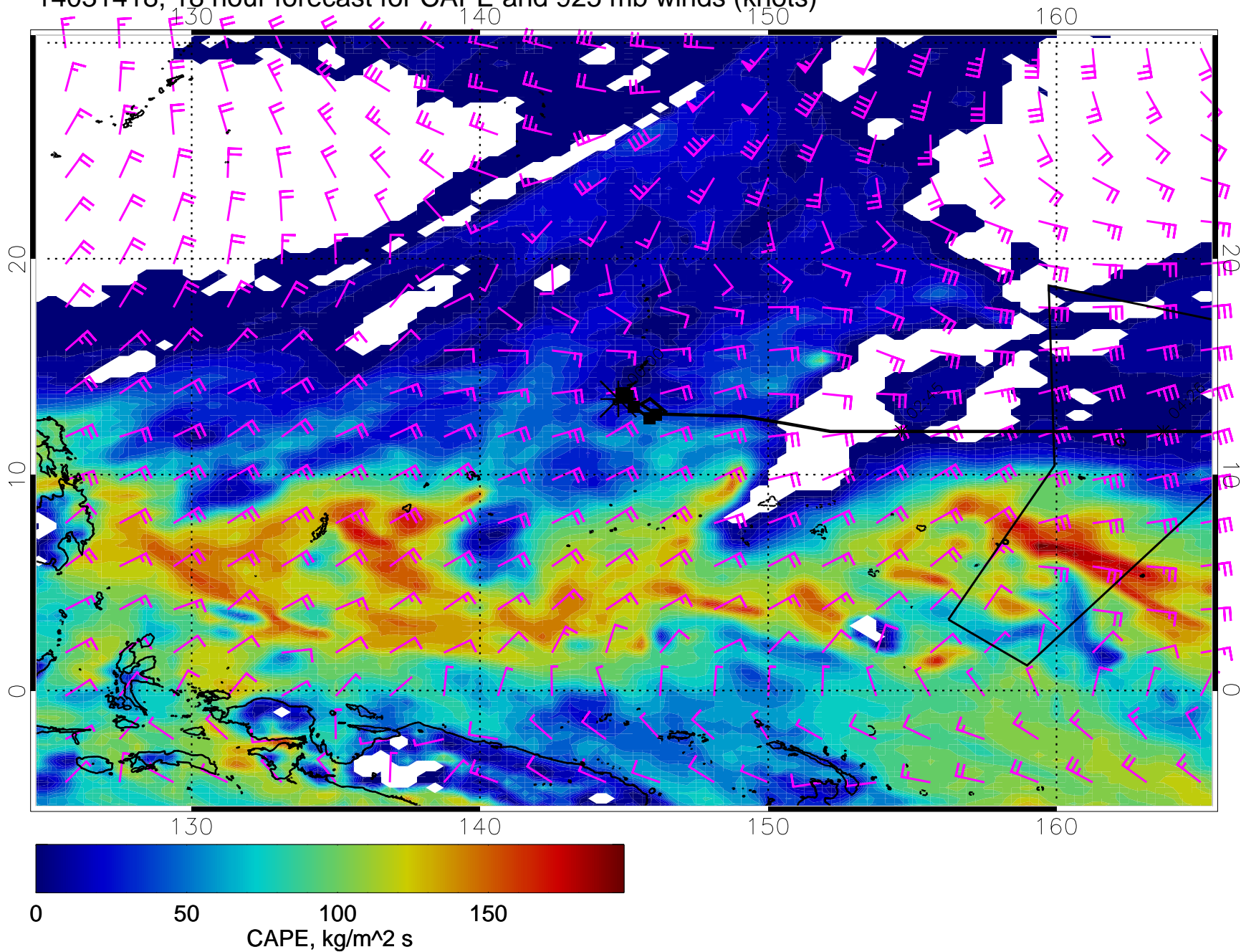
14031418, 18 hour forecast for CAPE and 925 mb winds (knots)
