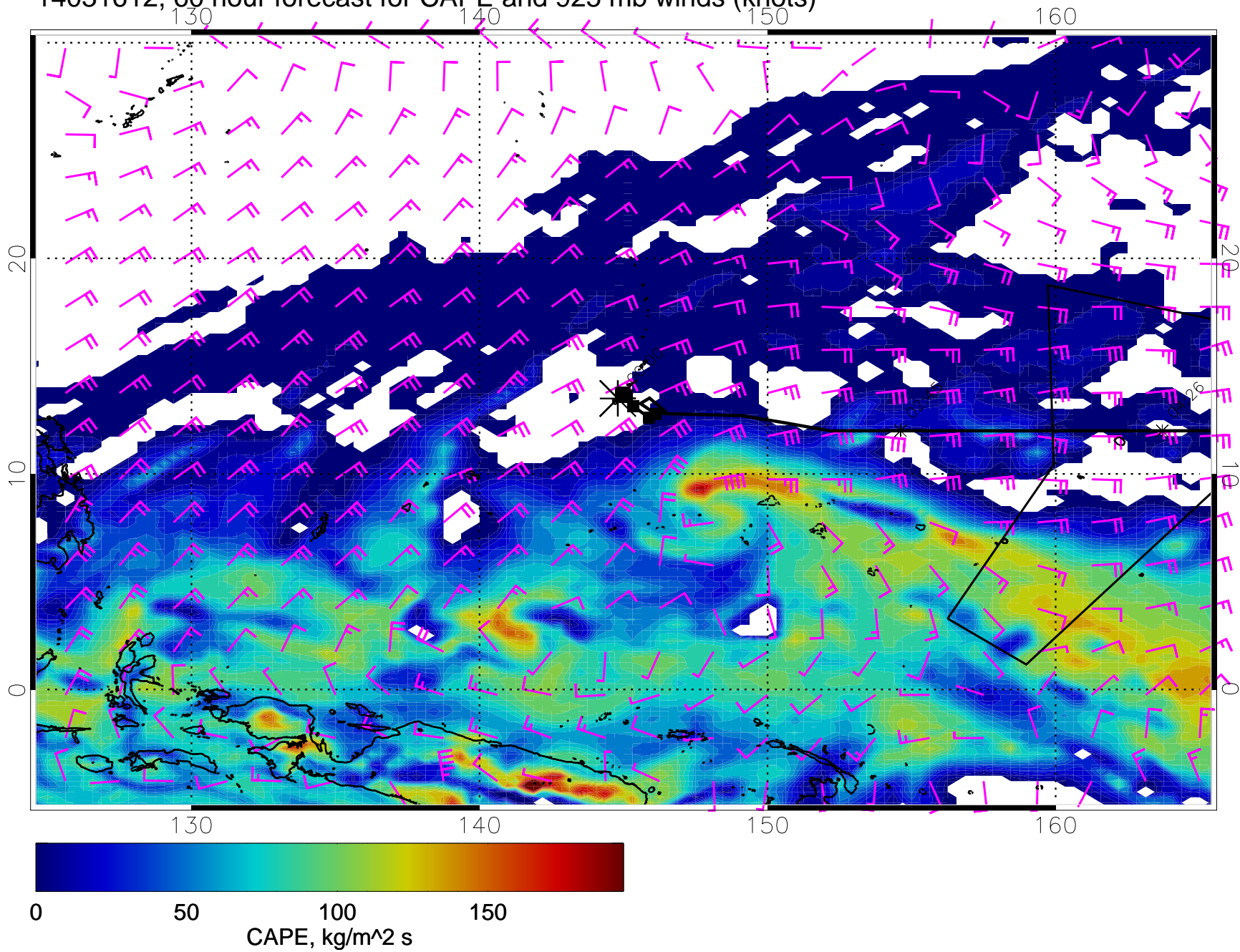
14031612, 60 hour forecast for CAPE and 925 mb winds (knots)
