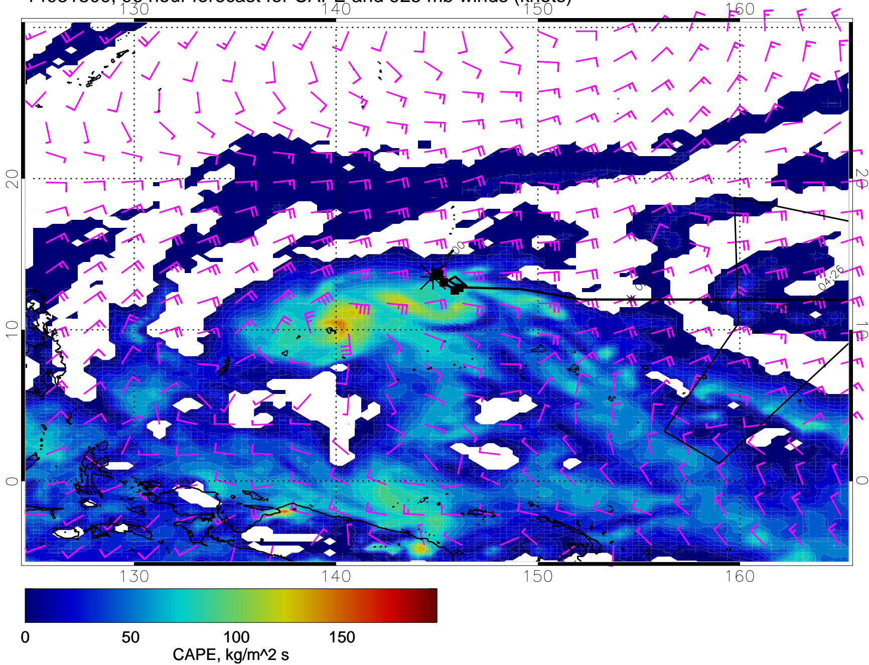
14031800, 96 hour forecast for CAPE and 925 mb winds (knots)
