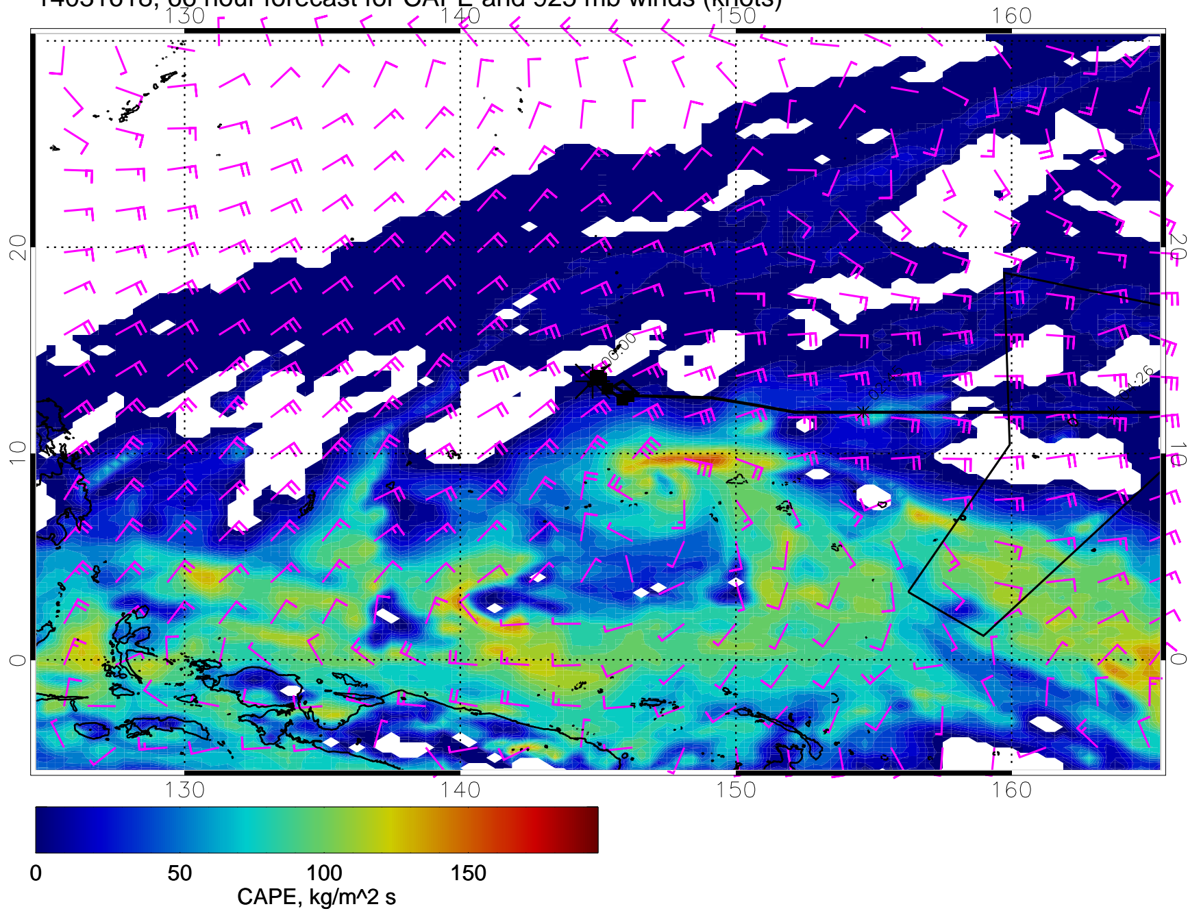
14031618, 66 hour forecast for CAPE and 925 mb winds (knots)
