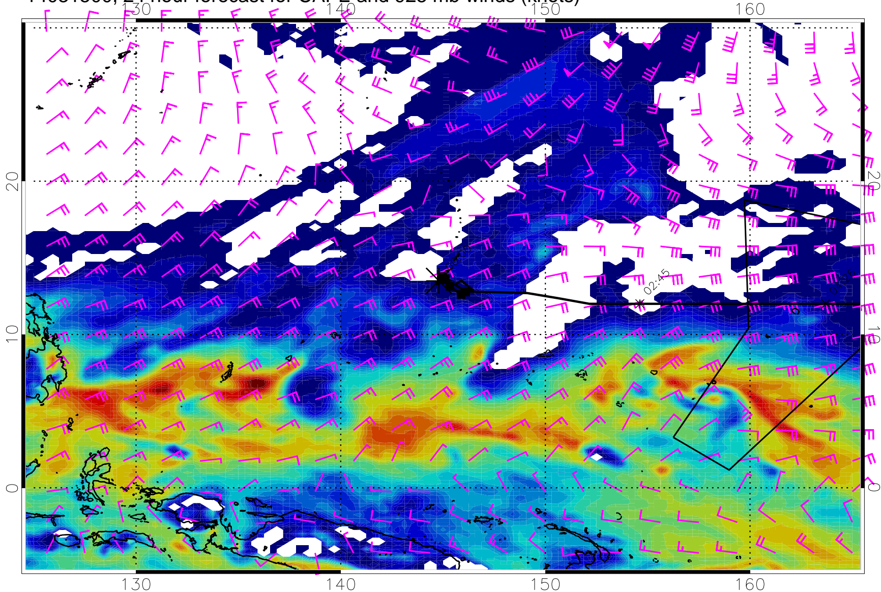
14031500, 24 hour forecast for CAPE and 925 mb winds (knots)
