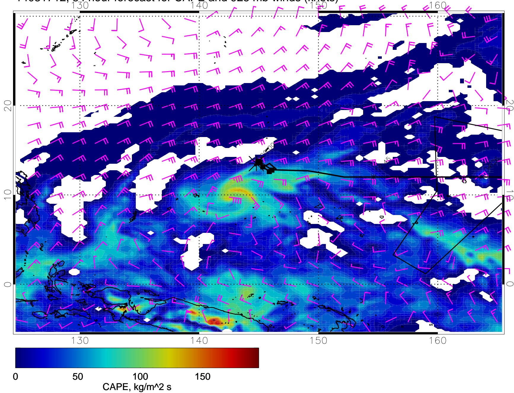
14031712, 84 hour forecast for CAPE and 925 mb winds (knots)
