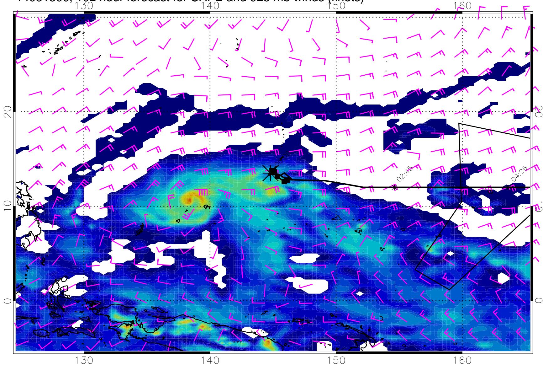
14031806, 102 hour forecast for CAPE and 925 mb winds (knots)
