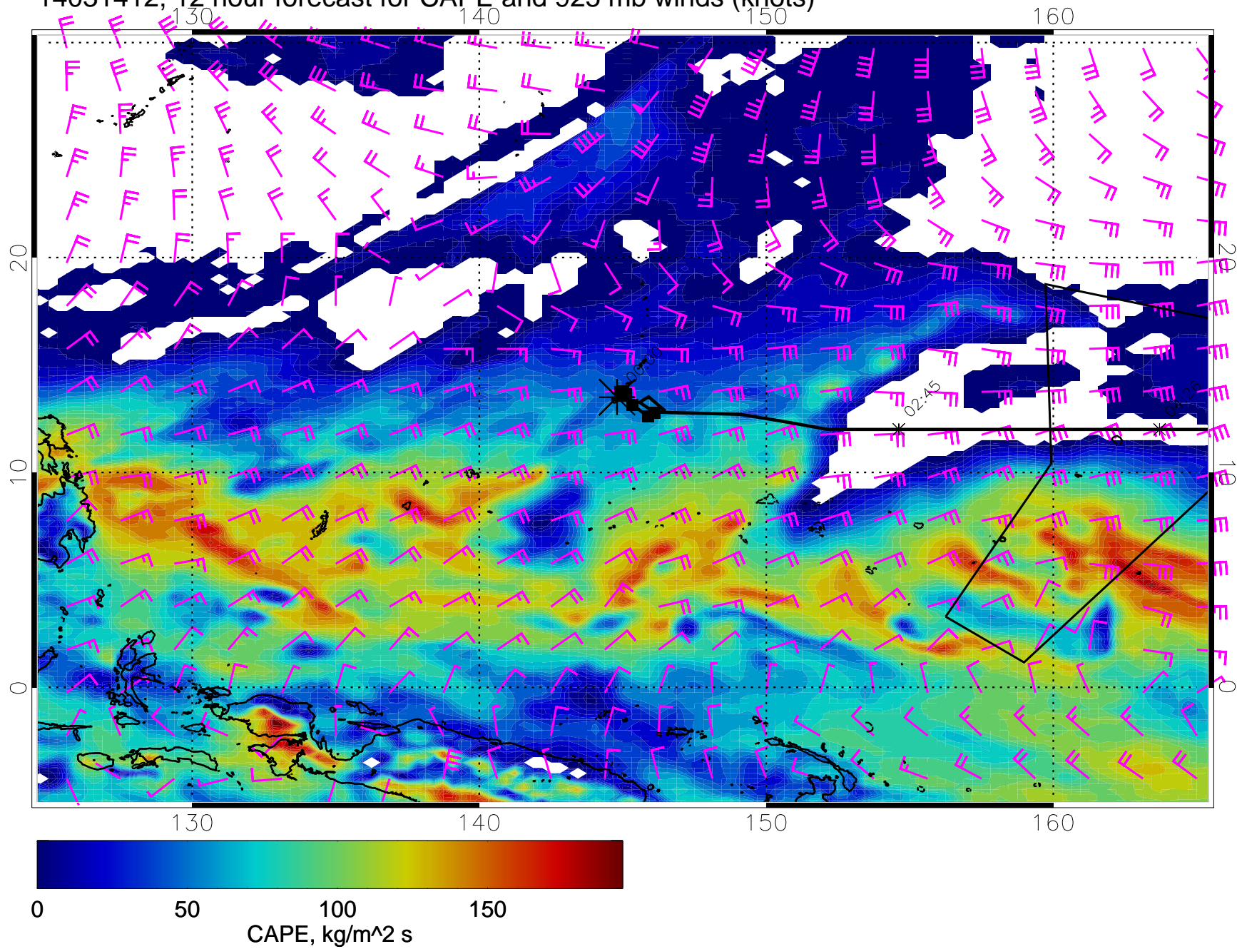
14031412, 12 hour forecast for CAPE and 925 mb winds (knots)
