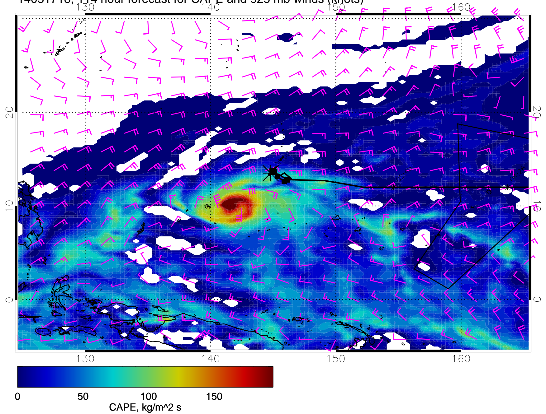
14031718, 114 hour forecast for CAPE and 925 mb winds (knots)
