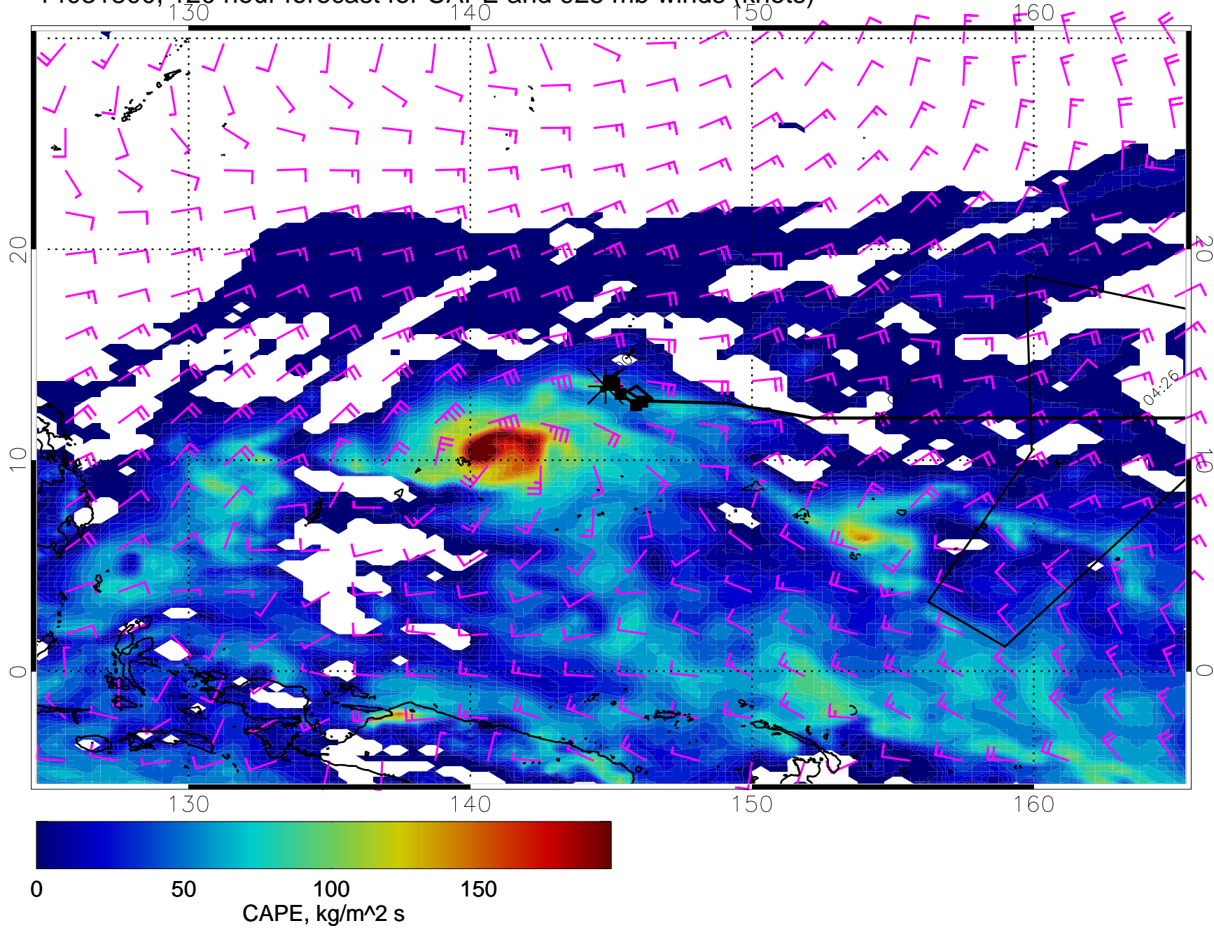
14031800, 120 hour forecast for CAPE and 925 mb winds (knots)
