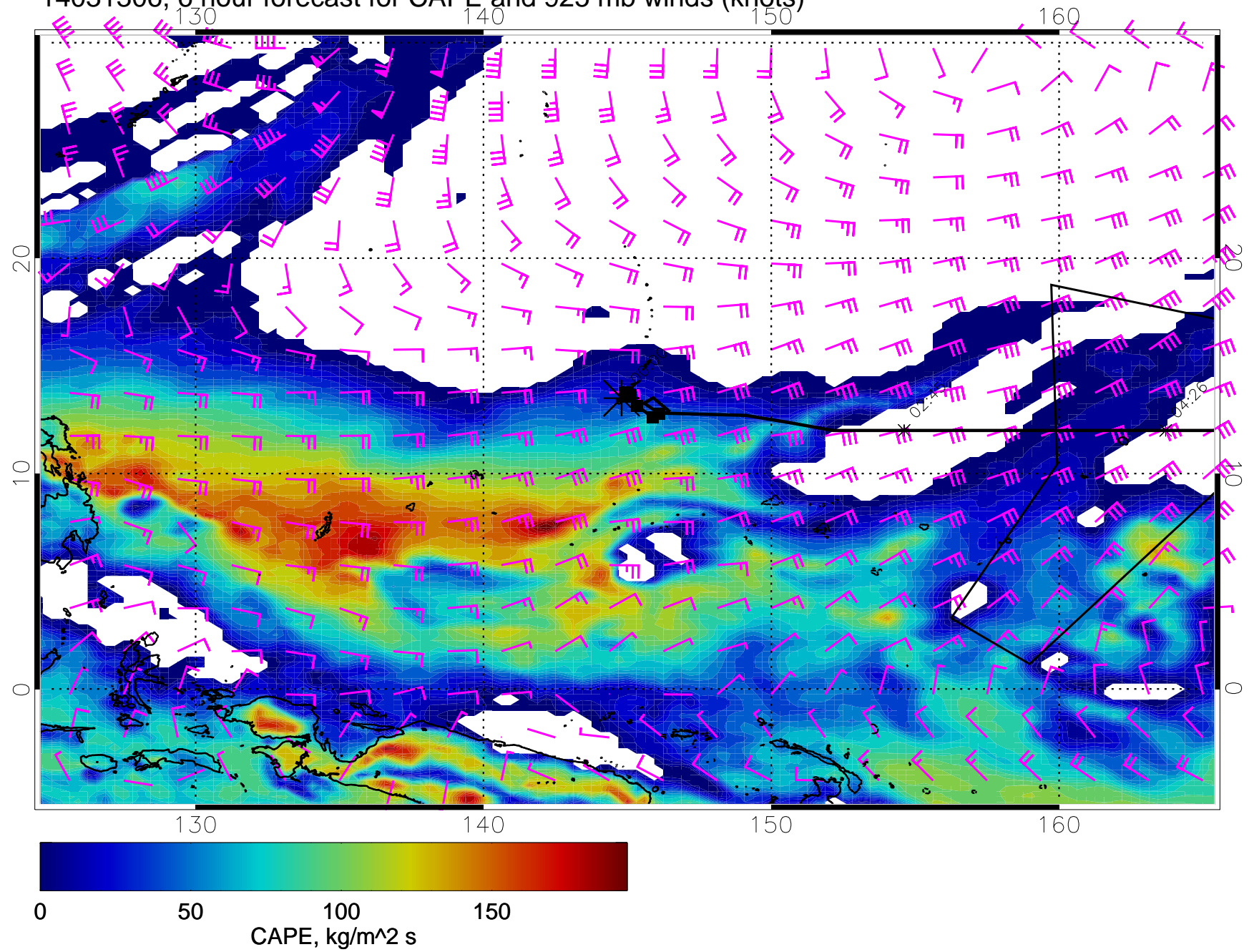
14031306, 6 hour forecast for CAPE and 925 mb winds (knots)
