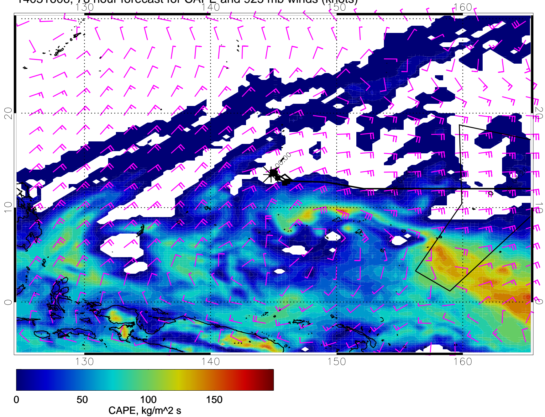
14031606, 78 hour forecast for CAPE and 925 mb winds (knots)
