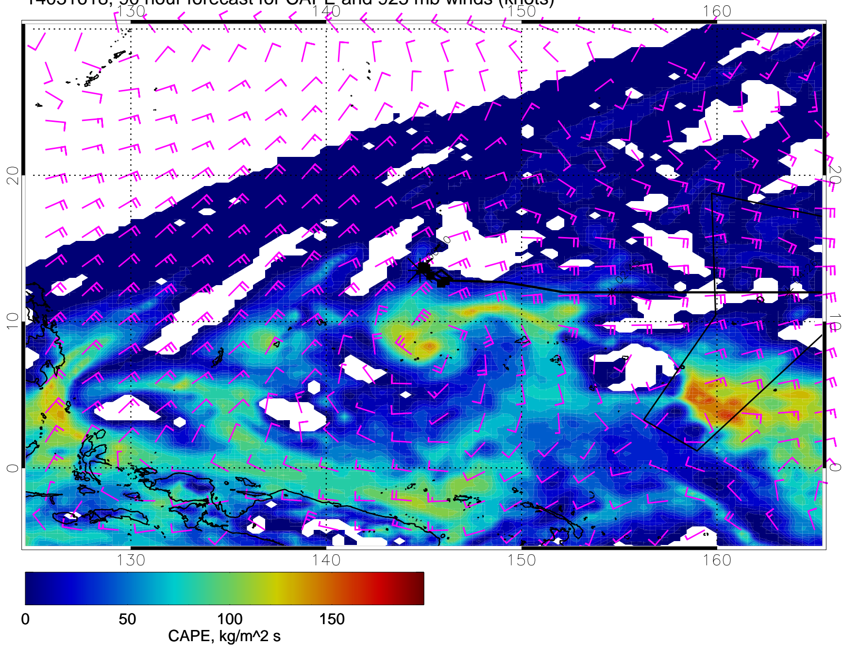
14031618, 90 hour forecast for CAPE and 925 mb winds (knots)
