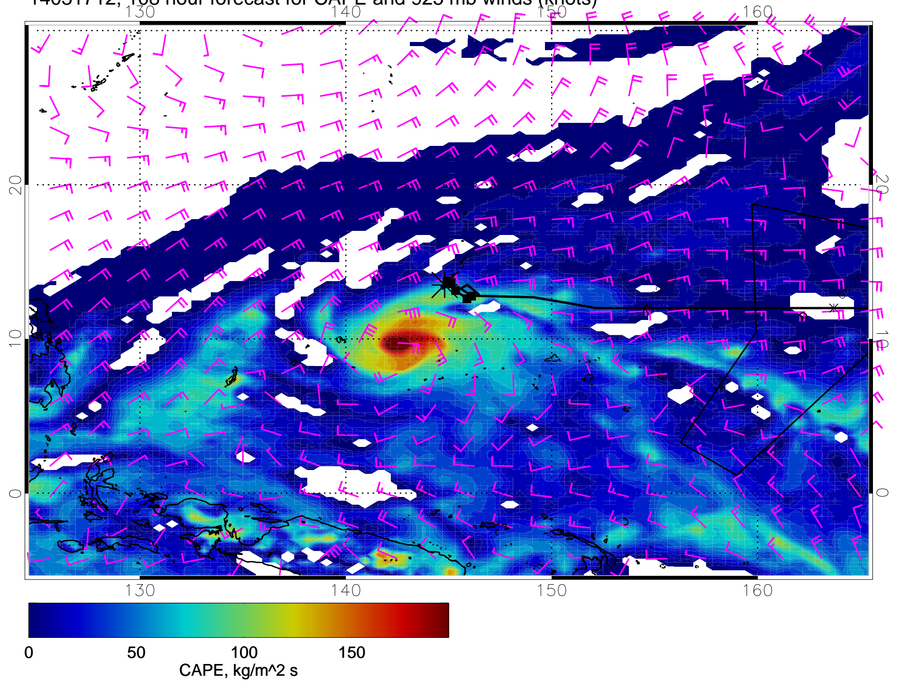
14031712, 108 hour forecast for CAPE and 925 mb winds (knots)
