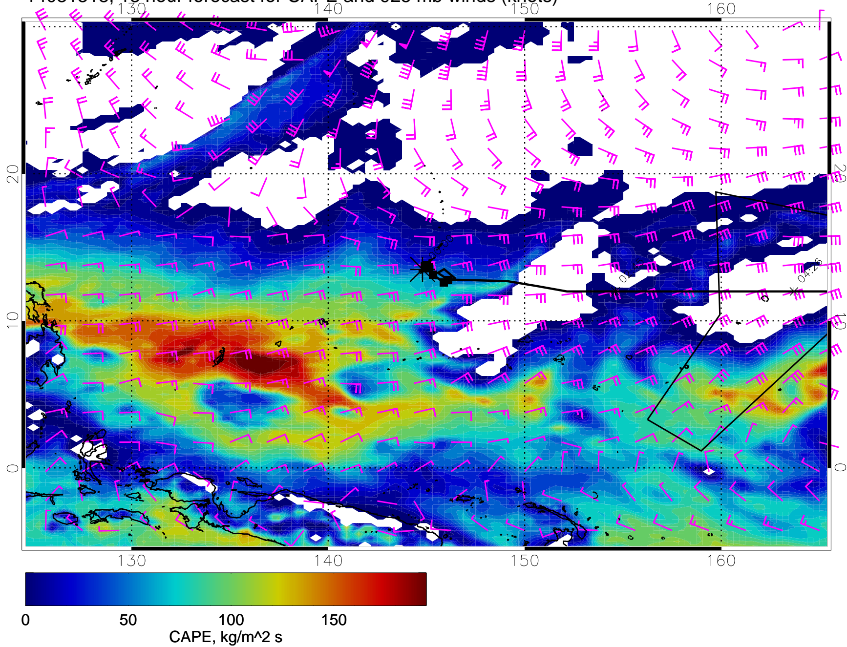
14031318, 18 hour forecast for CAPE and 925 mb winds (knots)
