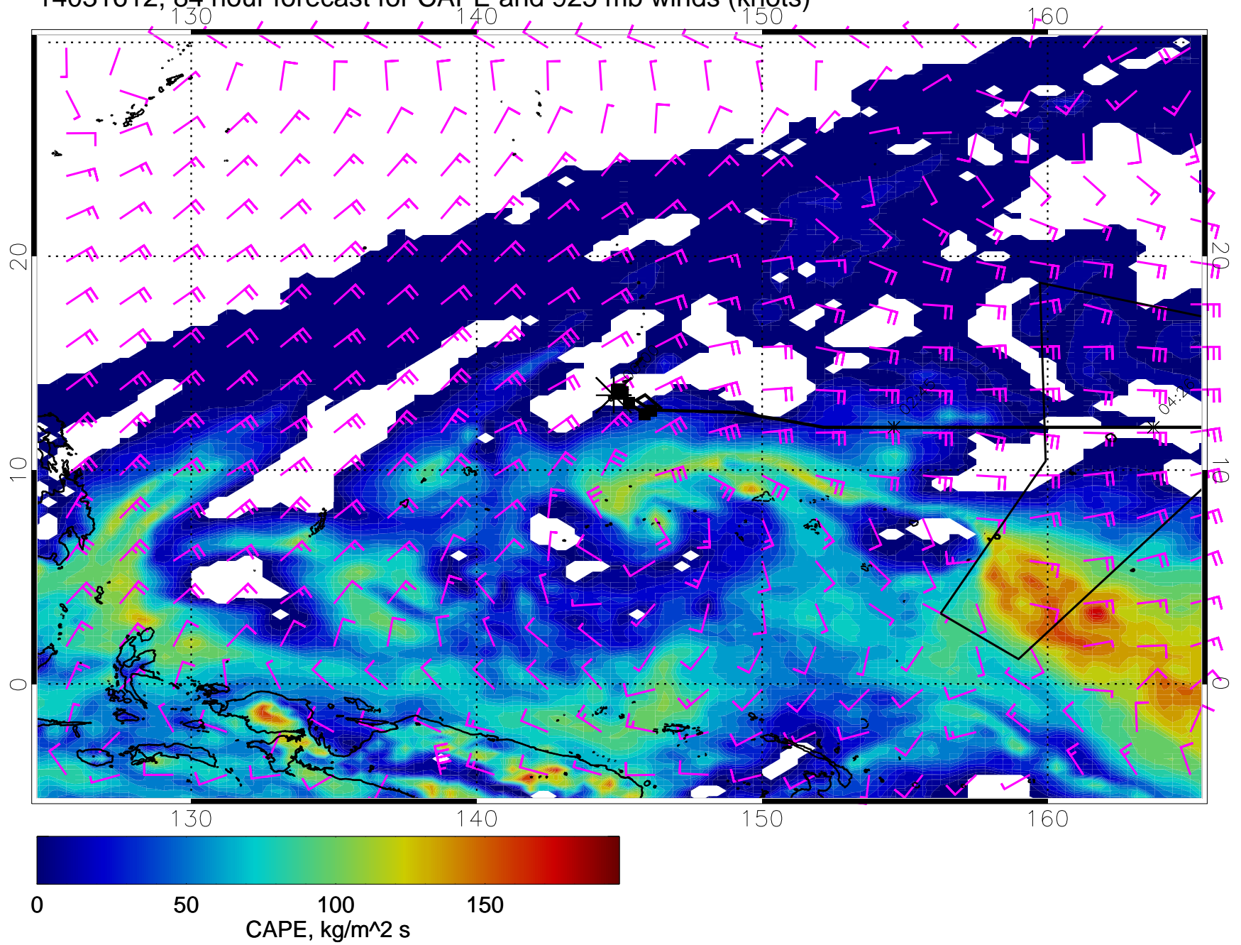
14031612, 84 hour forecast for CAPE and 925 mb winds (knots)
