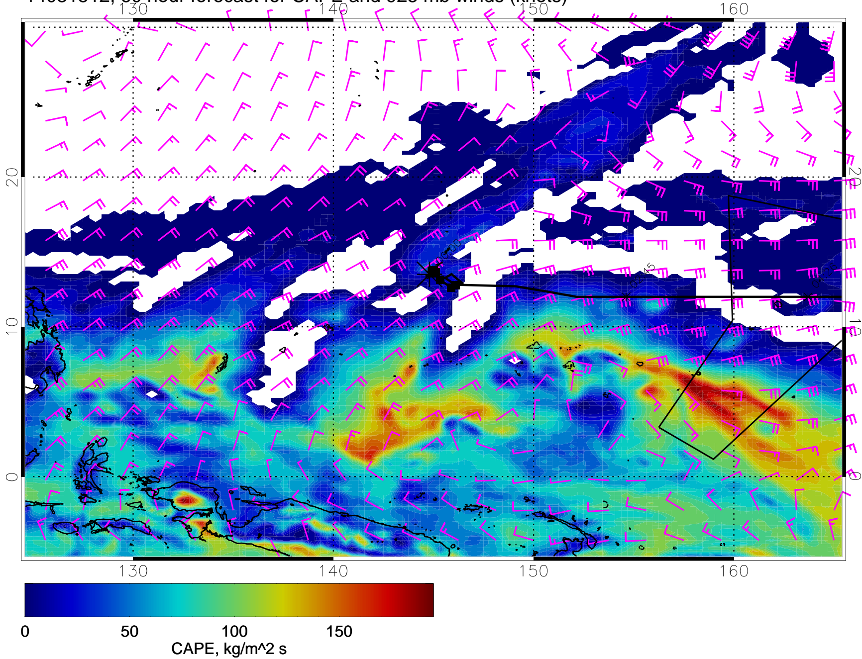
14031512, 60 hour forecast for CAPE and 925 mb winds (knots)
