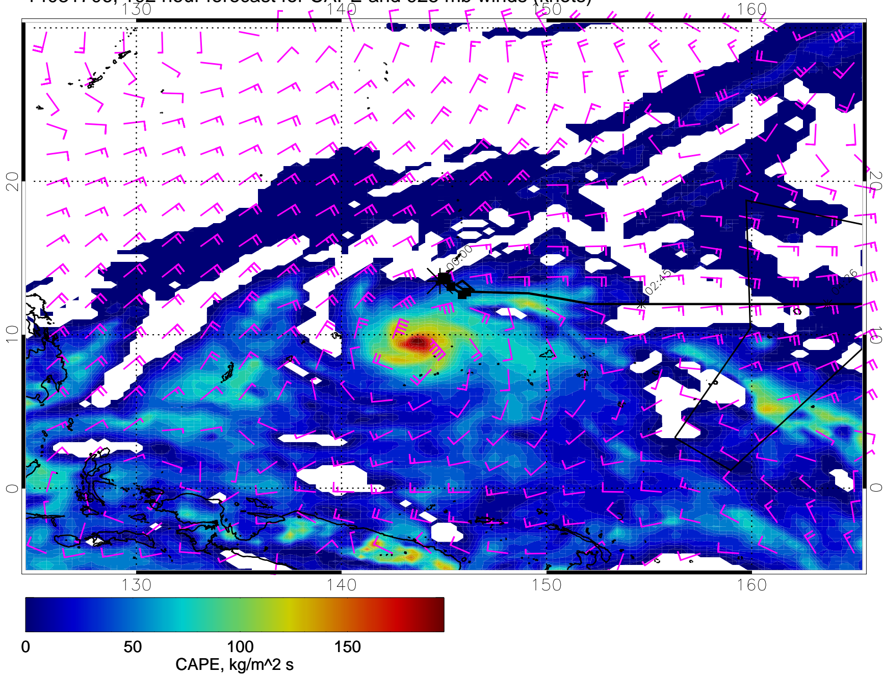
14031706, 102 hour forecast for CAPE and 925 mb winds (knots)
