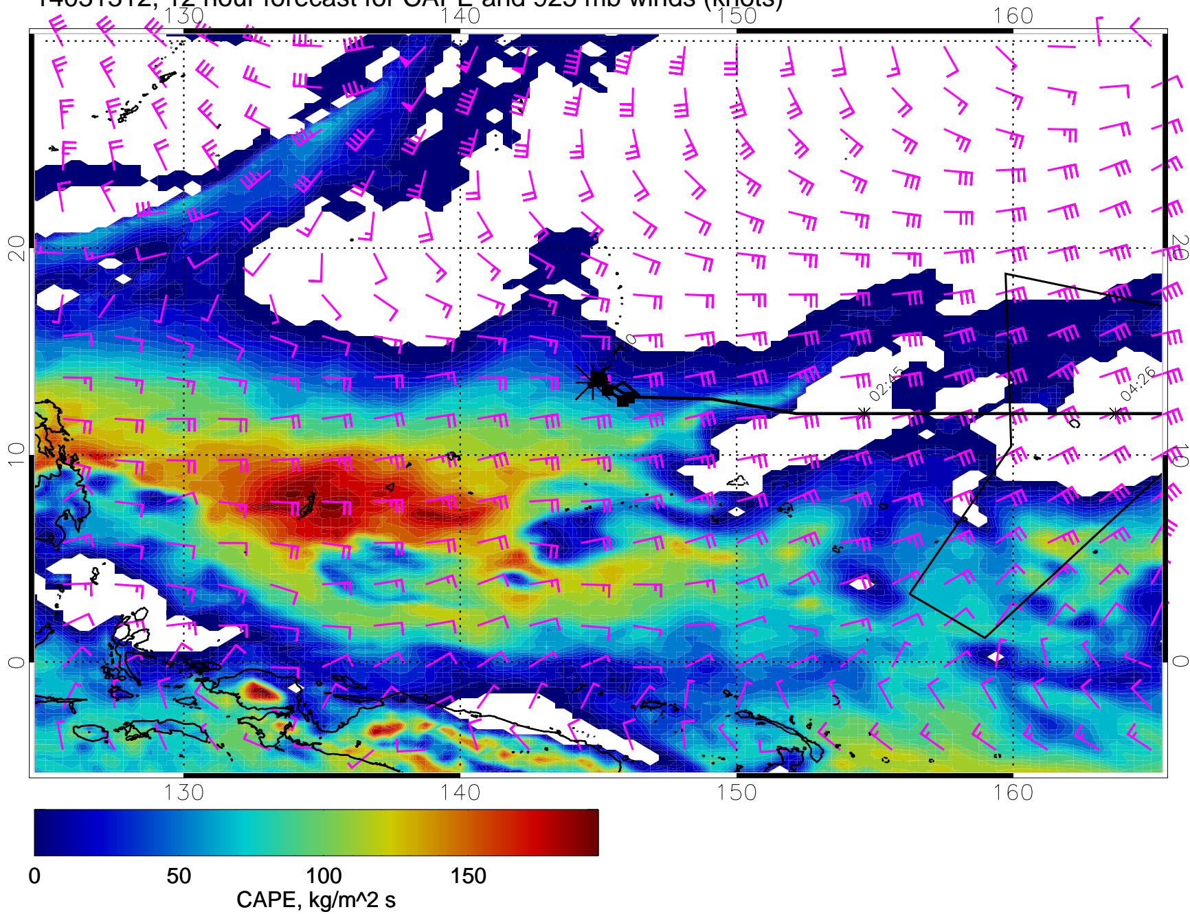
14031312, 12 hour forecast for CAPE and 925 mb winds (knots)
