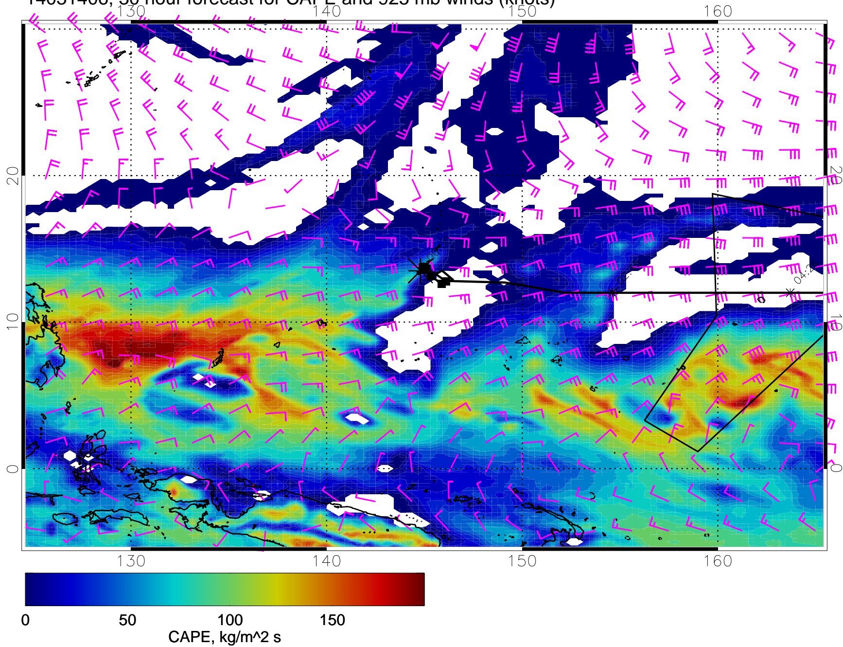
14031406, 30 hour forecast for CAPE and 925 mb winds (knots)
