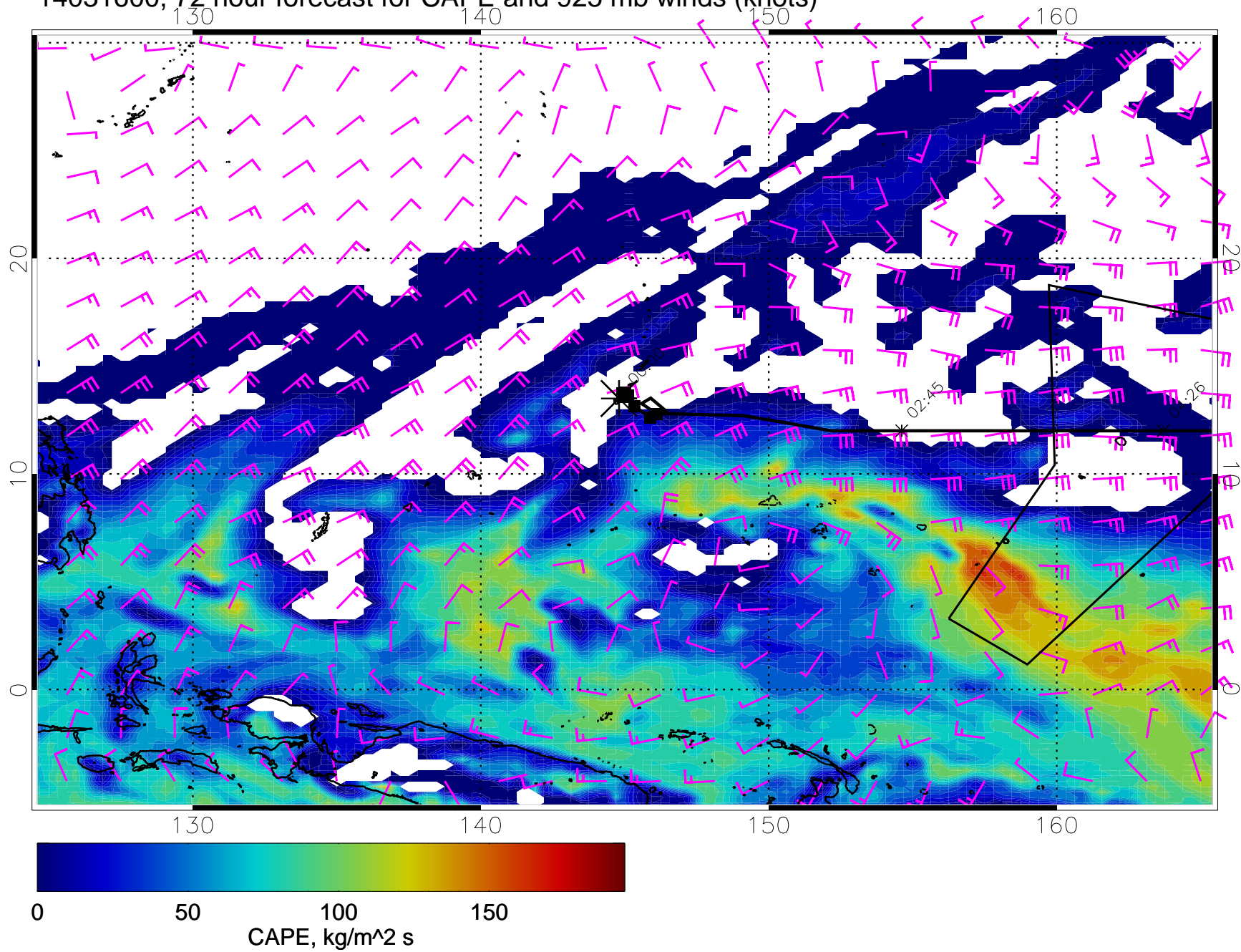
14031600, 72 hour forecast for CAPE and 925 mb winds (knots)
