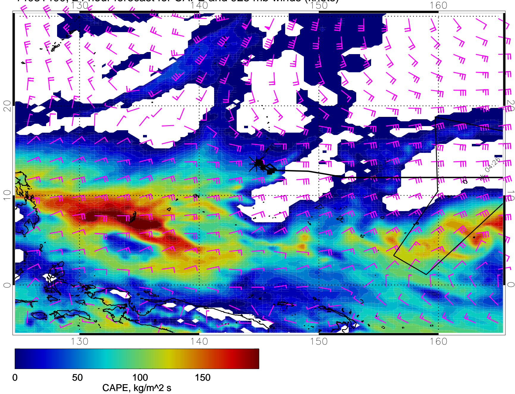
14031400, 24 hour forecast for CAPE and 925 mb winds (knots)
