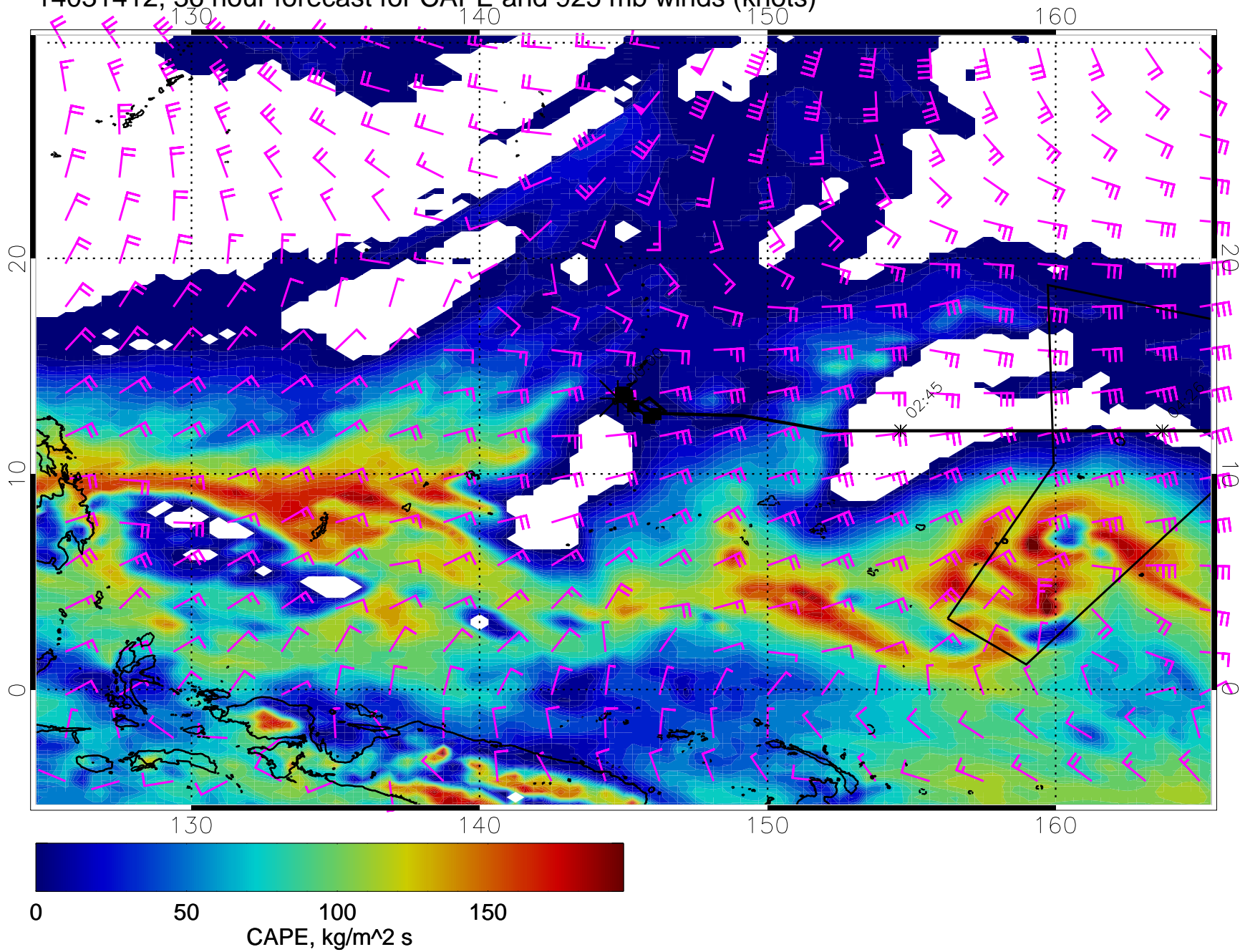
14031412, 36 hour forecast for CAPE and 925 mb winds (knots)
