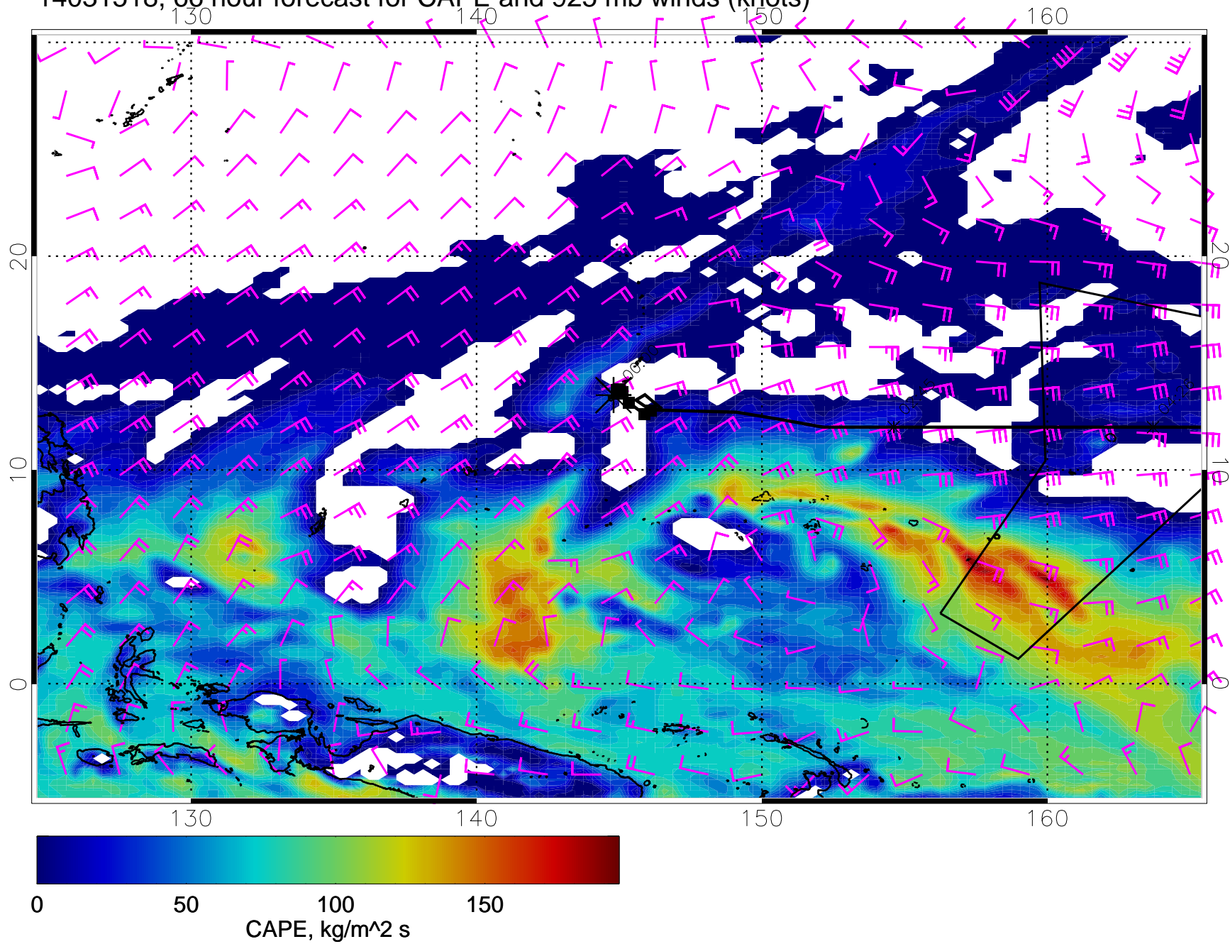
14031518, 66 hour forecast for CAPE and 925 mb winds (knots)
