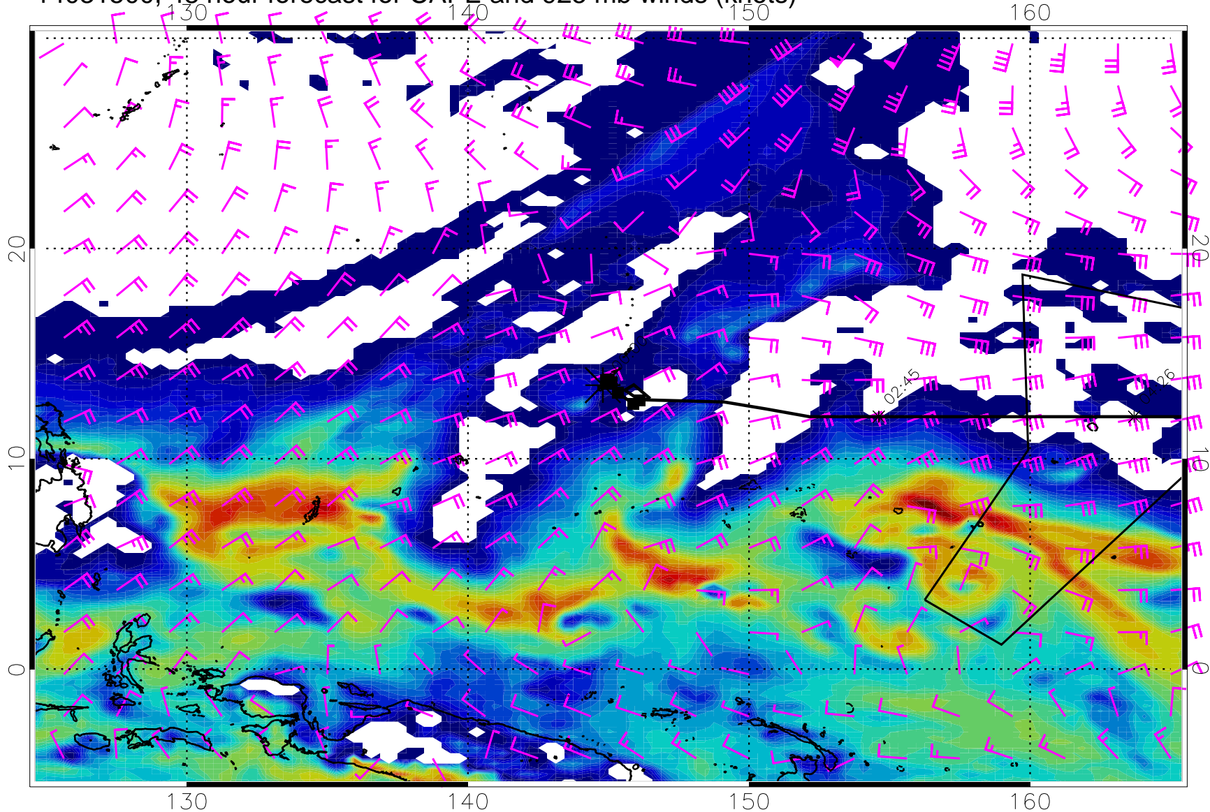
14031500, 48 hour forecast for CAPE and 925 mb winds (knots)
