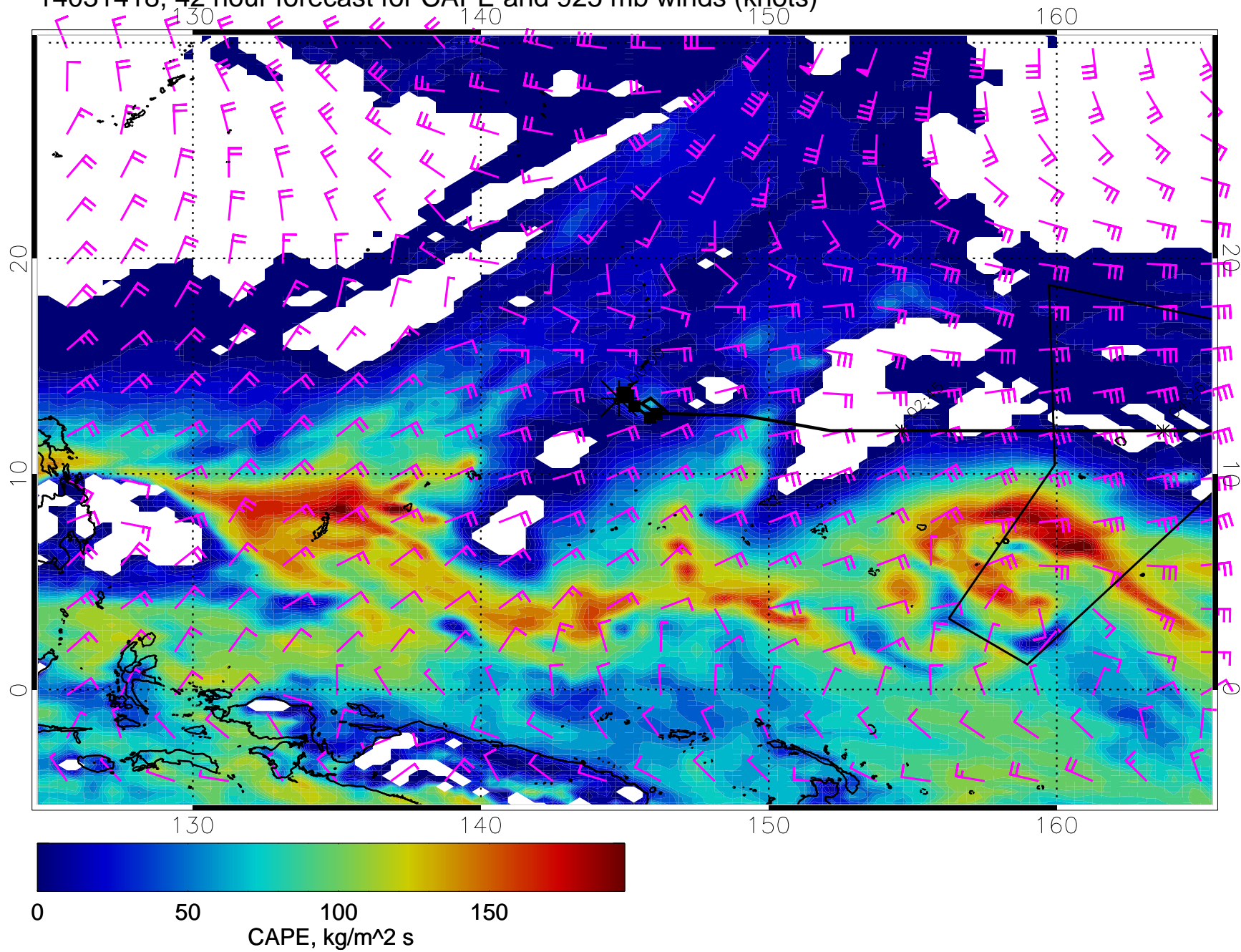
14031418, 42 hour forecast for CAPE and 925 mb winds (knots)
