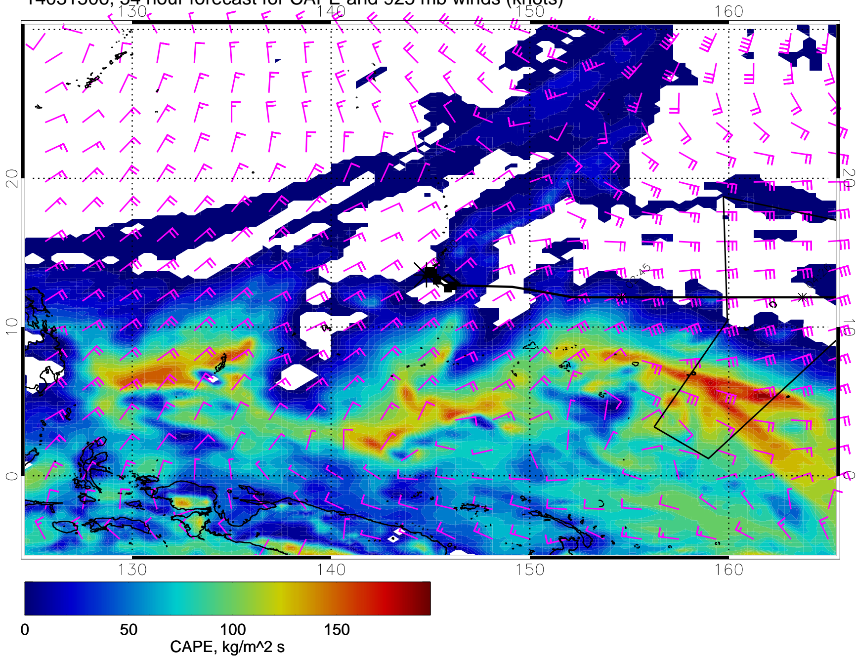
14031506, 54 hour forecast for CAPE and 925 mb winds (knots)
