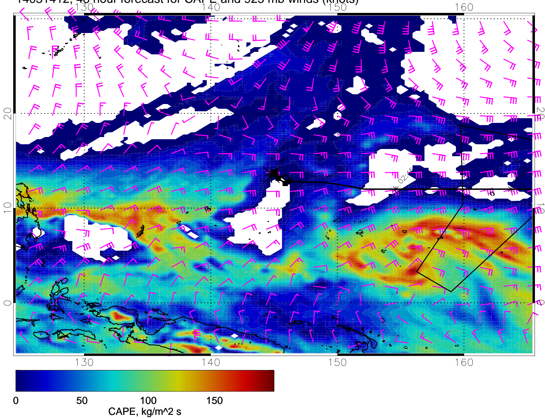
14031412, 48 hour forecast for CAPE and 925 mb winds (knots)
