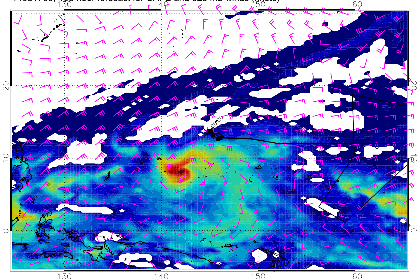
14031700, 108 hour forecast for CAPE and 925 mb winds (knots)
