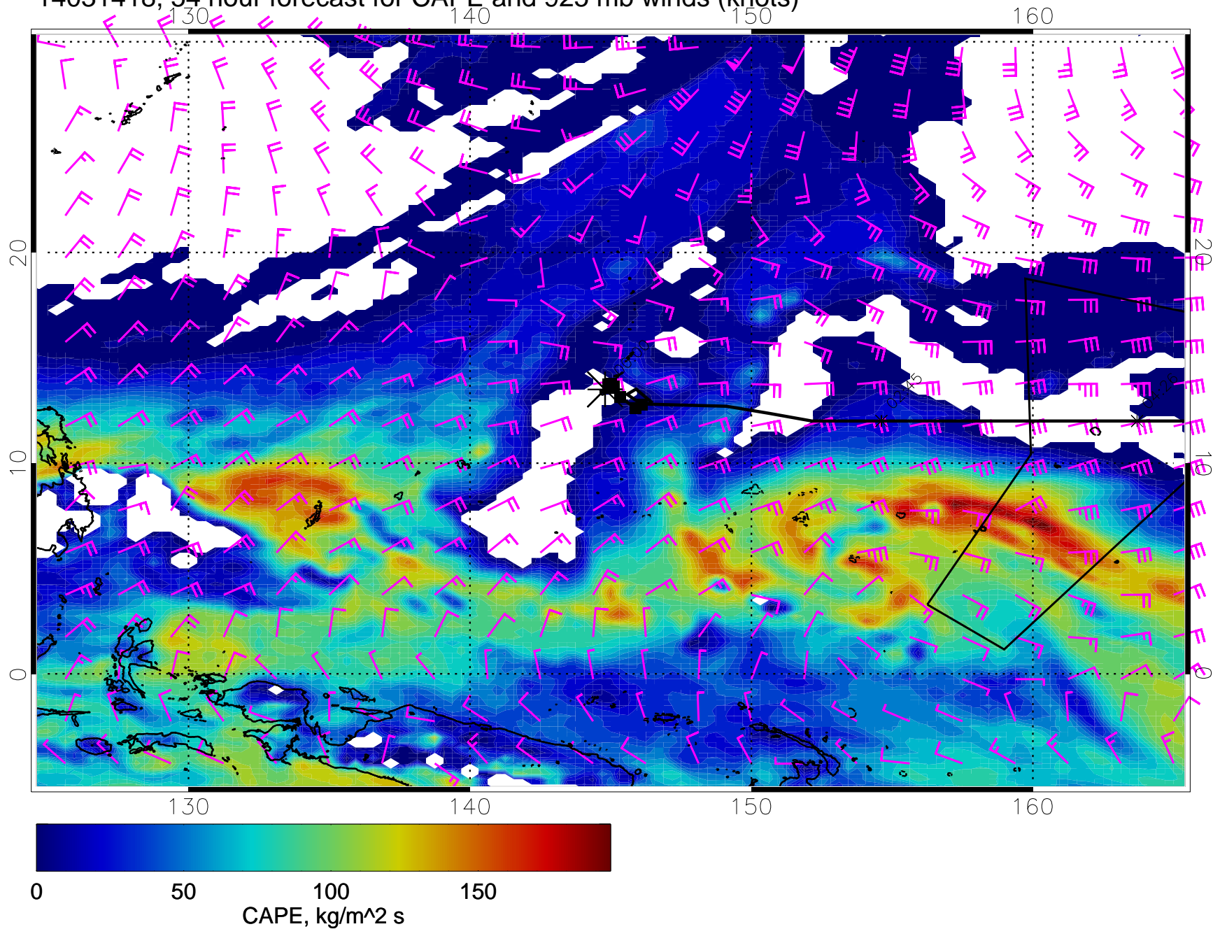
14031418, 54 hour forecast for CAPE and 925 mb winds (knots)
