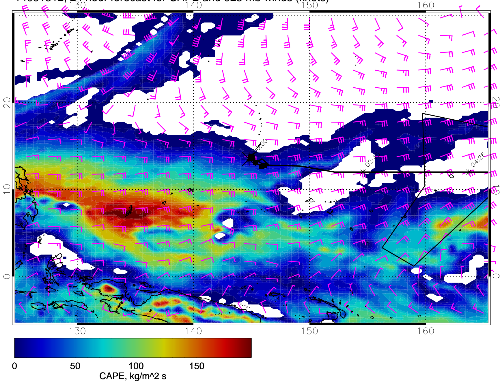
14031312, 24 hour forecast for CAPE and 925 mb winds (knots)
