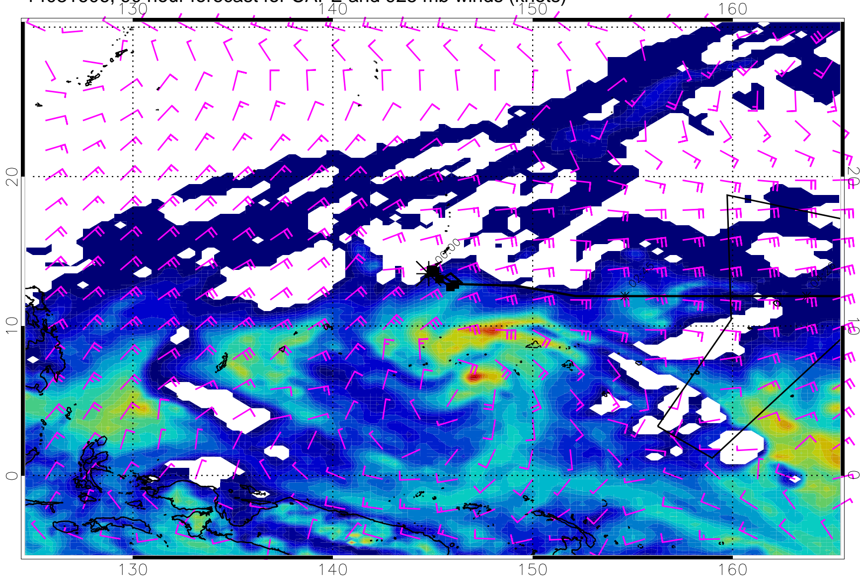
14031606, 90 hour forecast for CAPE and 925 mb winds (knots)
