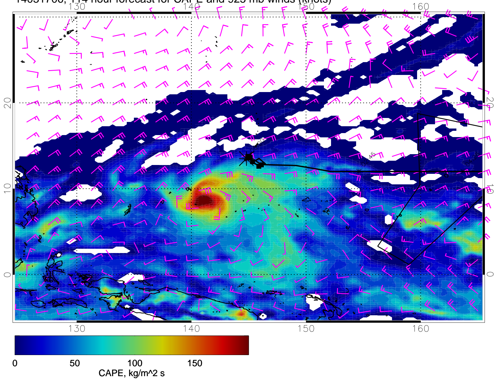
14031706, 114 hour forecast for CAPE and 925 mb winds (knots)
