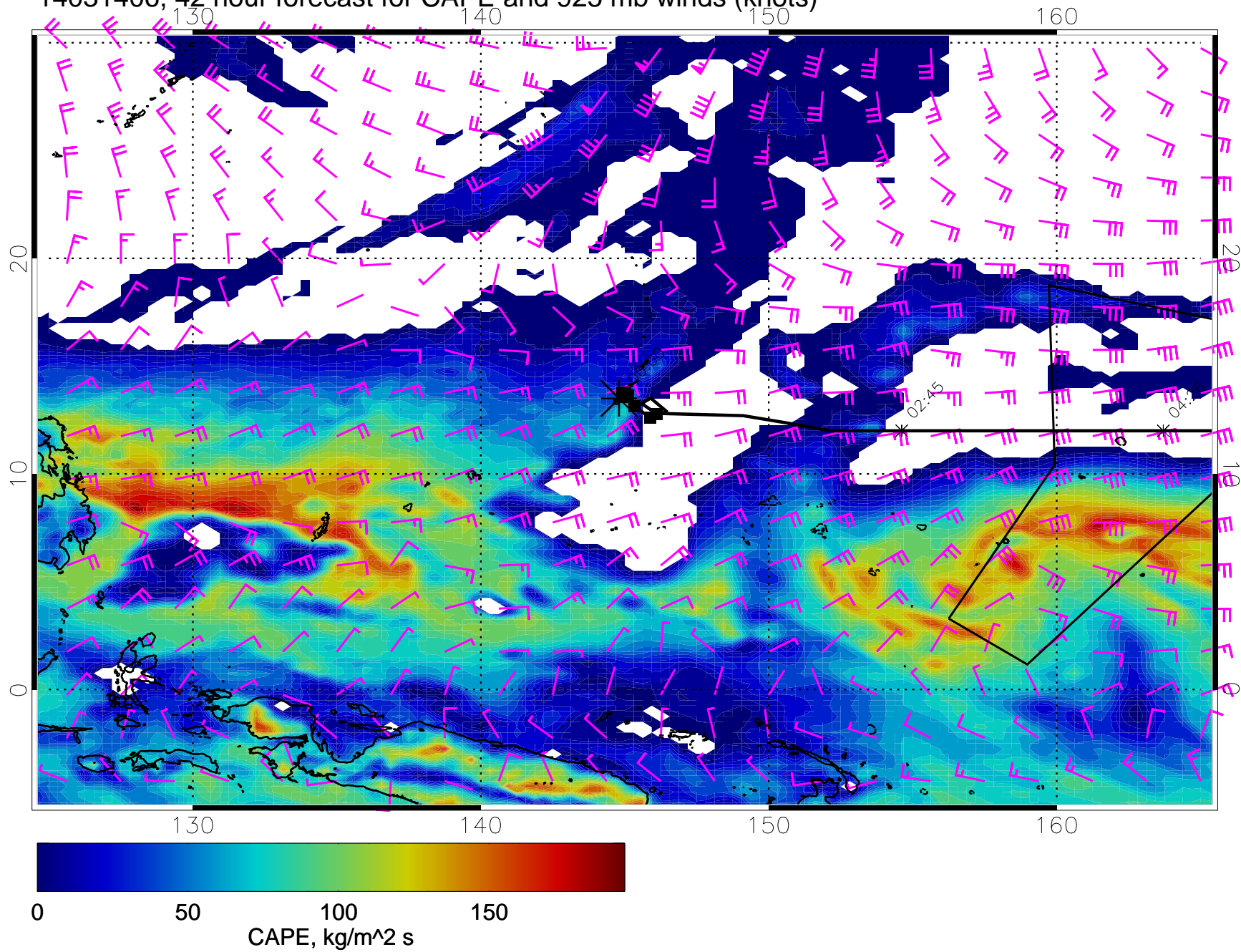
14031406, 42 hour forecast for CAPE and 925 mb winds (knots)
