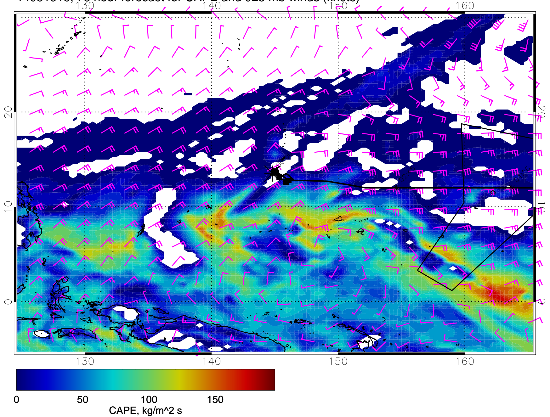
14031518, 78 hour forecast for CAPE and 925 mb winds (knots)
