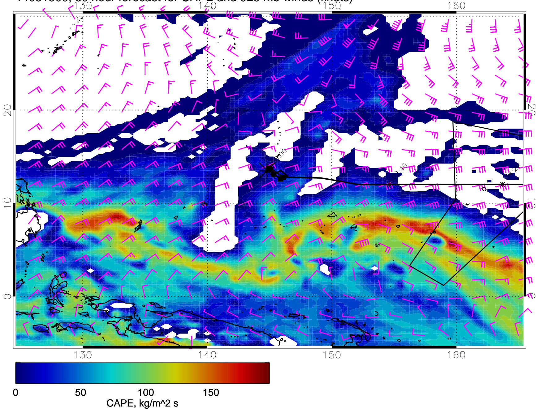
14031500, 60 hour forecast for CAPE and 925 mb winds (knots)
