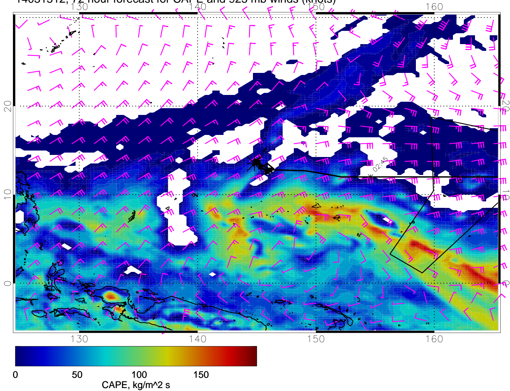
14031512, 72 hour forecast for CAPE and 925 mb winds (knots)
