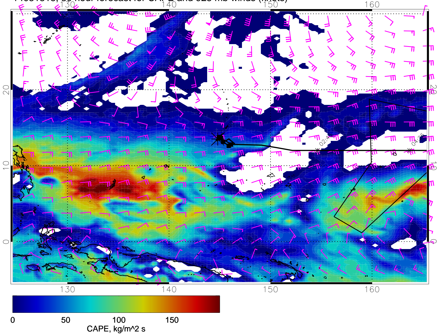
14031318, 30 hour forecast for CAPE and 925 mb winds (knots)
