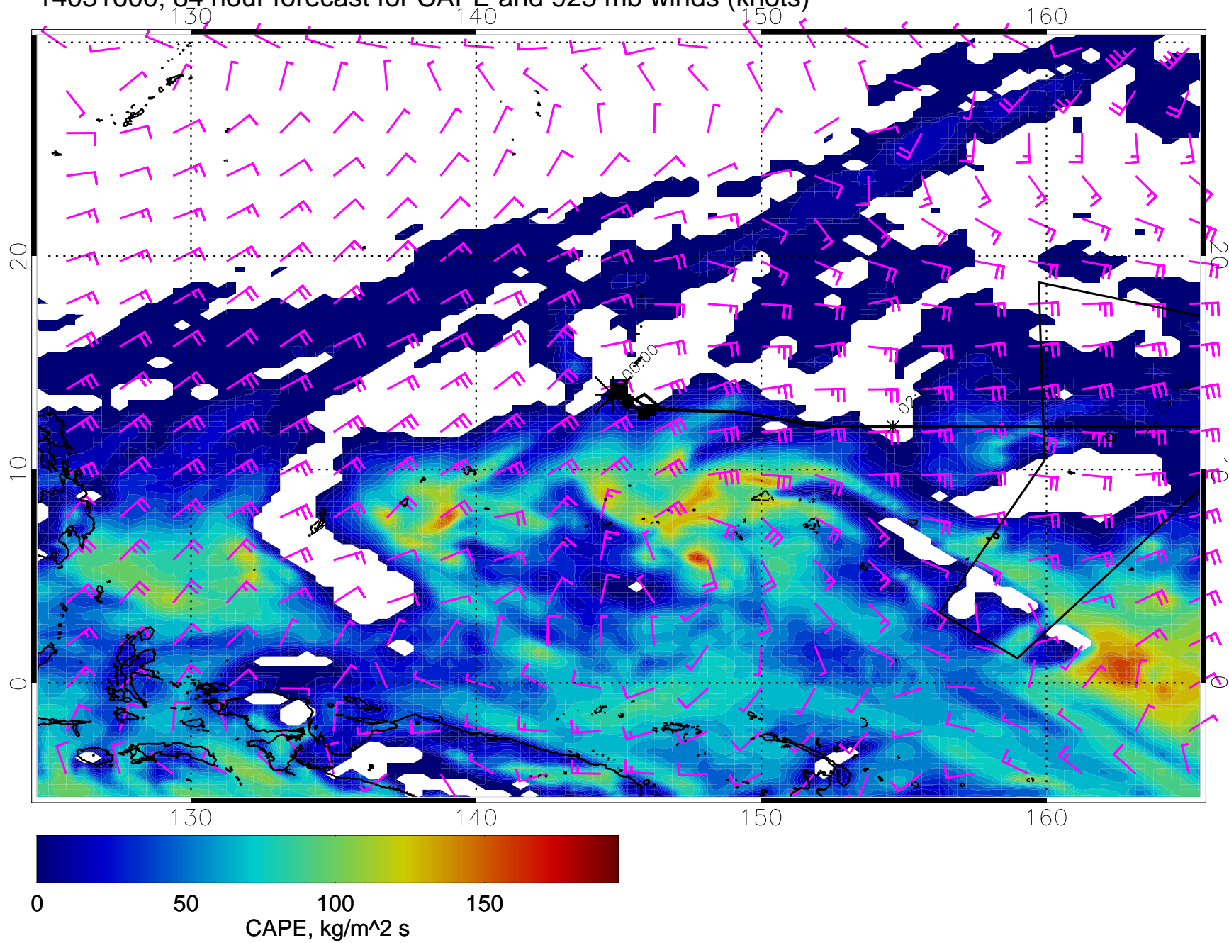
14031600, 84 hour forecast for CAPE and 925 mb winds (knots)
