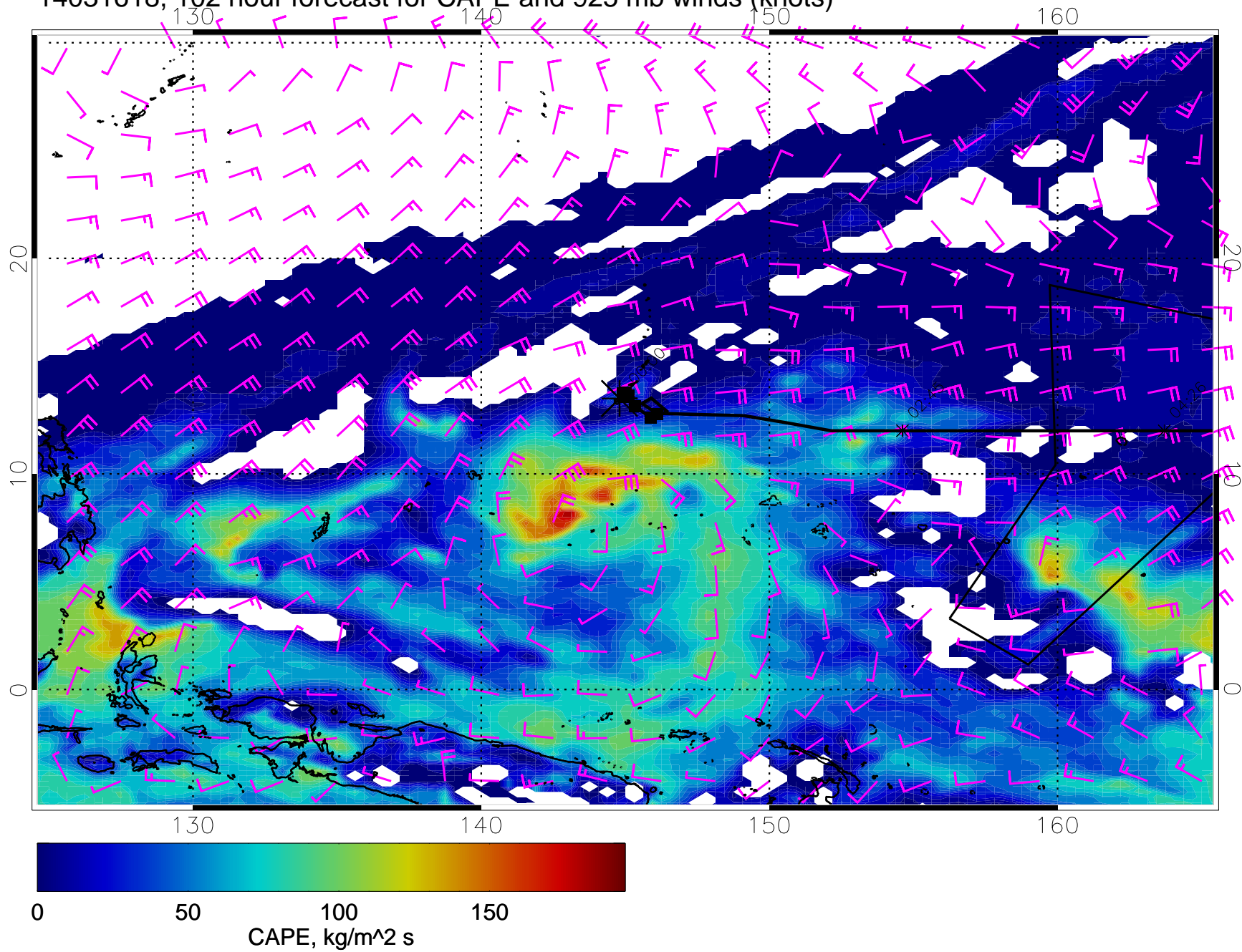
14031618, 102 hour forecast for CAPE and 925 mb winds (knots)
