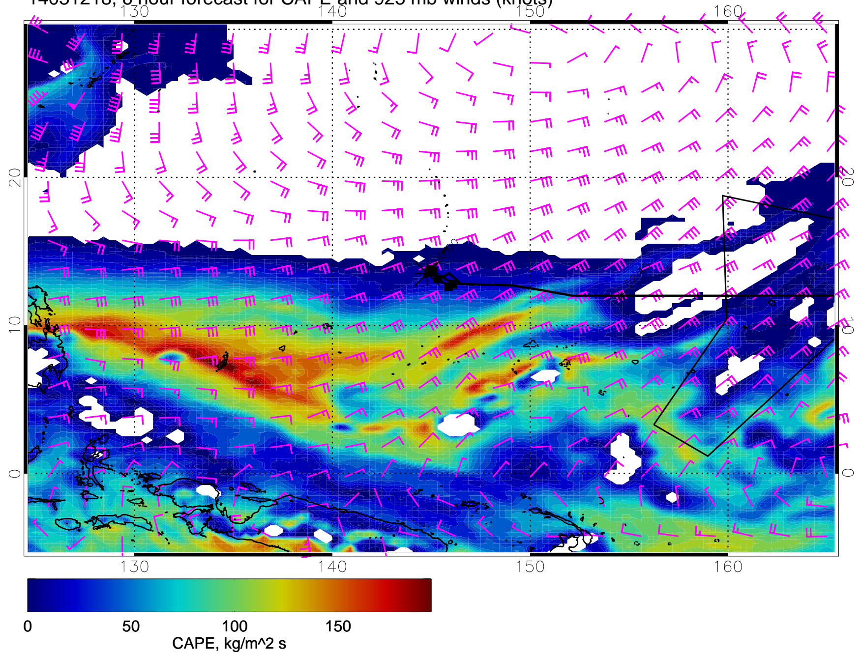
14031218, 6 hour forecast for CAPE and 925 mb winds (knots)
