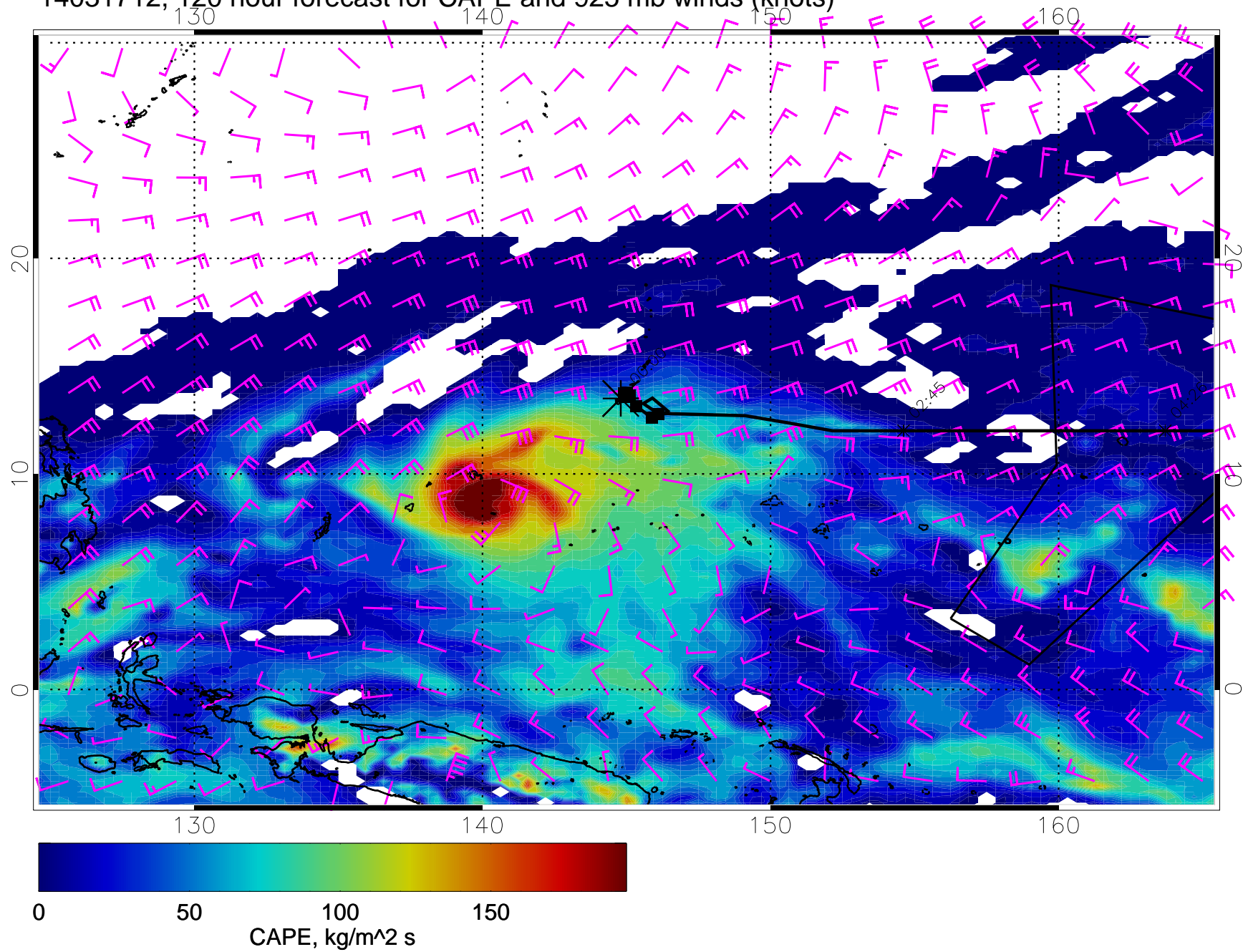
14031712, 120 hour forecast for CAPE and 925 mb winds (knots)
