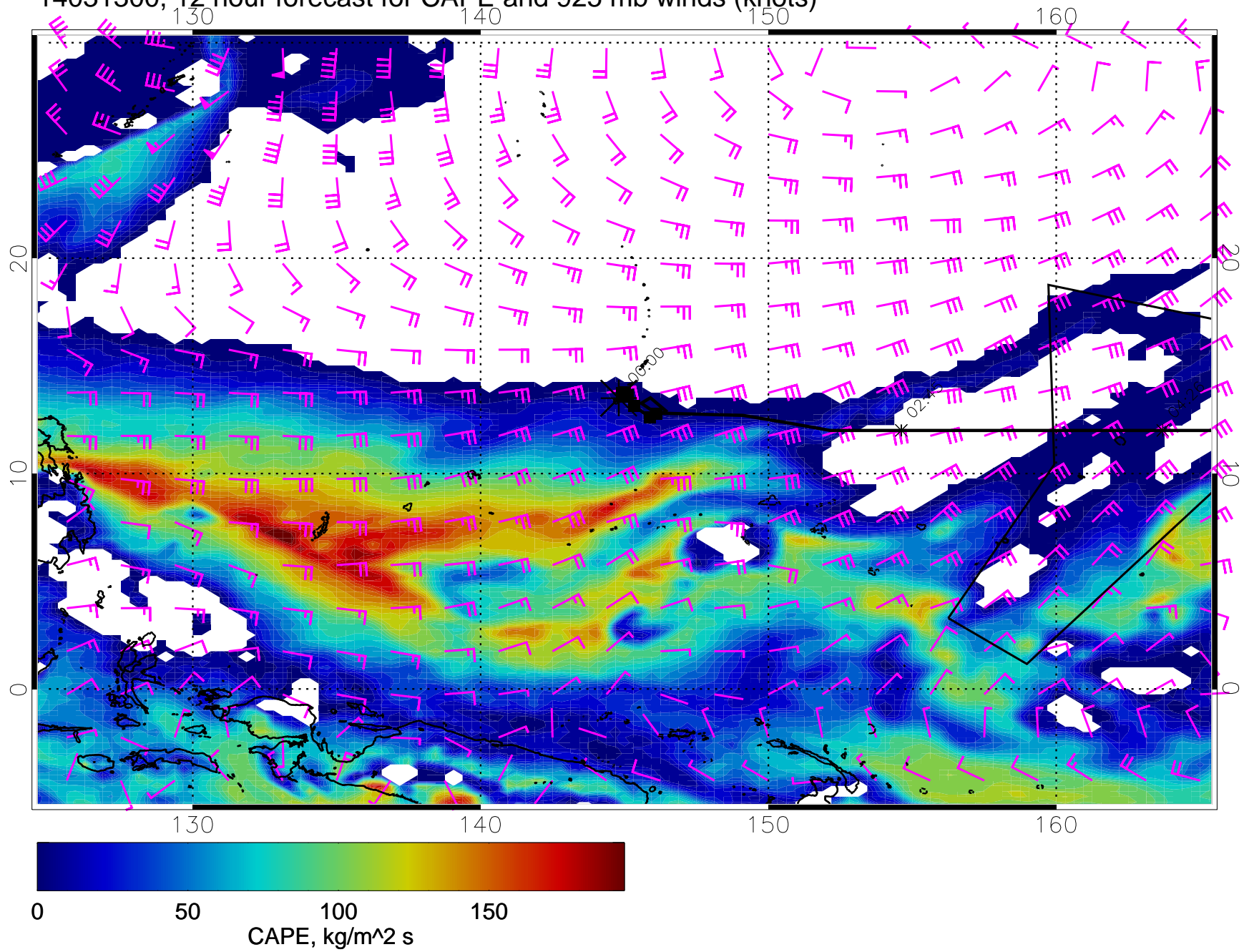
14031300, 12 hour forecast for CAPE and 925 mb winds (knots)
