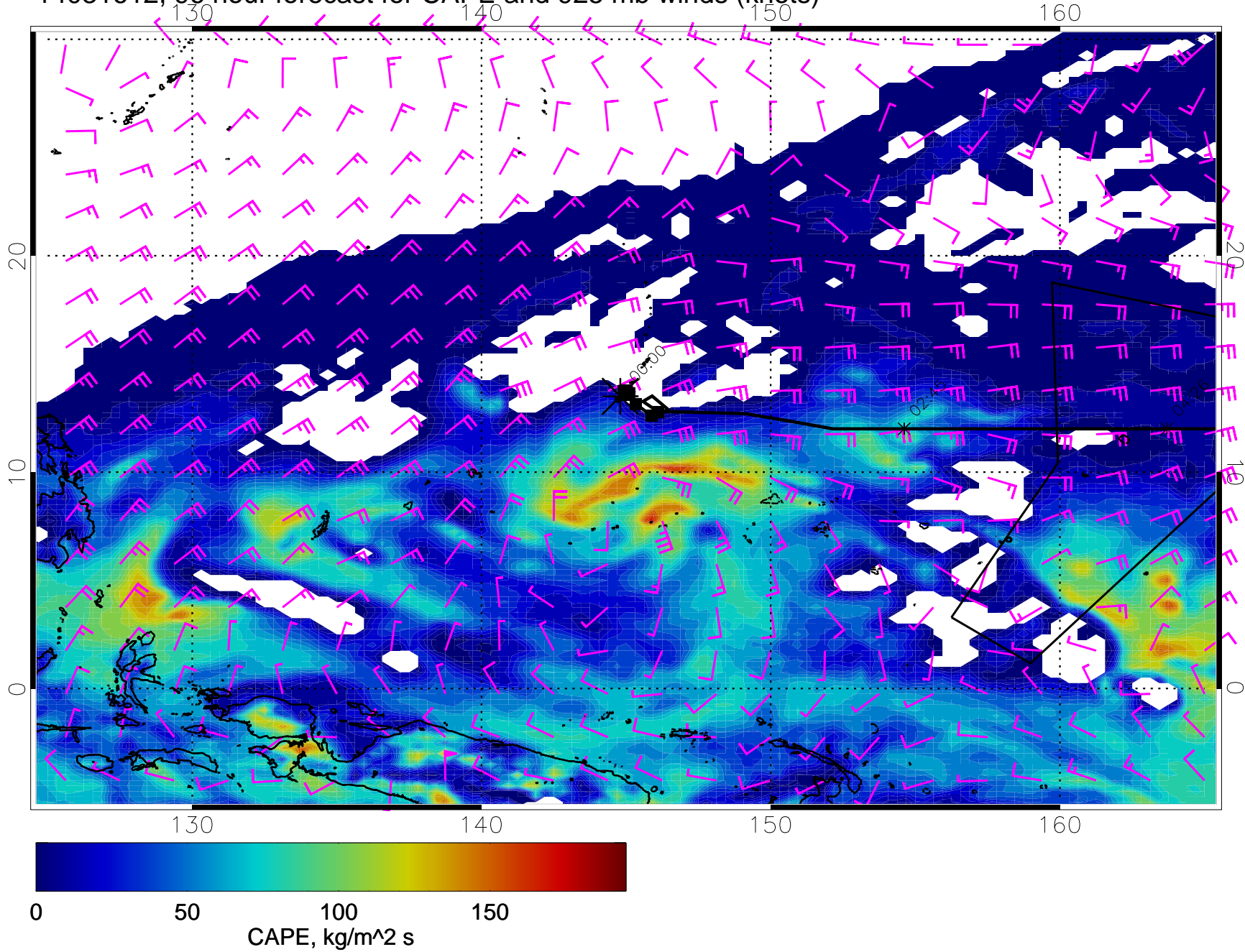
14031612, 96 hour forecast for CAPE and 925 mb winds (knots)
