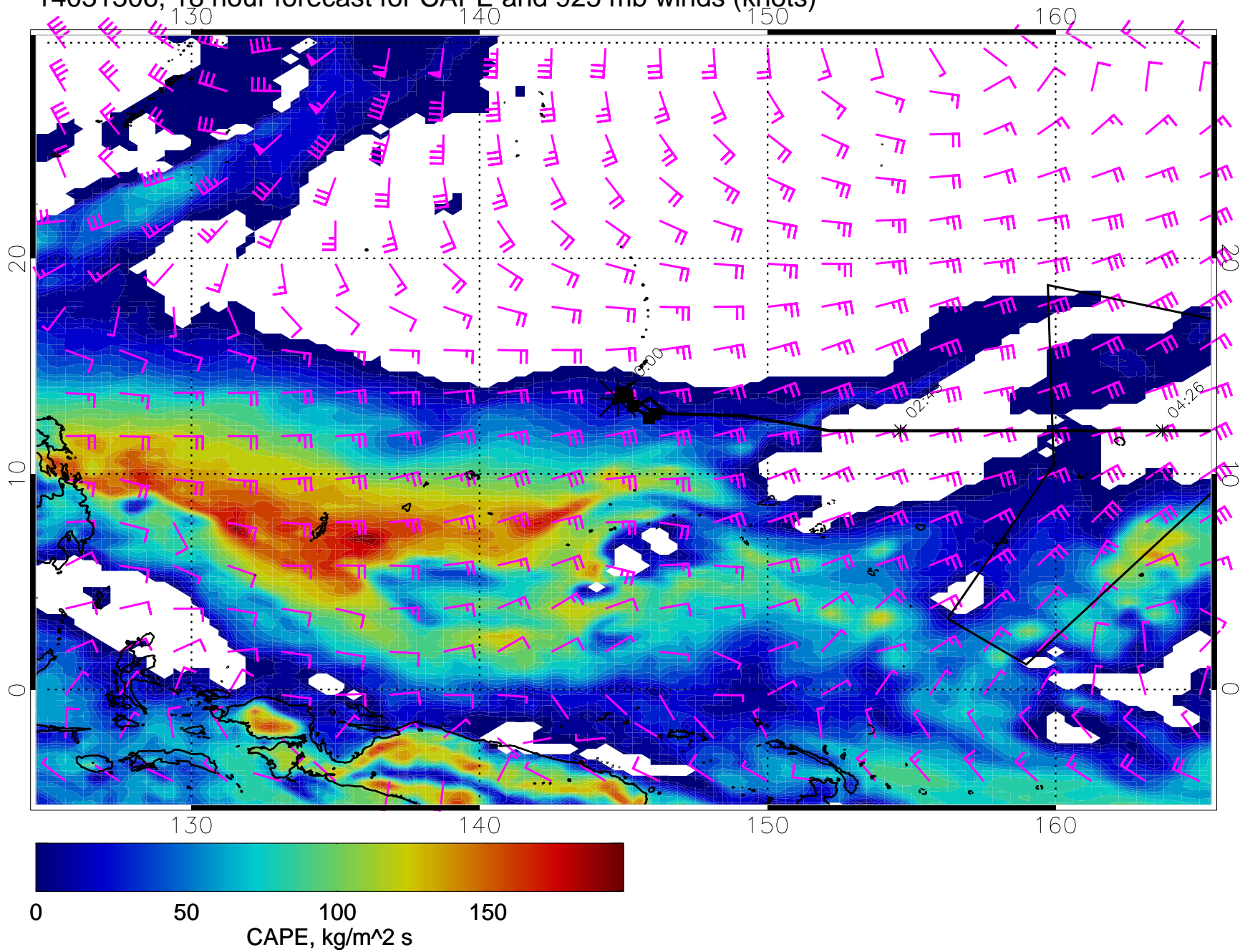
14031306, 18 hour forecast for CAPE and 925 mb winds (knots)
