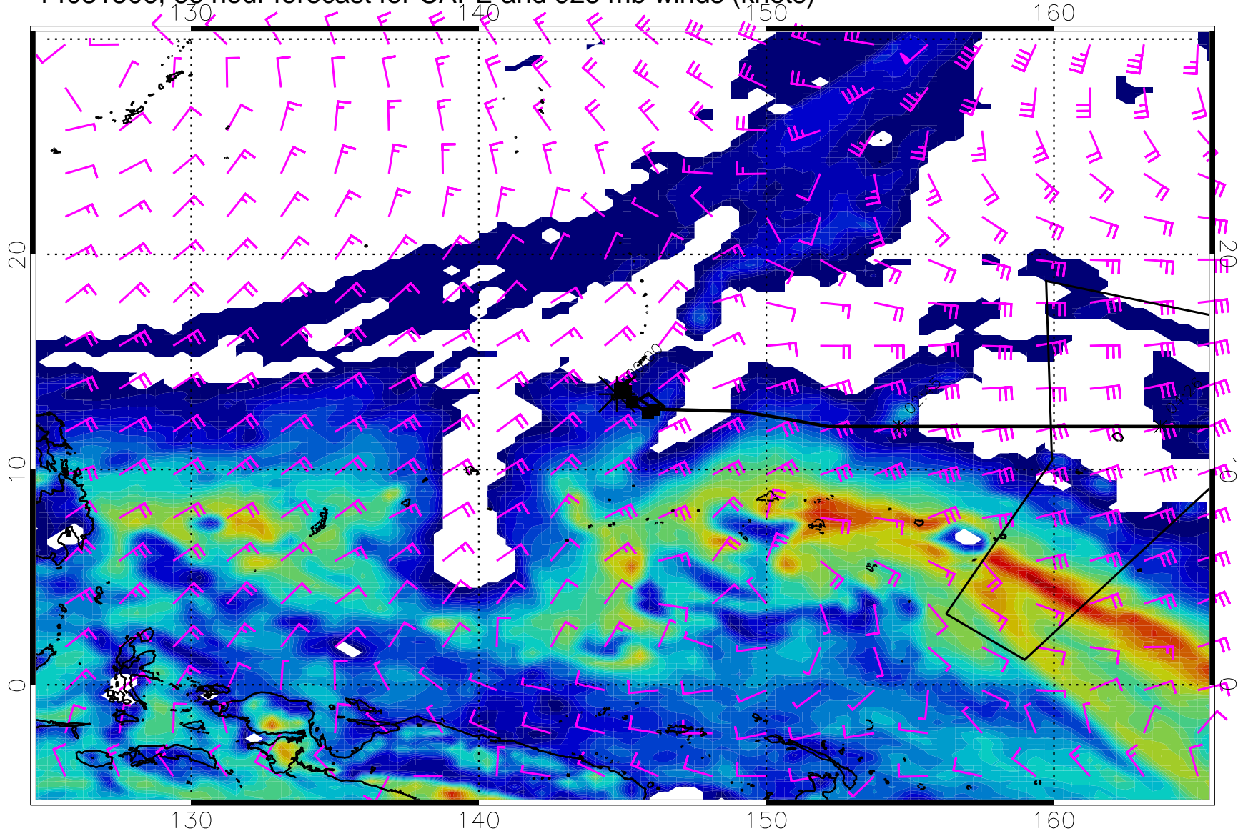
14031506, 66 hour forecast for CAPE and 925 mb winds (knots)
