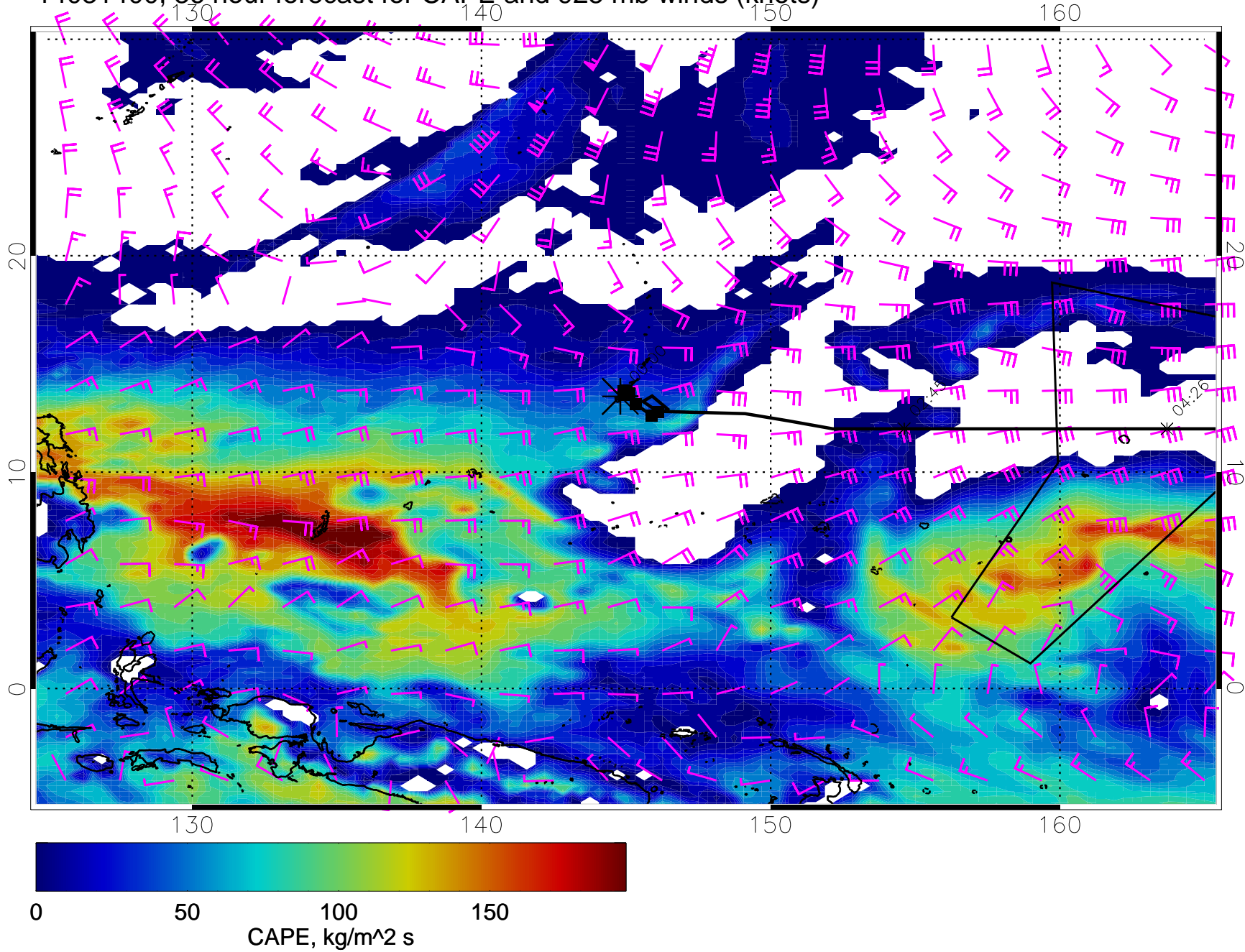
14031400, 36 hour forecast for CAPE and 925 mb winds (knots)
