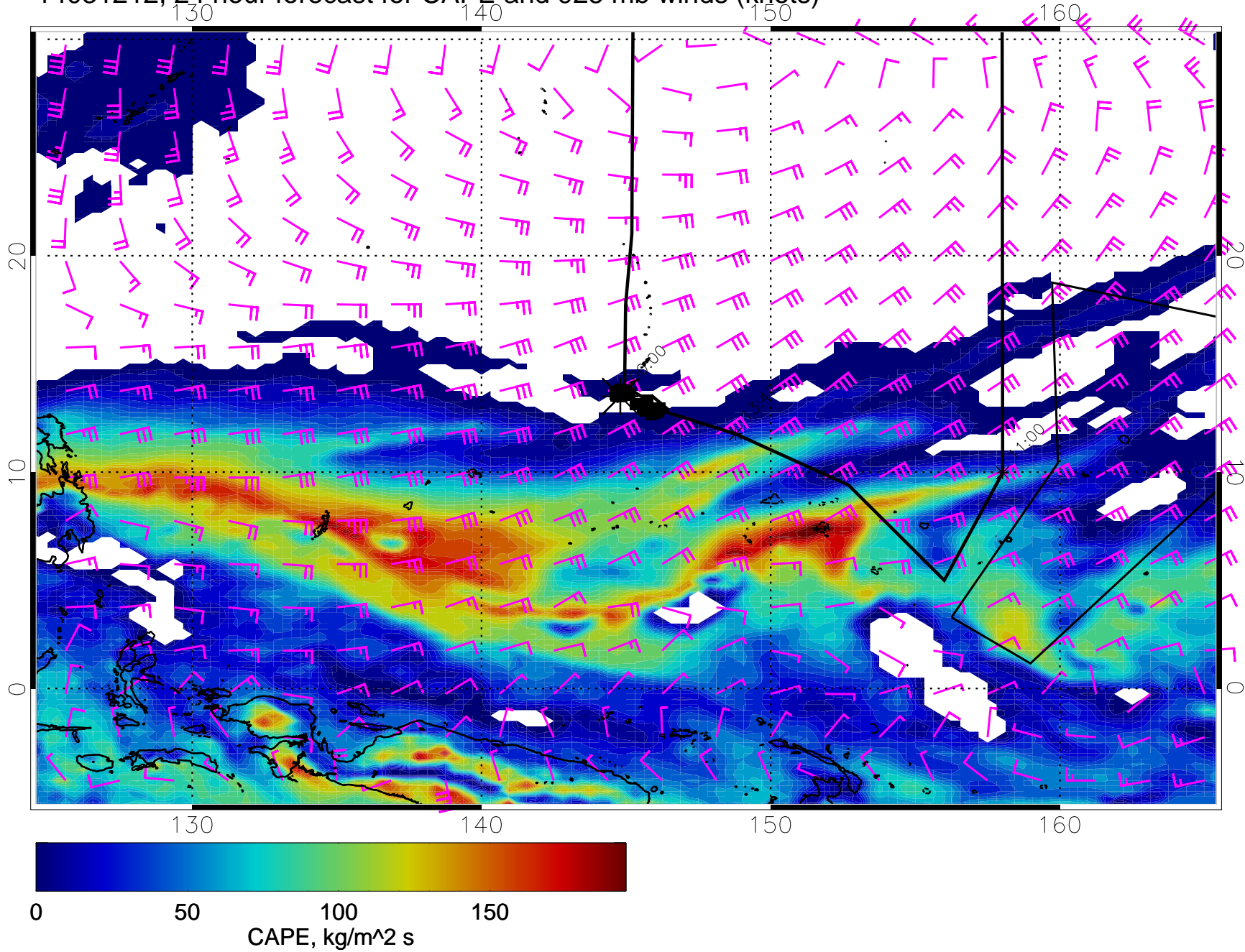
14031212, 24 hour forecast for CAPE and 925 mb winds (knots)
