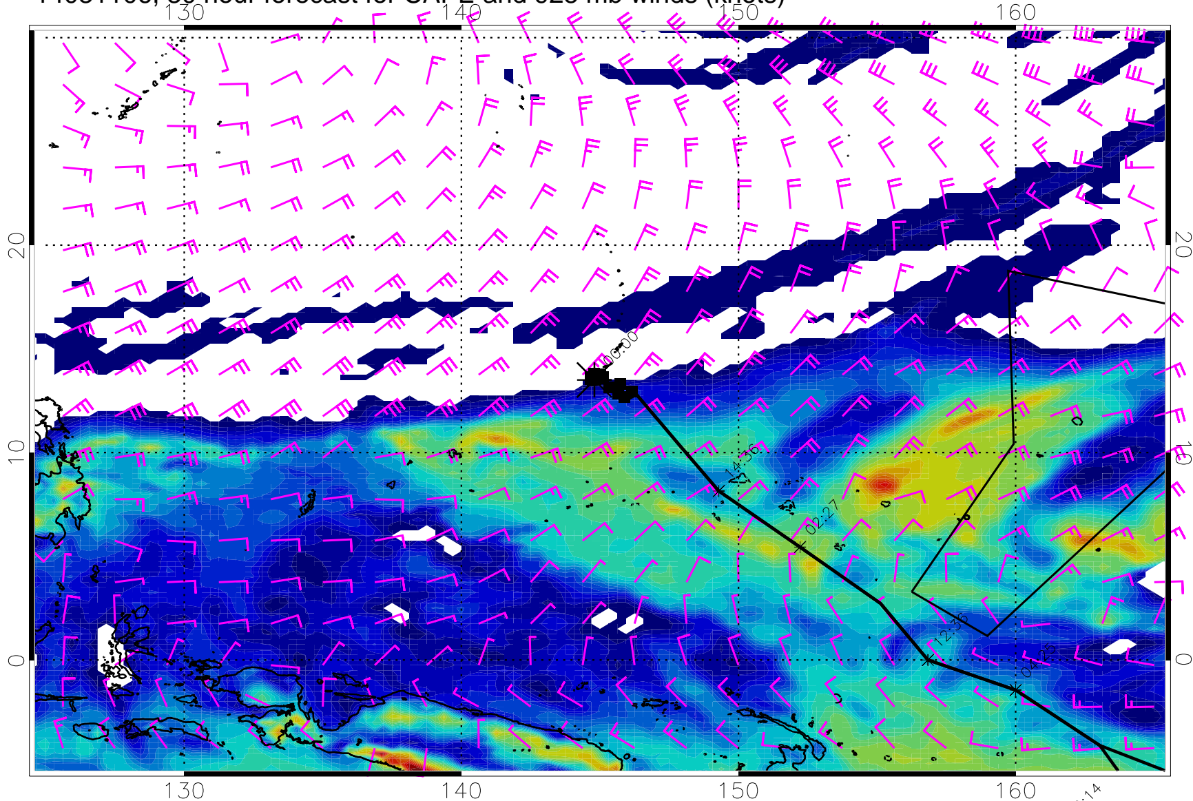
14031106, 30 hour forecast for CAPE and 925 mb winds (knots)
