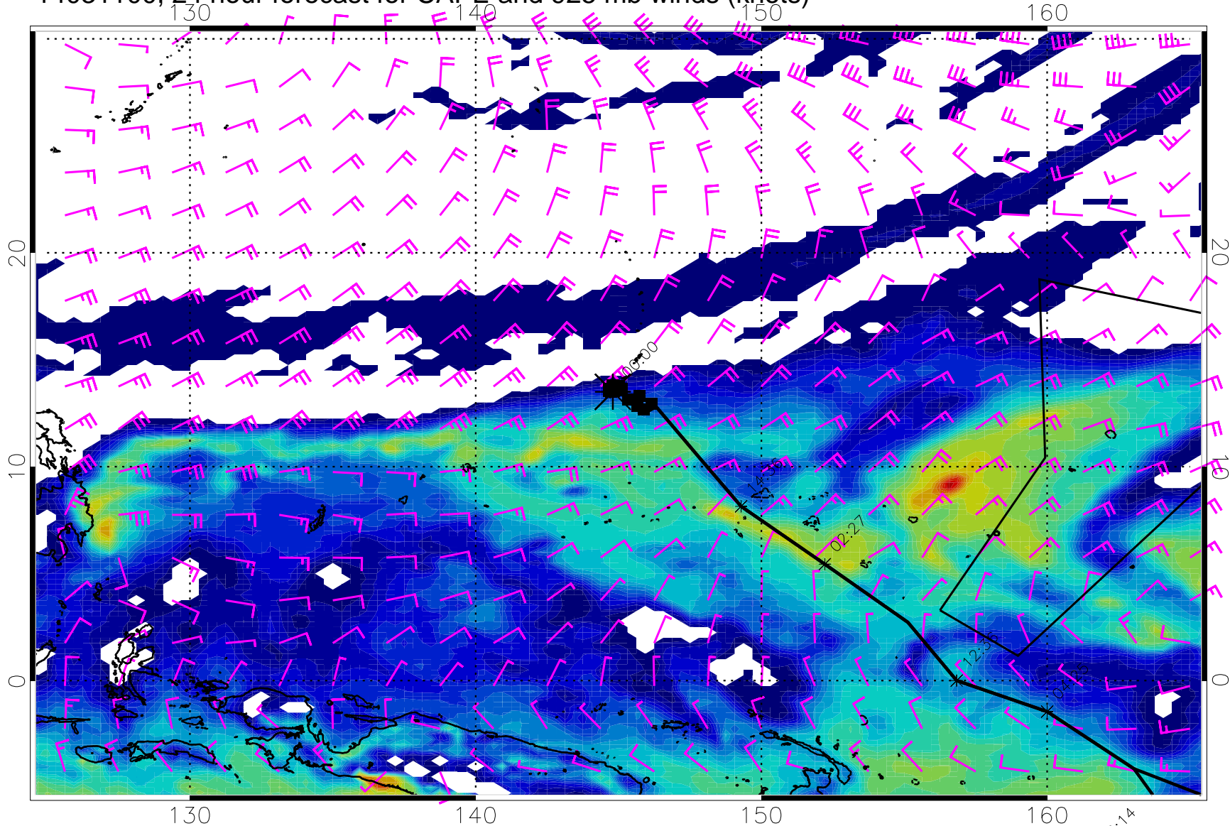
14031100, 24 hour forecast for CAPE and 925 mb winds (knots)
