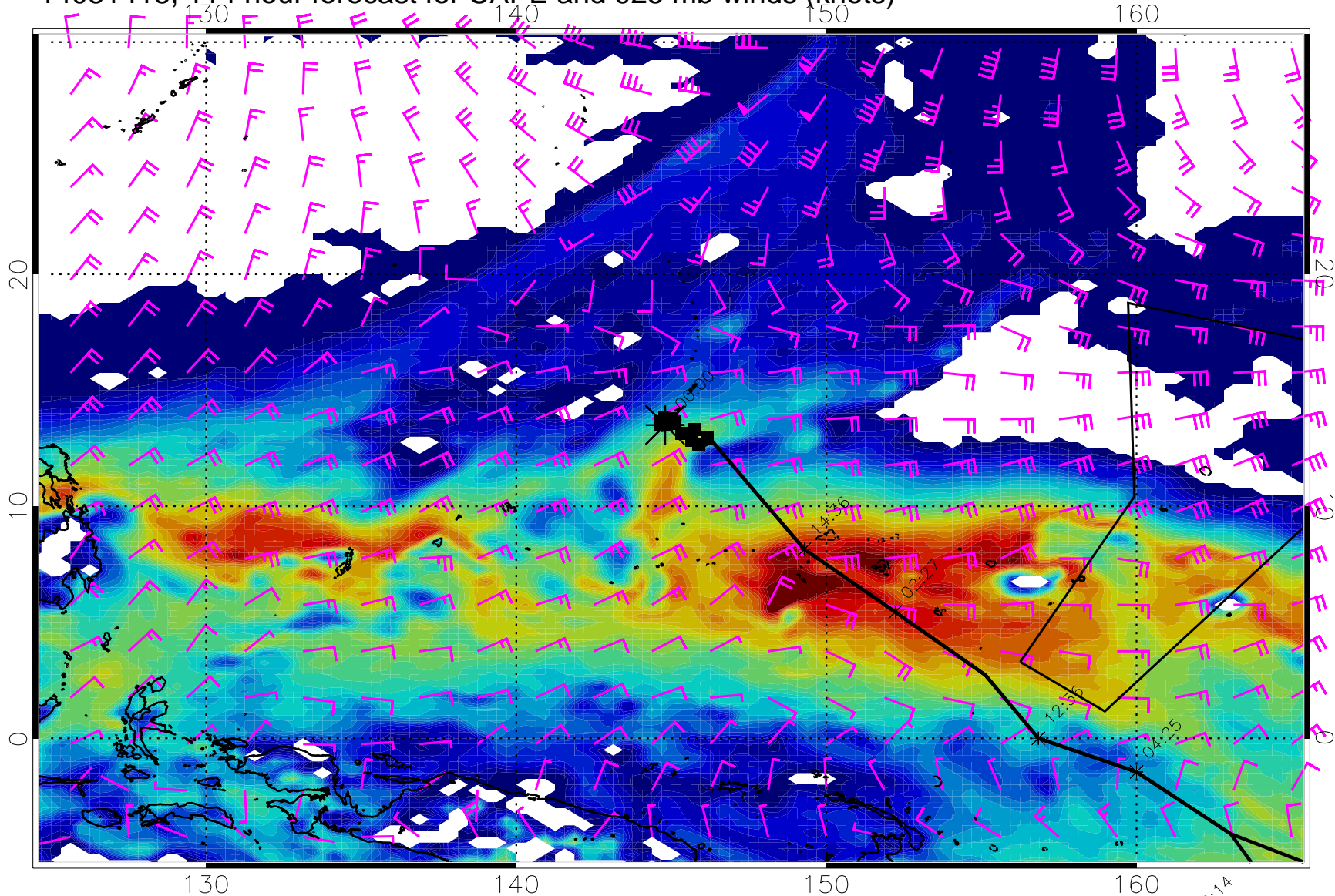
14031418, 114 hour forecast for CAPE and 925 mb winds (knots)
