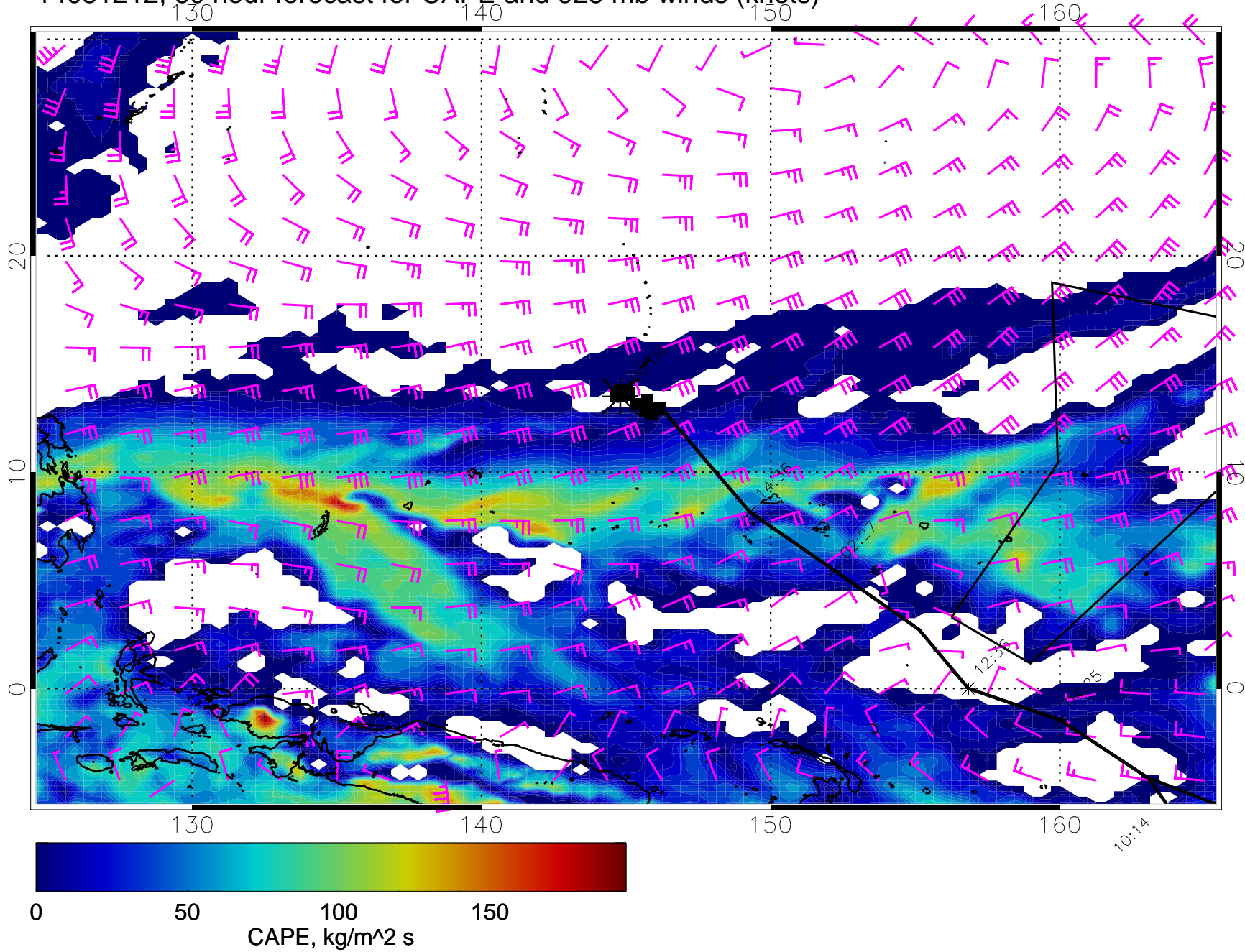
14031212, 60 hour forecast for CAPE and 925 mb winds (knots)
