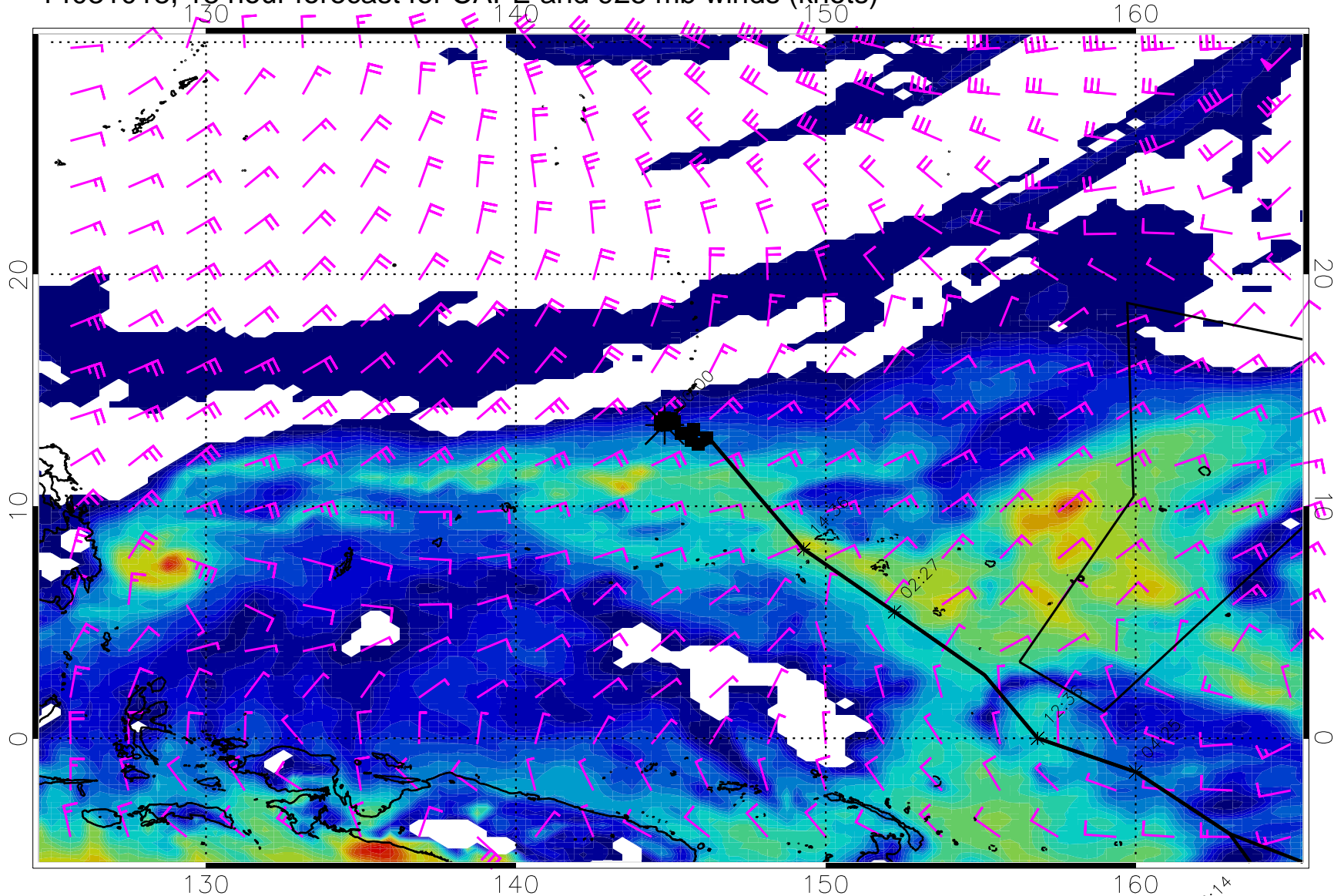
14031018, 18 hour forecast for CAPE and 925 mb winds (knots)
