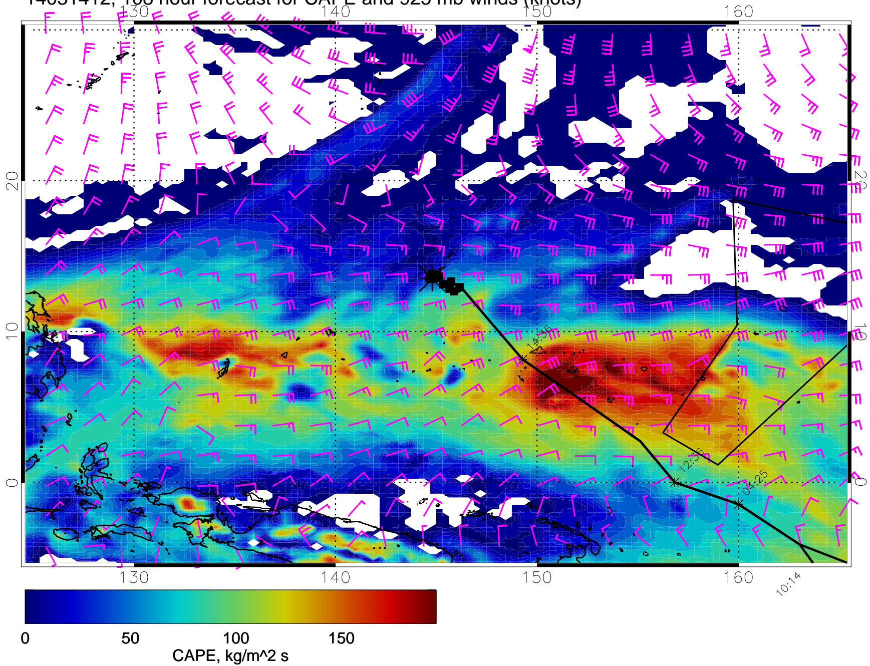
14031412, 108 hour forecast for CAPE and 925 mb winds (knots)
