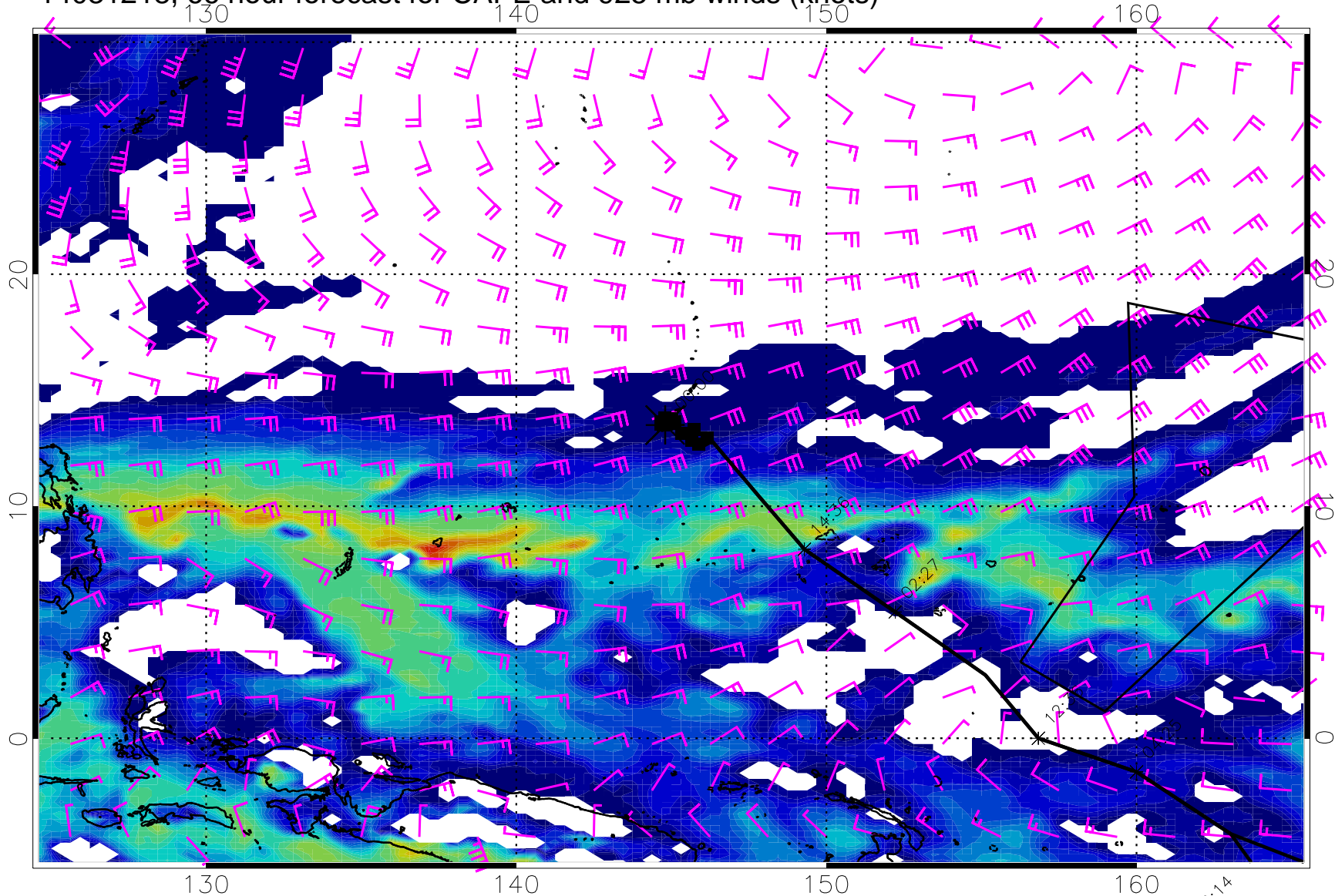
14031218, 66 hour forecast for CAPE and 925 mb winds (knots)
