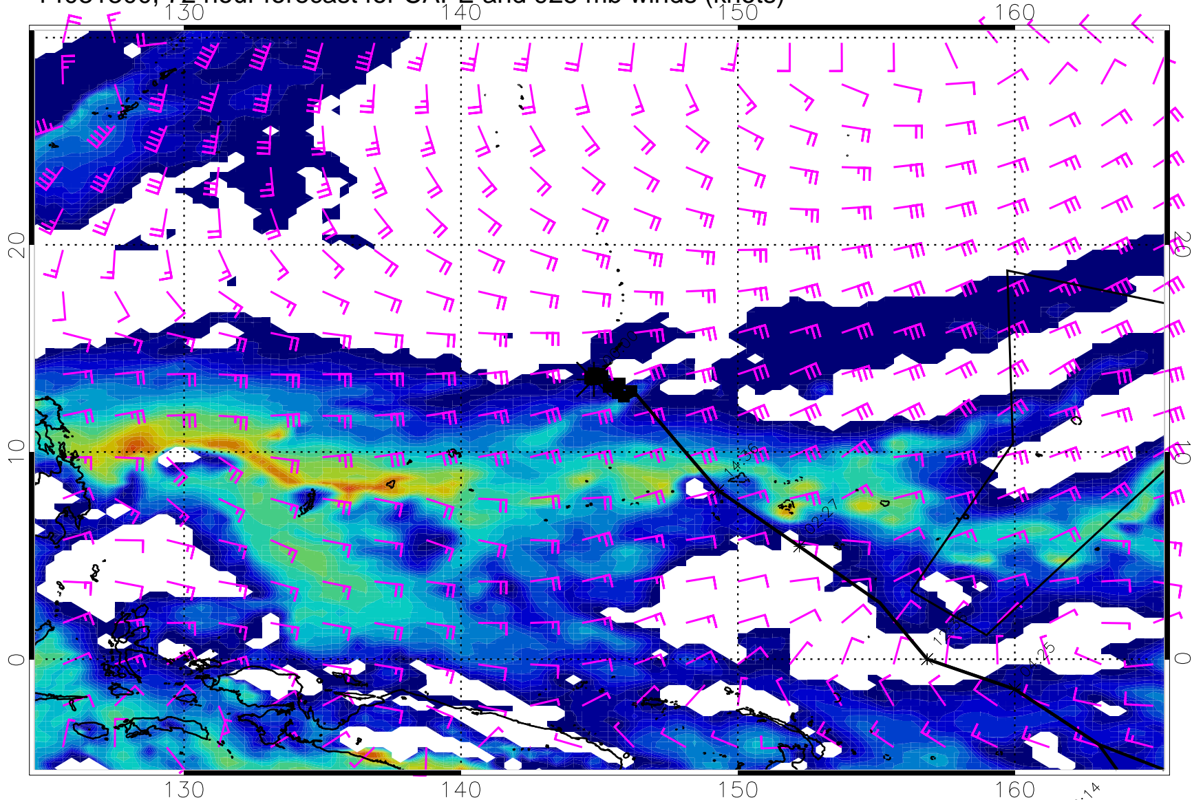
14031300, 72 hour forecast for CAPE and 925 mb winds (knots)
