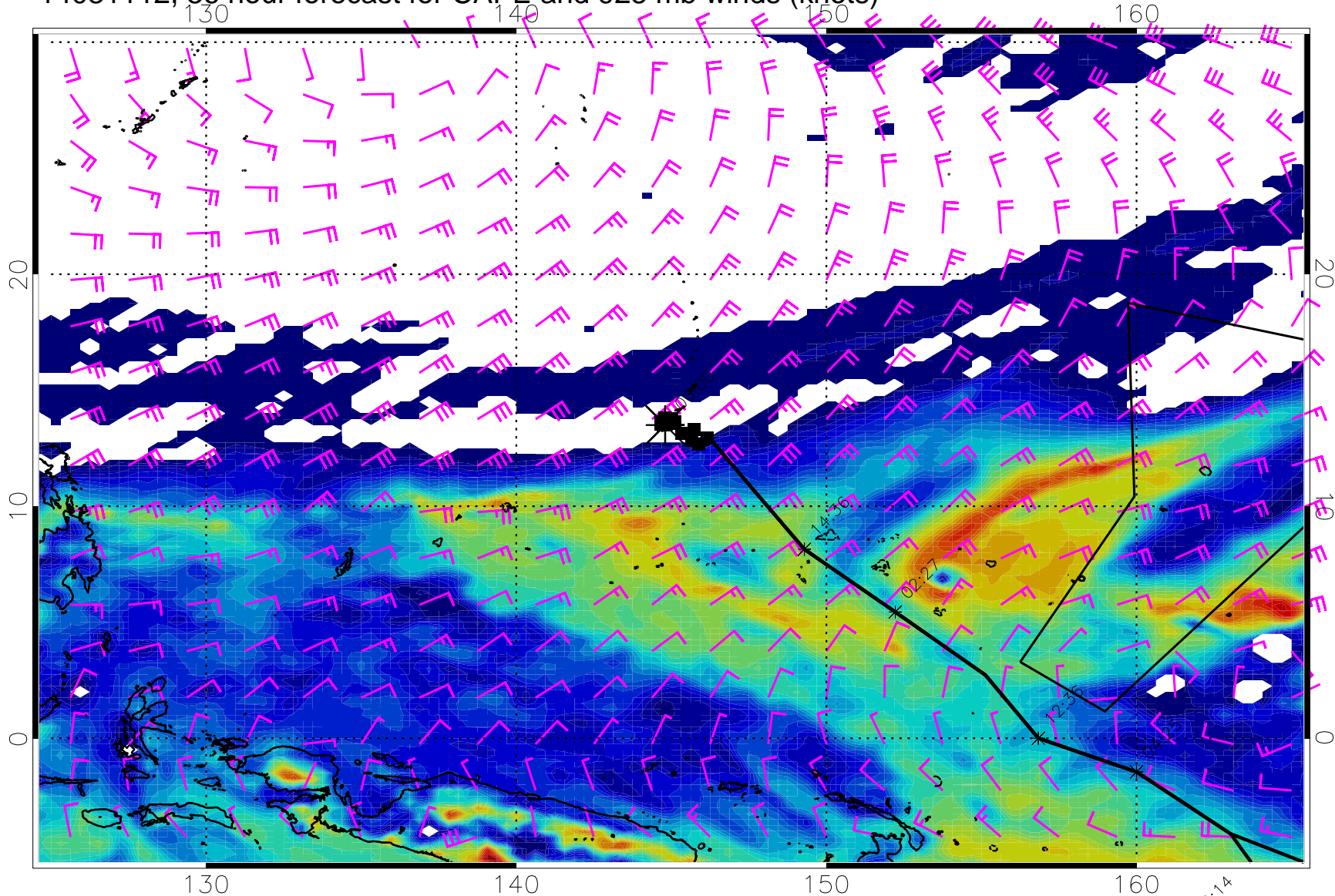
14031112, 36 hour forecast for CAPE and 925 mb winds (knots)
