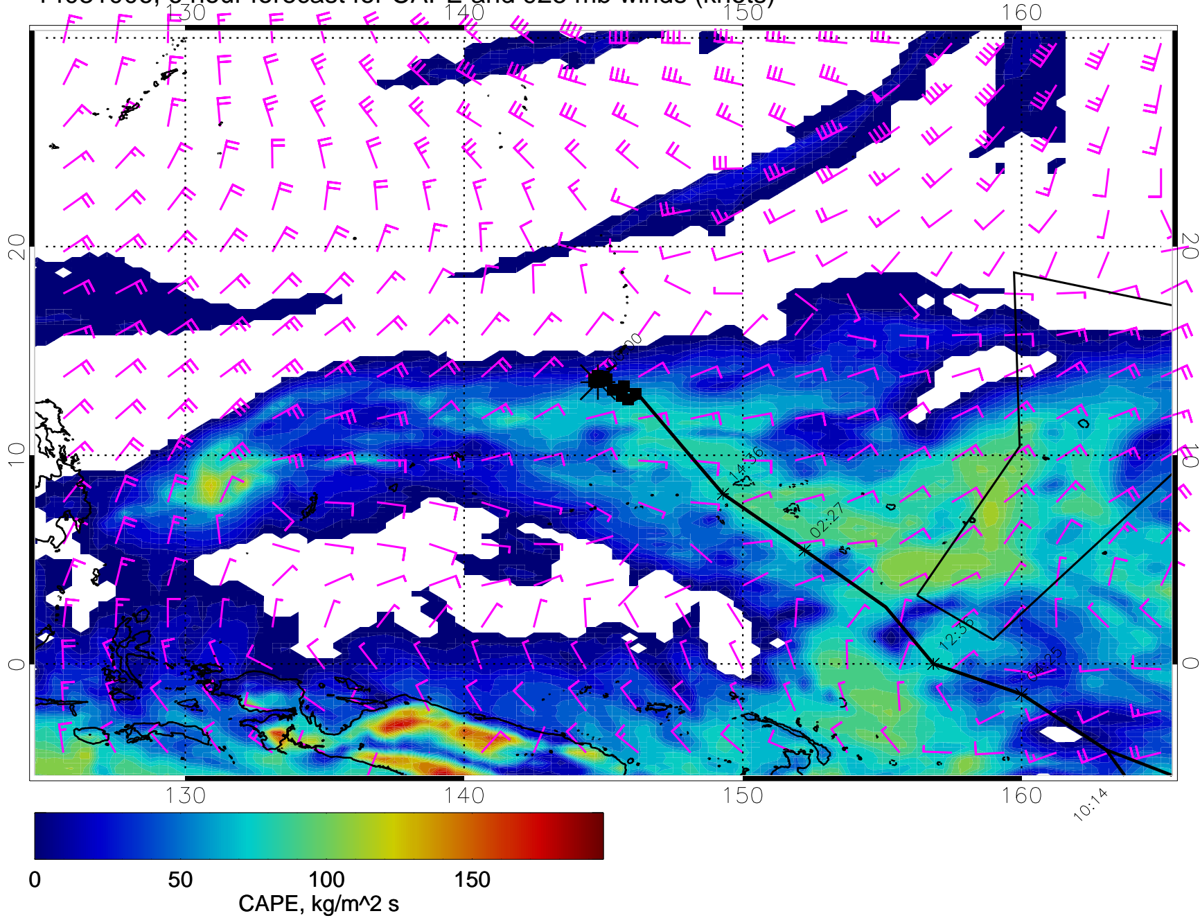
14031006, 6 hour forecast for CAPE and 925 mb winds (knots)
