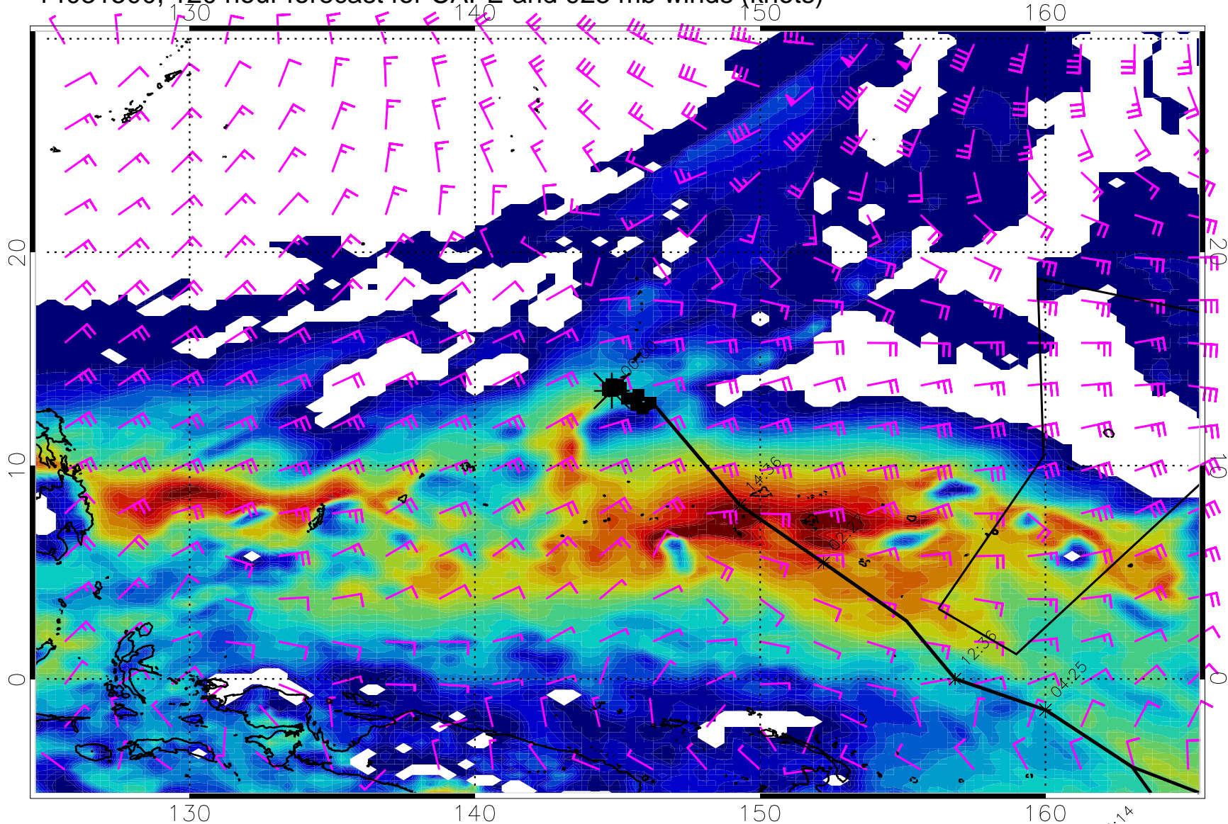
14031500, 120 hour forecast for CAPE and 925 mb winds (knots)
