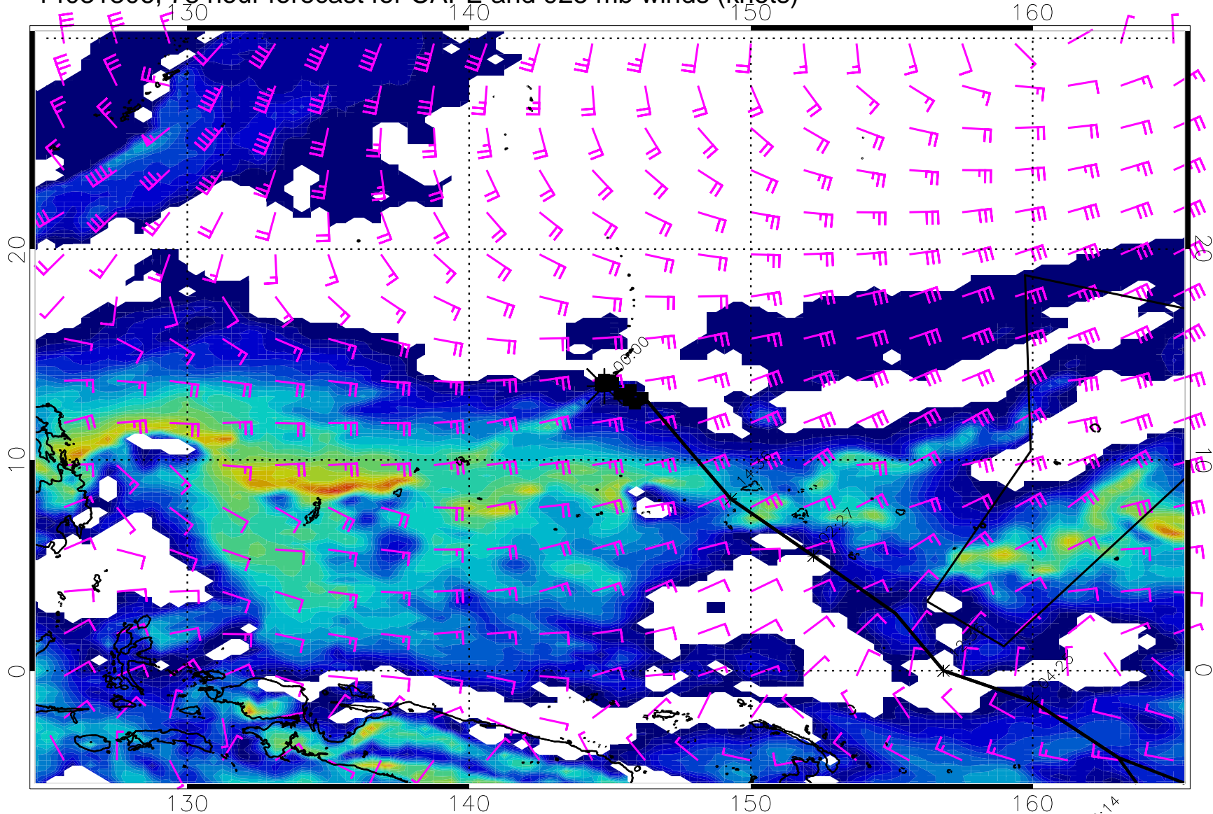
14031306, 78 hour forecast for CAPE and 925 mb winds (knots)
