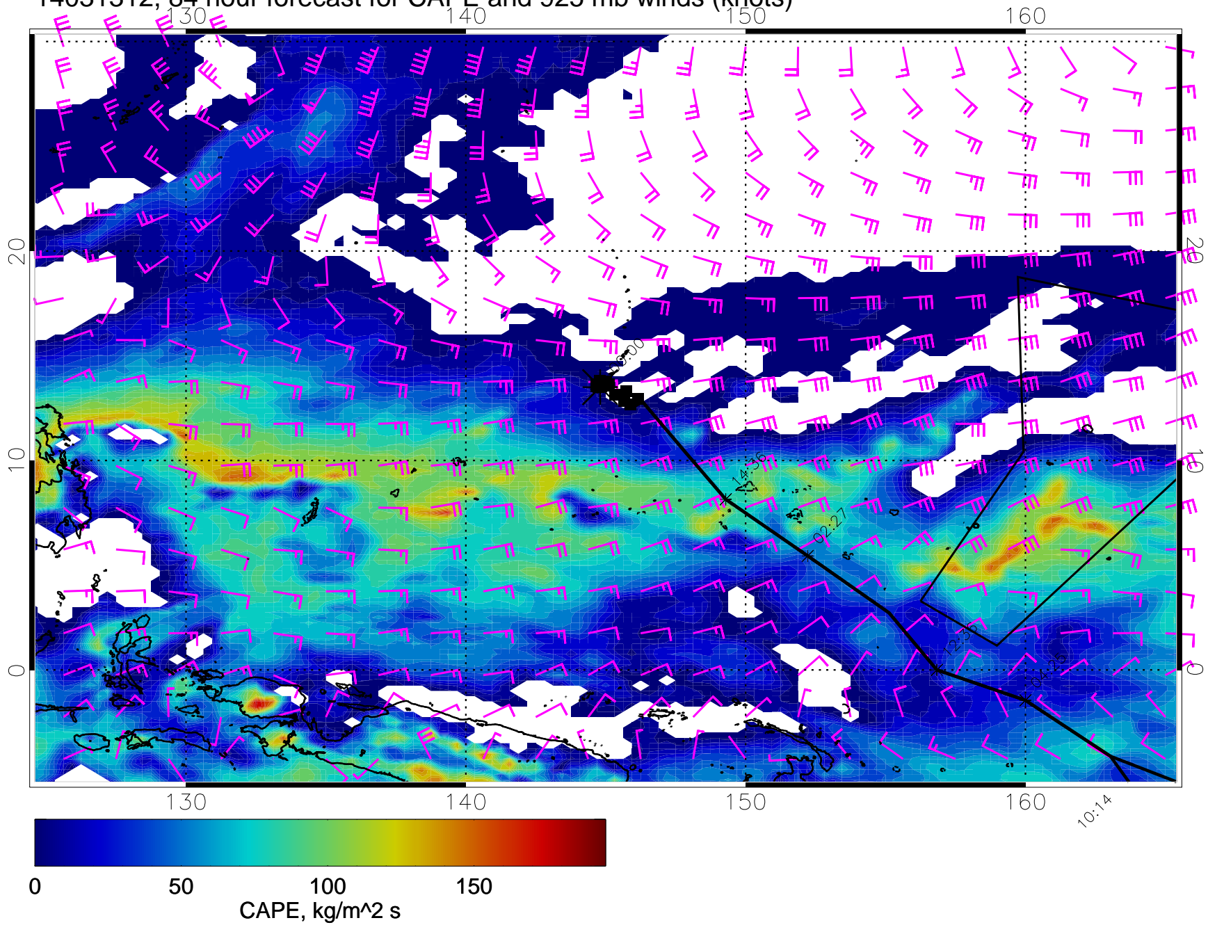
14031312, 84 hour forecast for CAPE and 925 mb winds (knots)
