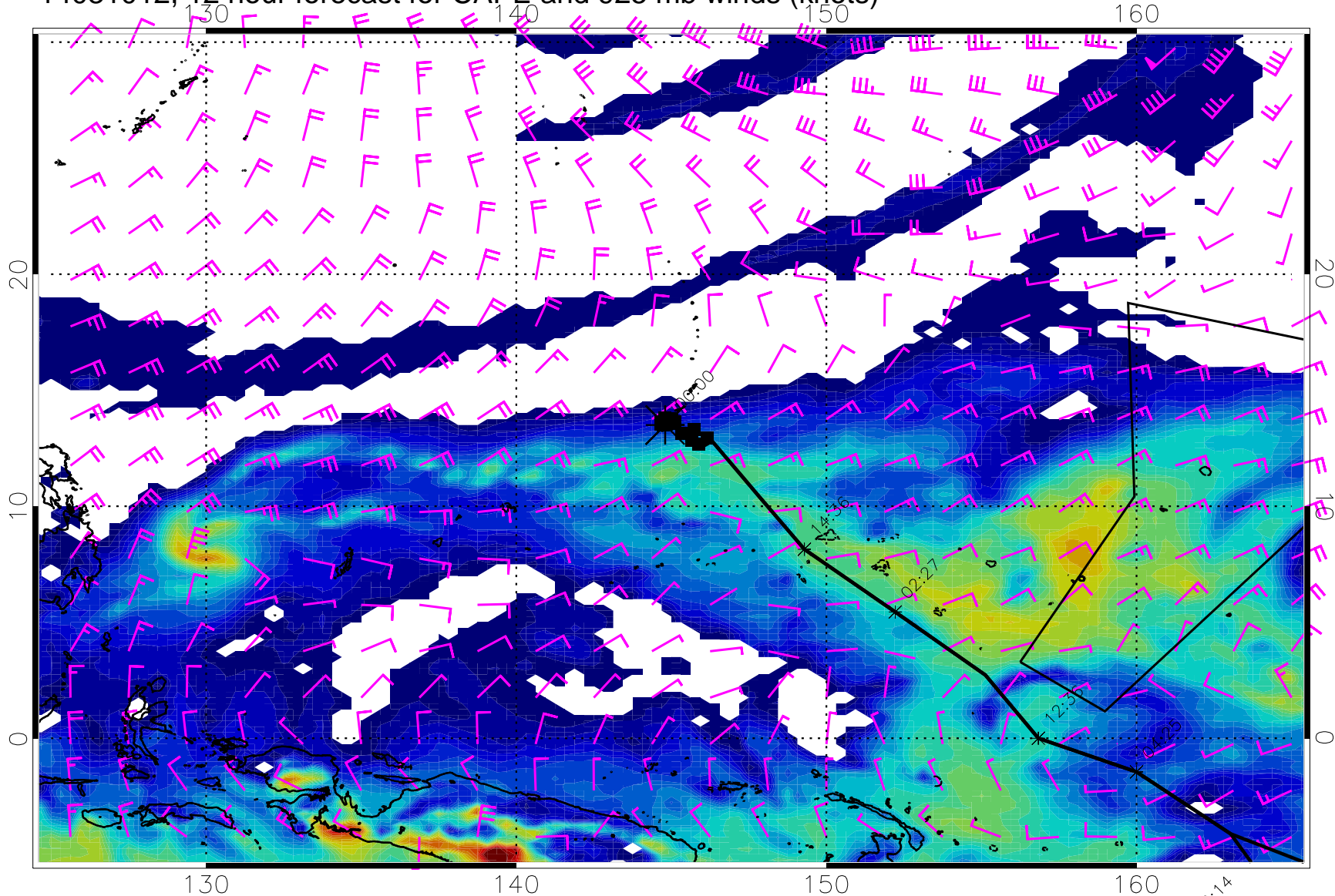
14031012, 12 hour forecast for CAPE and 925 mb winds (knots)
