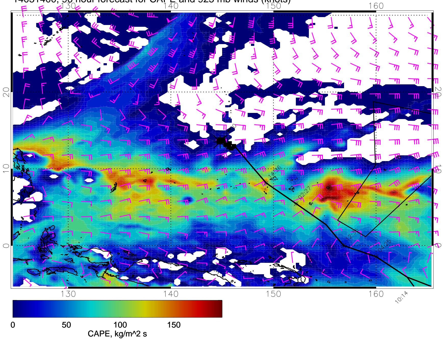
14031400, 96 hour forecast for CAPE and 925 mb winds (knots)
