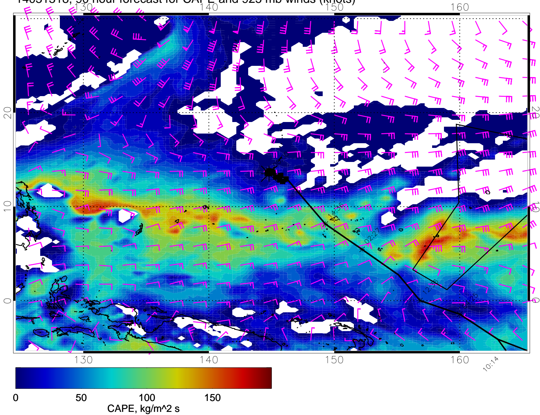
14031318, 90 hour forecast for CAPE and 925 mb winds (knots)
