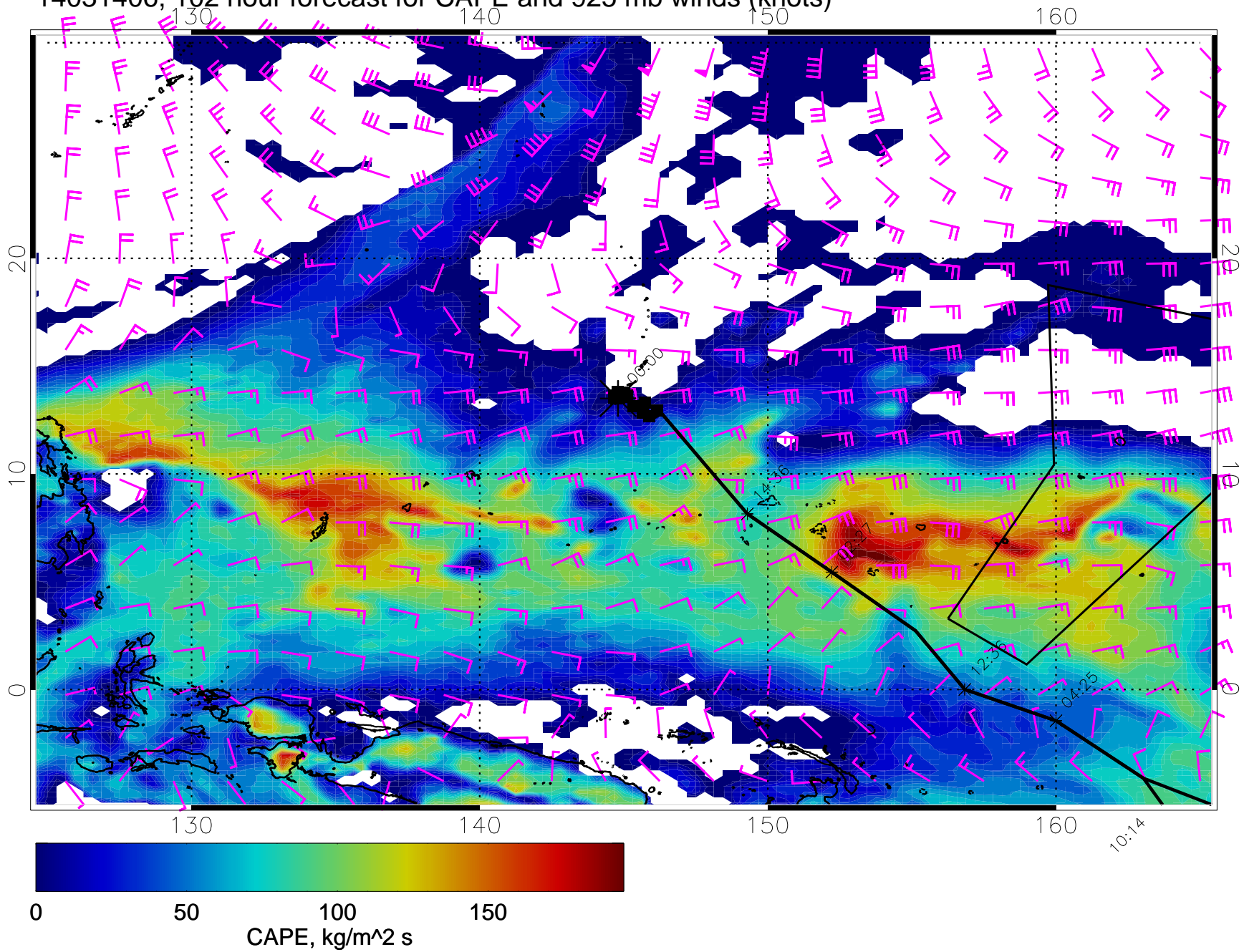
14031406, 102 hour forecast for CAPE and 925 mb winds (knots)
