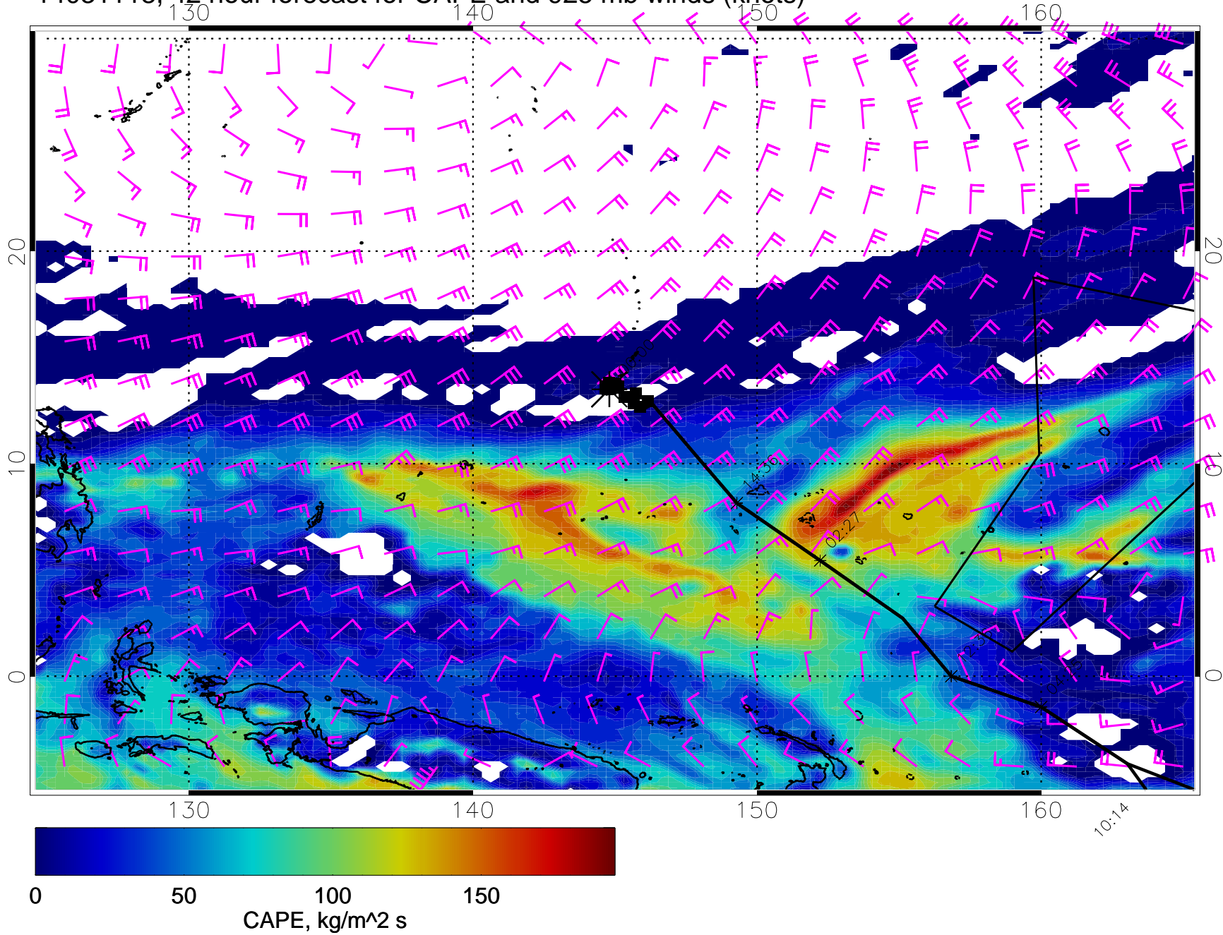
14031118, 42 hour forecast for CAPE and 925 mb winds (knots)
