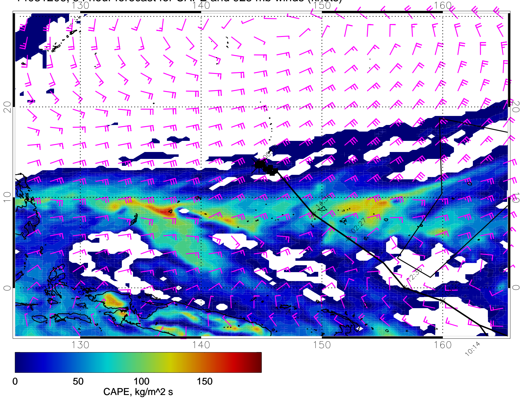
14031206, 54 hour forecast for CAPE and 925 mb winds (knots)
