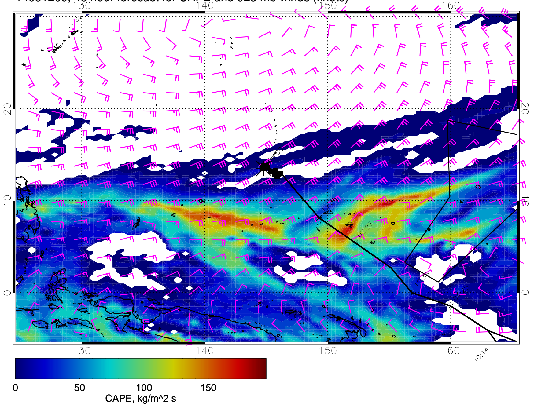
14031200, 48 hour forecast for CAPE and 925 mb winds (knots)
