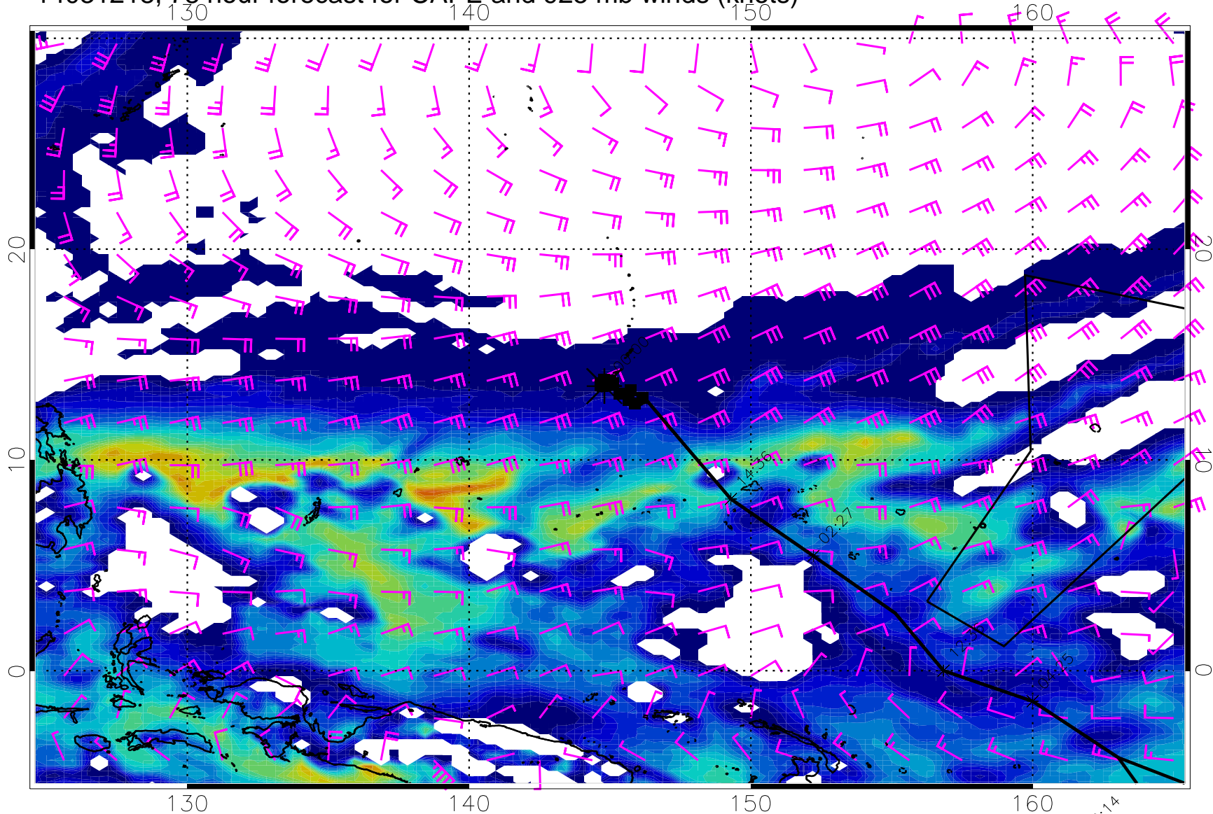
14031218, 78 hour forecast for CAPE and 925 mb winds (knots)
