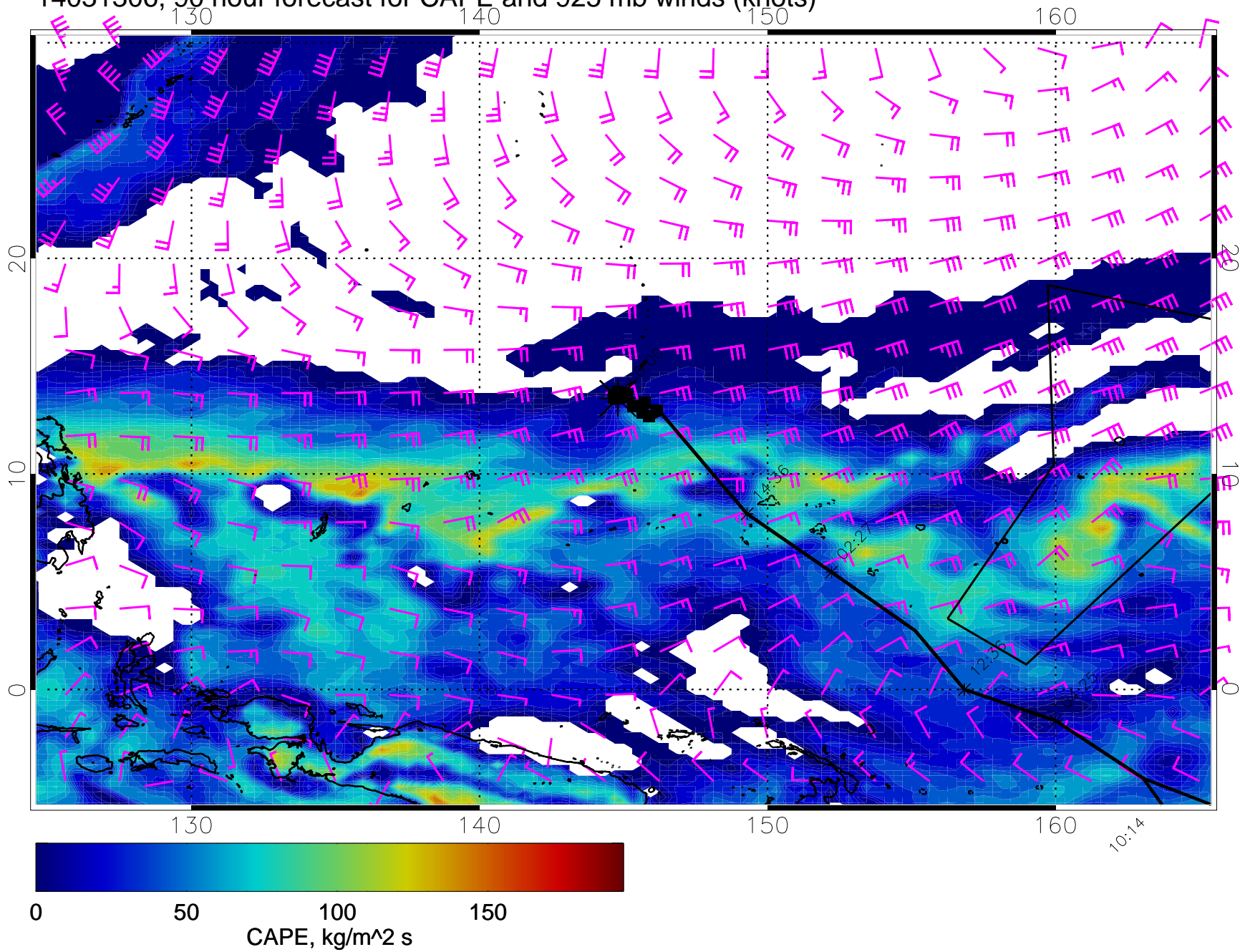
14031306, 90 hour forecast for CAPE and 925 mb winds (knots)
