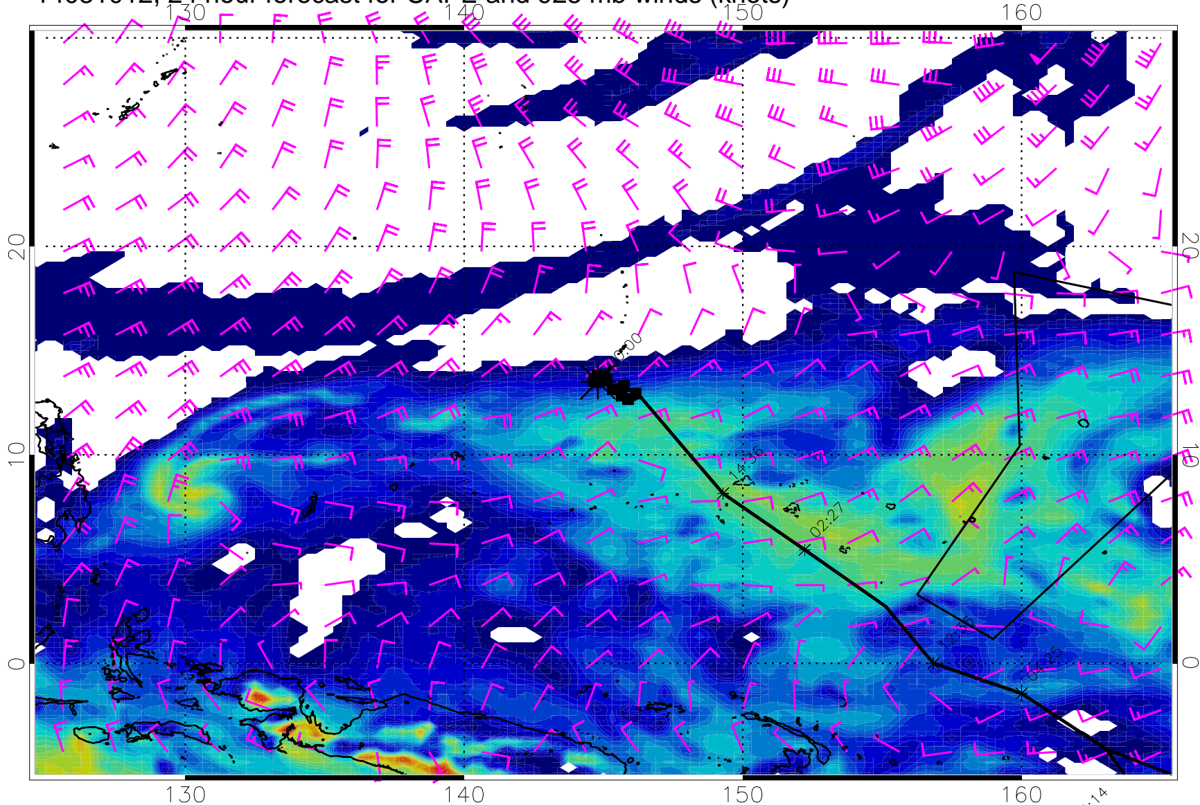
14031012, 24 hour forecast for CAPE and 925 mb winds (knots)
