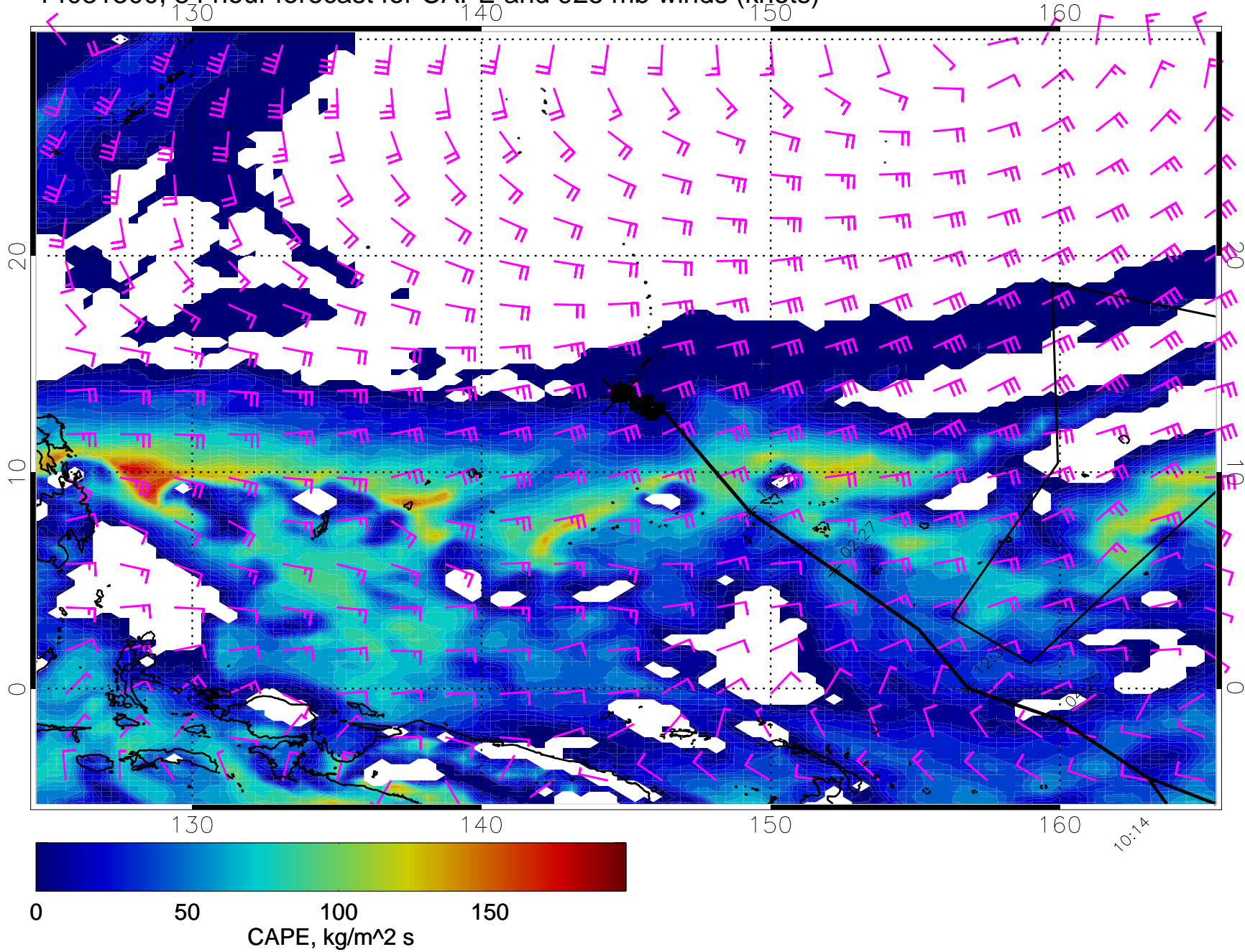
14031300, 84 hour forecast for CAPE and 925 mb winds (knots)
