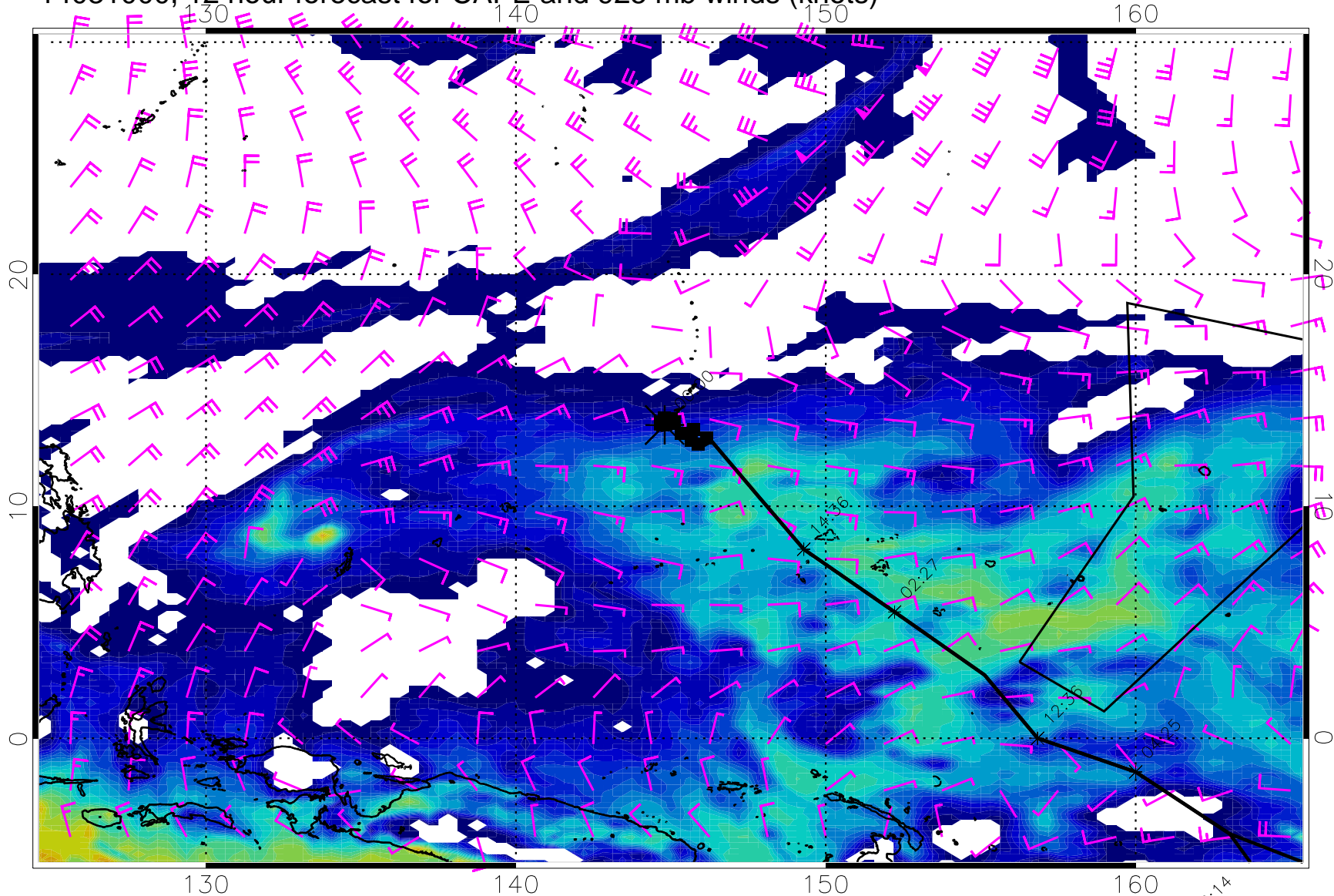
14031000, 12 hour forecast for CAPE and 925 mb winds (knots)
