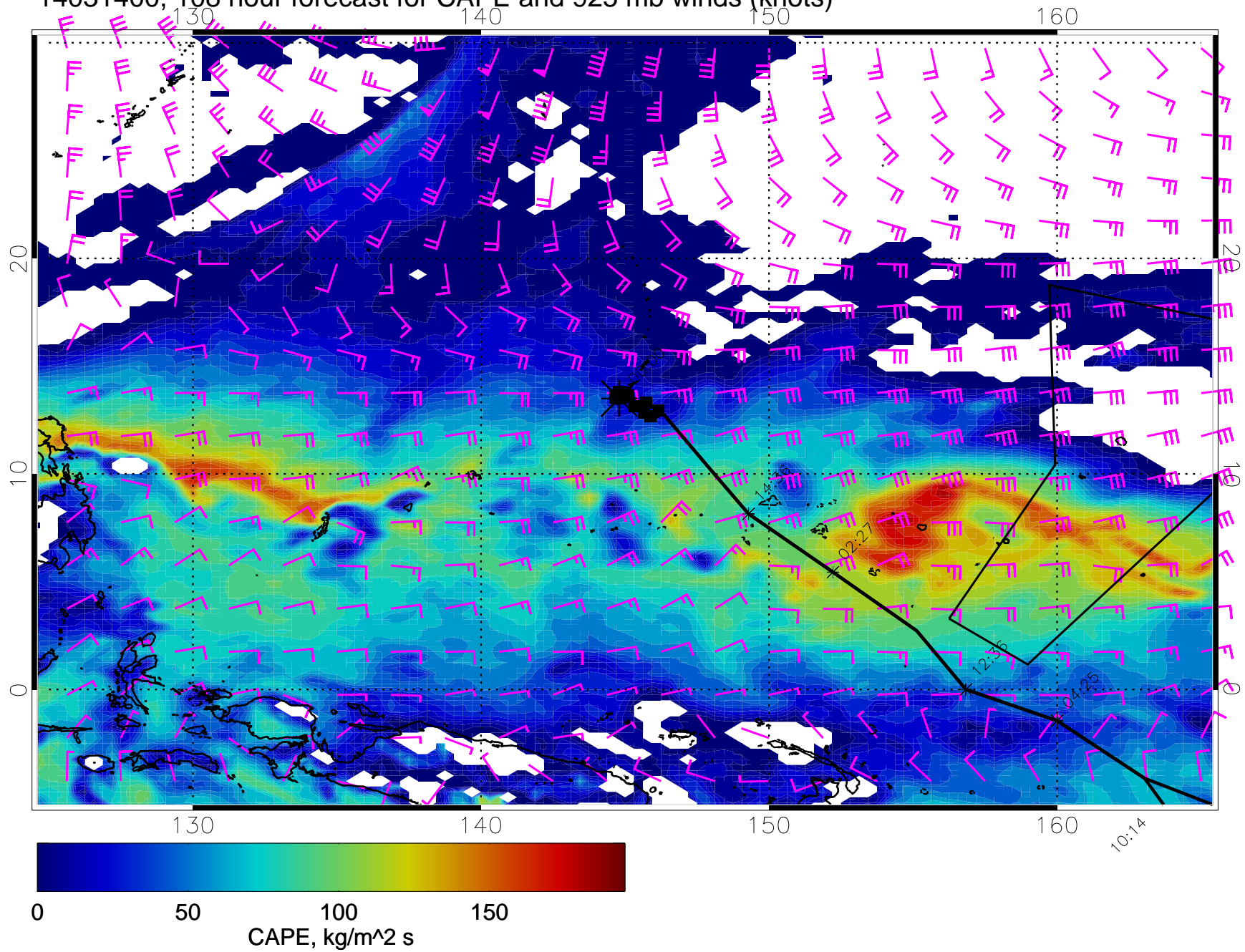
14031400, 108 hour forecast for CAPE and 925 mb winds (knots)
