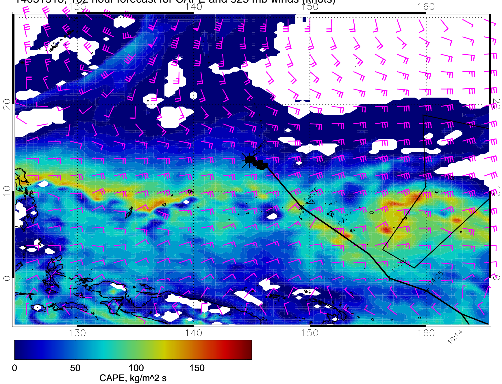
14031318, 102 hour forecast for CAPE and 925 mb winds (knots)
