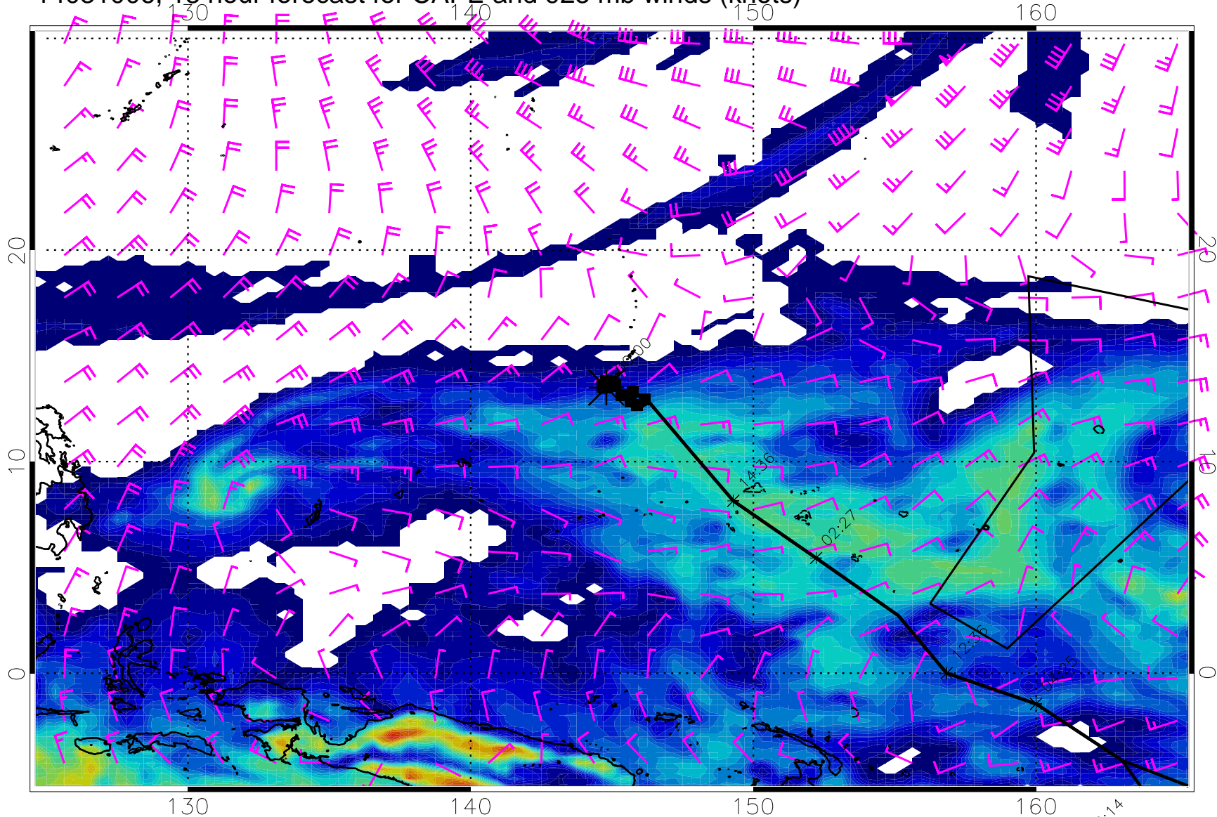
14031006, 18 hour forecast for CAPE and 925 mb winds (knots)
