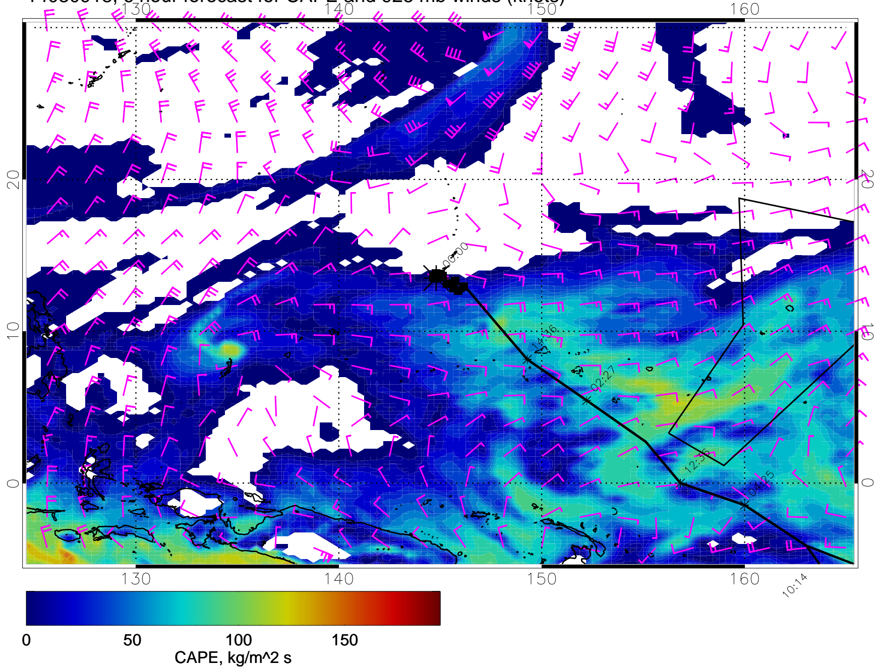
14030918, 6 hour forecast for CAPE and 925 mb winds (knots)
