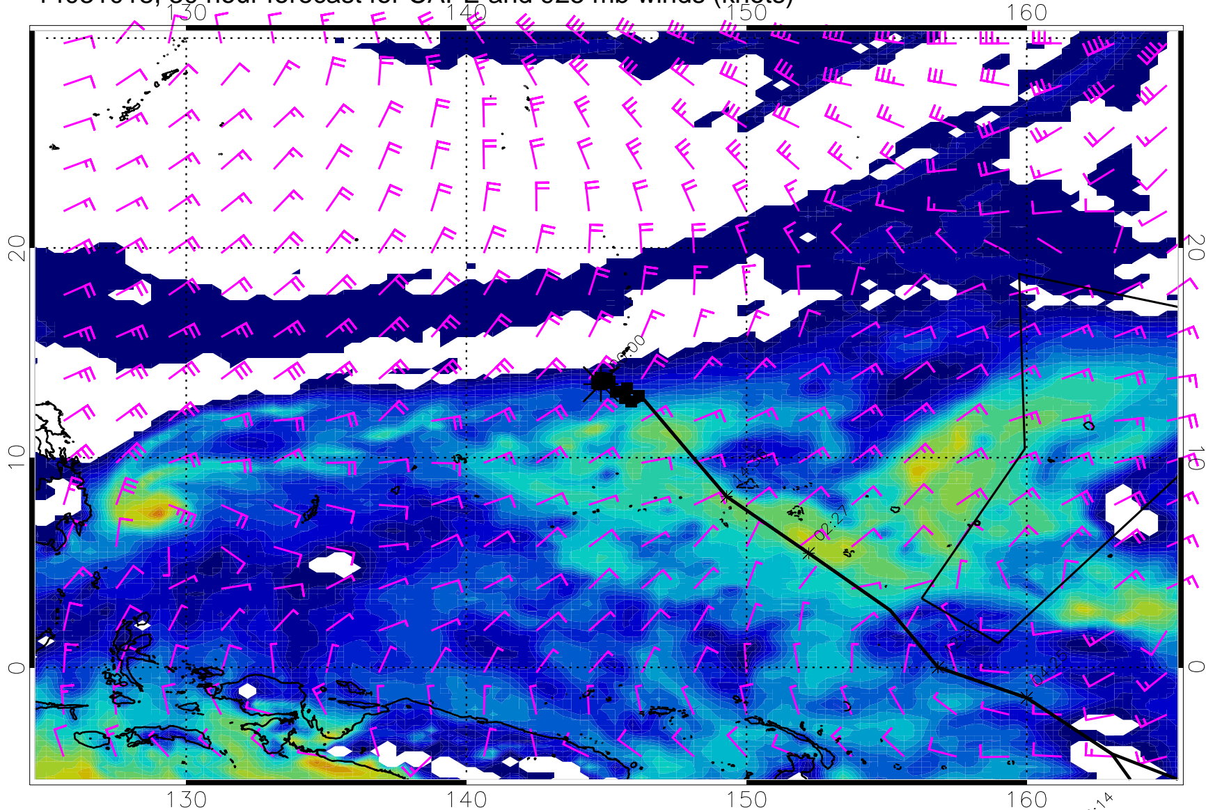
14031018, 30 hour forecast for CAPE and 925 mb winds (knots)
