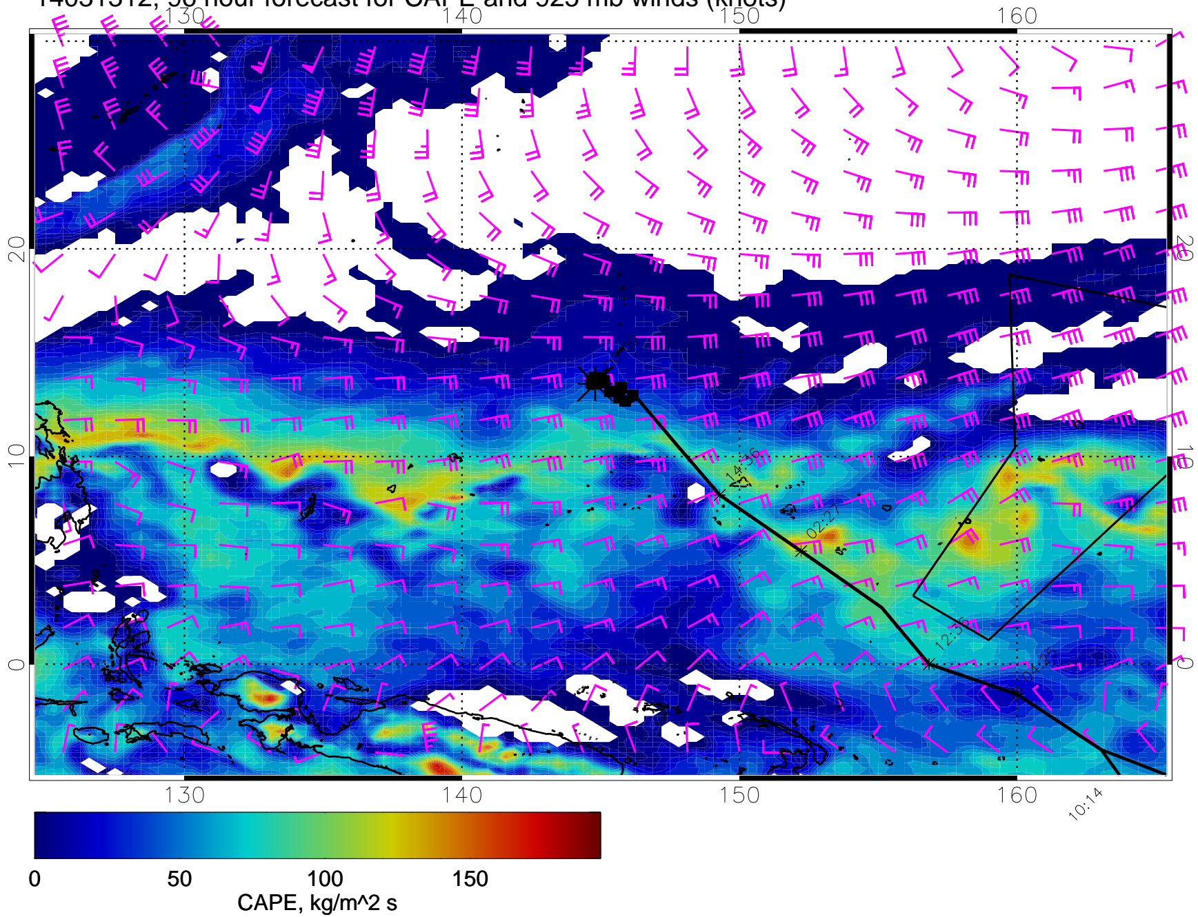
14031312, 96 hour forecast for CAPE and 925 mb winds (knots)
