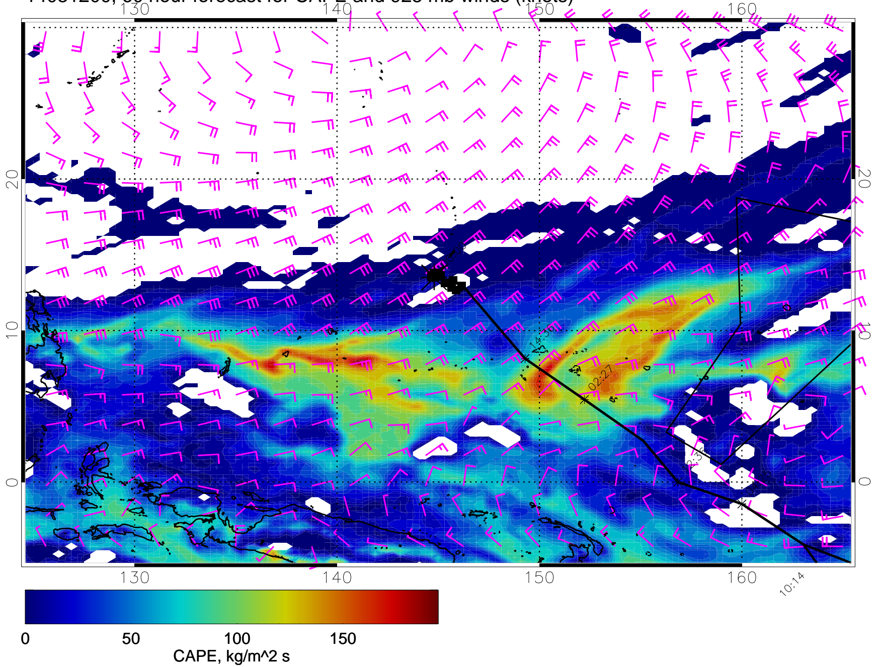
14031200, 60 hour forecast for CAPE and 925 mb winds (knots)
