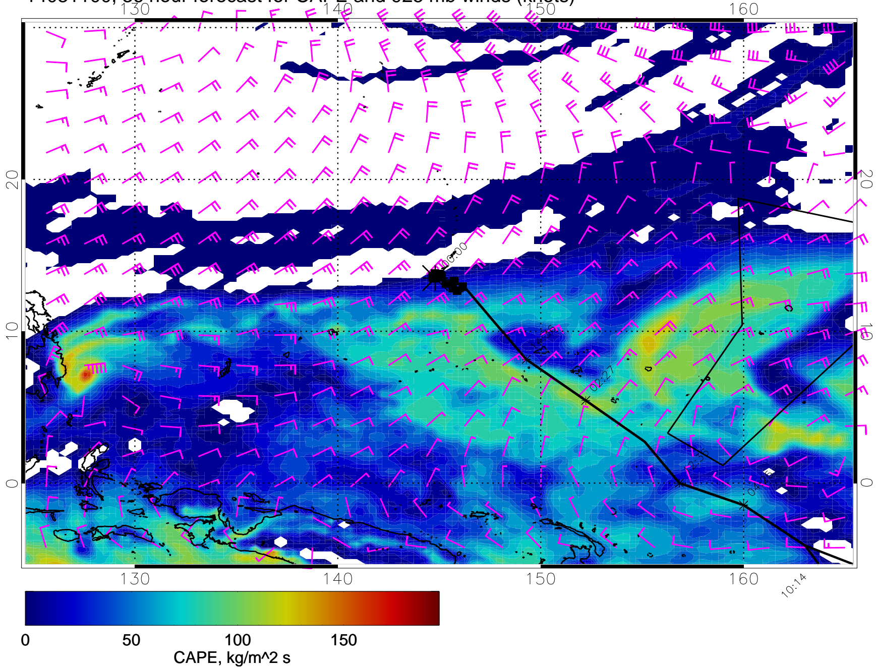
14031100, 36 hour forecast for CAPE and 925 mb winds (knots)
