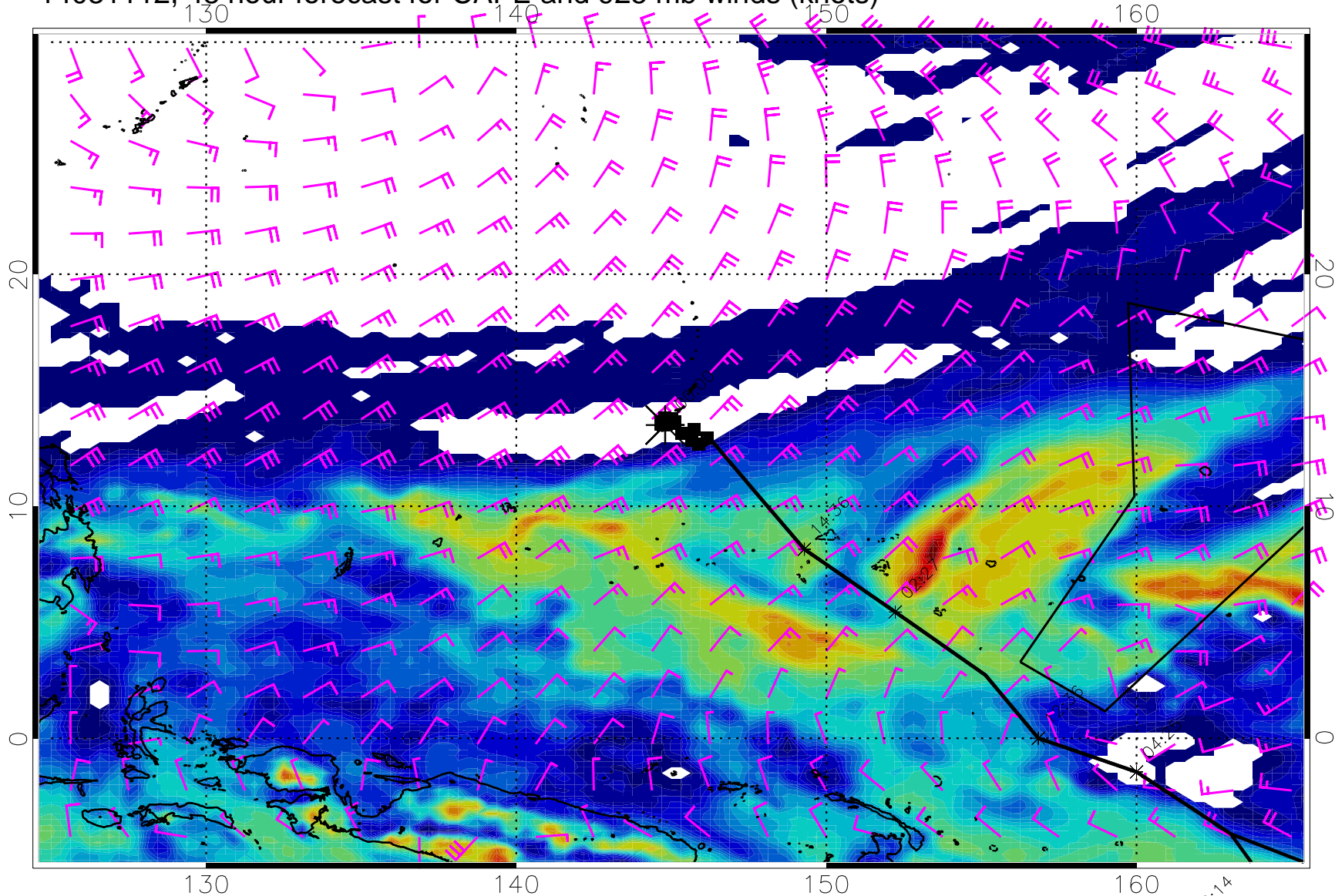
14031112, 48 hour forecast for CAPE and 925 mb winds (knots)
