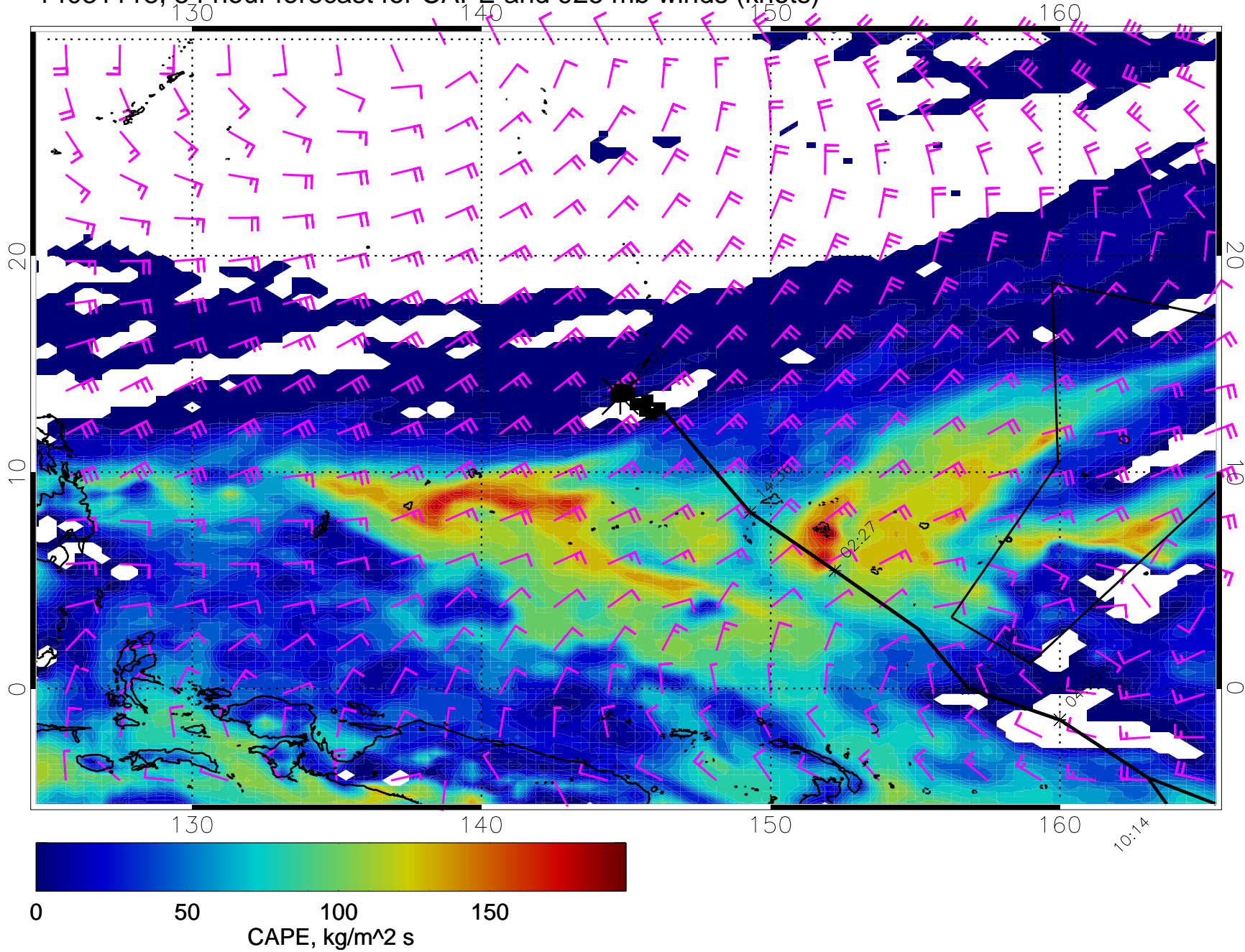
14031118, 54 hour forecast for CAPE and 925 mb winds (knots)
