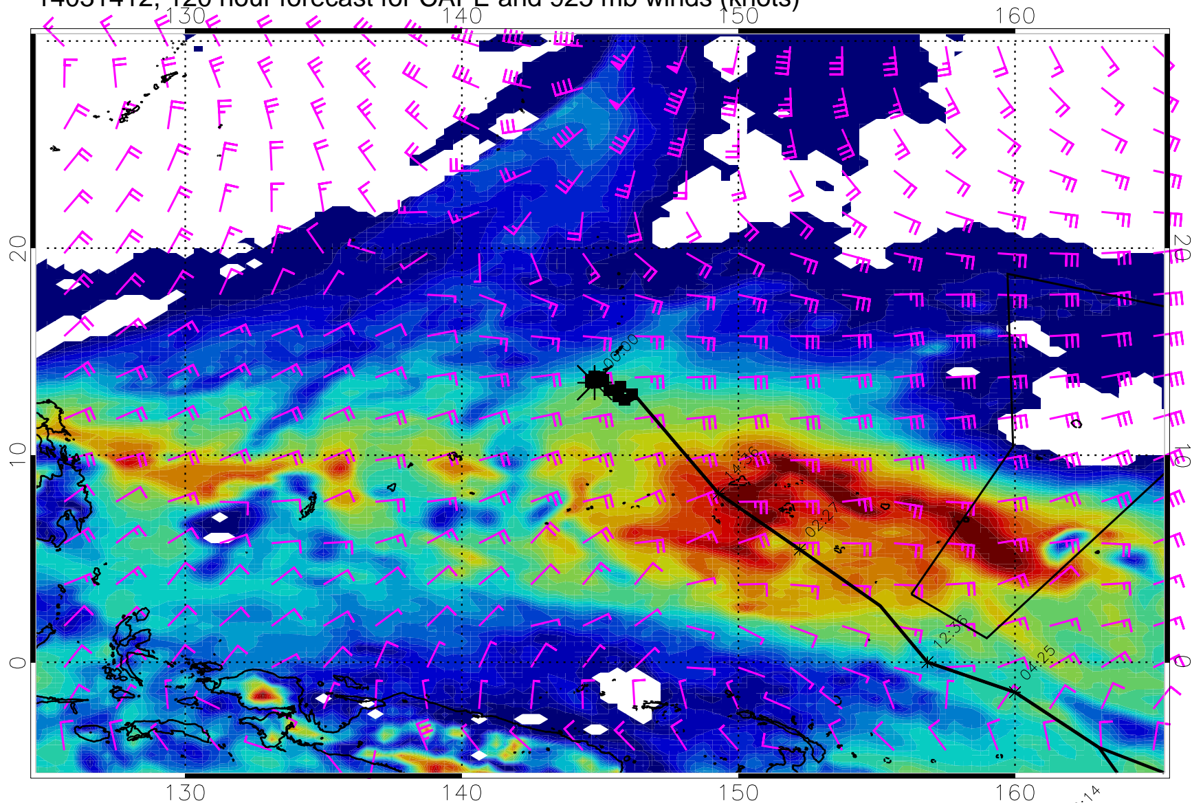
14031412, 120 hour forecast for CAPE and 925 mb winds (knots)
