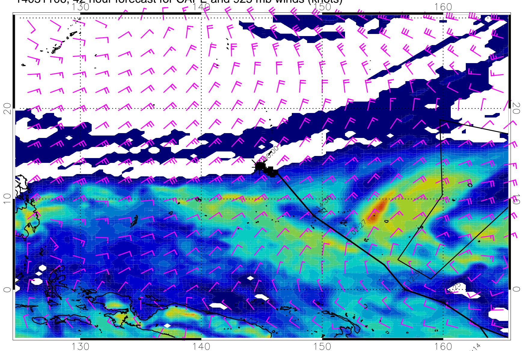
14031106, 42 hour forecast for CAPE and 925 mb winds (knots)
