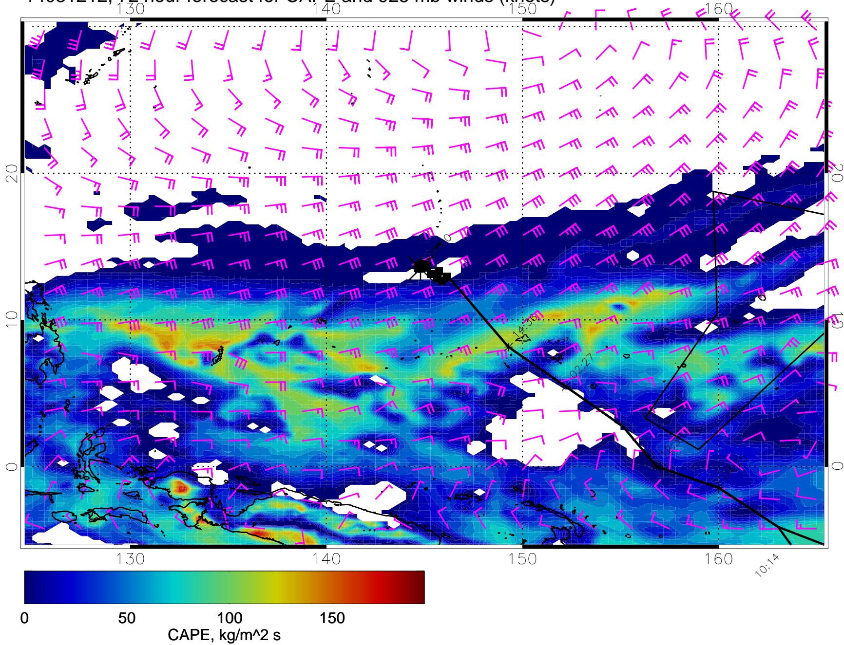
14031212, 72 hour forecast for CAPE and 925 mb winds (knots)
