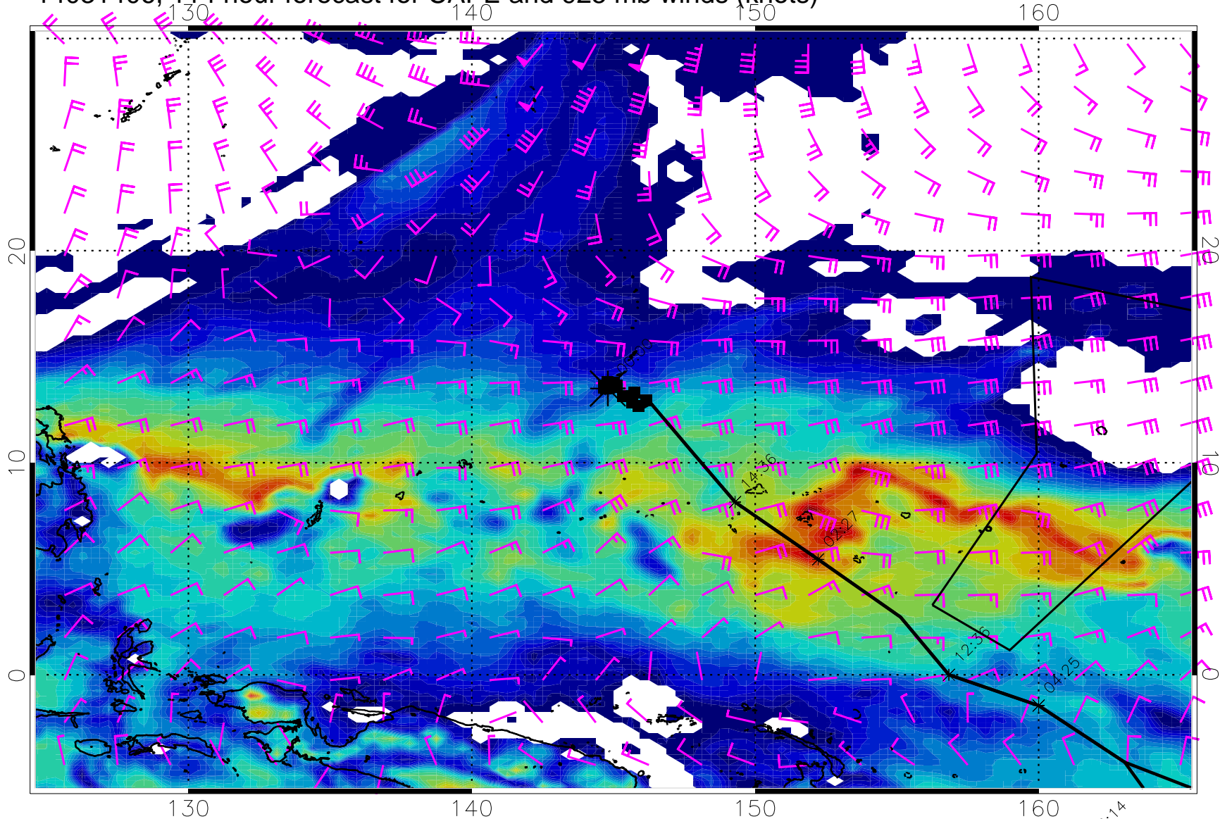
14031406, 114 hour forecast for CAPE and 925 mb winds (knots)
