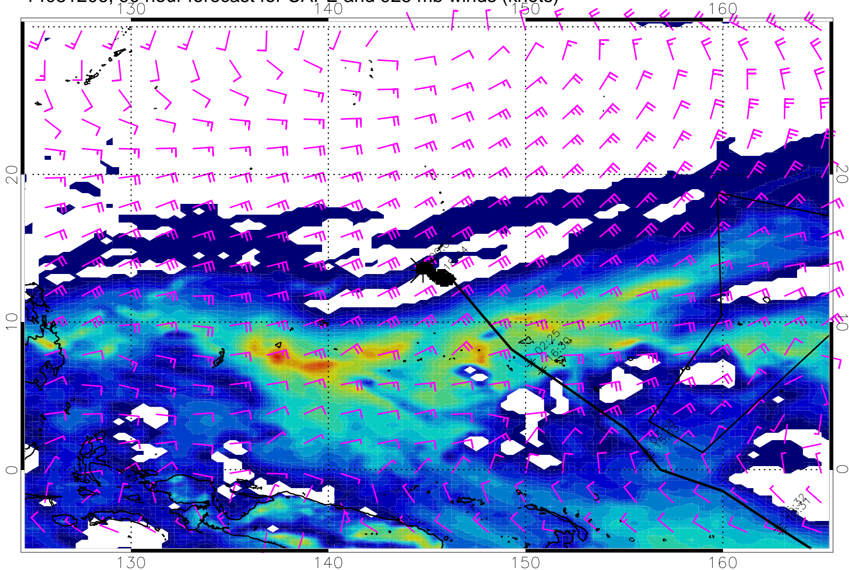
14031206, 90 hour forecast for CAPE and 925 mb winds (knots)
