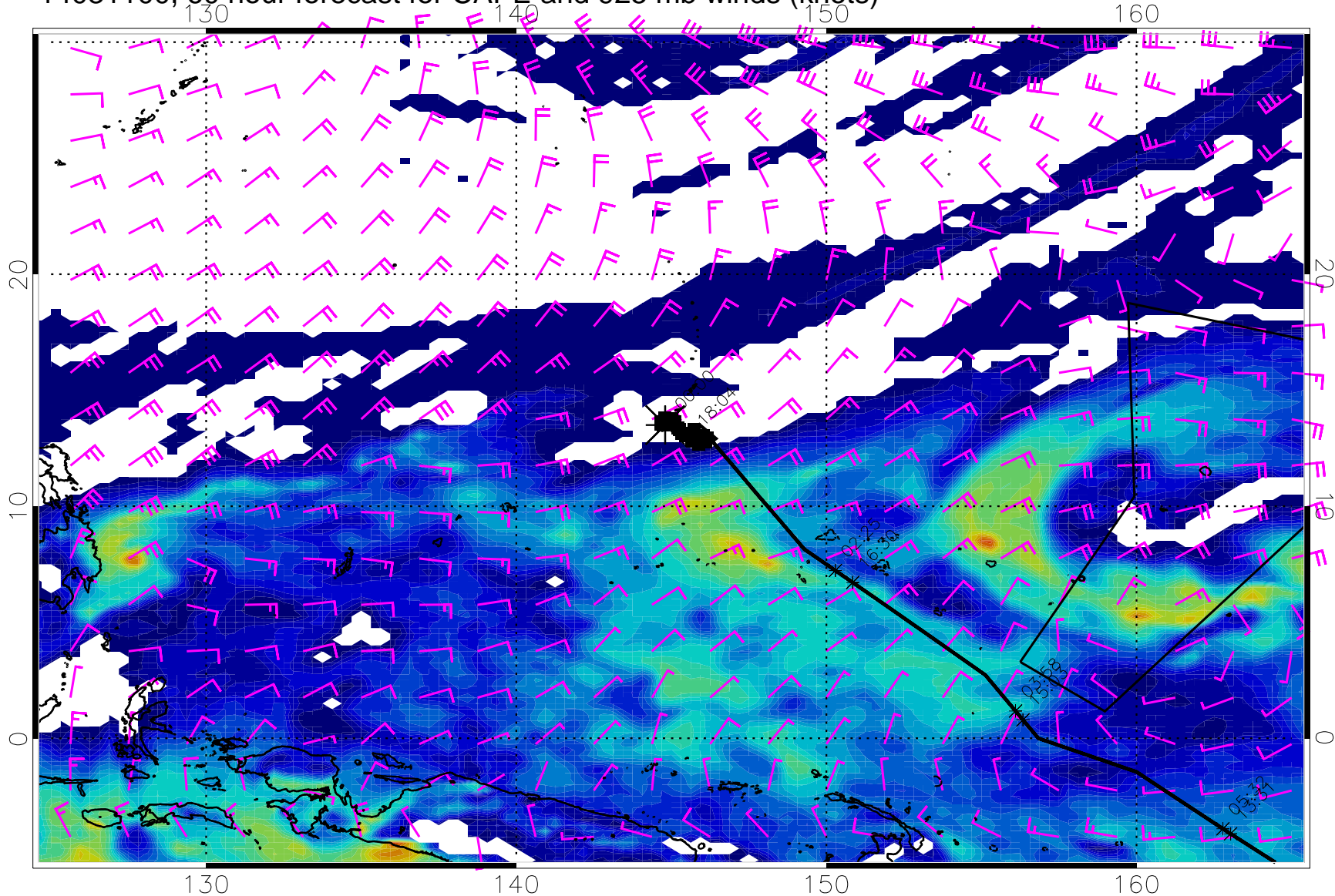
14031100, 60 hour forecast for CAPE and 925 mb winds (knots)
