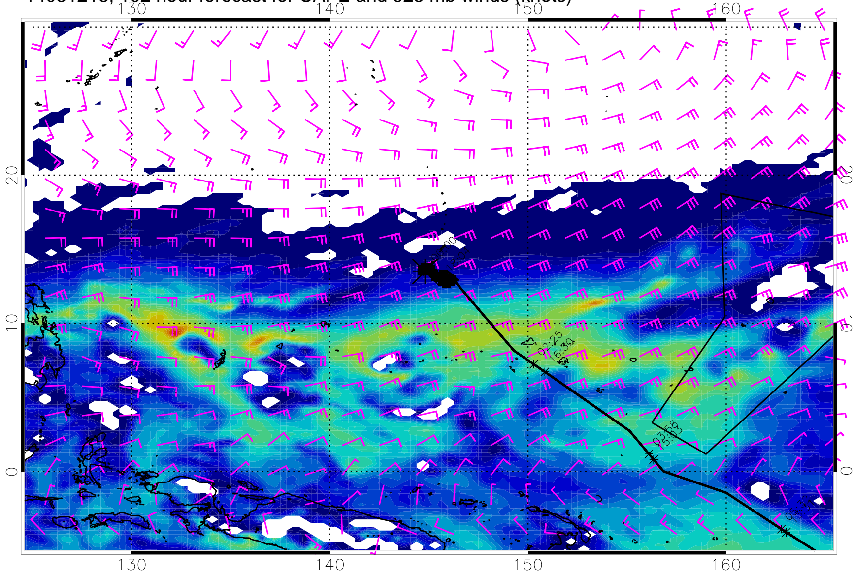
14031218, 102 hour forecast for CAPE and 925 mb winds (knots)
