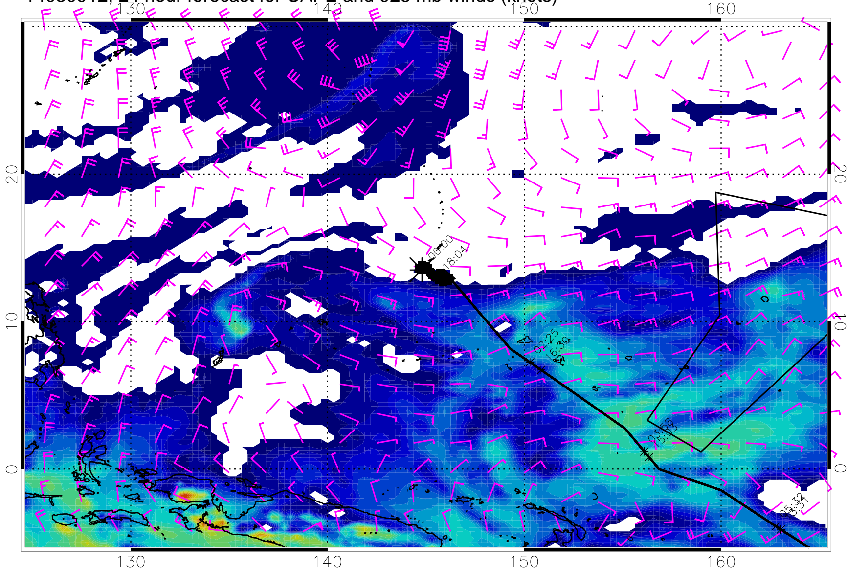
14030912, 24 hour forecast for CAPE and 925 mb winds (knots)
