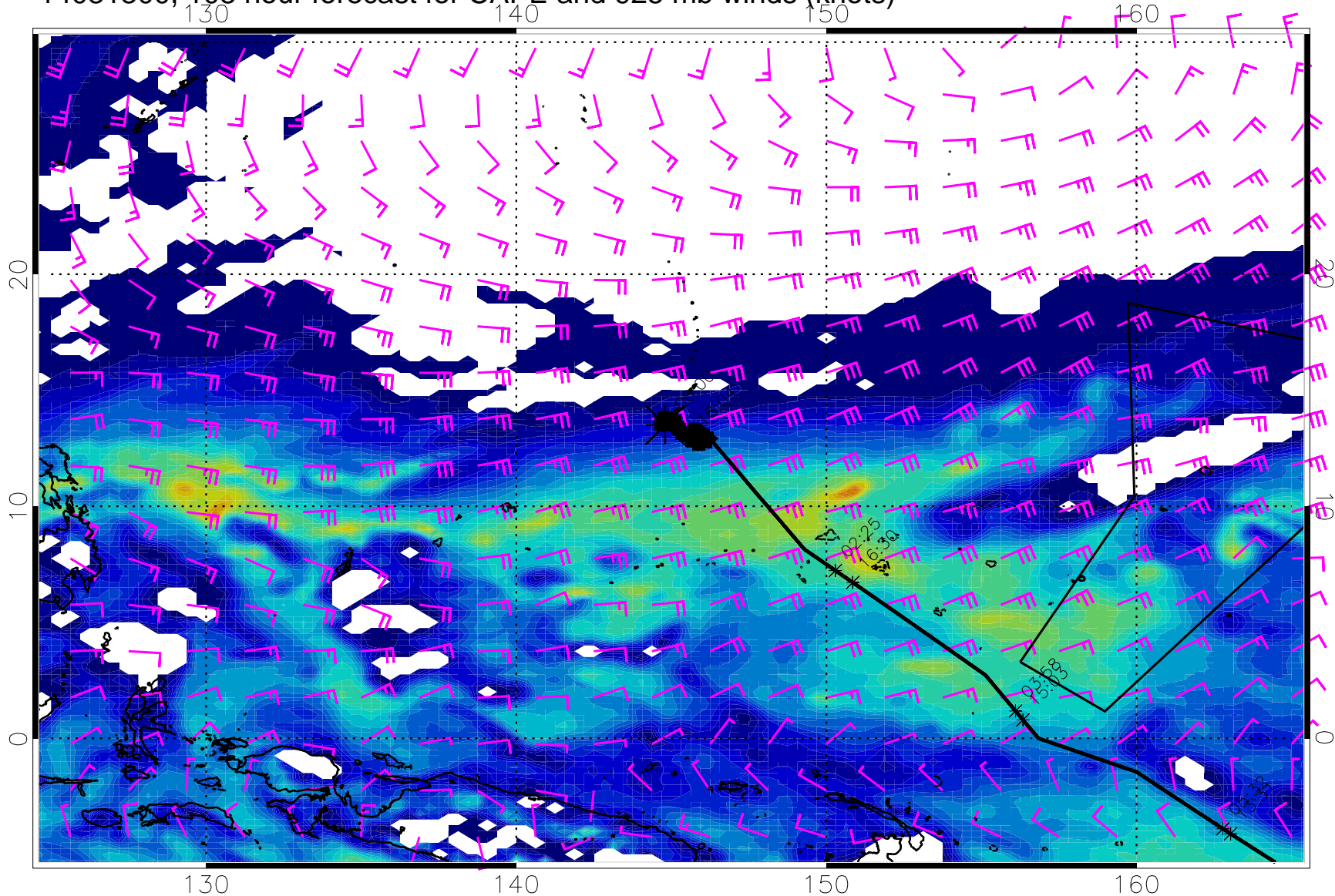
14031300, 108 hour forecast for CAPE and 925 mb winds (knots)
