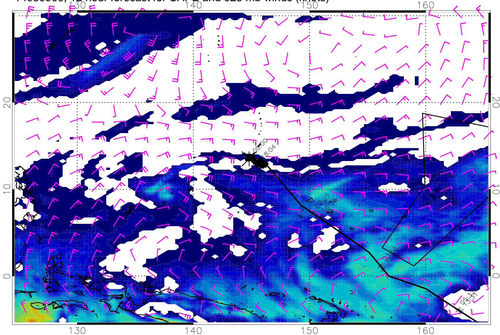
14030900, 12 hour forecast for CAPE and 925 mb winds (knots)
