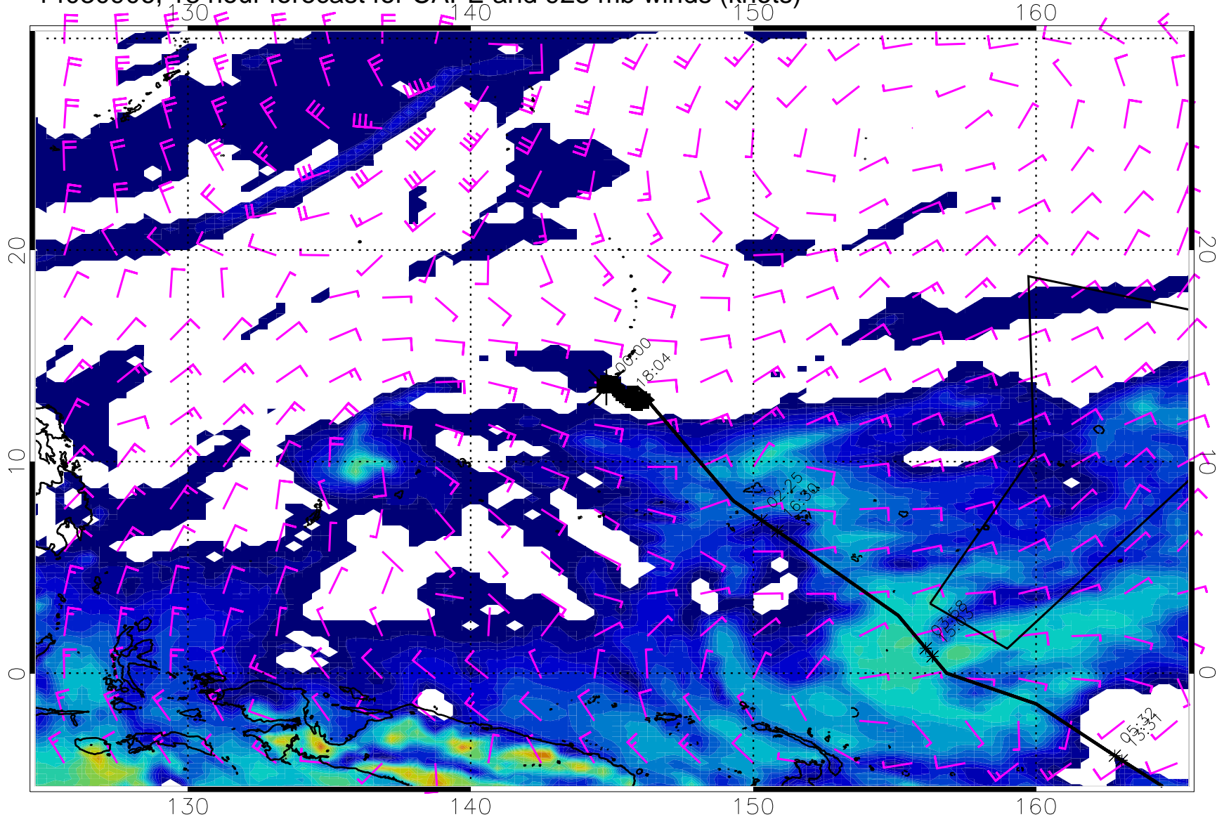
14030906, 18 hour forecast for CAPE and 925 mb winds (knots)
