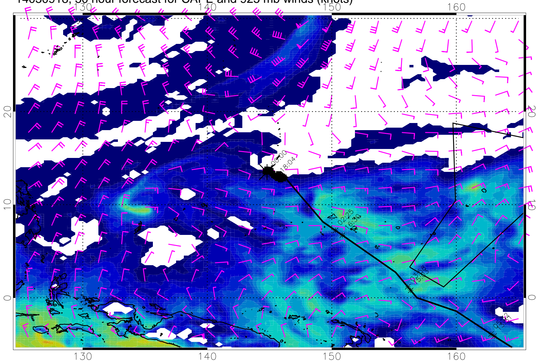
14030918, 30 hour forecast for CAPE and 925 mb winds (knots)
