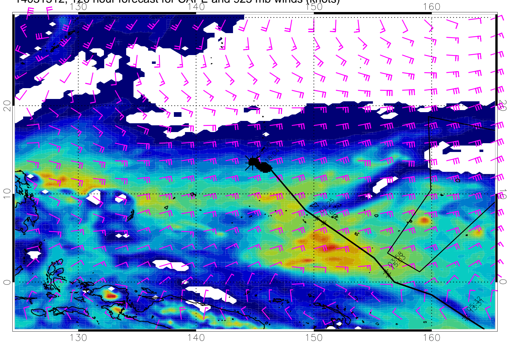
14031312, 120 hour forecast for CAPE and 925 mb winds (knots)
