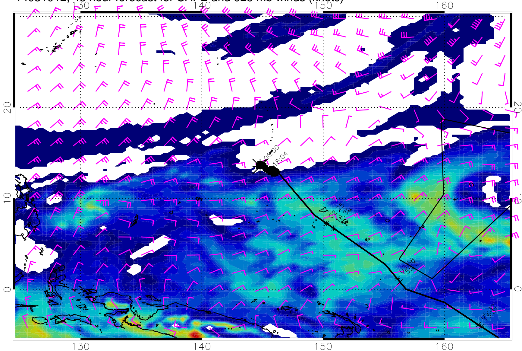
14031012, 48 hour forecast for CAPE and 925 mb winds (knots)
