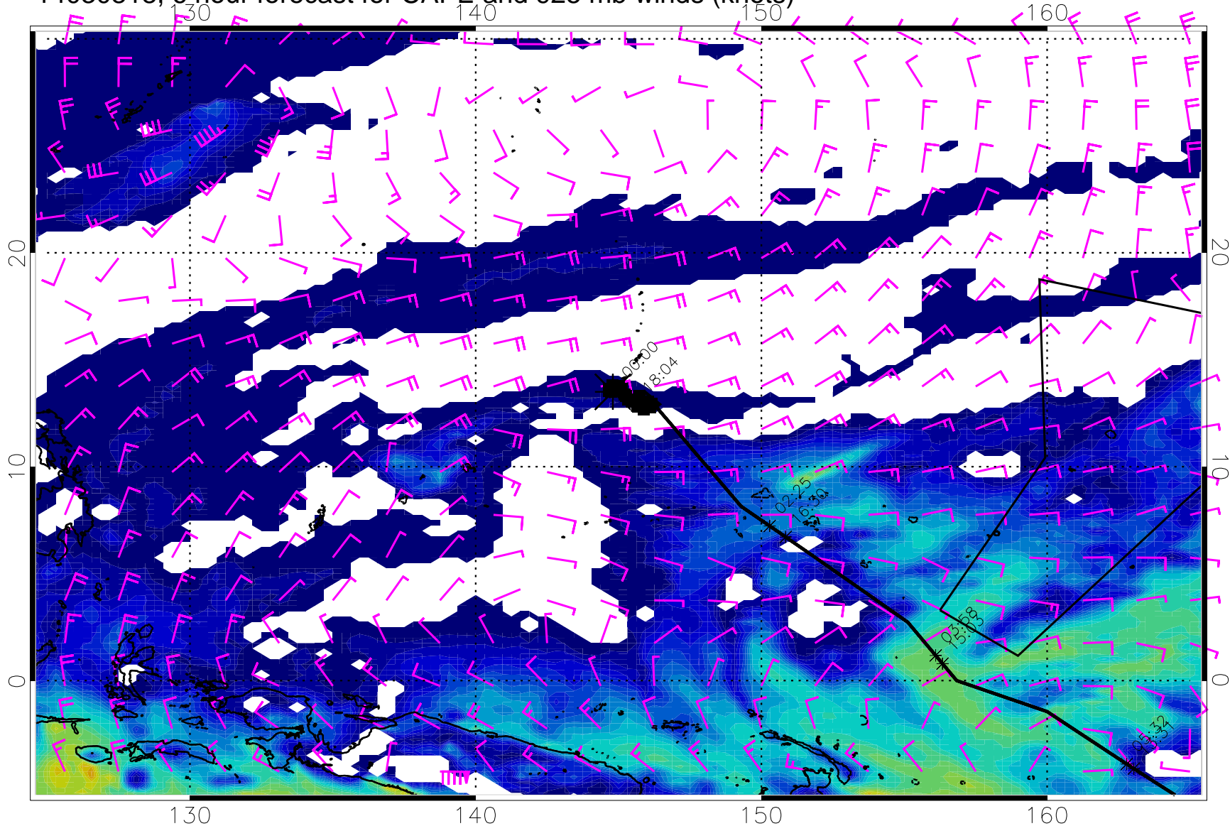
14030818, 6 hour forecast for CAPE and 925 mb winds (knots)
