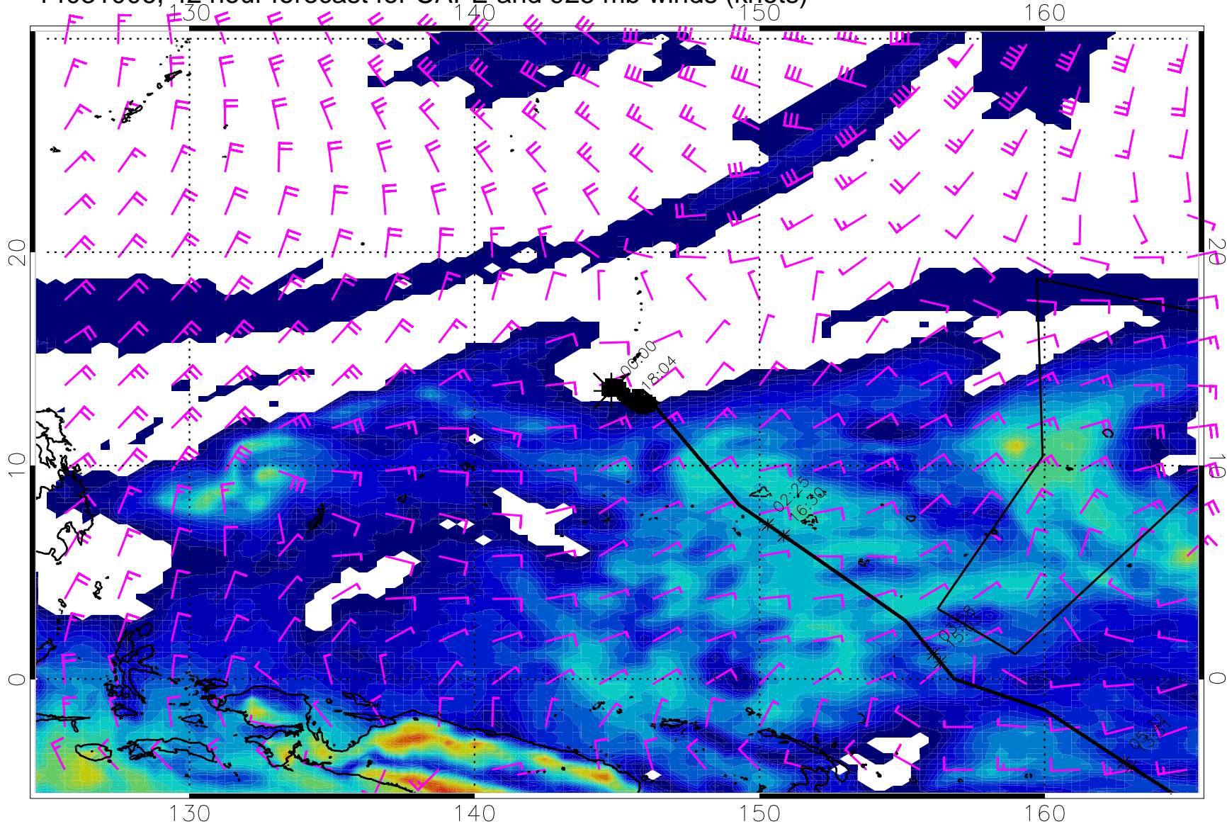
14031006, 42 hour forecast for CAPE and 925 mb winds (knots)
