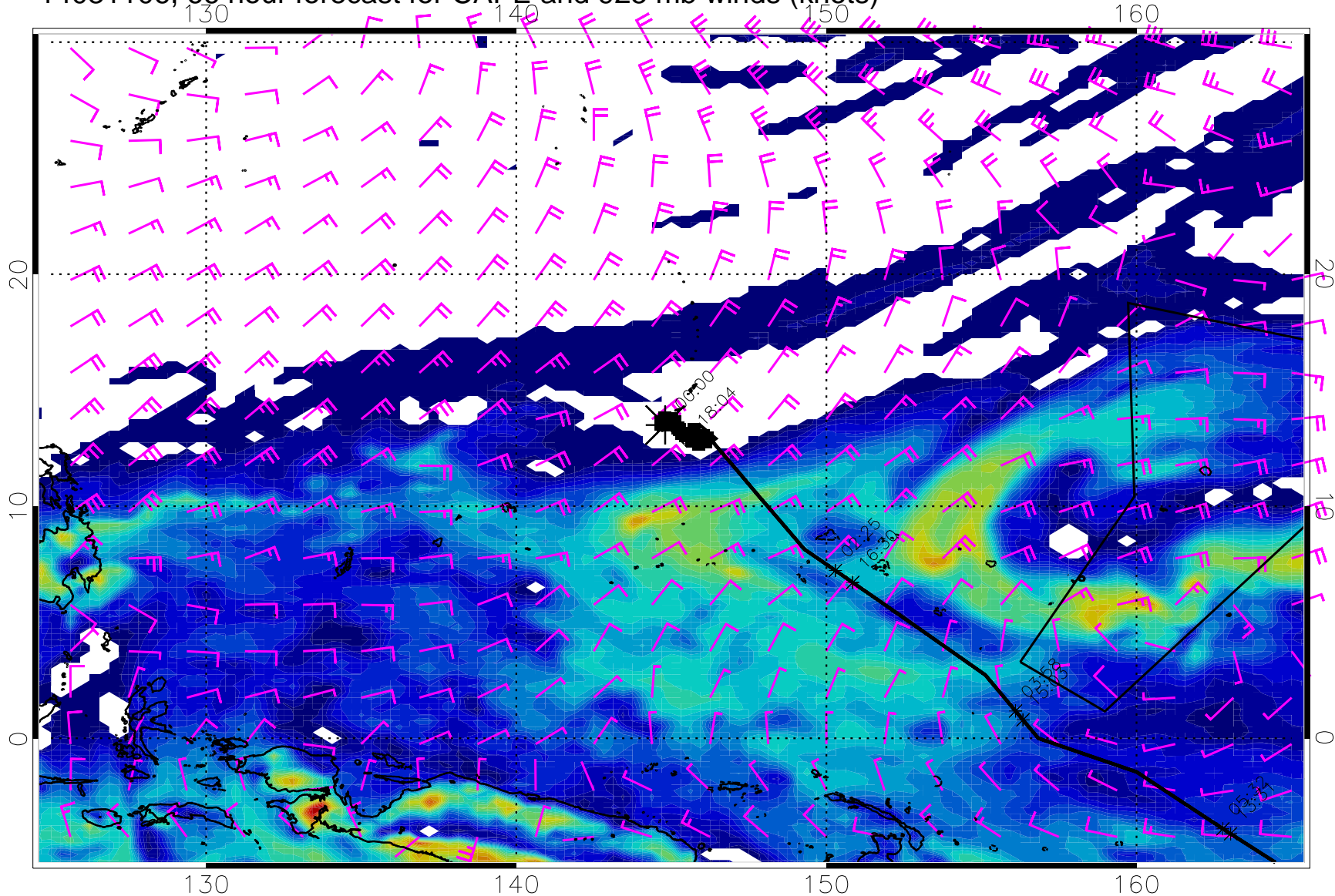
14031106, 66 hour forecast for CAPE and 925 mb winds (knots)
