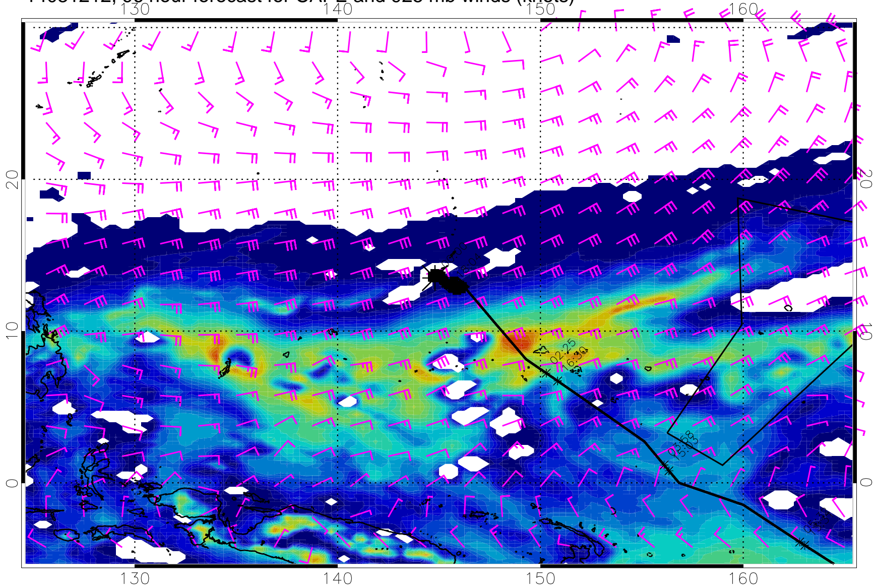
14031212, 96 hour forecast for CAPE and 925 mb winds (knots)
