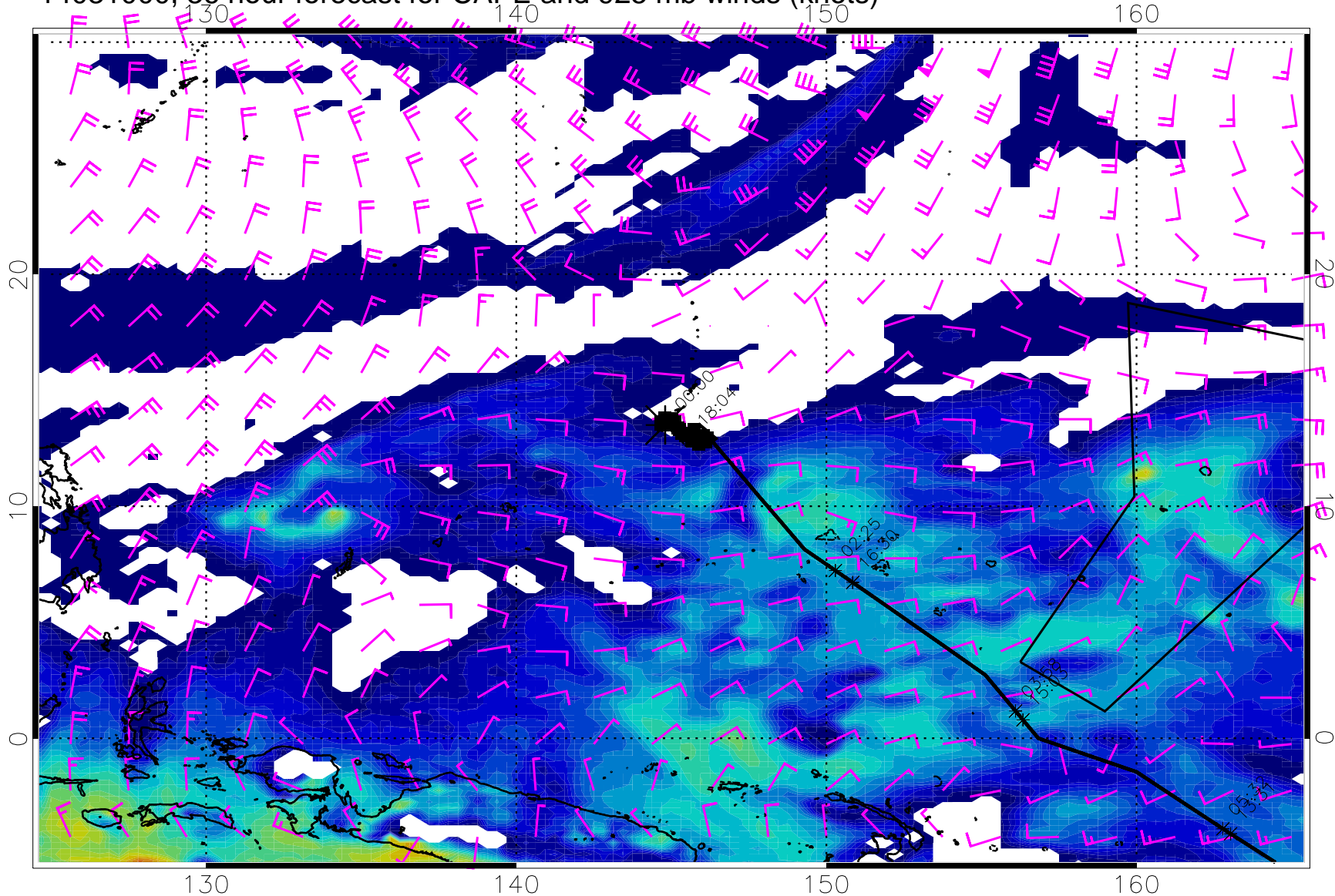
14031000, 36 hour forecast for CAPE and 925 mb winds (knots)
