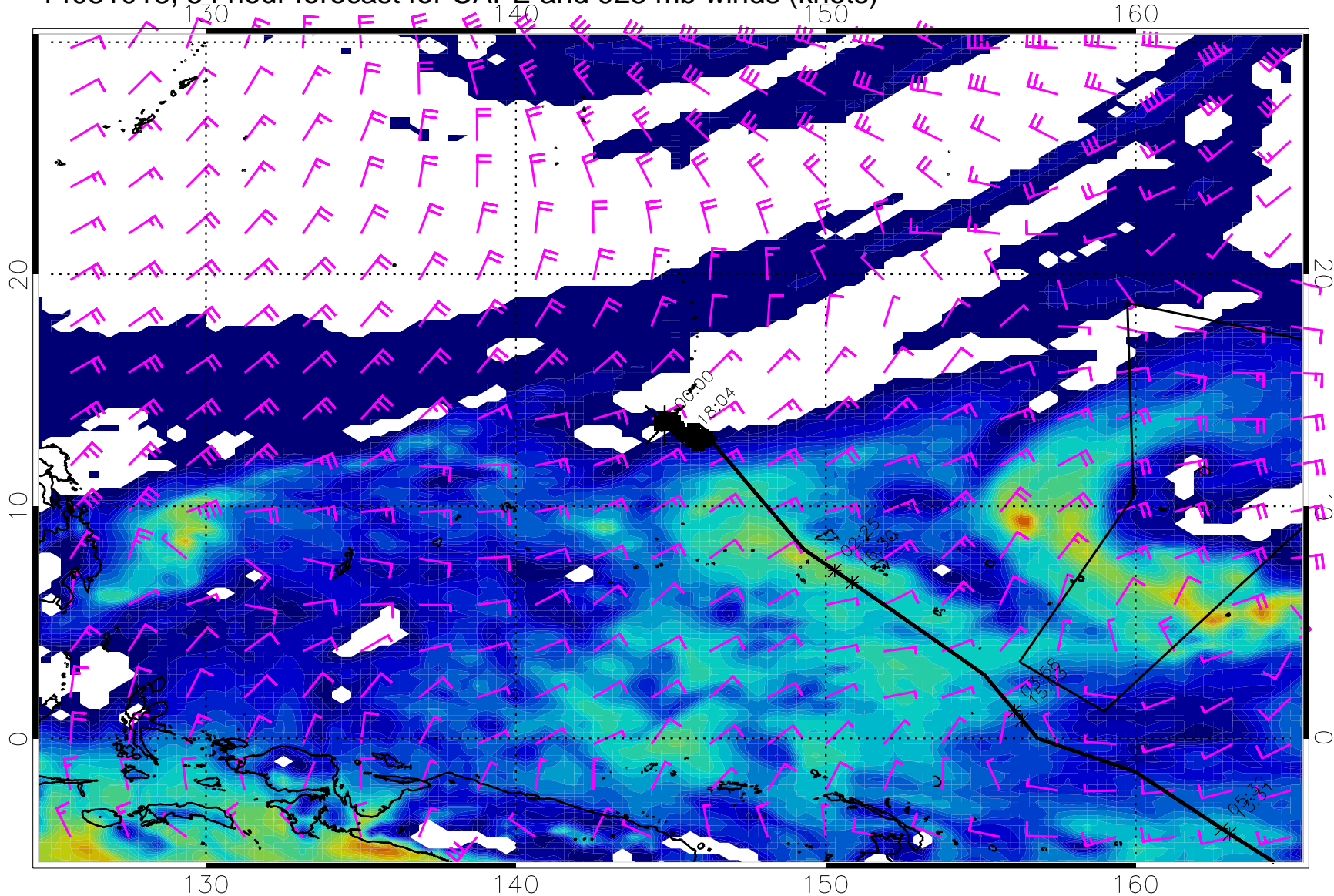
14031018, 54 hour forecast for CAPE and 925 mb winds (knots)
