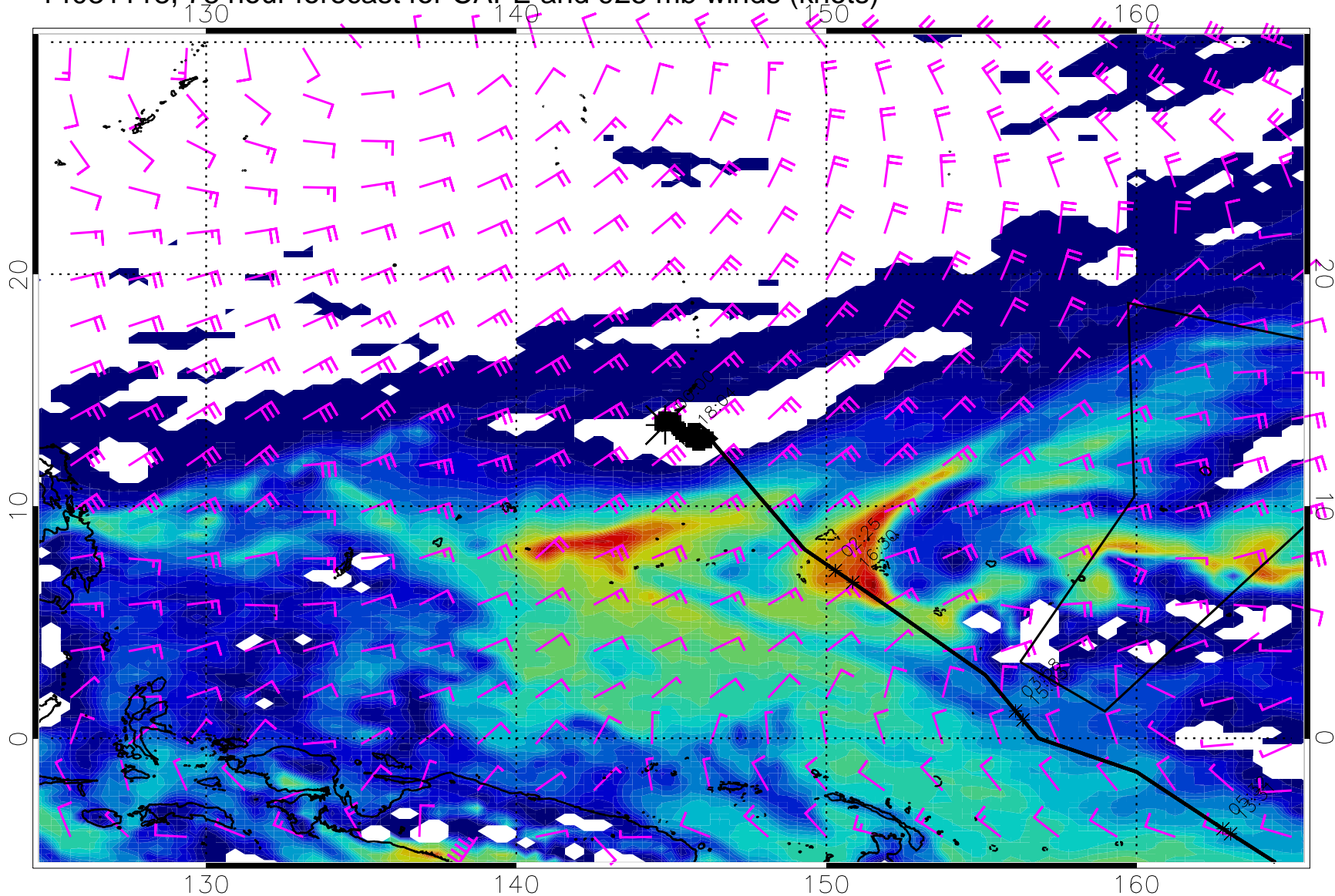
14031118, 78 hour forecast for CAPE and 925 mb winds (knots)
