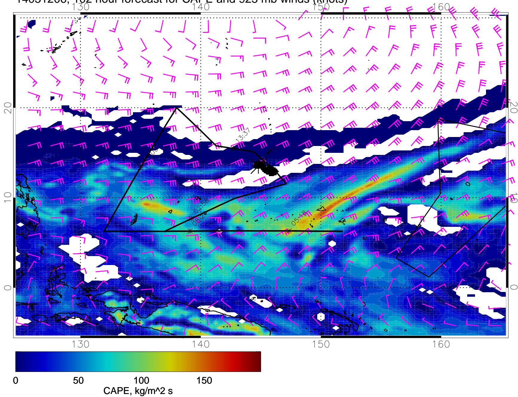
14031206, 102 hour forecast for CAPE and 925 mb winds (knots)
