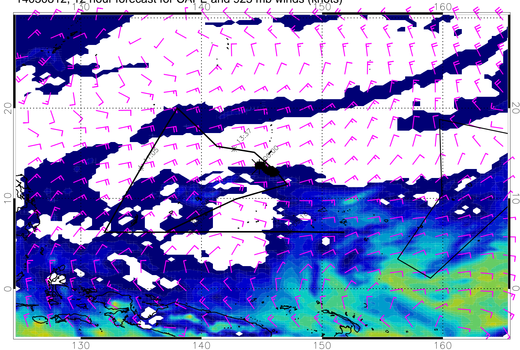
14030812, 12 hour forecast for CAPE and 925 mb winds (knots)
