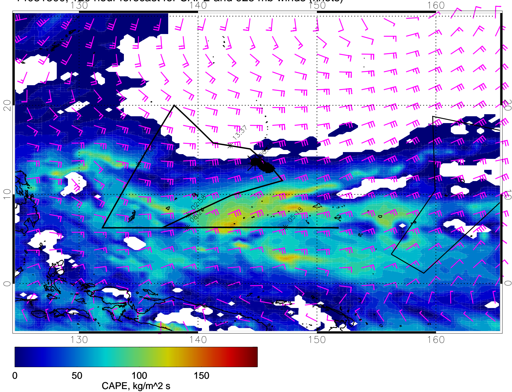
14031300, 120 hour forecast for CAPE and 925 mb winds (knots)
