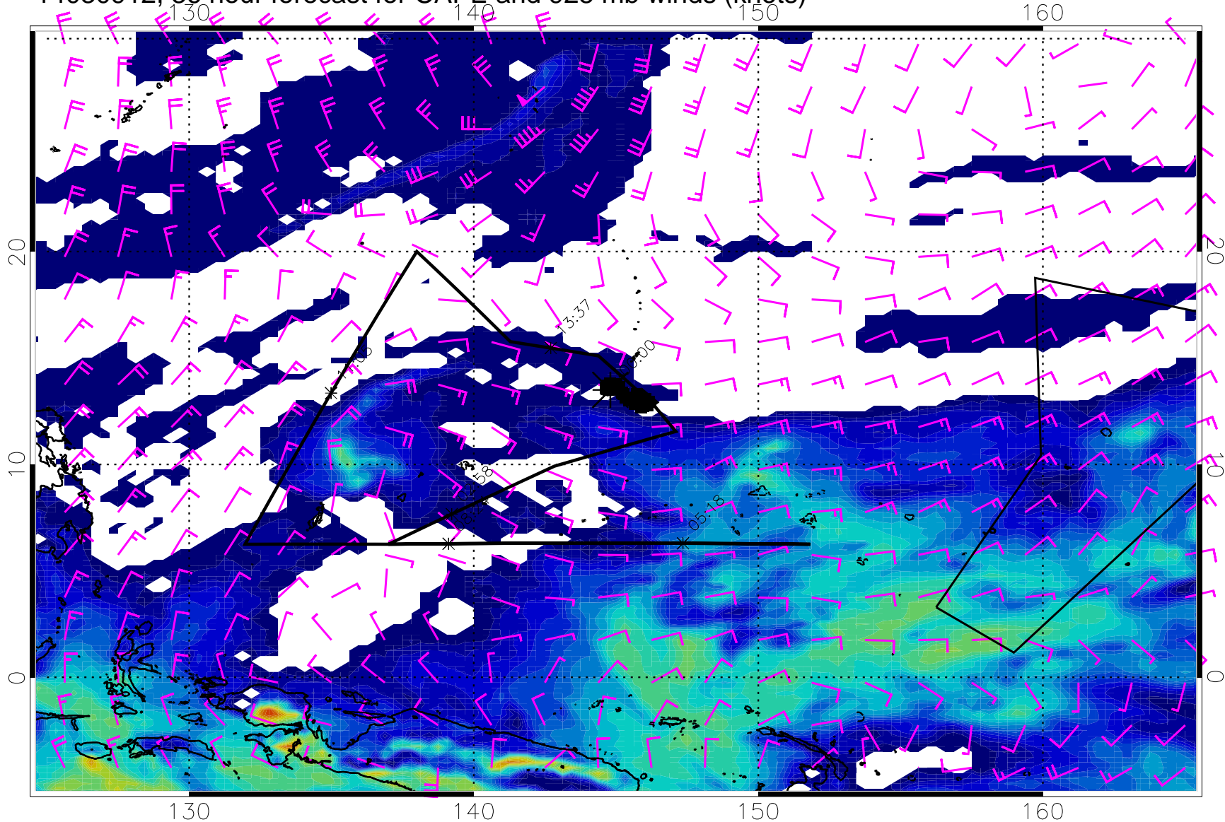
14030912, 36 hour forecast for CAPE and 925 mb winds (knots)
