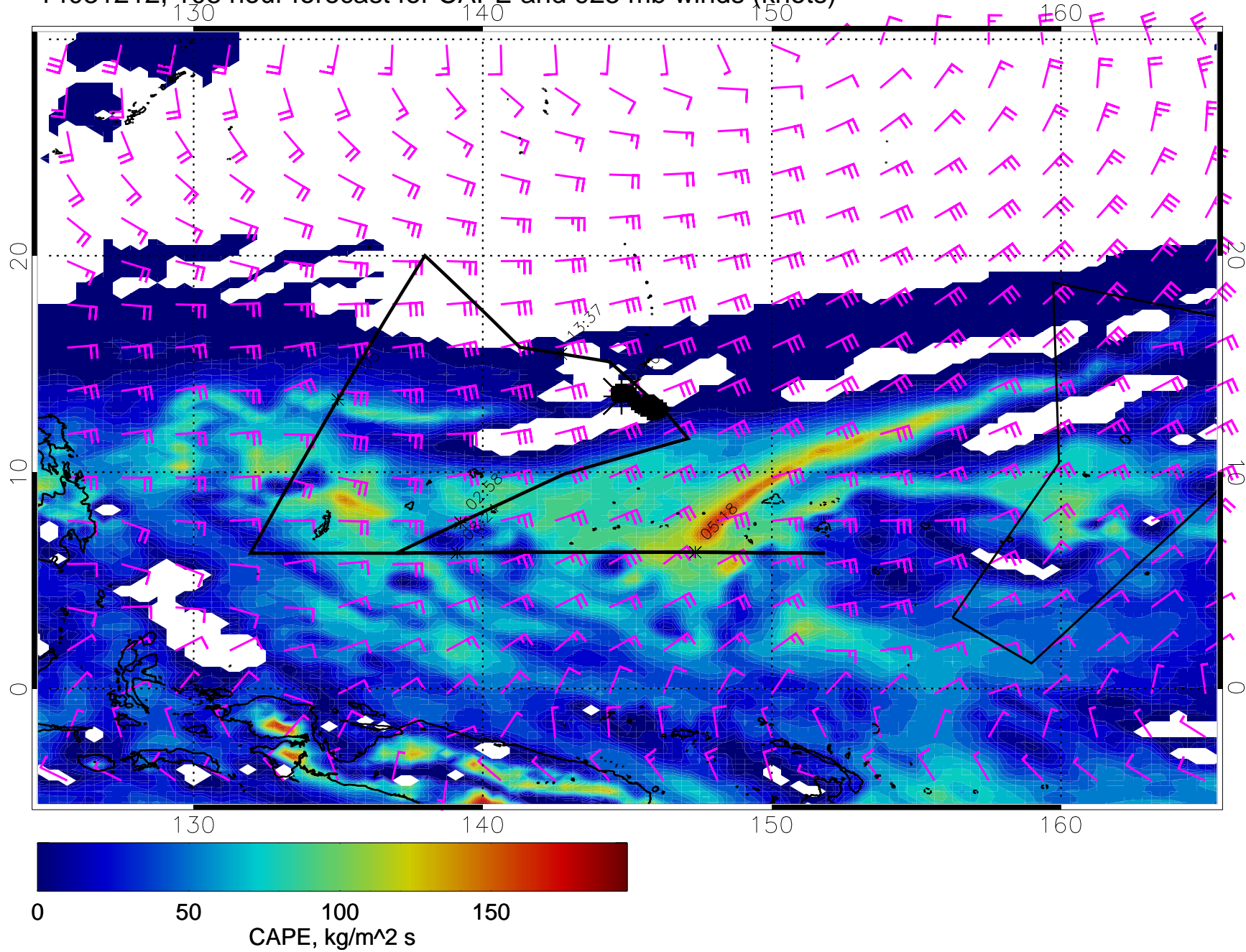
14031212, 108 hour forecast for CAPE and 925 mb winds (knots)
