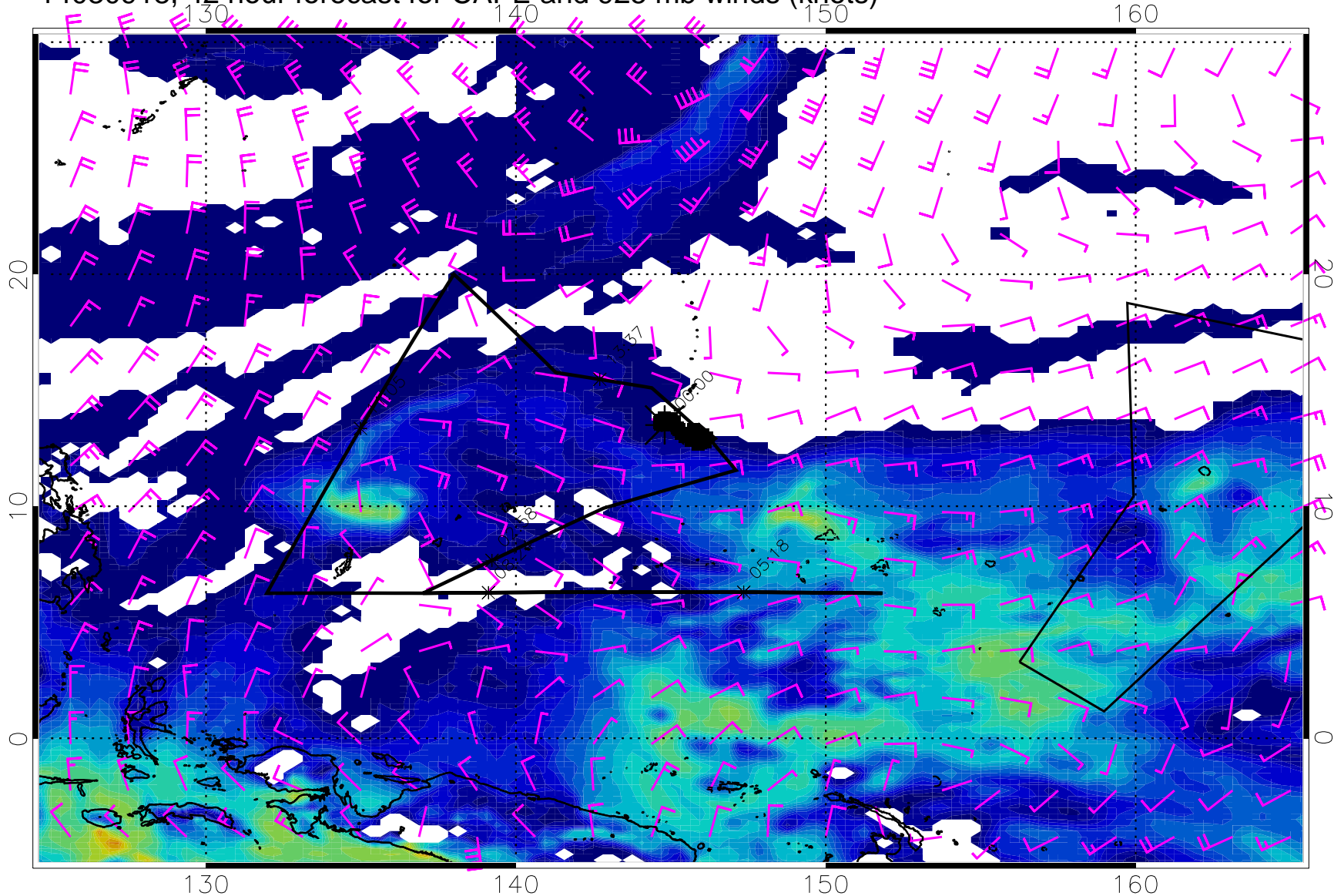
14030918, 42 hour forecast for CAPE and 925 mb winds (knots)
