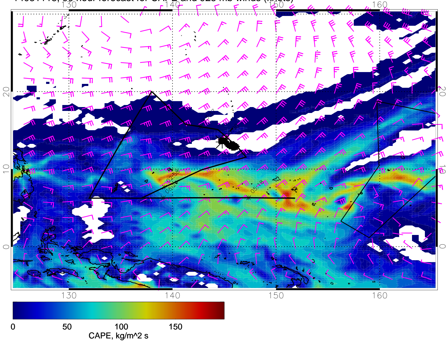
14031118, 90 hour forecast for CAPE and 925 mb winds (knots)
