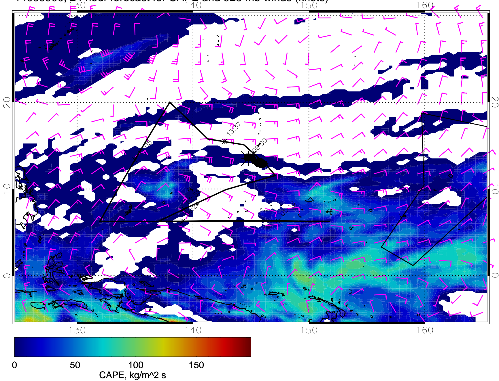
14030900, 24 hour forecast for CAPE and 925 mb winds (knots)
