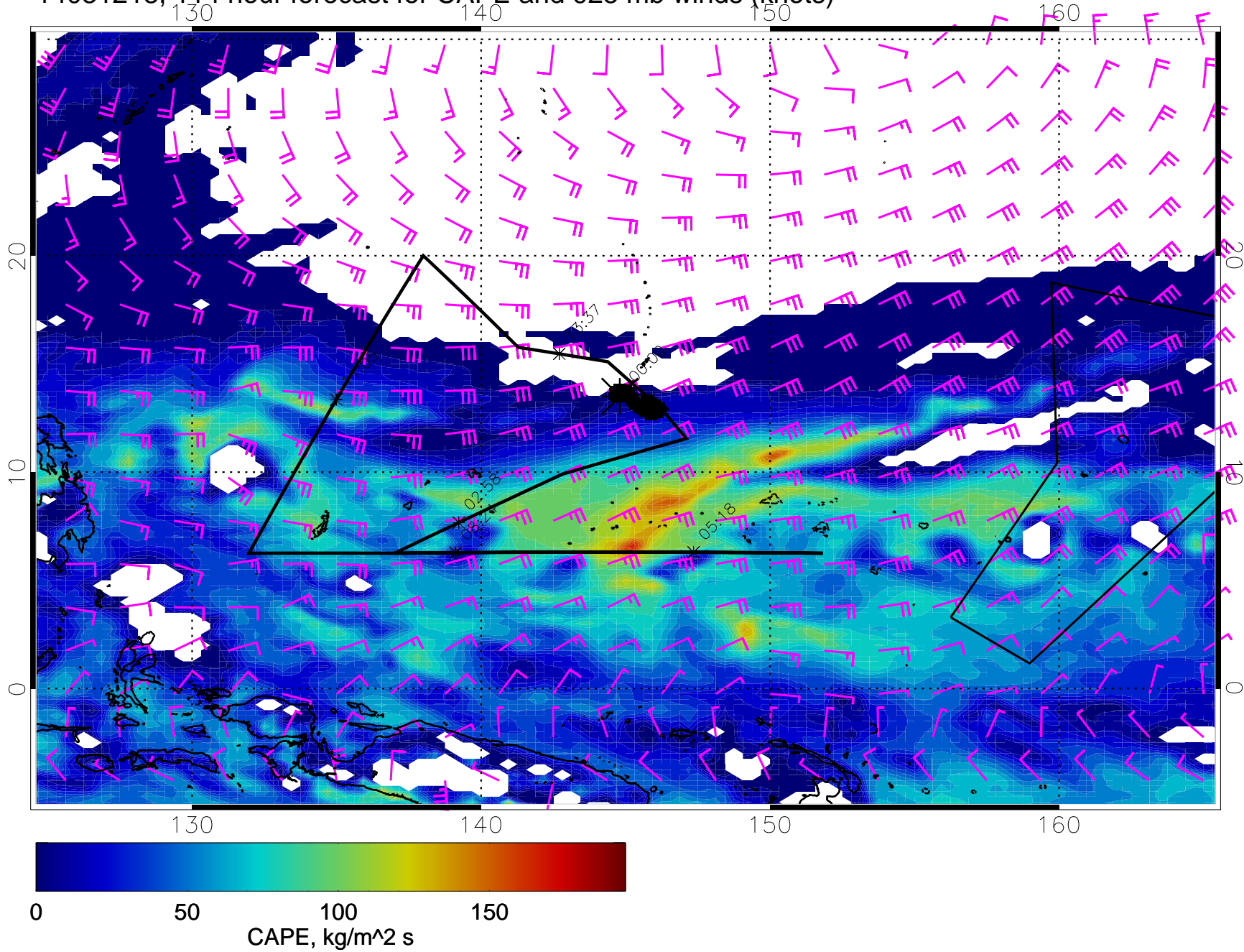
14031218, 114 hour forecast for CAPE and 925 mb winds (knots)
