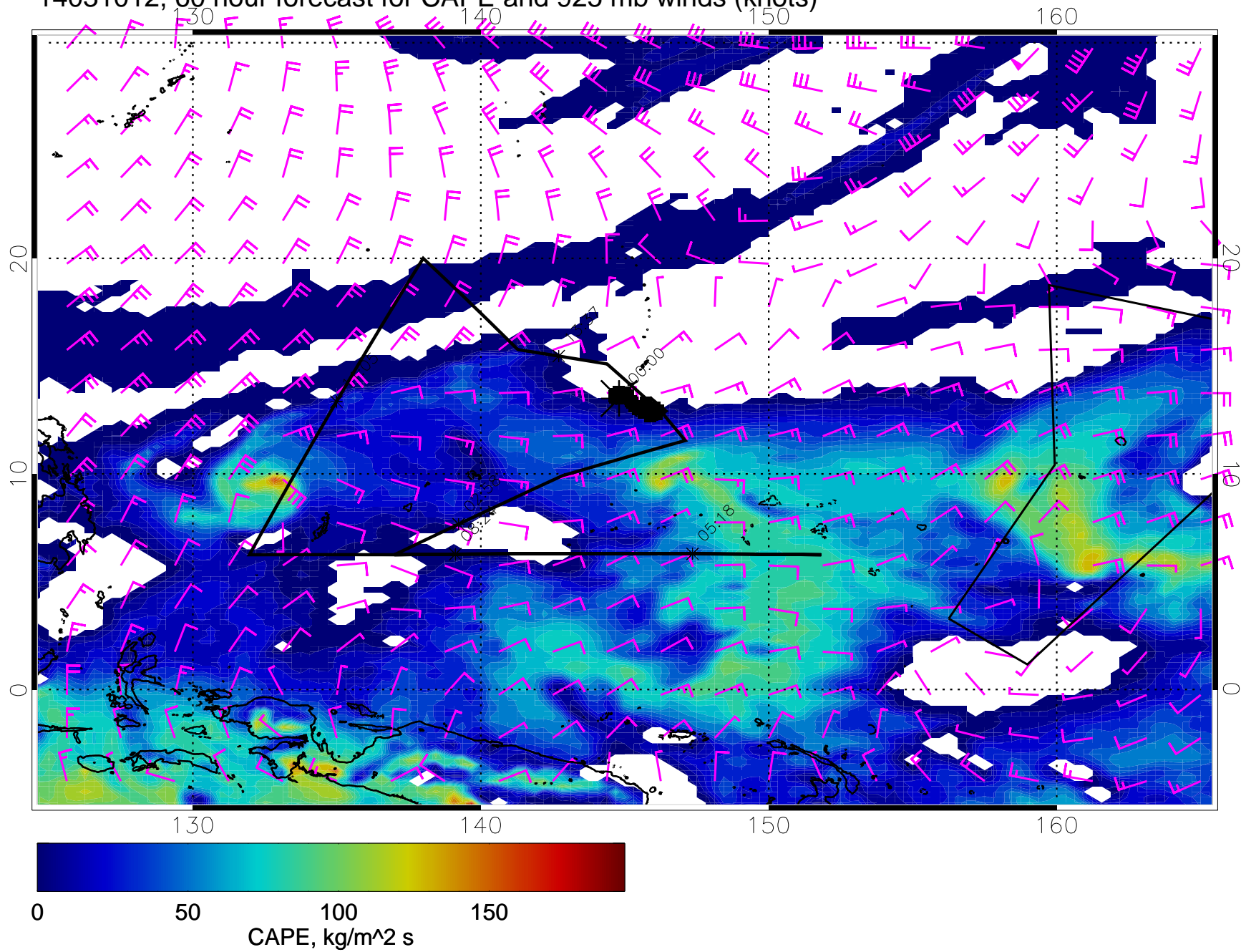
14031012, 60 hour forecast for CAPE and 925 mb winds (knots)
