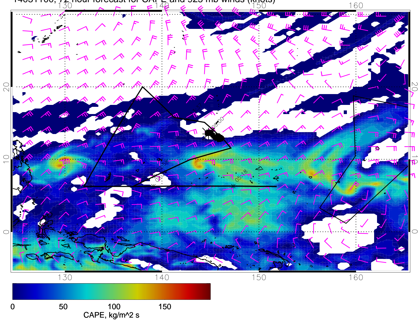
14031100, 72 hour forecast for CAPE and 925 mb winds (knots)
