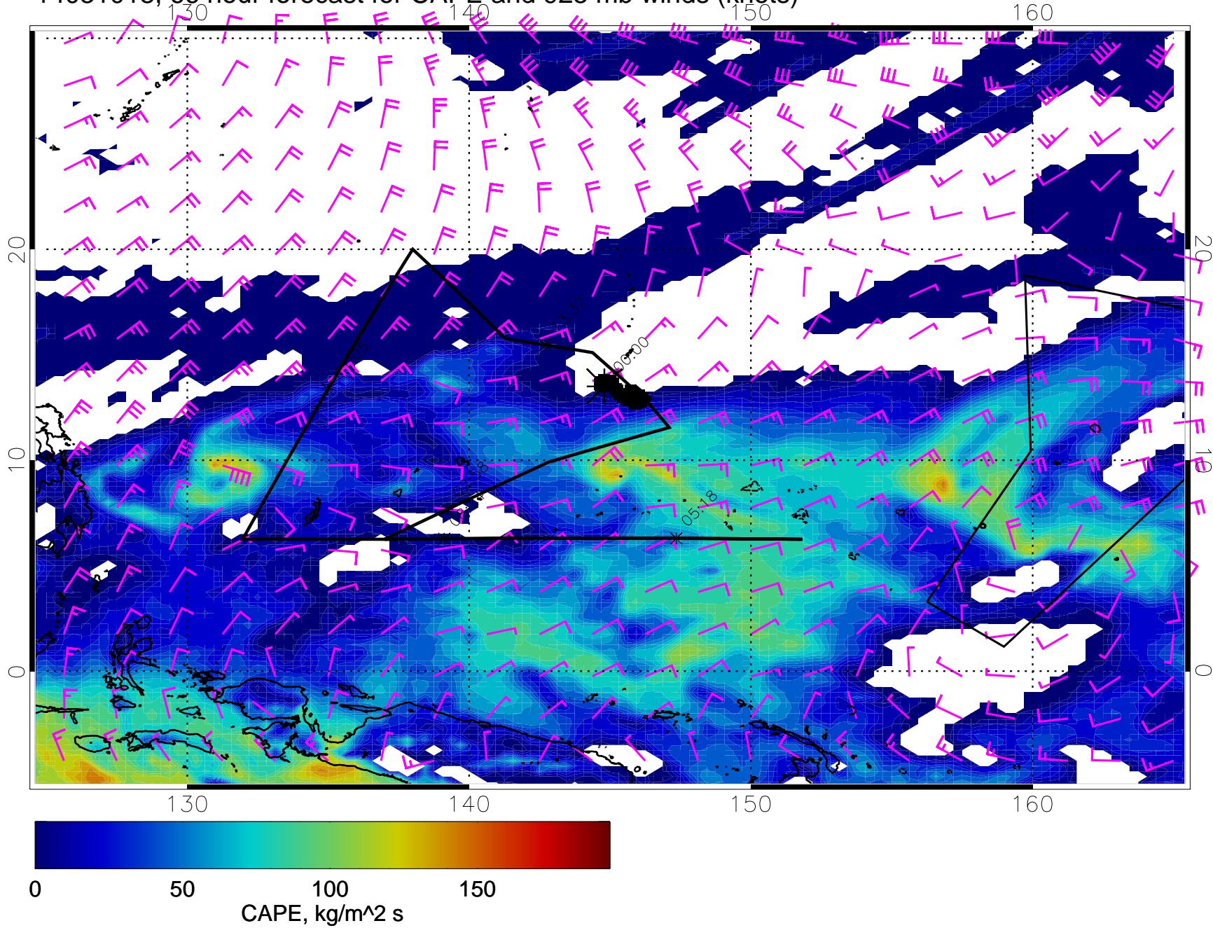
14031018, 66 hour forecast for CAPE and 925 mb winds (knots)
