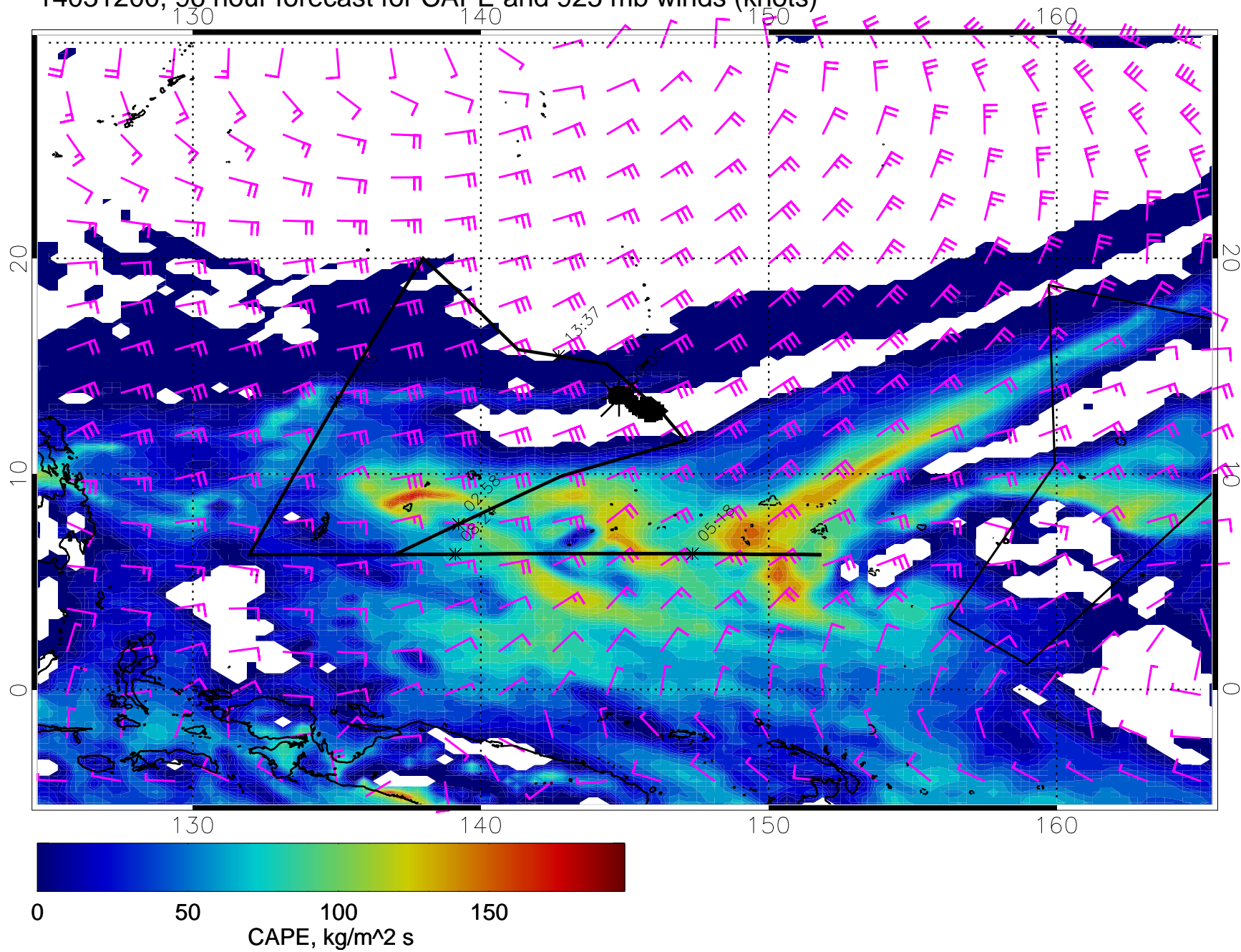
14031200, 96 hour forecast for CAPE and 925 mb winds (knots)
