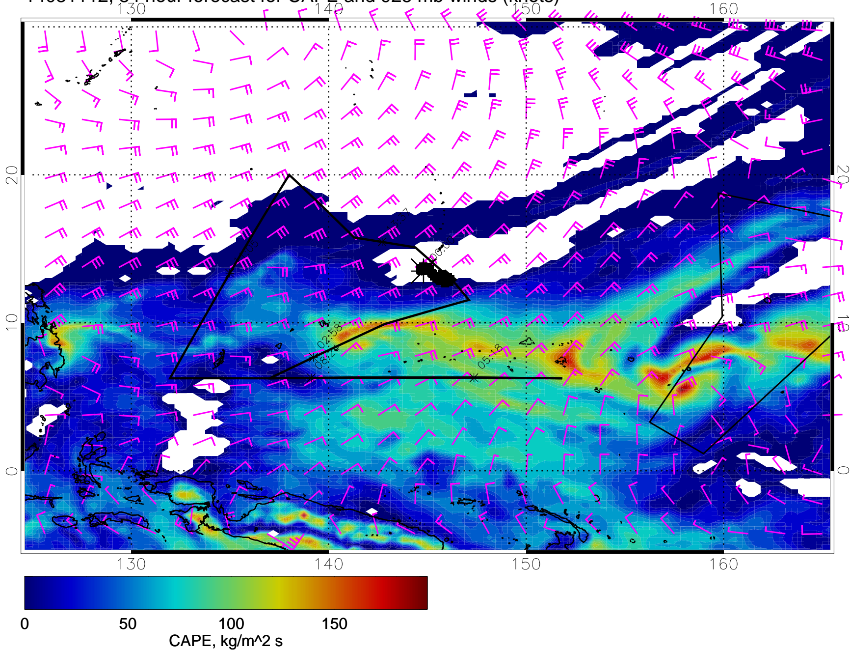
14031112, 84 hour forecast for CAPE and 925 mb winds (knots)
