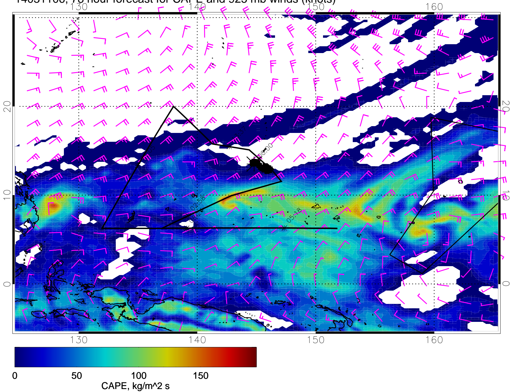
14031106, 78 hour forecast for CAPE and 925 mb winds (knots)
