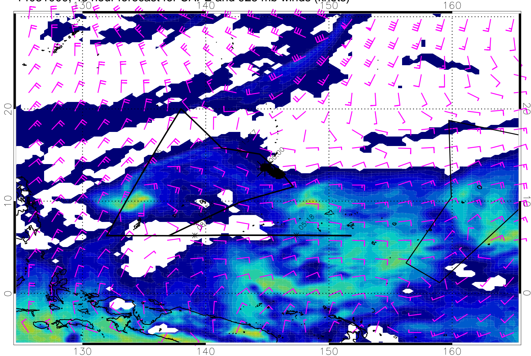
14031000, 48 hour forecast for CAPE and 925 mb winds (knots)
