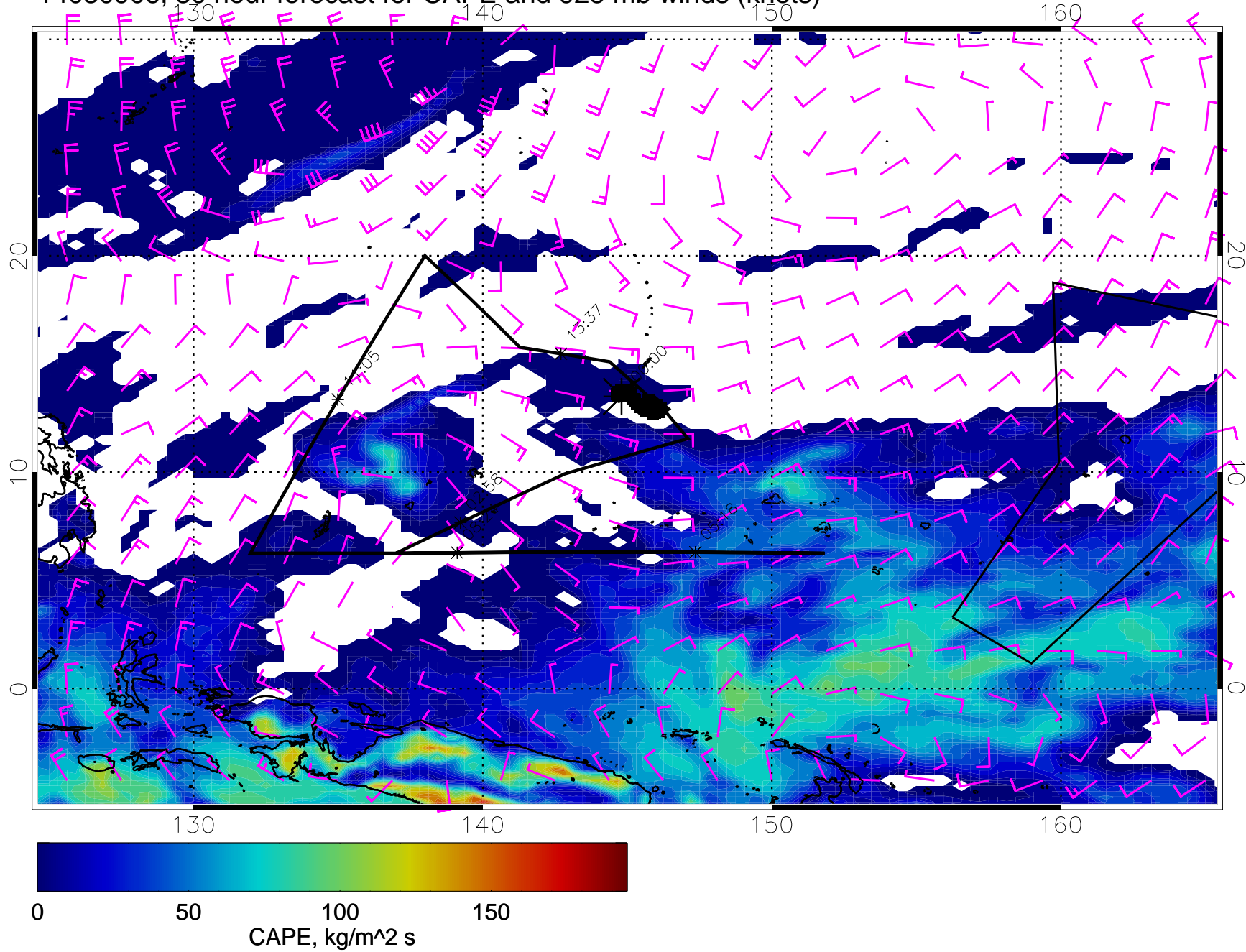
14030906, 30 hour forecast for CAPE and 925 mb winds (knots)
