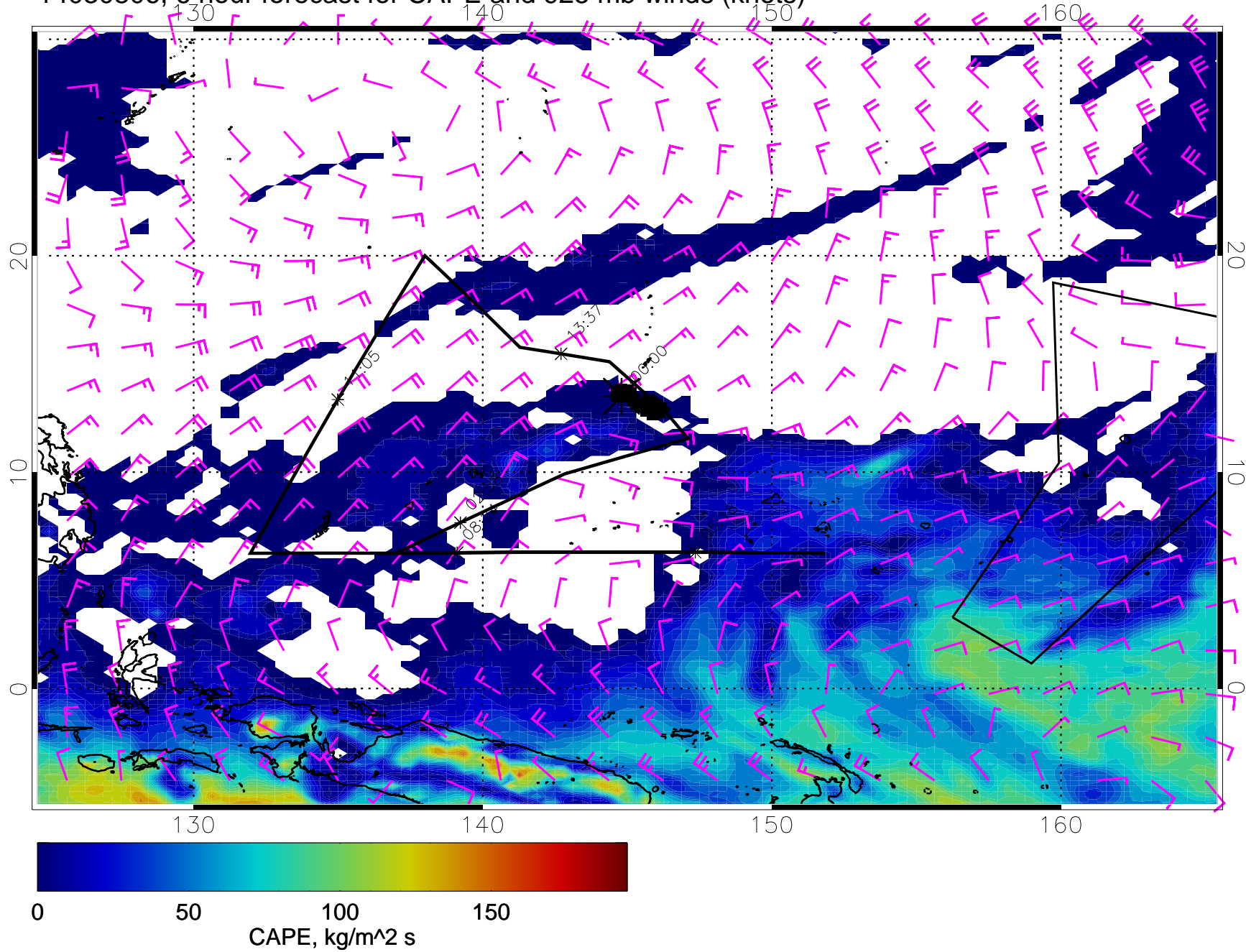
14030806, 6 hour forecast for CAPE and 925 mb winds (knots)
