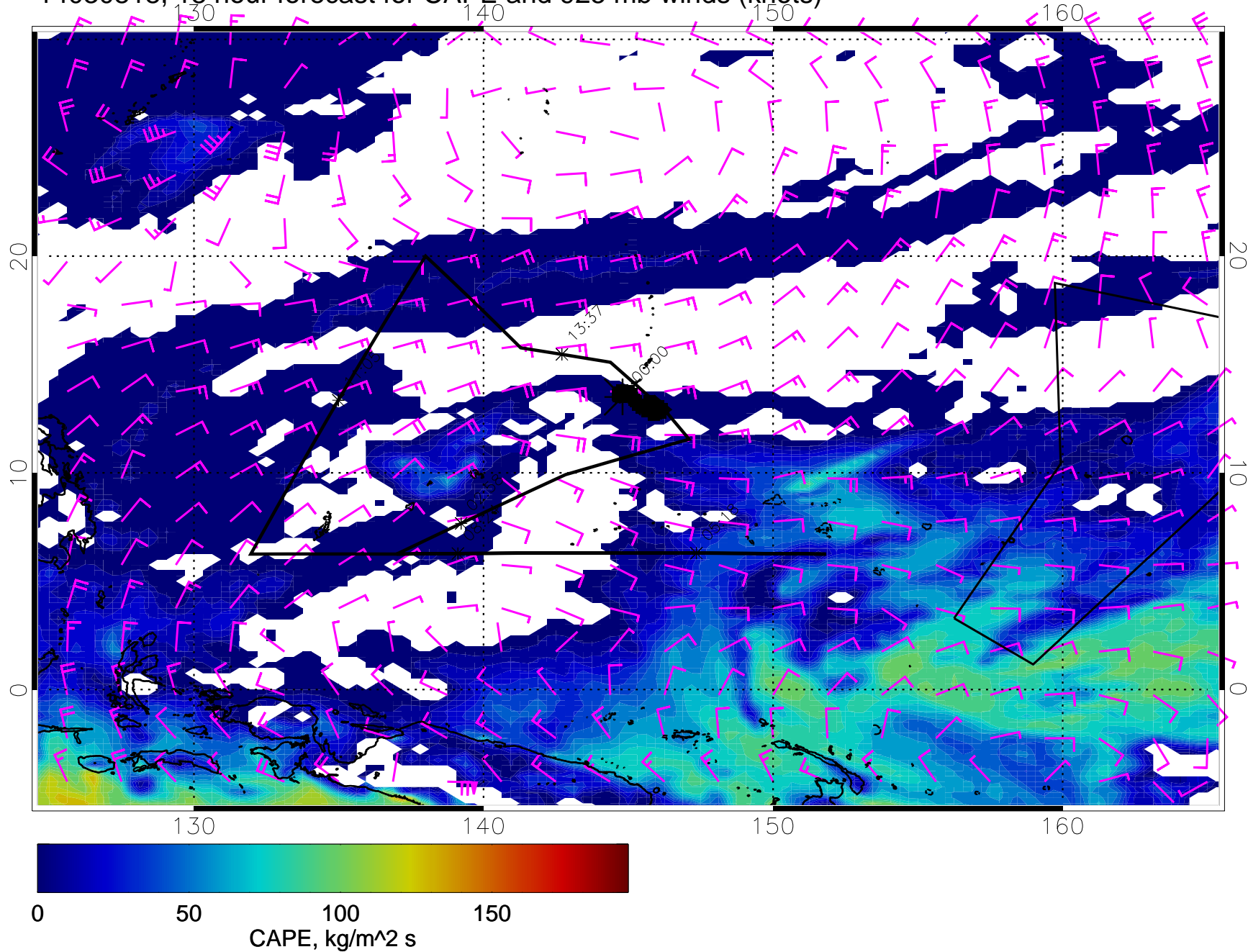
14030818, 18 hour forecast for CAPE and 925 mb winds (knots)
