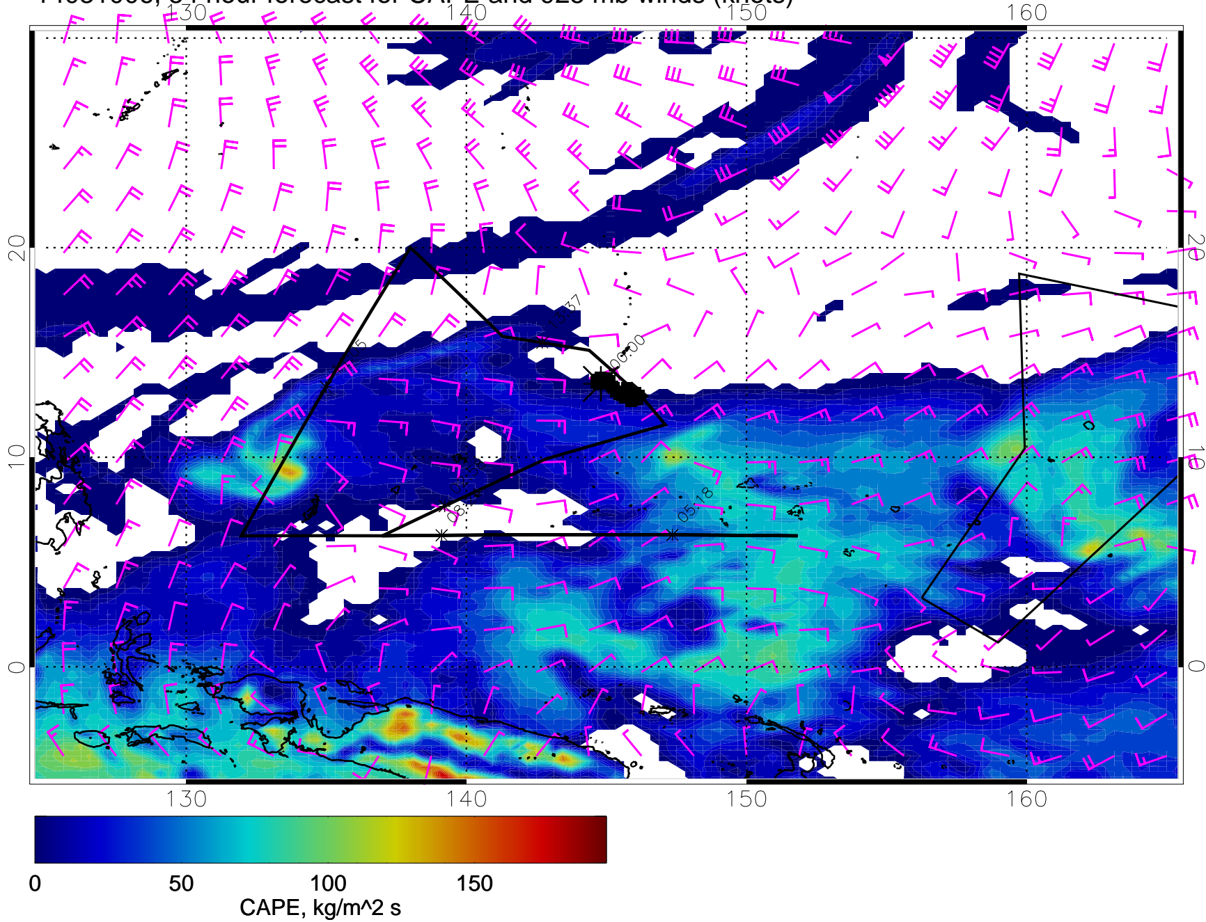
14031006, 54 hour forecast for CAPE and 925 mb winds (knots)
