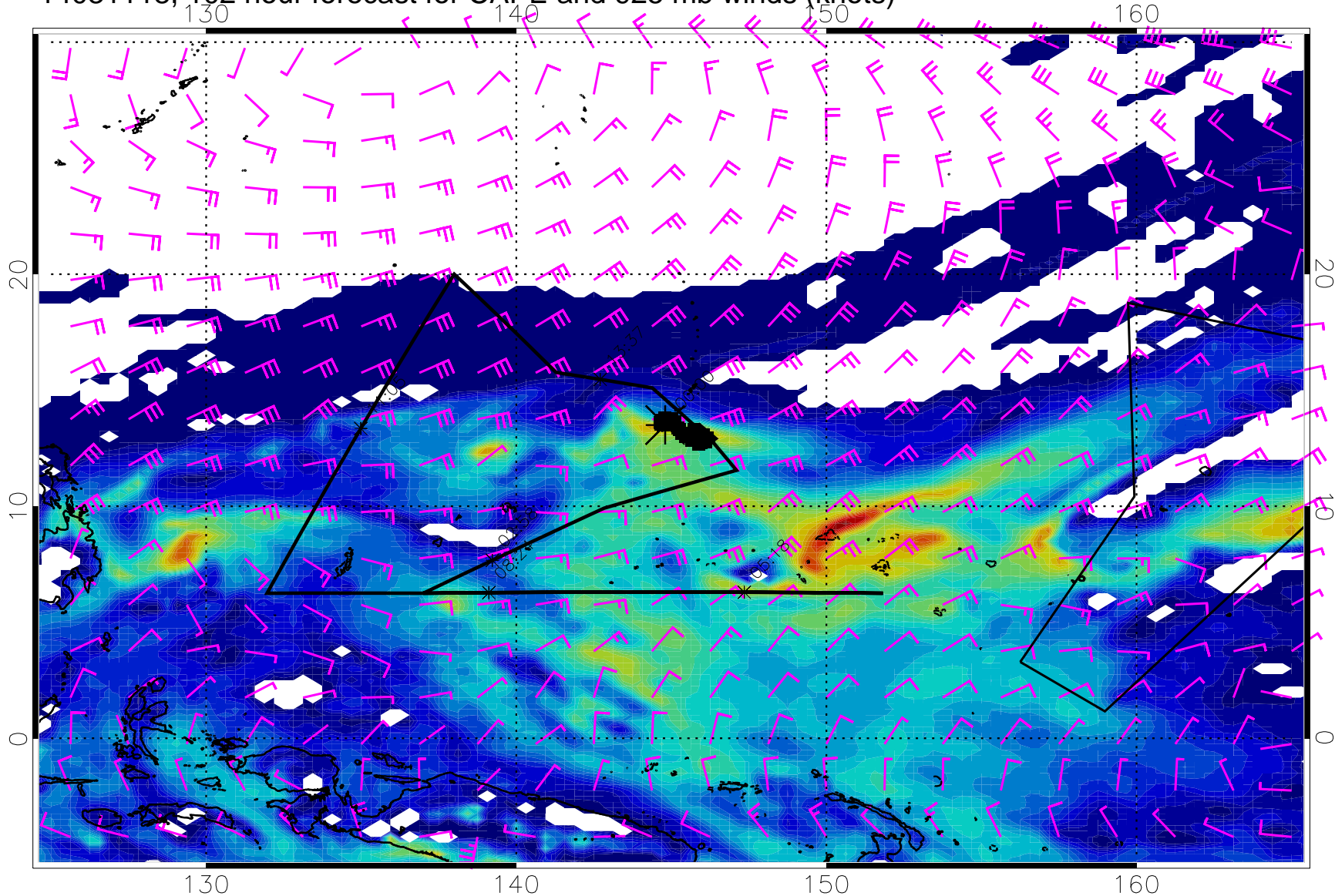
14031118, 102 hour forecast for CAPE and 925 mb winds (knots)
