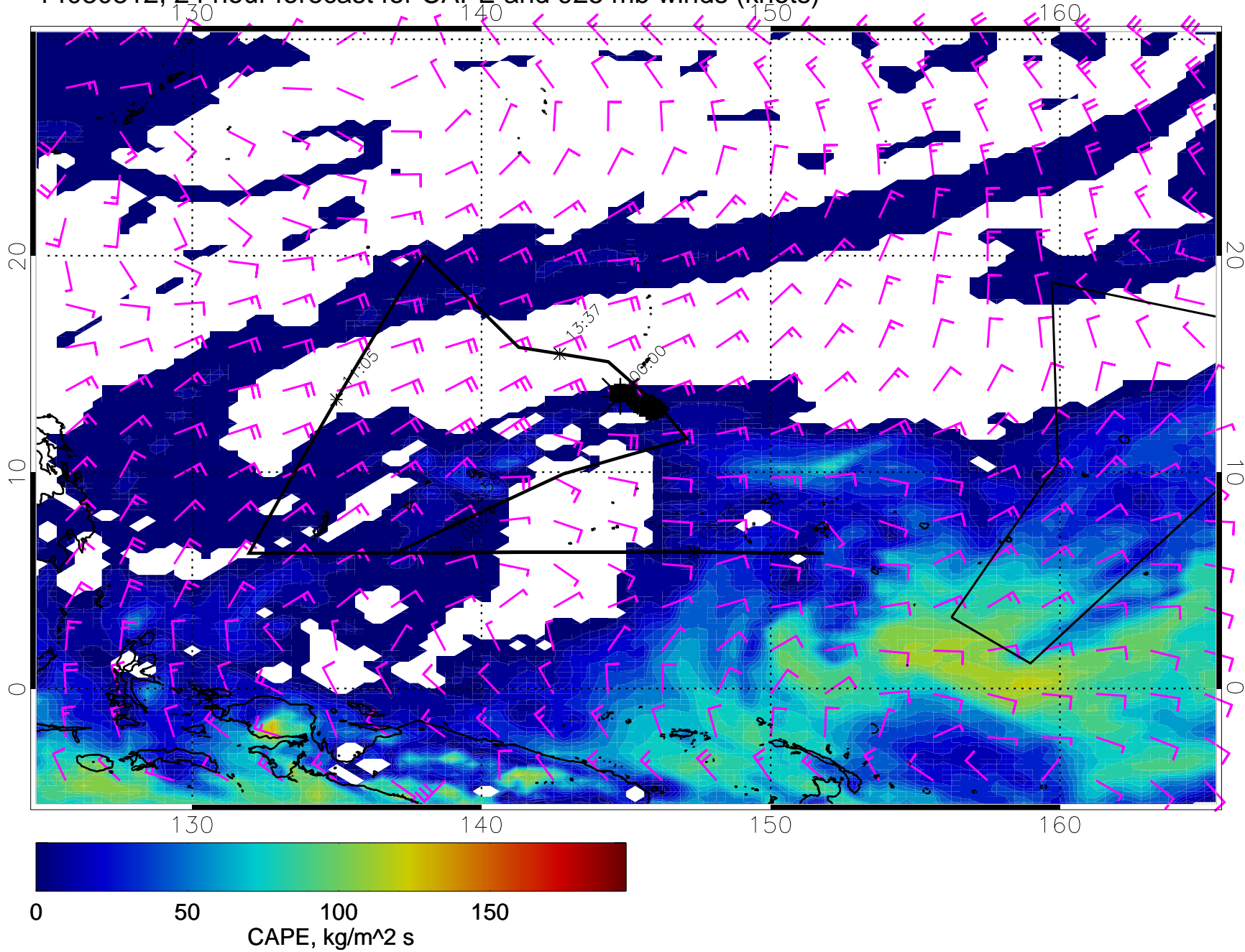
14030812, 24 hour forecast for CAPE and 925 mb winds (knots)
