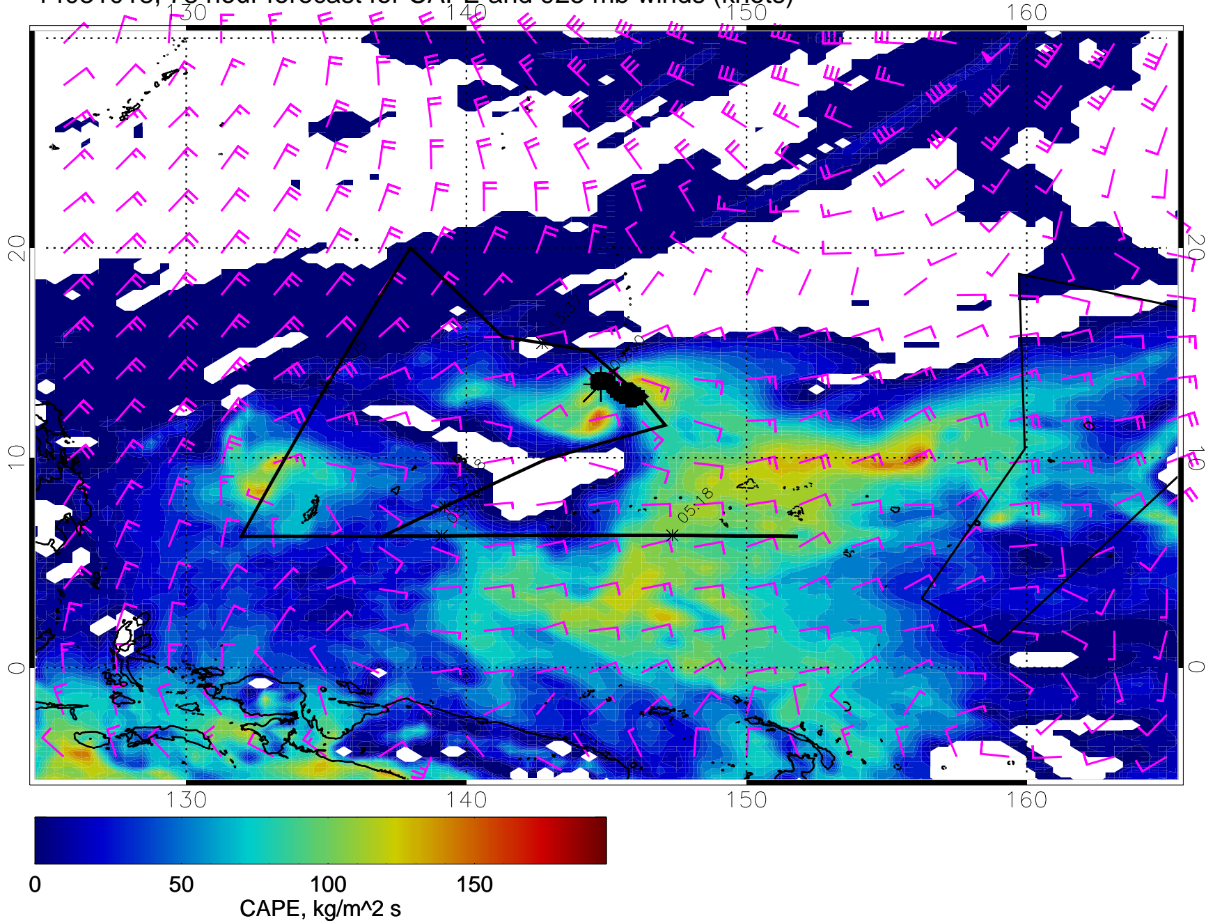
14031018, 78 hour forecast for CAPE and 925 mb winds (knots)
