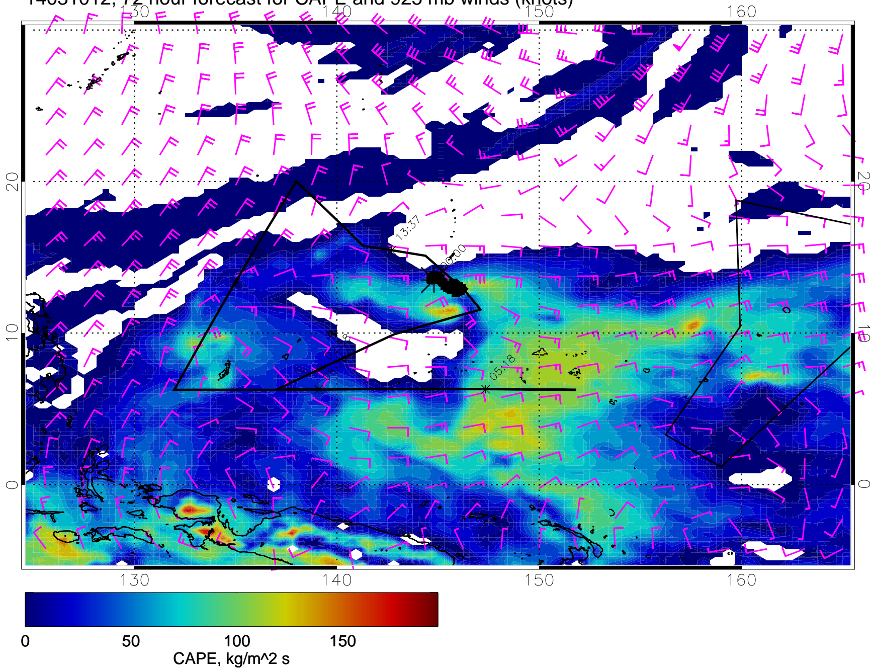
14031012, 72 hour forecast for CAPE and 925 mb winds (knots)
