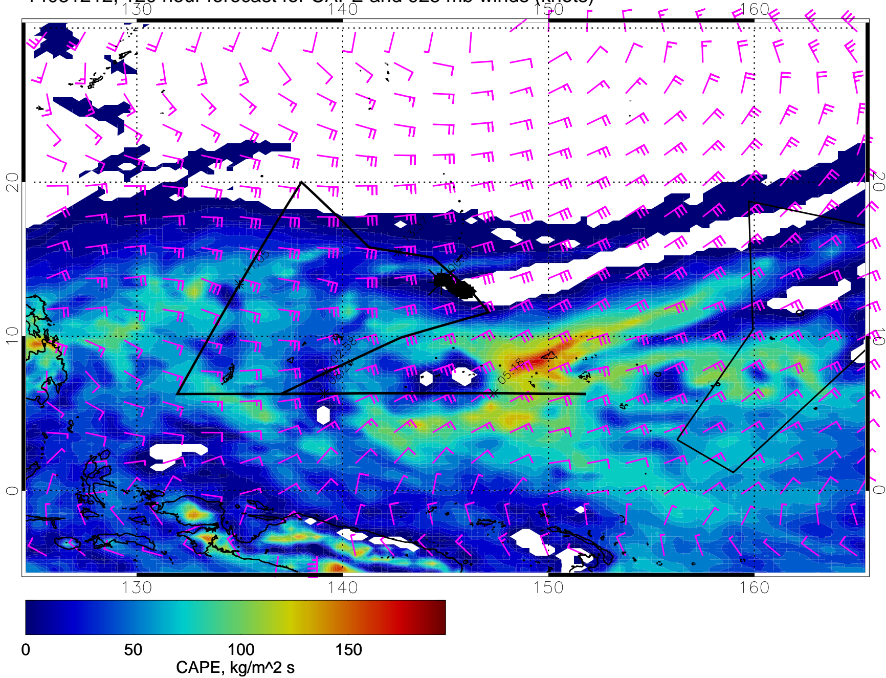
14031212, 120 hour forecast for CAPE and 925 mb winds (knots)
