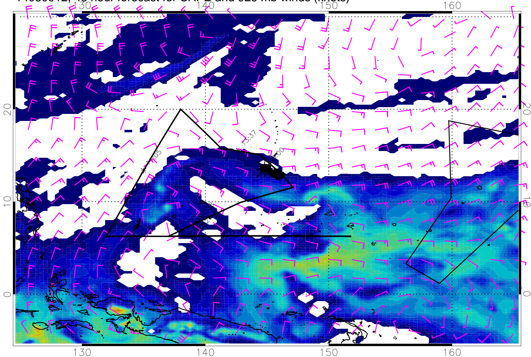
14030912, 48 hour forecast for CAPE and 925 mb winds (knots)
