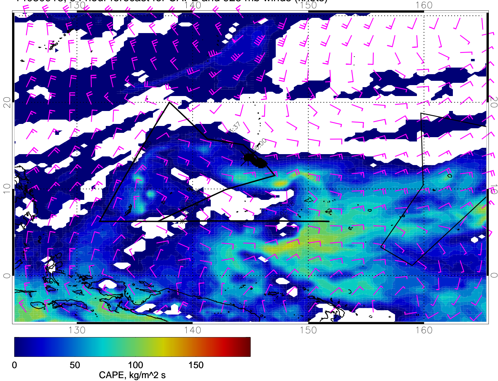
14030918, 54 hour forecast for CAPE and 925 mb winds (knots)
