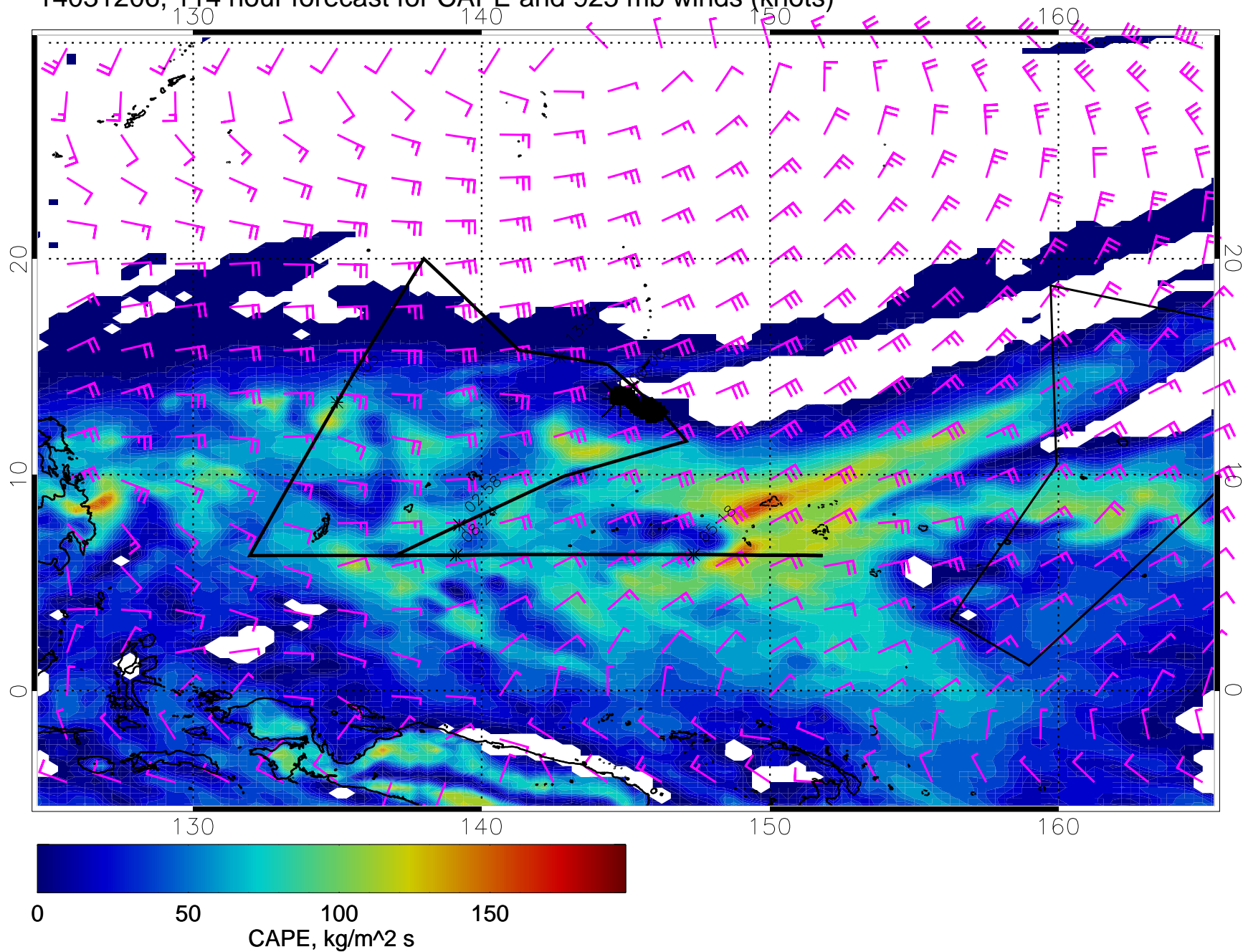
14031206, 114 hour forecast for CAPE and 925 mb winds (knots)
