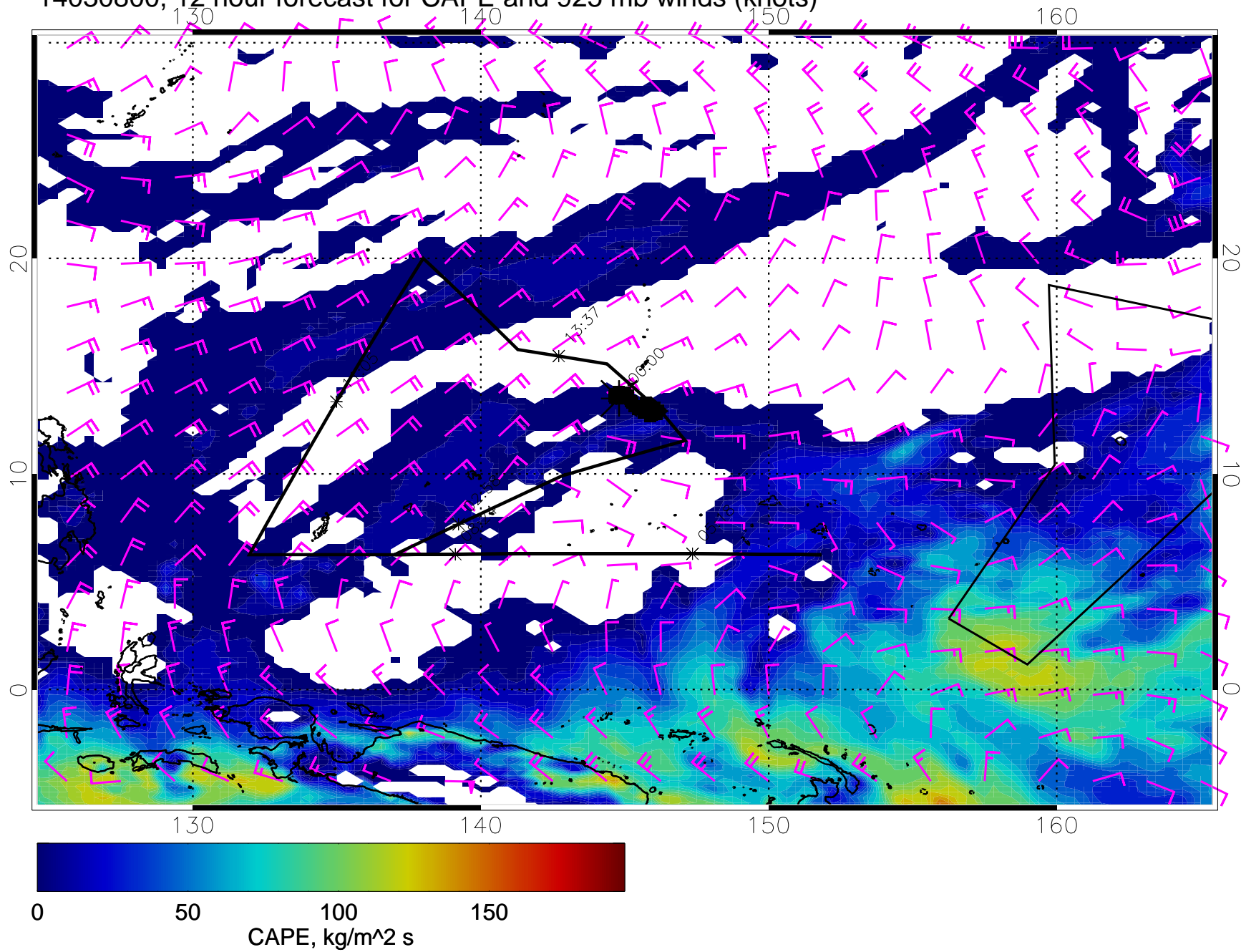
14030800, 12 hour forecast for CAPE and 925 mb winds (knots)
