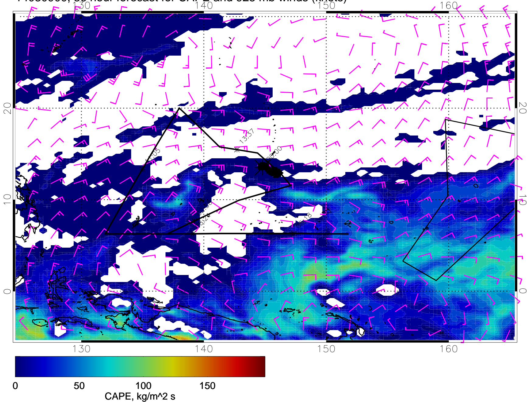
14030900, 36 hour forecast for CAPE and 925 mb winds (knots)
