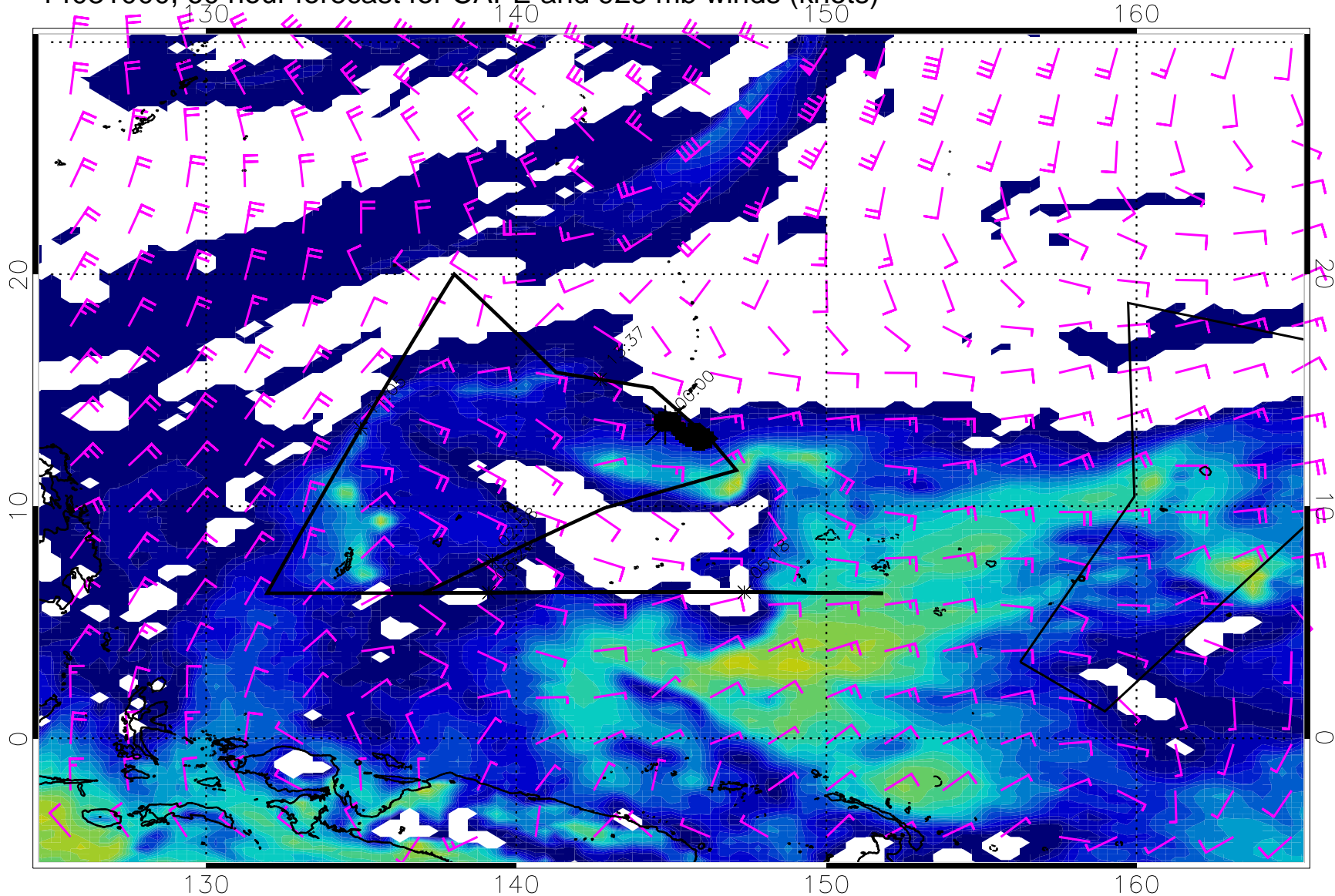
14031000, 60 hour forecast for CAPE and 925 mb winds (knots)
