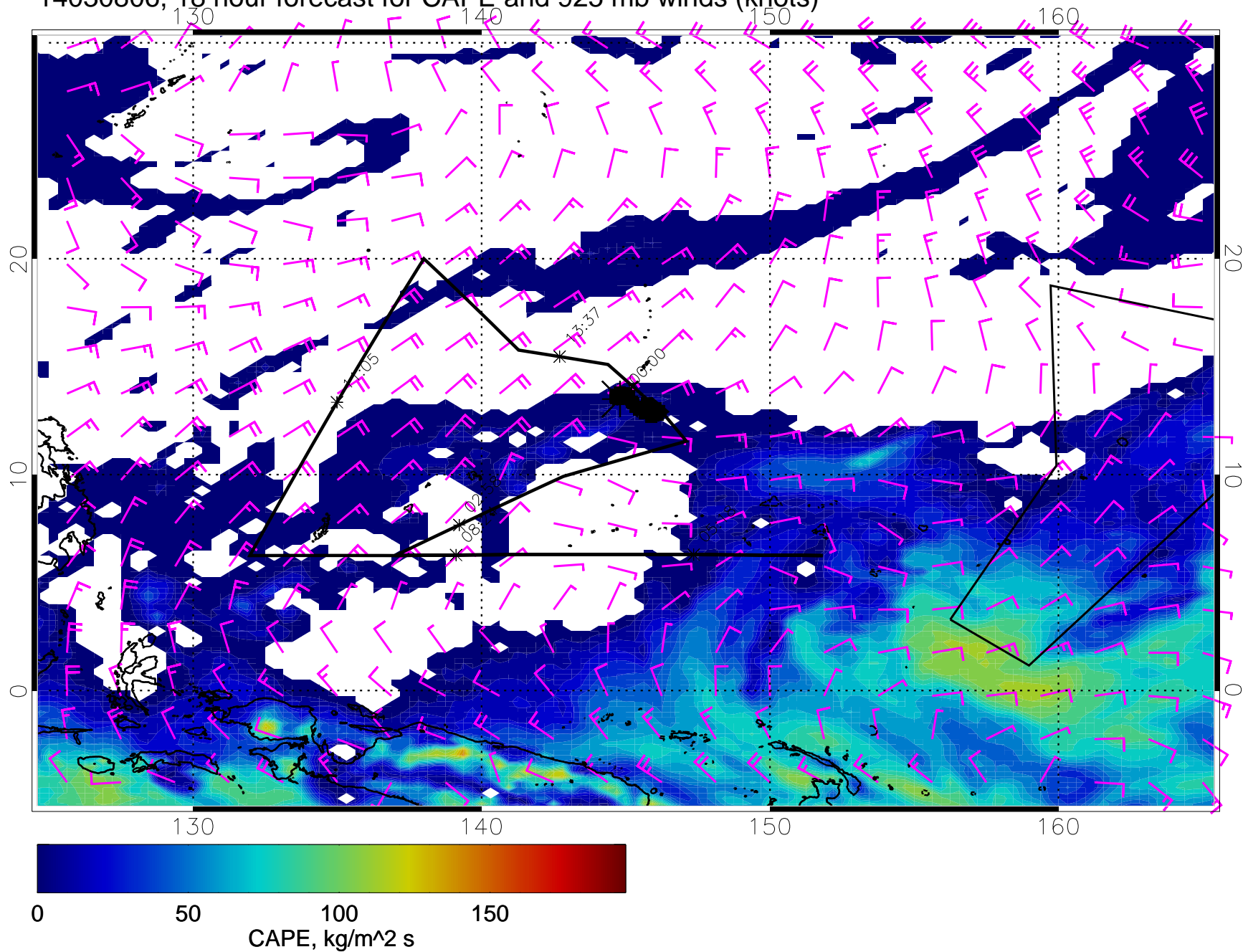
14030806, 18 hour forecast for CAPE and 925 mb winds (knots)
