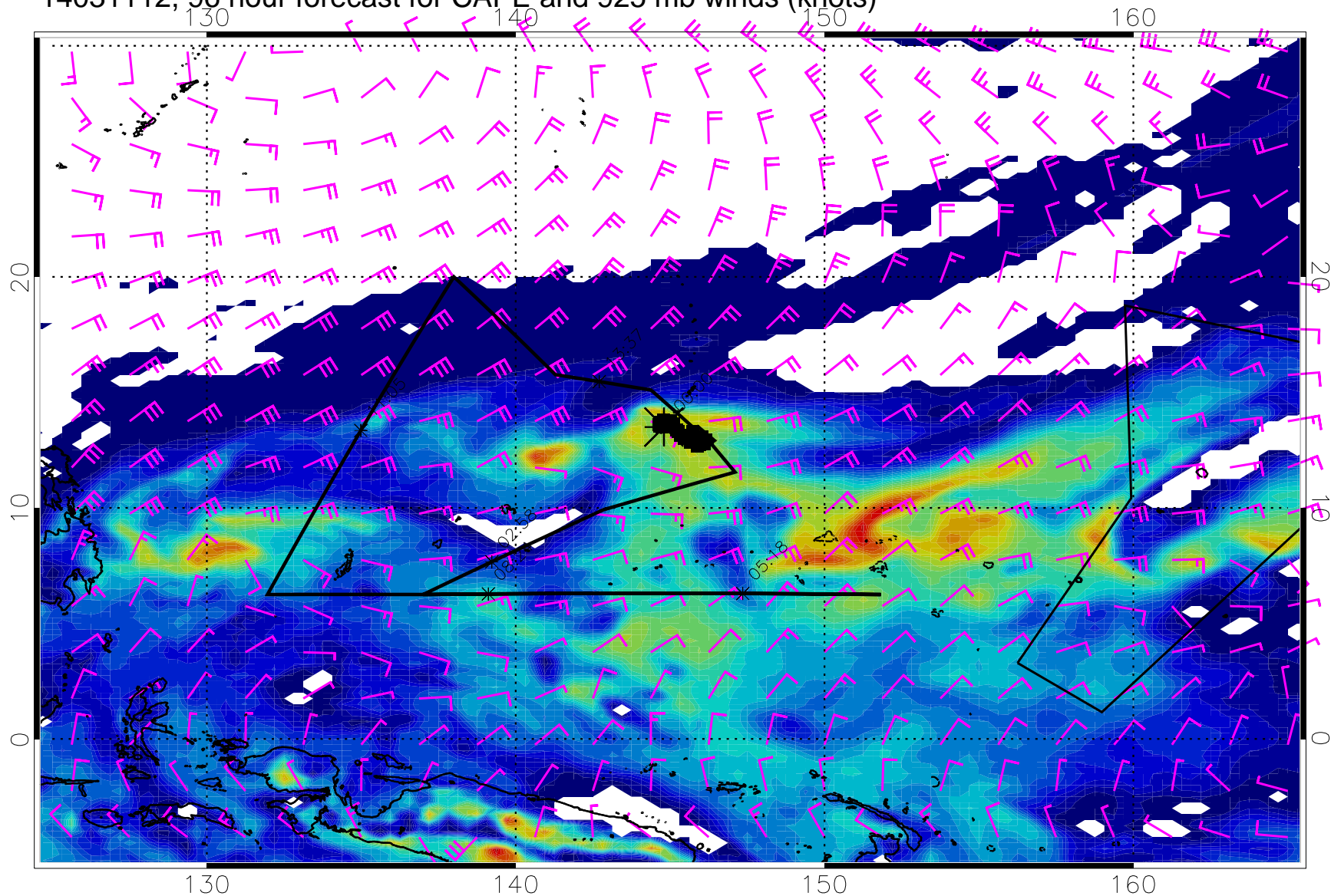
14031112, 96 hour forecast for CAPE and 925 mb winds (knots)
