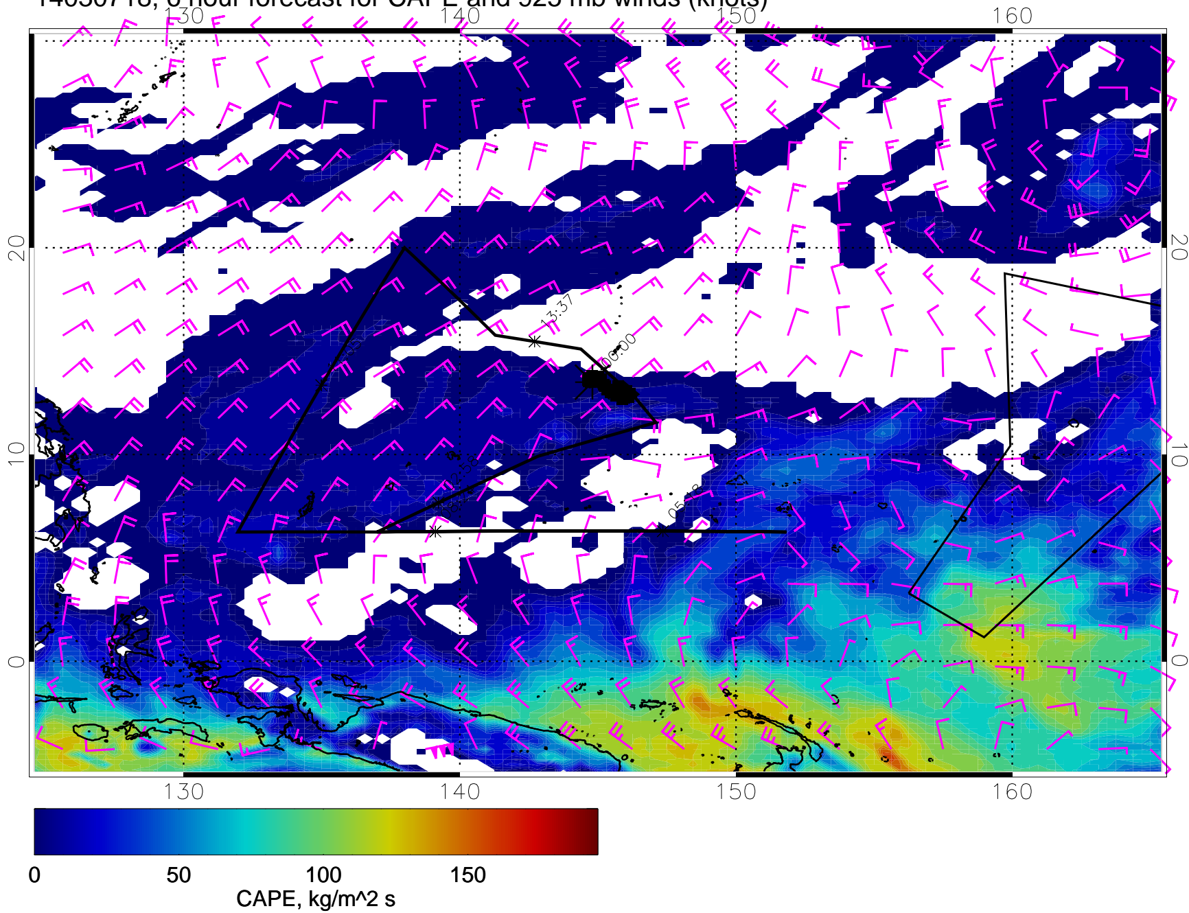
14030718, 6 hour forecast for CAPE and 925 mb winds (knots)
