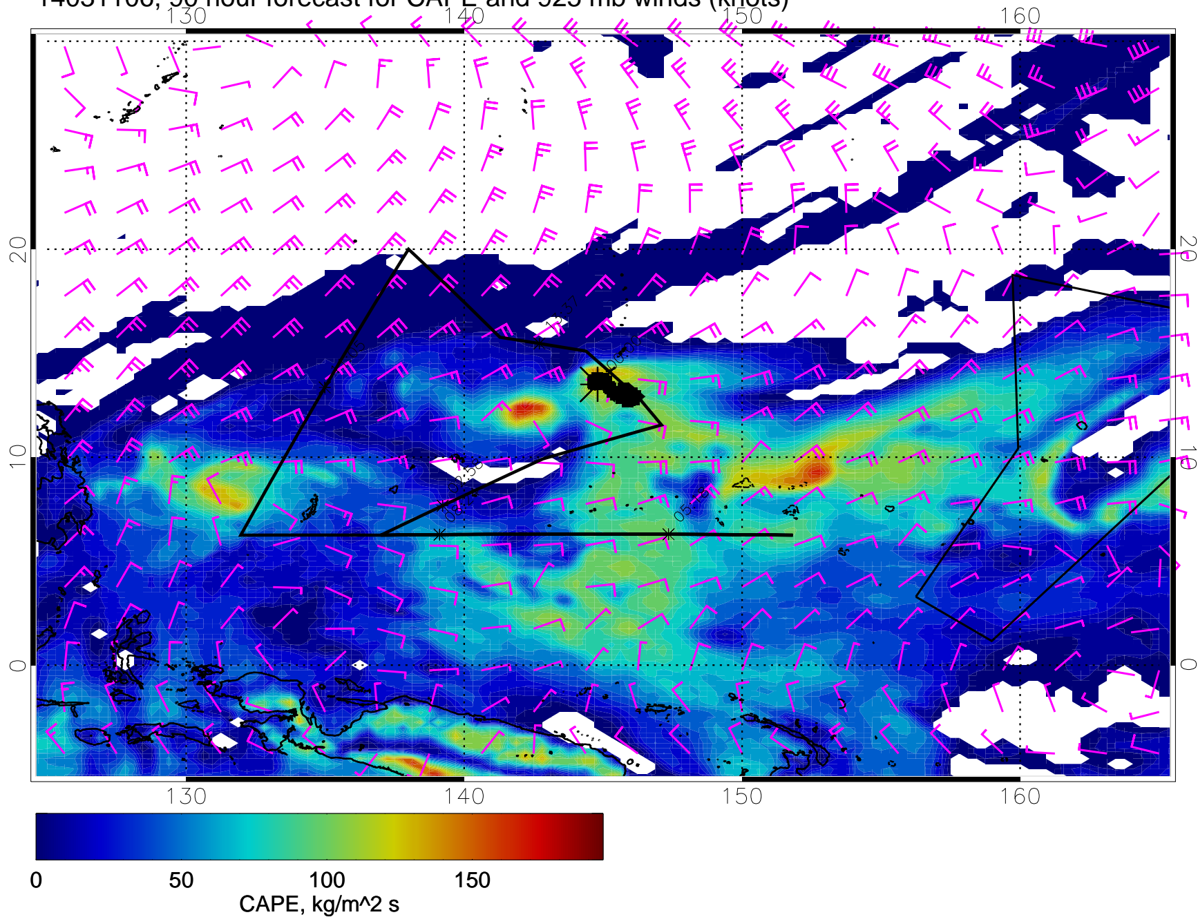
14031106, 90 hour forecast for CAPE and 925 mb winds (knots)
