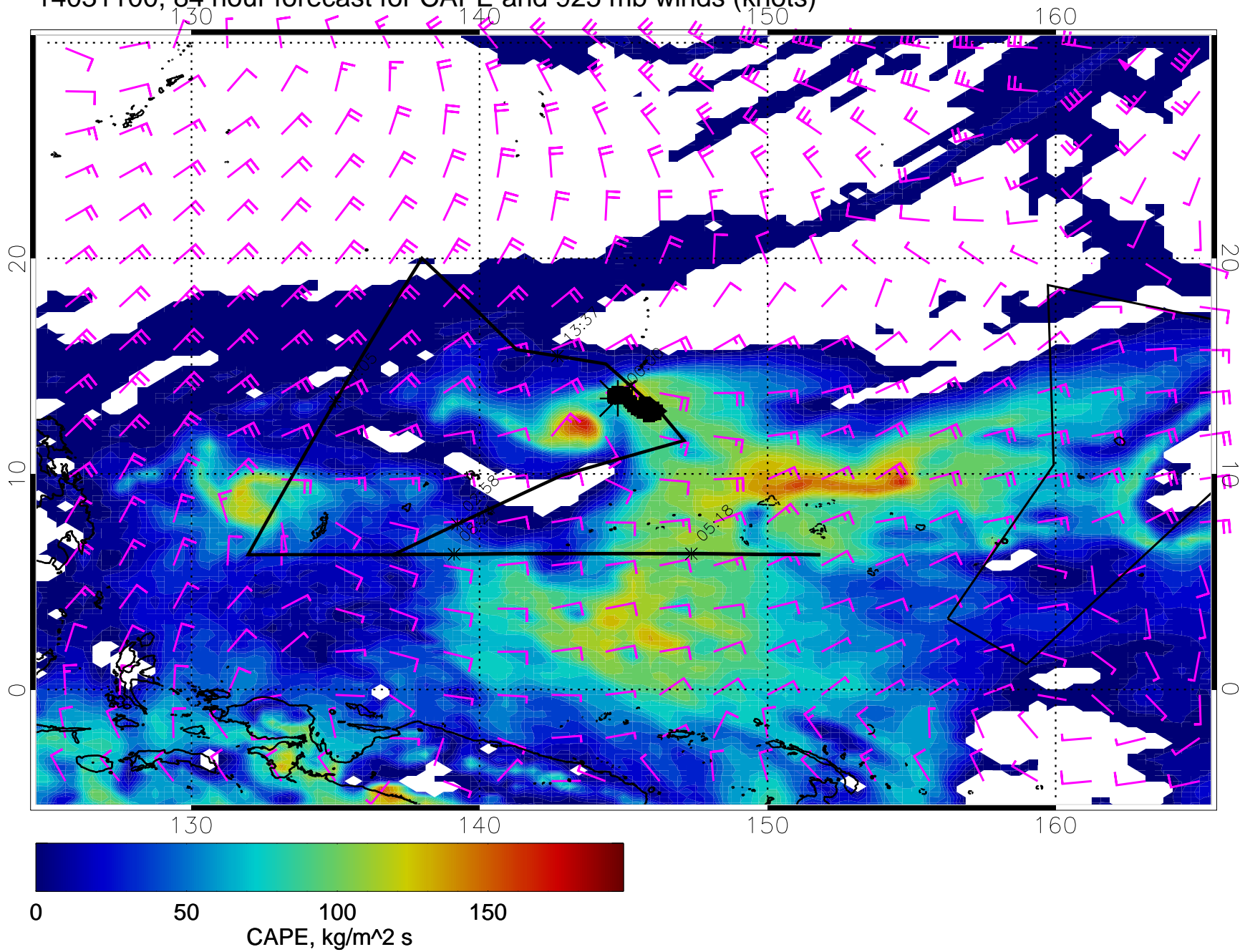
14031100, 84 hour forecast for CAPE and 925 mb winds (knots)
