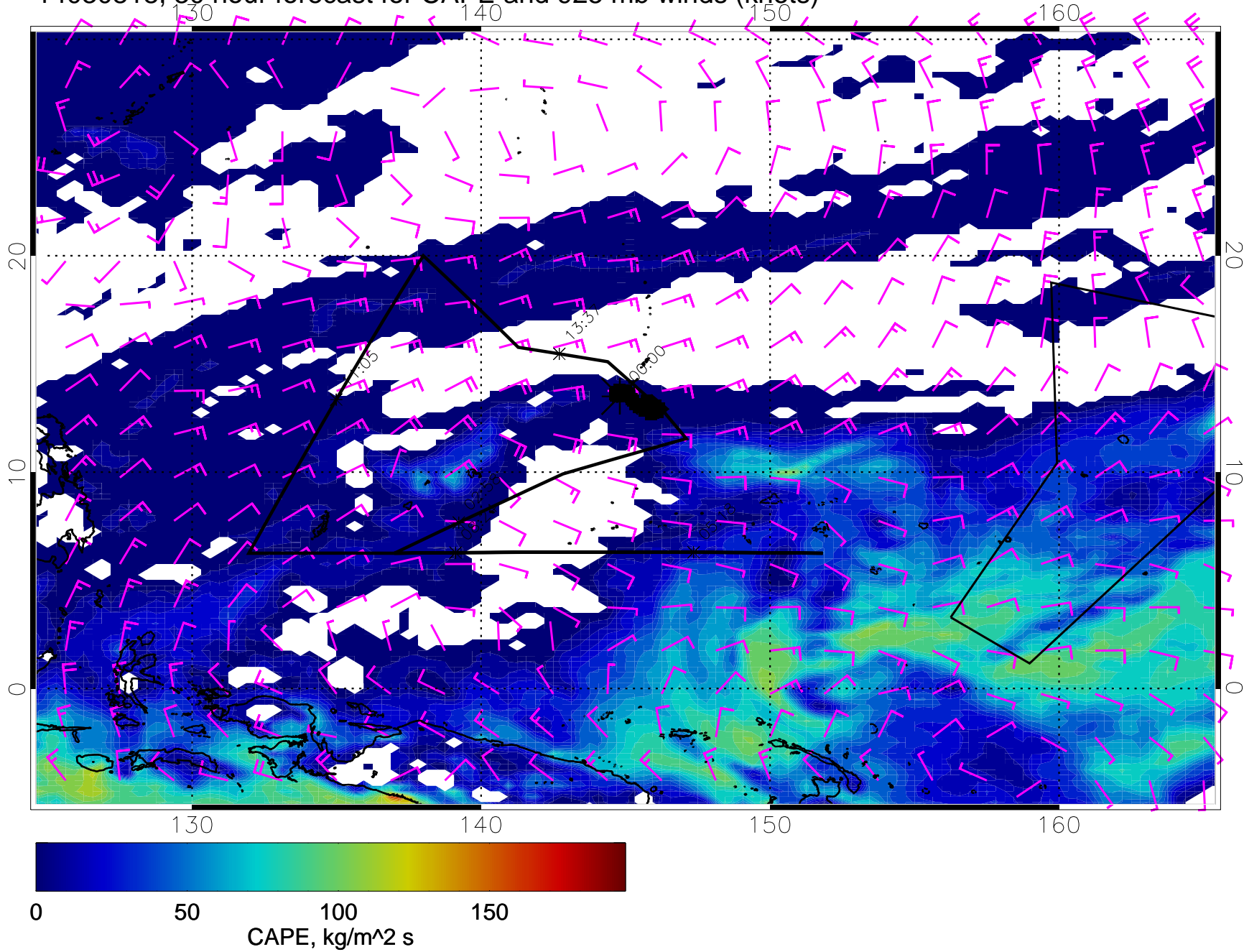
14030818, 30 hour forecast for CAPE and 925 mb winds (knots)
