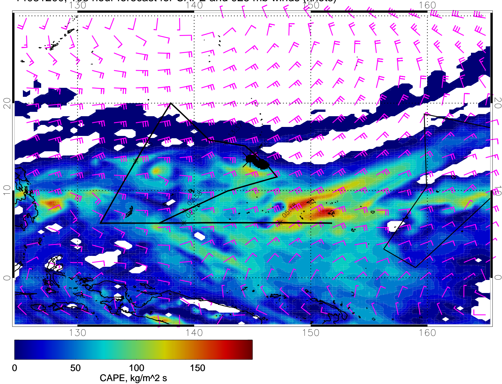
14031200, 108 hour forecast for CAPE and 925 mb winds (knots)
