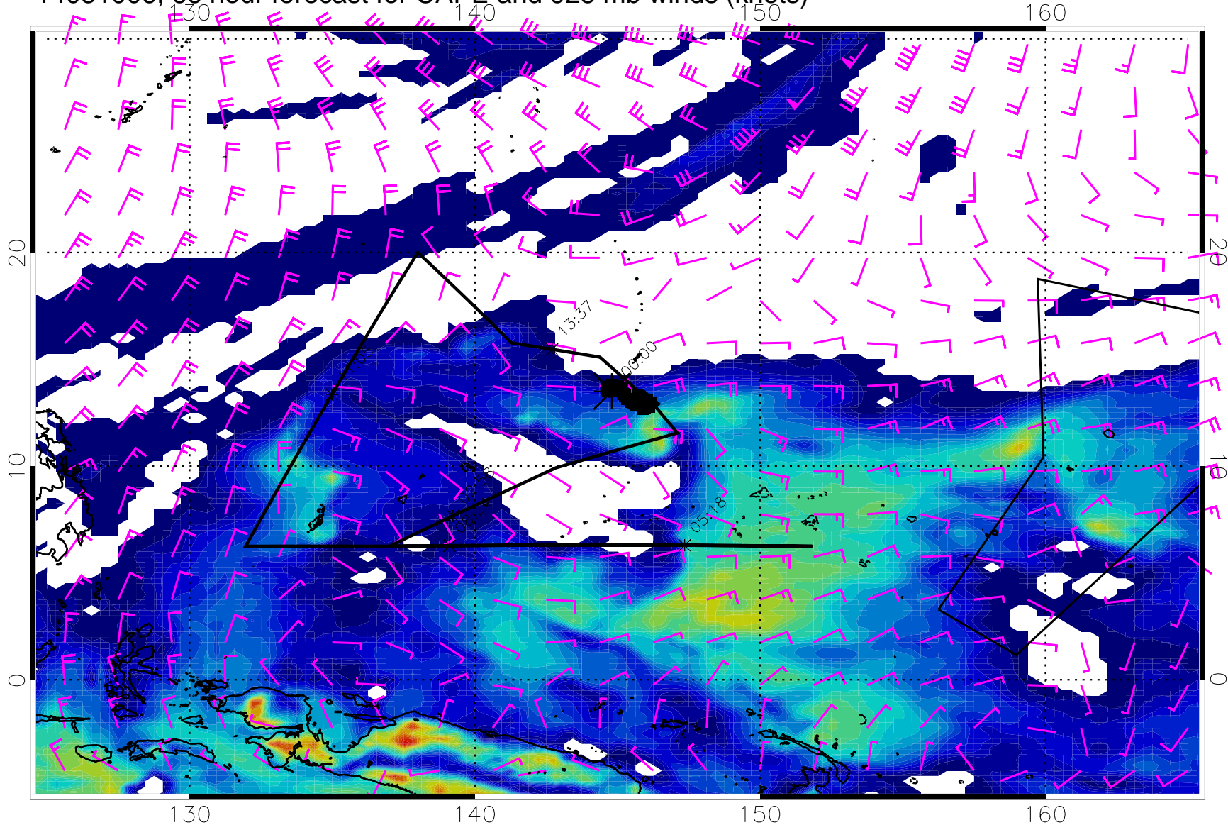
14031006, 66 hour forecast for CAPE and 925 mb winds (knots)
