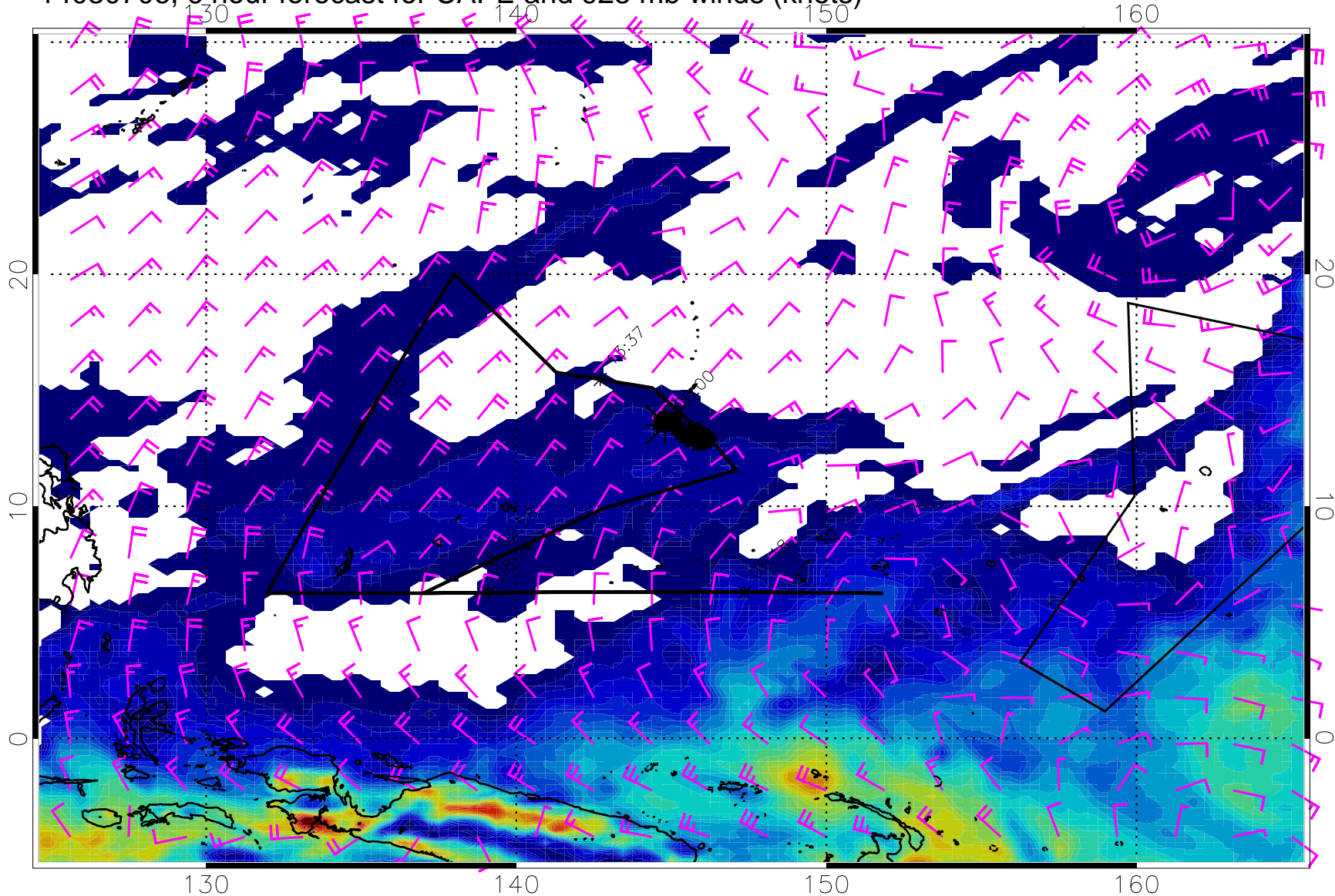
14030706, 6 hour forecast for CAPE and 925 mb winds (knots)
