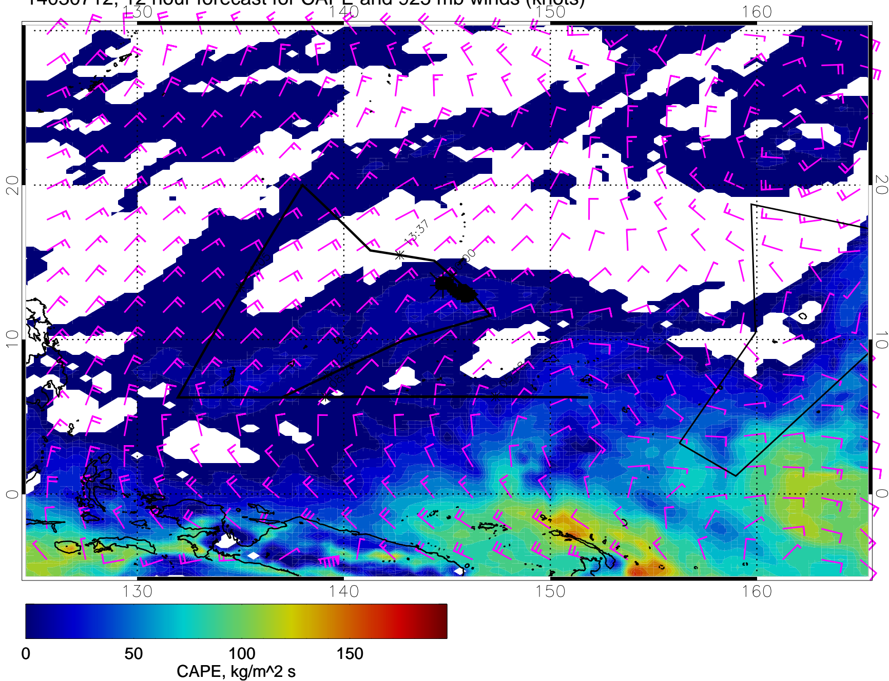
14030712, 12 hour forecast for CAPE and 925 mb winds (knots)
