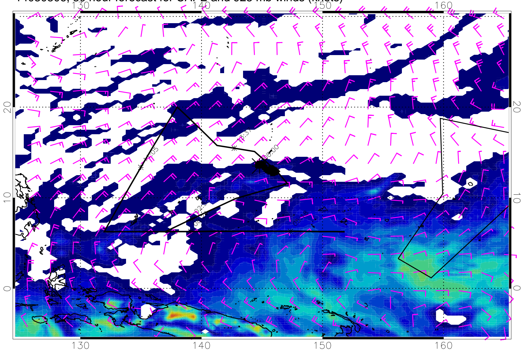
14030806, 30 hour forecast for CAPE and 925 mb winds (knots)
