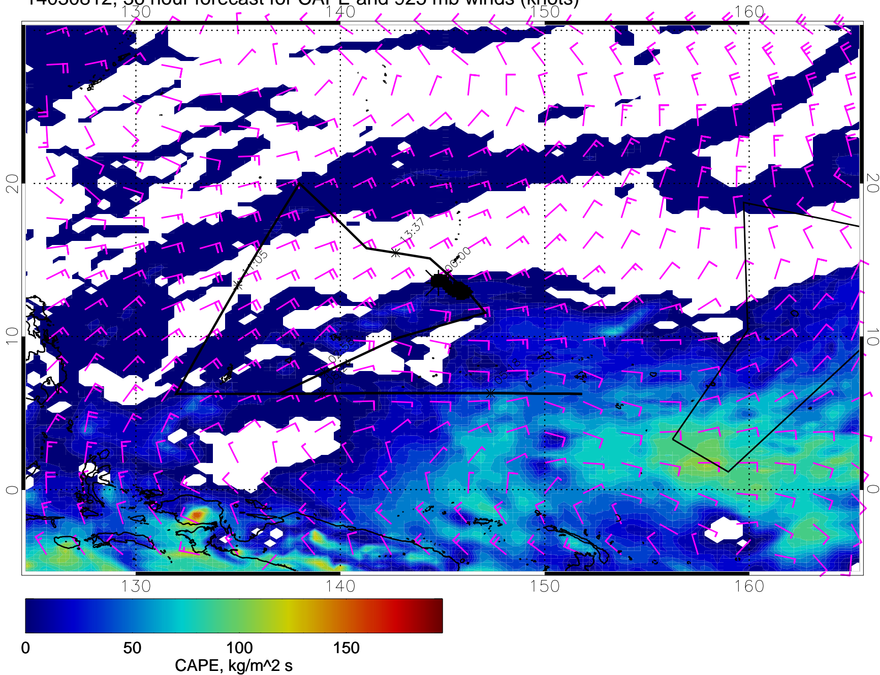
14030812, 36 hour forecast for CAPE and 925 mb winds (knots)
