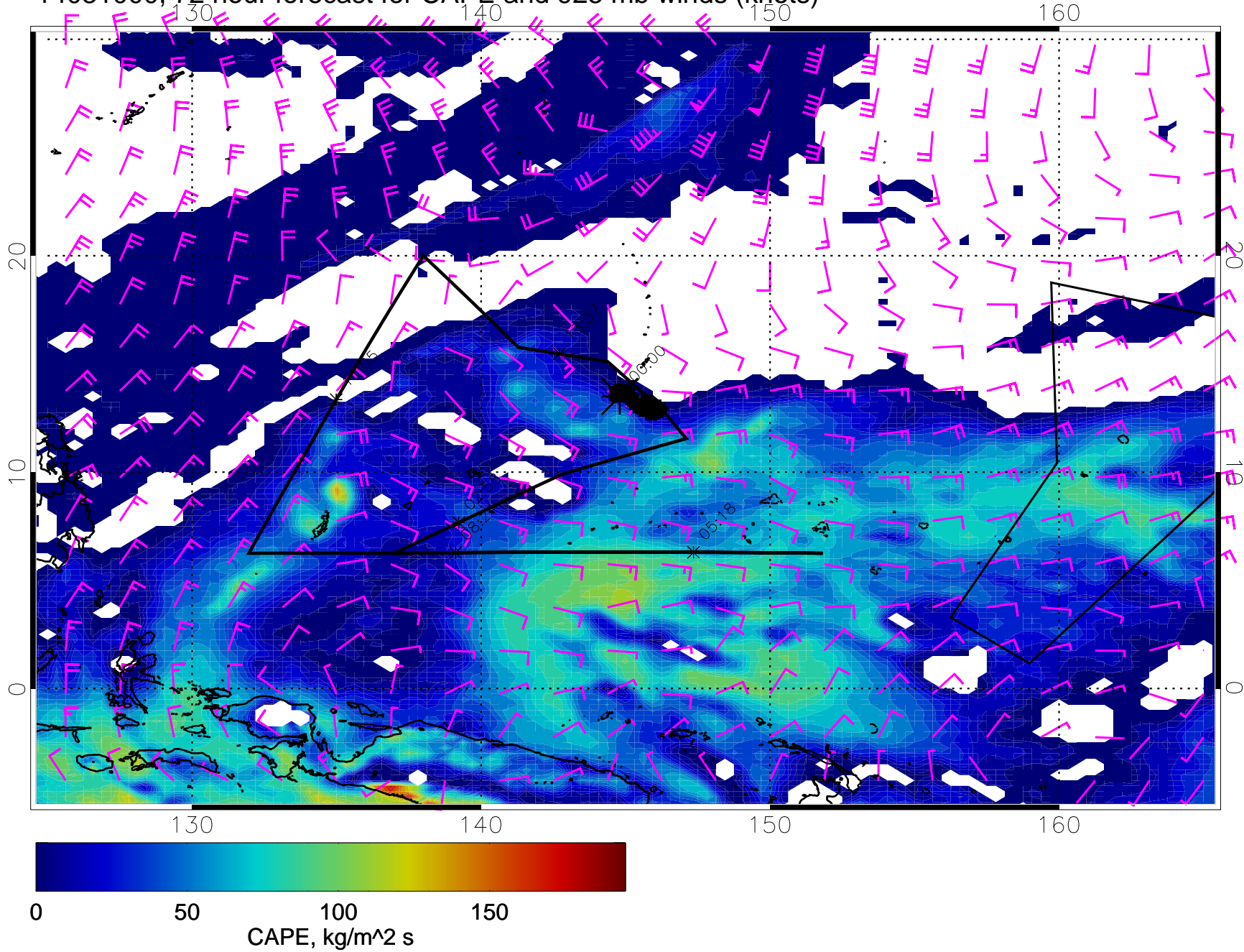
14031000, 72 hour forecast for CAPE and 925 mb winds (knots)
