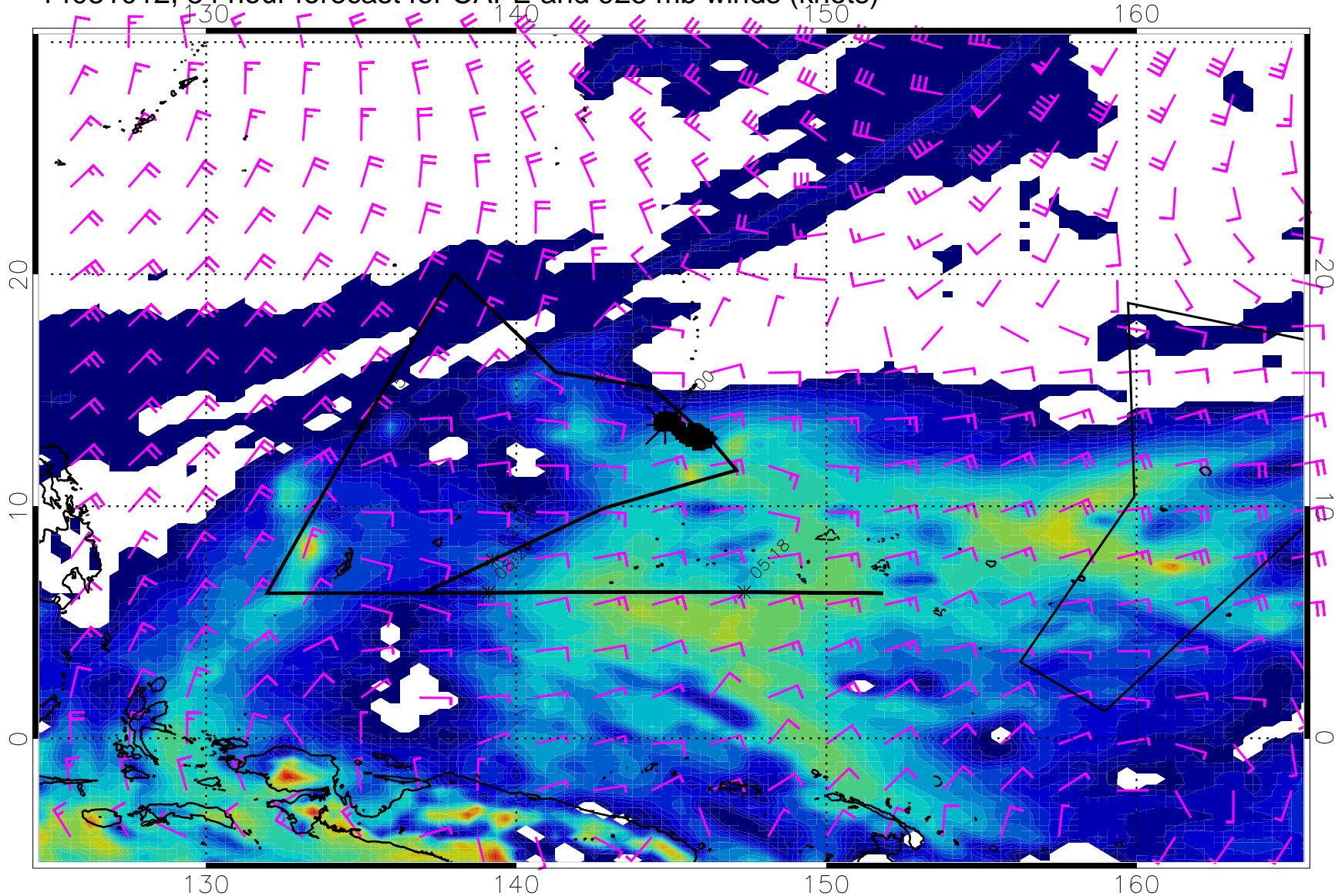
14031012, 84 hour forecast for CAPE and 925 mb winds (knots)
