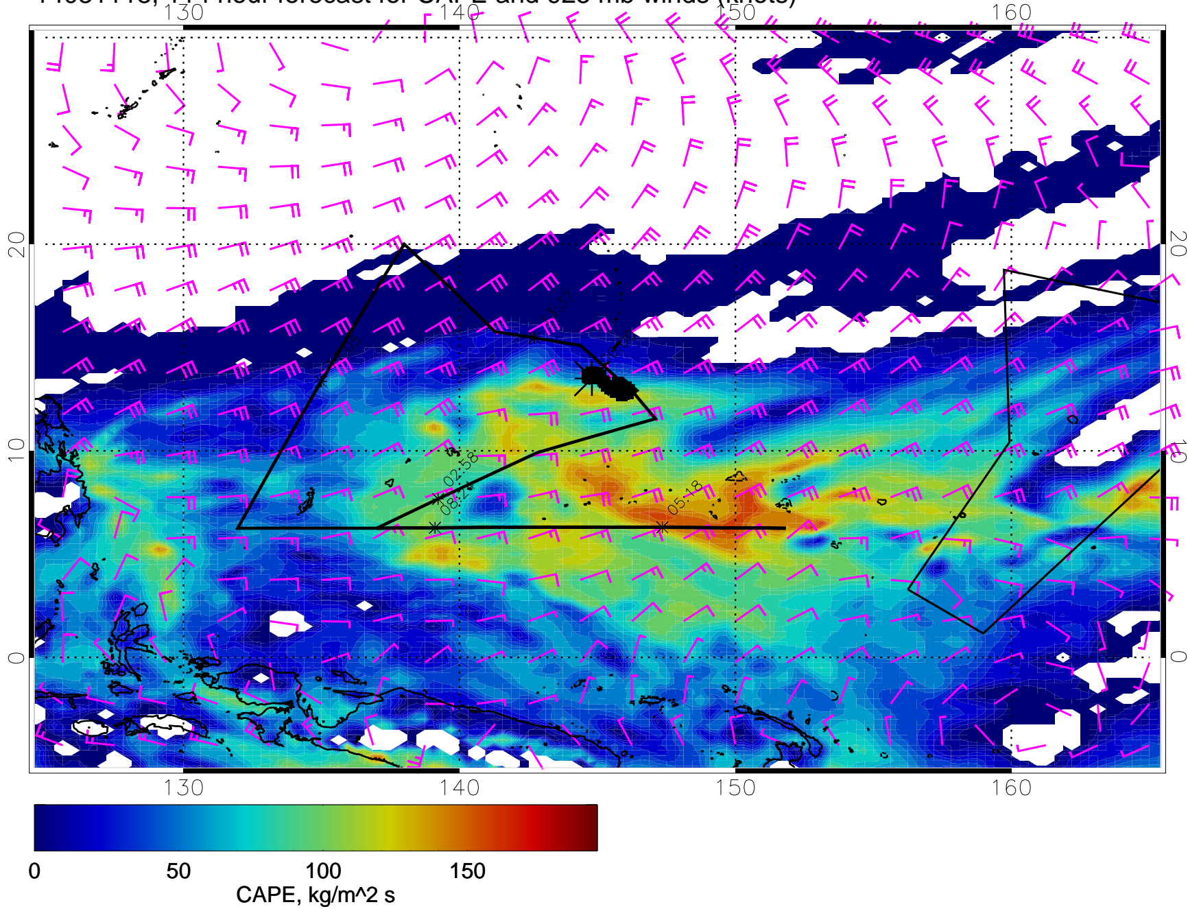
14031118, 114 hour forecast for CAPE and 925 mb winds (knots)
