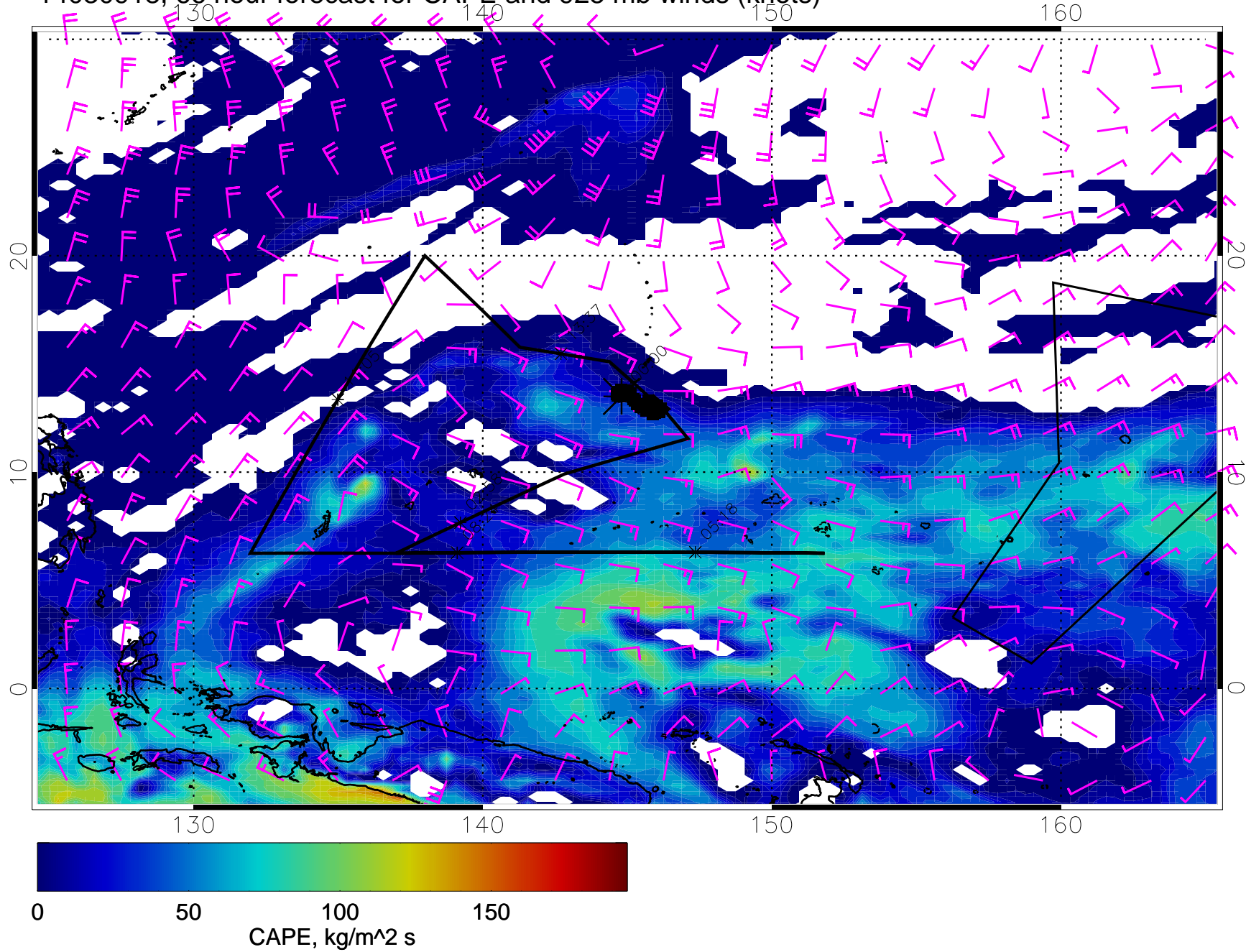
14030918, 66 hour forecast for CAPE and 925 mb winds (knots)
