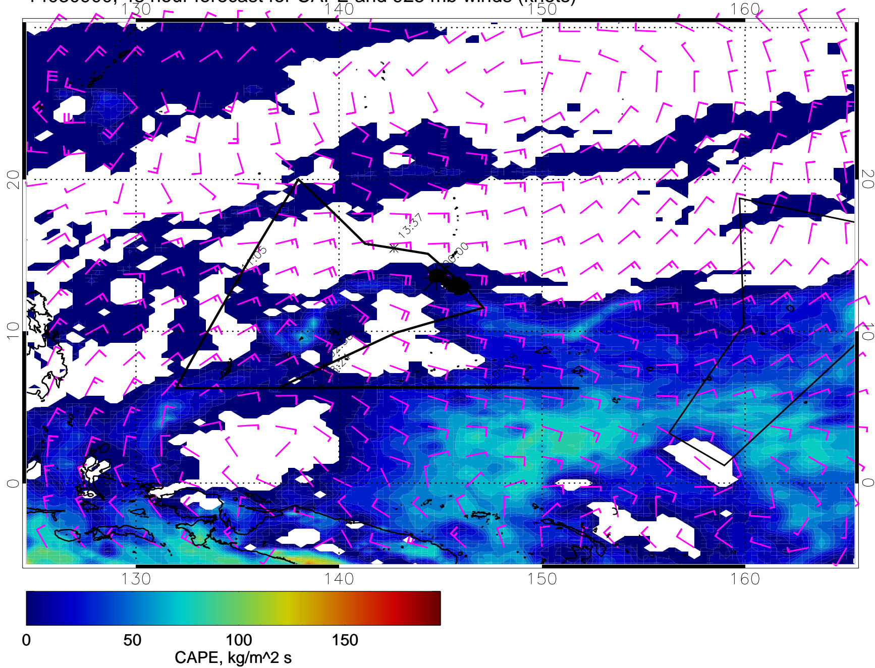
14030900, 48 hour forecast for CAPE and 925 mb winds (knots)
