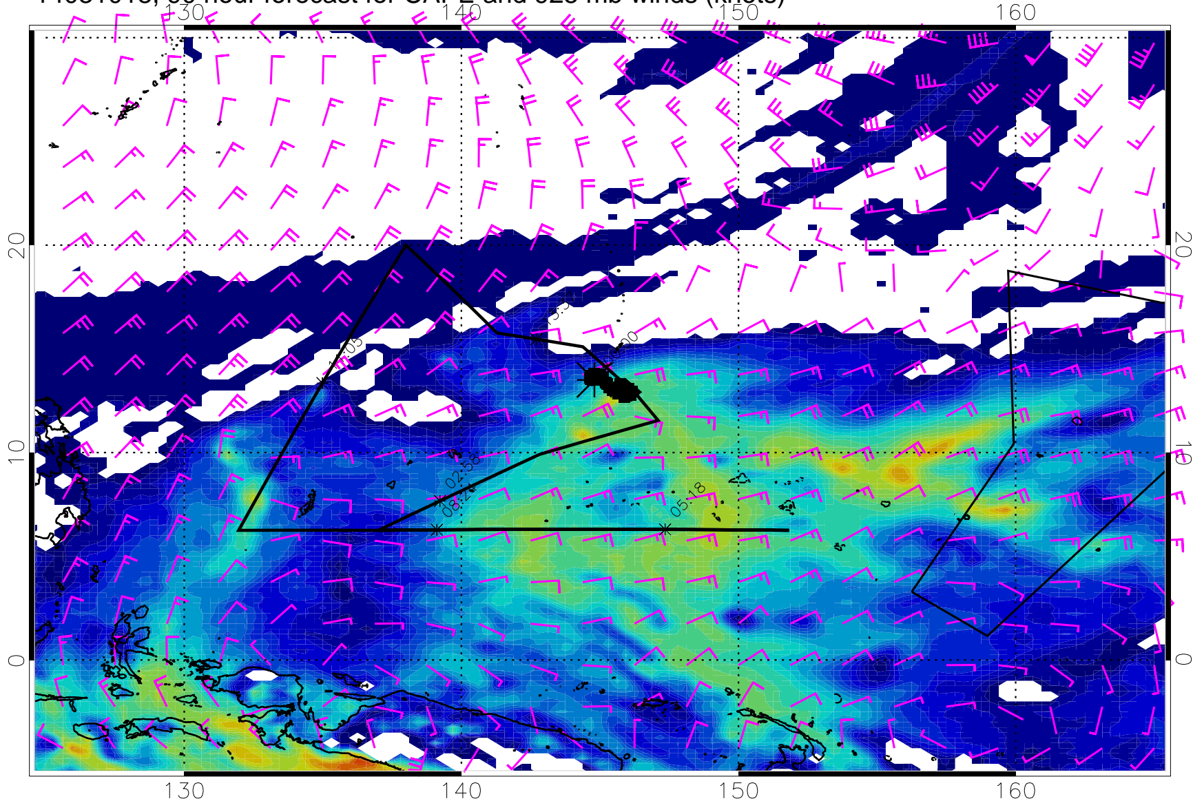
14031018, 90 hour forecast for CAPE and 925 mb winds (knots)
