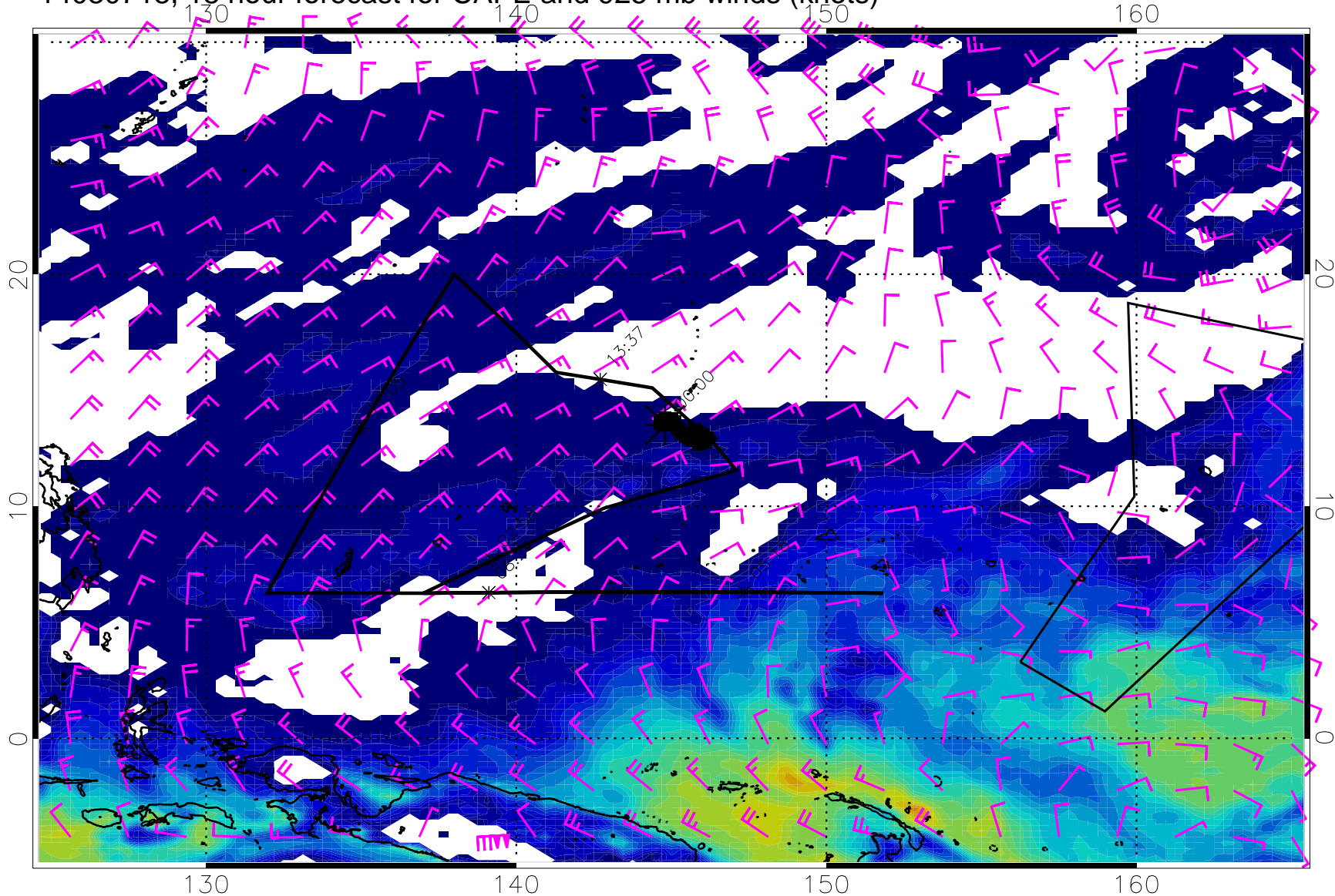
14030718, 18 hour forecast for CAPE and 925 mb winds (knots)
