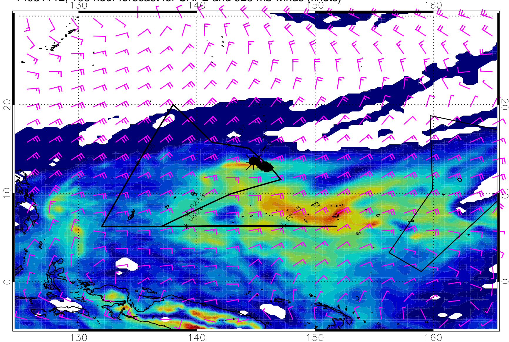
14031112, 108 hour forecast for CAPE and 925 mb winds (knots)
