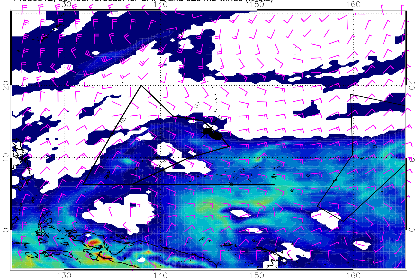
14030912, 60 hour forecast for CAPE and 925 mb winds (knots)
