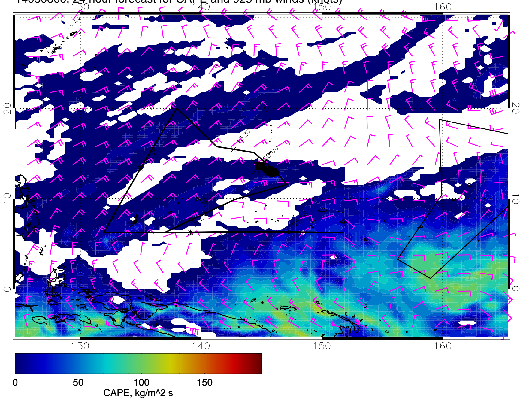
14030800, 24 hour forecast for CAPE and 925 mb winds (knots)
