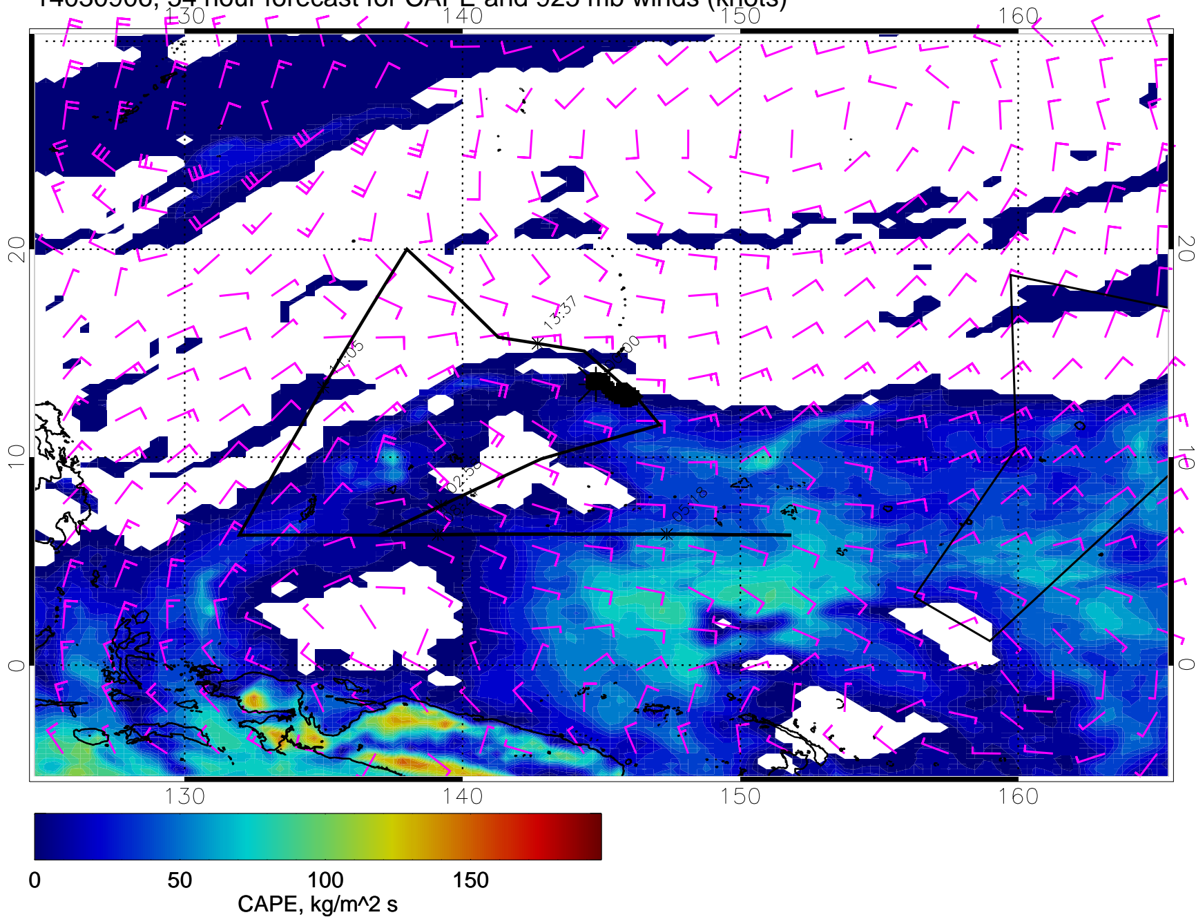
14030906, 54 hour forecast for CAPE and 925 mb winds (knots)
