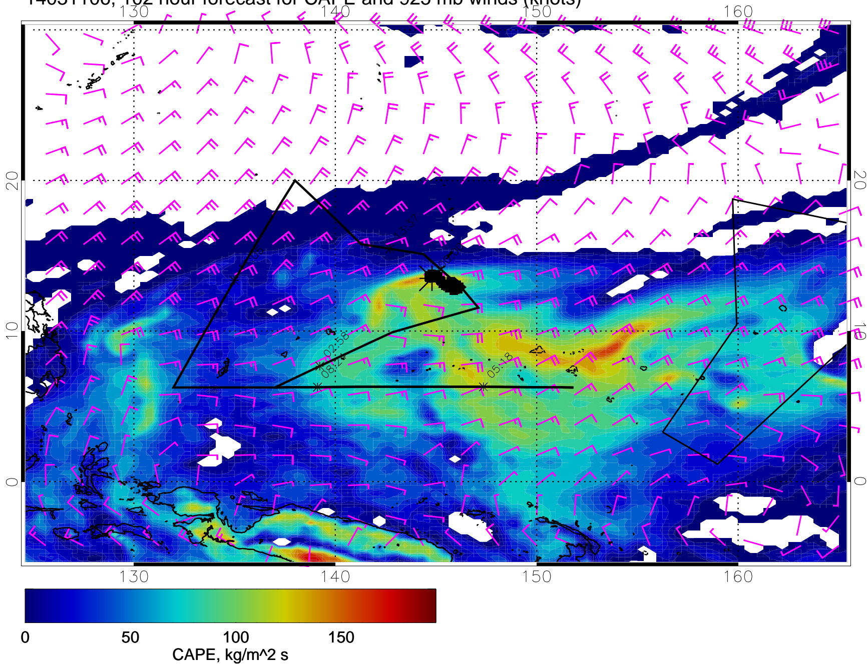
14031106, 102 hour forecast for CAPE and 925 mb winds (knots)
