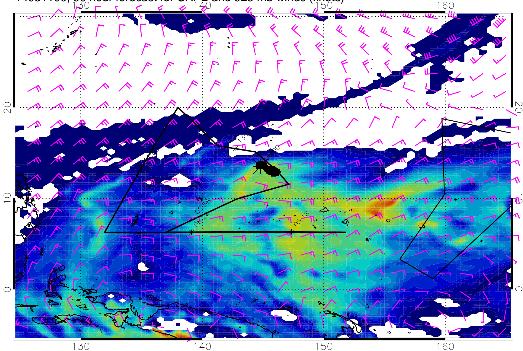
14031100, 96 hour forecast for CAPE and 925 mb winds (knots)
