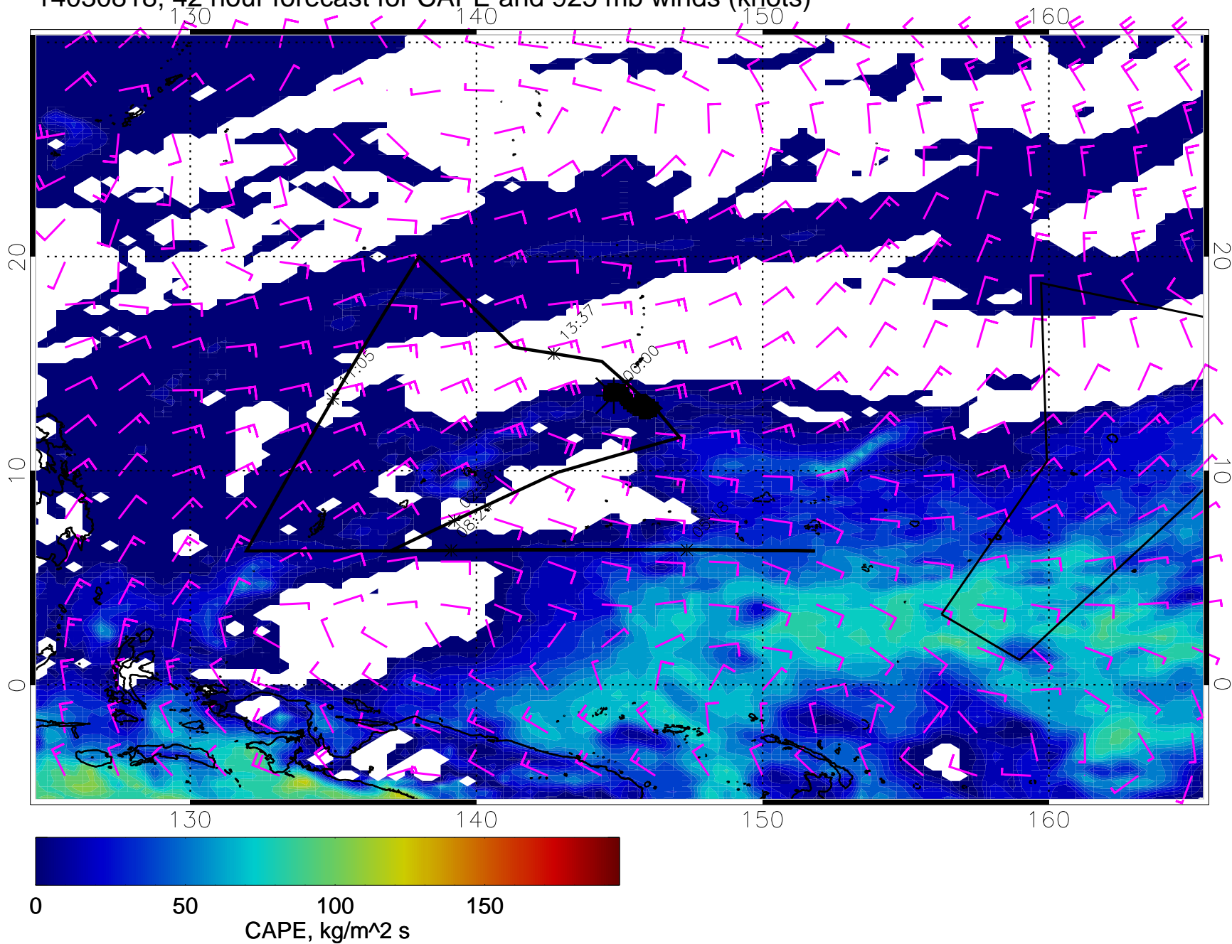
14030818, 42 hour forecast for CAPE and 925 mb winds (knots)
