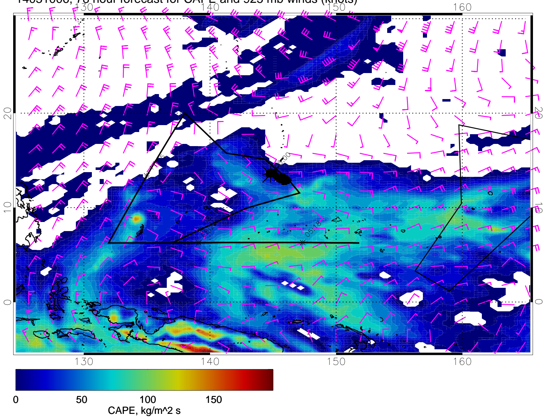
14031006, 78 hour forecast for CAPE and 925 mb winds (knots)
