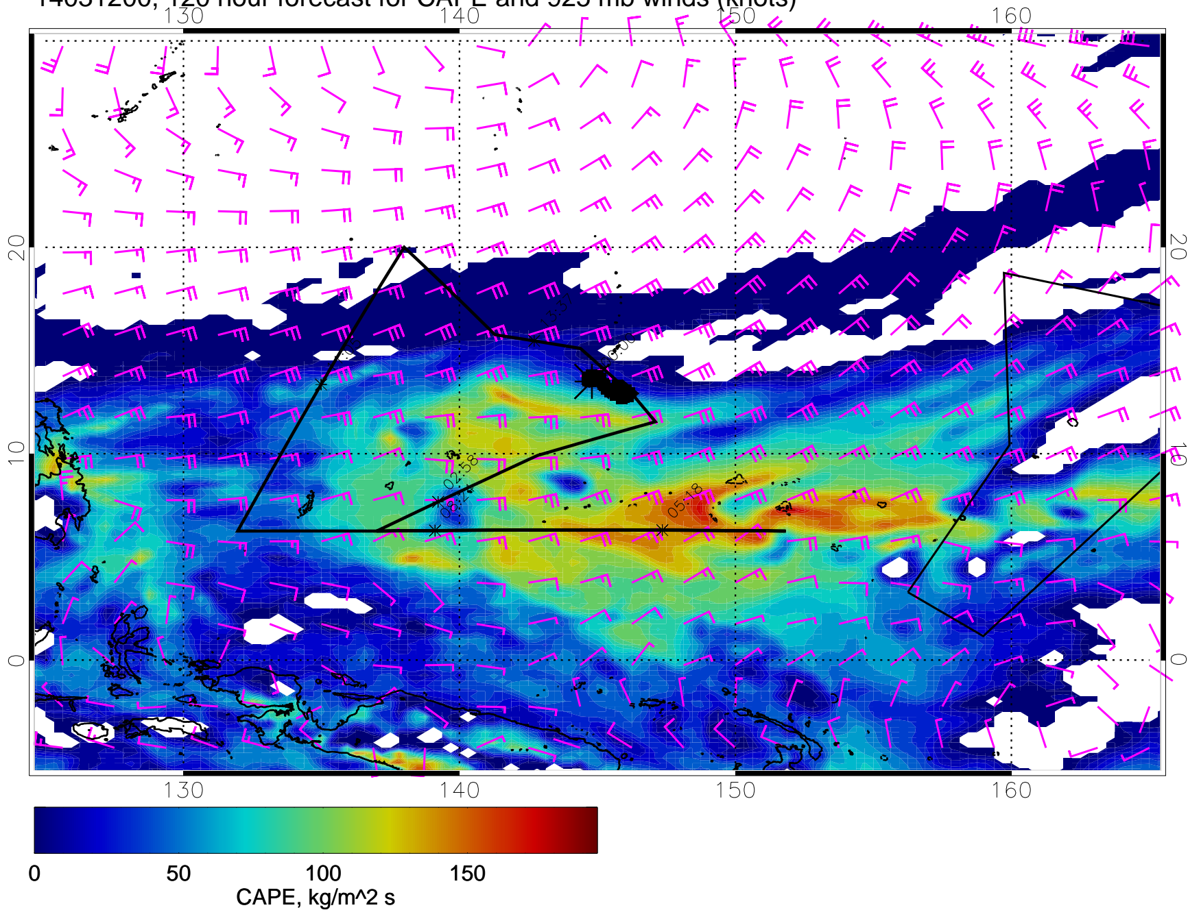
14031200, 120 hour forecast for CAPE and 925 mb winds (knots)
