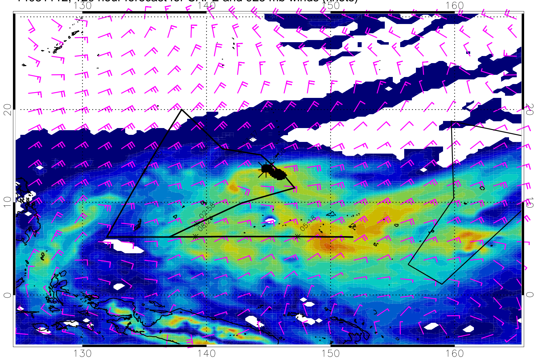
14031112, 120 hour forecast for CAPE and 925 mb winds (knots)
