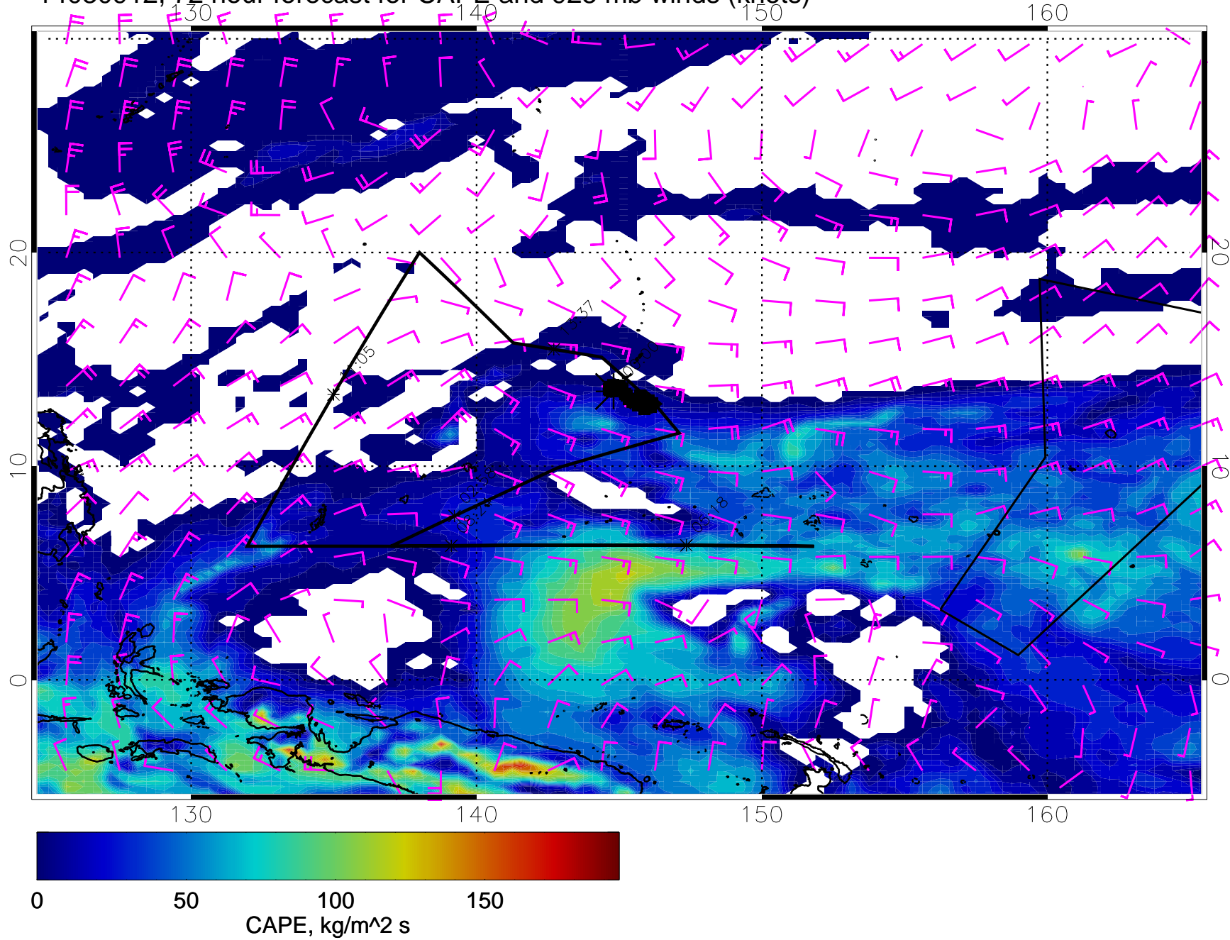
14030912, 72 hour forecast for CAPE and 925 mb winds (knots)
