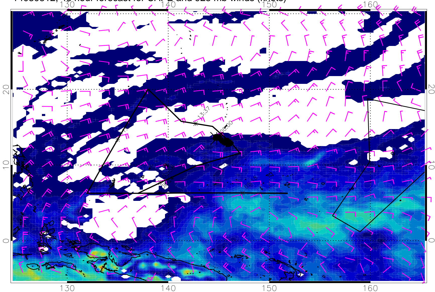
14030812, 48 hour forecast for CAPE and 925 mb winds (knots)
