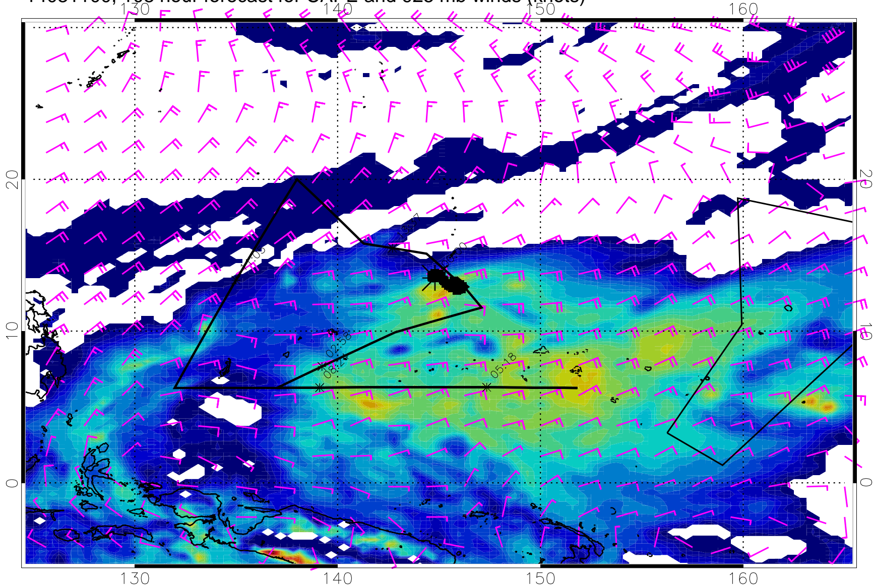
14031100, 108 hour forecast for CAPE and 925 mb winds (knots)
