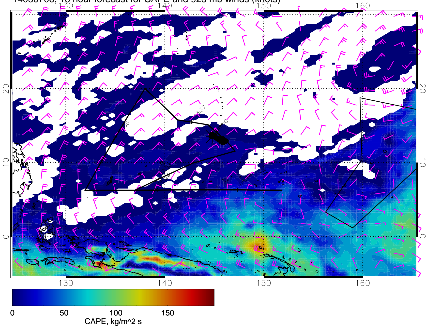
14030706, 18 hour forecast for CAPE and 925 mb winds (knots)
