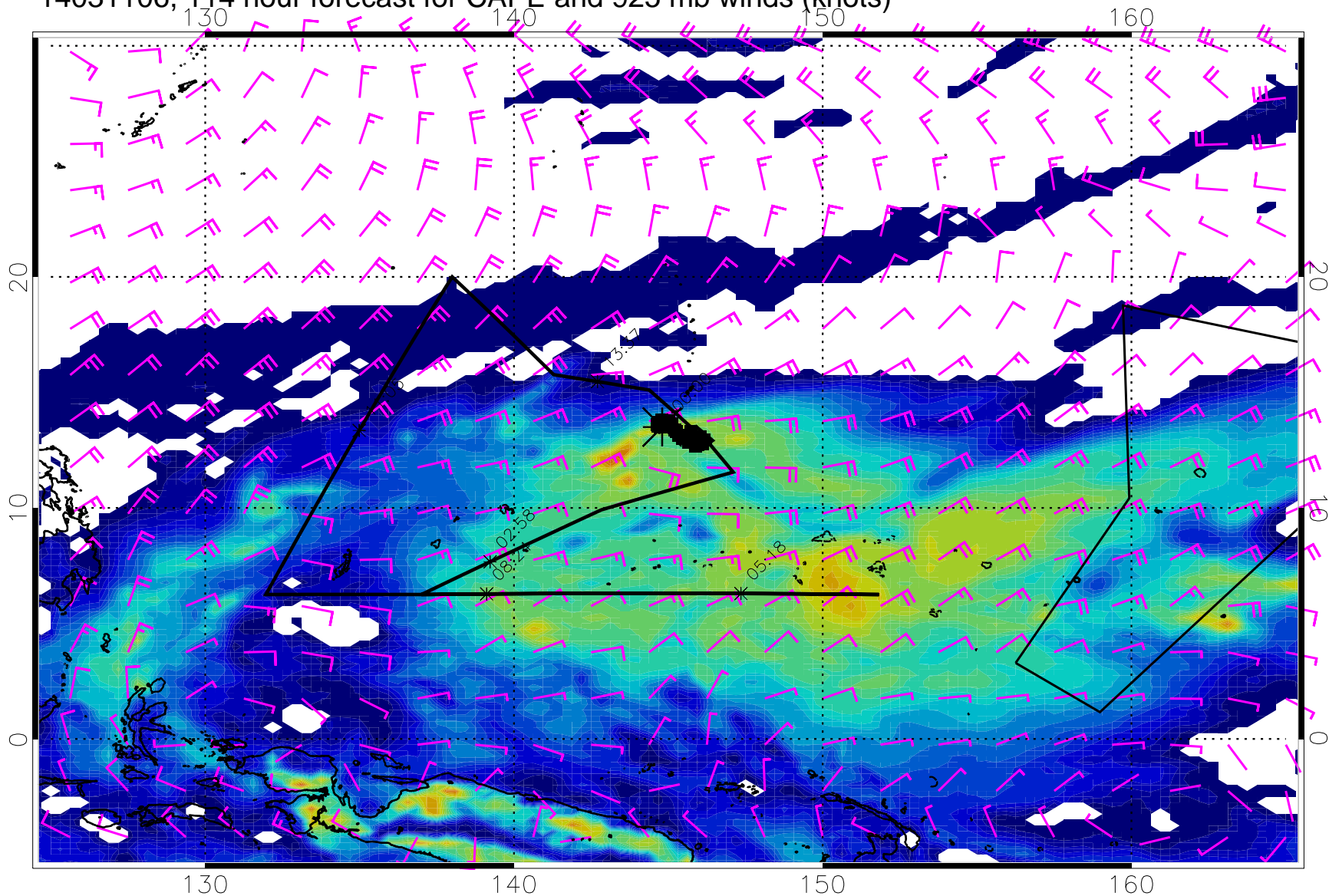
14031106, 114 hour forecast for CAPE and 925 mb winds (knots)
