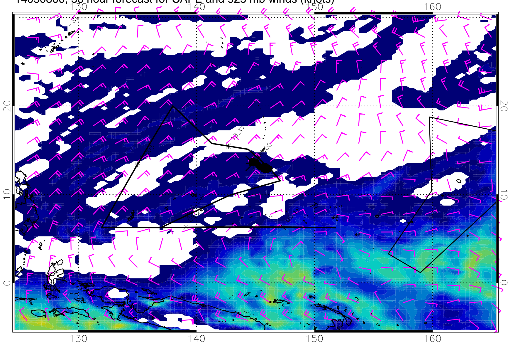
14030800, 36 hour forecast for CAPE and 925 mb winds (knots)
