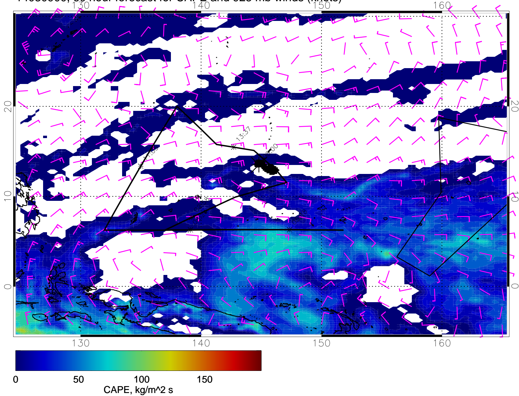
14030900, 60 hour forecast for CAPE and 925 mb winds (knots)
