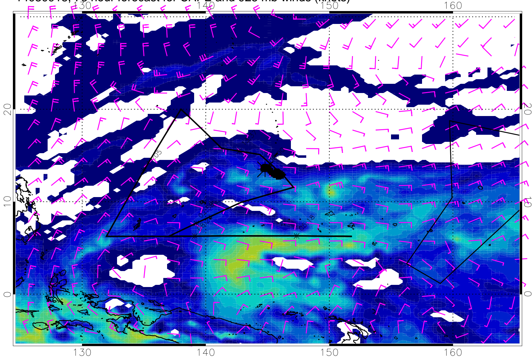
14030918, 78 hour forecast for CAPE and 925 mb winds (knots)
