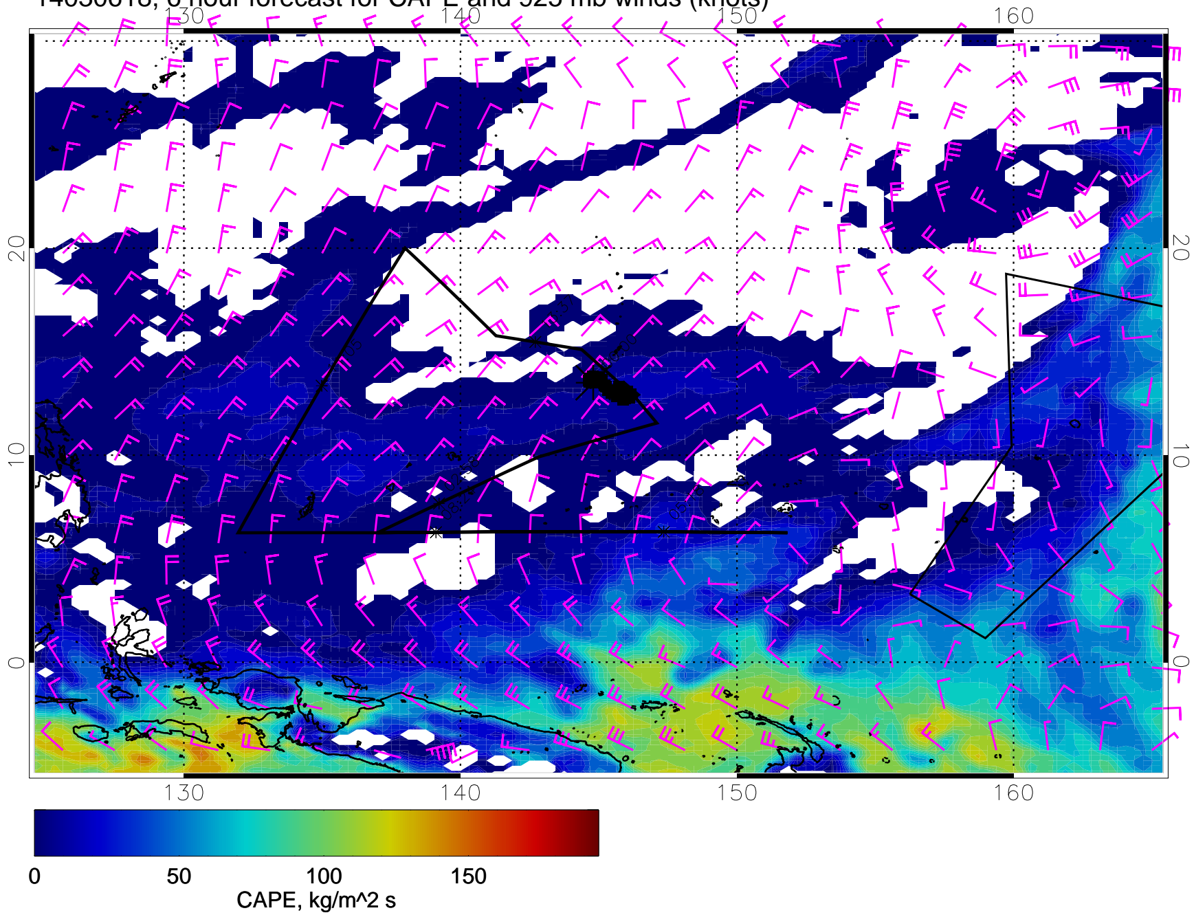
14030618, 6 hour forecast for CAPE and 925 mb winds (knots)
