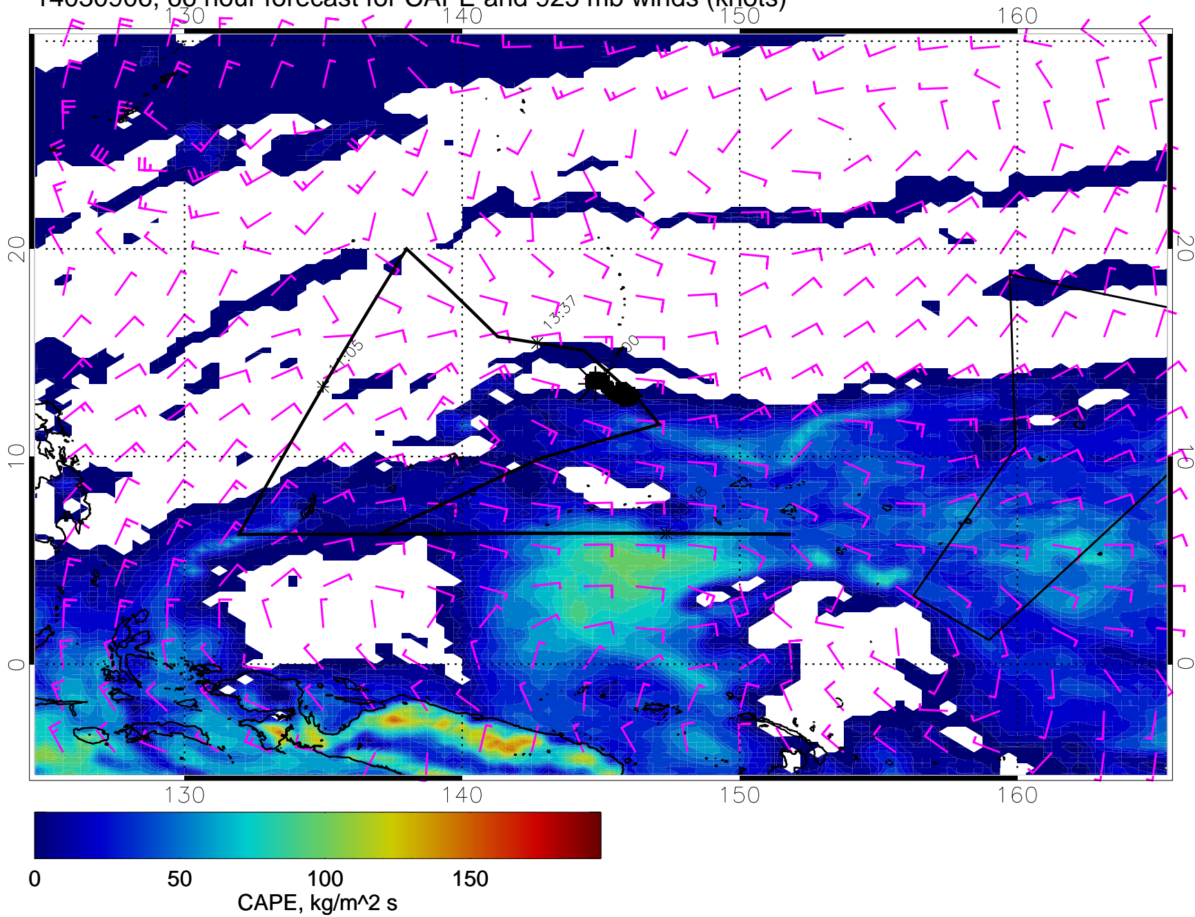
14030906, 66 hour forecast for CAPE and 925 mb winds (knots)
