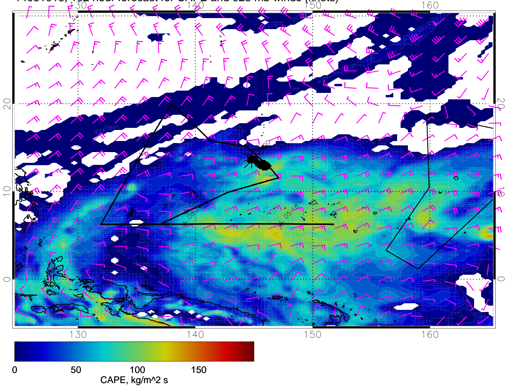
14031018, 102 hour forecast for CAPE and 925 mb winds (knots)
