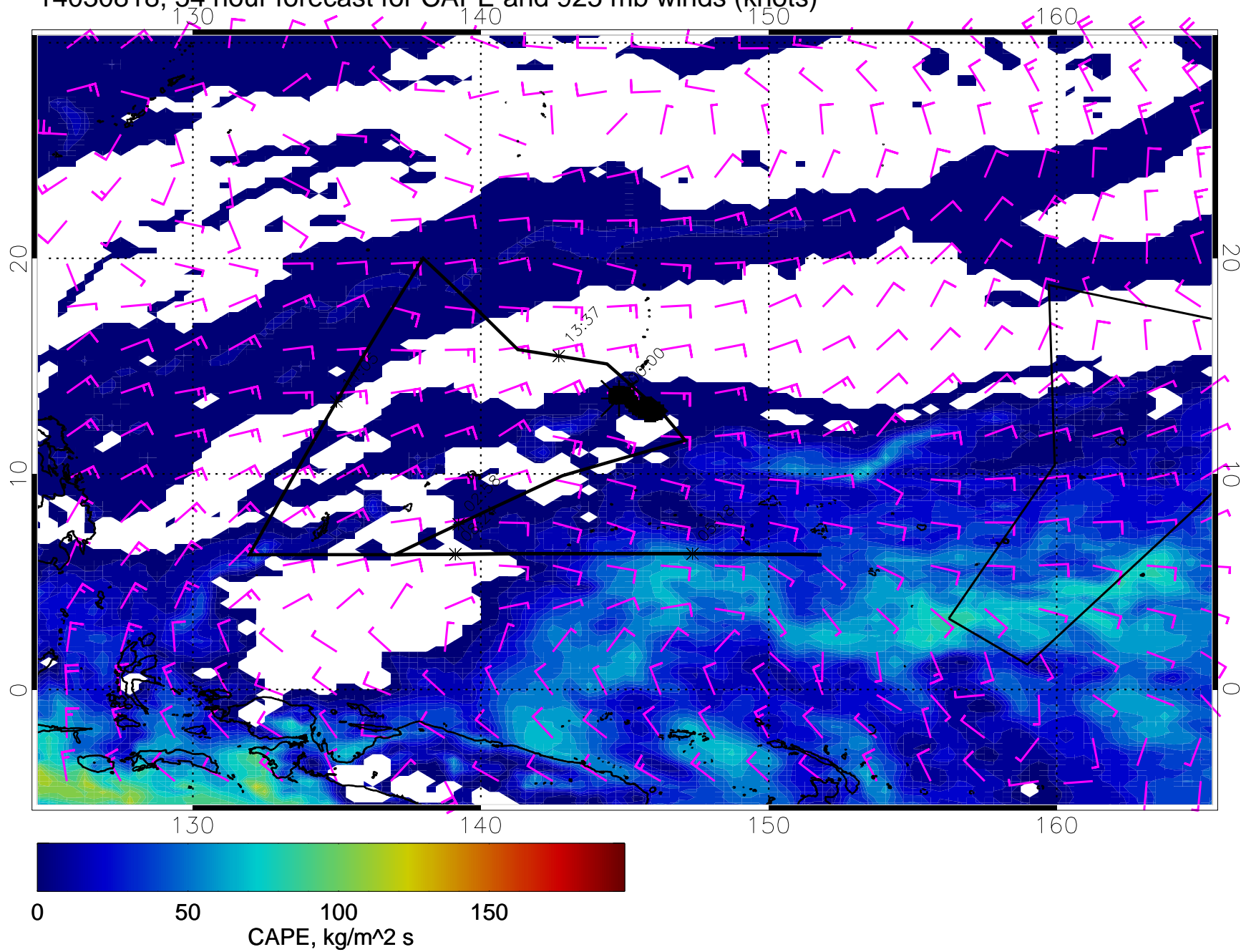
14030818, 54 hour forecast for CAPE and 925 mb winds (knots)
