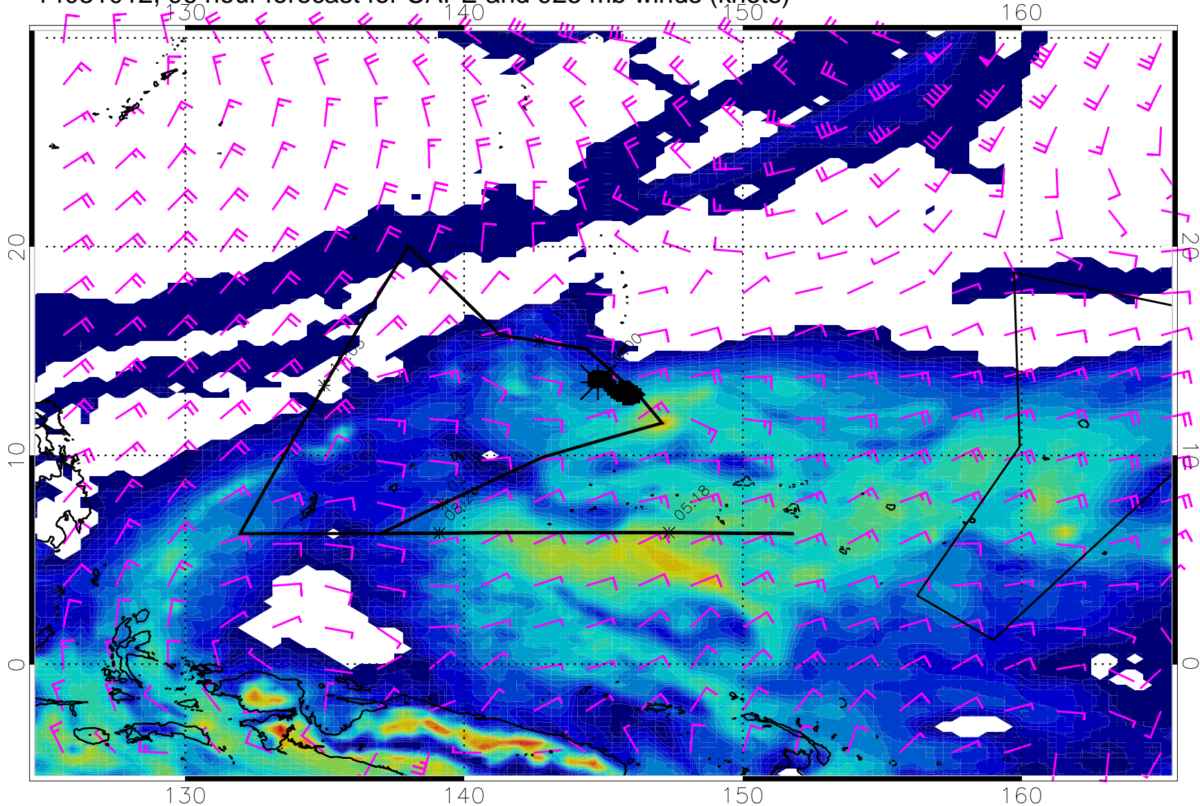
14031012, 96 hour forecast for CAPE and 925 mb winds (knots)
