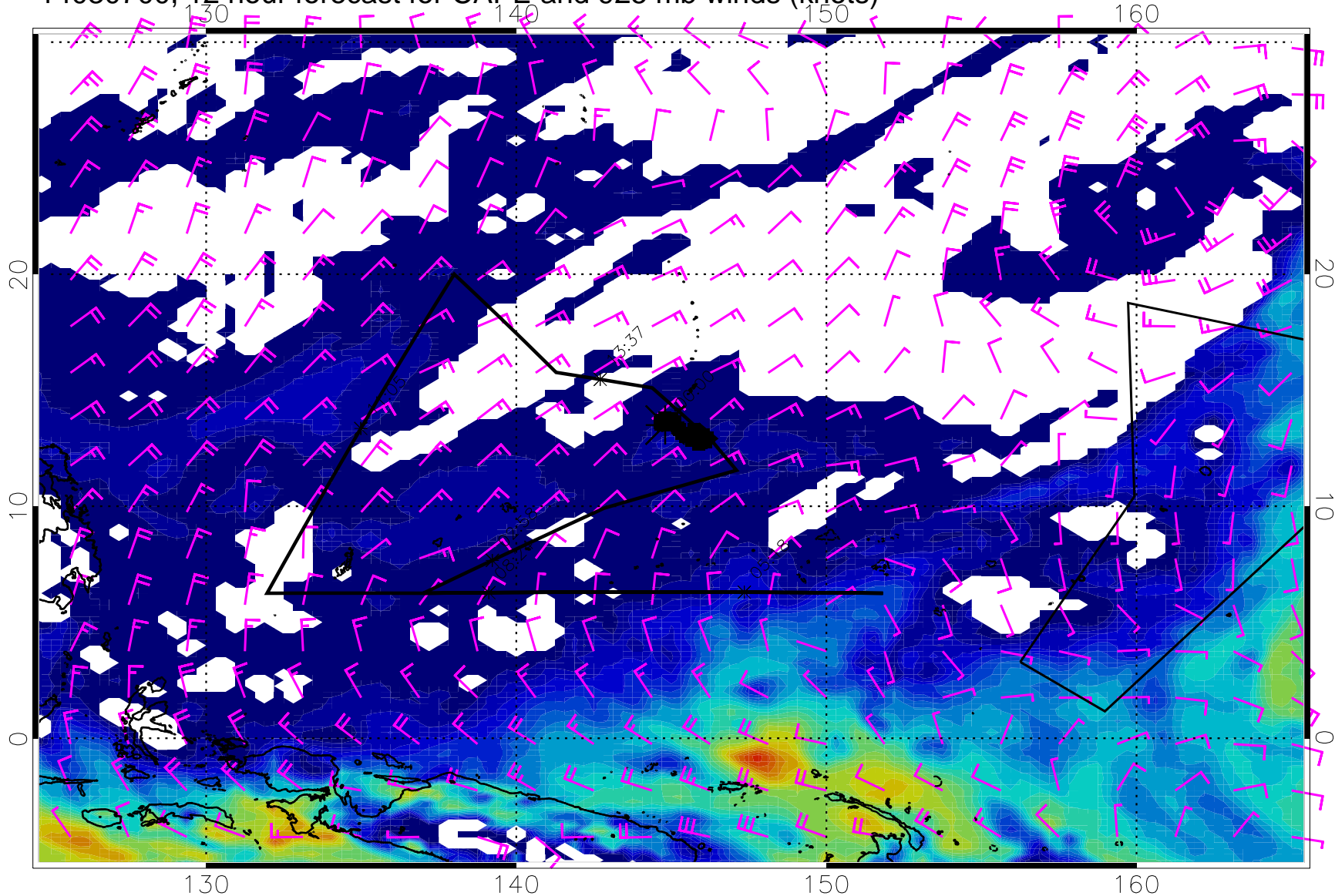
14030700, 12 hour forecast for CAPE and 925 mb winds (knots)
