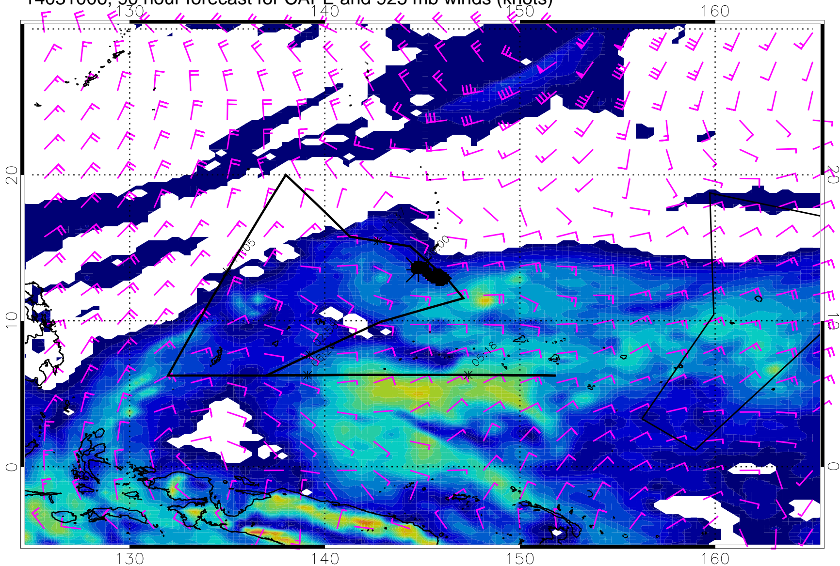
14031006, 90 hour forecast for CAPE and 925 mb winds (knots)
