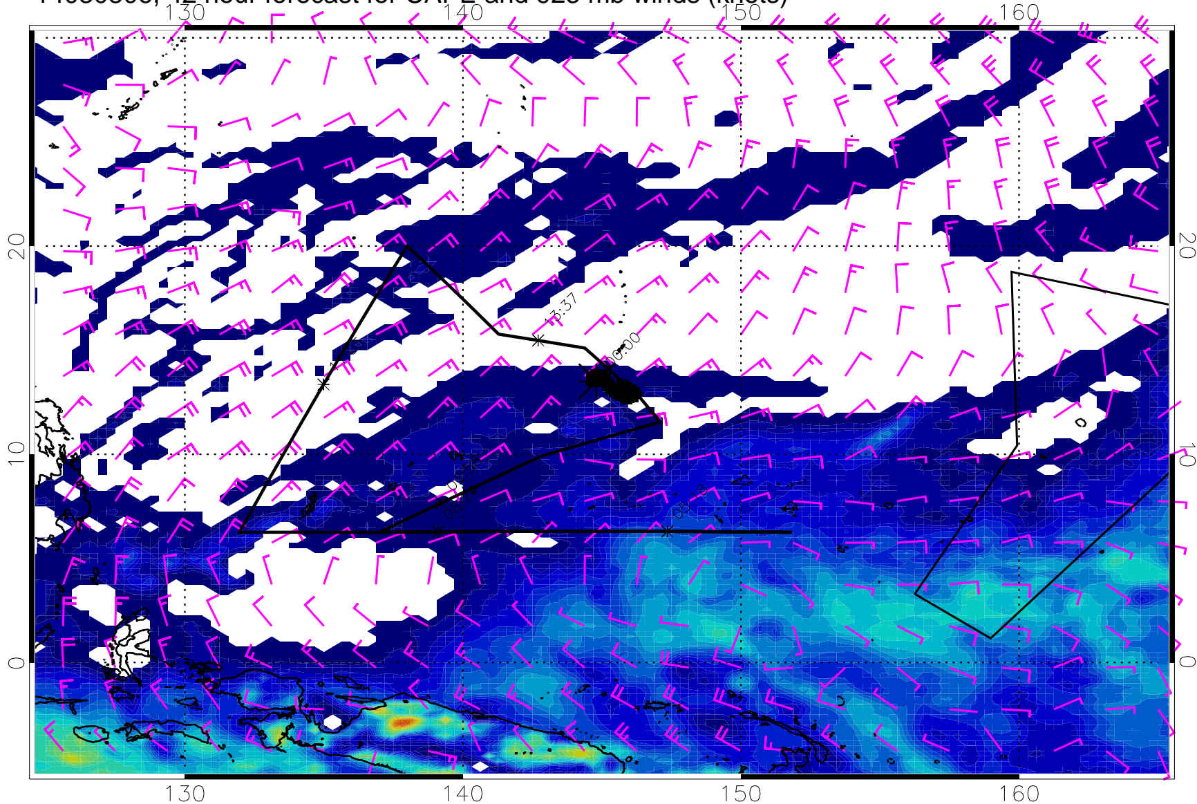
14030806, 42 hour forecast for CAPE and 925 mb winds (knots)
