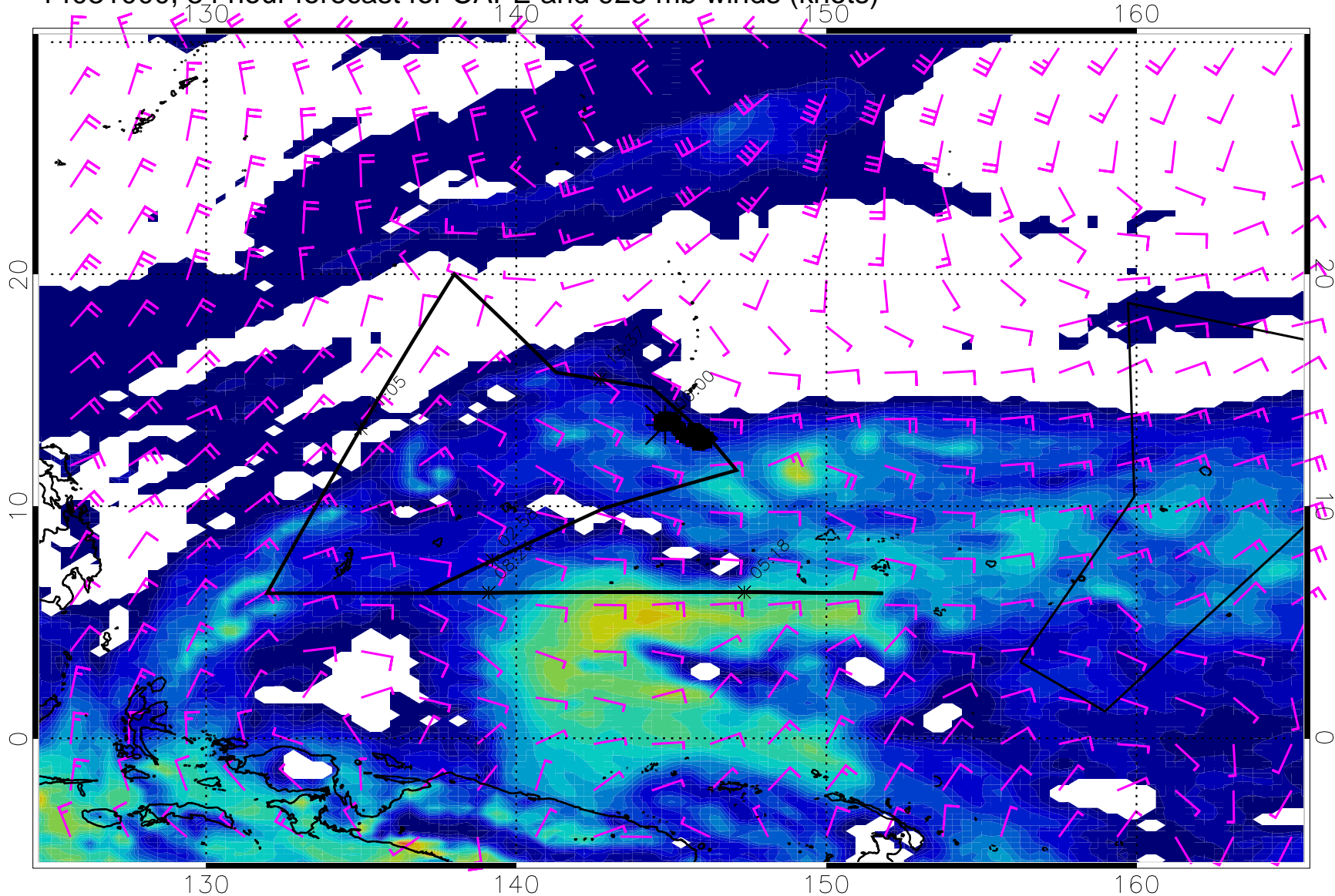
14031000, 84 hour forecast for CAPE and 925 mb winds (knots)
