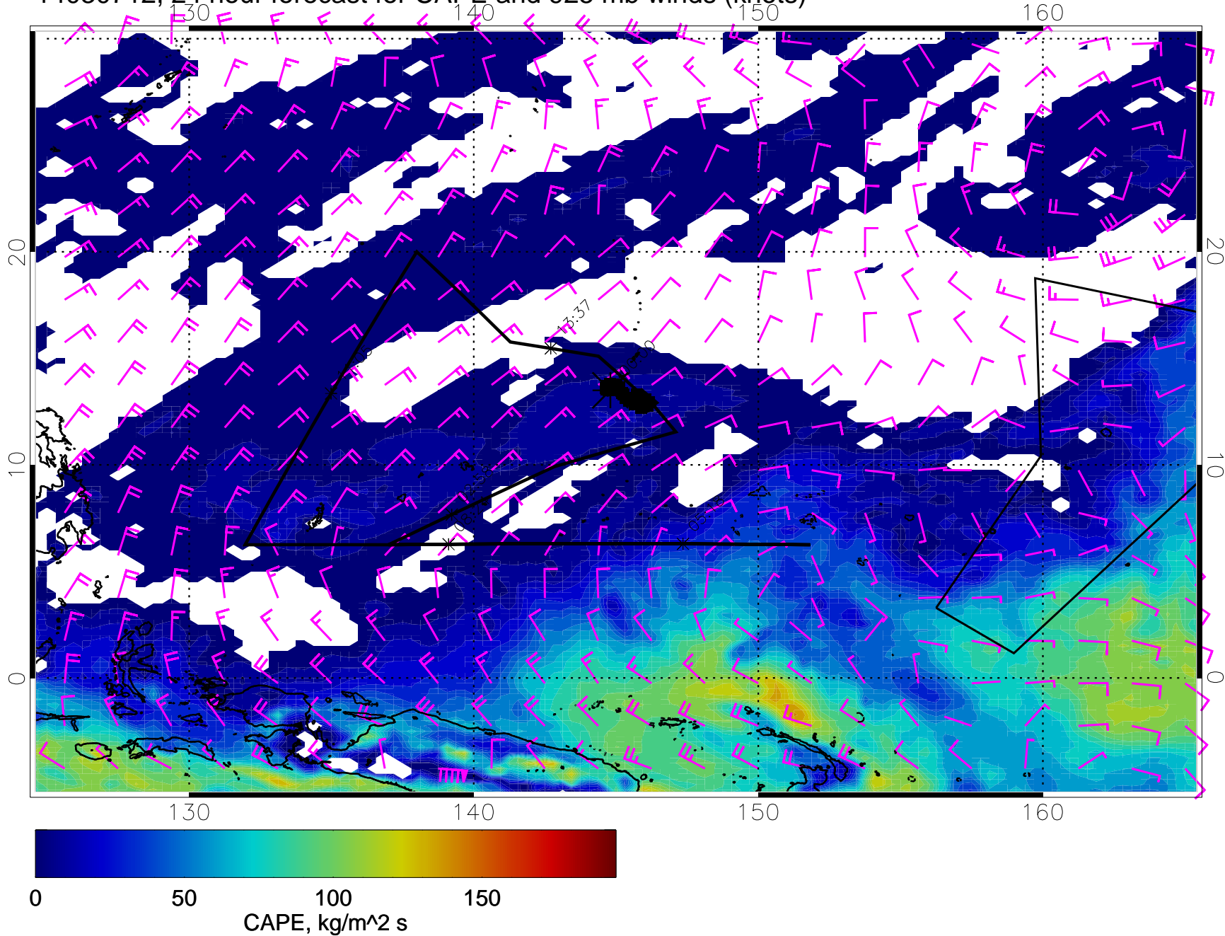
14030712, 24 hour forecast for CAPE and 925 mb winds (knots)
