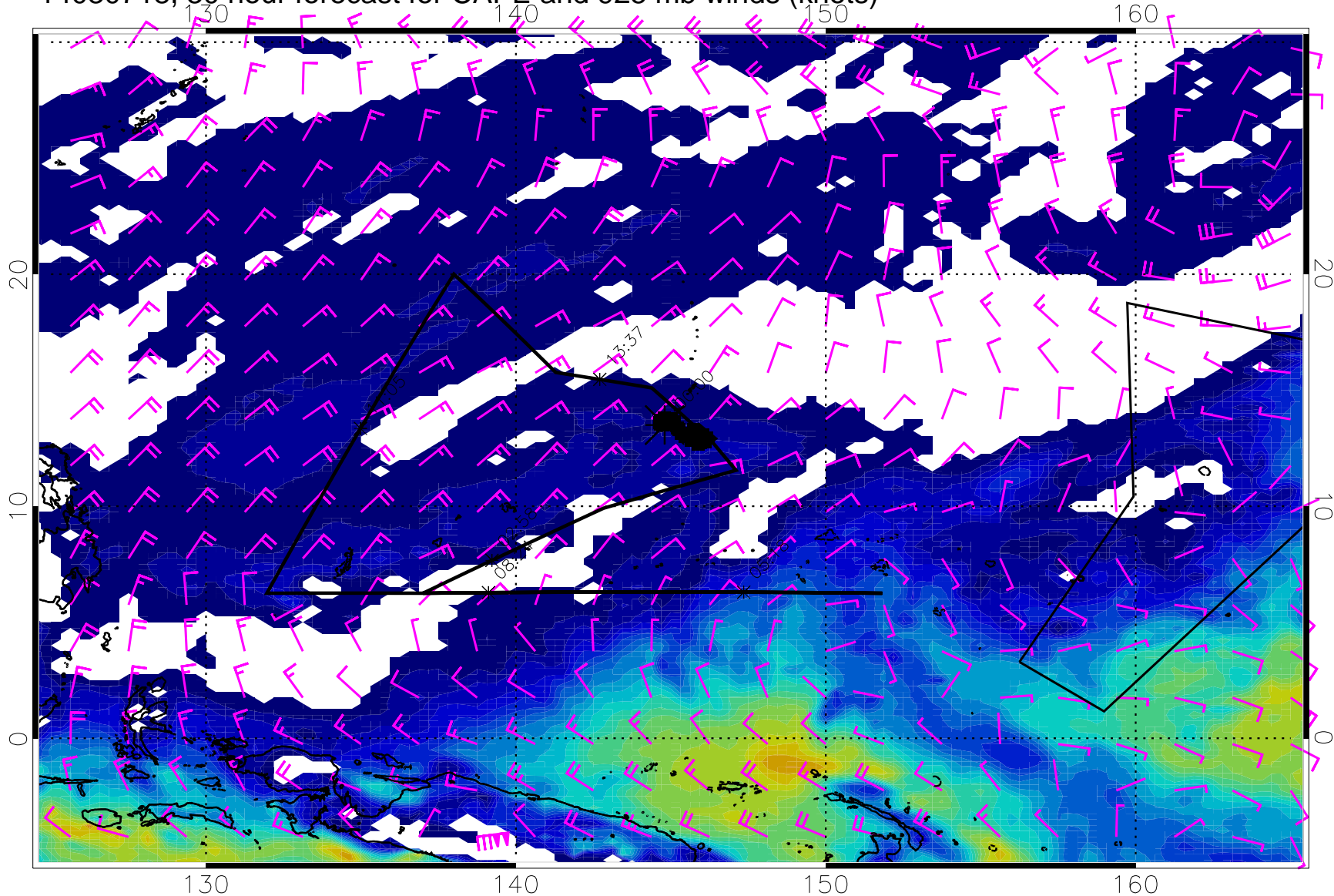
14030718, 30 hour forecast for CAPE and 925 mb winds (knots)
