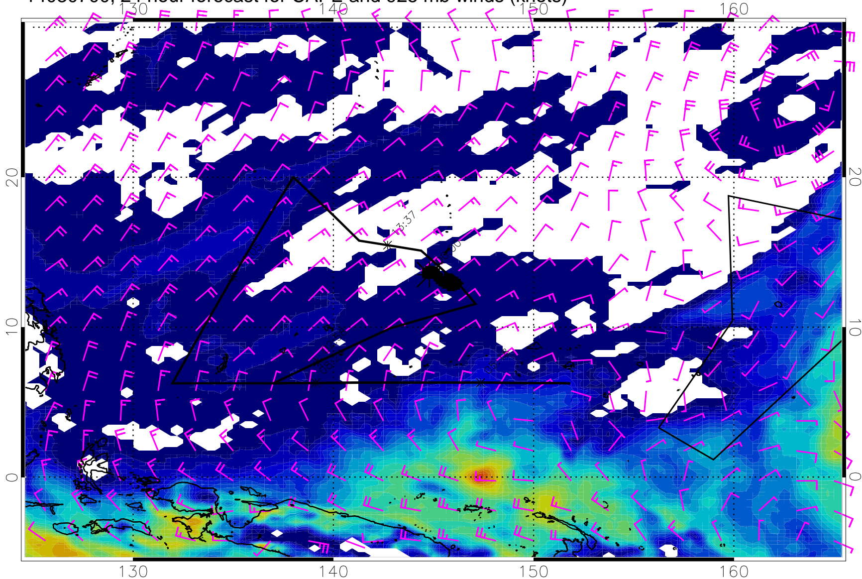
14030700, 24 hour forecast for CAPE and 925 mb winds (knots)
