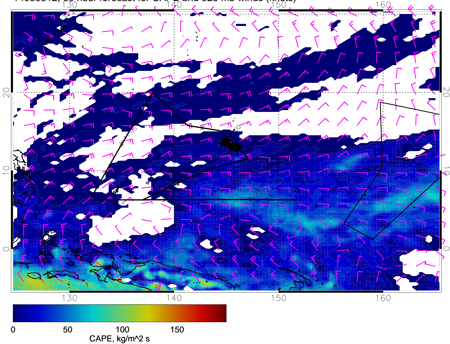
14030812, 60 hour forecast for CAPE and 925 mb winds (knots)
