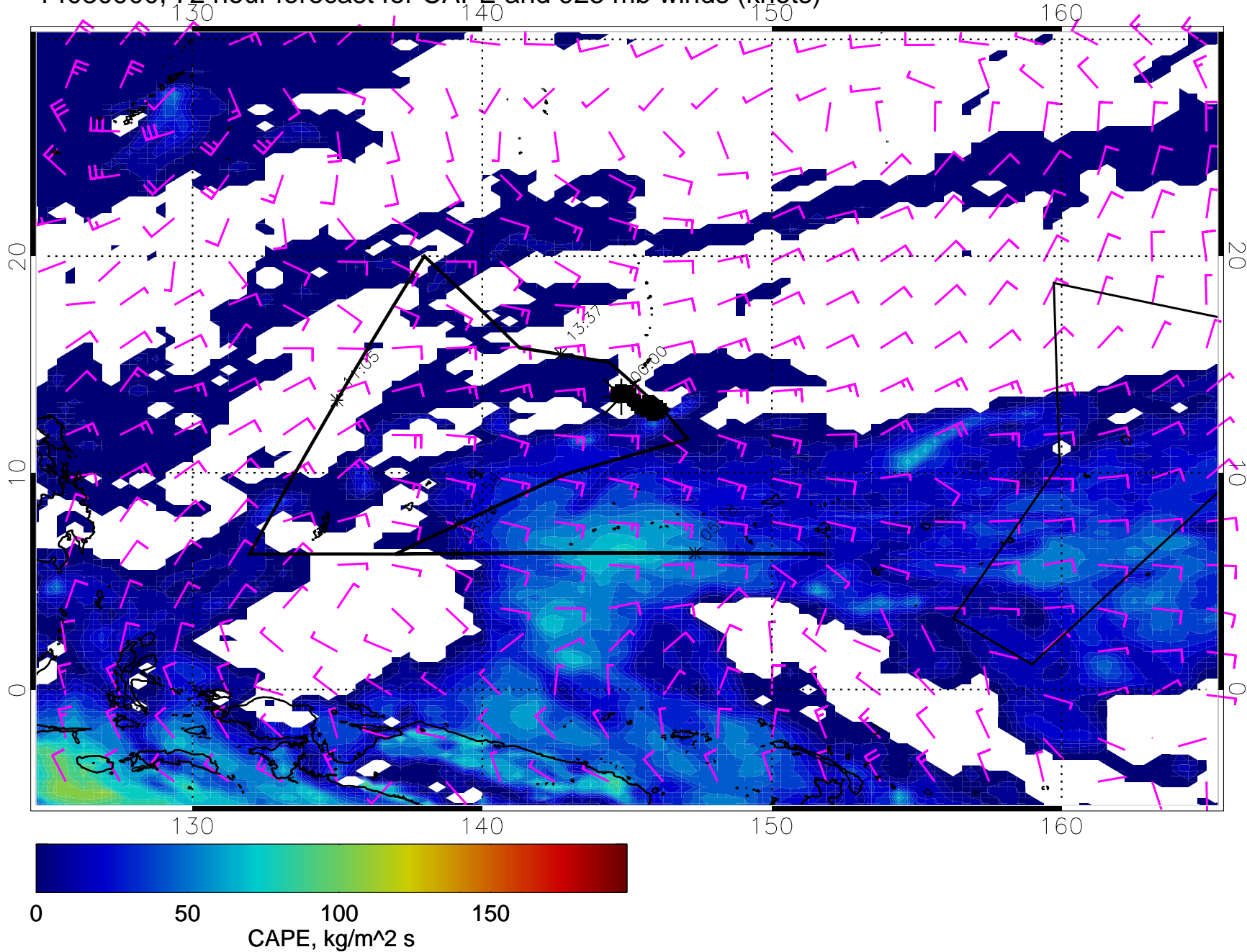
14030900, 72 hour forecast for CAPE and 925 mb winds (knots)
