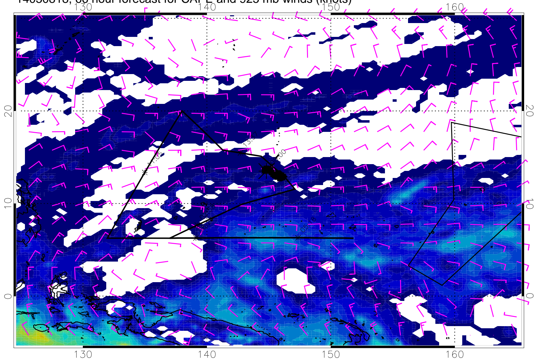
14030818, 66 hour forecast for CAPE and 925 mb winds (knots)
