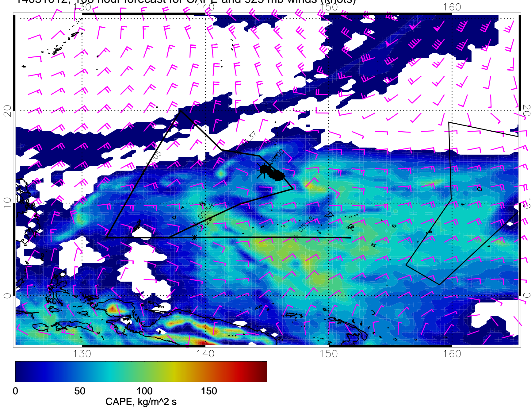
14031012, 108 hour forecast for CAPE and 925 mb winds (knots)
