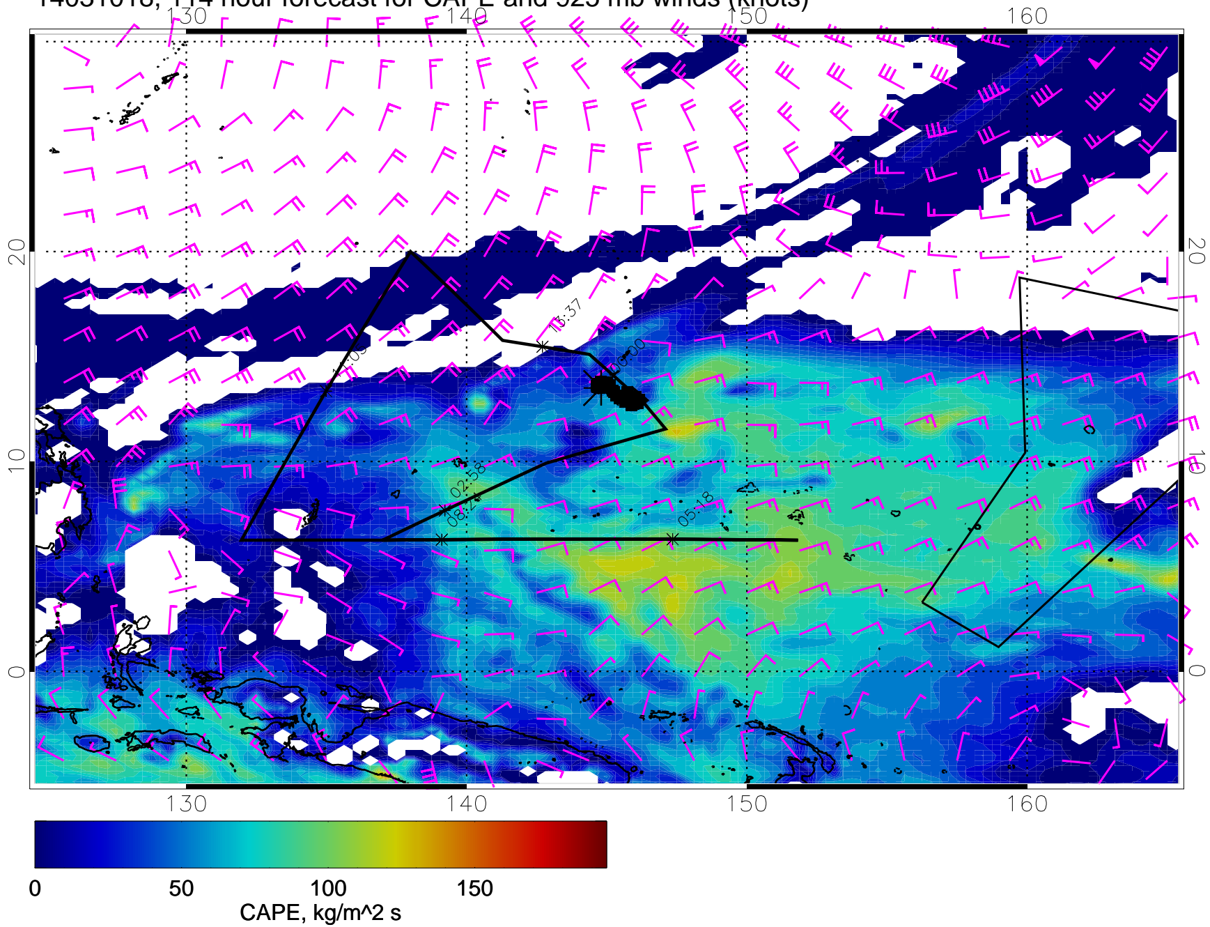
14031018, 114 hour forecast for CAPE and 925 mb winds (knots)
