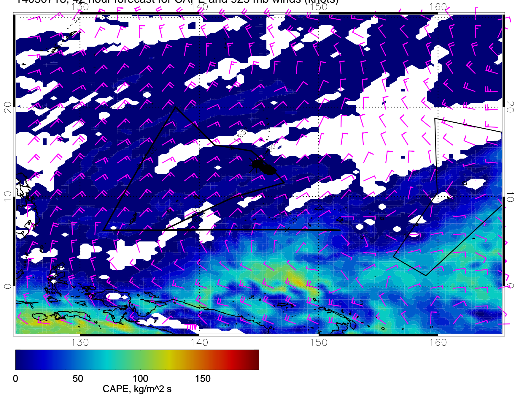
14030718, 42 hour forecast for CAPE and 925 mb winds (knots)
