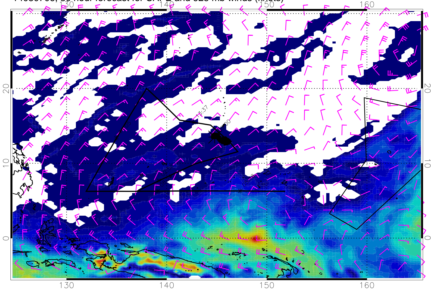
14030706, 30 hour forecast for CAPE and 925 mb winds (knots)
