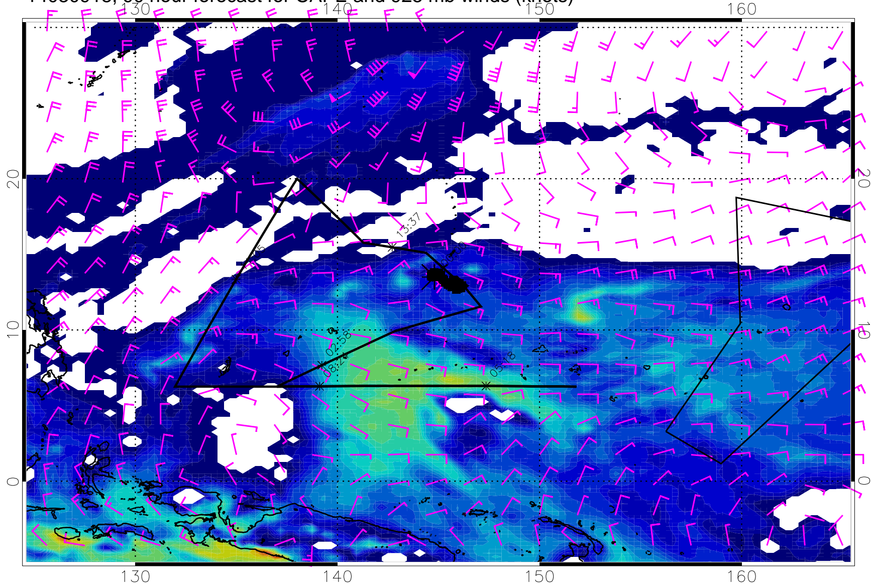
14030918, 90 hour forecast for CAPE and 925 mb winds (knots)
