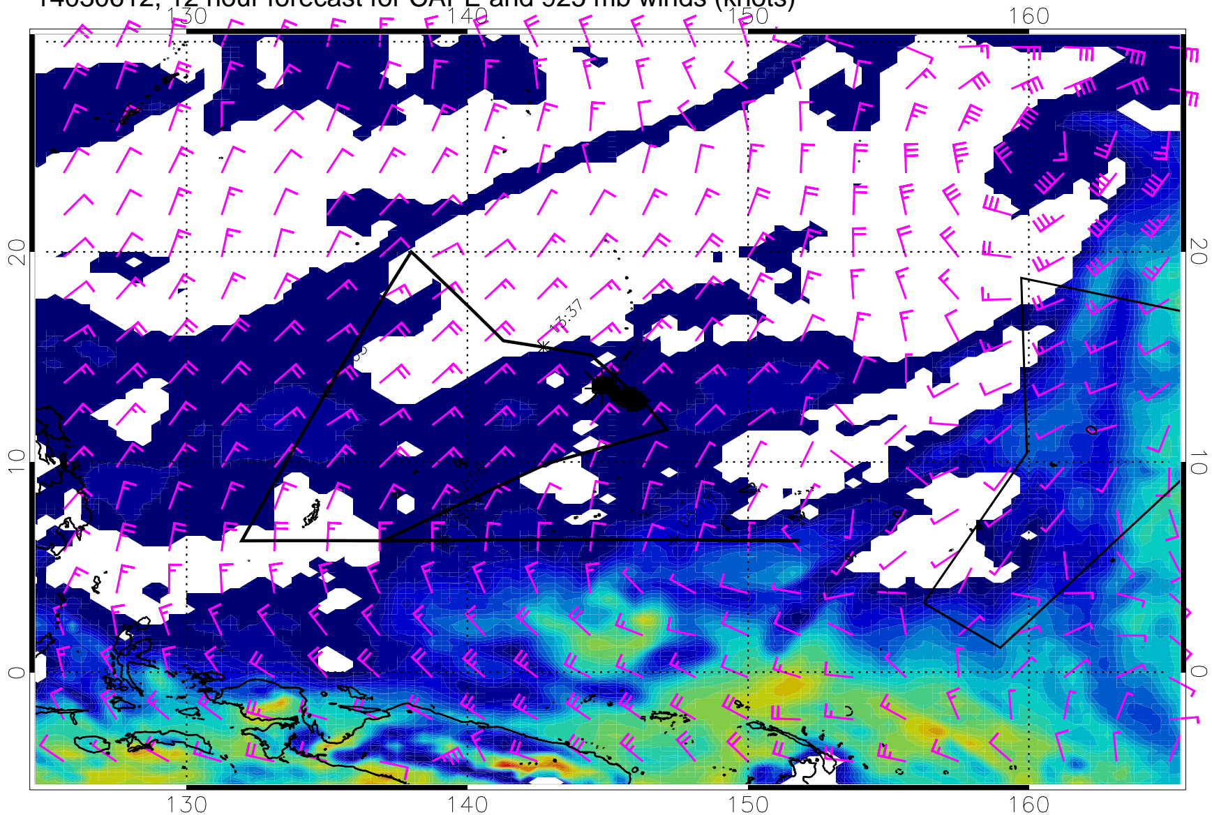
14030612, 12 hour forecast for CAPE and 925 mb winds (knots)
