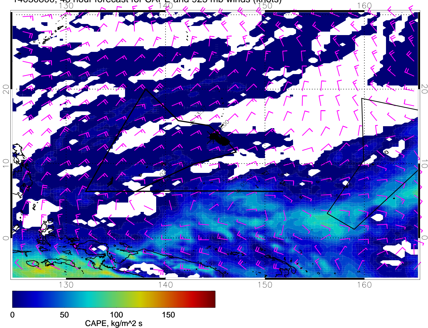
14030800, 48 hour forecast for CAPE and 925 mb winds (knots)
