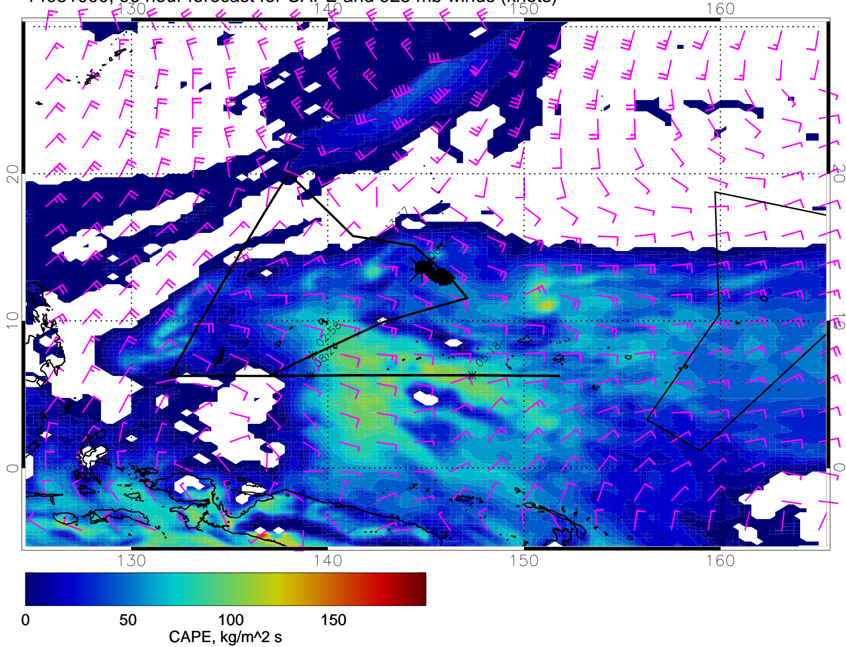
14031000, 96 hour forecast for CAPE and 925 mb winds (knots)
