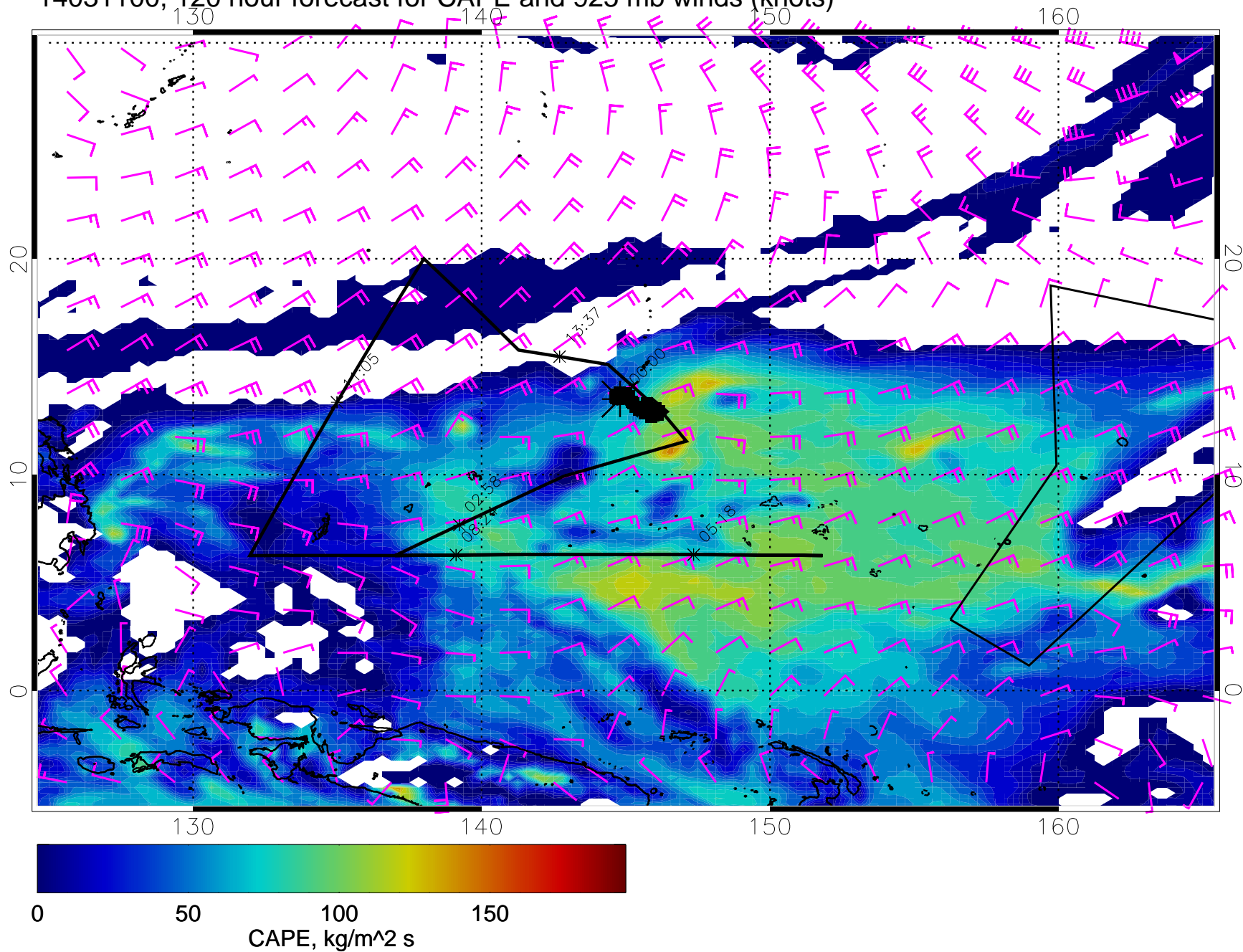
14031100, 120 hour forecast for CAPE and 925 mb winds (knots)
