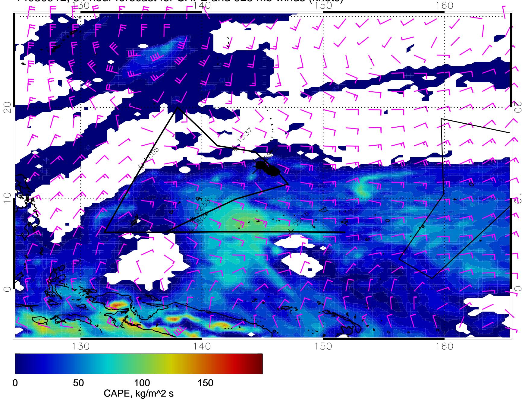
14030912, 84 hour forecast for CAPE and 925 mb winds (knots)
