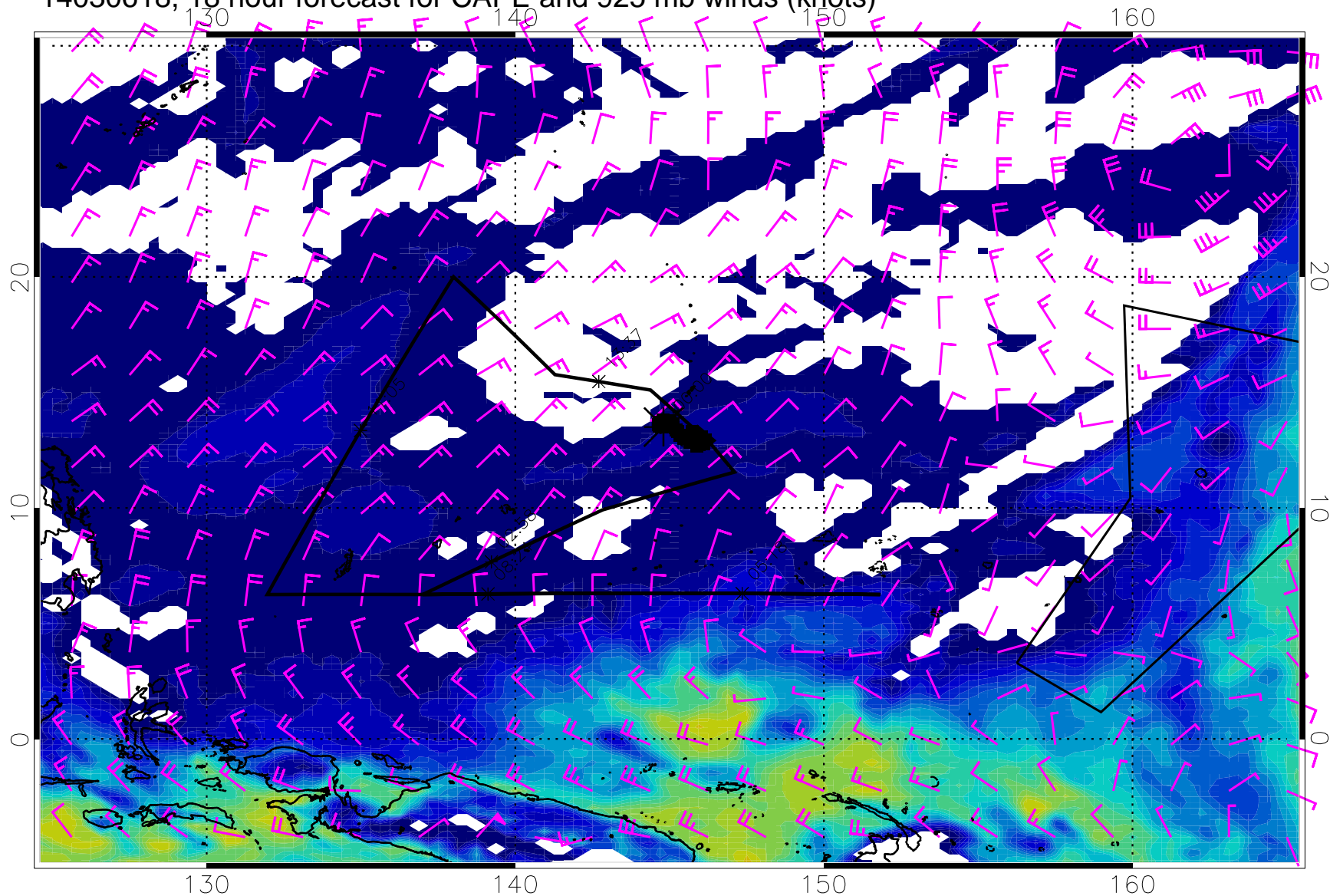
14030618, 18 hour forecast for CAPE and 925 mb winds (knots)
