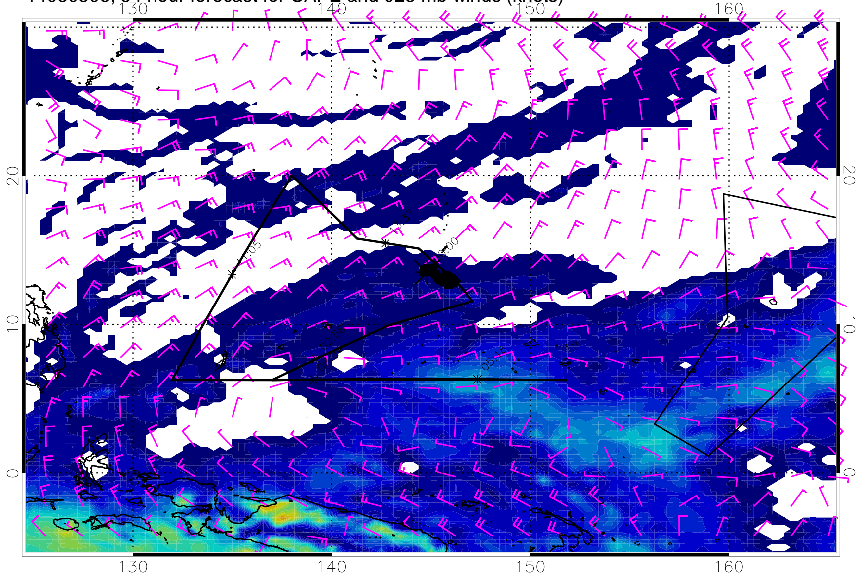
14030806, 54 hour forecast for CAPE and 925 mb winds (knots)
