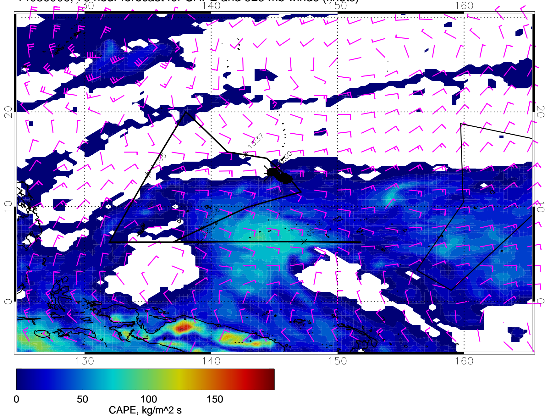
14030906, 78 hour forecast for CAPE and 925 mb winds (knots)
