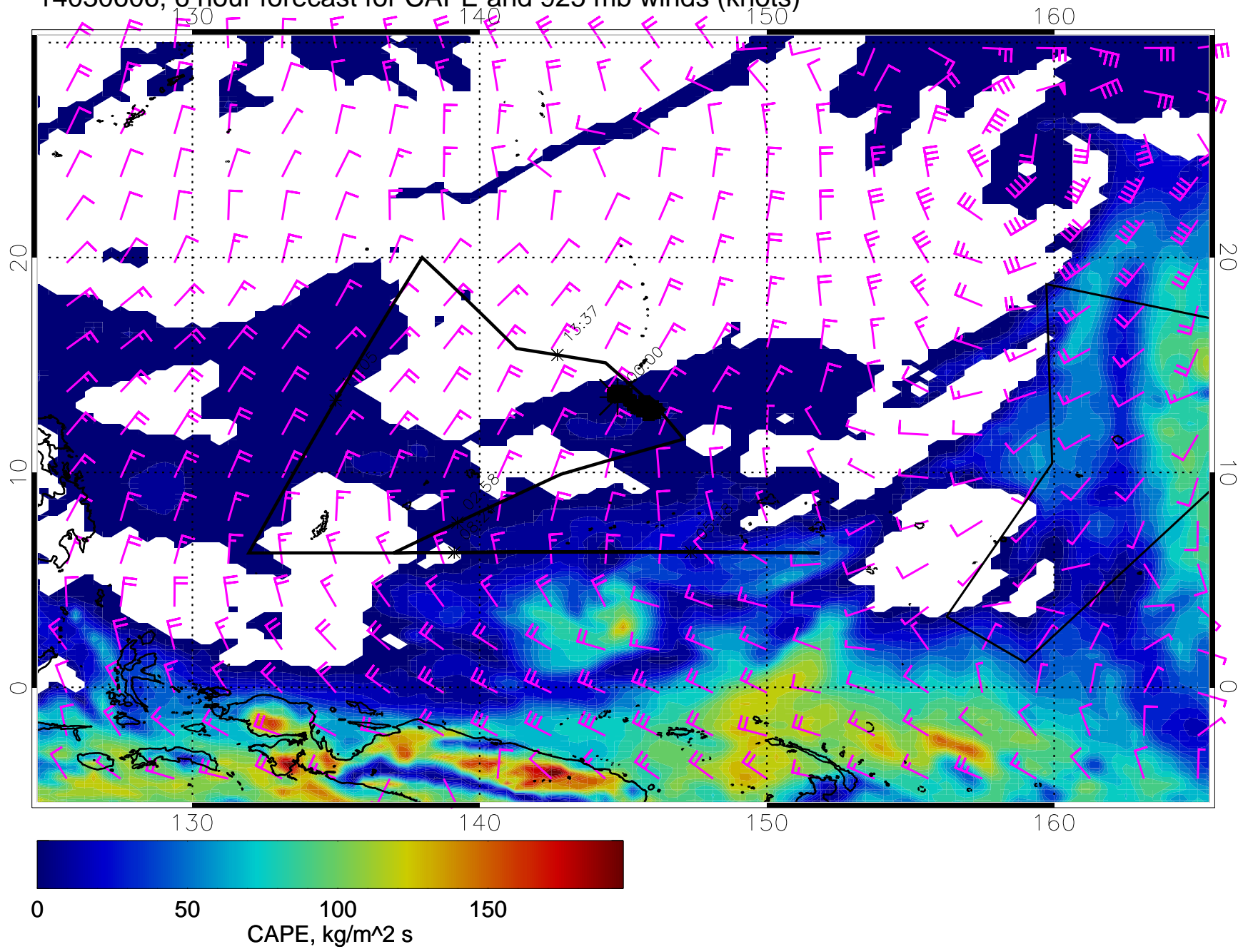
14030606, 6 hour forecast for CAPE and 925 mb winds (knots)
