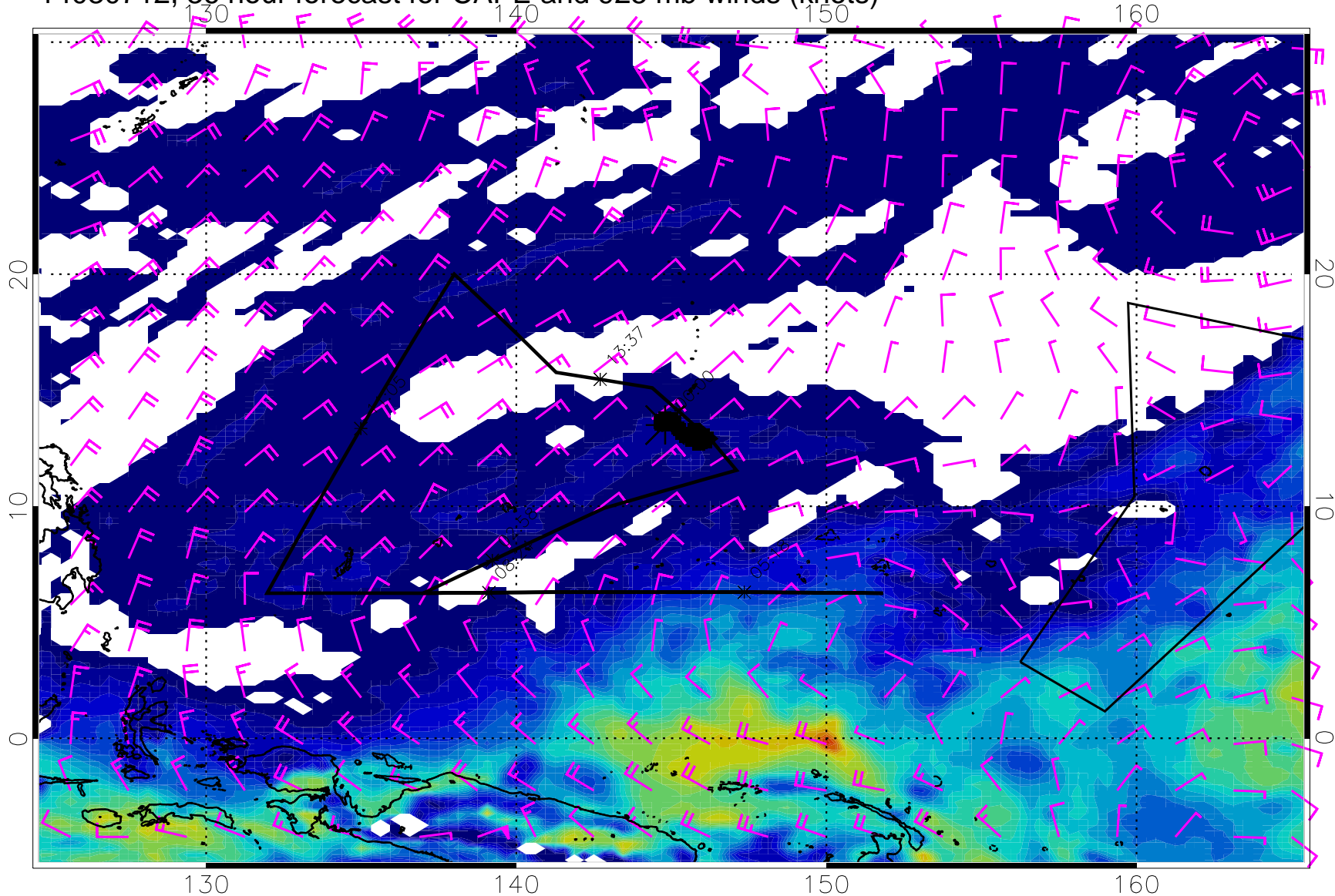
14030712, 36 hour forecast for CAPE and 925 mb winds (knots)
