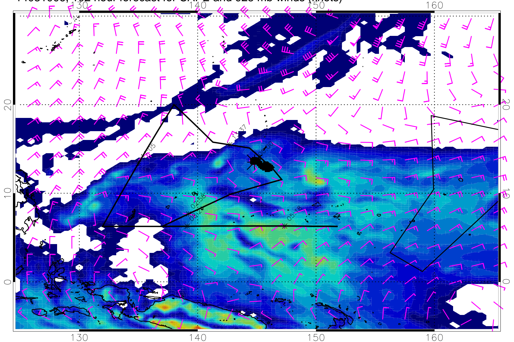
14031006, 102 hour forecast for CAPE and 925 mb winds (knots)
