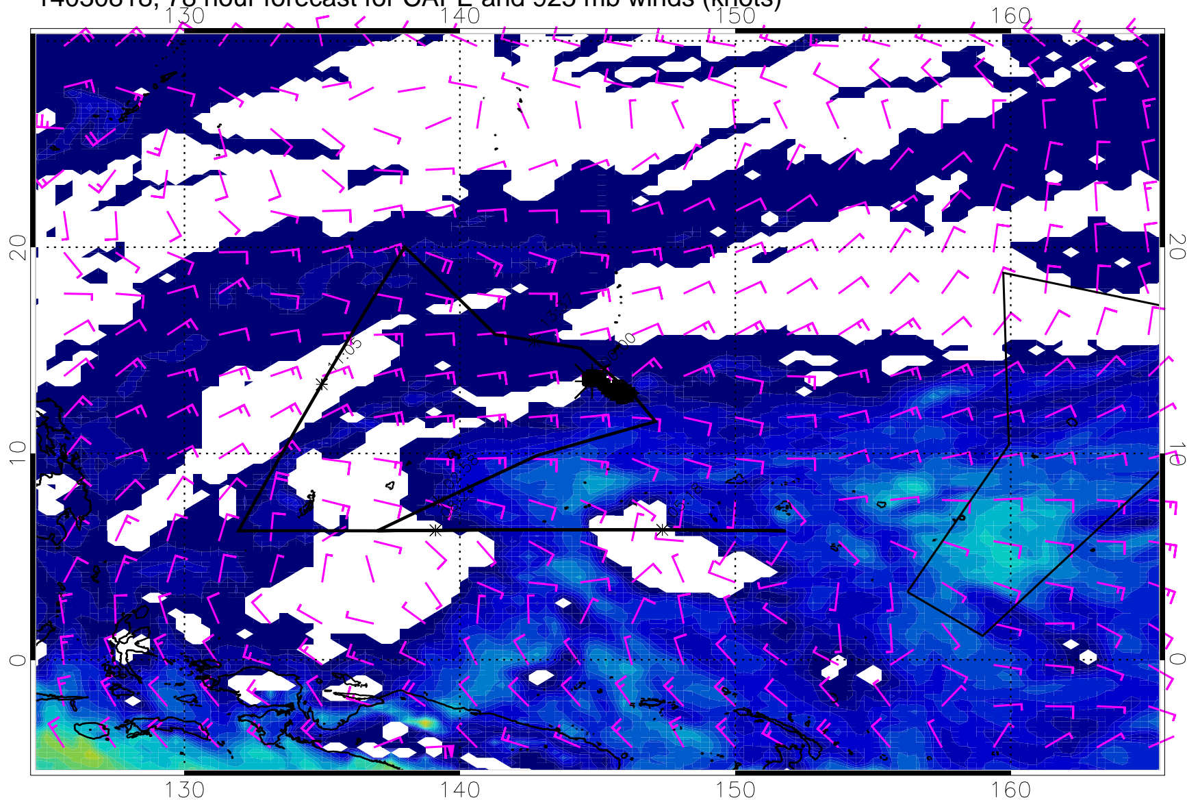
14030818, 78 hour forecast for CAPE and 925 mb winds (knots)
