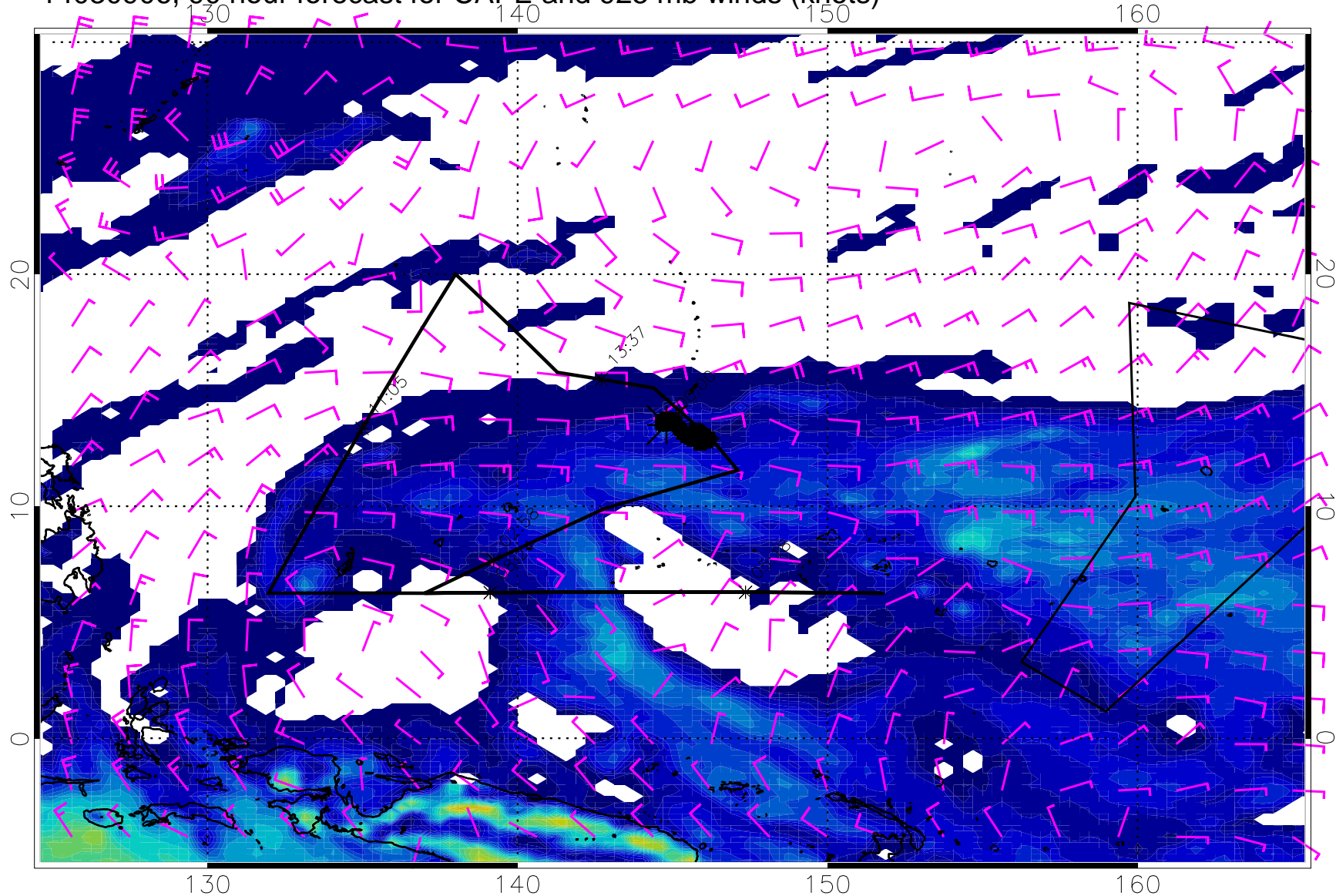
14030906, 90 hour forecast for CAPE and 925 mb winds (knots)
