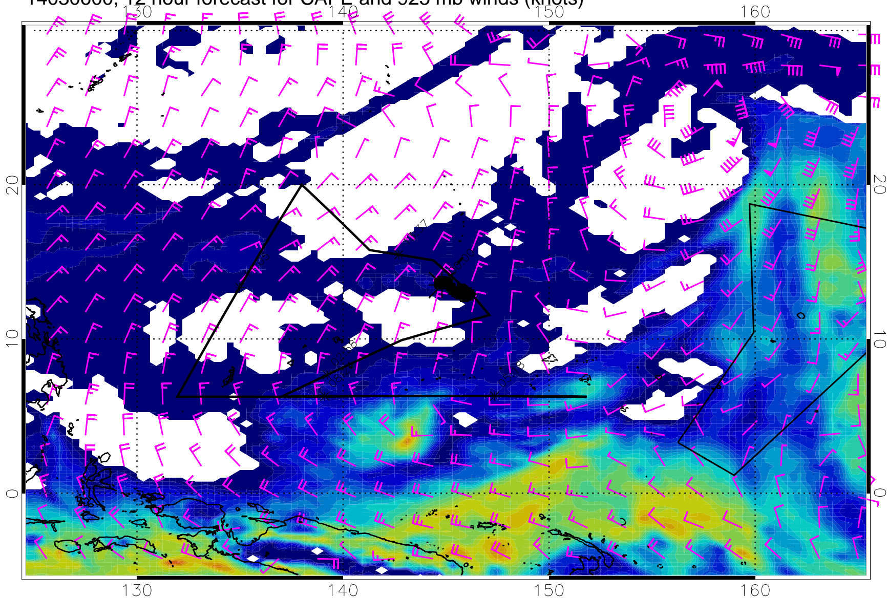
14030600, 12 hour forecast for CAPE and 925 mb winds (knots)
