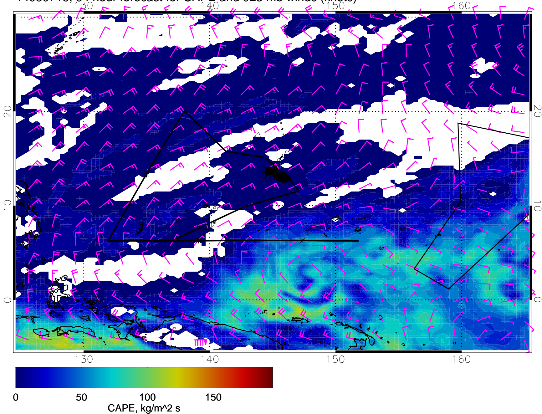
14030718, 54 hour forecast for CAPE and 925 mb winds (knots)
