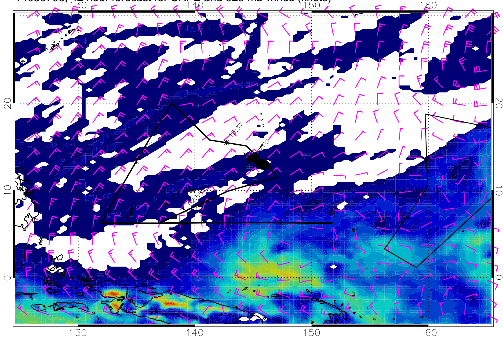
14030706, 42 hour forecast for CAPE and 925 mb winds (knots)
