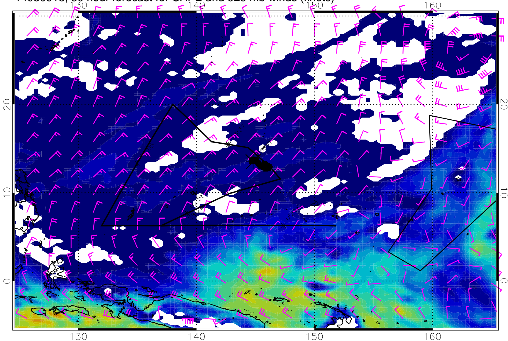
14030618, 30 hour forecast for CAPE and 925 mb winds (knots)
