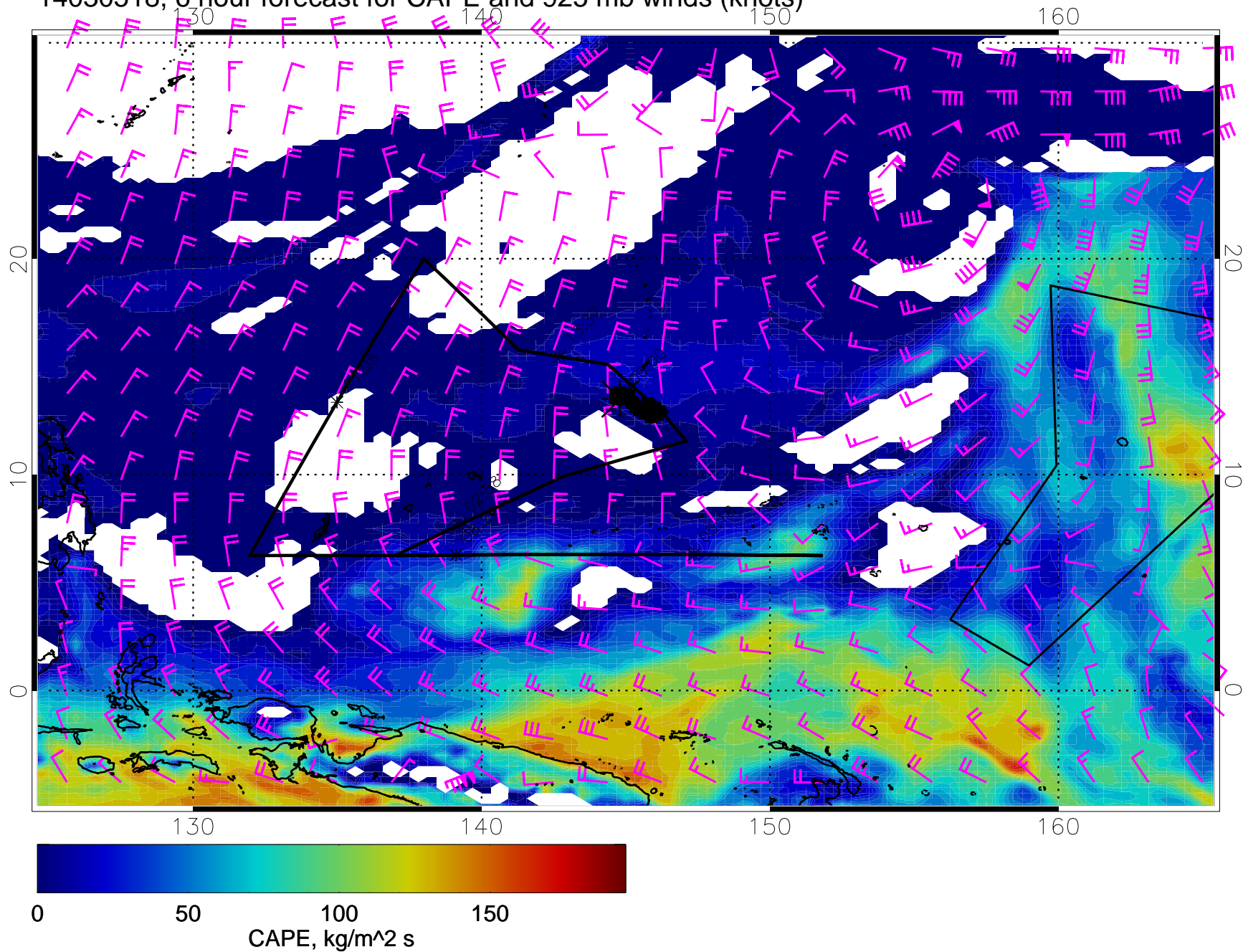
14030518, 6 hour forecast for CAPE and 925 mb winds (knots)
