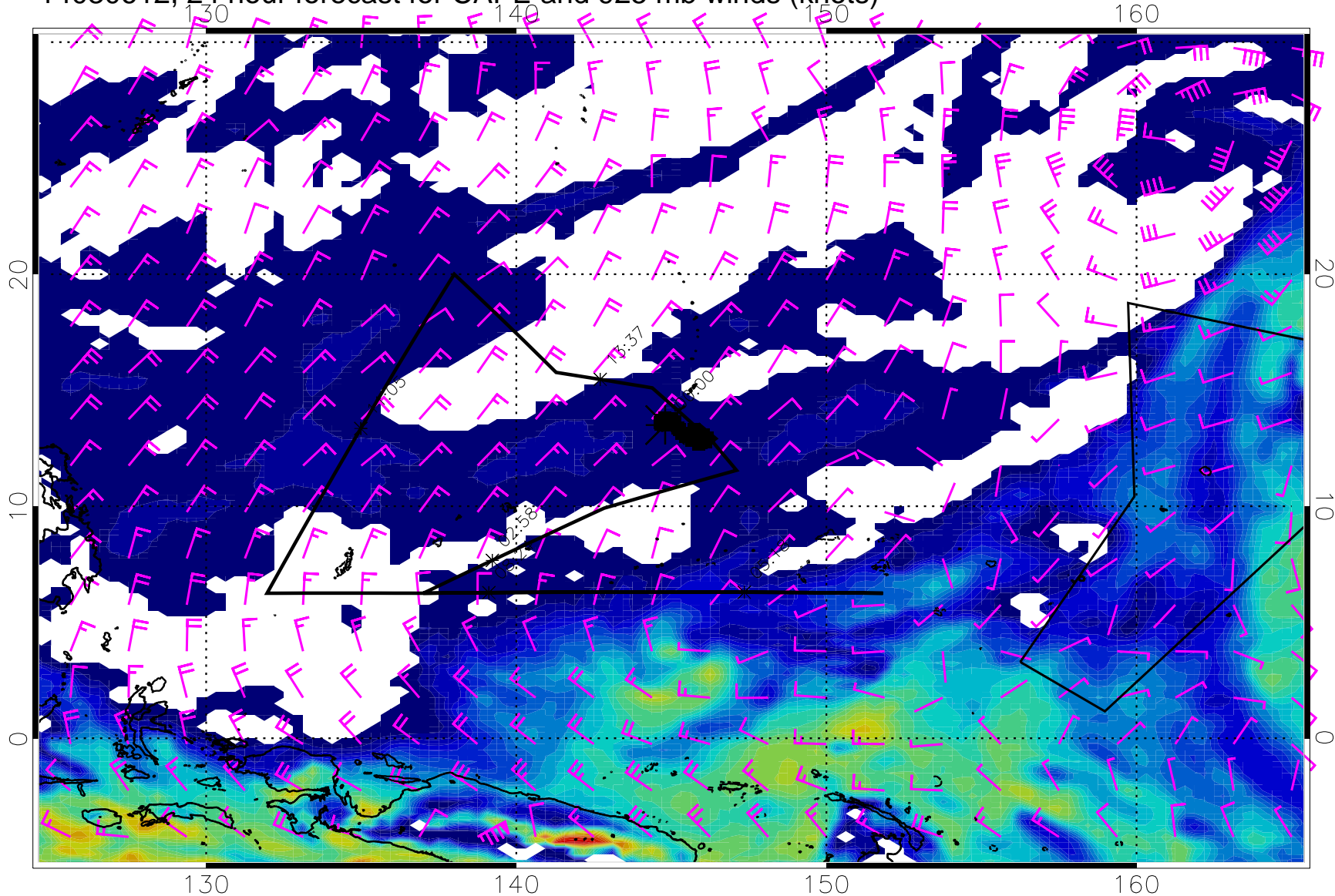
14030612, 24 hour forecast for CAPE and 925 mb winds (knots)
