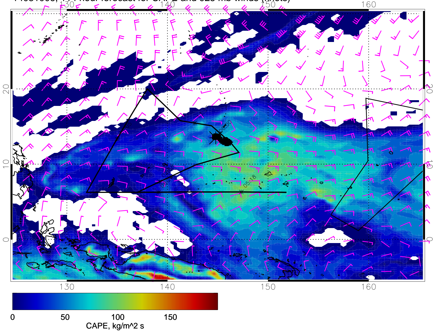
14031006, 114 hour forecast for CAPE and 925 mb winds (knots)
