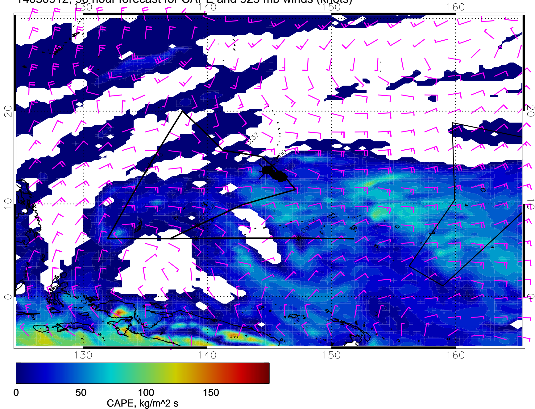
14030912, 96 hour forecast for CAPE and 925 mb winds (knots)
