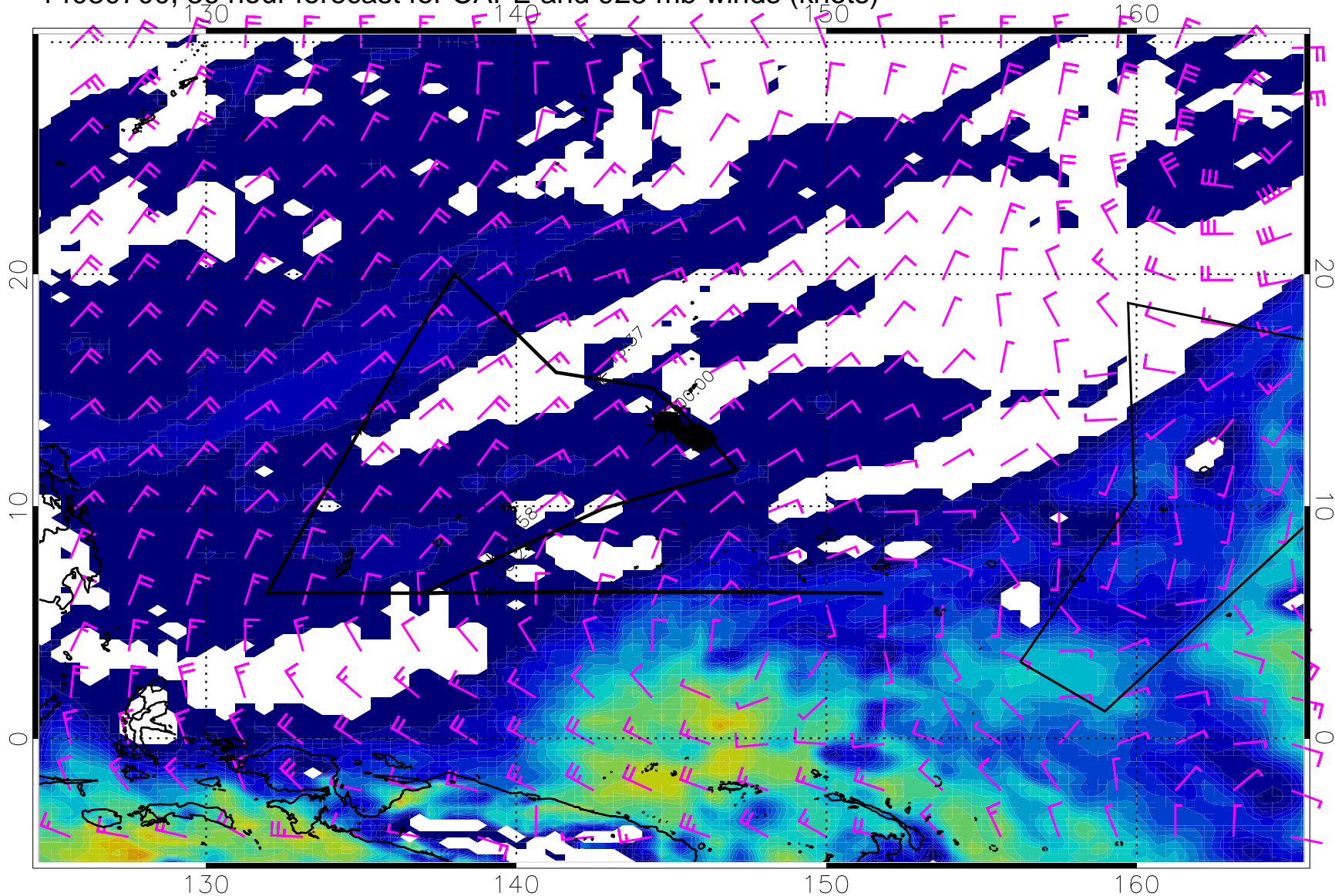
14030700, 36 hour forecast for CAPE and 925 mb winds (knots)
