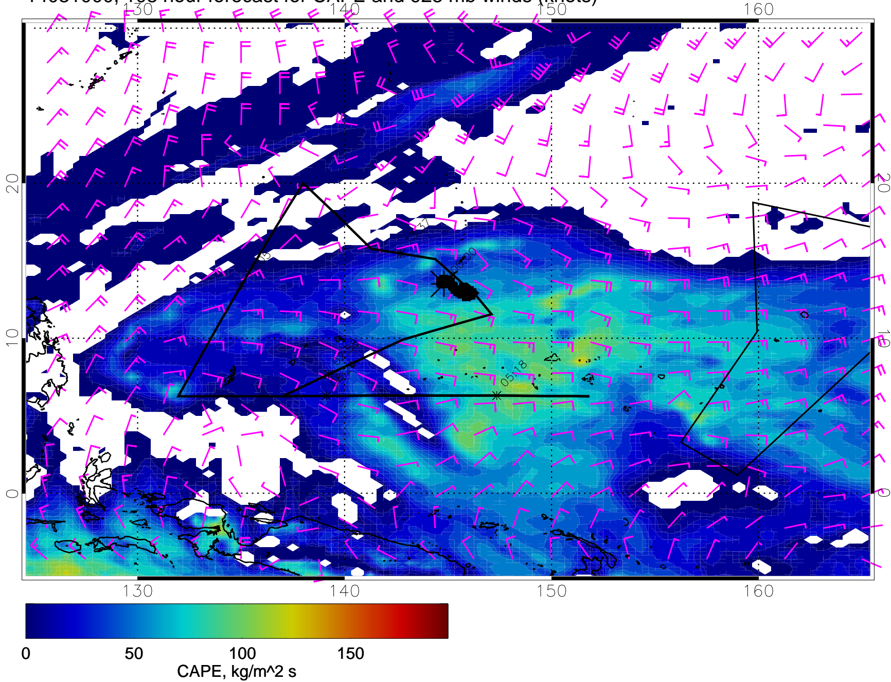
14031000, 108 hour forecast for CAPE and 925 mb winds (knots)
