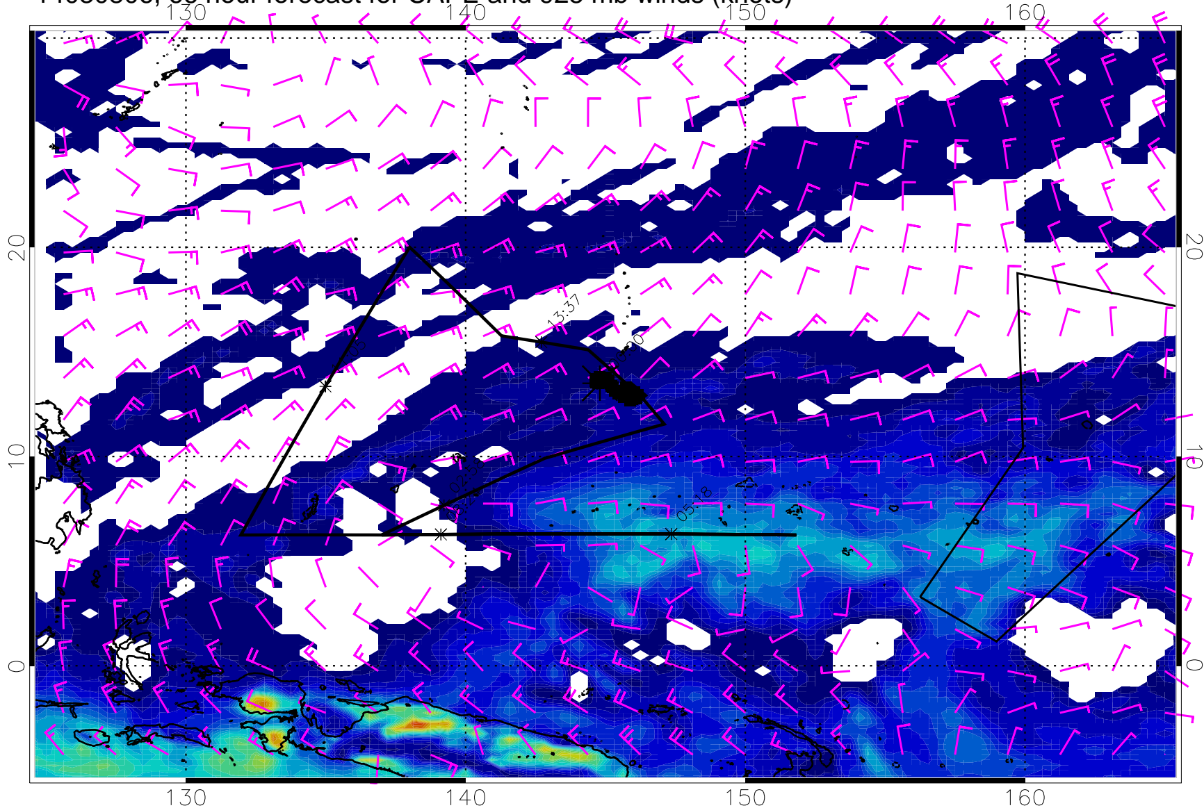
14030806, 66 hour forecast for CAPE and 925 mb winds (knots)
