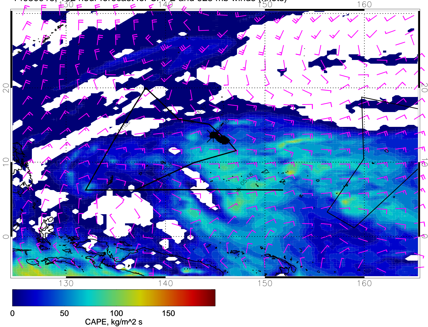
14030918, 102 hour forecast for CAPE and 925 mb winds (knots)
