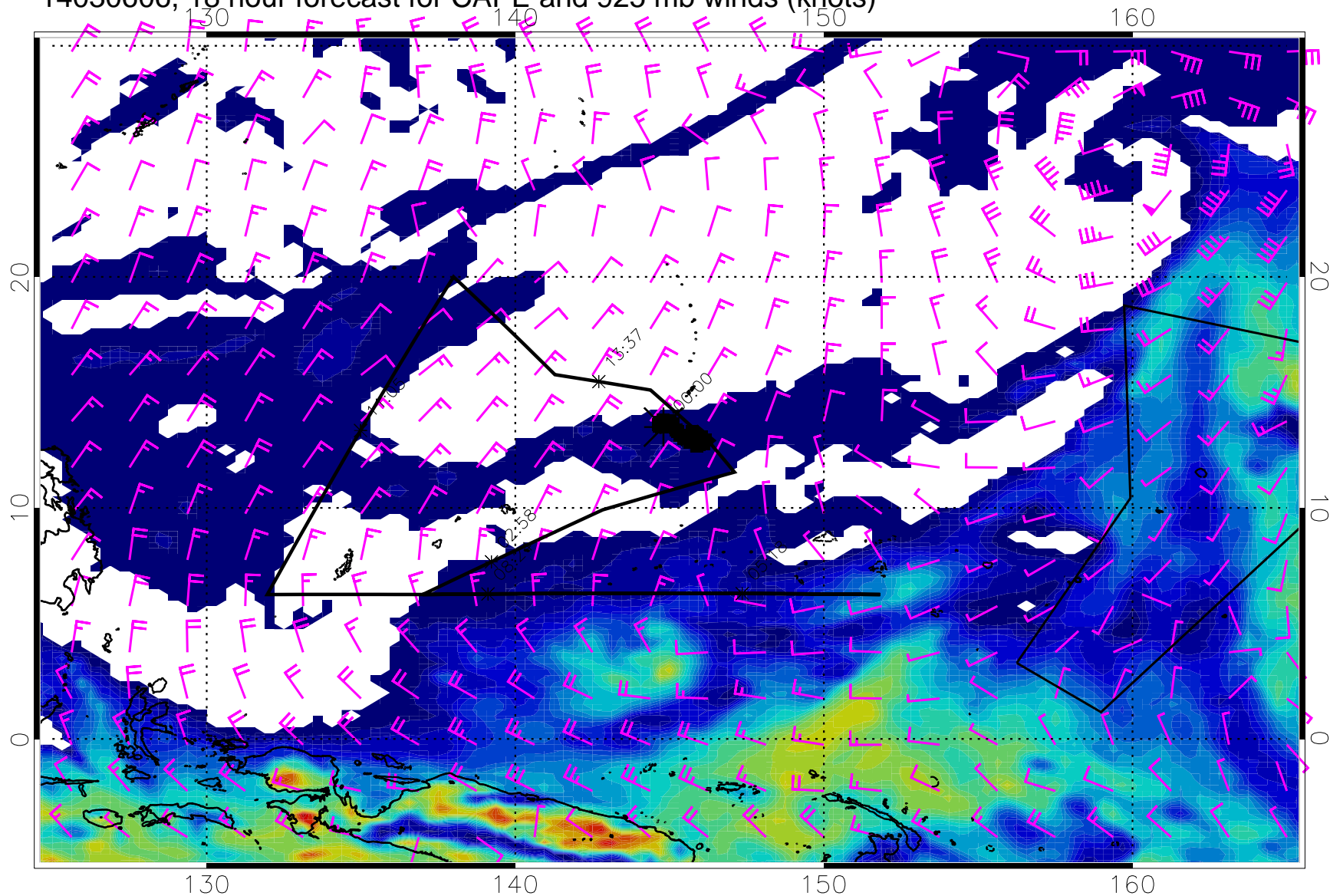
14030606, 18 hour forecast for CAPE and 925 mb winds (knots)
