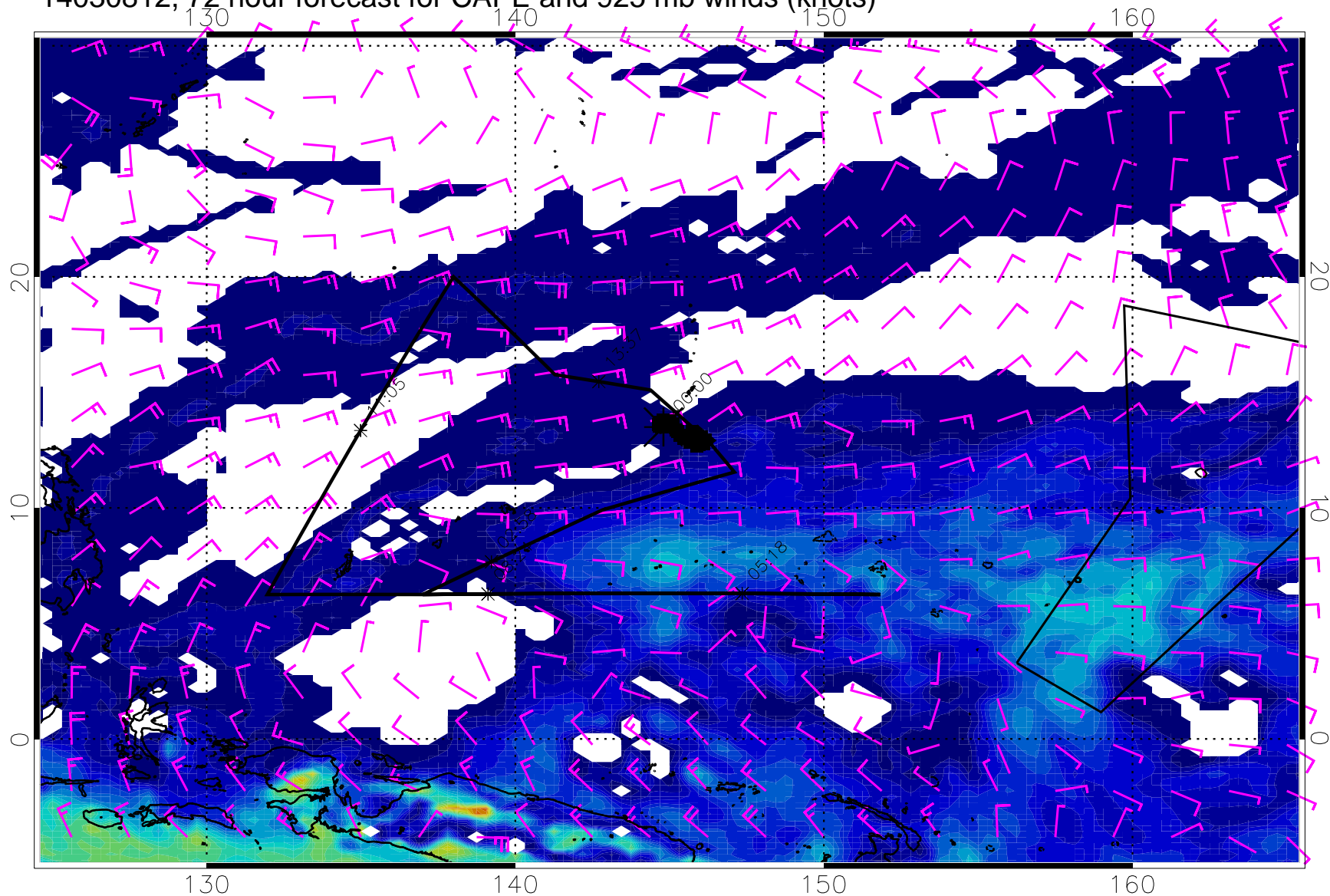
14030812, 72 hour forecast for CAPE and 925 mb winds (knots)
