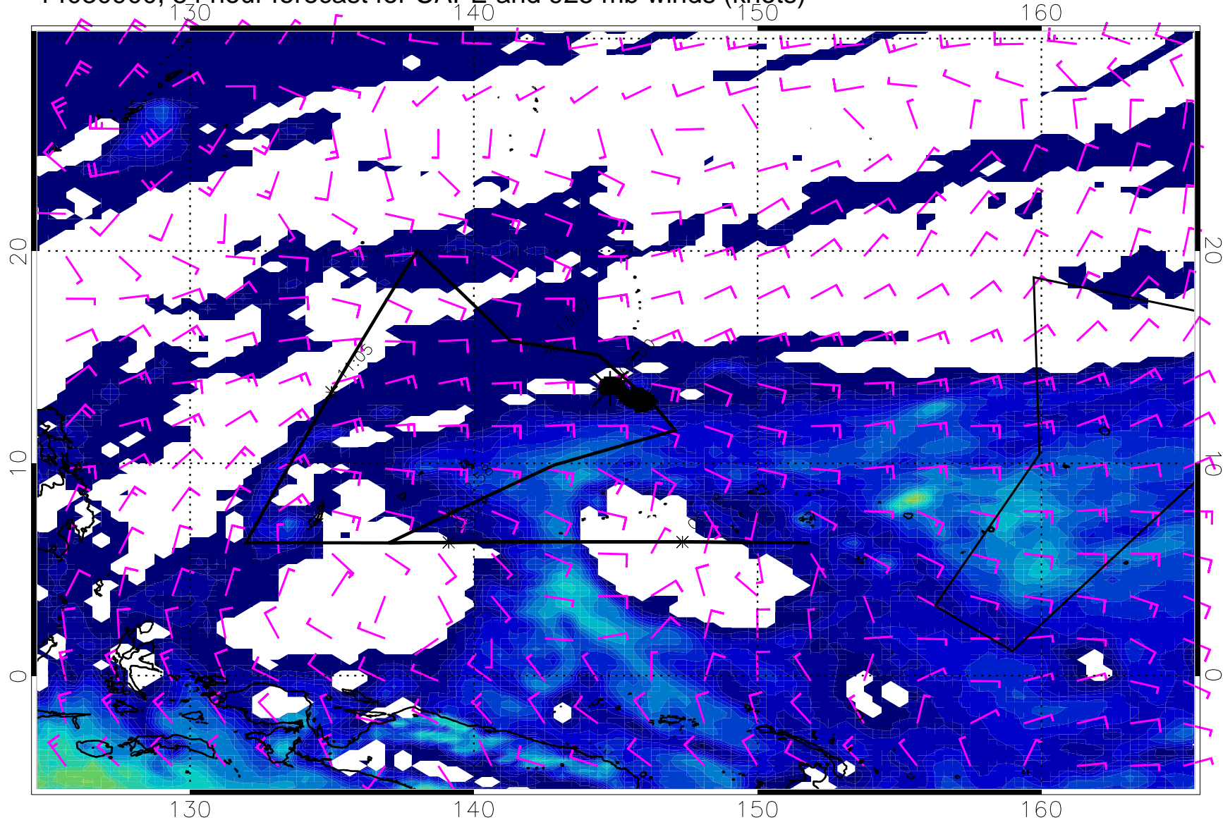
14030900, 84 hour forecast for CAPE and 925 mb winds (knots)
