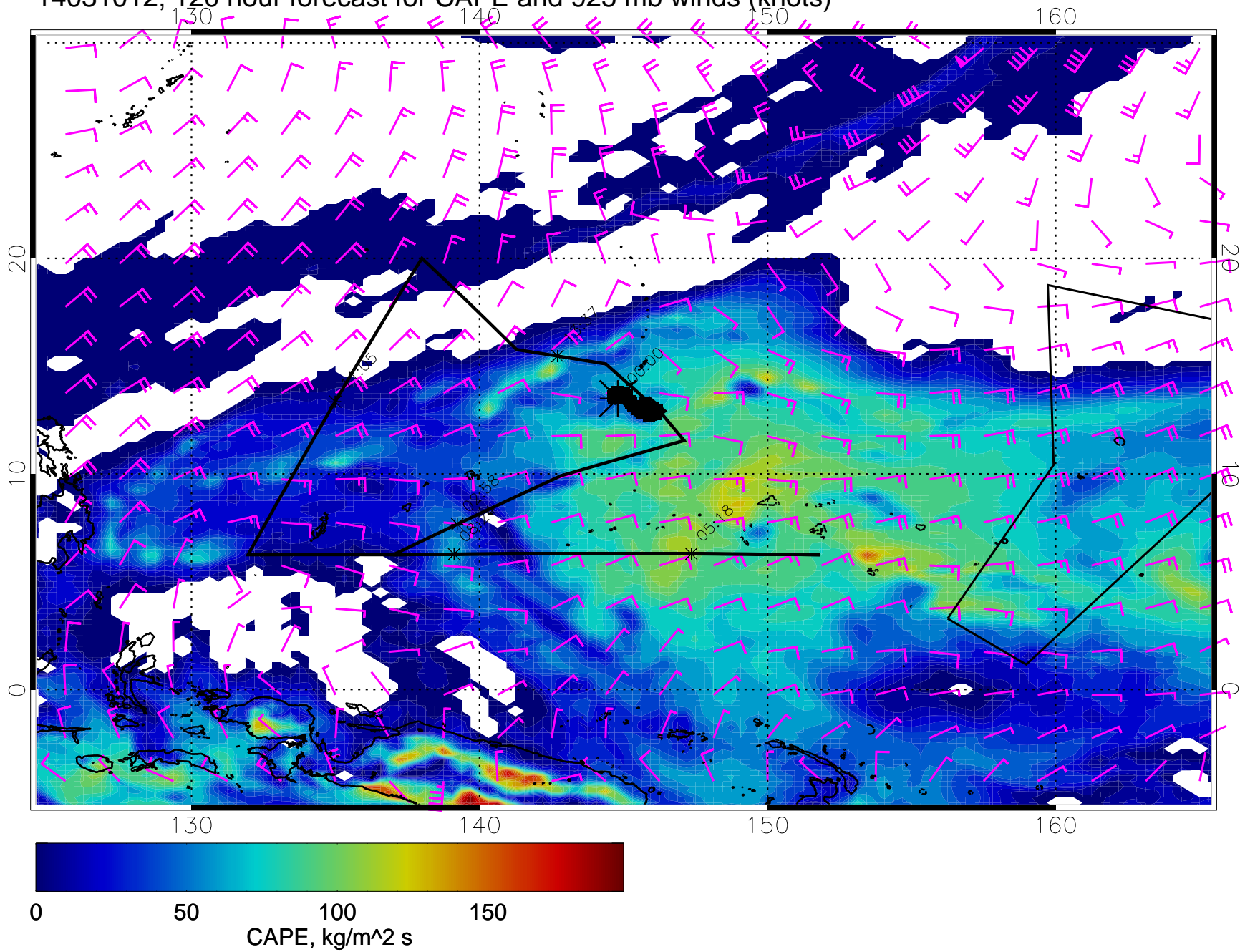
14031012, 120 hour forecast for CAPE and 925 mb winds (knots)
