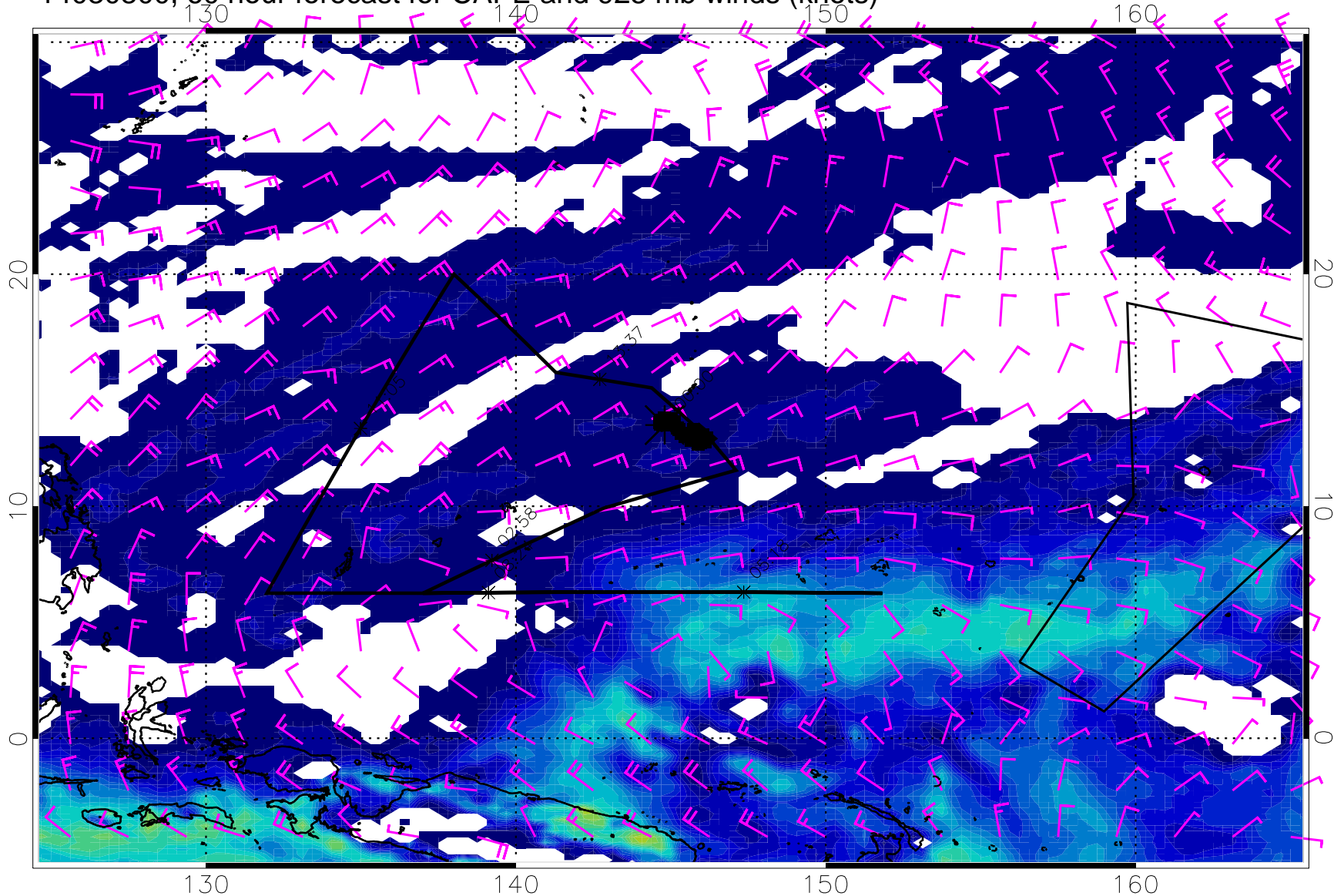
14030800, 60 hour forecast for CAPE and 925 mb winds (knots)
