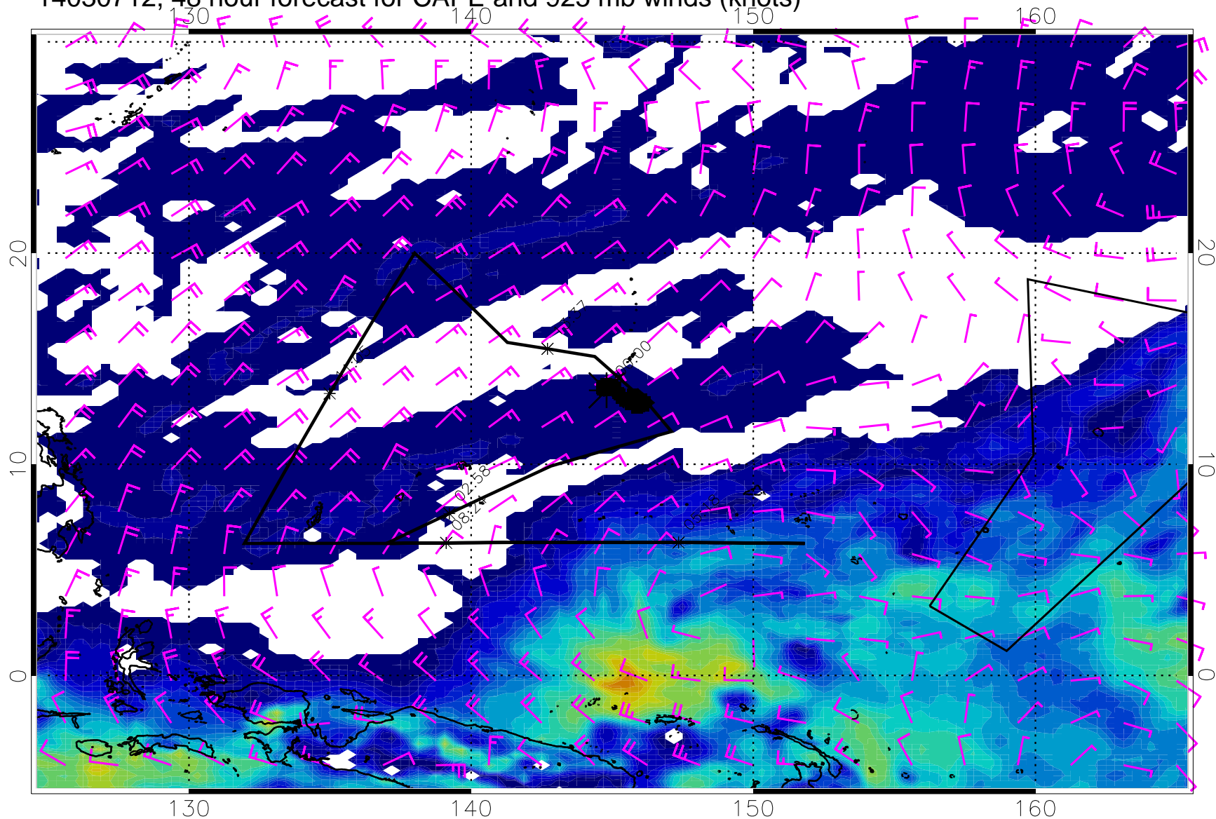
14030712, 48 hour forecast for CAPE and 925 mb winds (knots)
