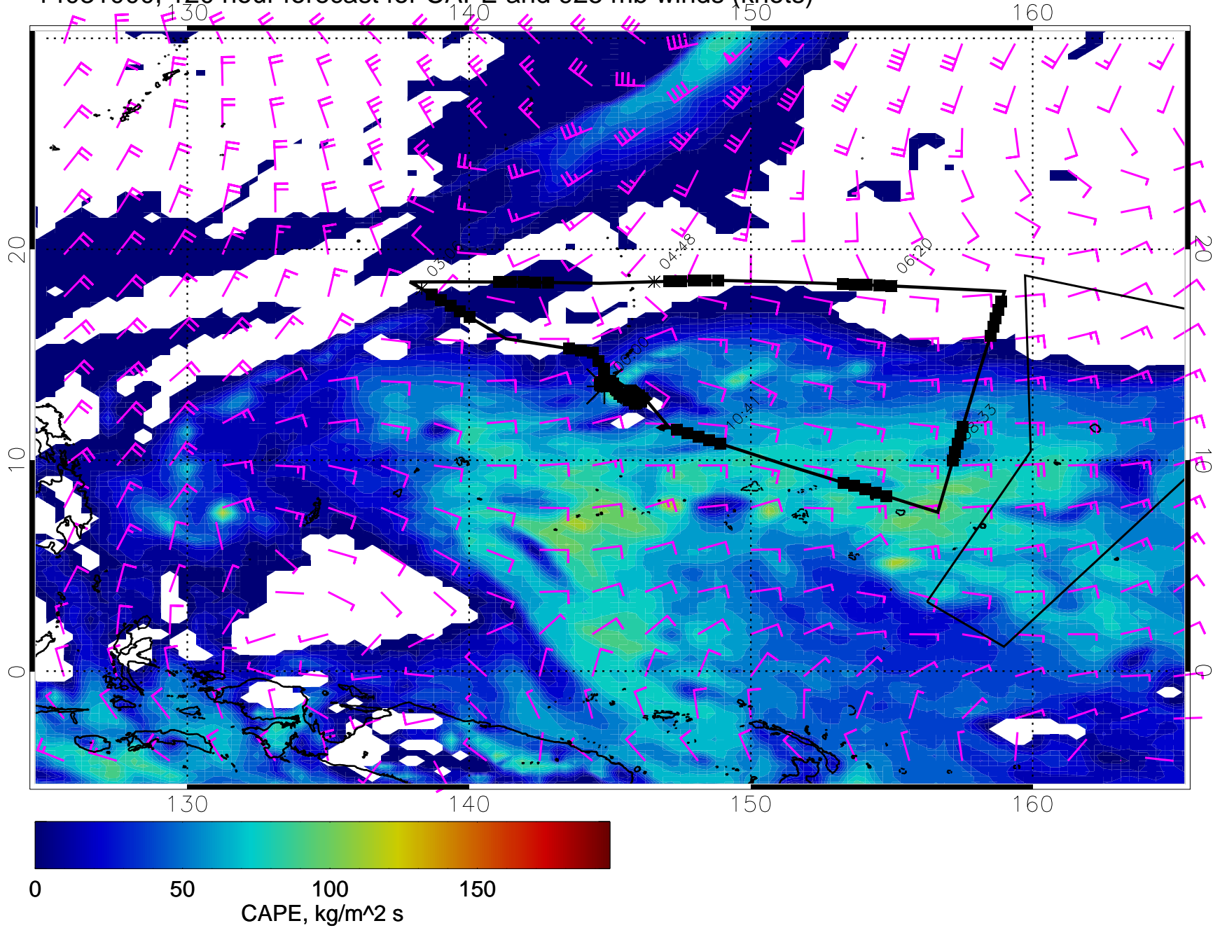
14031000, 120 hour forecast for CAPE and 925 mb winds (knots)
