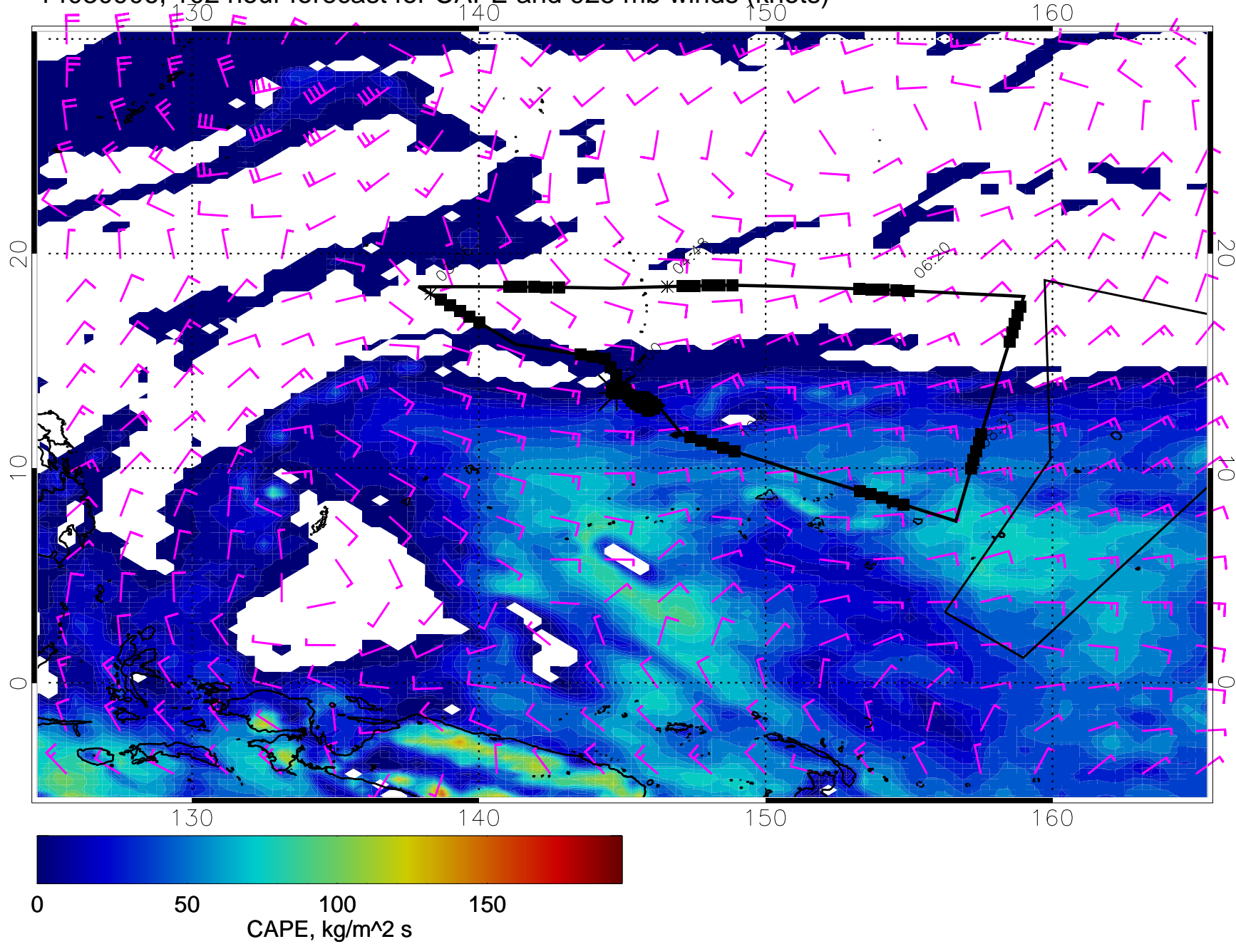
14030906, 102 hour forecast for CAPE and 925 mb winds (knots)
