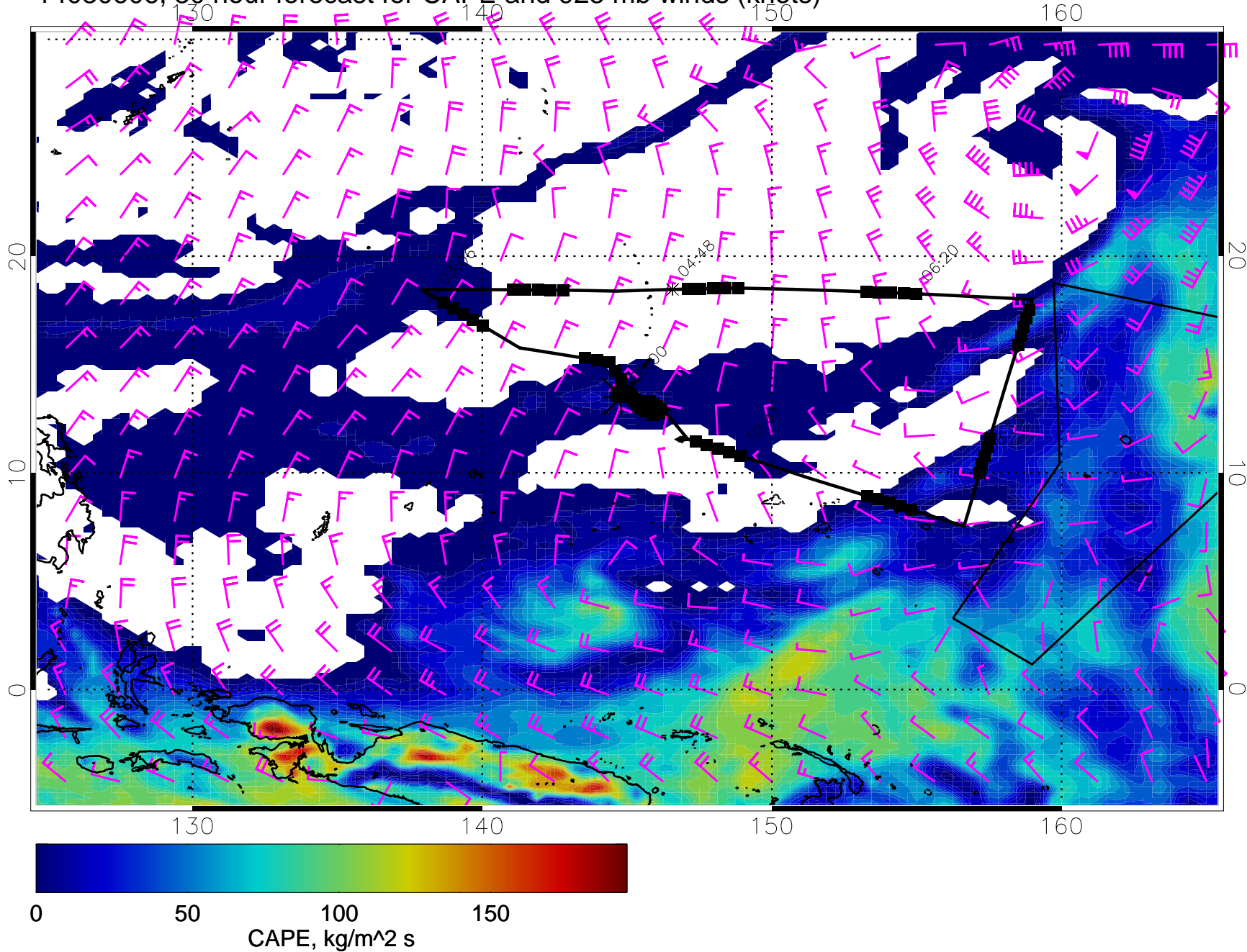
14030606, 30 hour forecast for CAPE and 925 mb winds (knots)
