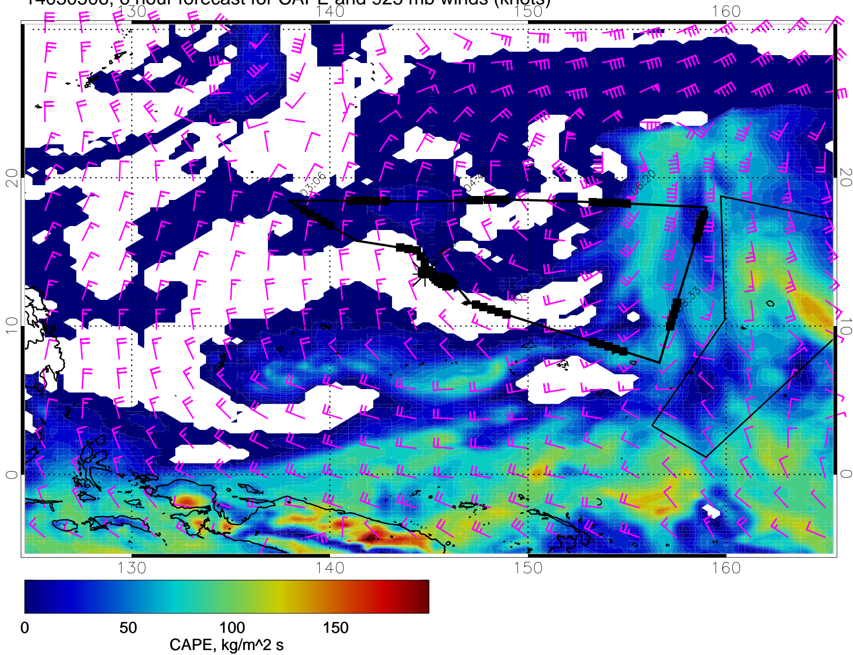
14030506, 6 hour forecast for CAPE and 925 mb winds (knots)
