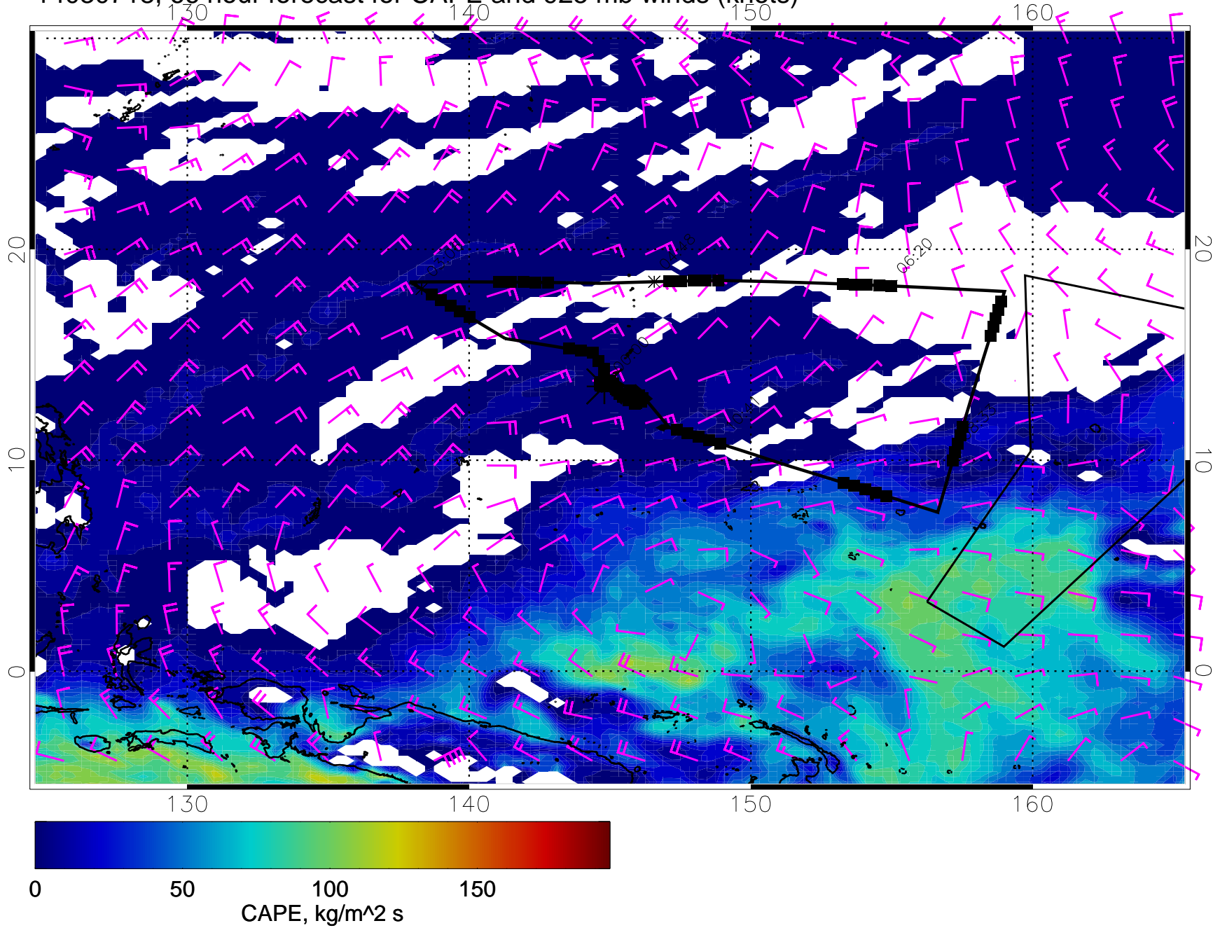
14030718, 66 hour forecast for CAPE and 925 mb winds (knots)
