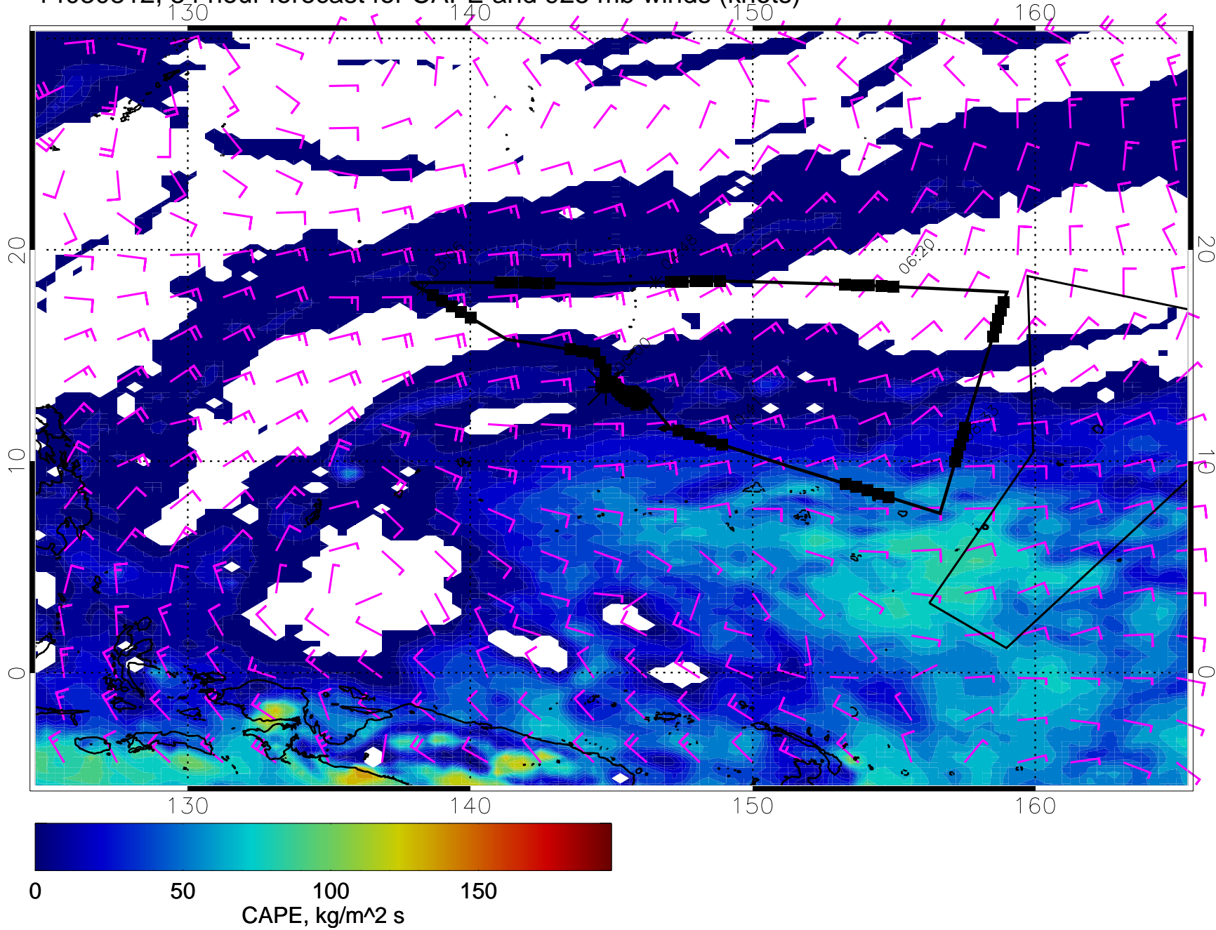
14030812, 84 hour forecast for CAPE and 925 mb winds (knots)
