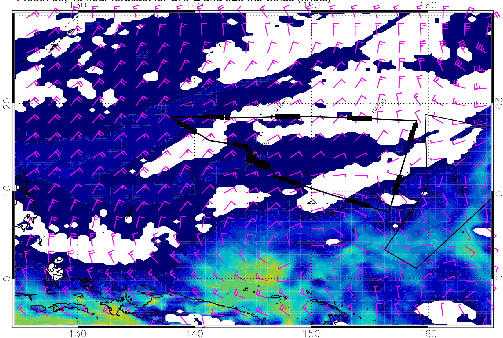
14030700, 48 hour forecast for CAPE and 925 mb winds (knots)
