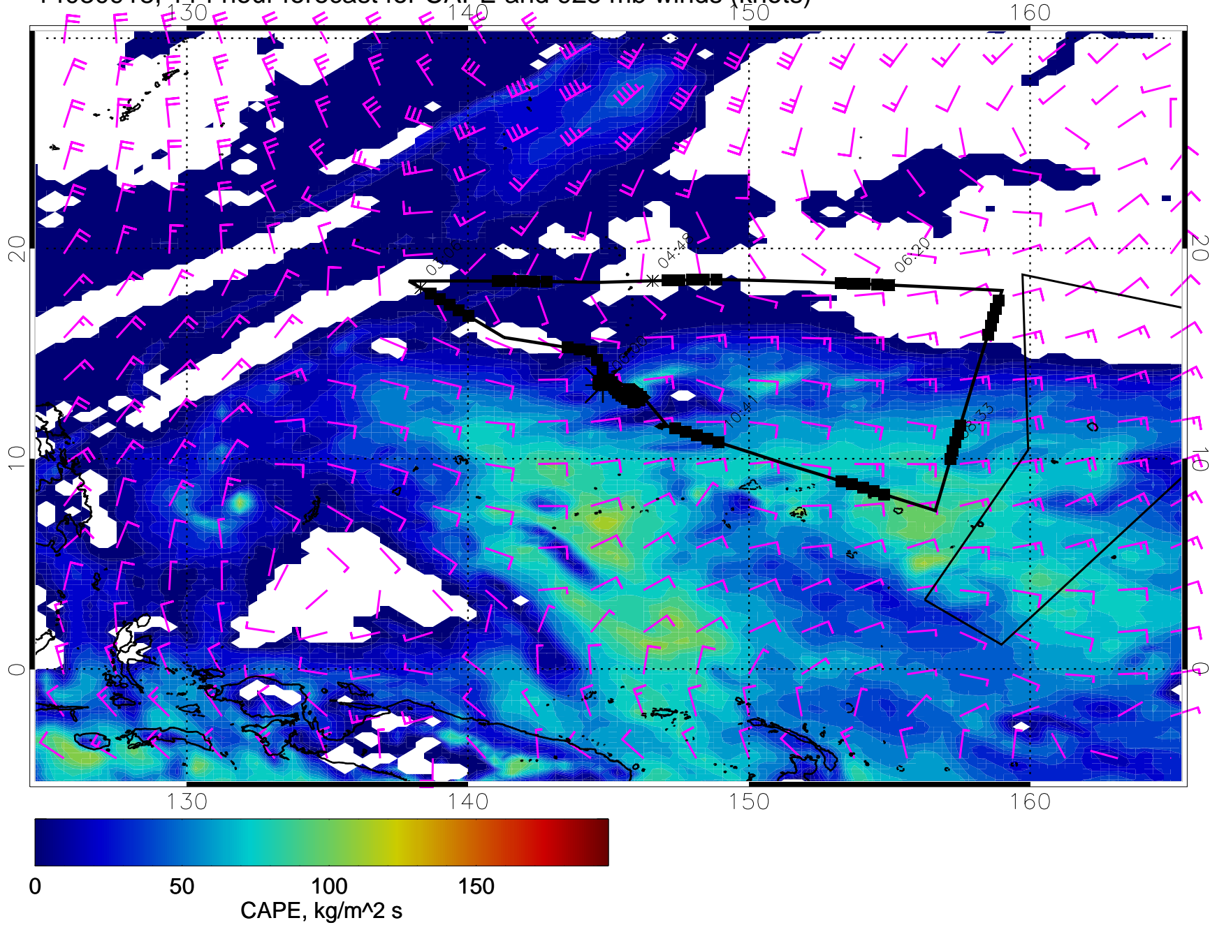
14030918, 114 hour forecast for CAPE and 925 mb winds (knots)
