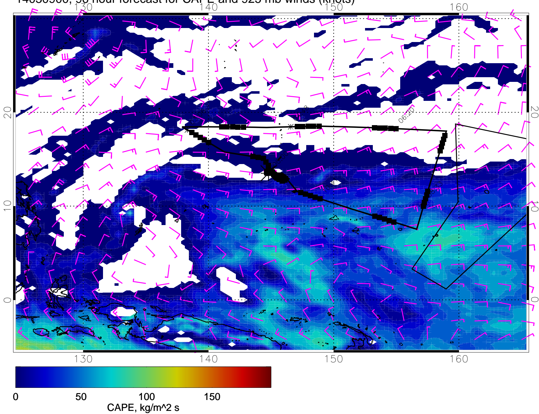
14030900, 96 hour forecast for CAPE and 925 mb winds (knots)
