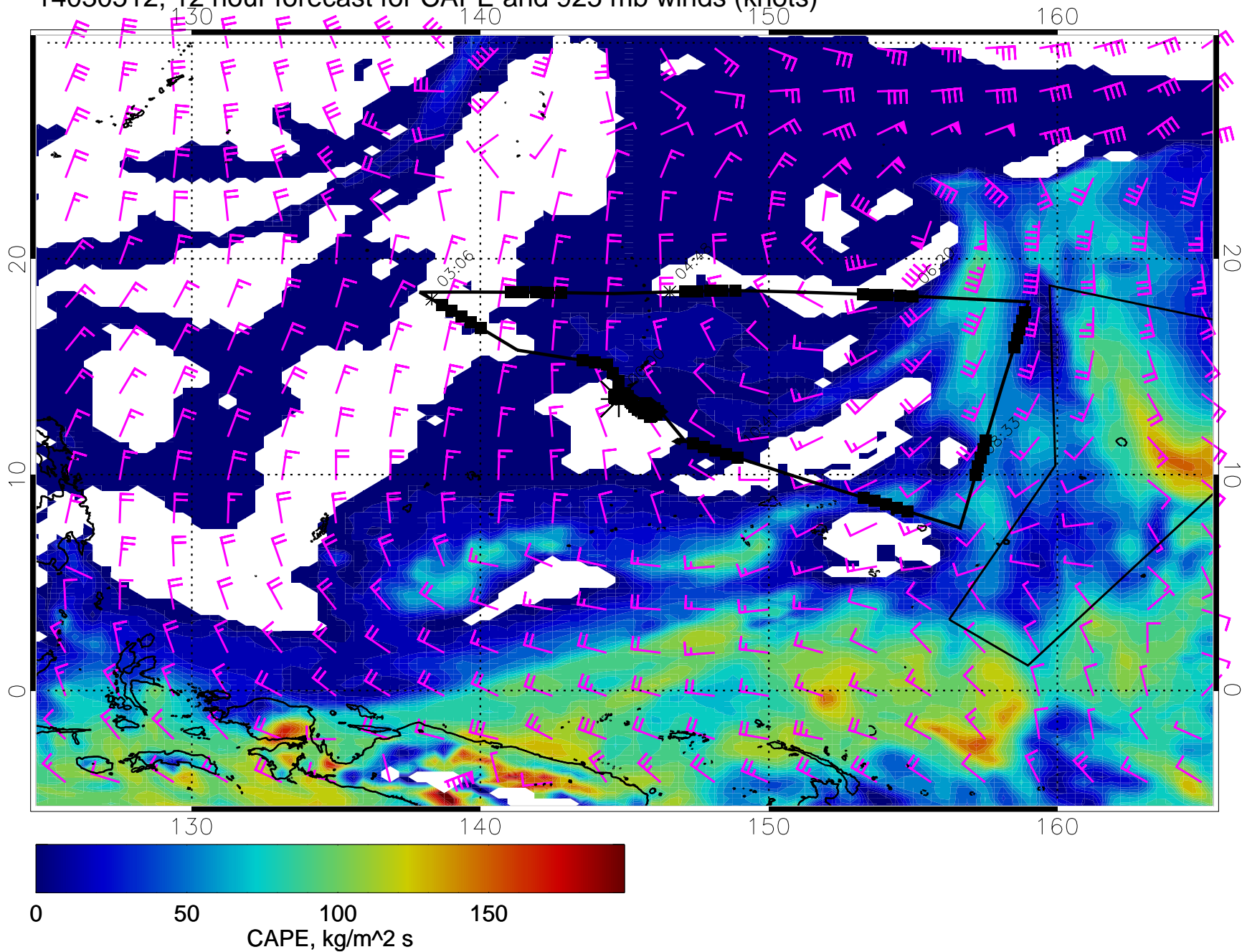
14030512, 12 hour forecast for CAPE and 925 mb winds (knots)
