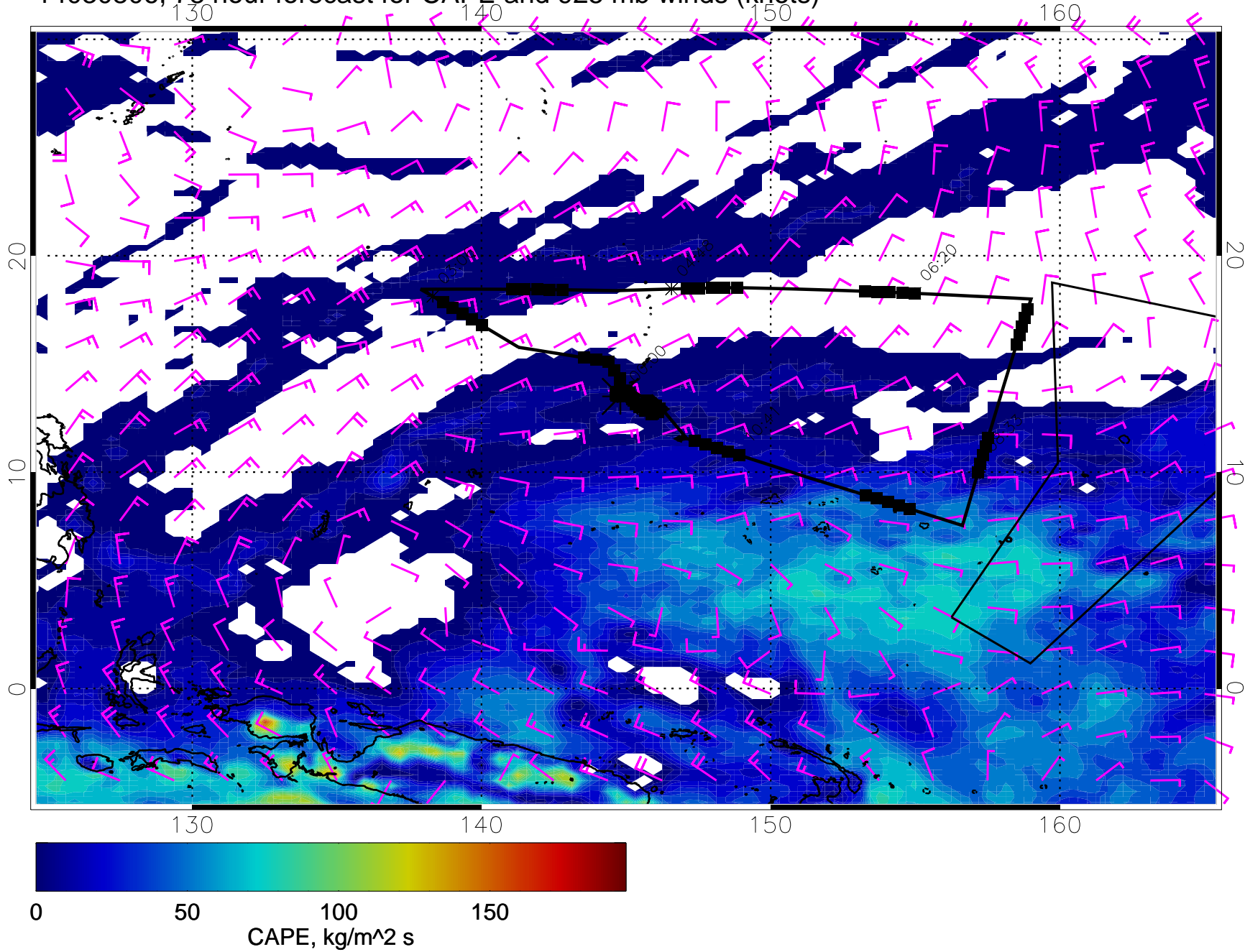
14030806, 78 hour forecast for CAPE and 925 mb winds (knots)
