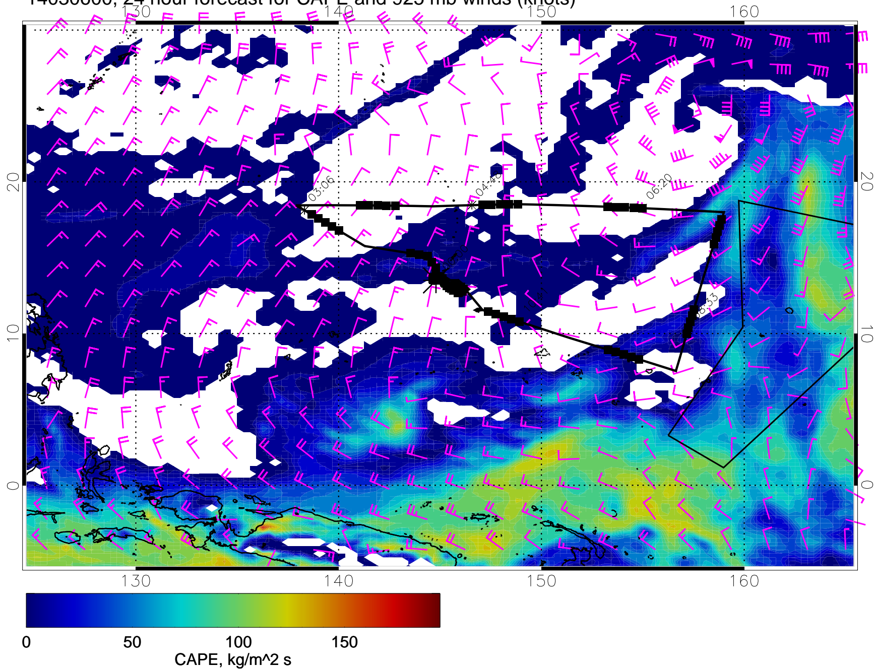
14030600, 24 hour forecast for CAPE and 925 mb winds (knots)
