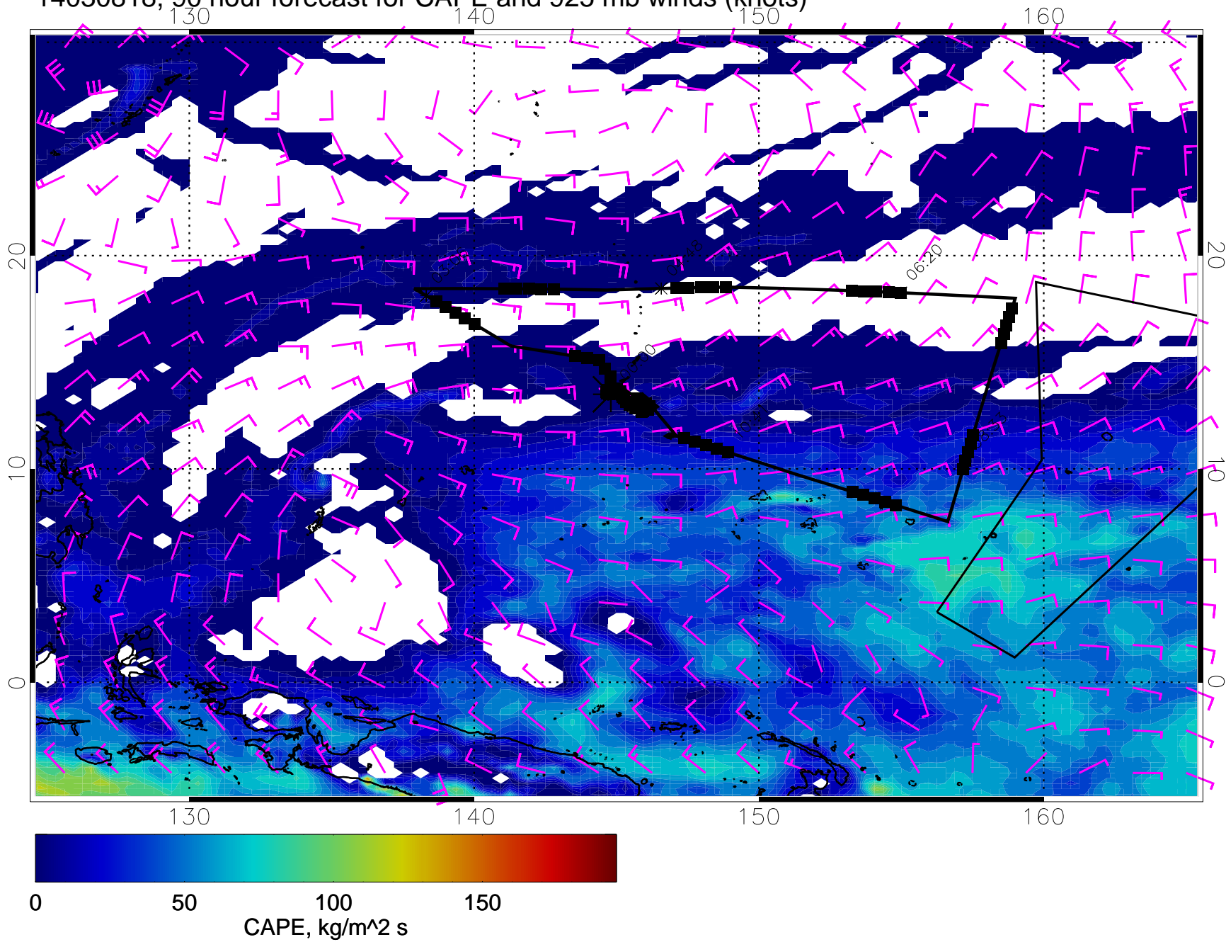
14030818, 90 hour forecast for CAPE and 925 mb winds (knots)
