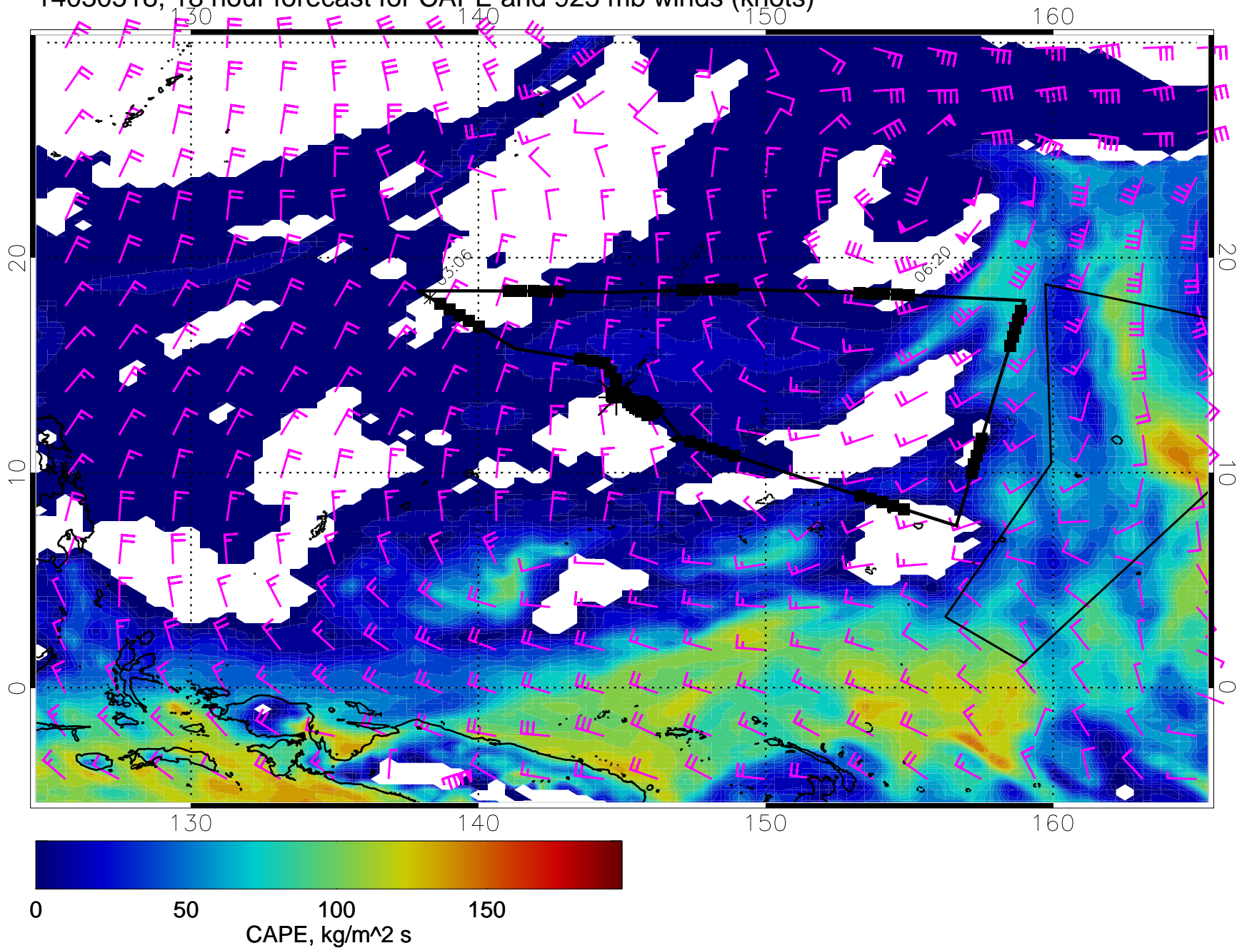
14030518, 18 hour forecast for CAPE and 925 mb winds (knots)
