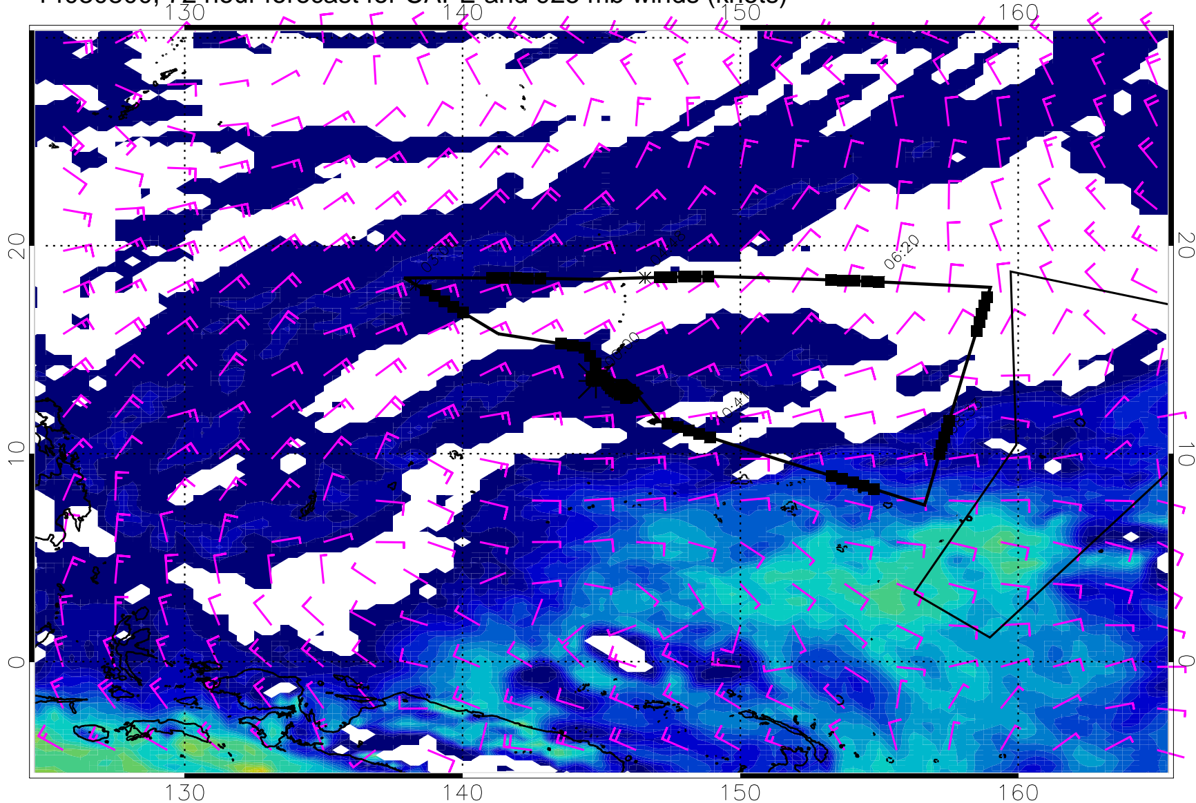
14030800, 72 hour forecast for CAPE and 925 mb winds (knots)
