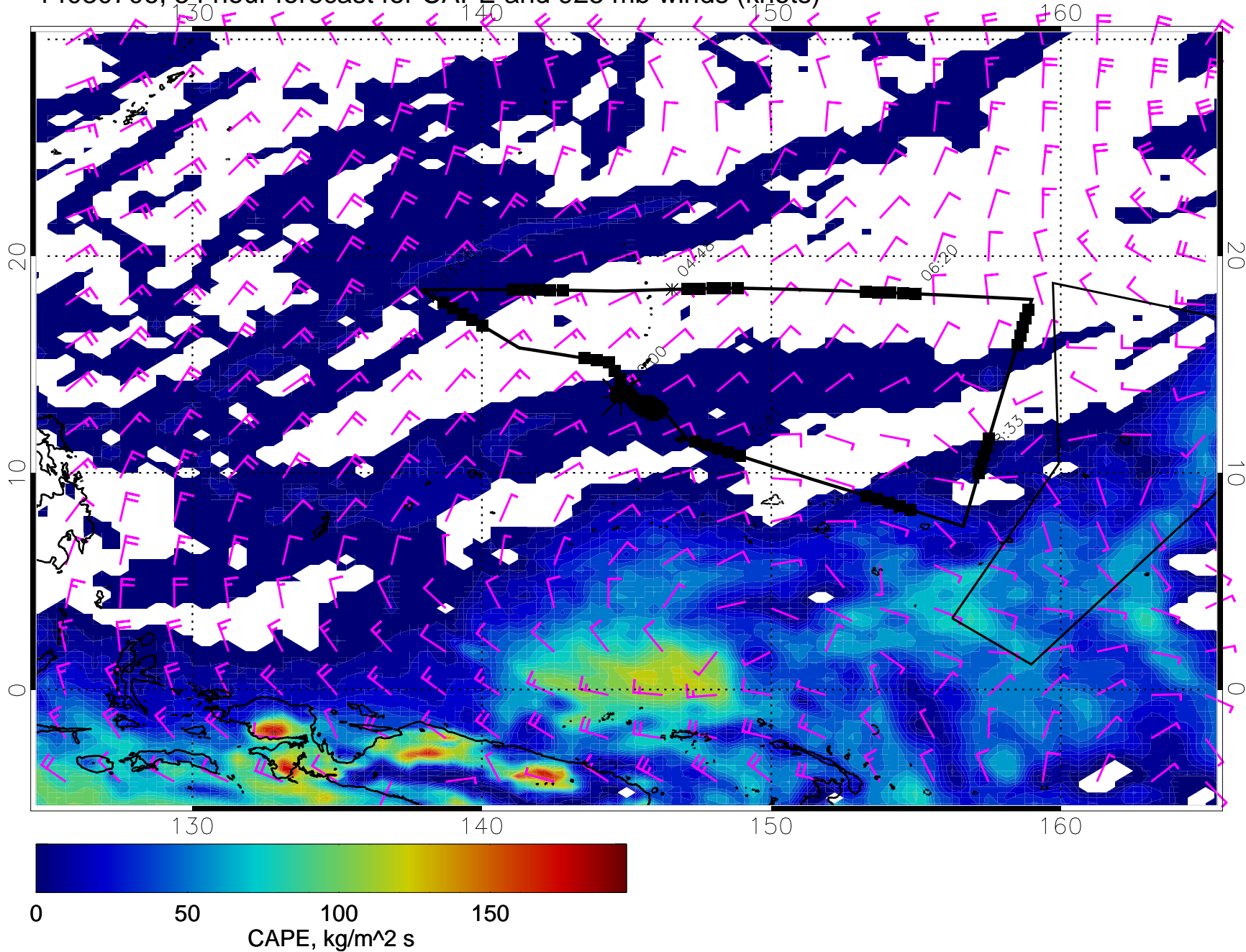
14030706, 54 hour forecast for CAPE and 925 mb winds (knots)
