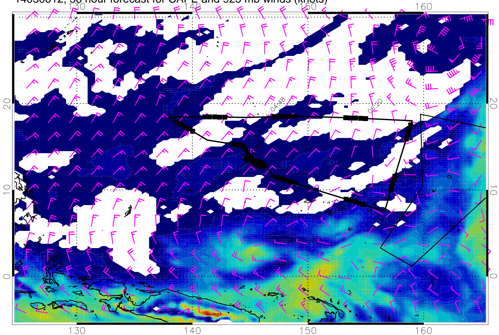
14030612, 36 hour forecast for CAPE and 925 mb winds (knots)
