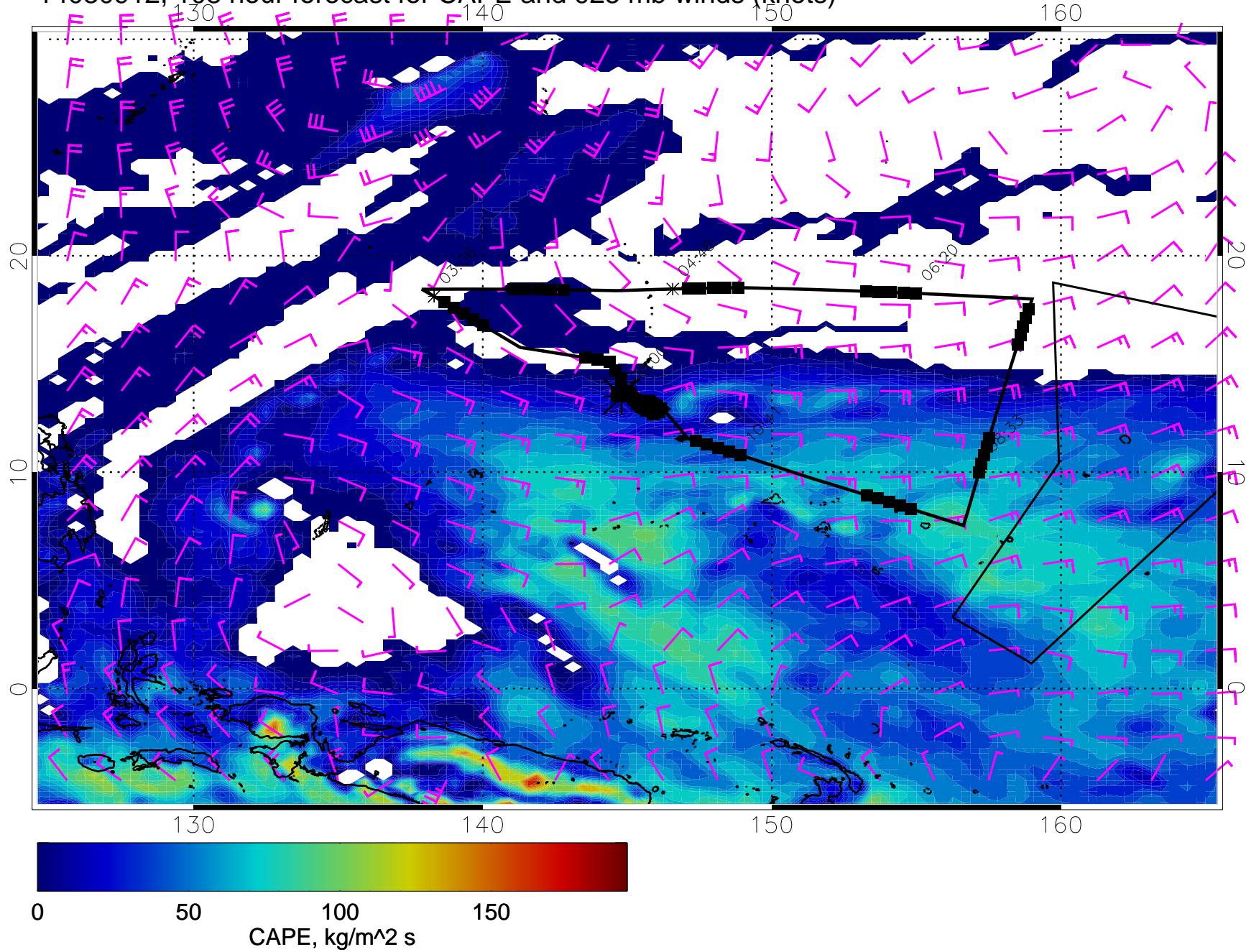
14030912, 108 hour forecast for CAPE and 925 mb winds (knots)
