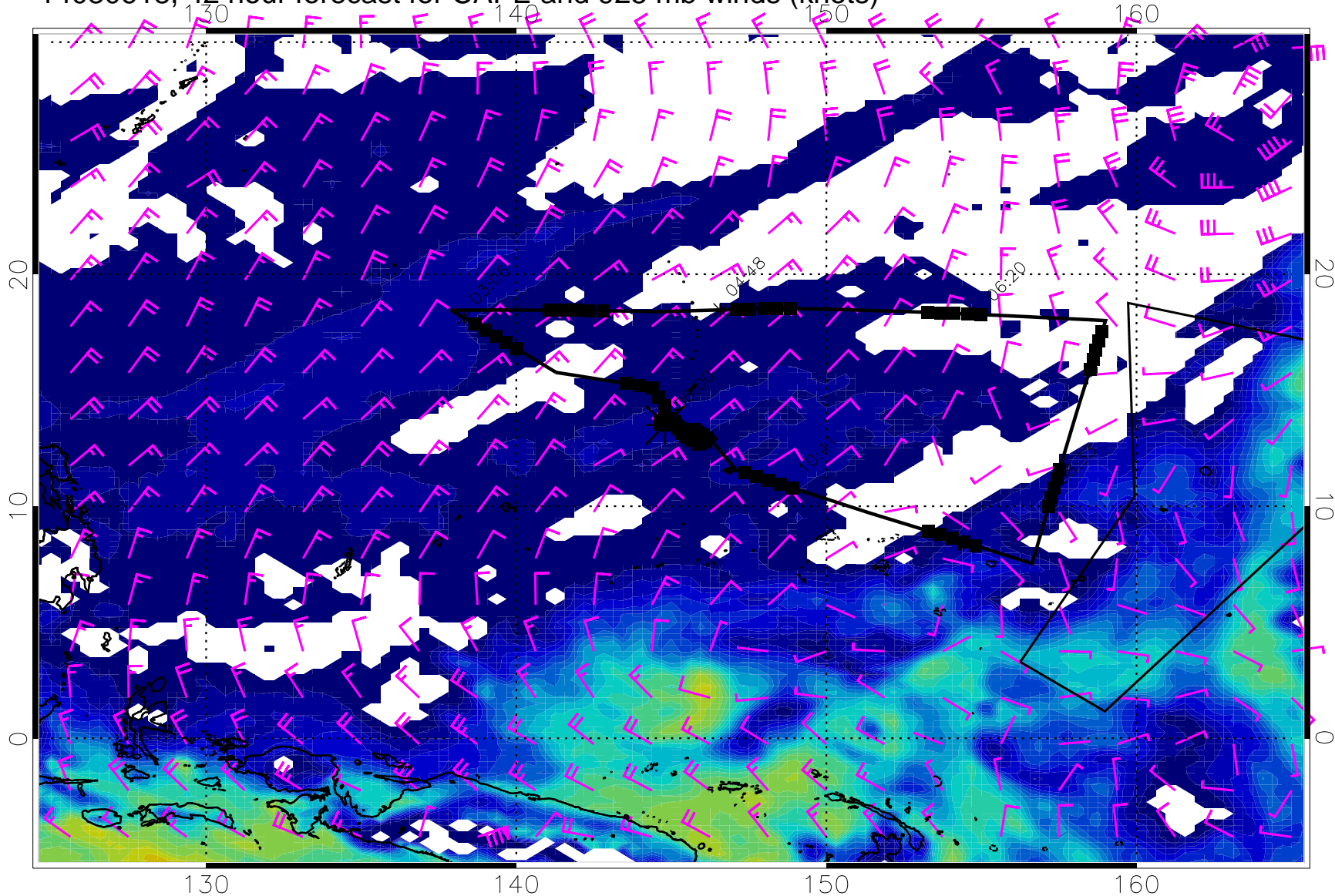
14030618, 42 hour forecast for CAPE and 925 mb winds (knots)
