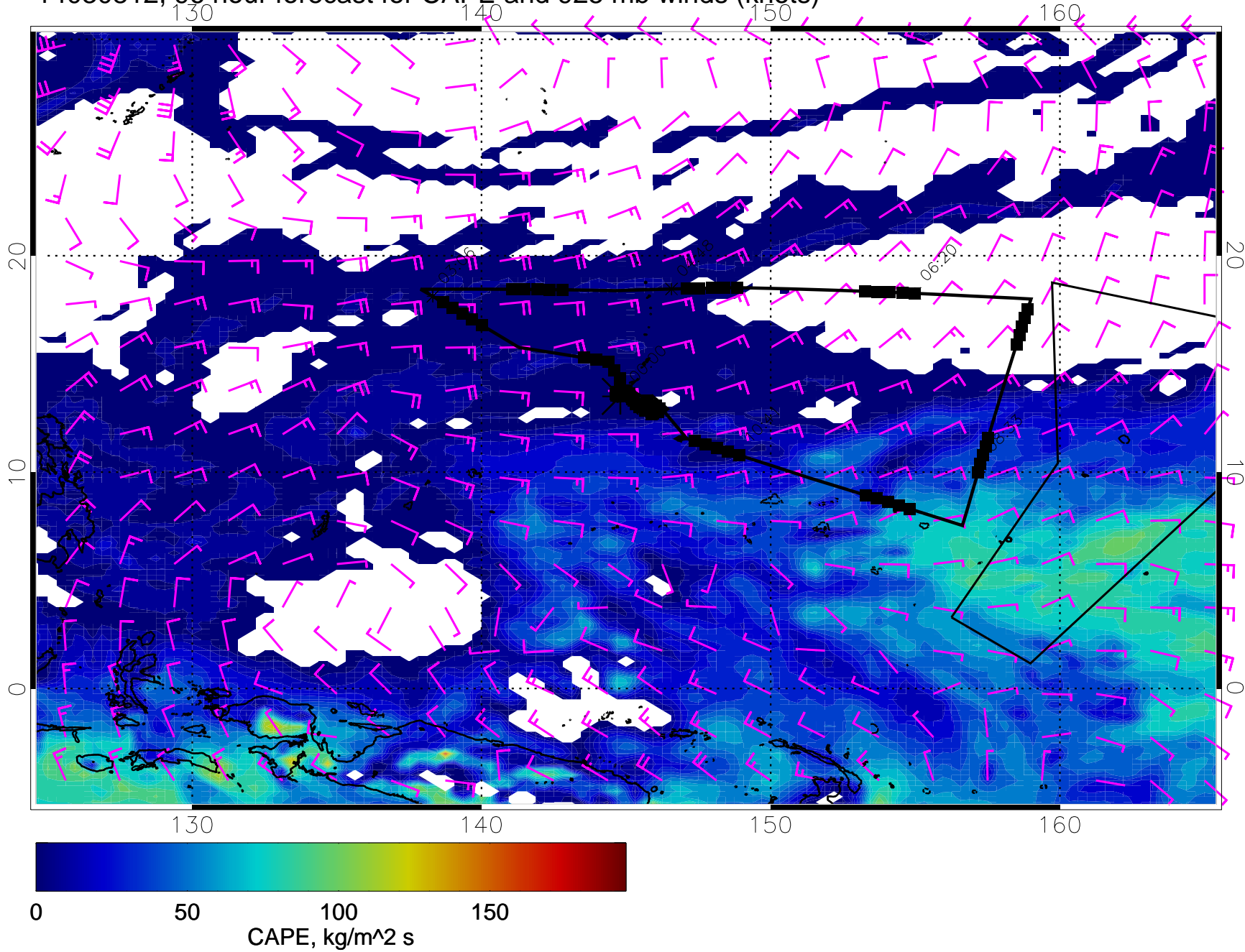
14030812, 96 hour forecast for CAPE and 925 mb winds (knots)
