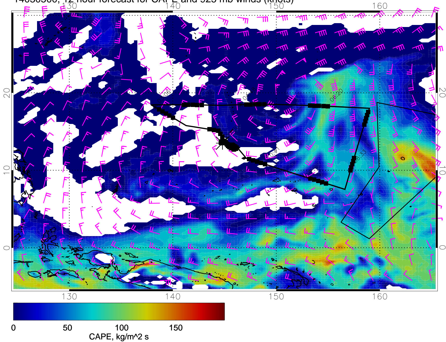
14030500, 12 hour forecast for CAPE and 925 mb winds (knots)
