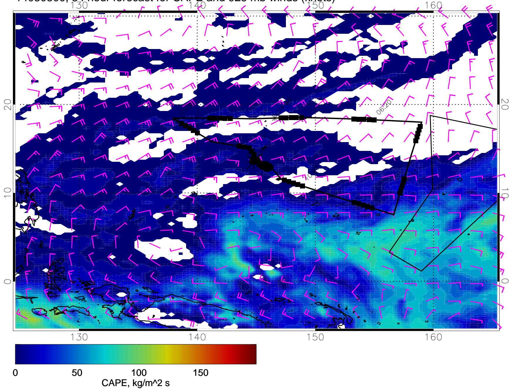
14030800, 84 hour forecast for CAPE and 925 mb winds (knots)
