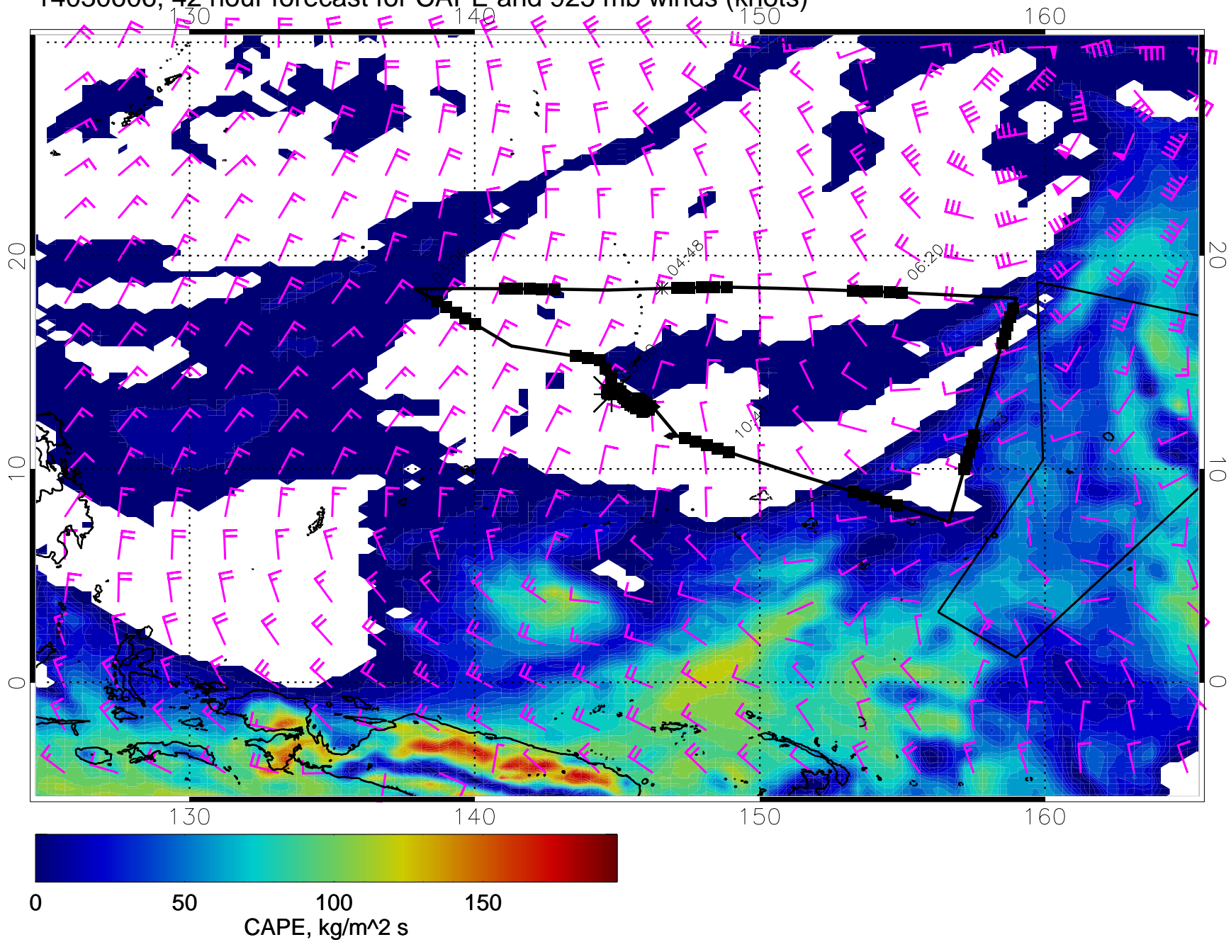
14030606, 42 hour forecast for CAPE and 925 mb winds (knots)
