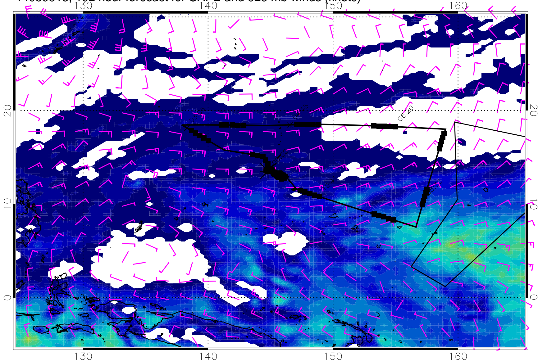
14030818, 102 hour forecast for CAPE and 925 mb winds (knots)
