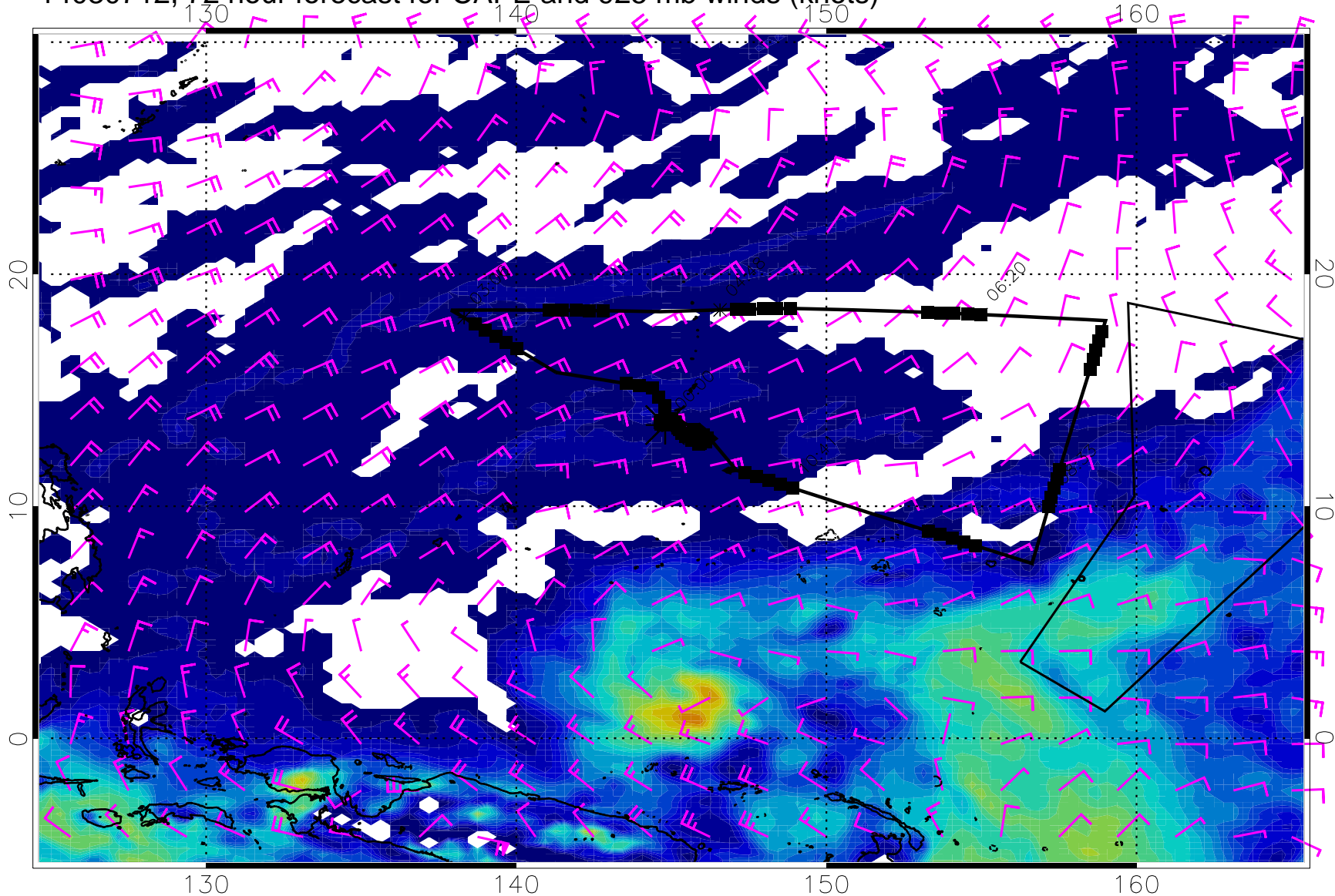
14030712, 72 hour forecast for CAPE and 925 mb winds (knots)
