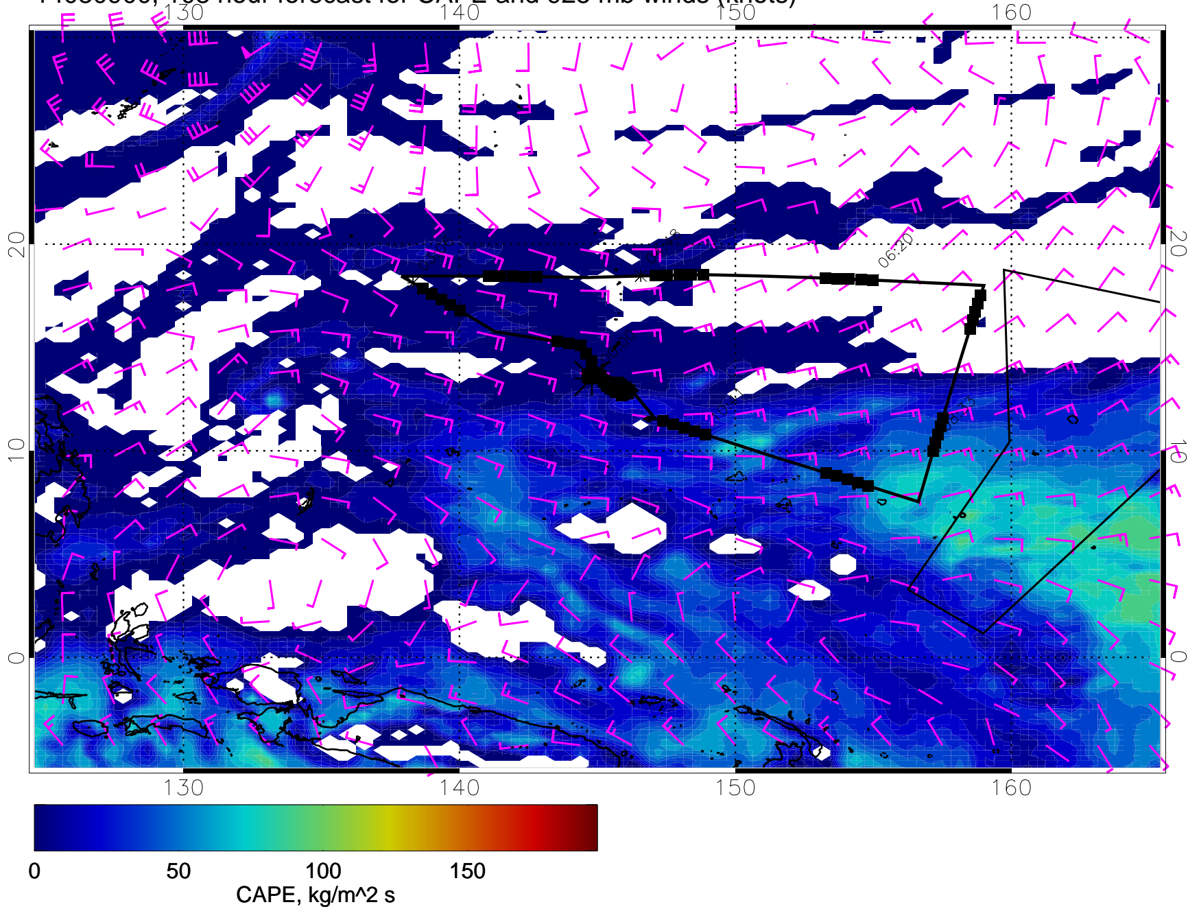
14030900, 108 hour forecast for CAPE and 925 mb winds (knots)
