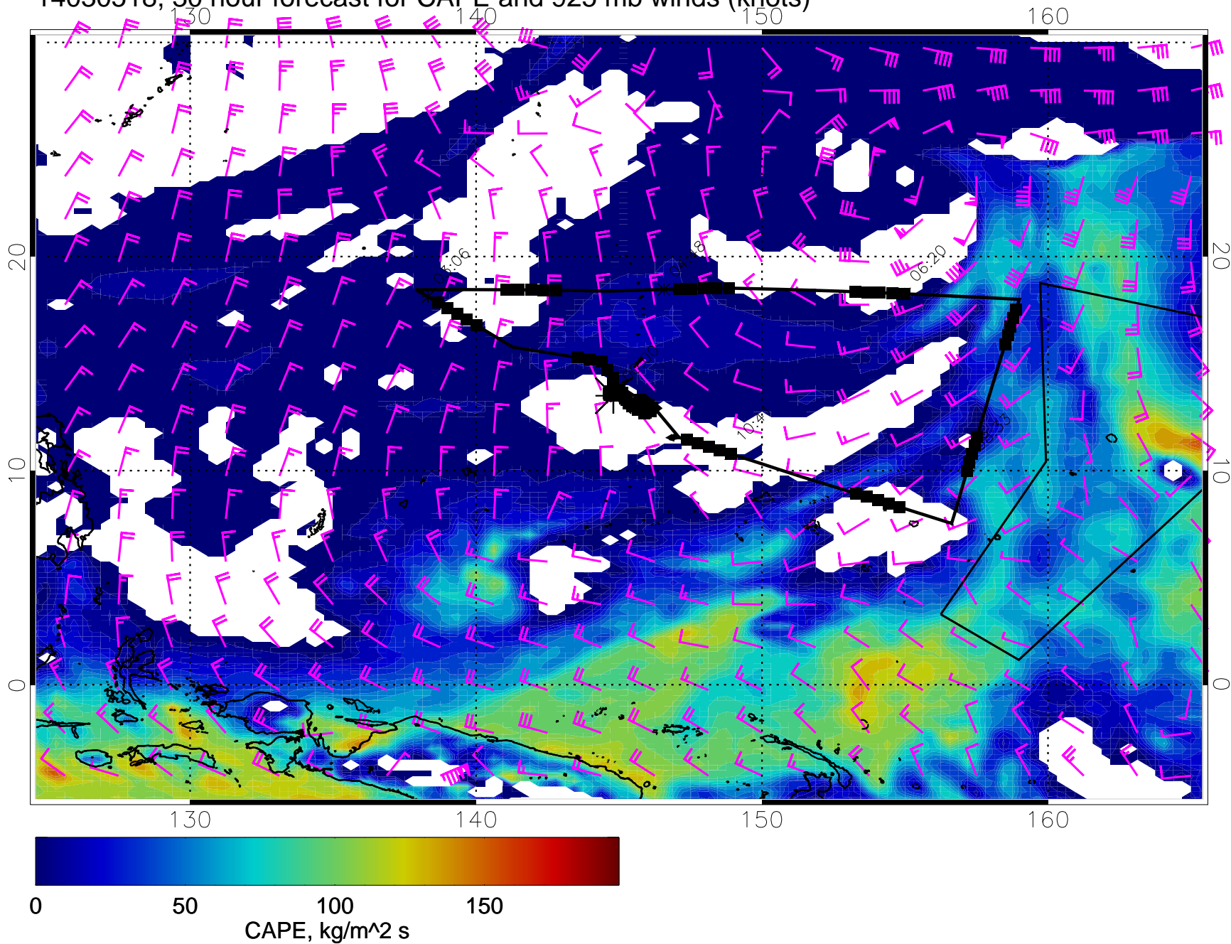
14030518, 30 hour forecast for CAPE and 925 mb winds (knots)
