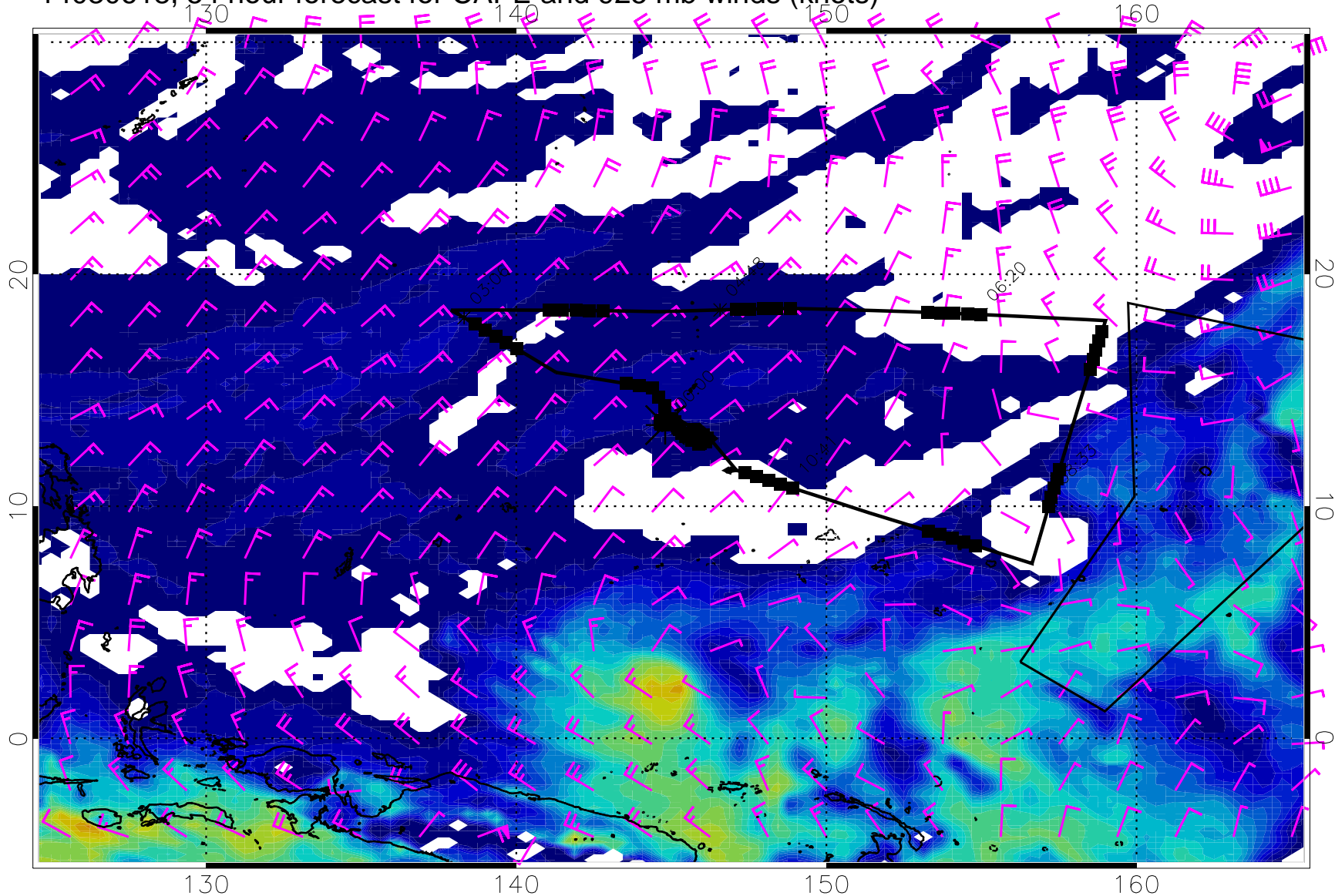
14030618, 54 hour forecast for CAPE and 925 mb winds (knots)
