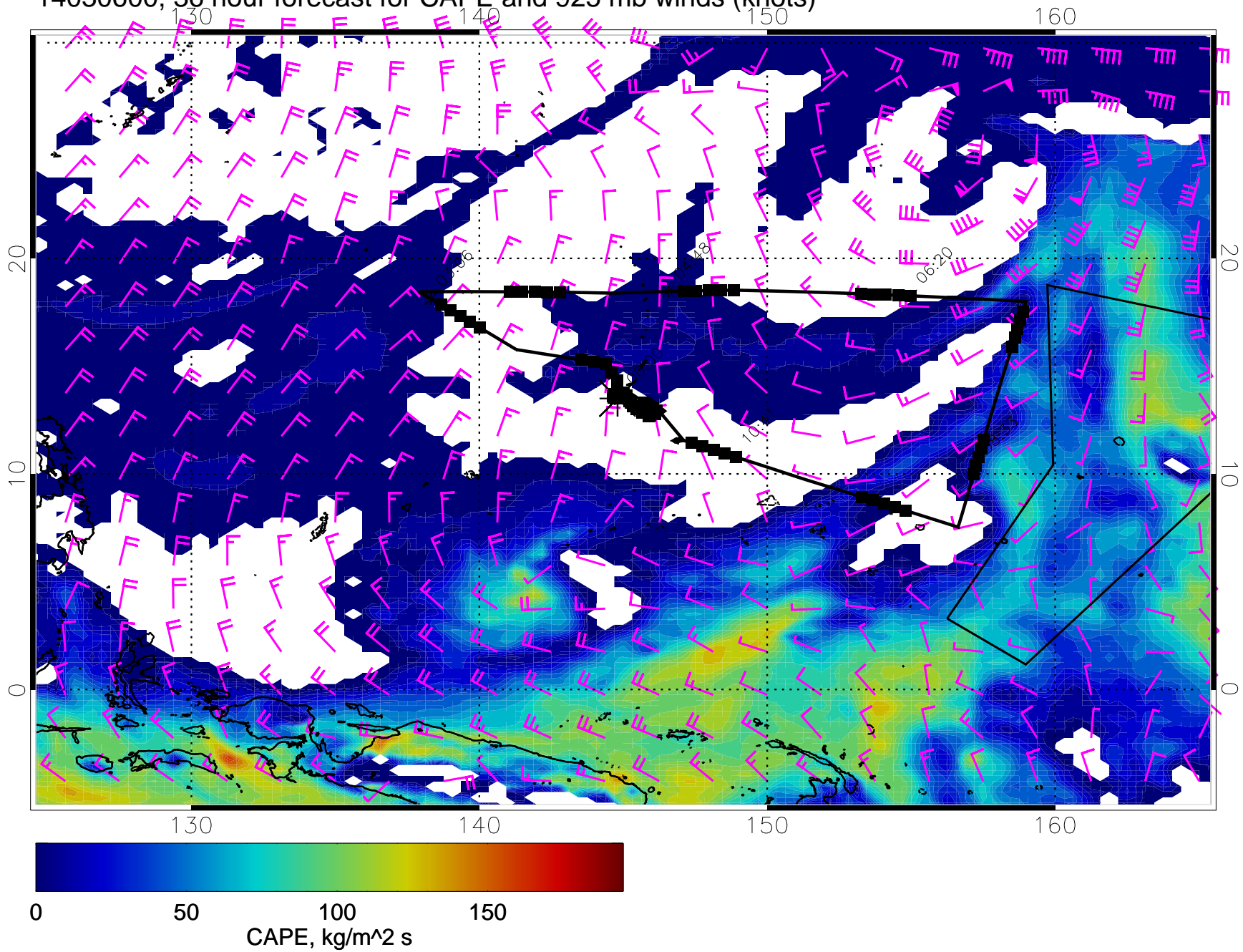
14030600, 36 hour forecast for CAPE and 925 mb winds (knots)
