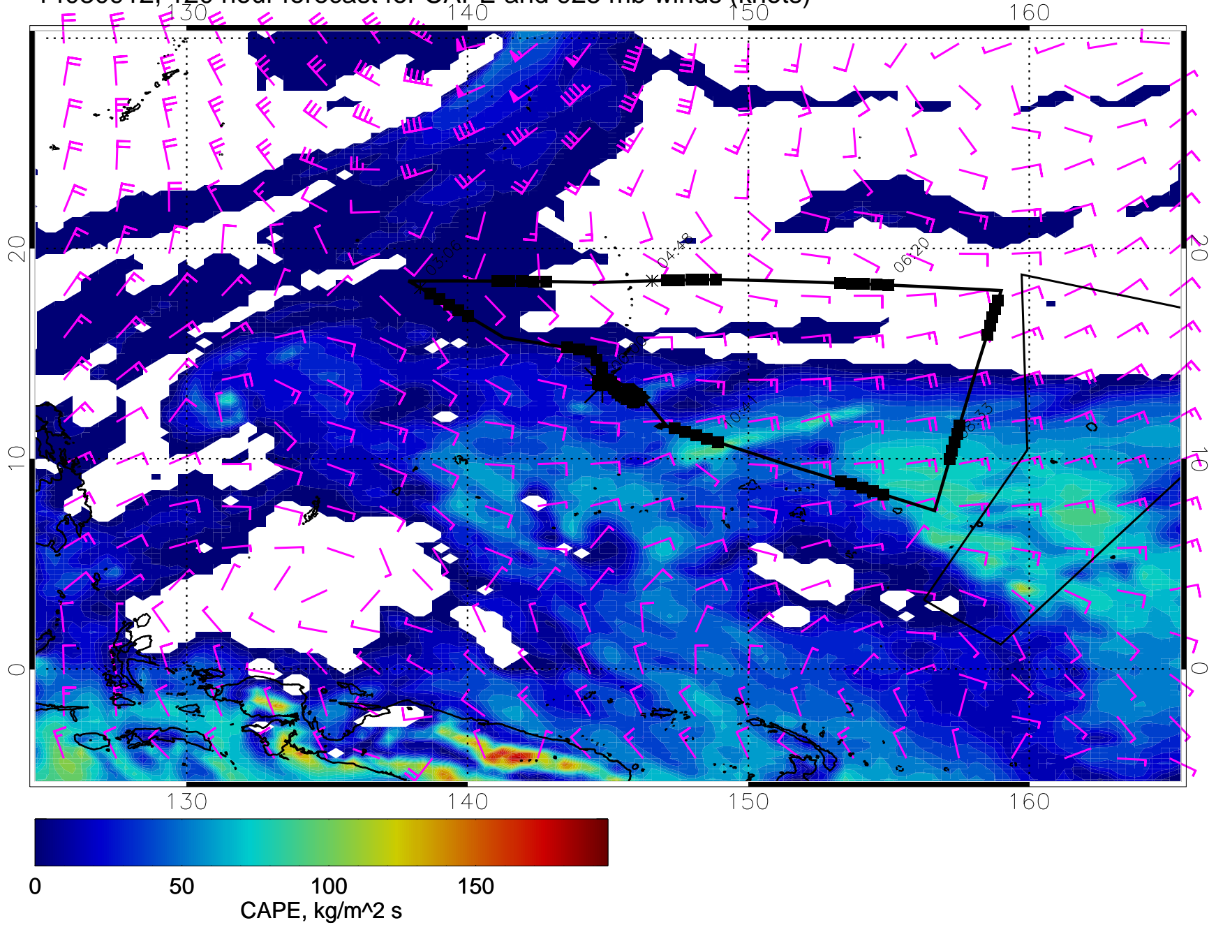
14030912, 120 hour forecast for CAPE and 925 mb winds (knots)
