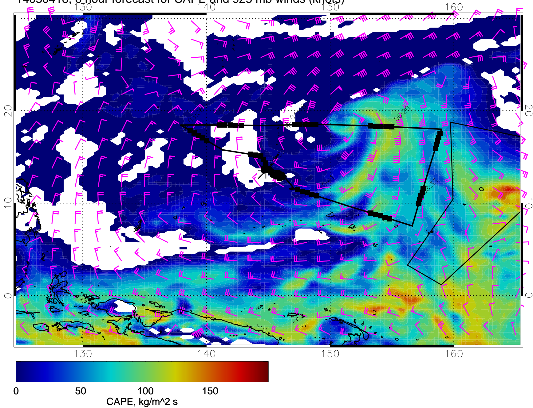
14030418, 6 hour forecast for CAPE and 925 mb winds (knots)
