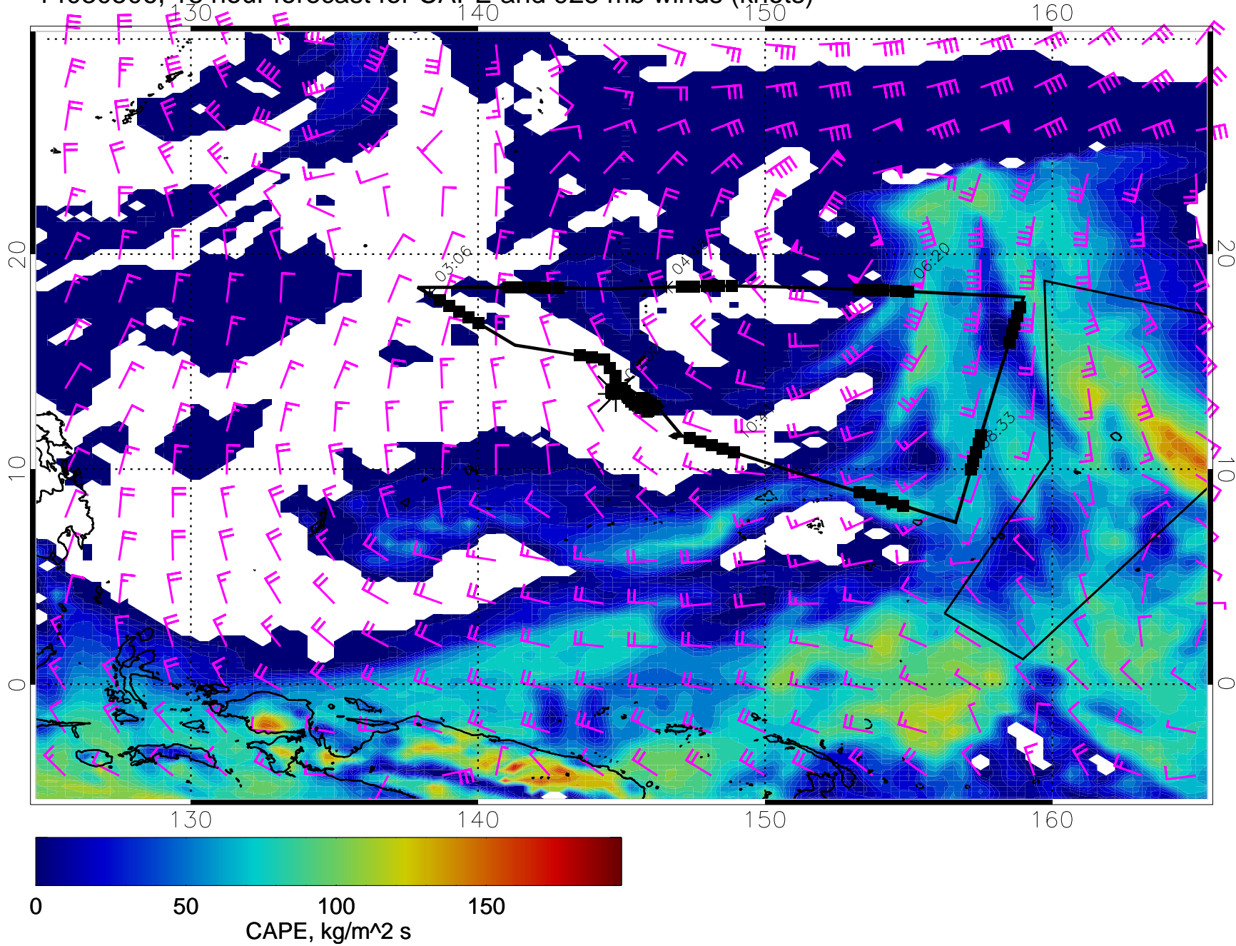
14030506, 18 hour forecast for CAPE and 925 mb winds (knots)
