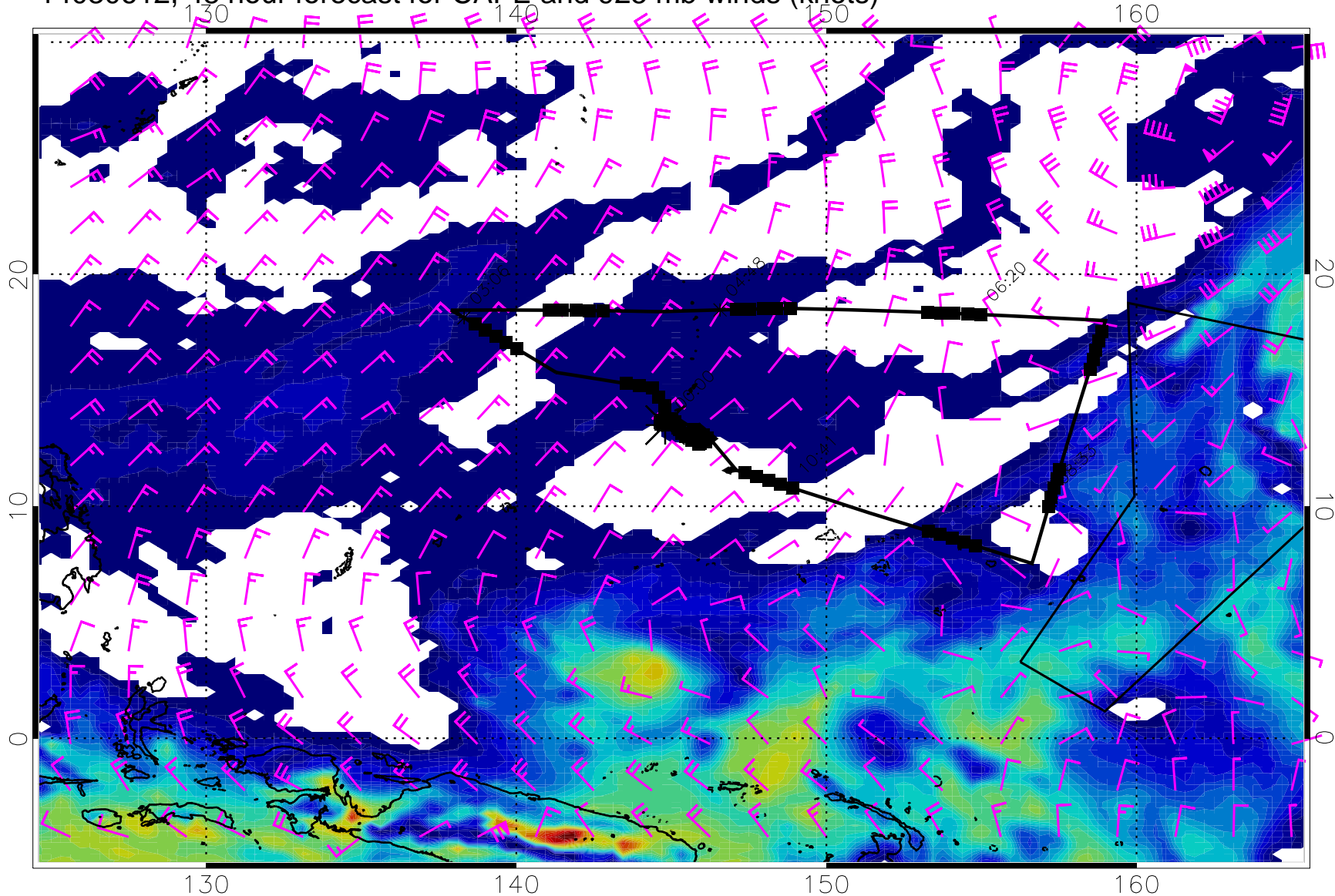
14030612, 48 hour forecast for CAPE and 925 mb winds (knots)
