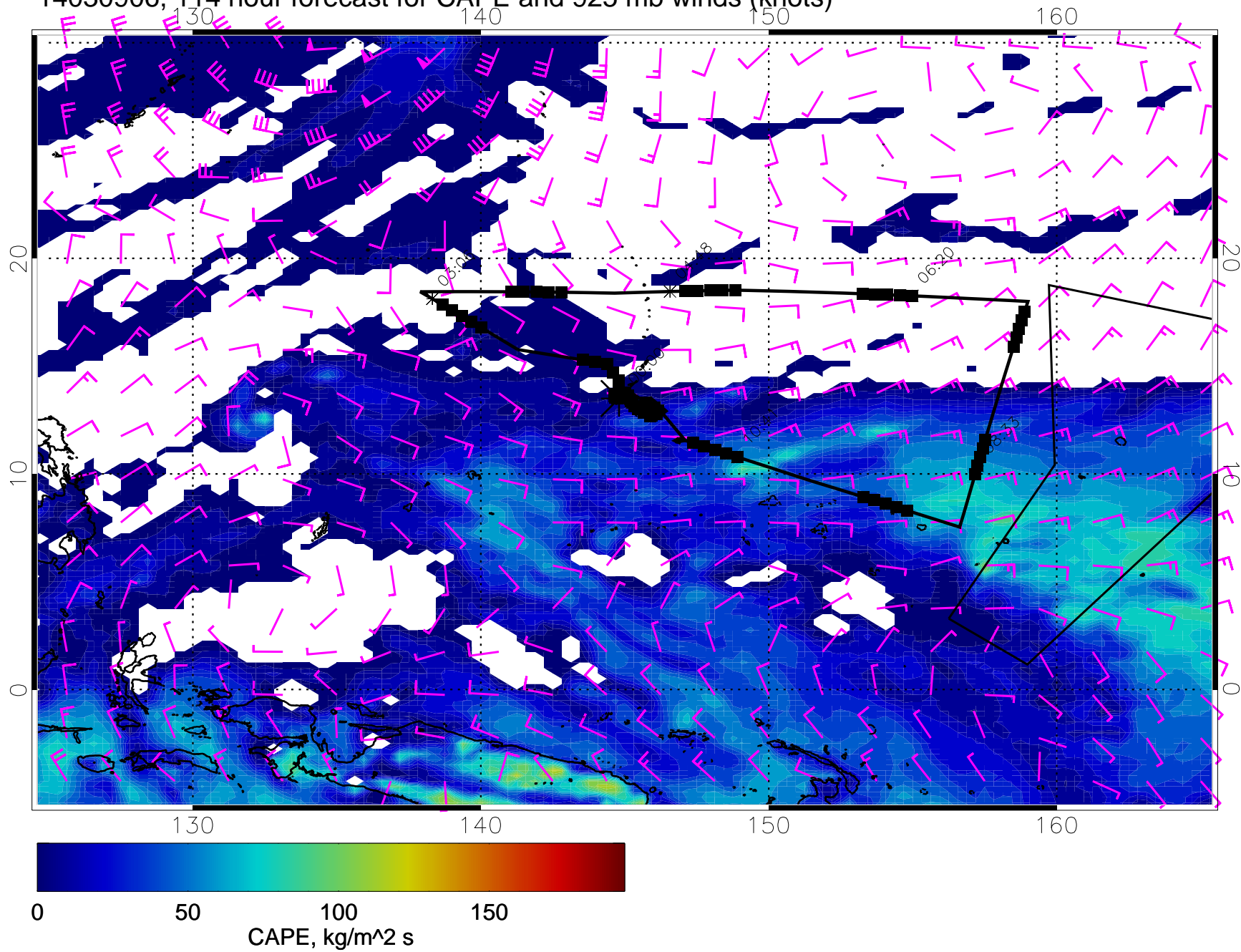
14030906, 114 hour forecast for CAPE and 925 mb winds (knots)
