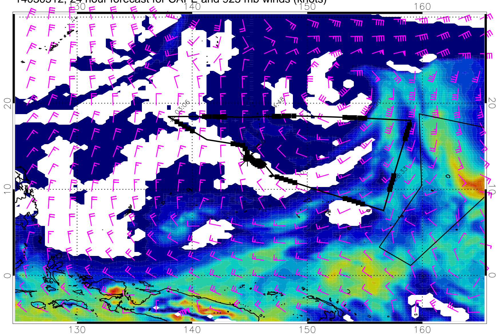
14030512, 24 hour forecast for CAPE and 925 mb winds (knots)
