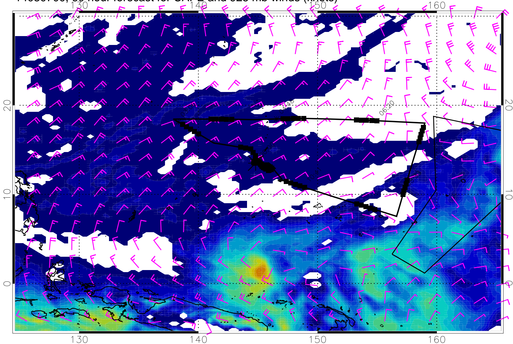
14030700, 60 hour forecast for CAPE and 925 mb winds (knots)
