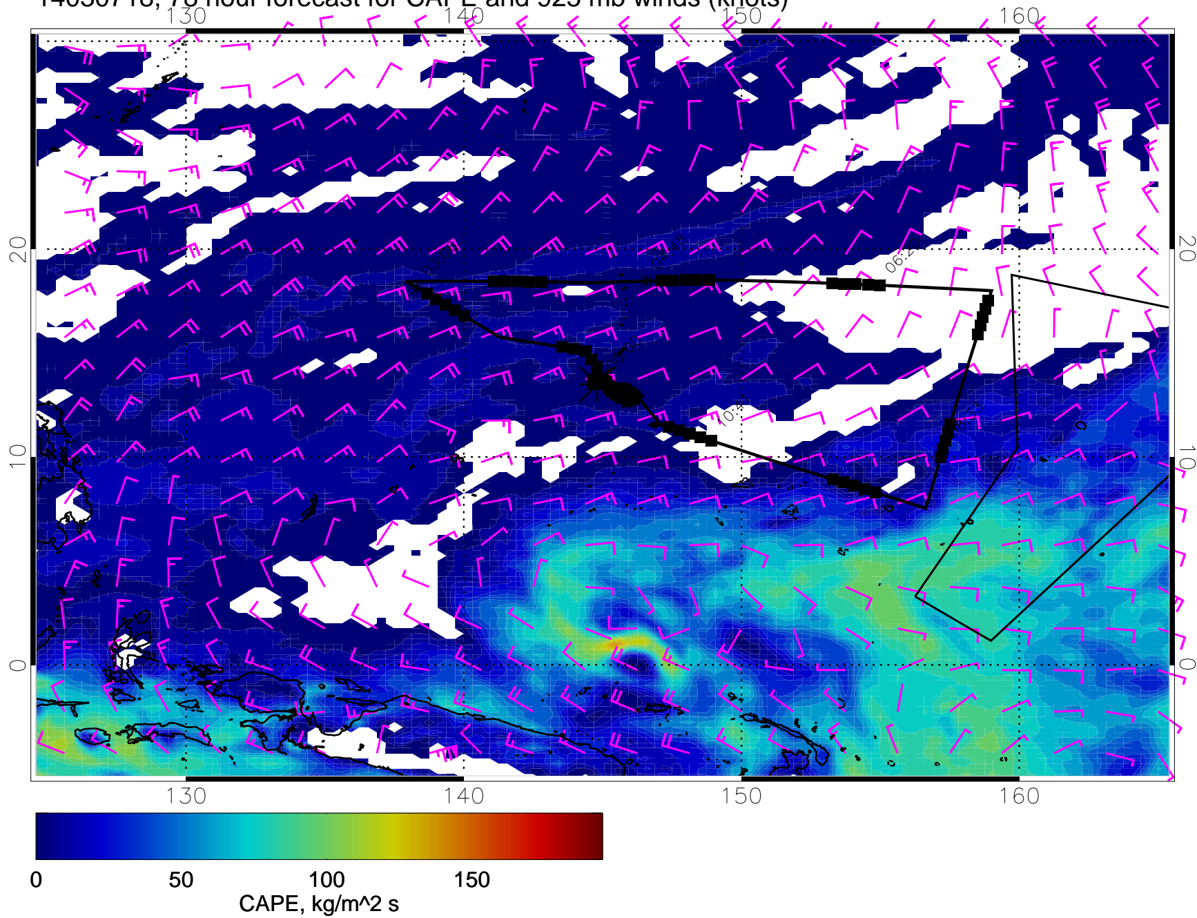
14030718, 78 hour forecast for CAPE and 925 mb winds (knots)
