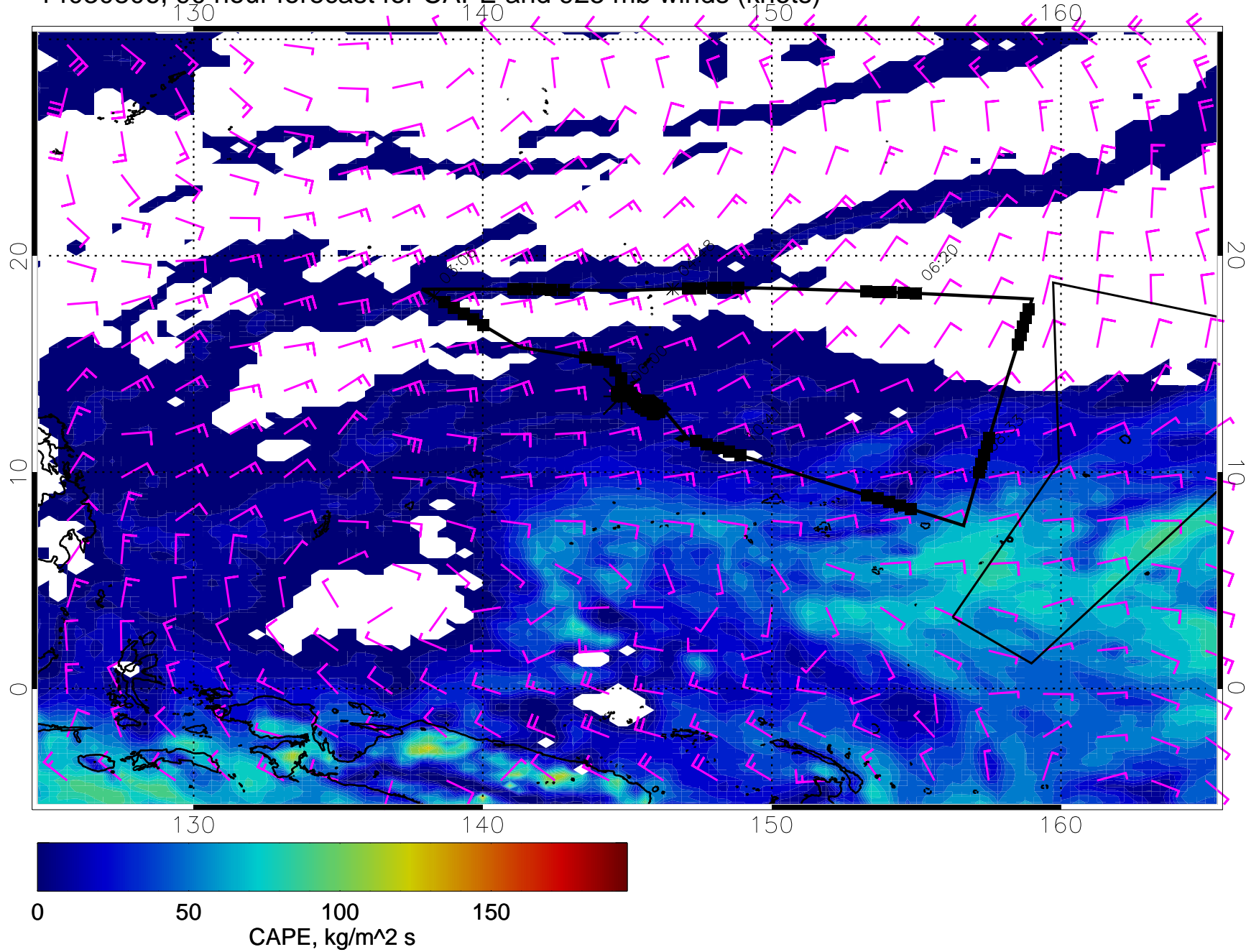
14030806, 90 hour forecast for CAPE and 925 mb winds (knots)
