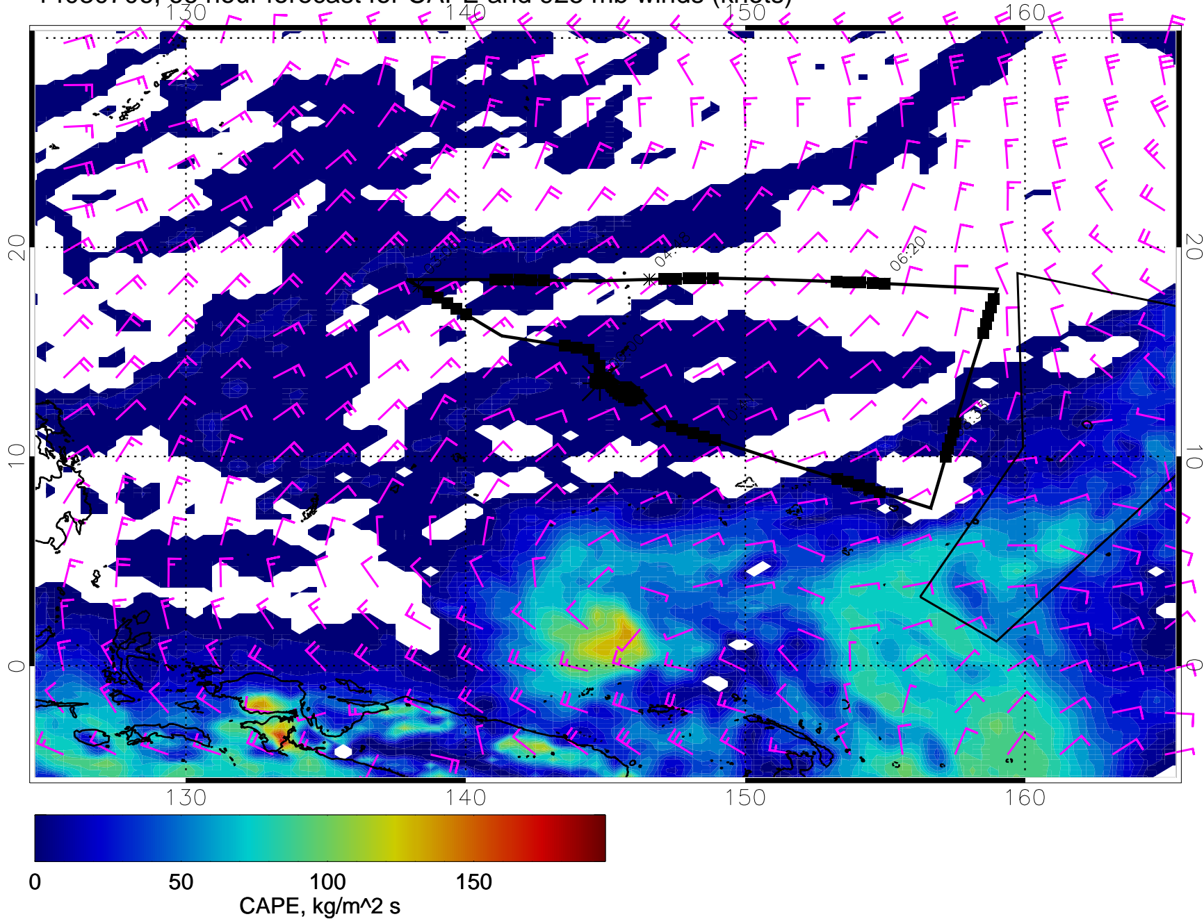
14030706, 66 hour forecast for CAPE and 925 mb winds (knots)
