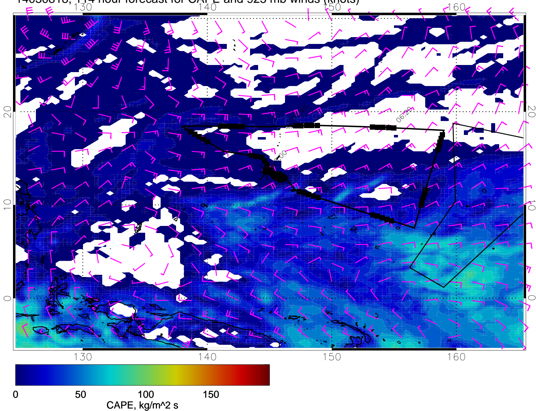
14030818, 114 hour forecast for CAPE and 925 mb winds (knots)
