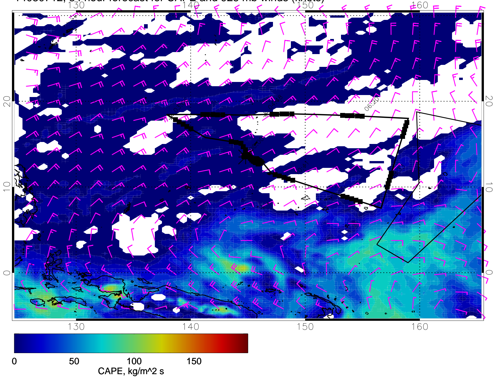
14030712, 84 hour forecast for CAPE and 925 mb winds (knots)
