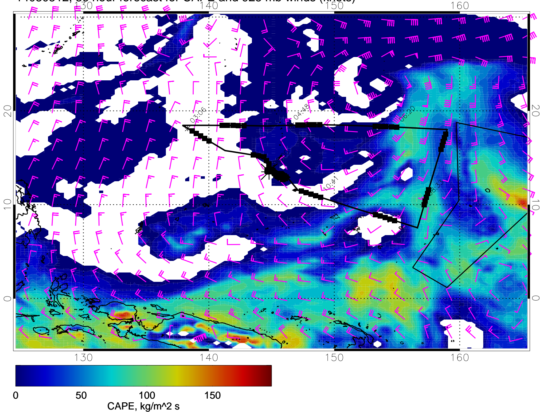
14030512, 36 hour forecast for CAPE and 925 mb winds (knots)
