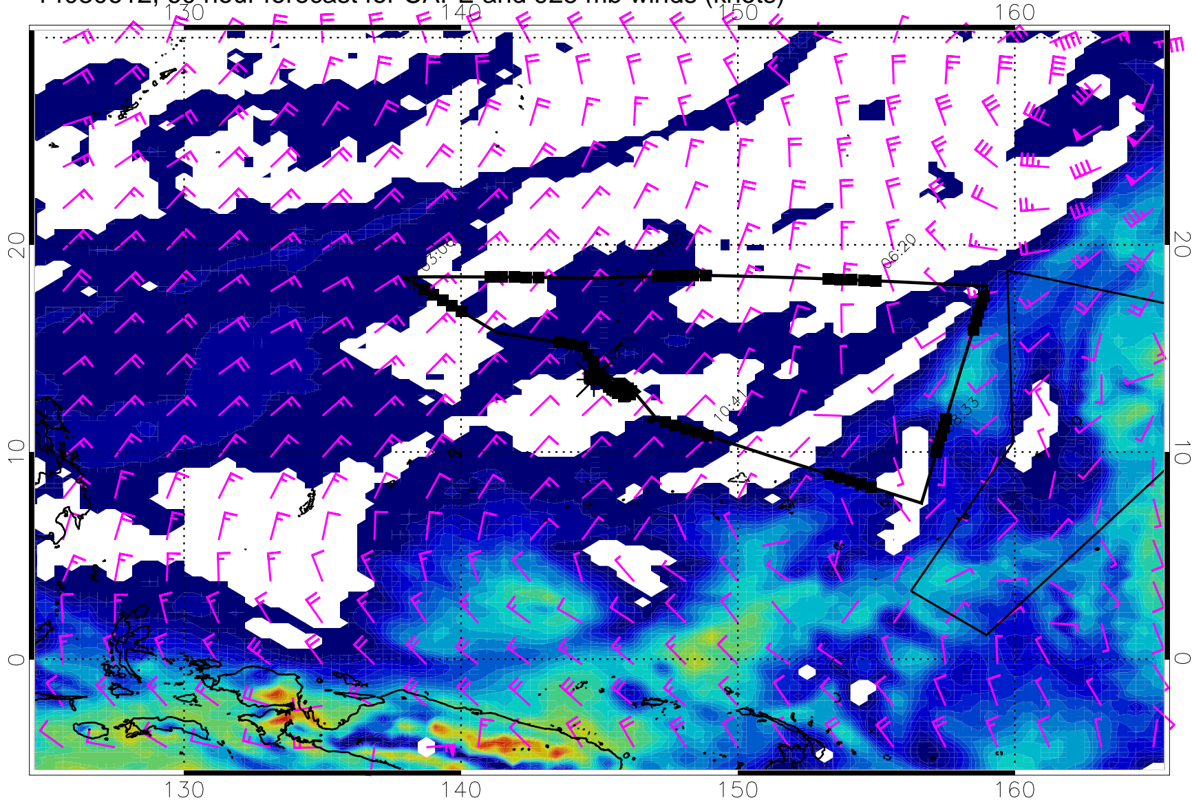
14030612, 60 hour forecast for CAPE and 925 mb winds (knots)
