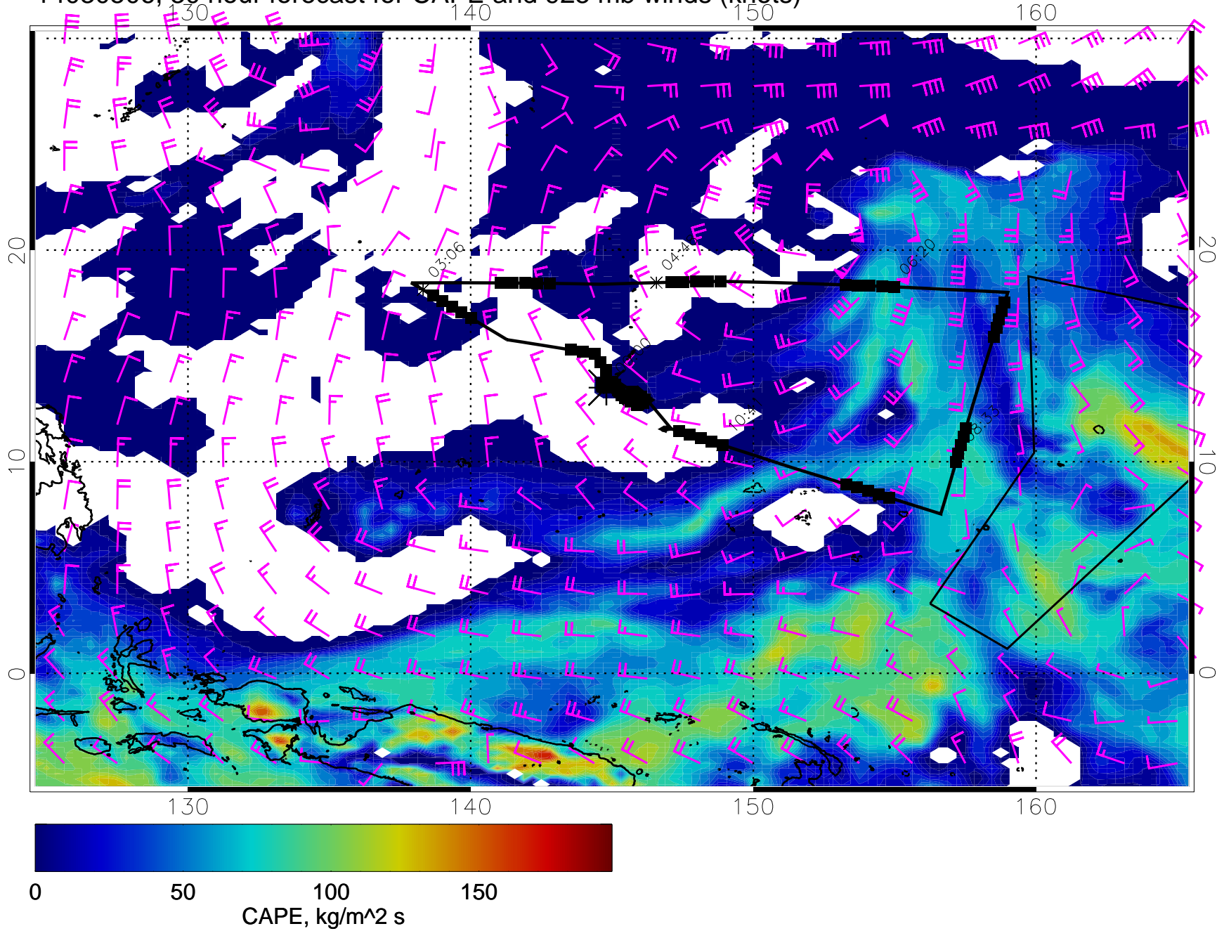
14030506, 30 hour forecast for CAPE and 925 mb winds (knots)
