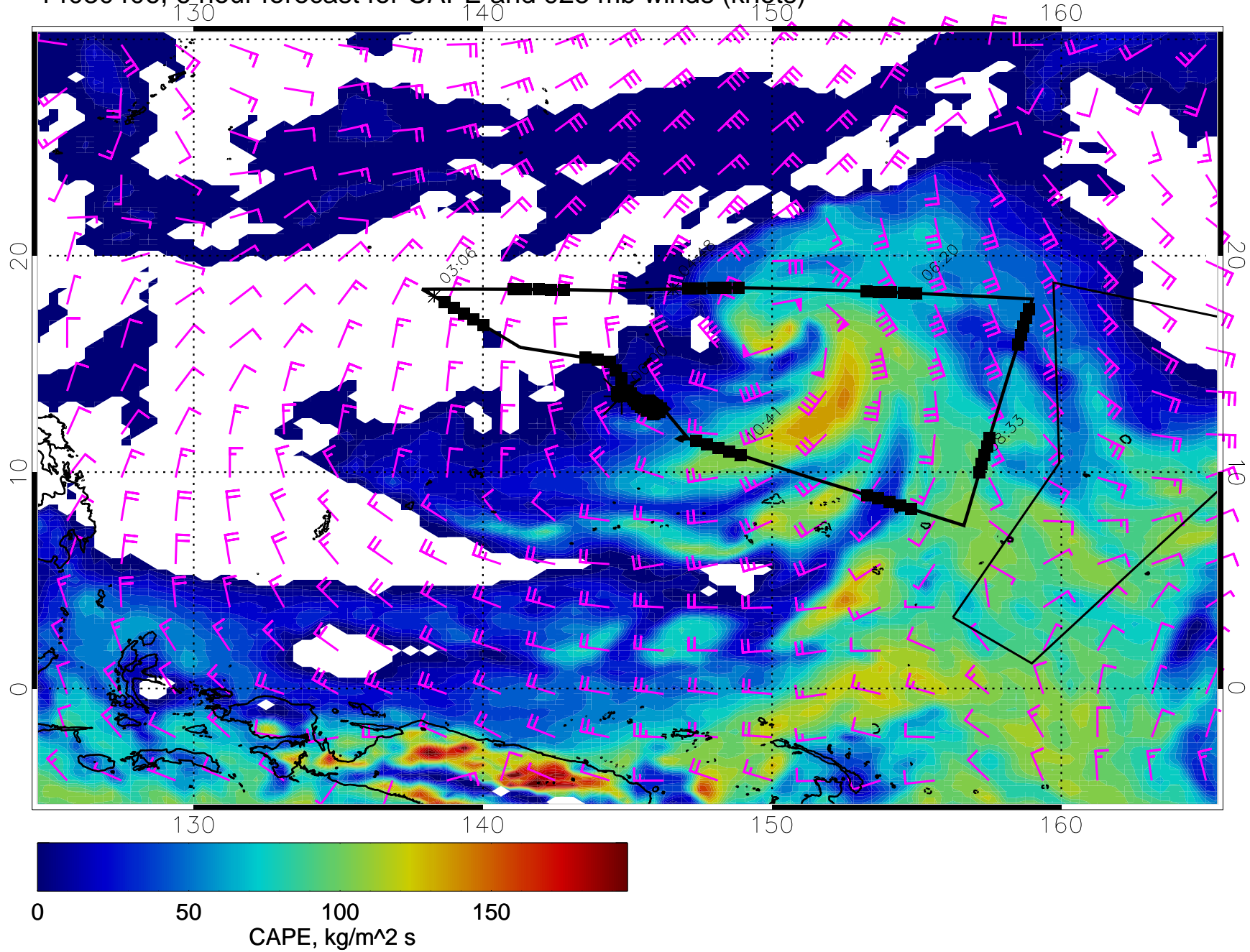
14030406, 6 hour forecast for CAPE and 925 mb winds (knots)
