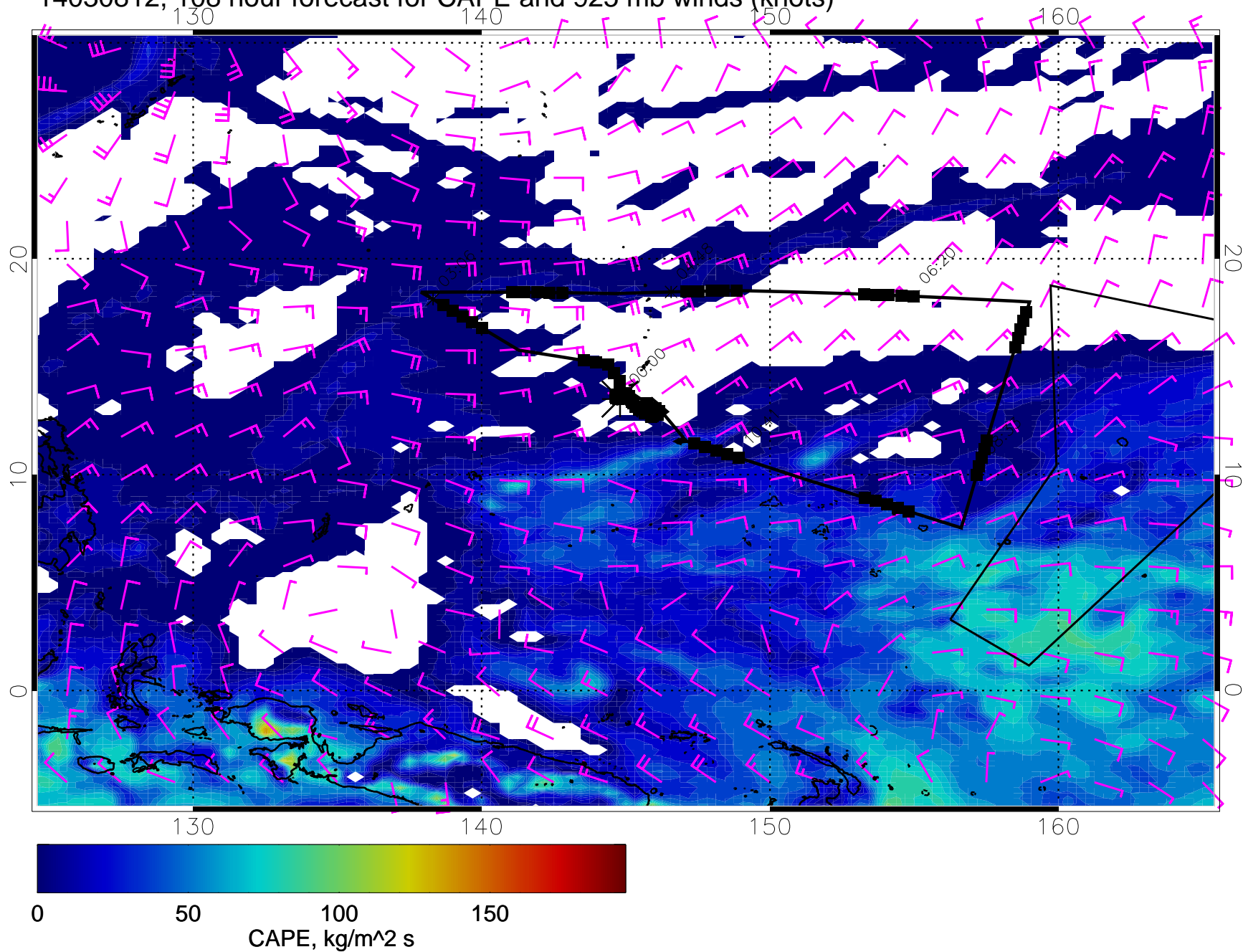
14030812, 108 hour forecast for CAPE and 925 mb winds (knots)
