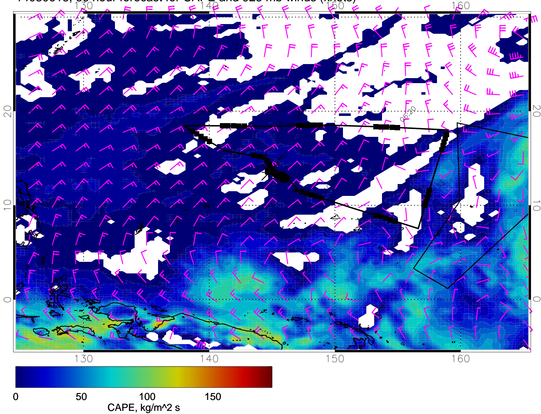
14030618, 66 hour forecast for CAPE and 925 mb winds (knots)
