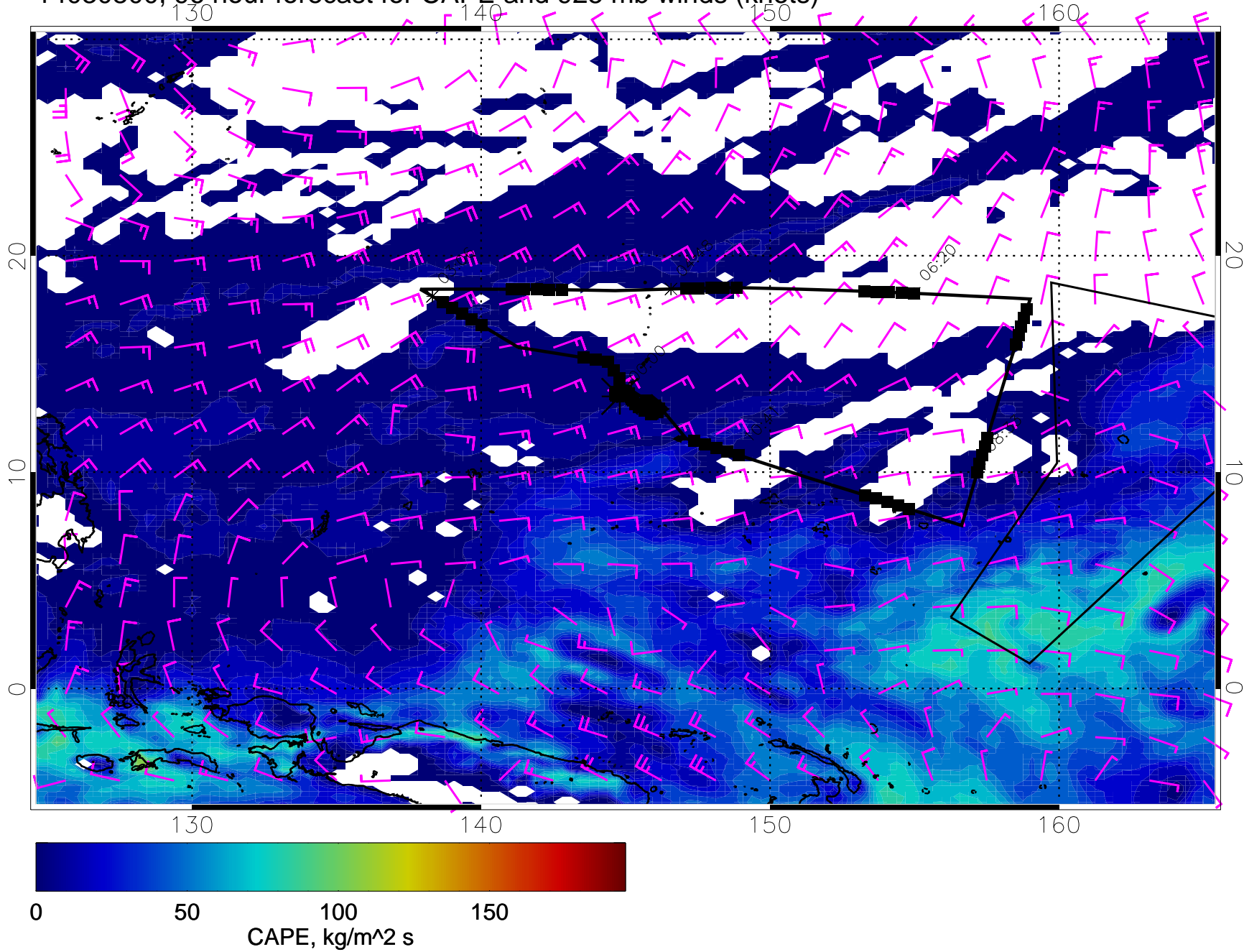
14030800, 96 hour forecast for CAPE and 925 mb winds (knots)
