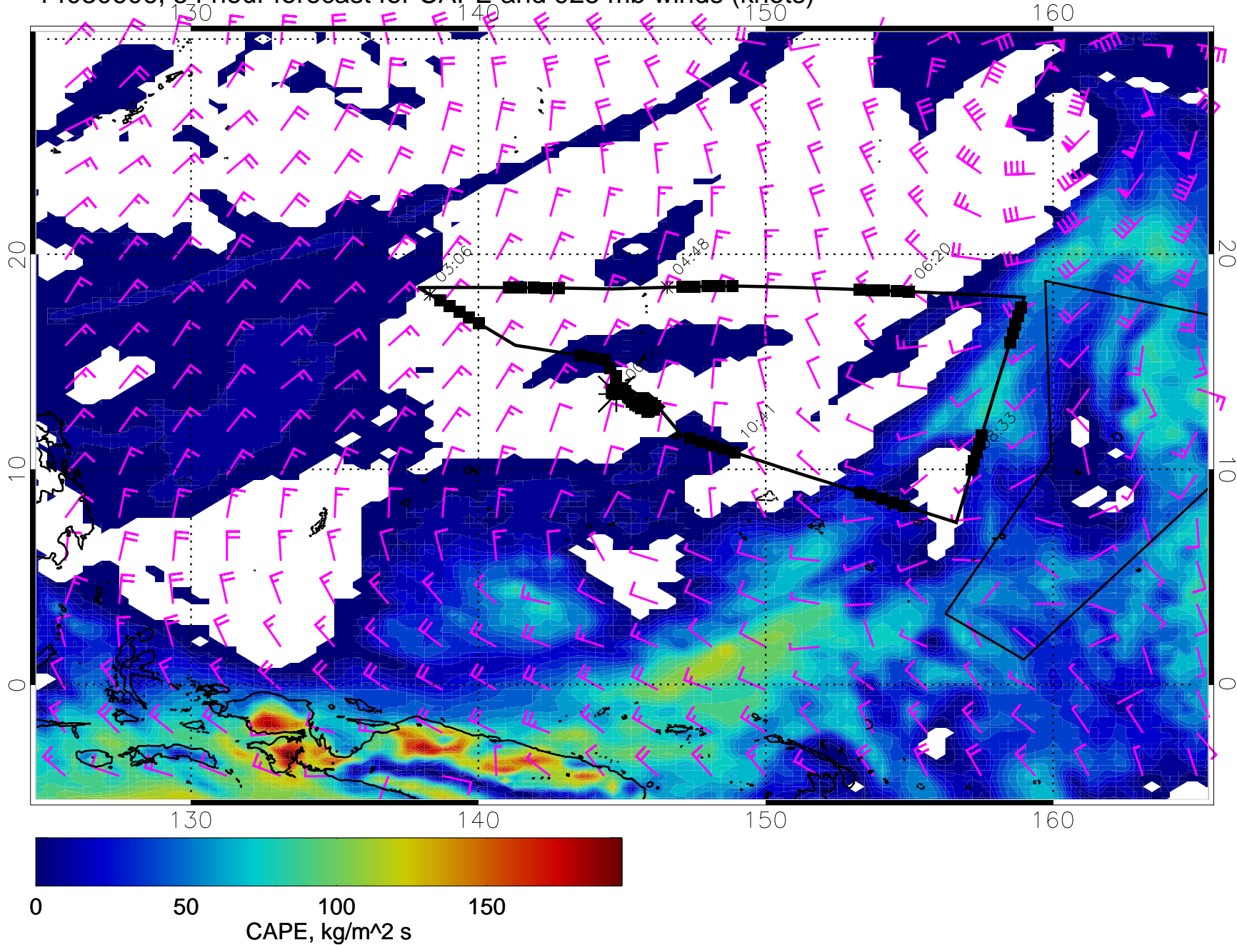
14030606, 54 hour forecast for CAPE and 925 mb winds (knots)
