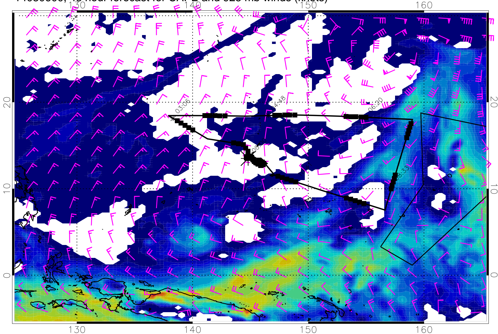
14030600, 48 hour forecast for CAPE and 925 mb winds (knots)
