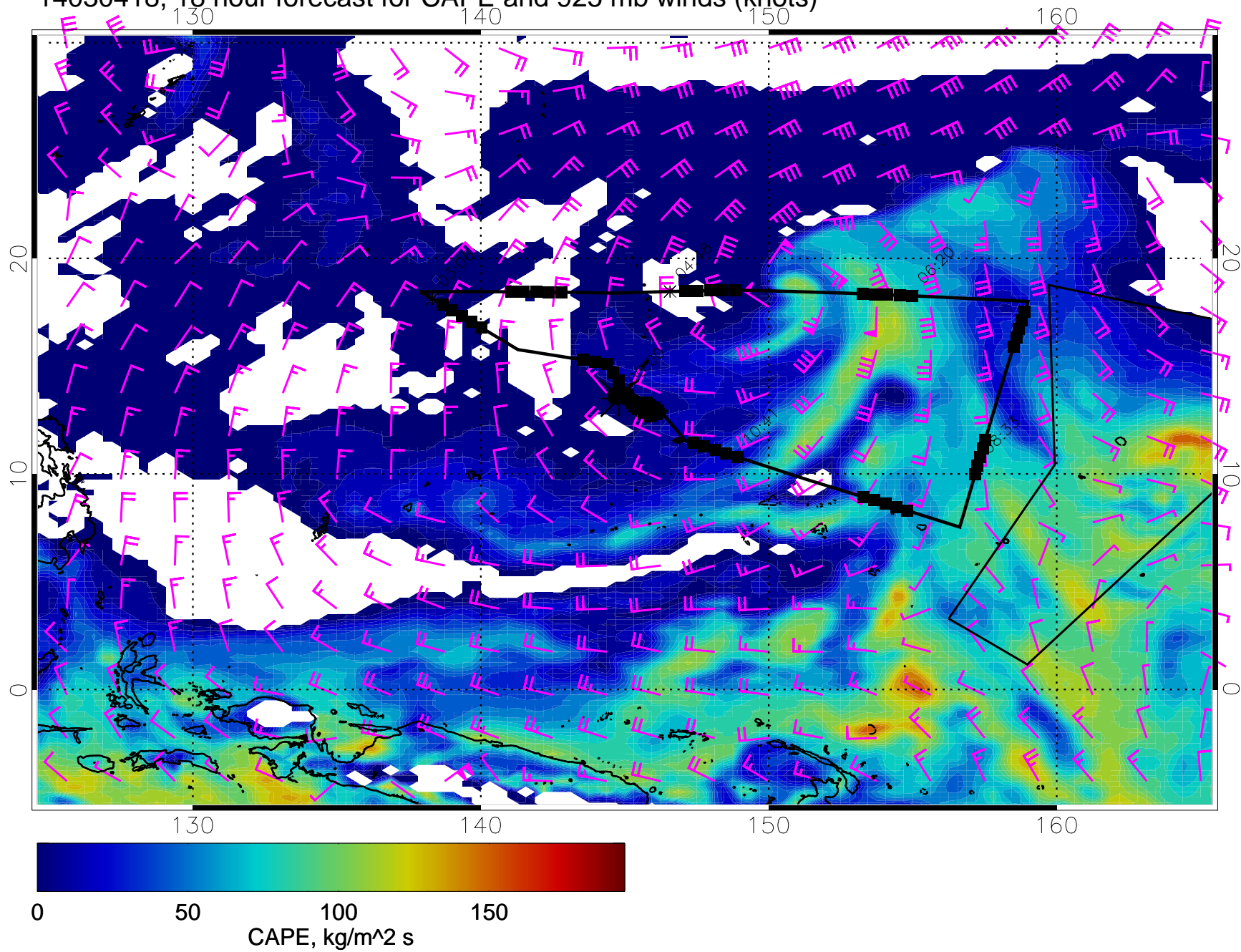
14030418, 18 hour forecast for CAPE and 925 mb winds (knots)
