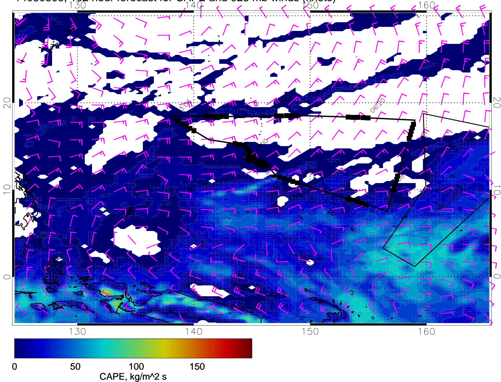
14030806, 102 hour forecast for CAPE and 925 mb winds (knots)
