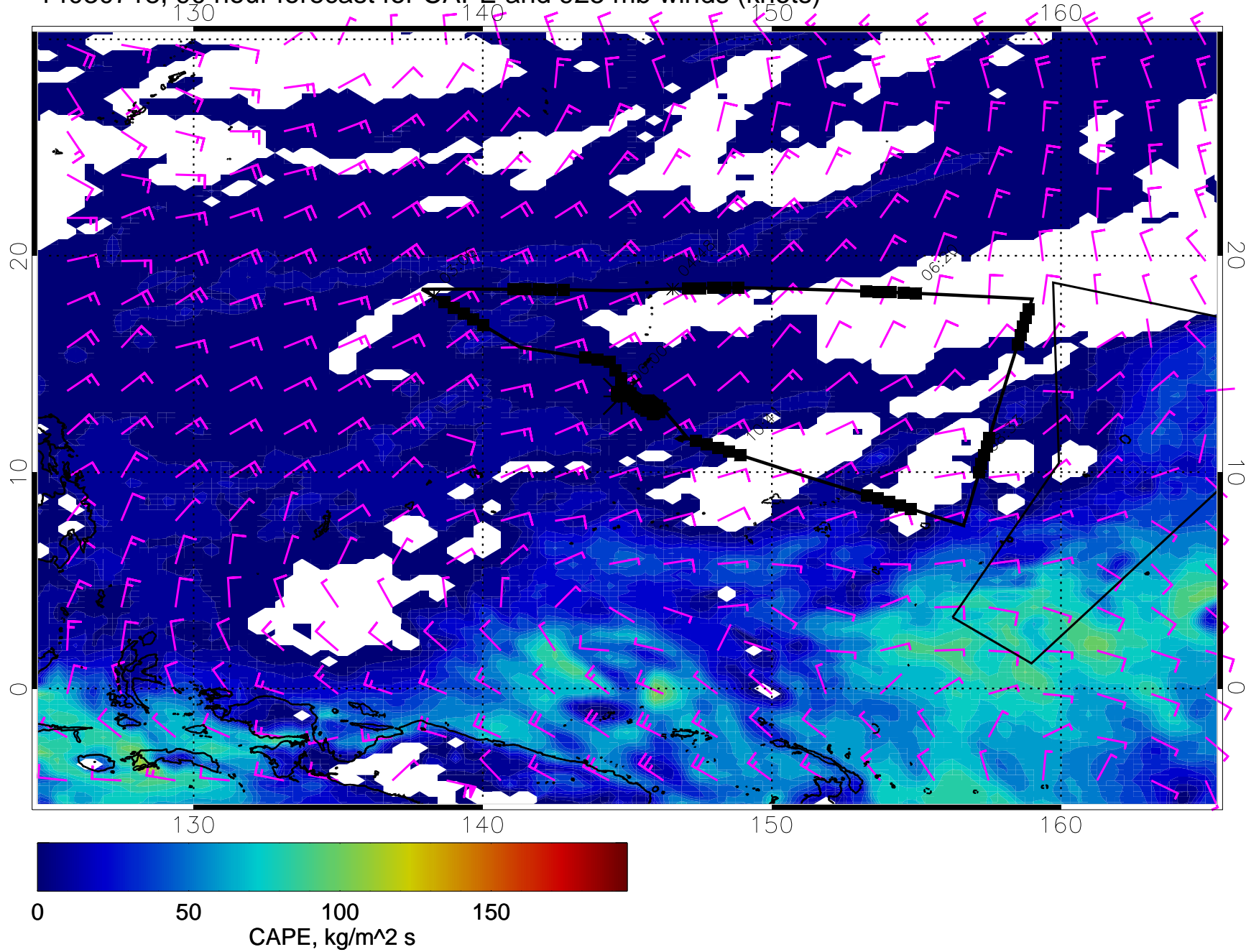
14030718, 90 hour forecast for CAPE and 925 mb winds (knots)
