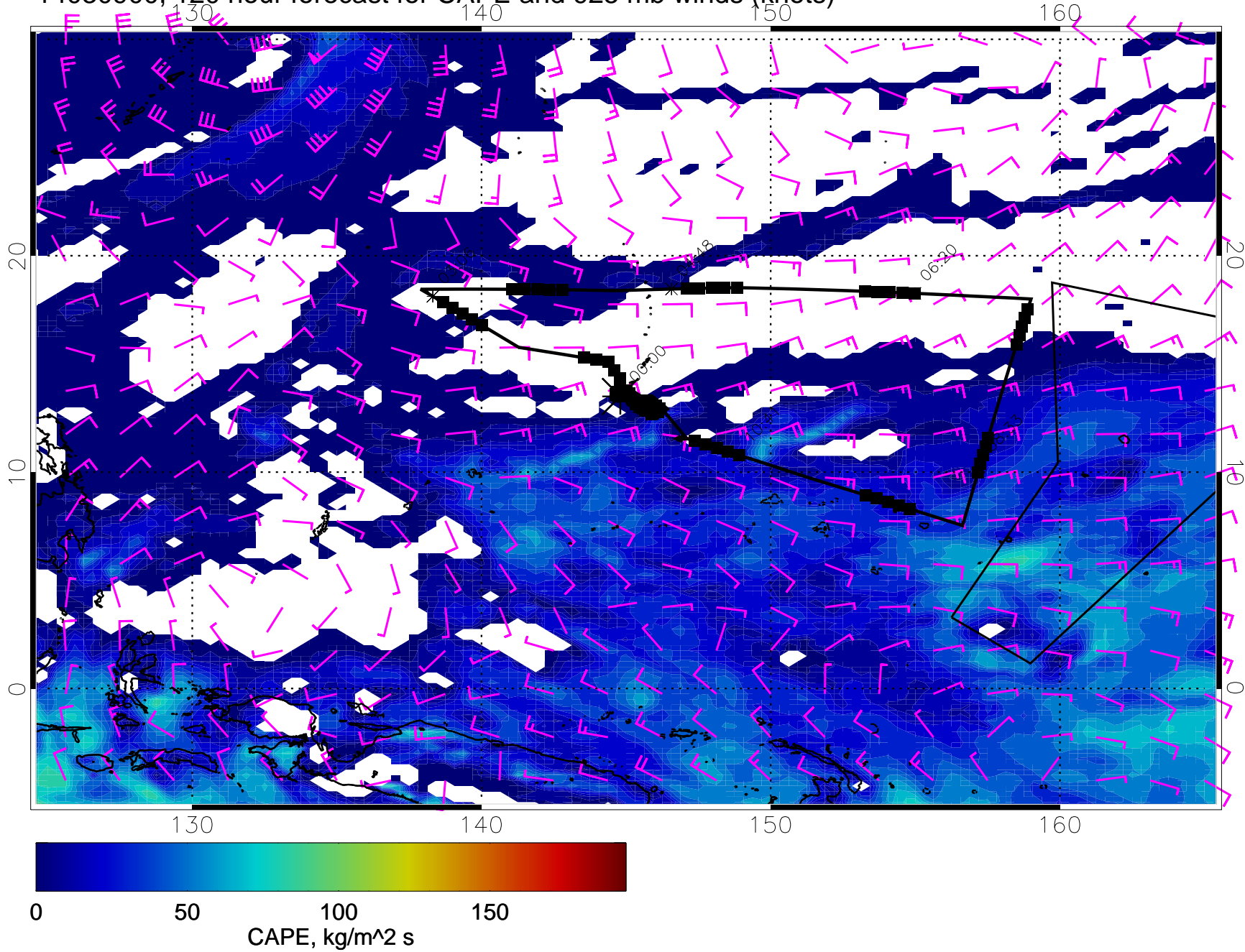
14030900, 120 hour forecast for CAPE and 925 mb winds (knots)
