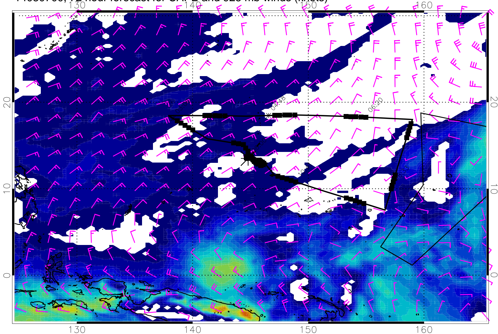
14030700, 72 hour forecast for CAPE and 925 mb winds (knots)
