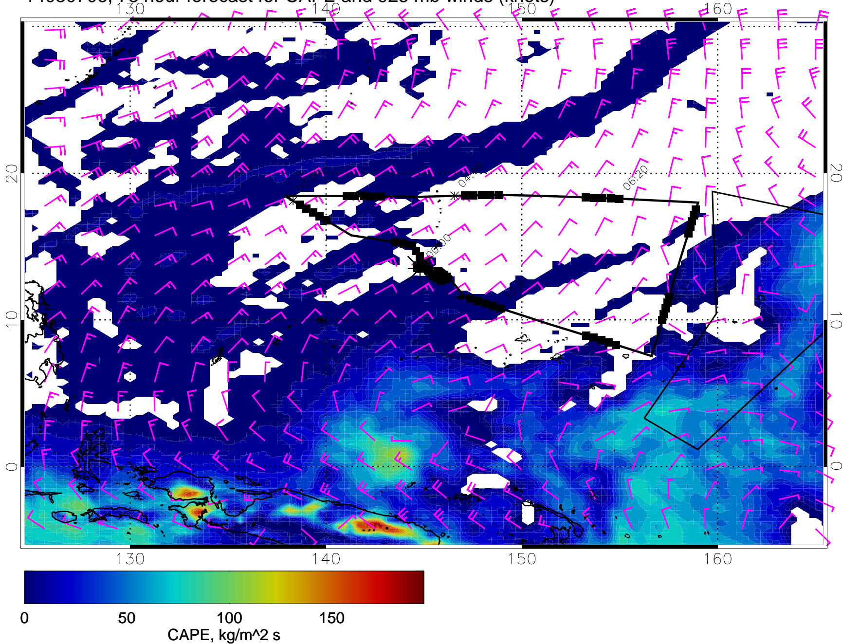
14030706, 78 hour forecast for CAPE and 925 mb winds (knots)
