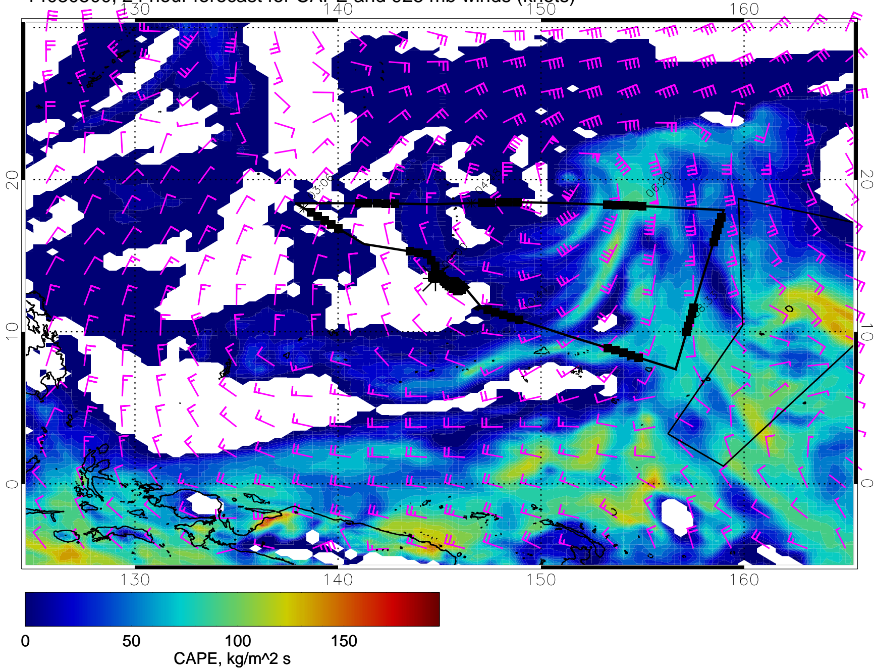
14030500, 24 hour forecast for CAPE and 925 mb winds (knots)
