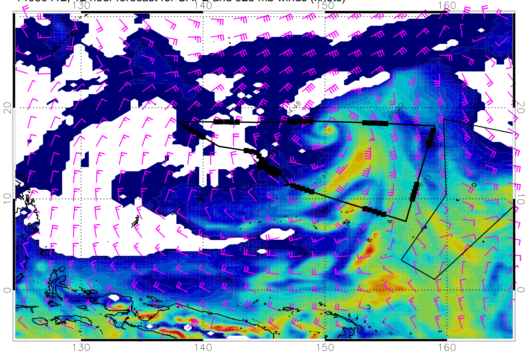
14030412, 12 hour forecast for CAPE and 925 mb winds (knots)
