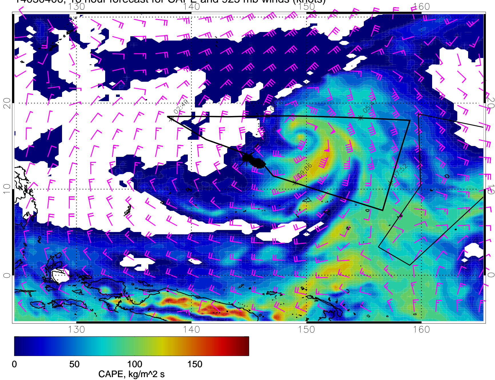
14030406, 18 hour forecast for CAPE and 925 mb winds (knots)
