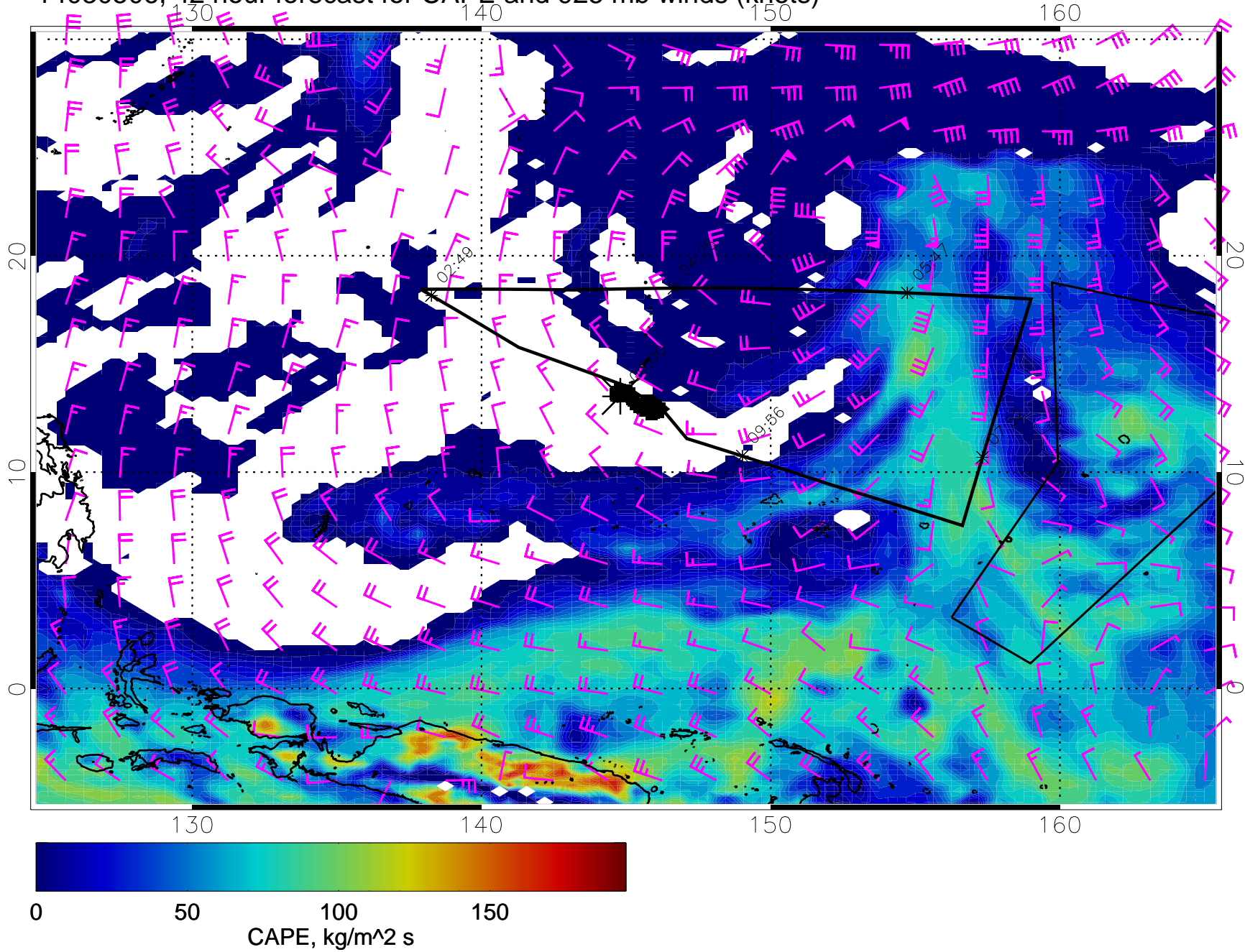
14030506, 42 hour forecast for CAPE and 925 mb winds (knots)
