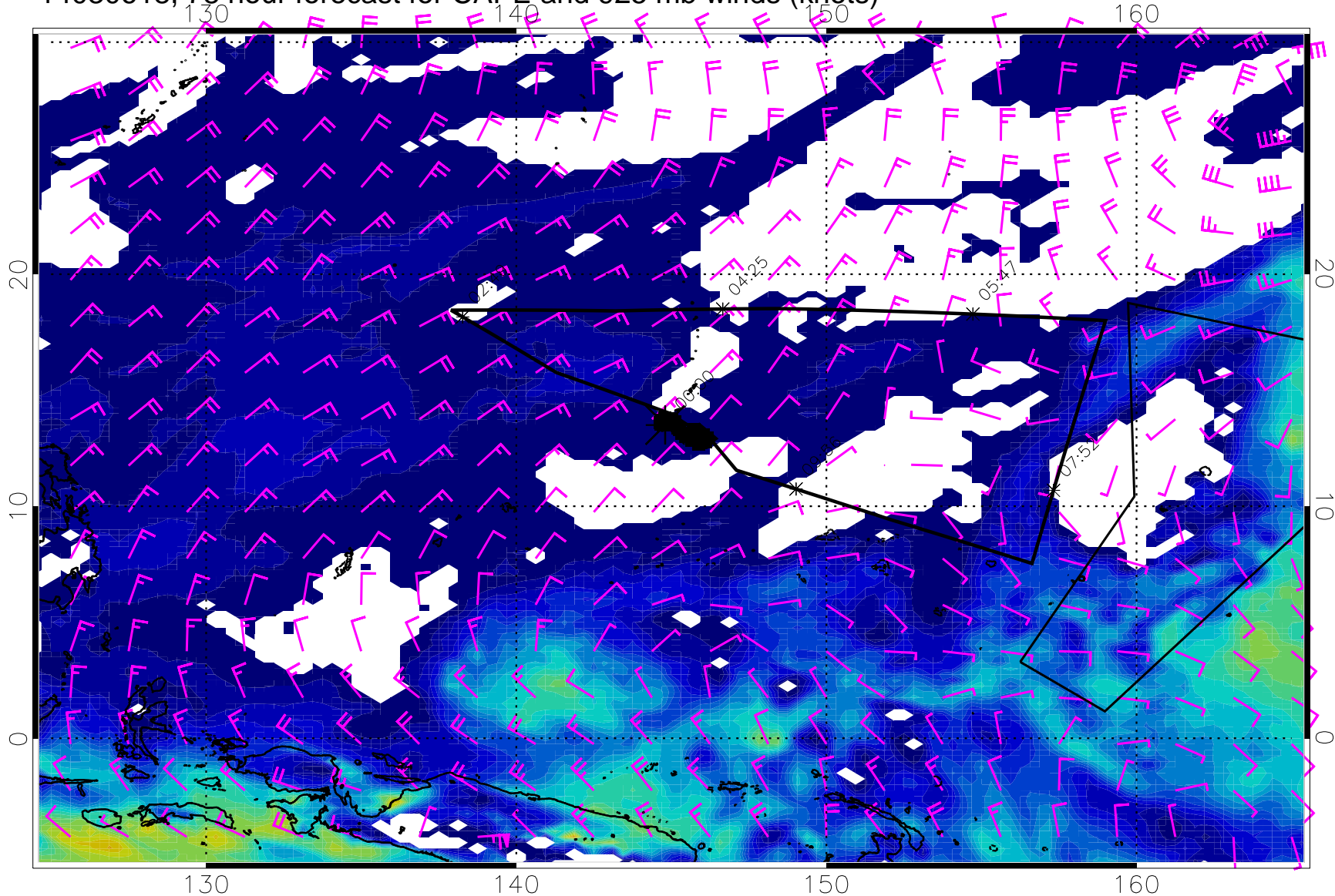
14030618, 78 hour forecast for CAPE and 925 mb winds (knots)
