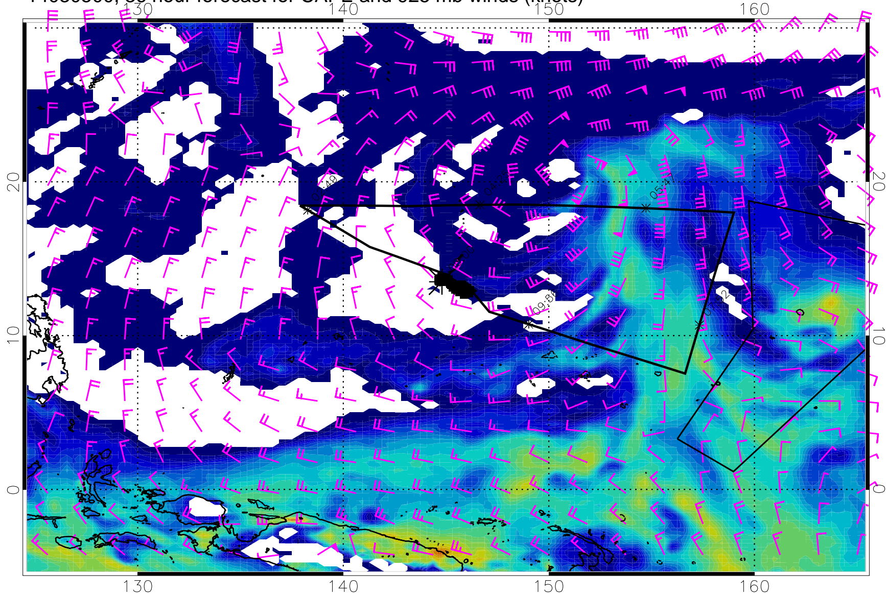
14030500, 36 hour forecast for CAPE and 925 mb winds (knots)
