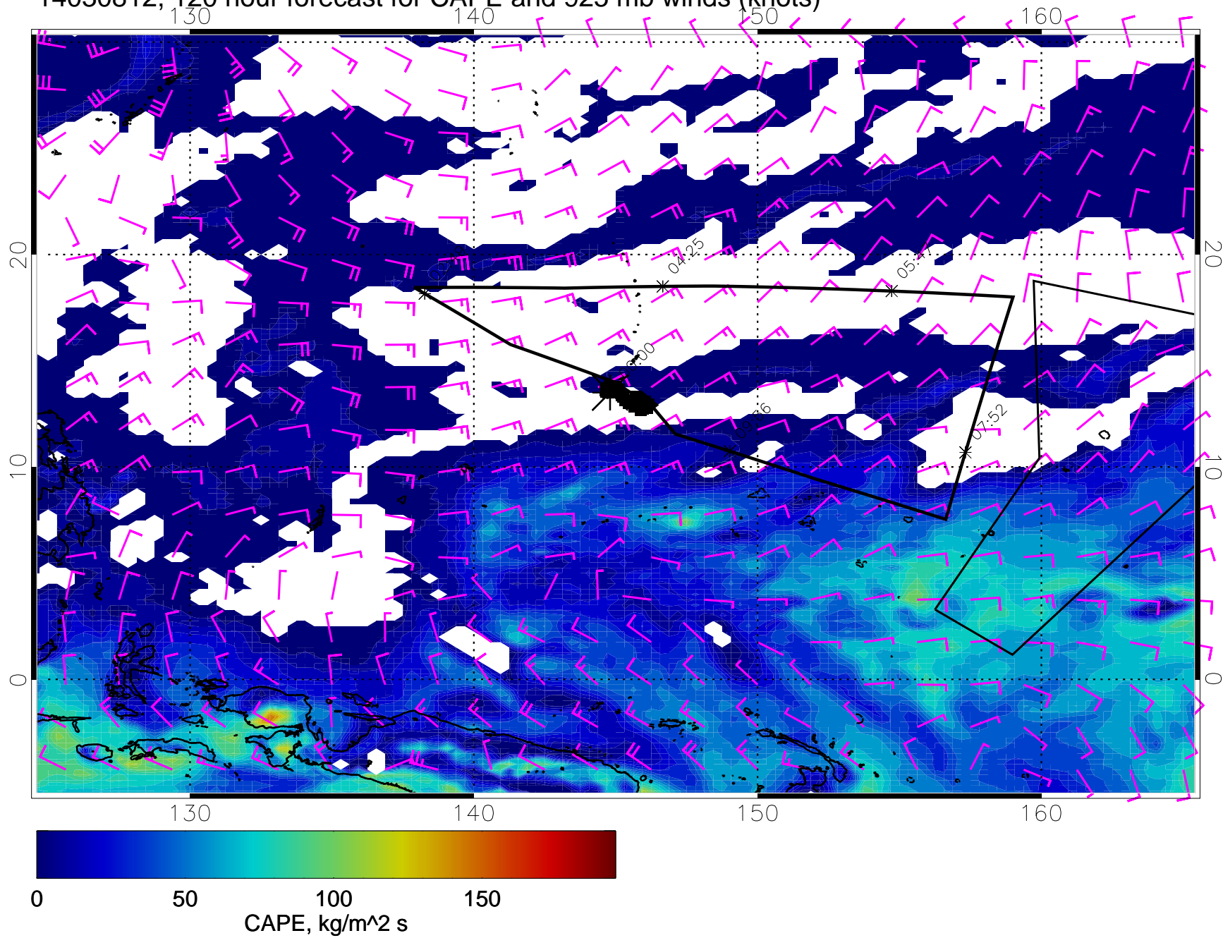
14030812, 120 hour forecast for CAPE and 925 mb winds (knots)
