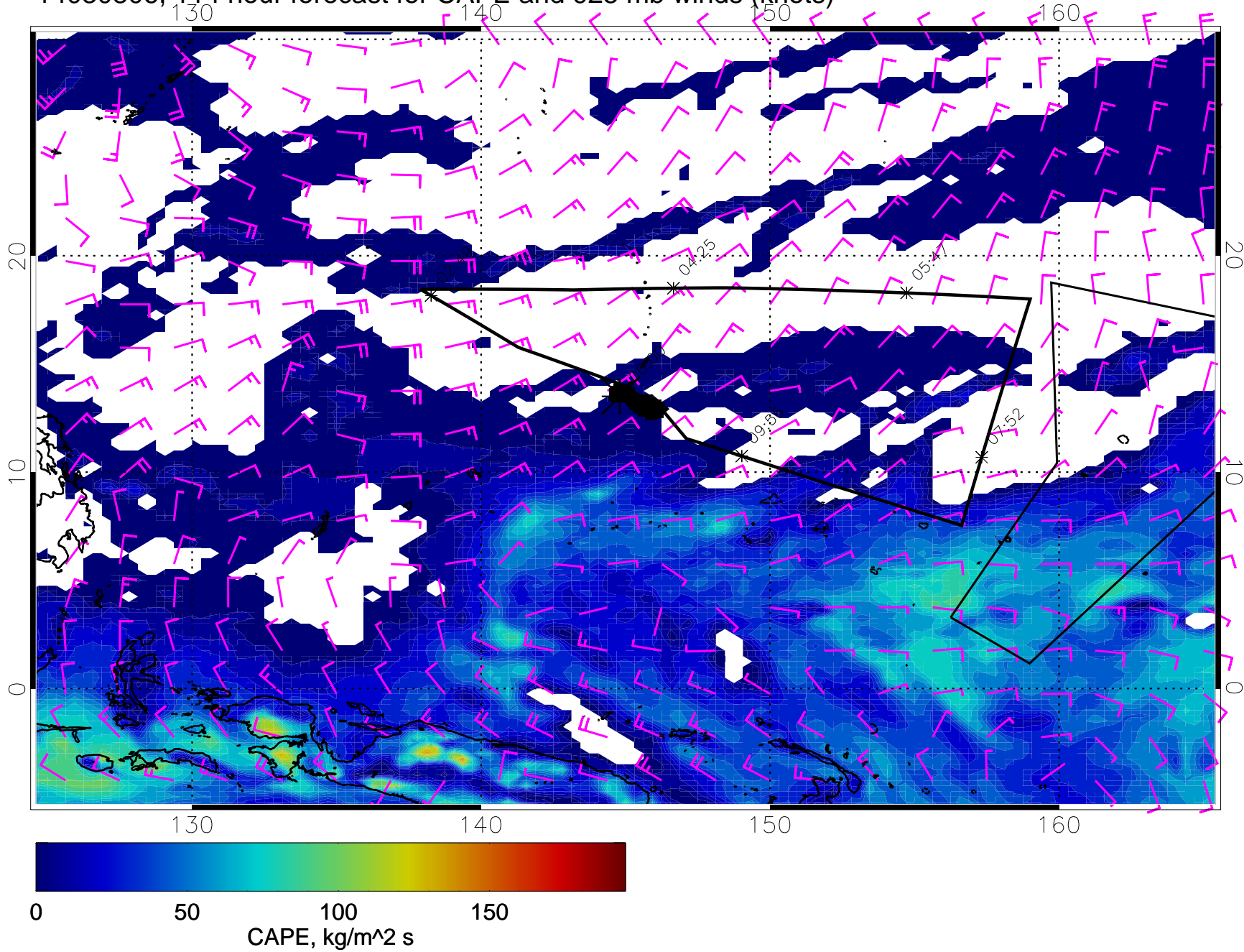
14030806, 114 hour forecast for CAPE and 925 mb winds (knots)
