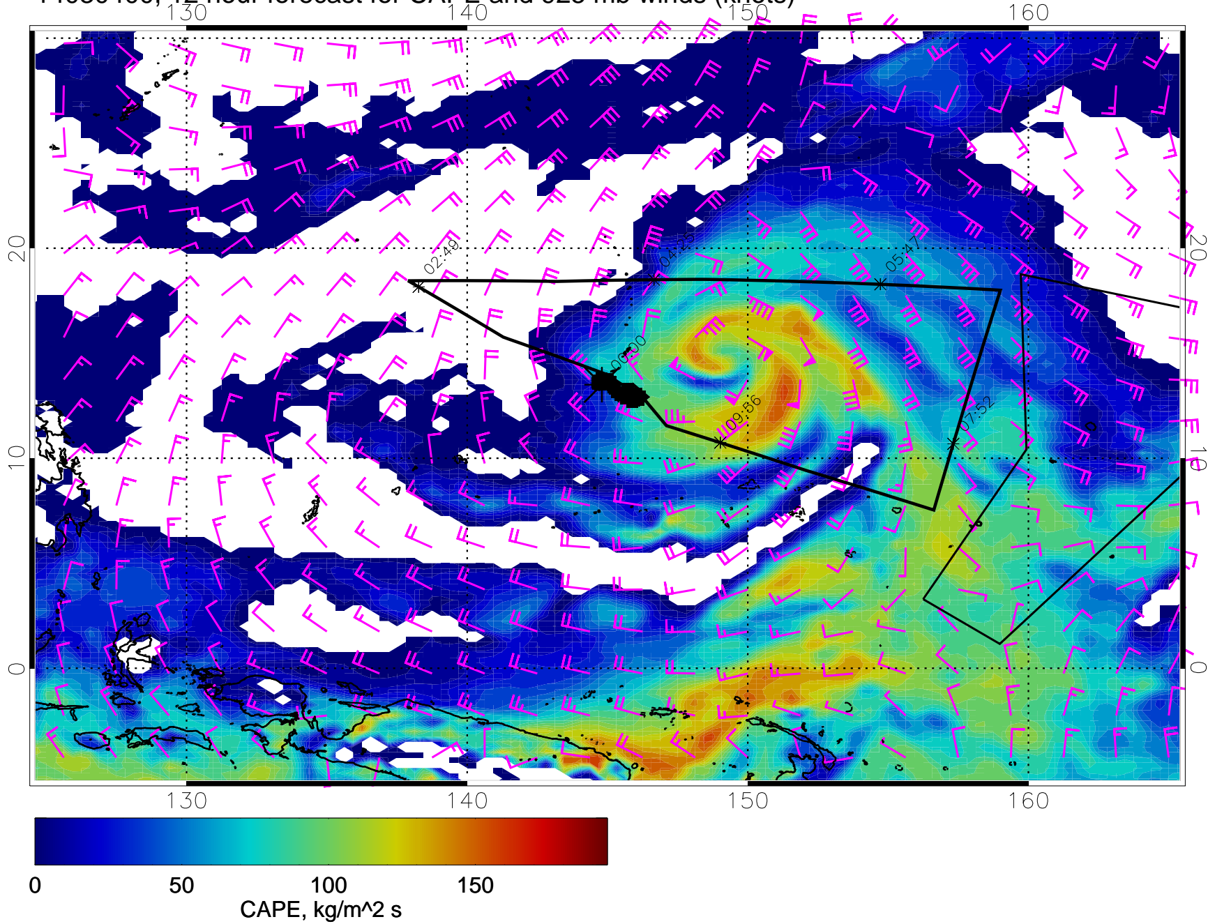
14030400, 12 hour forecast for CAPE and 925 mb winds (knots)
