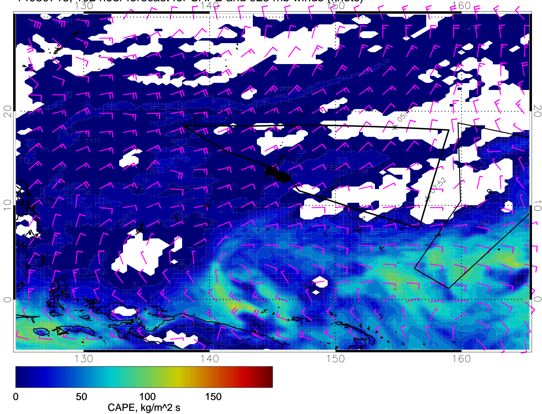
14030718, 102 hour forecast for CAPE and 925 mb winds (knots)
