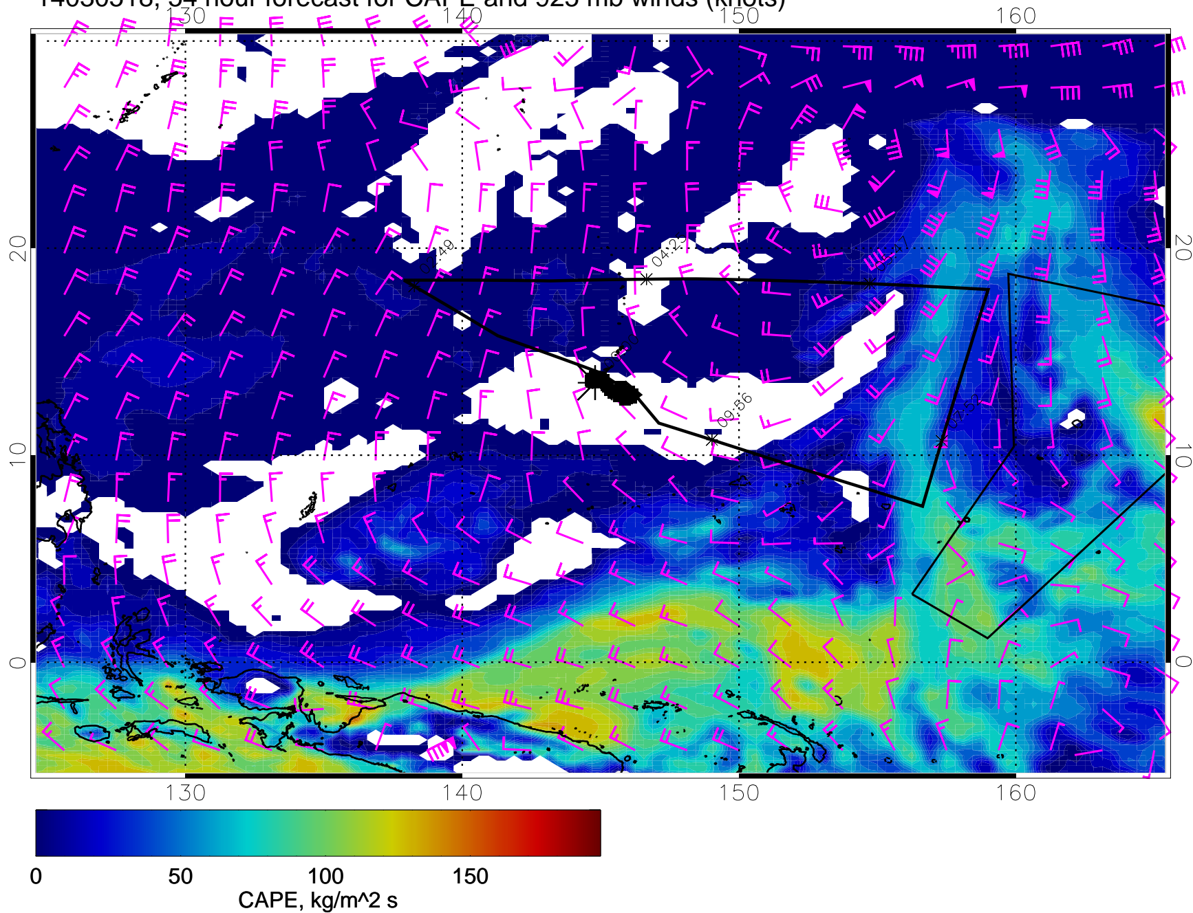
14030518, 54 hour forecast for CAPE and 925 mb winds (knots)
