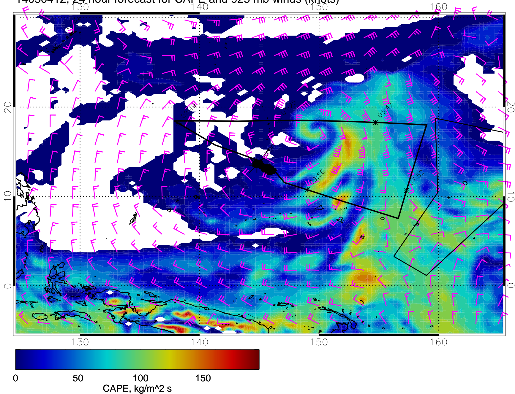
14030412, 24 hour forecast for CAPE and 925 mb winds (knots)
