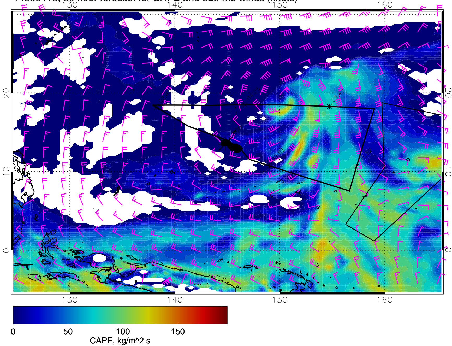
14030418, 30 hour forecast for CAPE and 925 mb winds (knots)
