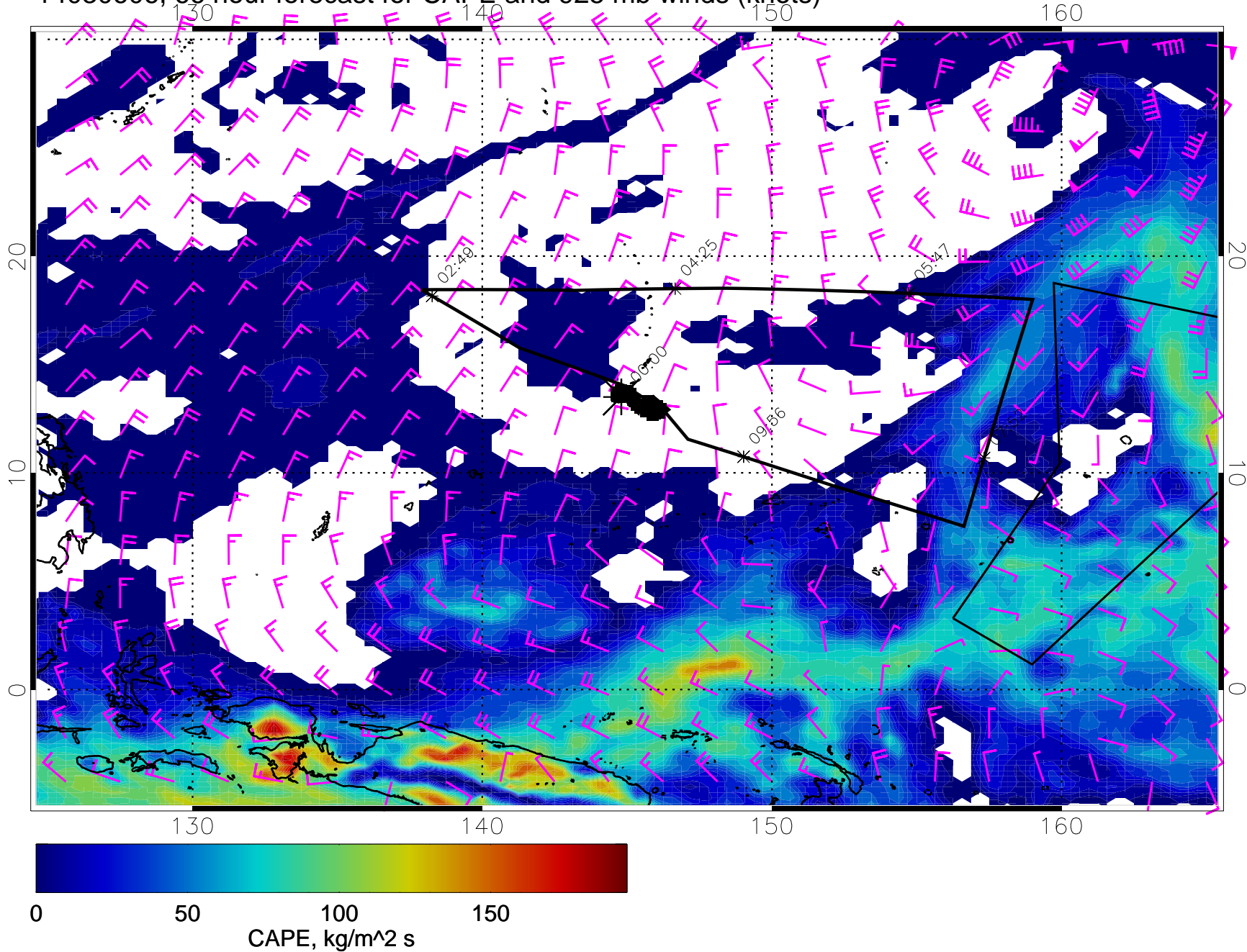
14030606, 66 hour forecast for CAPE and 925 mb winds (knots)
