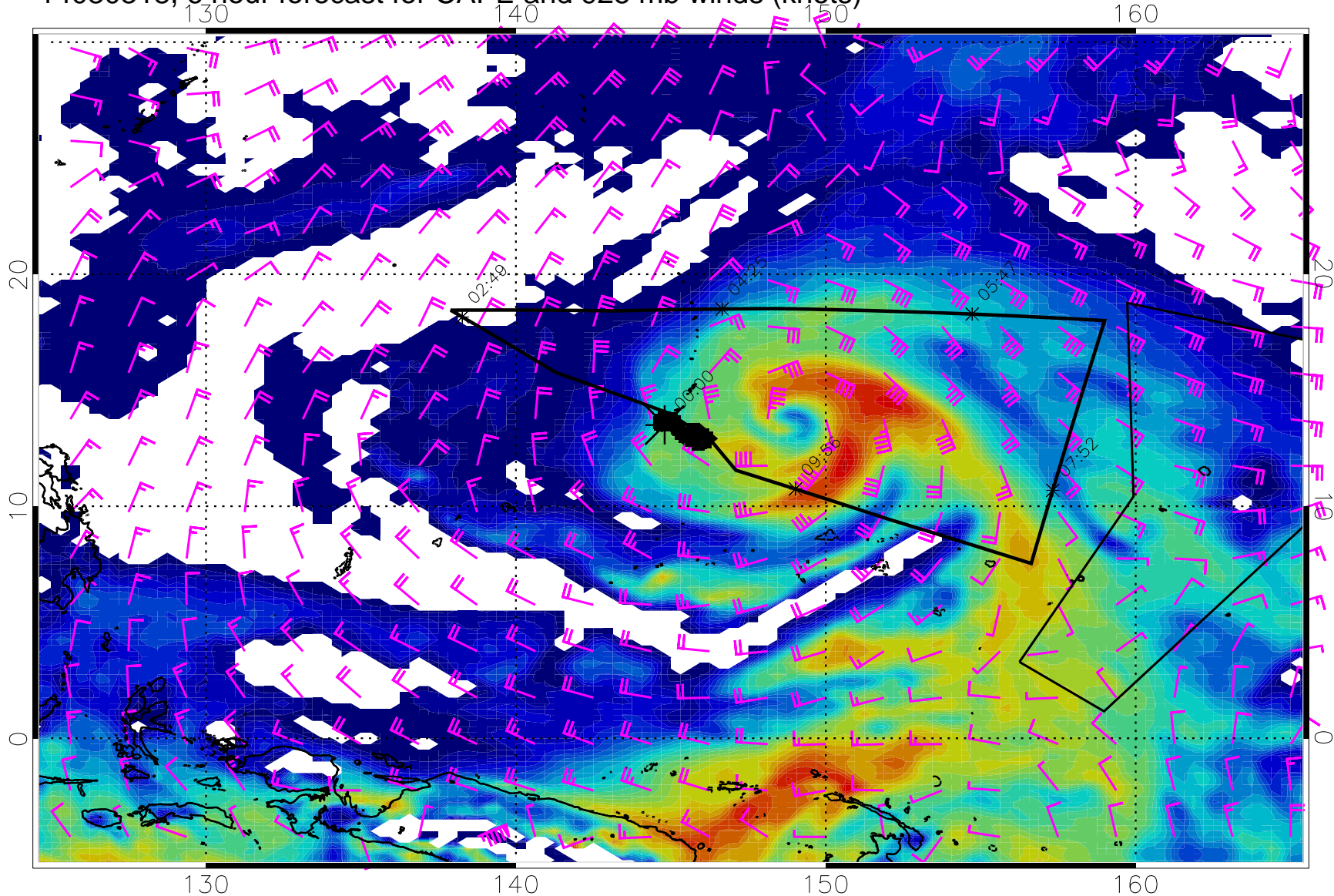
14030318, 6 hour forecast for CAPE and 925 mb winds (knots)
