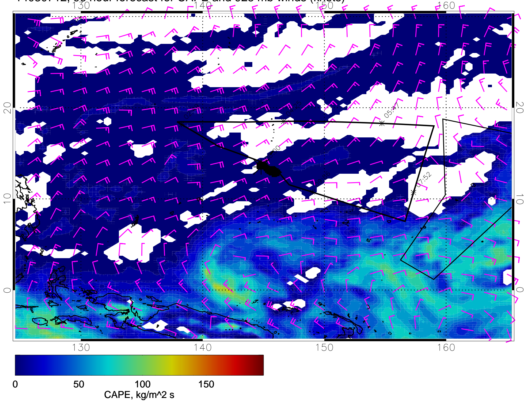
14030712, 96 hour forecast for CAPE and 925 mb winds (knots)
