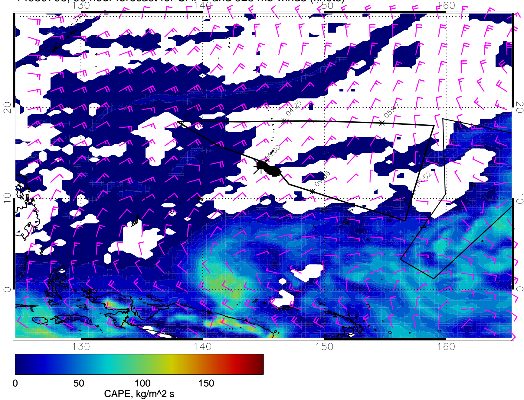
14030706, 90 hour forecast for CAPE and 925 mb winds (knots)
