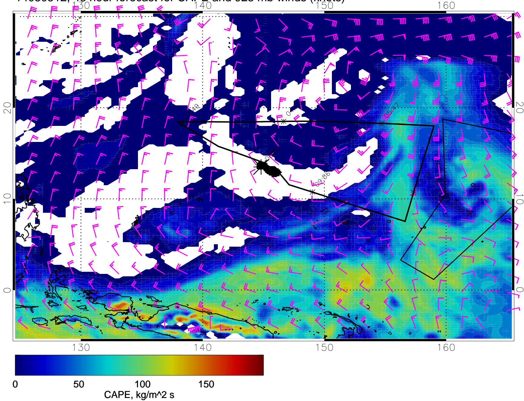
14030512, 48 hour forecast for CAPE and 925 mb winds (knots)
