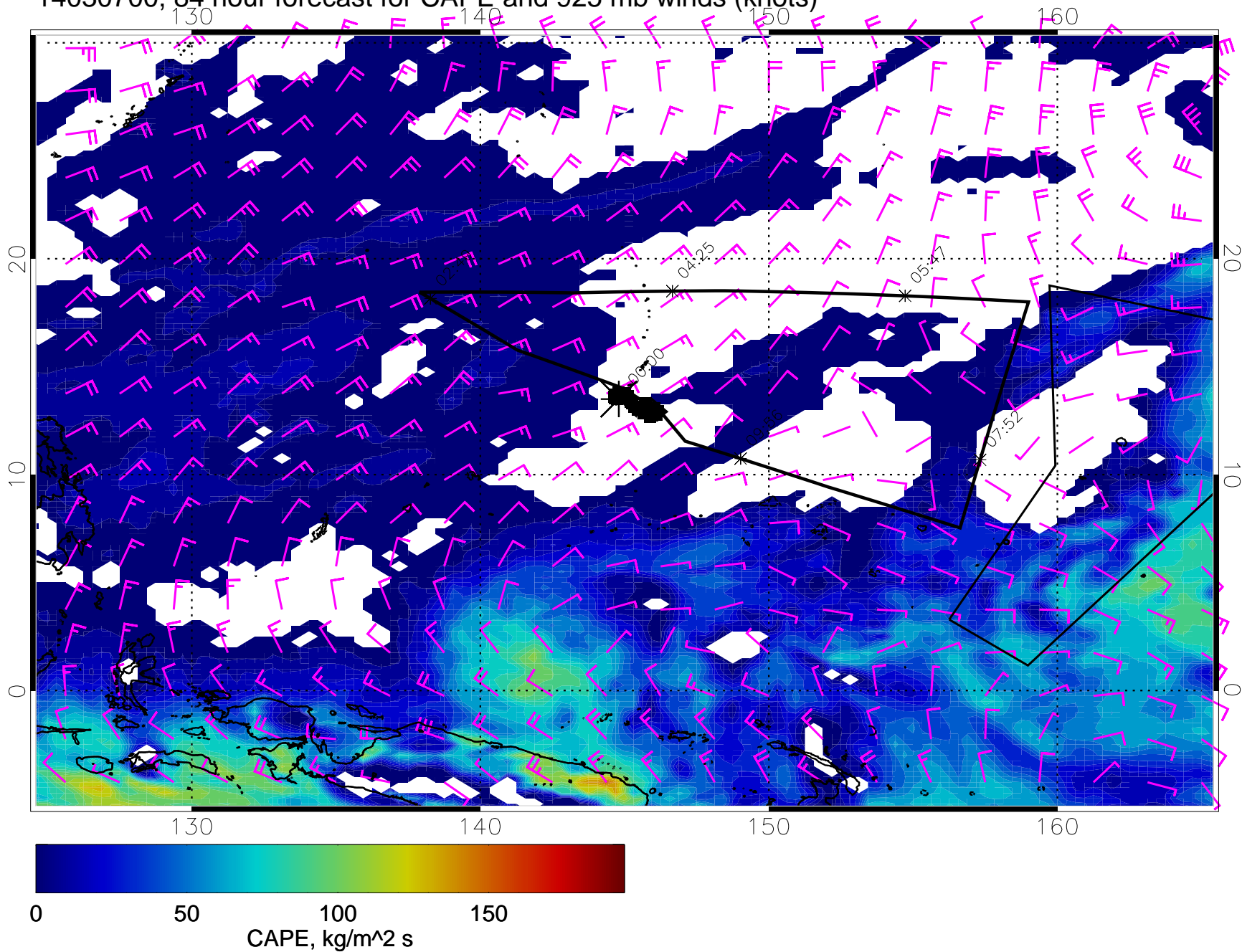
14030700, 84 hour forecast for CAPE and 925 mb winds (knots)
