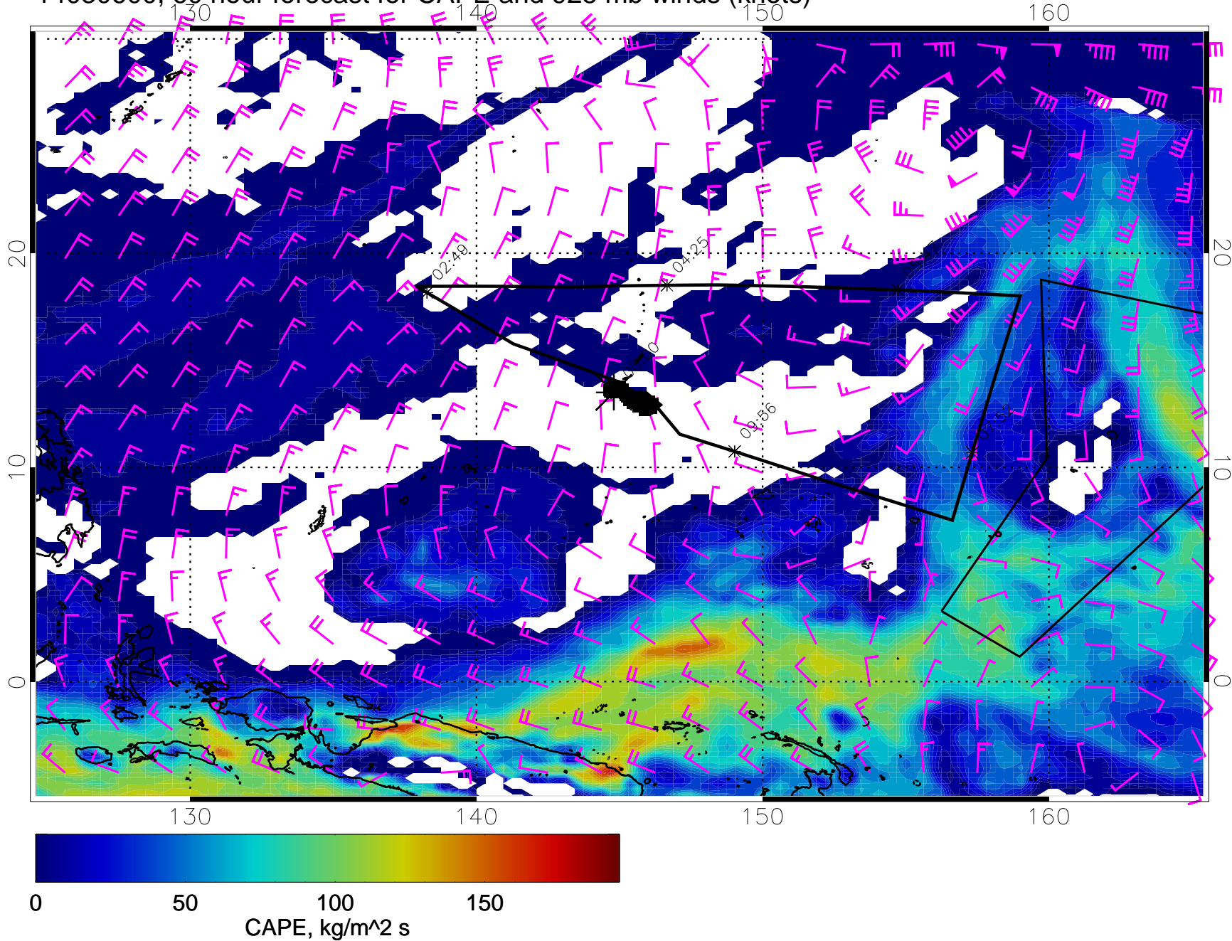
14030600, 60 hour forecast for CAPE and 925 mb winds (knots)
