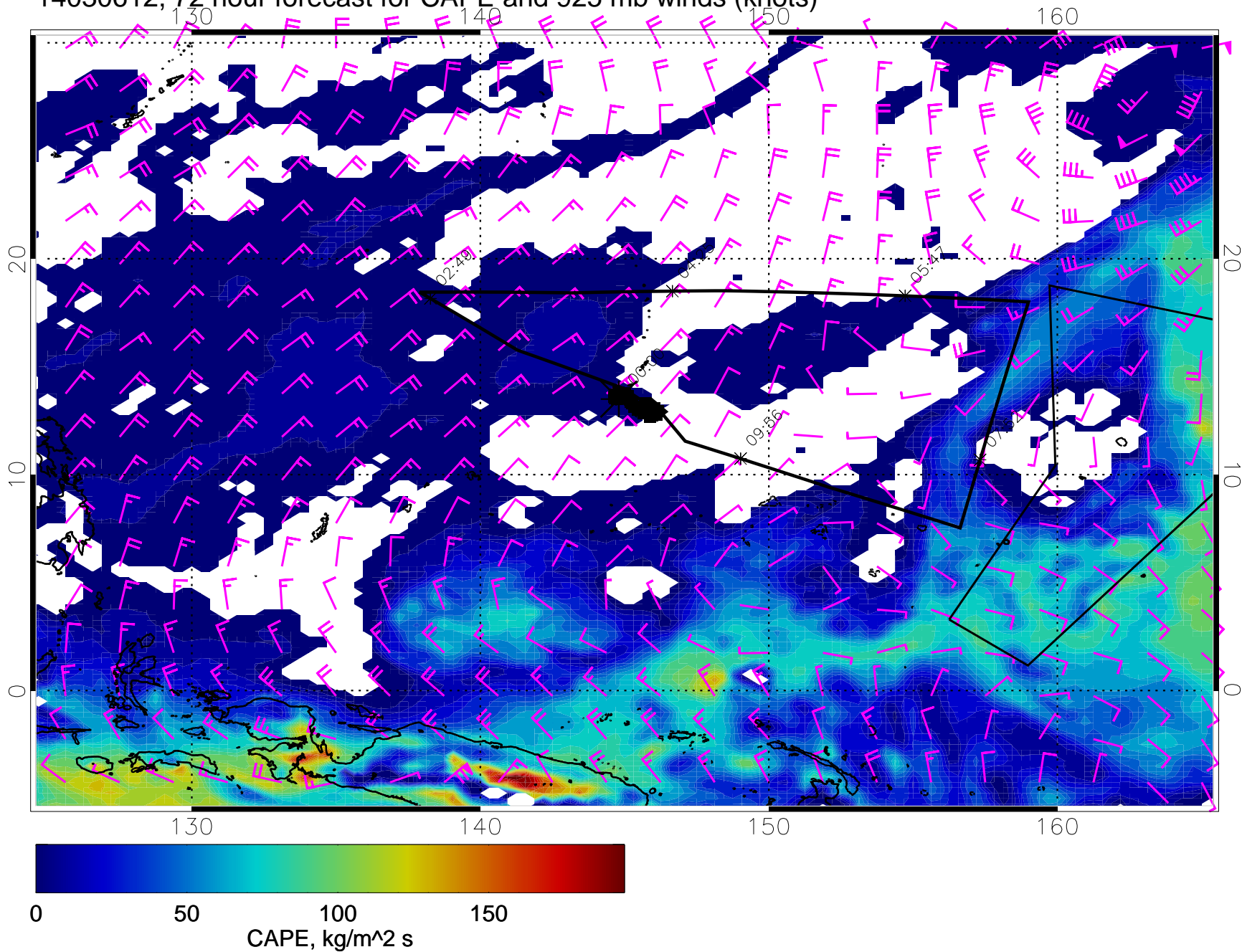
14030612, 72 hour forecast for CAPE and 925 mb winds (knots)
