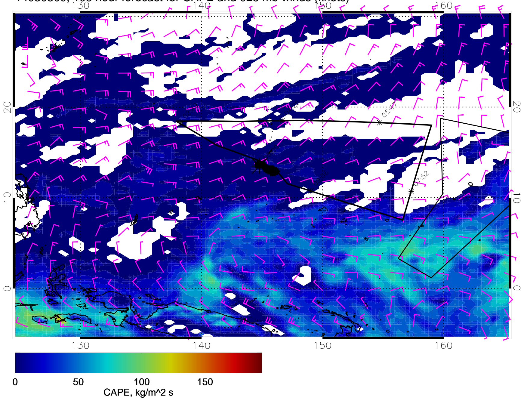
14030800, 108 hour forecast for CAPE and 925 mb winds (knots)
