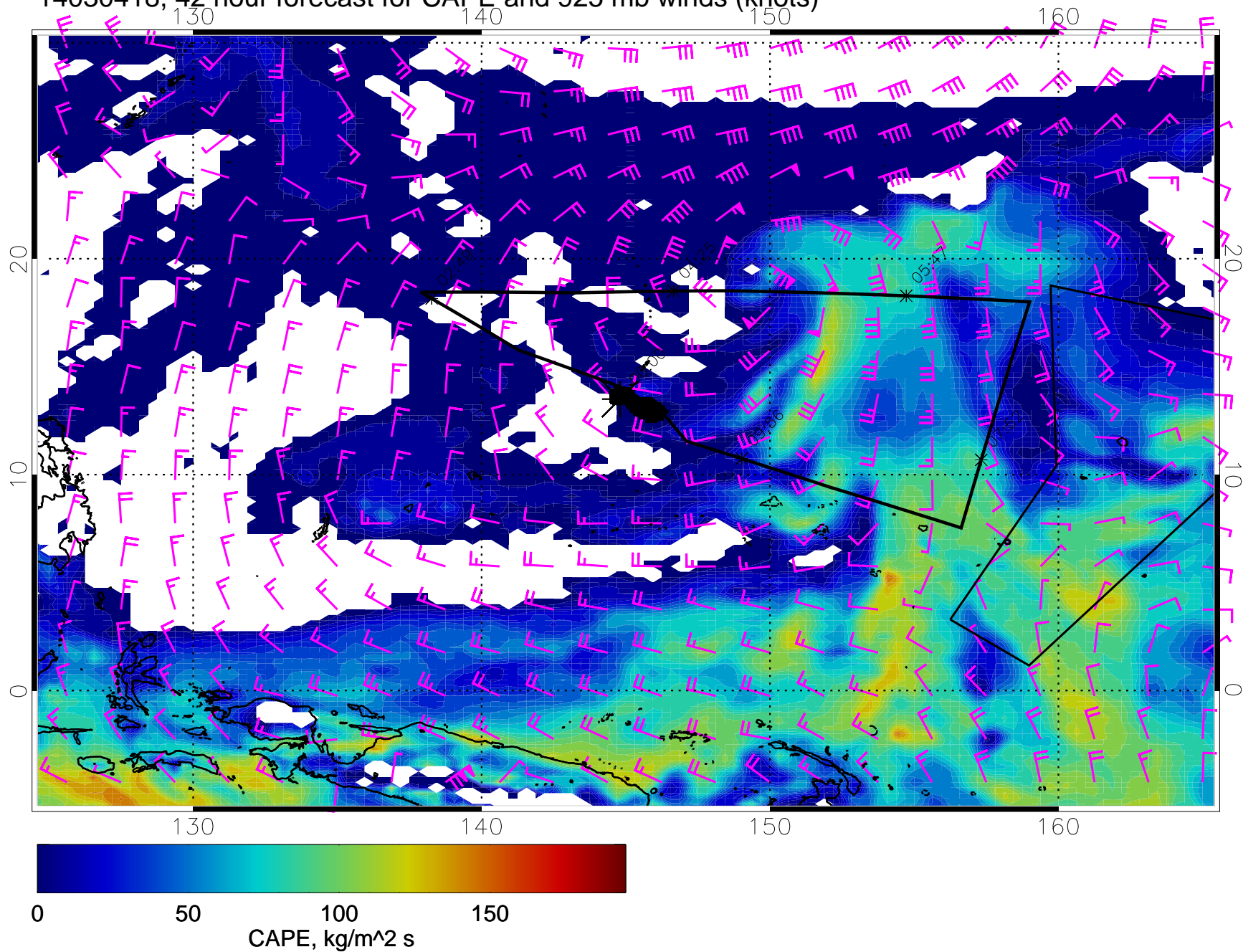
14030418, 42 hour forecast for CAPE and 925 mb winds (knots)
