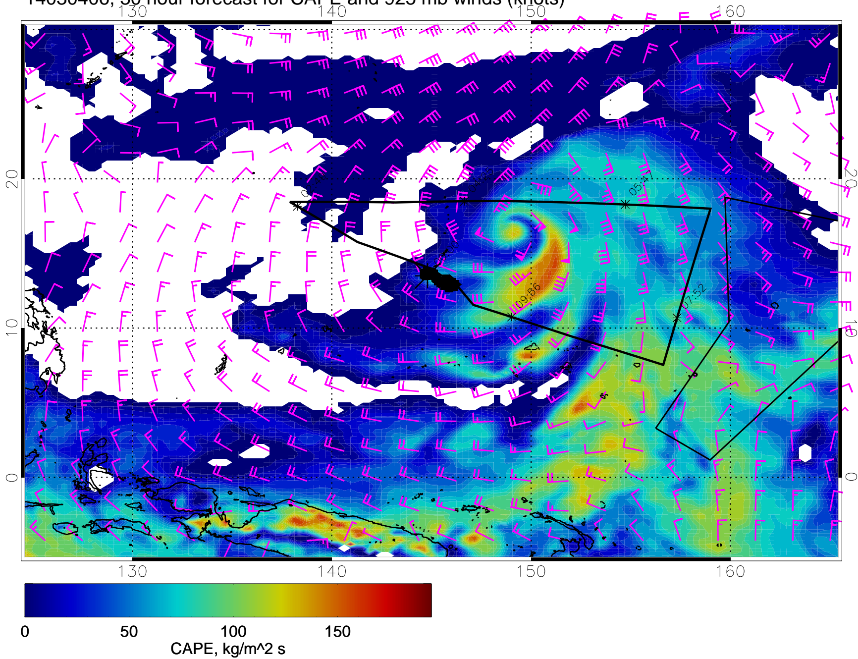
14030406, 30 hour forecast for CAPE and 925 mb winds (knots)
