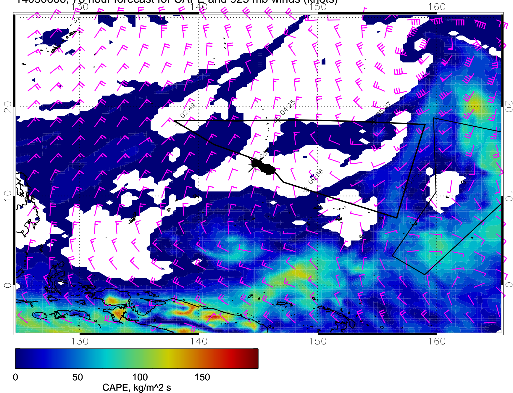
14030606, 78 hour forecast for CAPE and 925 mb winds (knots)
