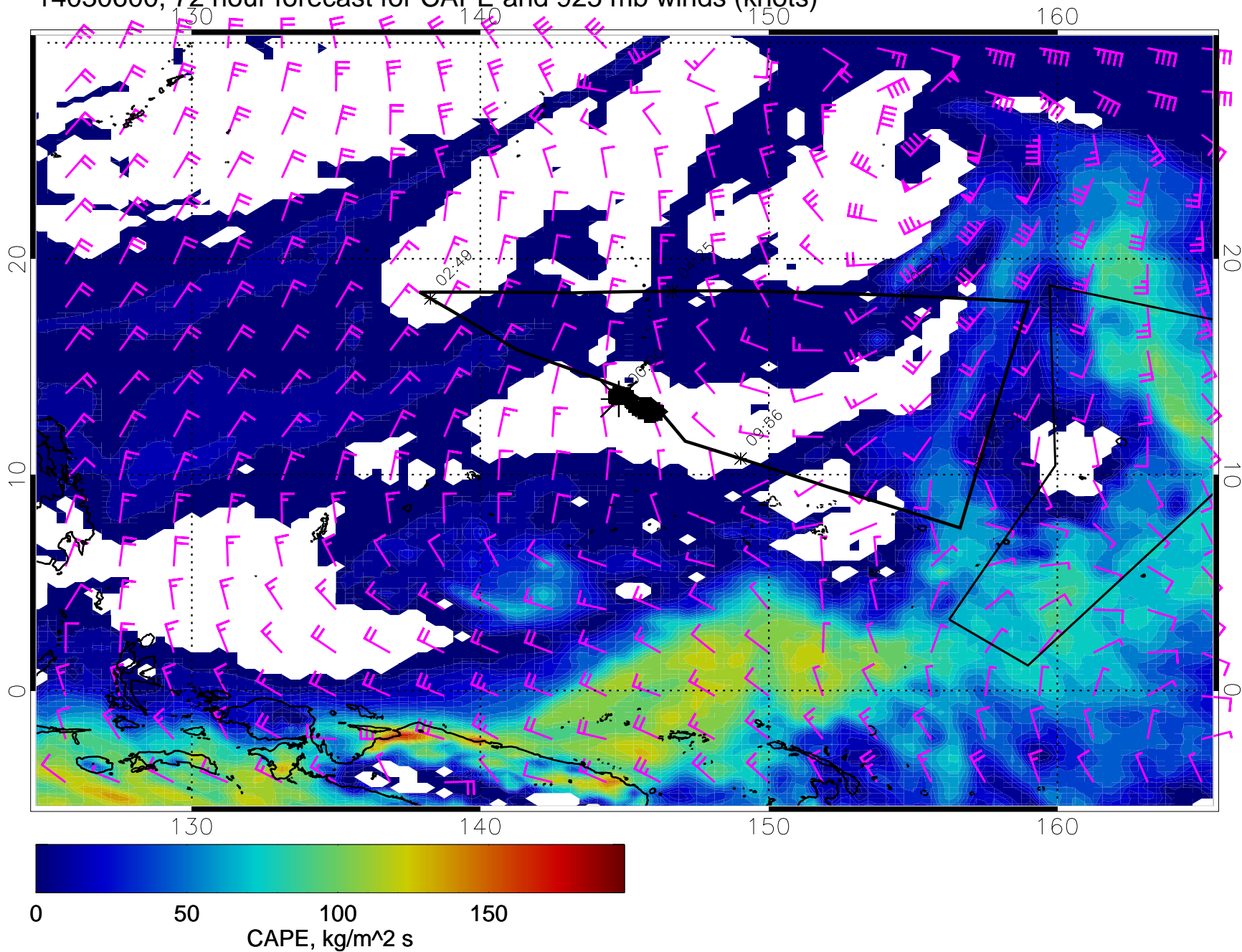
14030600, 72 hour forecast for CAPE and 925 mb winds (knots)
