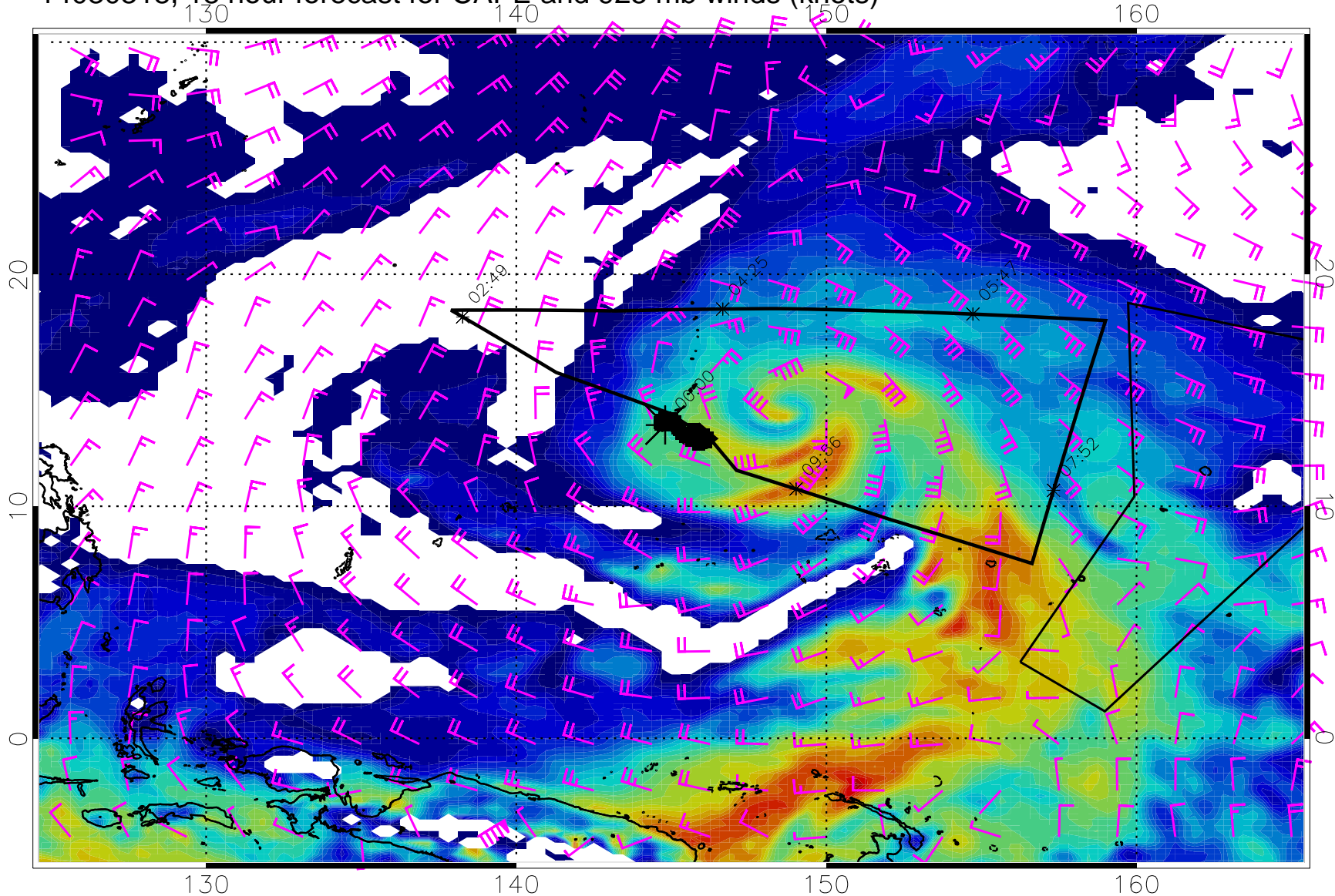
14030318, 18 hour forecast for CAPE and 925 mb winds (knots)
