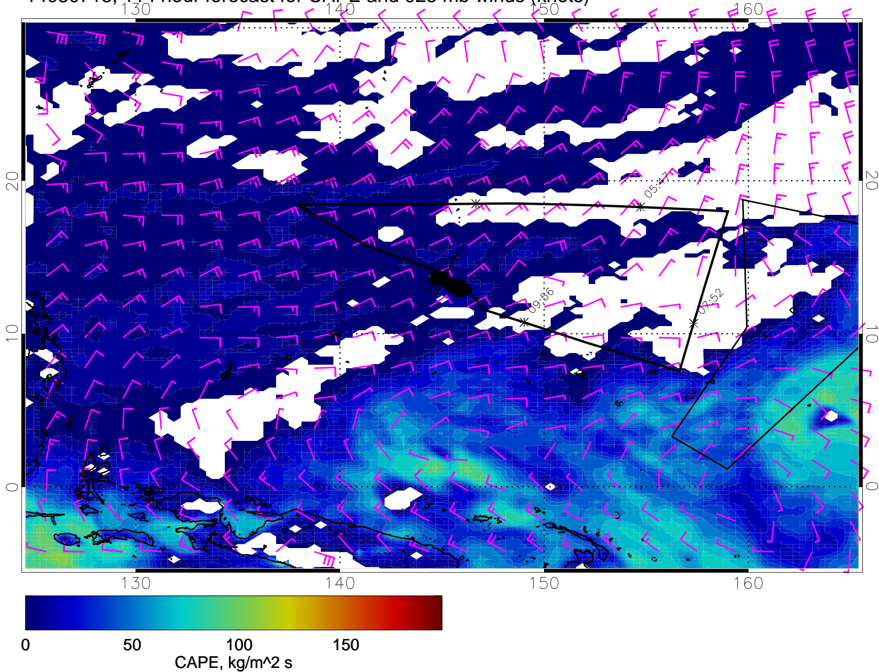
14030718, 114 hour forecast for CAPE and 925 mb winds (knots)
