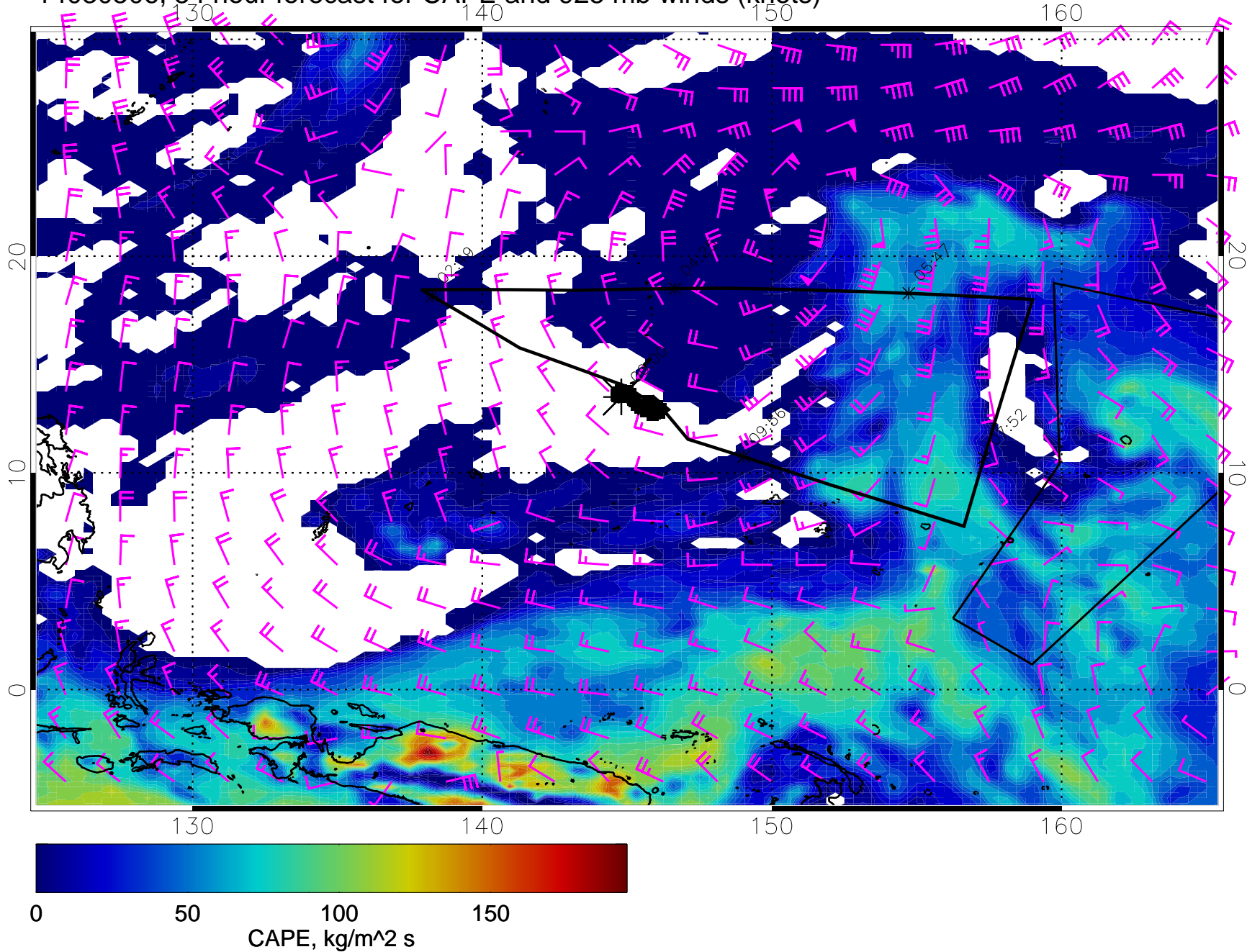
14030506, 54 hour forecast for CAPE and 925 mb winds (knots)
