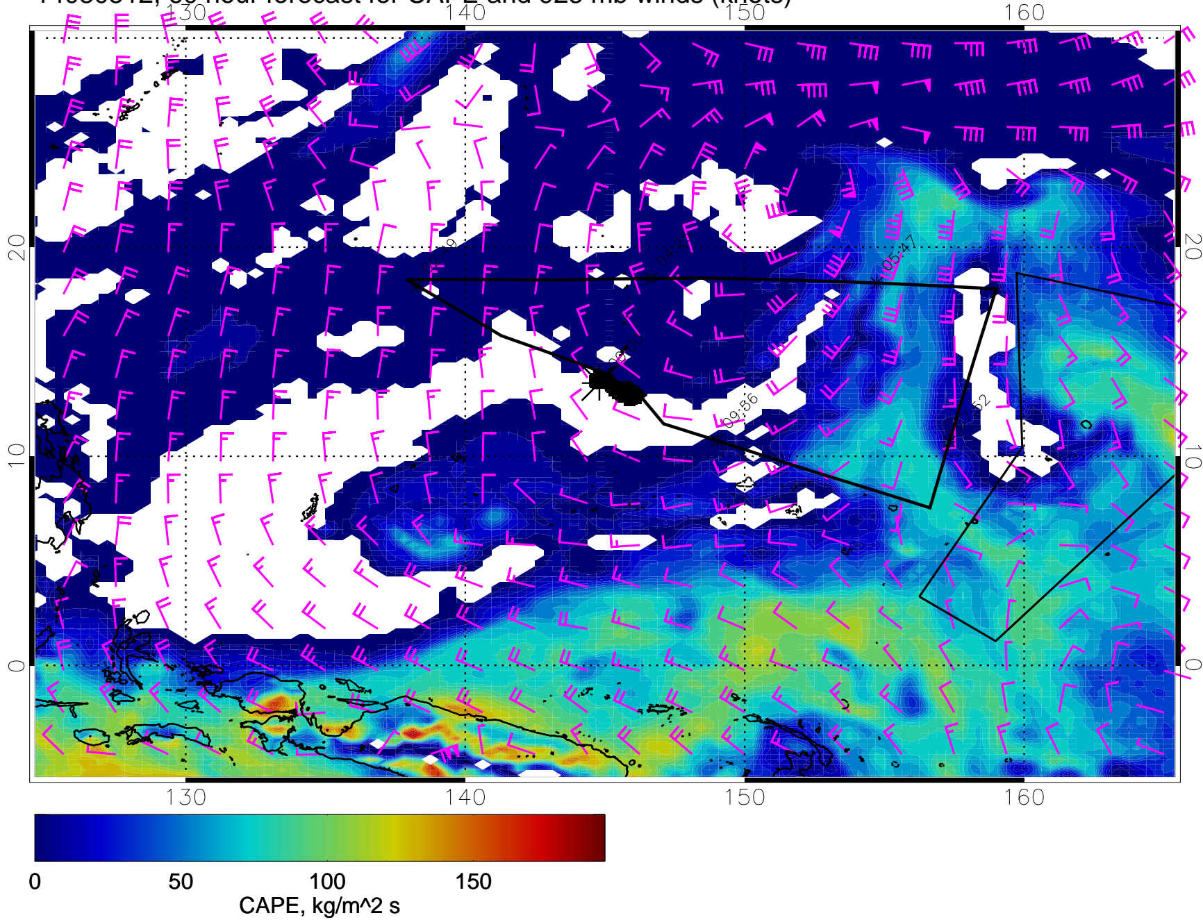
14030512, 60 hour forecast for CAPE and 925 mb winds (knots)
