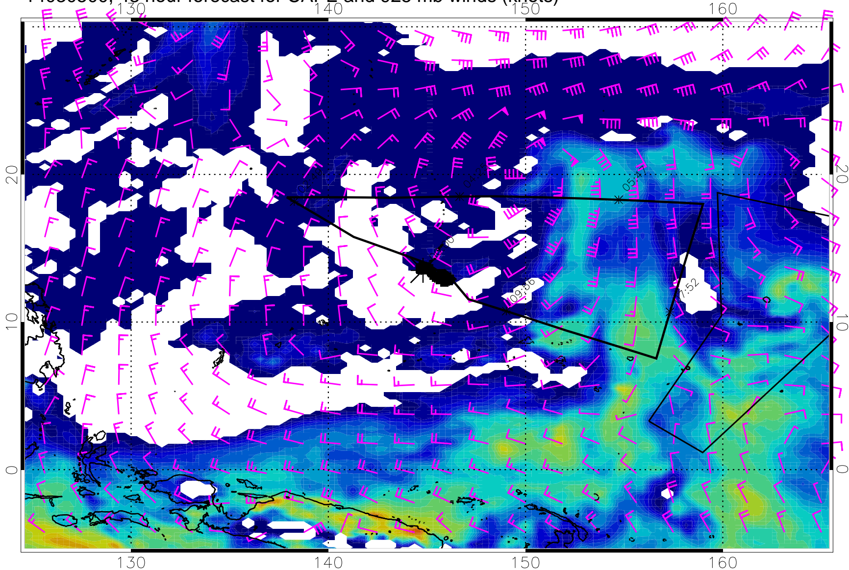
14030500, 48 hour forecast for CAPE and 925 mb winds (knots)
