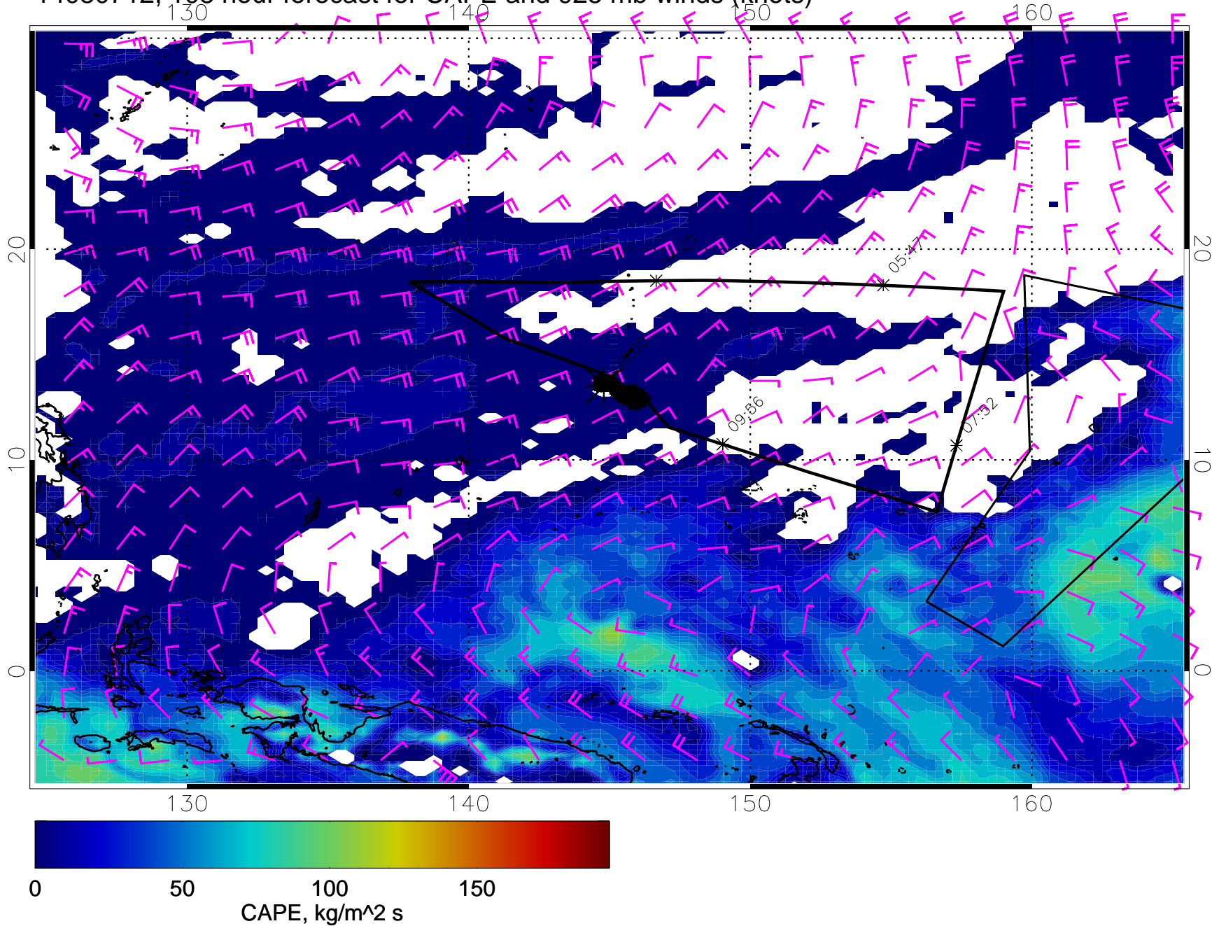
14030712, 108 hour forecast for CAPE and 925 mb winds (knots)
