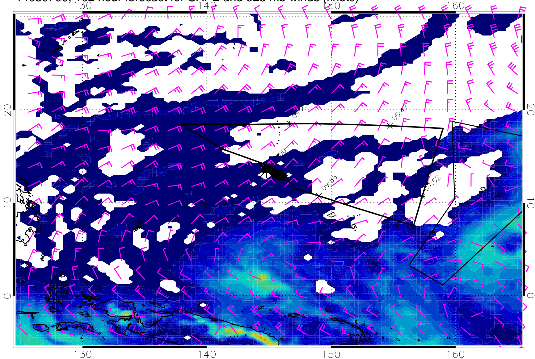
14030706, 102 hour forecast for CAPE and 925 mb winds (knots)
