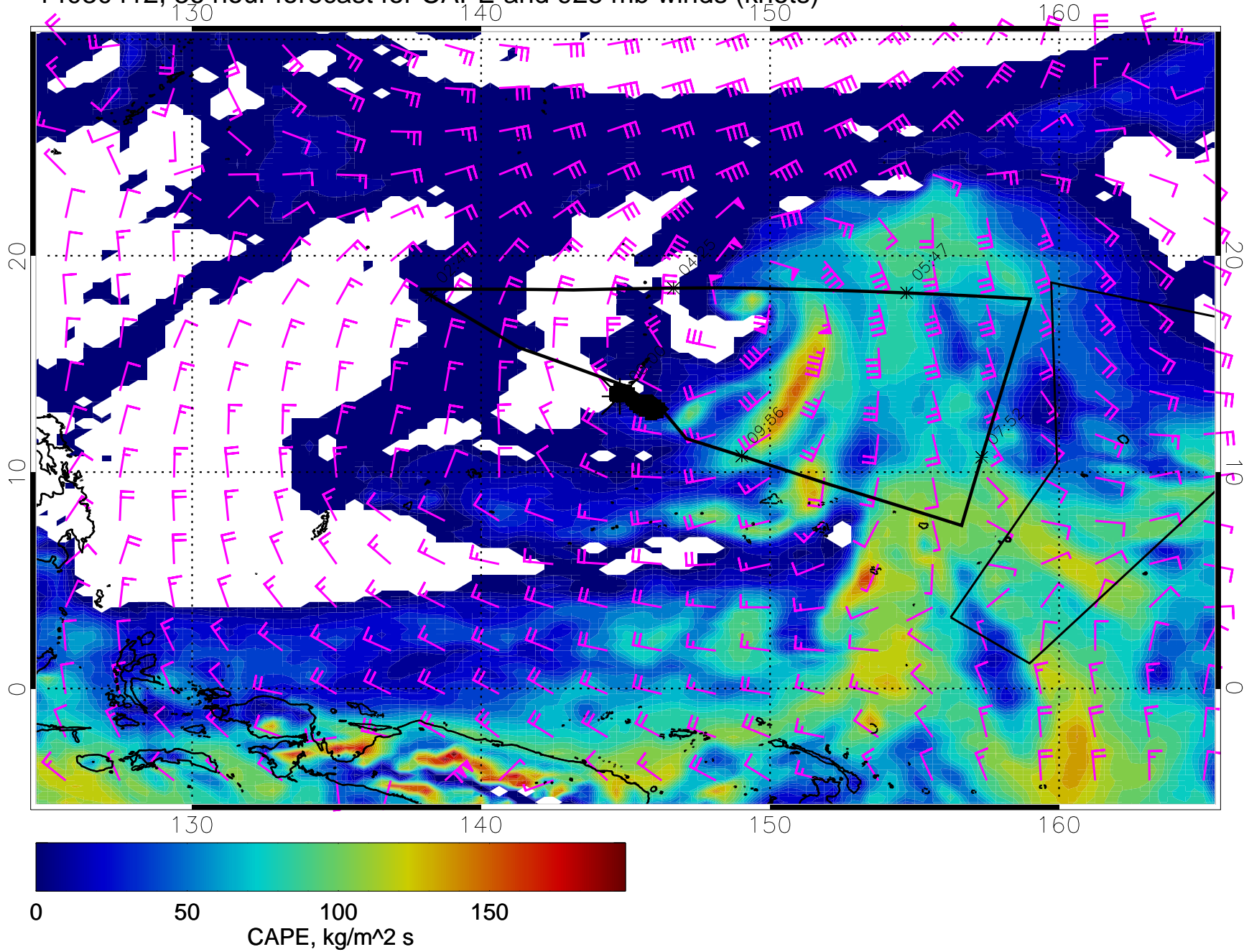
14030412, 36 hour forecast for CAPE and 925 mb winds (knots)
