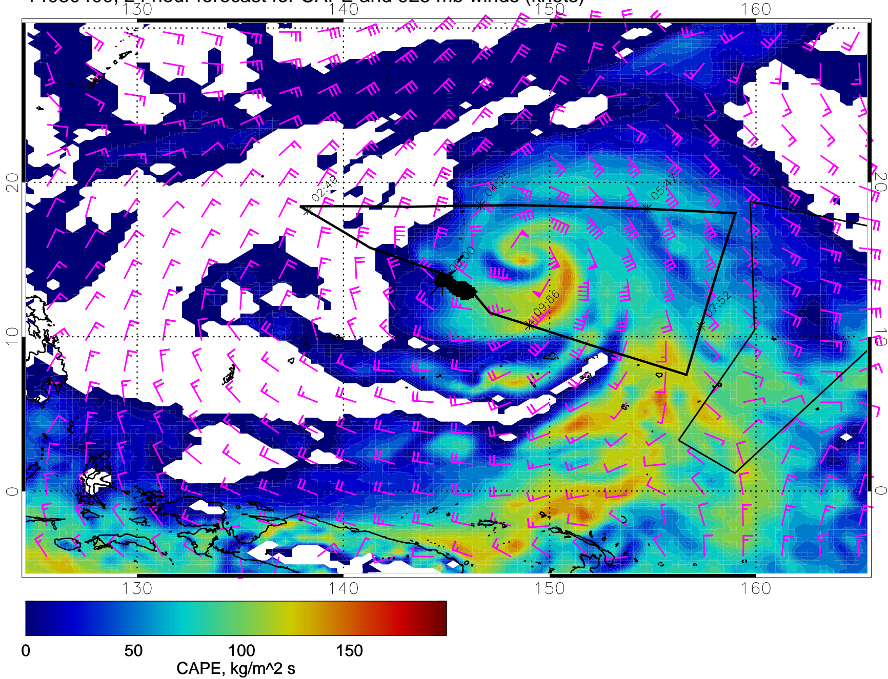
14030400, 24 hour forecast for CAPE and 925 mb winds (knots)
