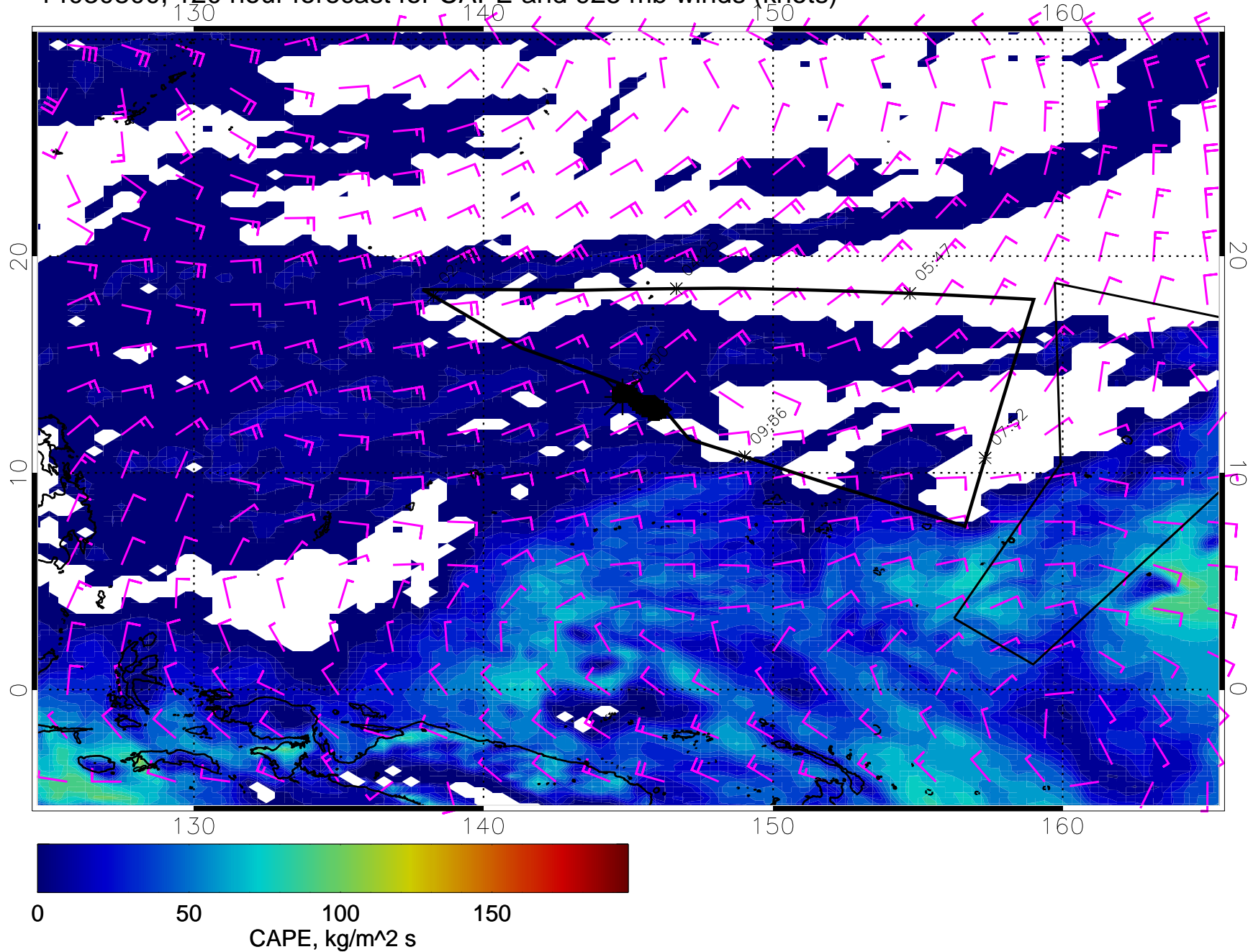
14030800, 120 hour forecast for CAPE and 925 mb winds (knots)
