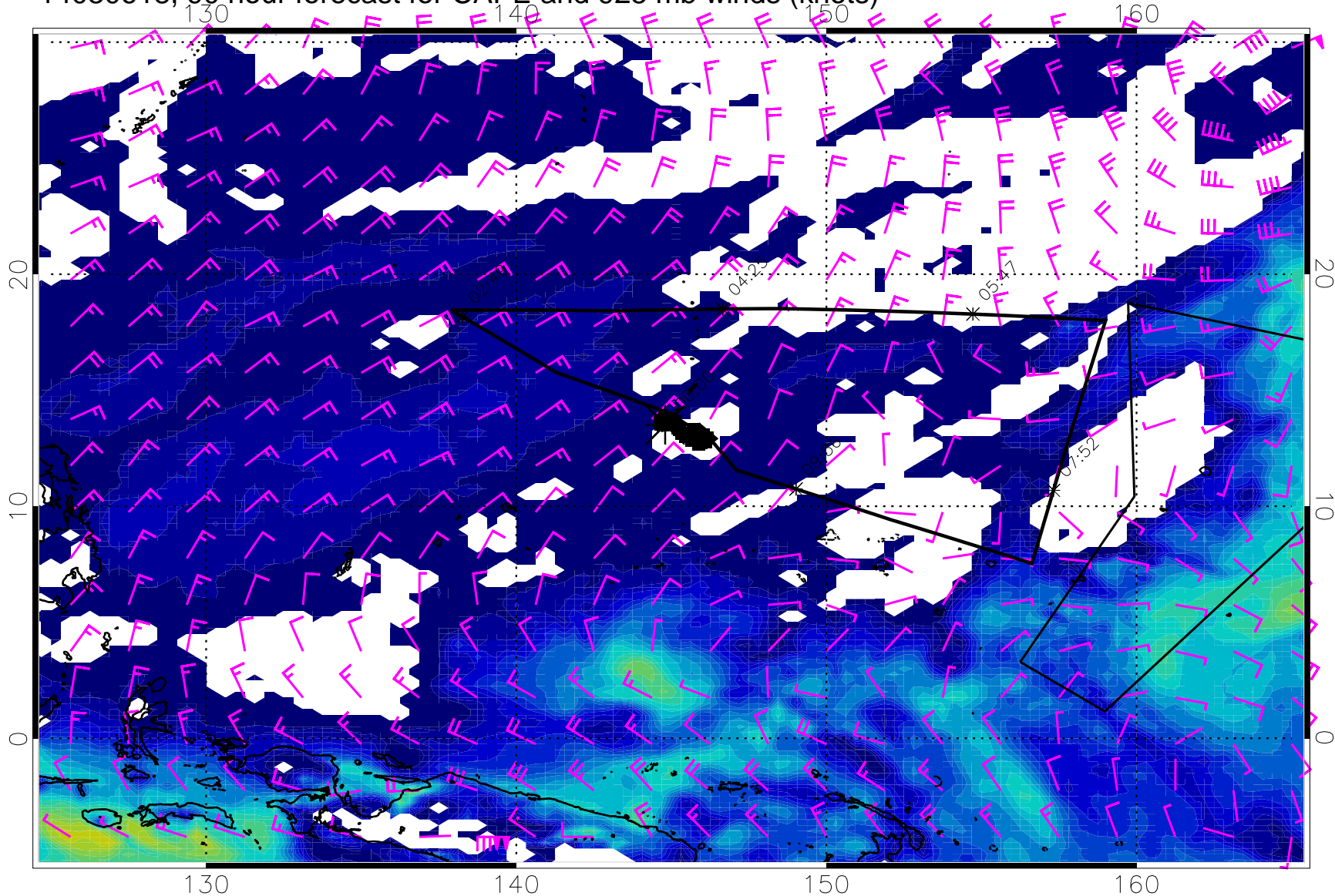
14030618, 90 hour forecast for CAPE and 925 mb winds (knots)
