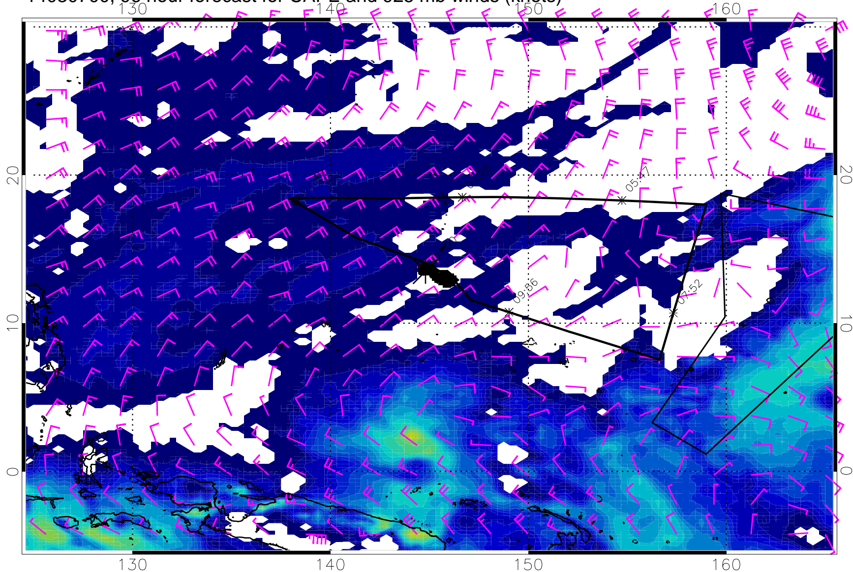
14030700, 96 hour forecast for CAPE and 925 mb winds (knots)
