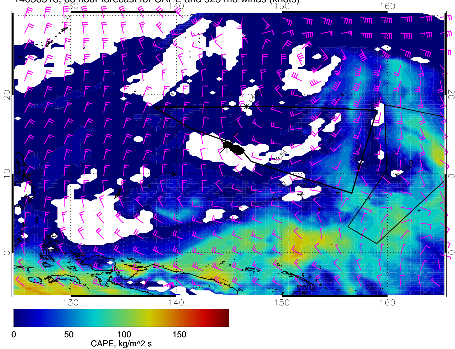
14030518, 66 hour forecast for CAPE and 925 mb winds (knots)
