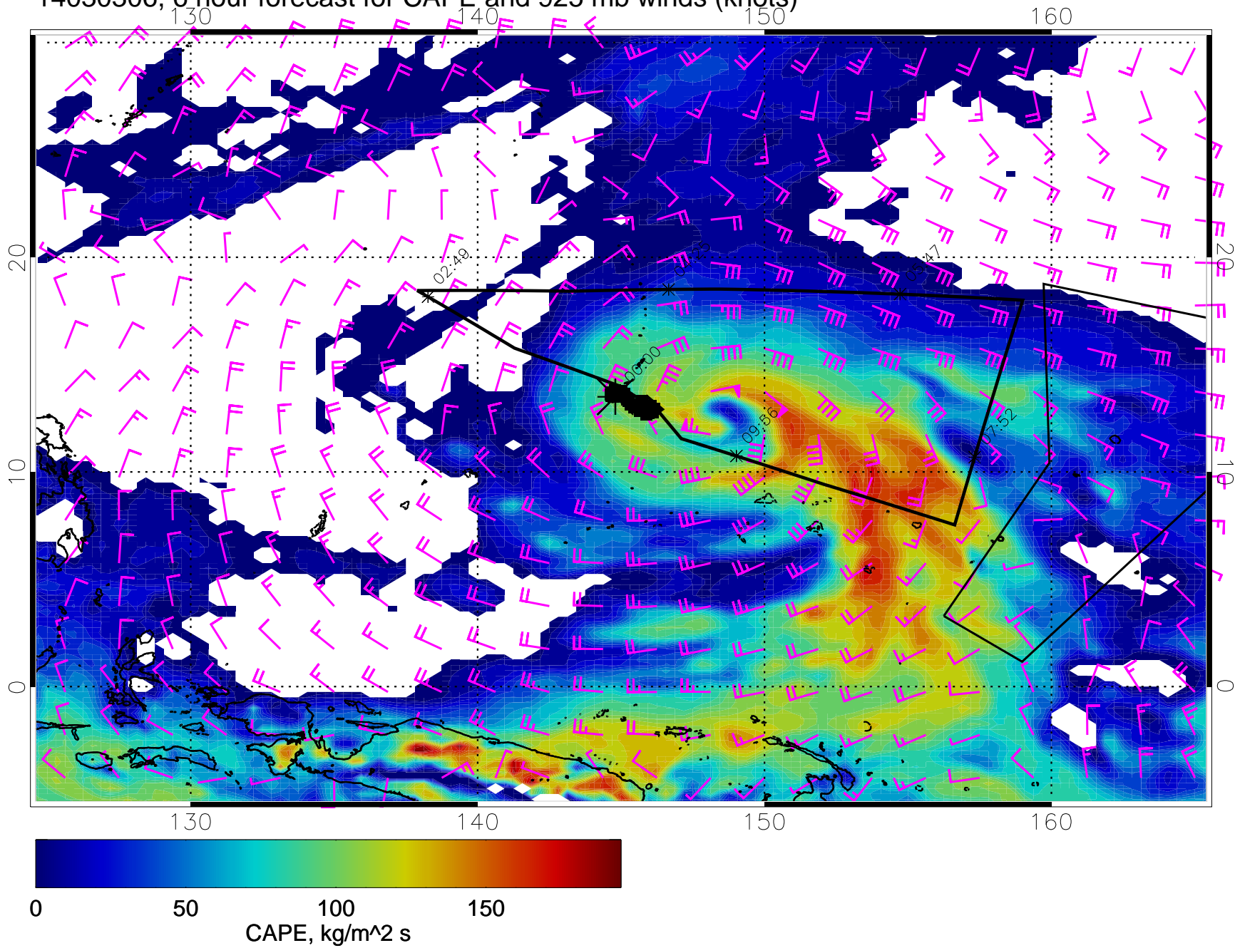
14030306, 6 hour forecast for CAPE and 925 mb winds (knots)
