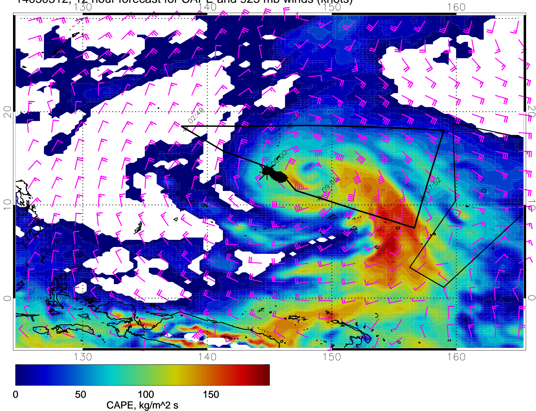
14030312, 12 hour forecast for CAPE and 925 mb winds (knots)
