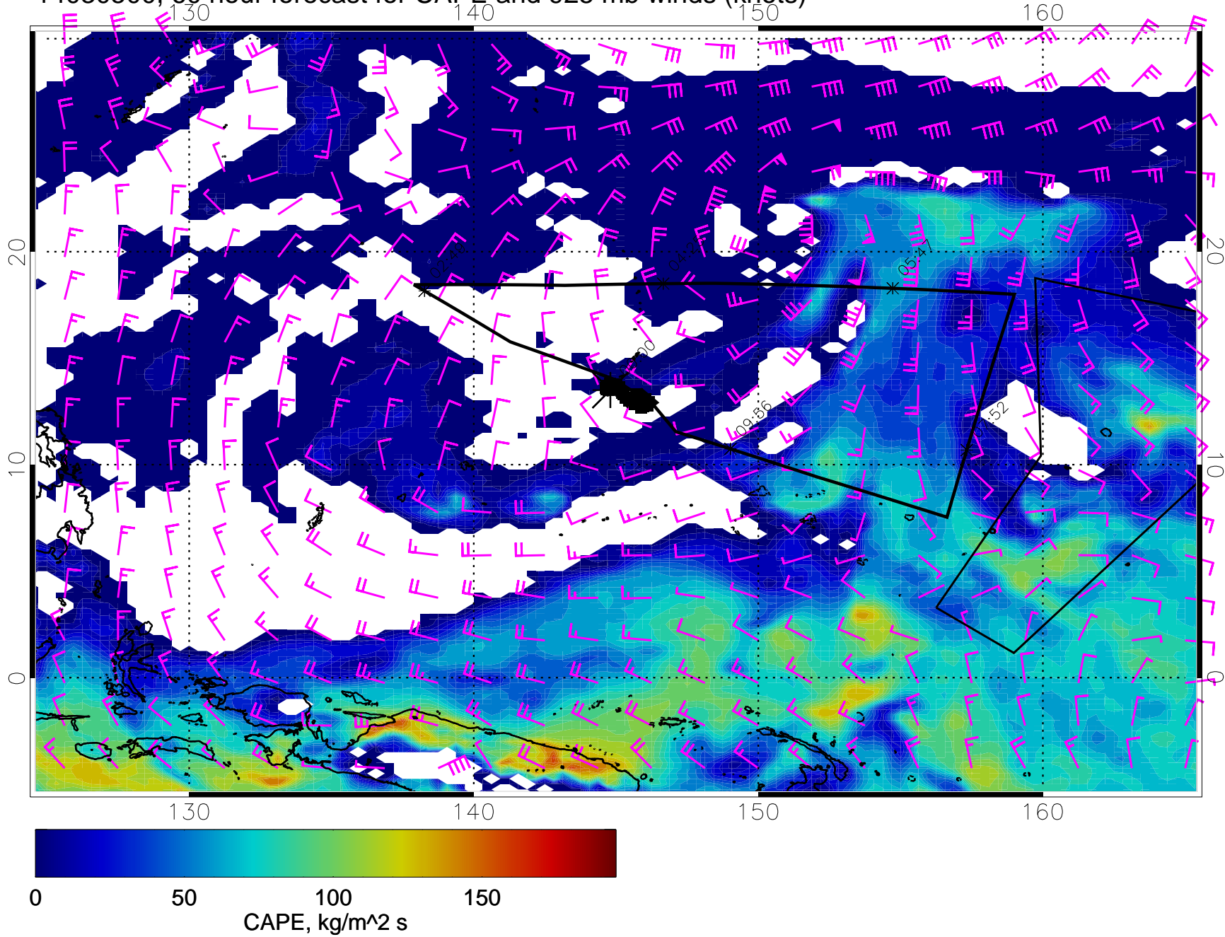
14030500, 60 hour forecast for CAPE and 925 mb winds (knots)
