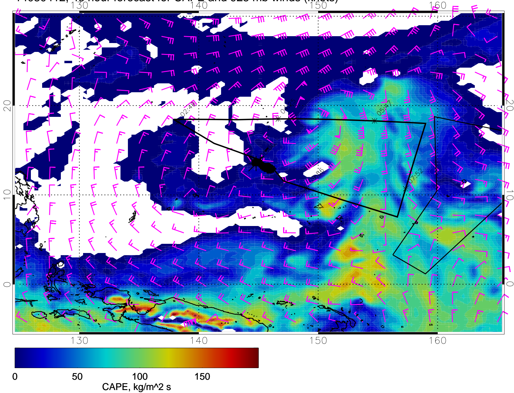
14030412, 48 hour forecast for CAPE and 925 mb winds (knots)
