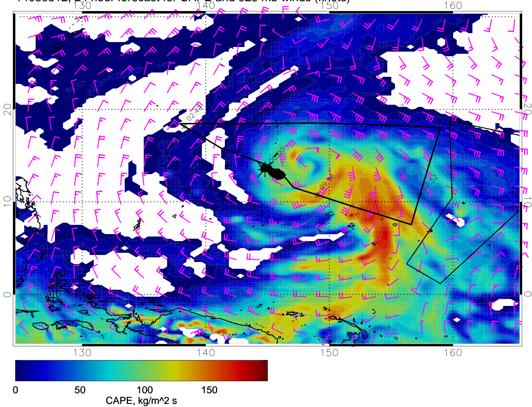
14030312, 24 hour forecast for CAPE and 925 mb winds (knots)
