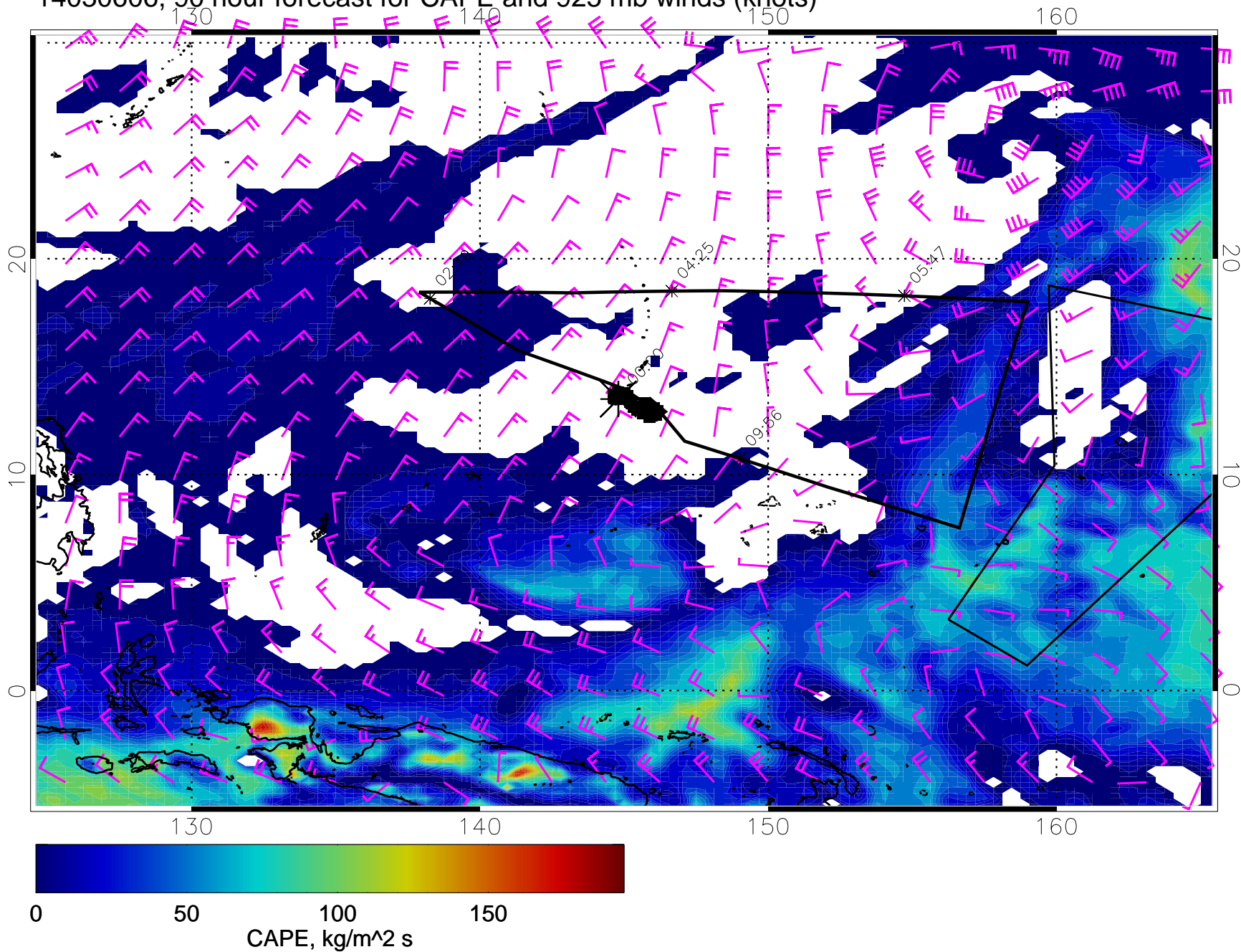
14030606, 90 hour forecast for CAPE and 925 mb winds (knots)
