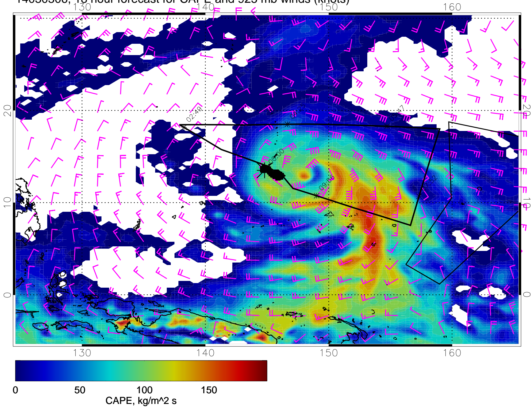
14030306, 18 hour forecast for CAPE and 925 mb winds (knots)
