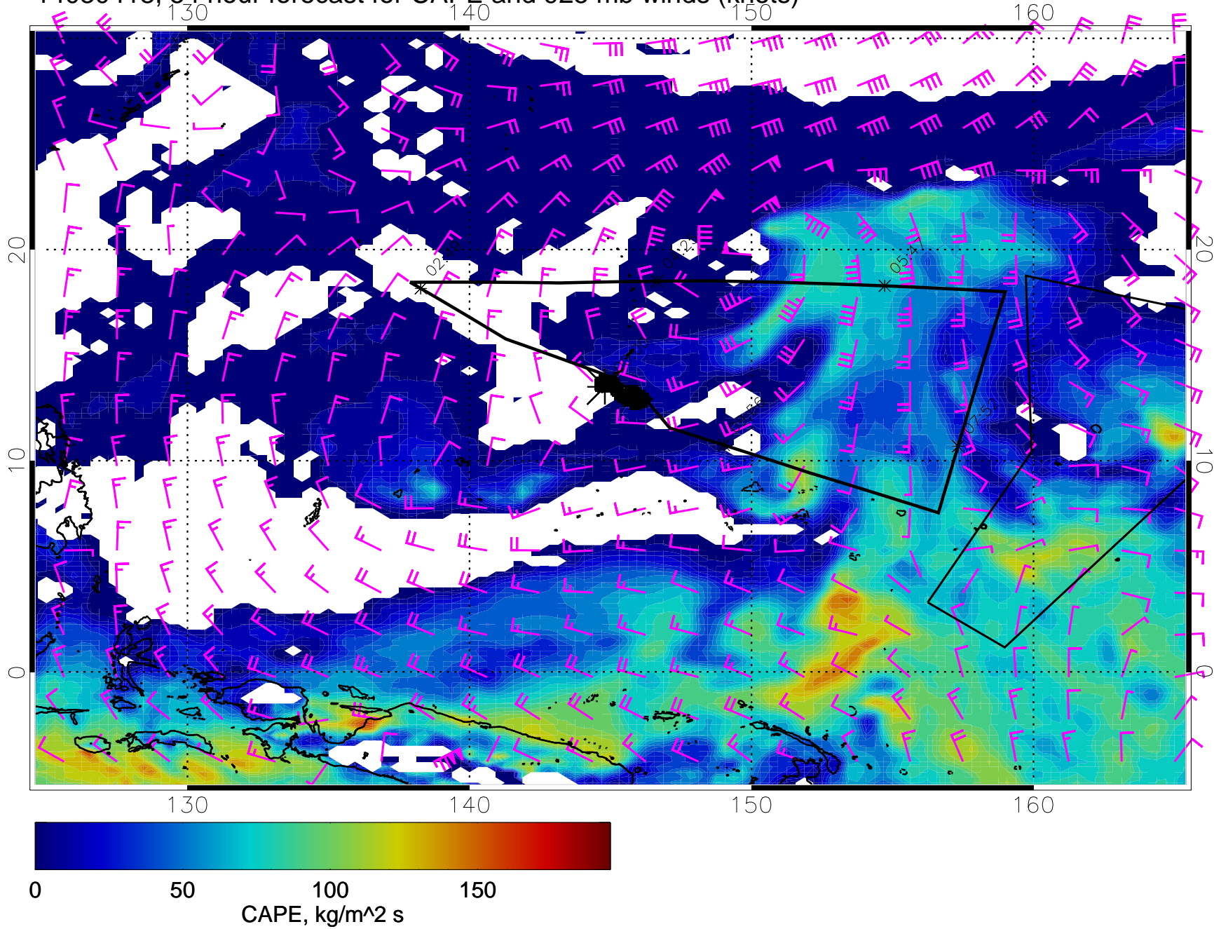
14030418, 54 hour forecast for CAPE and 925 mb winds (knots)
