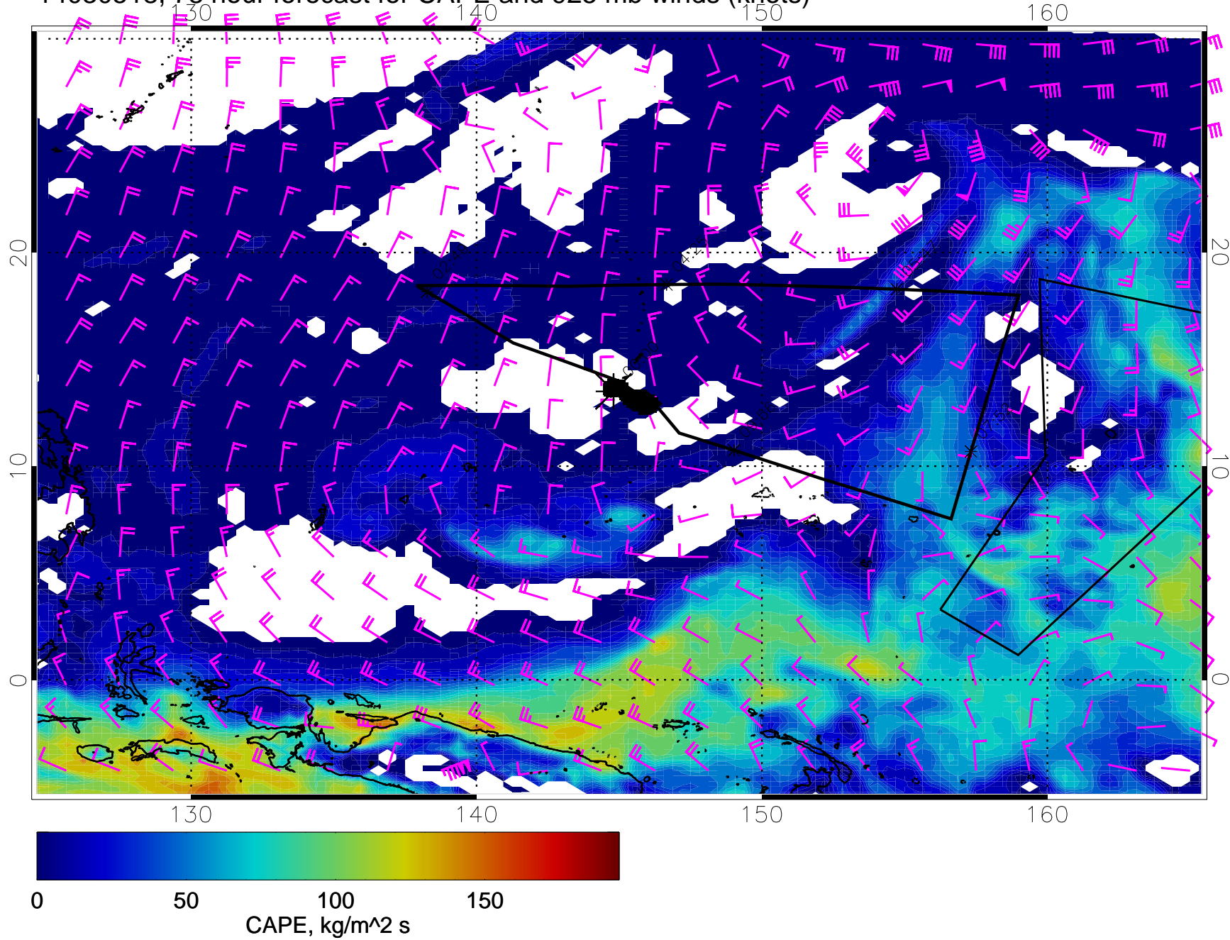
14030518, 78 hour forecast for CAPE and 925 mb winds (knots)
