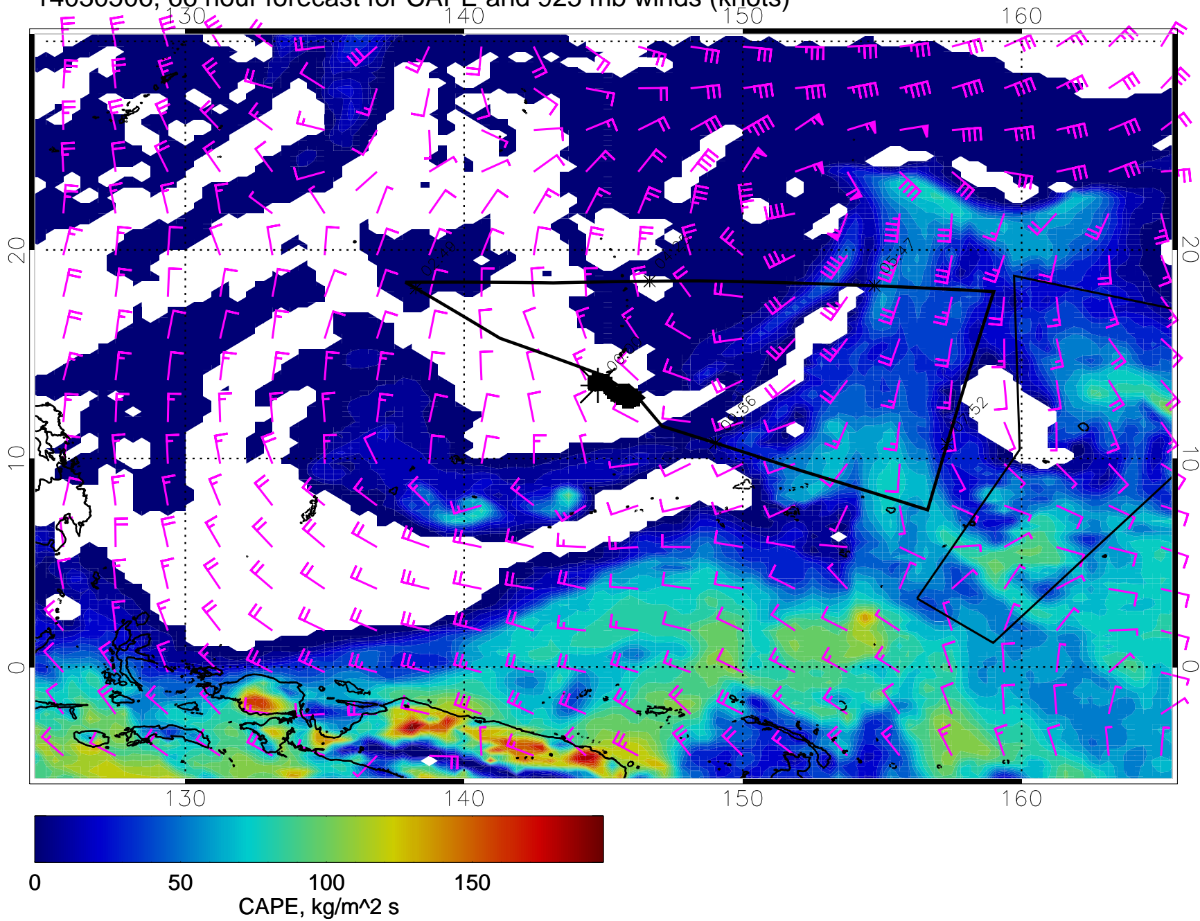
14030506, 66 hour forecast for CAPE and 925 mb winds (knots)
