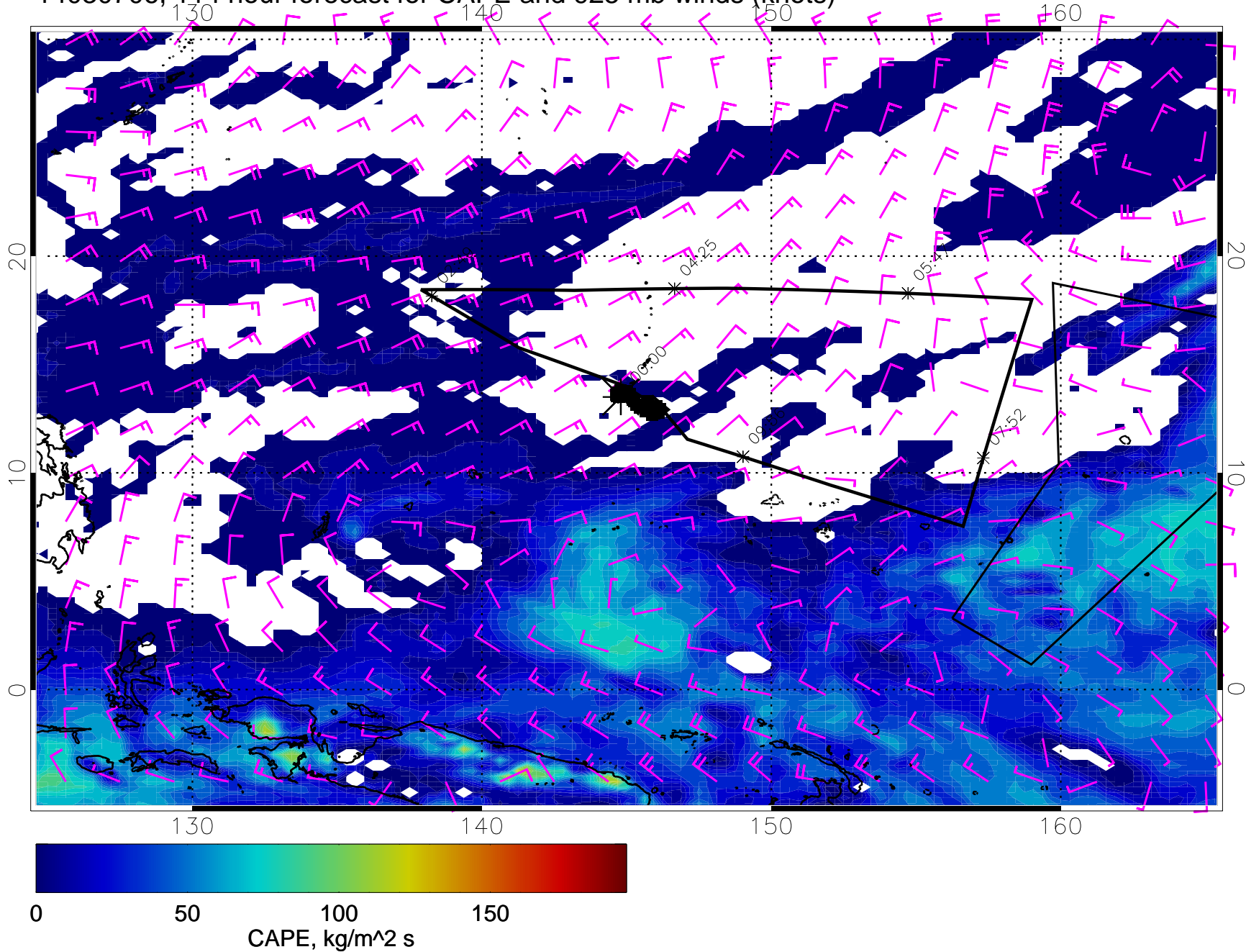
14030706, 114 hour forecast for CAPE and 925 mb winds (knots)
