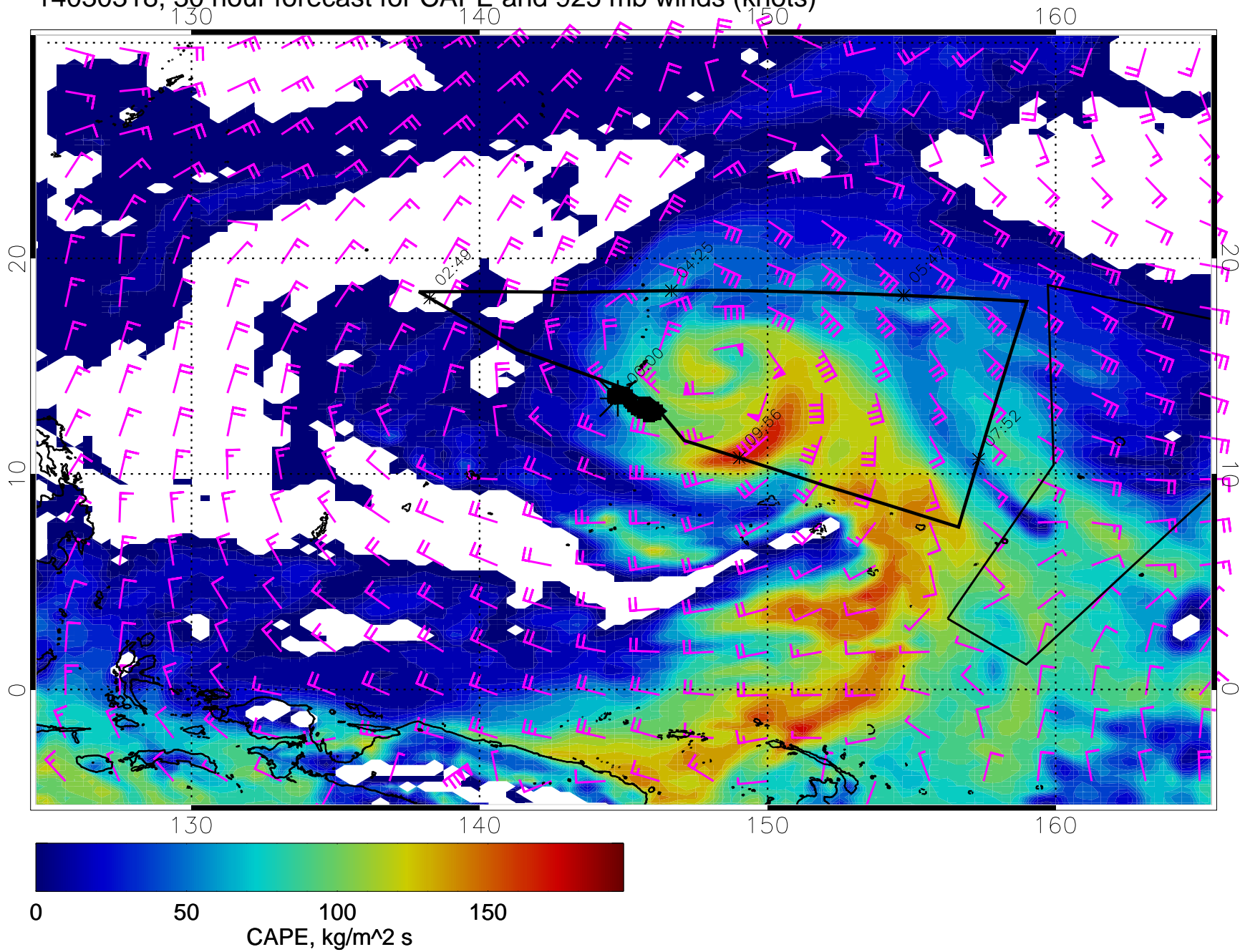
14030318, 30 hour forecast for CAPE and 925 mb winds (knots)
