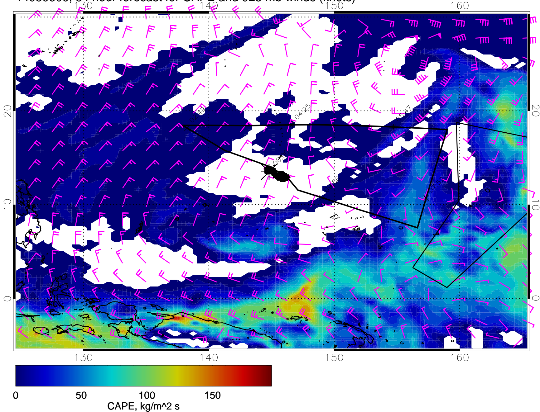
14030600, 84 hour forecast for CAPE and 925 mb winds (knots)
