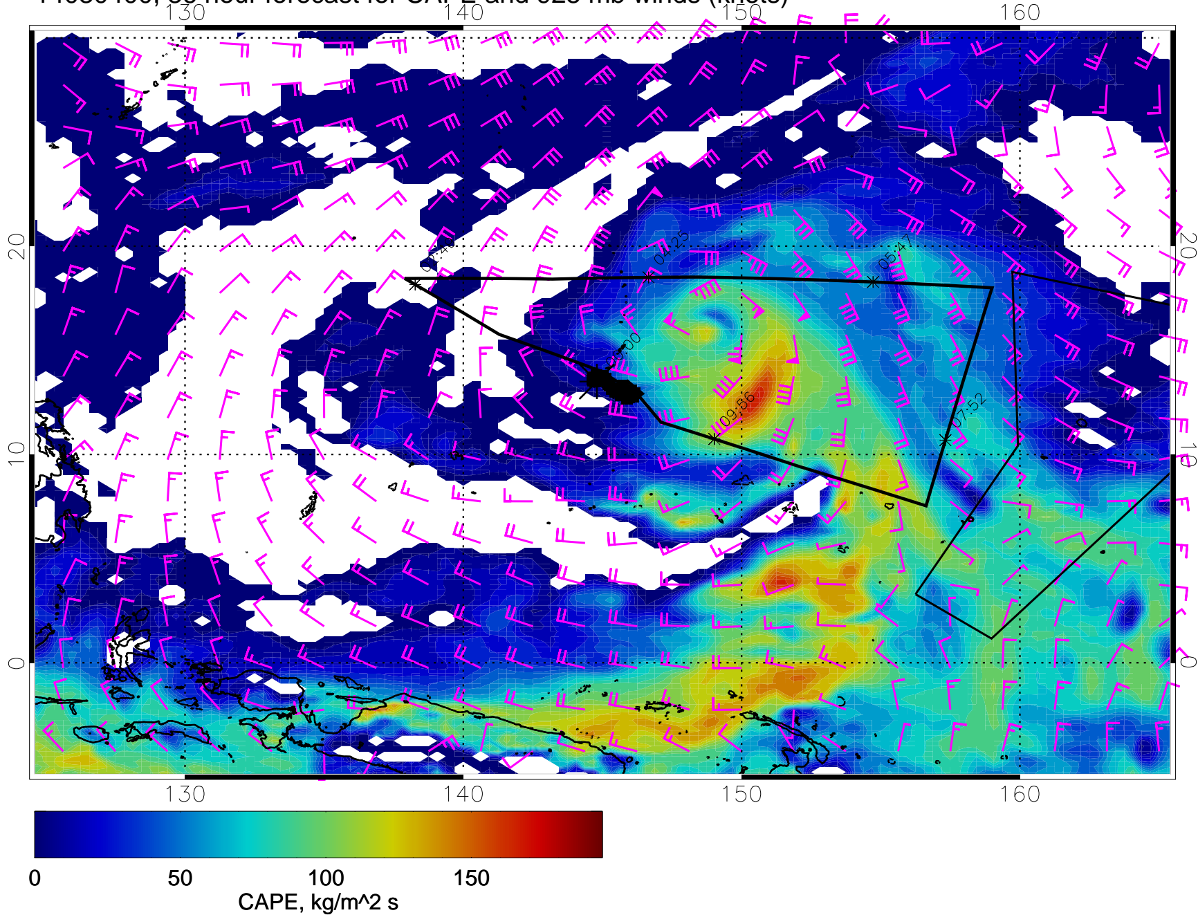
14030400, 36 hour forecast for CAPE and 925 mb winds (knots)
