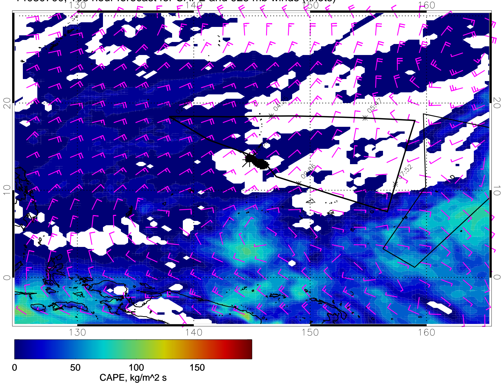
14030700, 108 hour forecast for CAPE and 925 mb winds (knots)
