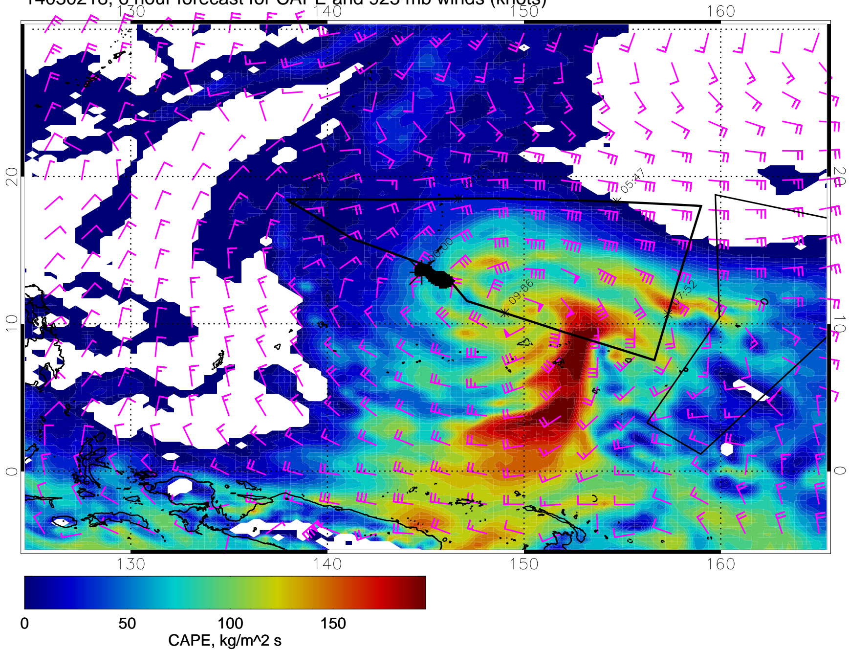
14030218, 6 hour forecast for CAPE and 925 mb winds (knots)
