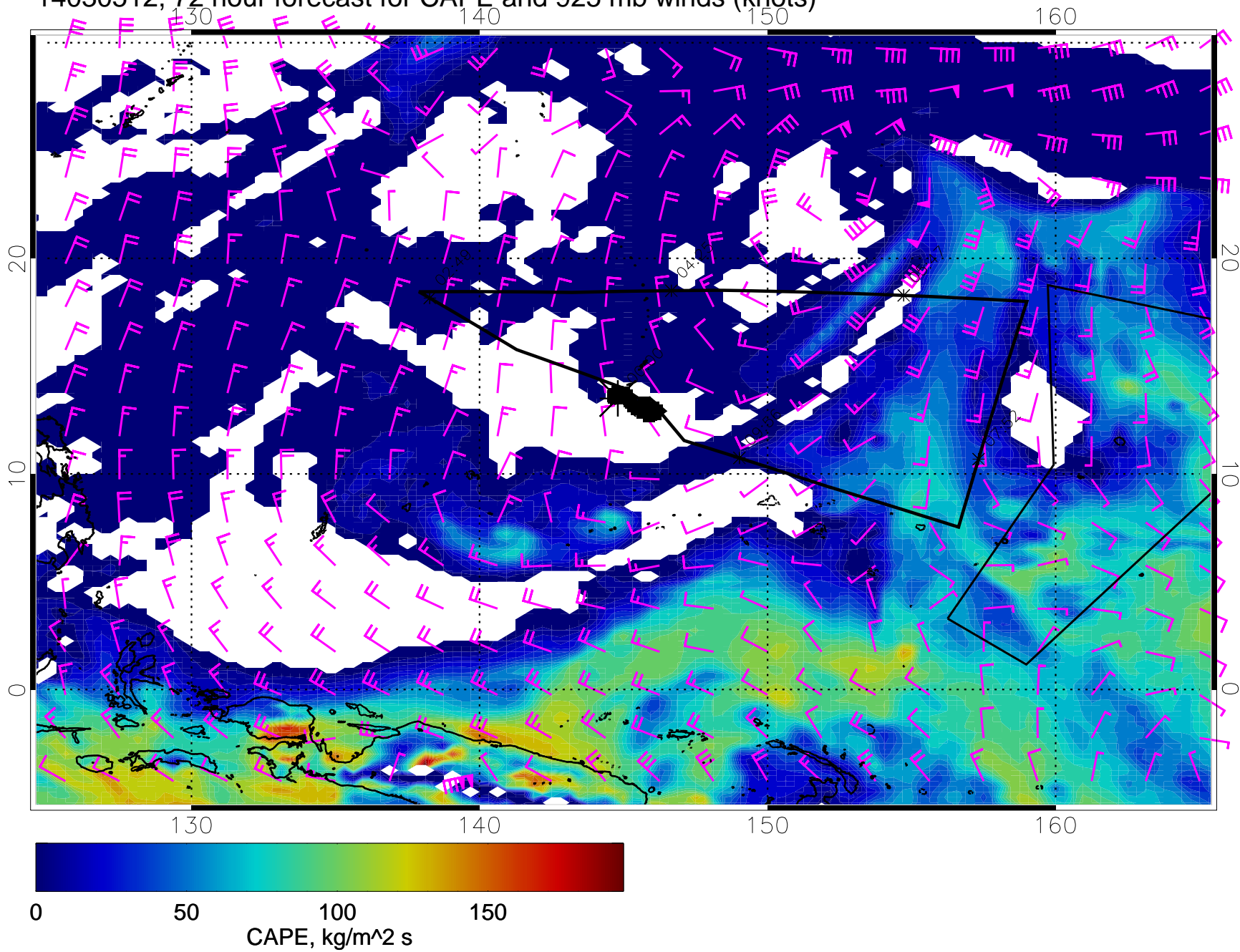
14030512, 72 hour forecast for CAPE and 925 mb winds (knots)
