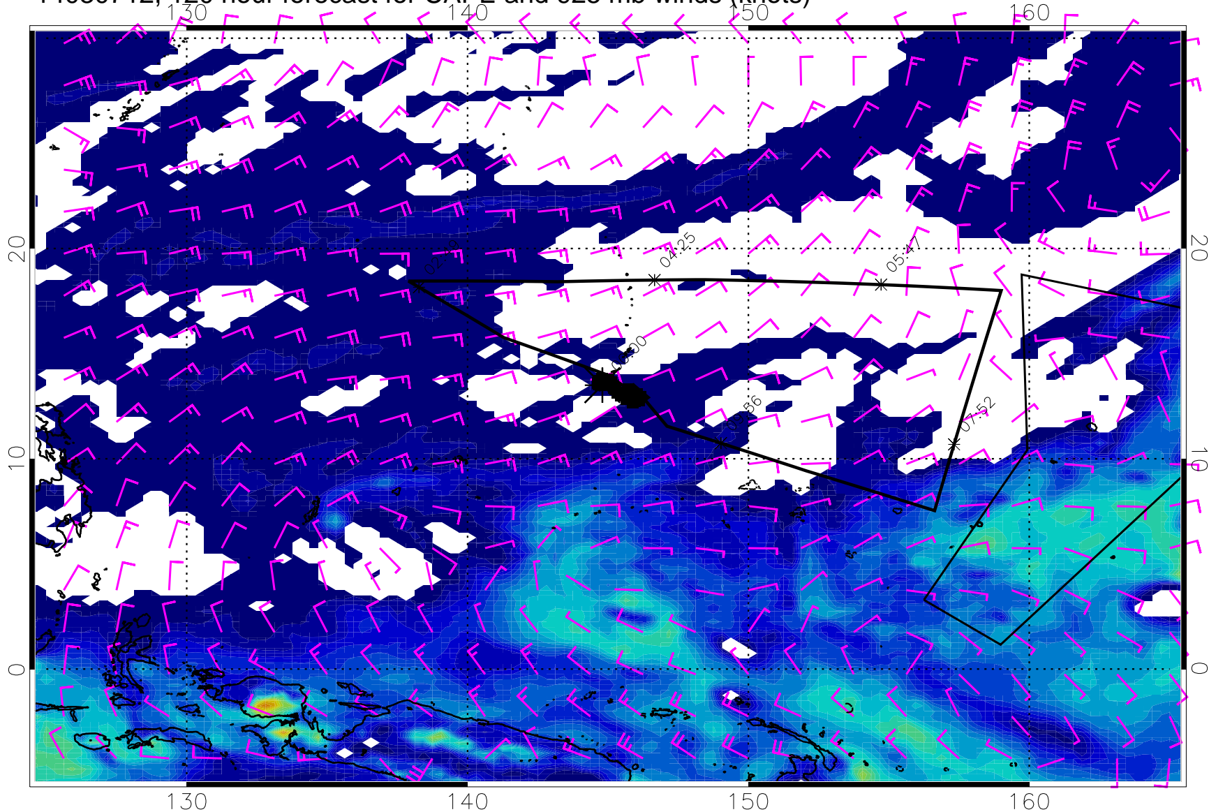
14030712, 120 hour forecast for CAPE and 925 mb winds (knots)
