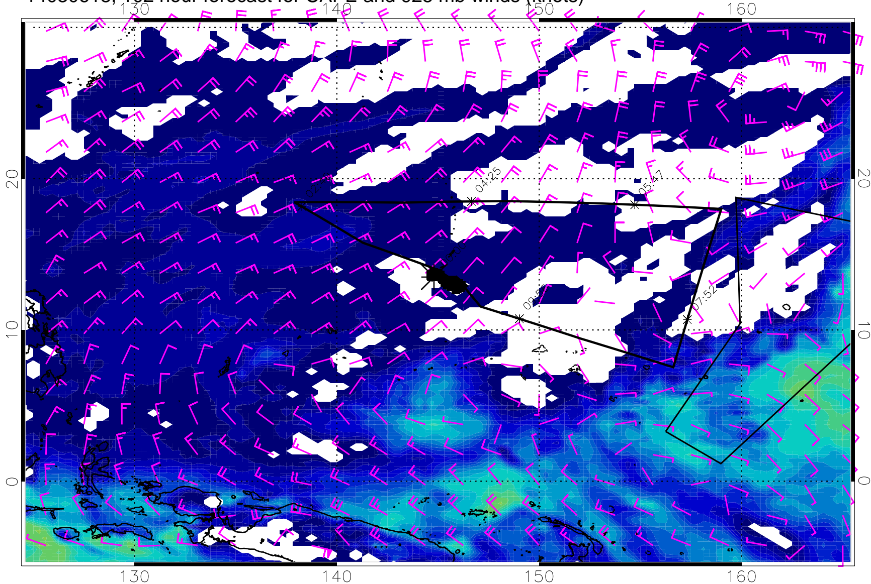
14030618, 102 hour forecast for CAPE and 925 mb winds (knots)
