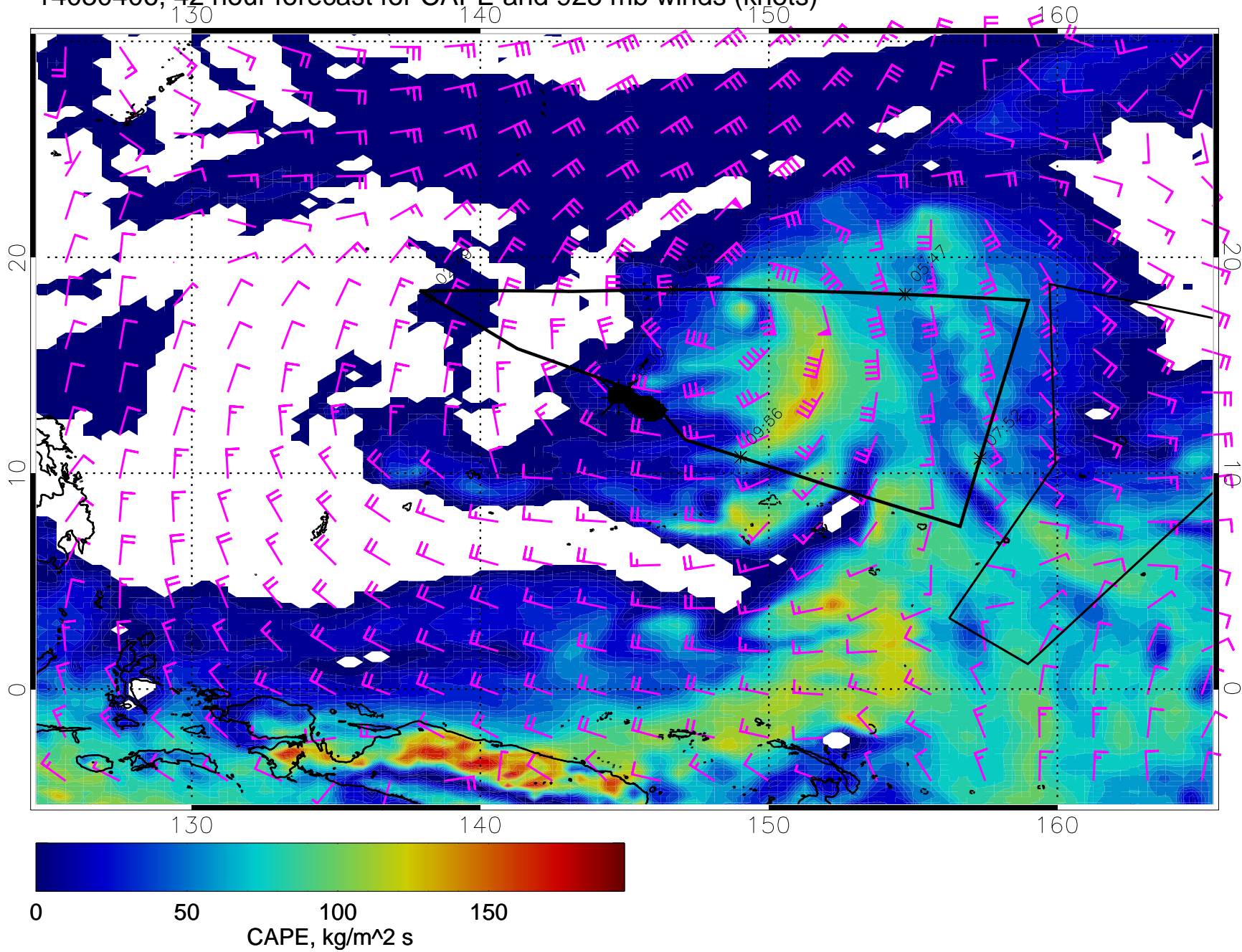
14030406, 42 hour forecast for CAPE and 925 mb winds (knots)
