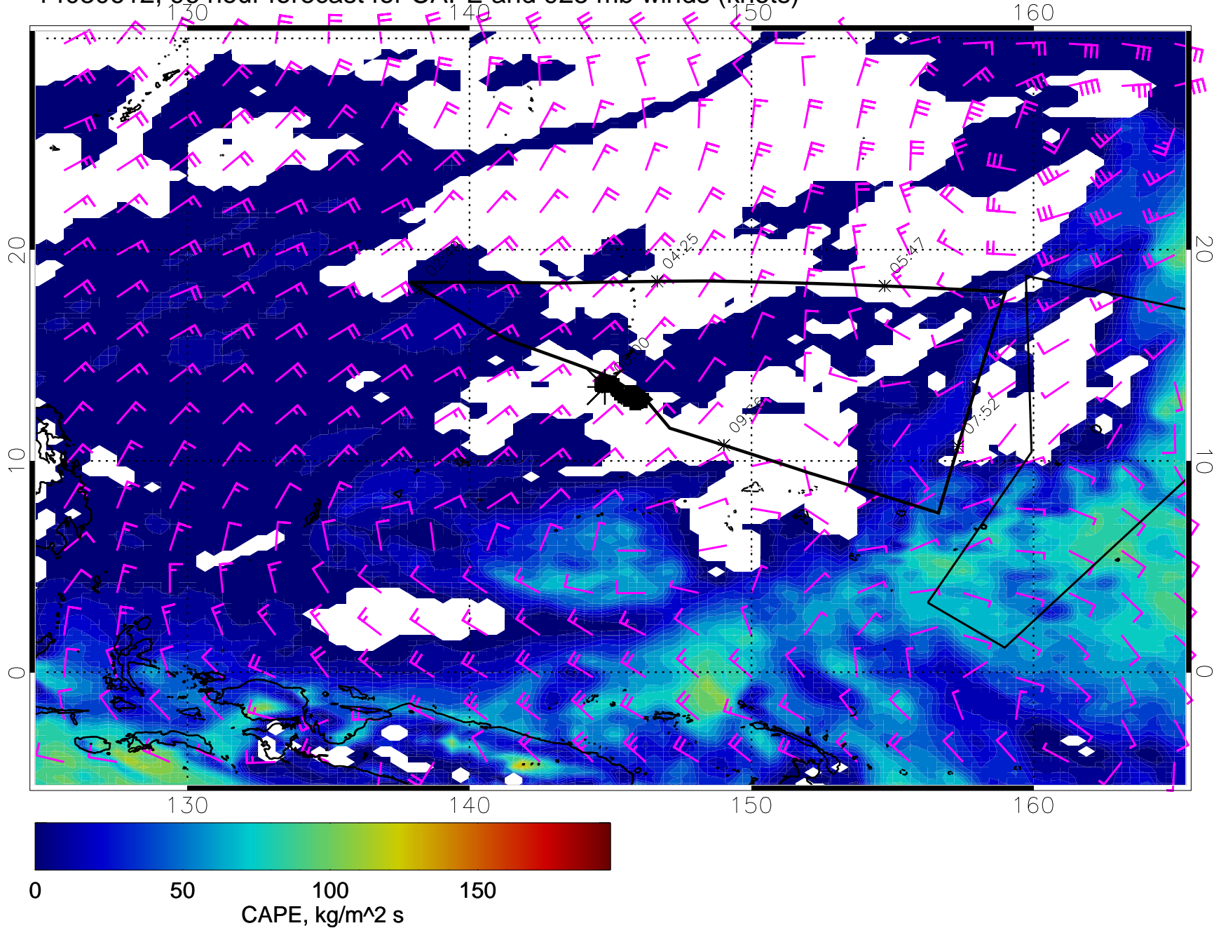
14030612, 96 hour forecast for CAPE and 925 mb winds (knots)
