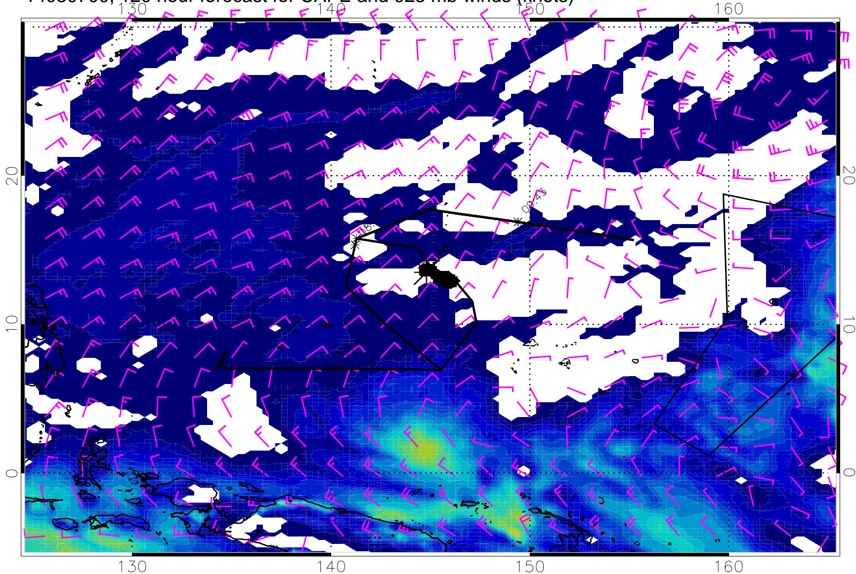
14030700, 120 hour forecast for CAPE and 925 mb winds (knots)
