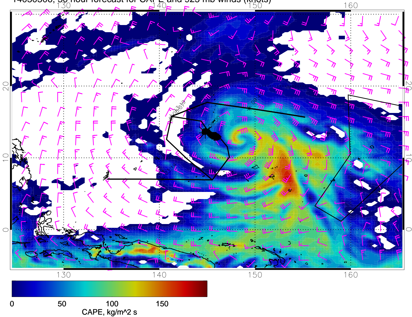
14030306, 30 hour forecast for CAPE and 925 mb winds (knots)
