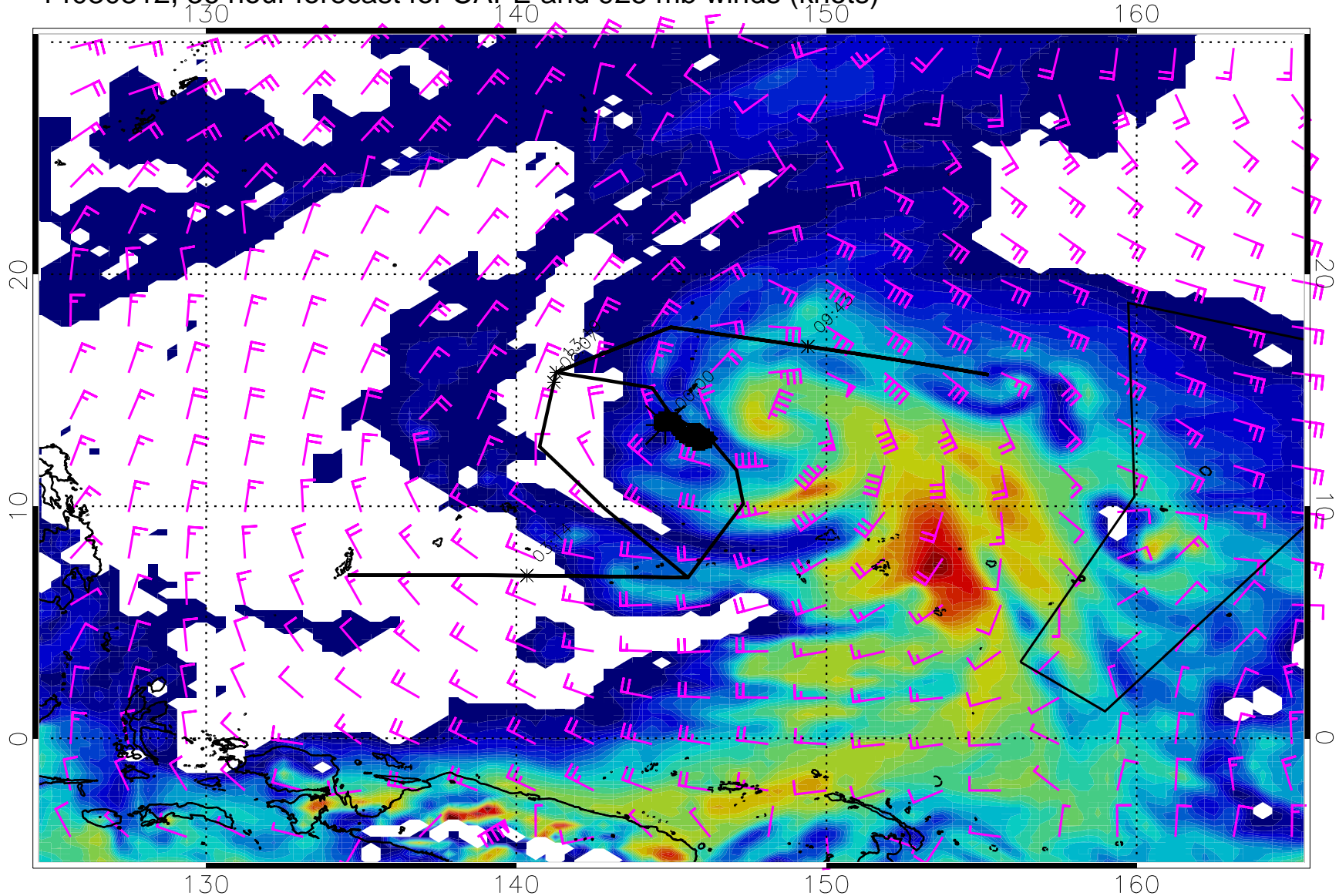
14030312, 36 hour forecast for CAPE and 925 mb winds (knots)
