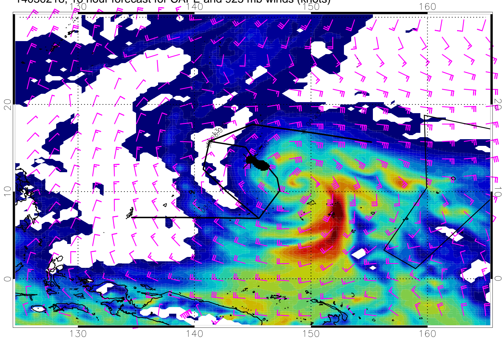
14030218, 18 hour forecast for CAPE and 925 mb winds (knots)
