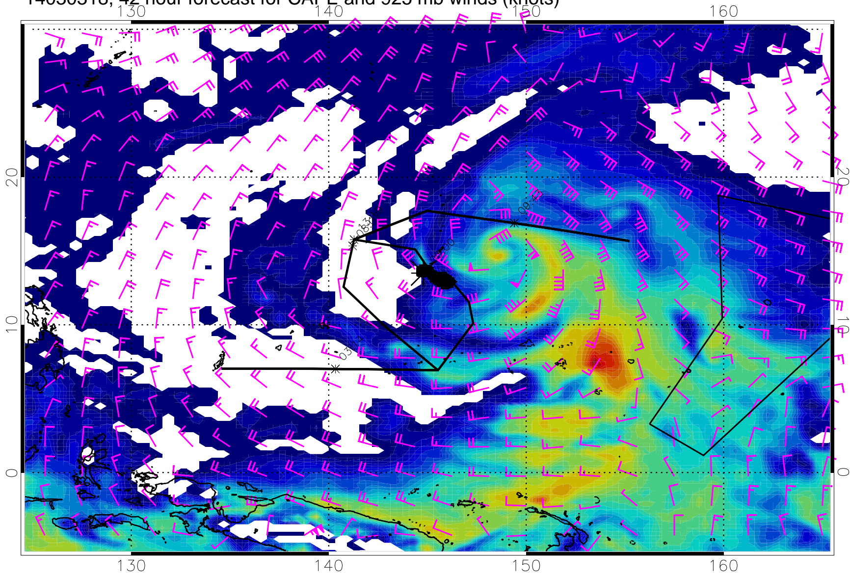
14030318, 42 hour forecast for CAPE and 925 mb winds (knots)
