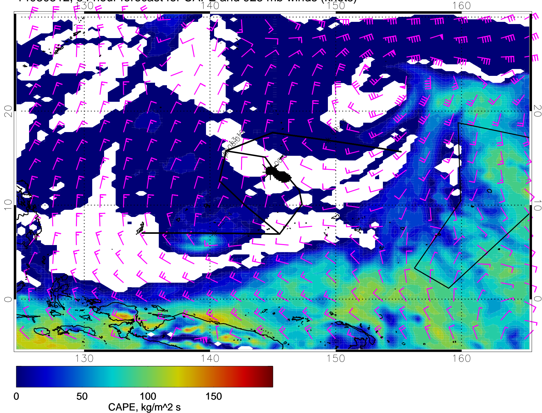
14030512, 84 hour forecast for CAPE and 925 mb winds (knots)
