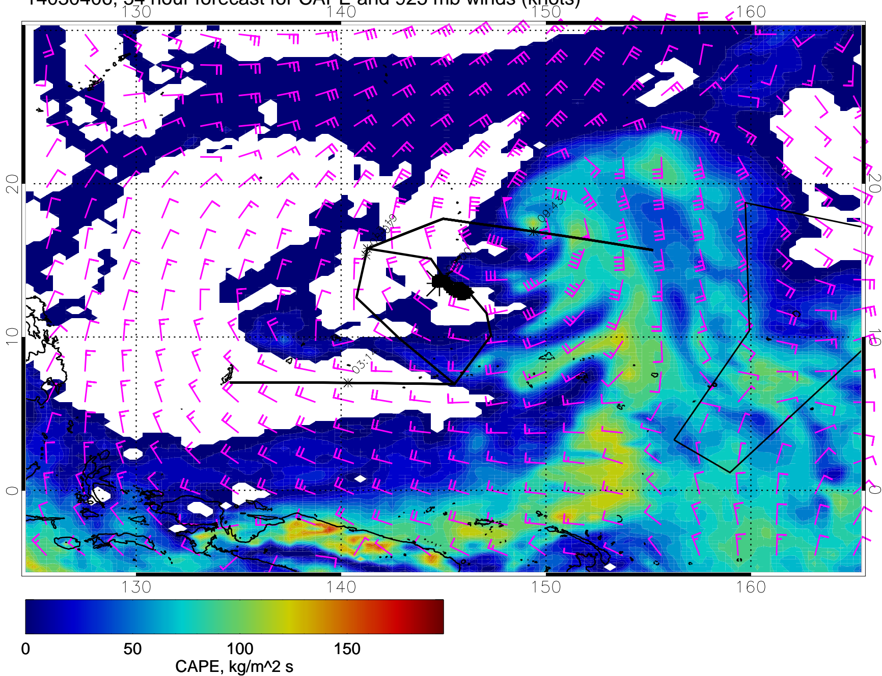
14030406, 54 hour forecast for CAPE and 925 mb winds (knots)
