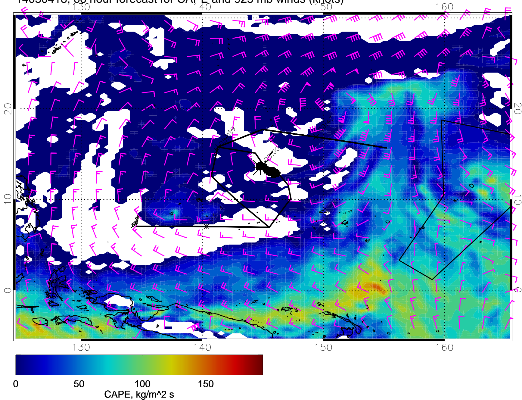
14030418, 66 hour forecast for CAPE and 925 mb winds (knots)
