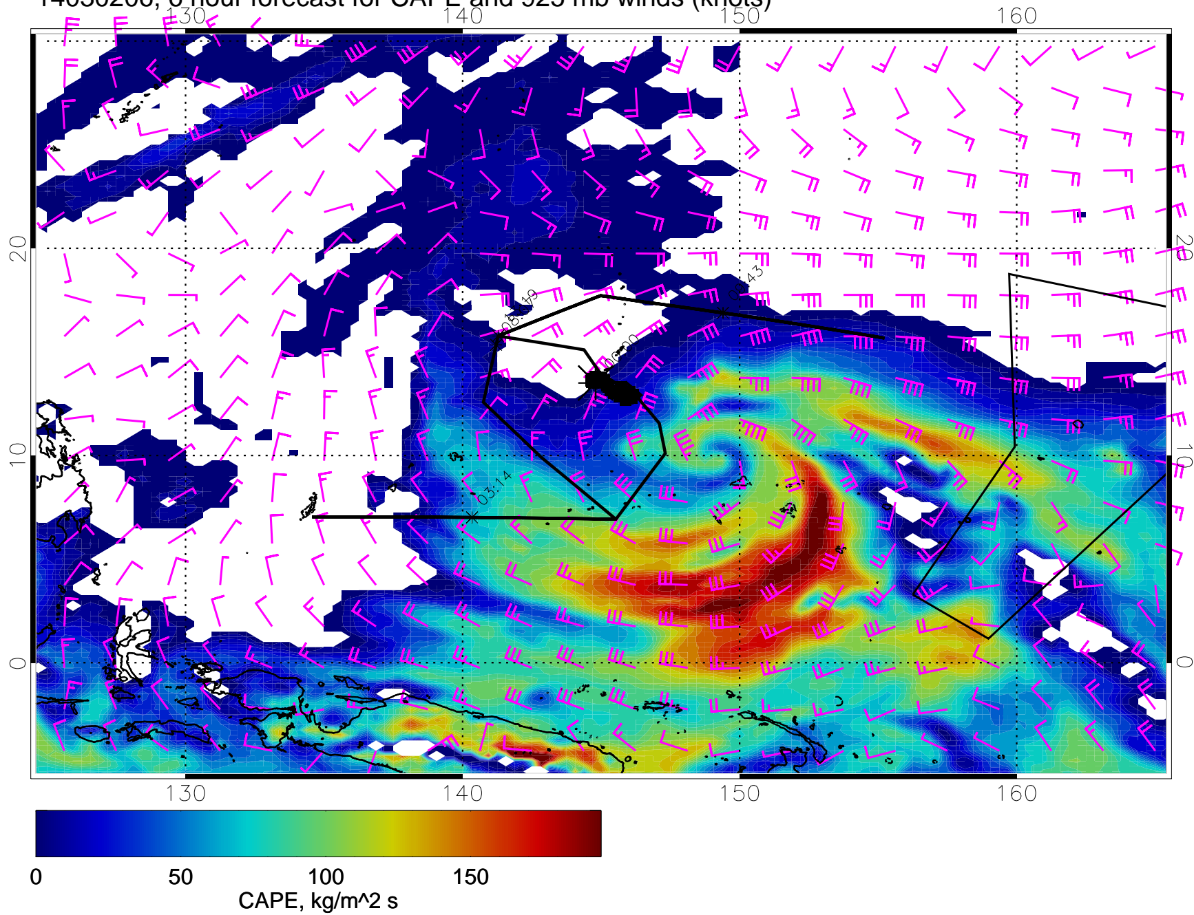
14030206, 6 hour forecast for CAPE and 925 mb winds (knots)
