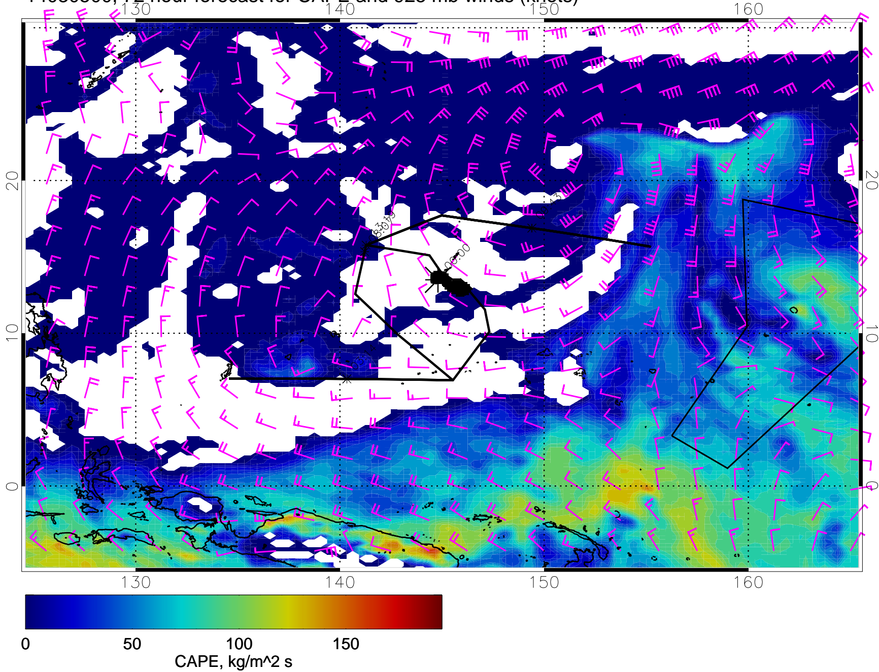
14030500, 72 hour forecast for CAPE and 925 mb winds (knots)
