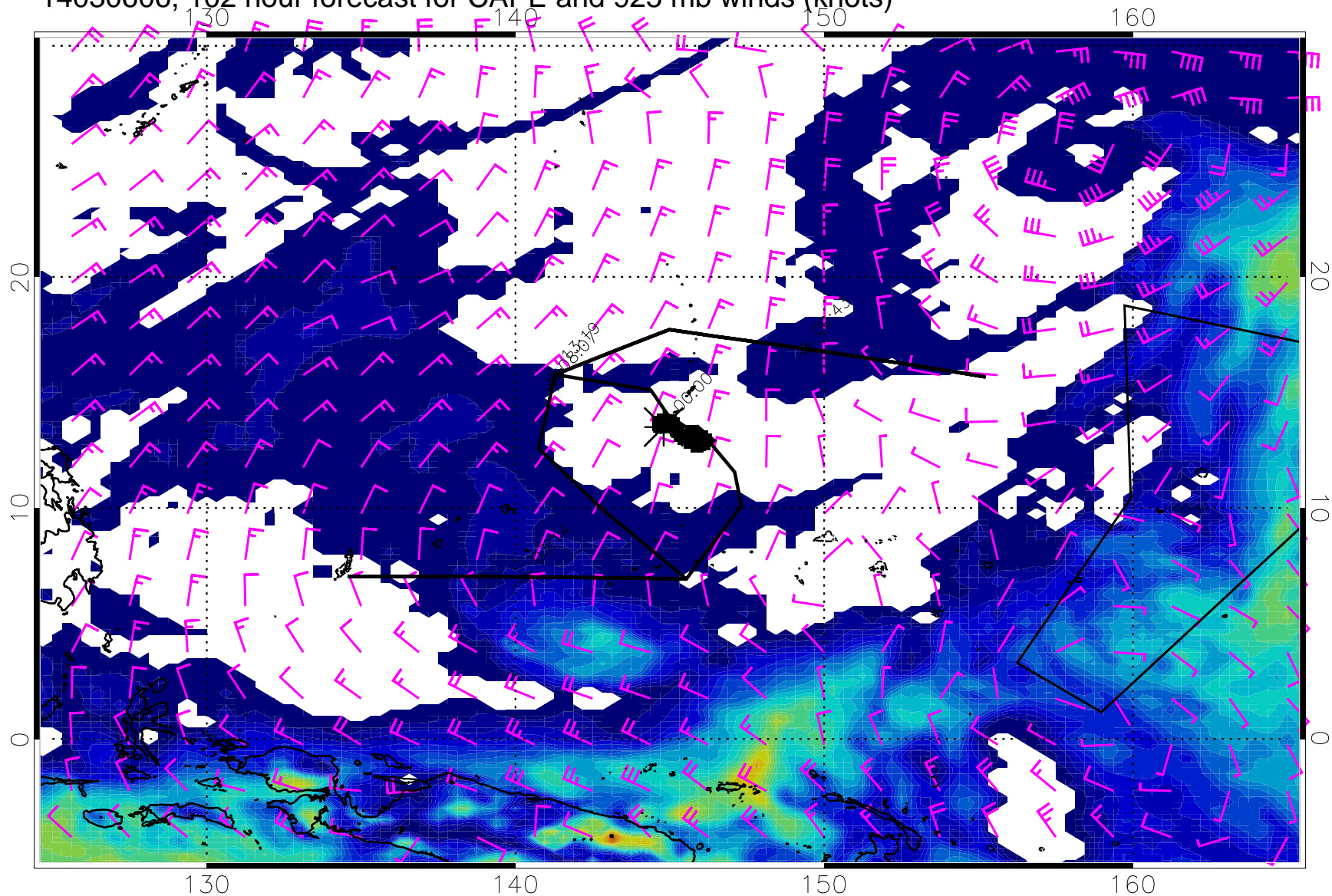
14030606, 102 hour forecast for CAPE and 925 mb winds (knots)
