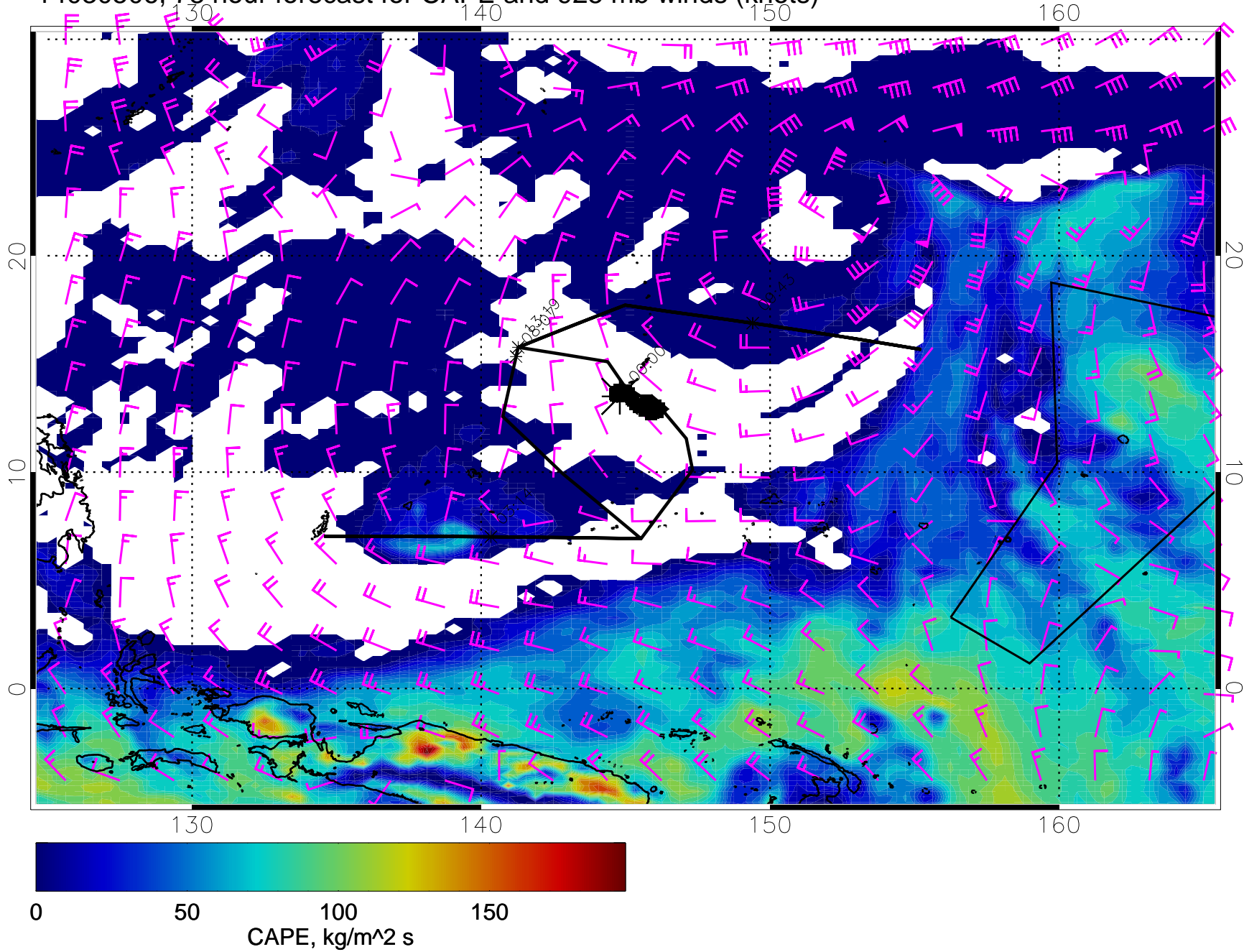
14030506, 78 hour forecast for CAPE and 925 mb winds (knots)
