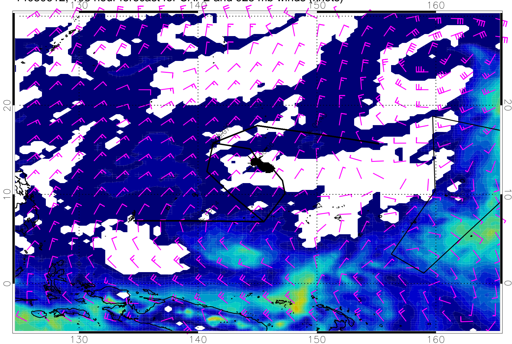
14030612, 108 hour forecast for CAPE and 925 mb winds (knots)
