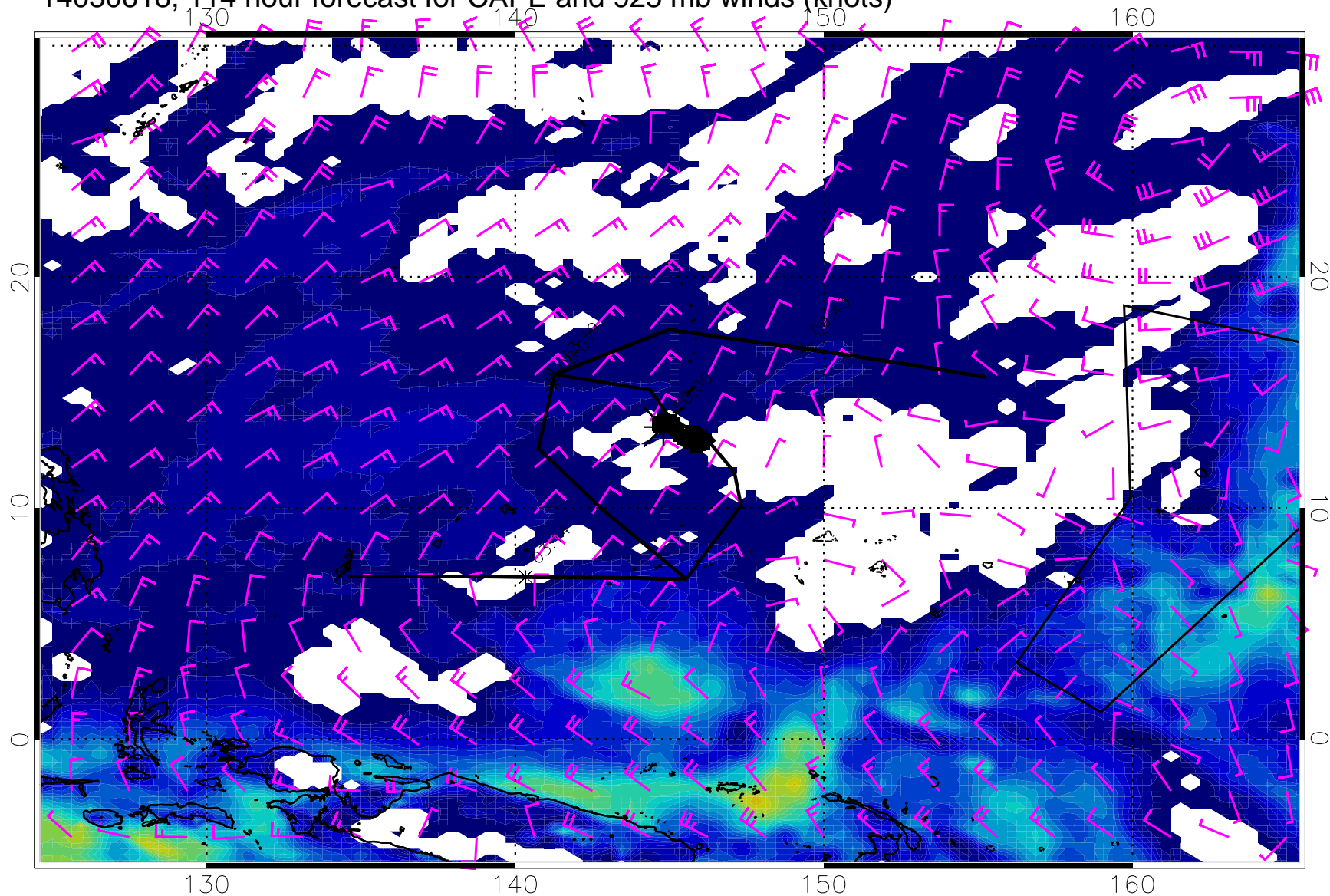
14030618, 114 hour forecast for CAPE and 925 mb winds (knots)
