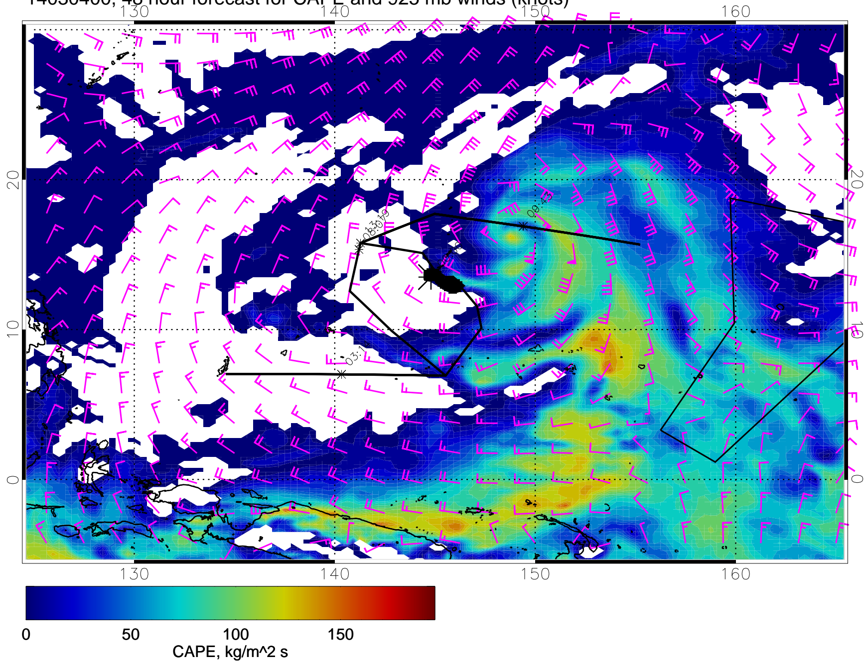
14030400, 48 hour forecast for CAPE and 925 mb winds (knots)
