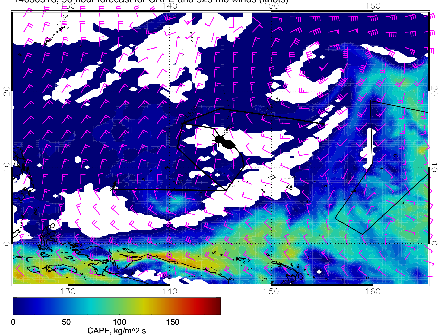
14030518, 90 hour forecast for CAPE and 925 mb winds (knots)
