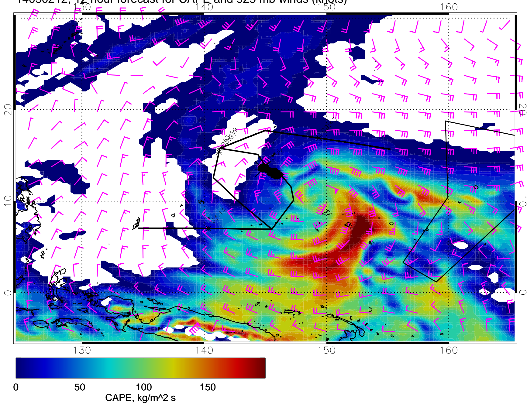
14030212, 12 hour forecast for CAPE and 925 mb winds (knots)
