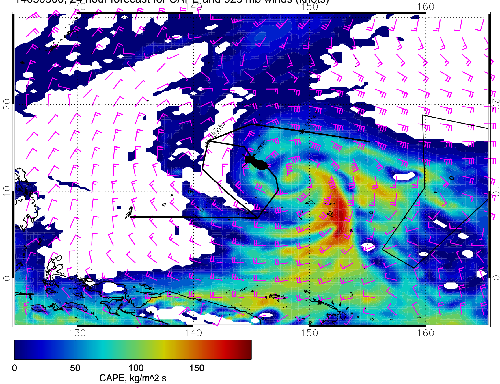
14030300, 24 hour forecast for CAPE and 925 mb winds (knots)
