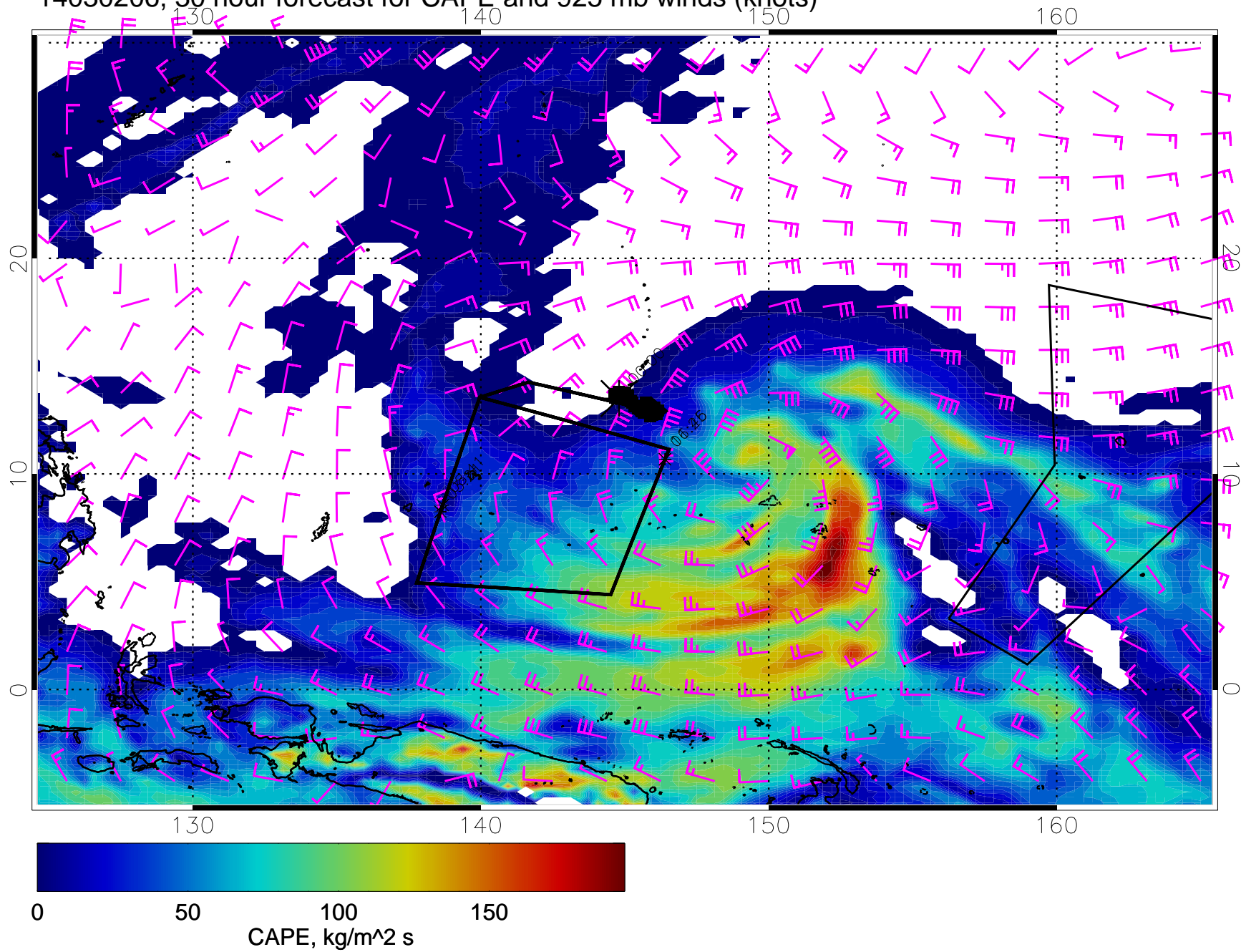
14030206, 30 hour forecast for CAPE and 925 mb winds (knots)
