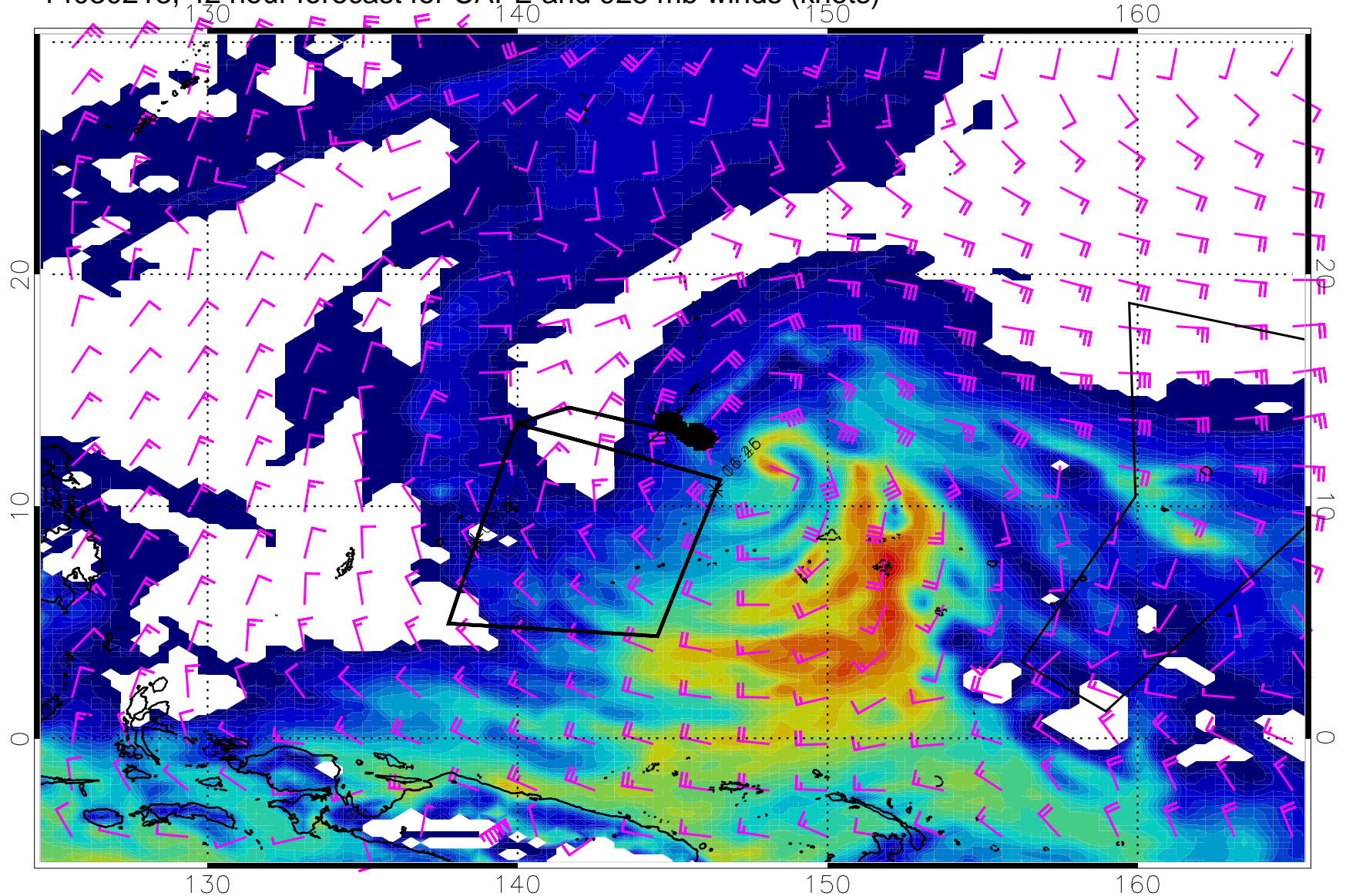
14030218, 42 hour forecast for CAPE and 925 mb winds (knots)
