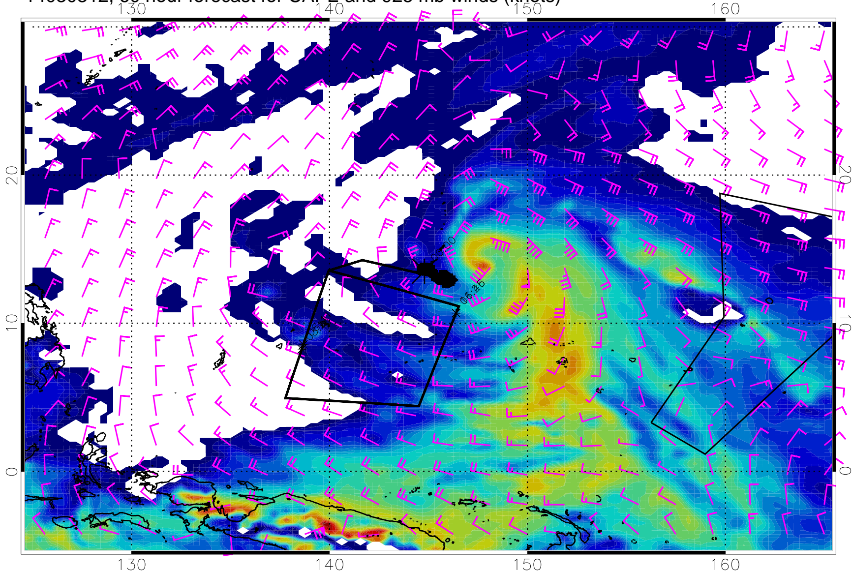
14030312, 60 hour forecast for CAPE and 925 mb winds (knots)
