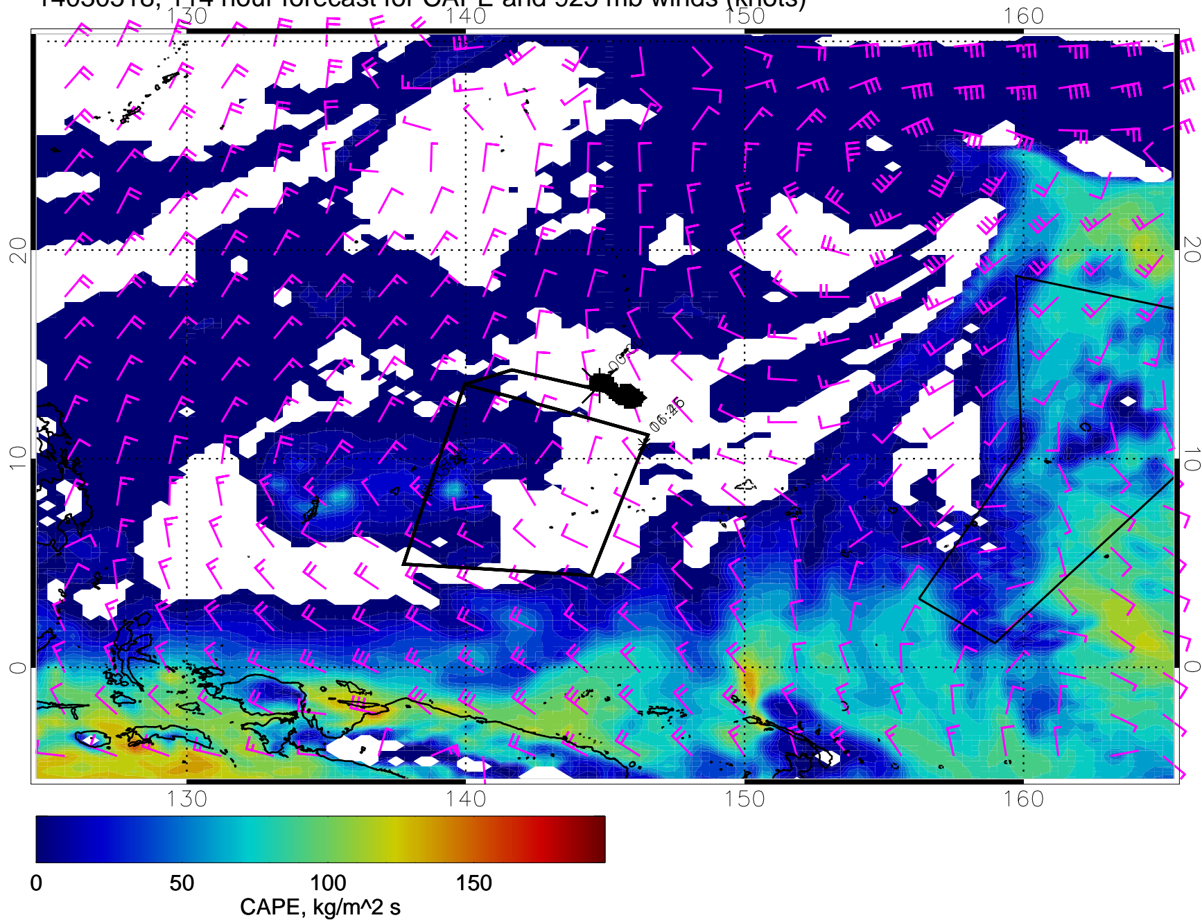
14030518, 114 hour forecast for CAPE and 925 mb winds (knots)
