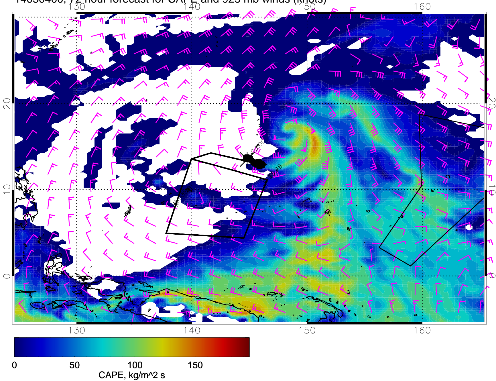
14030400, 72 hour forecast for CAPE and 925 mb winds (knots)
