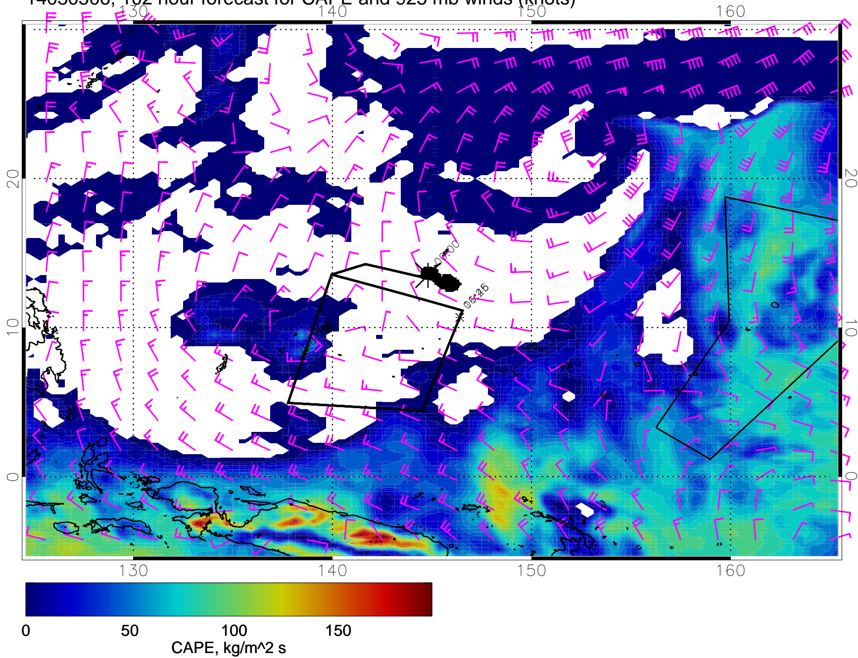
14030506, 102 hour forecast for CAPE and 925 mb winds (knots)
