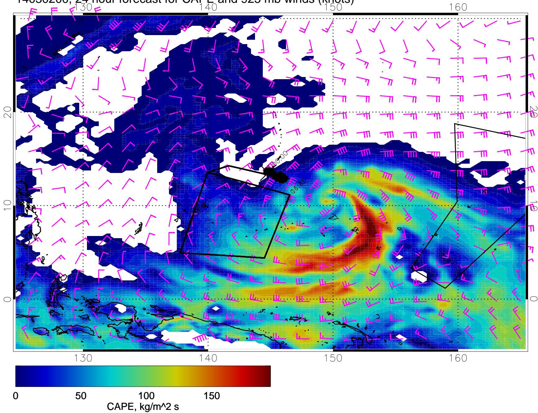
14030200, 24 hour forecast for CAPE and 925 mb winds (knots)
