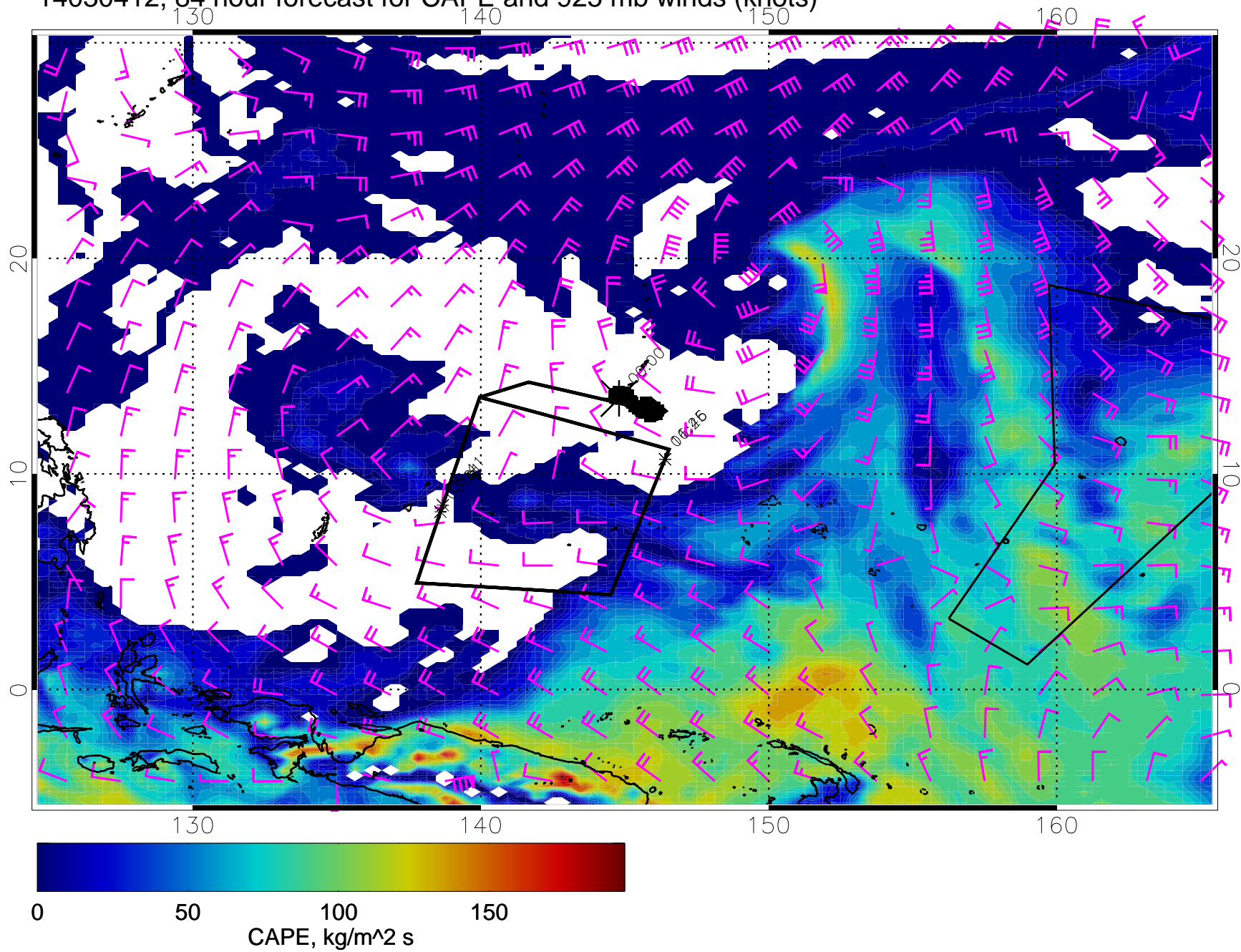
14030412, 84 hour forecast for CAPE and 925 mb winds (knots)
