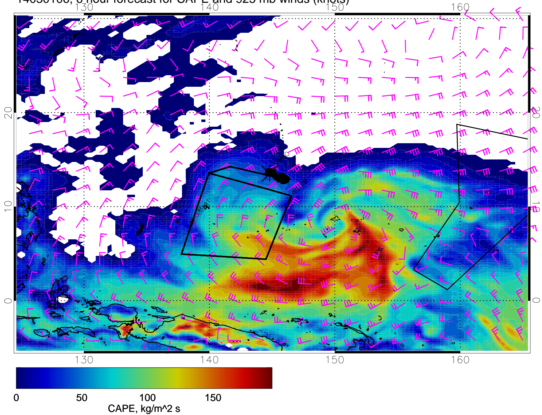
14030106, 6 hour forecast for CAPE and 925 mb winds (knots)
