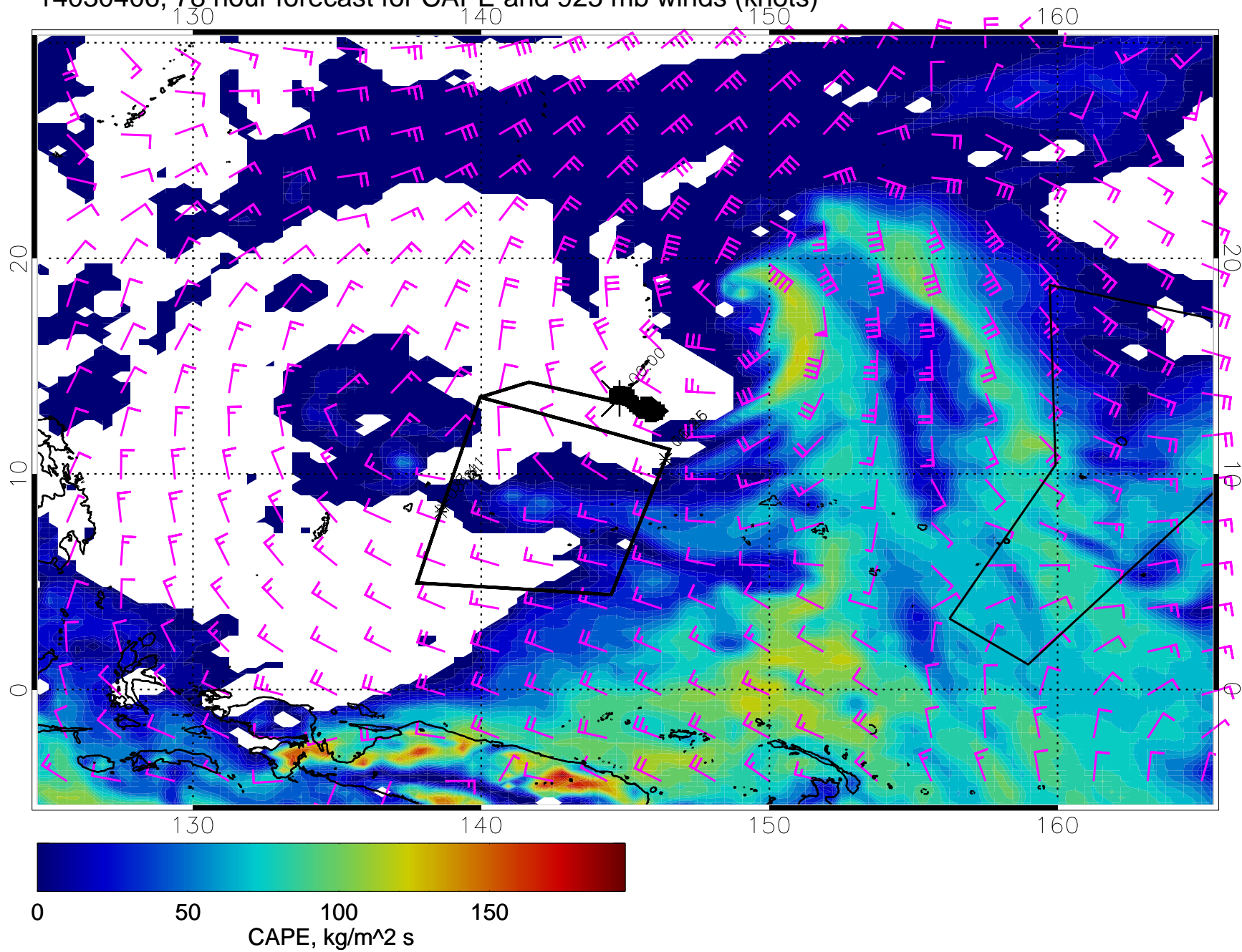
14030406, 78 hour forecast for CAPE and 925 mb winds (knots)
