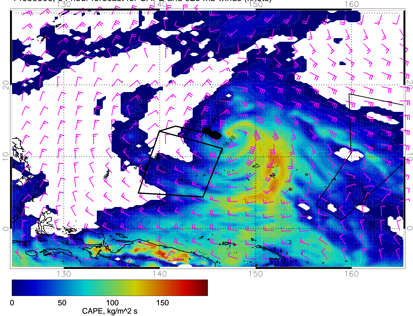
14030306, 54 hour forecast for CAPE and 925 mb winds (knots)
