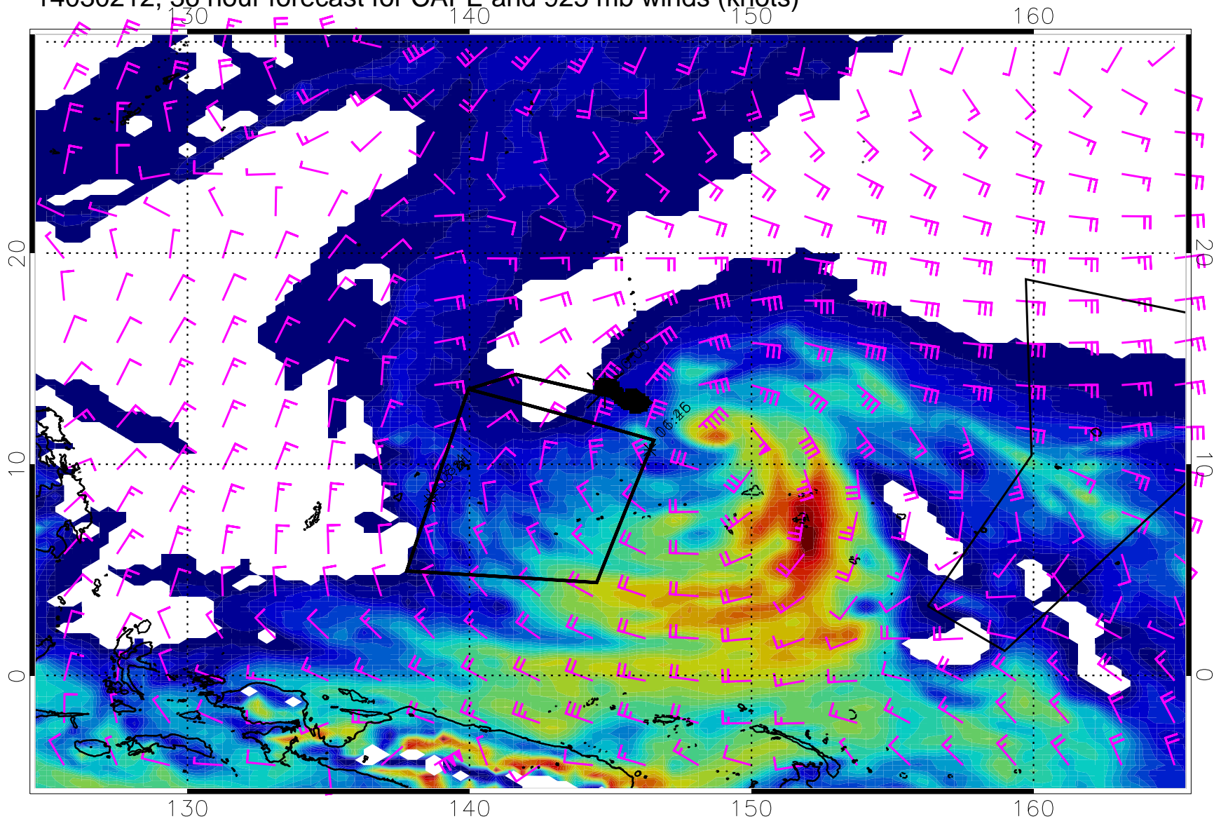
14030212, 36 hour forecast for CAPE and 925 mb winds (knots)
