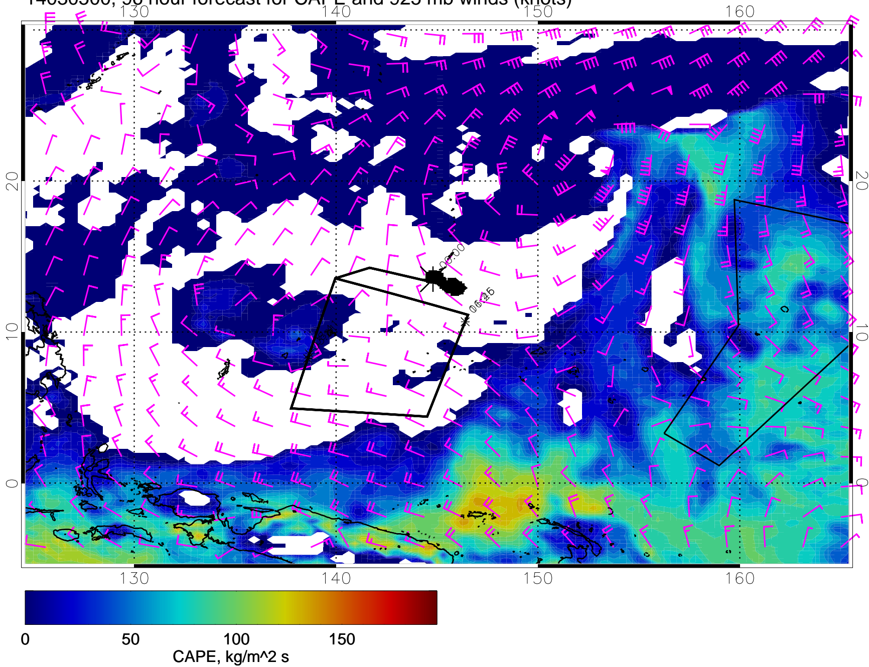
14030500, 96 hour forecast for CAPE and 925 mb winds (knots)
