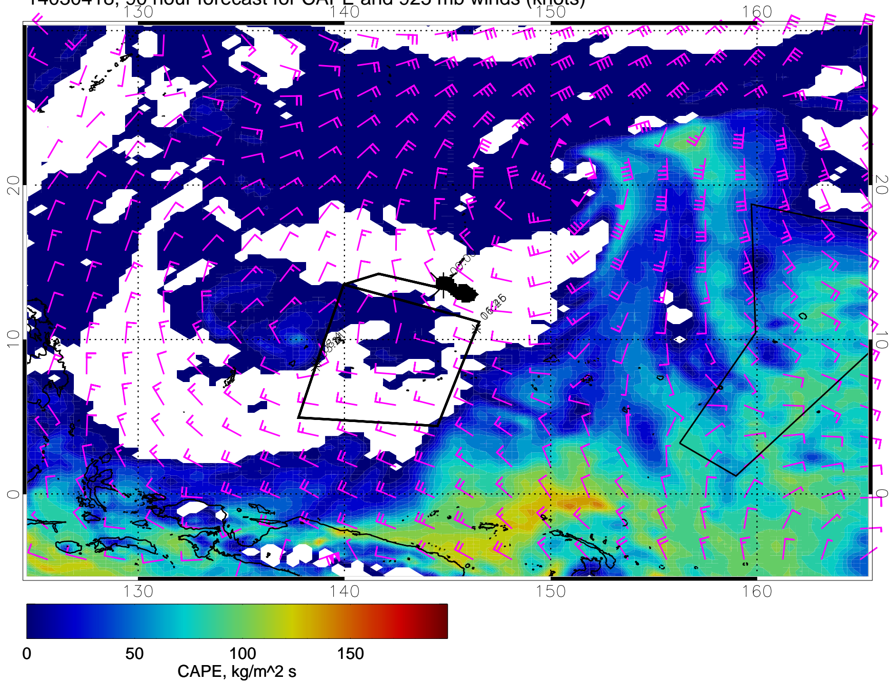
14030418, 90 hour forecast for CAPE and 925 mb winds (knots)
