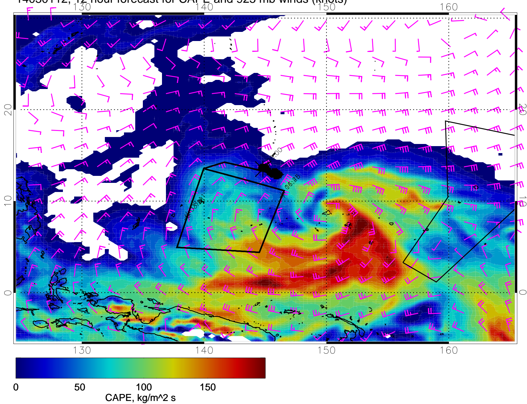
14030112, 12 hour forecast for CAPE and 925 mb winds (knots)
