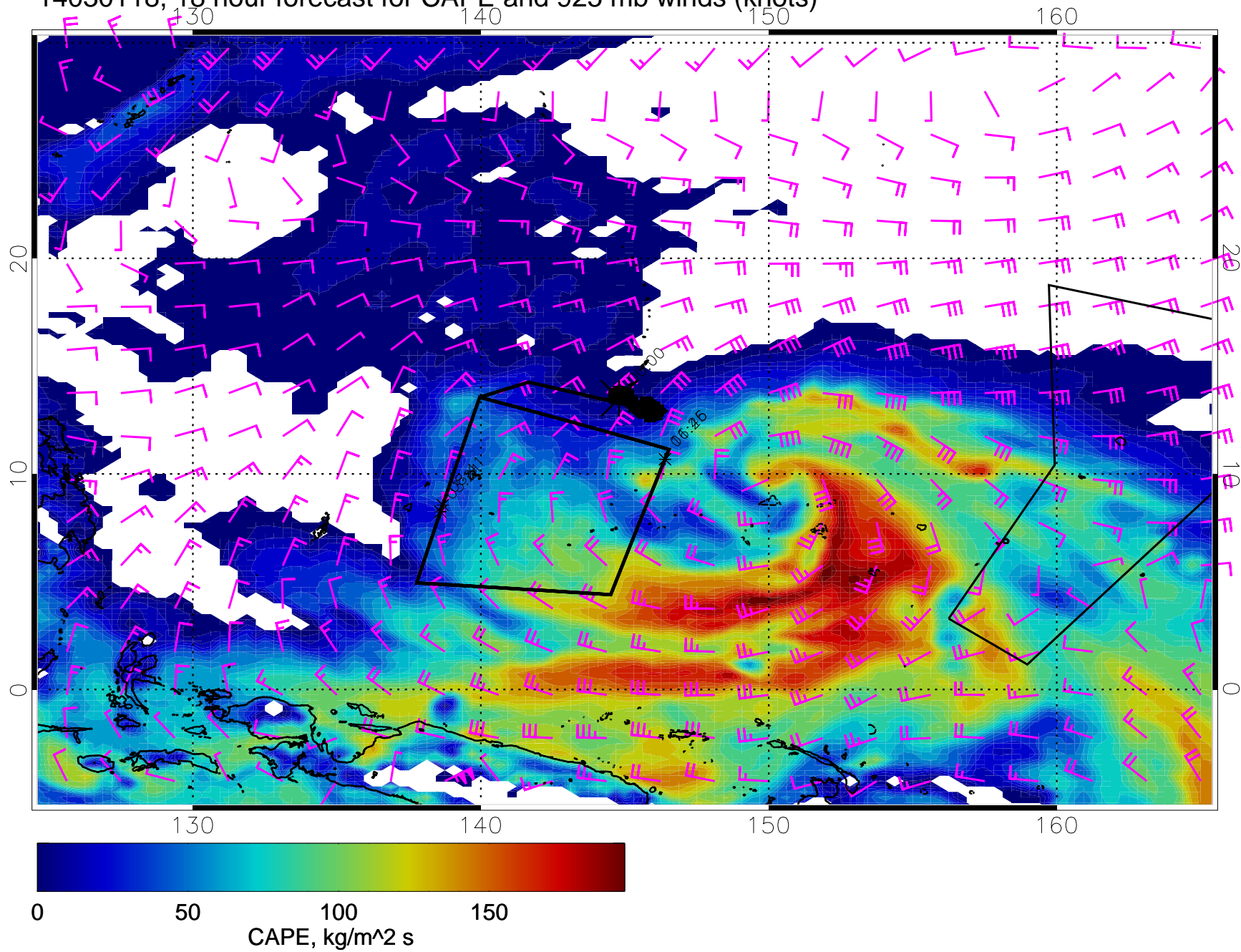
14030118, 18 hour forecast for CAPE and 925 mb winds (knots)
