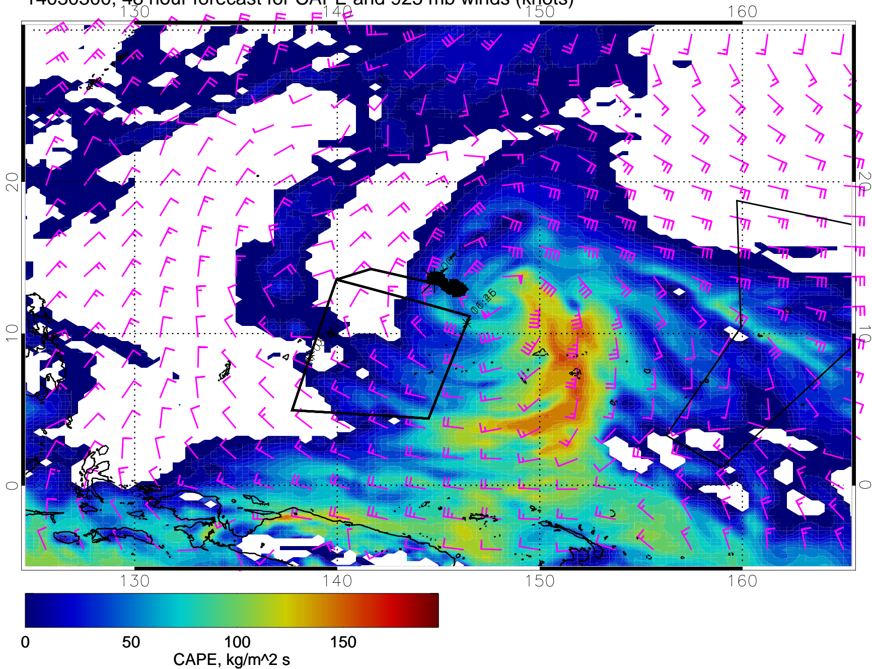
14030300, 48 hour forecast for CAPE and 925 mb winds (knots)
