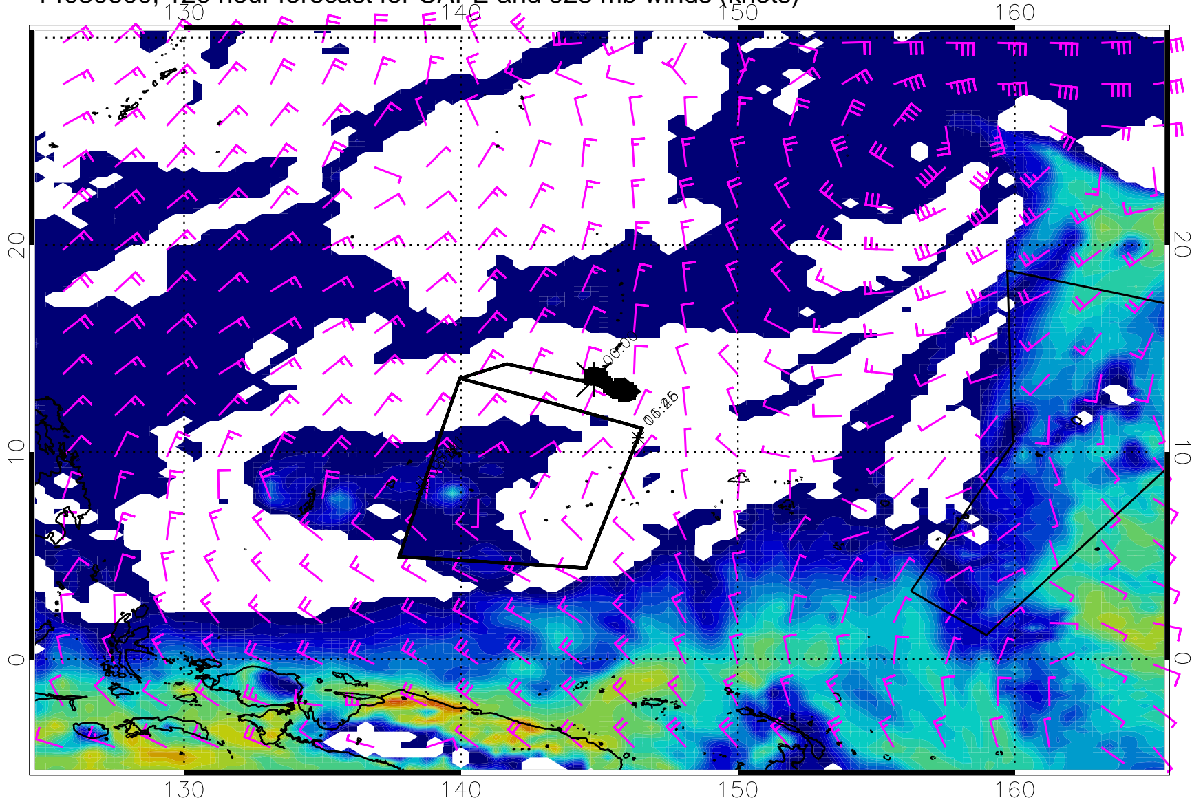
14030600, 120 hour forecast for CAPE and 925 mb winds (knots)
