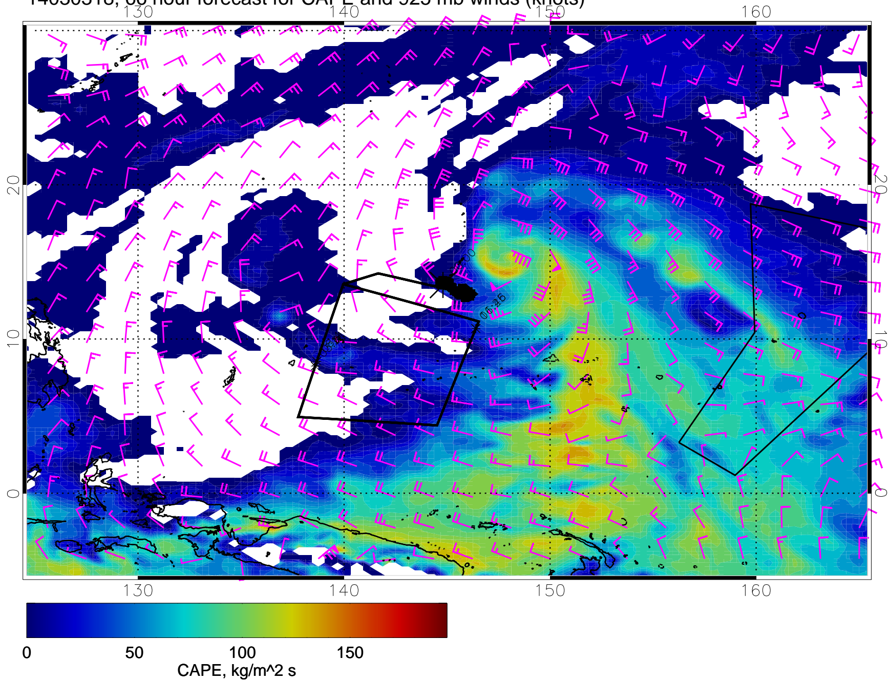
14030318, 66 hour forecast for CAPE and 925 mb winds (knots)
