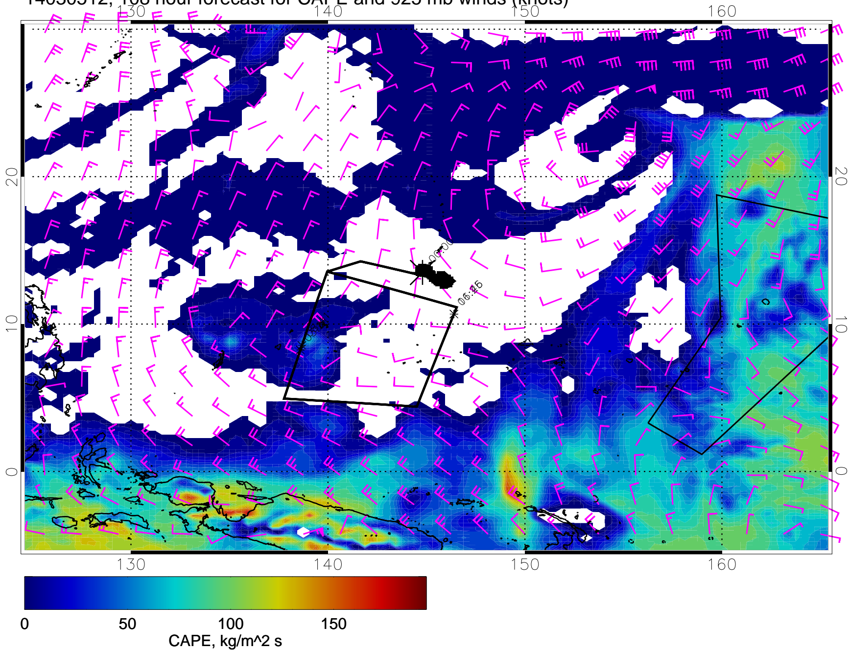
14030512, 108 hour forecast for CAPE and 925 mb winds (knots)
