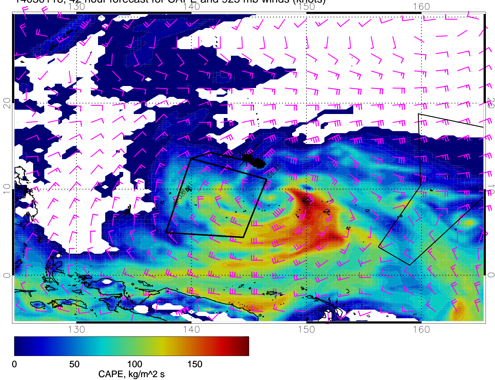
14030118, 42 hour forecast for CAPE and 925 mb winds (knots)
