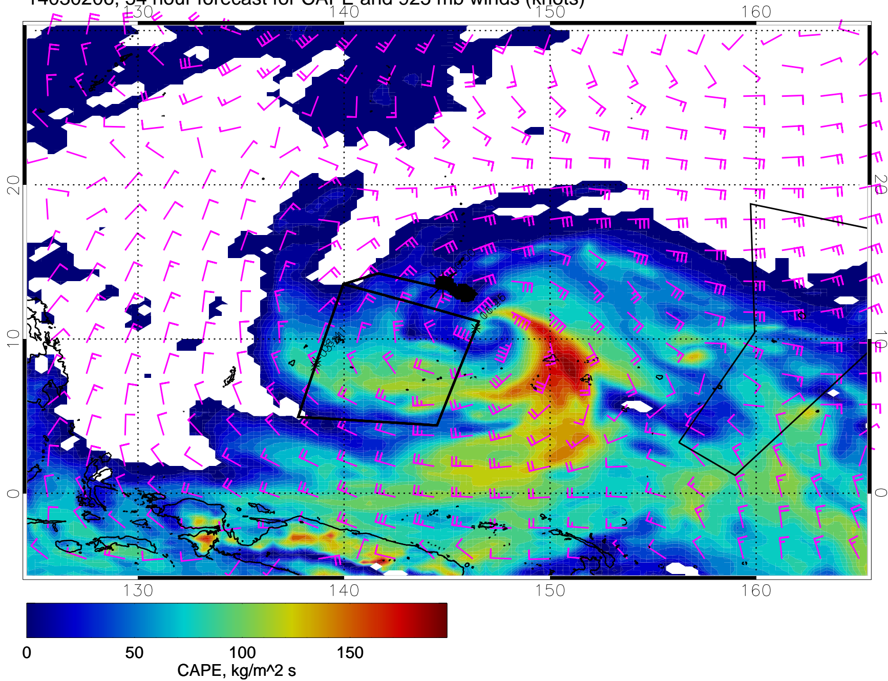
14030206, 54 hour forecast for CAPE and 925 mb winds (knots)
