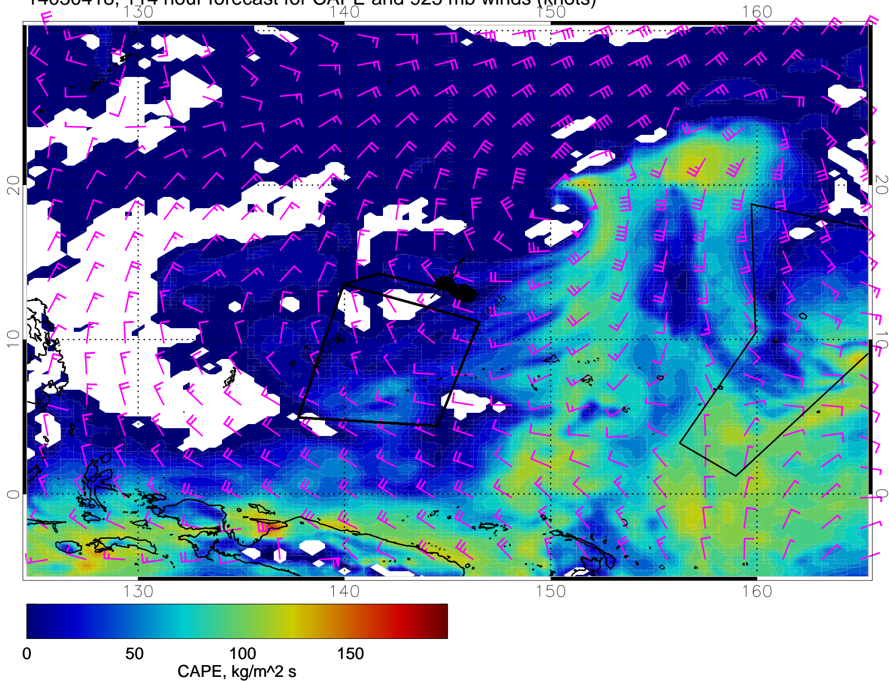
14030418, 114 hour forecast for CAPE and 925 mb winds (knots)
