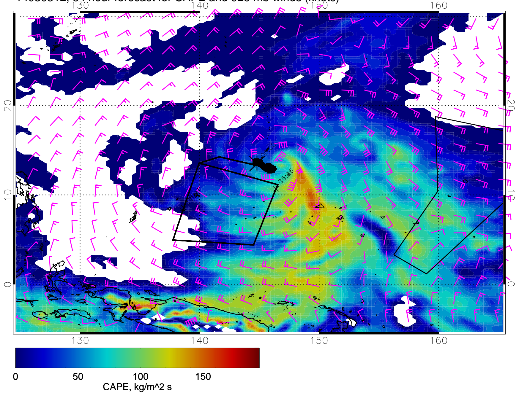
14030312, 84 hour forecast for CAPE and 925 mb winds (knots)
