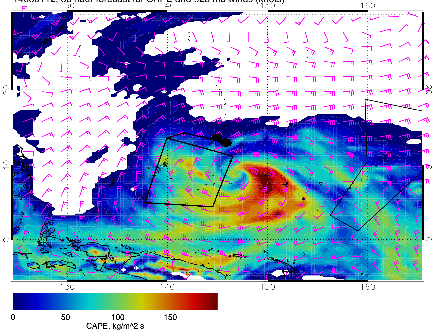
14030112, 36 hour forecast for CAPE and 925 mb winds (knots)
