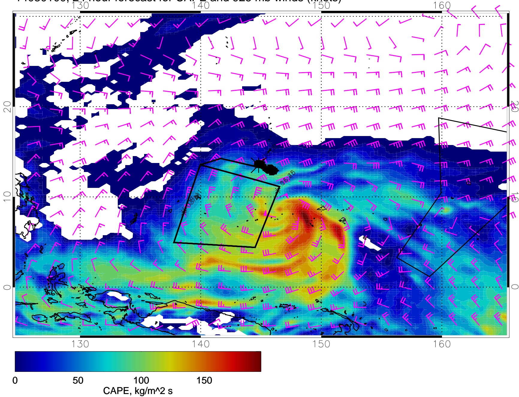
14030100, 24 hour forecast for CAPE and 925 mb winds (knots)
