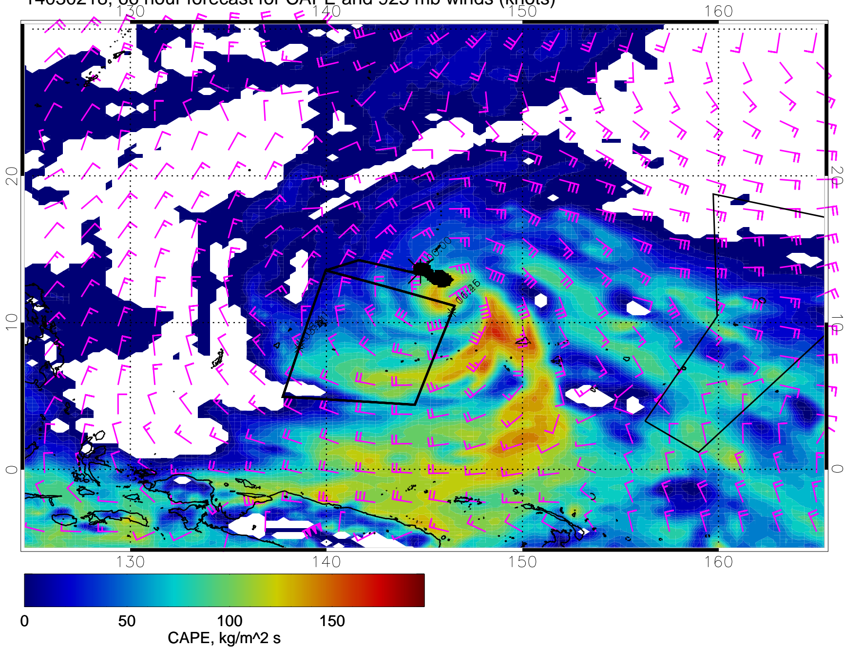
14030218, 66 hour forecast for CAPE and 925 mb winds (knots)
