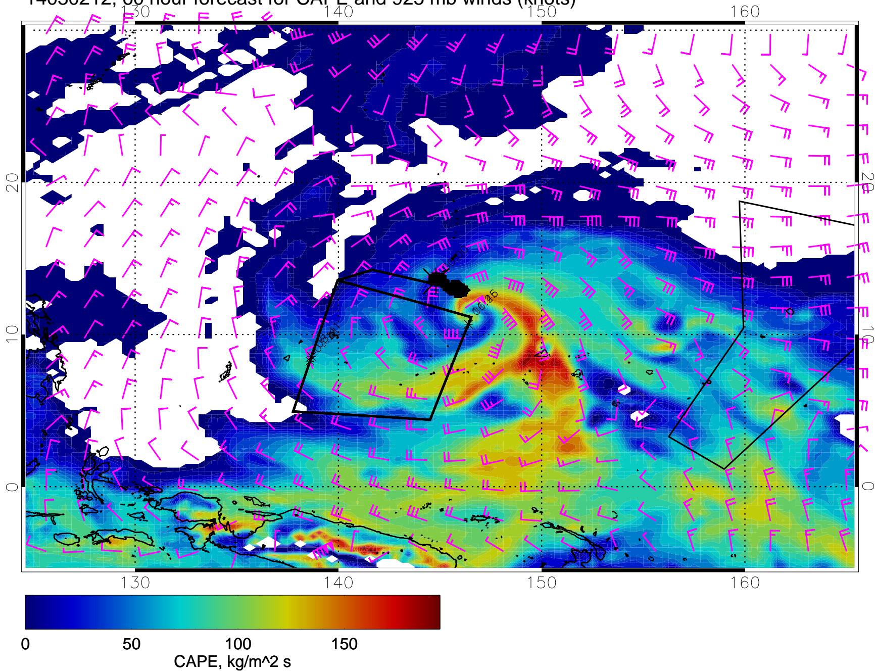
14030212, 60 hour forecast for CAPE and 925 mb winds (knots)
