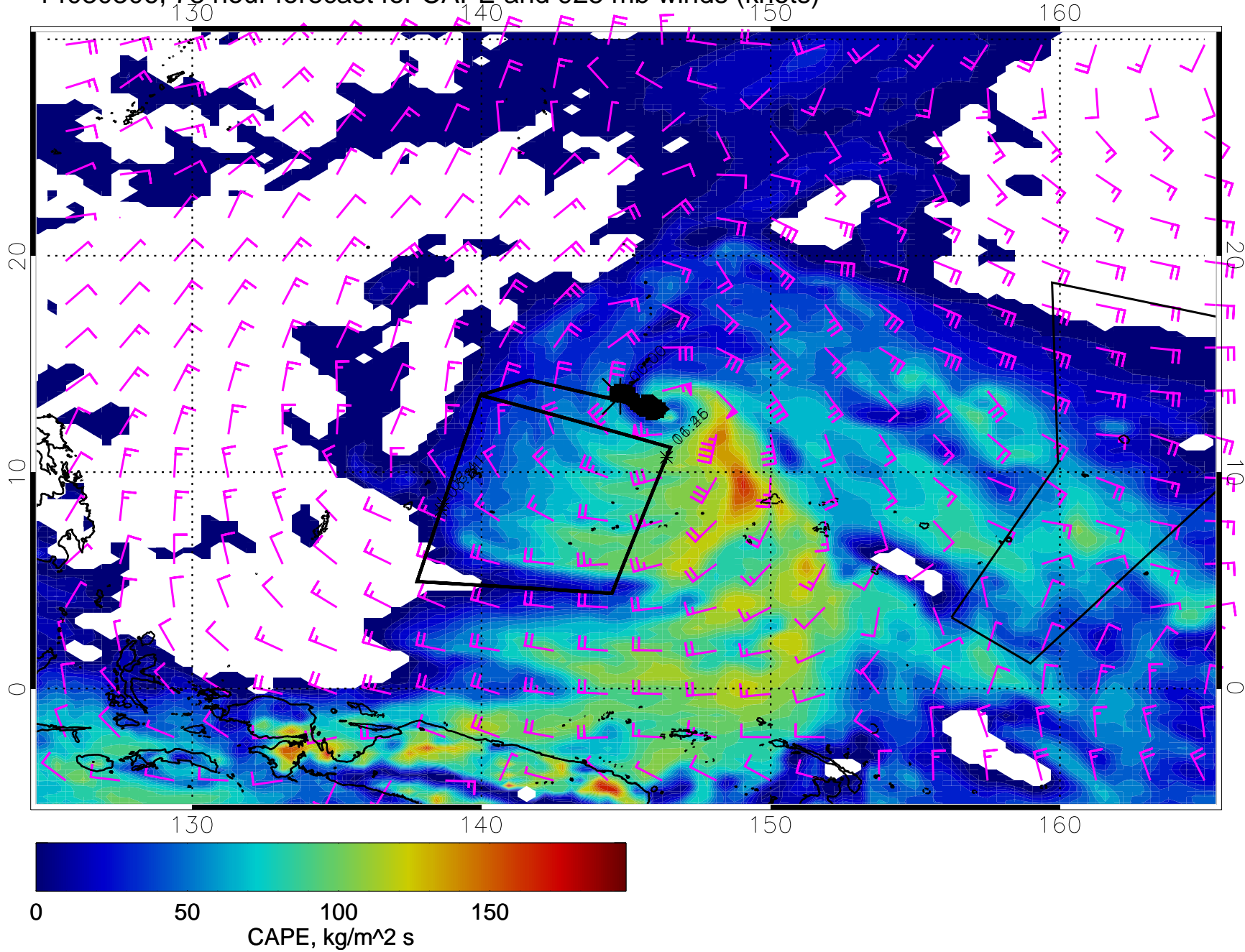
14030306, 78 hour forecast for CAPE and 925 mb winds (knots)
