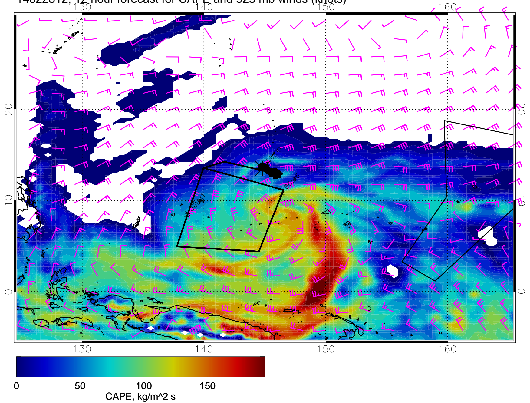
14022812, 12 hour forecast for CAPE and 925 mb winds (knots)
