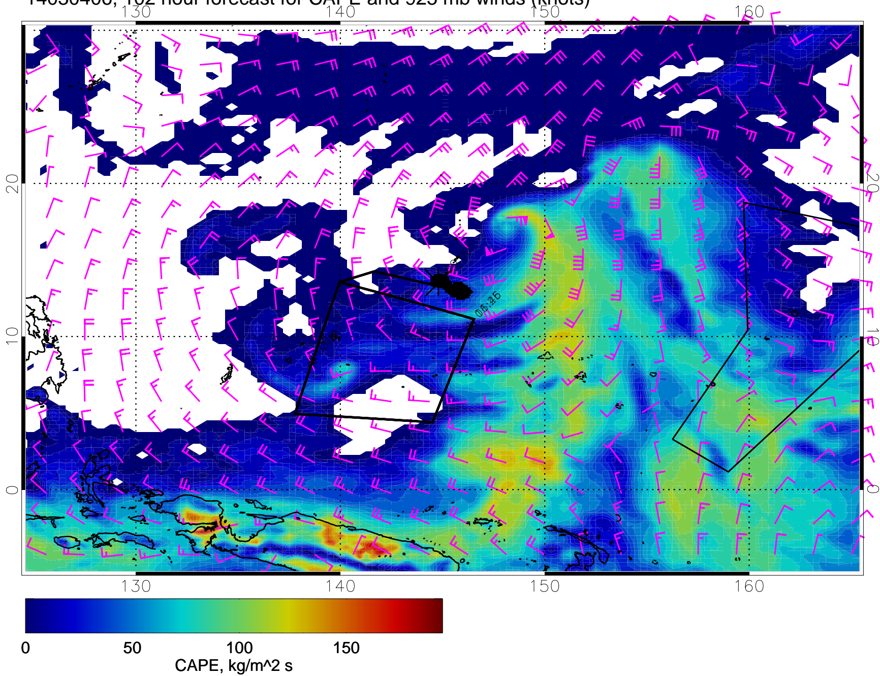
14030406, 102 hour forecast for CAPE and 925 mb winds (knots)
