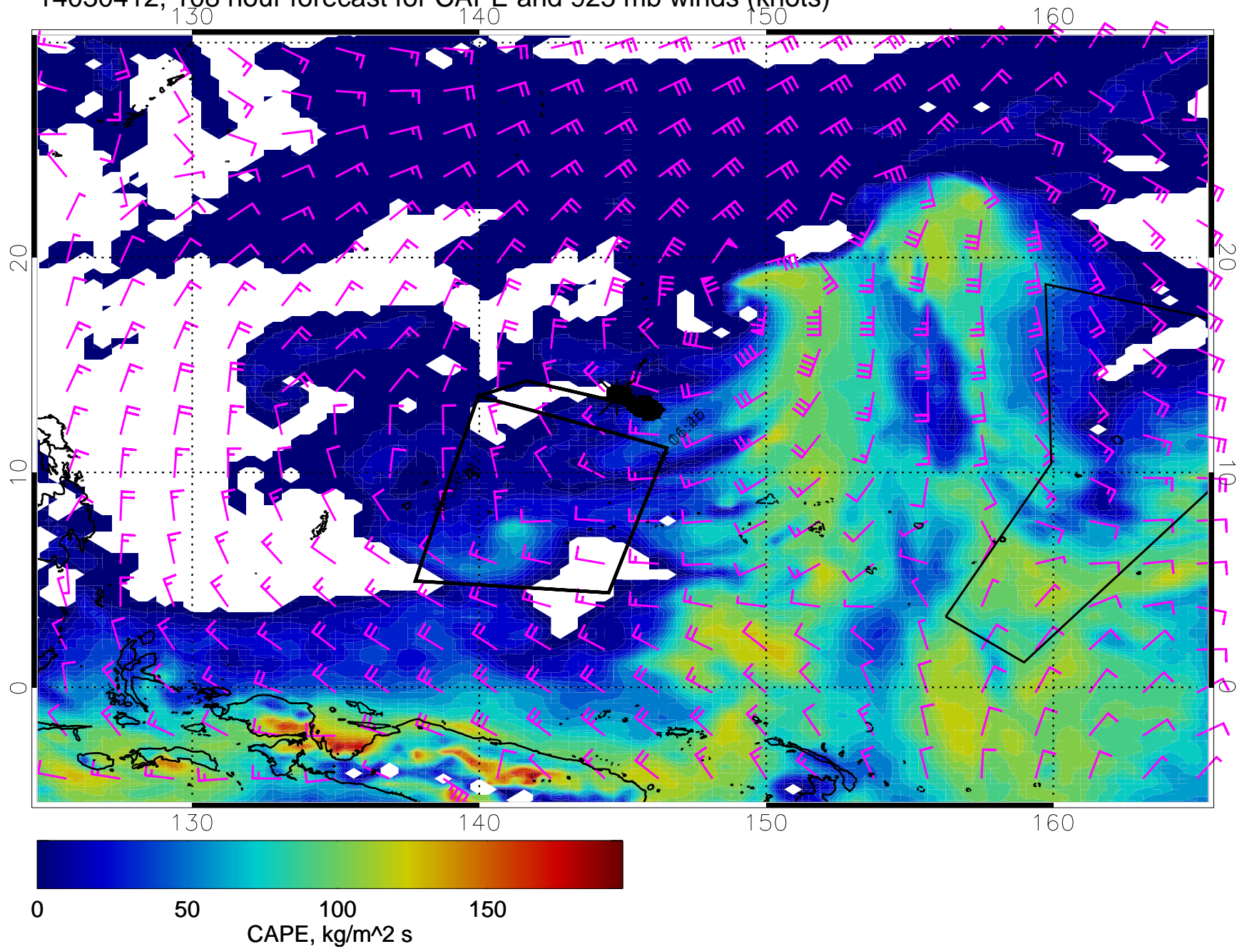
14030412, 108 hour forecast for CAPE and 925 mb winds (knots)
