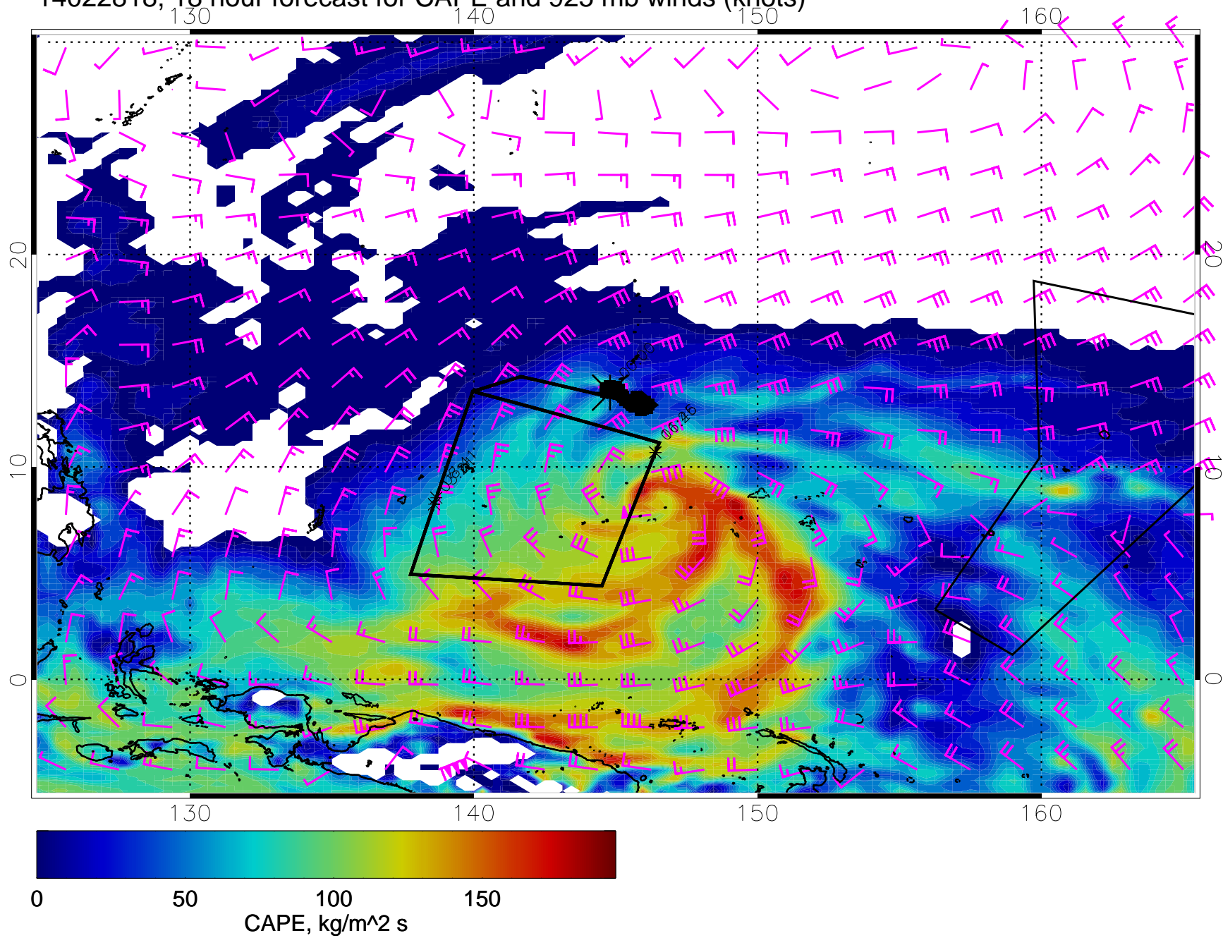
14022818, 18 hour forecast for CAPE and 925 mb winds (knots)
