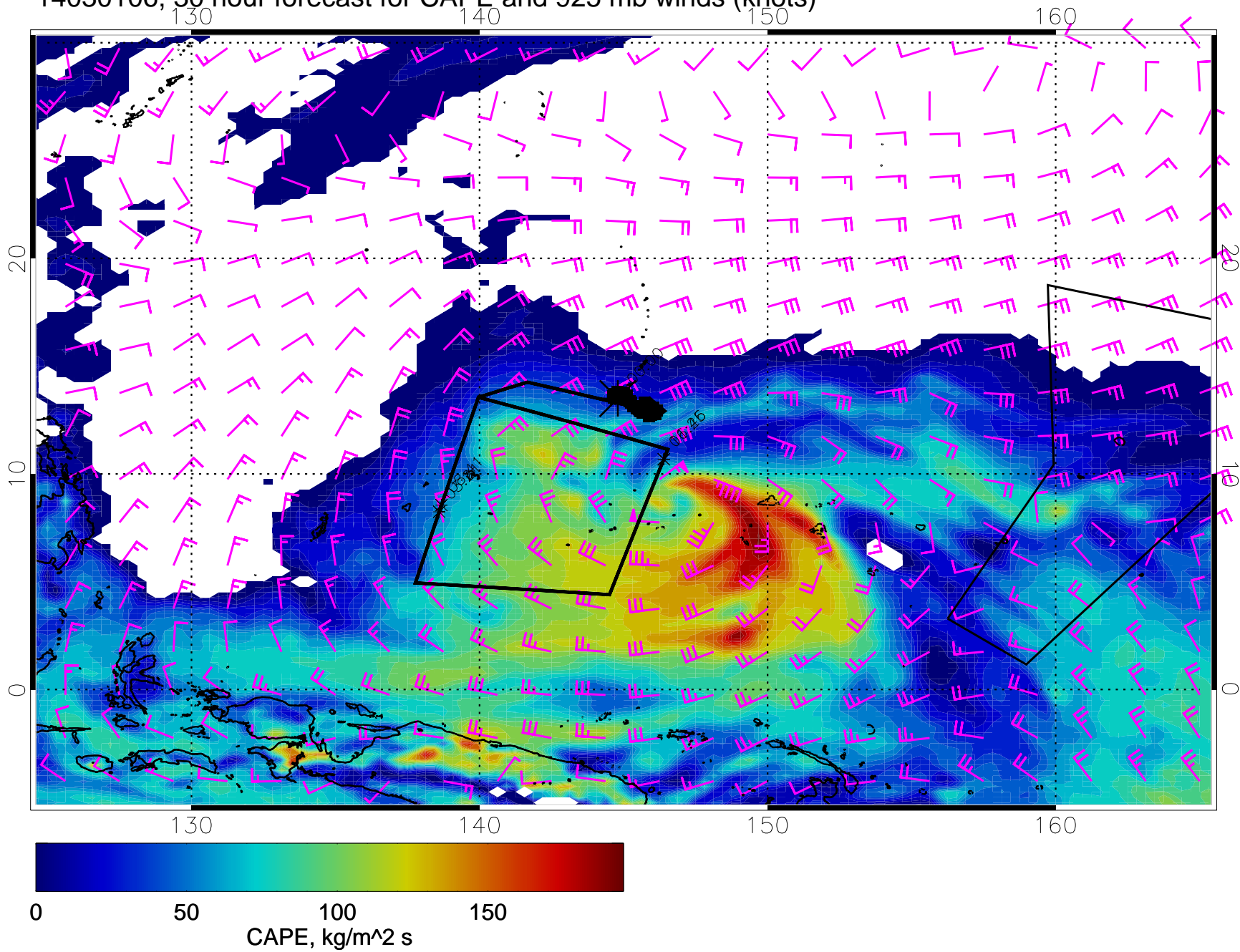
14030106, 30 hour forecast for CAPE and 925 mb winds (knots)
