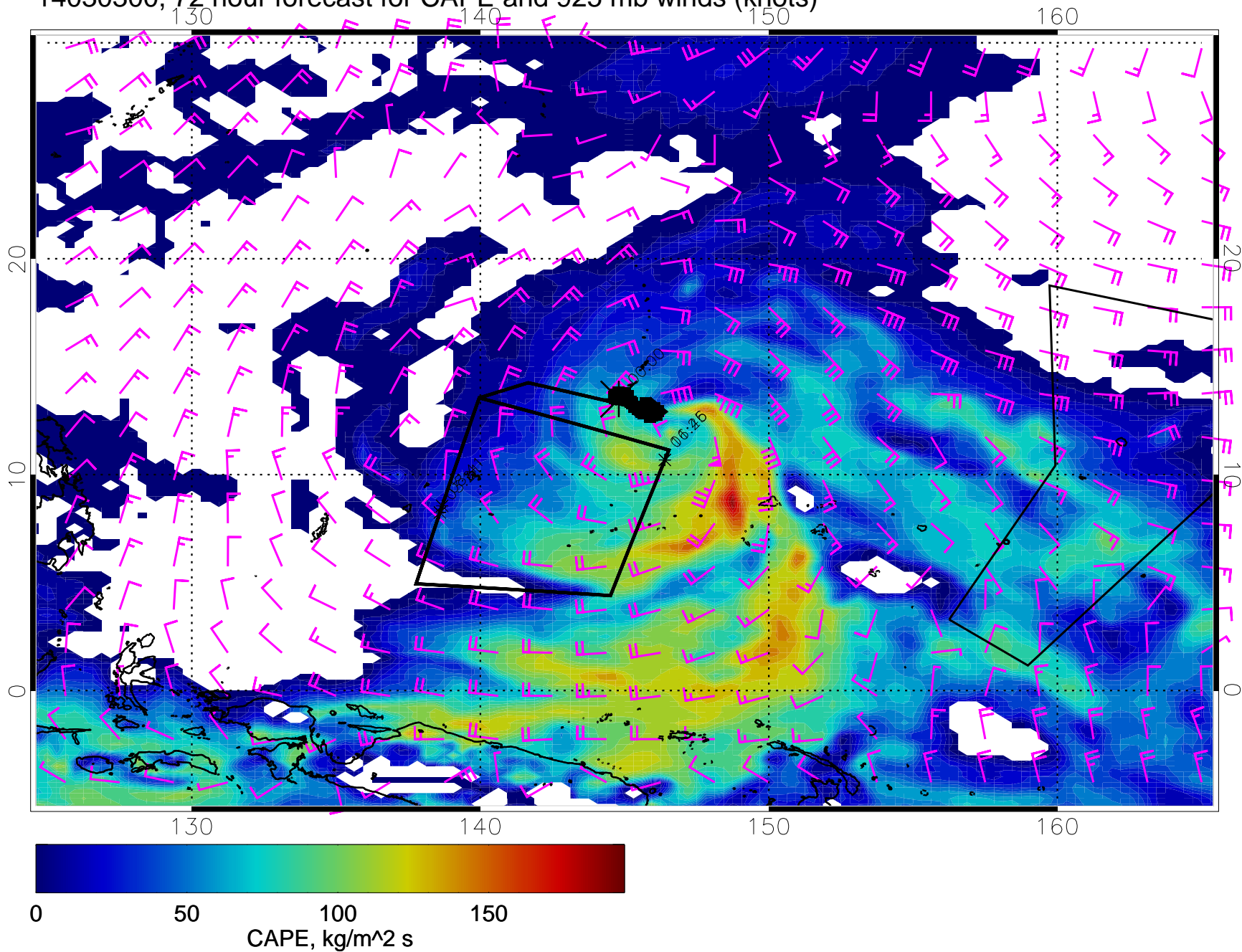
14030300, 72 hour forecast for CAPE and 925 mb winds (knots)
