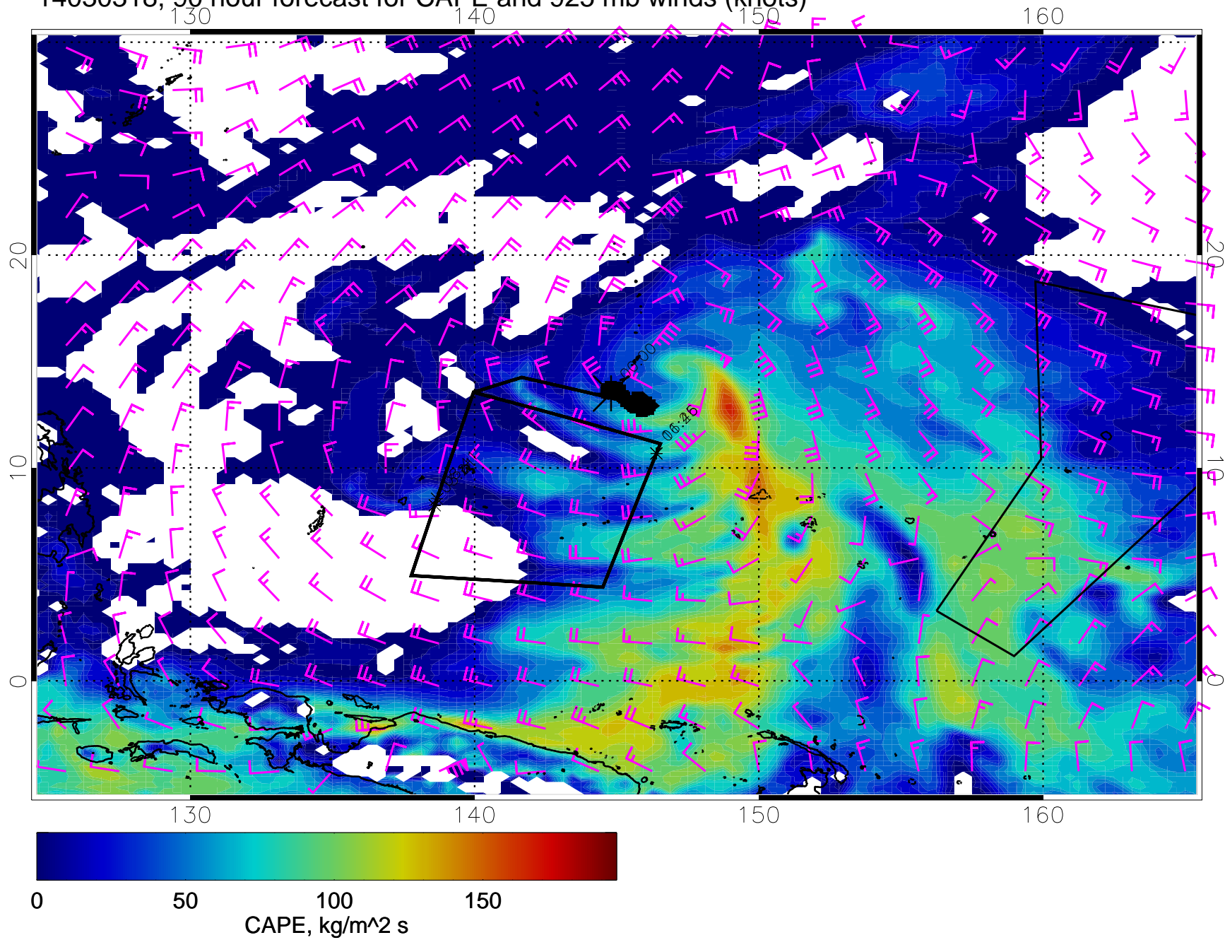
14030318, 90 hour forecast for CAPE and 925 mb winds (knots)
