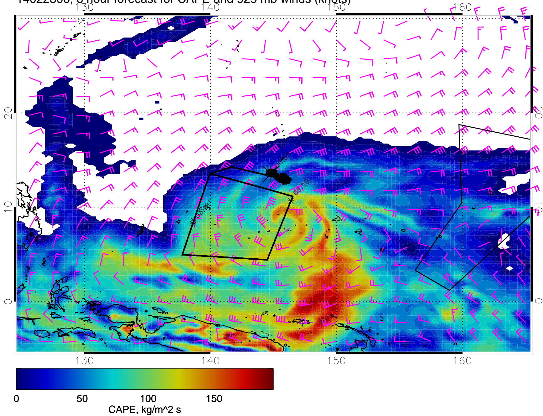
14022806, 6 hour forecast for CAPE and 925 mb winds (knots)
