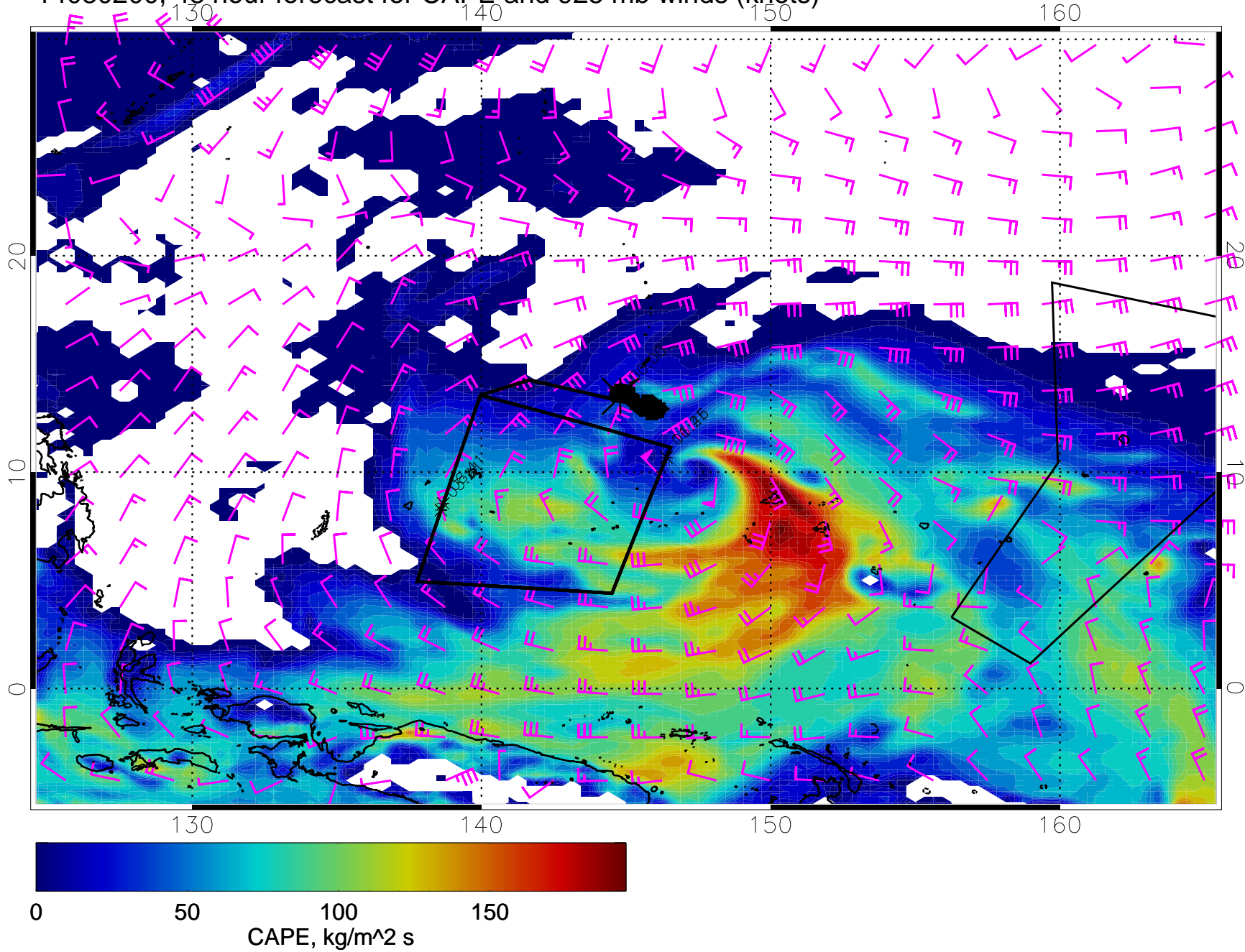
14030200, 48 hour forecast for CAPE and 925 mb winds (knots)
