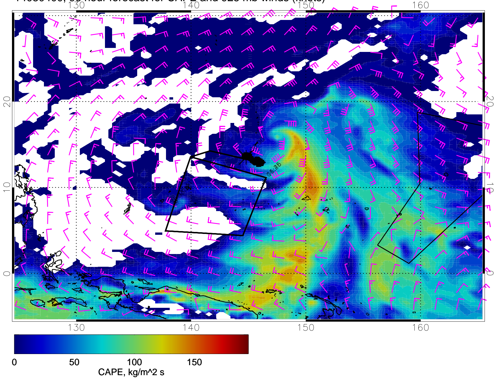
14030400, 96 hour forecast for CAPE and 925 mb winds (knots)
