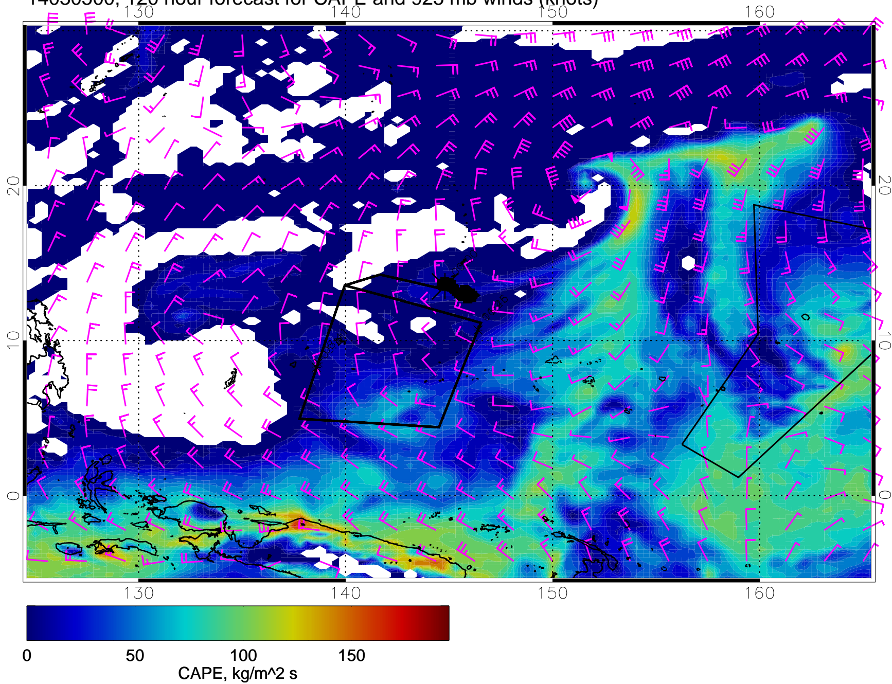
14030500, 120 hour forecast for CAPE and 925 mb winds (knots)
