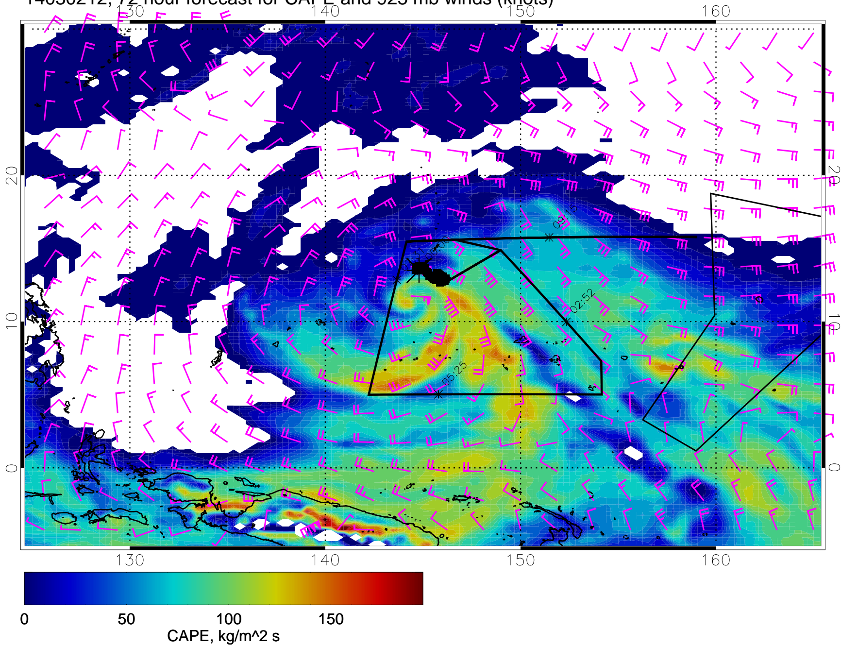
14030212, 72 hour forecast for CAPE and 925 mb winds (knots)
