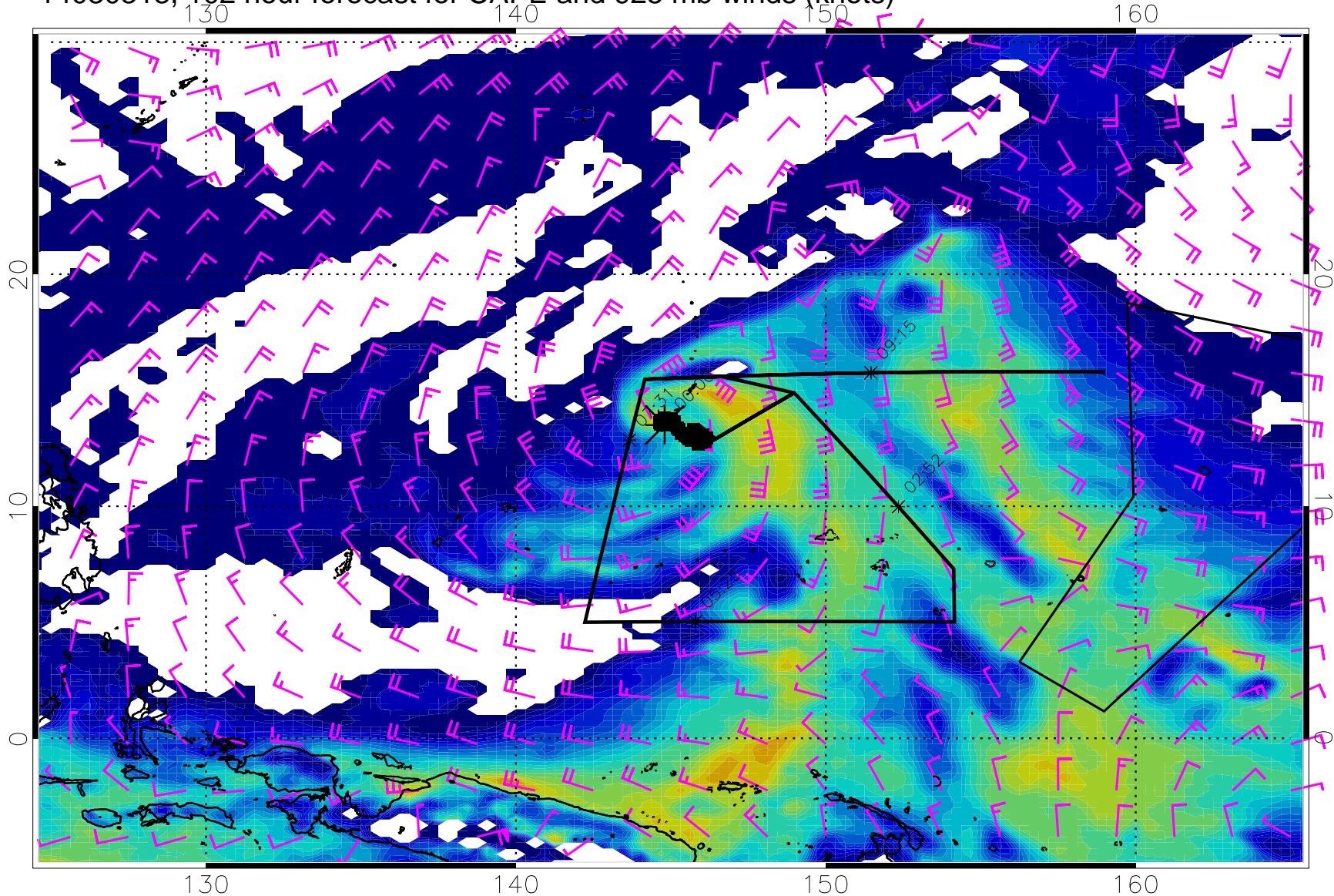
14030318, 102 hour forecast for CAPE and 925 mb winds (knots)
