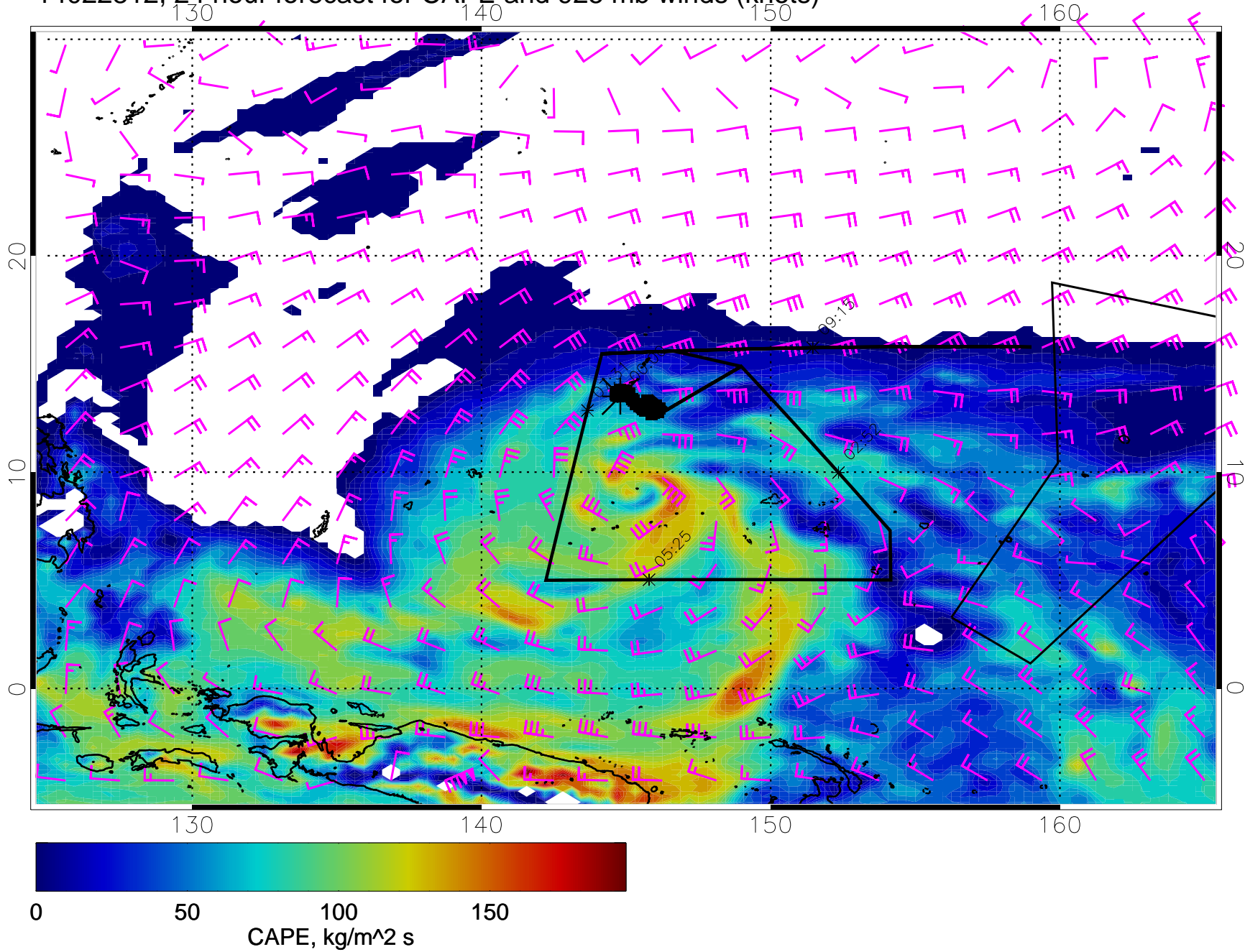
14022812, 24 hour forecast for CAPE and 925 mb winds (knots)
