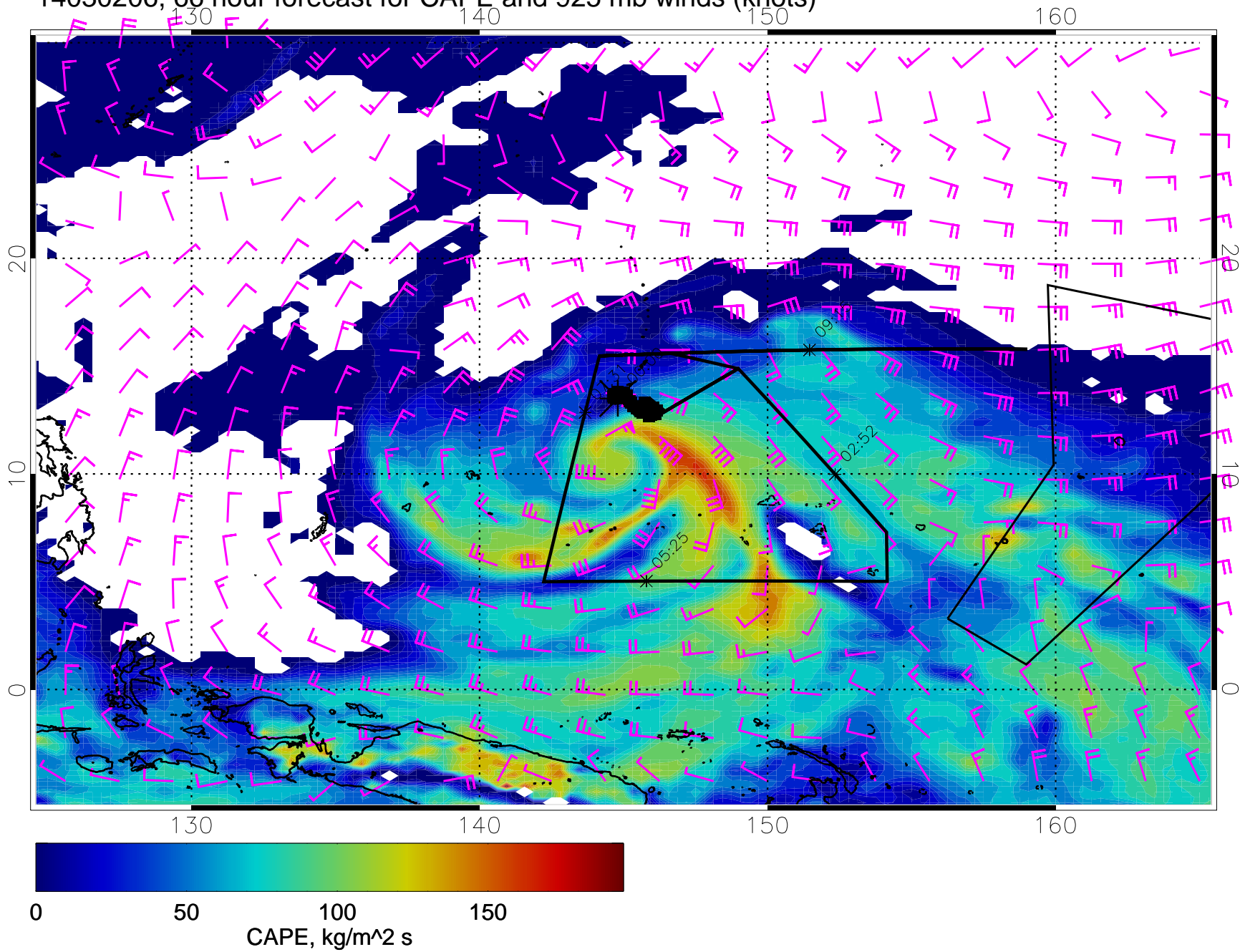
14030206, 66 hour forecast for CAPE and 925 mb winds (knots)
