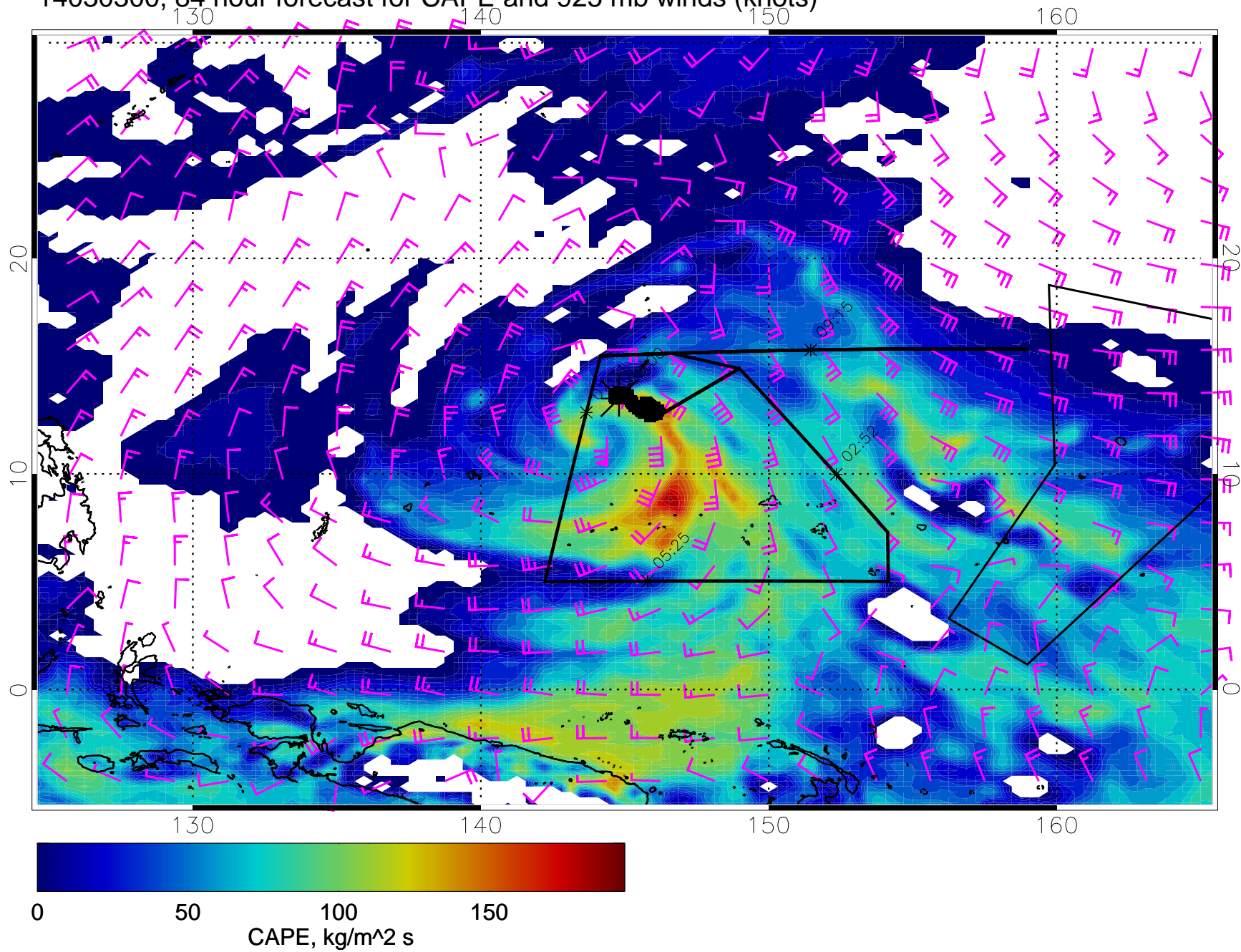
14030300, 84 hour forecast for CAPE and 925 mb winds (knots)
