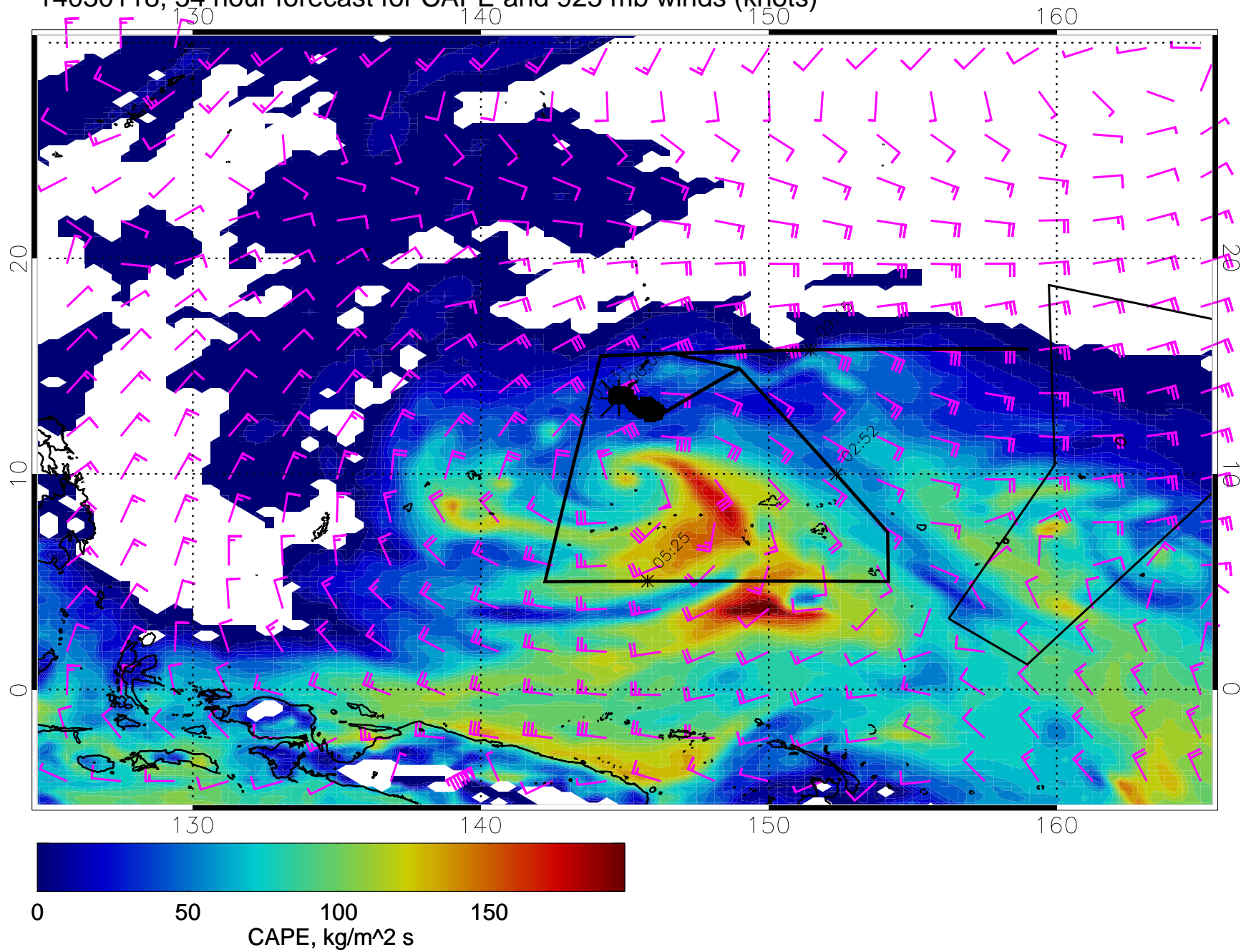
14030118, 54 hour forecast for CAPE and 925 mb winds (knots)
