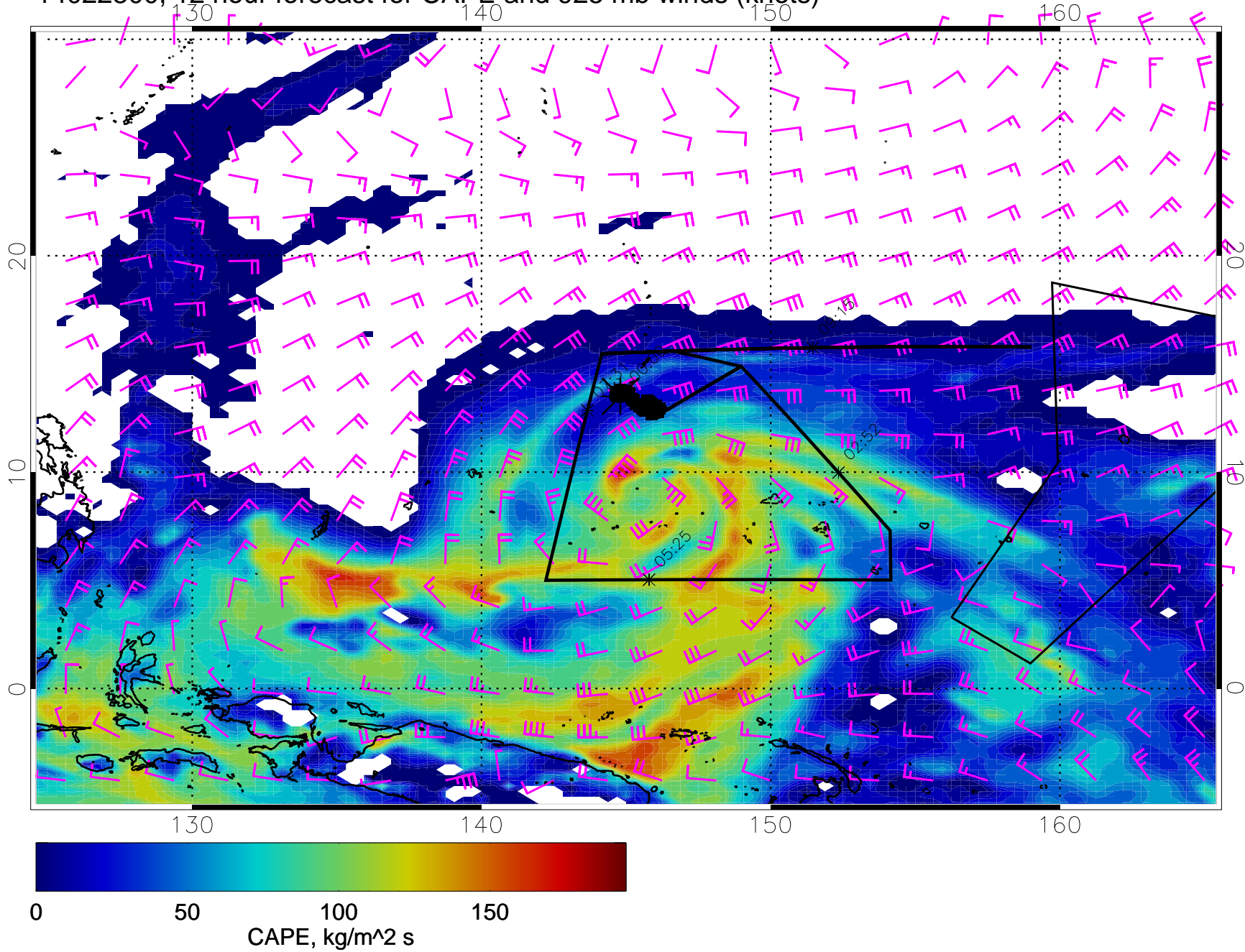
14022800, 12 hour forecast for CAPE and 925 mb winds (knots)
