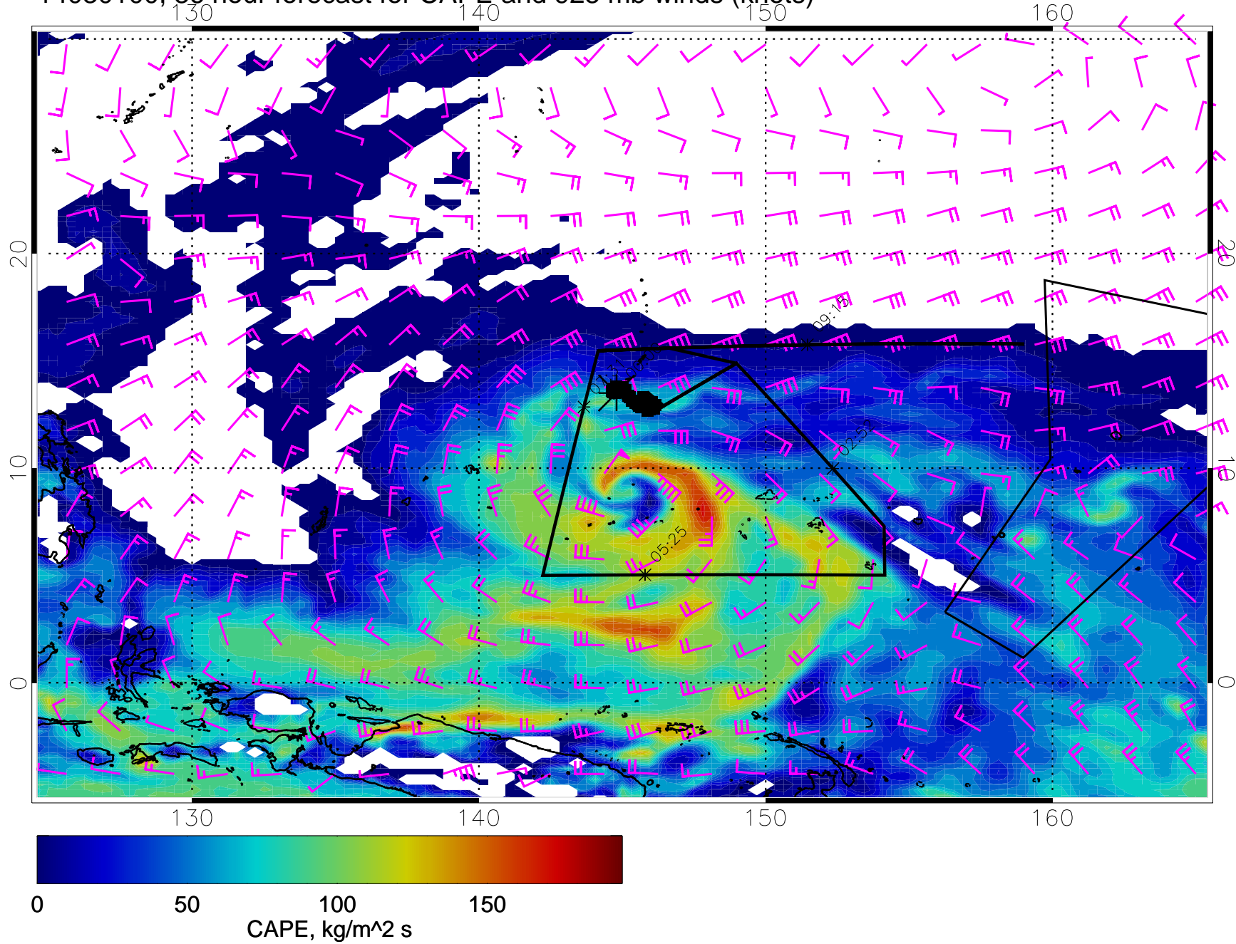
14030100, 36 hour forecast for CAPE and 925 mb winds (knots)
