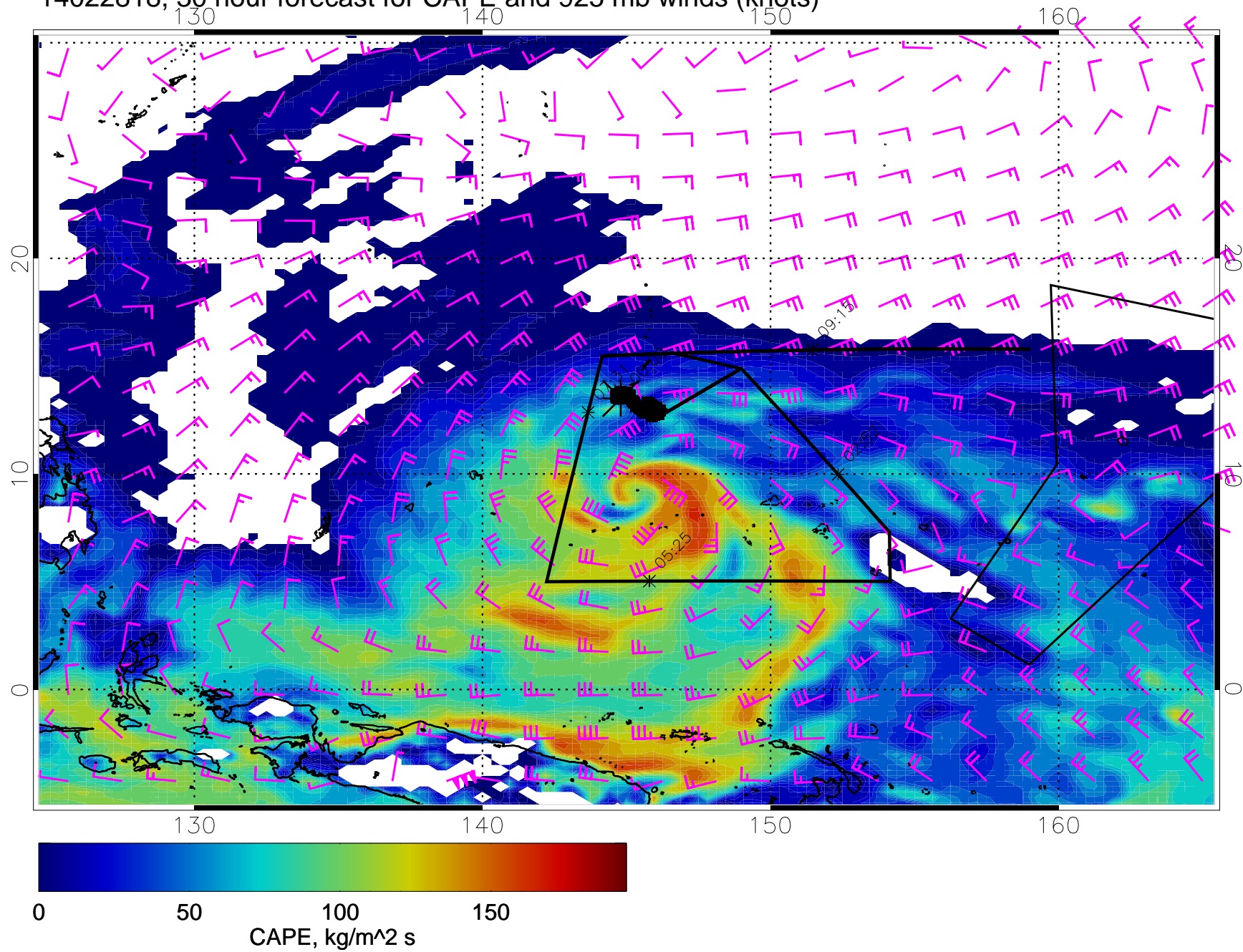
14022818, 30 hour forecast for CAPE and 925 mb winds (knots)
