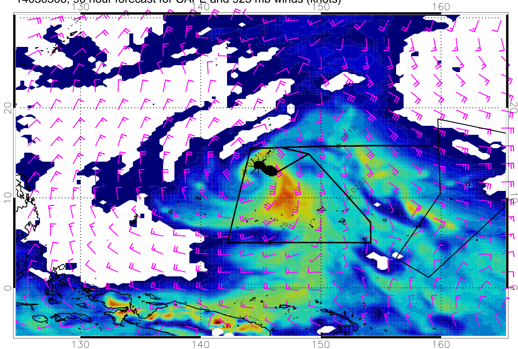
14030306, 90 hour forecast for CAPE and 925 mb winds (knots)
