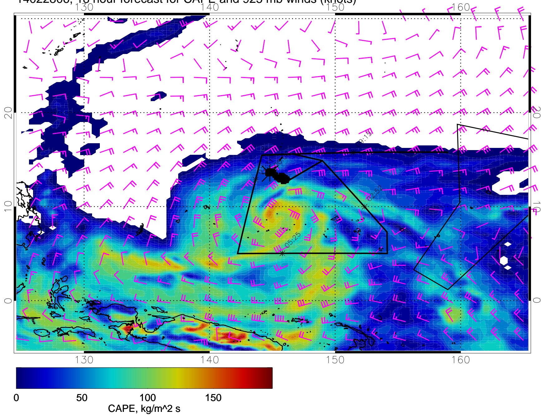
14022806, 18 hour forecast for CAPE and 925 mb winds (knots)
