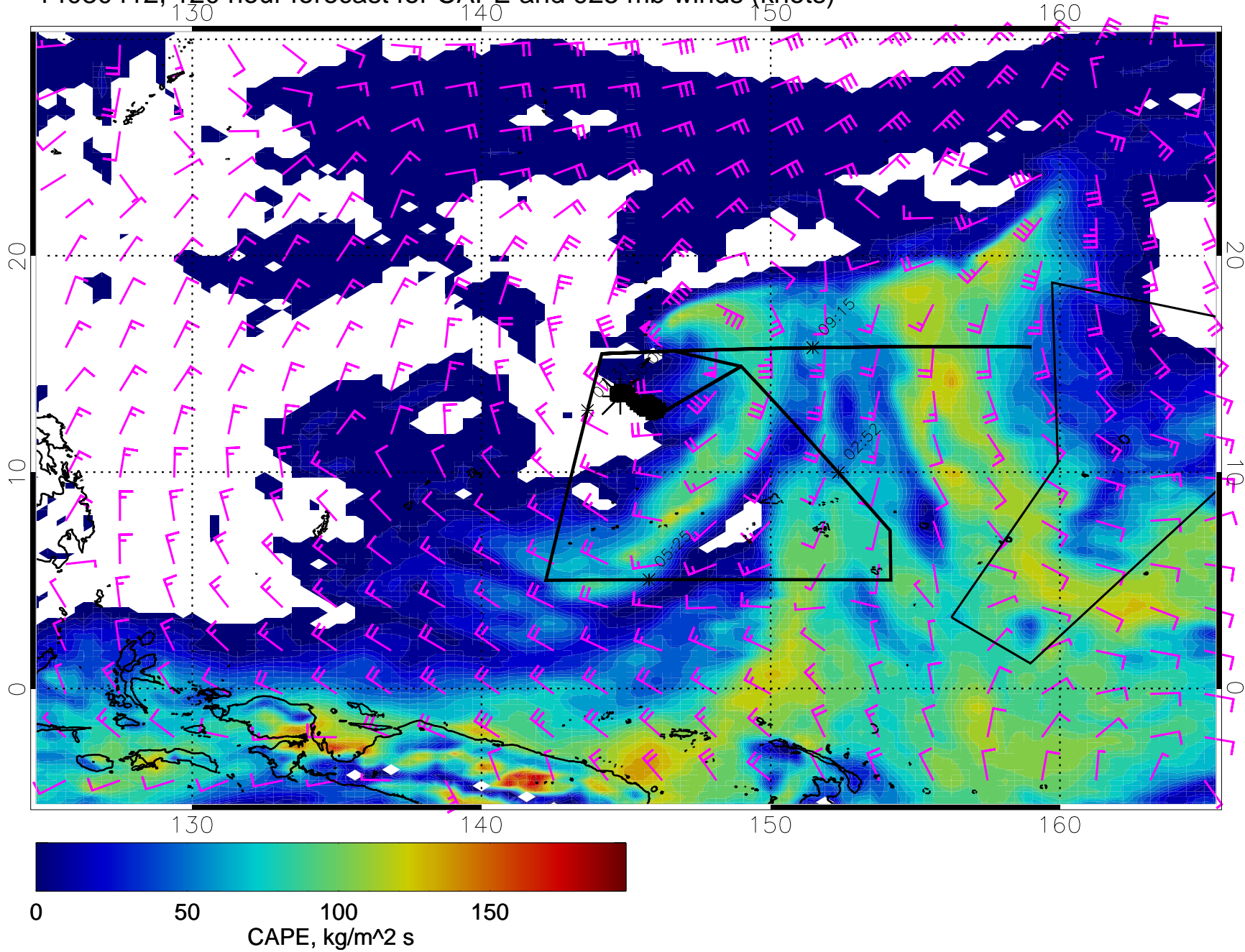
14030412, 120 hour forecast for CAPE and 925 mb winds (knots)
