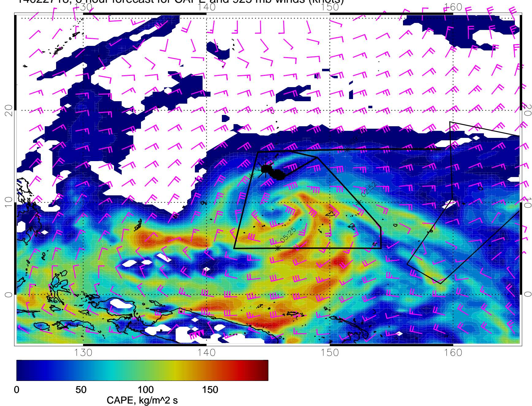
14022718, 6 hour forecast for CAPE and 925 mb winds (knots)
