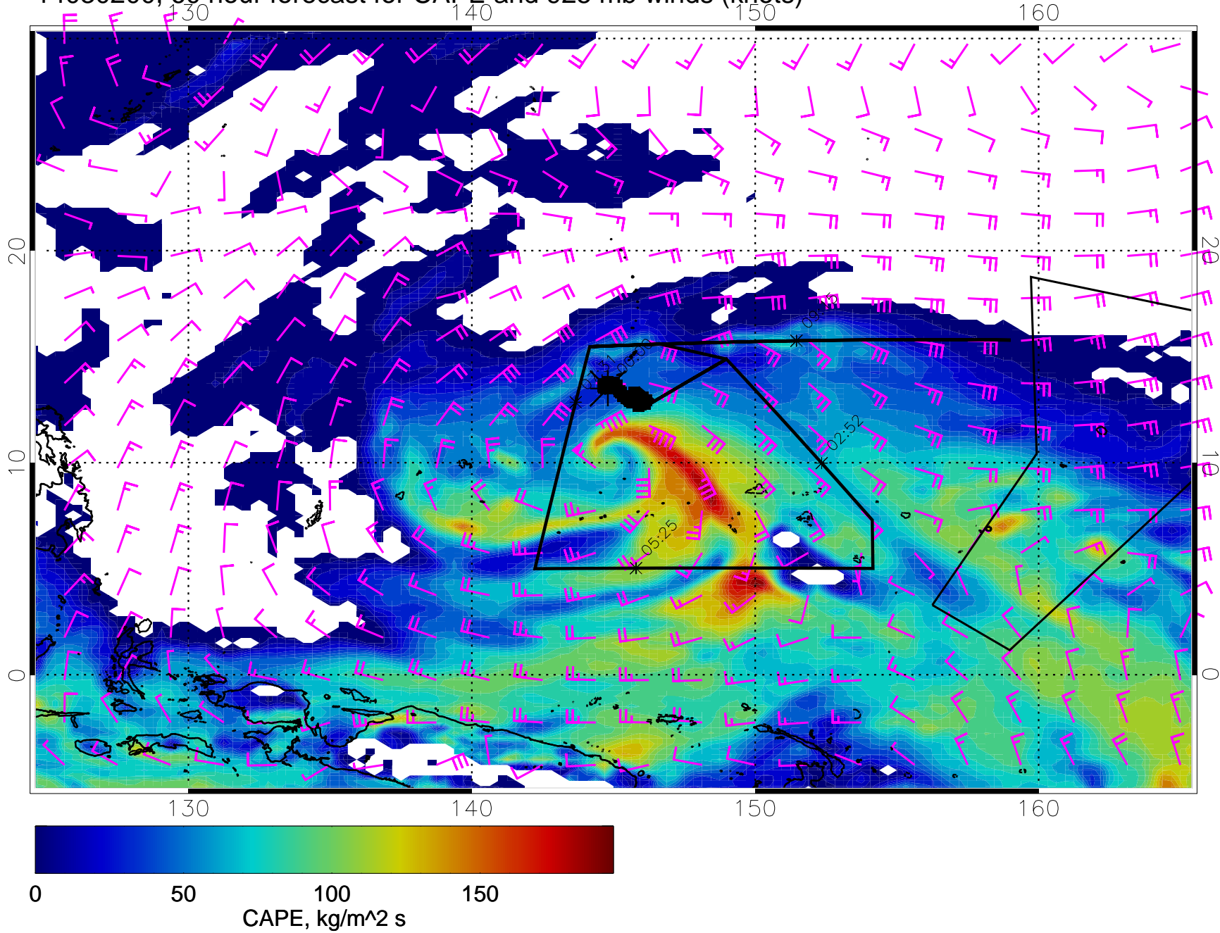
14030200, 60 hour forecast for CAPE and 925 mb winds (knots)
