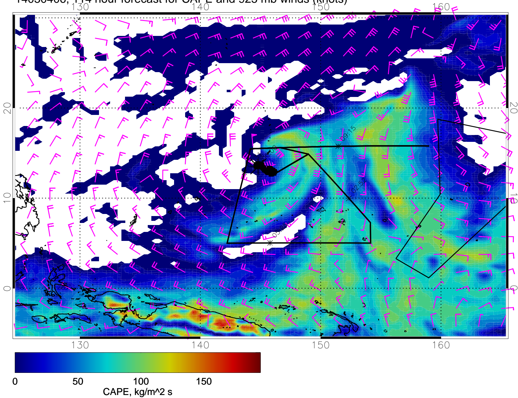
14030406, 114 hour forecast for CAPE and 925 mb winds (knots)
