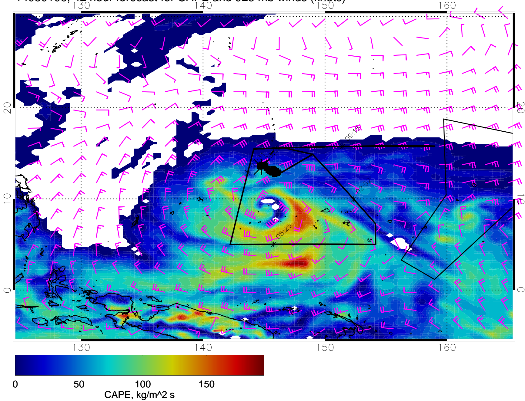
14030106, 42 hour forecast for CAPE and 925 mb winds (knots)
