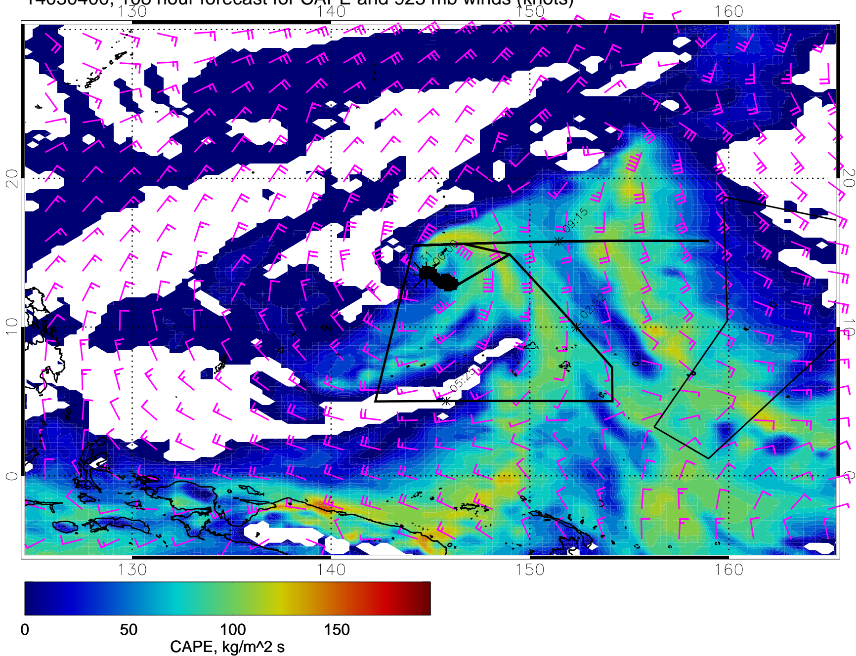
14030400, 108 hour forecast for CAPE and 925 mb winds (knots)
