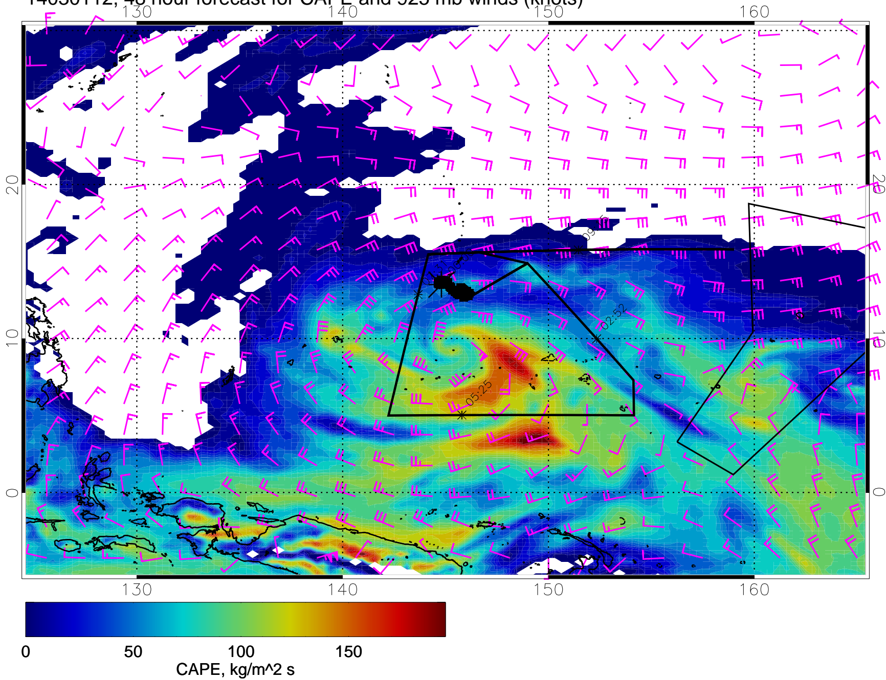
14030112, 48 hour forecast for CAPE and 925 mb winds (knots)
