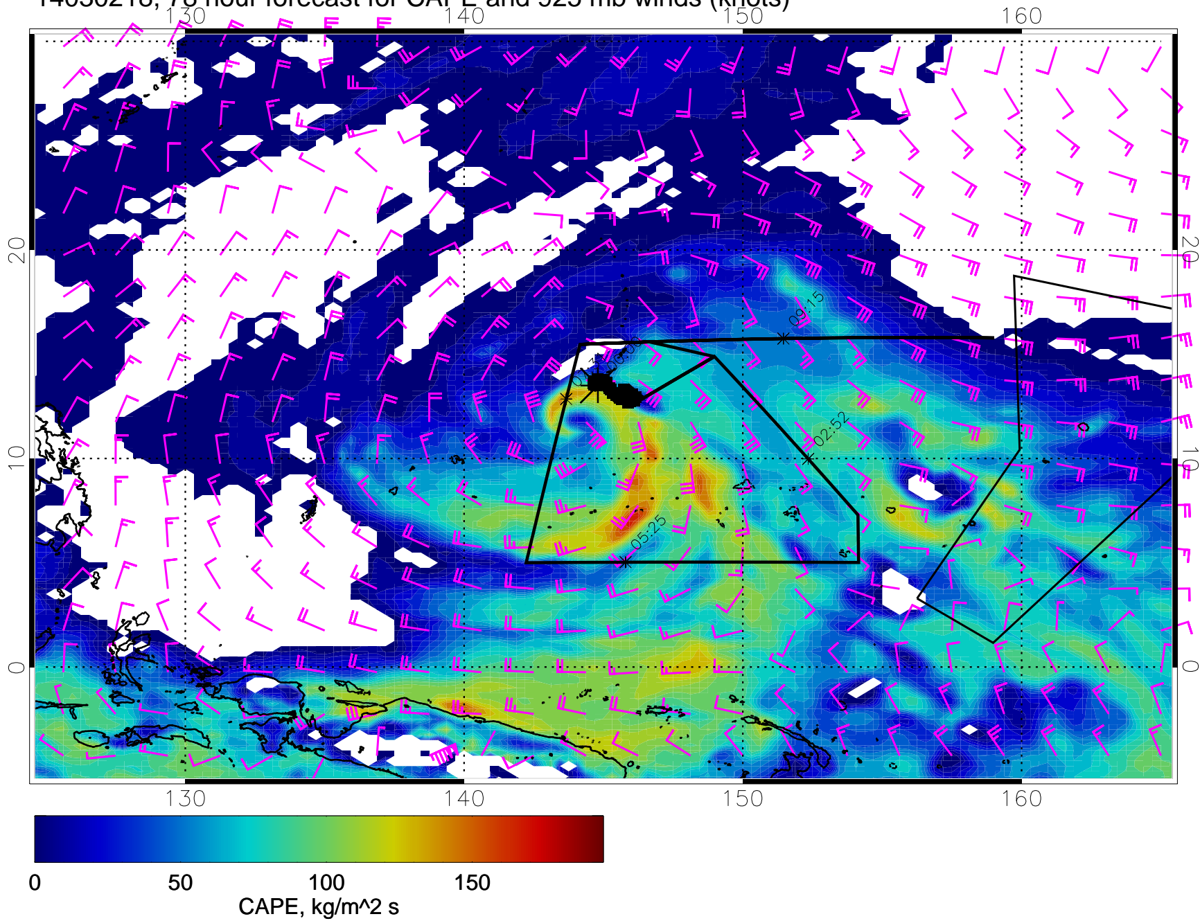
14030218, 78 hour forecast for CAPE and 925 mb winds (knots)
