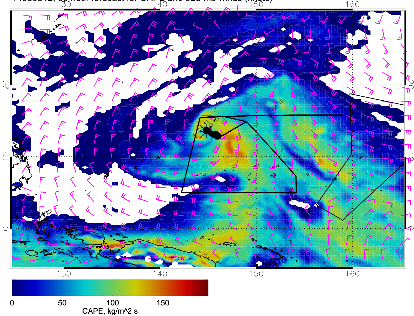
14030312, 96 hour forecast for CAPE and 925 mb winds (knots)
