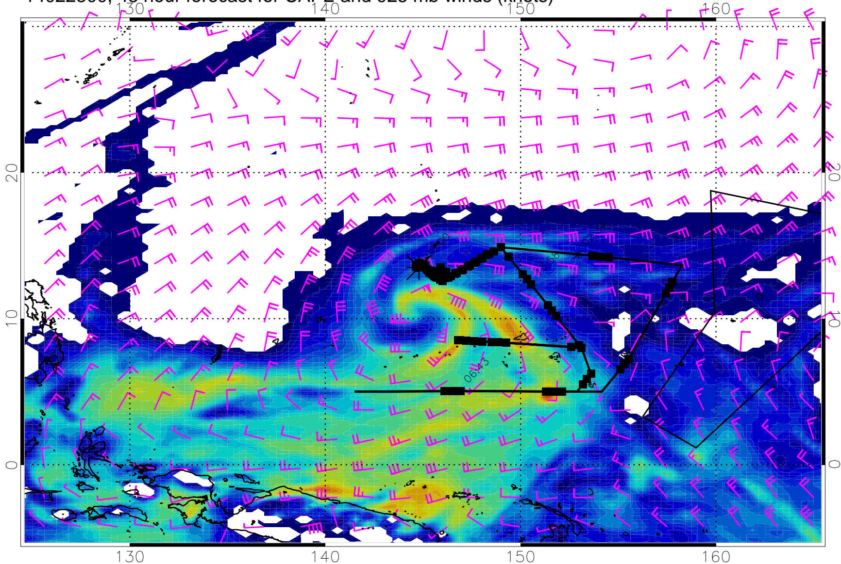
14022800, 48 hour forecast for CAPE and 925 mb winds (knots)
