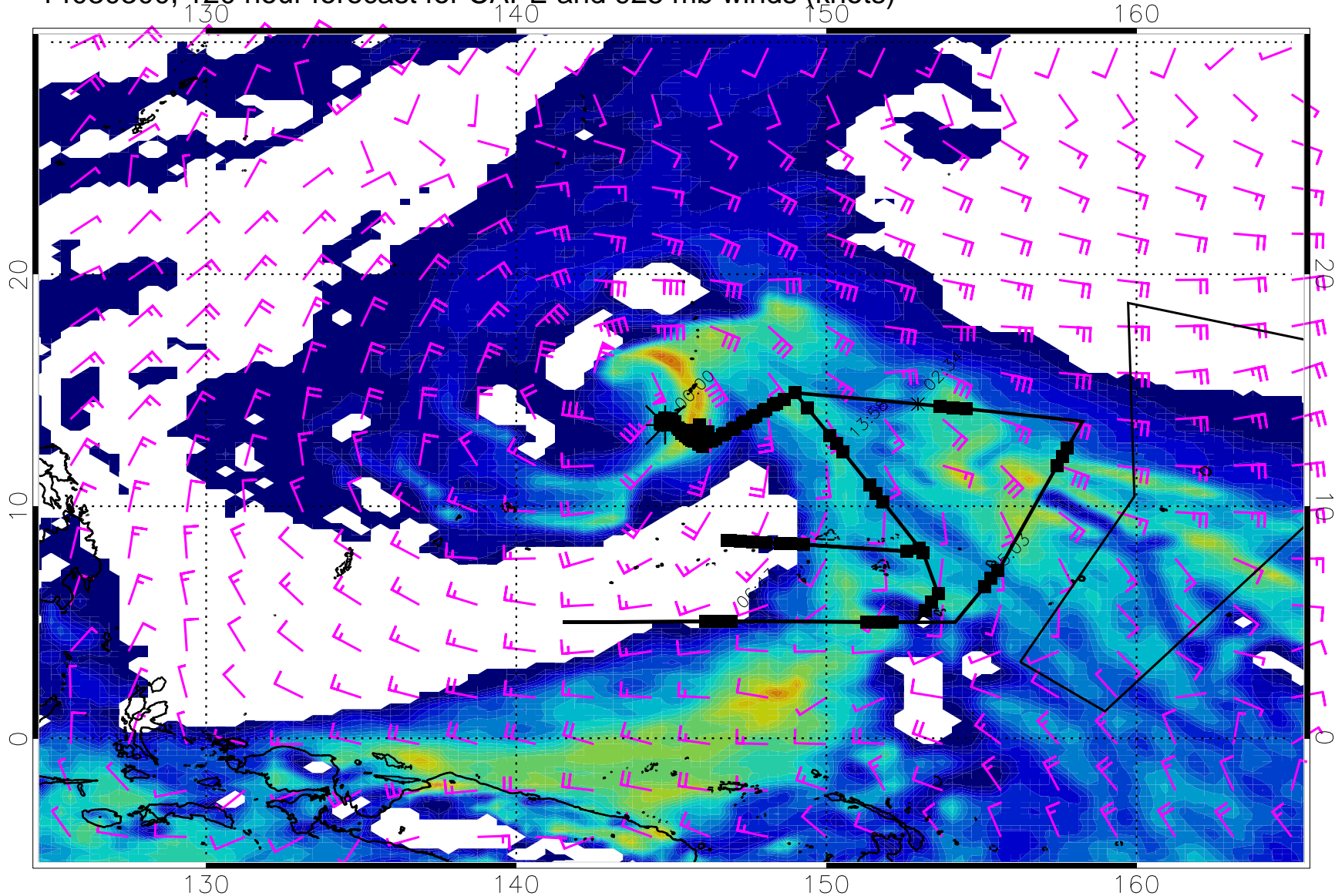
14030300, 120 hour forecast for CAPE and 925 mb winds (knots)
