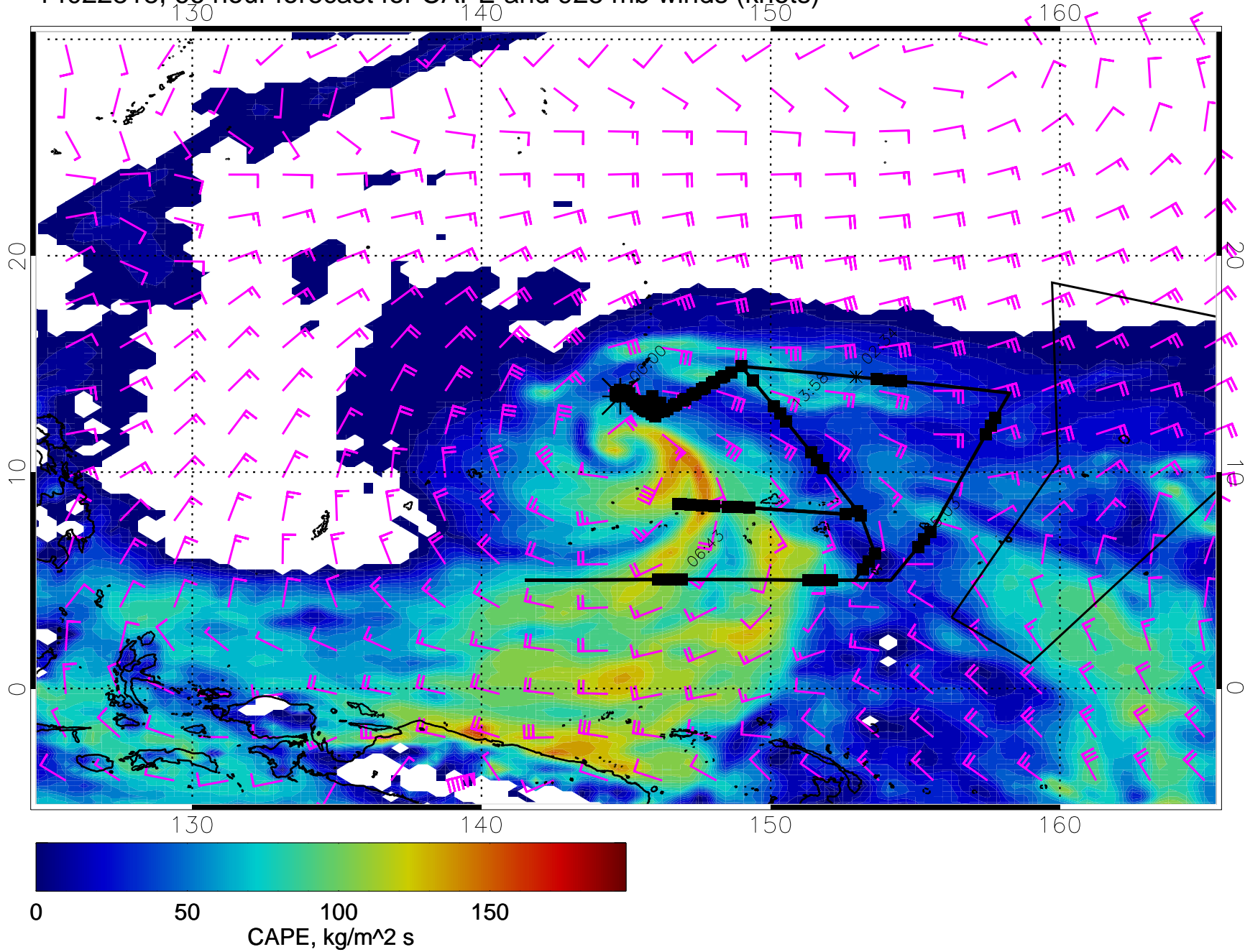
14022818, 66 hour forecast for CAPE and 925 mb winds (knots)
