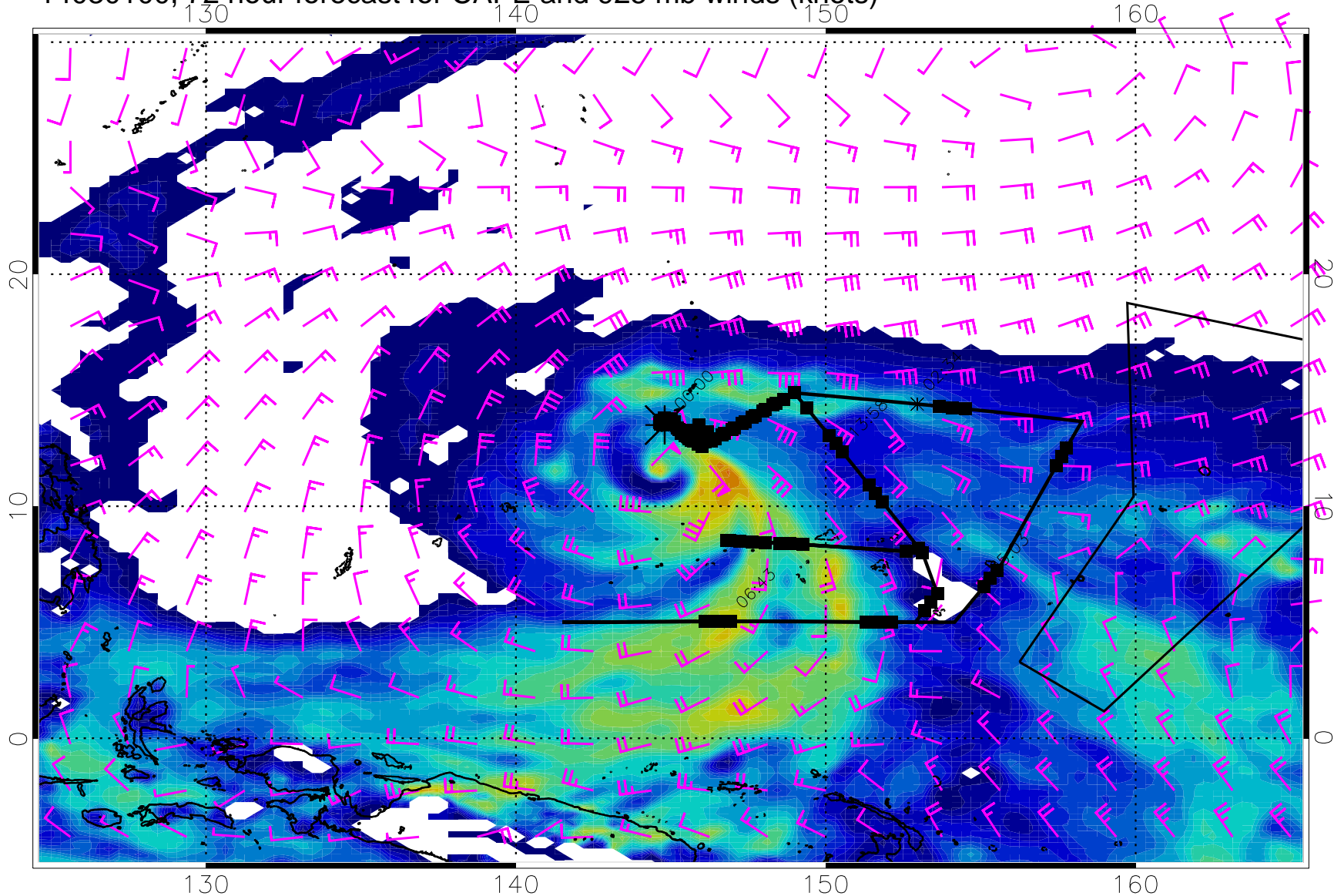
14030100, 72 hour forecast for CAPE and 925 mb winds (knots)
