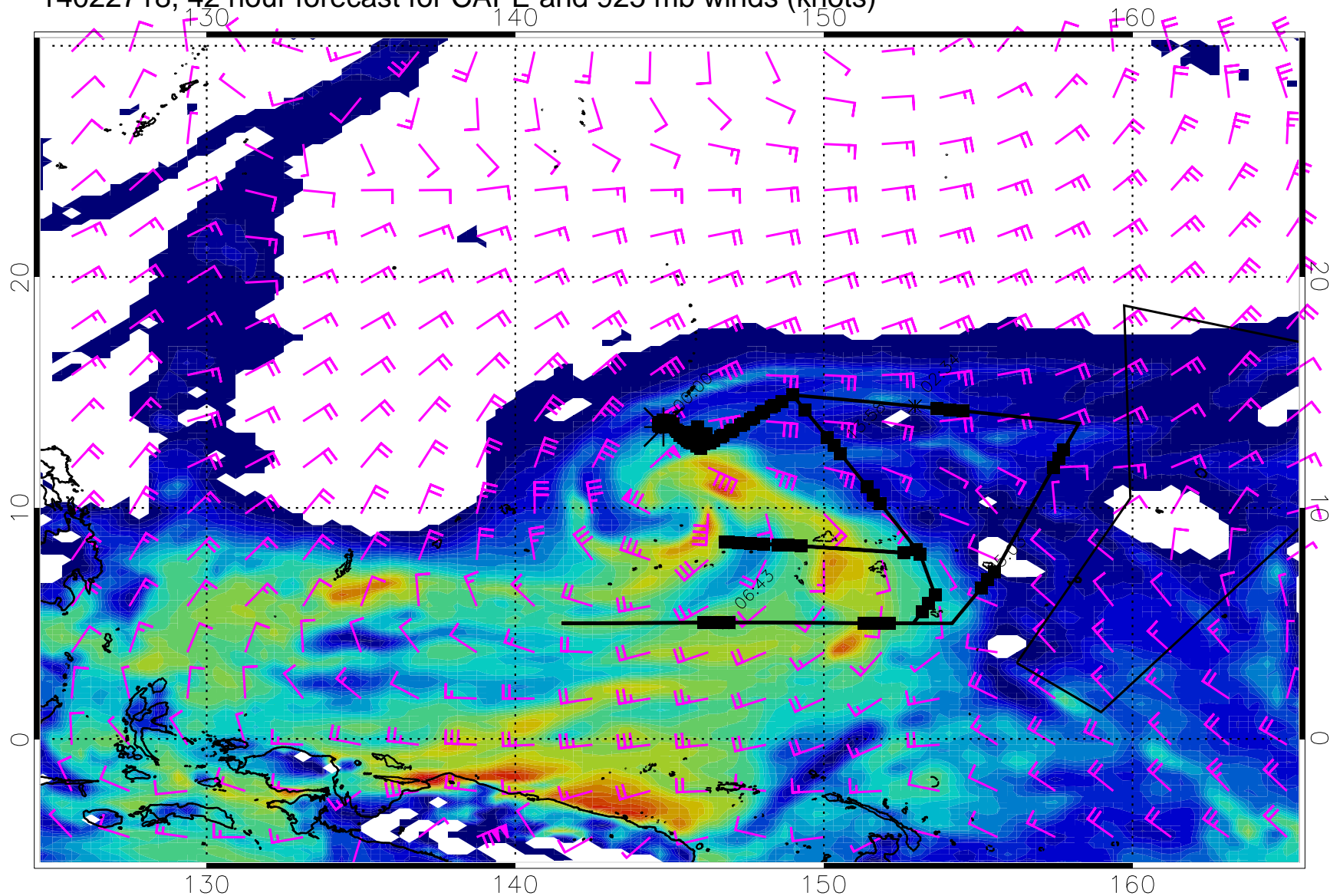
14022718, 42 hour forecast for CAPE and 925 mb winds (knots)
