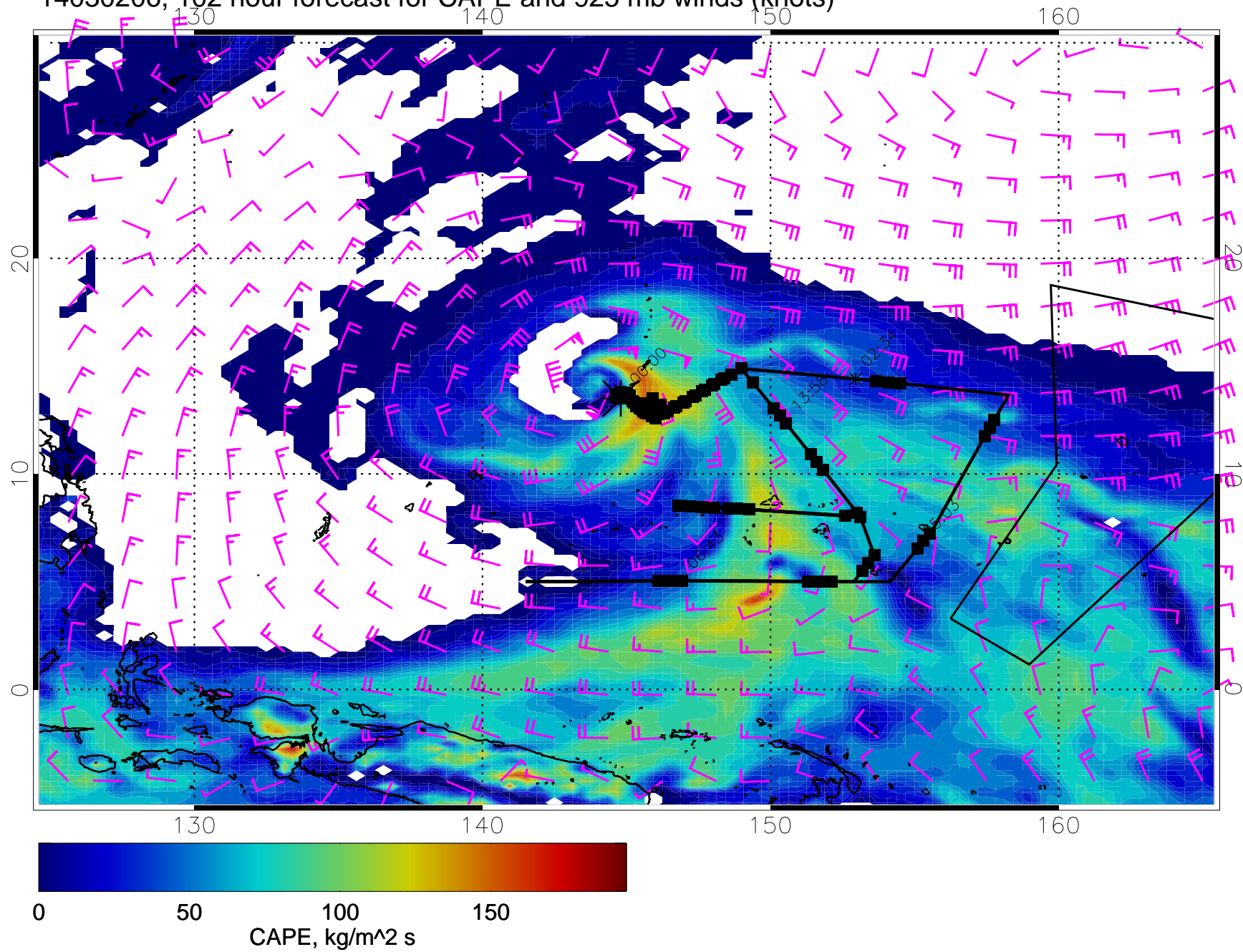
14030206, 102 hour forecast for CAPE and 925 mb winds (knots)
