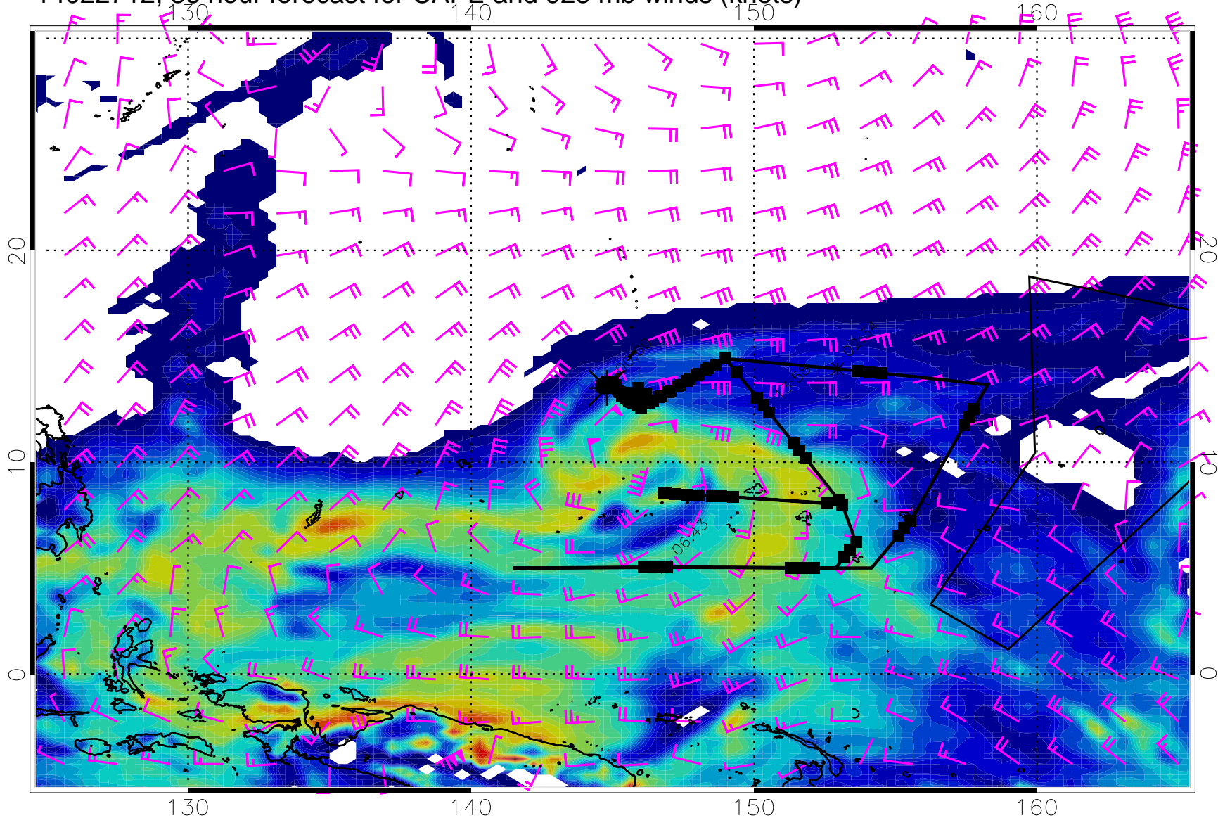
14022712, 36 hour forecast for CAPE and 925 mb winds (knots)
