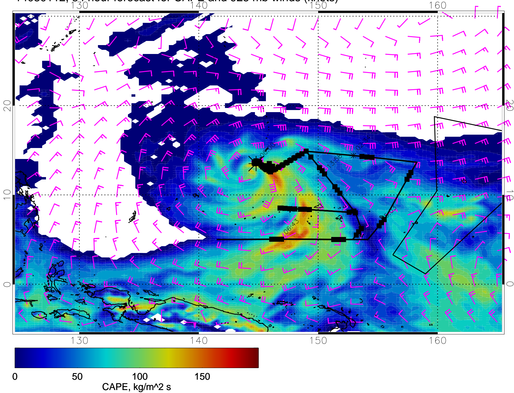
14030112, 84 hour forecast for CAPE and 925 mb winds (knots)
