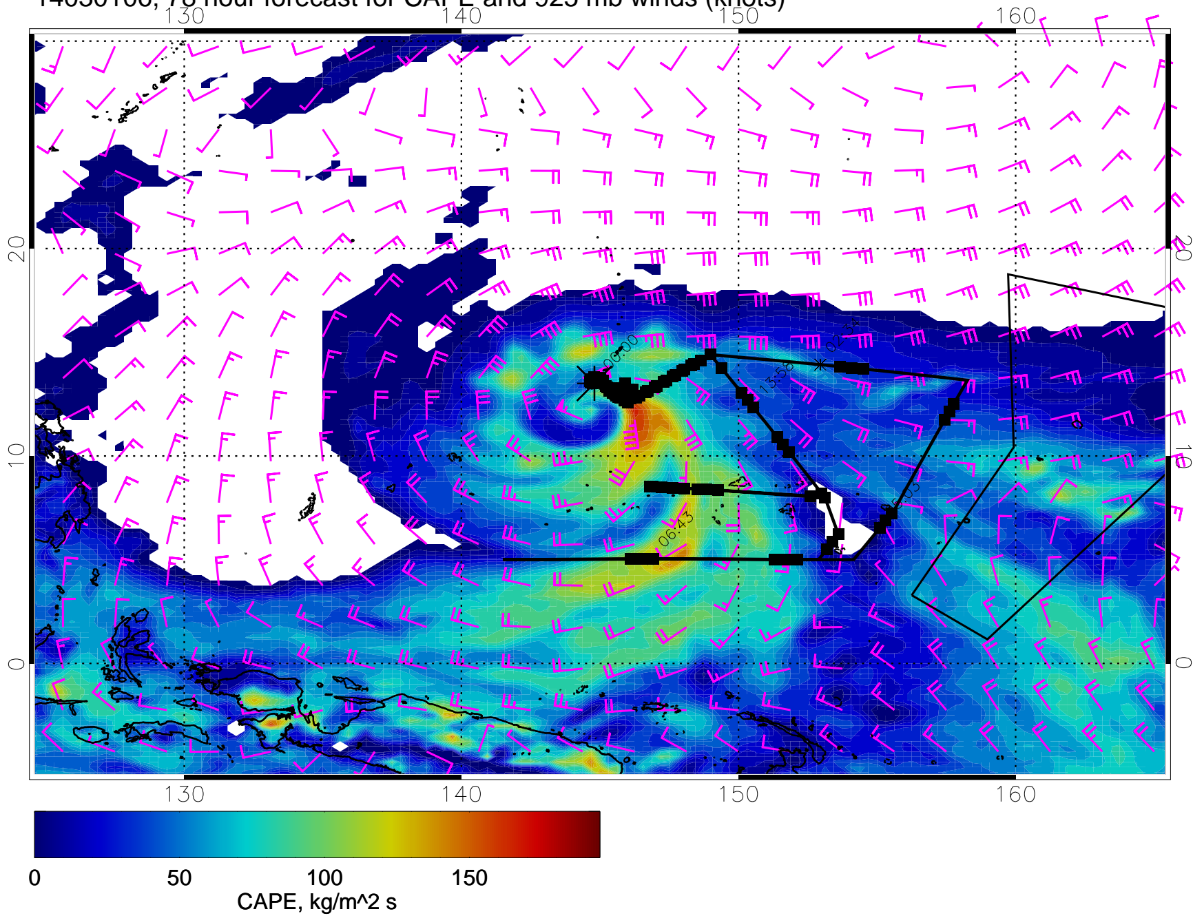
14030106, 78 hour forecast for CAPE and 925 mb winds (knots)
