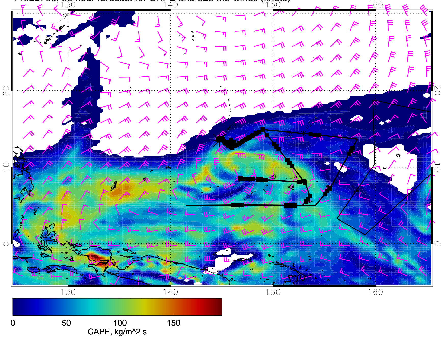
14022706, 30 hour forecast for CAPE and 925 mb winds (knots)
