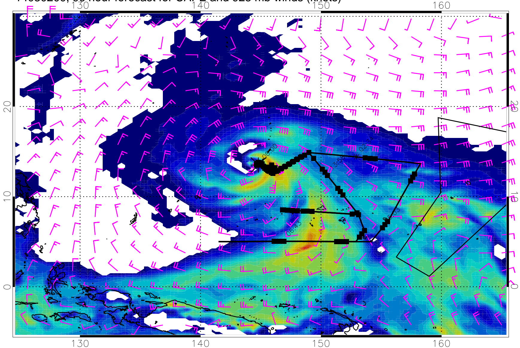
14030200, 96 hour forecast for CAPE and 925 mb winds (knots)
