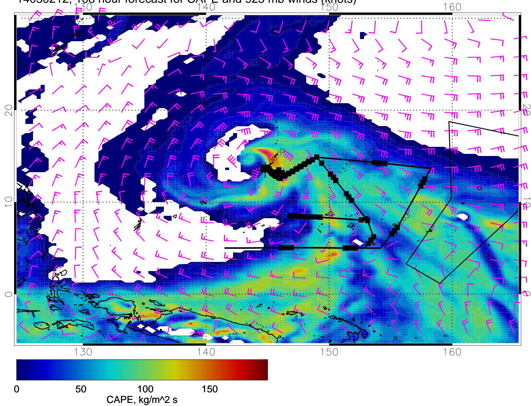
14030212, 108 hour forecast for CAPE and 925 mb winds (knots)
