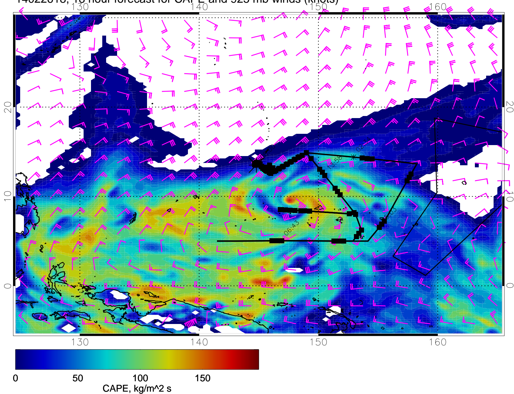
14022618, 18 hour forecast for CAPE and 925 mb winds (knots)
