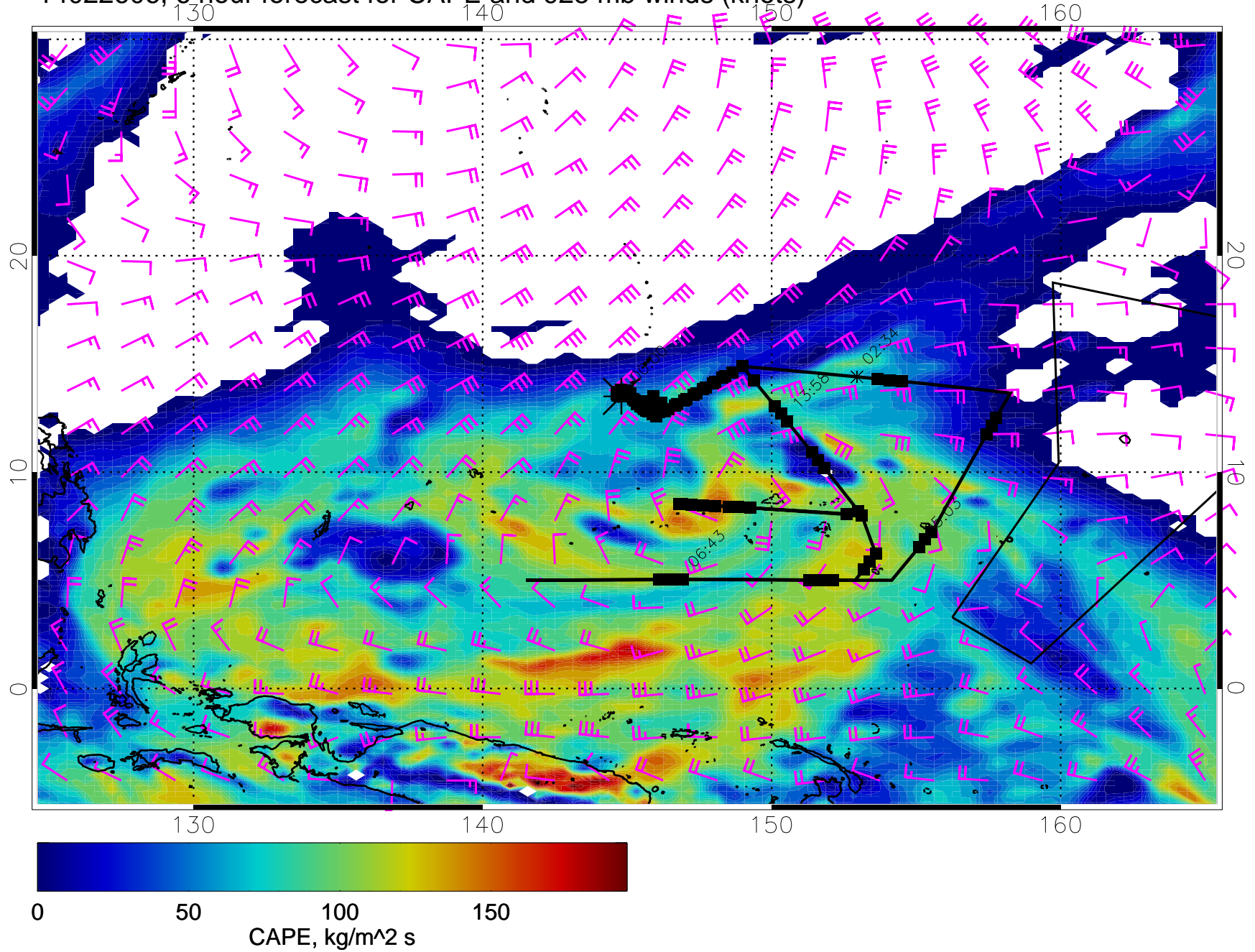
14022606, 6 hour forecast for CAPE and 925 mb winds (knots)
