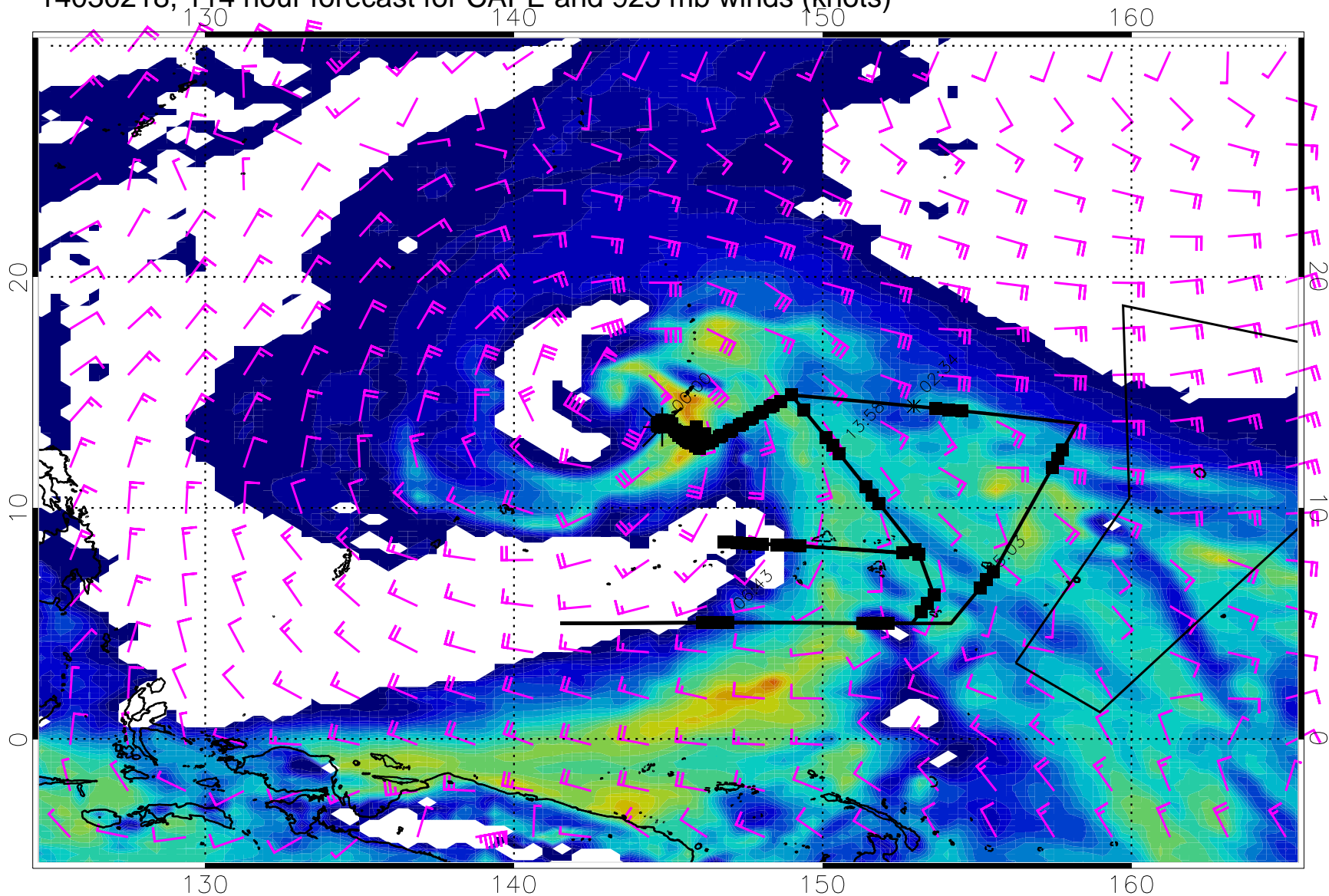
14030218, 114 hour forecast for CAPE and 925 mb winds (knots)
