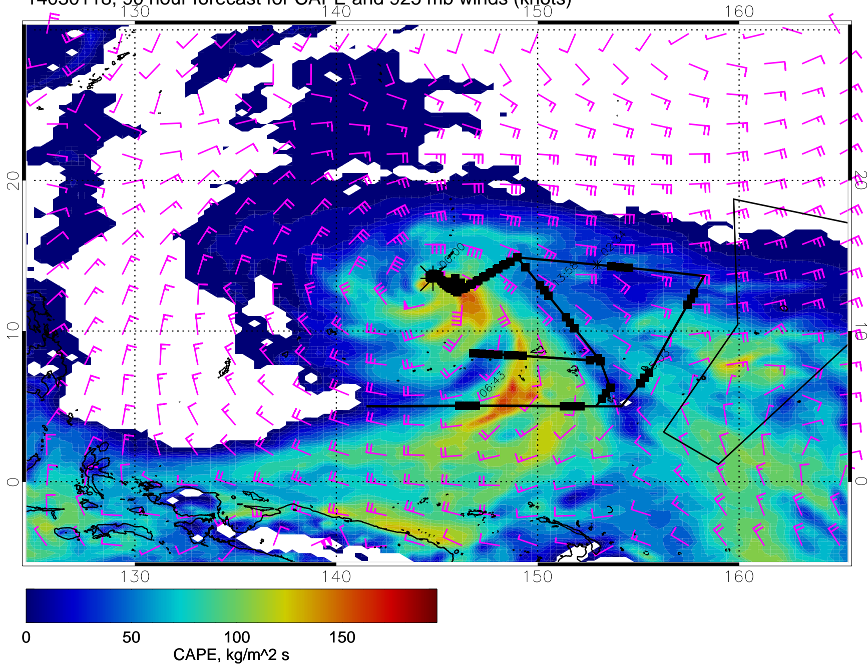
14030118, 90 hour forecast for CAPE and 925 mb winds (knots)
