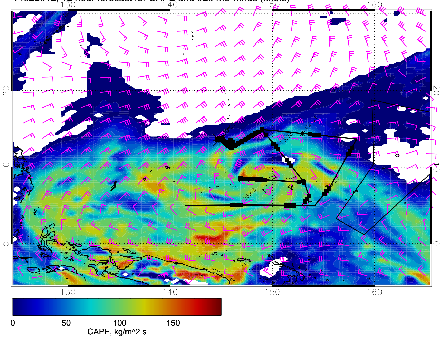
14022612, 12 hour forecast for CAPE and 925 mb winds (knots)
