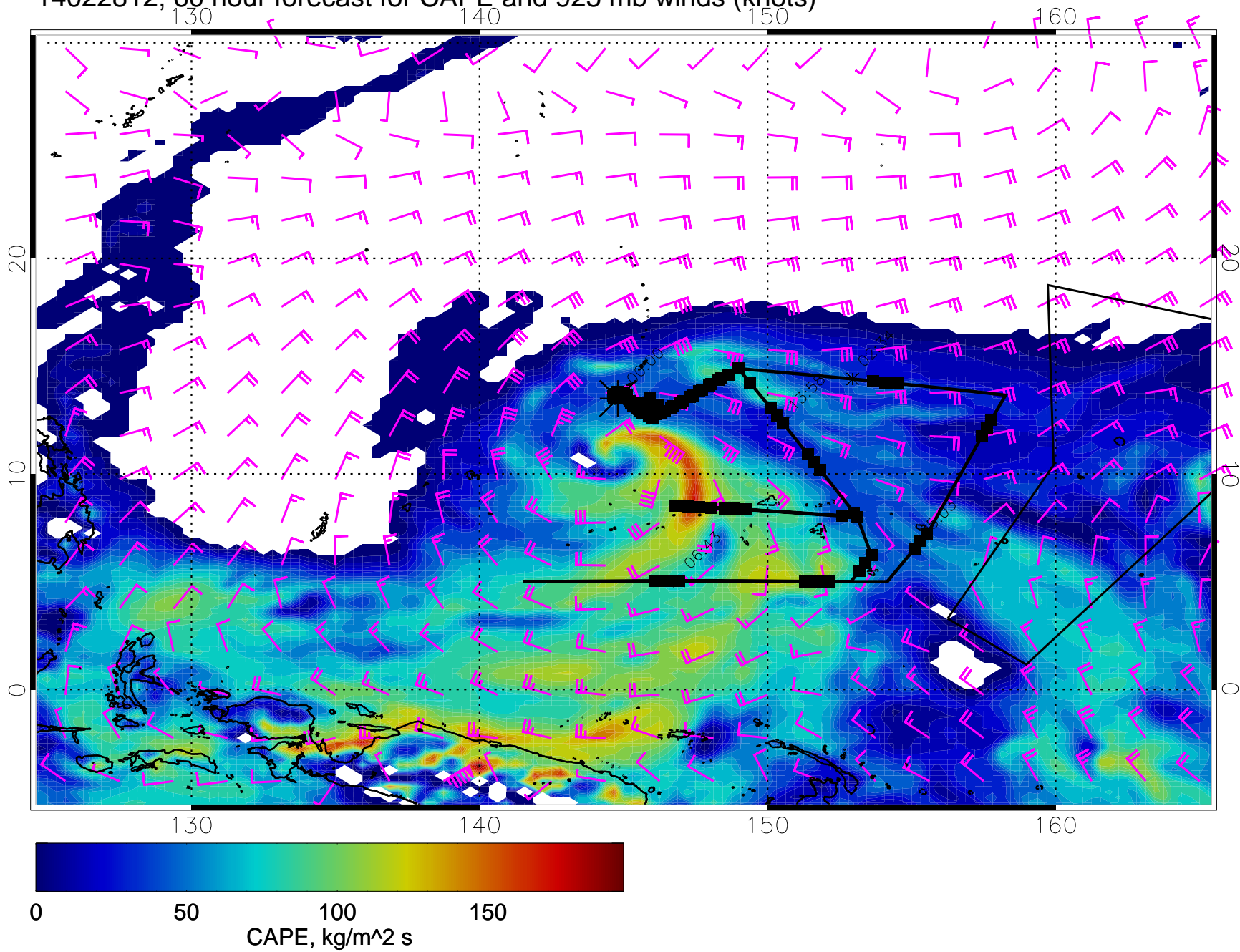
14022812, 60 hour forecast for CAPE and 925 mb winds (knots)
