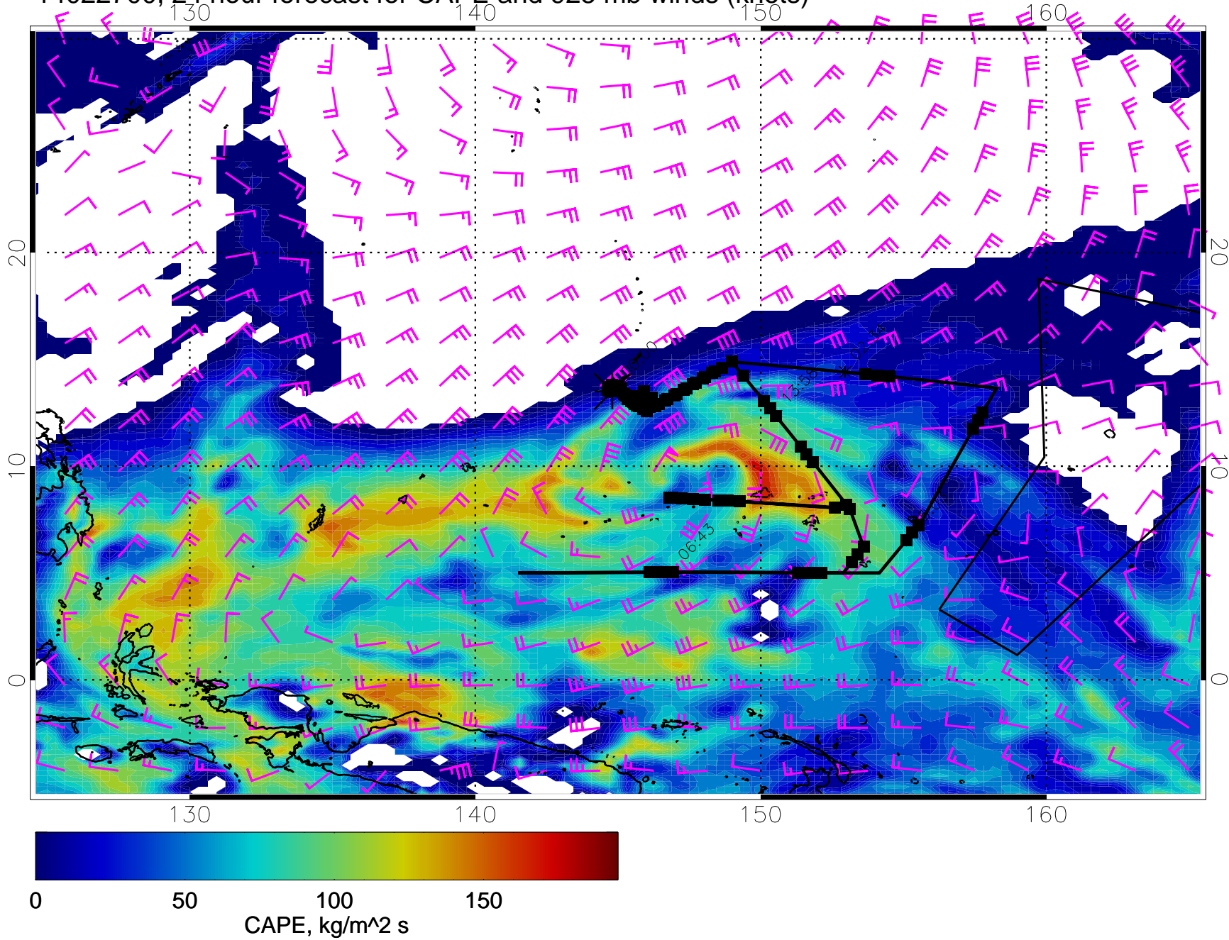
14022700, 24 hour forecast for CAPE and 925 mb winds (knots)
