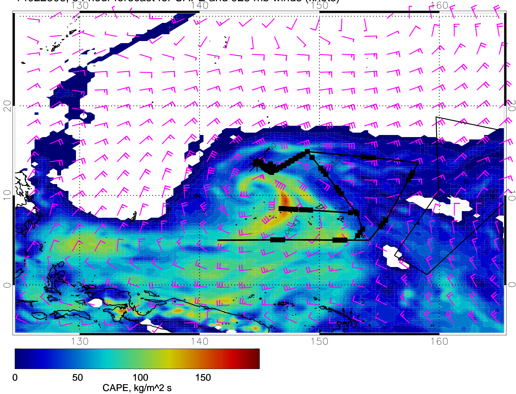
14022806, 54 hour forecast for CAPE and 925 mb winds (knots)
