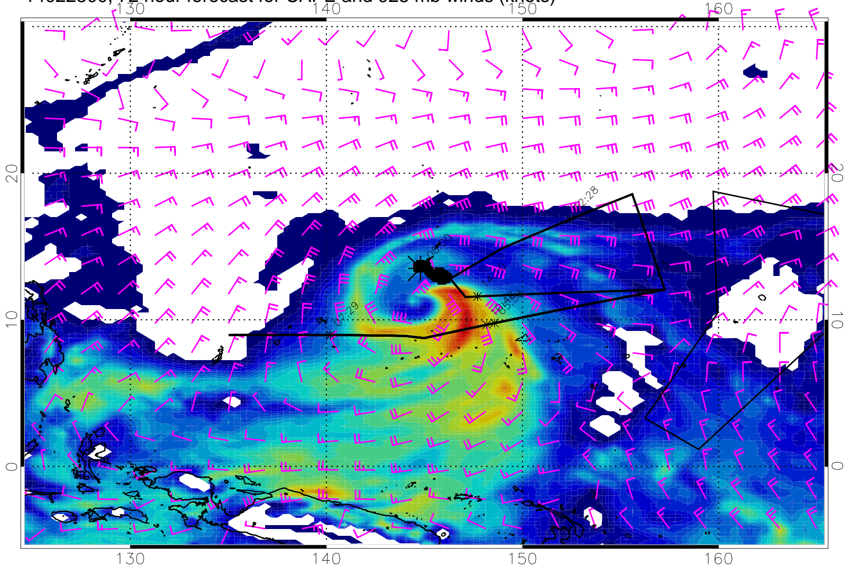
14022800, 72 hour forecast for CAPE and 925 mb winds (knots)
