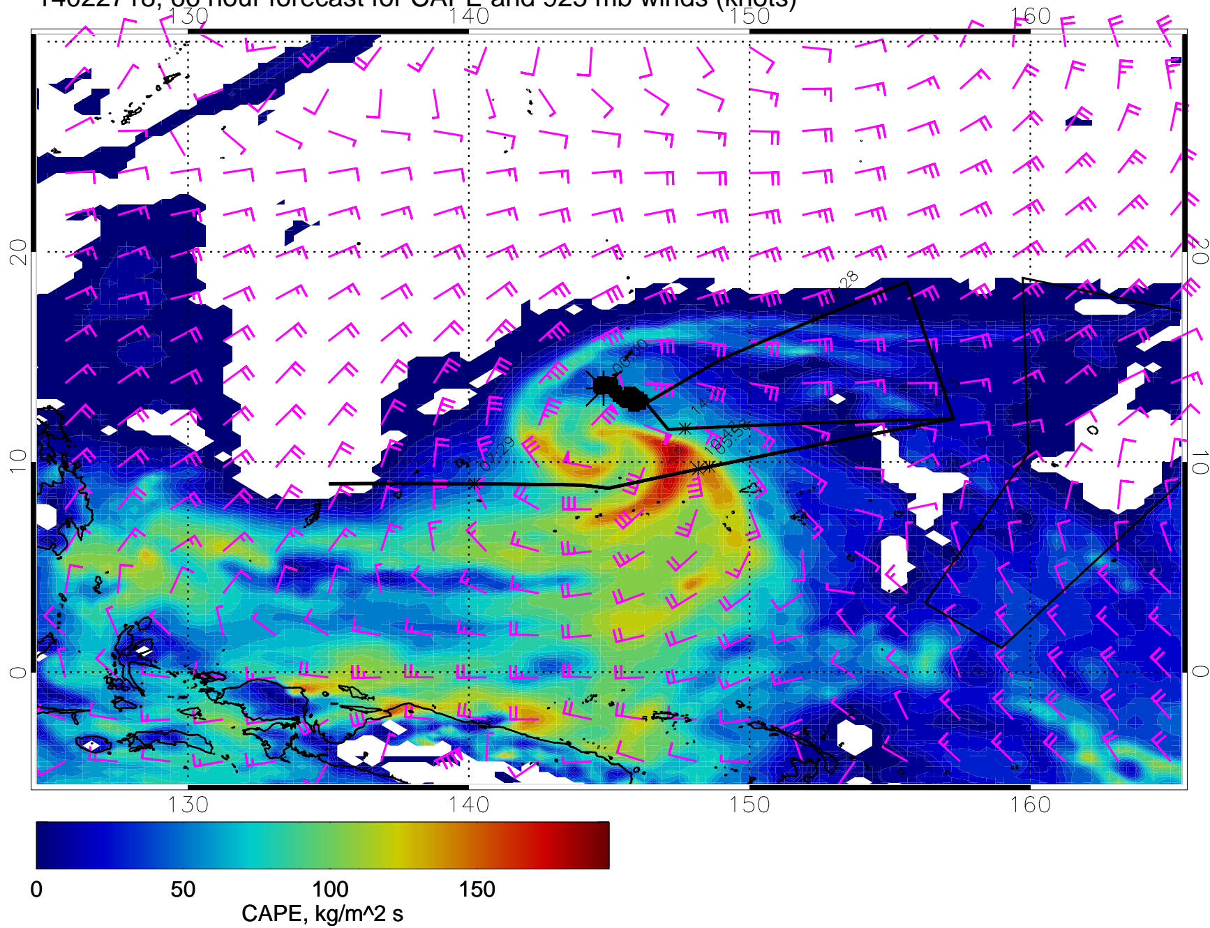
14022718, 66 hour forecast for CAPE and 925 mb winds (knots)
