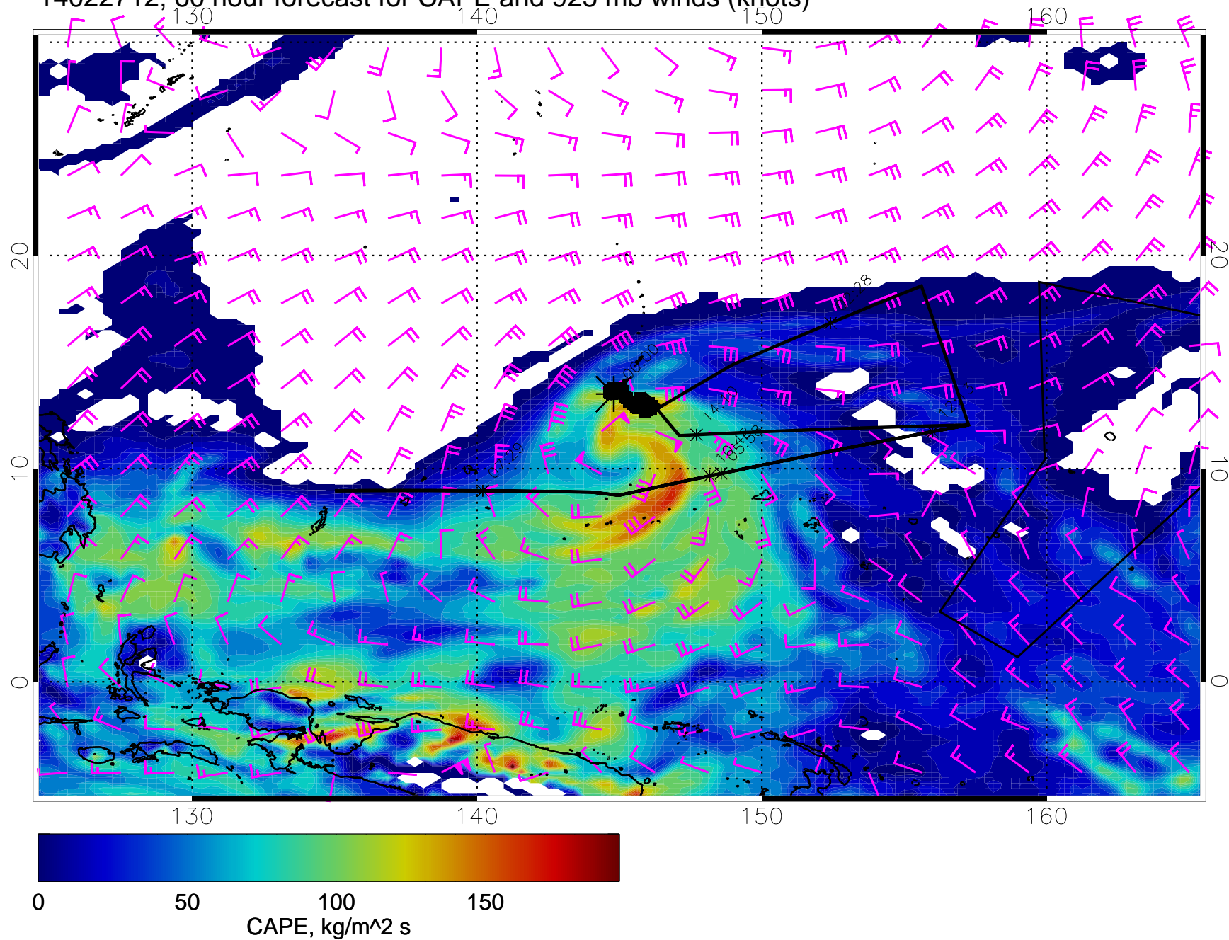
14022712, 60 hour forecast for CAPE and 925 mb winds (knots)
