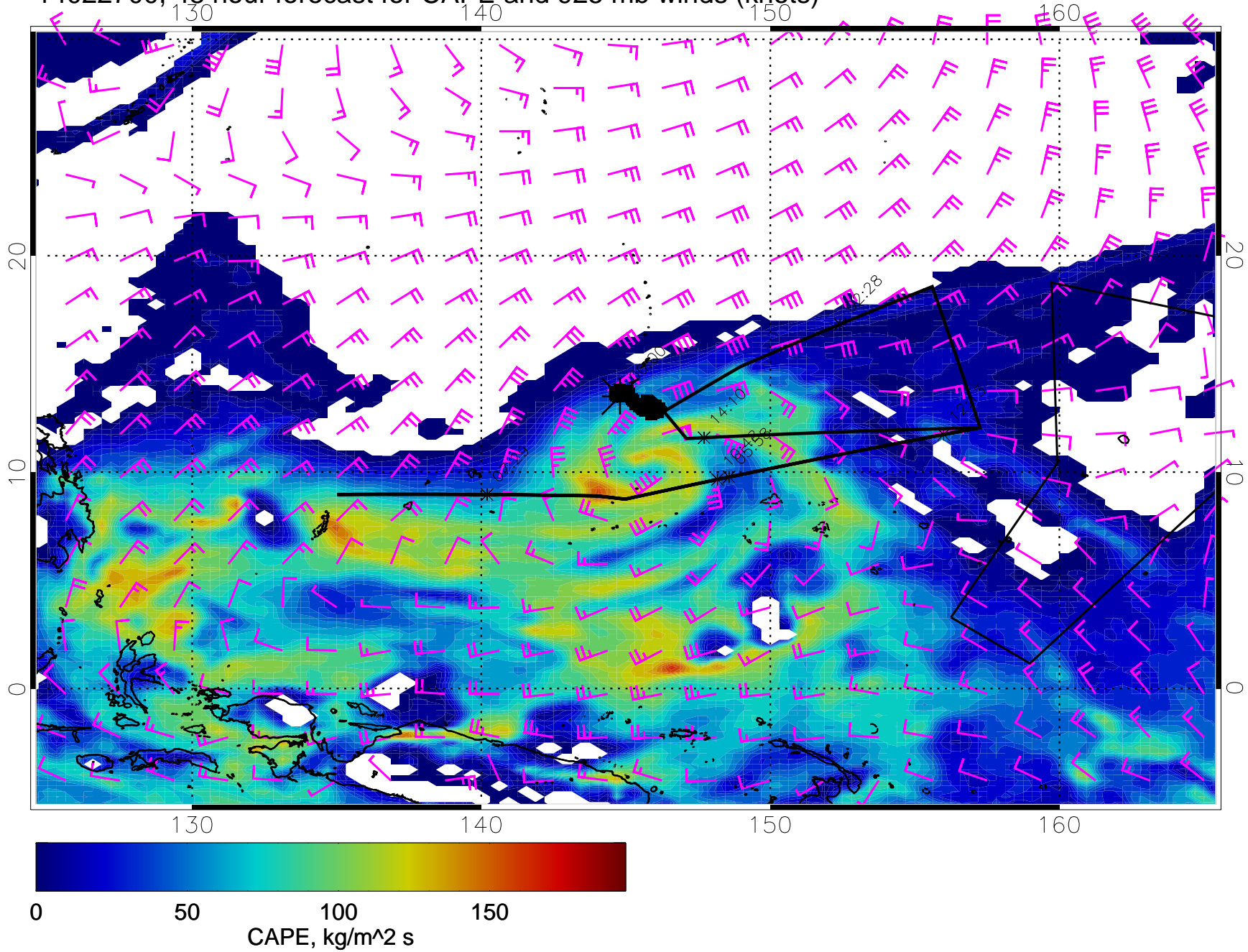
14022700, 48 hour forecast for CAPE and 925 mb winds (knots)
