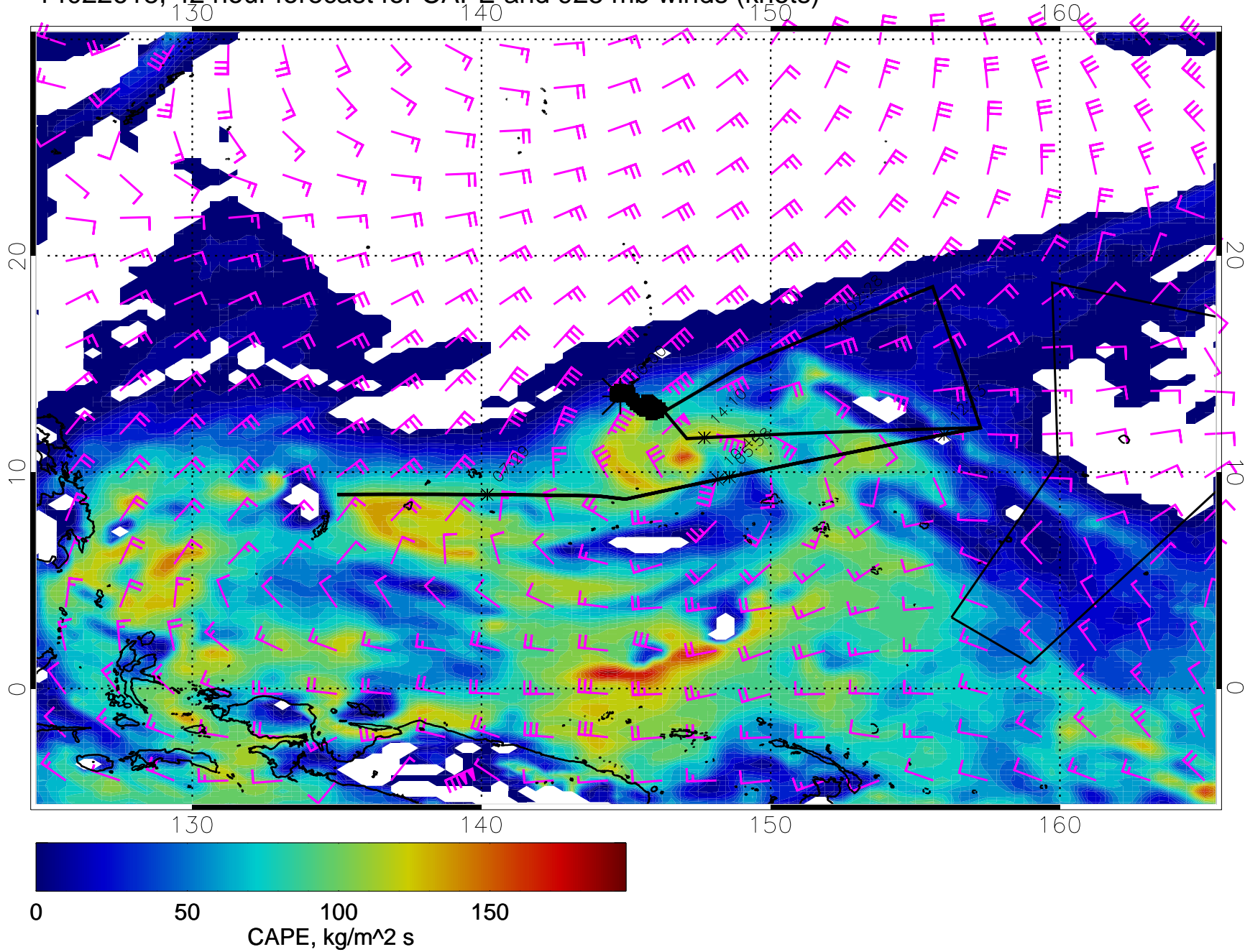
14022618, 42 hour forecast for CAPE and 925 mb winds (knots)
