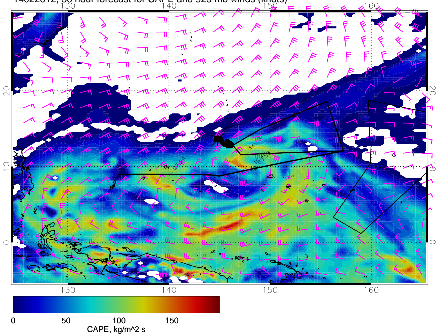
14022612, 36 hour forecast for CAPE and 925 mb winds (knots)
