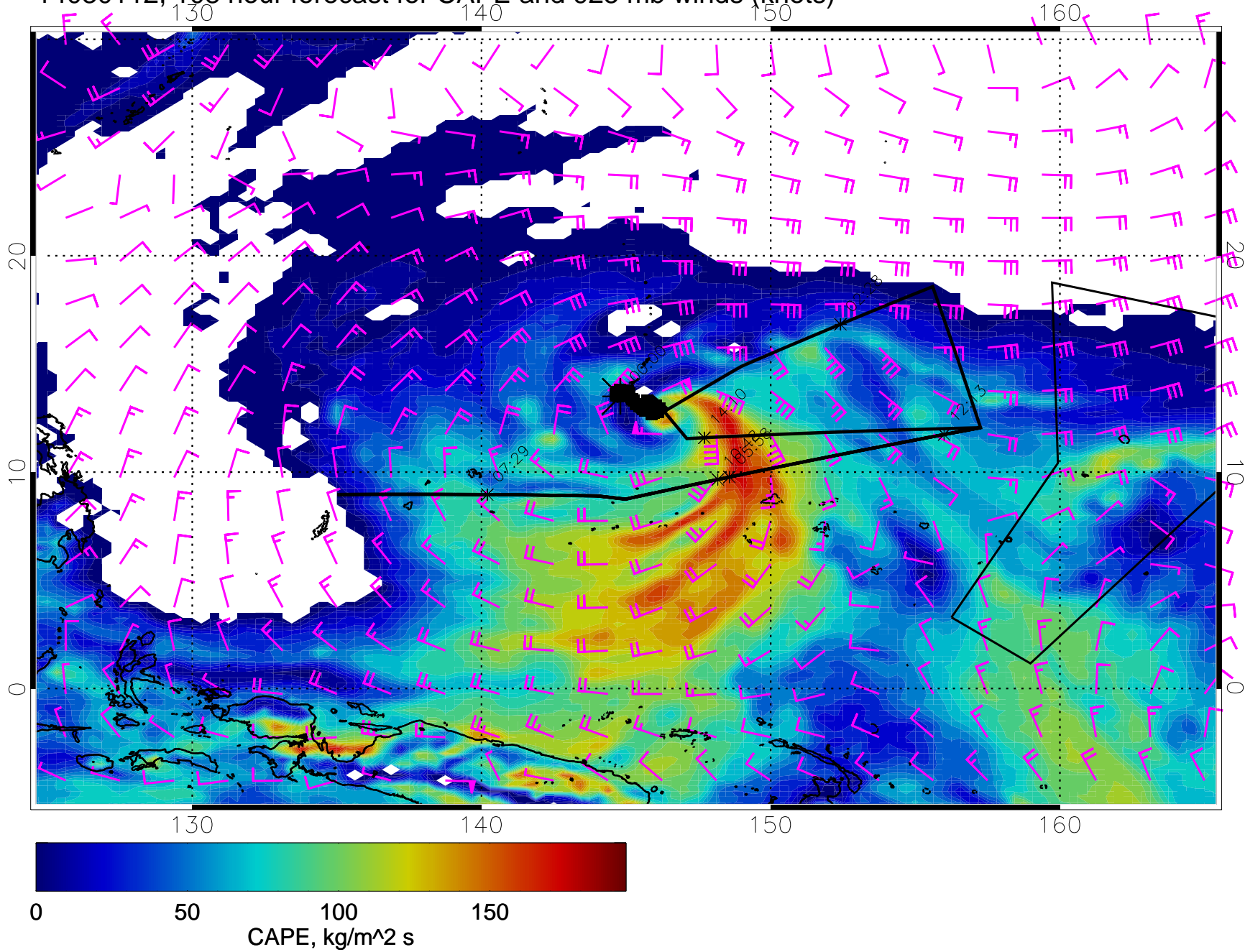
14030112, 108 hour forecast for CAPE and 925 mb winds (knots)
