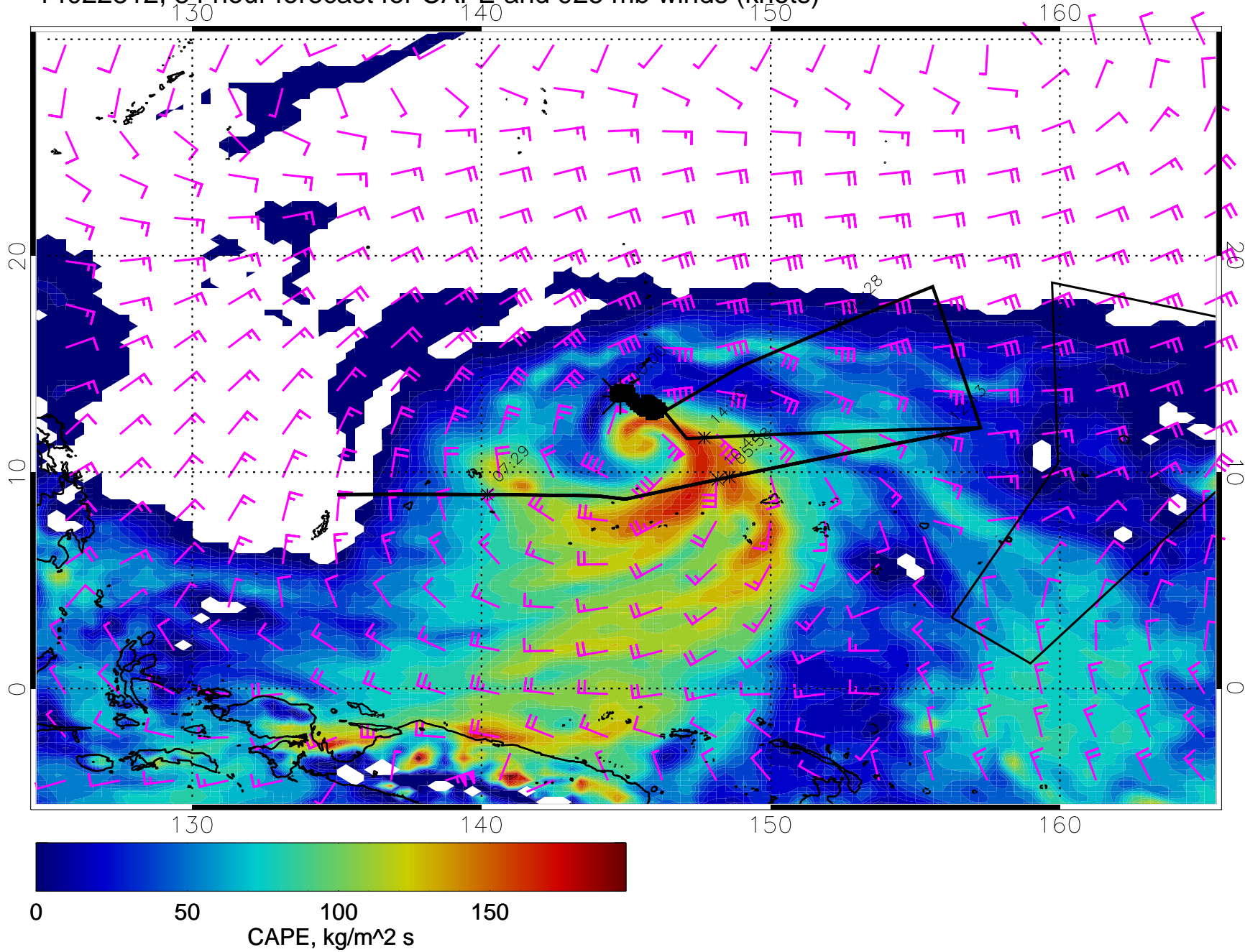
14022812, 84 hour forecast for CAPE and 925 mb winds (knots)
