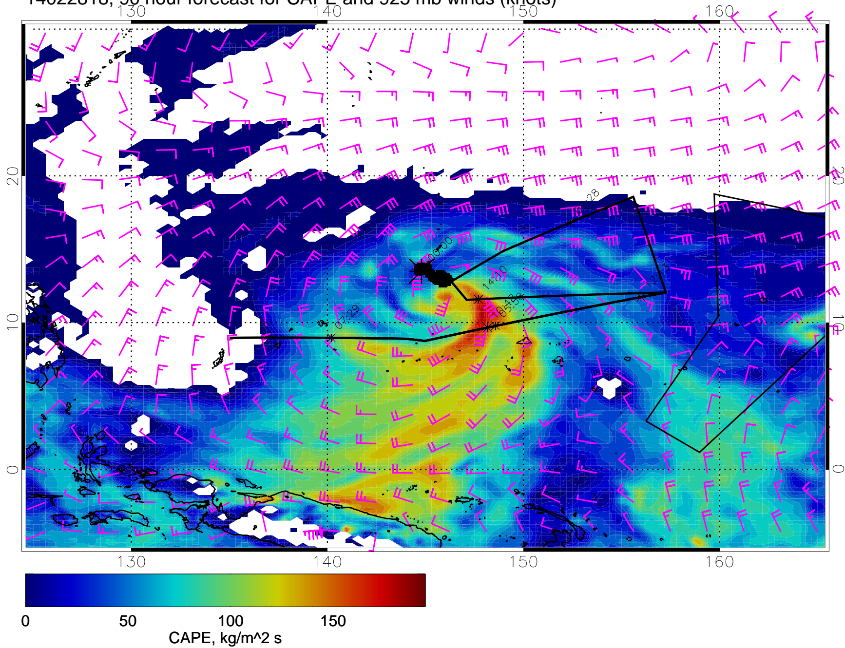
14022818, 90 hour forecast for CAPE and 925 mb winds (knots)
