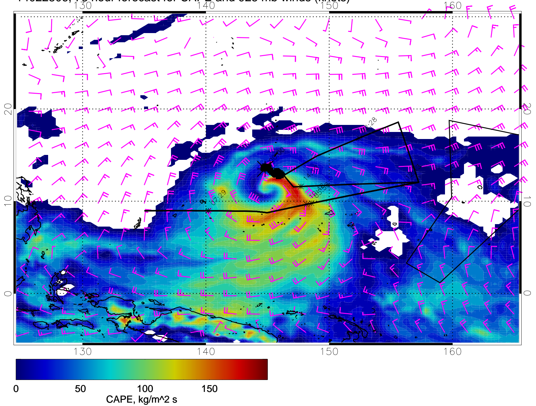
14022806, 78 hour forecast for CAPE and 925 mb winds (knots)
