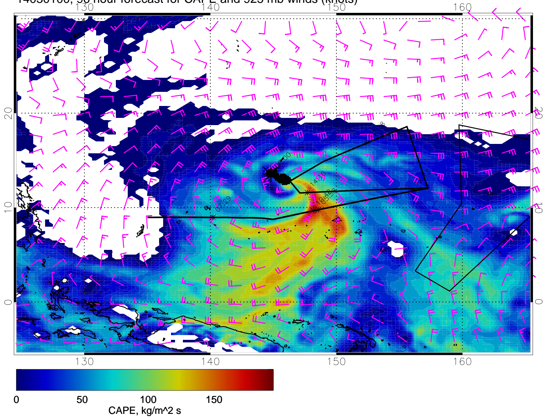
14030100, 96 hour forecast for CAPE and 925 mb winds (knots)
