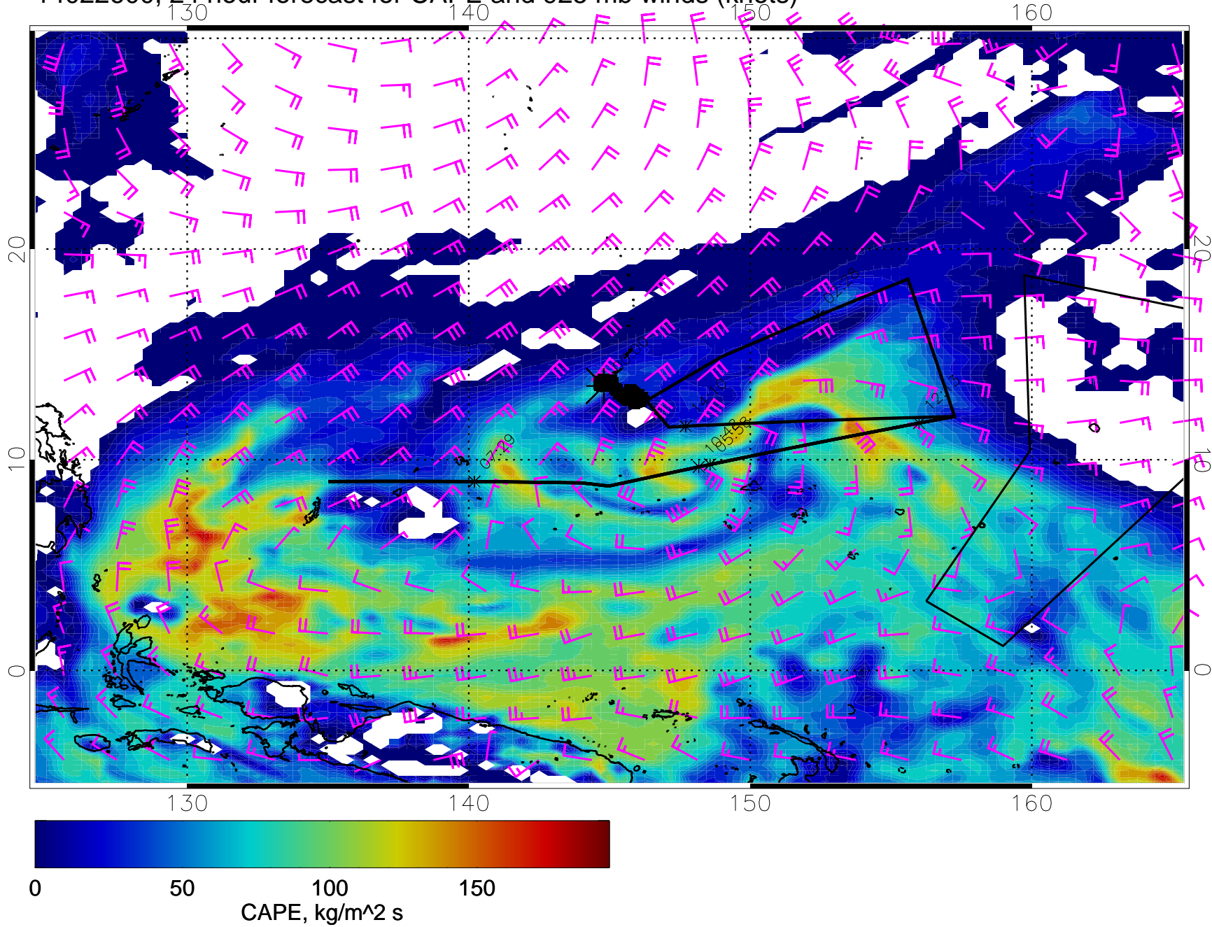
14022600, 24 hour forecast for CAPE and 925 mb winds (knots)
