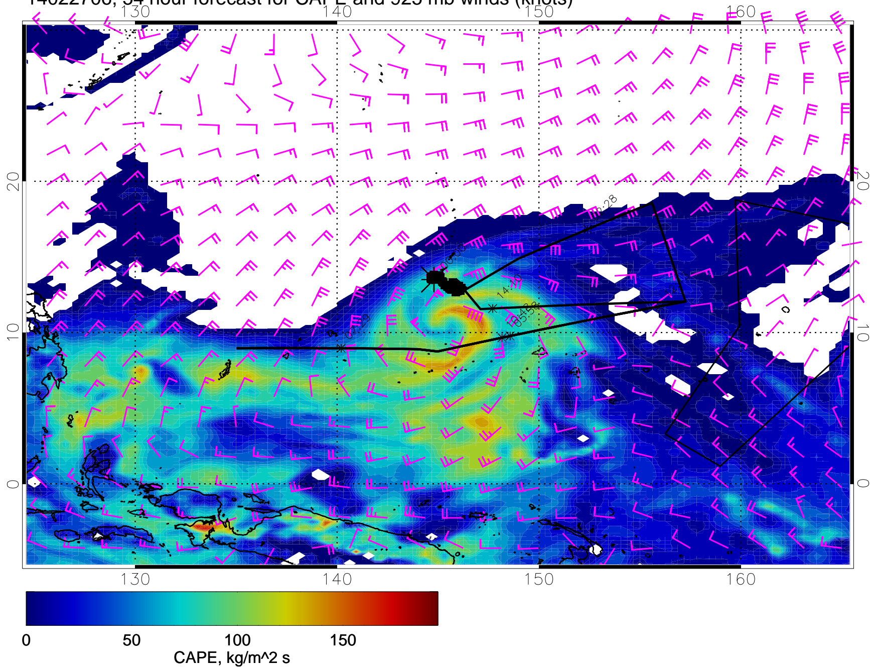
14022706, 54 hour forecast for CAPE and 925 mb winds (knots)
