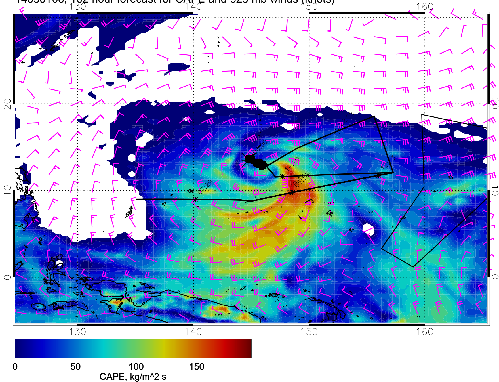
14030106, 102 hour forecast for CAPE and 925 mb winds (knots)
