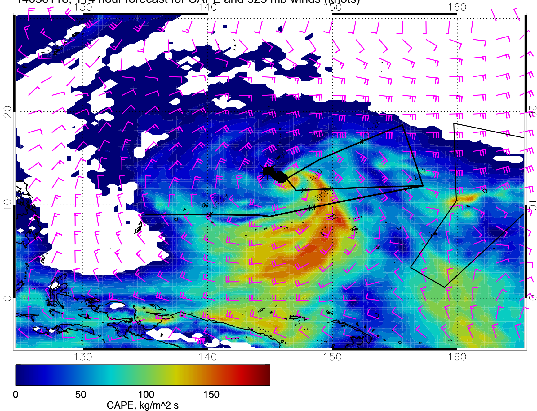
14030118, 114 hour forecast for CAPE and 925 mb winds (knots)
