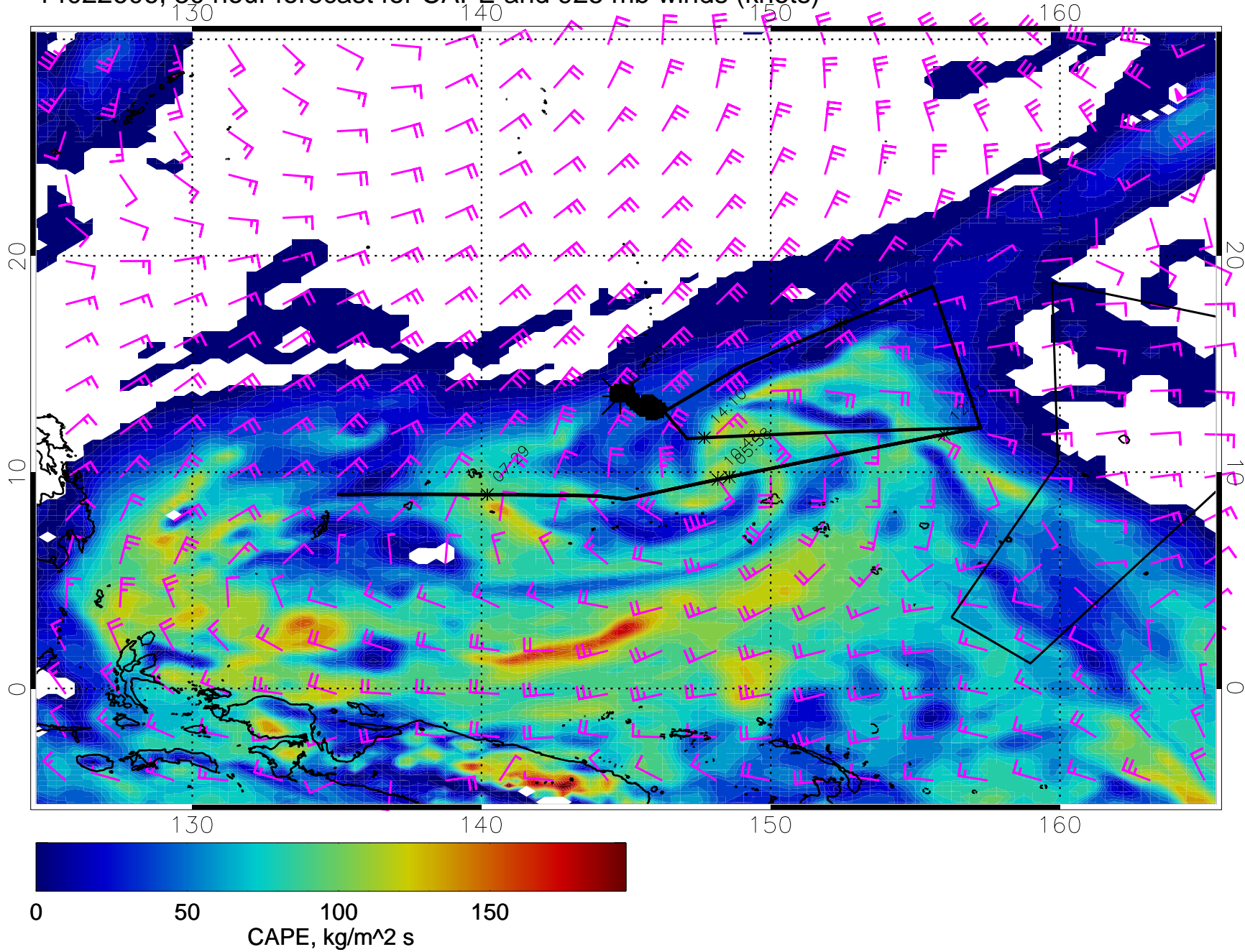
14022606, 30 hour forecast for CAPE and 925 mb winds (knots)
