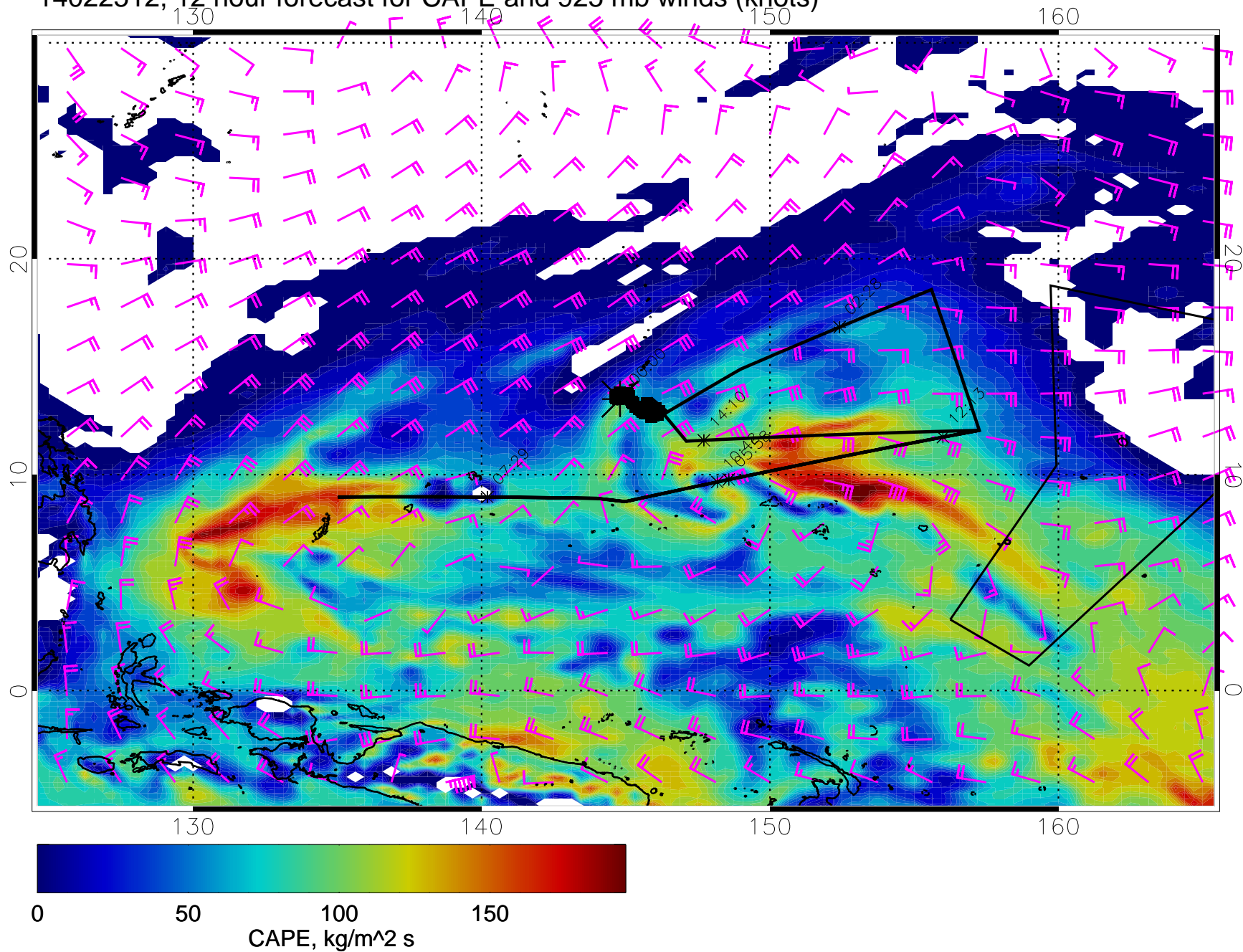
14022512, 12 hour forecast for CAPE and 925 mb winds (knots)
