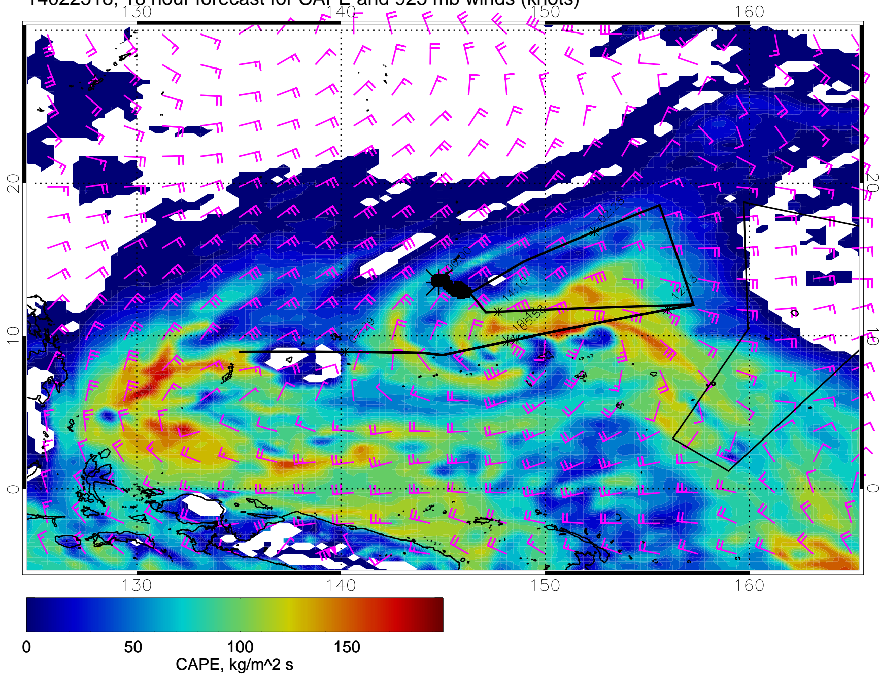
14022518, 18 hour forecast for CAPE and 925 mb winds (knots)
