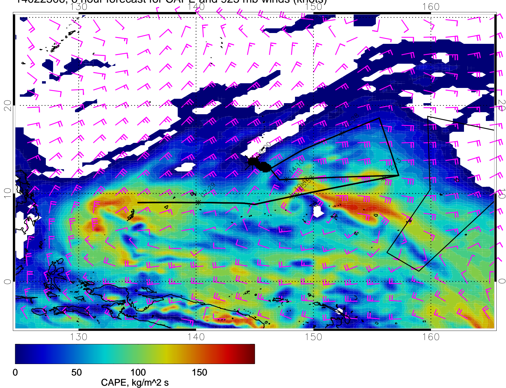
14022506, 6 hour forecast for CAPE and 925 mb winds (knots)
