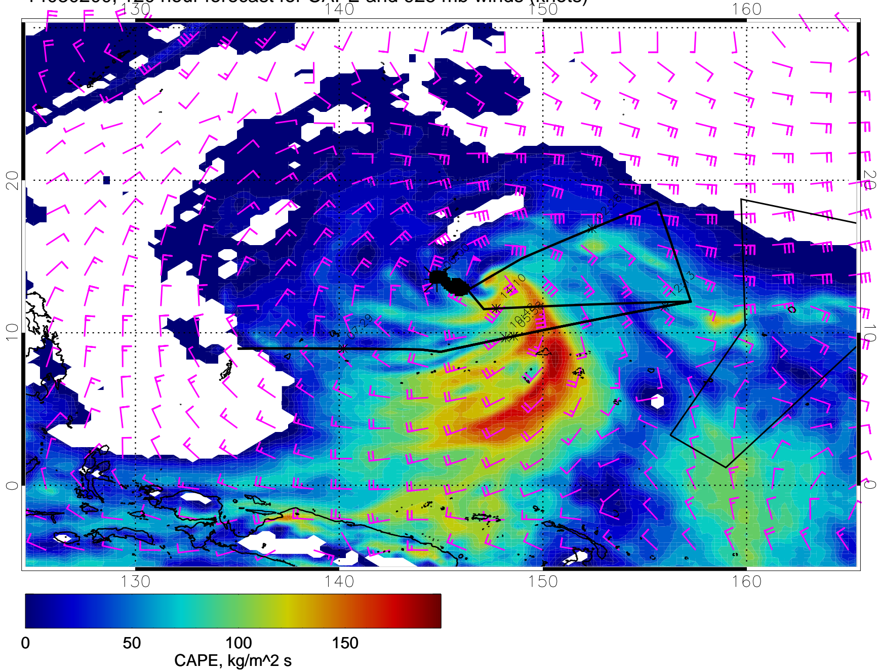
14030200, 120 hour forecast for CAPE and 925 mb winds (knots)
