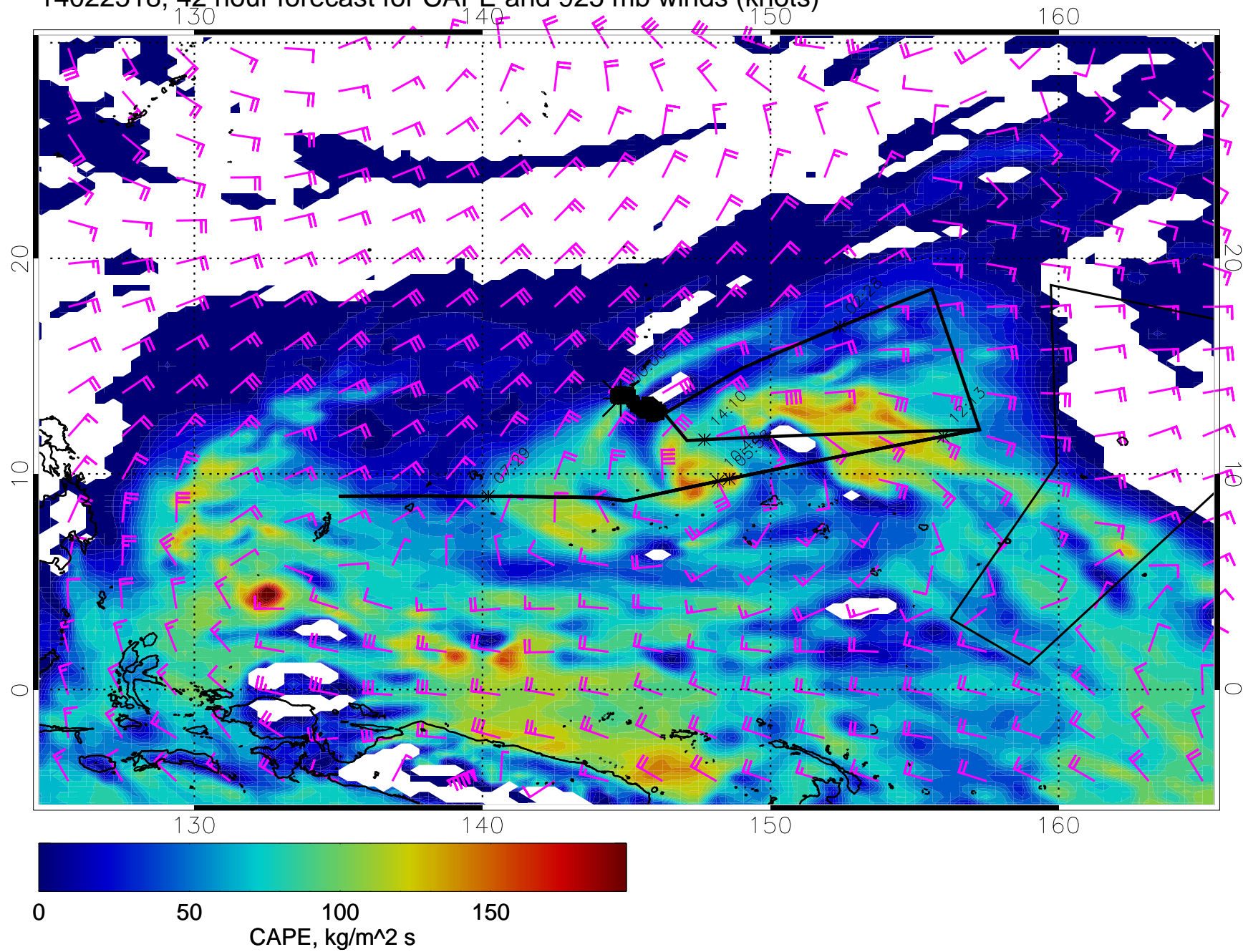
14022518, 42 hour forecast for CAPE and 925 mb winds (knots)
