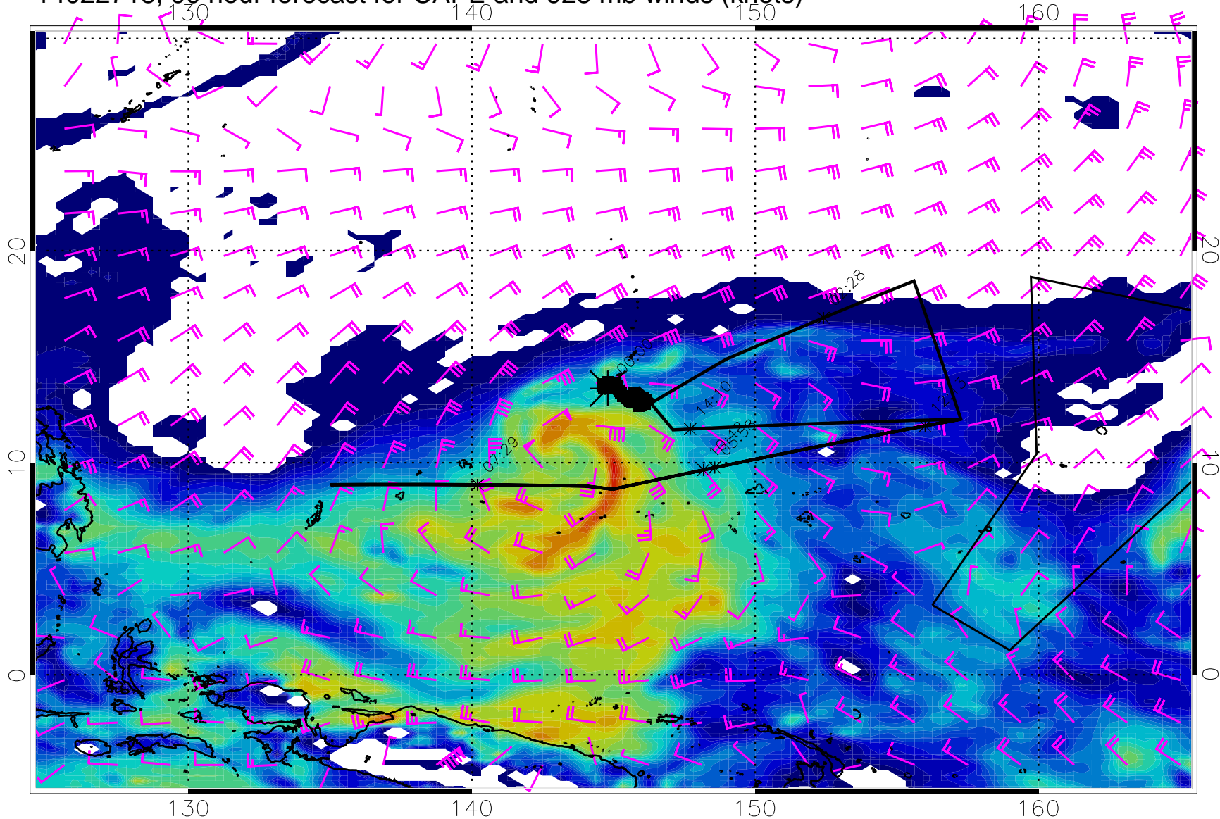
14022718, 90 hour forecast for CAPE and 925 mb winds (knots)
