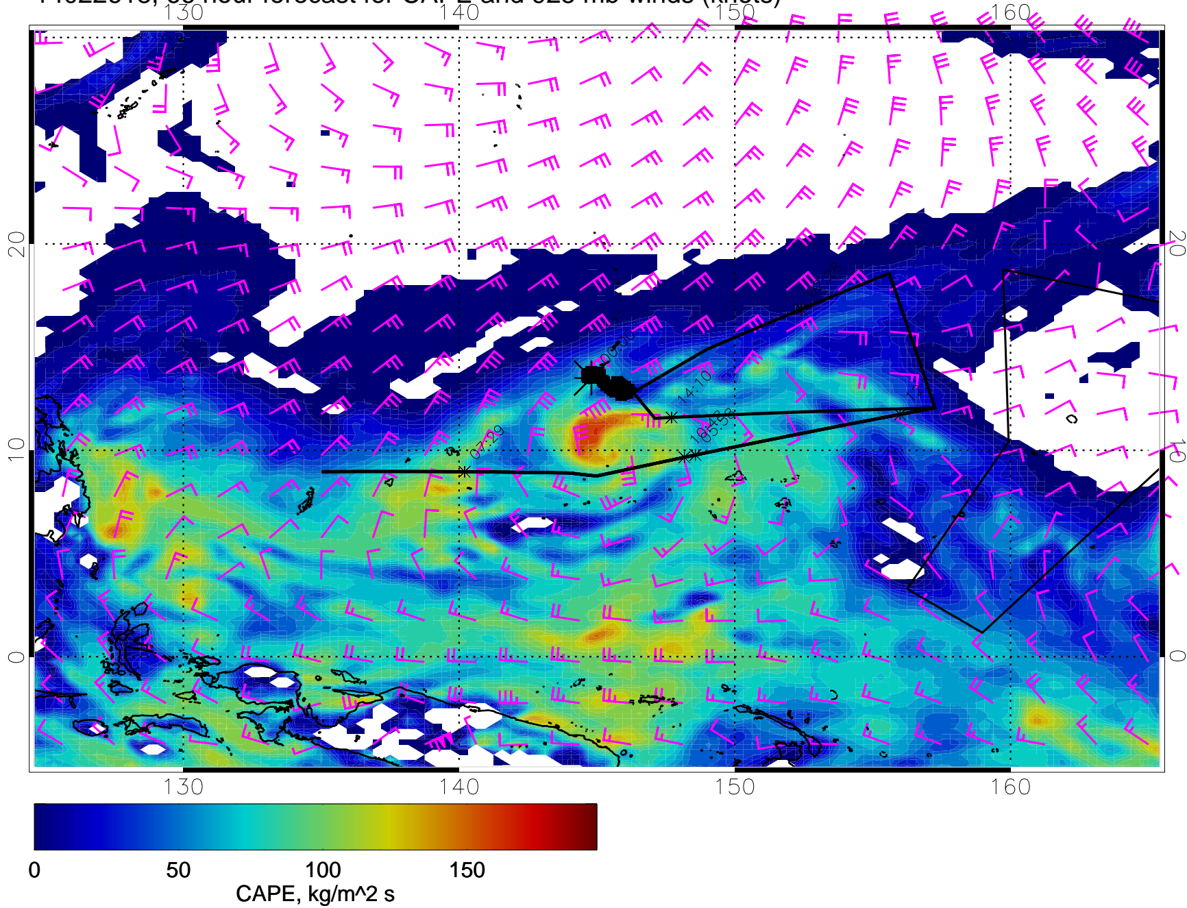
14022618, 66 hour forecast for CAPE and 925 mb winds (knots)
