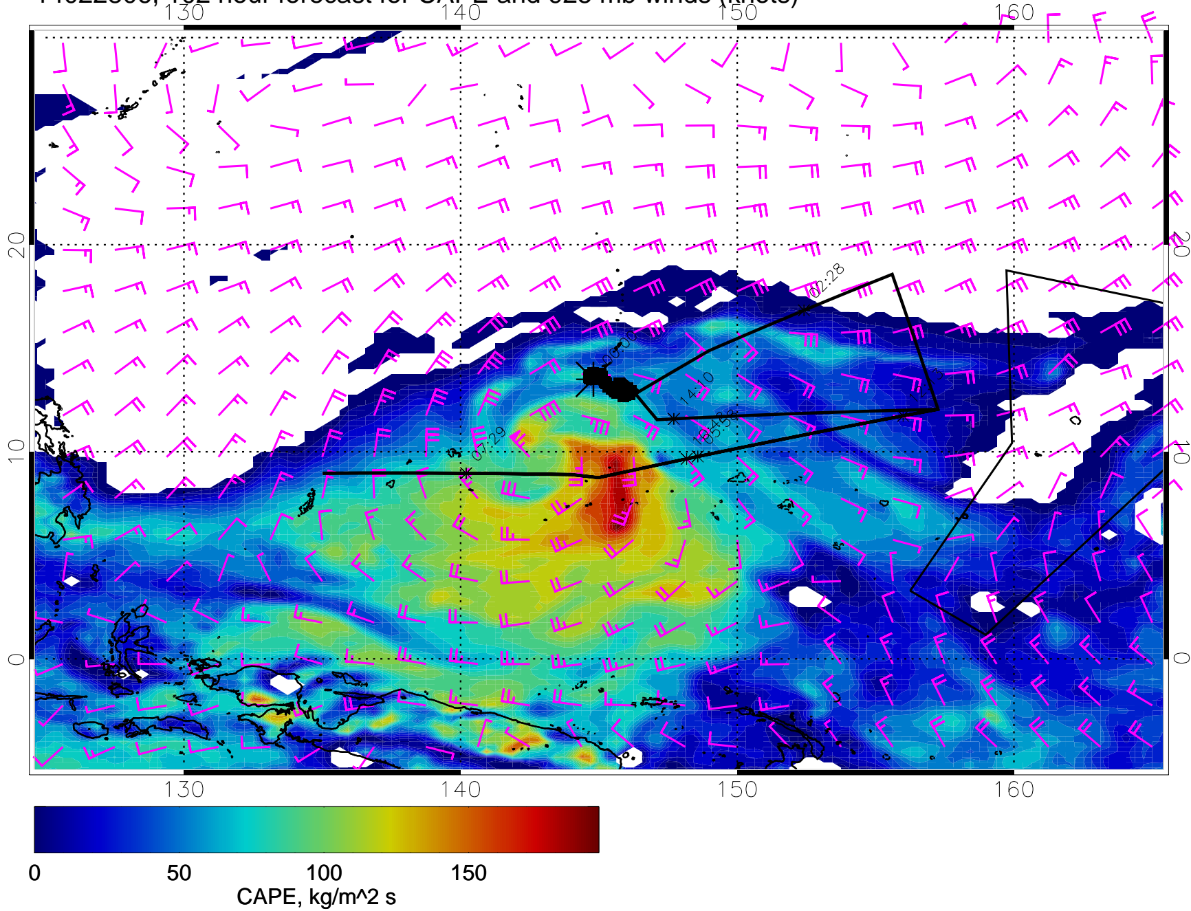
14022806, 102 hour forecast for CAPE and 925 mb winds (knots)
