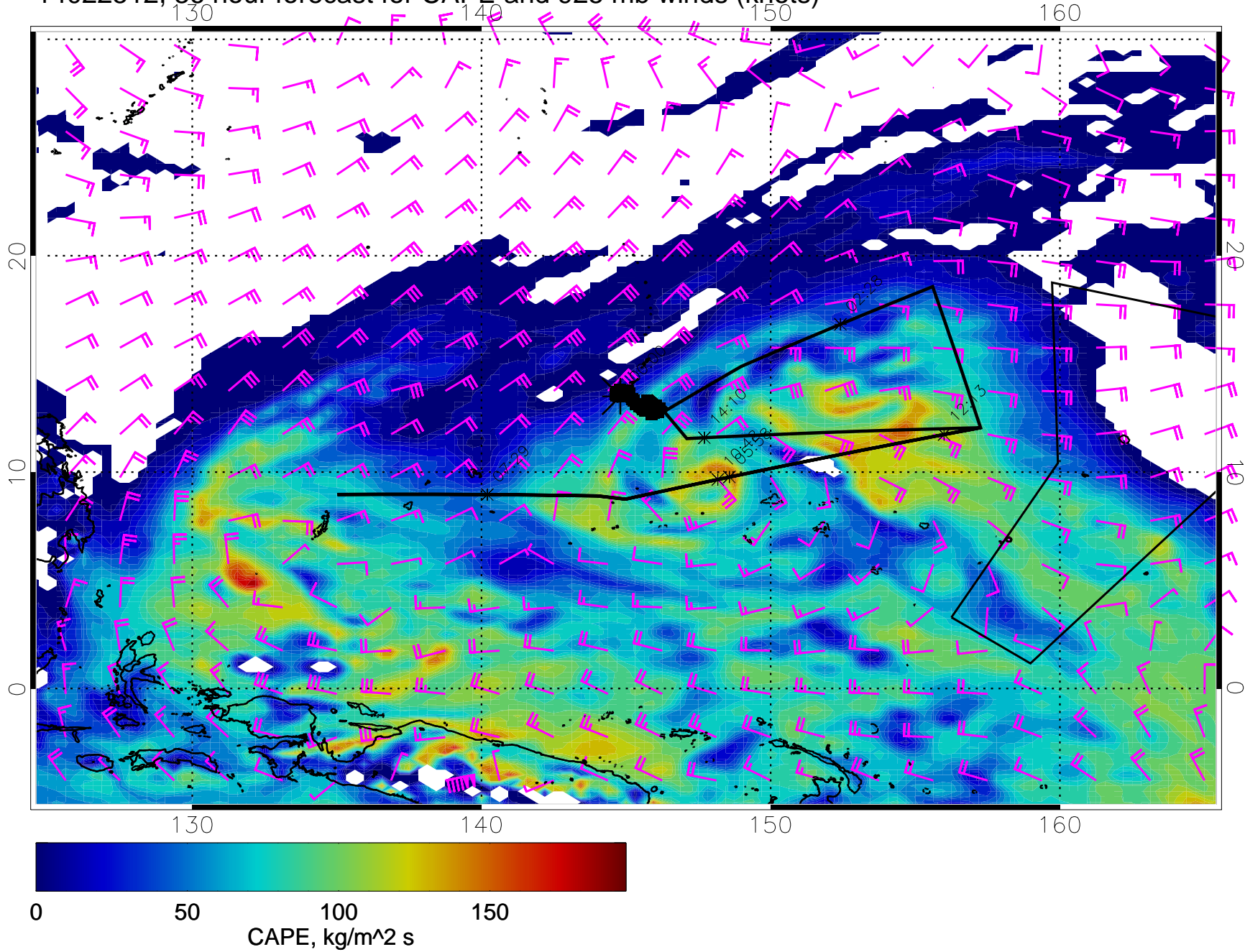
14022512, 36 hour forecast for CAPE and 925 mb winds (knots)
