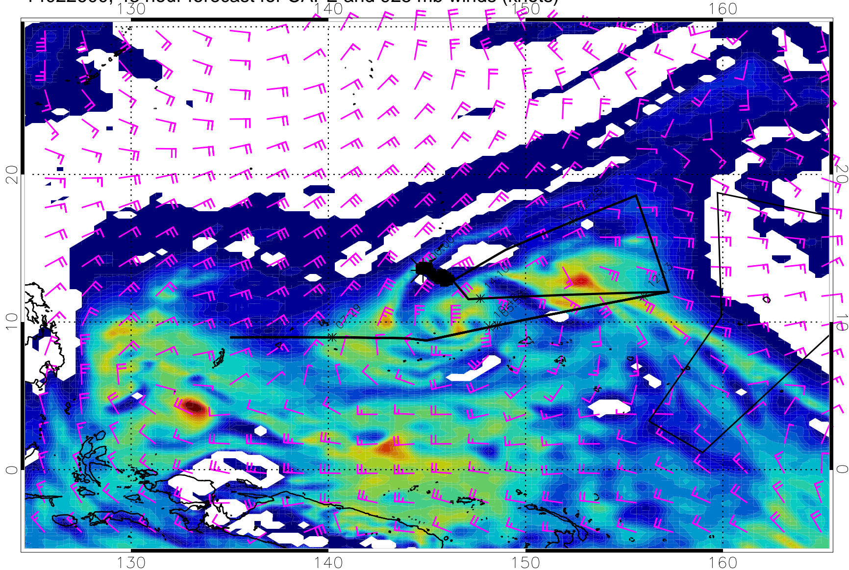
14022600, 48 hour forecast for CAPE and 925 mb winds (knots)
