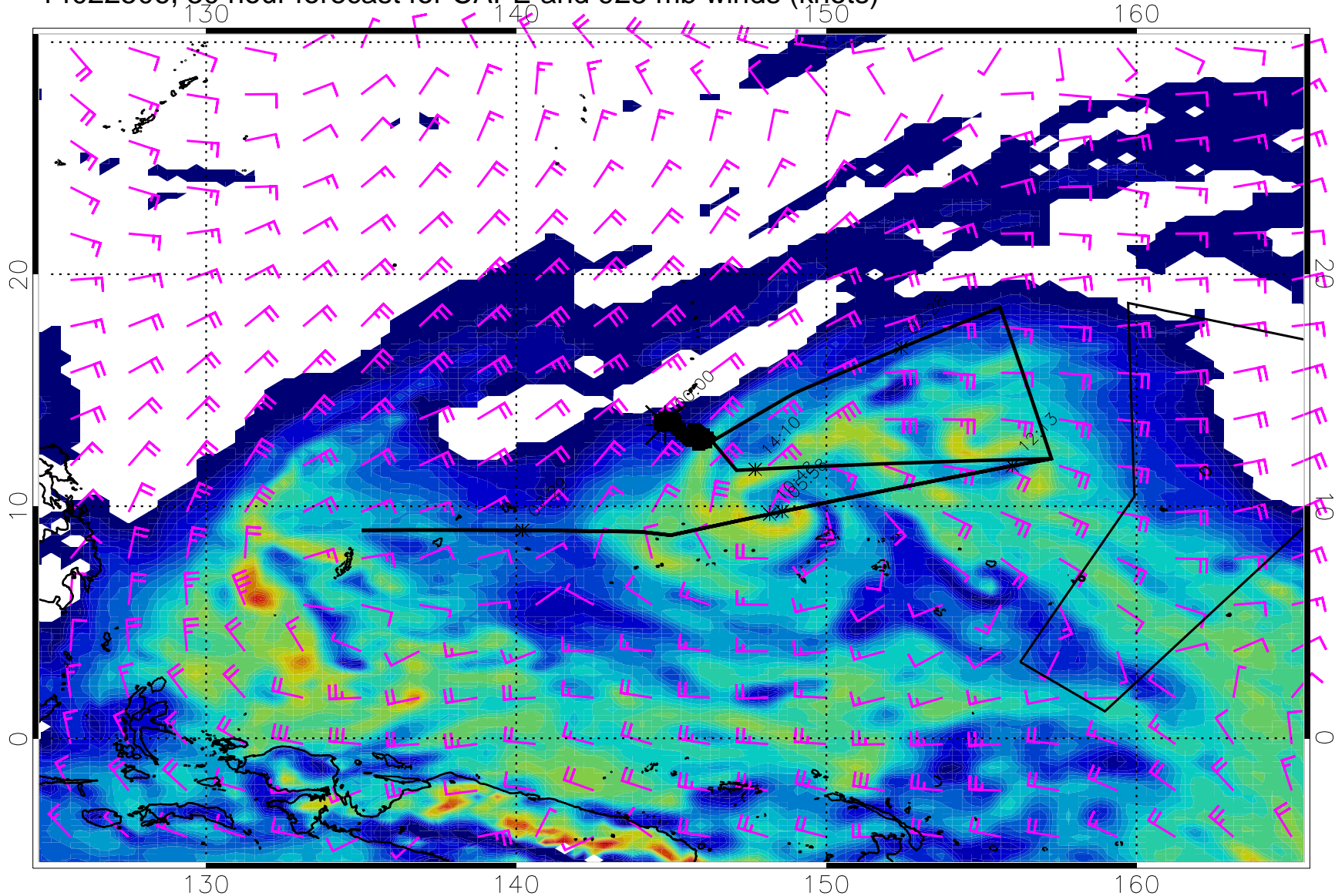
14022506, 30 hour forecast for CAPE and 925 mb winds (knots)
