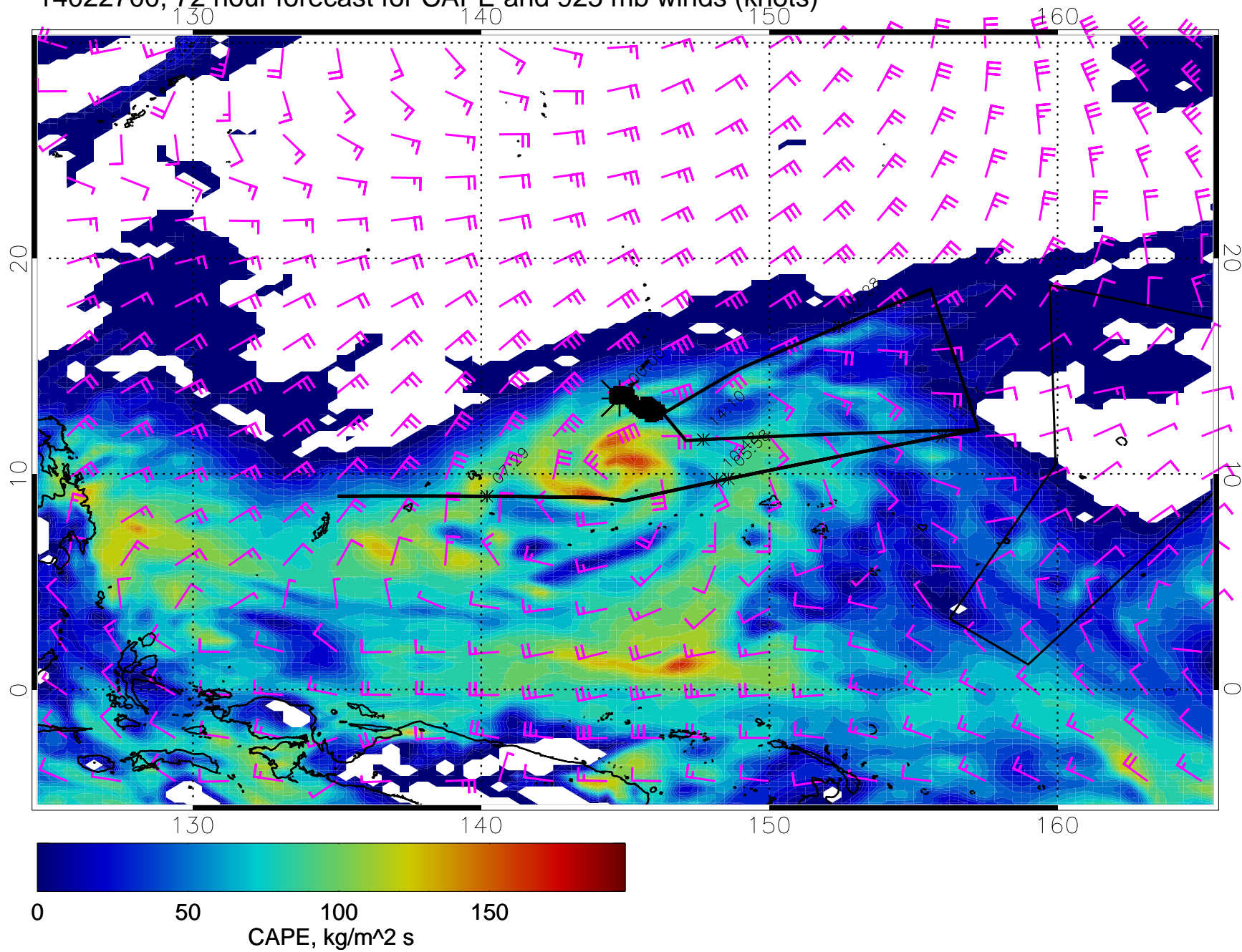
14022700, 72 hour forecast for CAPE and 925 mb winds (knots)
