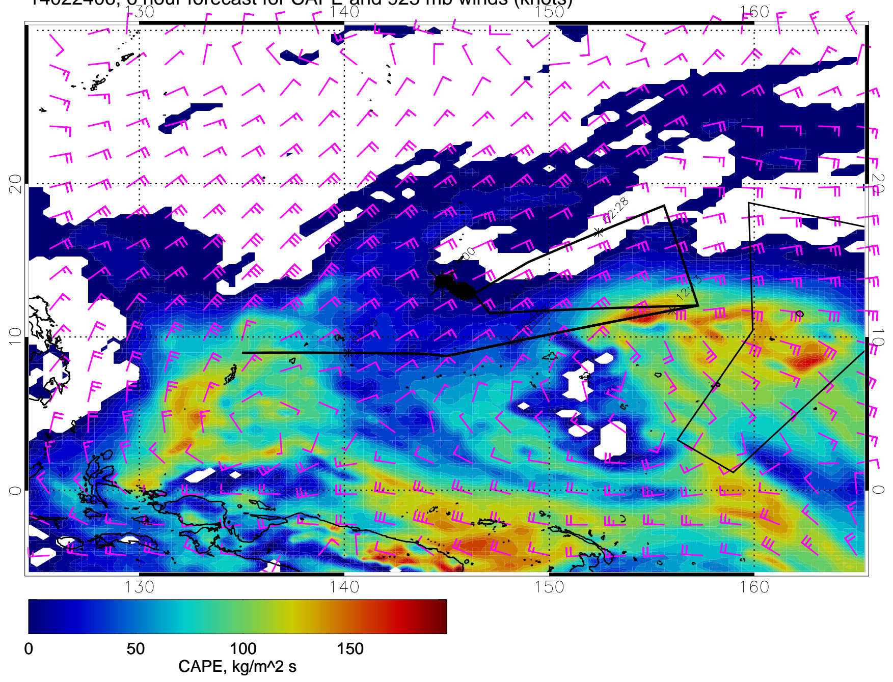
14022406, 6 hour forecast for CAPE and 925 mb winds (knots)
