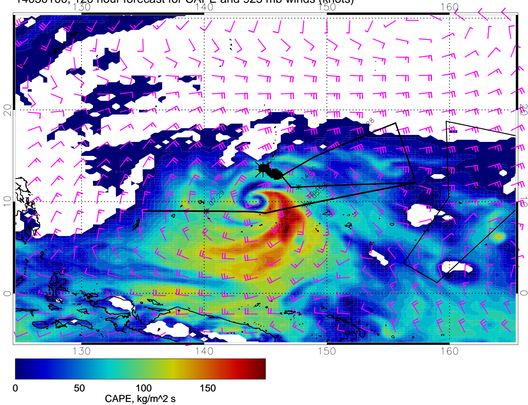
14030100, 120 hour forecast for CAPE and 925 mb winds (knots)
