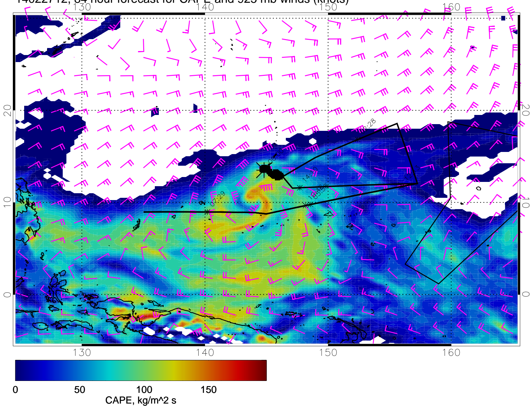
14022712, 84 hour forecast for CAPE and 925 mb winds (knots)
