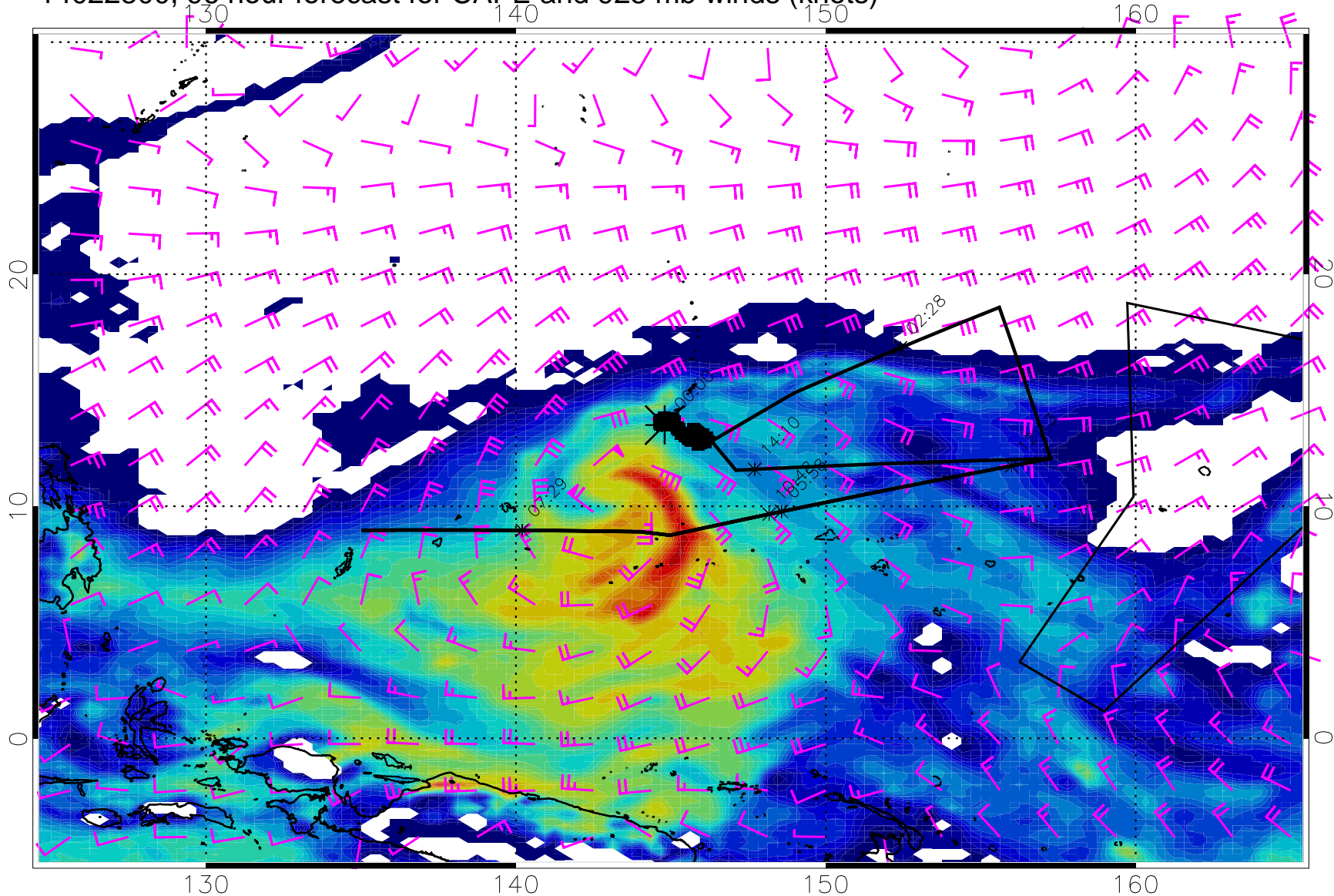
14022800, 96 hour forecast for CAPE and 925 mb winds (knots)
