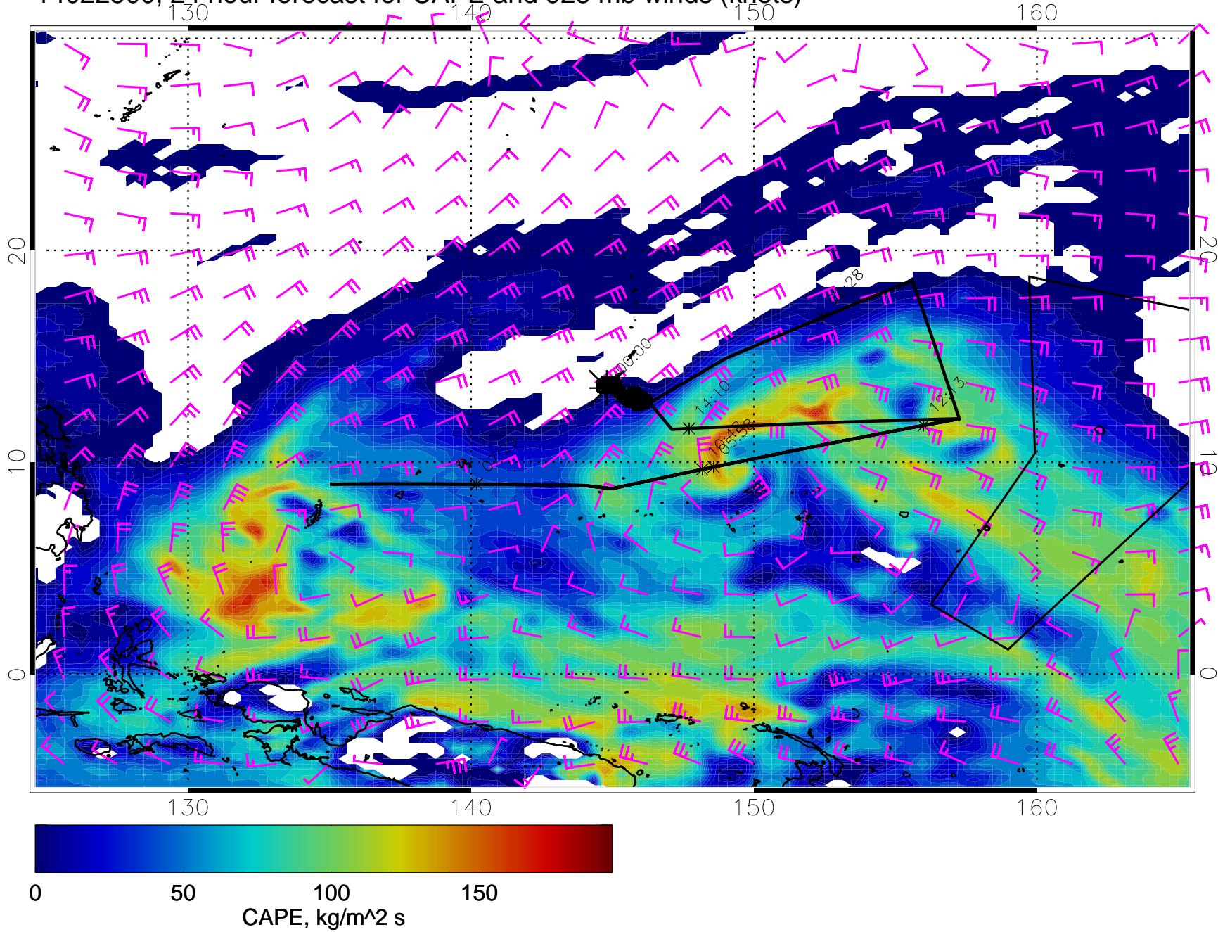
14022500, 24 hour forecast for CAPE and 925 mb winds (knots)
