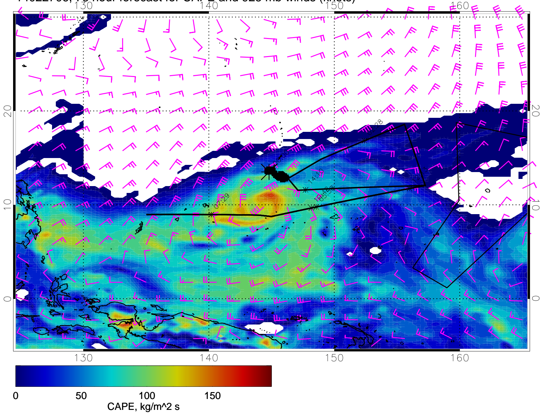
14022706, 78 hour forecast for CAPE and 925 mb winds (knots)
