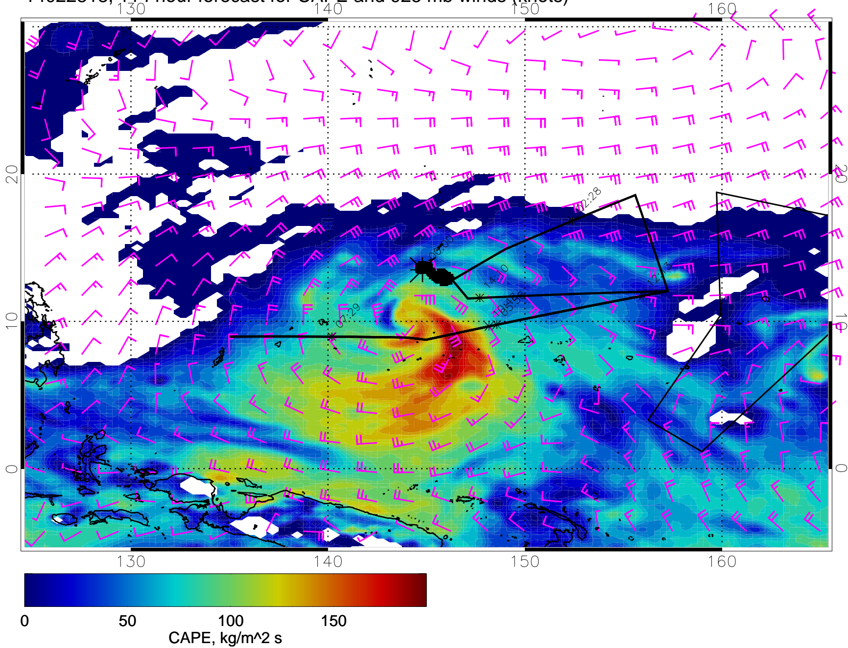
14022818, 114 hour forecast for CAPE and 925 mb winds (knots)
