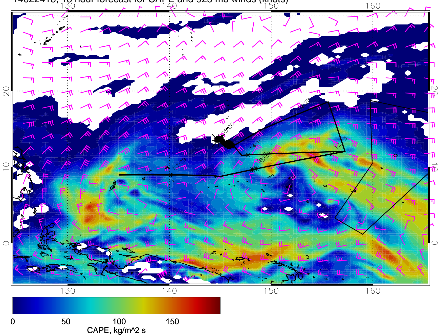
14022418, 18 hour forecast for CAPE and 925 mb winds (knots)
