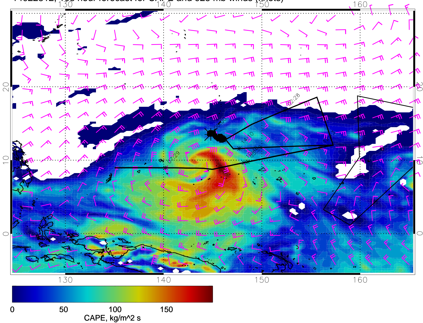
14022812, 108 hour forecast for CAPE and 925 mb winds (knots)
