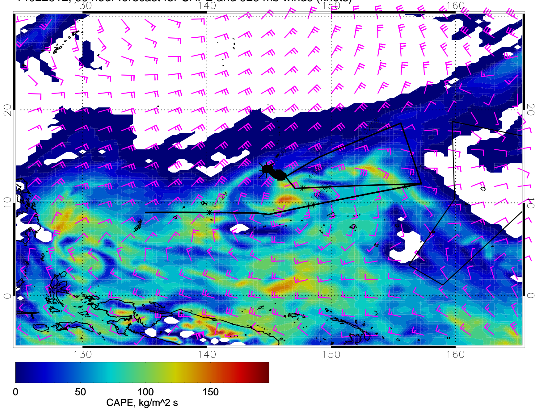
14022612, 60 hour forecast for CAPE and 925 mb winds (knots)
