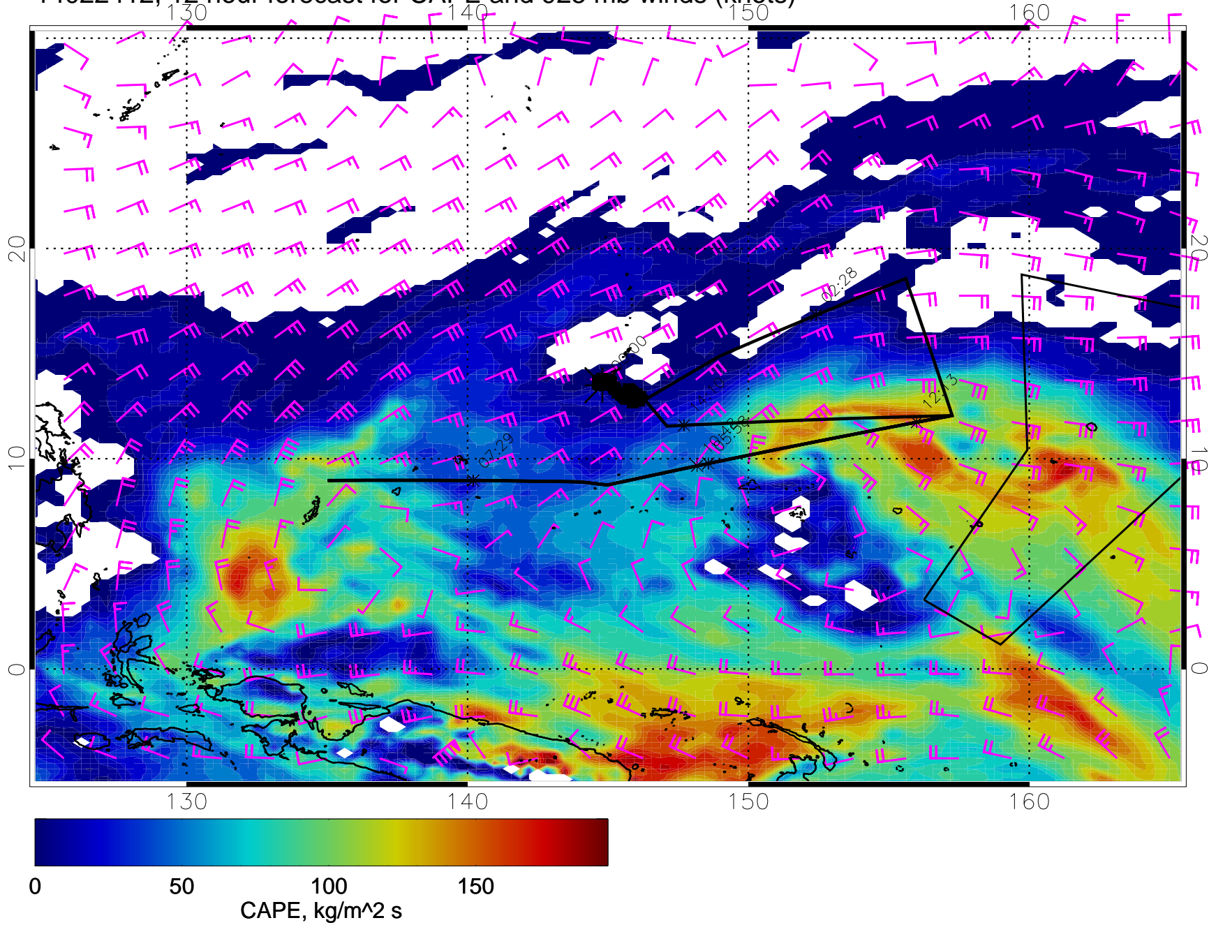
14022412, 12 hour forecast for CAPE and 925 mb winds (knots)
