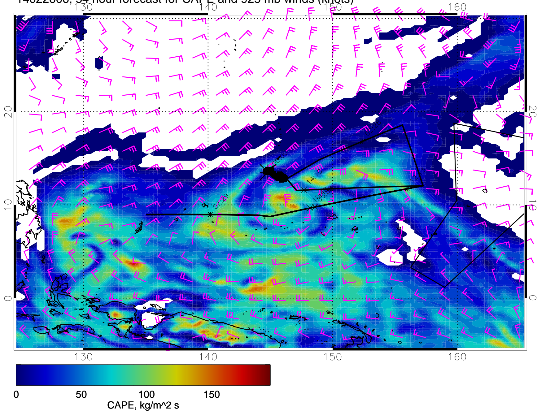
14022606, 54 hour forecast for CAPE and 925 mb winds (knots)
