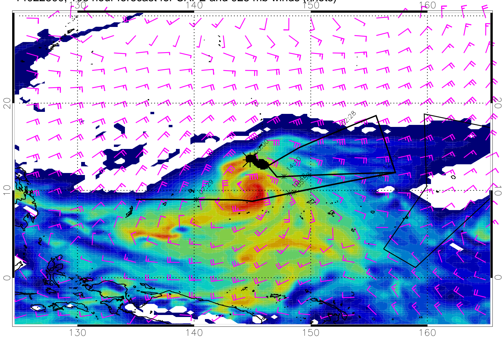
14022800, 108 hour forecast for CAPE and 925 mb winds (knots)
