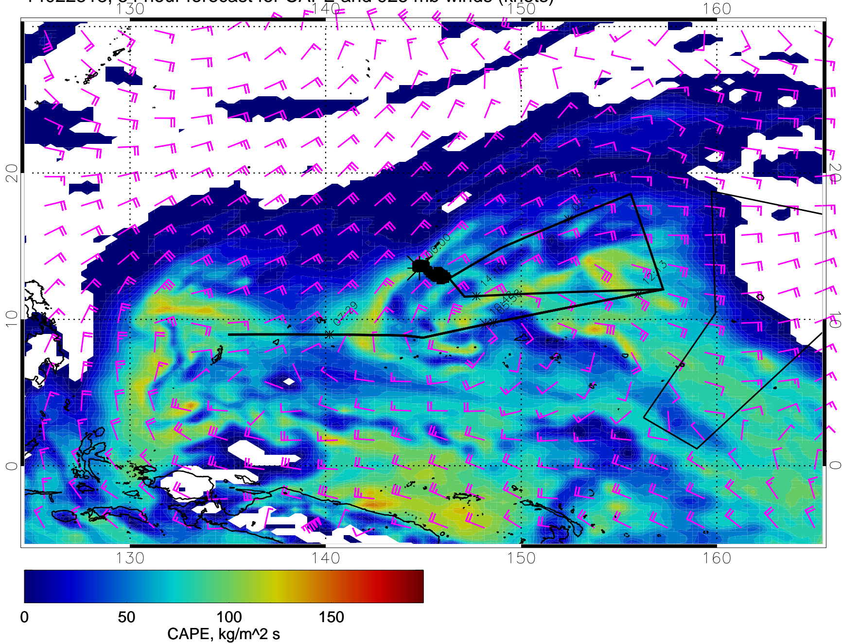
14022518, 54 hour forecast for CAPE and 925 mb winds (knots)
