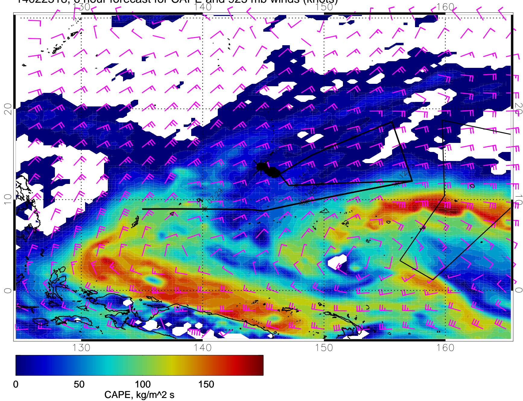
14022318, 6 hour forecast for CAPE and 925 mb winds (knots)
