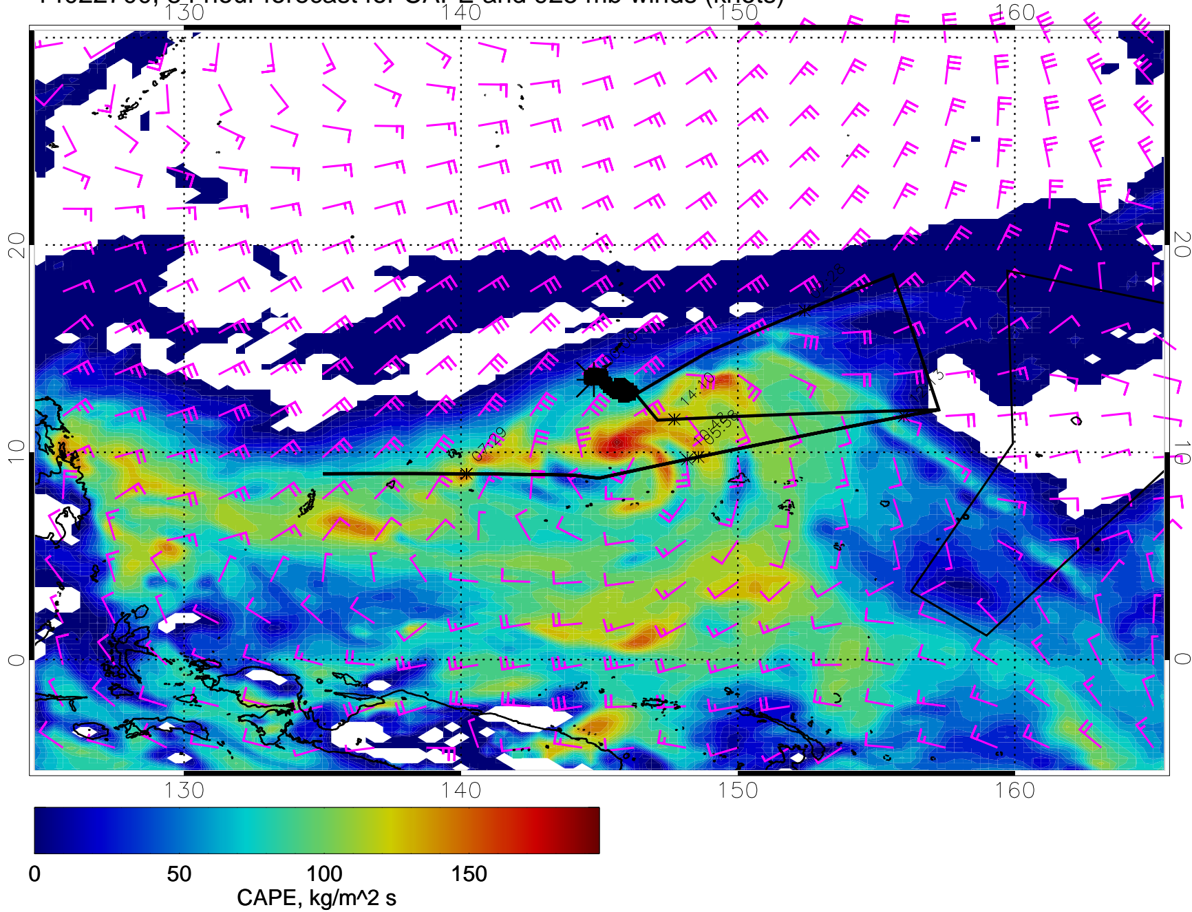
14022700, 84 hour forecast for CAPE and 925 mb winds (knots)
