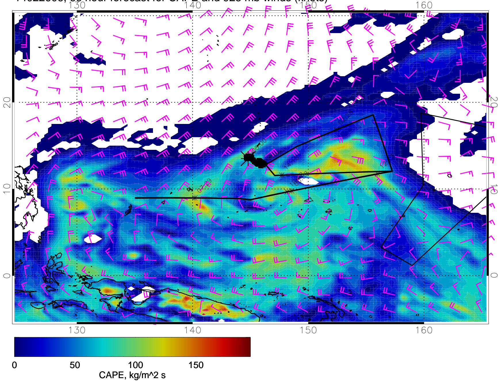
14022606, 66 hour forecast for CAPE and 925 mb winds (knots)
