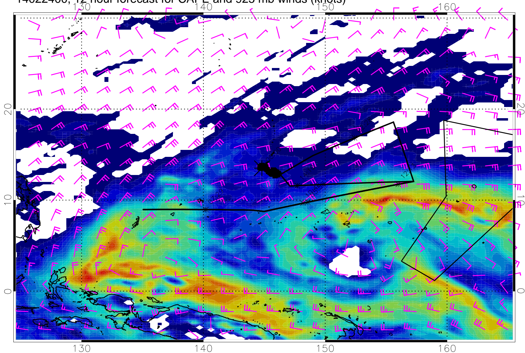
14022400, 12 hour forecast for CAPE and 925 mb winds (knots)
