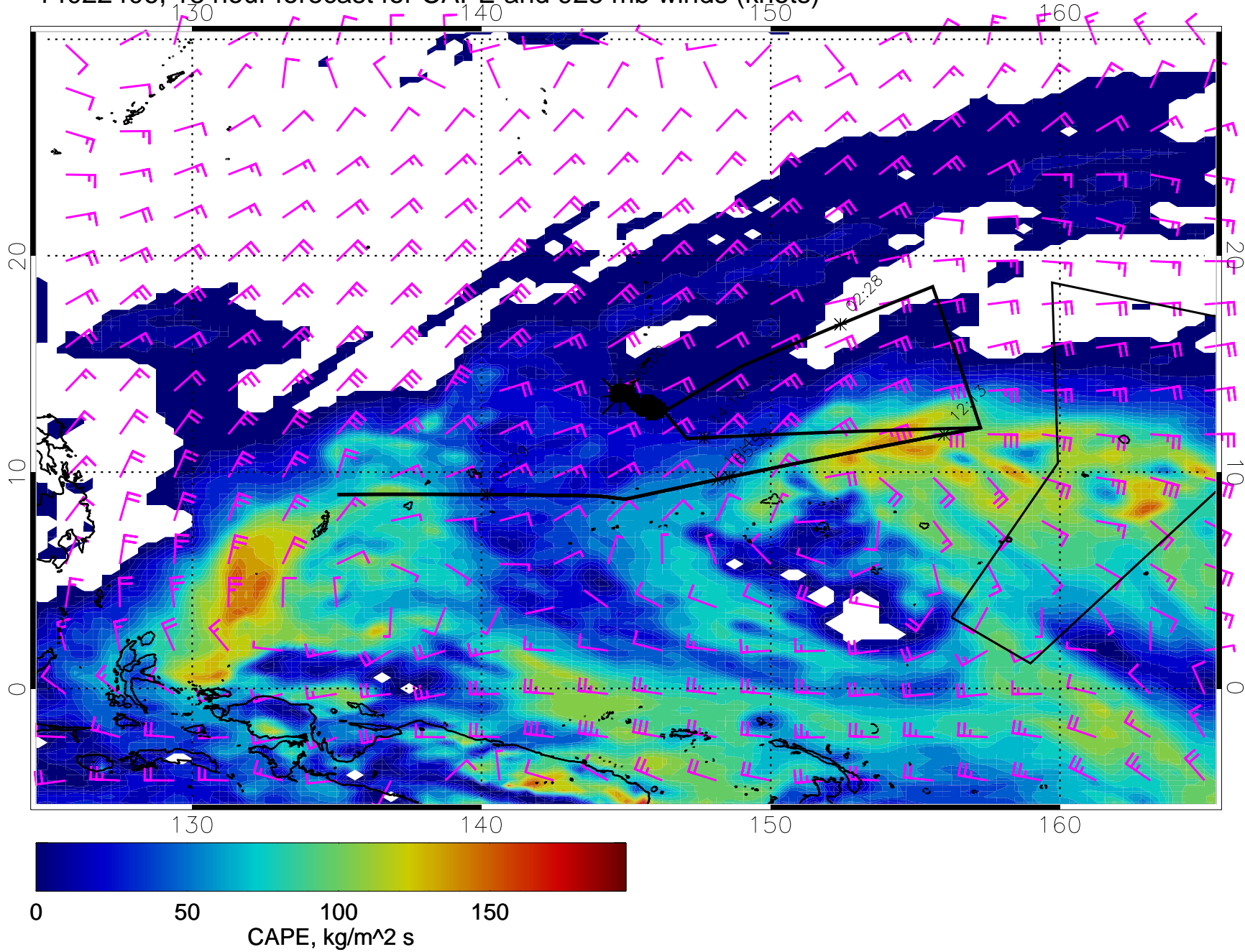
14022406, 18 hour forecast for CAPE and 925 mb winds (knots)
