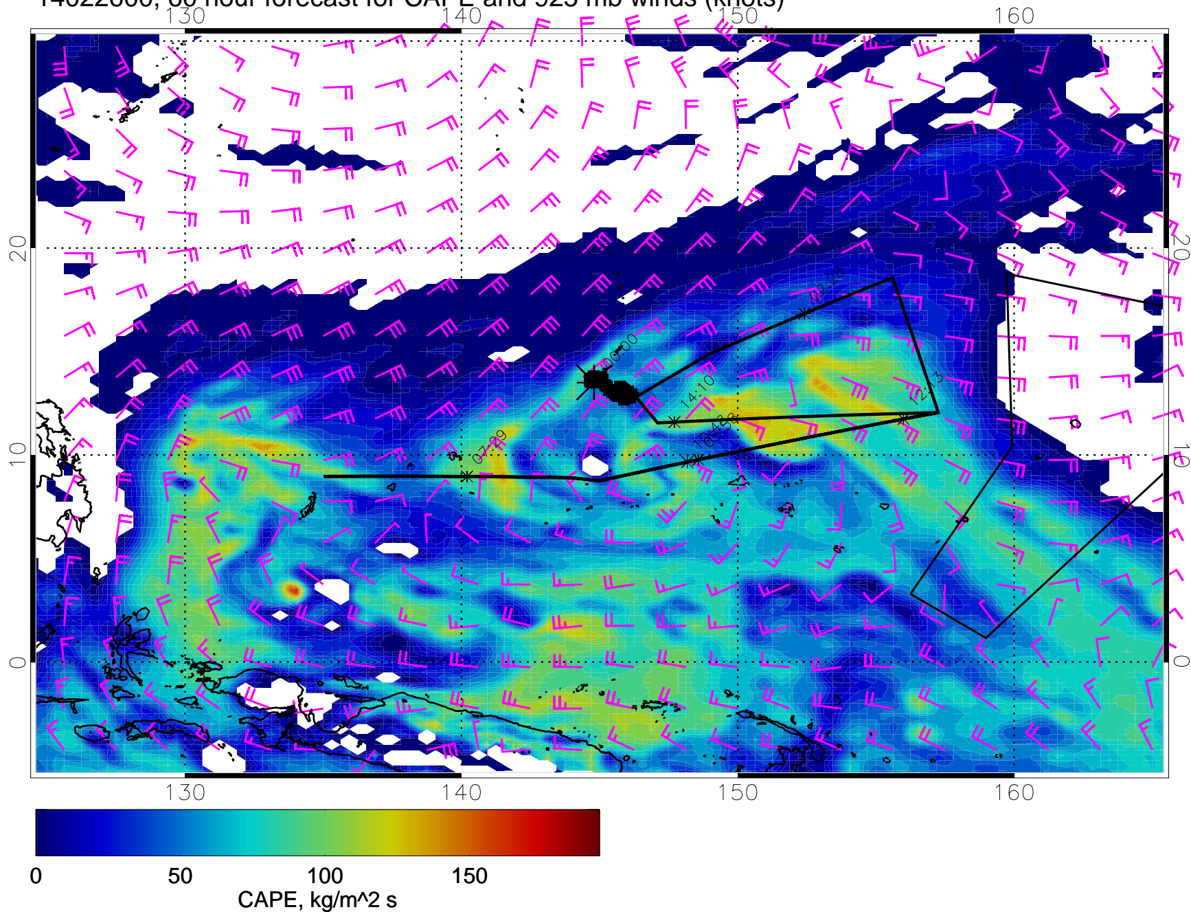
14022600, 60 hour forecast for CAPE and 925 mb winds (knots)
