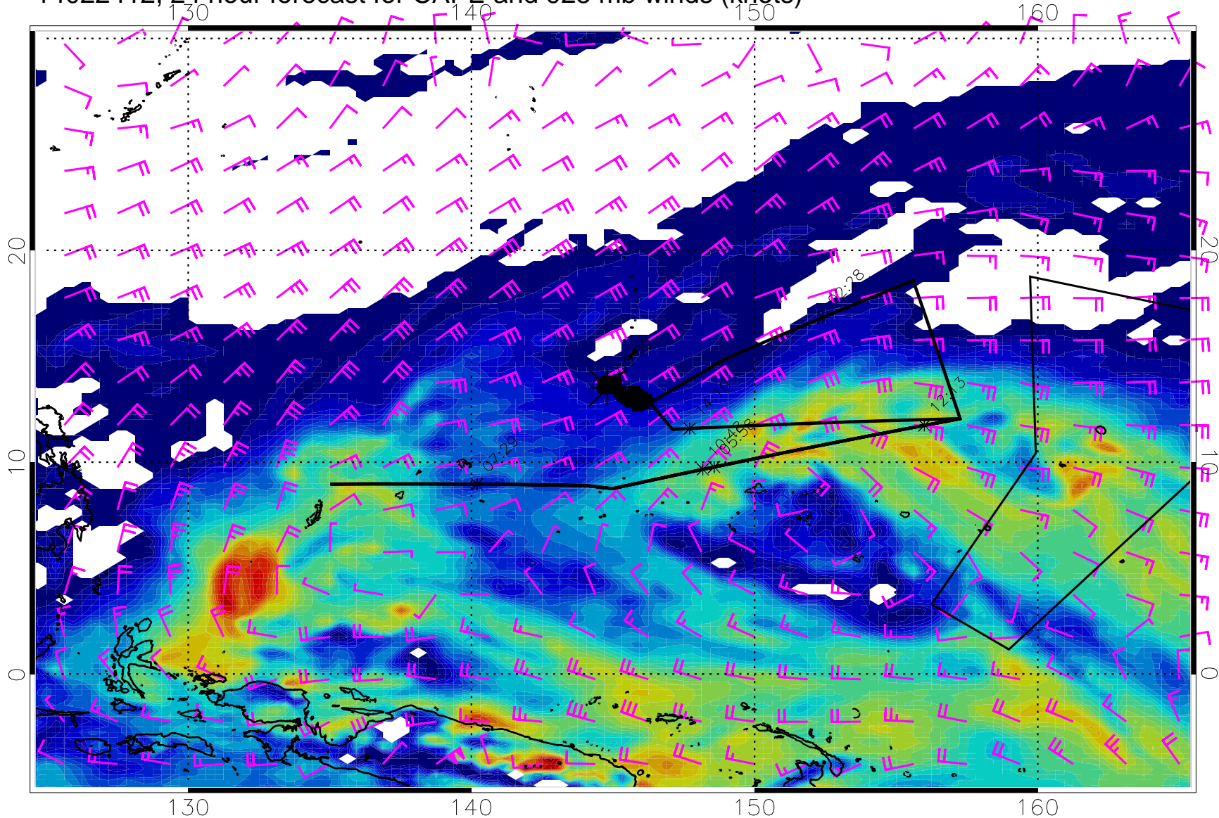
14022412, 24 hour forecast for CAPE and 925 mb winds (knots)
