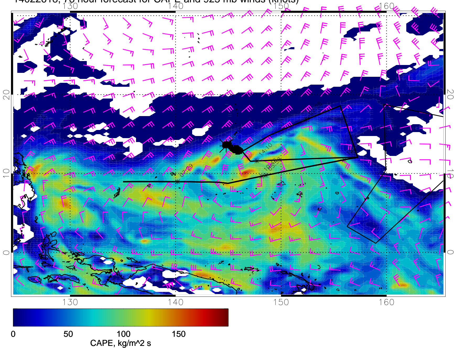
14022618, 78 hour forecast for CAPE and 925 mb winds (knots)
