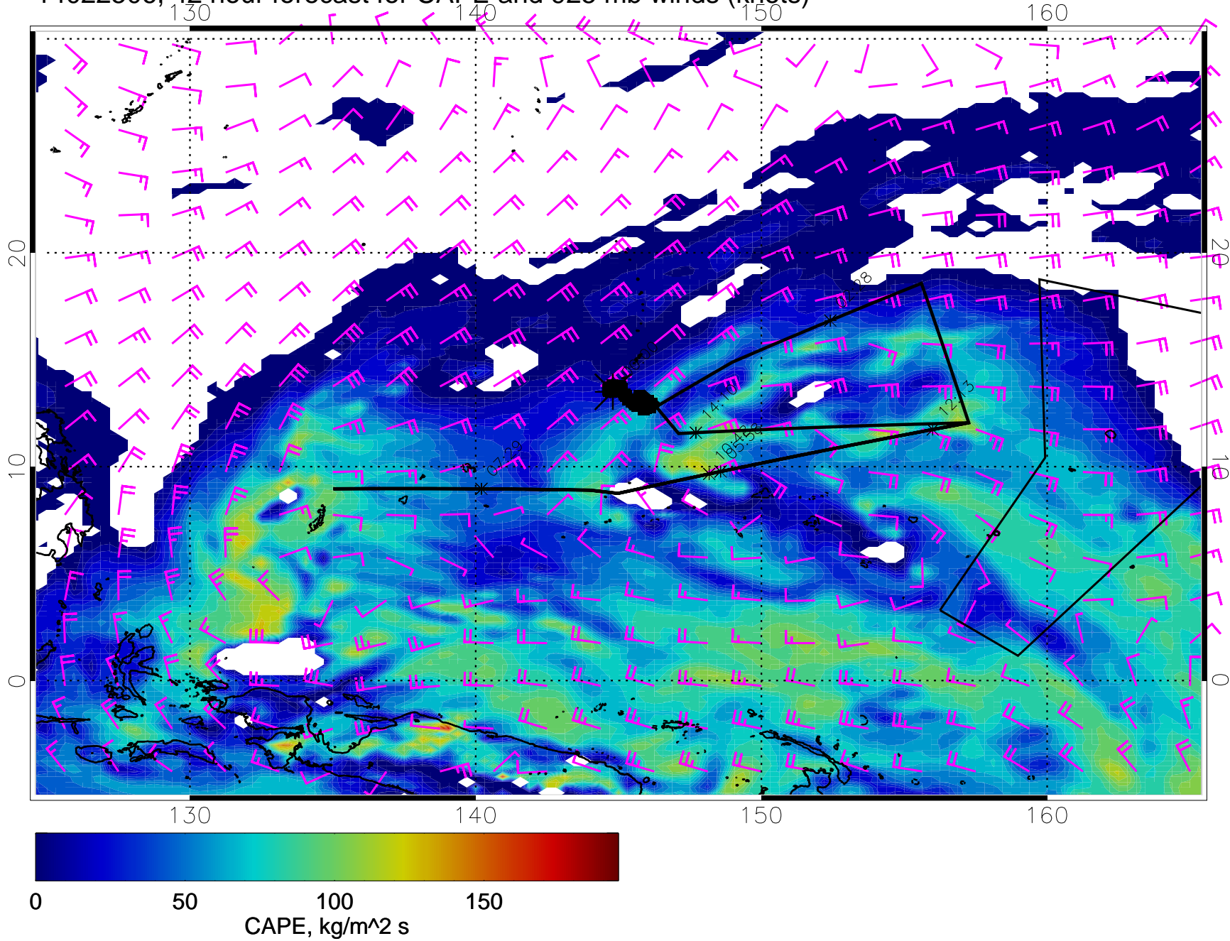
14022506, 42 hour forecast for CAPE and 925 mb winds (knots)
