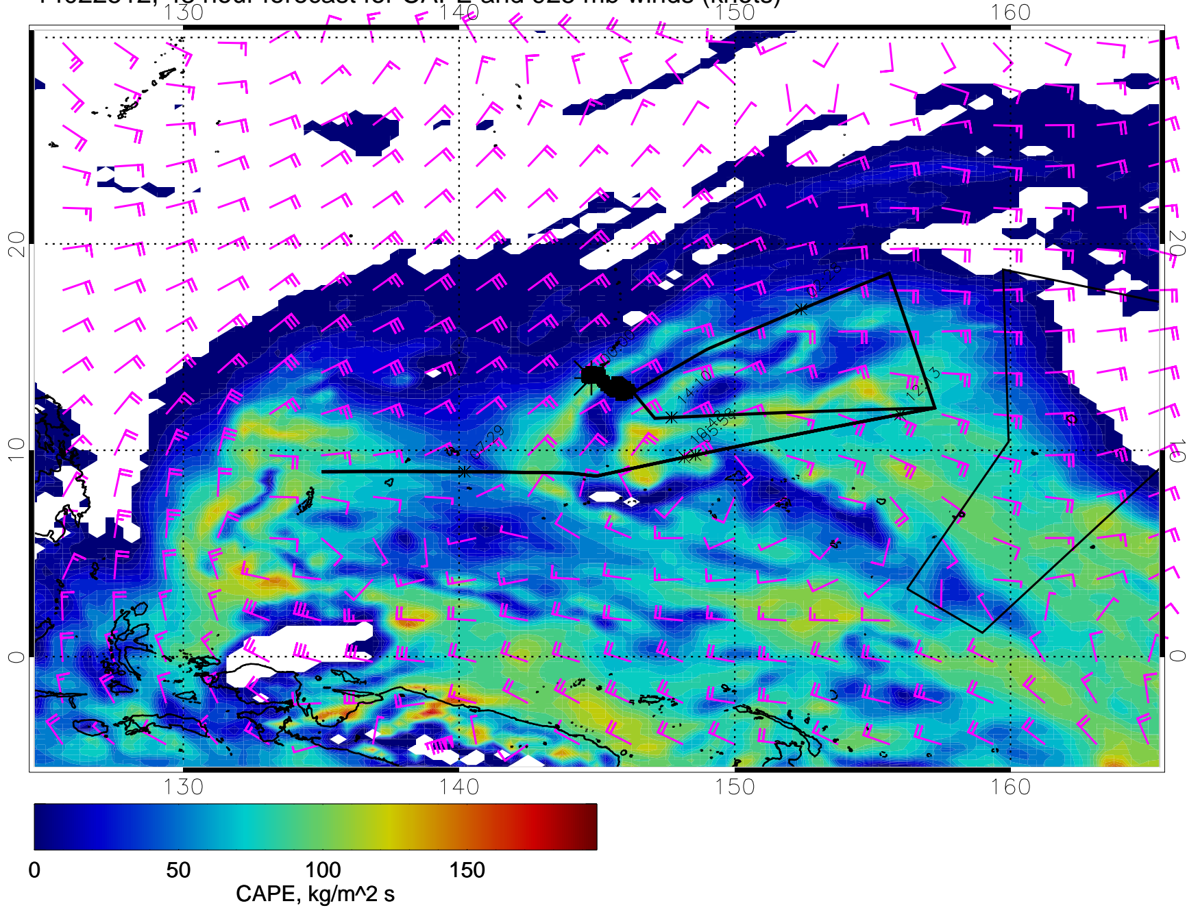
14022512, 48 hour forecast for CAPE and 925 mb winds (knots)
