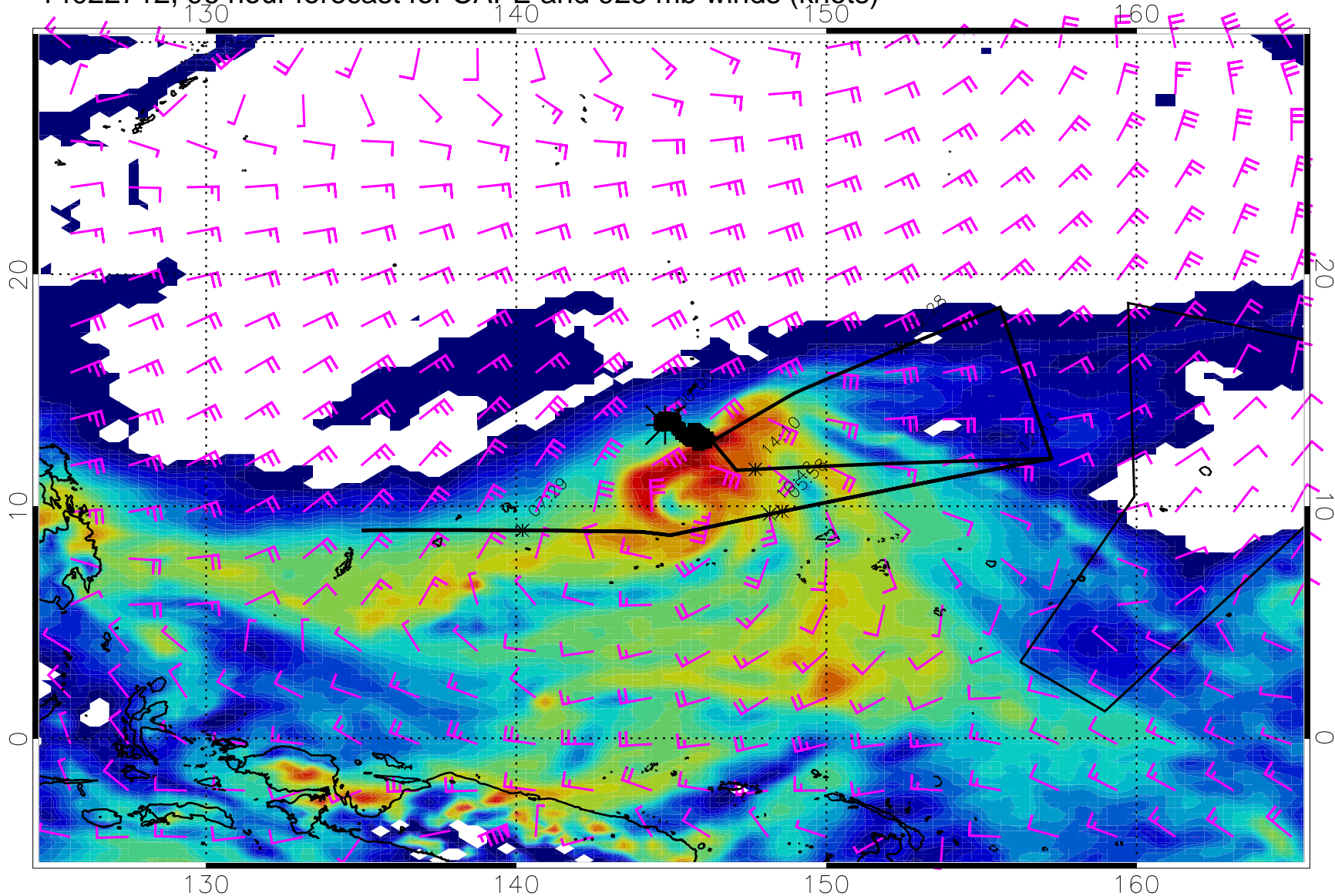
14022712, 96 hour forecast for CAPE and 925 mb winds (knots)
