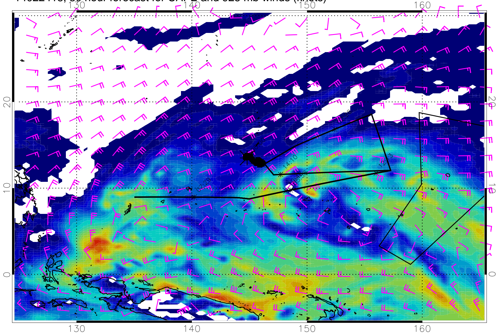
14022418, 30 hour forecast for CAPE and 925 mb winds (knots)
