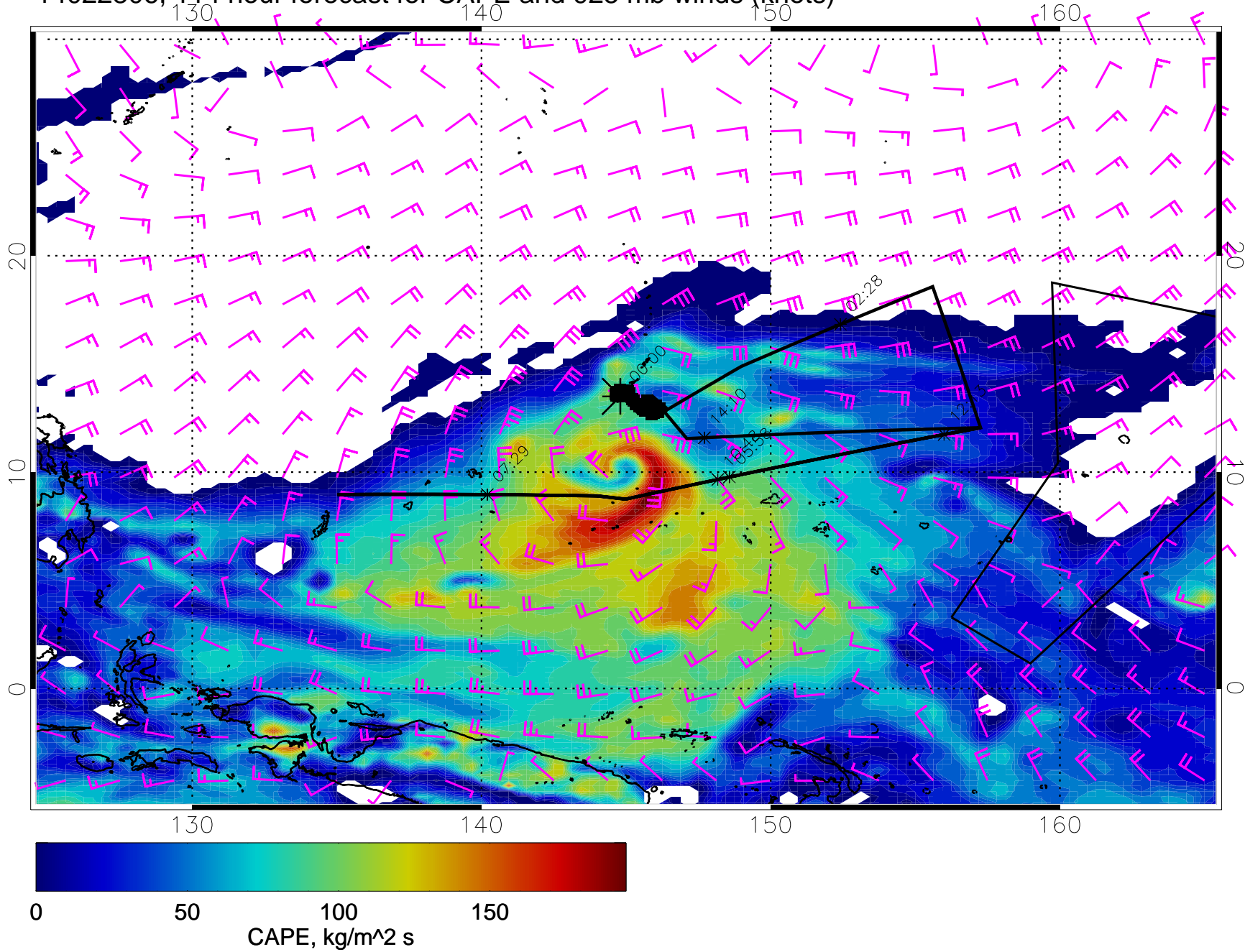
14022806, 114 hour forecast for CAPE and 925 mb winds (knots)
