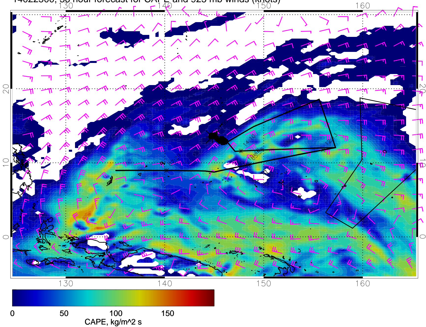
14022500, 36 hour forecast for CAPE and 925 mb winds (knots)
