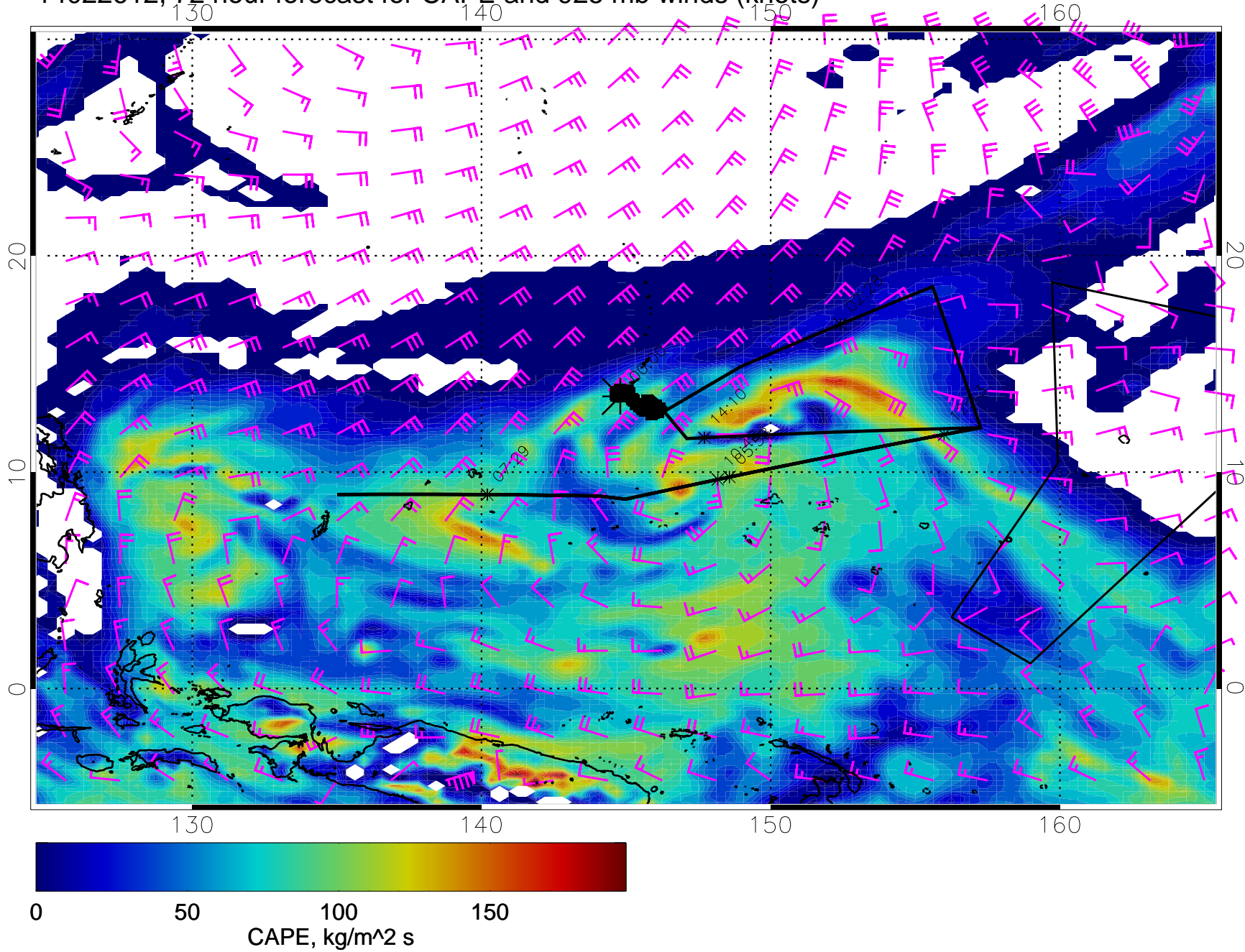
14022612, 72 hour forecast for CAPE and 925 mb winds (knots)
