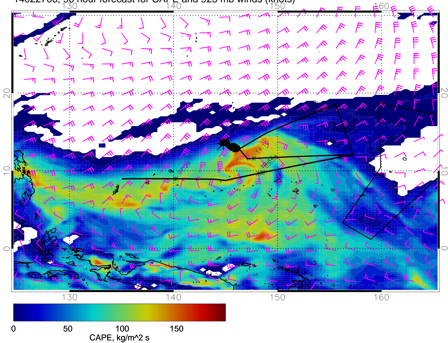
14022706, 90 hour forecast for CAPE and 925 mb winds (knots)
