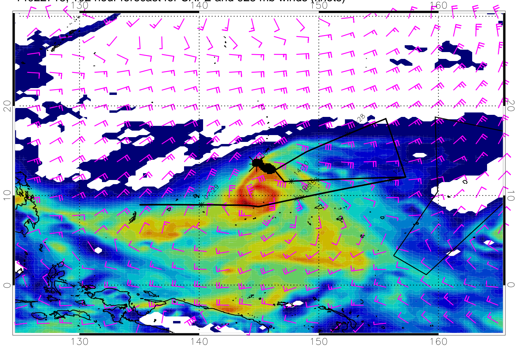
14022718, 102 hour forecast for CAPE and 925 mb winds (knots)
