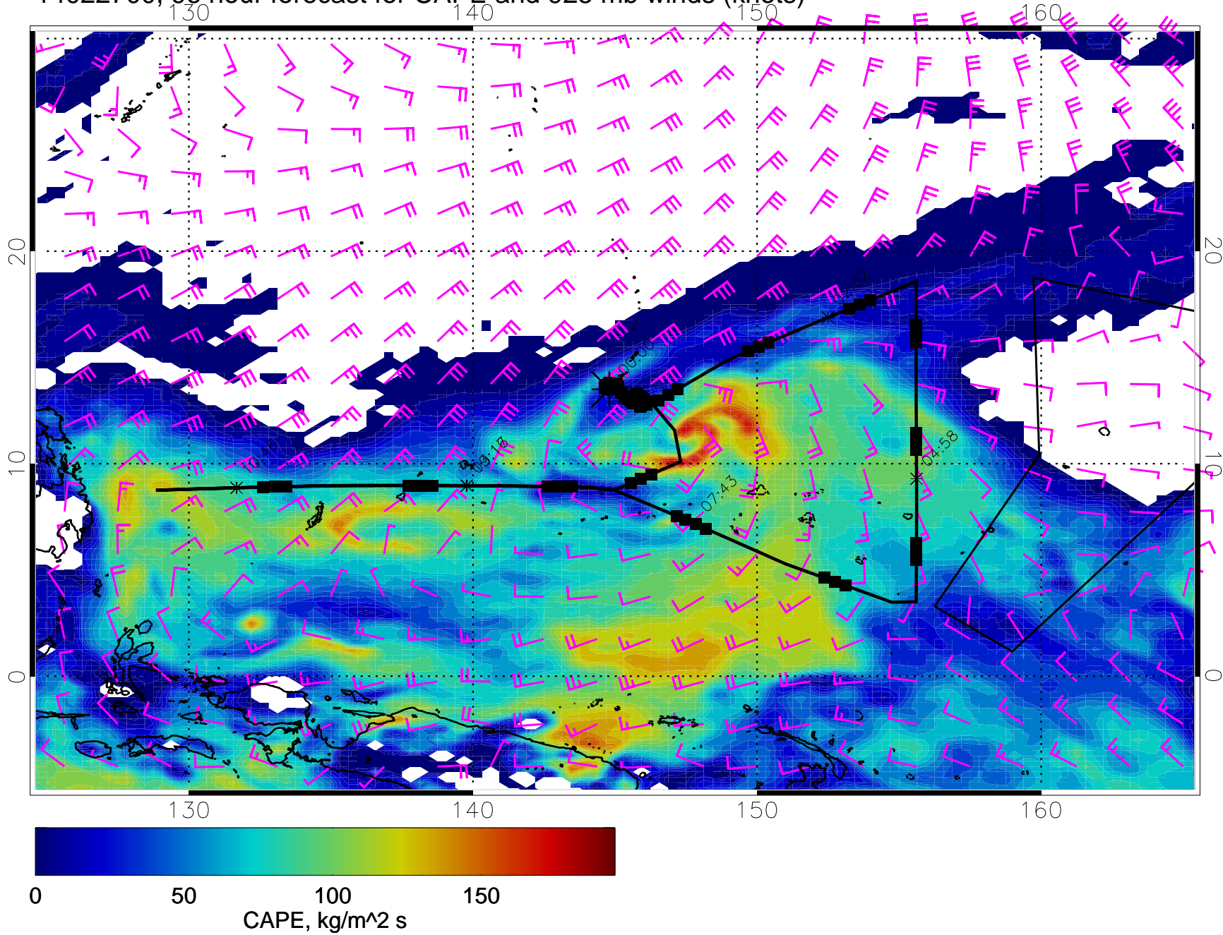
14022700, 96 hour forecast for CAPE and 925 mb winds (knots)
