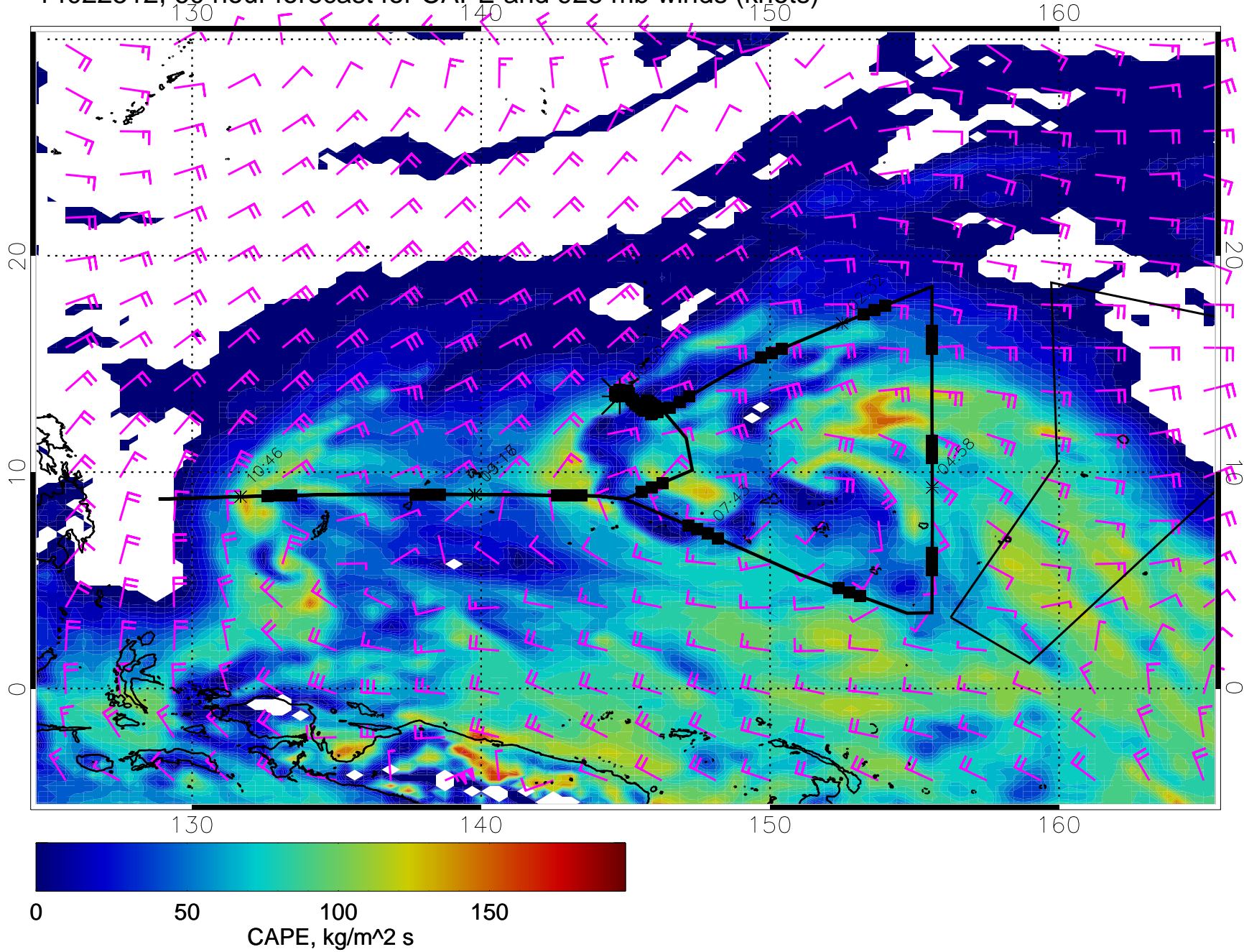
14022512, 60 hour forecast for CAPE and 925 mb winds (knots)
