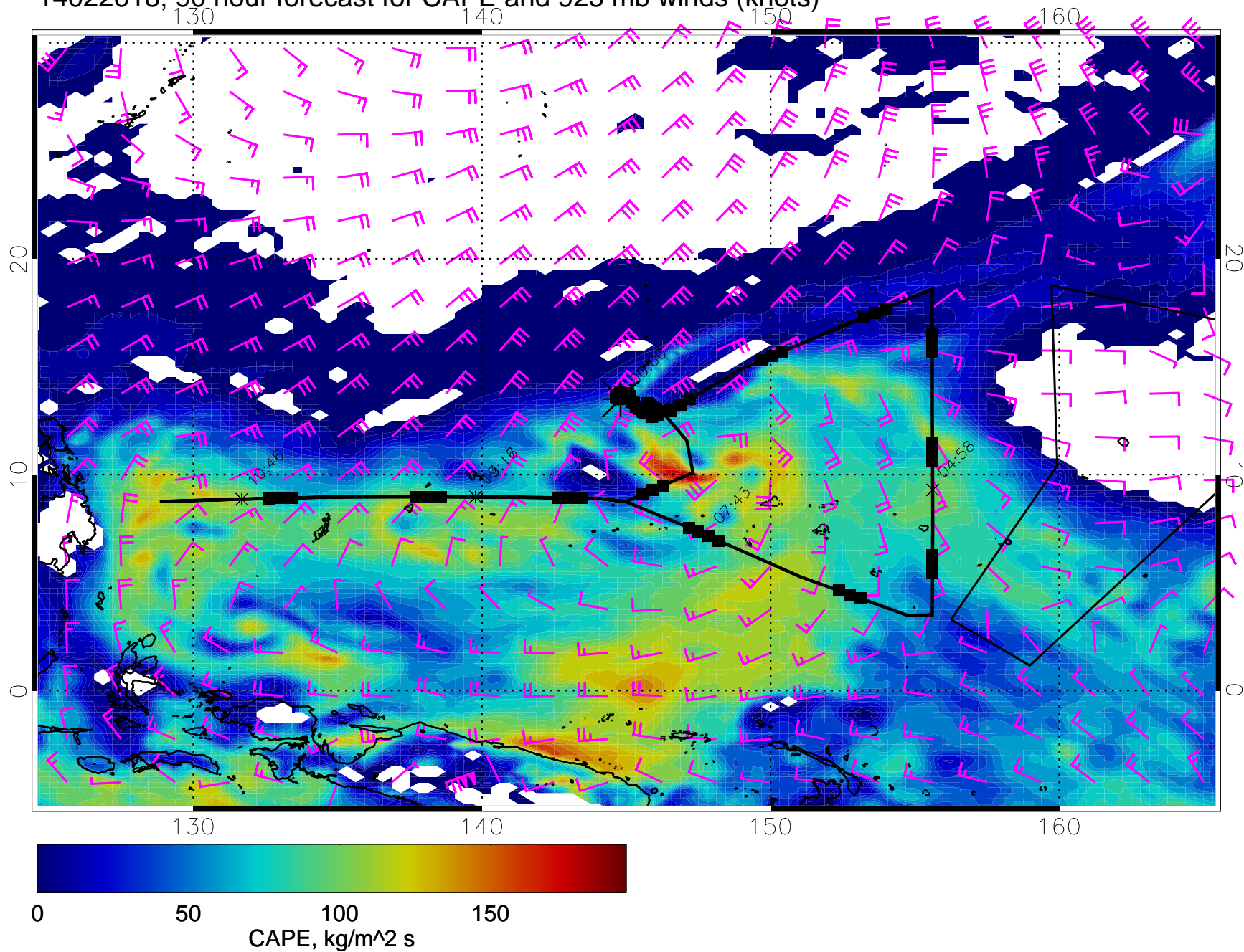
14022618, 90 hour forecast for CAPE and 925 mb winds (knots)
