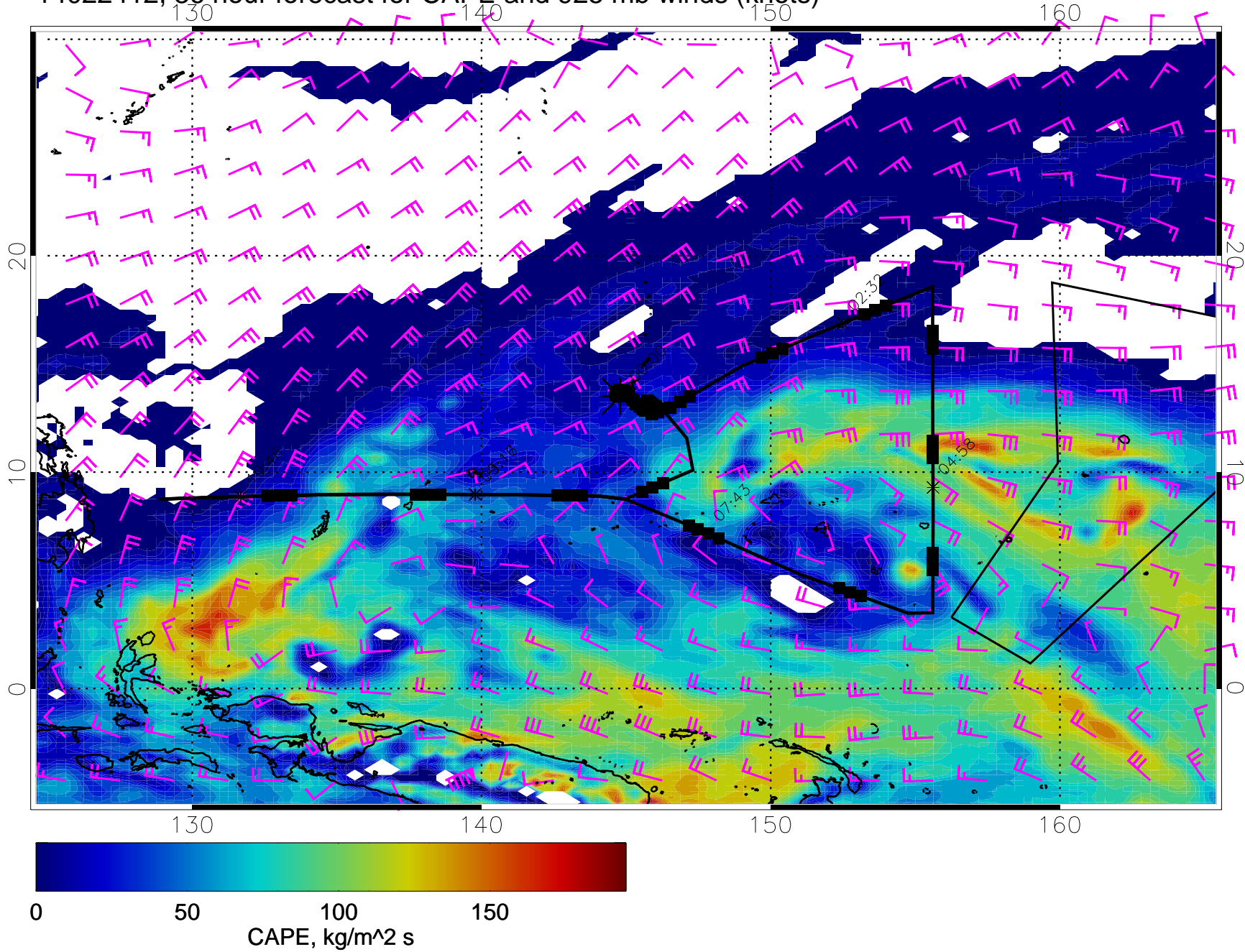
14022412, 36 hour forecast for CAPE and 925 mb winds (knots)
