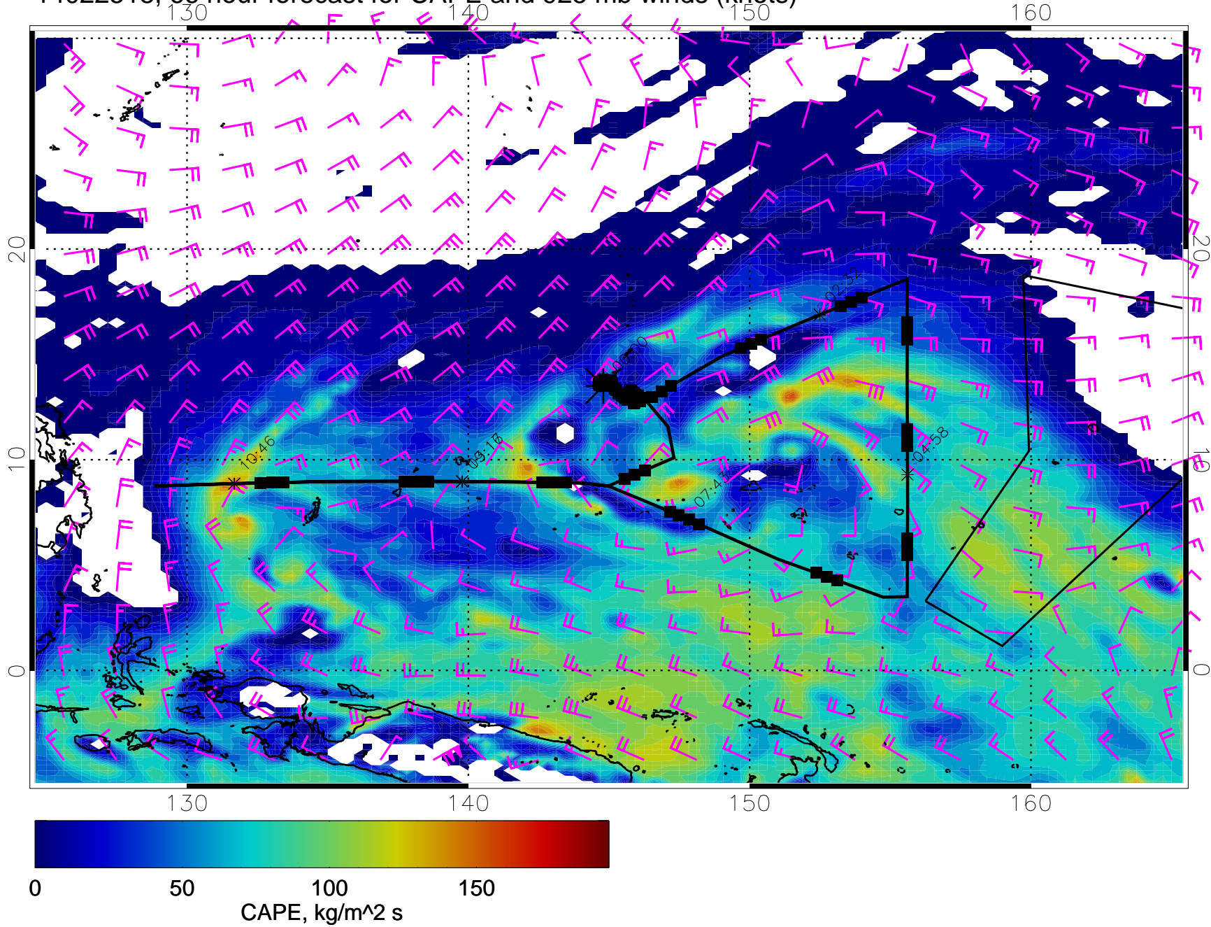
14022518, 66 hour forecast for CAPE and 925 mb winds (knots)
