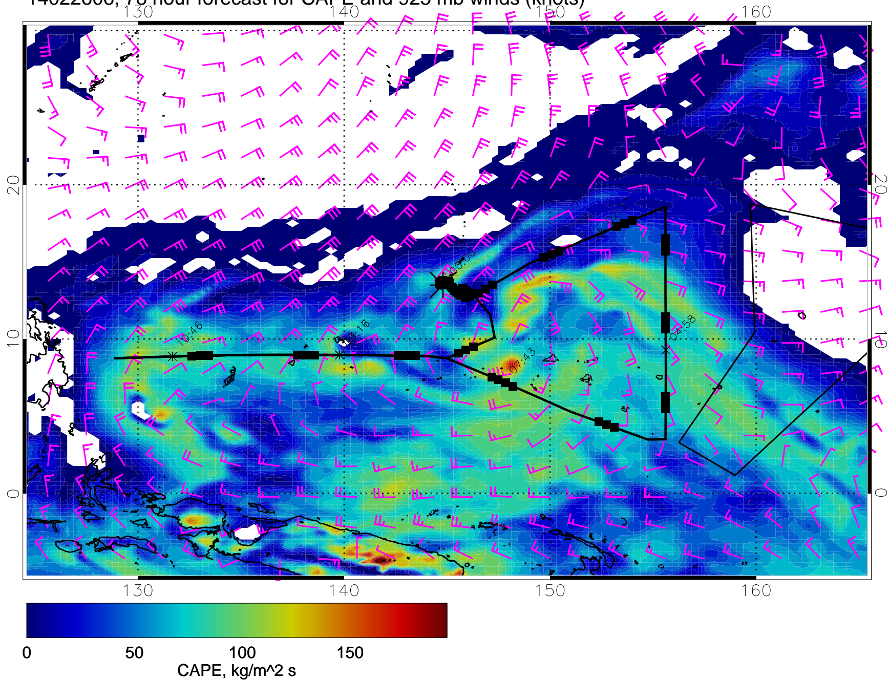
14022606, 78 hour forecast for CAPE and 925 mb winds (knots)
