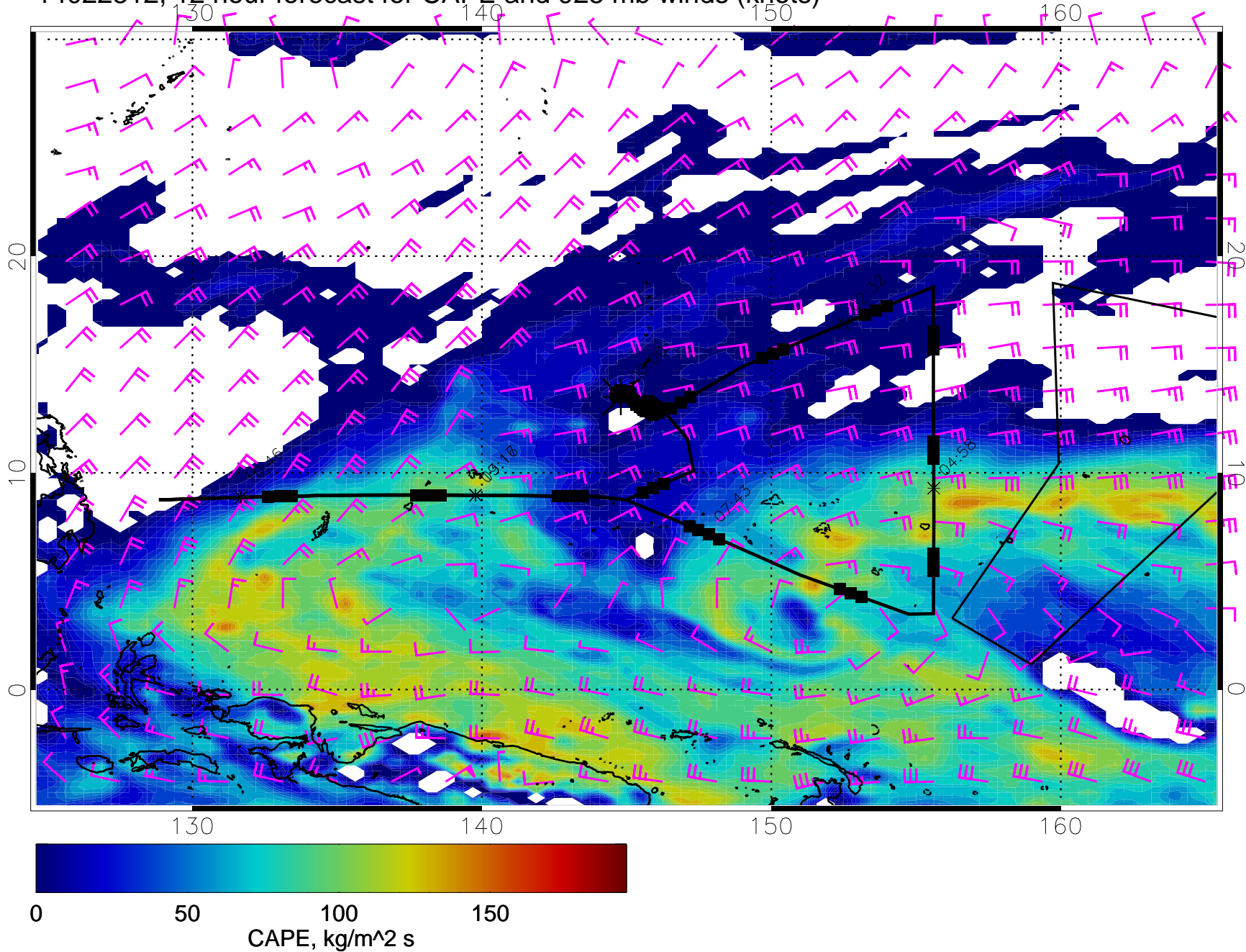
14022312, 12 hour forecast for CAPE and 925 mb winds (knots)
