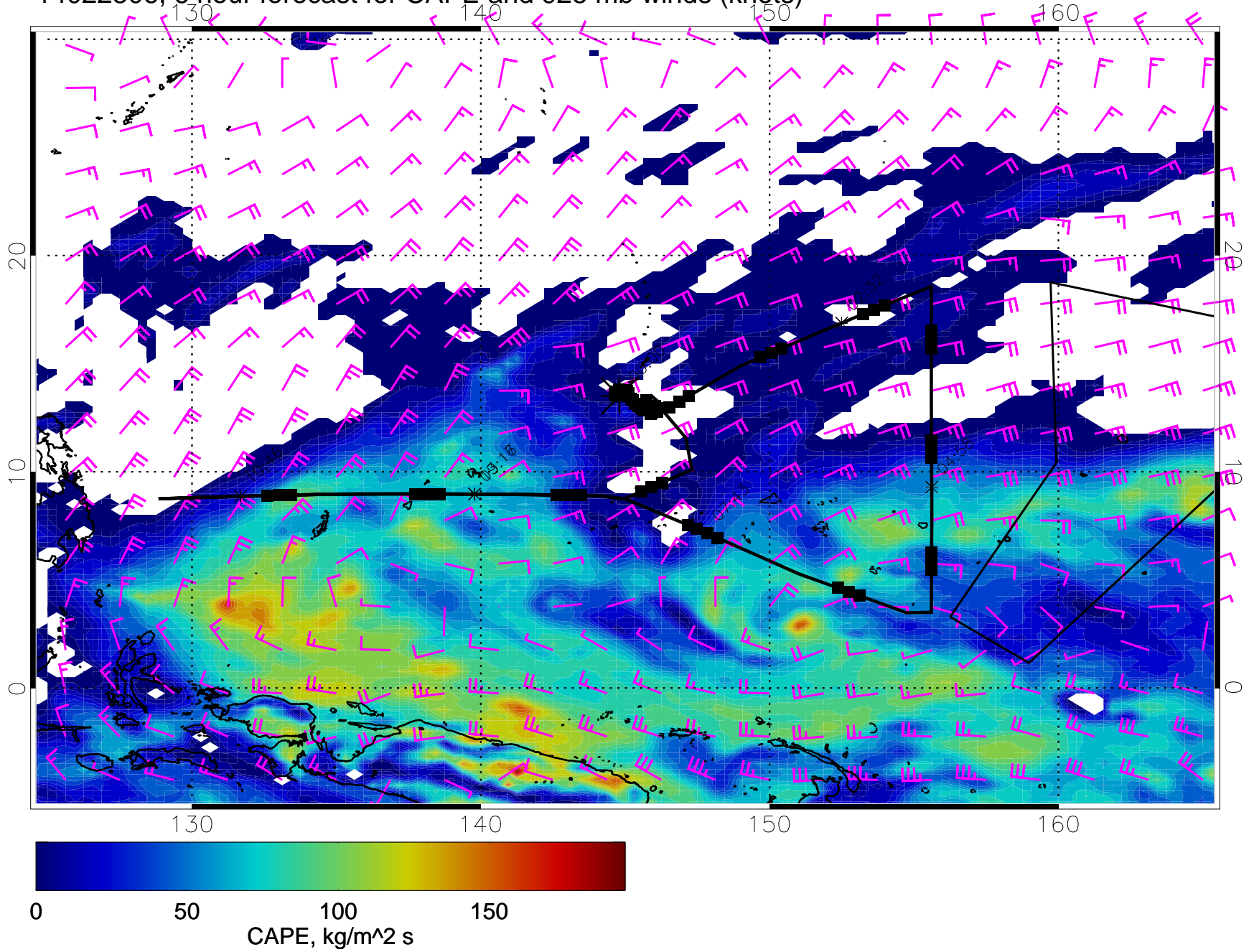
14022306, 6 hour forecast for CAPE and 925 mb winds (knots)
