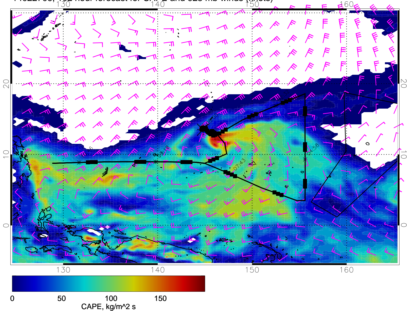
14022706, 102 hour forecast for CAPE and 925 mb winds (knots)
