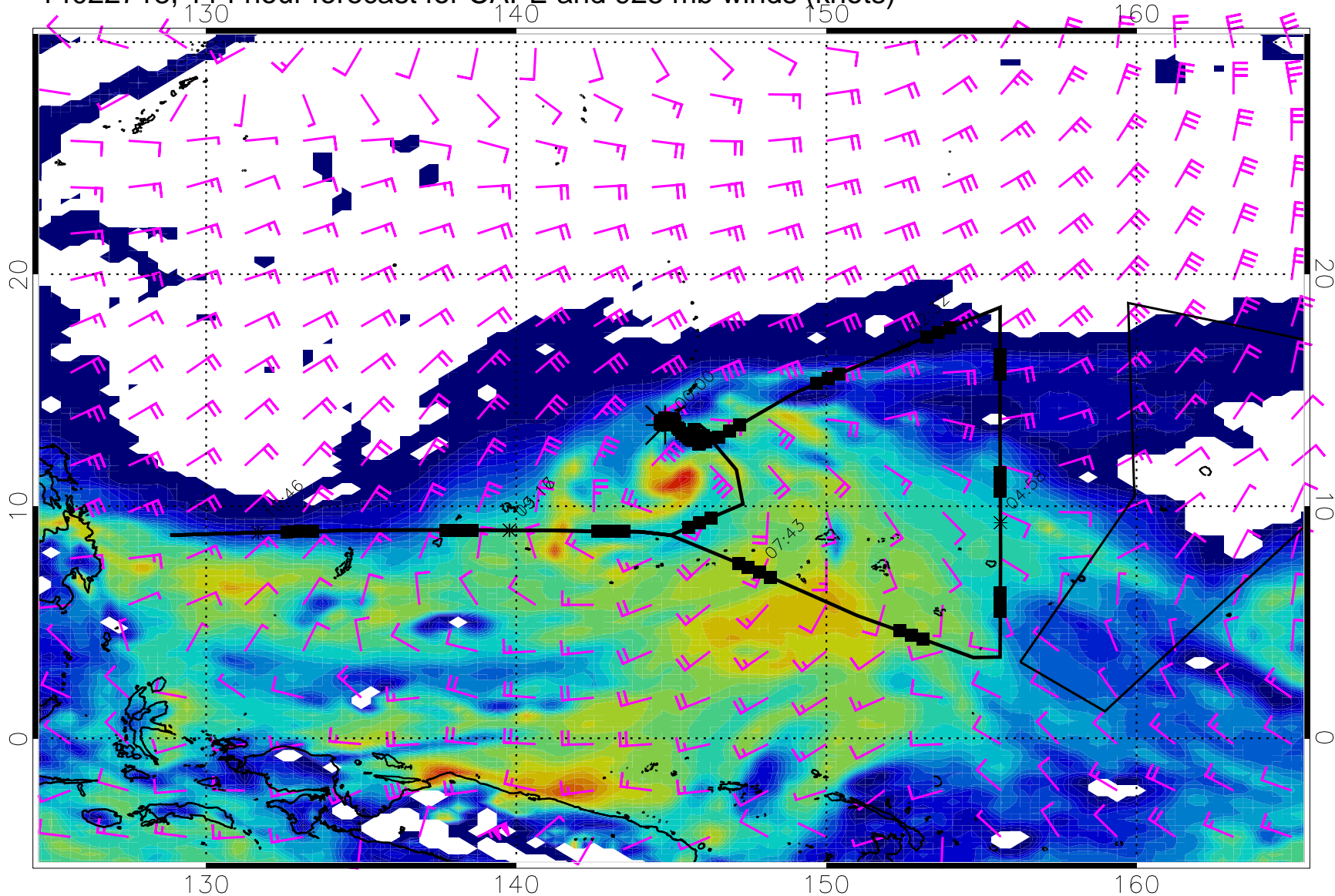
14022718, 114 hour forecast for CAPE and 925 mb winds (knots)
