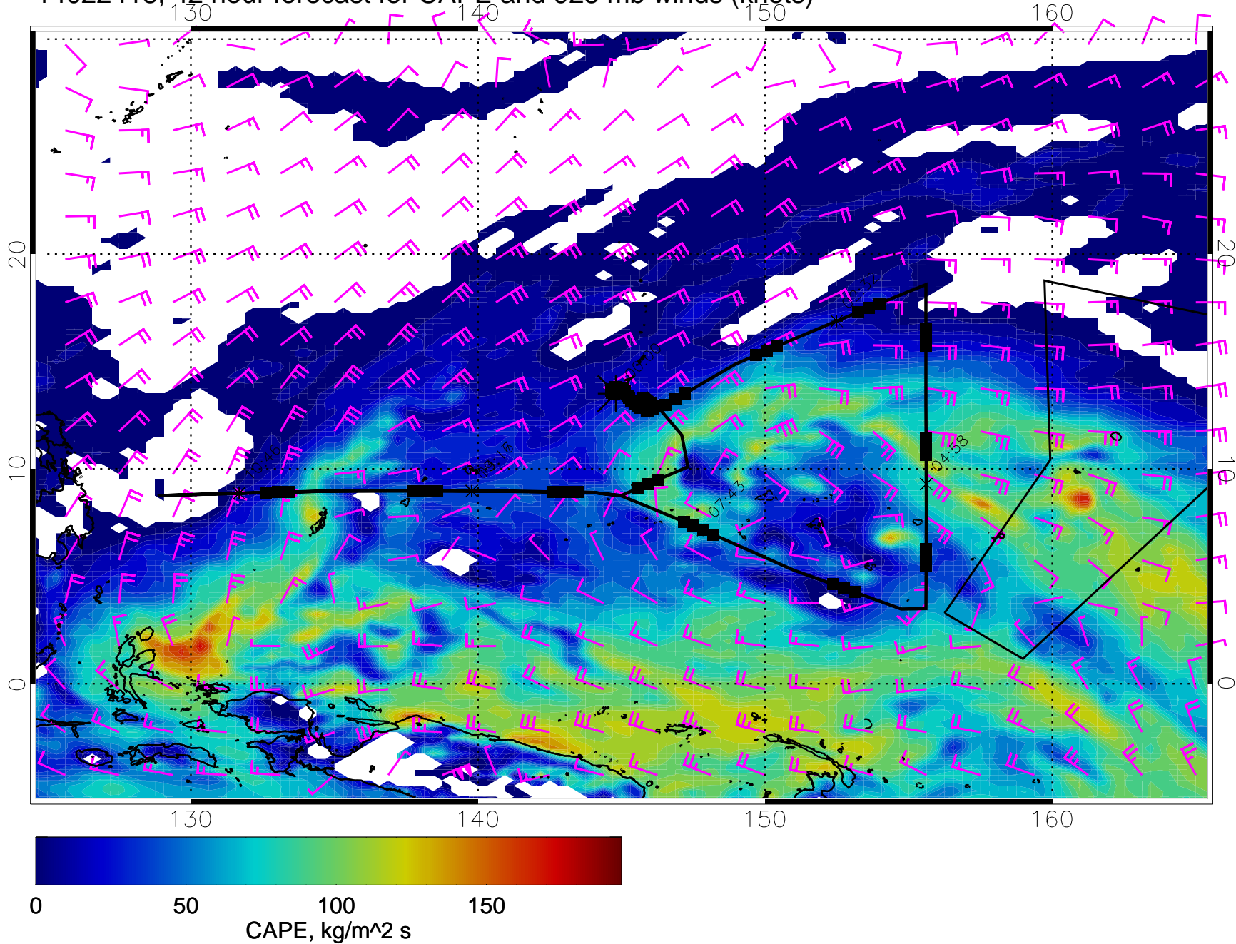
14022418, 42 hour forecast for CAPE and 925 mb winds (knots)
