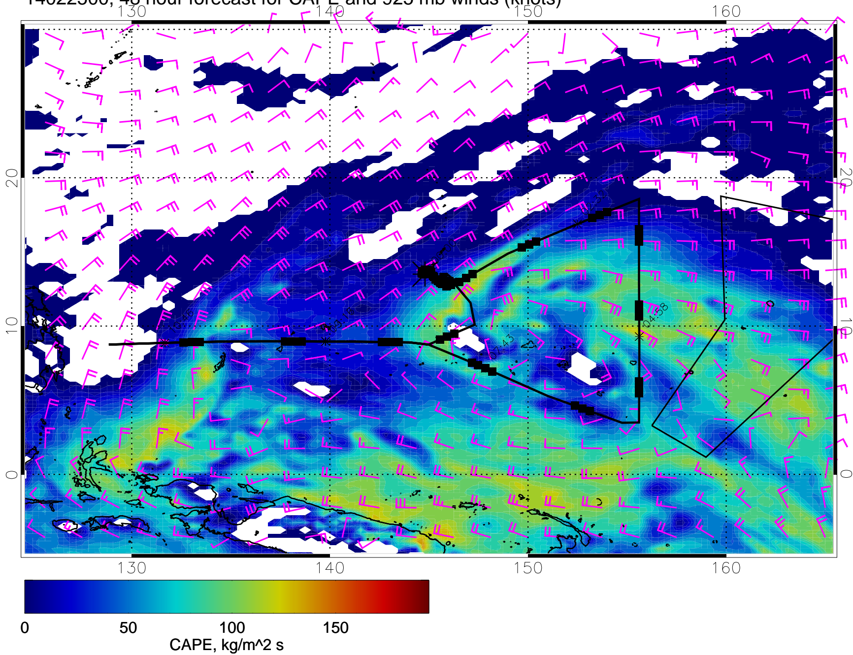
14022500, 48 hour forecast for CAPE and 925 mb winds (knots)
