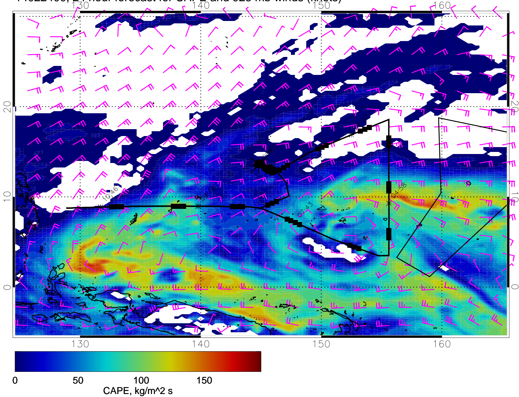
14022400, 24 hour forecast for CAPE and 925 mb winds (knots)
