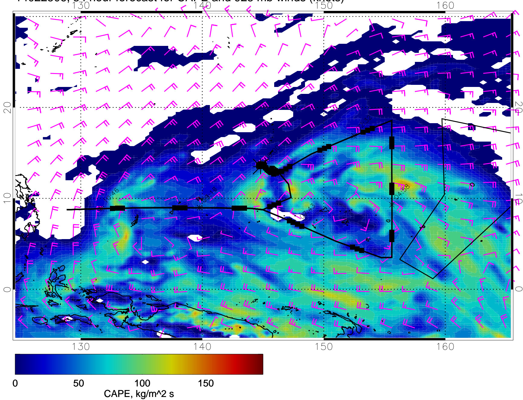
14022506, 54 hour forecast for CAPE and 925 mb winds (knots)
