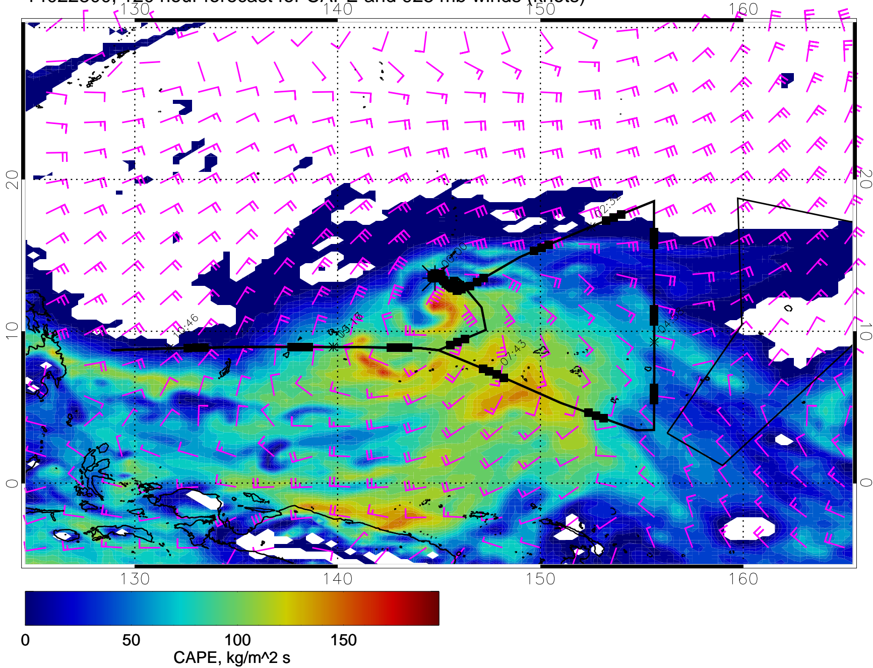
14022800, 120 hour forecast for CAPE and 925 mb winds (knots)
