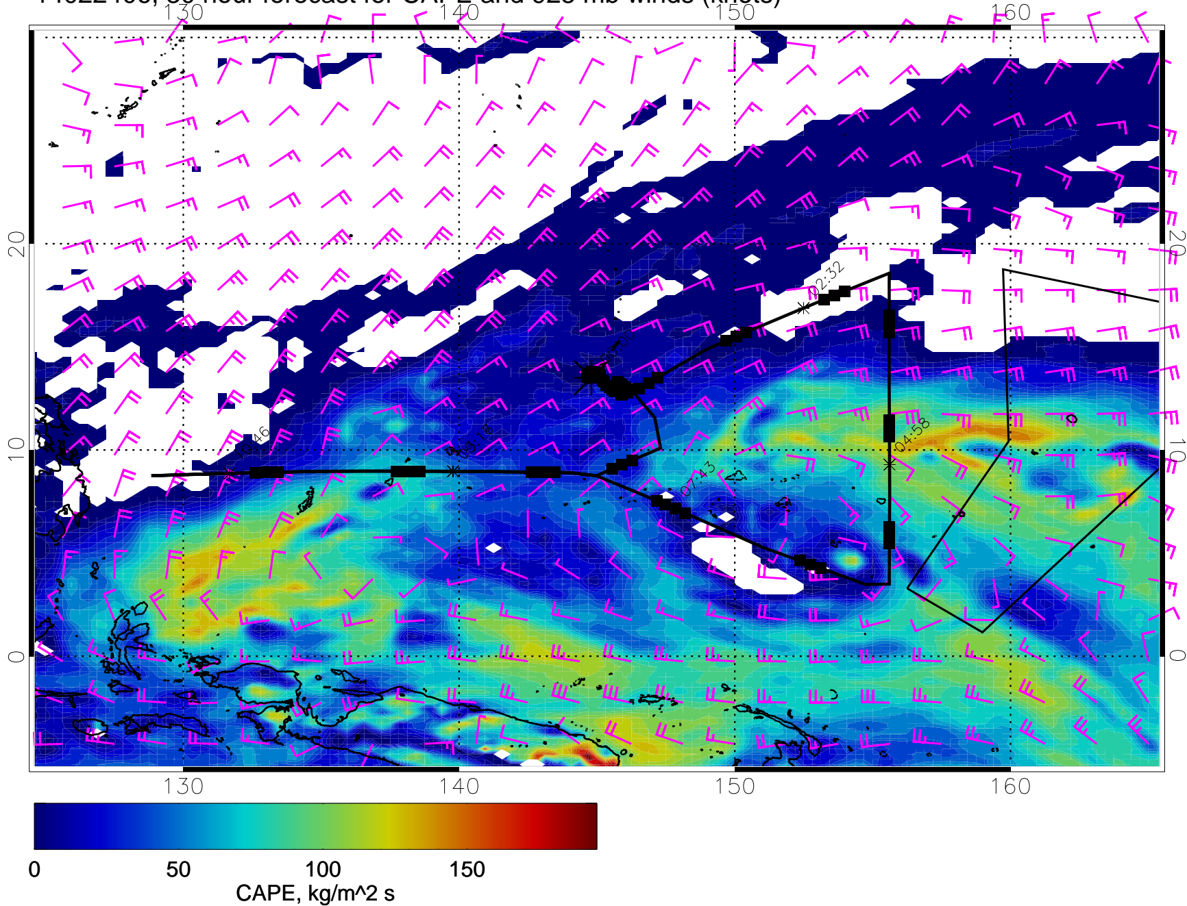
14022406, 30 hour forecast for CAPE and 925 mb winds (knots)
