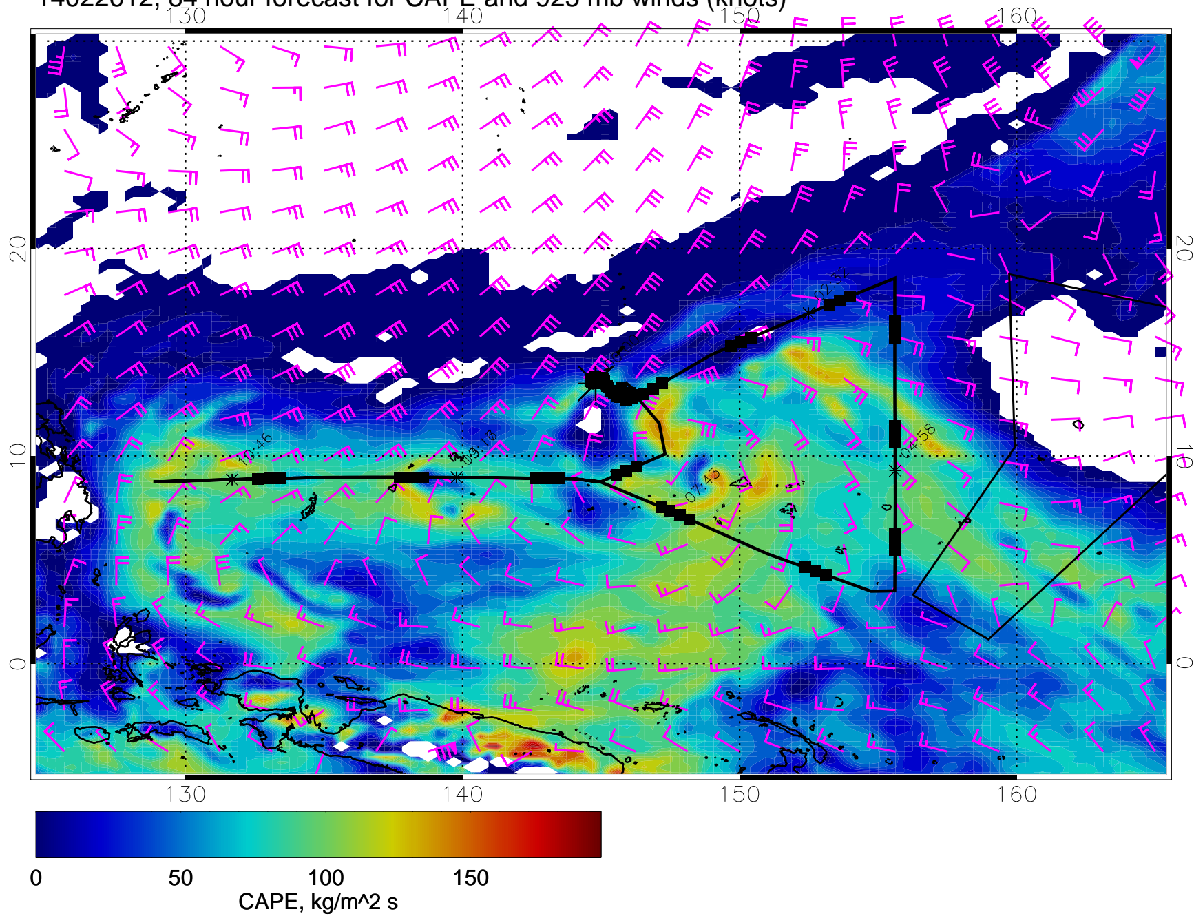
14022612, 84 hour forecast for CAPE and 925 mb winds (knots)
