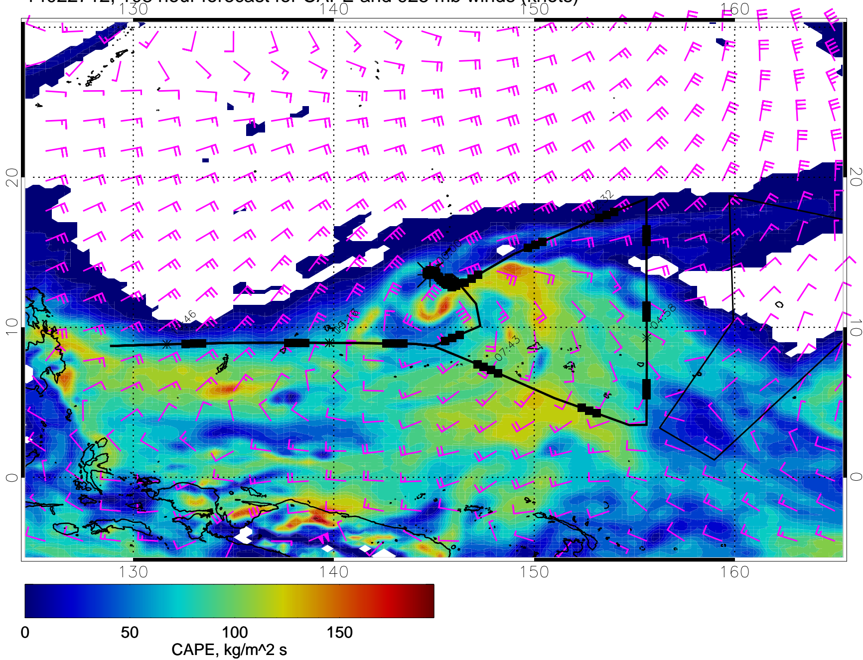
14022712, 108 hour forecast for CAPE and 925 mb winds (knots)
