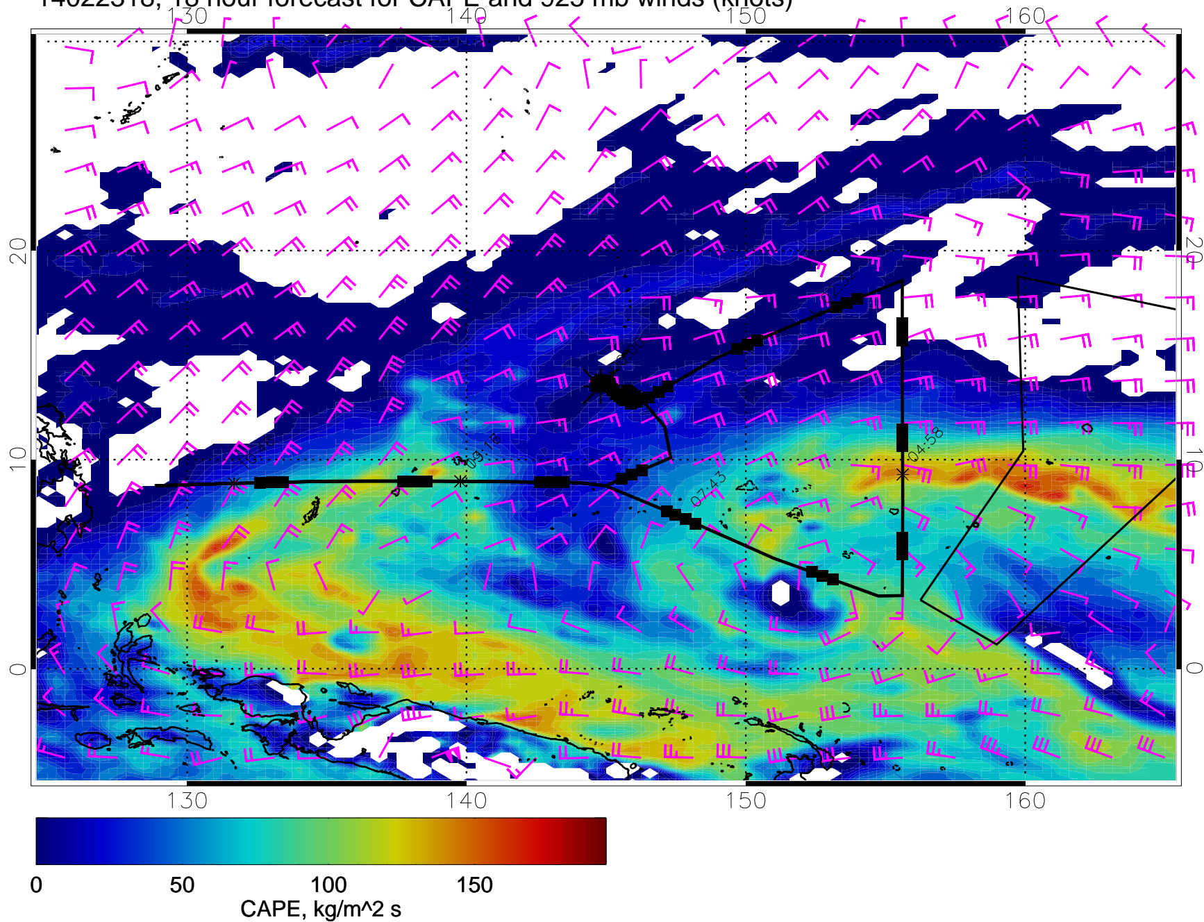
14022318, 18 hour forecast for CAPE and 925 mb winds (knots)
