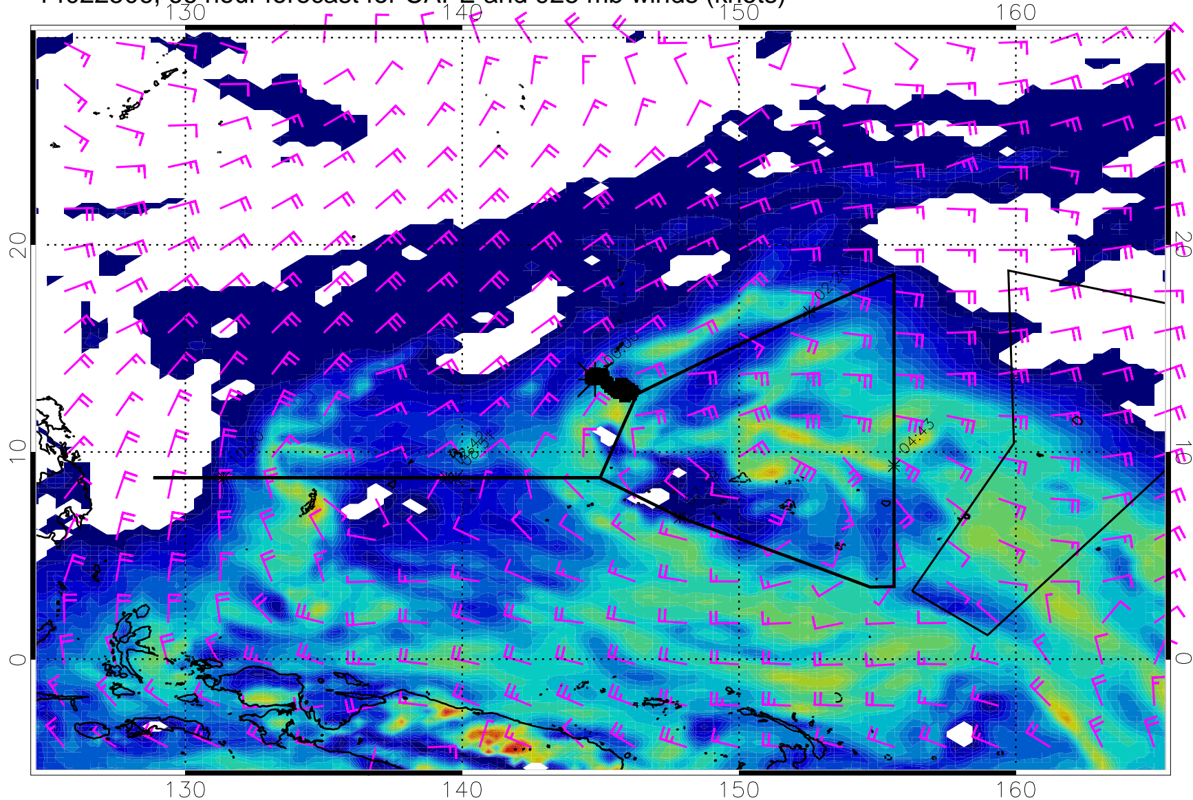
14022506, 66 hour forecast for CAPE and 925 mb winds (knots)
