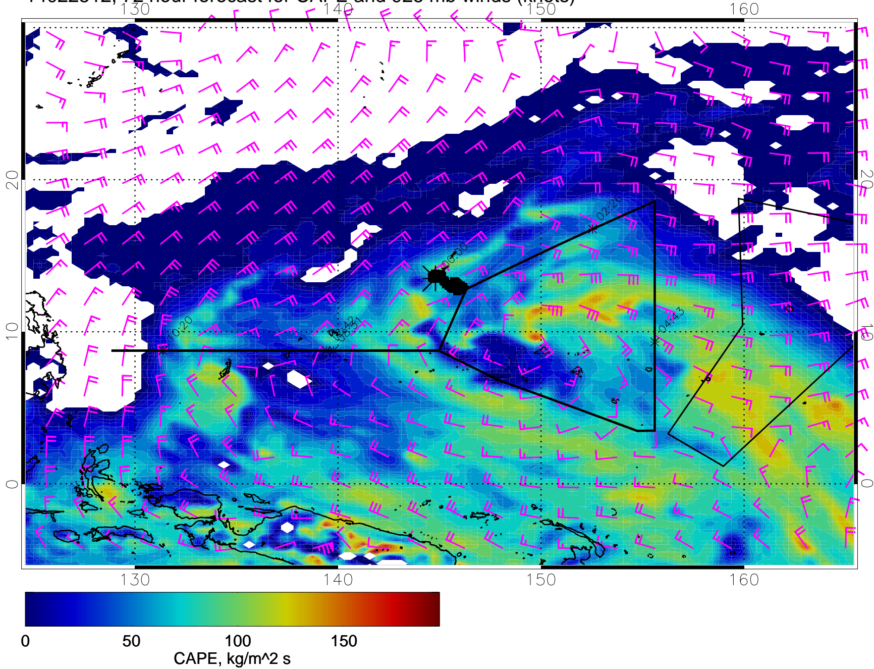
14022512, 72 hour forecast for CAPE and 925 mb winds (knots)
