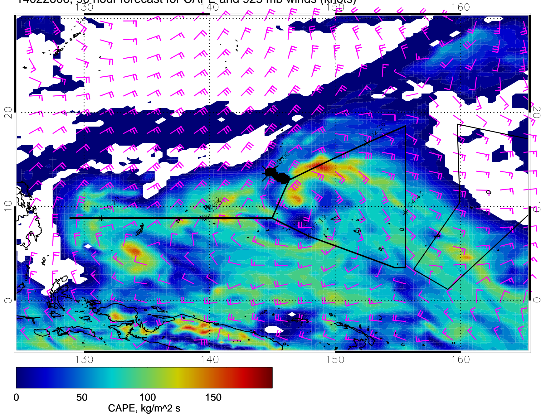
14022606, 90 hour forecast for CAPE and 925 mb winds (knots)
