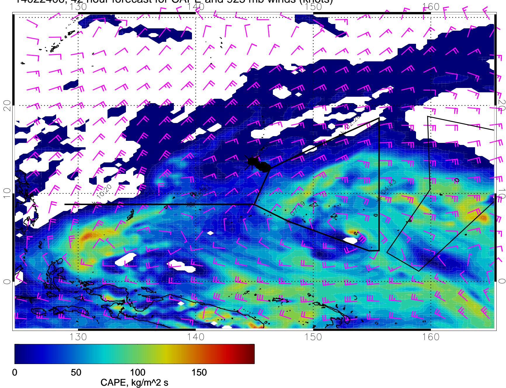
14022406, 42 hour forecast for CAPE and 925 mb winds (knots)
