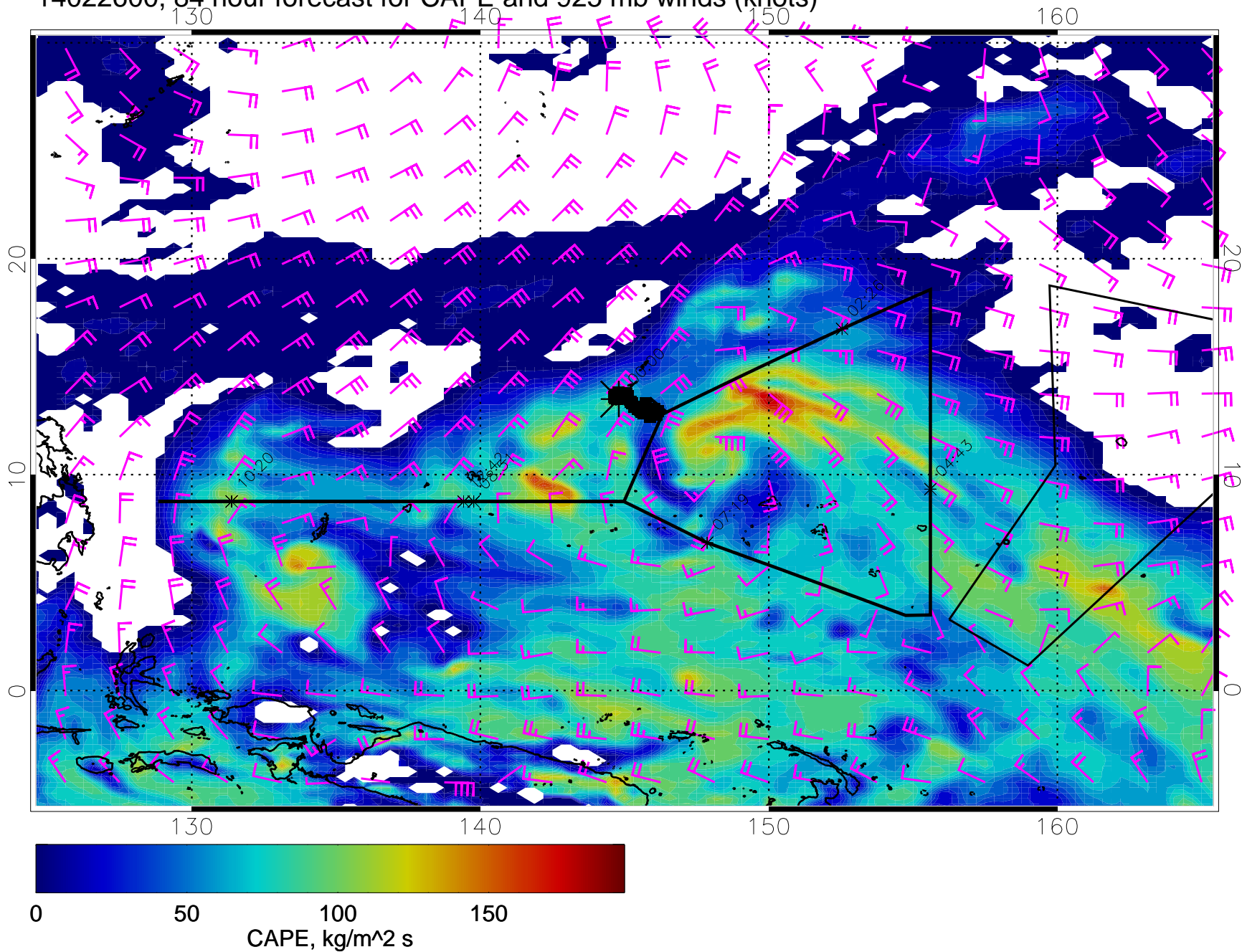
14022600, 84 hour forecast for CAPE and 925 mb winds (knots)
