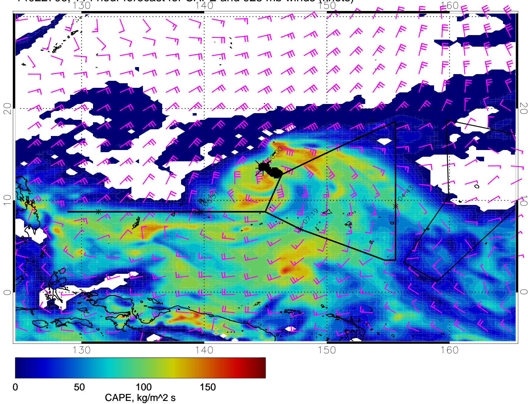
14022706, 114 hour forecast for CAPE and 925 mb winds (knots)
