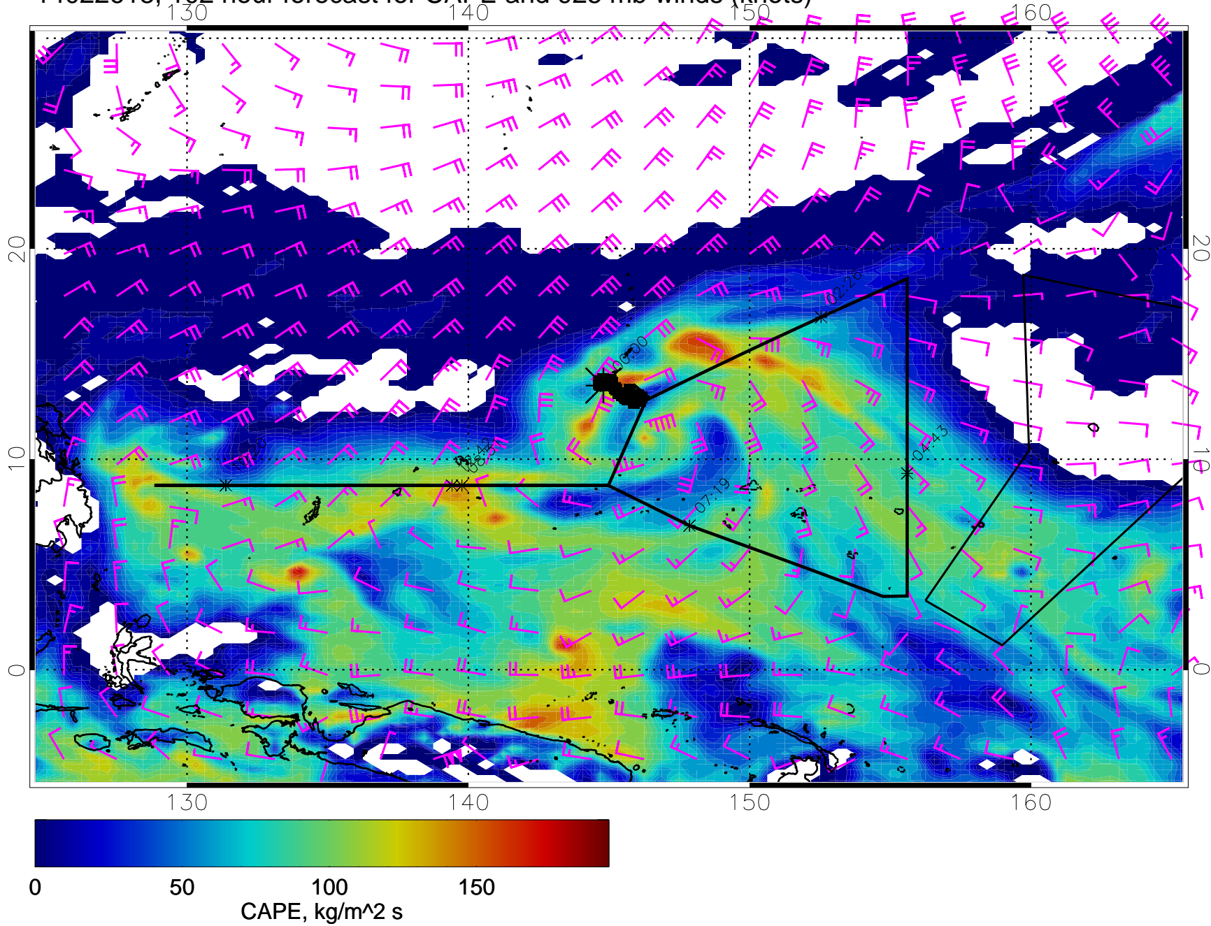
14022618, 102 hour forecast for CAPE and 925 mb winds (knots)
