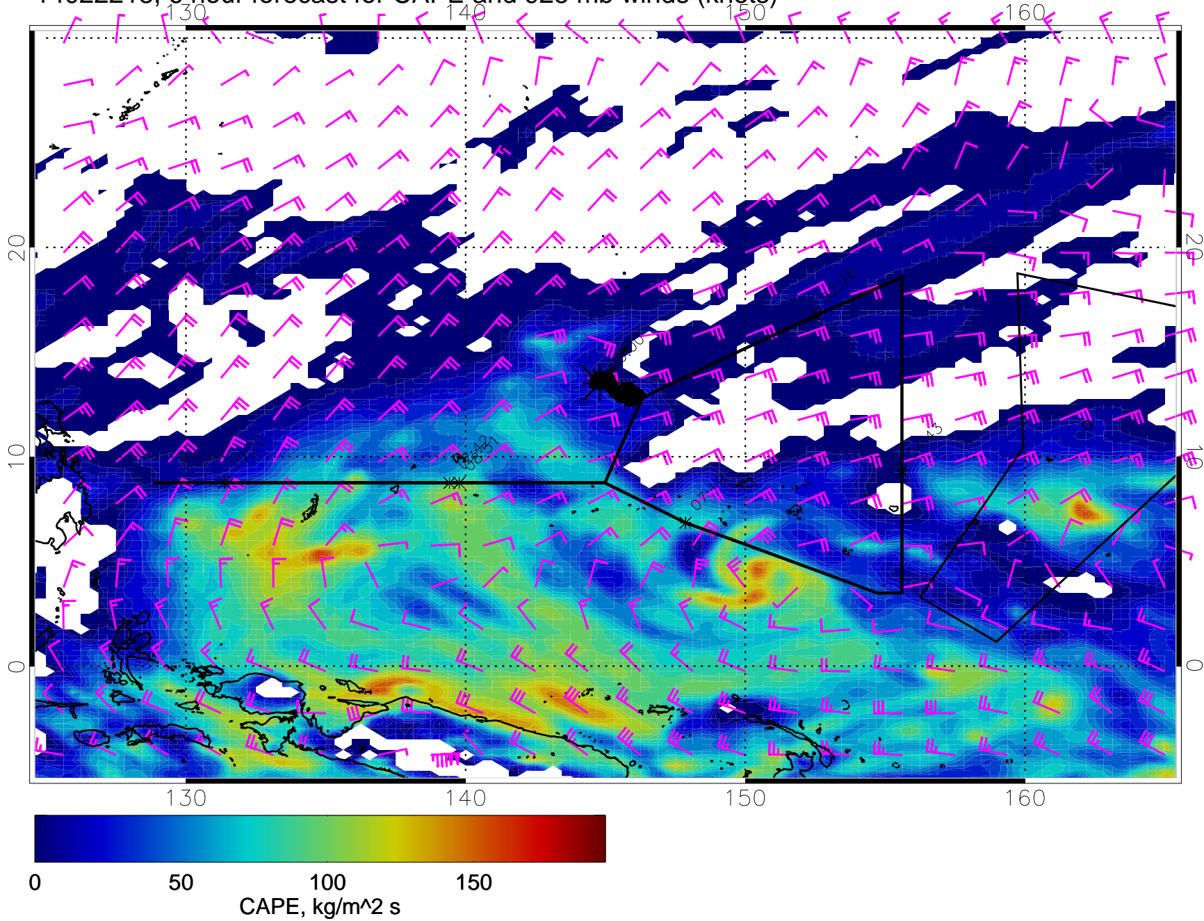
14022218, 6 hour forecast for CAPE and 925 mb winds (knots)
