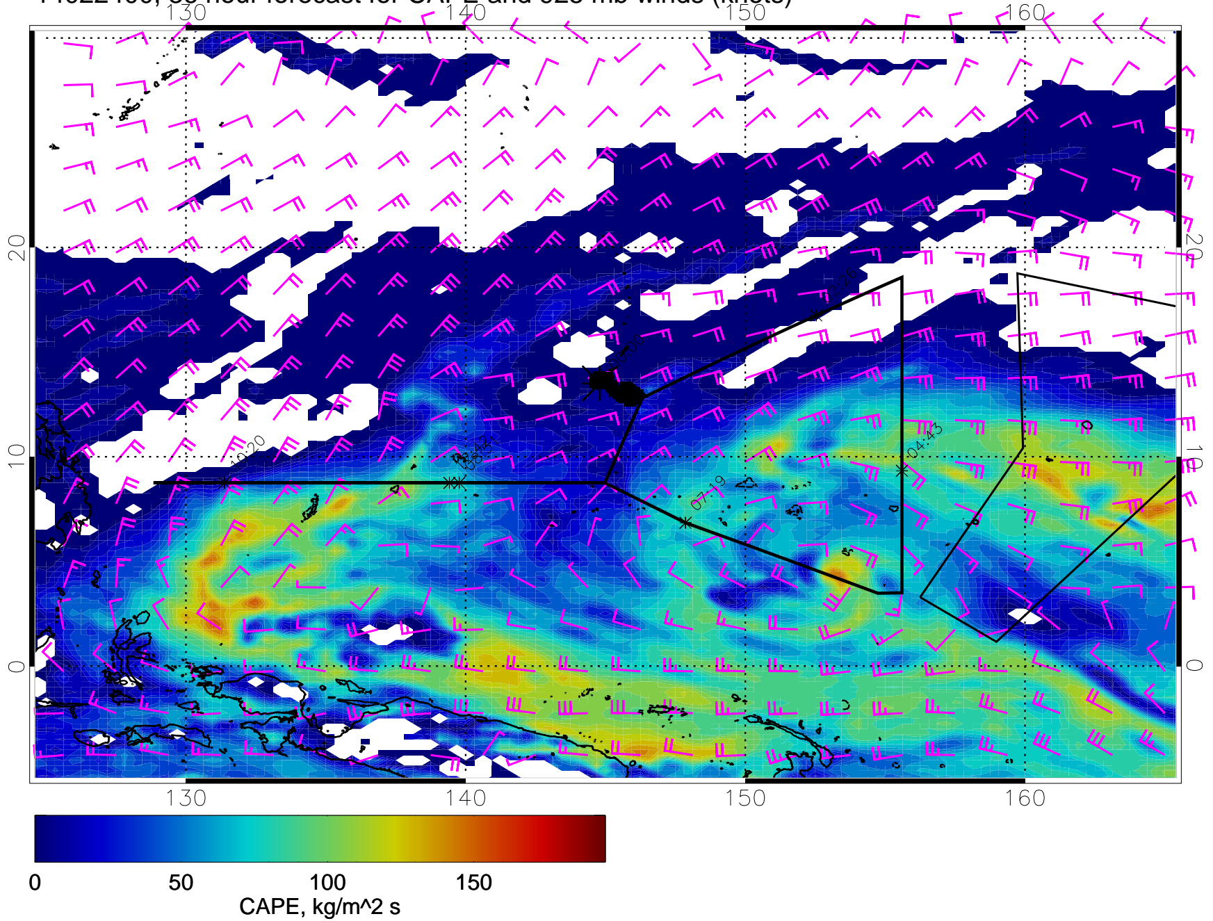
14022400, 36 hour forecast for CAPE and 925 mb winds (knots)
