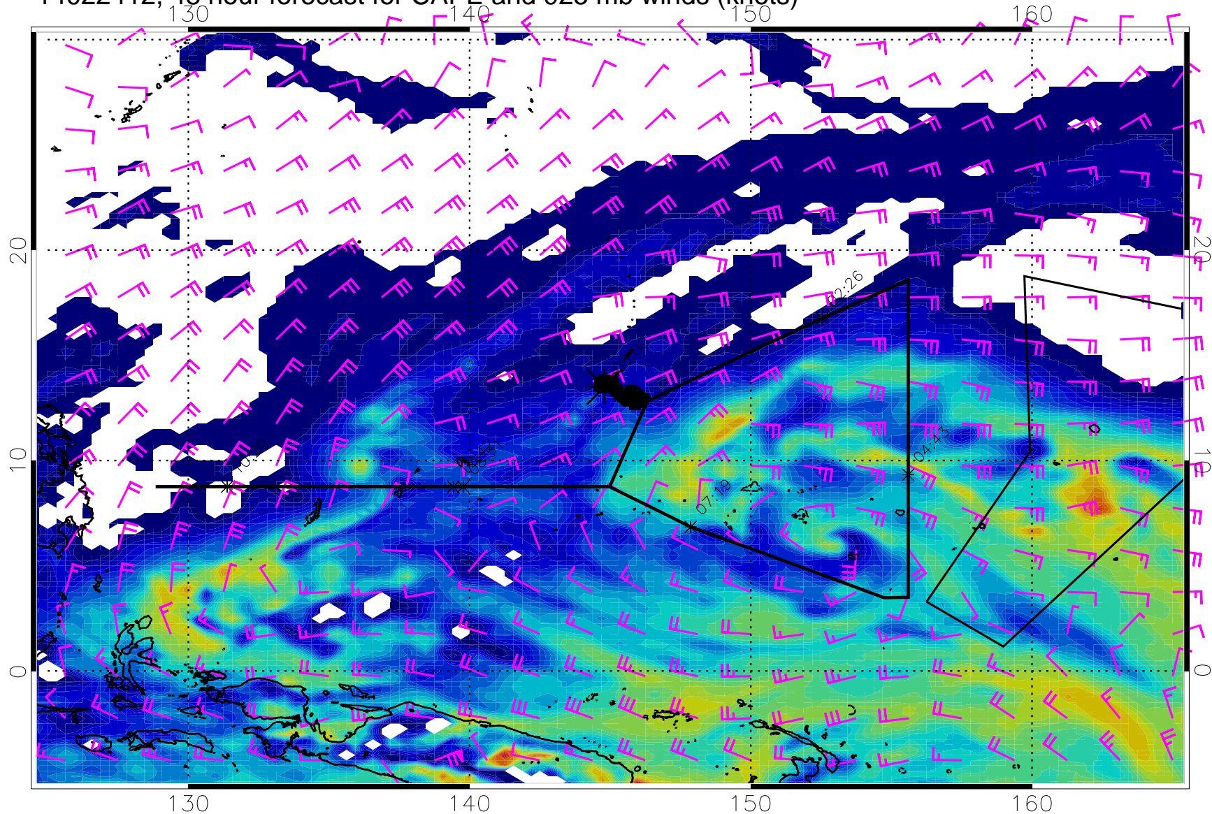
14022412, 48 hour forecast for CAPE and 925 mb winds (knots)
