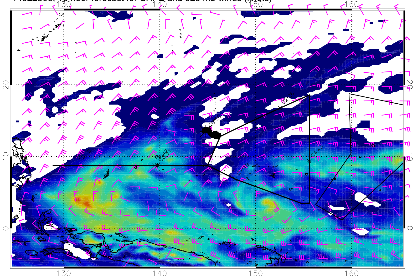
14022306, 18 hour forecast for CAPE and 925 mb winds (knots)
