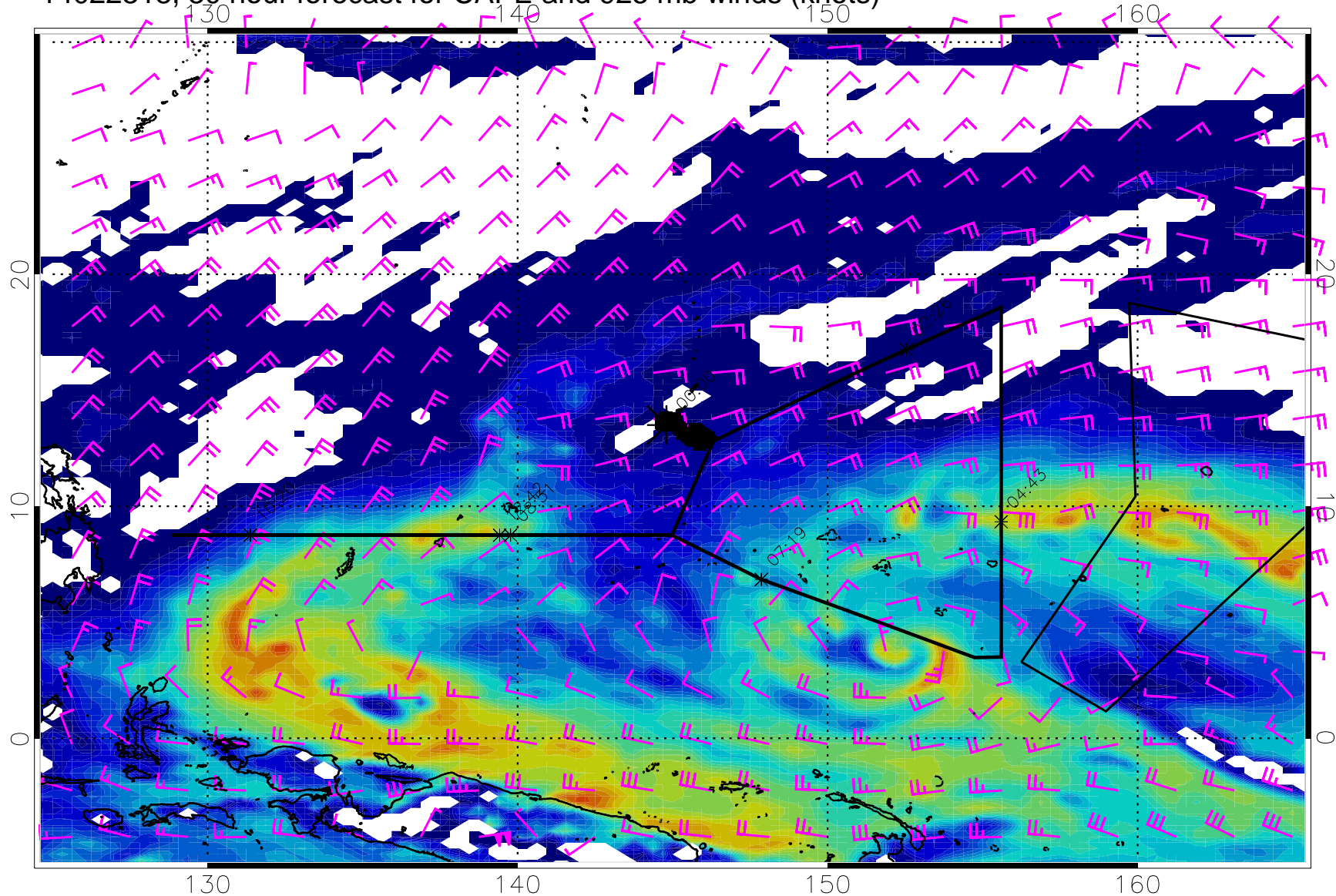
14022318, 30 hour forecast for CAPE and 925 mb winds (knots)
