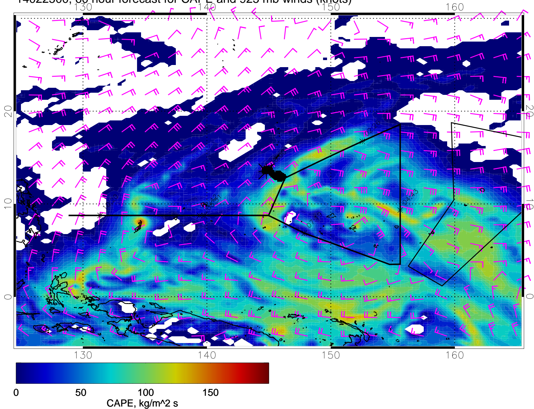
14022500, 60 hour forecast for CAPE and 925 mb winds (knots)
