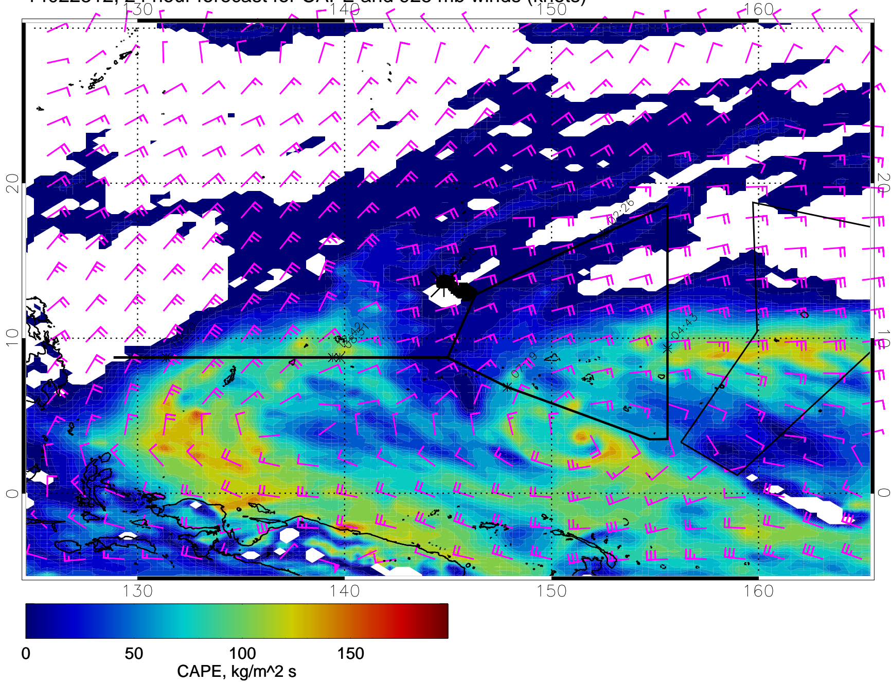
14022312, 24 hour forecast for CAPE and 925 mb winds (knots)
