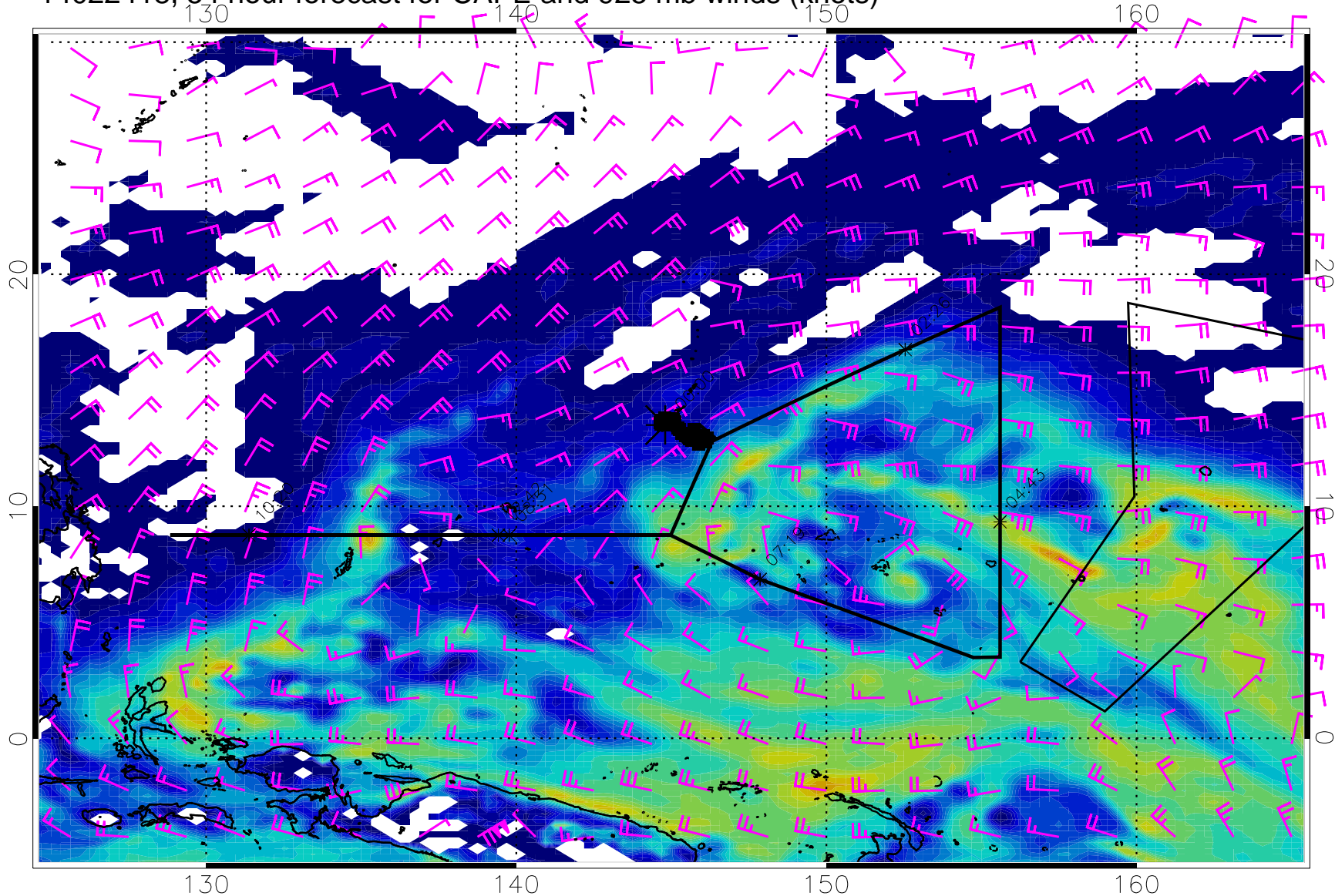
14022418, 54 hour forecast for CAPE and 925 mb winds (knots)
