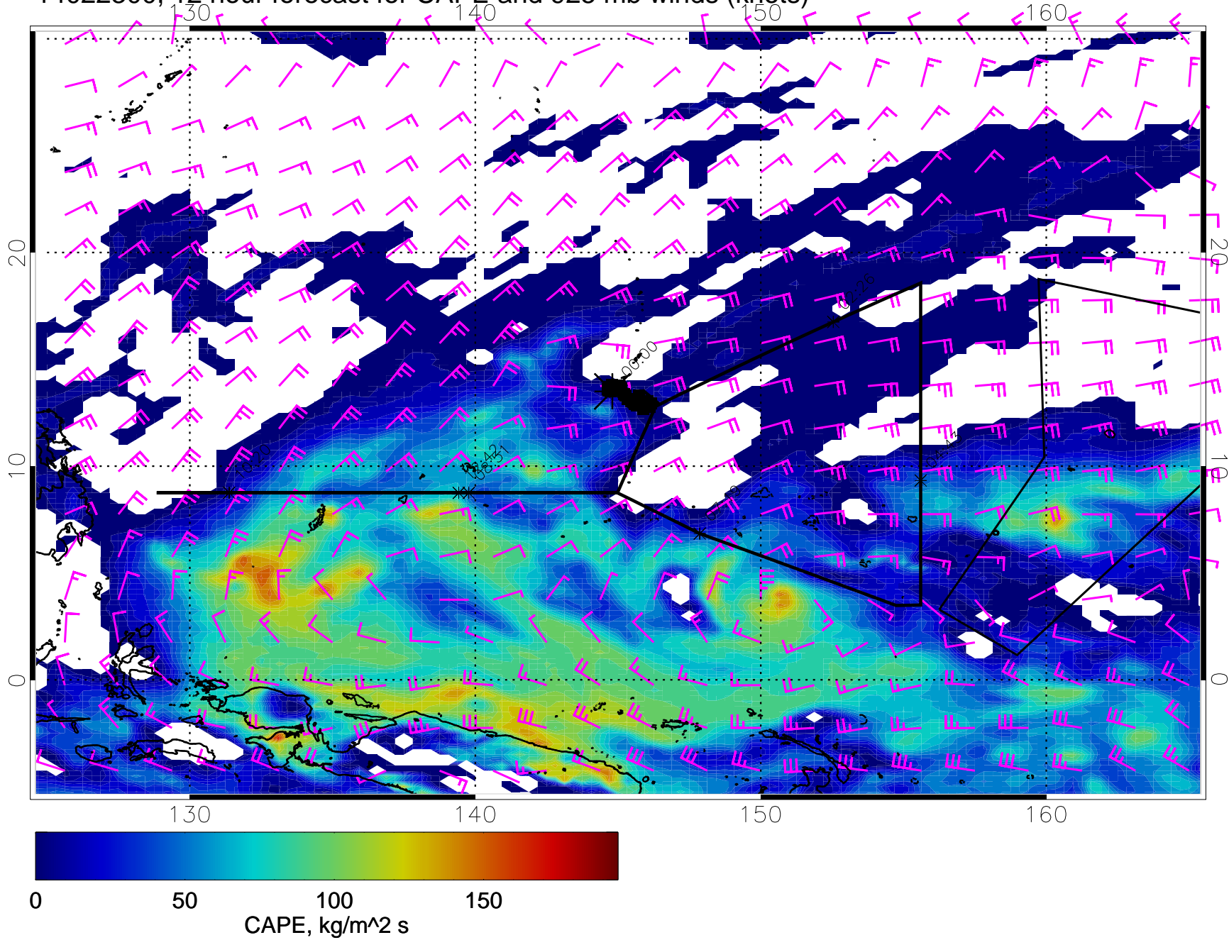
14022300, 12 hour forecast for CAPE and 925 mb winds (knots)
