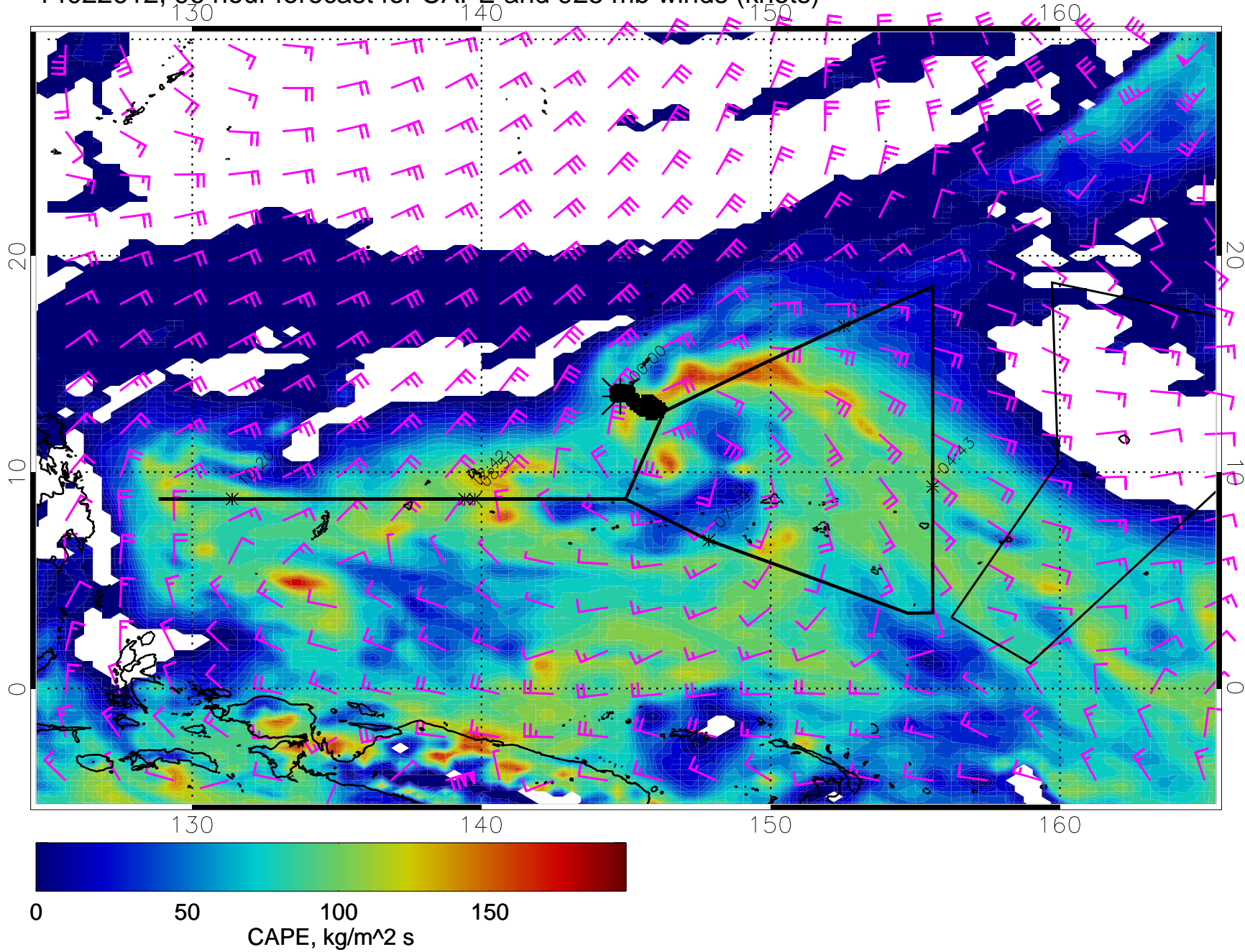
14022612, 96 hour forecast for CAPE and 925 mb winds (knots)
