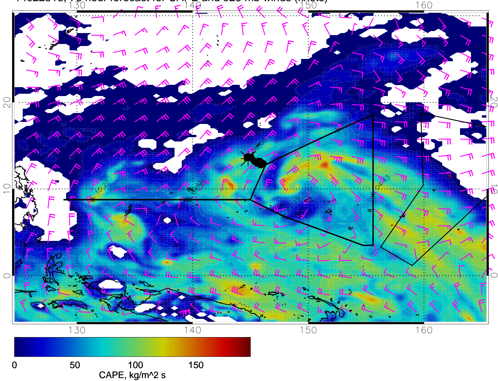
14022518, 78 hour forecast for CAPE and 925 mb winds (knots)
