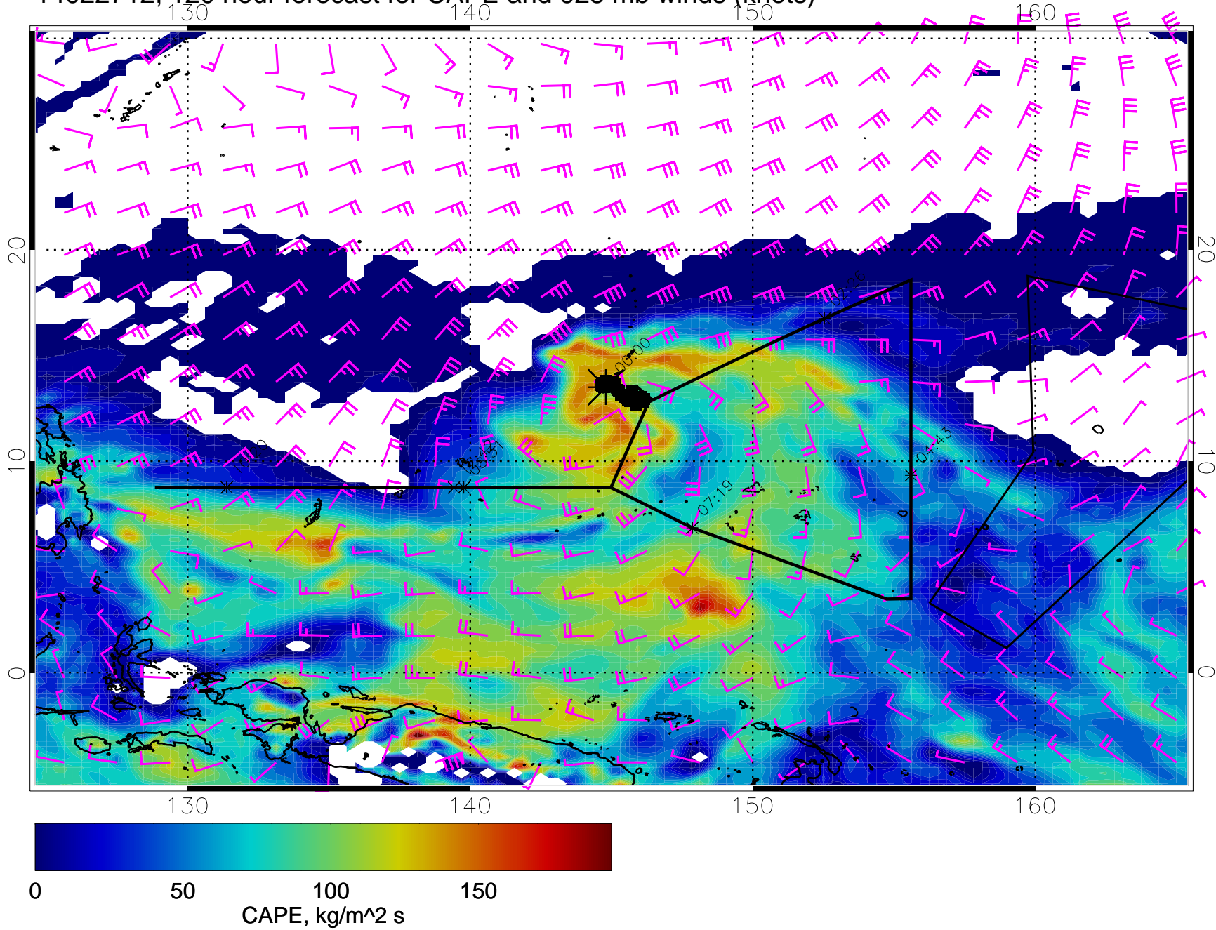
14022712, 120 hour forecast for CAPE and 925 mb winds (knots)
