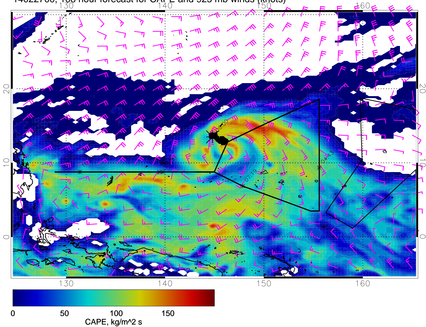
14022700, 108 hour forecast for CAPE and 925 mb winds (knots)
