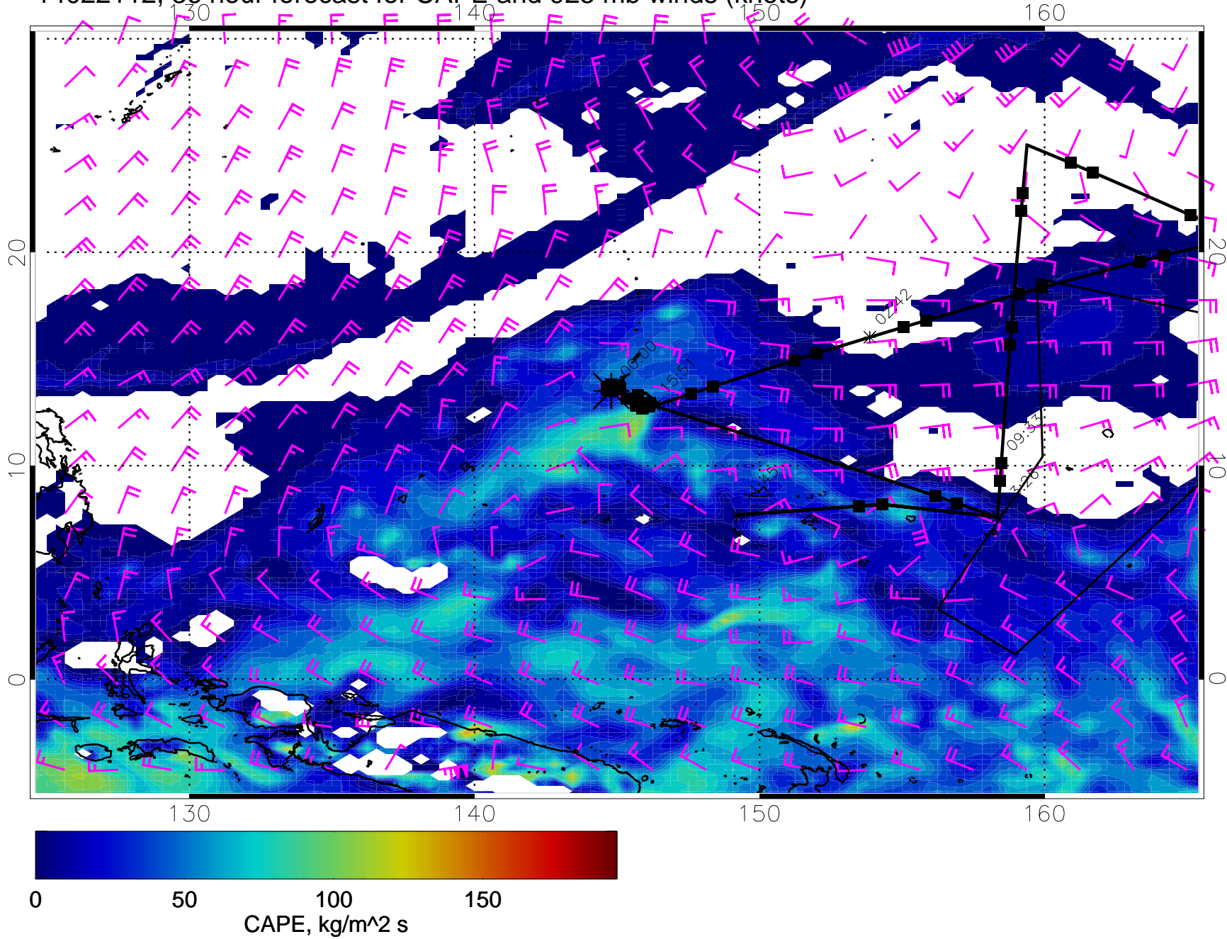
14022112, 36 hour forecast for CAPE and 925 mb winds (knots)
