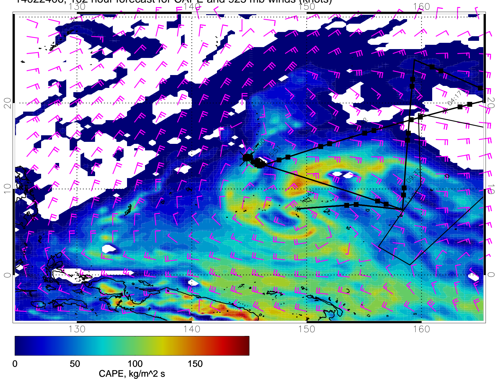
14022406, 102 hour forecast for CAPE and 925 mb winds (knots)
