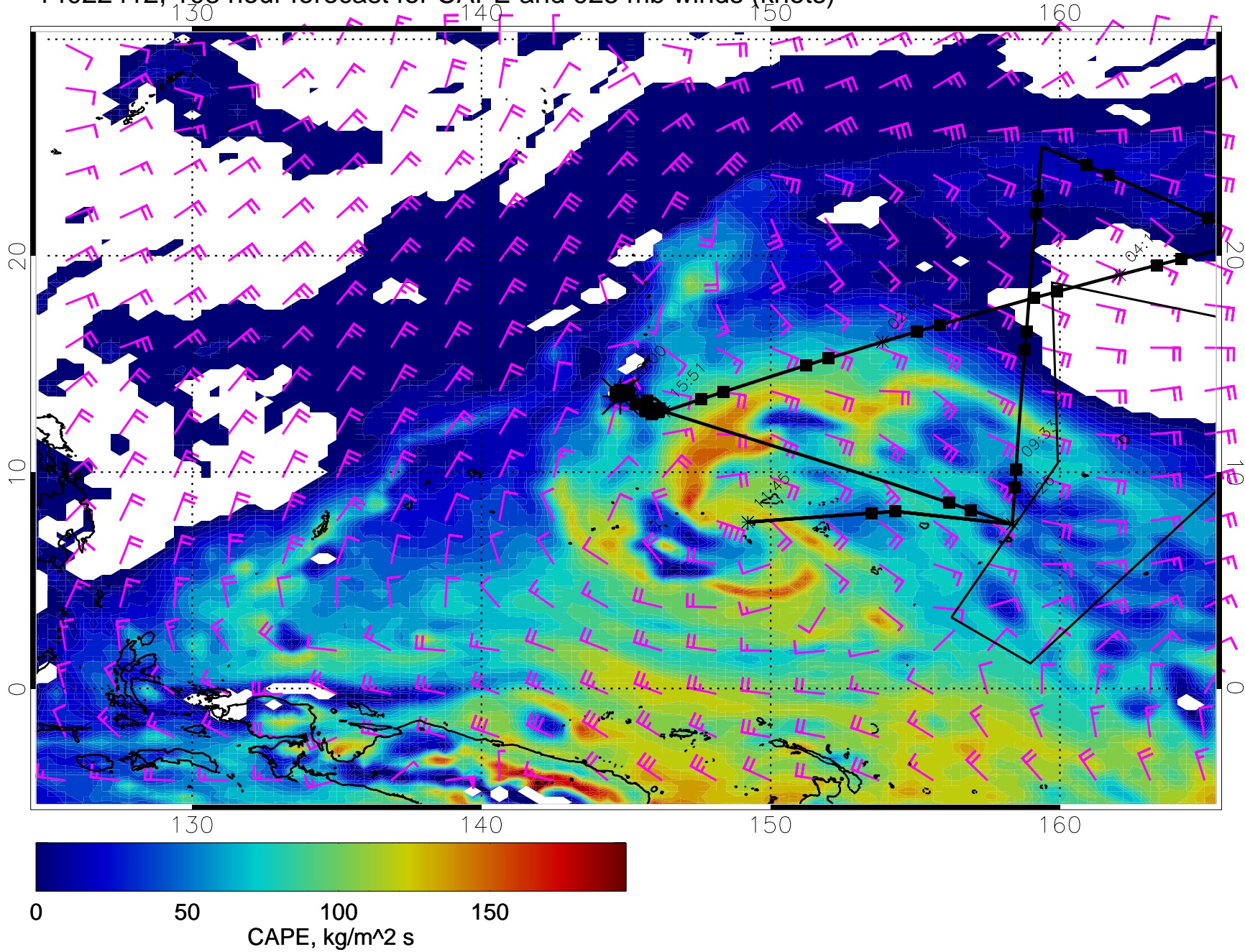
14022412, 108 hour forecast for CAPE and 925 mb winds (knots)
