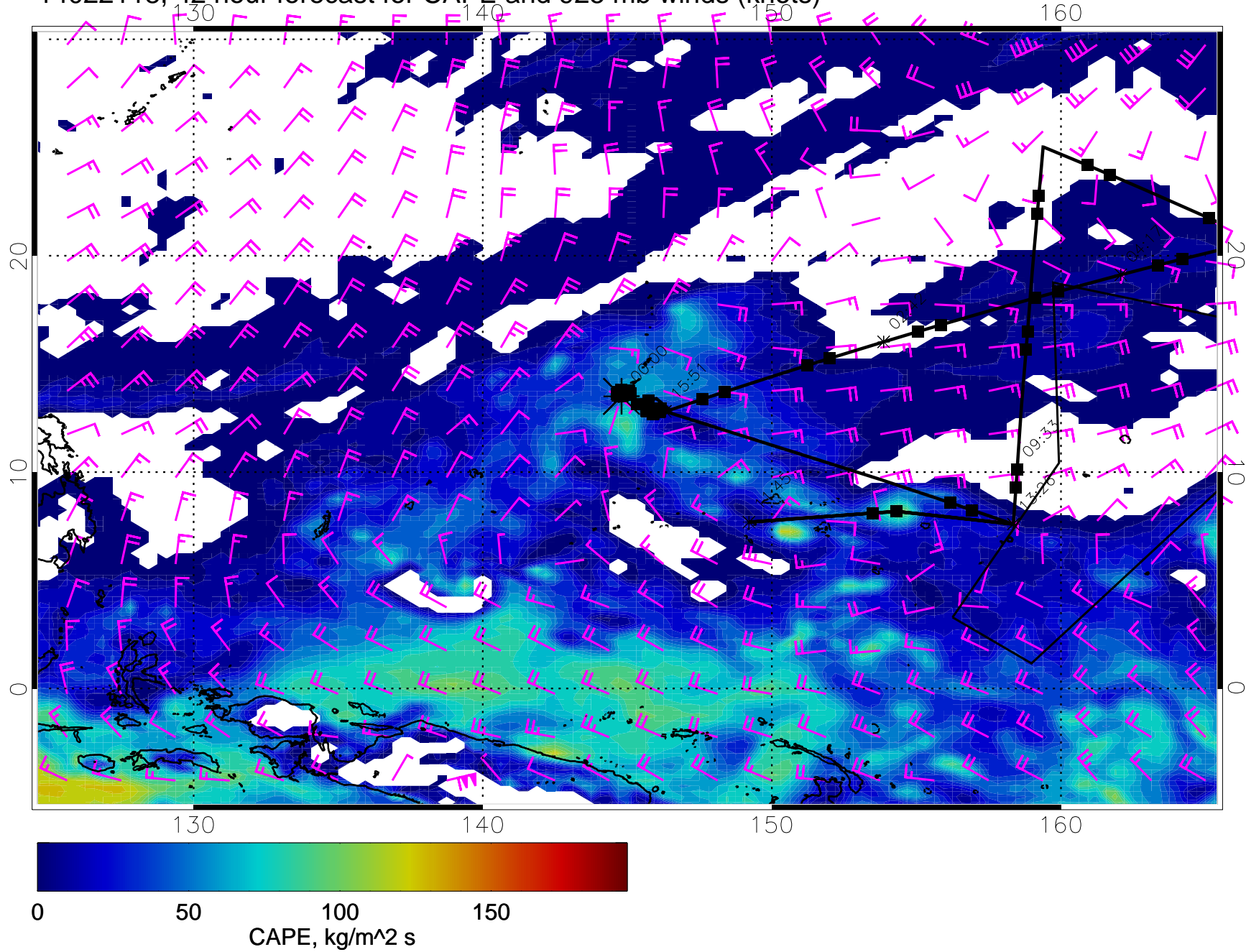
14022118, 42 hour forecast for CAPE and 925 mb winds (knots)
