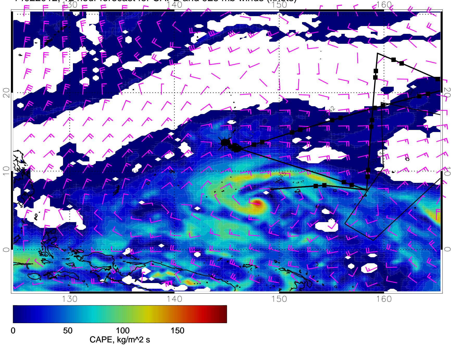
14022012, 12 hour forecast for CAPE and 925 mb winds (knots)
