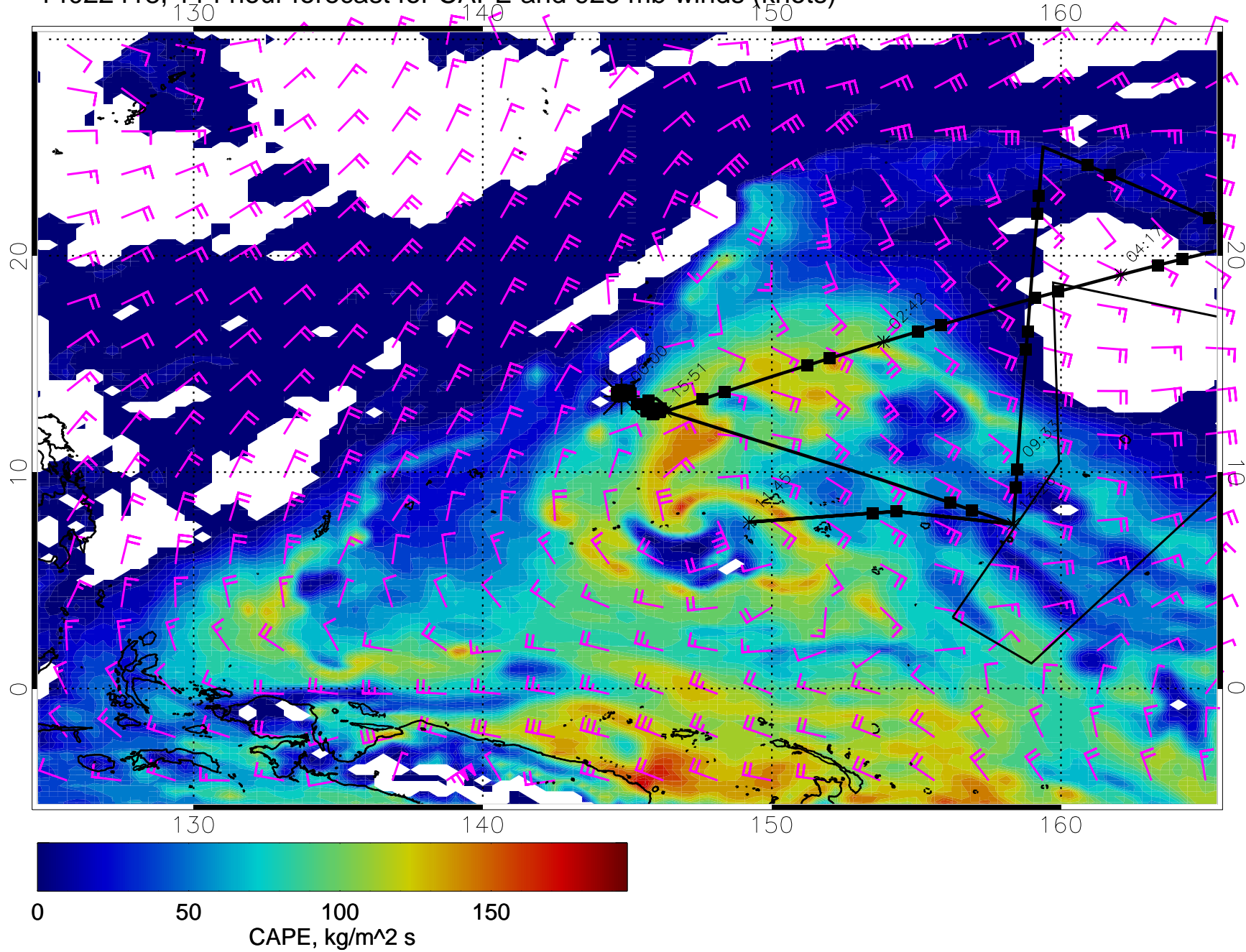
14022418, 114 hour forecast for CAPE and 925 mb winds (knots)
