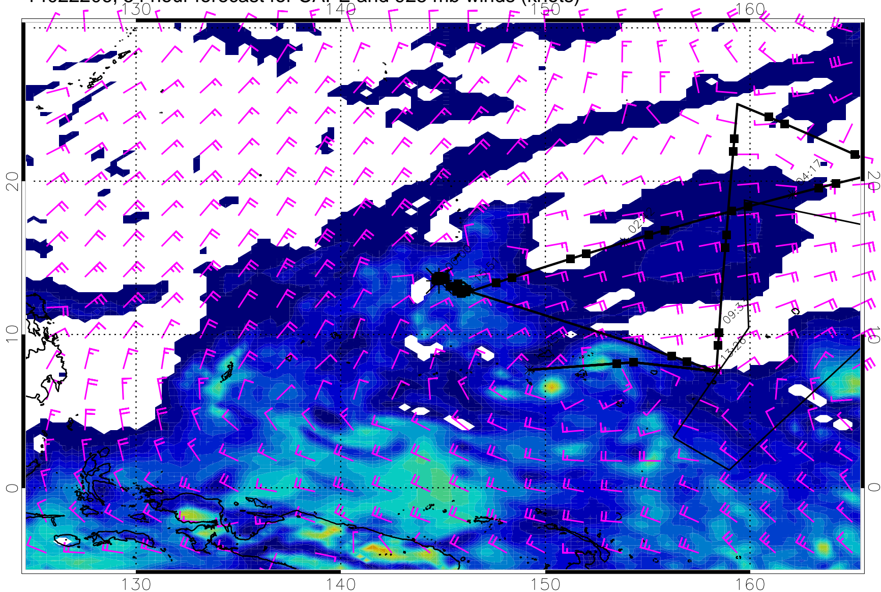
14022206, 54 hour forecast for CAPE and 925 mb winds (knots)
