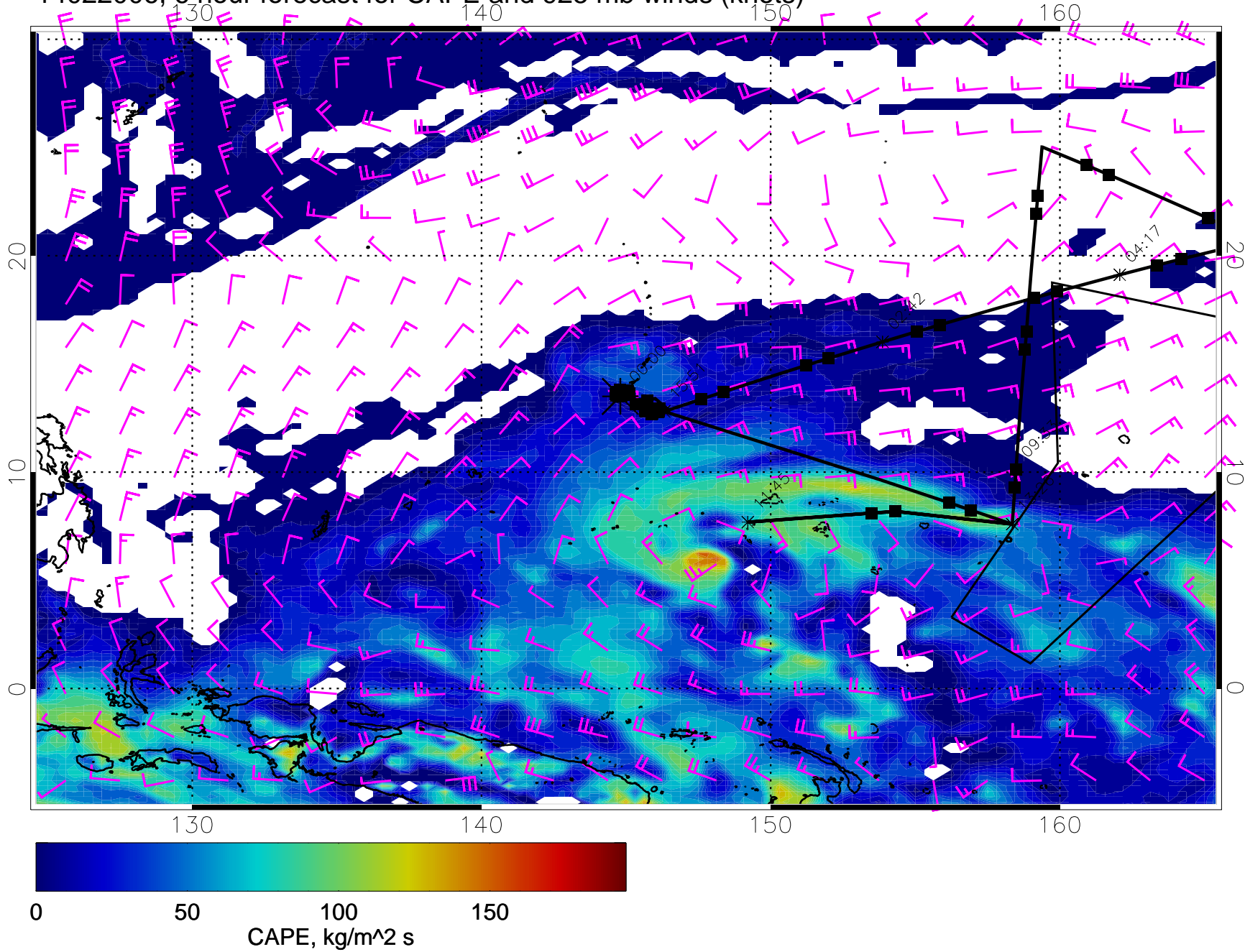
14022006, 6 hour forecast for CAPE and 925 mb winds (knots)
