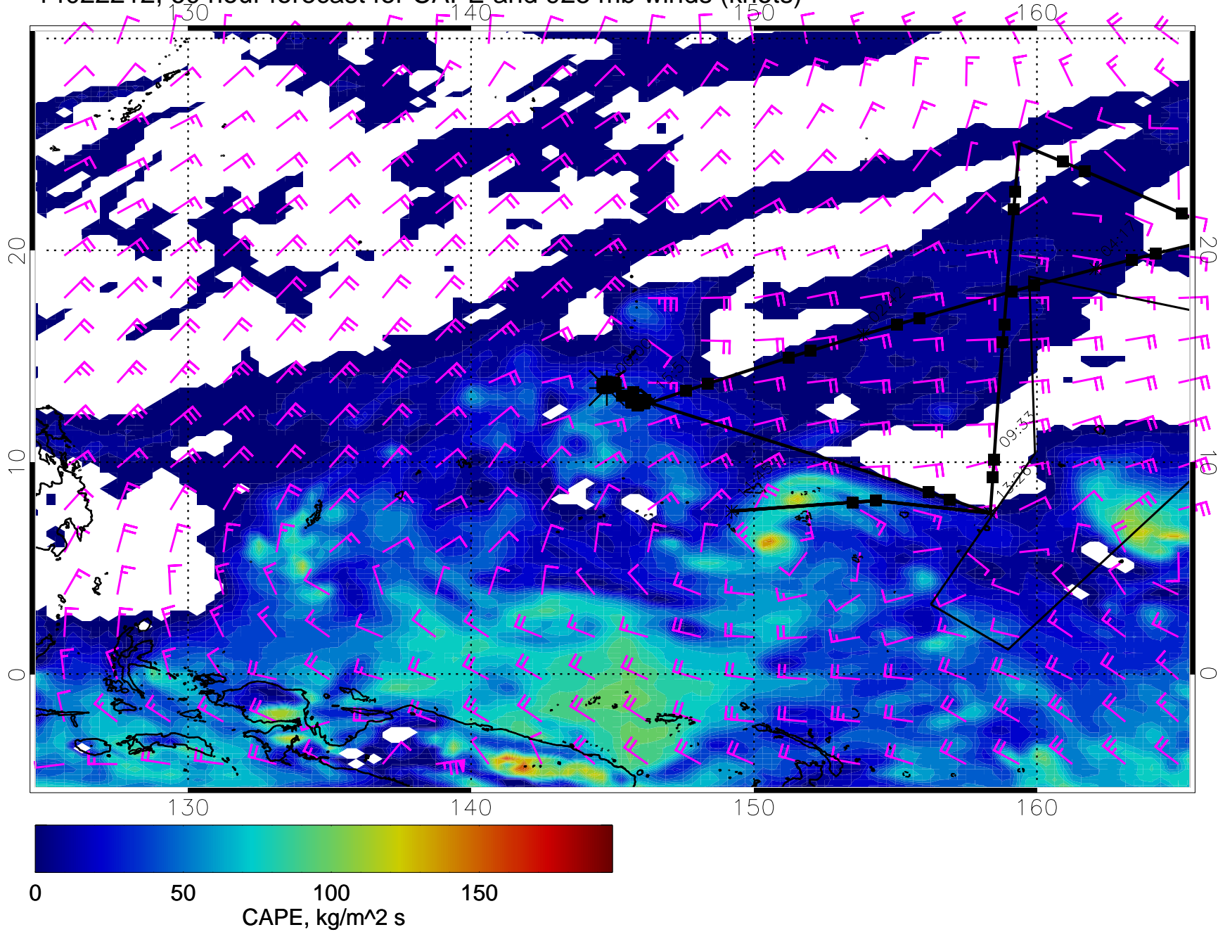
14022212, 60 hour forecast for CAPE and 925 mb winds (knots)
