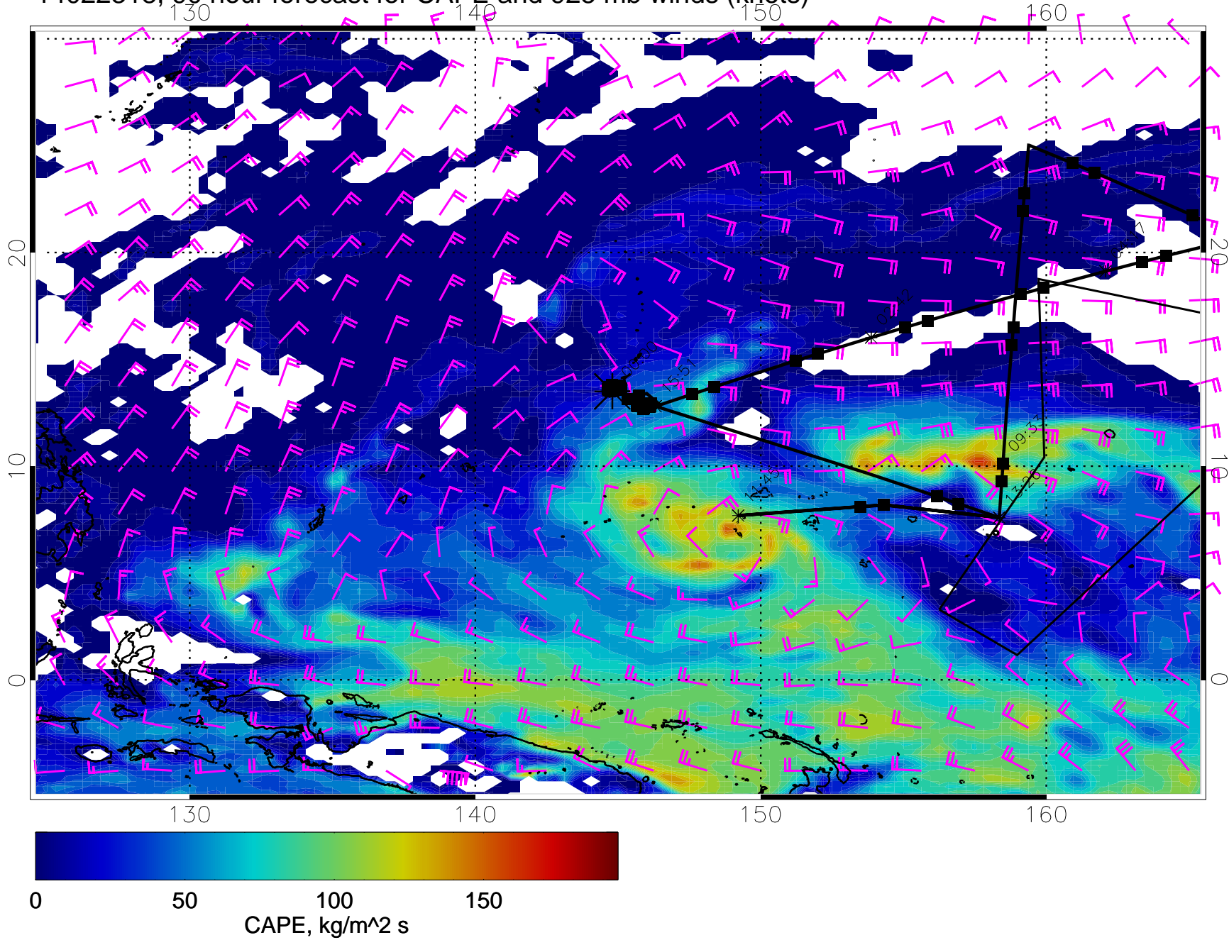
14022318, 90 hour forecast for CAPE and 925 mb winds (knots)
