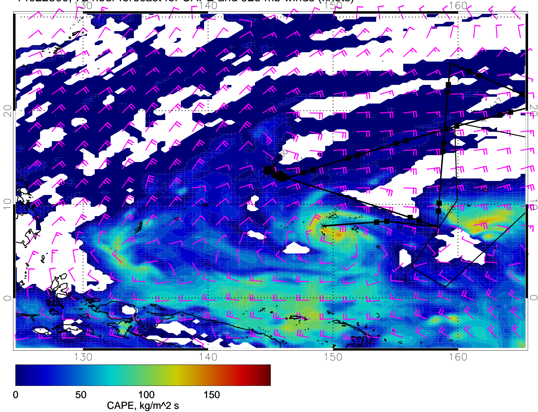
14022300, 72 hour forecast for CAPE and 925 mb winds (knots)
