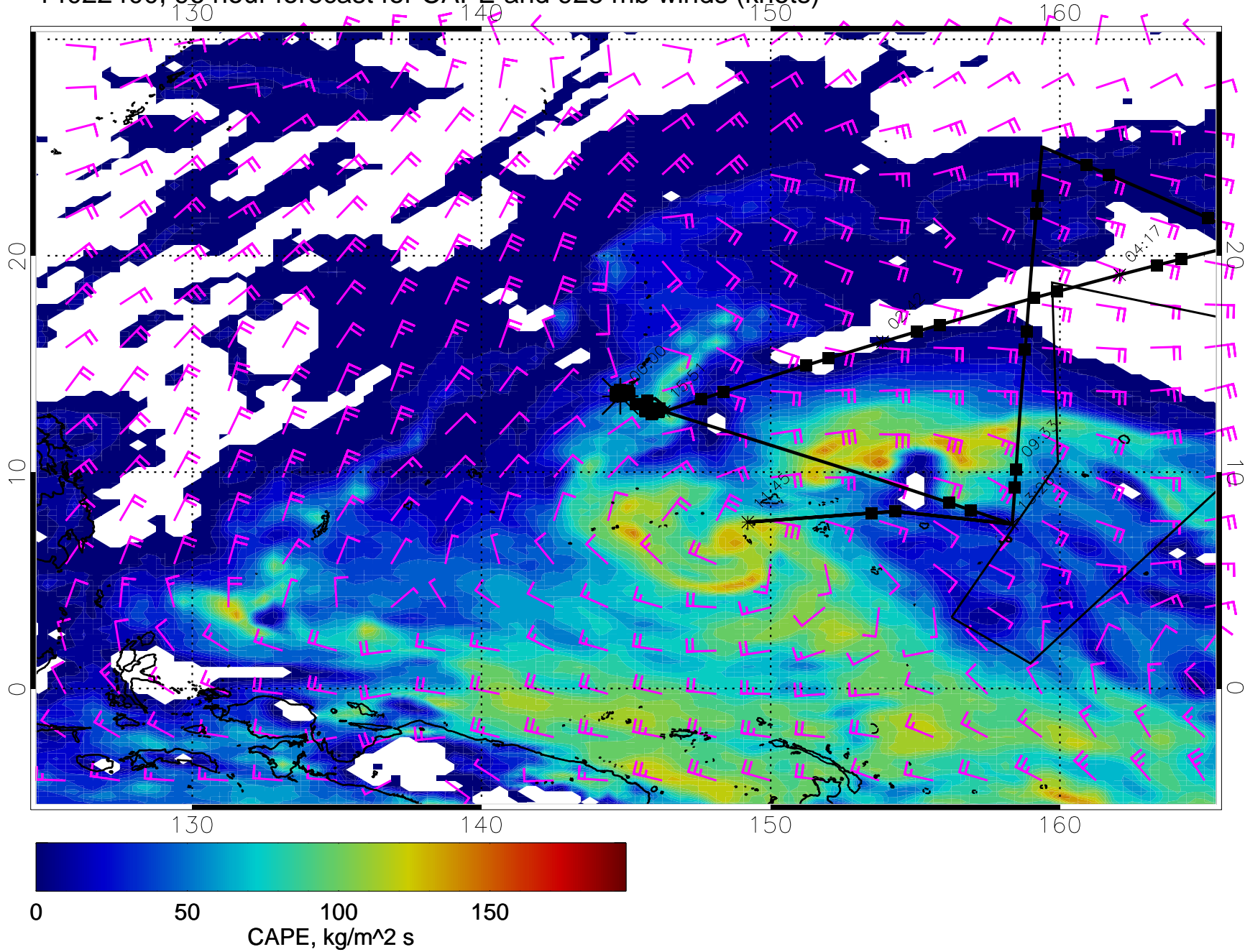
14022400, 96 hour forecast for CAPE and 925 mb winds (knots)
