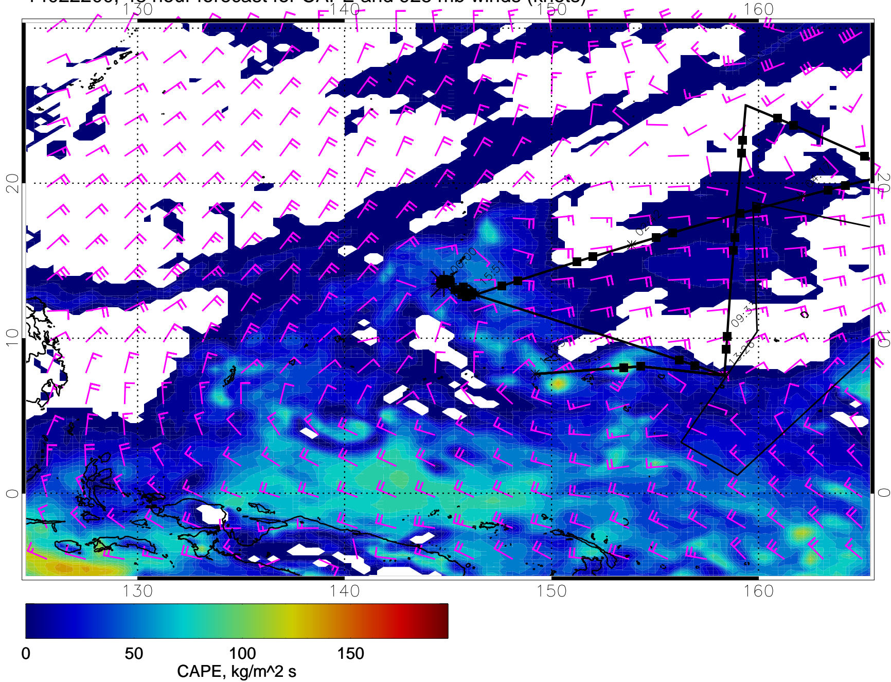
14022200, 48 hour forecast for CAPE and 925 mb winds (knots)
