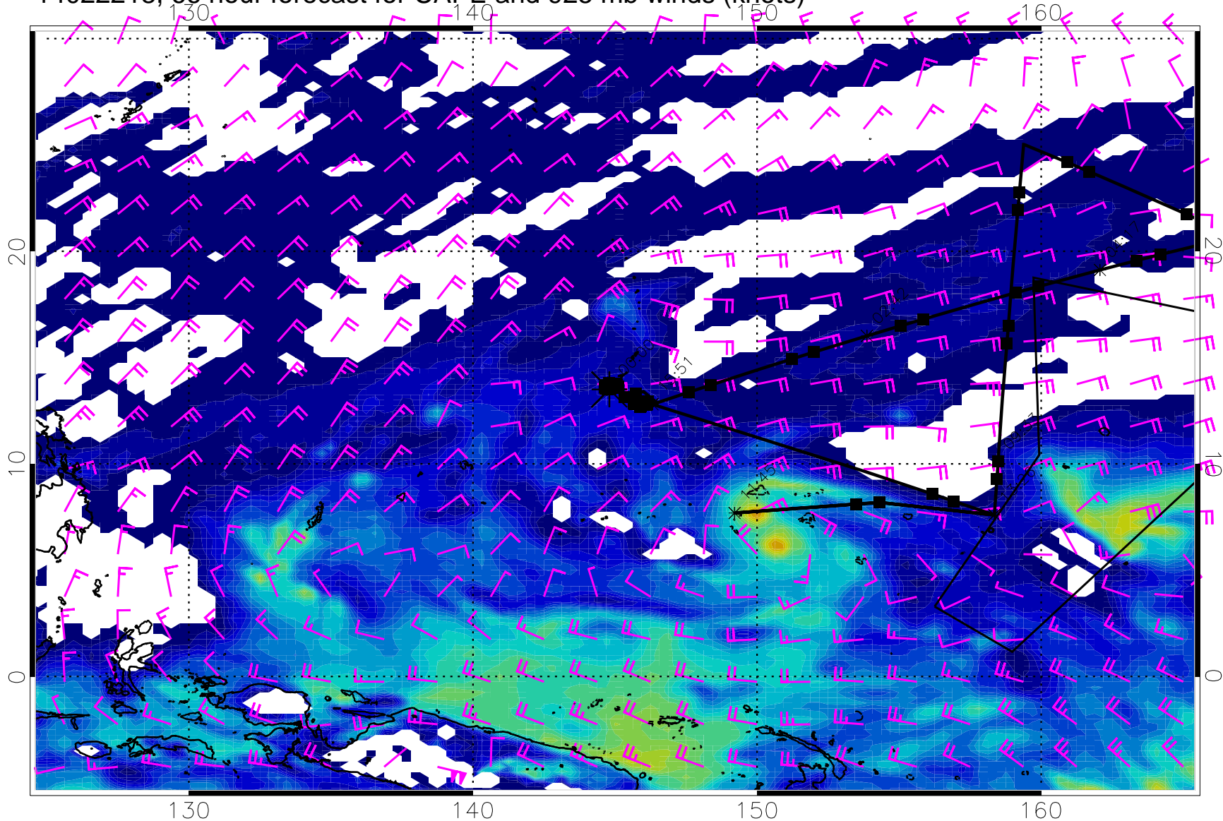
14022218, 66 hour forecast for CAPE and 925 mb winds (knots)
