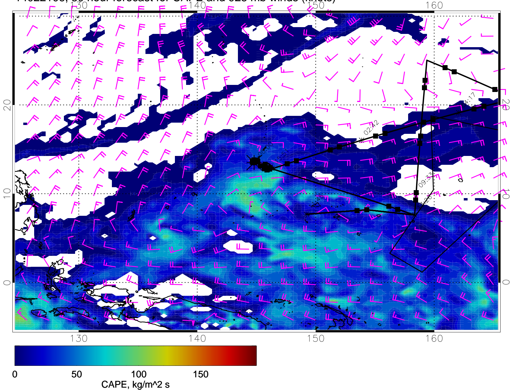
14022106, 30 hour forecast for CAPE and 925 mb winds (knots)
