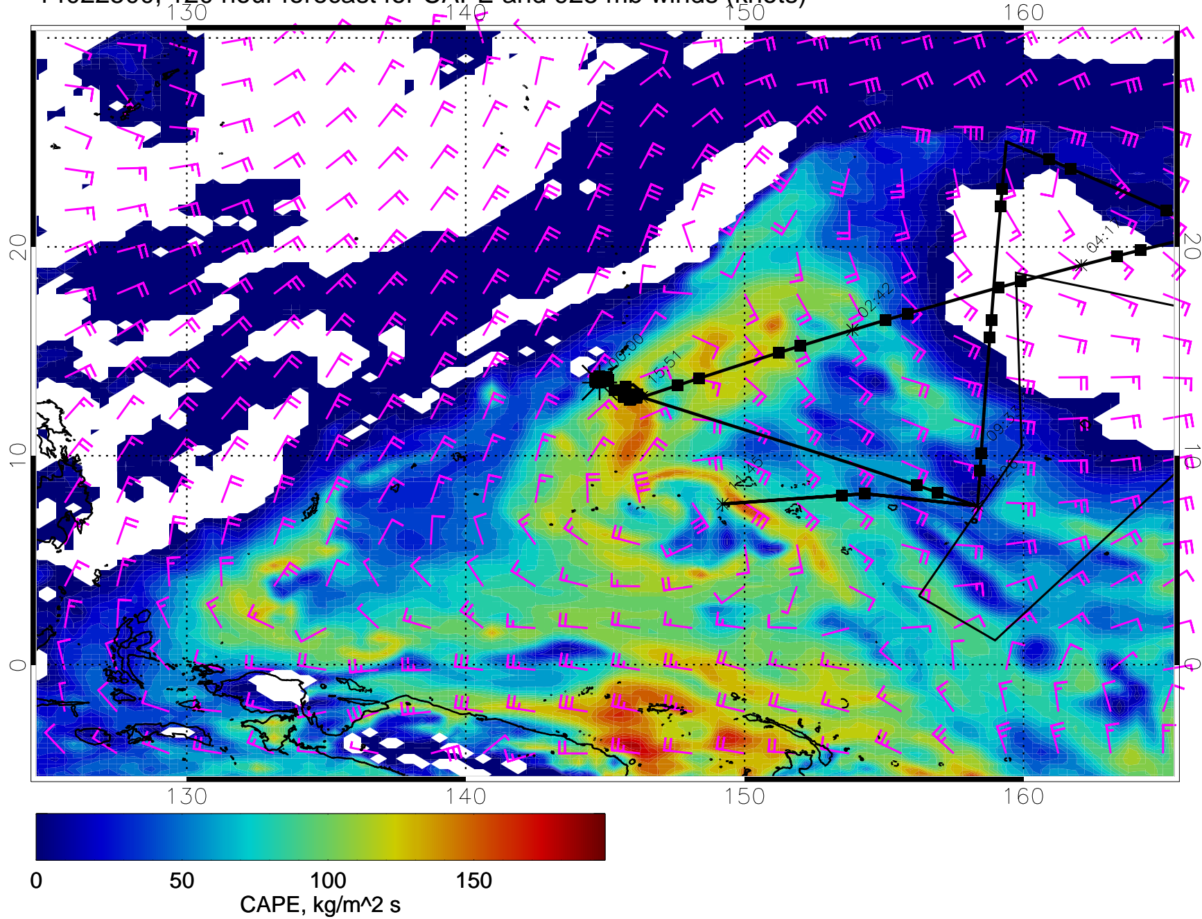
14022500, 120 hour forecast for CAPE and 925 mb winds (knots)
