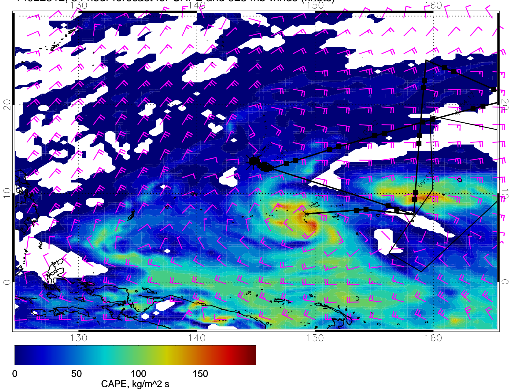
14022312, 84 hour forecast for CAPE and 925 mb winds (knots)
