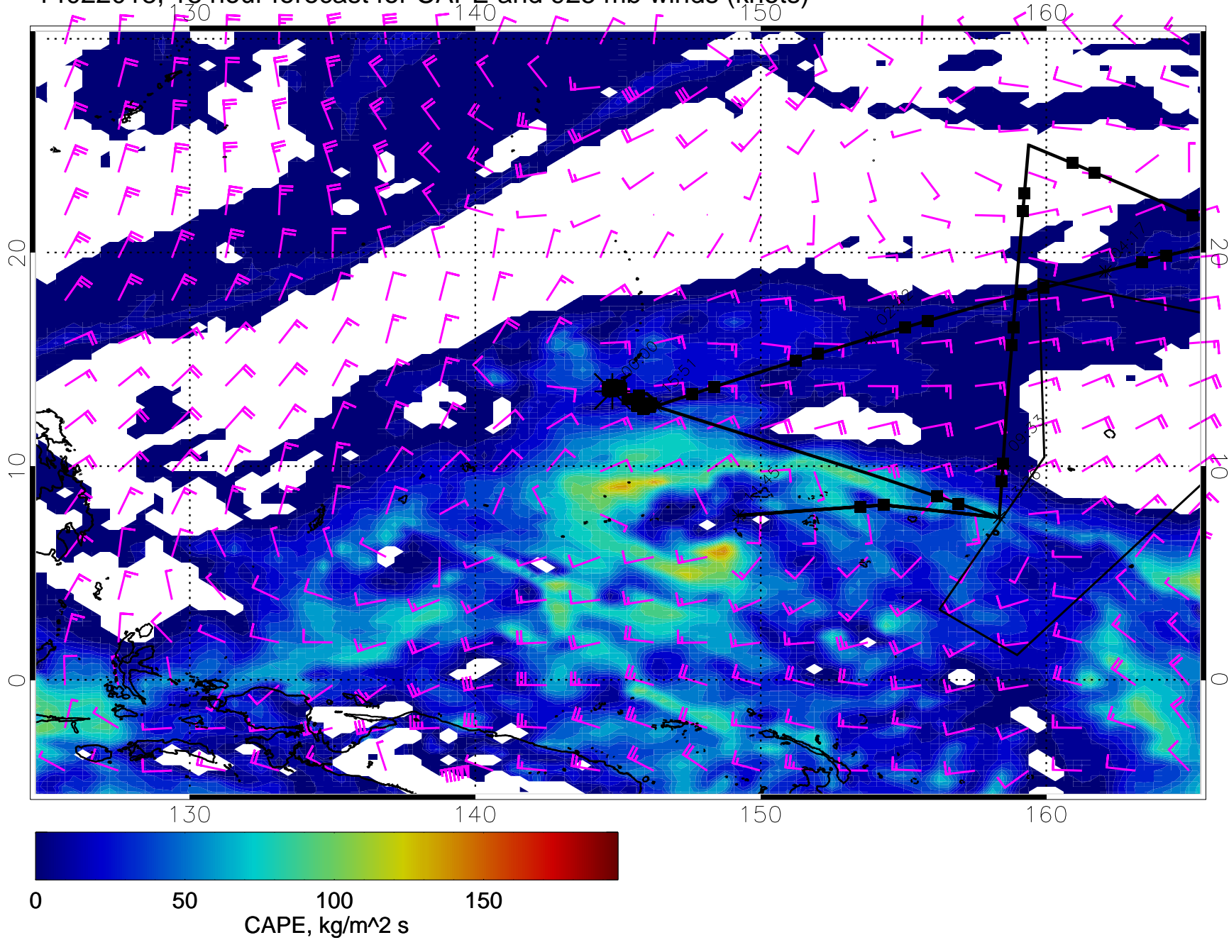
14022018, 18 hour forecast for CAPE and 925 mb winds (knots)
