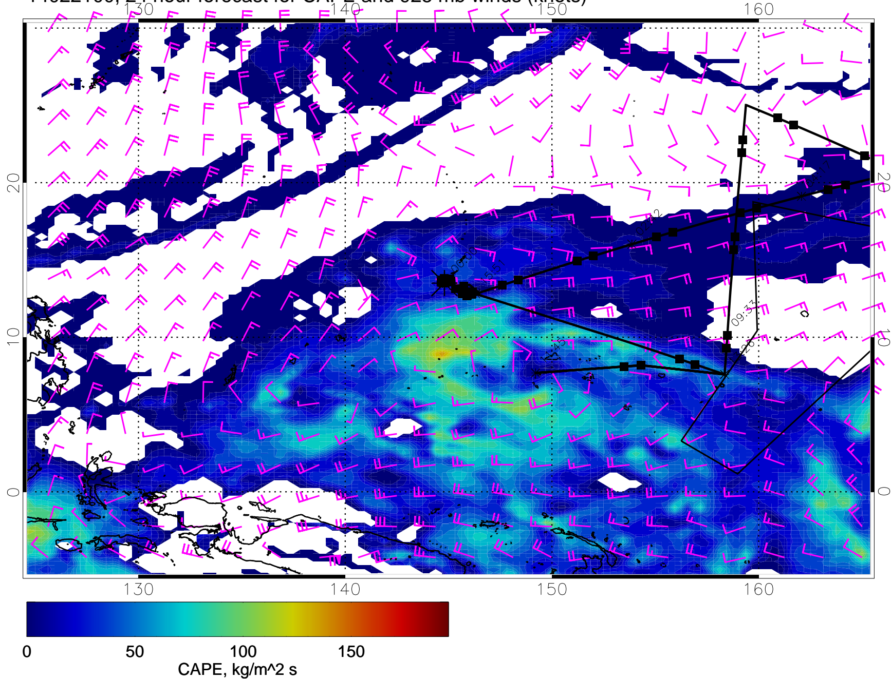
14022100, 24 hour forecast for CAPE and 925 mb winds (knots)
