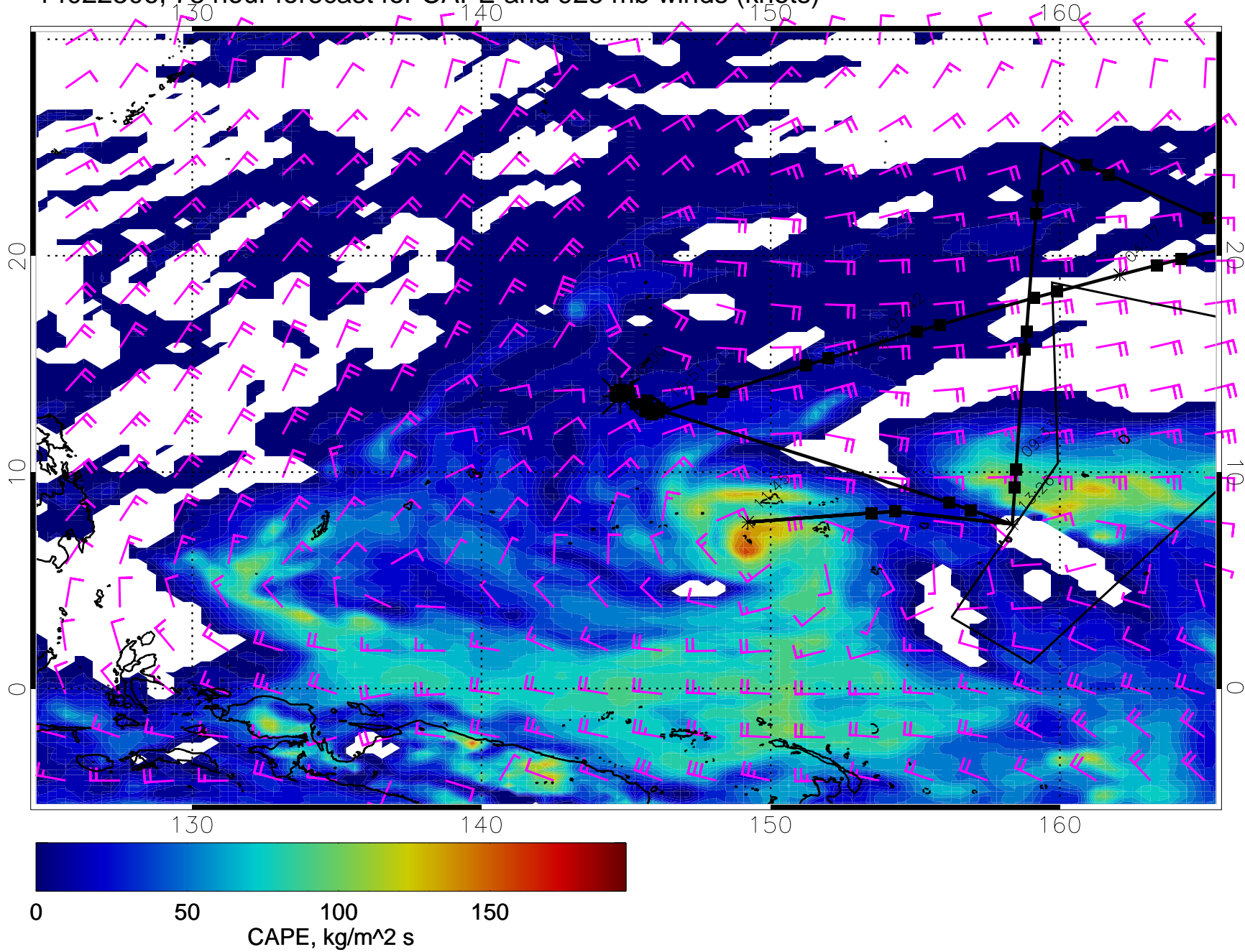
14022306, 78 hour forecast for CAPE and 925 mb winds (knots)
