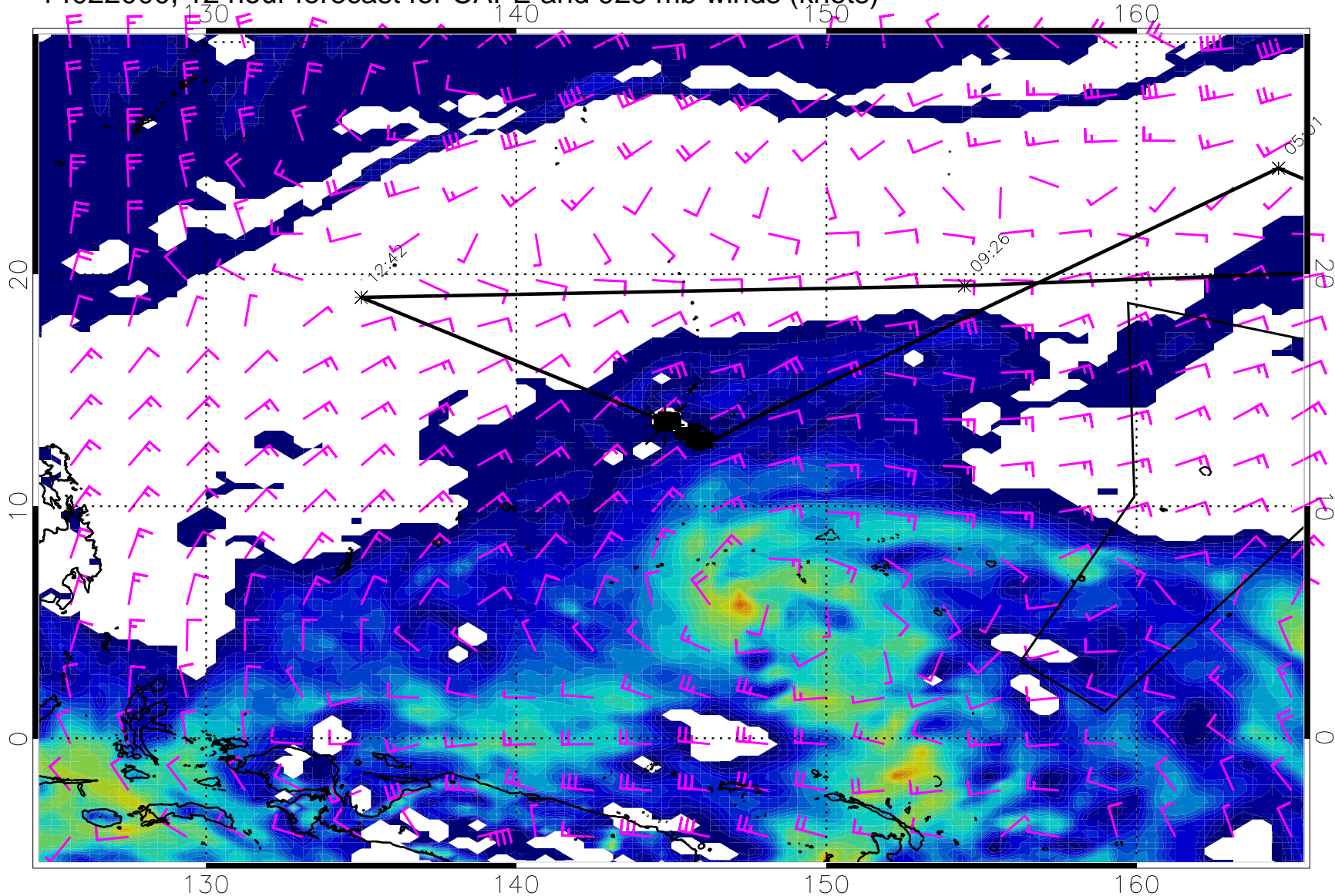
14022000, 12 hour forecast for CAPE and 925 mb winds (knots)
