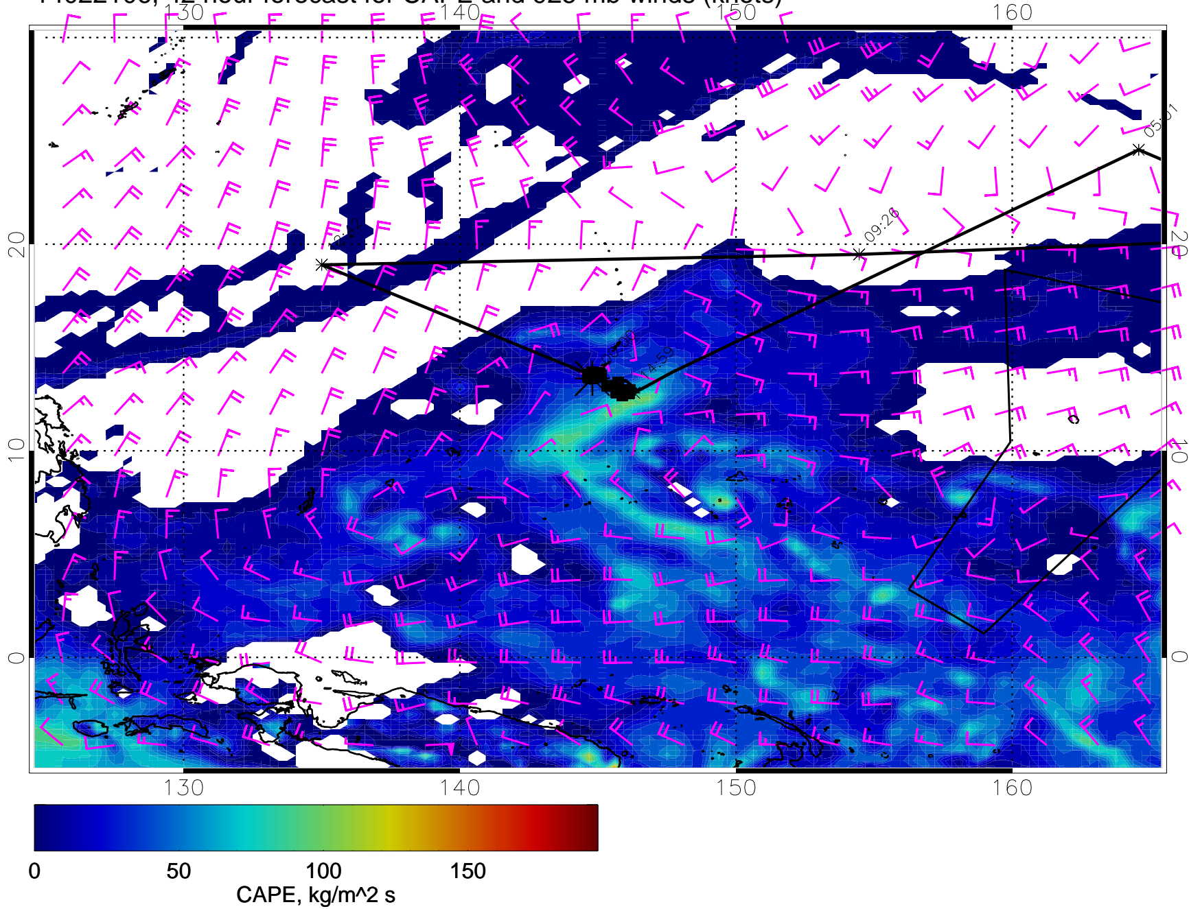
14022106, 42 hour forecast for CAPE and 925 mb winds (knots)
