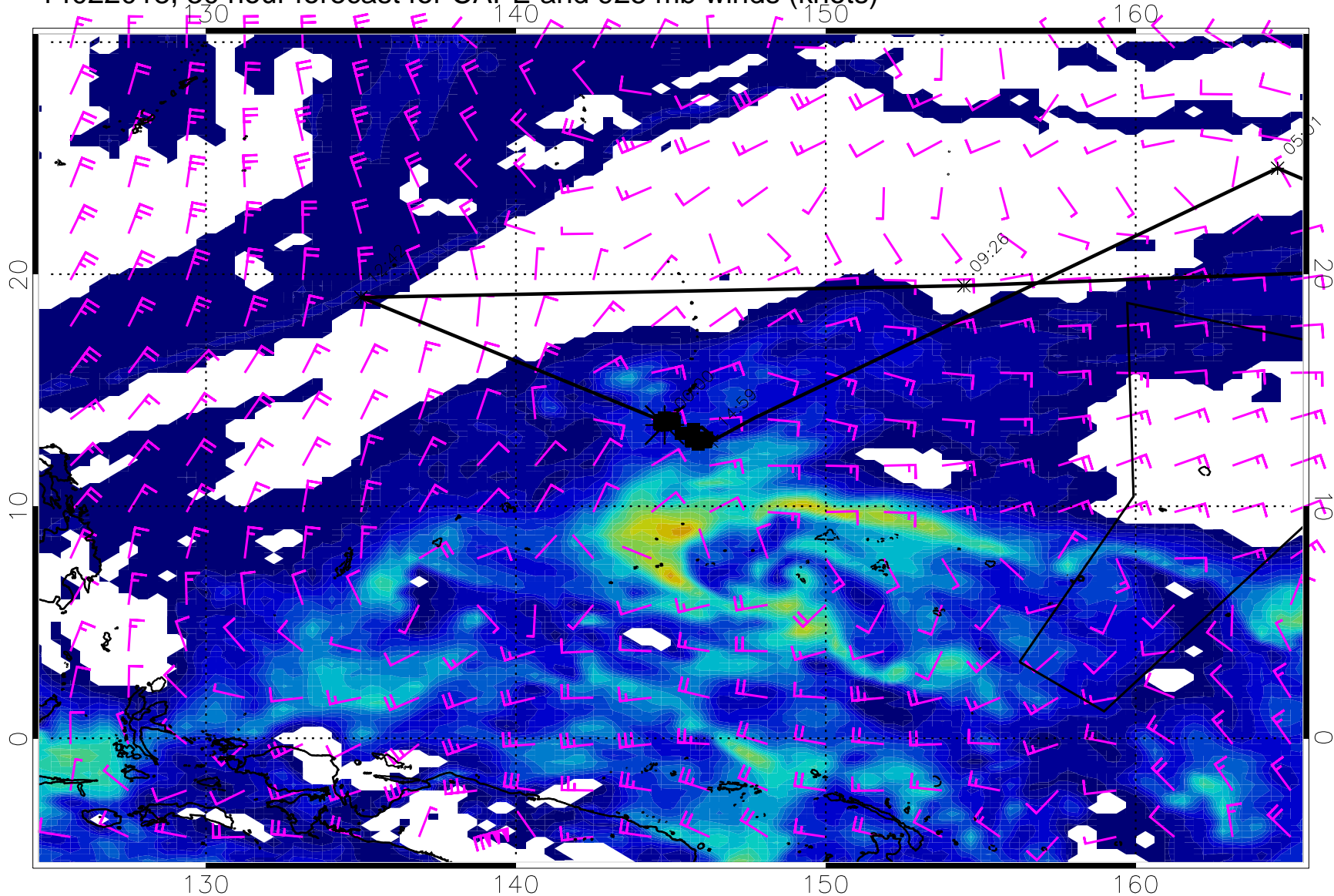
14022018, 30 hour forecast for CAPE and 925 mb winds (knots)
