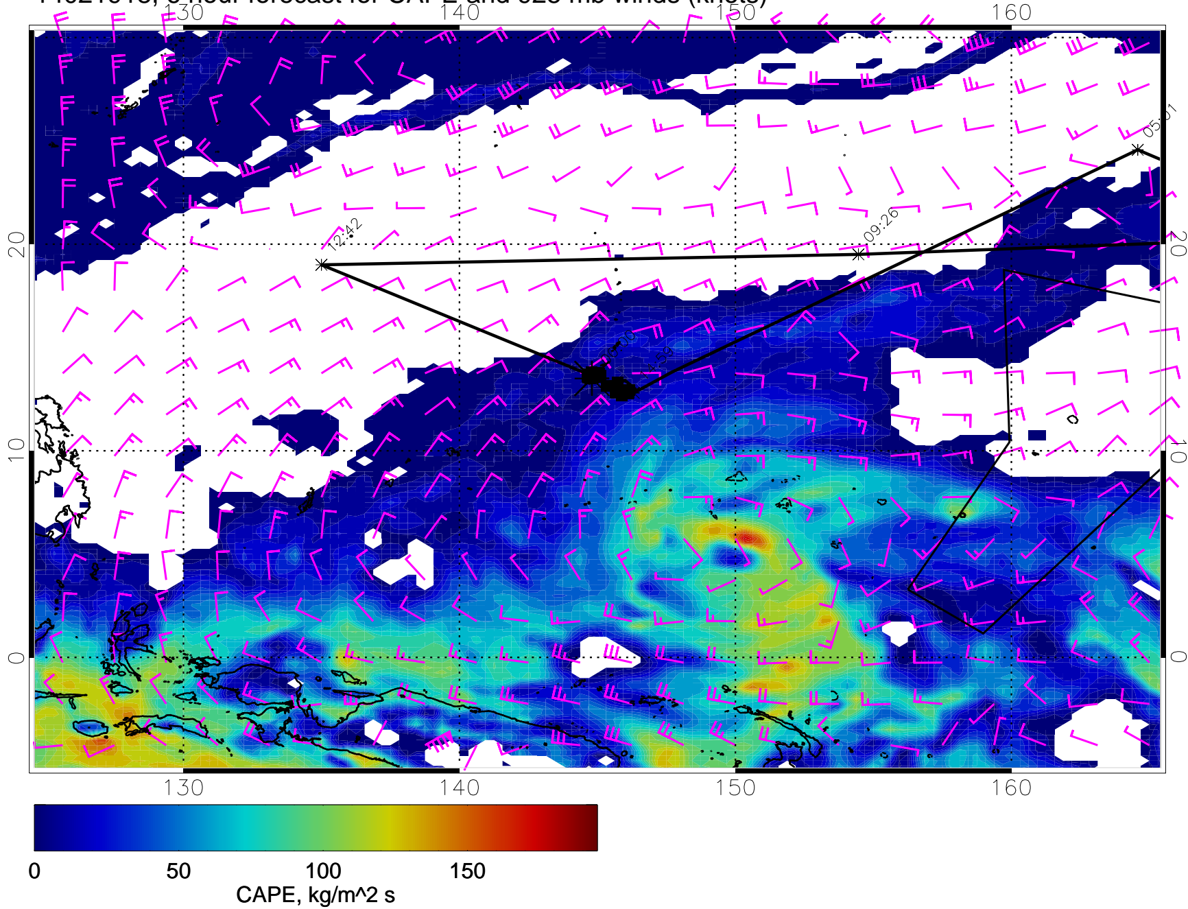
14021918, 6 hour forecast for CAPE and 925 mb winds (knots)
