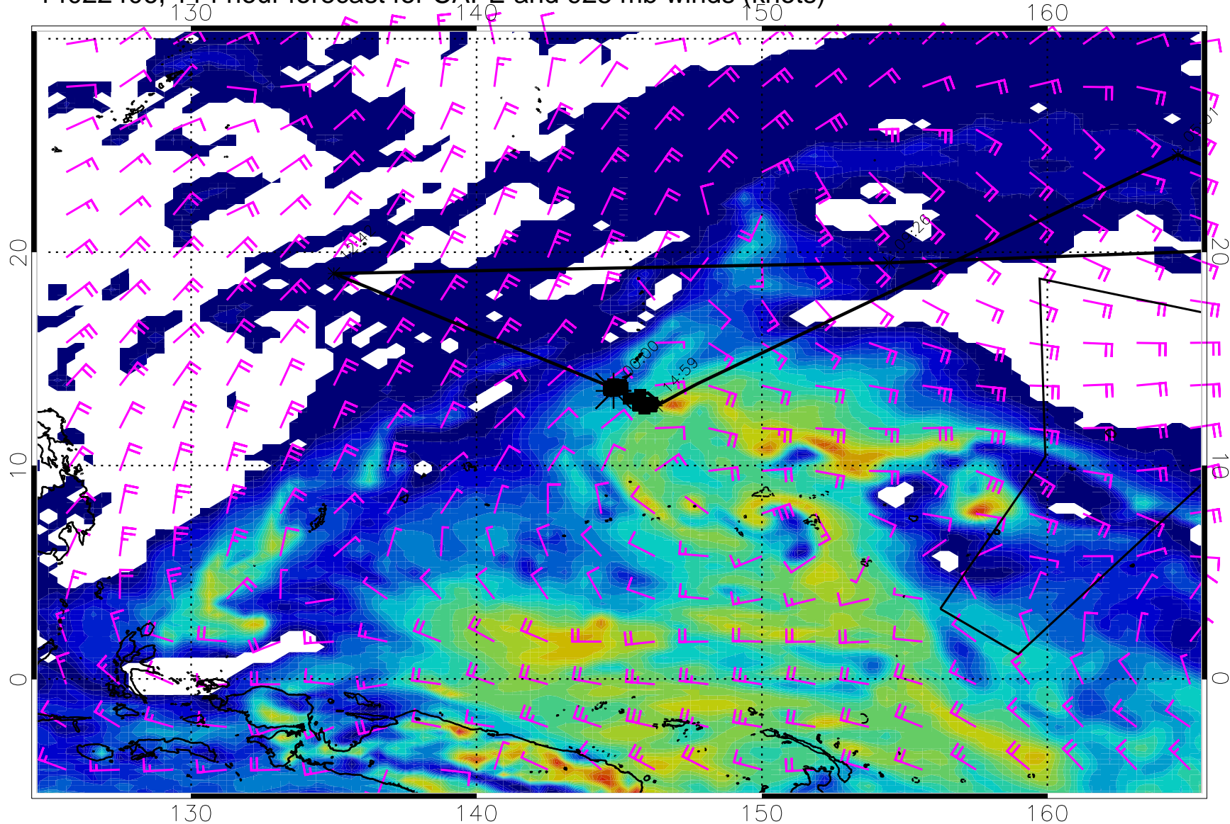
14022406, 114 hour forecast for CAPE and 925 mb winds (knots)
