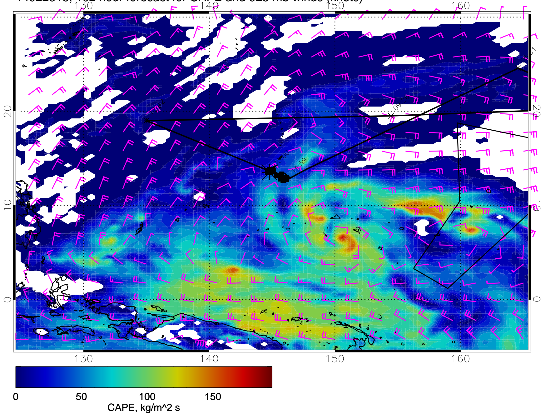
14022318, 102 hour forecast for CAPE and 925 mb winds (knots)
