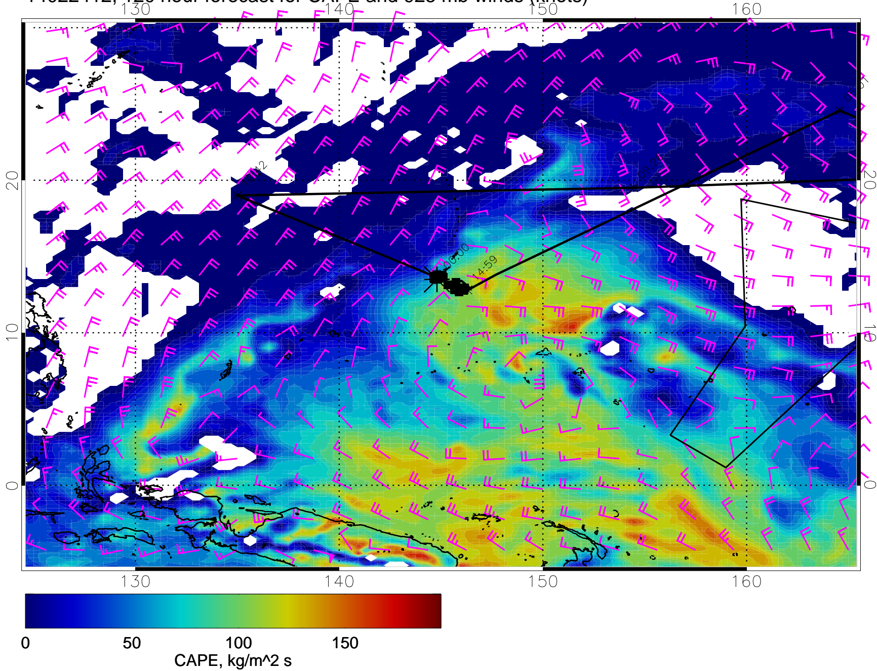
14022412, 120 hour forecast for CAPE and 925 mb winds (knots)
