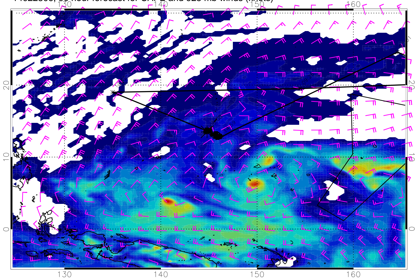
14022306, 90 hour forecast for CAPE and 925 mb winds (knots)
