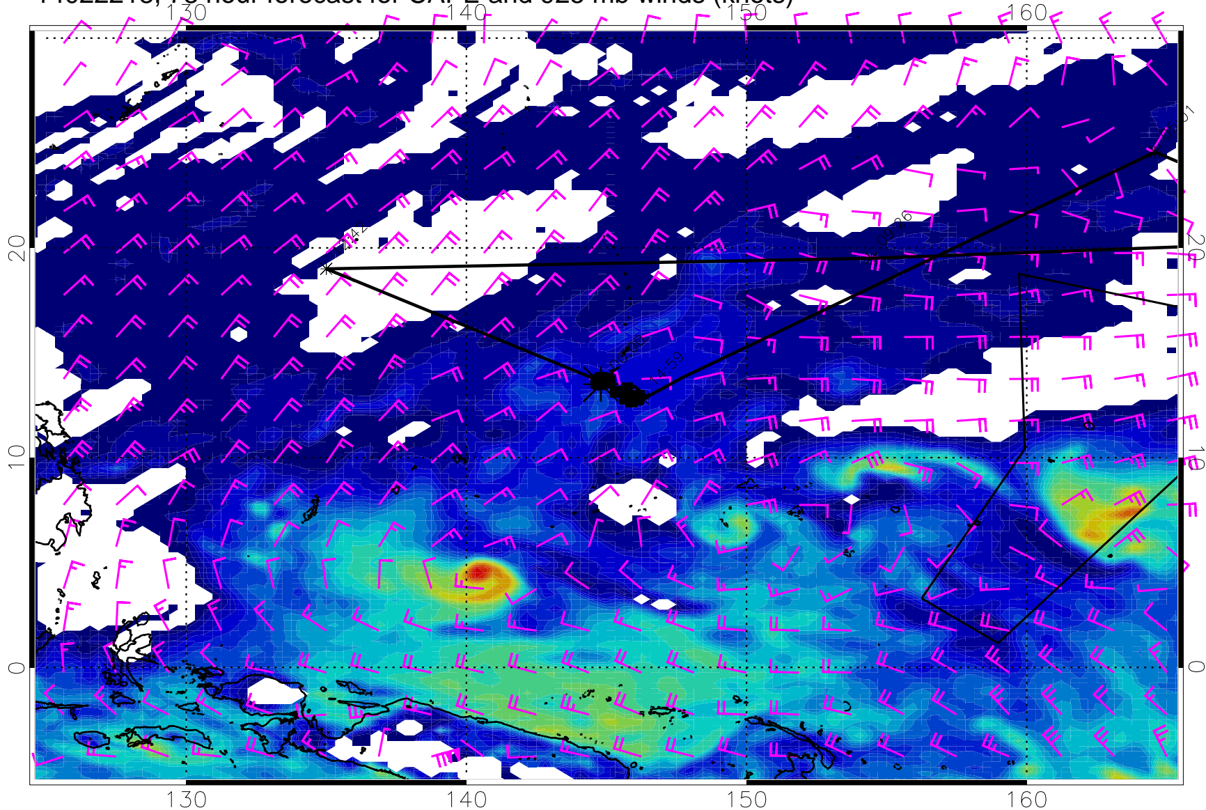
14022218, 78 hour forecast for CAPE and 925 mb winds (knots)
