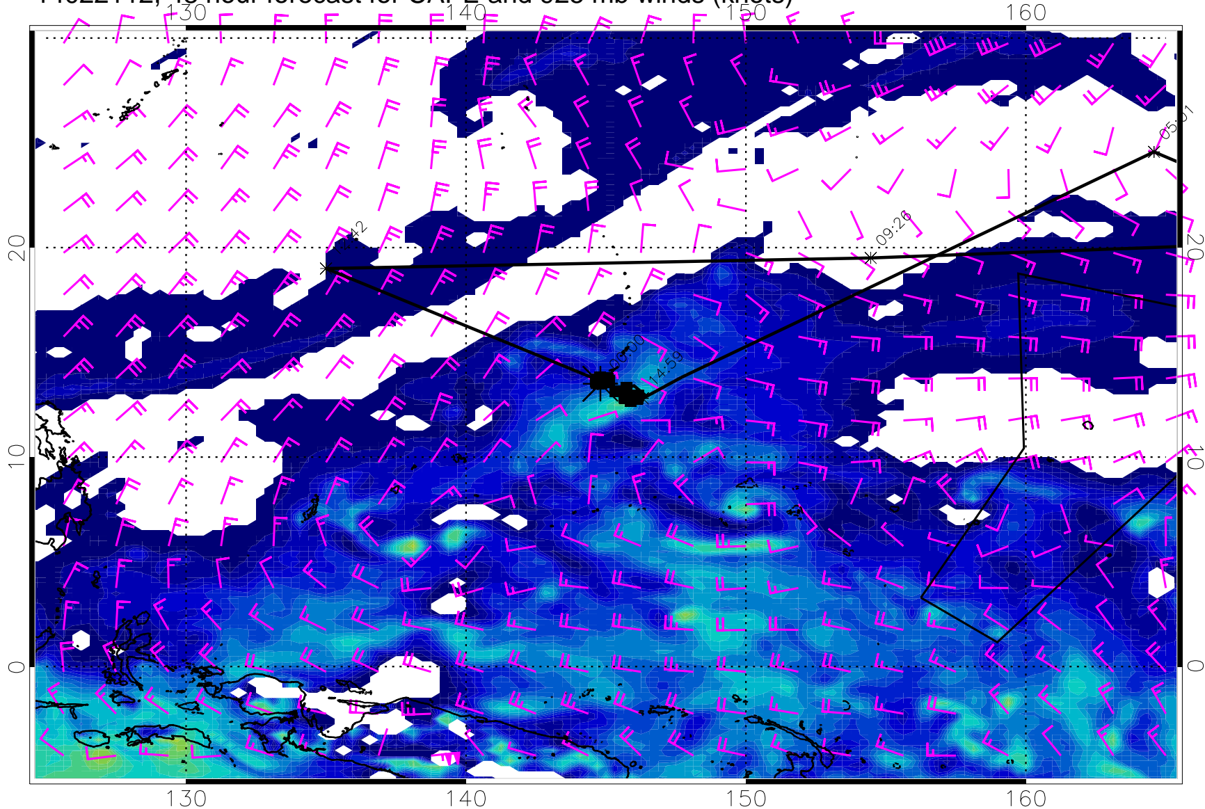
14022112, 48 hour forecast for CAPE and 925 mb winds (knots)
