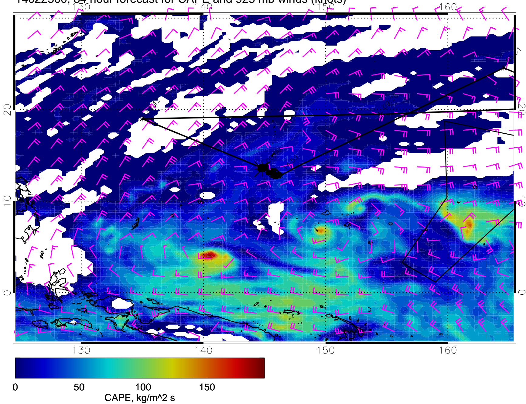
14022300, 84 hour forecast for CAPE and 925 mb winds (knots)
