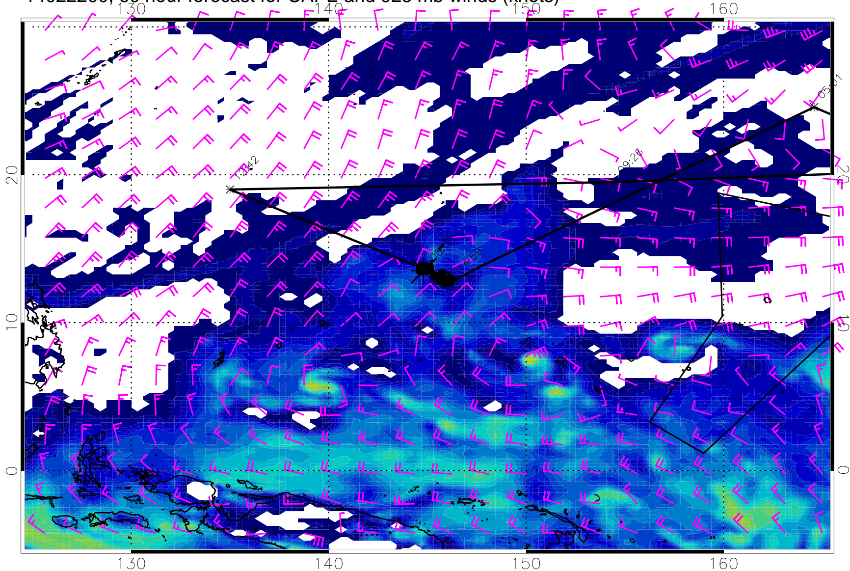
14022200, 60 hour forecast for CAPE and 925 mb winds (knots)
