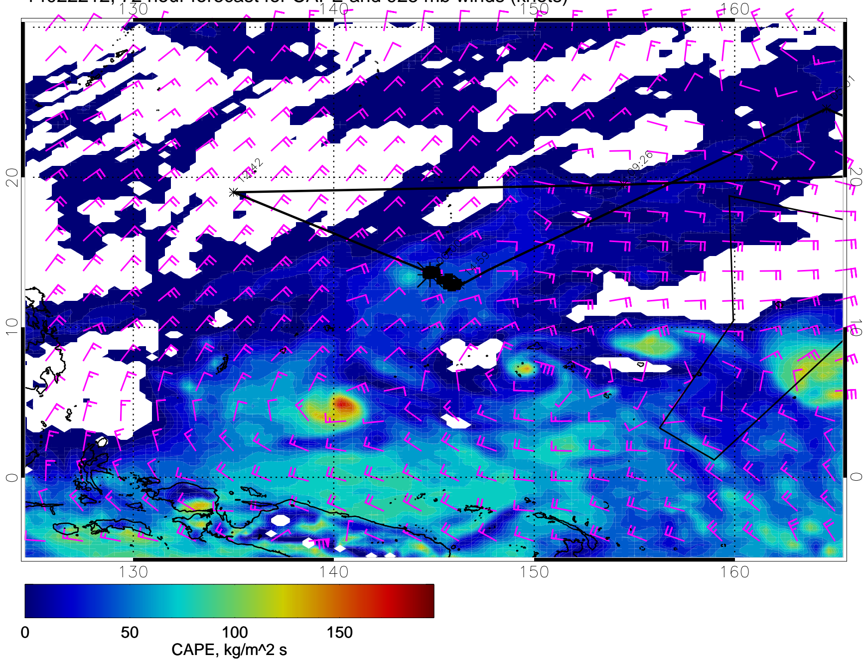
14022212, 72 hour forecast for CAPE and 925 mb winds (knots)
