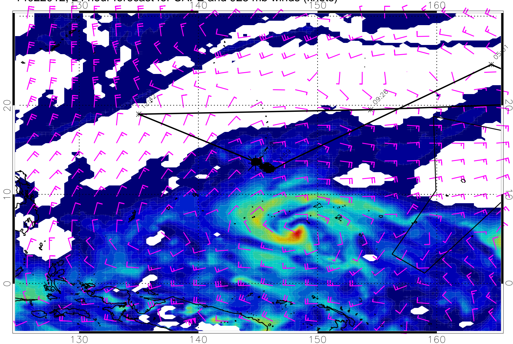
14022012, 24 hour forecast for CAPE and 925 mb winds (knots)
