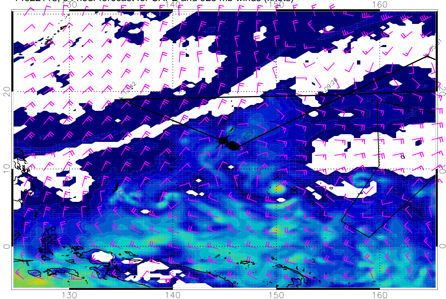
14022118, 54 hour forecast for CAPE and 925 mb winds (knots)
