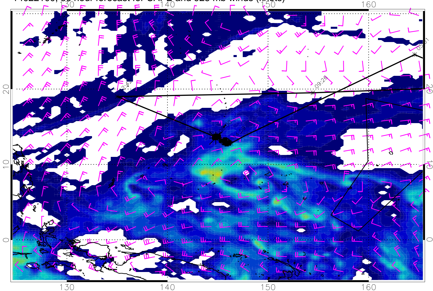
14022100, 36 hour forecast for CAPE and 925 mb winds (knots)
