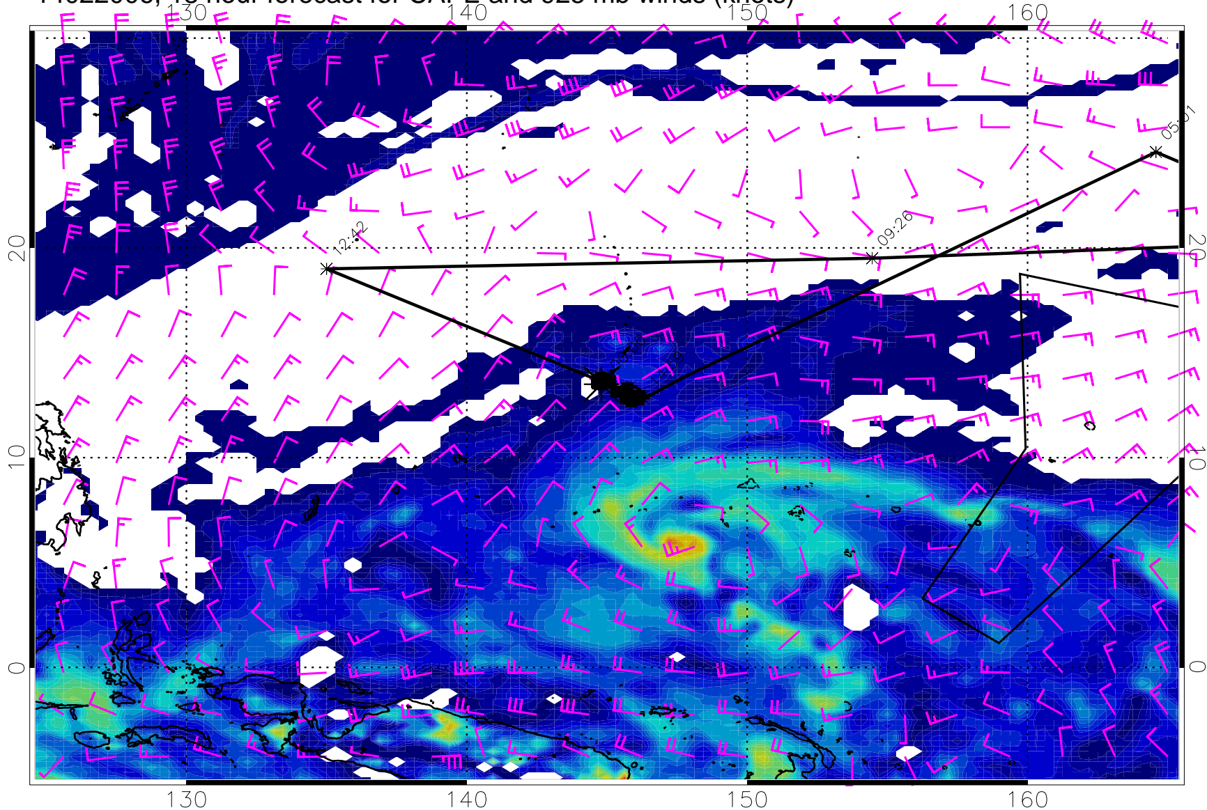
14022006, 18 hour forecast for CAPE and 925 mb winds (knots)
