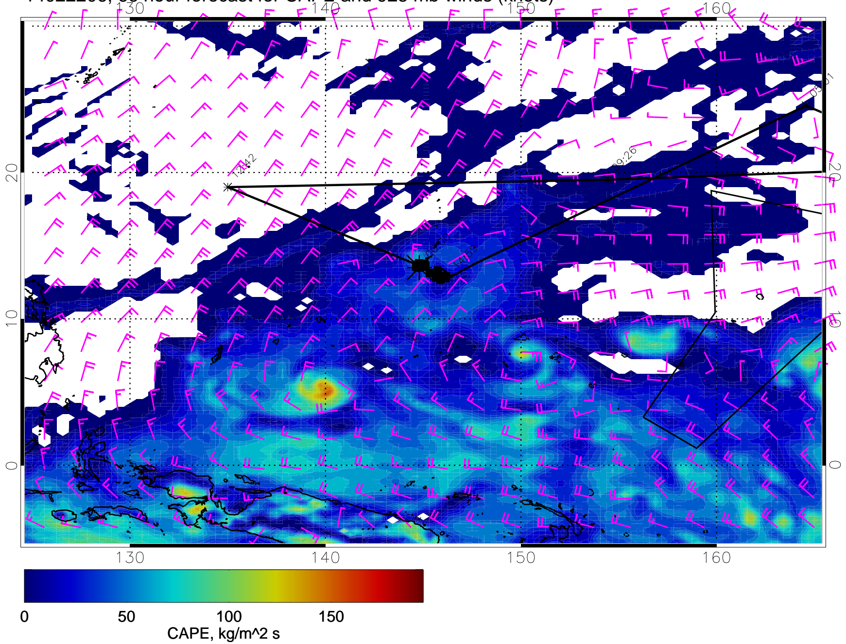
14022206, 66 hour forecast for CAPE and 925 mb winds (knots)
