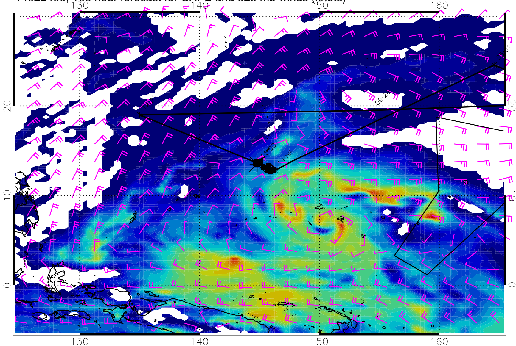
14022400, 108 hour forecast for CAPE and 925 mb winds (knots)
