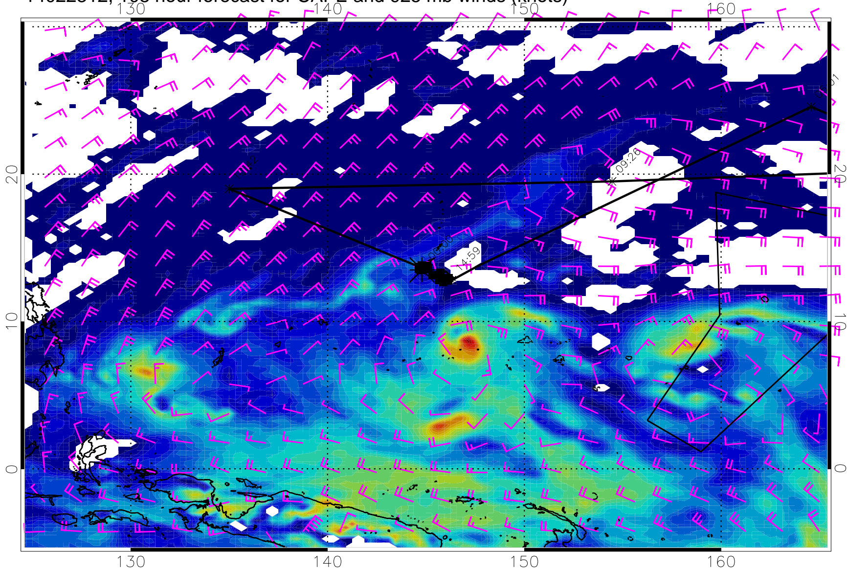
14022312, 108 hour forecast for CAPE and 925 mb winds (knots)
