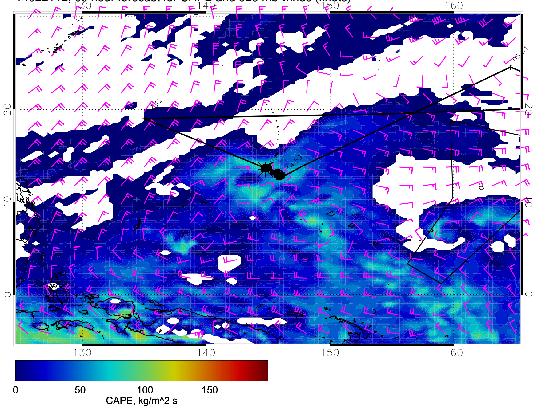
14022112, 60 hour forecast for CAPE and 925 mb winds (knots)
