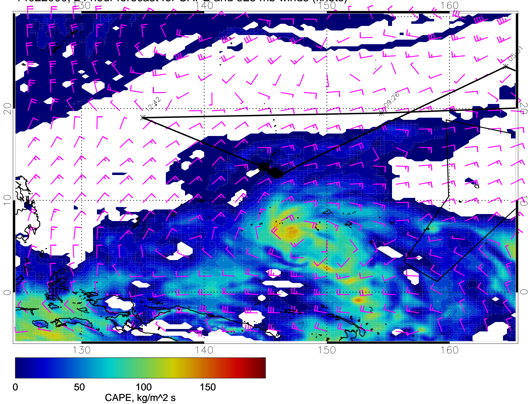
14022000, 24 hour forecast for CAPE and 925 mb winds (knots)
