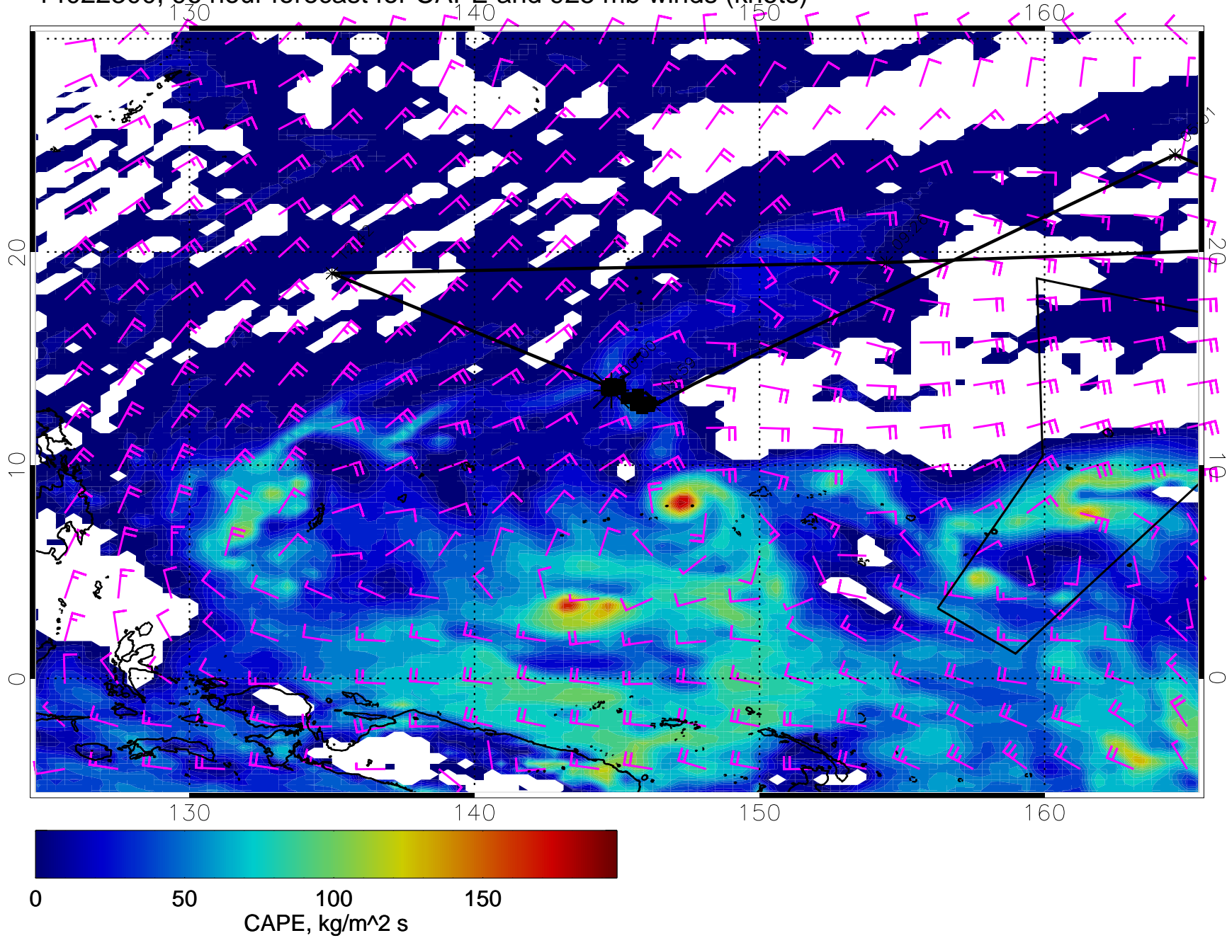
14022300, 96 hour forecast for CAPE and 925 mb winds (knots)
