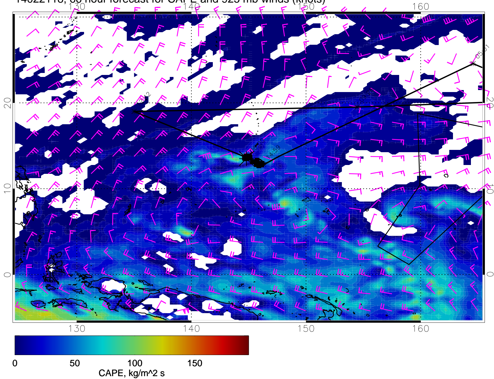
14022118, 66 hour forecast for CAPE and 925 mb winds (knots)
