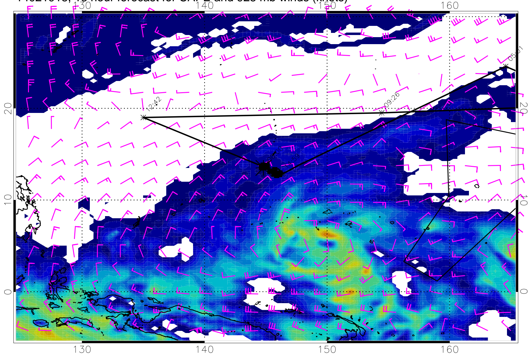
14021918, 18 hour forecast for CAPE and 925 mb winds (knots)
