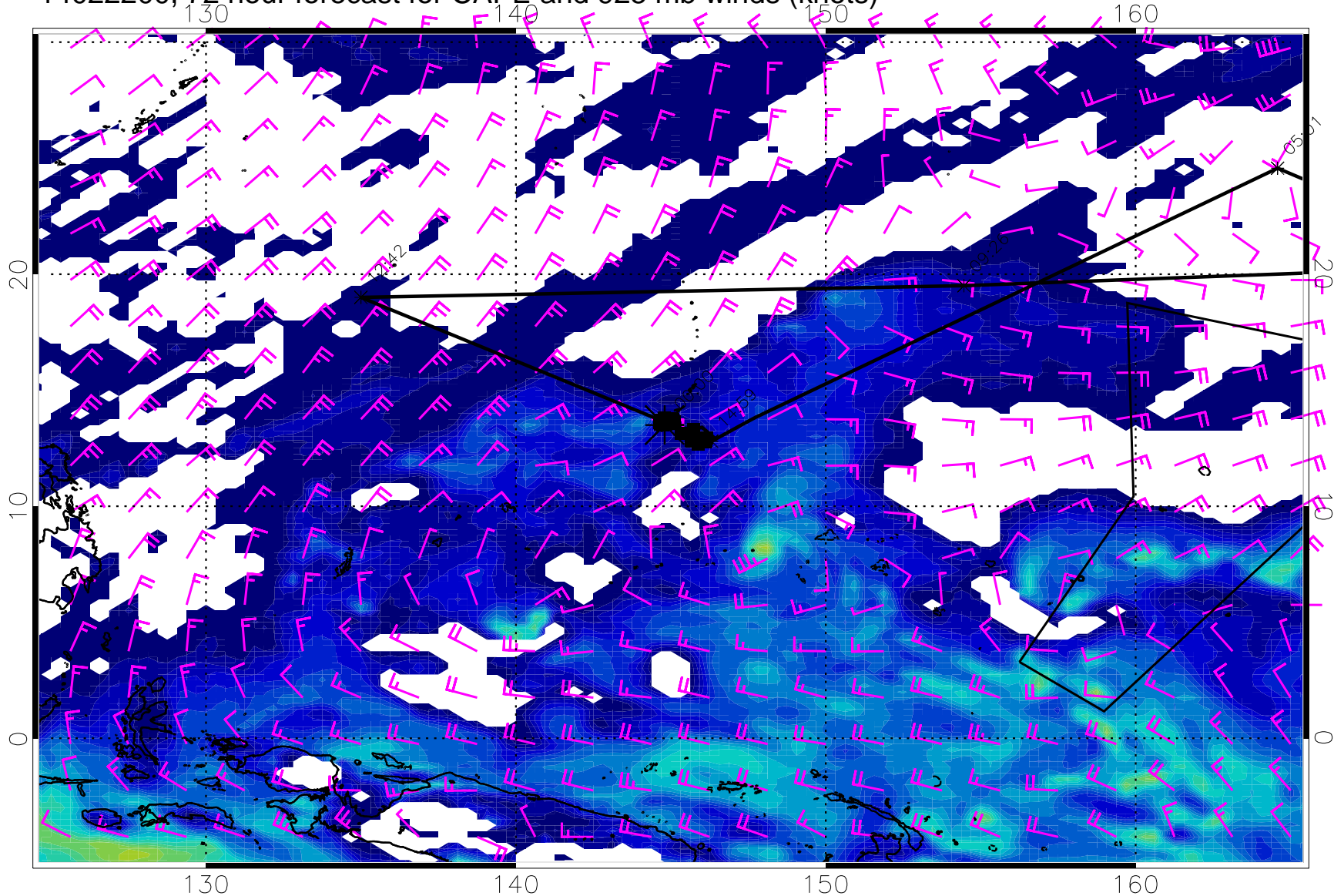
14022200, 72 hour forecast for CAPE and 925 mb winds (knots)
