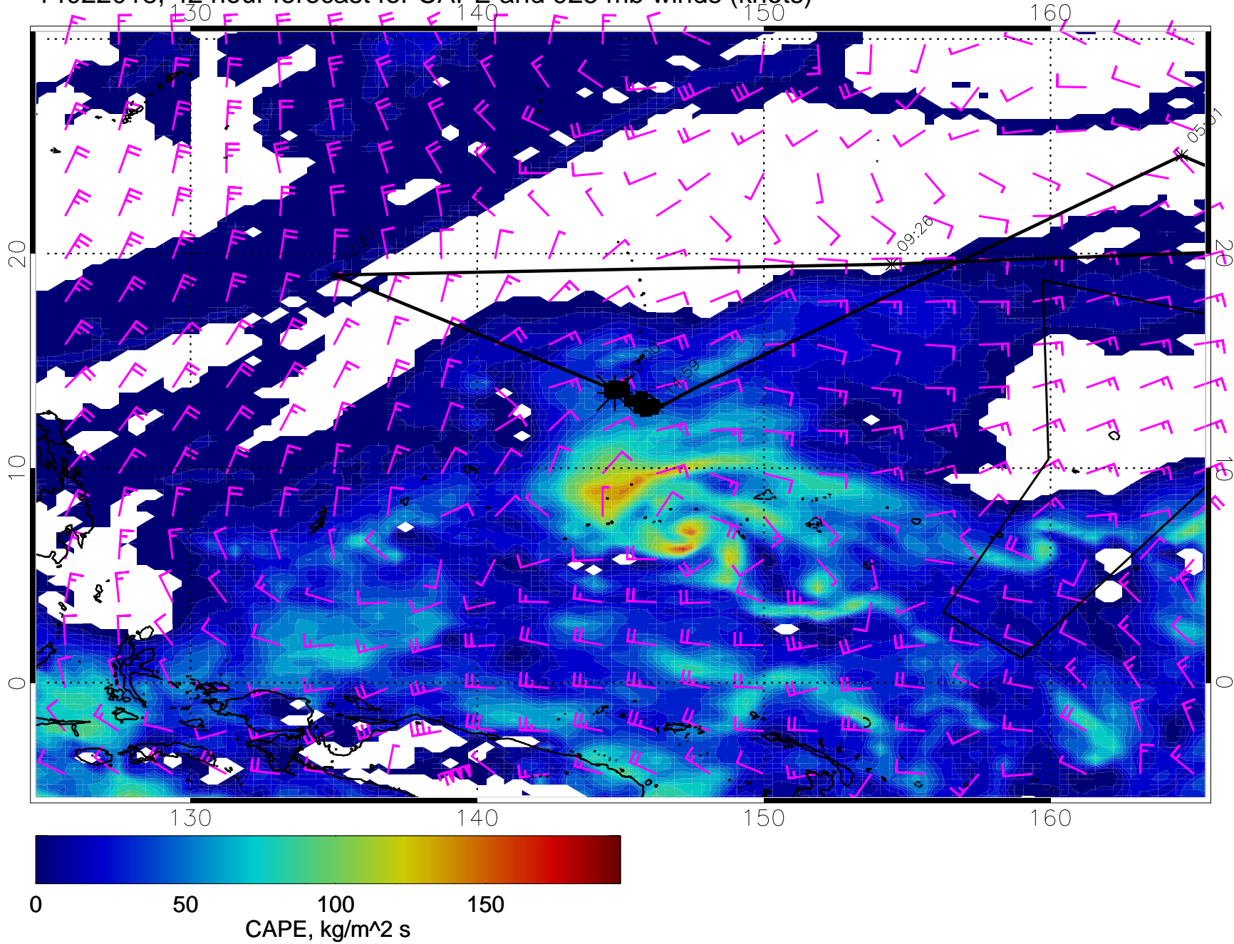
14022018, 42 hour forecast for CAPE and 925 mb winds (knots)
