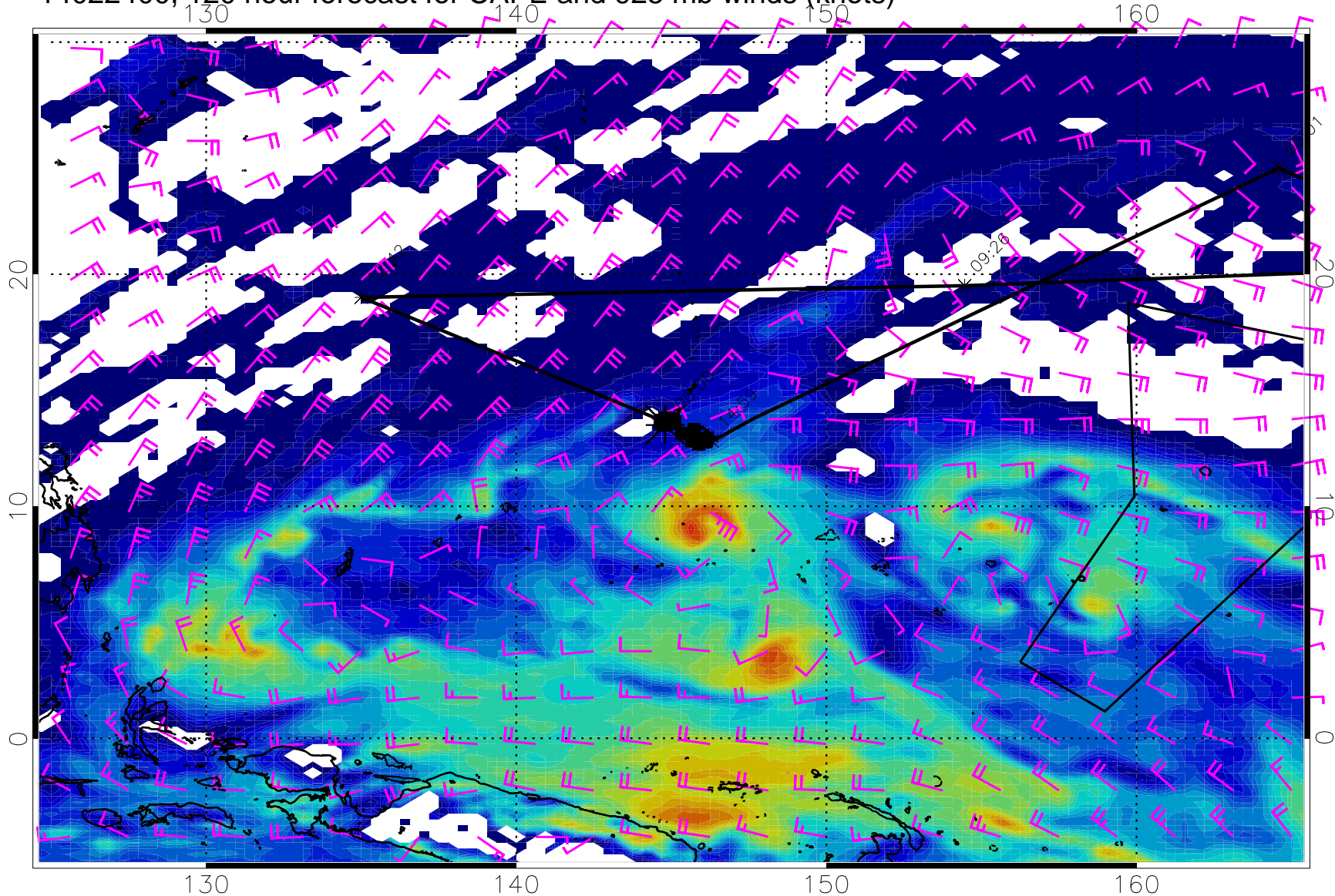
14022400, 120 hour forecast for CAPE and 925 mb winds (knots)
