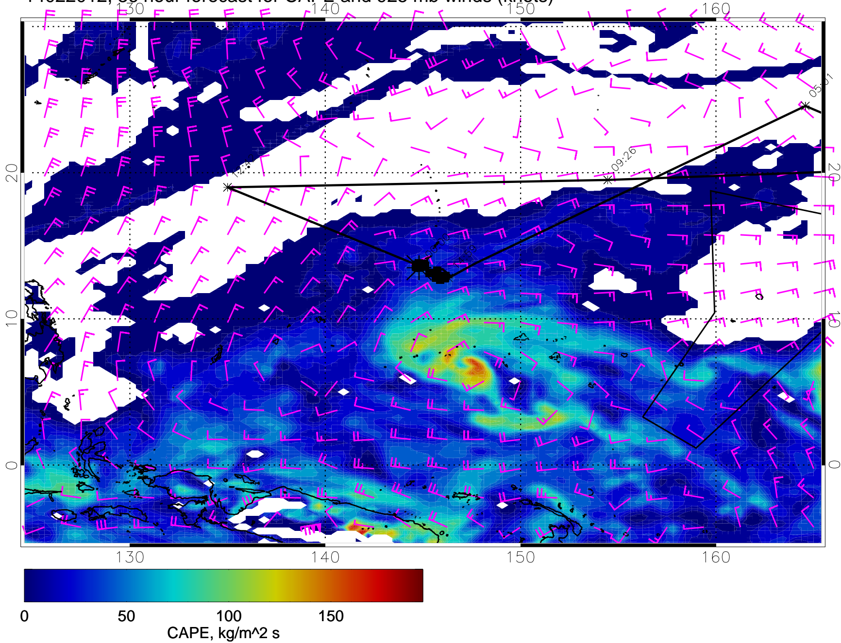
14022012, 36 hour forecast for CAPE and 925 mb winds (knots)
