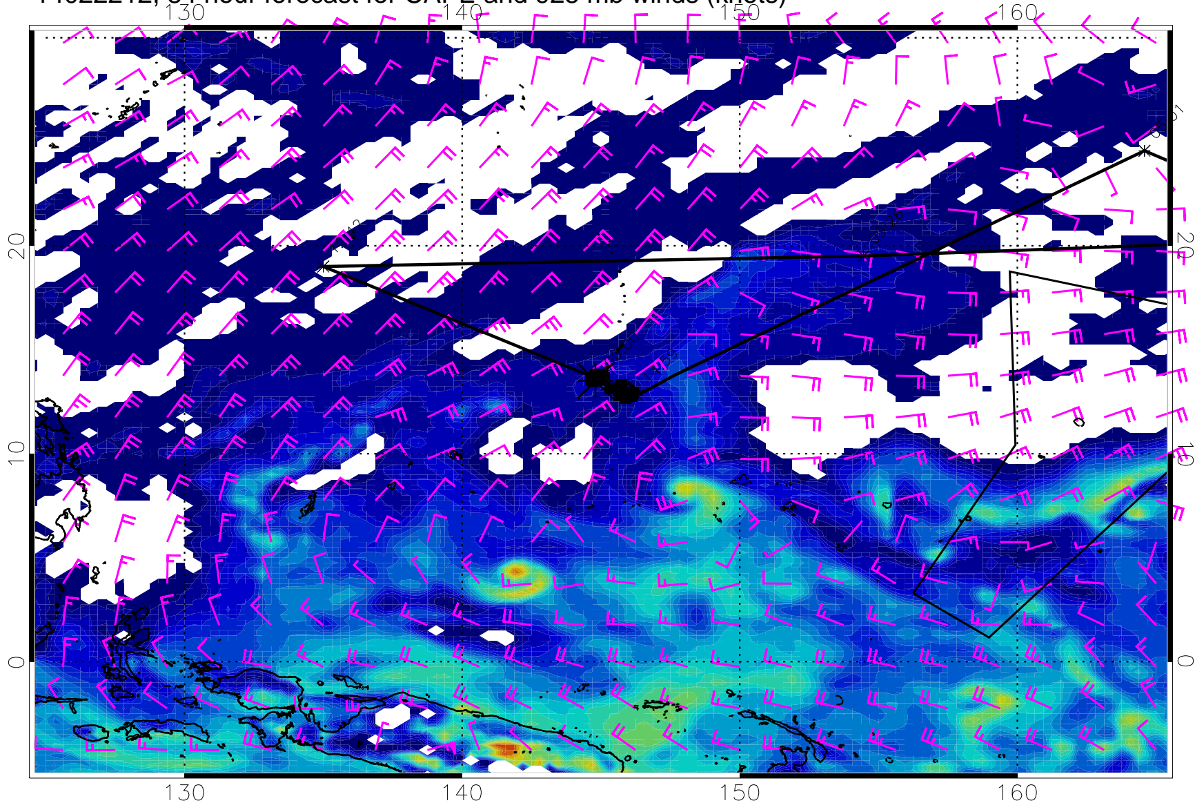
14022212, 84 hour forecast for CAPE and 925 mb winds (knots)
