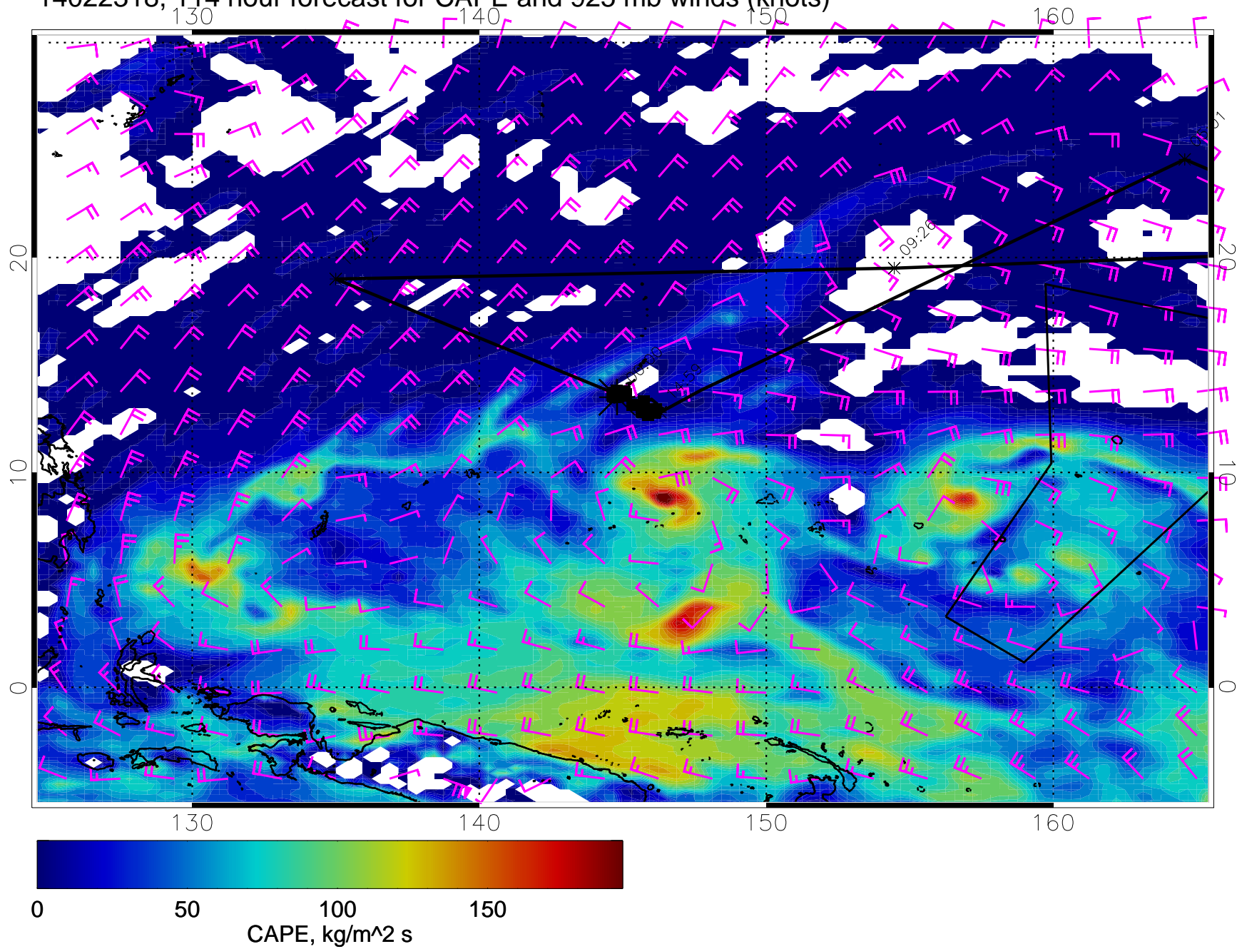
14022318, 114 hour forecast for CAPE and 925 mb winds (knots)
