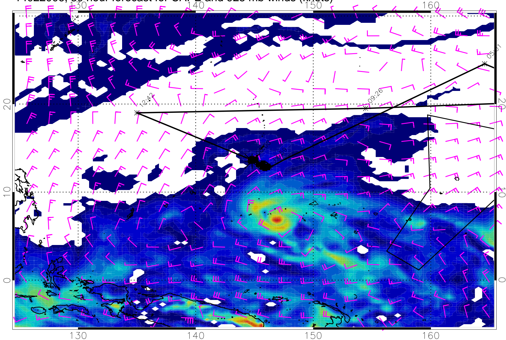
14022006, 30 hour forecast for CAPE and 925 mb winds (knots)
