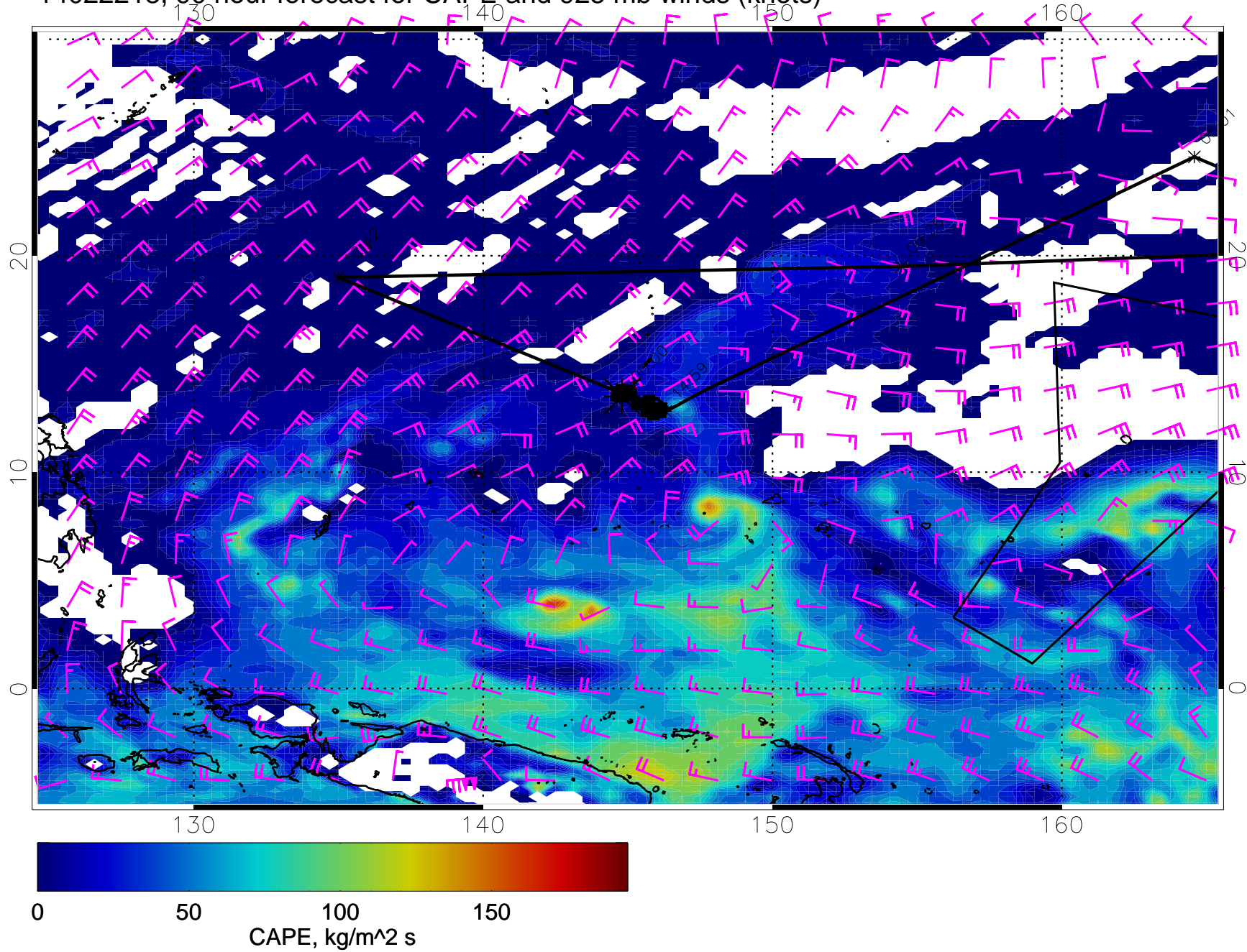
14022218, 90 hour forecast for CAPE and 925 mb winds (knots)
