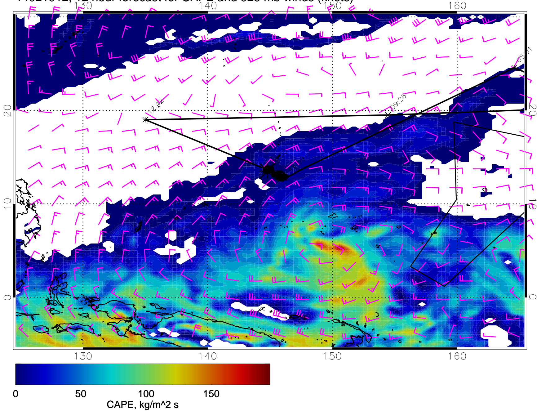
14021912, 12 hour forecast for CAPE and 925 mb winds (knots)
