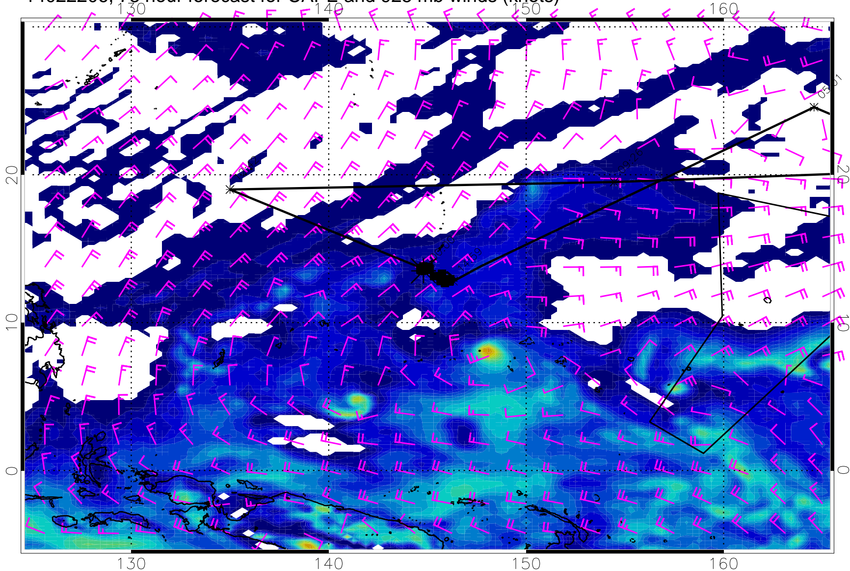
14022206, 78 hour forecast for CAPE and 925 mb winds (knots)
