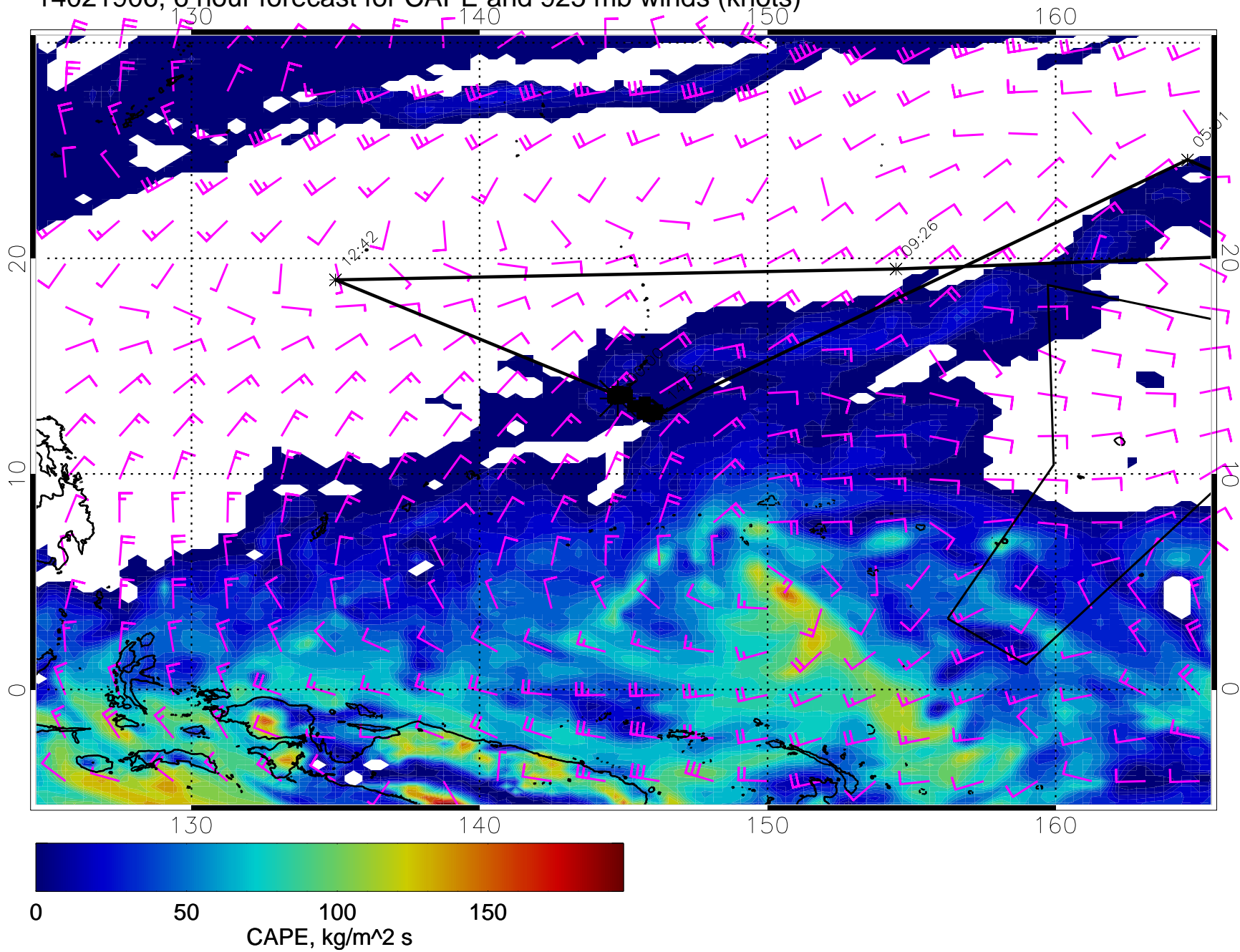
14021906, 6 hour forecast for CAPE and 925 mb winds (knots)
