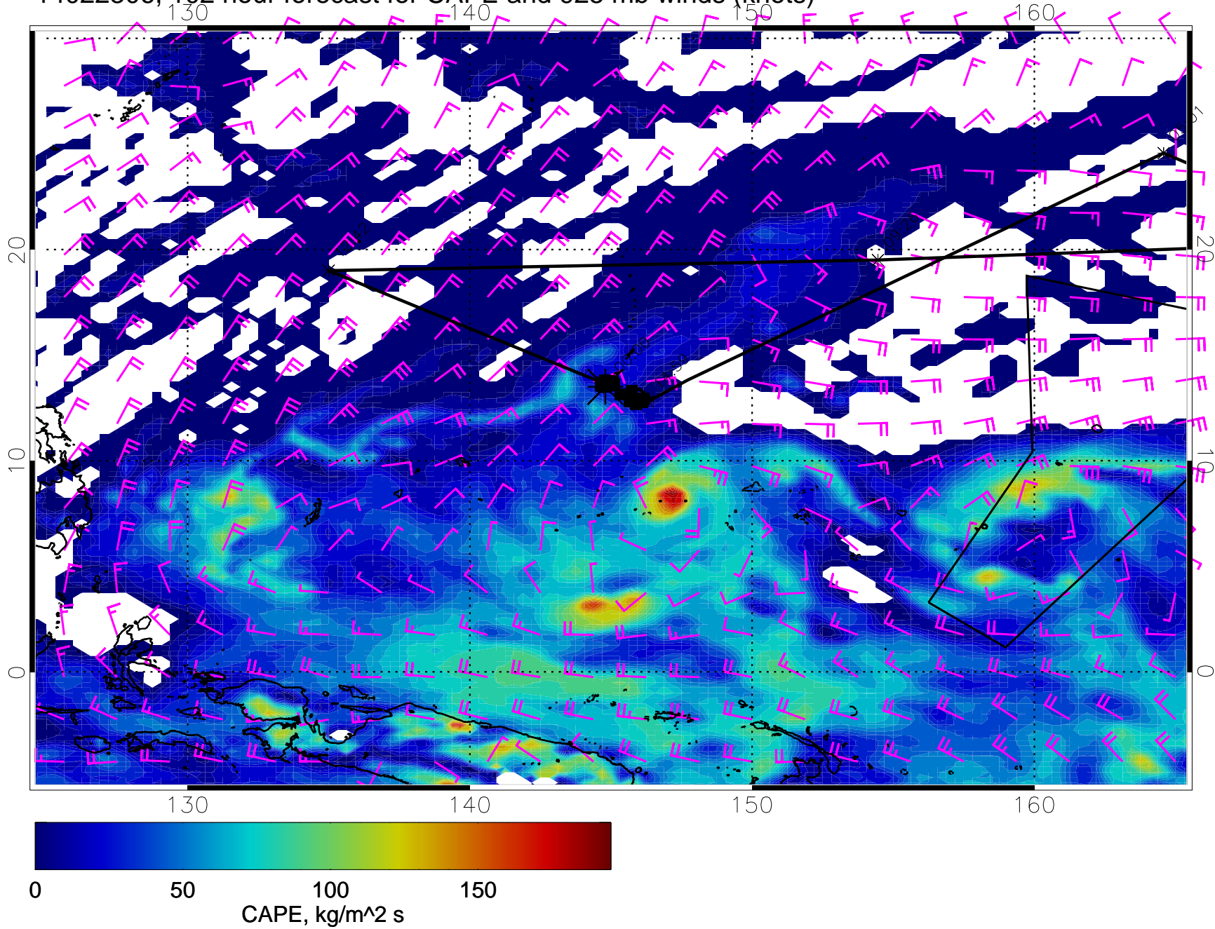
14022306, 102 hour forecast for CAPE and 925 mb winds (knots)
