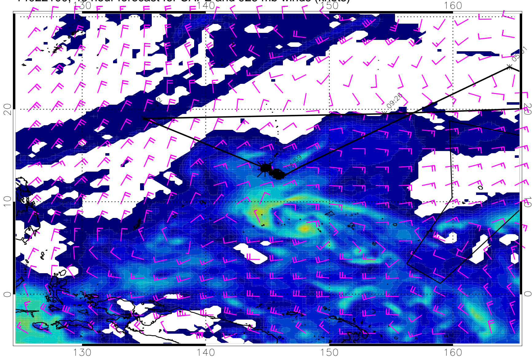
14022100, 48 hour forecast for CAPE and 925 mb winds (knots)
