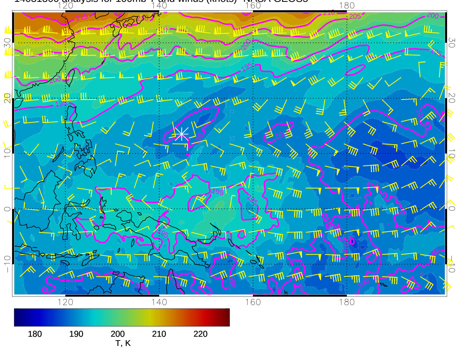
14031300 analysis for 100mb T and winds (knots)- NASA GEOS5
