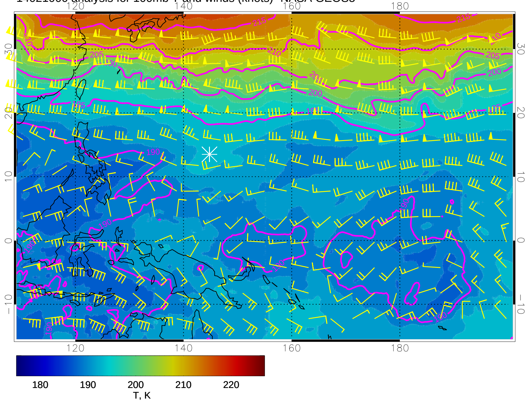
14021000 analysis for 100mb T and winds (knots)- NASA GEOS5
