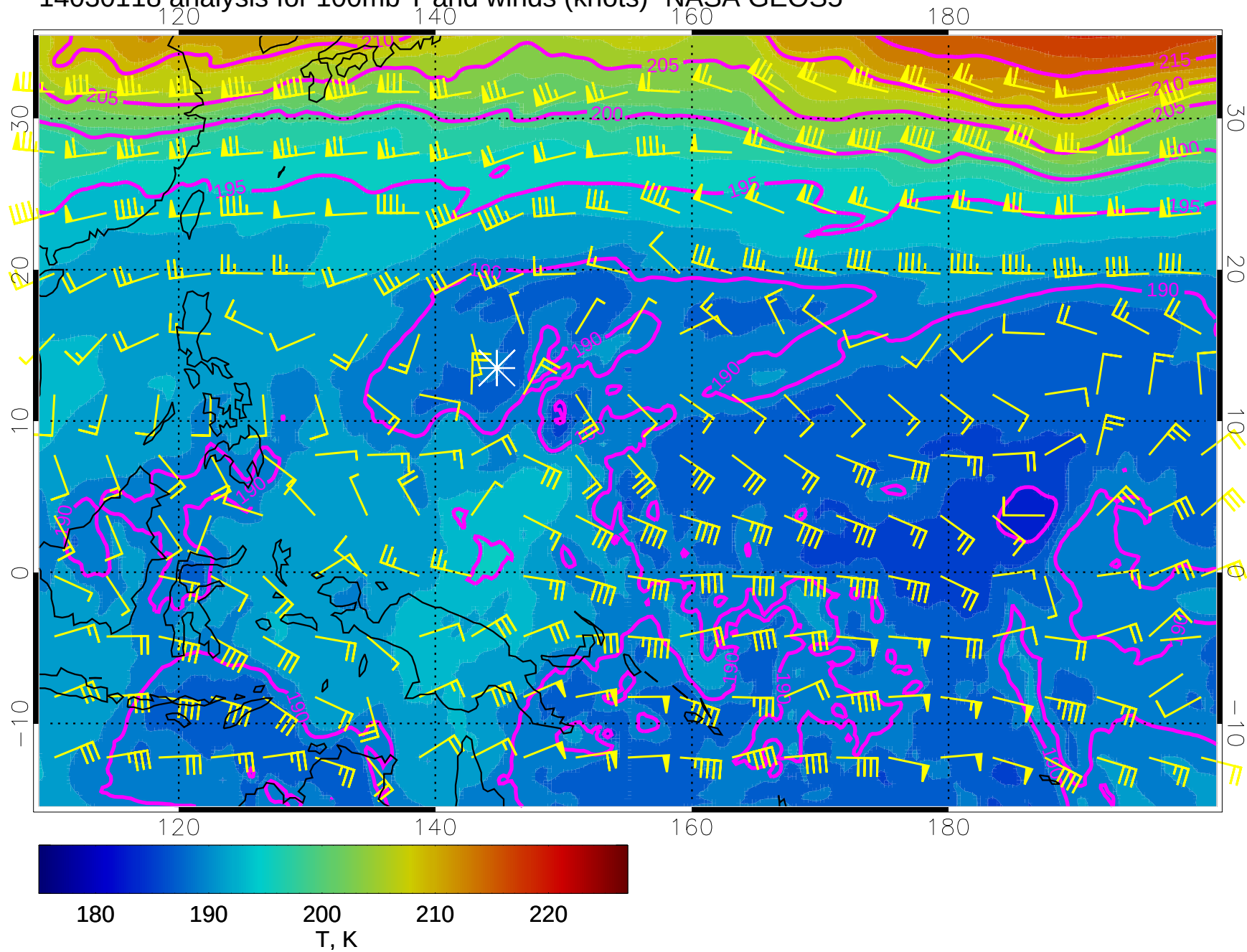
14030118 analysis for 100mb T and winds (knots)- NASA GEOS5
