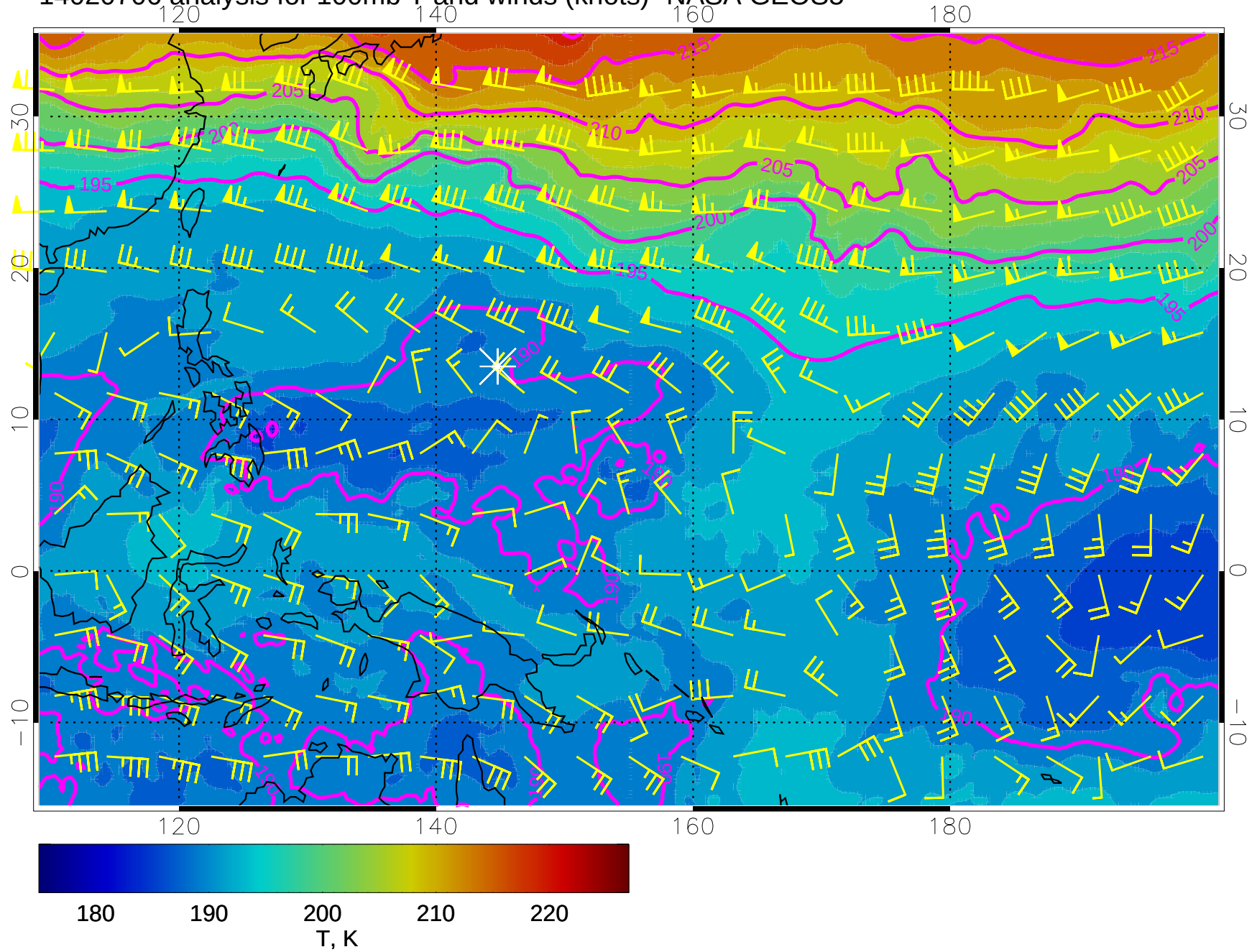
14020706 analysis for 100mb T and winds (knots)- NASA GEOS5
