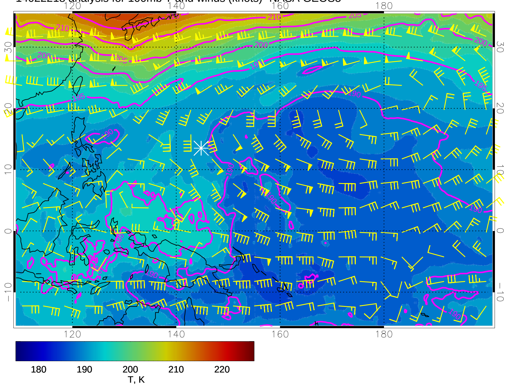
14022218 analysis for 100mb T and winds (knots)- NASA GEOS5
