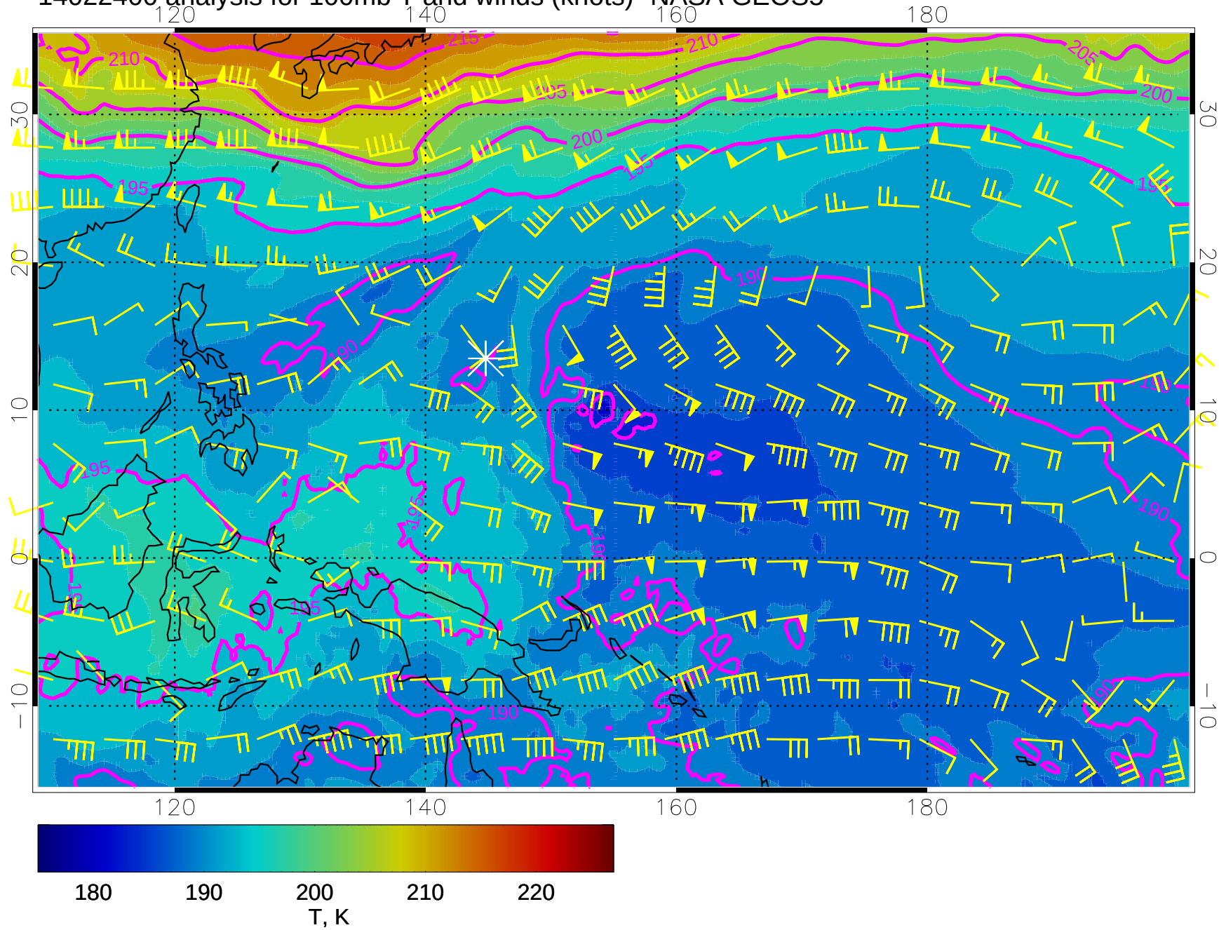
14022400 analysis for 100mb T and winds (knots)- NASA GEOS5
