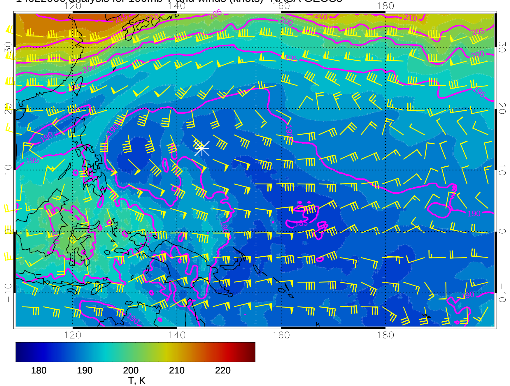
14022006 analysis for 100mb T and winds (knots)- NASA GEOS5
