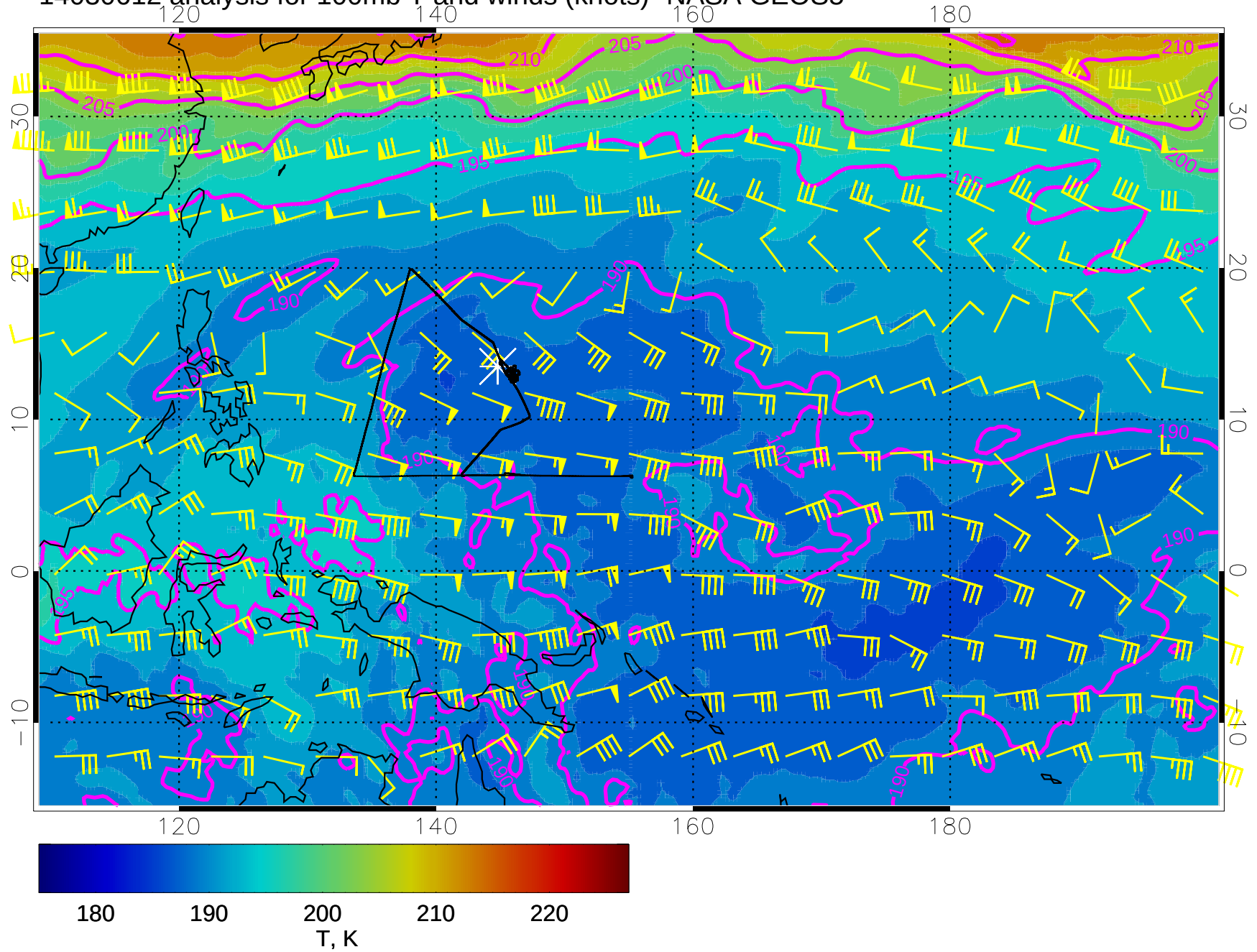
14030612 analysis for 100mb T and winds (knots)- NASA GEOS5
