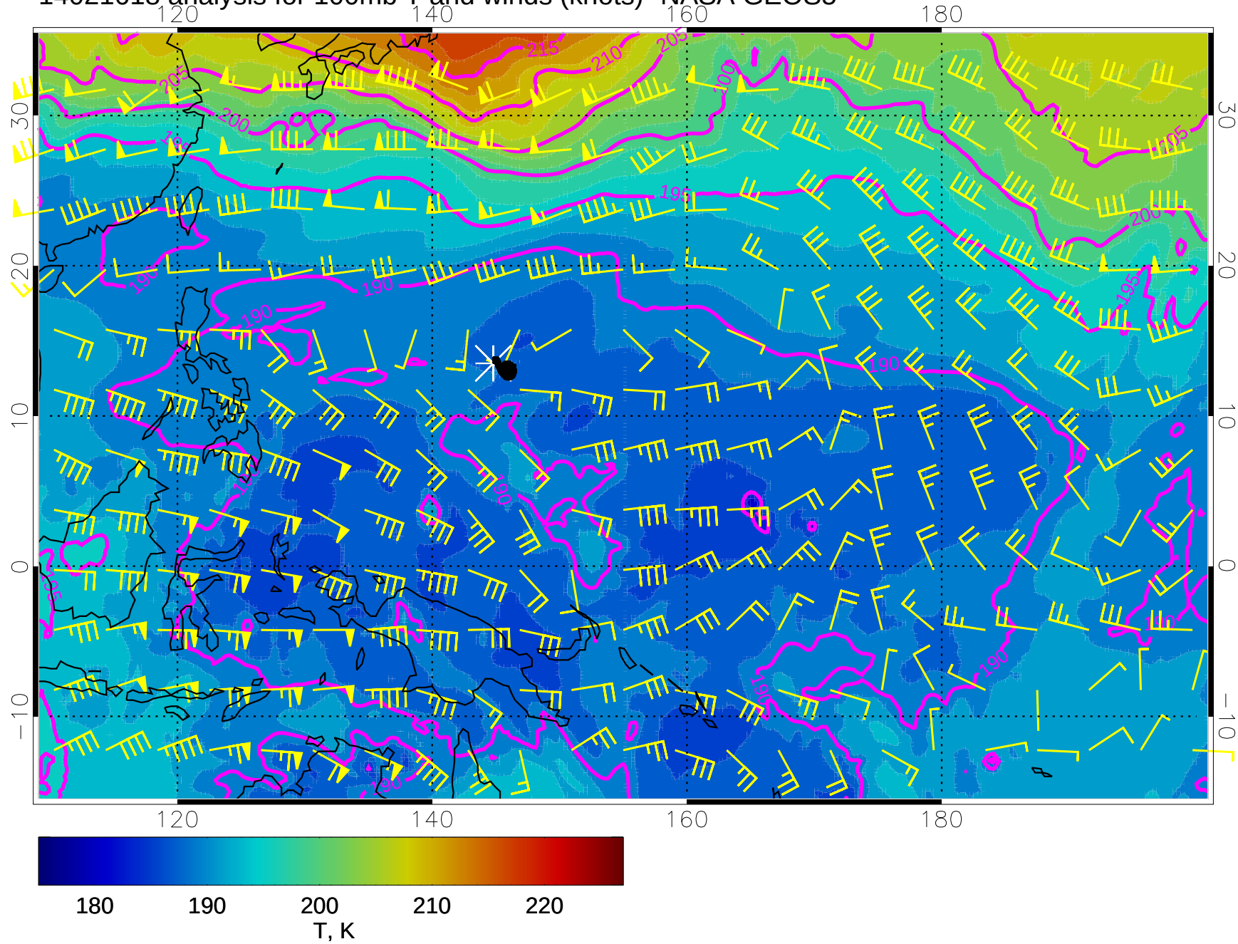
14021618 analysis for 100mb T and winds (knots)- NASA GEOS5
