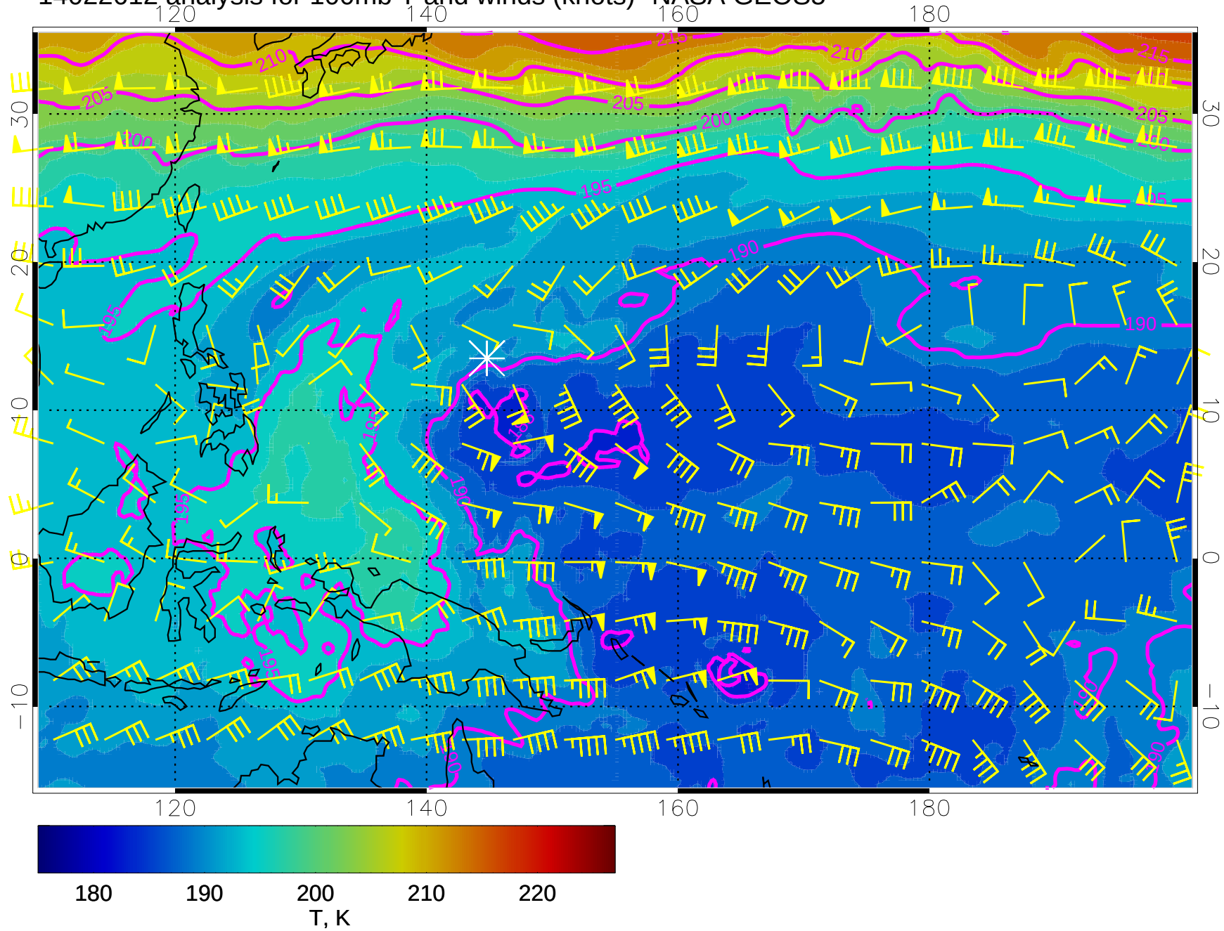
14022612 analysis for 100mb T and winds (knots)- NASA GEOS5
