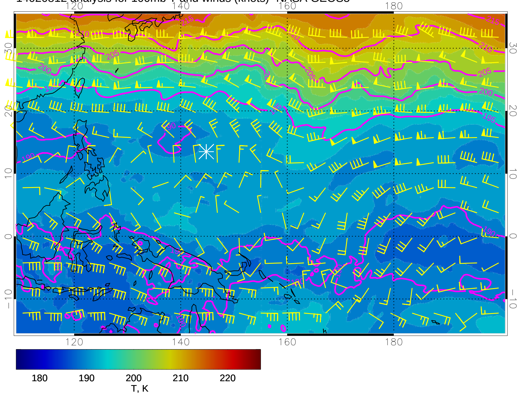
14020812 analysis for 100mb T and winds (knots)- NASA GEOS5
