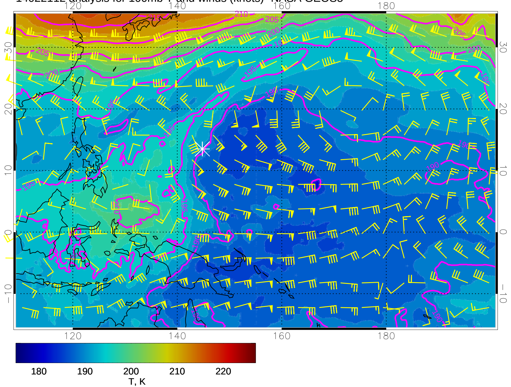
14022112 analysis for 100mb T and winds (knots)- NASA GEOS5
