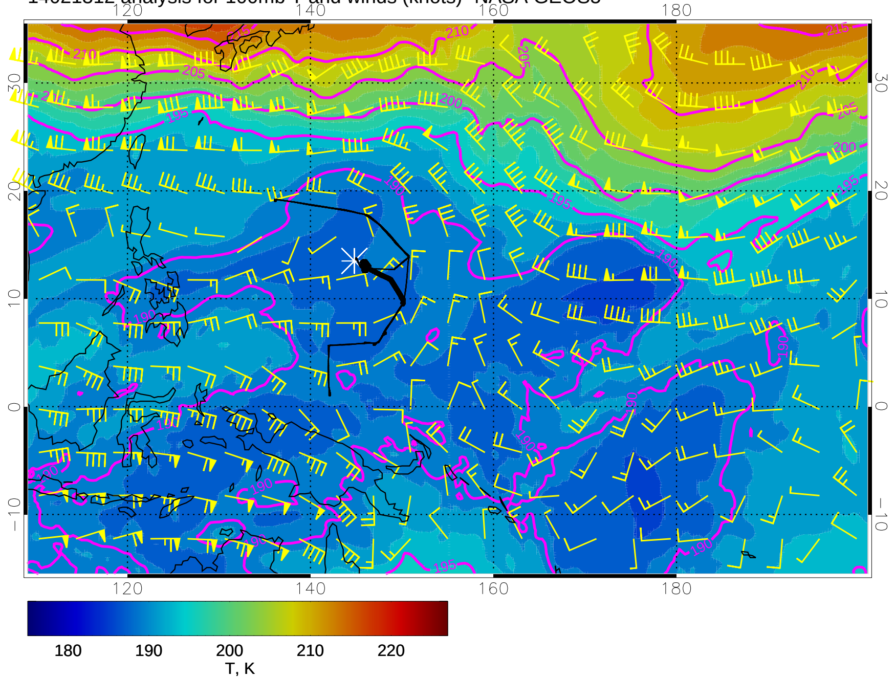
14021312 analysis for 100mb T and winds (knots)- NASA GEOS5
