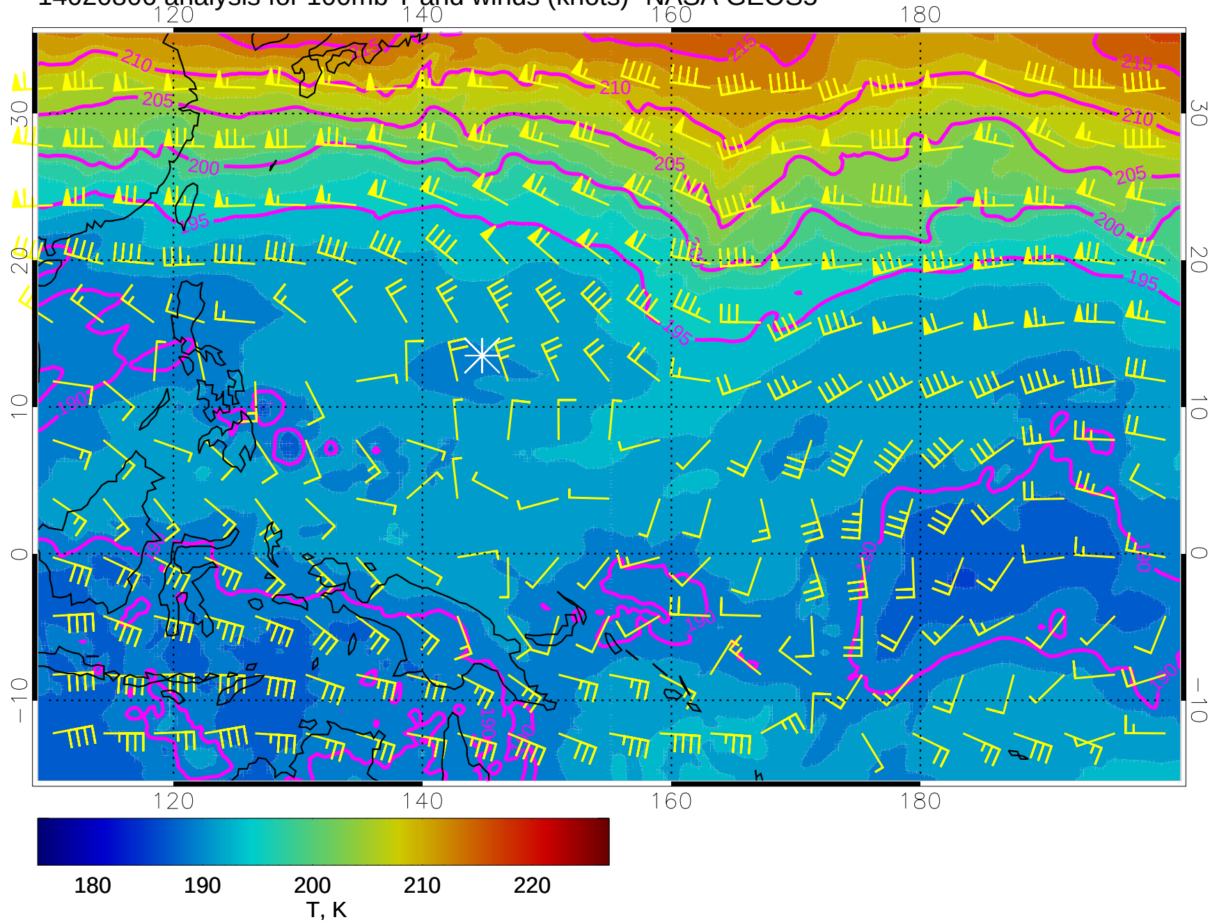
14020806 analysis for 100mb T and winds (knots)- NASA GEOS5
