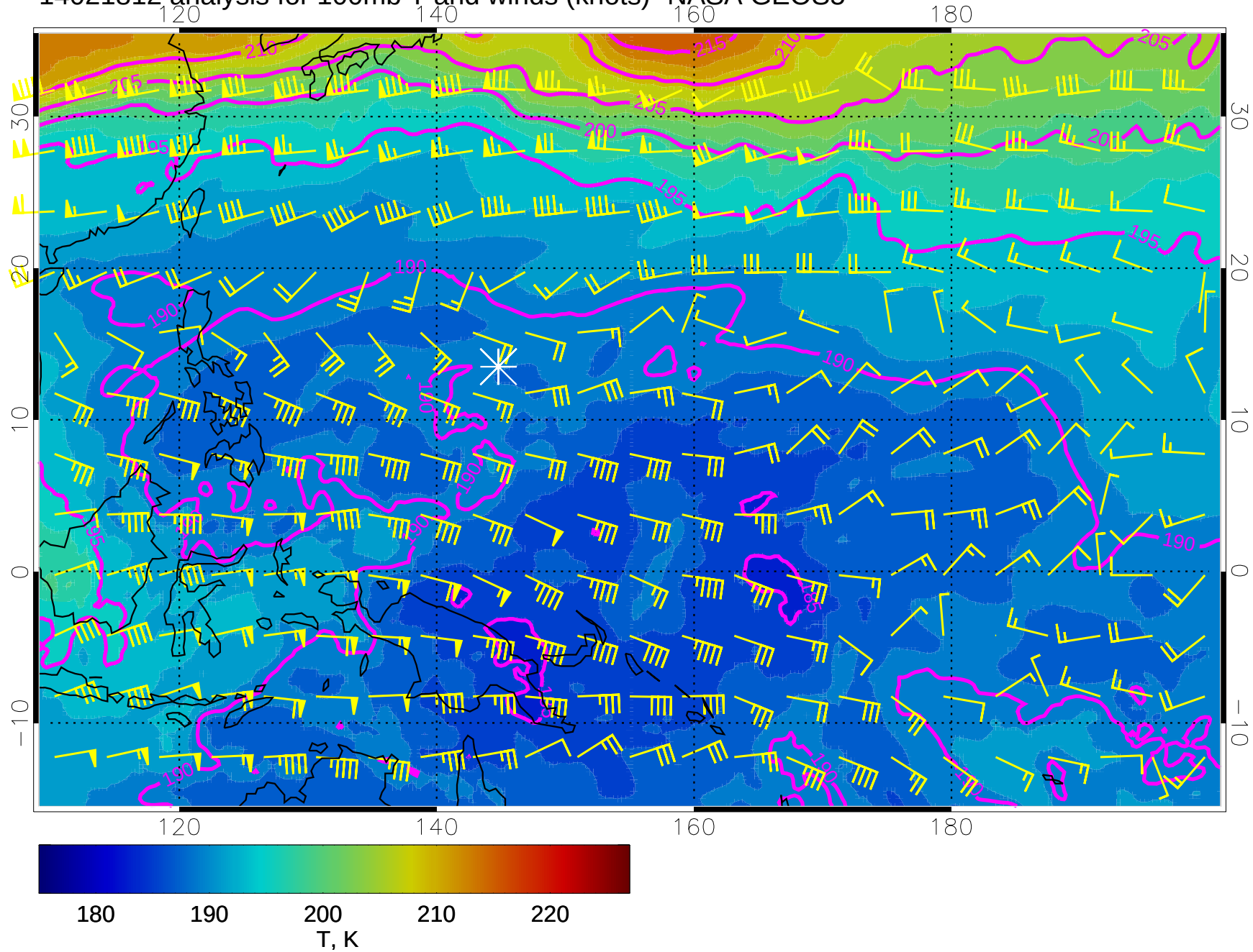
14021812 analysis for 100mb T and winds (knots)- NASA GEOS5
