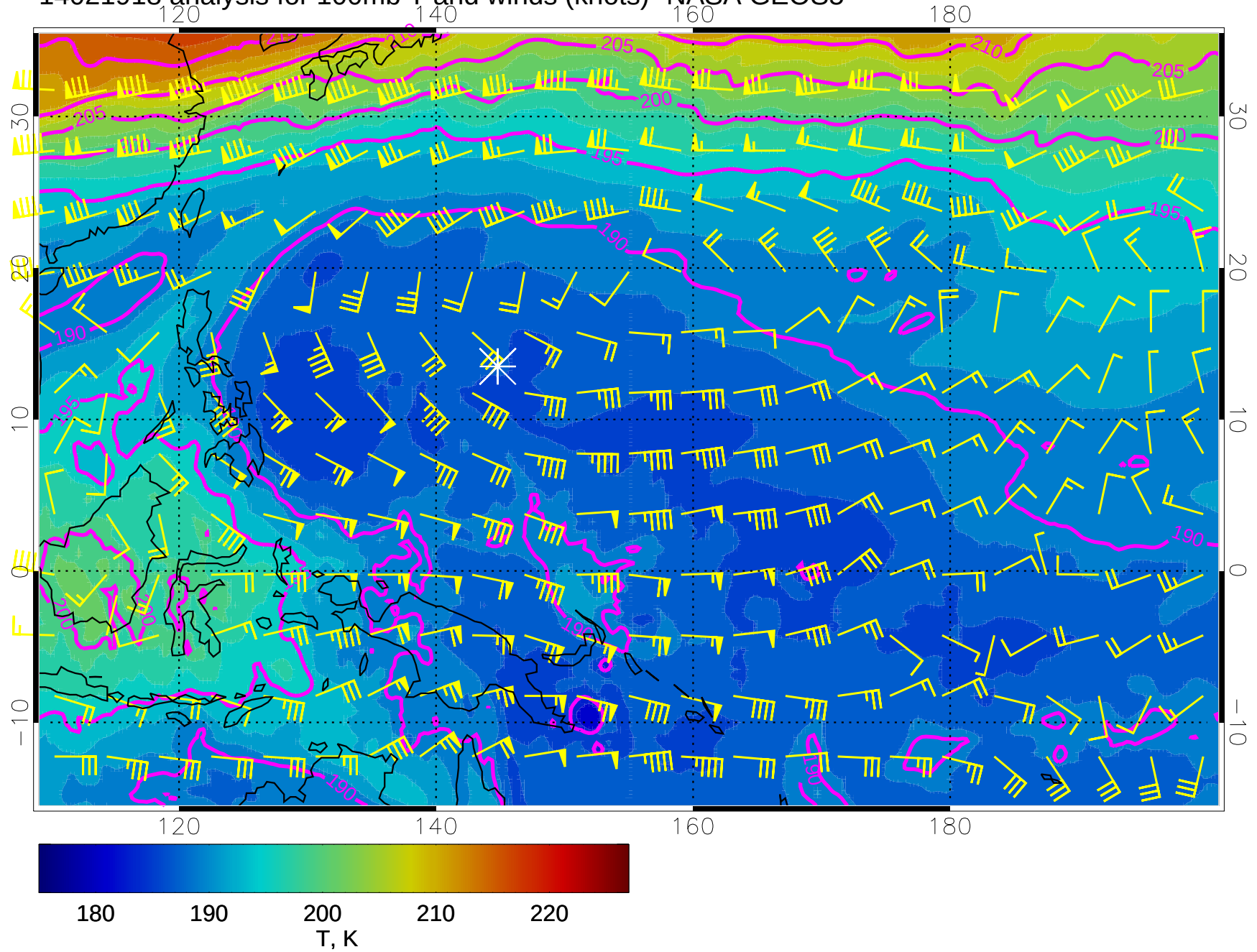
14021918 analysis for 100mb T and winds (knots)- NASA GEOS5
