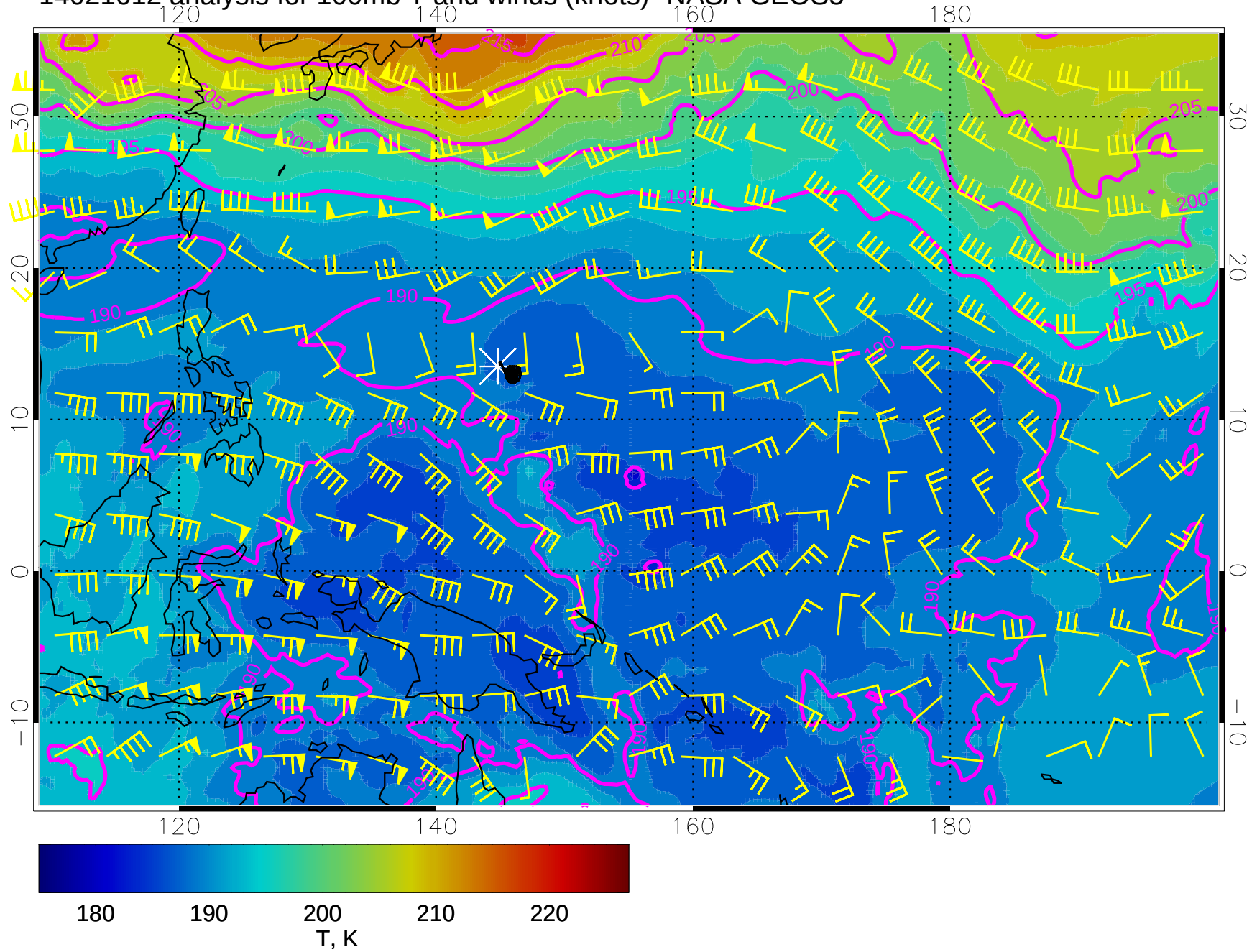
14021612 analysis for 100mb T and winds (knots)- NASA GEOS5
