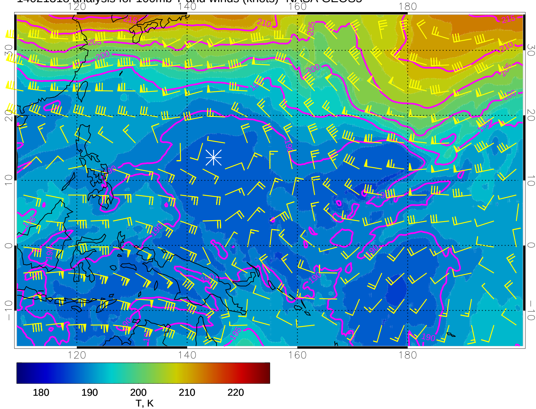
14021318 analysis for 100mb T and winds (knots)- NASA GEOS5
