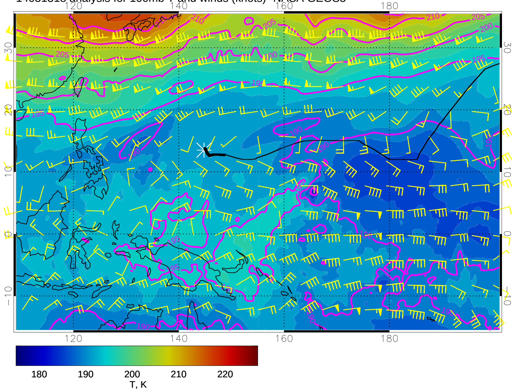
14031318 analysis for 100mb T and winds (knots)- NASA GEOS5
