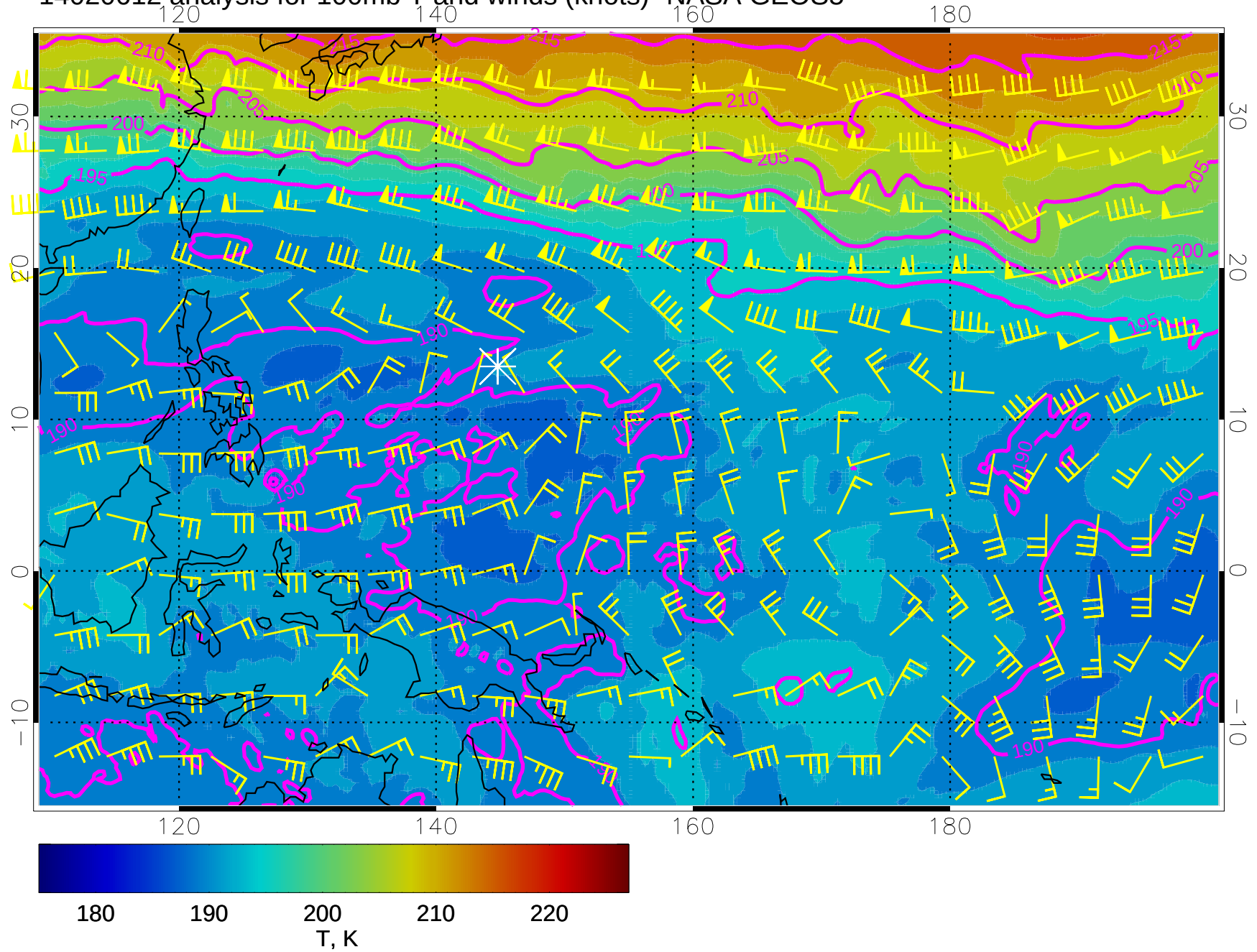
14020612 analysis for 100mb T and winds (knots)- NASA GEOS5
