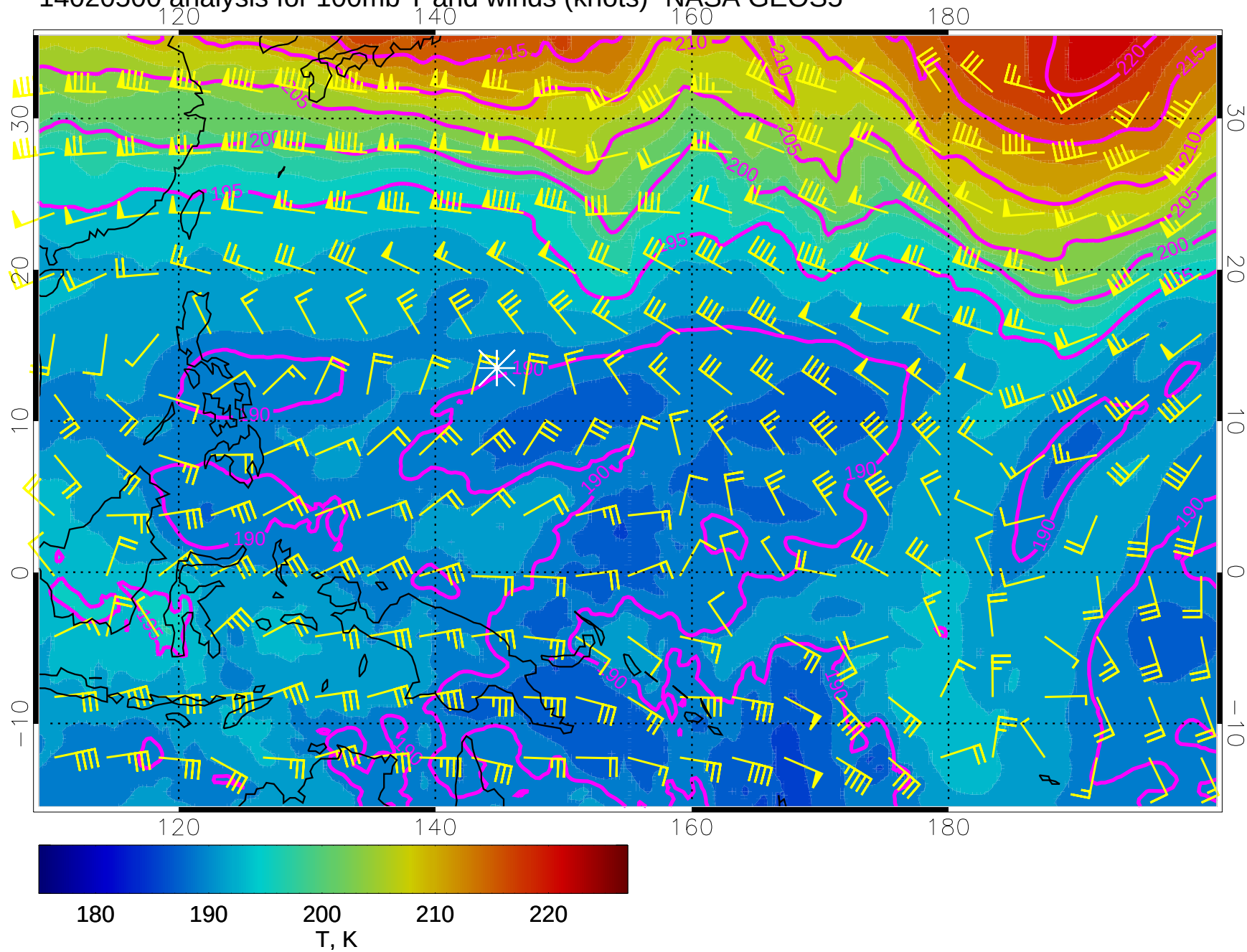
14020500 analysis for 100mb T and winds (knots)- NASA GEOS5
