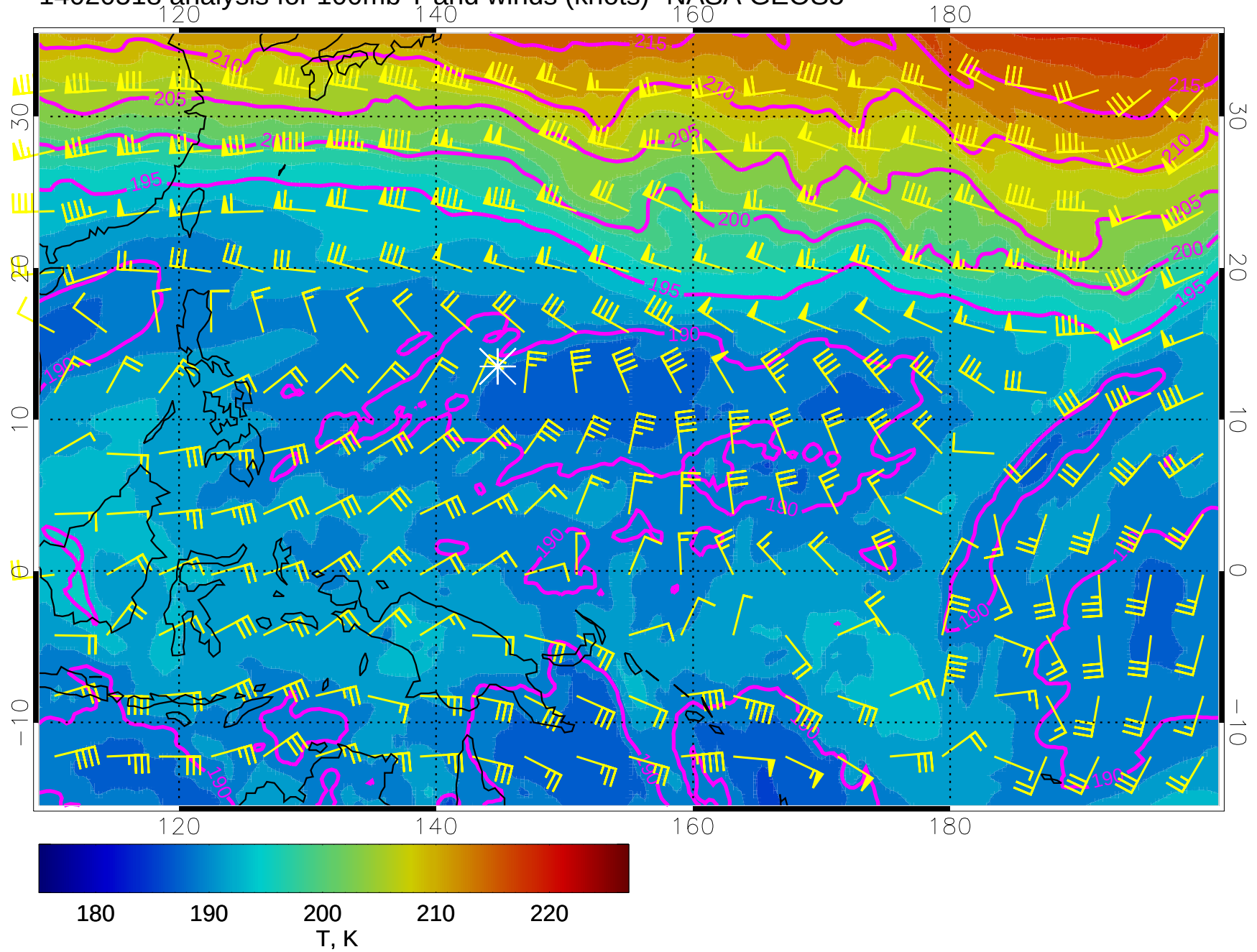
14020518 analysis for 100mb T and winds (knots)- NASA GEOS5
