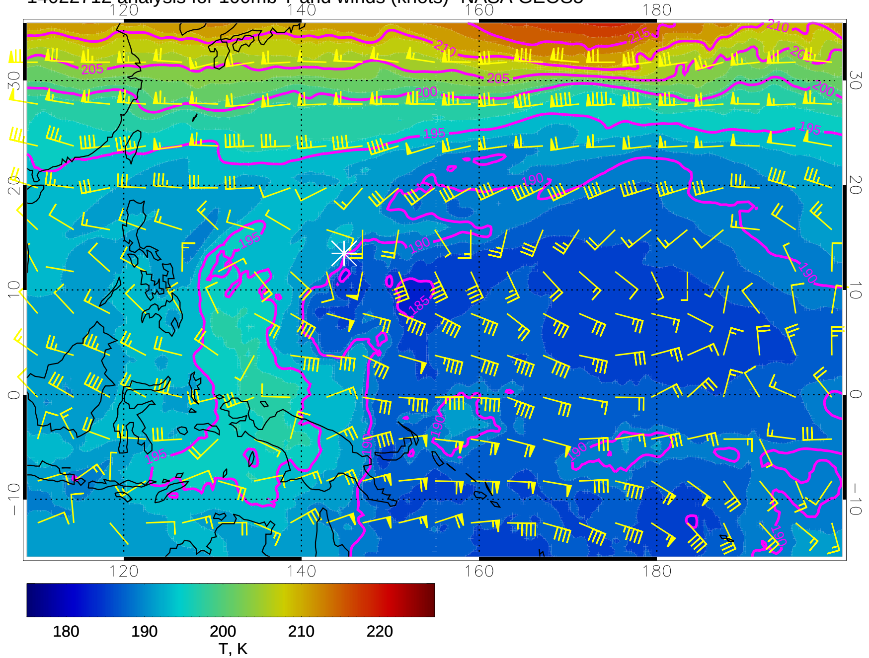
14022712 analysis for 100mb T and winds (knots)- NASA GEOS5
