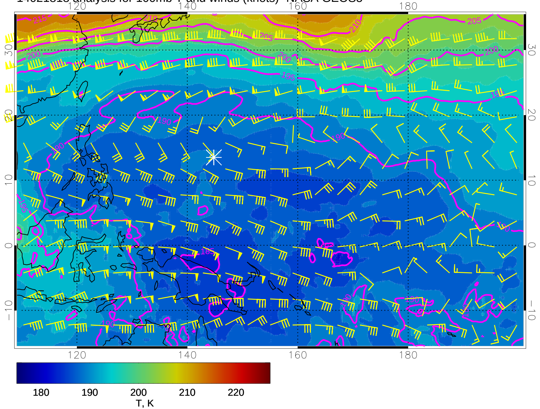
14021818 analysis for 100mb T and winds (knots)- NASA GEOS5
