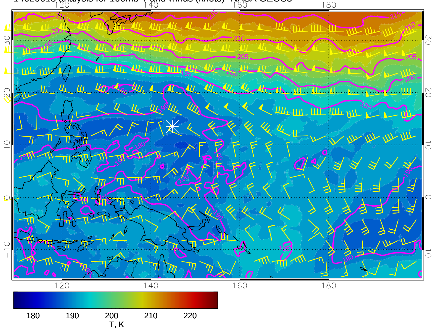
14020618 analysis for 100mb T and winds (knots)- NASA GEOS5
