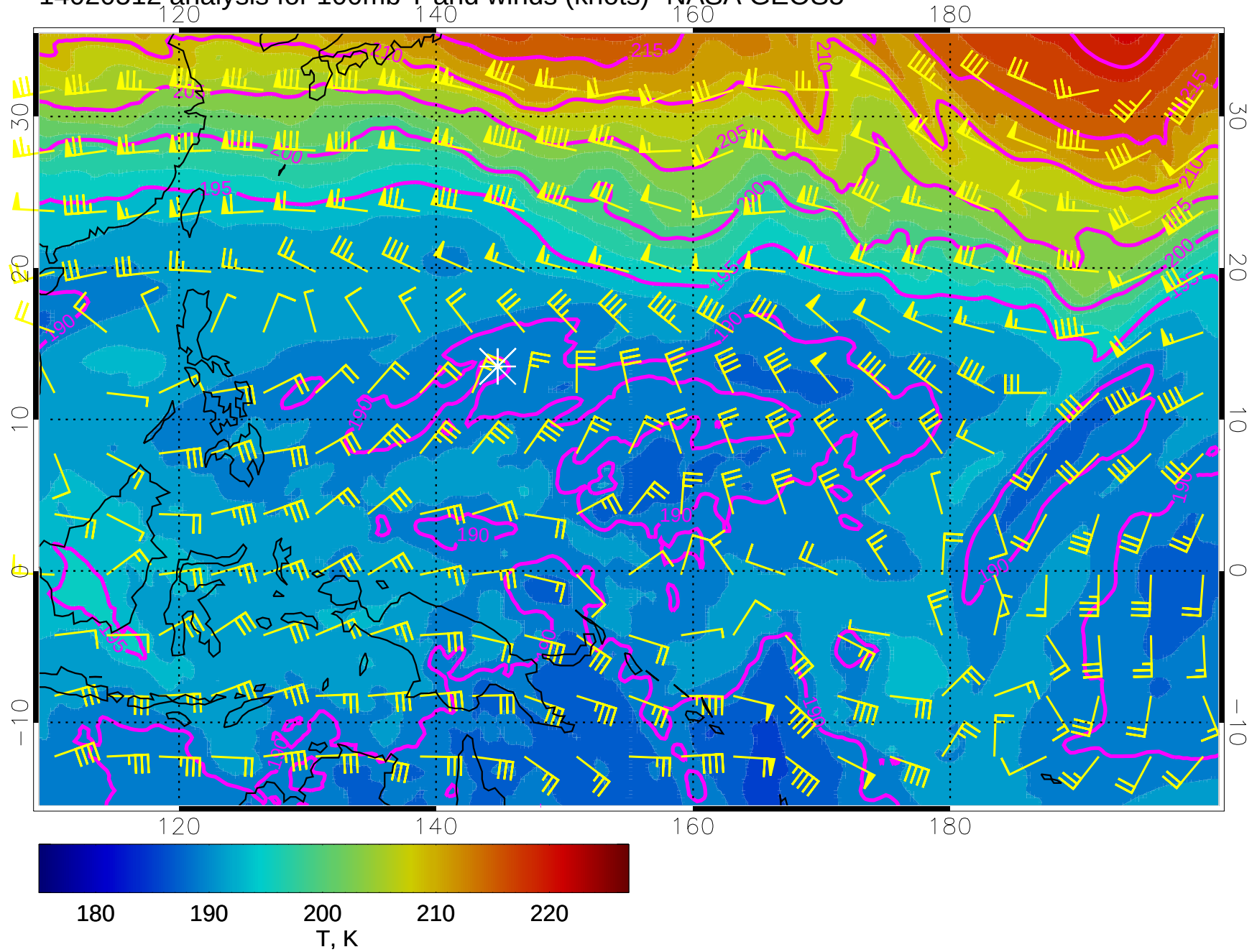
14020512 analysis for 100mb T and winds (knots)- NASA GEOS5
