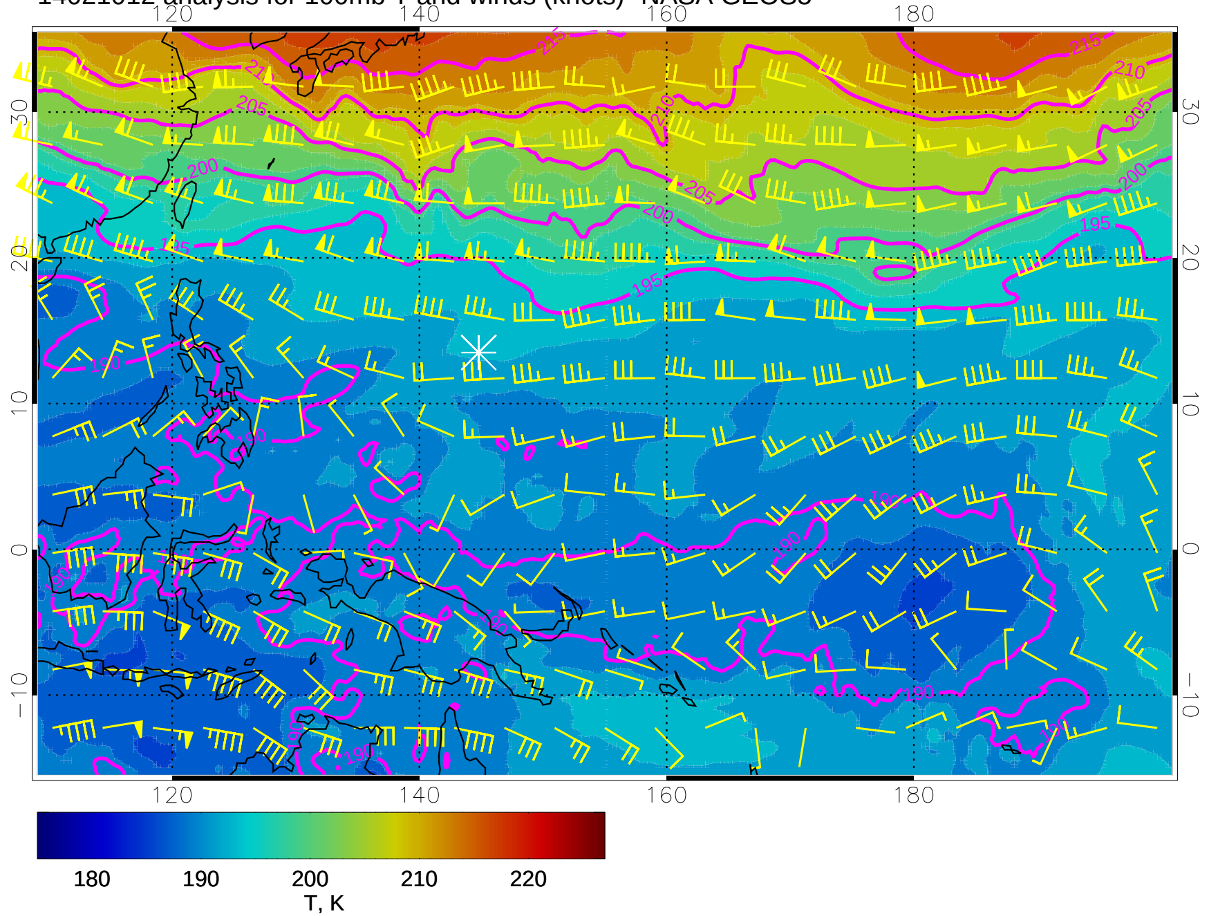
14021012 analysis for 100mb T and winds (knots)- NASA GEOS5
