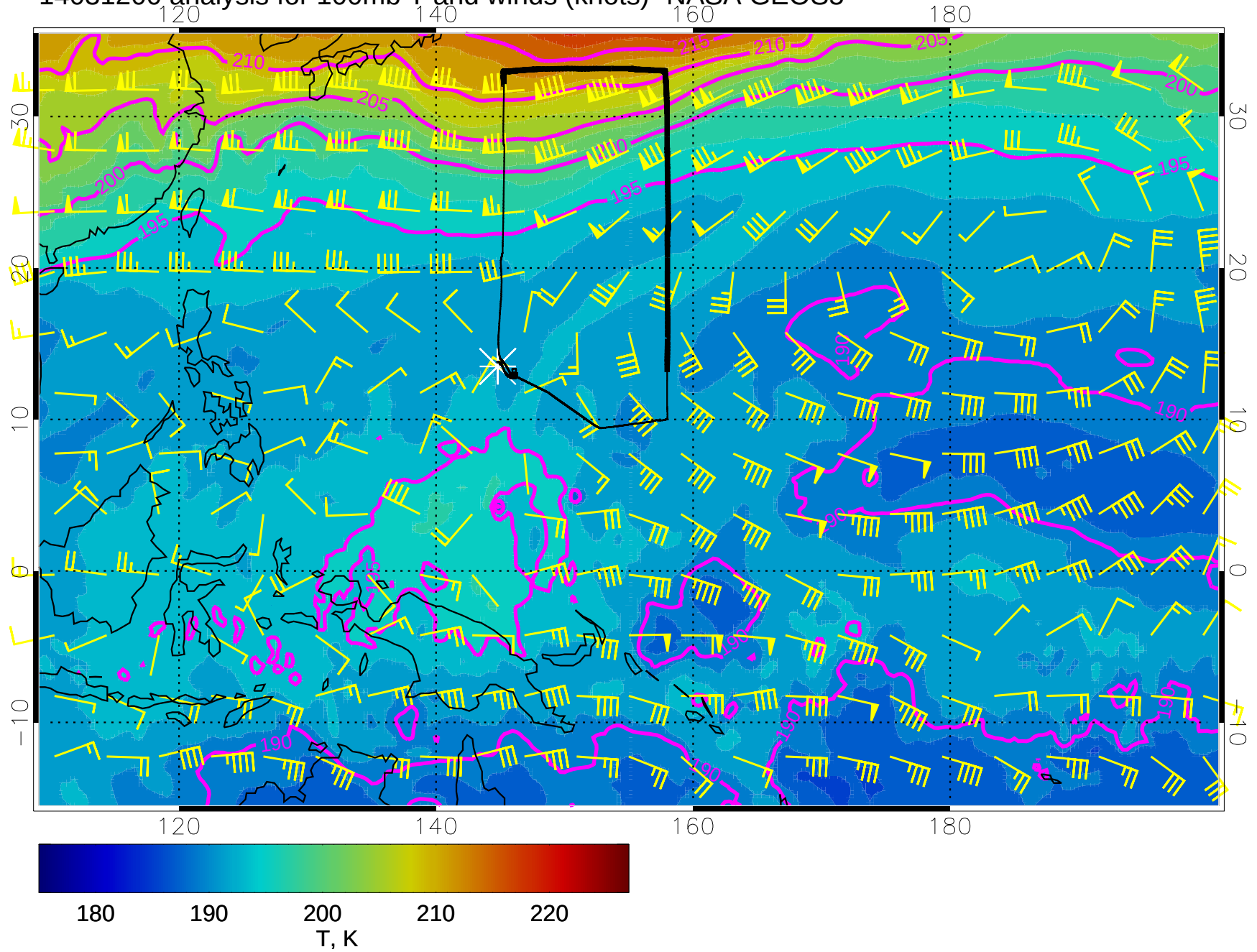
14031200 analysis for 100mb T and winds (knots)- NASA GEOS5
