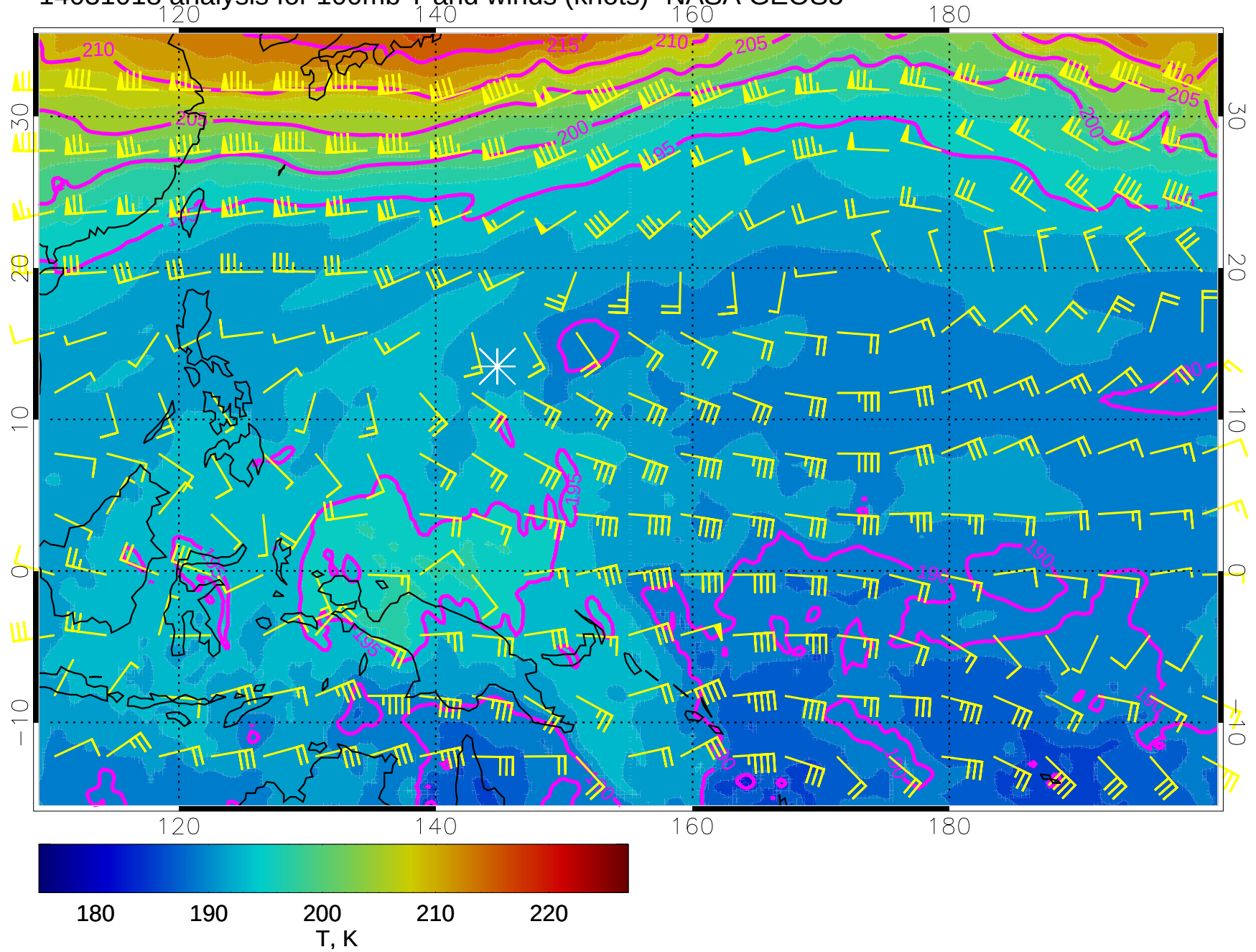
14031018 analysis for 100mb T and winds (knots)- NASA GEOS5
