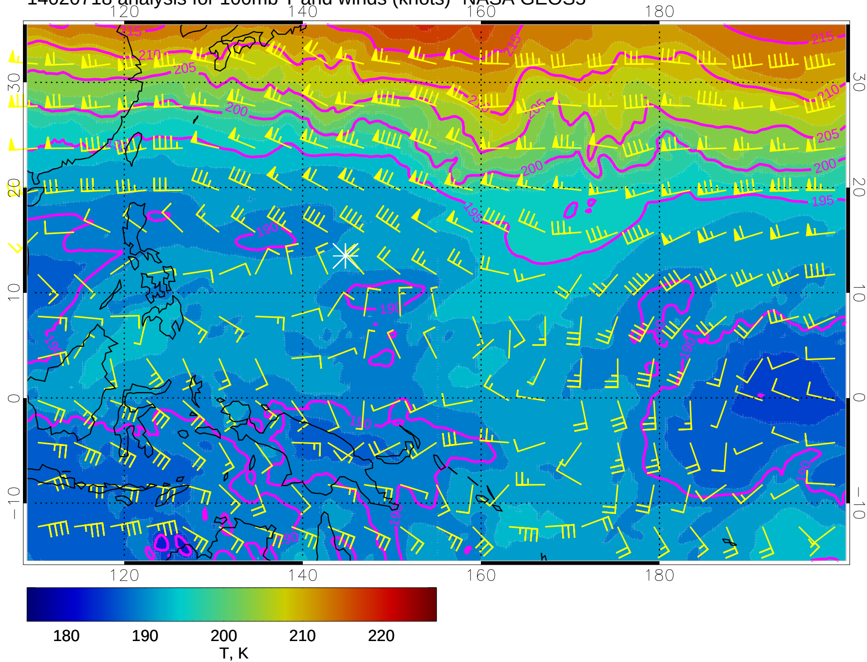
14020718 analysis for 100mb T and winds (knots)- NASA GEOS5
