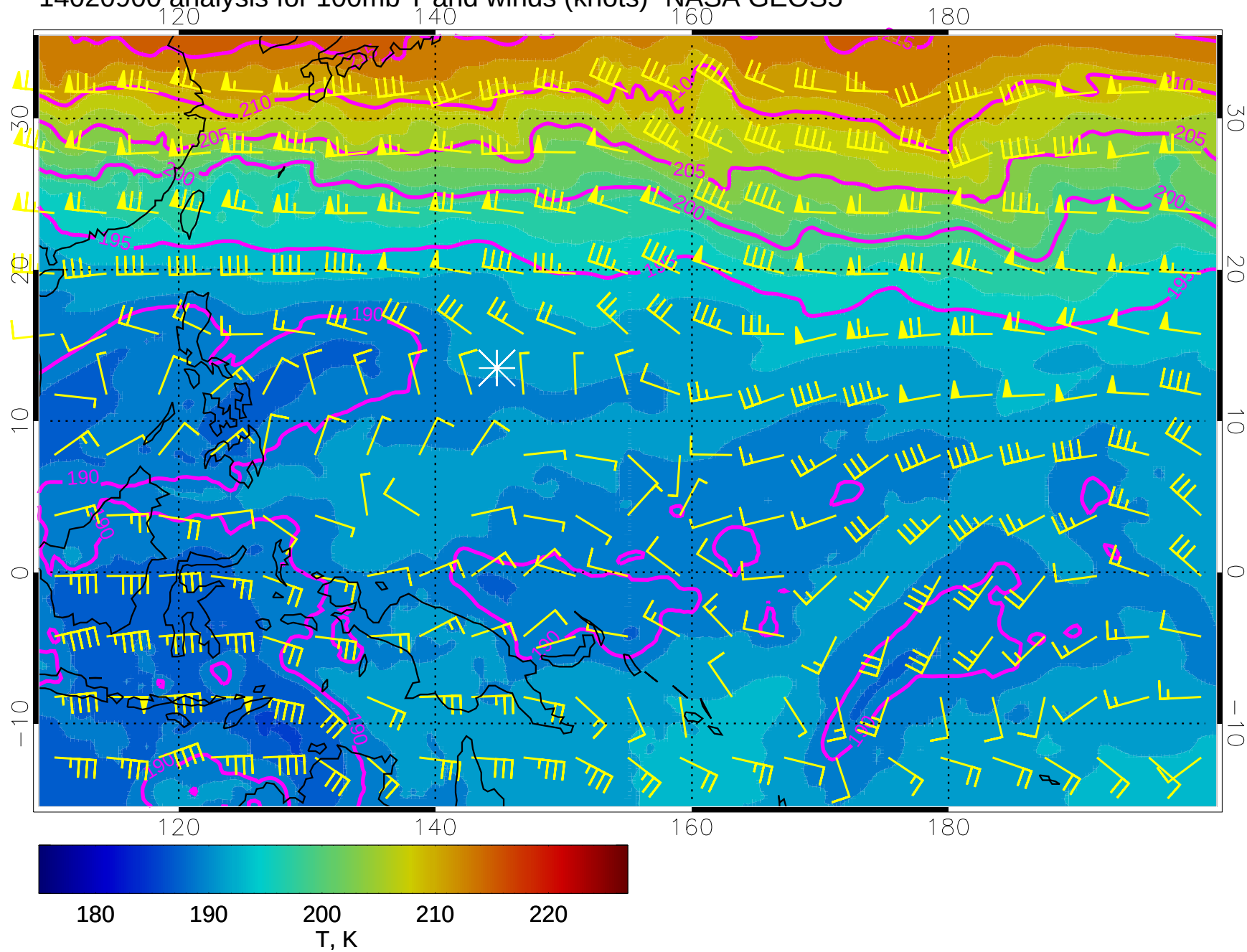
14020900 analysis for 100mb T and winds (knots)- NASA GEOS5
