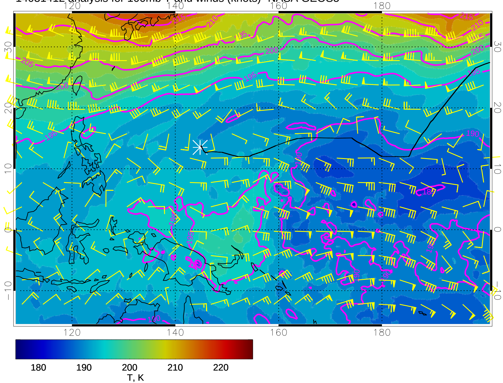
14031412 analysis for 100mb T and winds (knots)- NASA GEOS5
