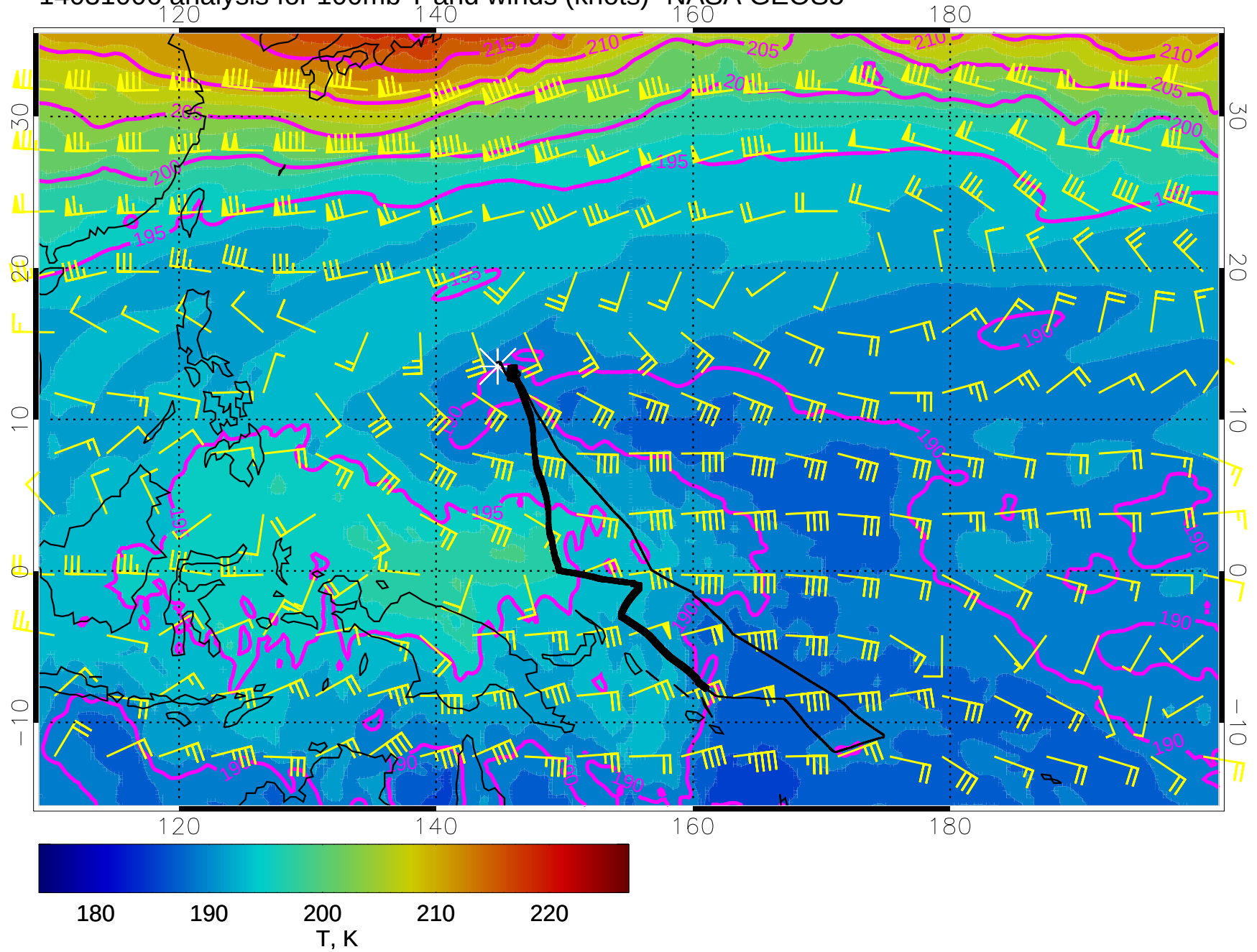
14031006 analysis for 100mb T and winds (knots)- NASA GEOS5
