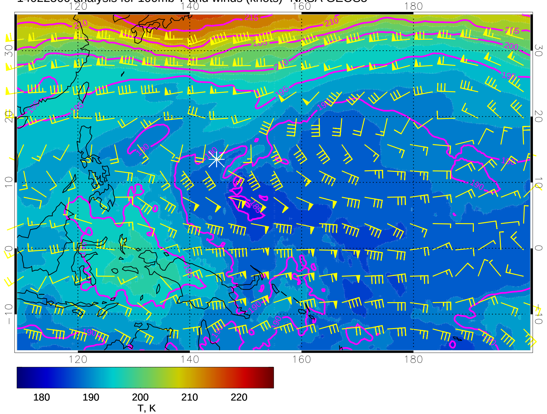
14022500 analysis for 100mb T and winds (knots)- NASA GEOS5
