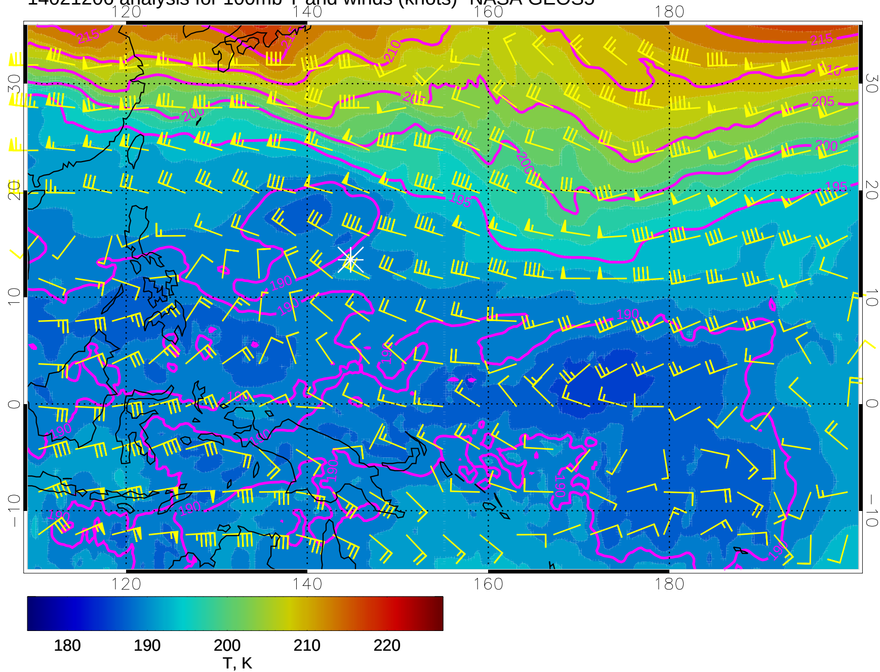
14021206 analysis for 100mb T and winds (knots)- NASA GEOS5
