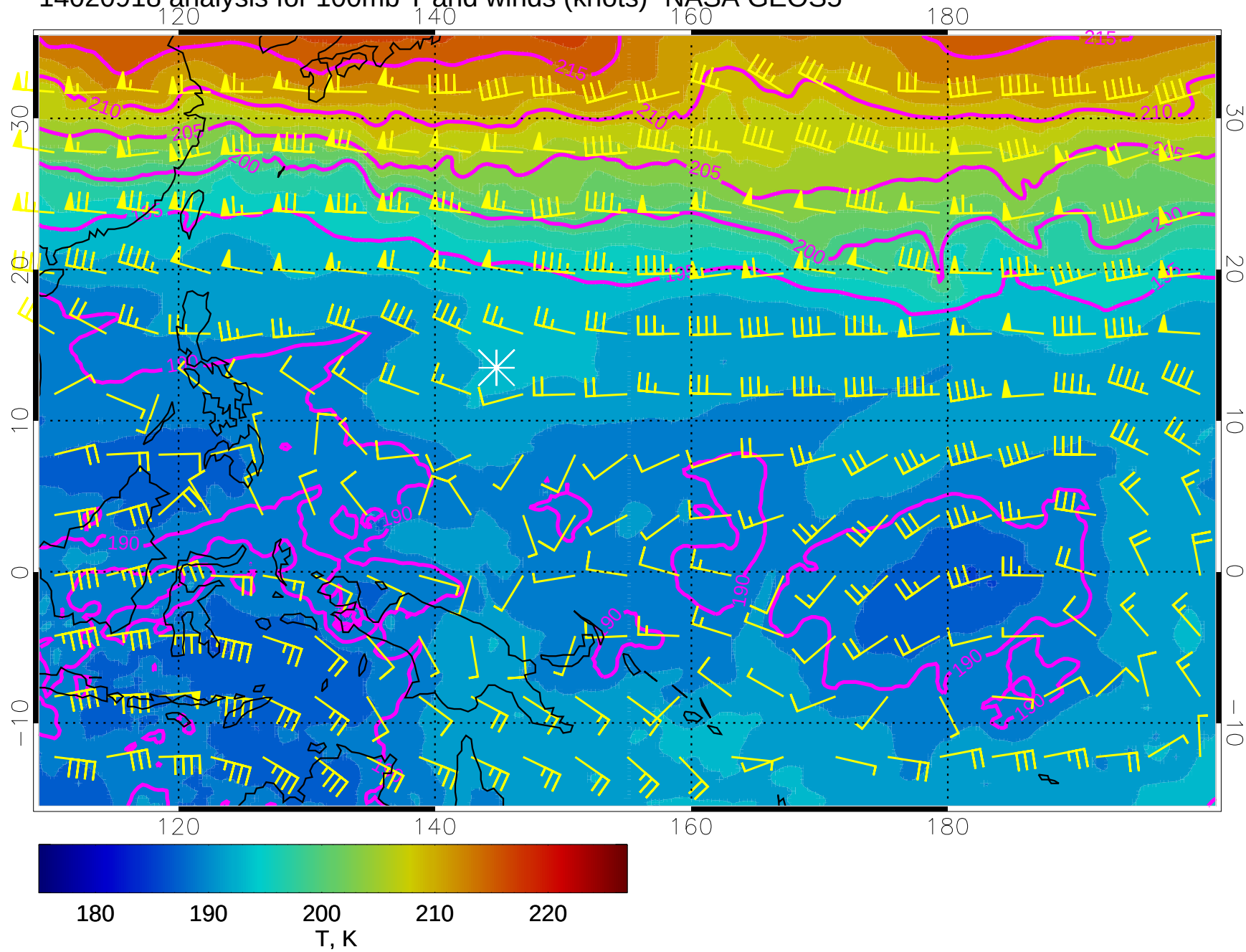
14020918 analysis for 100mb T and winds (knots)- NASA GEOS5
