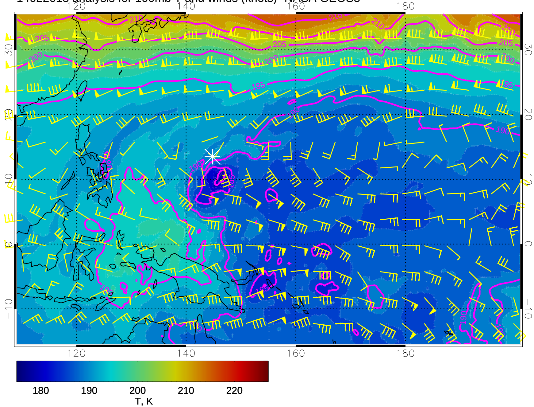
14022618 analysis for 100mb T and winds (knots)- NASA GEOS5
