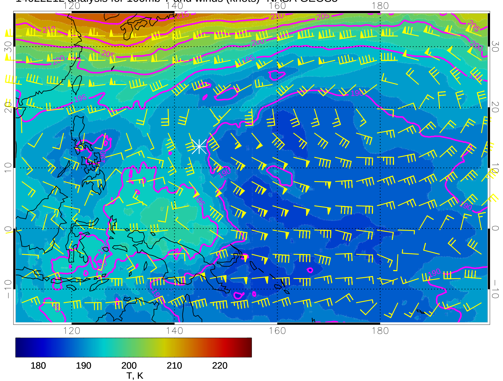
14022212 analysis for 100mb T and winds (knots)- NASA GEOS5
