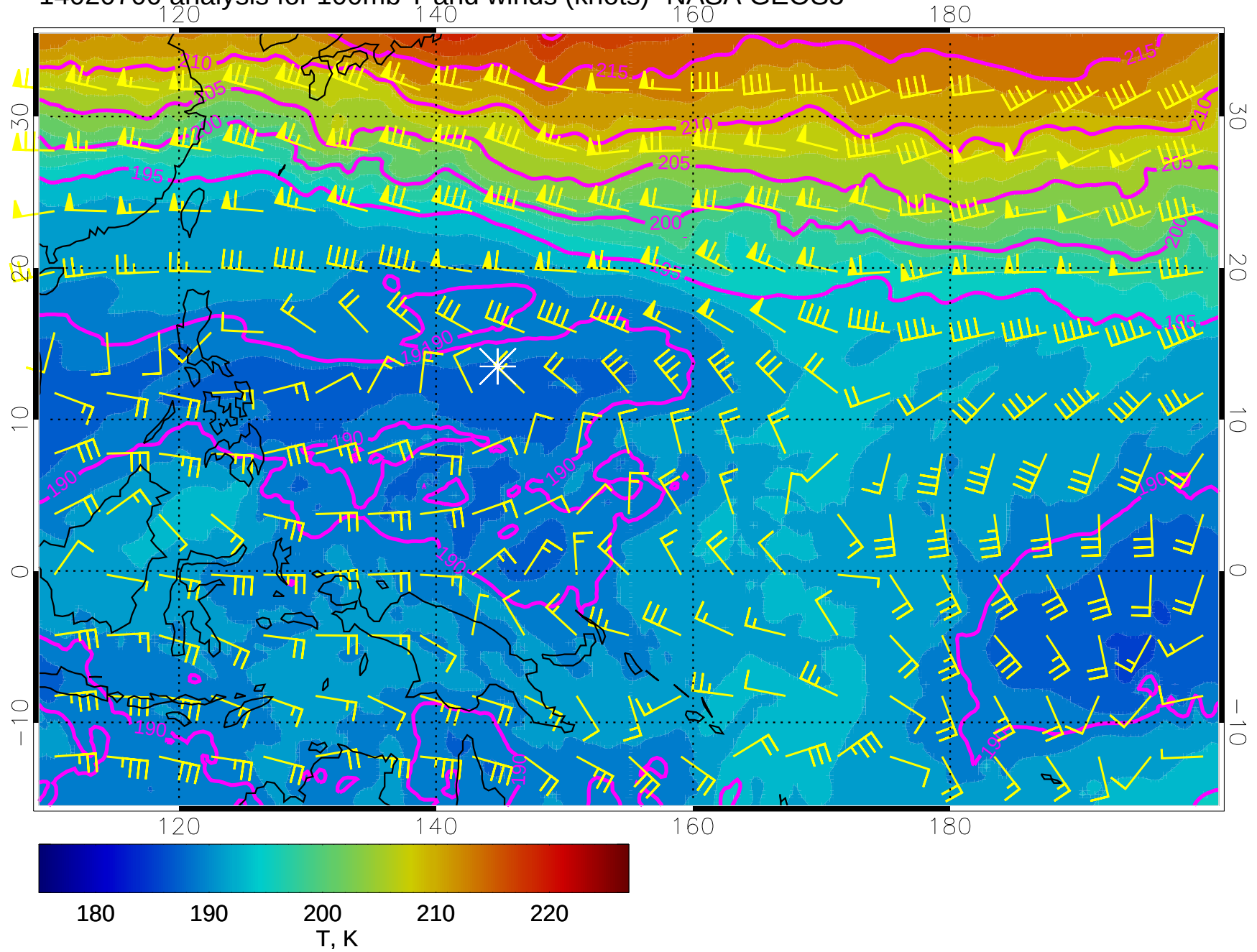
14020700 analysis for 100mb T and winds (knots)- NASA GEOS5
