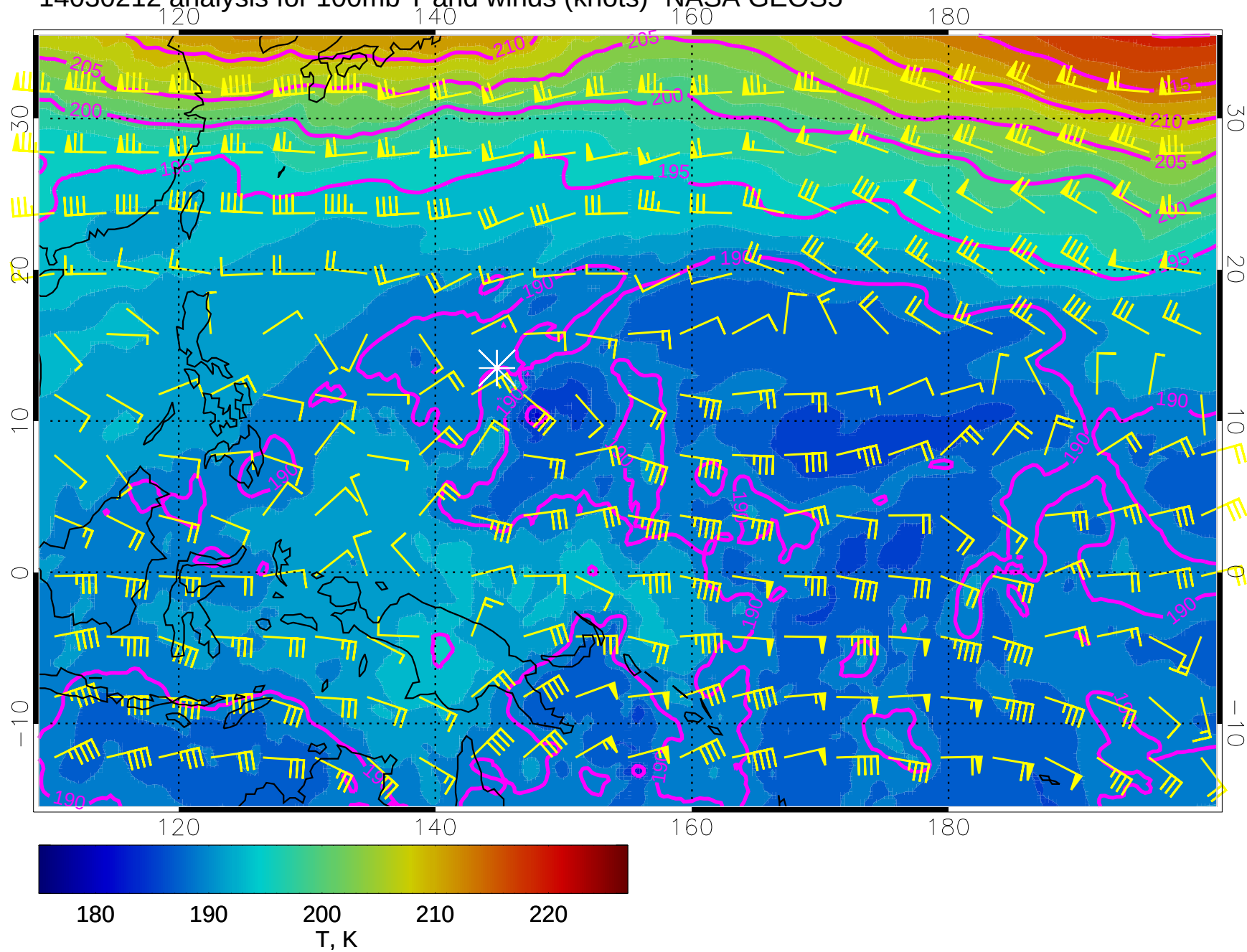
14030212 analysis for 100mb T and winds (knots)- NASA GEOS5
