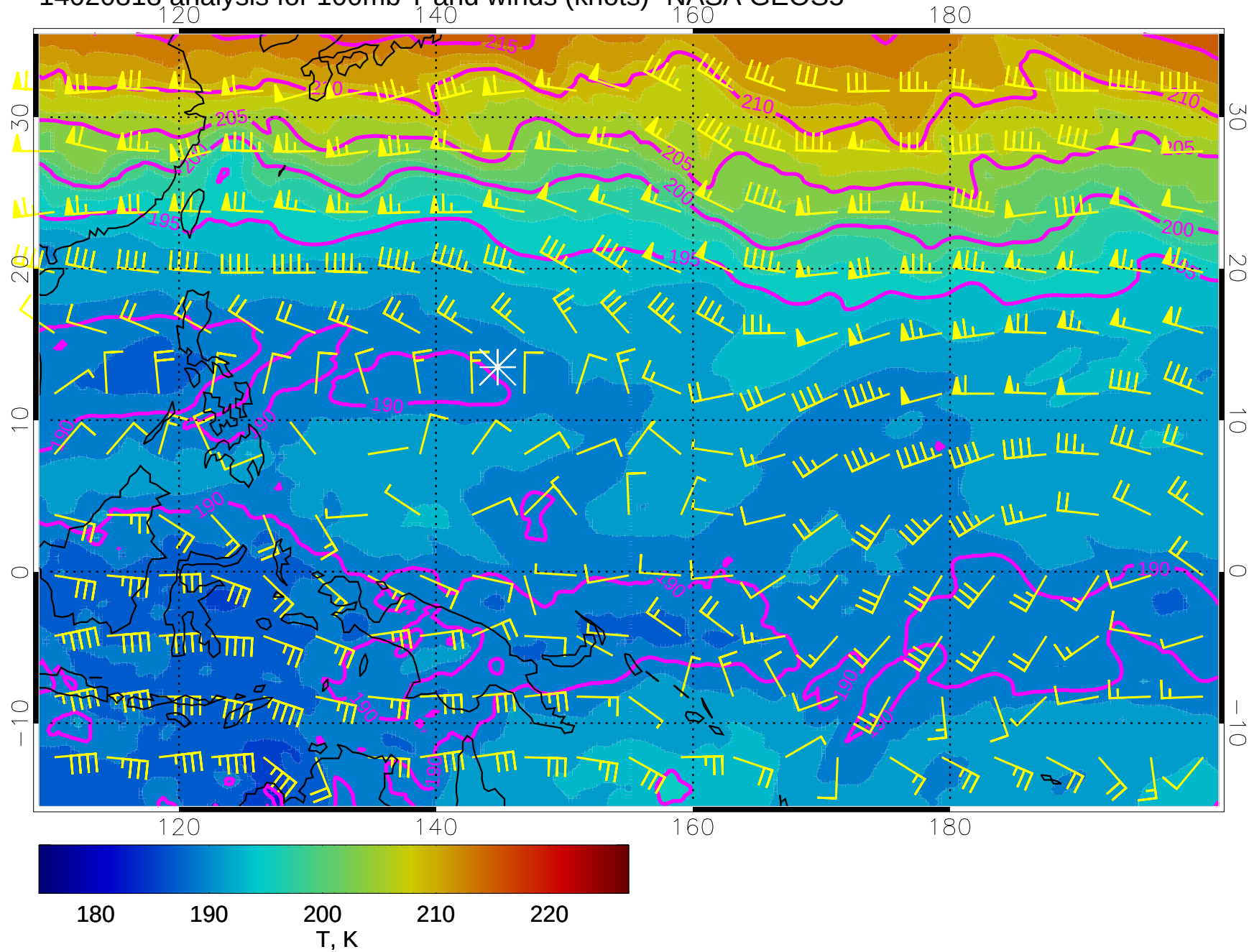
14020818 analysis for 100mb T and winds (knots)- NASA GEOS5
