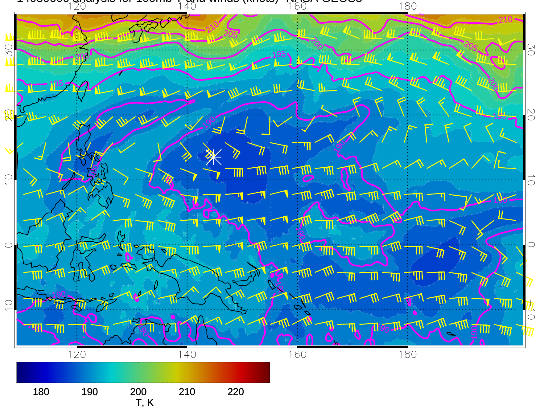
14030600 analysis for 100mb T and winds (knots)- NASA GEOS5
