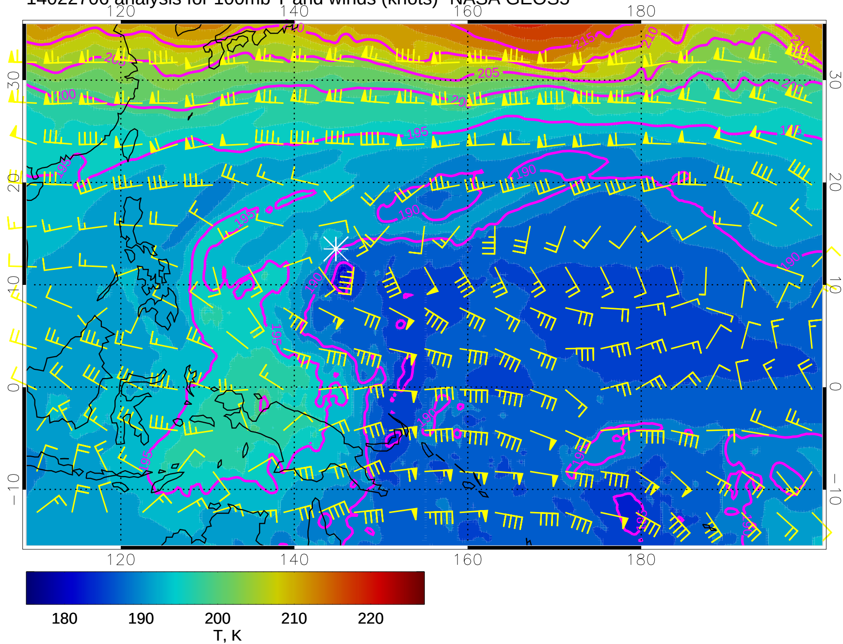
14022706 analysis for 100mb T and winds (knots)- NASA GEOS5
