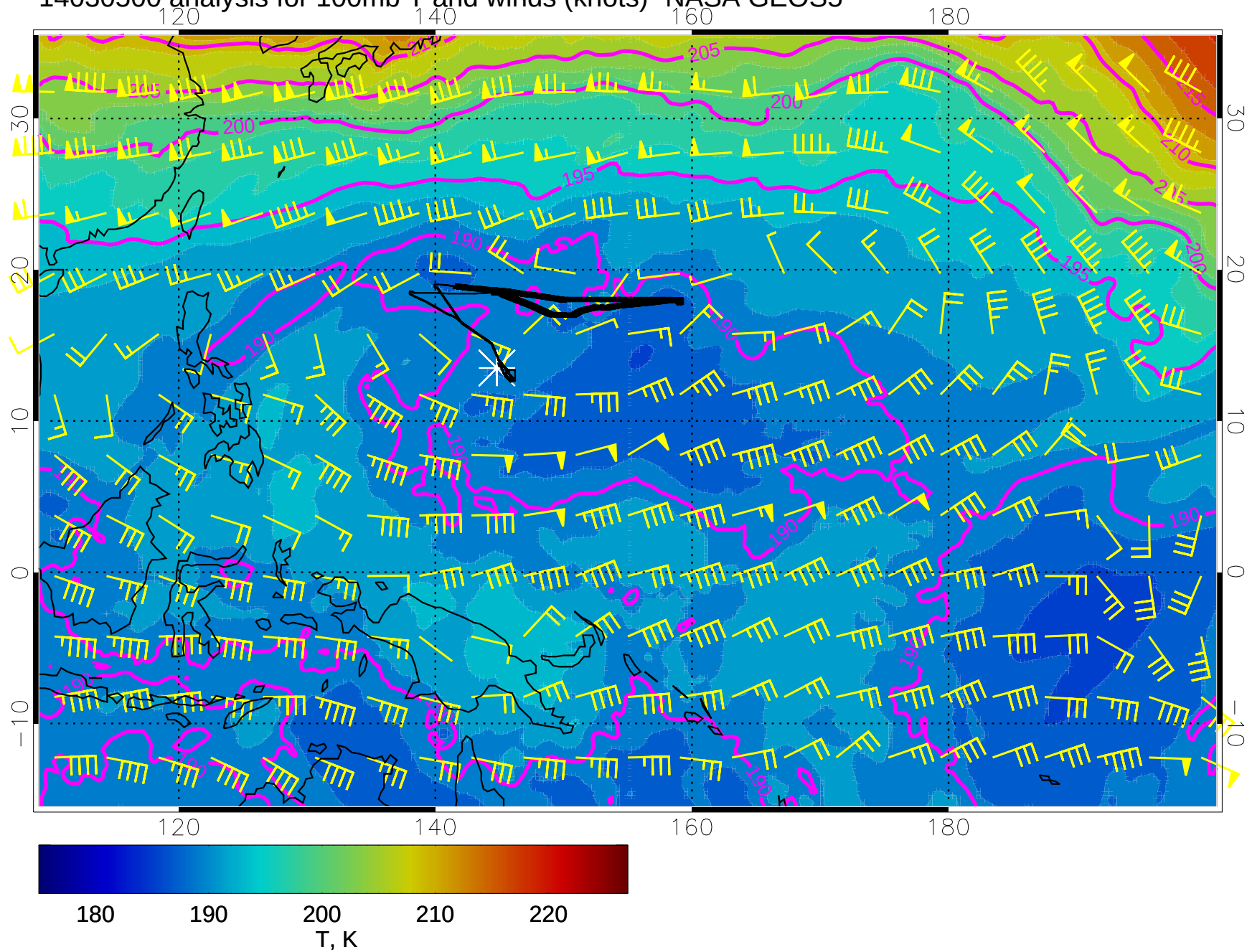
14030500 analysis for 100mb T and winds (knots)- NASA GEOS5
