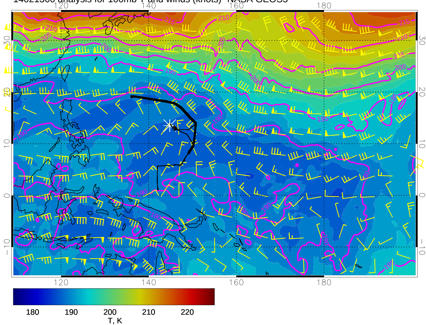
14021300 analysis for 100mb T and winds (knots)- NASA GEOS5
