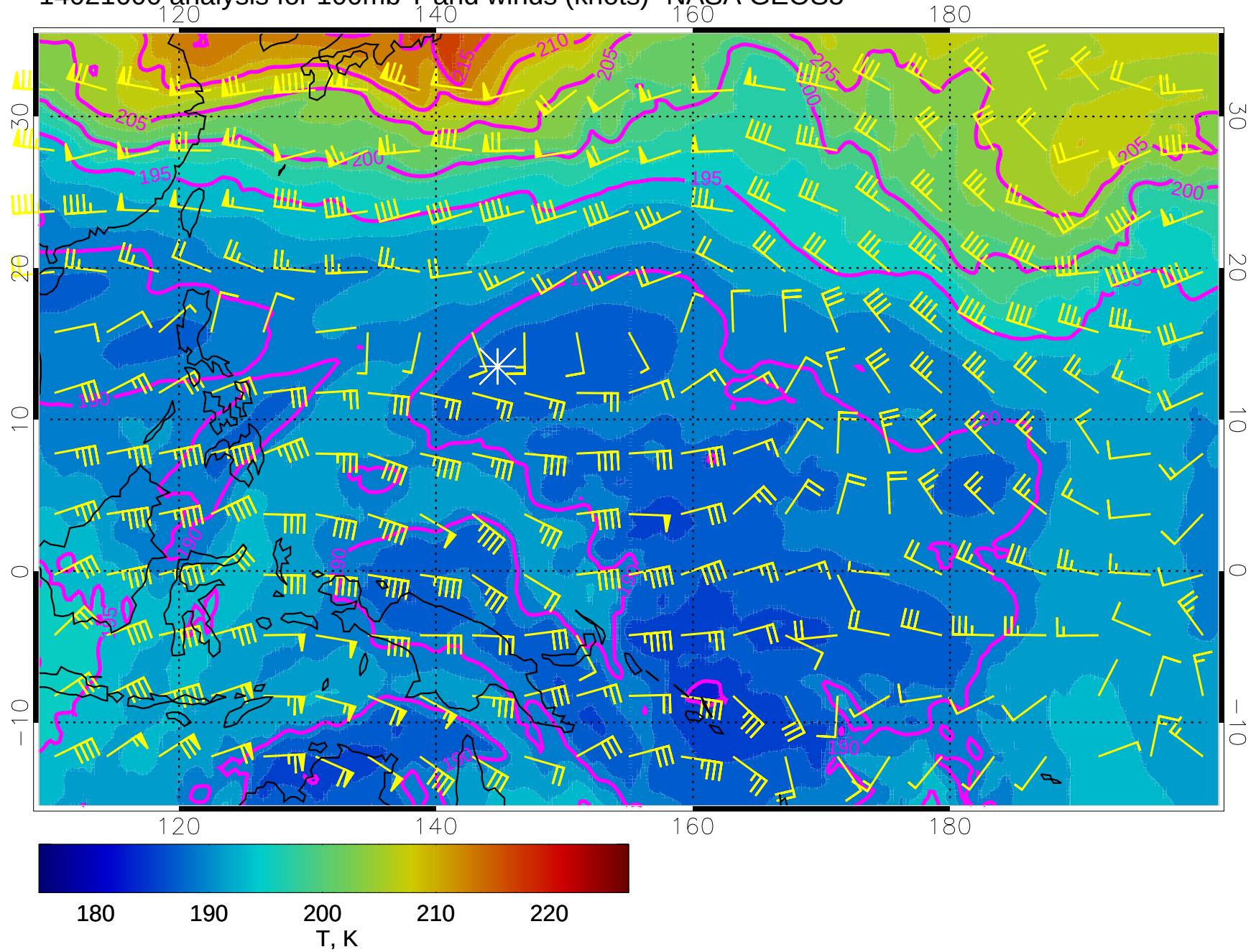
14021600 analysis for 100mb T and winds (knots)- NASA GEOS5
