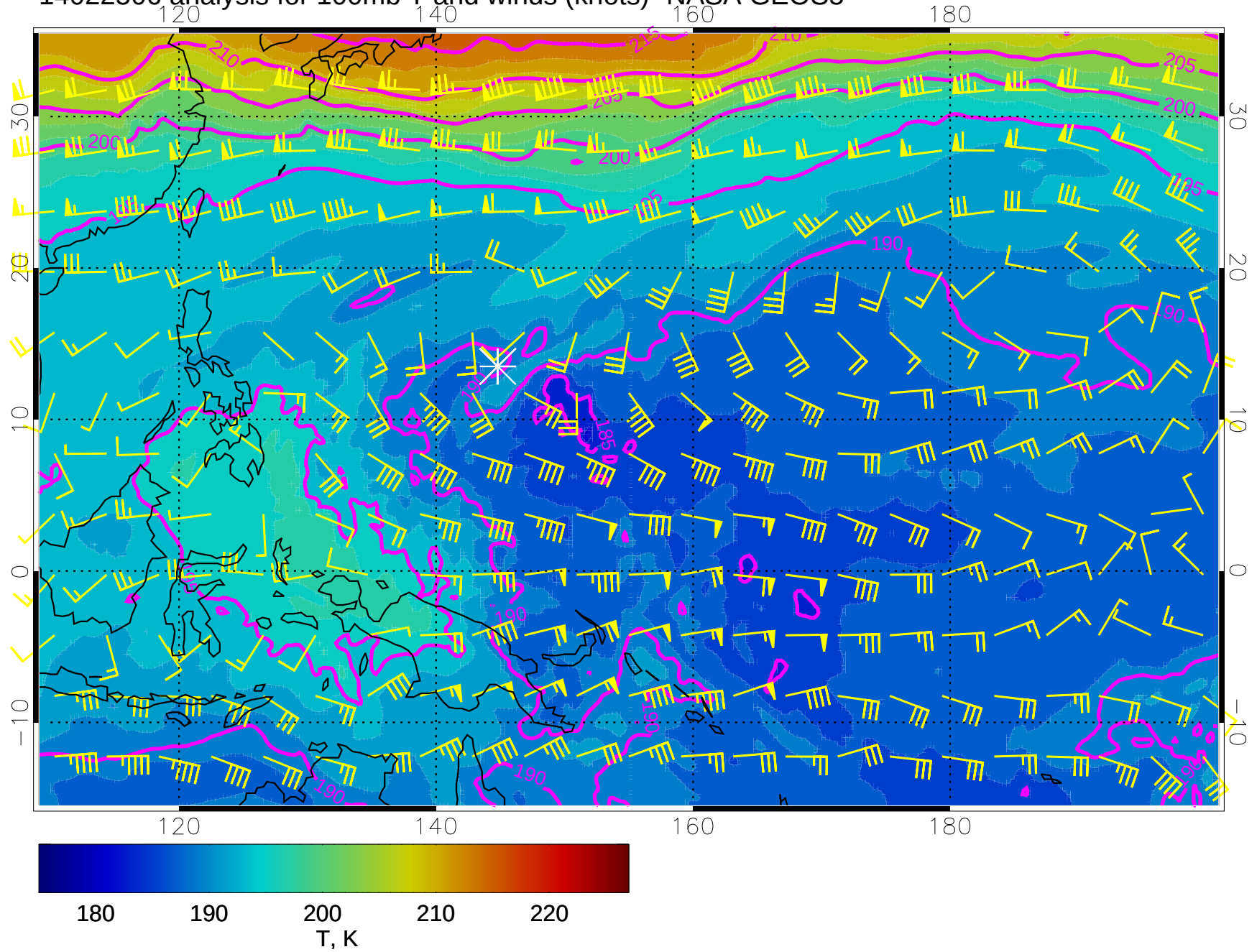
14022506 analysis for 100mb T and winds (knots)- NASA GEOS5
