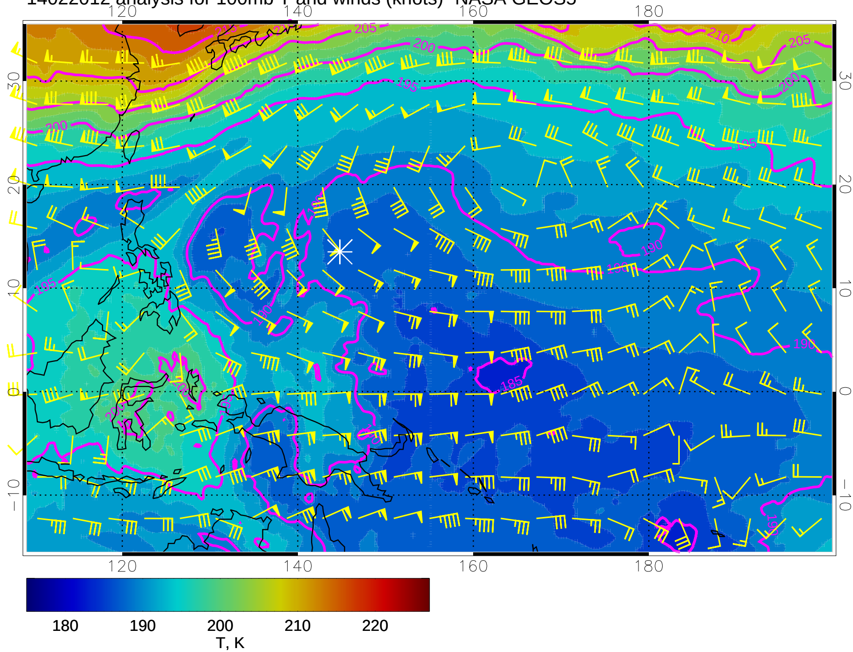
14022012 analysis for 100mb T and winds (knots)- NASA GEOS5
