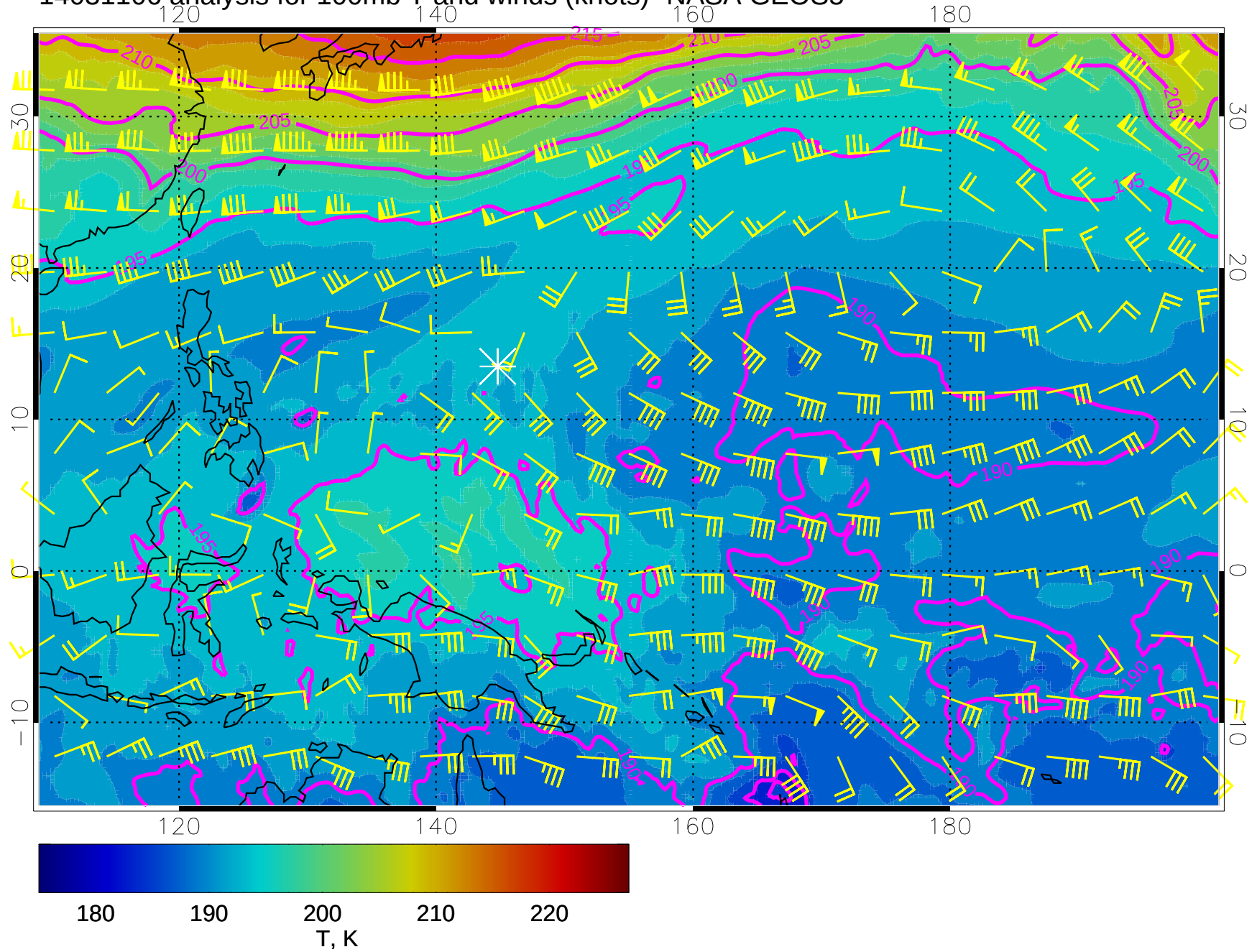
14031106 analysis for 100mb T and winds (knots)- NASA GEOS5
