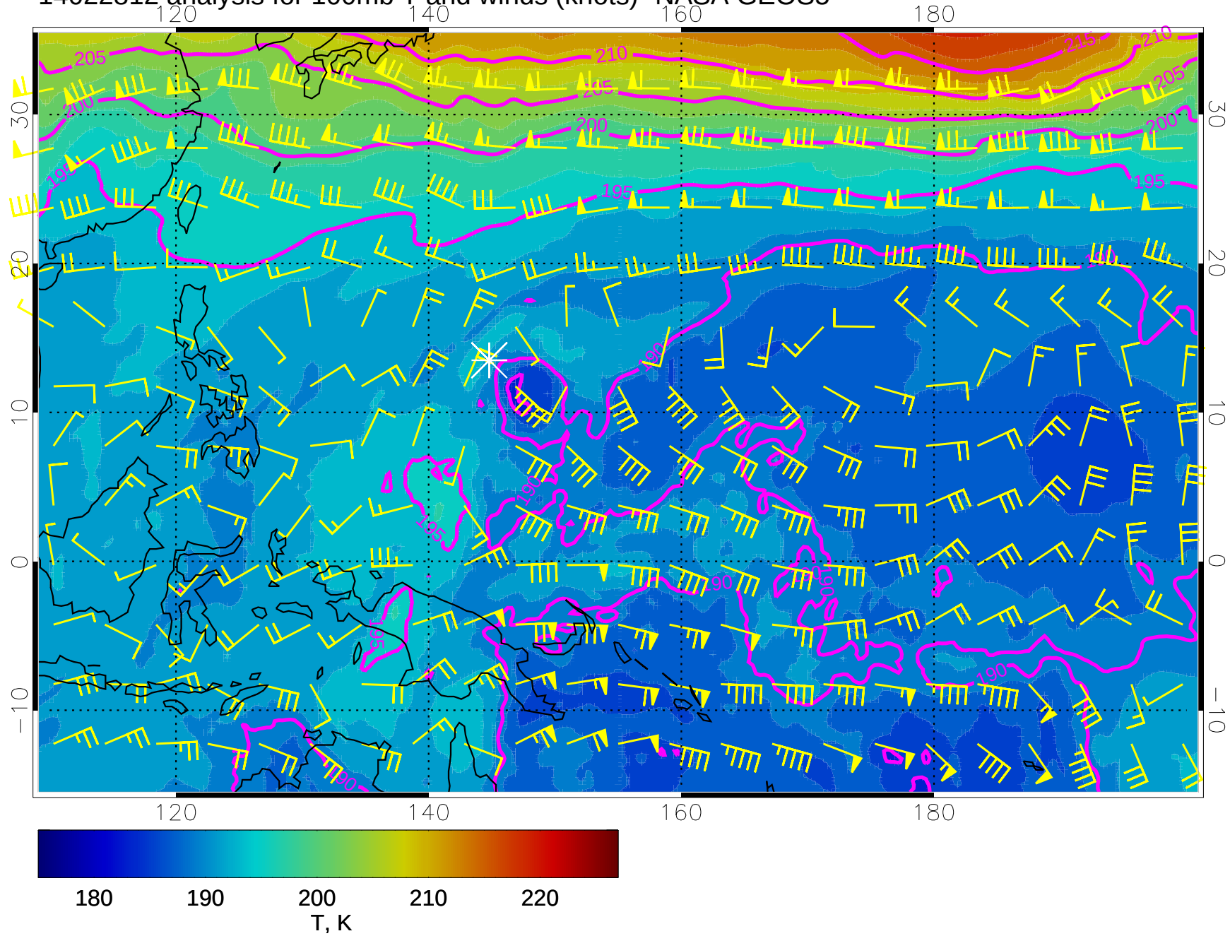
14022812 analysis for 100mb T and winds (knots)- NASA GEOS5
