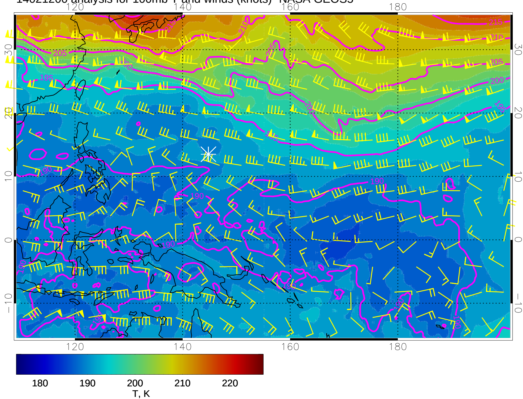
14021200 analysis for 100mb T and winds (knots)- NASA GEOS5
