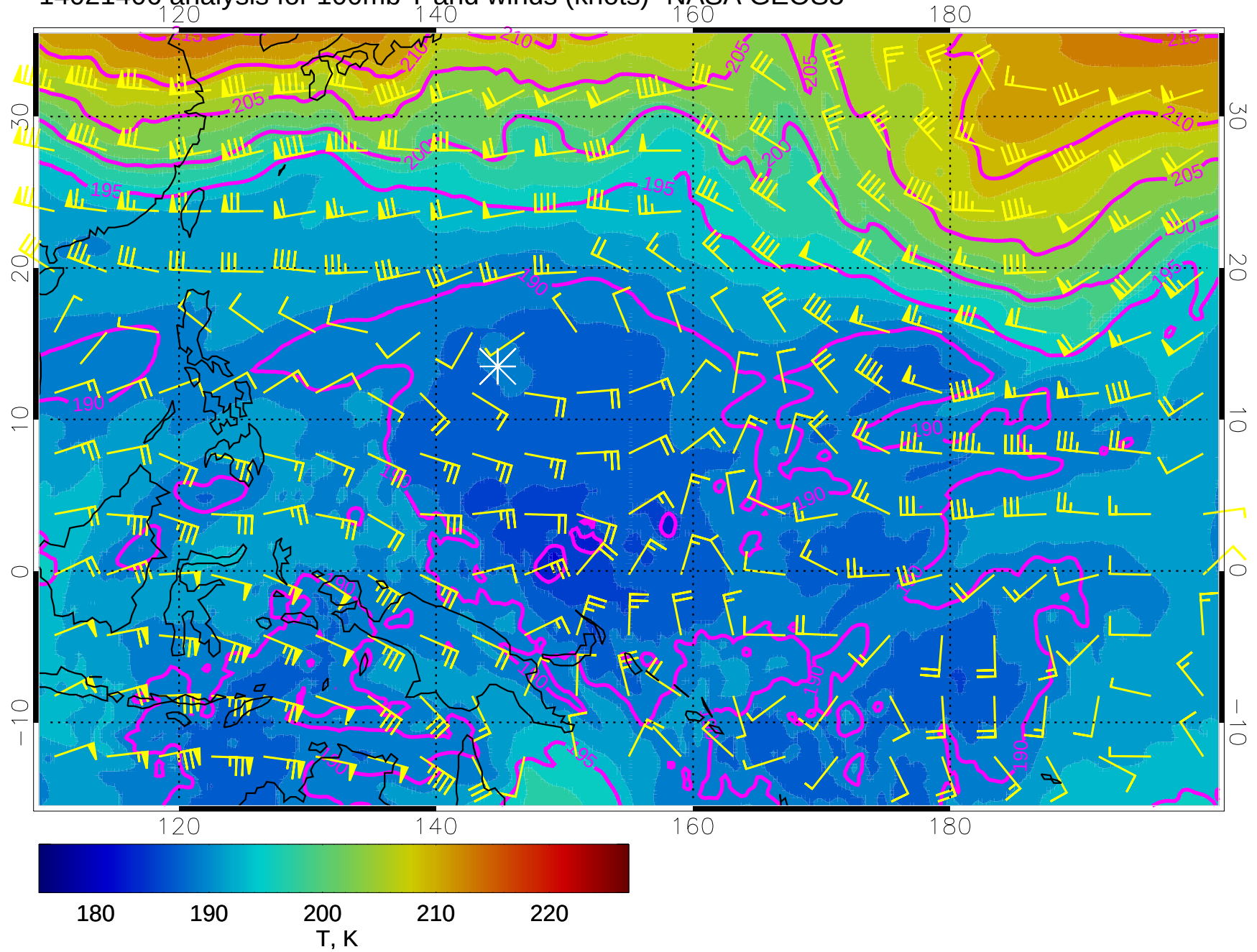
14021406 analysis for 100mb T and winds (knots)- NASA GEOS5
