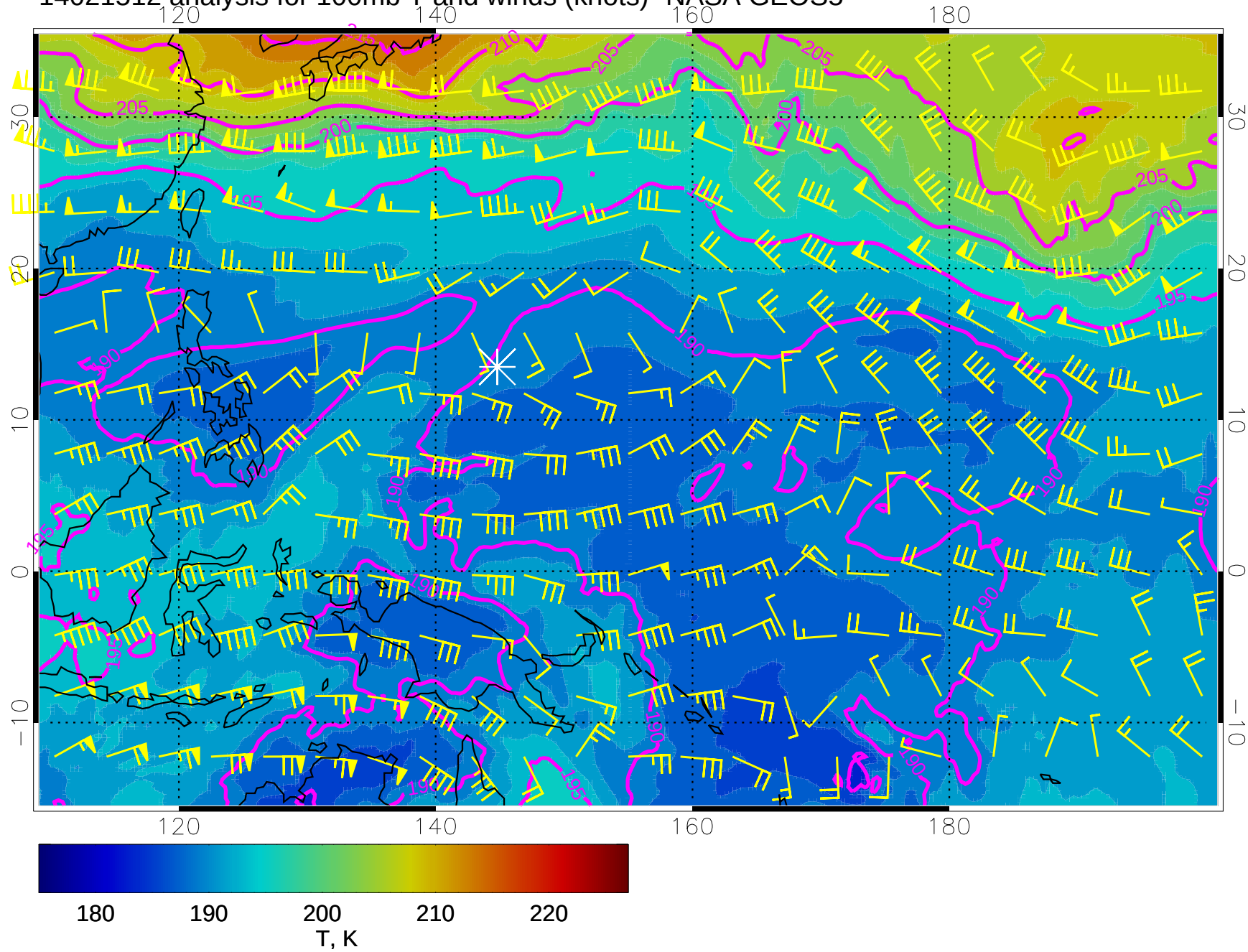
14021512 analysis for 100mb T and winds (knots)- NASA GEOS5
