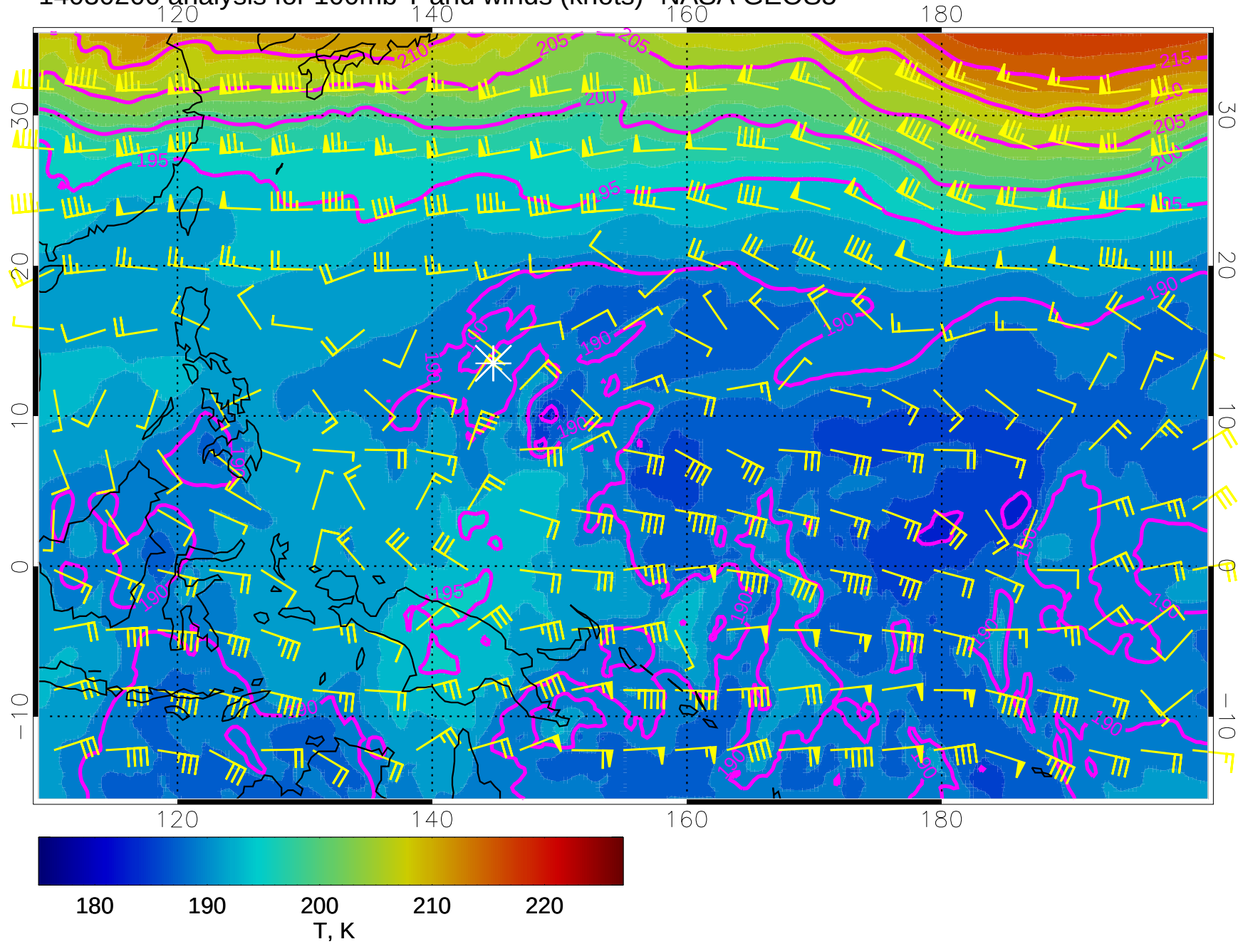
14030200 analysis for 100mb T and winds (knots)- NASA GEOS5
