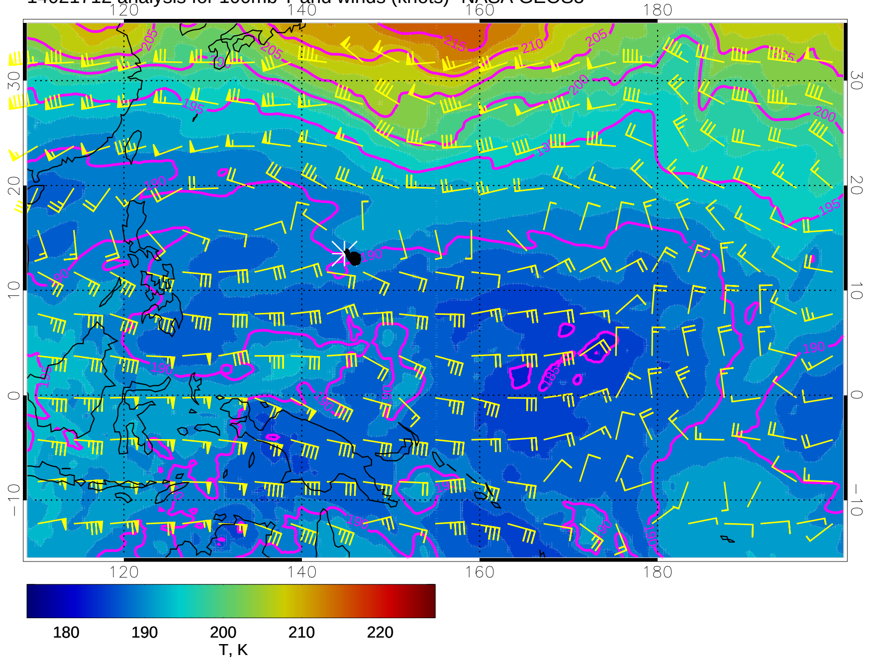
14021712 analysis for 100mb T and winds (knots)- NASA GEOS5
