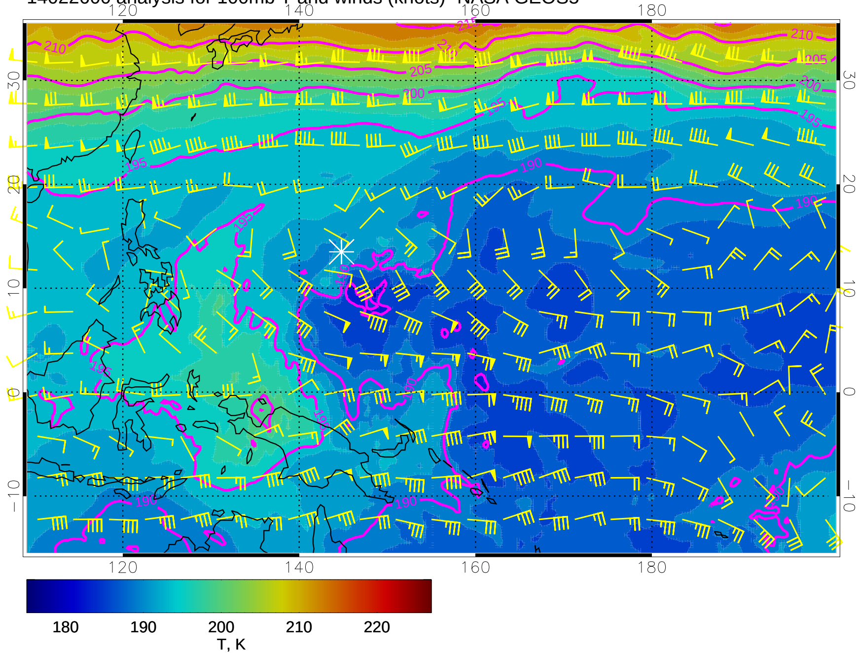
14022600 analysis for 100mb T and winds (knots)- NASA GEOS5
