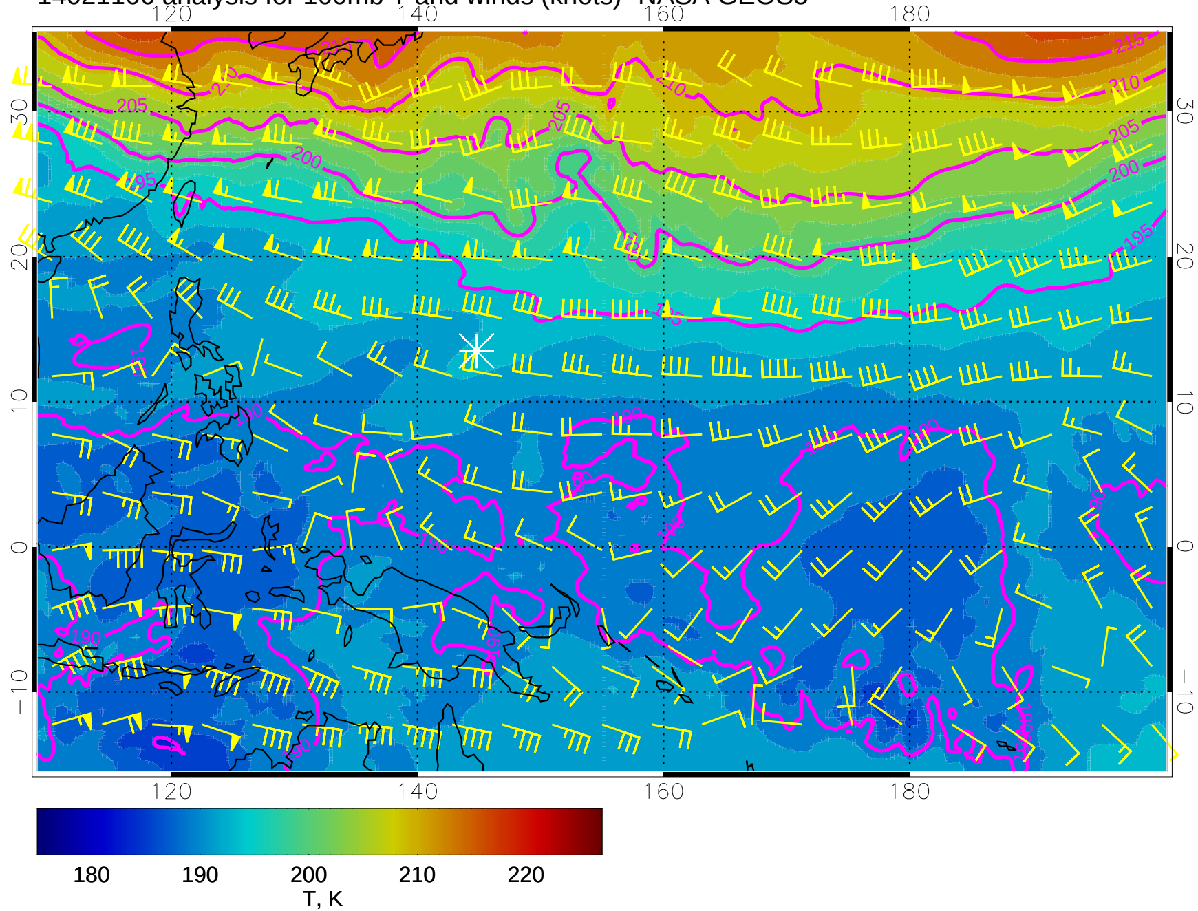
14021106 analysis for 100mb T and winds (knots)- NASA GEOS5
