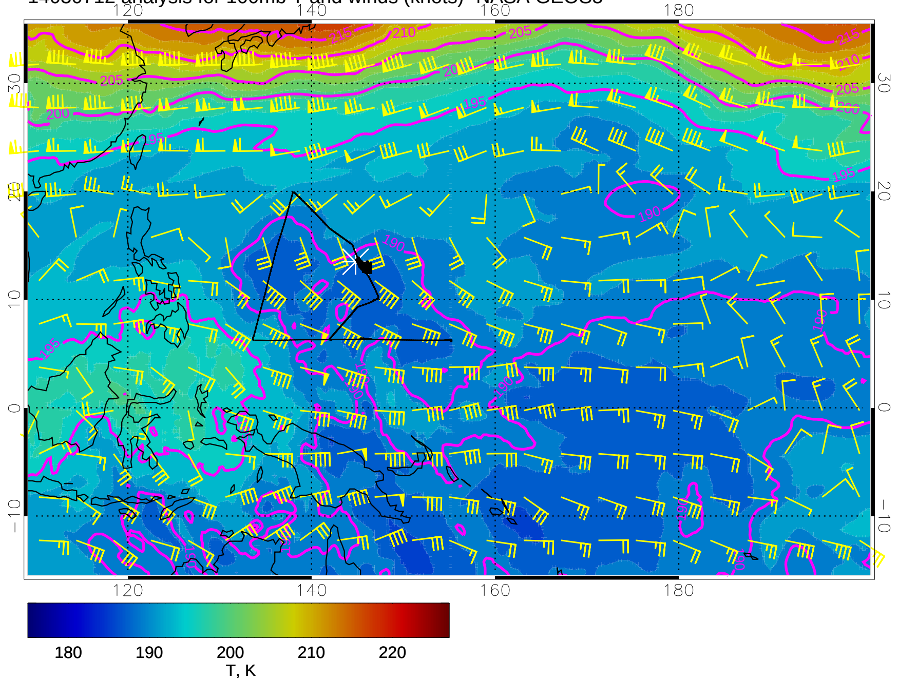
14030712 analysis for 100mb T and winds (knots)- NASA GEOS5
