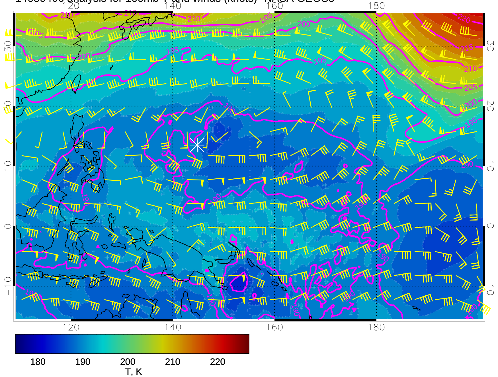
14030406 analysis for 100mb T and winds (knots)- NASA GEOS5
