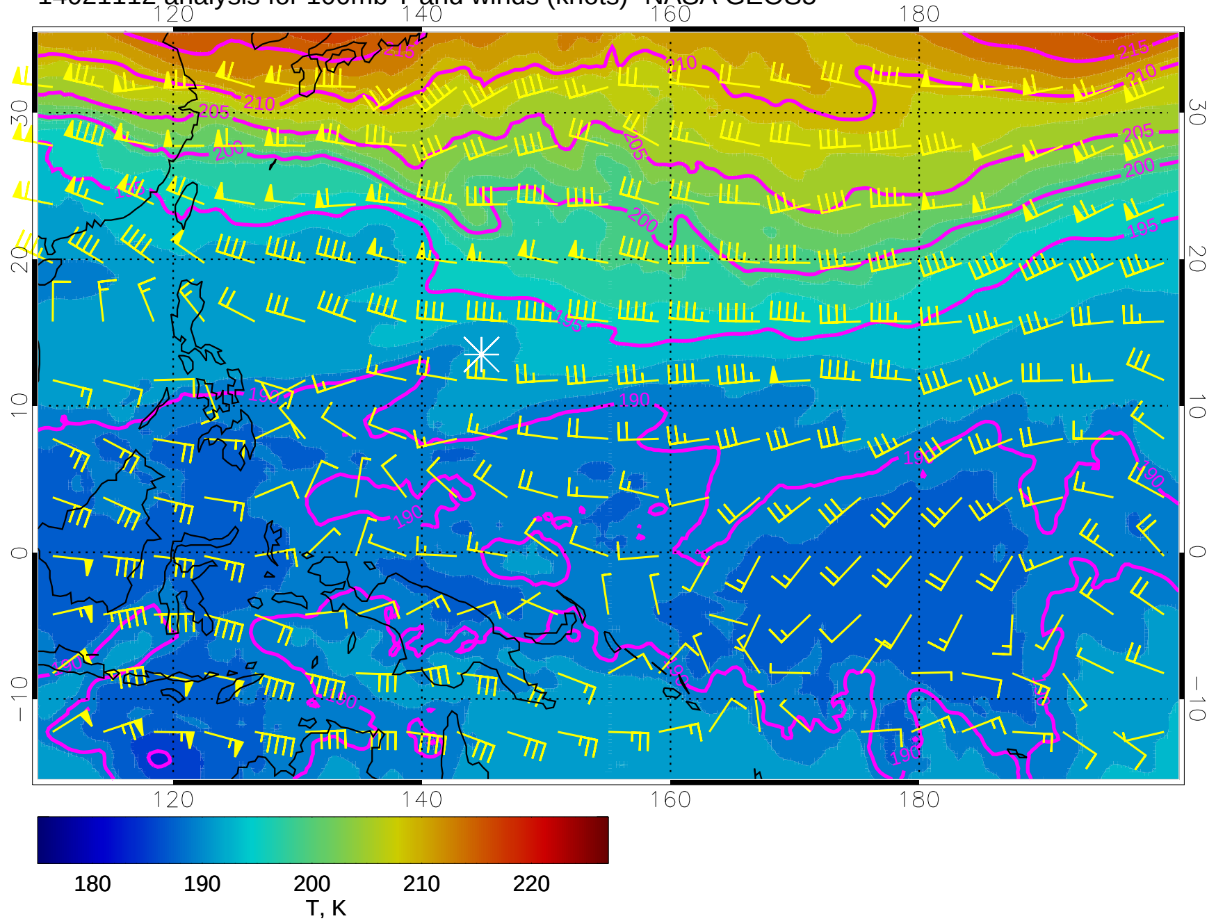
14021112 analysis for 100mb T and winds (knots)- NASA GEOS5
