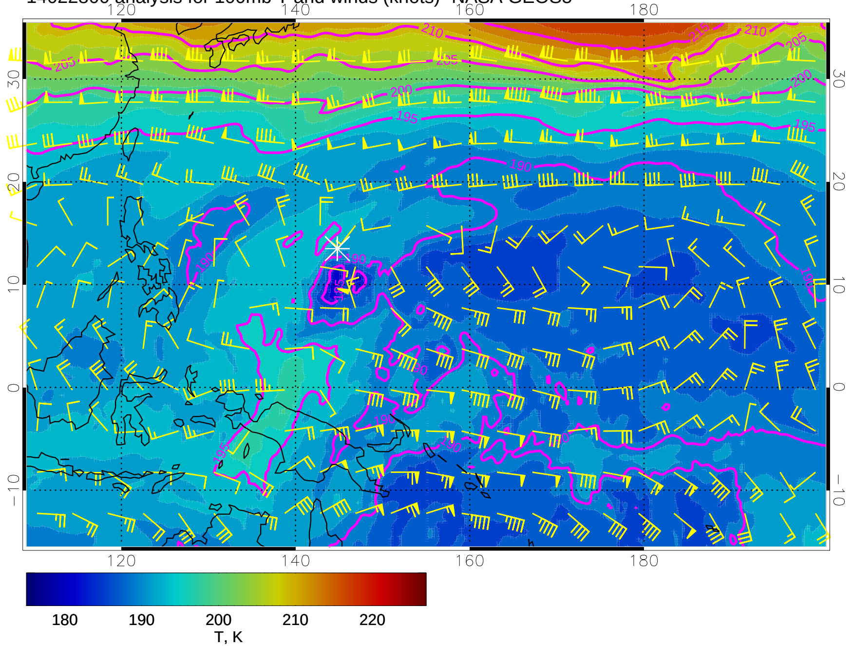
14022800 analysis for 100mb T and winds (knots)- NASA GEOS5
