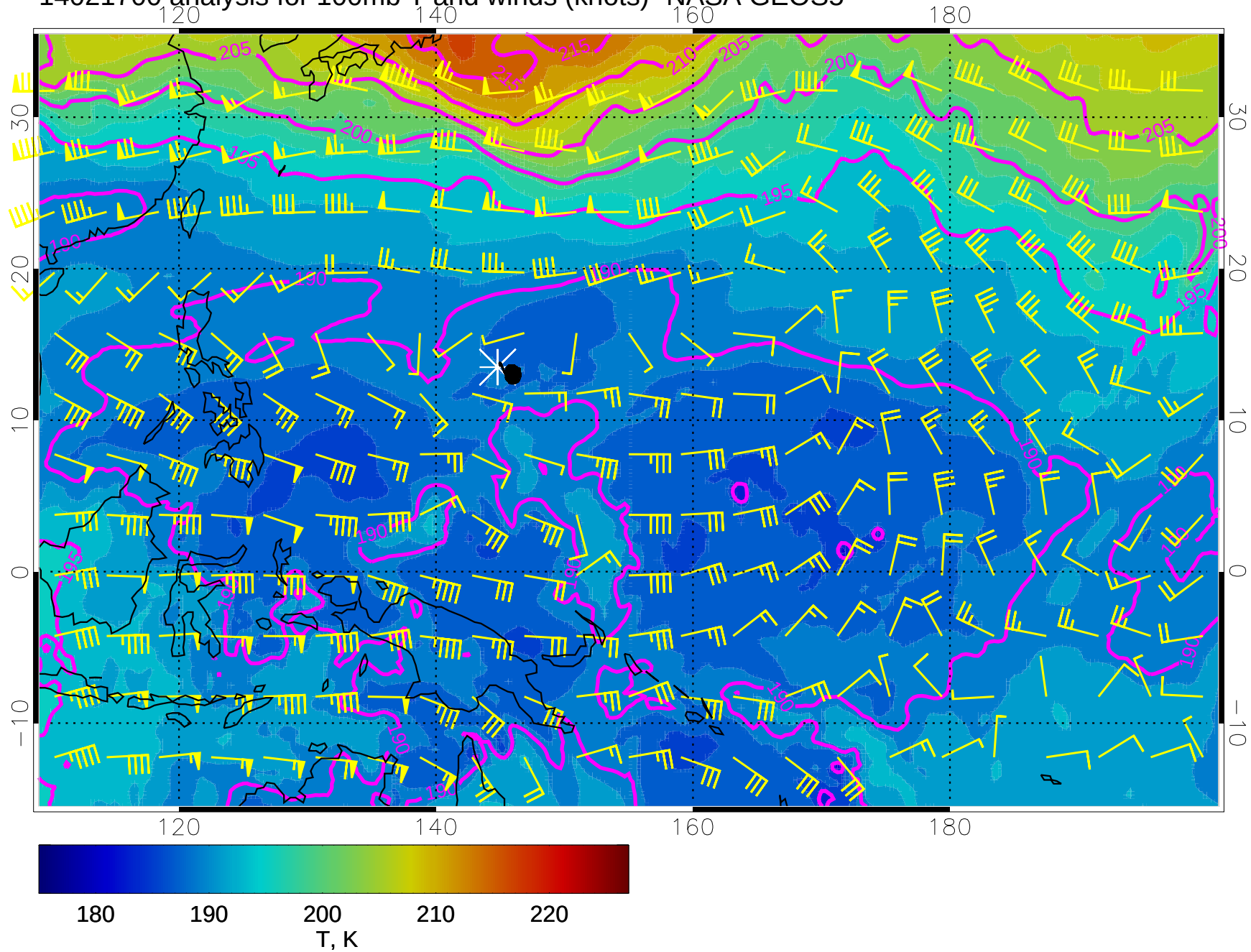
14021700 analysis for 100mb T and winds (knots)- NASA GEOS5
