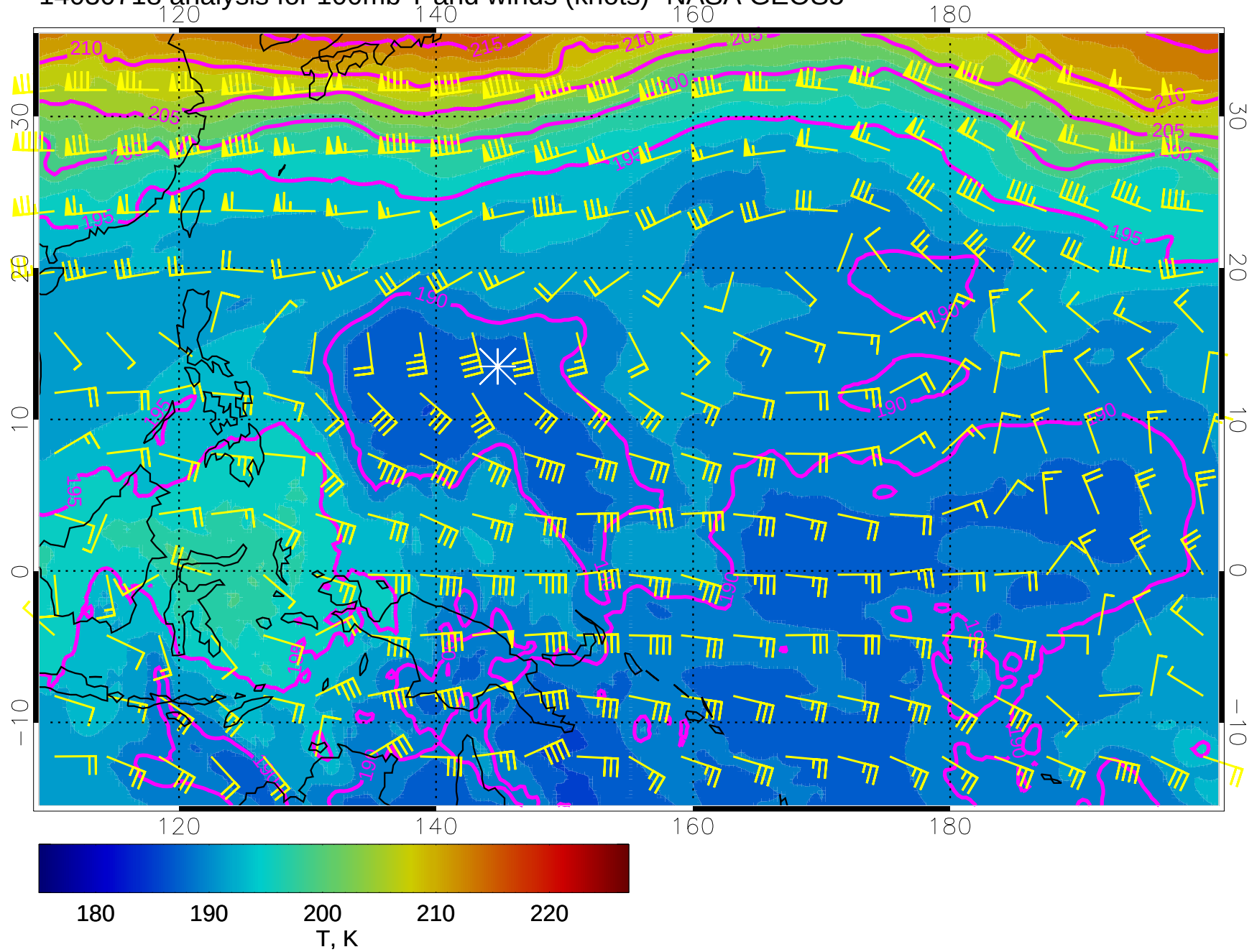
14030718 analysis for 100mb T and winds (knots)- NASA GEOS5
