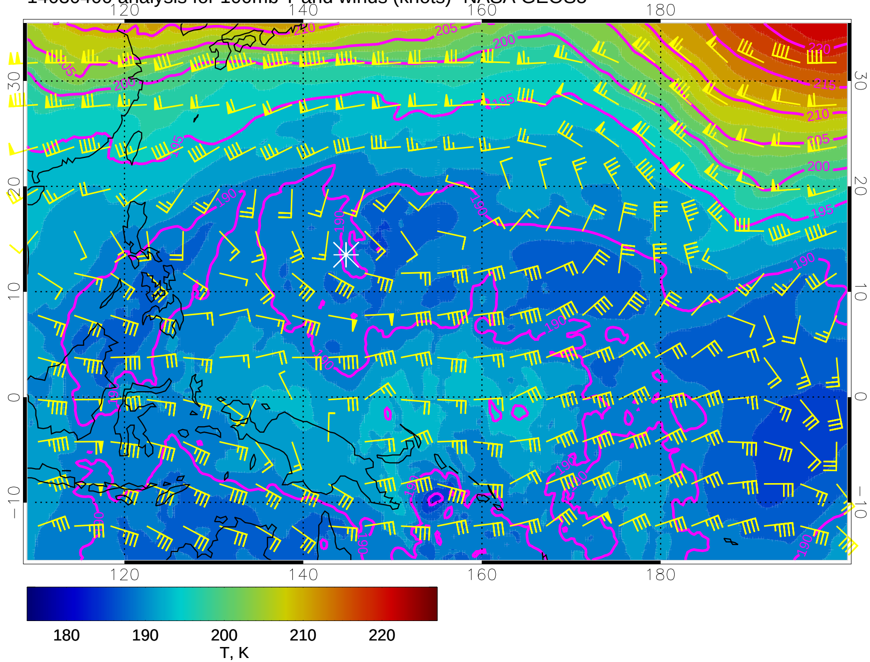
14030400 analysis for 100mb T and winds (knots)- NASA GEOS5
