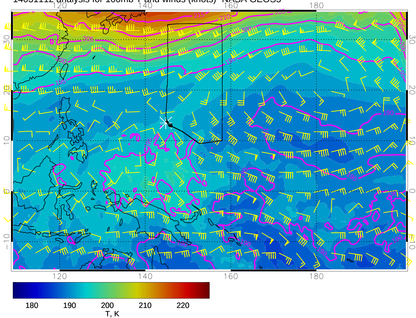
14031112 analysis for 100mb T and winds (knots)- NASA GEOS5
