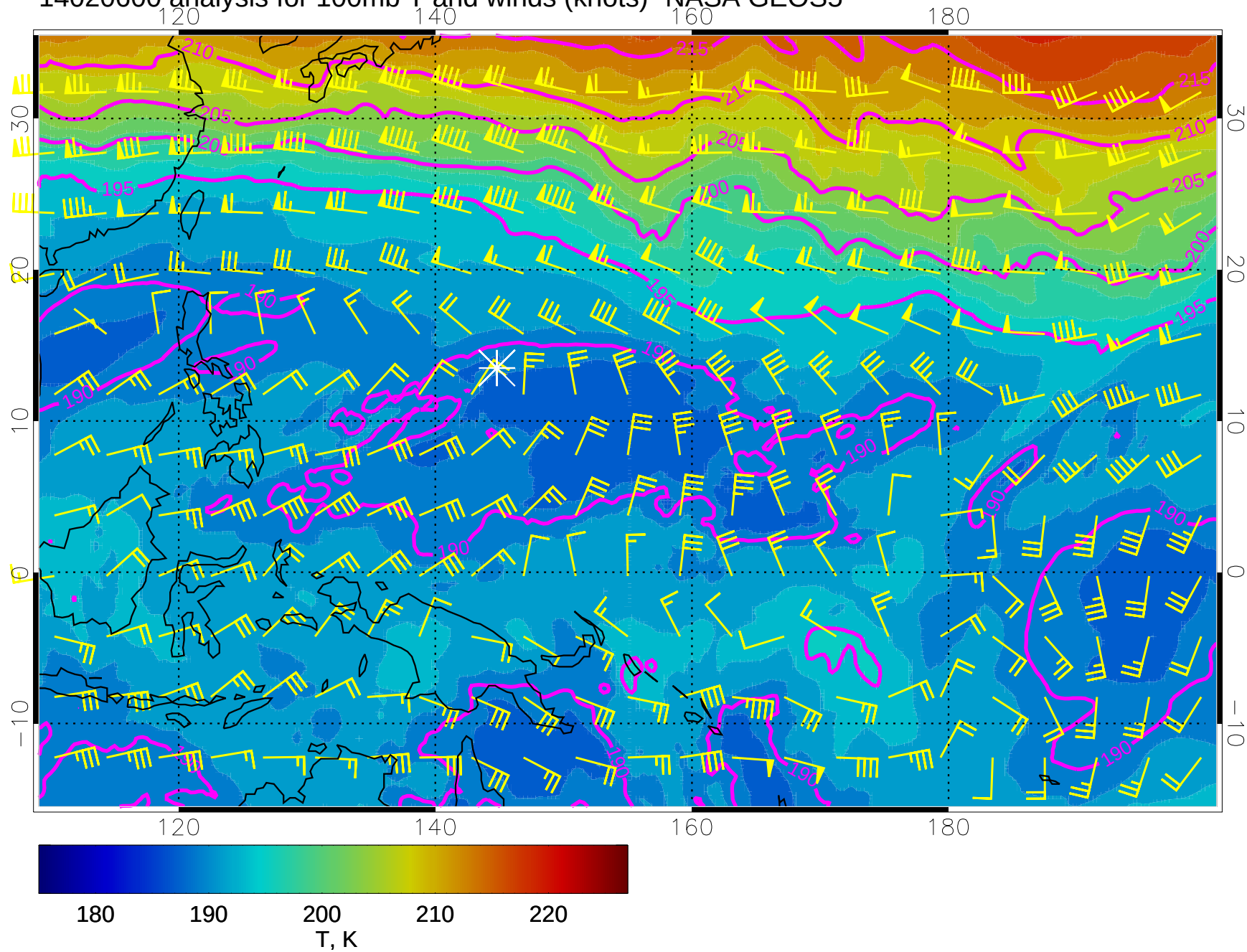
14020600 analysis for 100mb T and winds (knots)- NASA GEOS5
