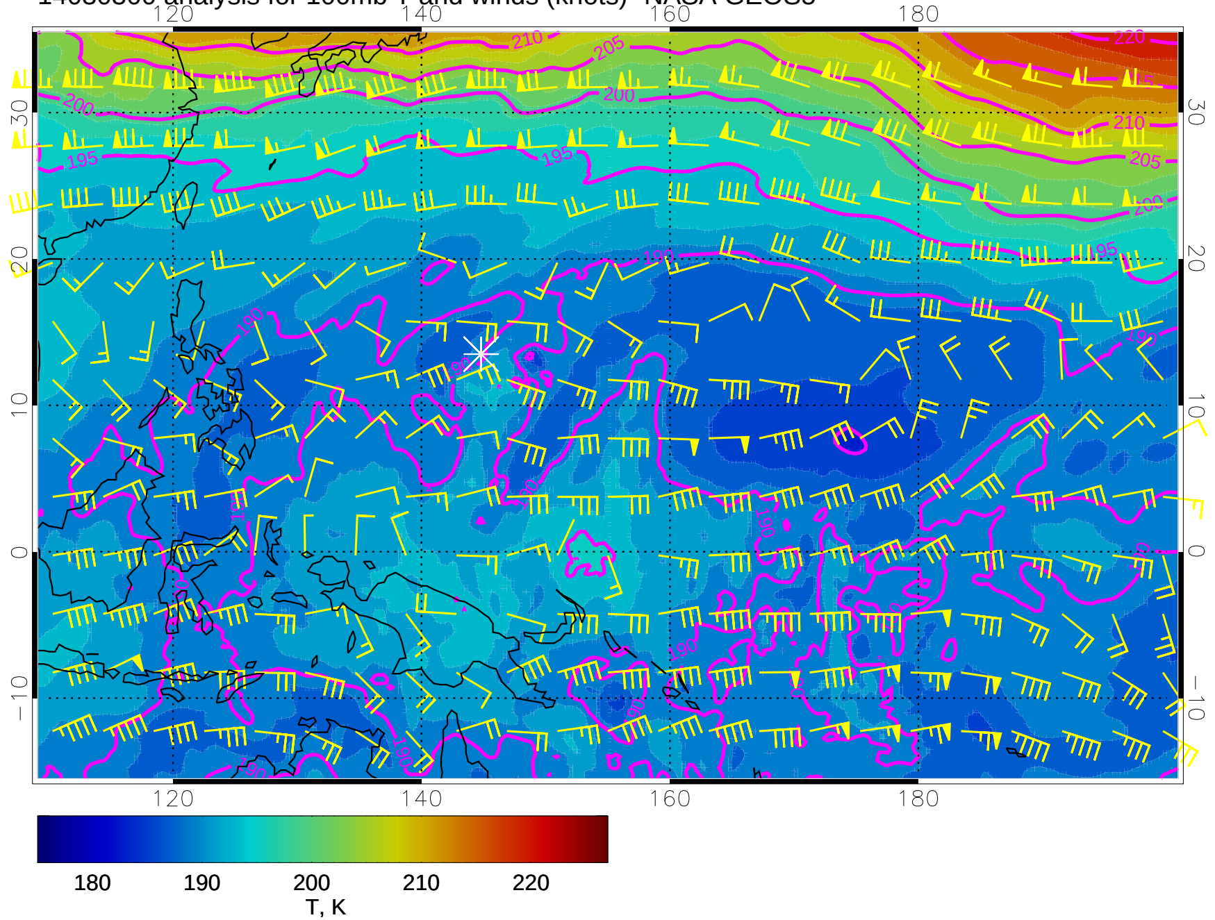
14030300 analysis for 100mb T and winds (knots)- NASA GEOS5
