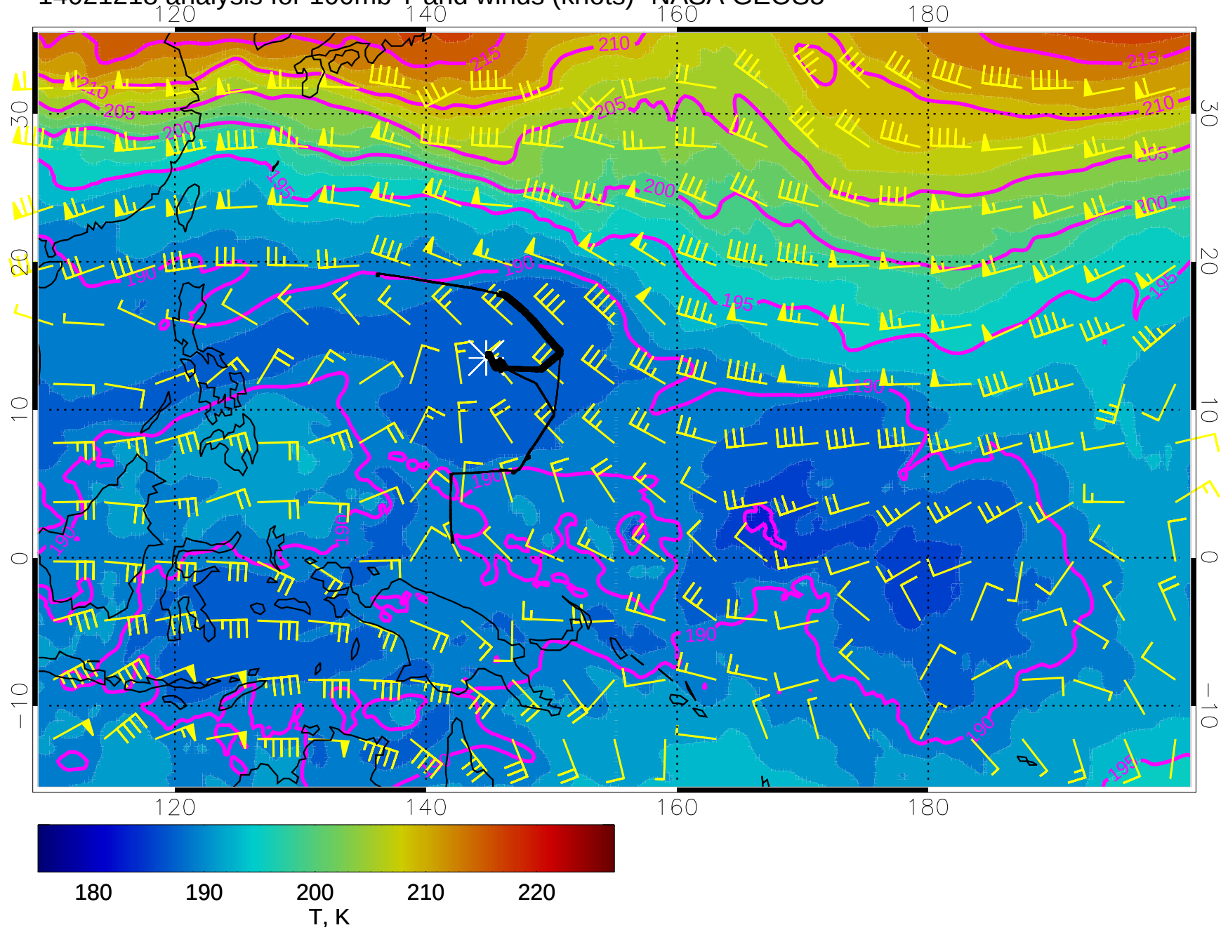
14021218 analysis for 100mb T and winds (knots)- NASA GEOS5
