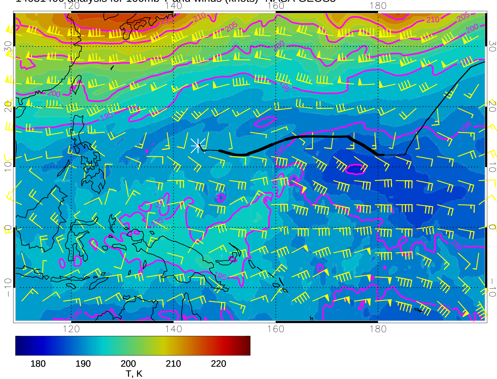
14031400 analysis for 100mb T and winds (knots)- NASA GEOS5
