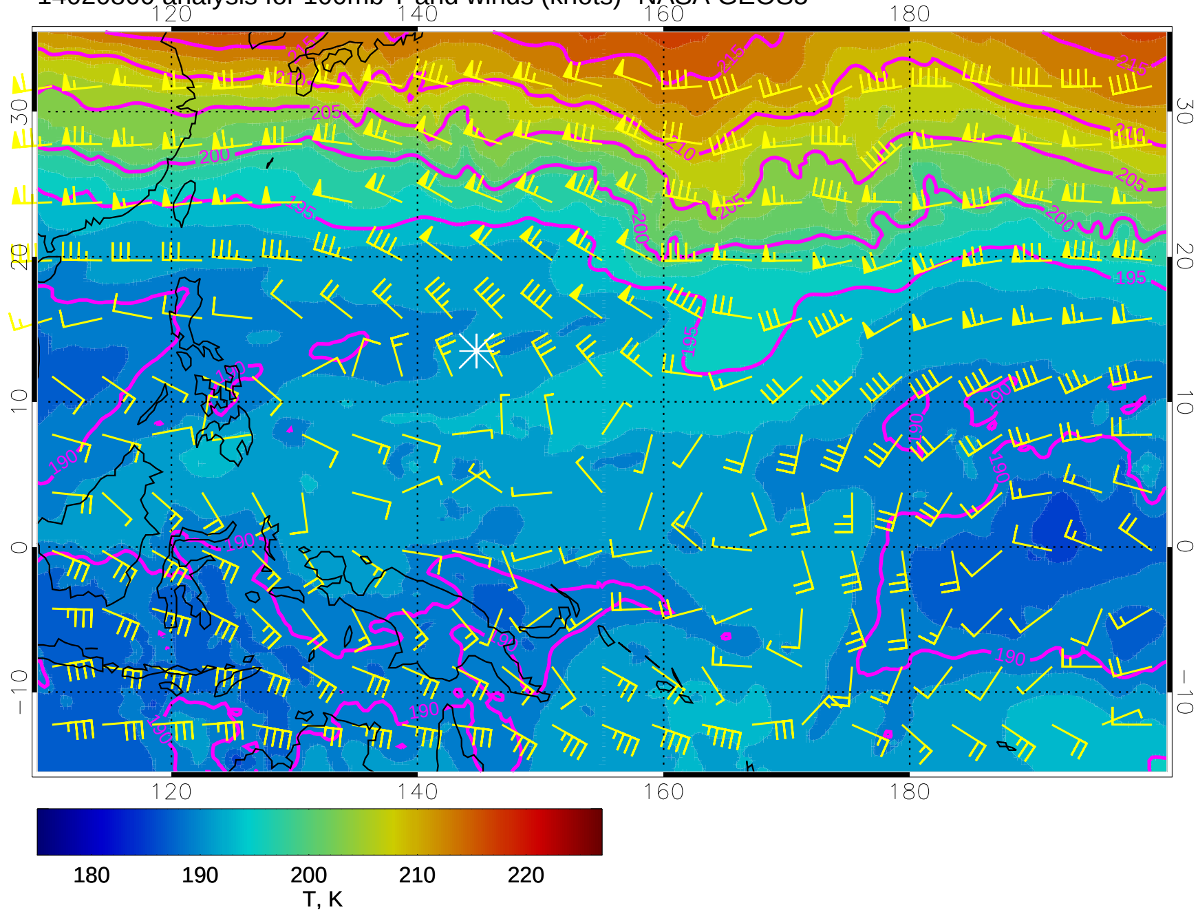
14020800 analysis for 100mb T and winds (knots)- NASA GEOS5
