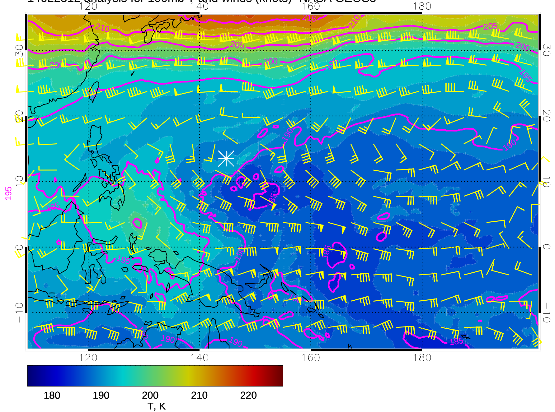
14022512 analysis for 100mb T and winds (knots)- NASA GEOS5
