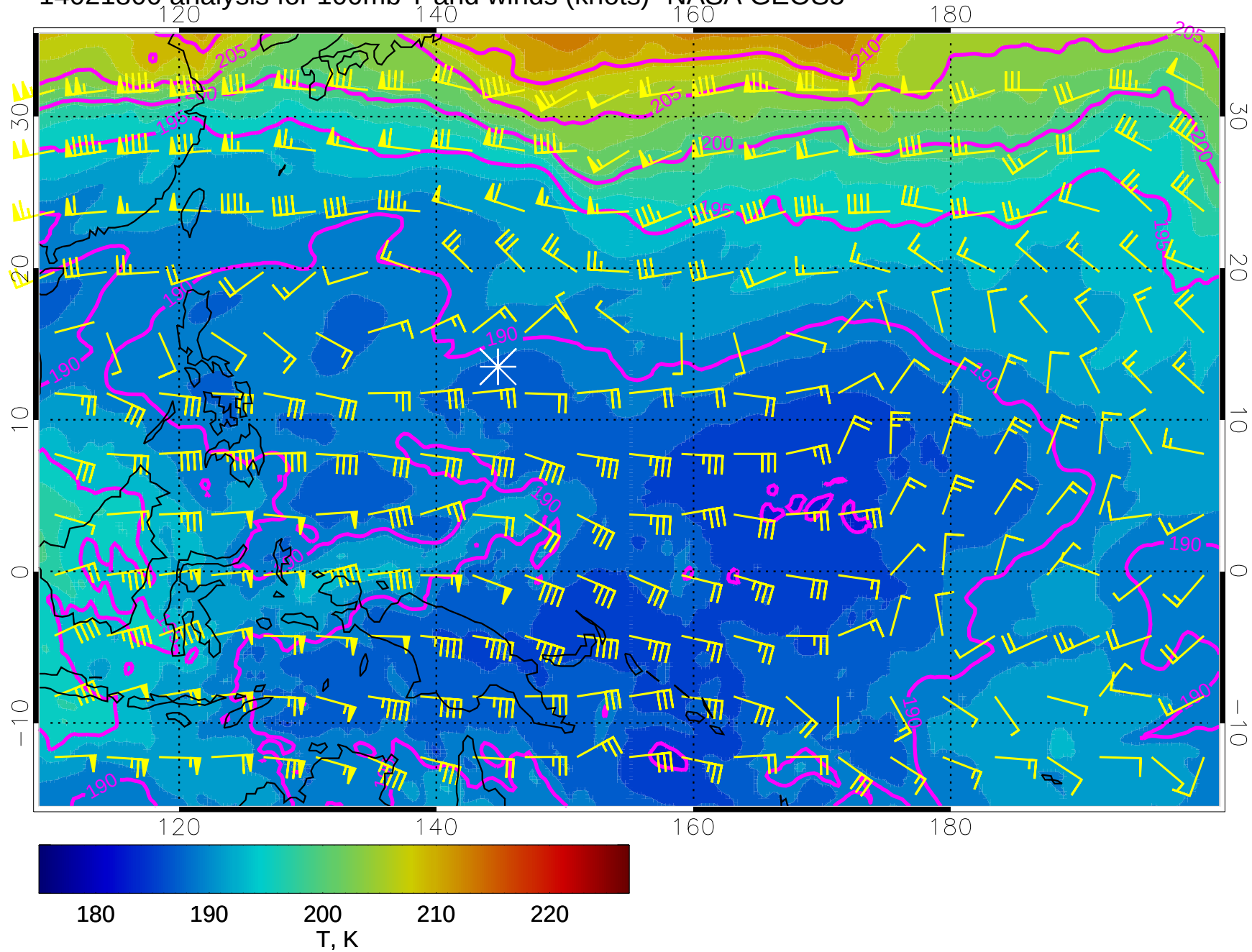
14021800 analysis for 100mb T and winds (knots)- NASA GEOS5
