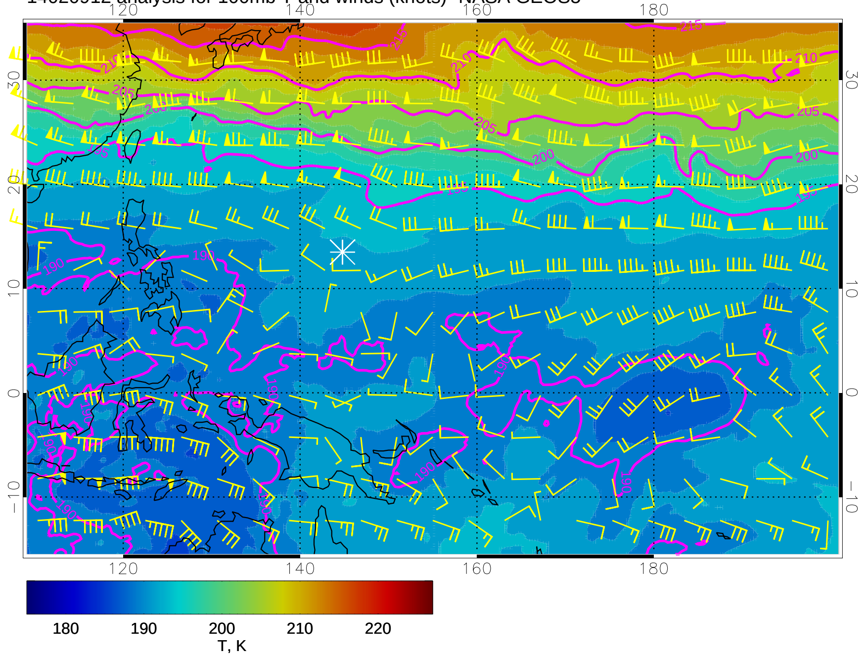
14020912 analysis for 100mb T and winds (knots)- NASA GEOS5
