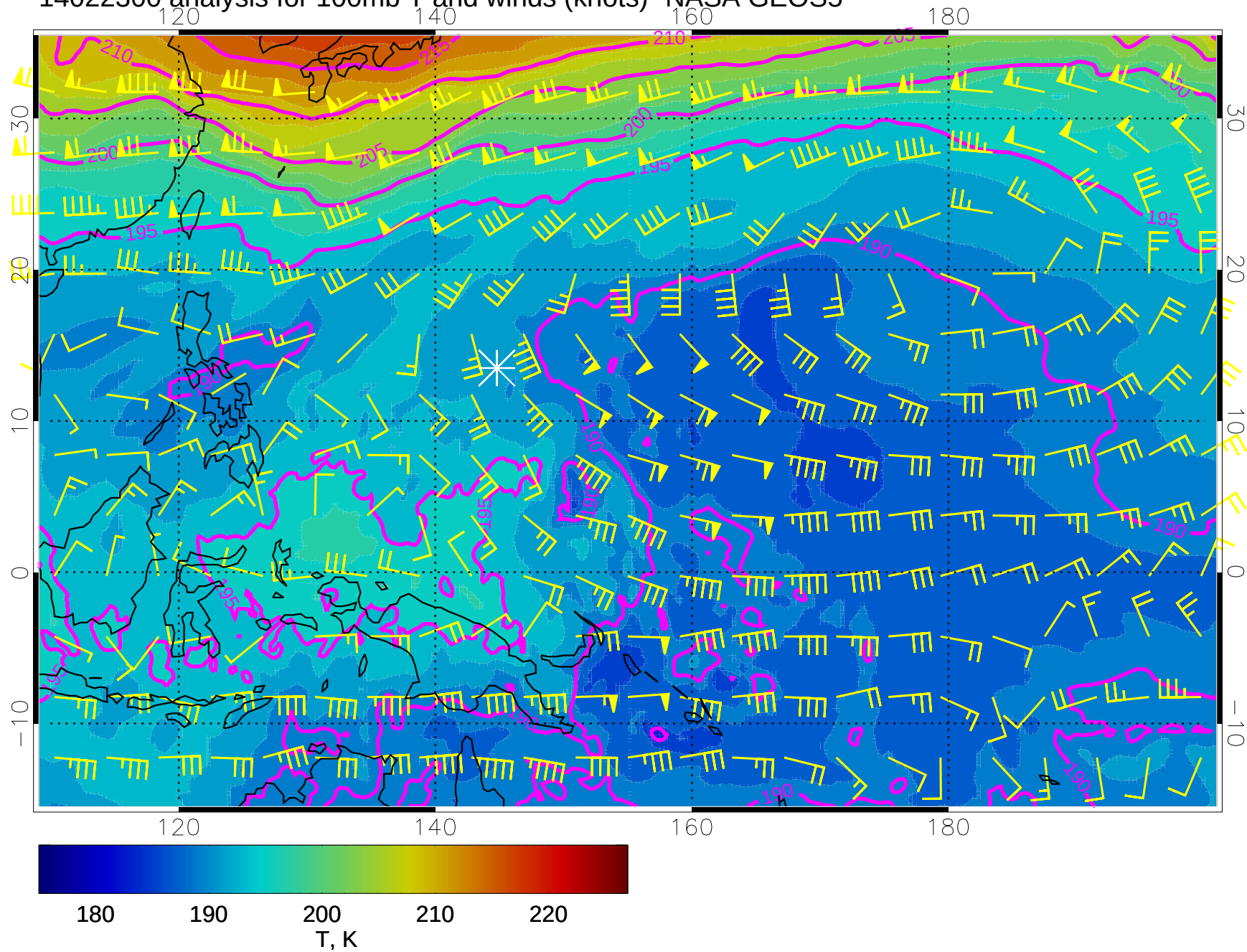
14022300 analysis for 100mb T and winds (knots)- NASA GEOS5
