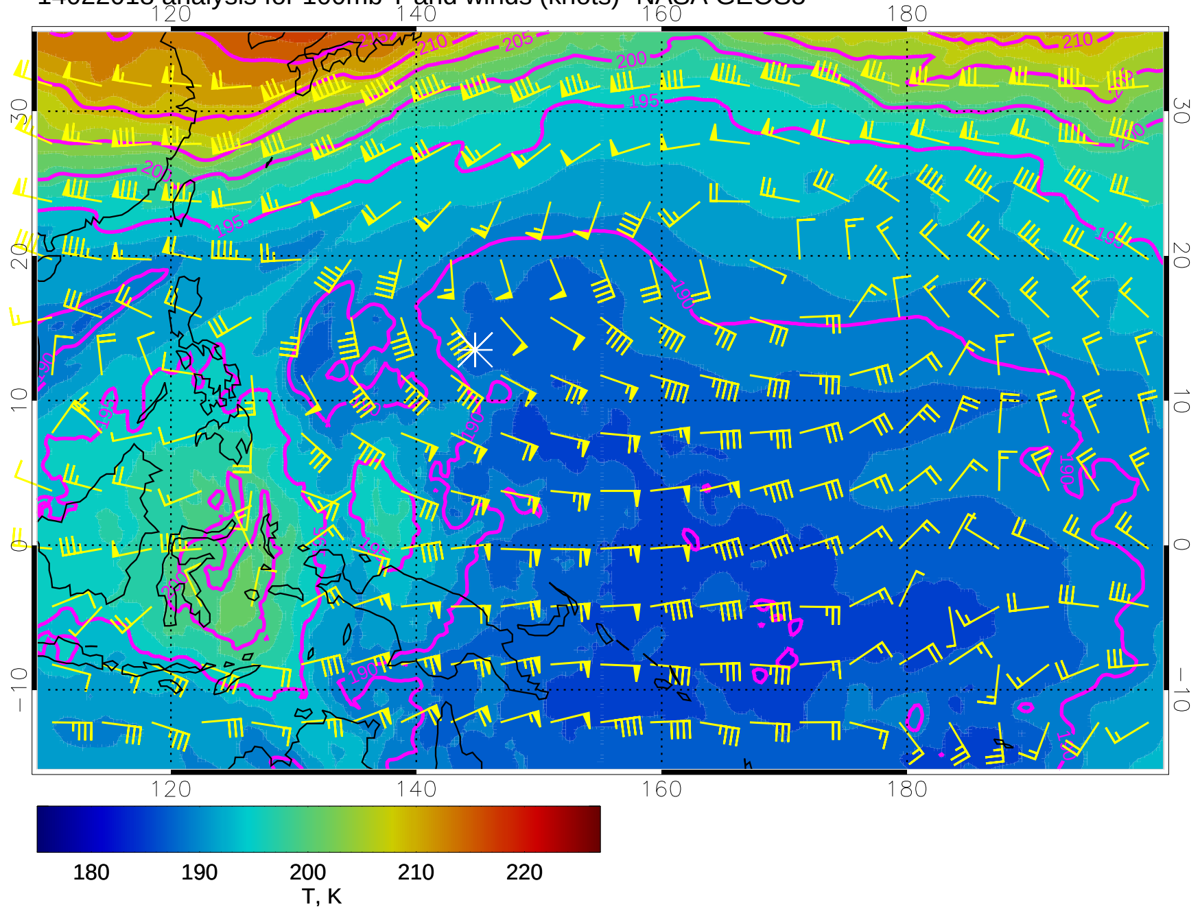
14022018 analysis for 100mb T and winds (knots)- NASA GEOS5
