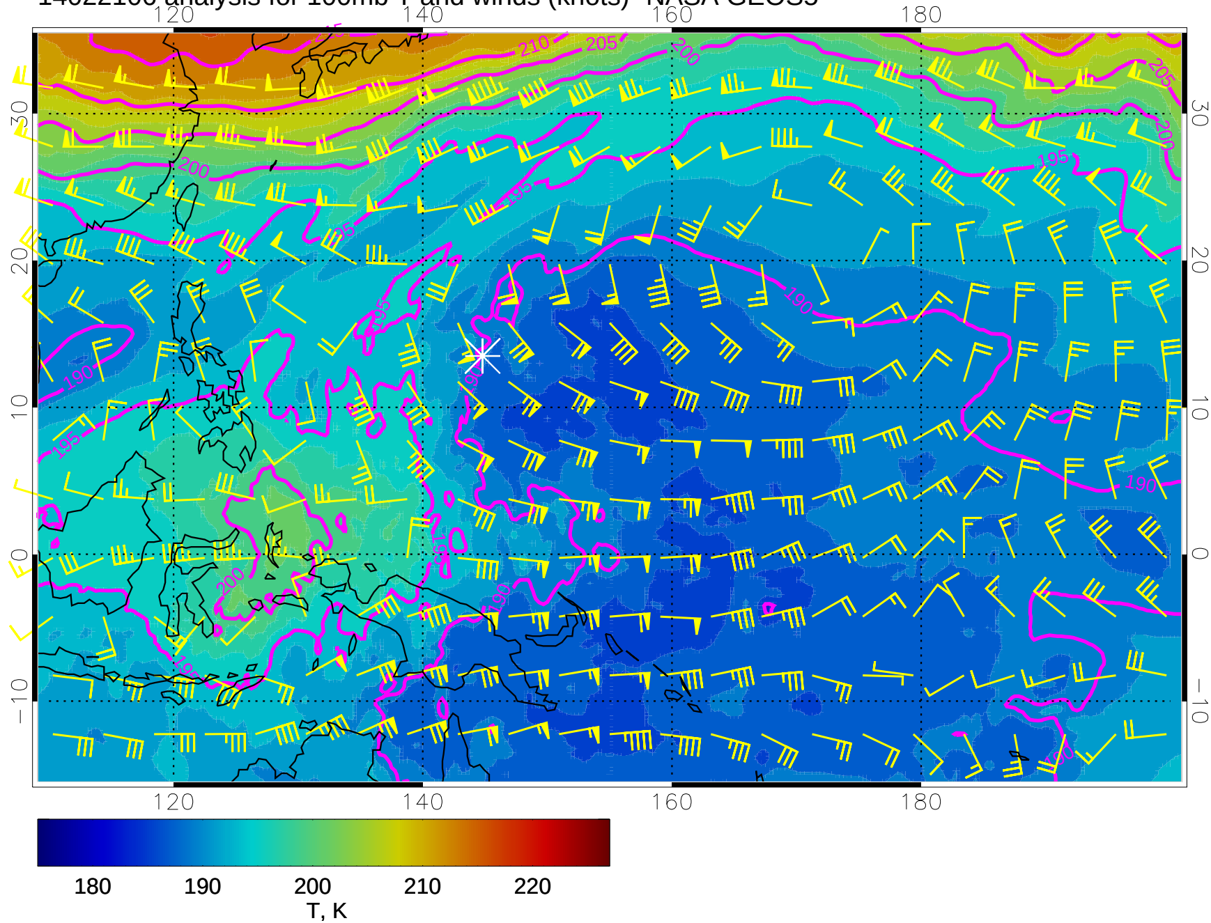
14022106 analysis for 100mb T and winds (knots)- NASA GEOS5
