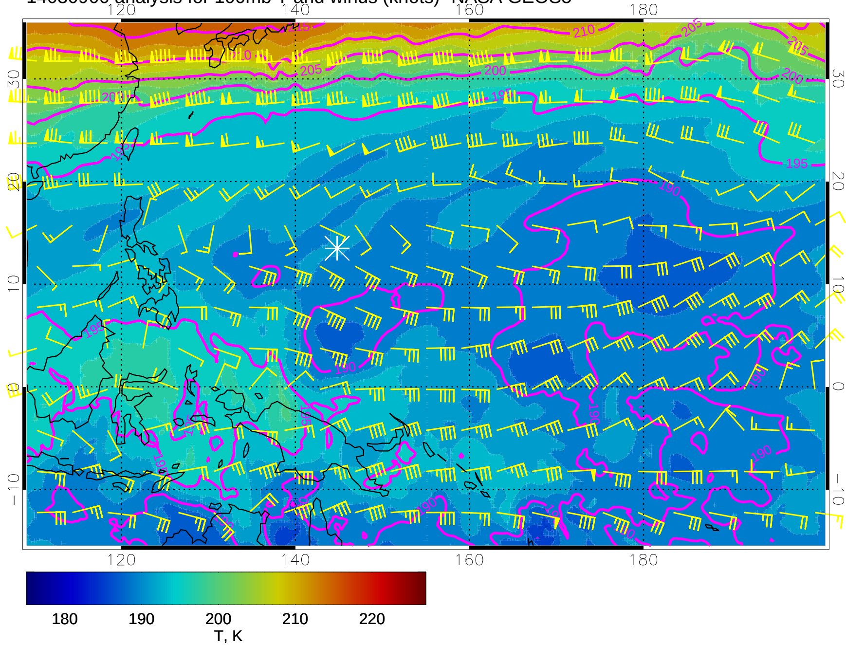
14030900 analysis for 100mb T and winds (knots)- NASA GEOS5
