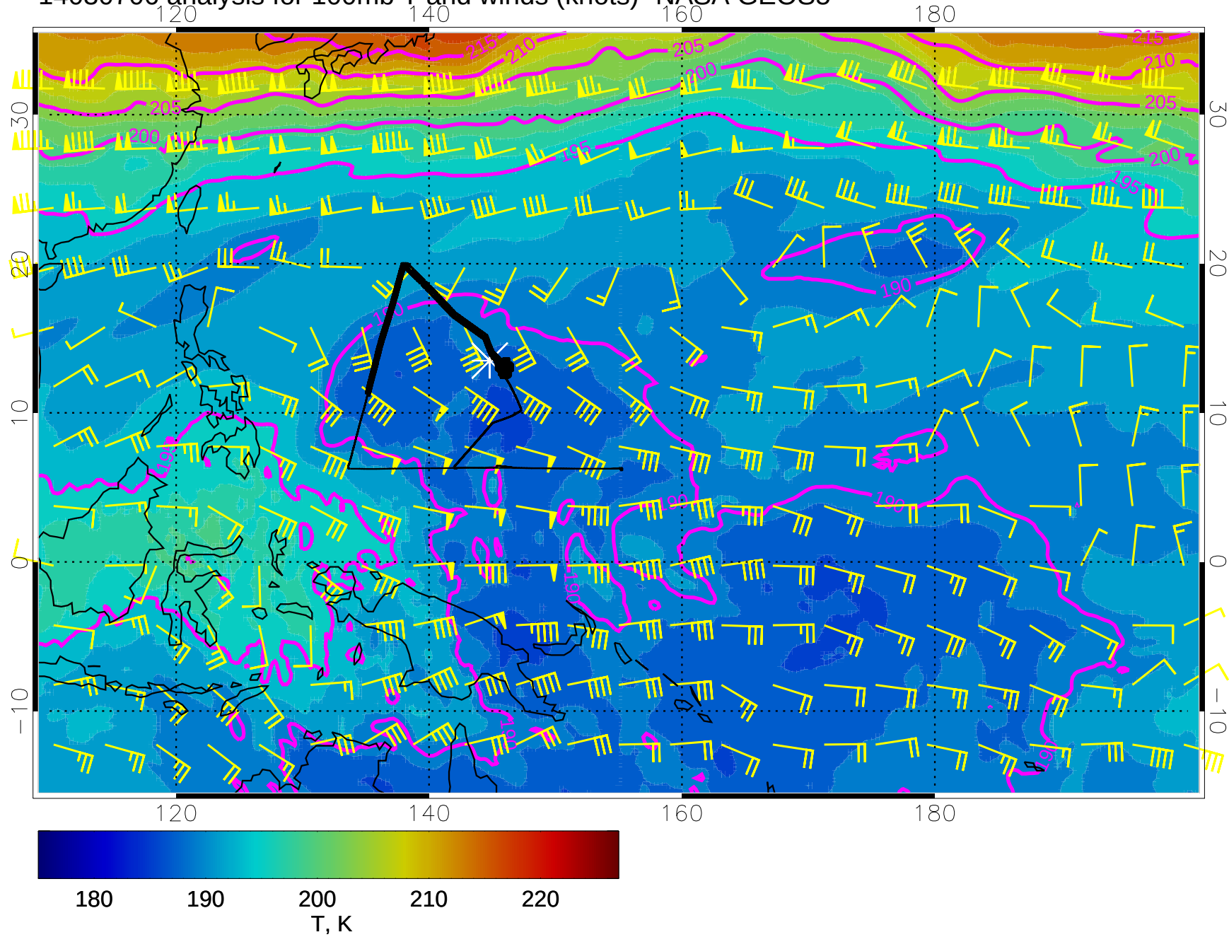
14030706 analysis for 100mb T and winds (knots)- NASA GEOS5
