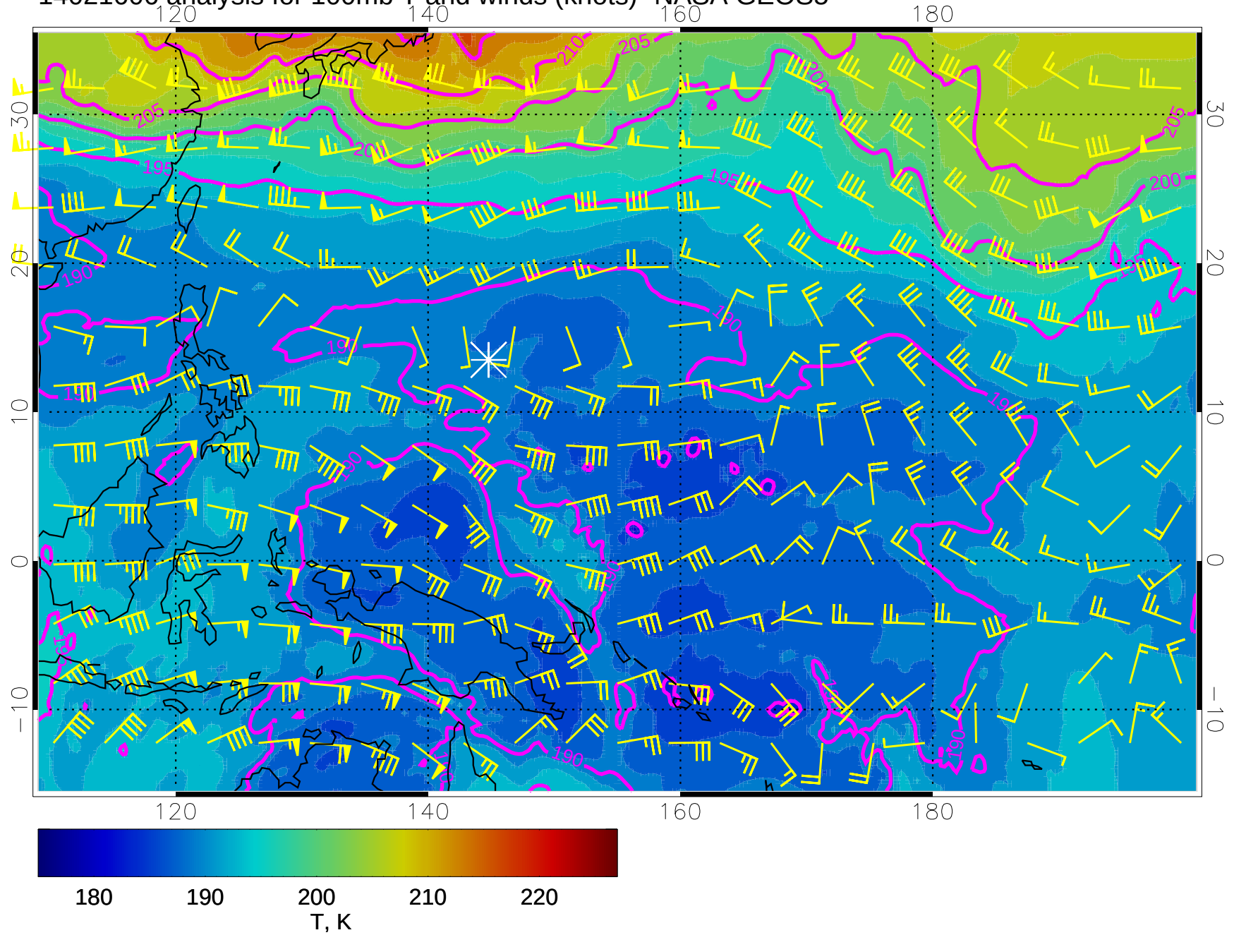
14021606 analysis for 100mb T and winds (knots)- NASA GEOS5
