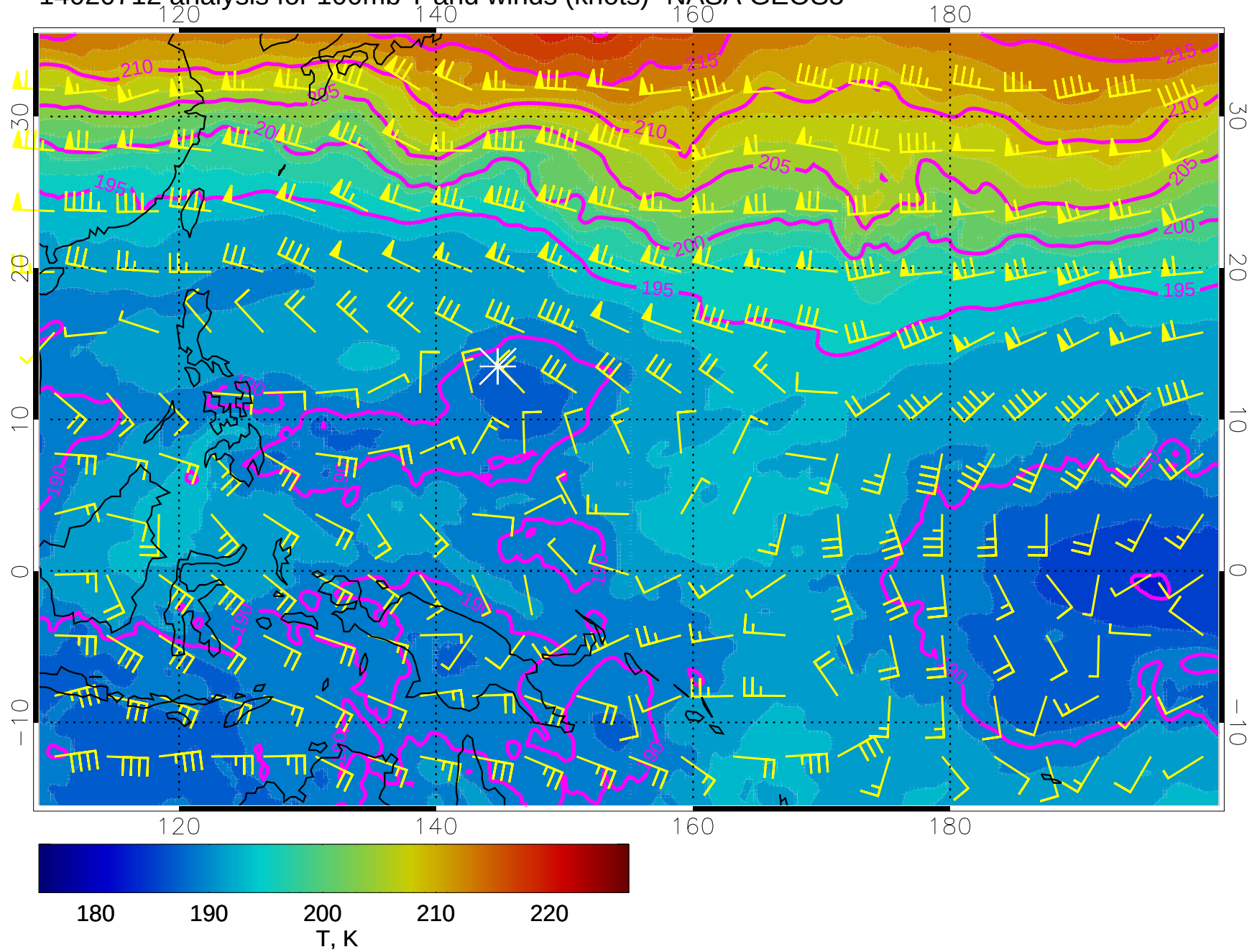
14020712 analysis for 100mb T and winds (knots)- NASA GEOS5
