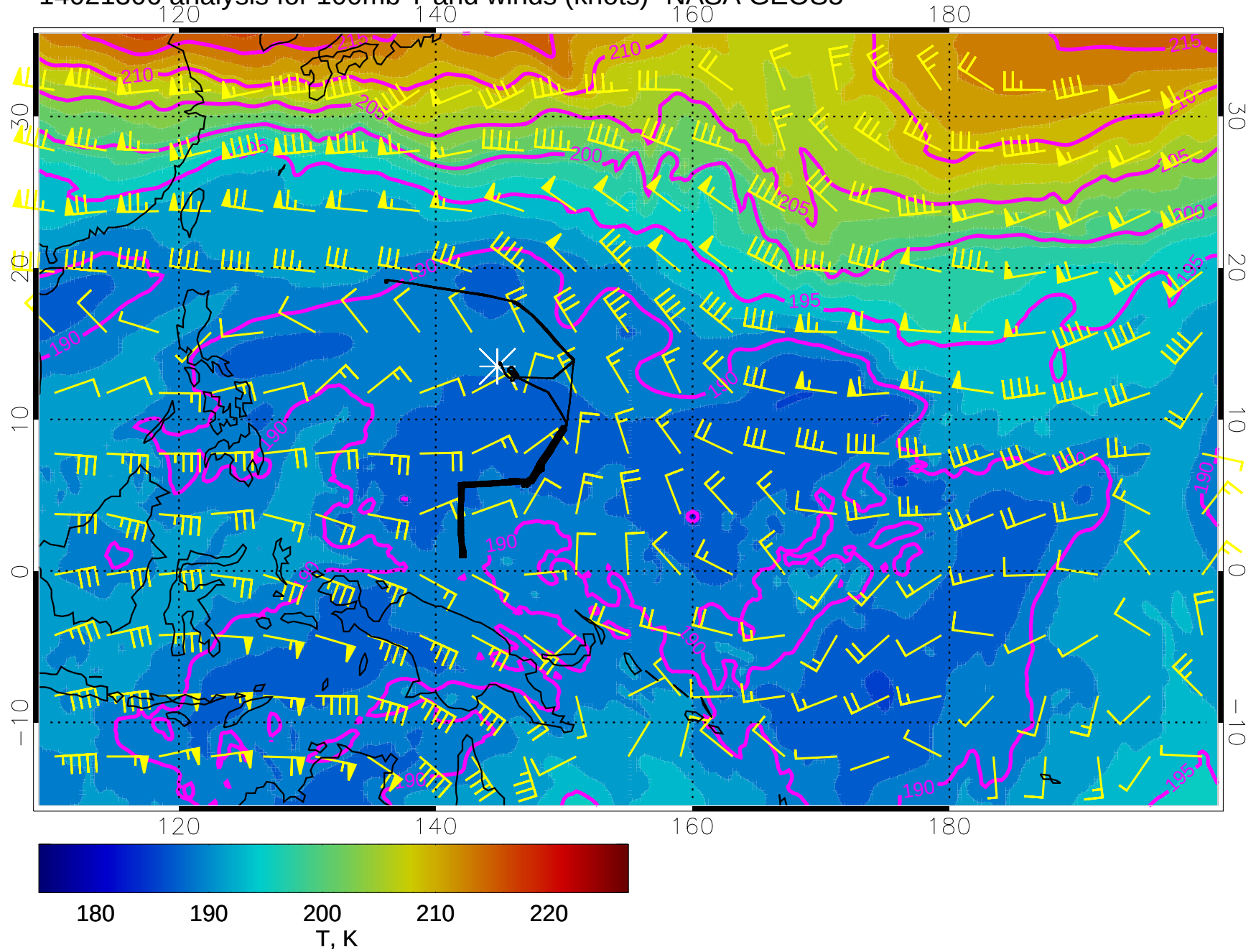
14021306 analysis for 100mb T and winds (knots)- NASA GEOS5
