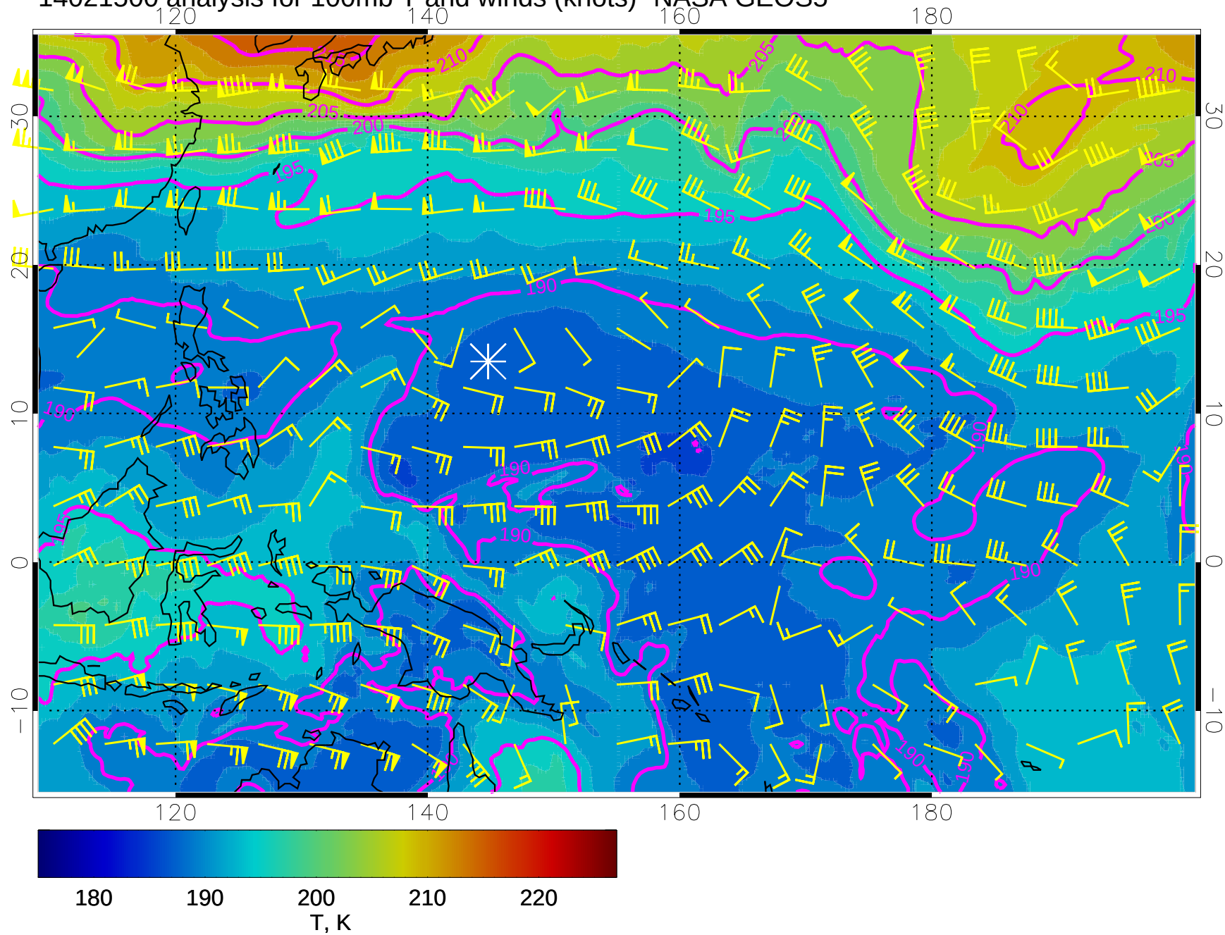
14021500 analysis for 100mb T and winds (knots)- NASA GEOS5
