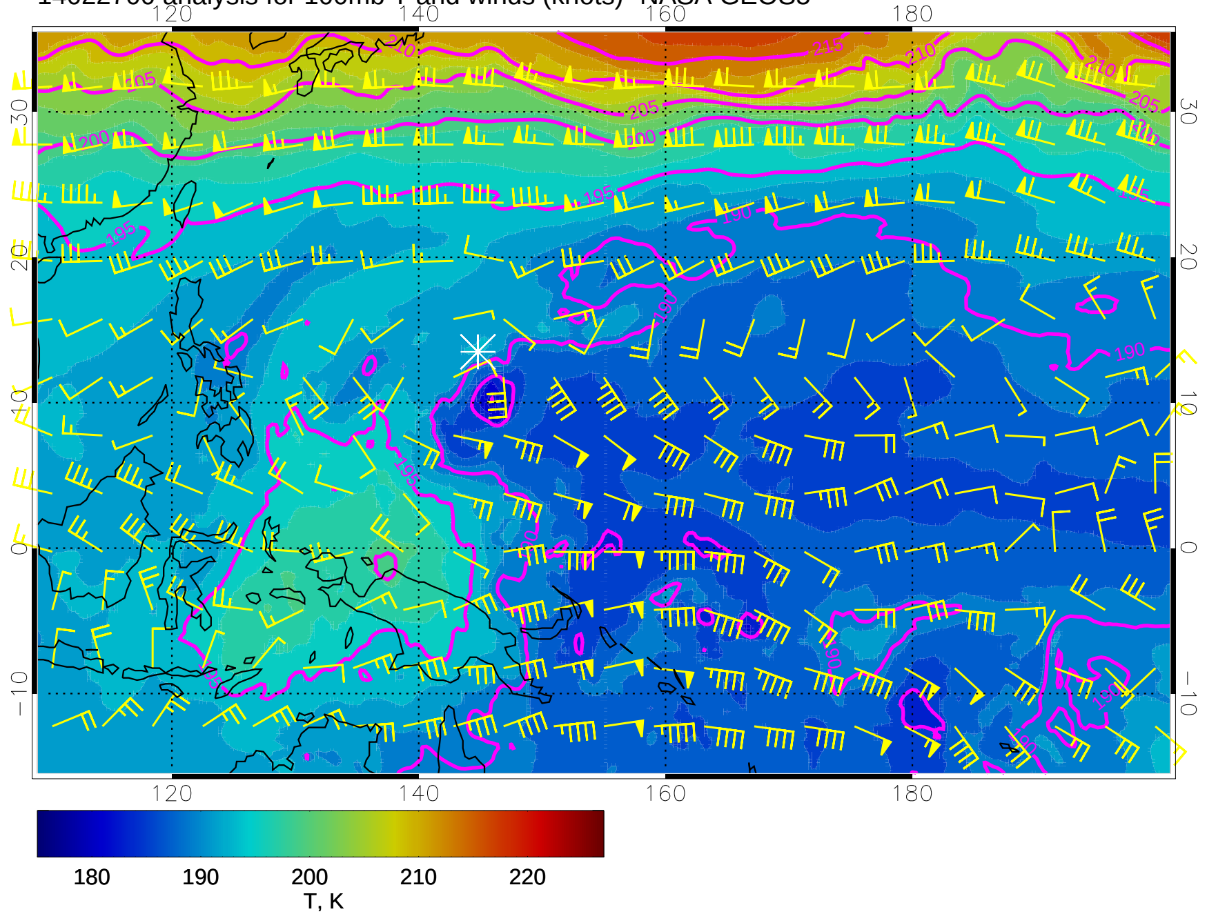
14022700 analysis for 100mb T and winds (knots)- NASA GEOS5
