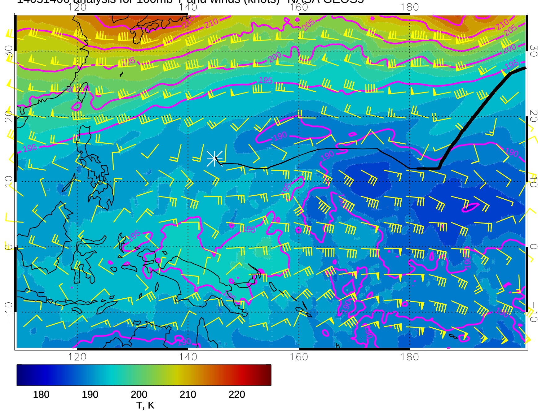
14031406 analysis for 100mb T and winds (knots)- NASA GEOS5
