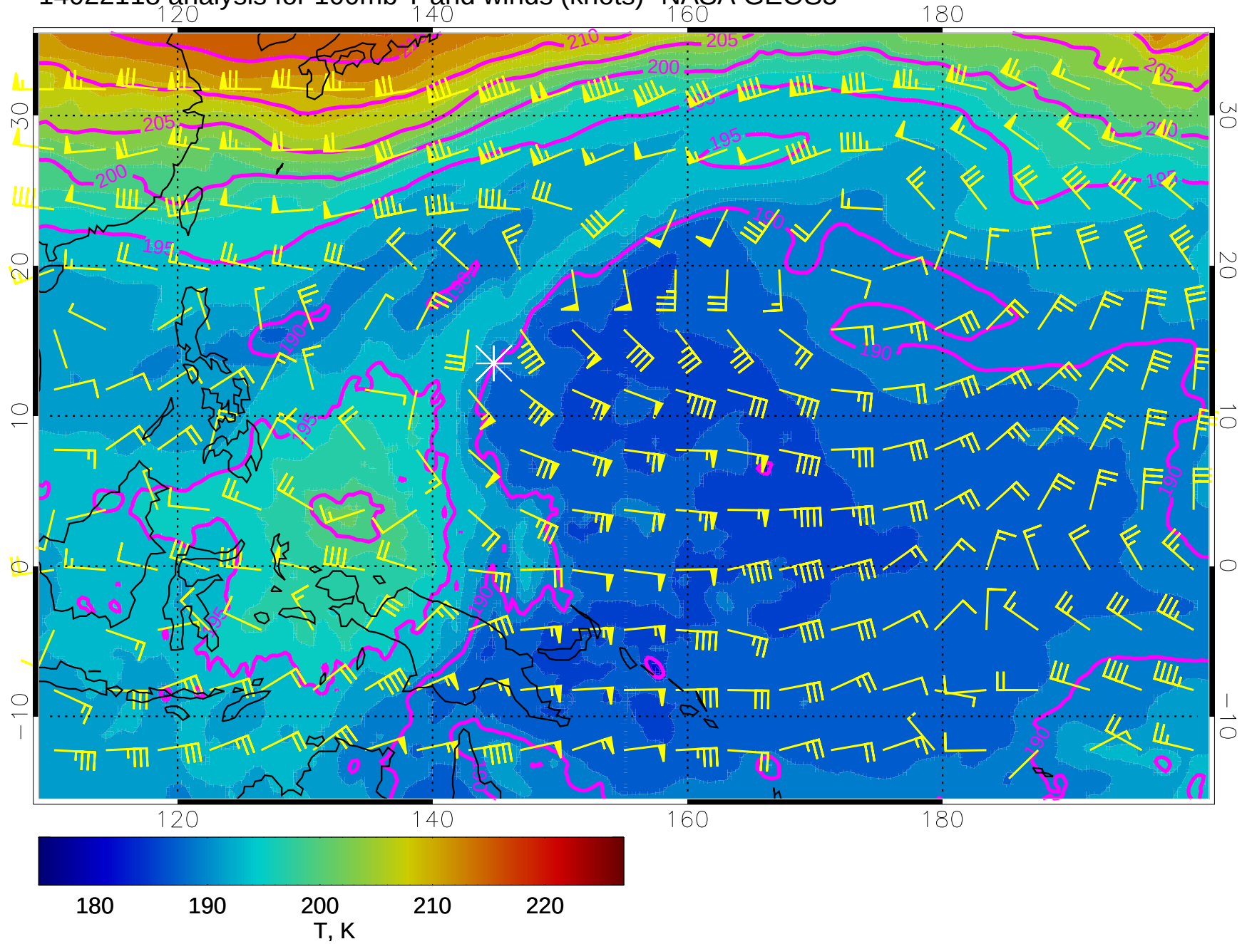
14022118 analysis for 100mb T and winds (knots)- NASA GEOS5
