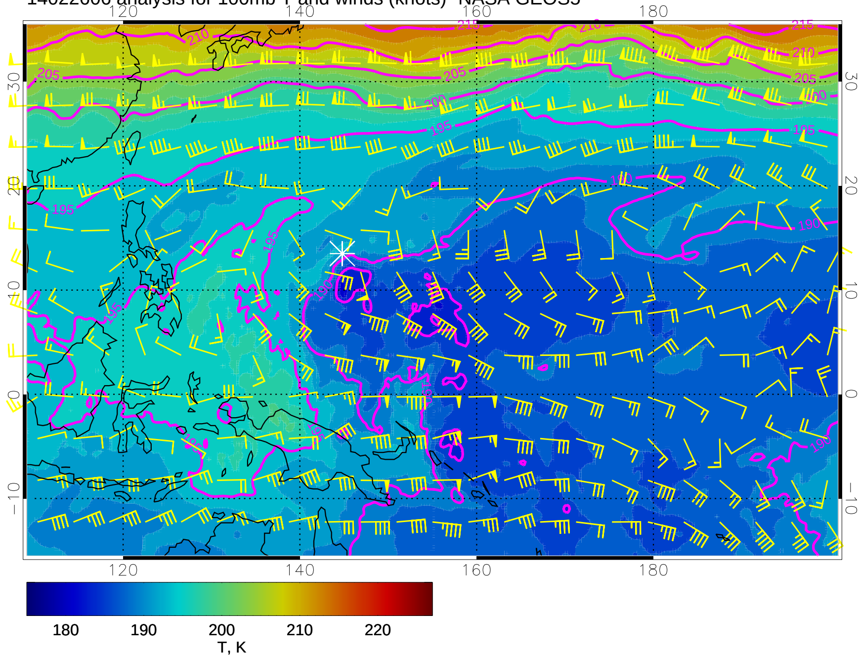
14022606 analysis for 100mb T and winds (knots)- NASA GEOS5
