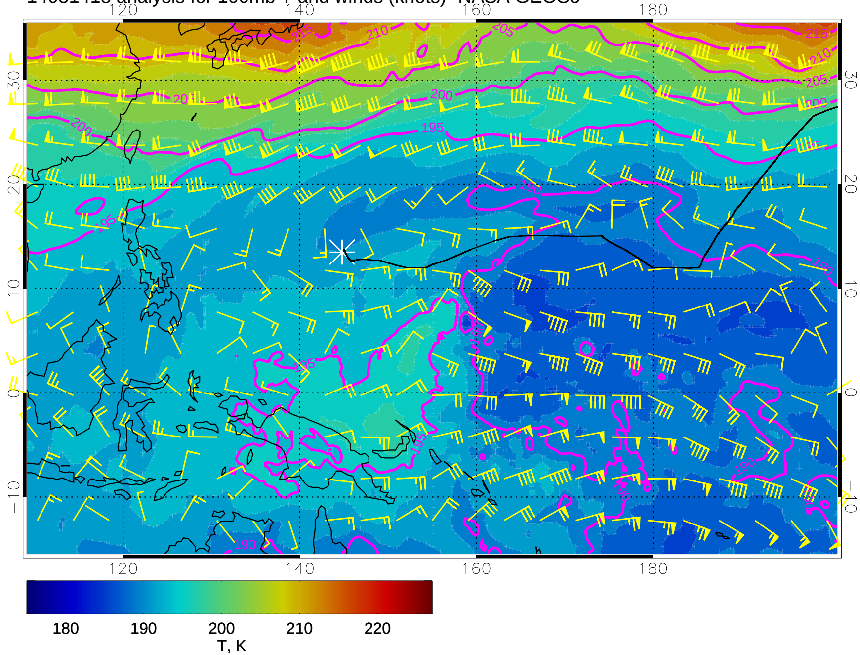
14031418 analysis for 100mb T and winds (knots)- NASA GEOS5
