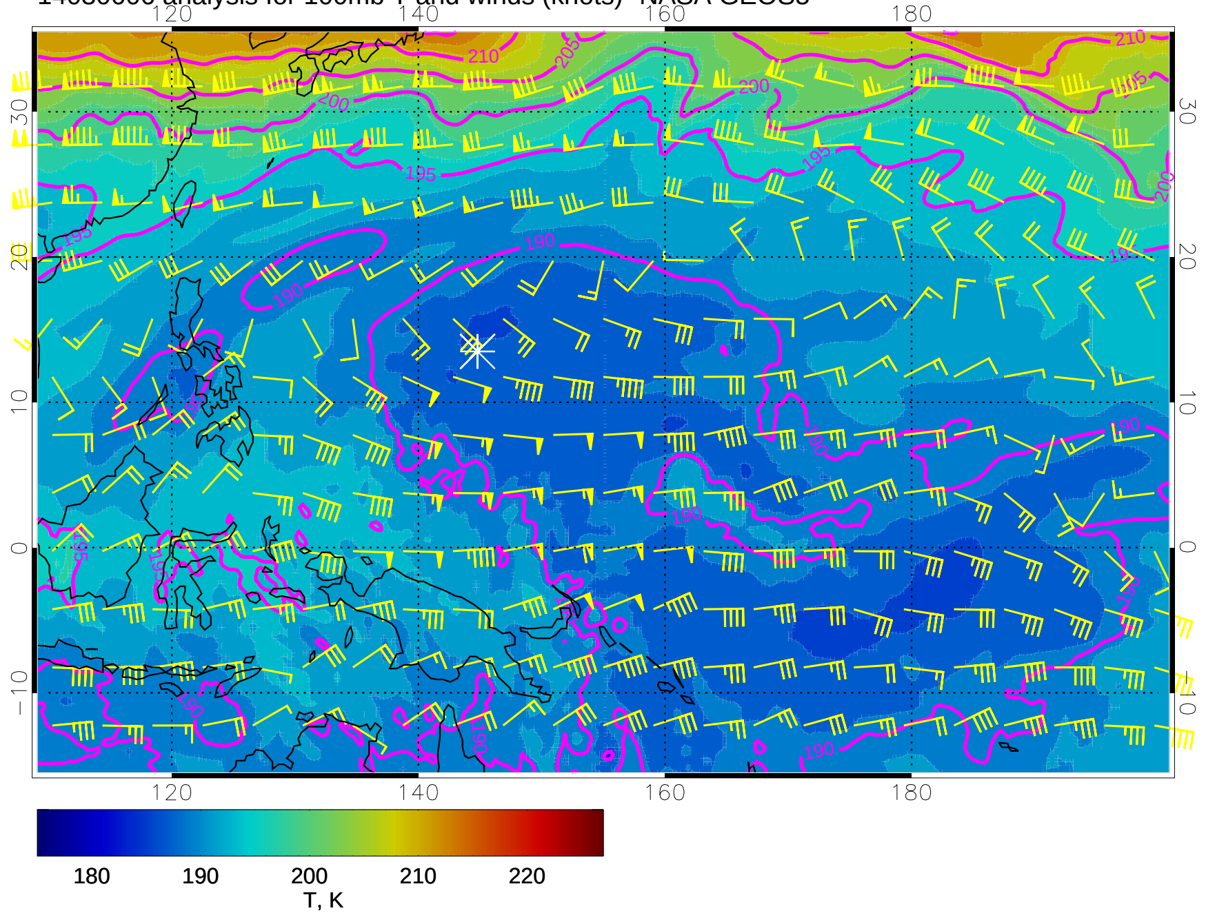
14030606 analysis for 100mb T and winds (knots)- NASA GEOS5
