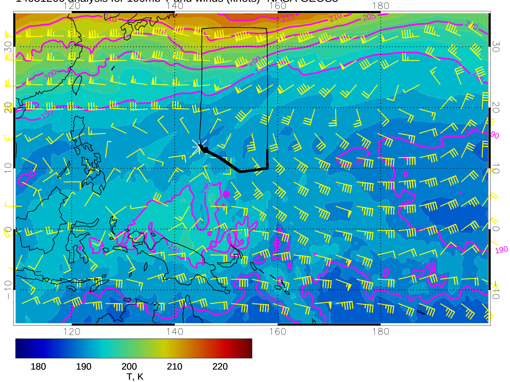
14031206 analysis for 100mb T and winds (knots)- NASA GEOS5
