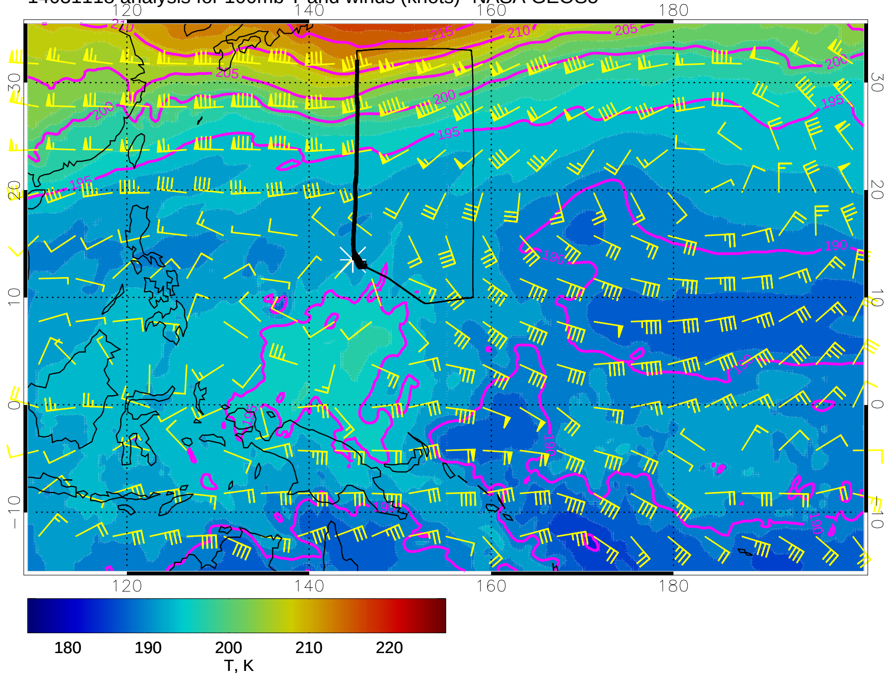
14031118 analysis for 100mb T and winds (knots)- NASA GEOS5
