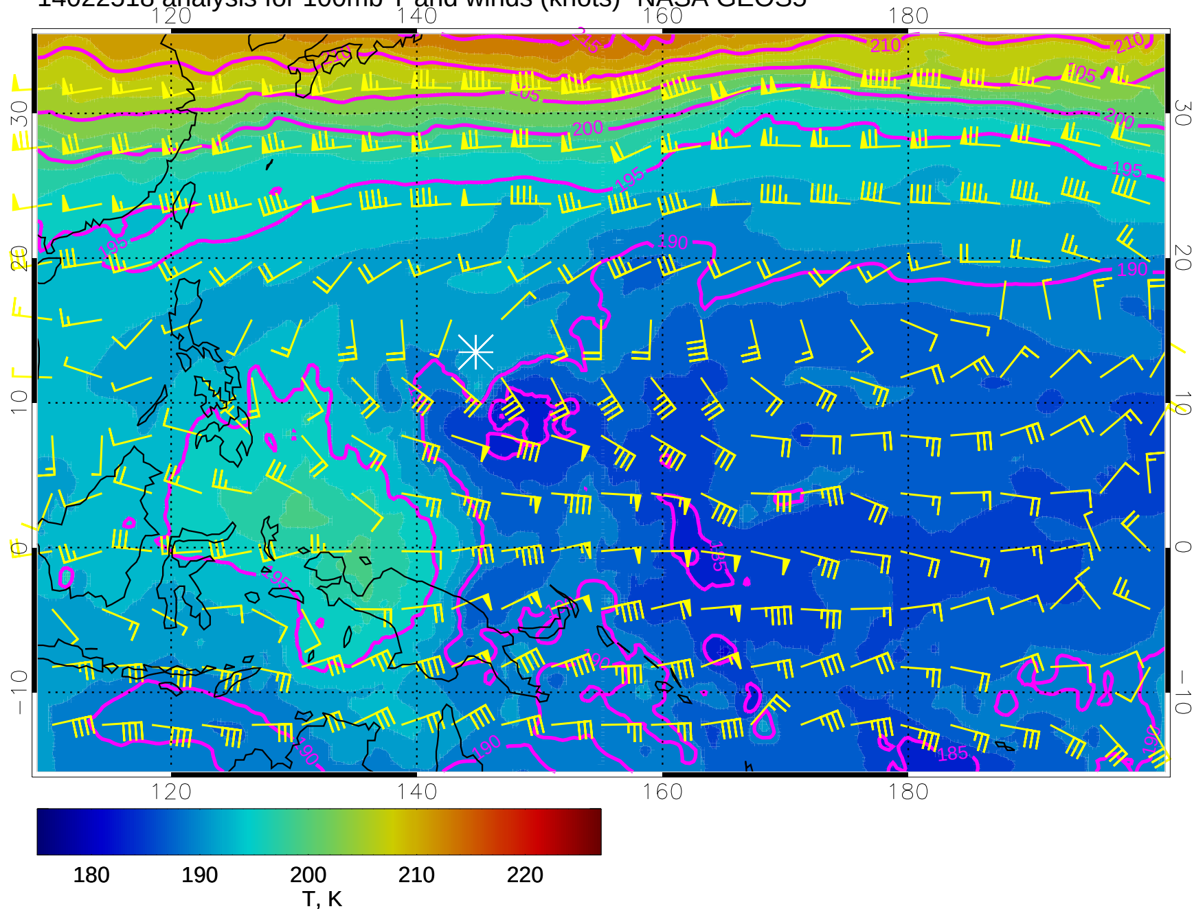
14022518 analysis for 100mb T and winds (knots)- NASA GEOS5
