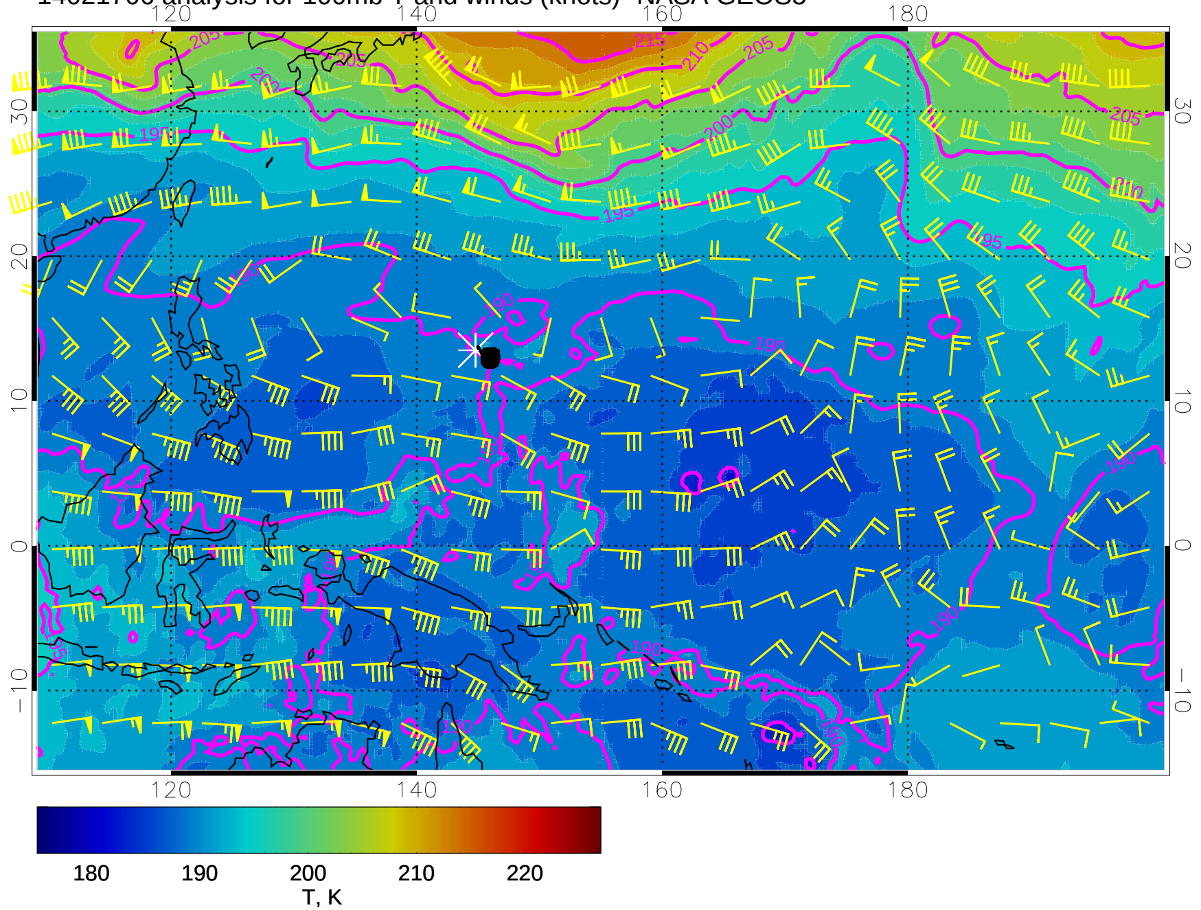
14021706 analysis for 100mb T and winds (knots)- NASA GEOS5
