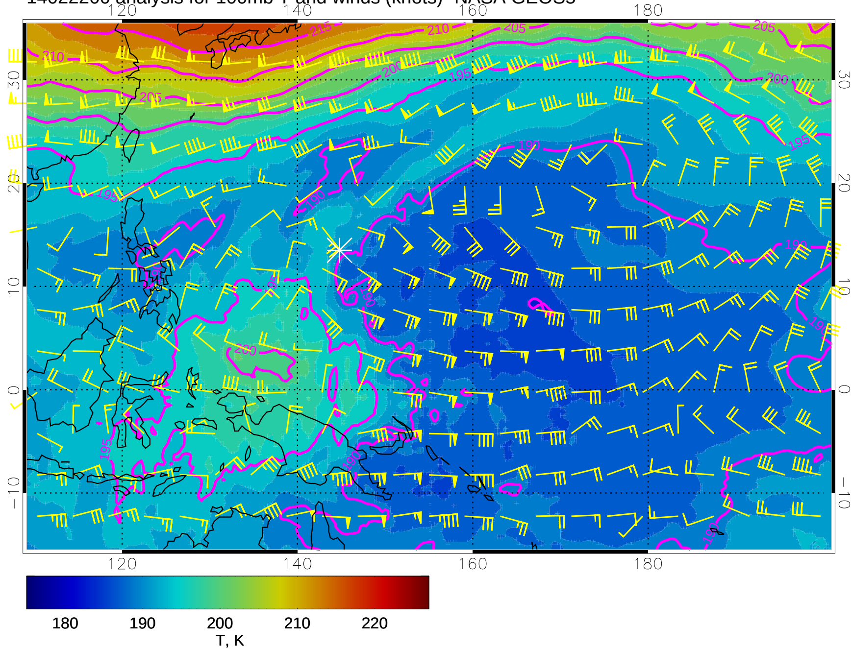
14022200 analysis for 100mb T and winds (knots)- NASA GEOS5
