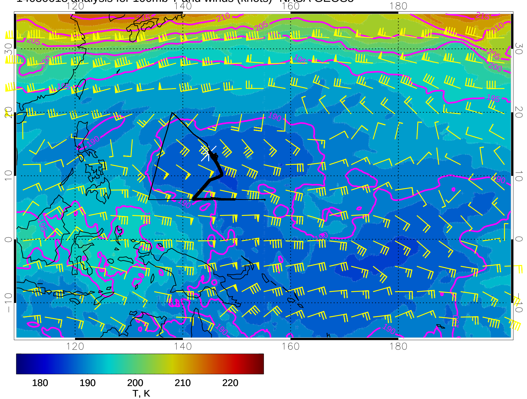
14030618 analysis for 100mb T and winds (knots)- NASA GEOS5
