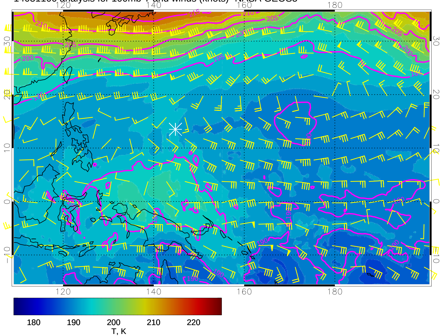
14031100 analysis for 100mb T and winds (knots)- NASA GEOS5
