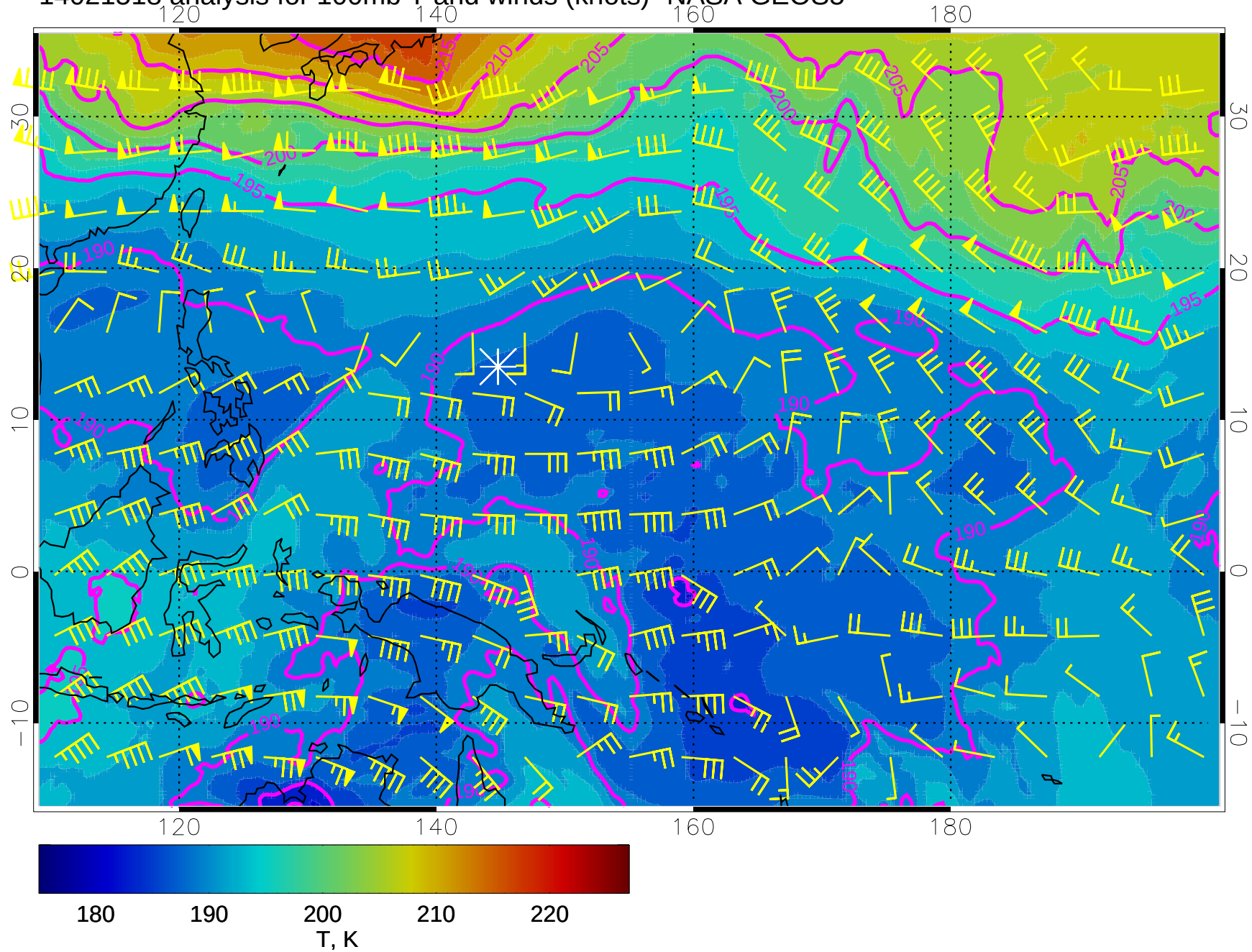
14021518 analysis for 100mb T and winds (knots)- NASA GEOS5
