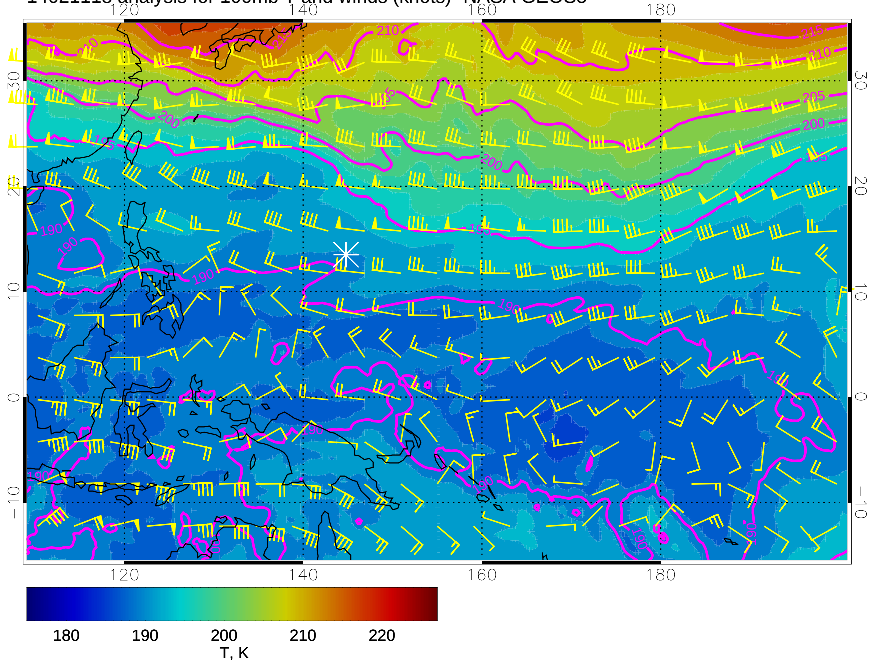
14021118 analysis for 100mb T and winds (knots)- NASA GEOS5
