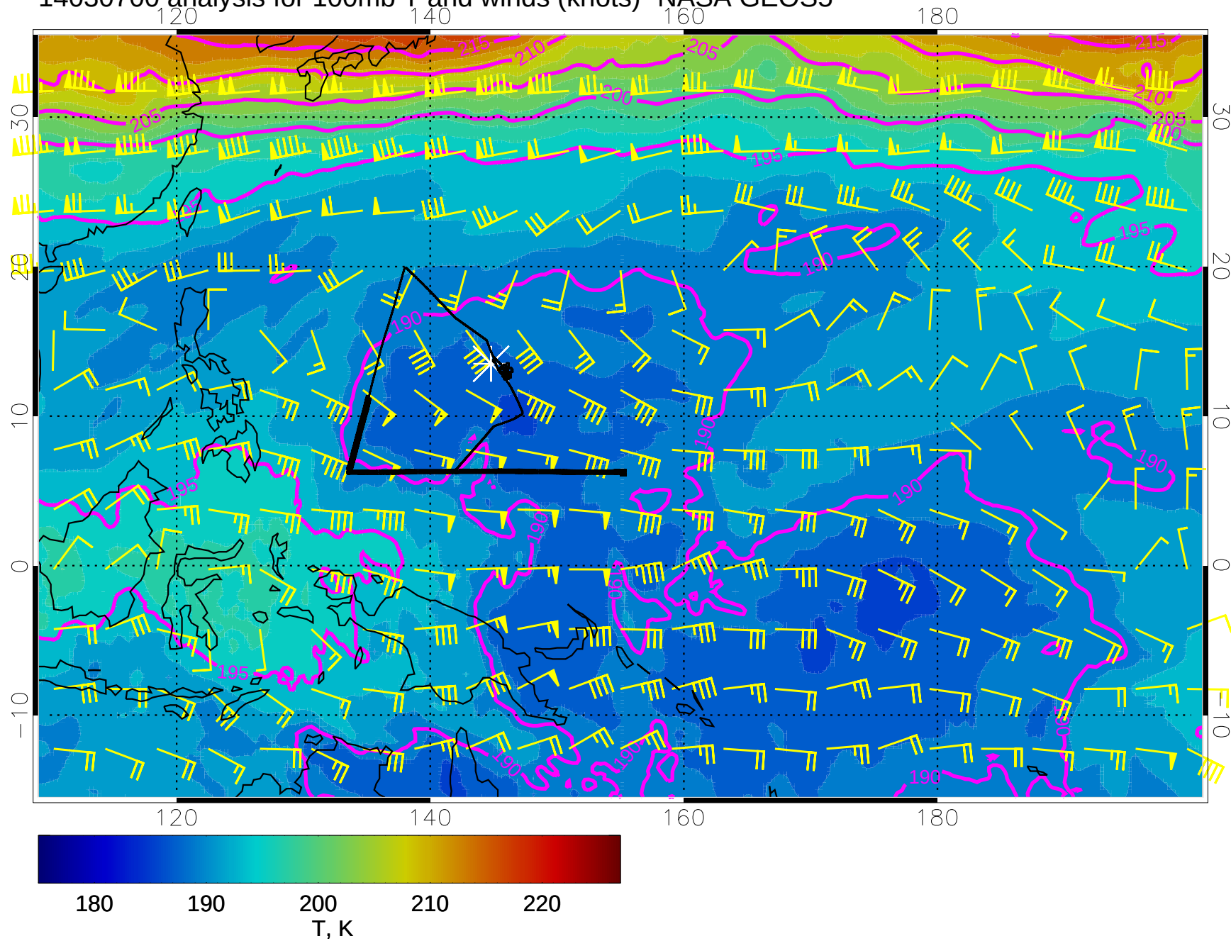
14030700 analysis for 100mb T and winds (knots)- NASA GEOS5
