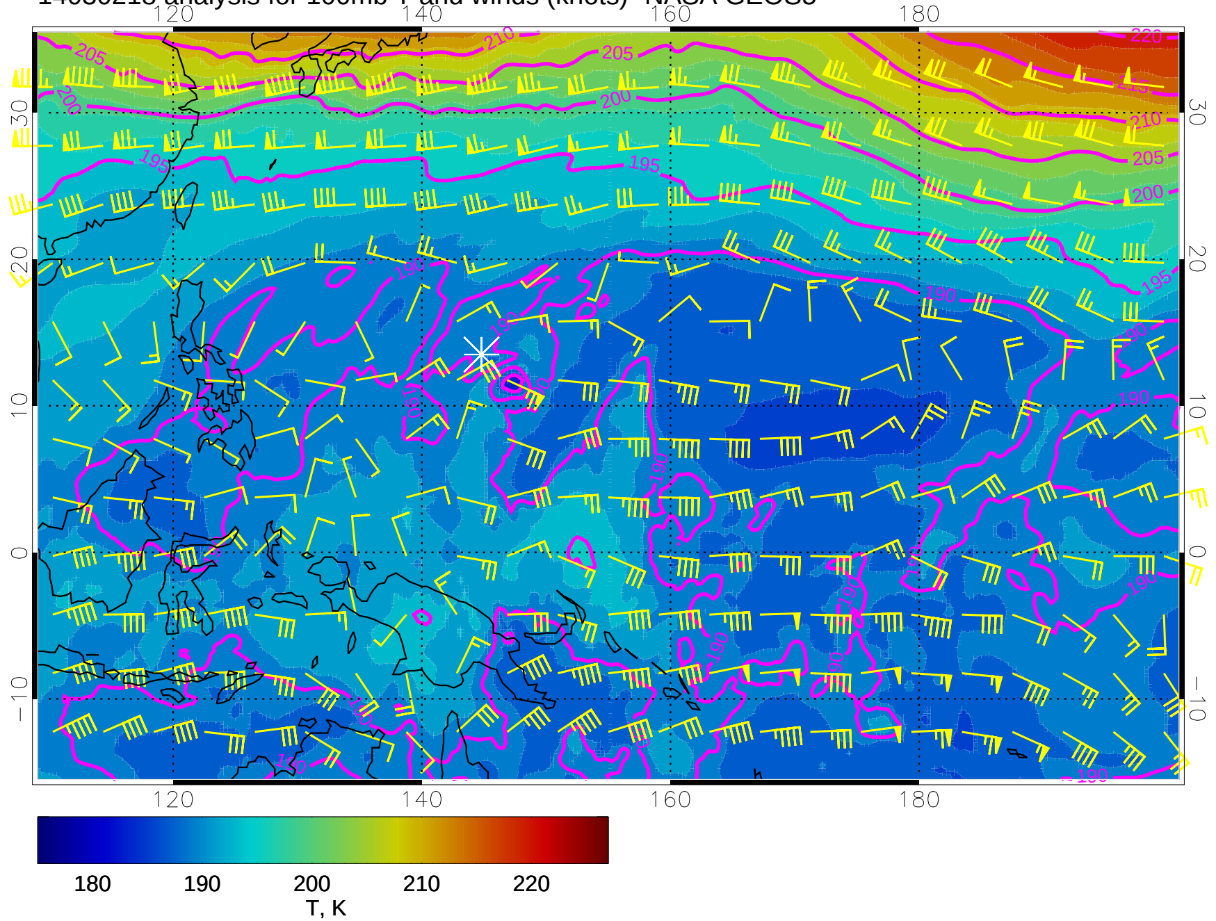
14030218 analysis for 100mb T and winds (knots)- NASA GEOS5
