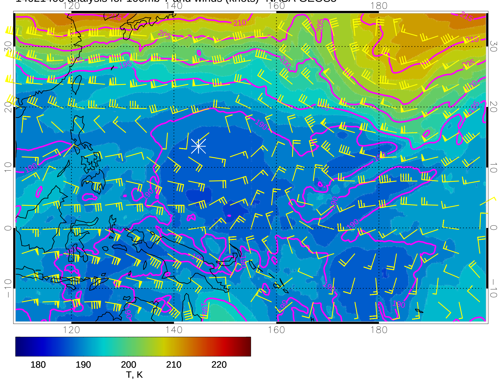
14021400 analysis for 100mb T and winds (knots)- NASA GEOS5
