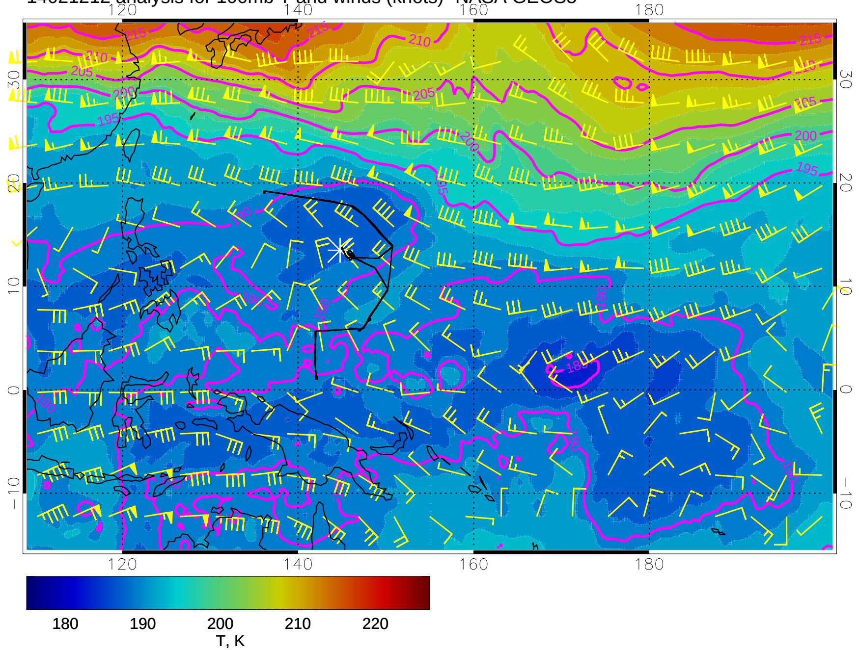
14021212 analysis for 100mb T and winds (knots)- NASA GEOS5
