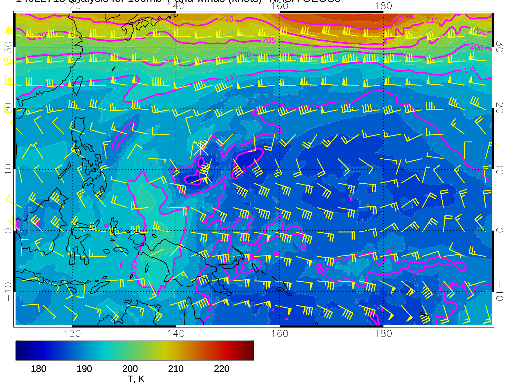
14022718 analysis for 100mb T and winds (knots)- NASA GEOS5
