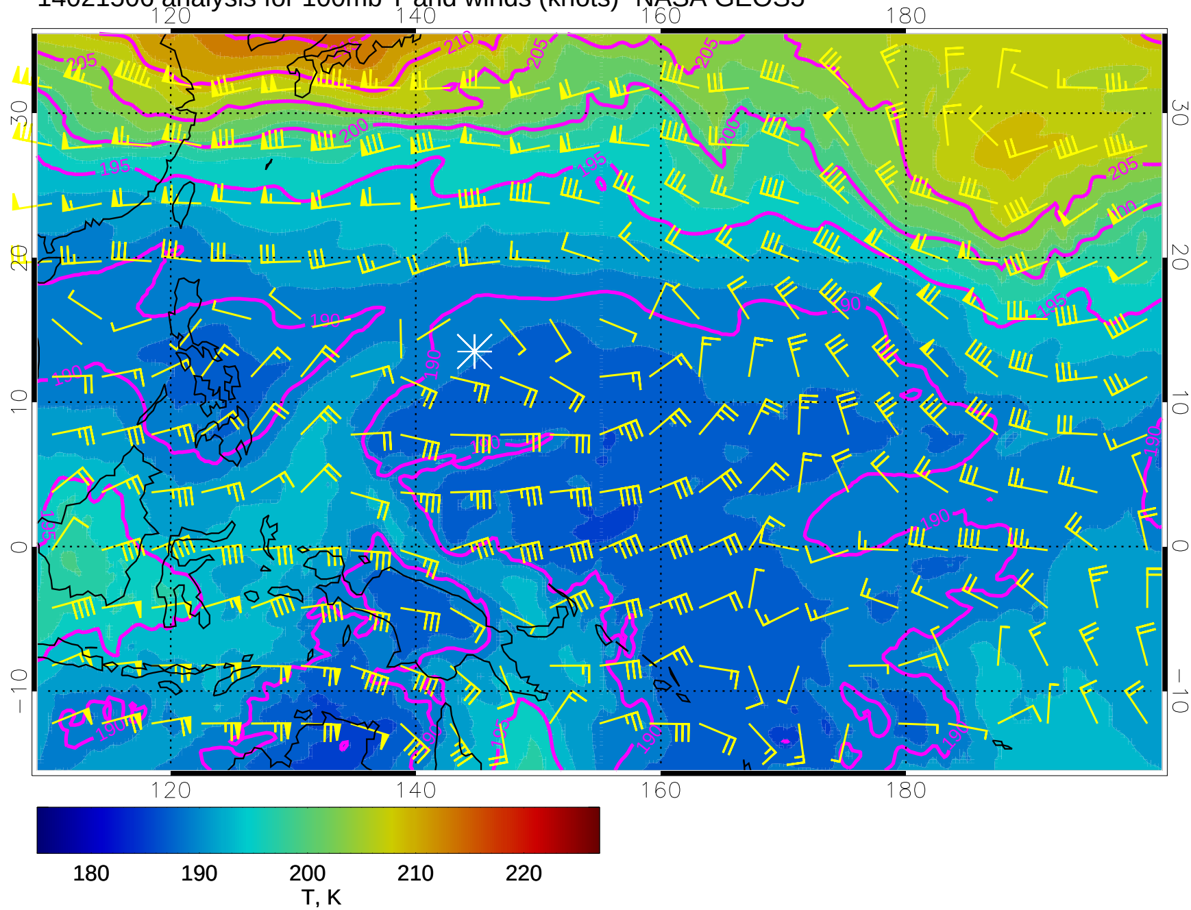
14021506 analysis for 100mb T and winds (knots)- NASA GEOS5
