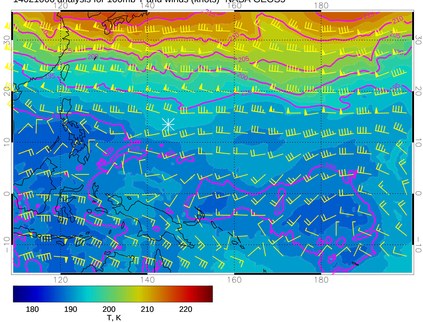
14021006 analysis for 100mb T and winds (knots)- NASA GEOS5
