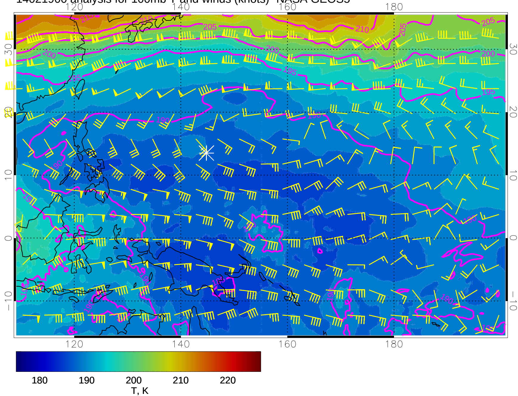
14021900 analysis for 100mb T and winds (knots)- NASA GEOS5
