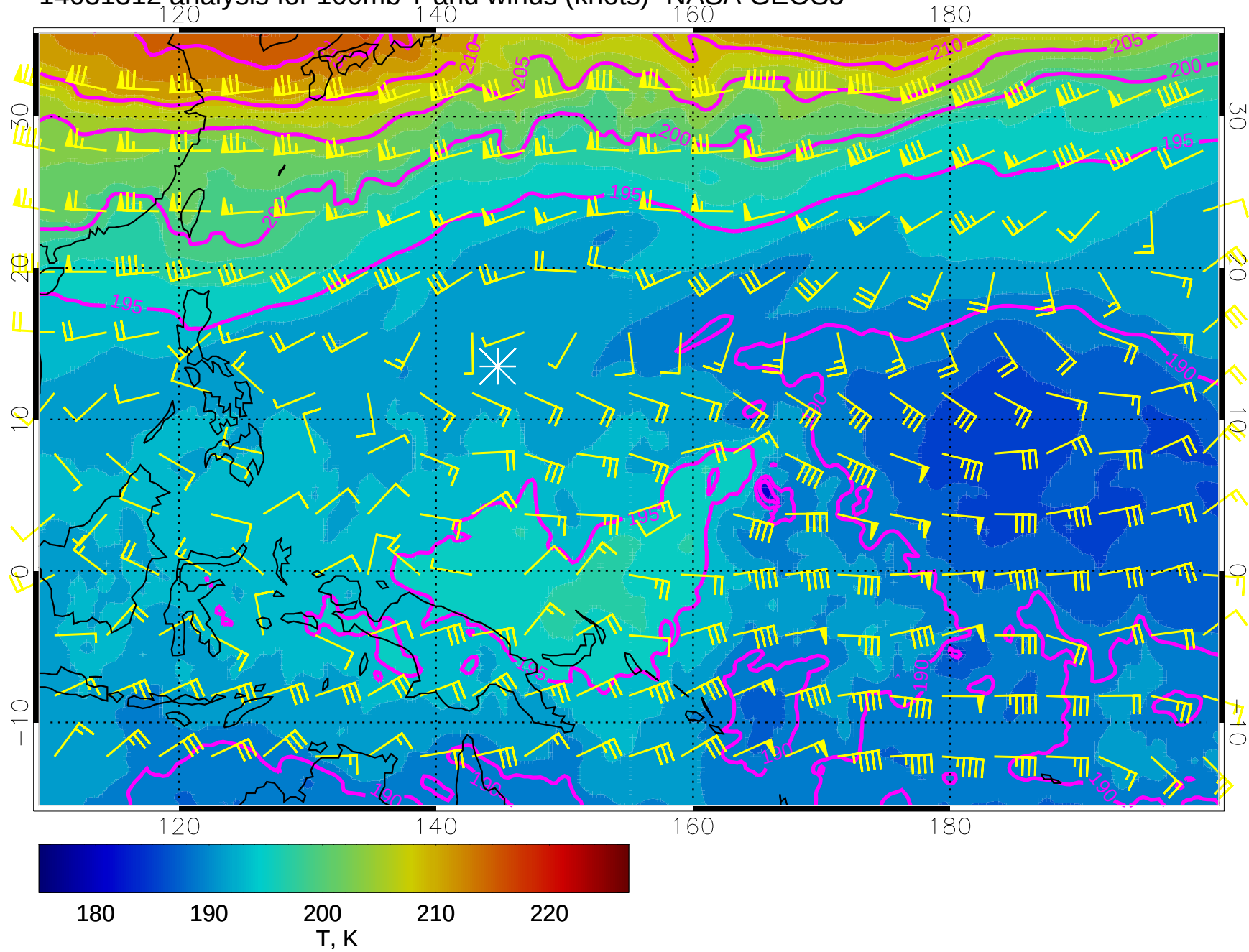
14031312 analysis for 100mb T and winds (knots)- NASA GEOS5
