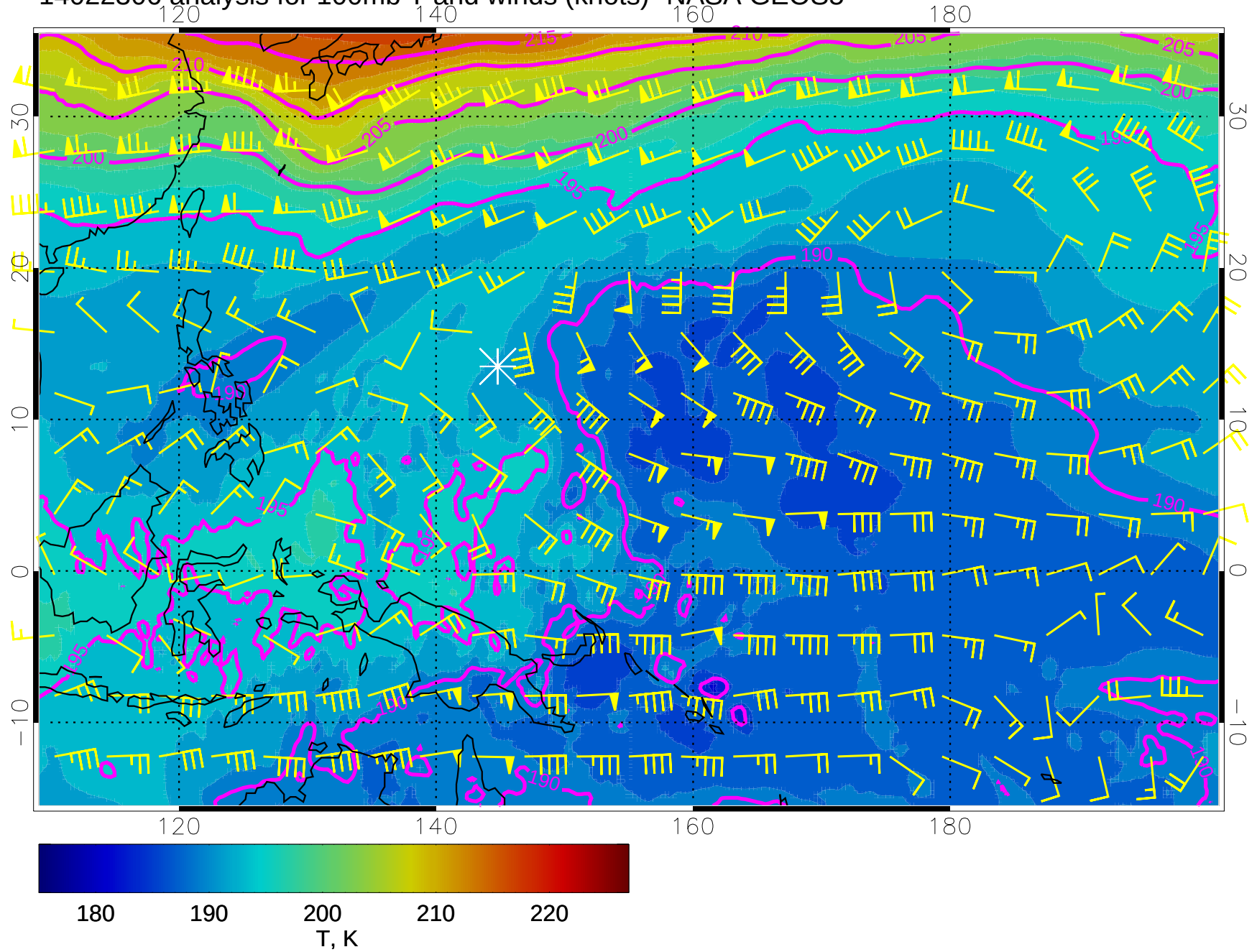
14022306 analysis for 100mb T and winds (knots)- NASA GEOS5
