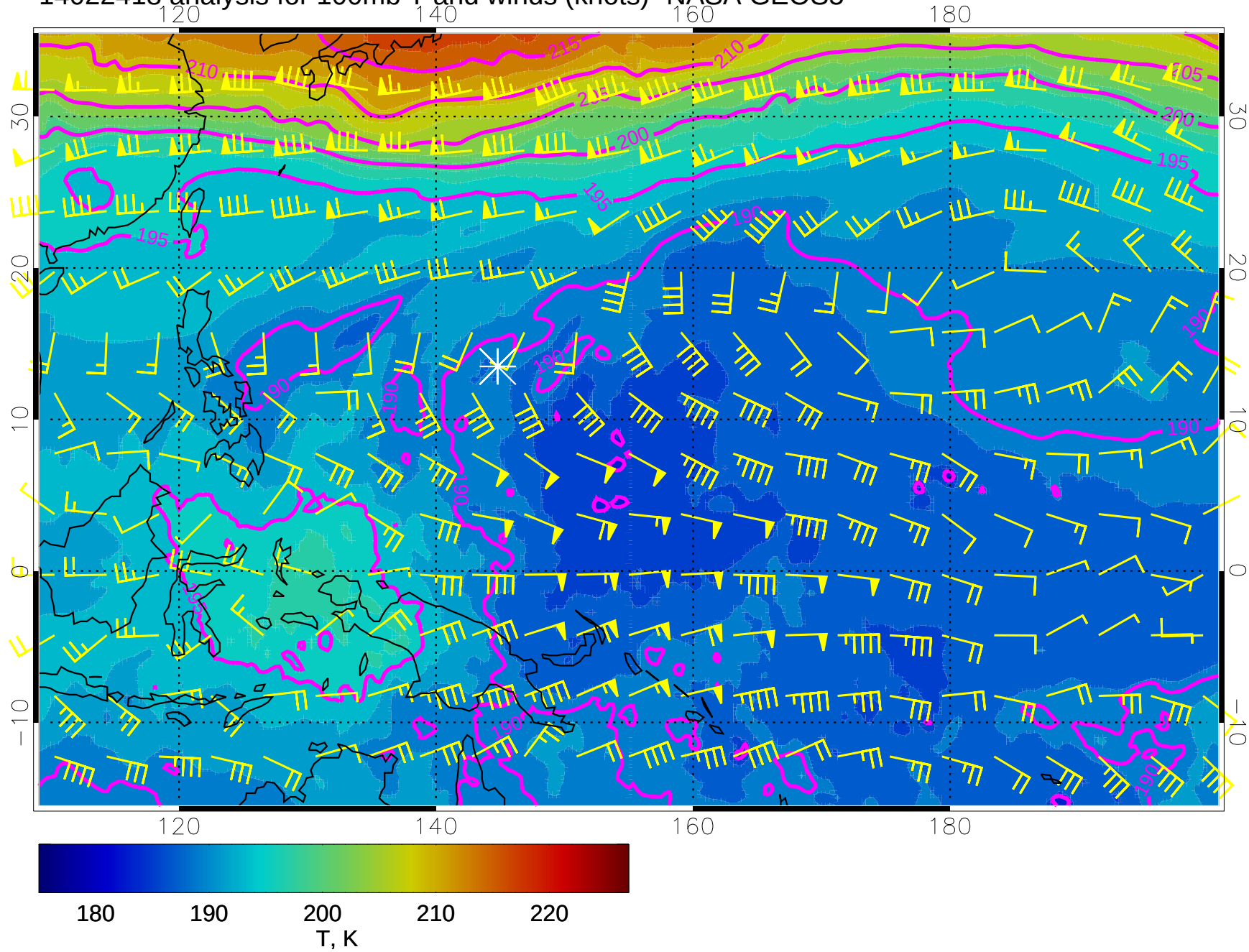
14022418 analysis for 100mb T and winds (knots)- NASA GEOS5
