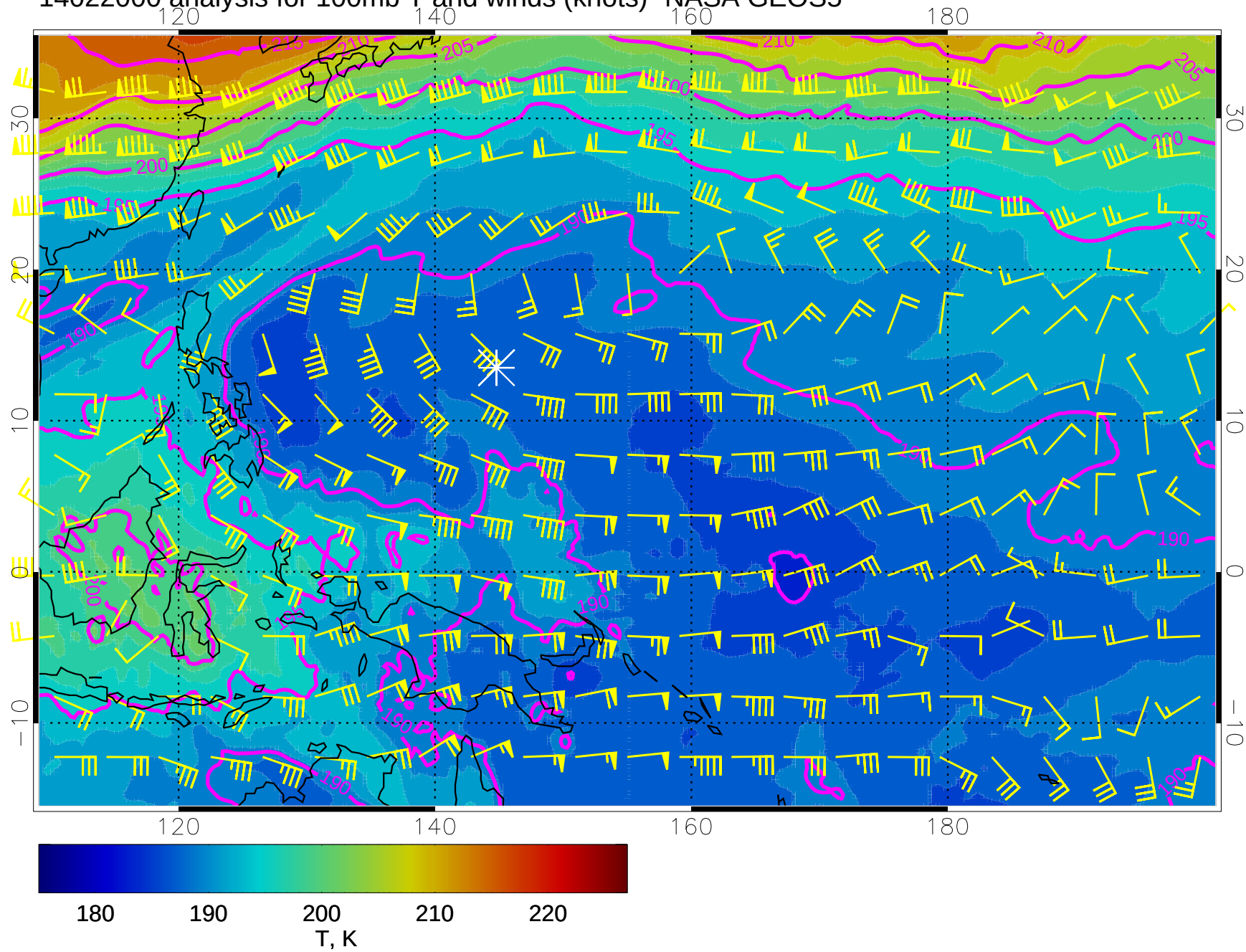
14022000 analysis for 100mb T and winds (knots)- NASA GEOS5
