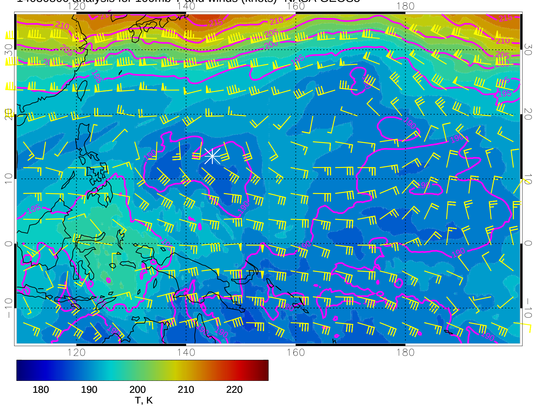
14030800 analysis for 100mb T and winds (knots)- NASA GEOS5
