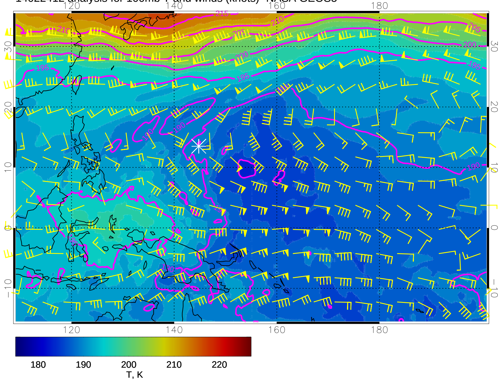
14022412 analysis for 100mb T and winds (knots)- NASA GEOS5
