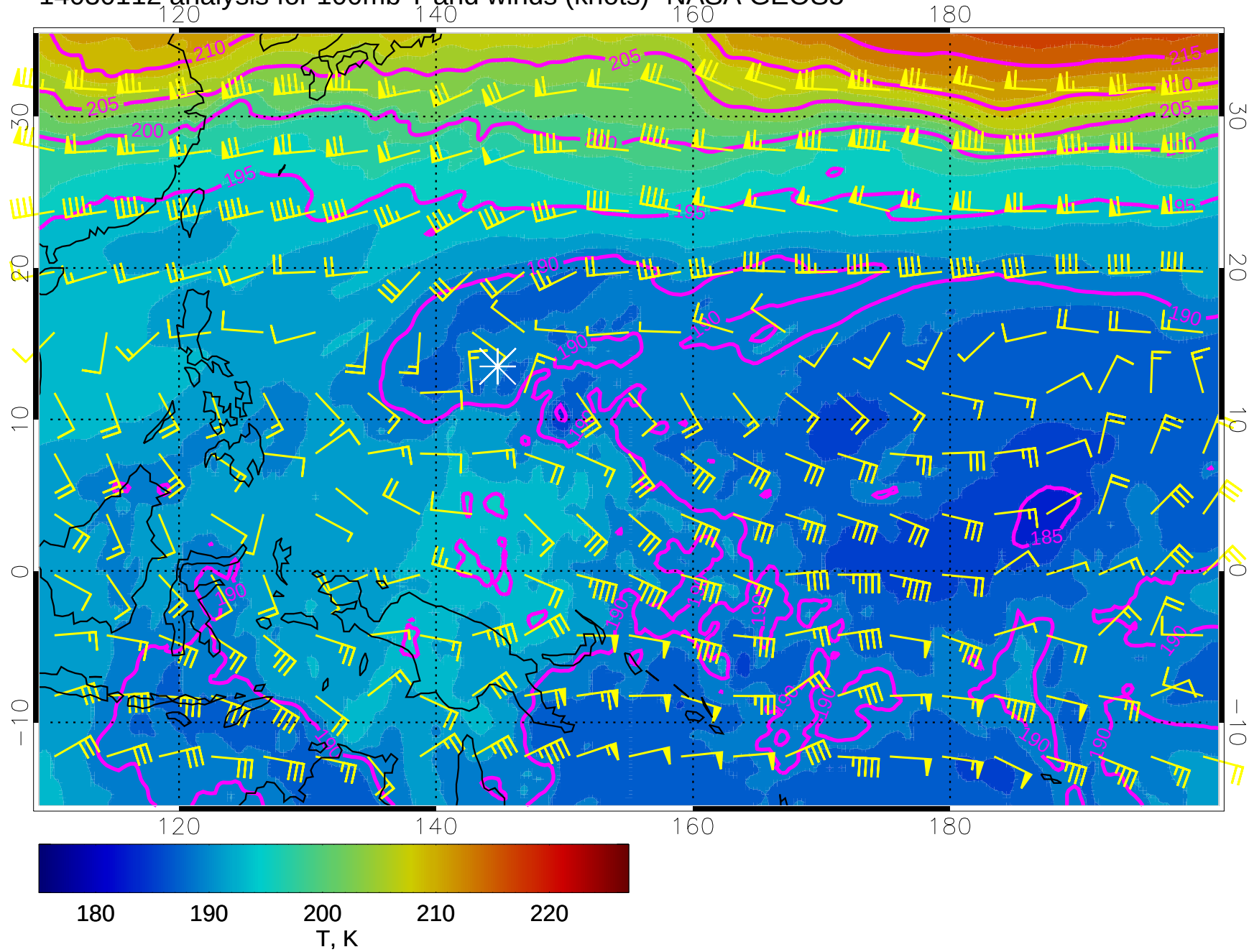
14030112 analysis for 100mb T and winds (knots)- NASA GEOS5
