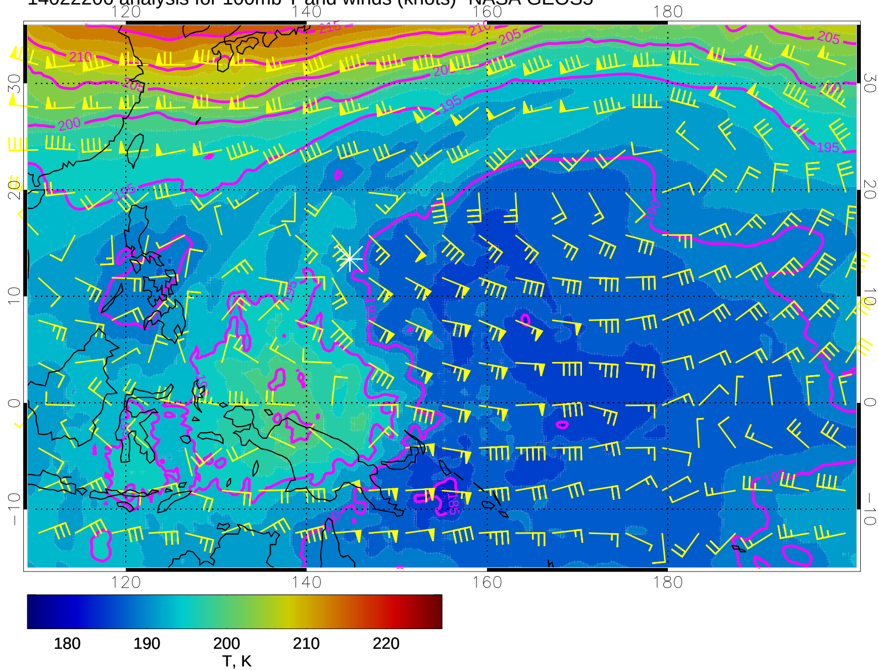
14022206 analysis for 100mb T and winds (knots)- NASA GEOS5
