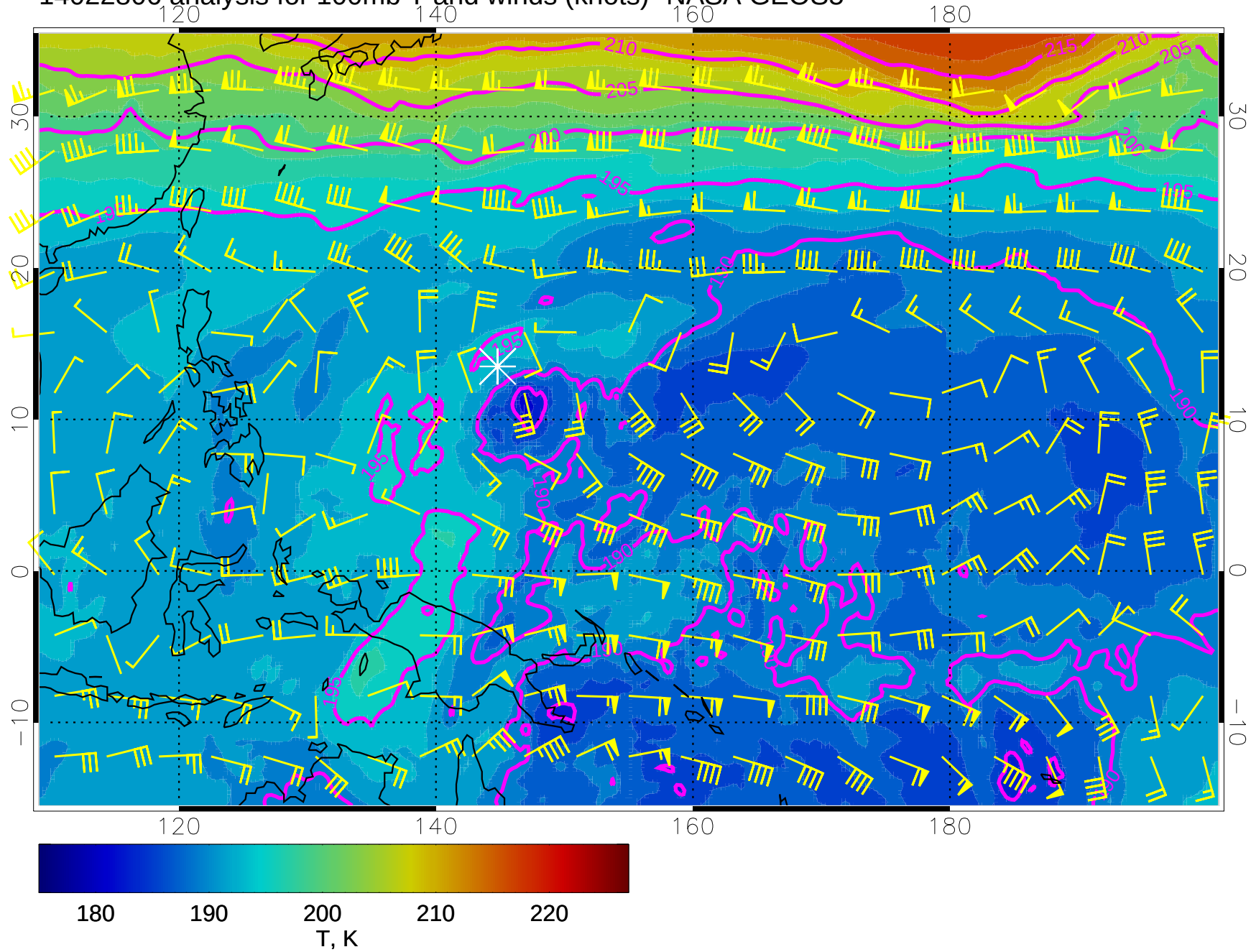
14022806 analysis for 100mb T and winds (knots)- NASA GEOS5
