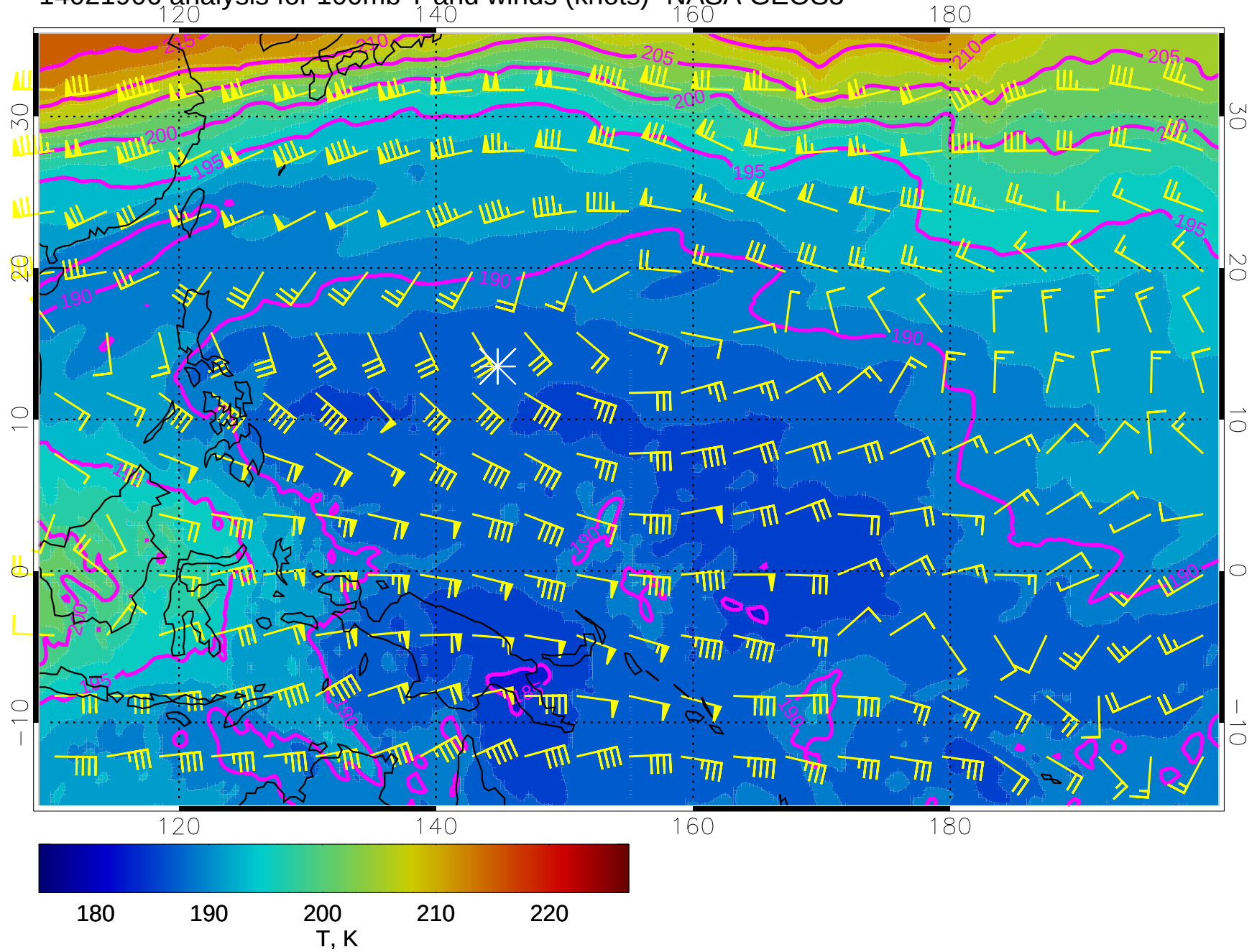
14021906 analysis for 100mb T and winds (knots)- NASA GEOS5
