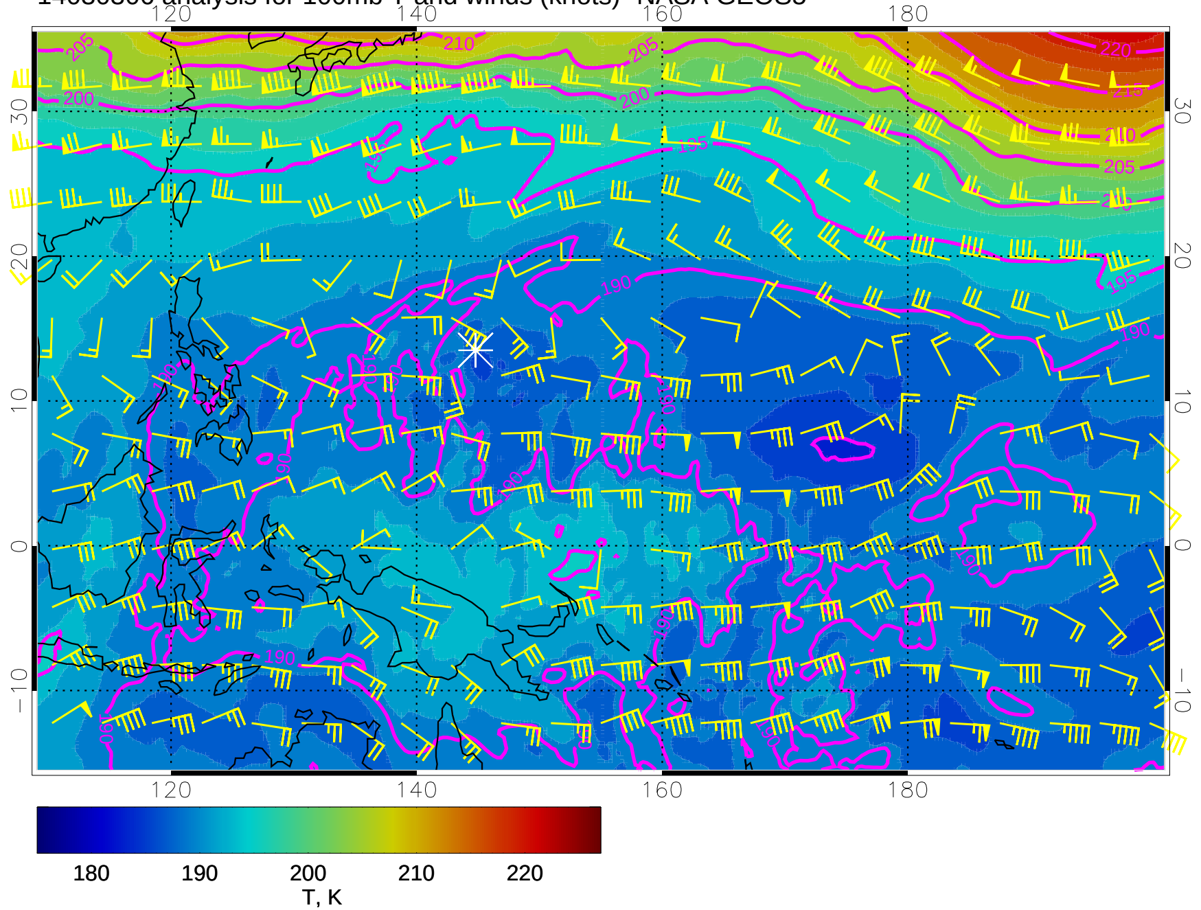
14030306 analysis for 100mb T and winds (knots)- NASA GEOS5
