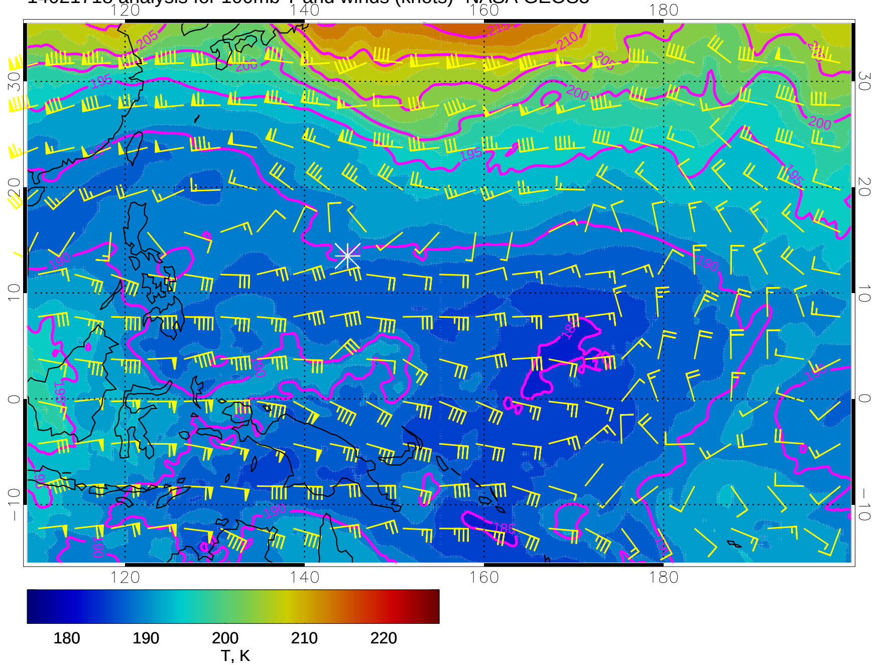
14021718 analysis for 100mb T and winds (knots)- NASA GEOS5
