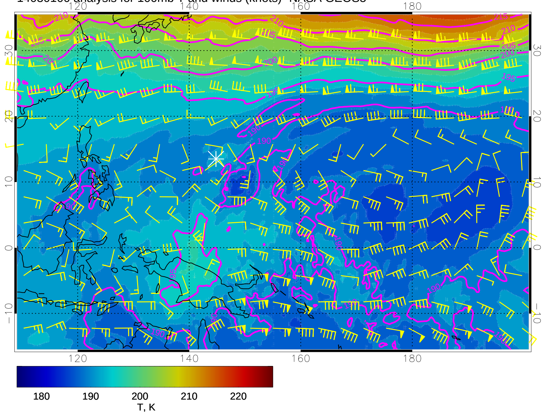
14030100 analysis for 100mb T and winds (knots)- NASA GEOS5
