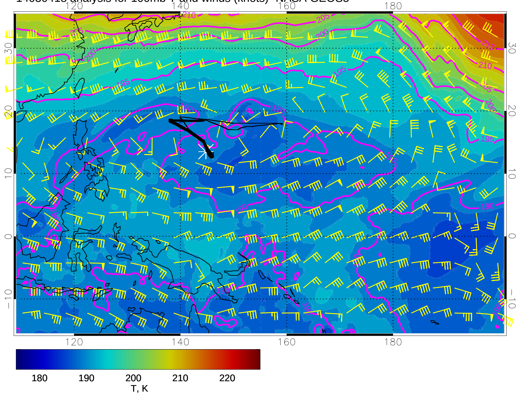
14030418 analysis for 100mb T and winds (knots)- NASA GEOS5
