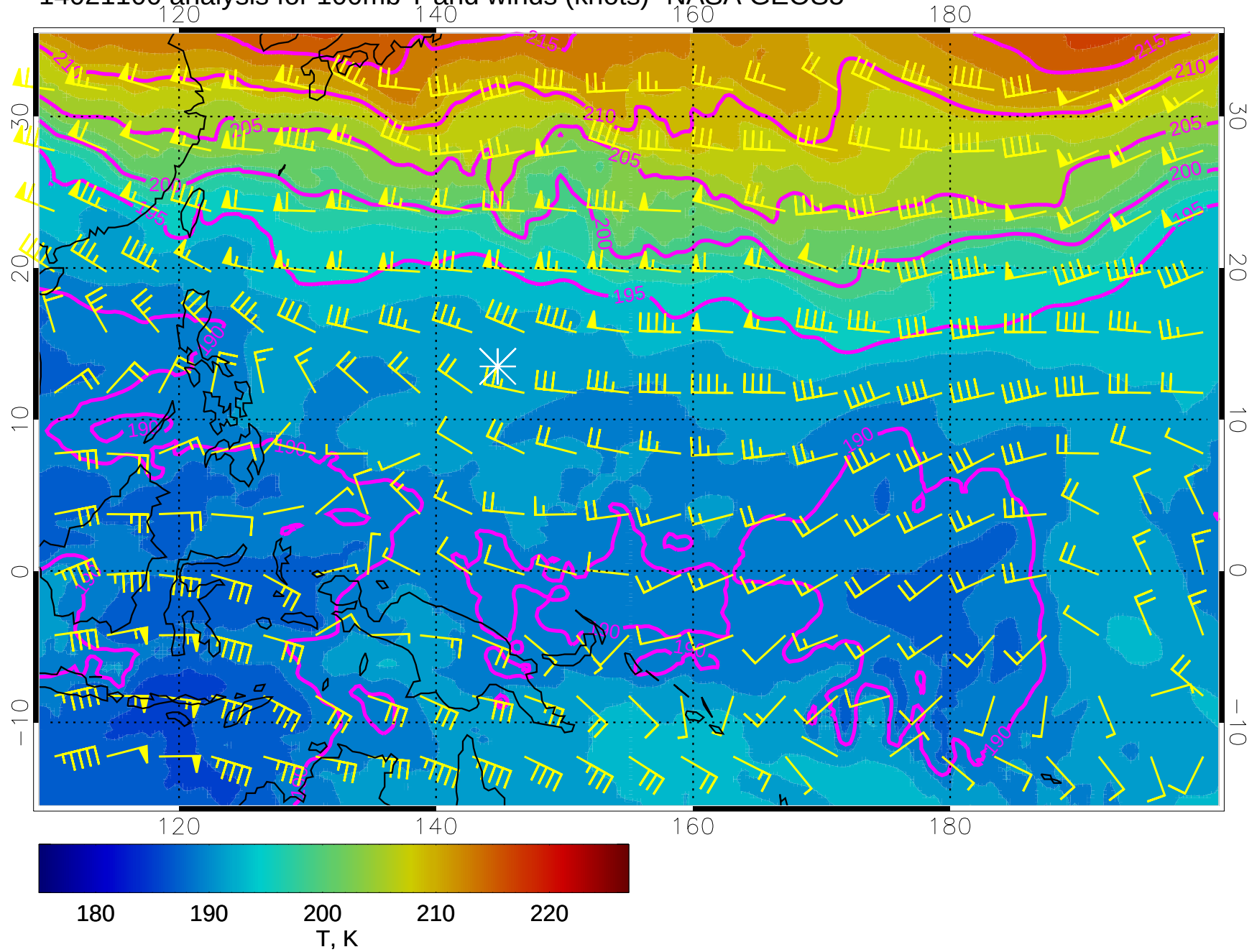
14021100 analysis for 100mb T and winds (knots)- NASA GEOS5
