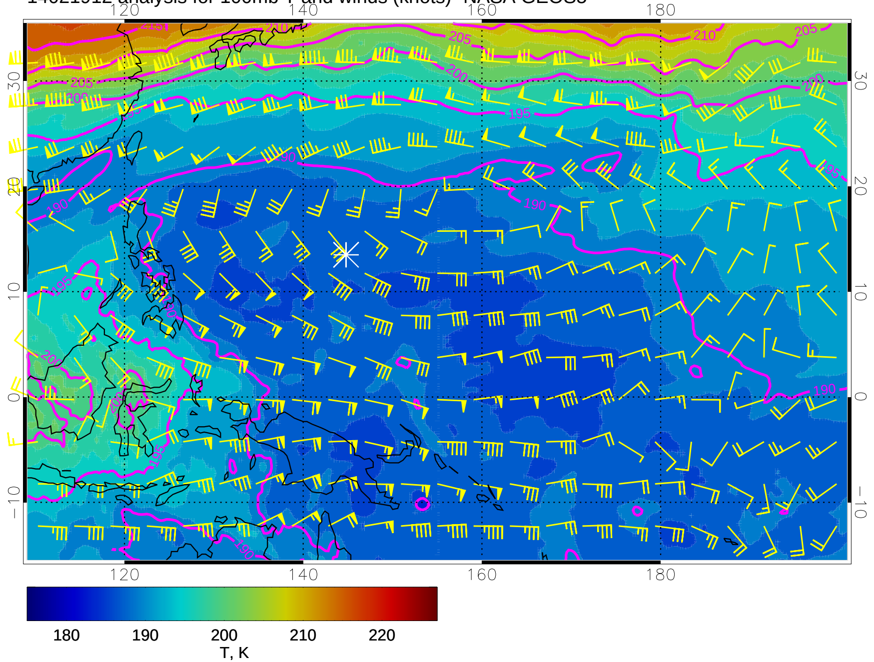
14021912 analysis for 100mb T and winds (knots)- NASA GEOS5
