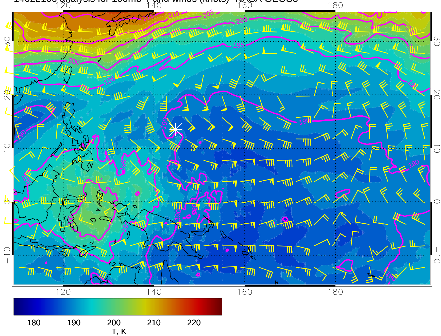
14022100 analysis for 100mb T and winds (knots)- NASA GEOS5
