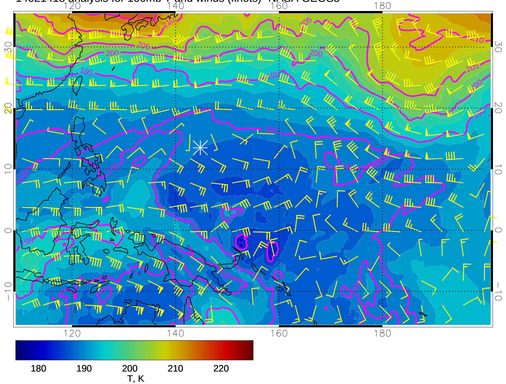
14021418 analysis for 100mb T and winds (knots)- NASA GEOS5
