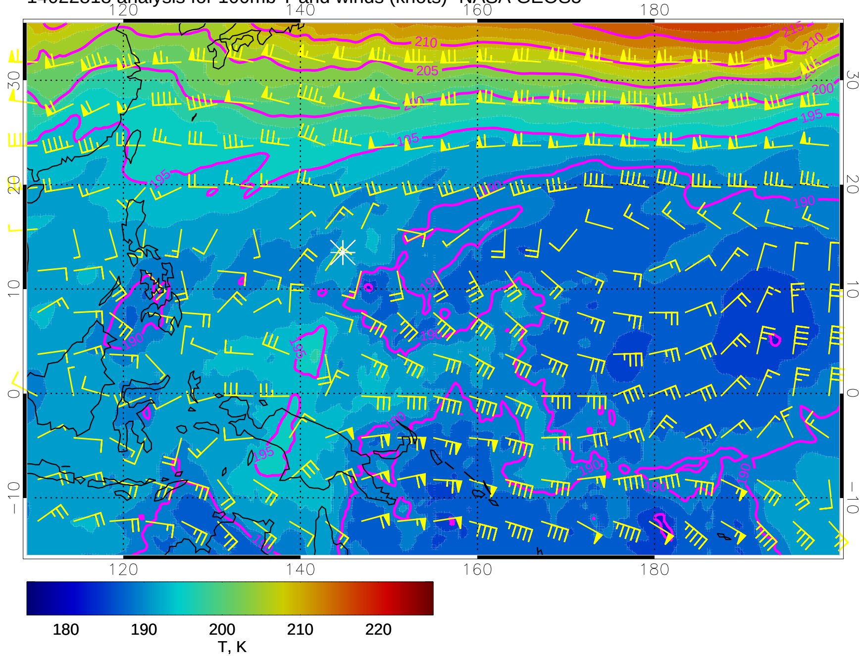
14022818 analysis for 100mb T and winds (knots)- NASA GEOS5
