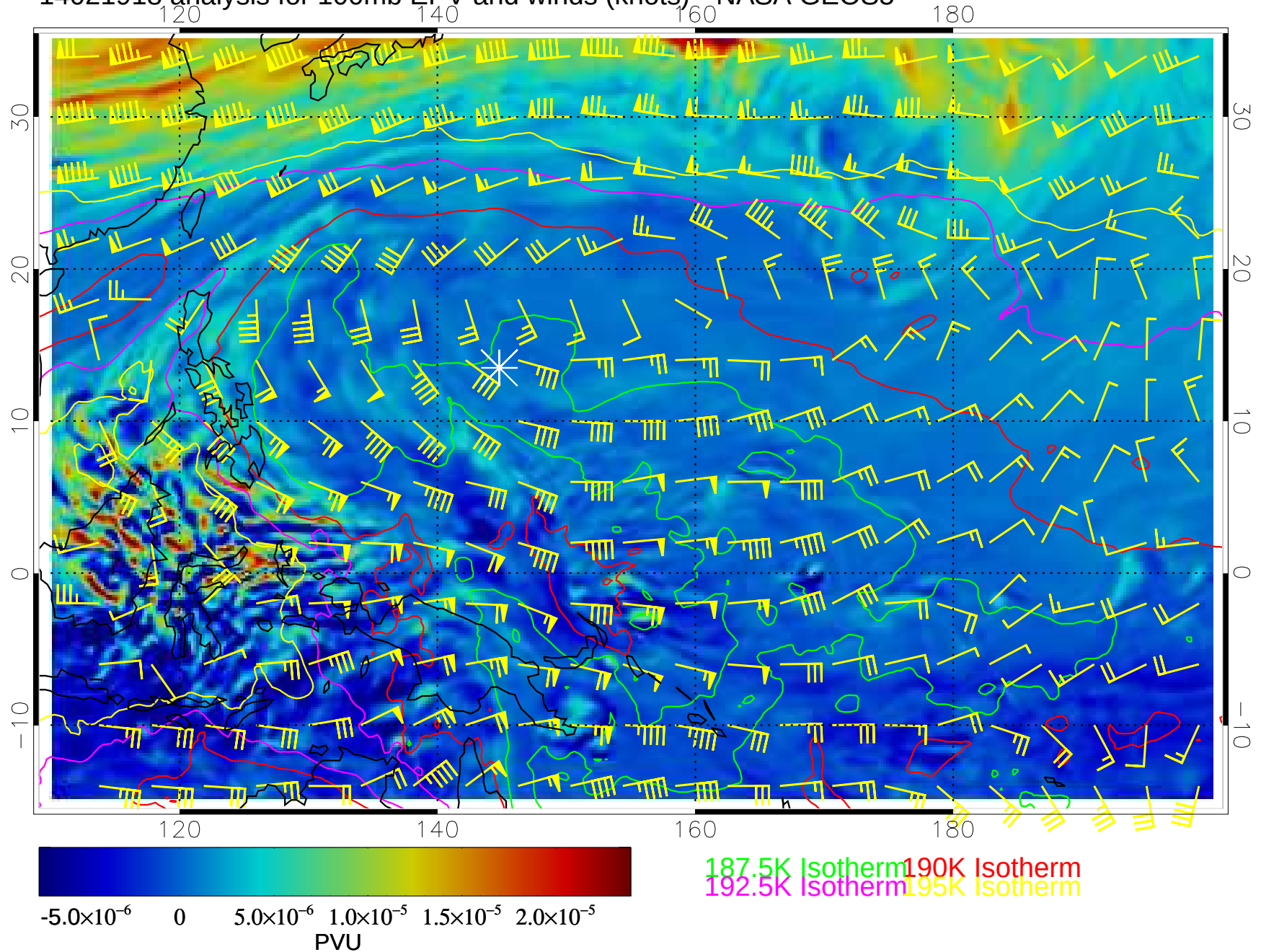
14021918 analysis for 100mb EPV and winds (knots)-- NASA GEOS5
